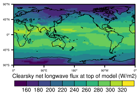
SCREAM (259.9)
