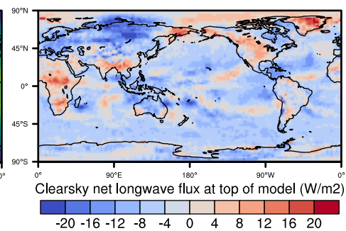
SCREAM minus CERES-EBAF (-4.3)
