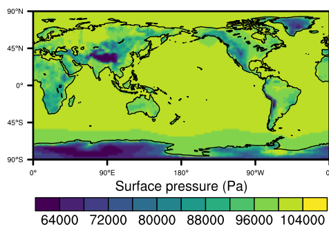
SCREAM (98568.9)
