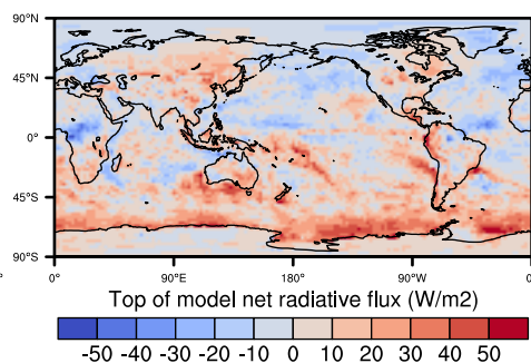
SCREAM minus CERES-EBAF (4.5)
