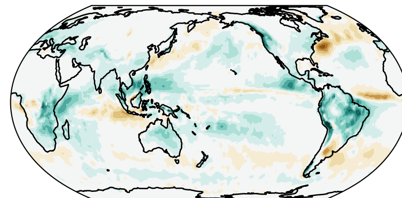
EAMv3 - GPCP (DJF) (Bias: 0.16 mm d -1 / RMSE: 1.10 mm d -1 / r : 0.91)
