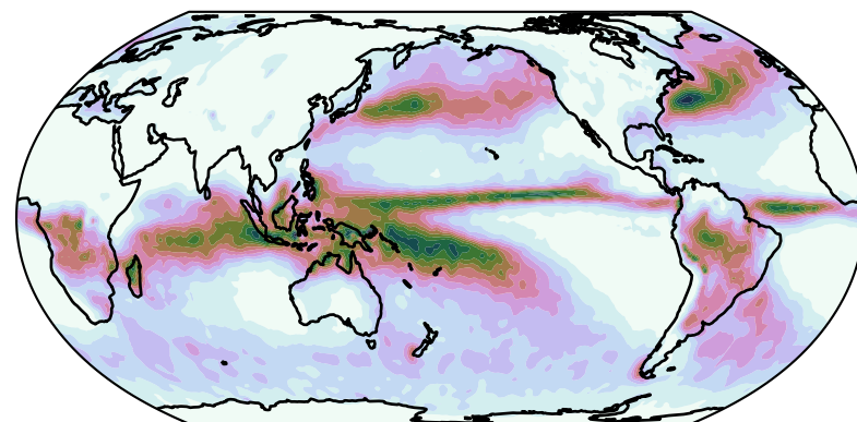
Precipitation rate (DJF) GPCP
