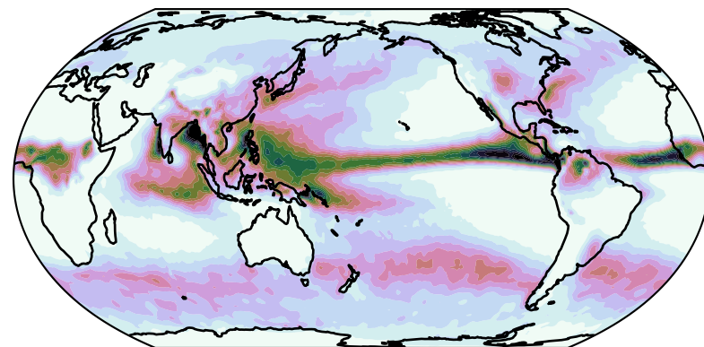
Precipitation rate (JJA) GPCP
