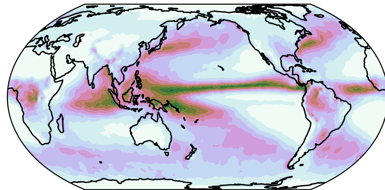
Precipitation rate (ANN) GPCP
