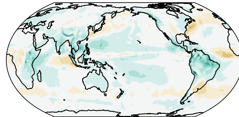
EAMv3 - GPCP (ANN) (Bias: 0.18 mm d -1 / RMSE: 0.84 mm d -1 / r : 0.92)
