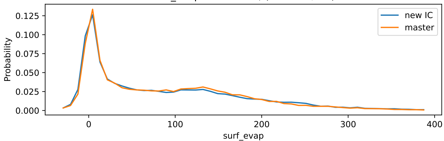
surf_evap Global PDF, (units=W/m2)
