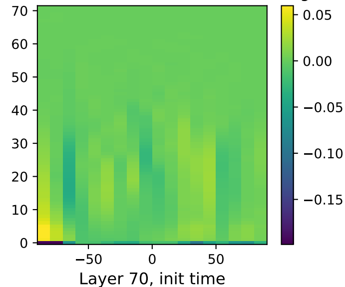
time-ave lat vs ht, units= \text{m}^{-1} \text{s}^{-3} \text{kg}
