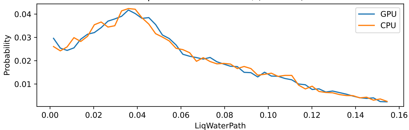
LiqWaterPath Global PDF, (units=m)
