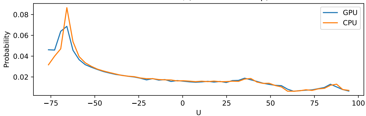
U Global PDF, (units=m s -1 top)
