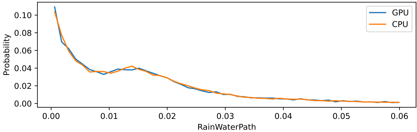
RainWaterPath Global PDF, (units=m)
