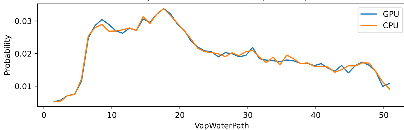
VapWaterPath Global PDF, (units=m)
