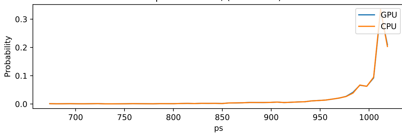
ps Global PDF, (units=hPa)
