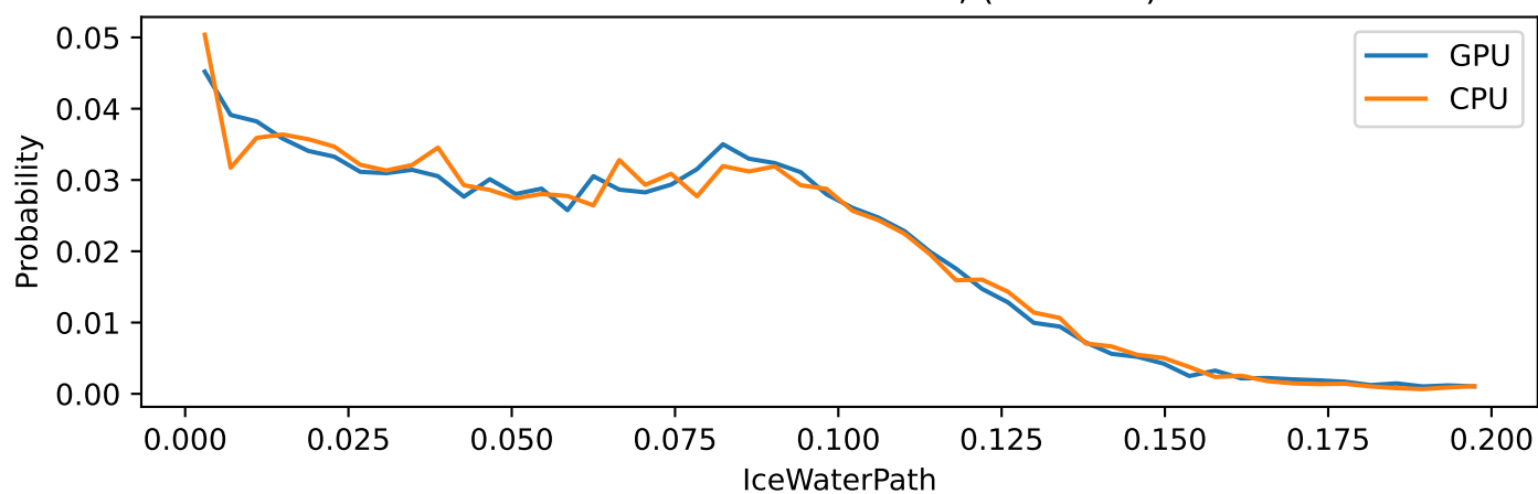
IceWaterPath Global PDF, (units=m)
