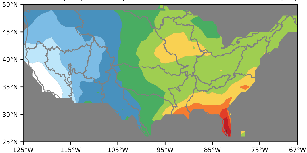
GPCP 1 degree (1997-2016)
