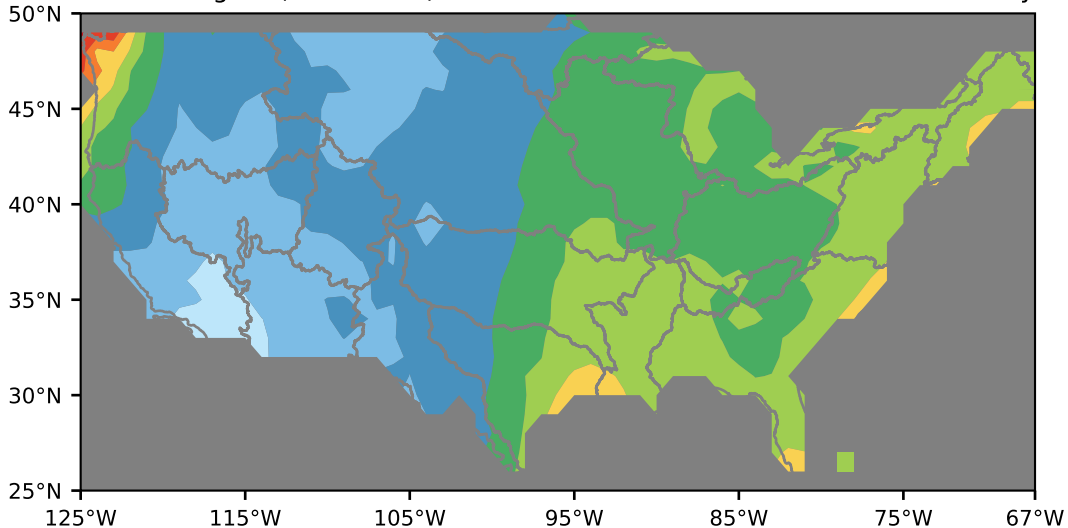
GPCP 1 degree (1997-2016)
