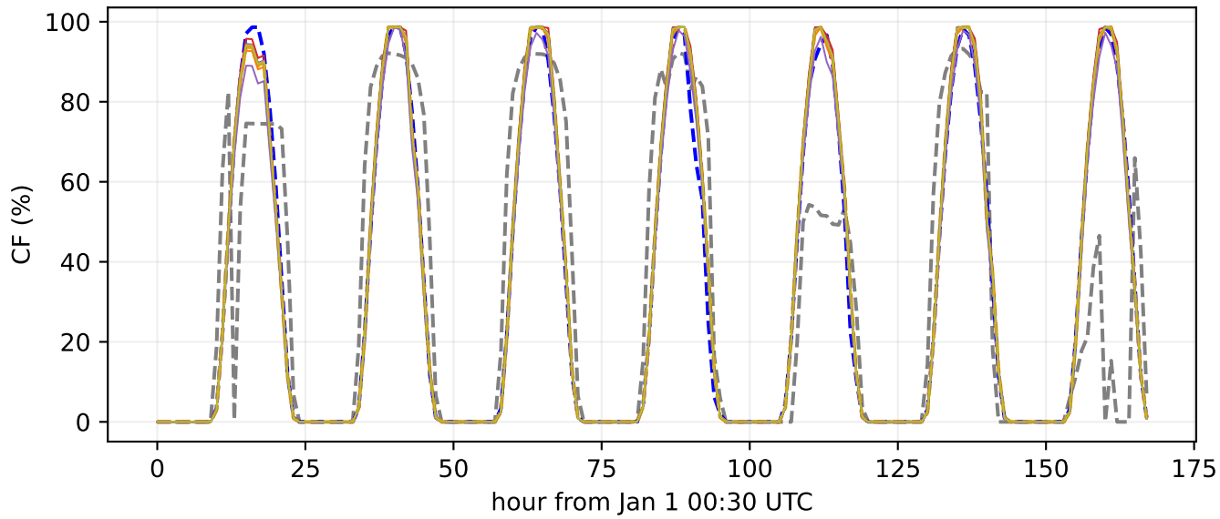
bus 561 | PMGD PFV RINCONADA
