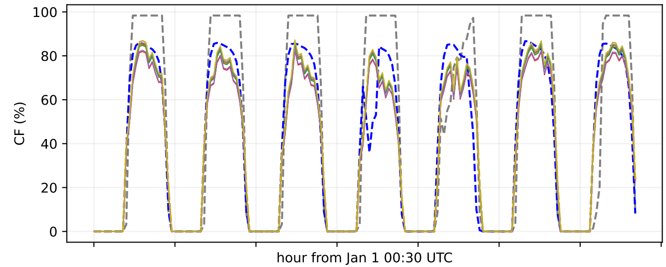
bus 804 | PMGD PFV MITCHI
