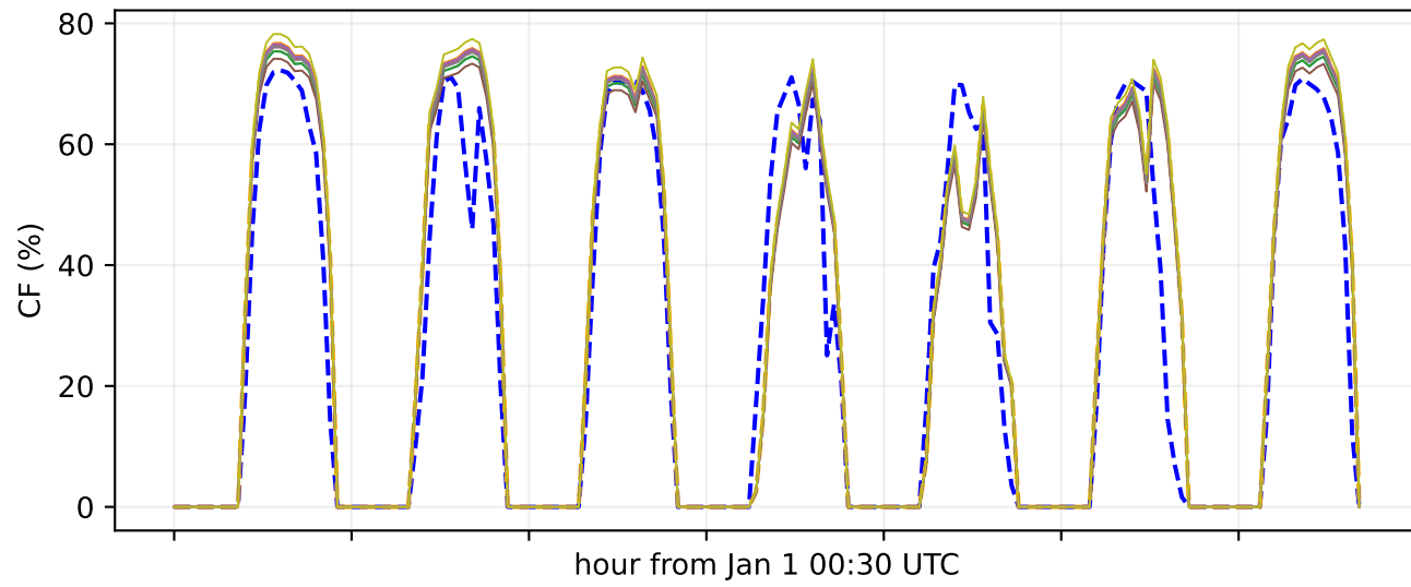
bus 1127 | PMGD PFV PERSEFONE
