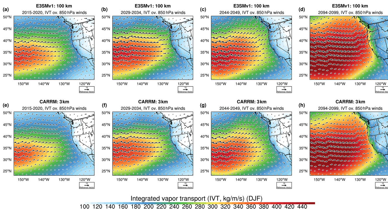
Figure A13. Similar to Fig. 6 but for total vertically integrated vapor transport (referred to as IVT) with 850 hPa horizontal wind vectors.
