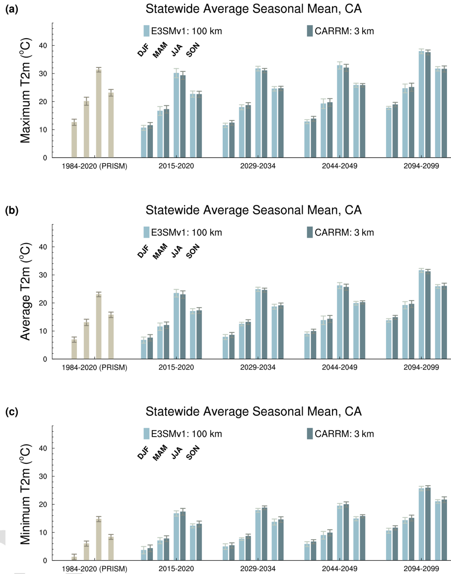
Figure 7. The 5-year seasonal average and standard deviation of daily (a) maximum, (b) mean, and (c) minimum T2m during four simulation segments. SCREAMv0 CARRM ( 1^\circ E3SMv1) is denoted by dark (light) blue histograms. Each segment shows winter (December–January–February, DJF), spring (March–April–May, MAM), summer (June–July–August, JJA), and autumn (September–October–November, SON) in order. PRISM (yellow histograms) from 1984 to 2020 water years is shown in the leftmost column for a baseline comparison with the 2015–2020 simulation period.
