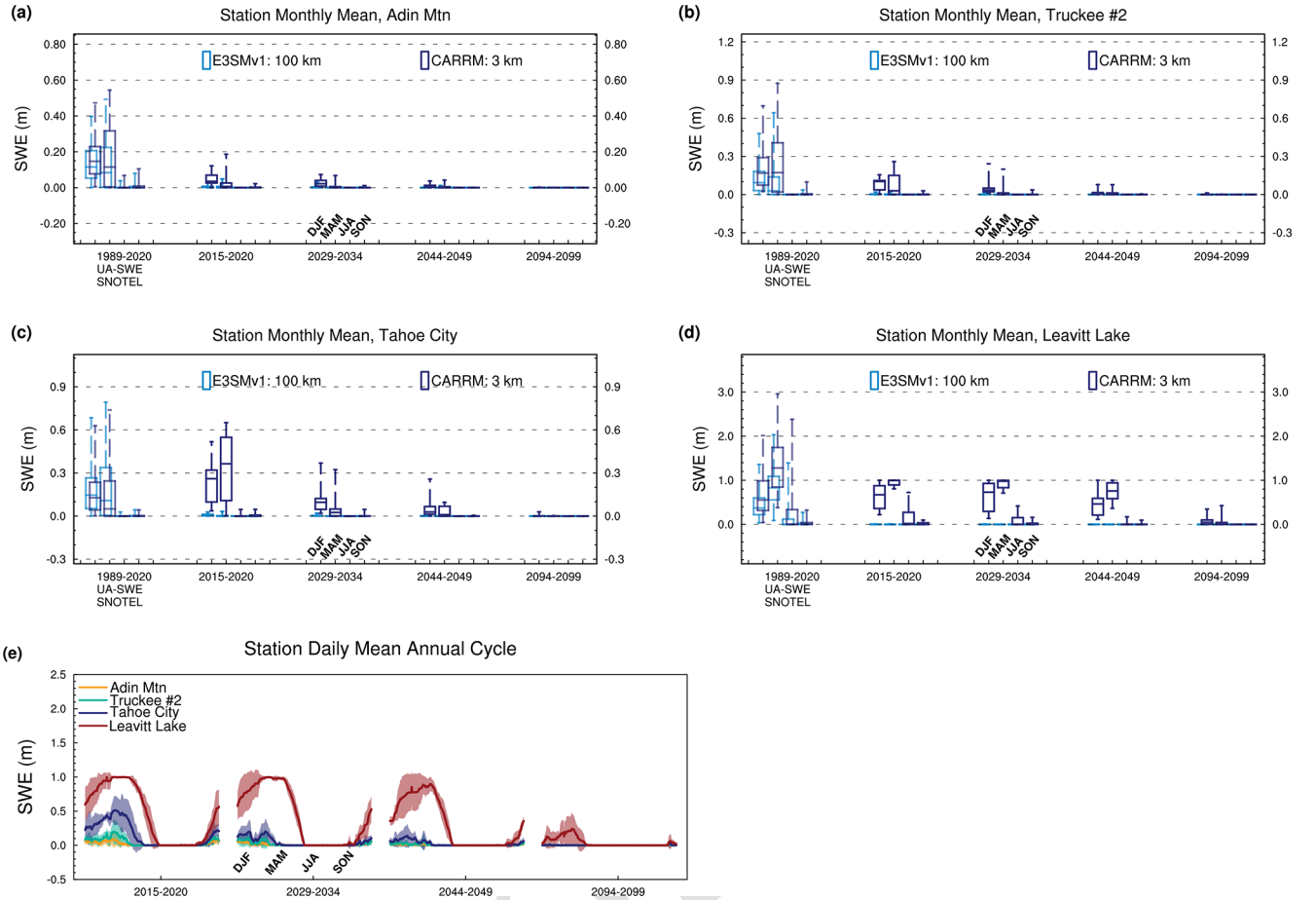
Figure 14. Same as Fig. 8 but for monthly mean of SWE in (a) Adin Mtn, (b) Truckee, (c) Tahoe City, and (d) Leavitt Lake. (e) Daily mean annual cycle at four stations. The shading shows the standard deviation of each segment.
