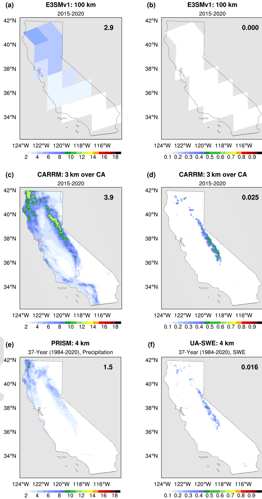
Figure 5. Same as Fig. 4 but for precipitation ( \text{mm d}^{-1} ; a, c, e ) and snow water equivalent (referred to as SWE; m; b, d, f ). The observation-based gridded products used for comparison are PRISM ( e ) and UA-SWE ( f ). The megaton (Mt) of the multi-year mean statewide SWE storage is 0.16, 10, and 6.3 Mt for E3SMv1, CARRM, and UA-SWE, respectively.
