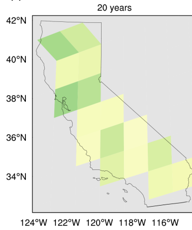
(b) CARRM 10-year return value, DJF
