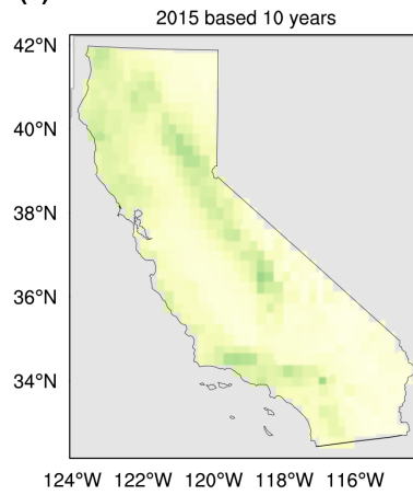
(c) LULNUQ 10-year return value, DJF
