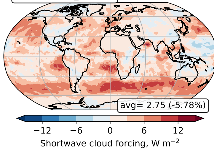
(e) diff: GCCN_D4 - Ctrl
