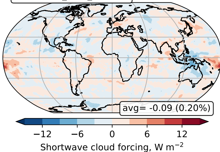
(d) diff: GA_inert_D4 - Ctrl
