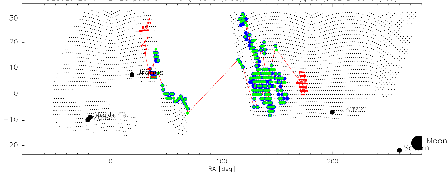
DECaLS 2016-12-28 pass 3: 170 g-band (blue), 175 r-band (green), 52 z-band (red)
