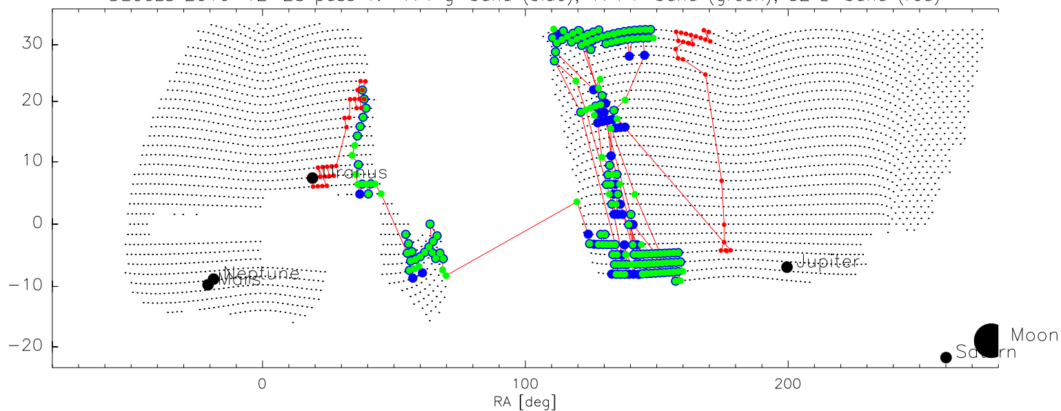
DECaLS 2016-12-28 pass 2: 171 g-band (blue), 174 r-band (green), 52 z-band (red)
