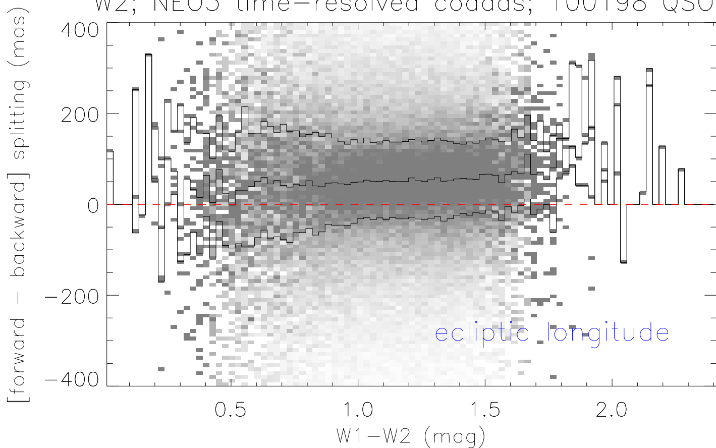
W2; NEO3 time-resolved coadds; 100198 QSOs
