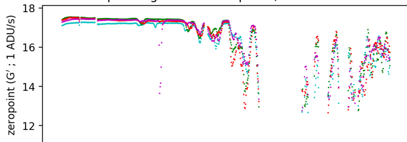
pointing camera sky brightness ; 20210704
