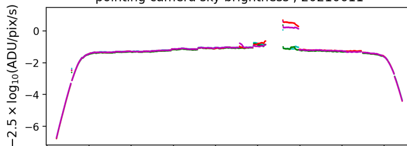
sky monitor sky brightness ; 20210611
