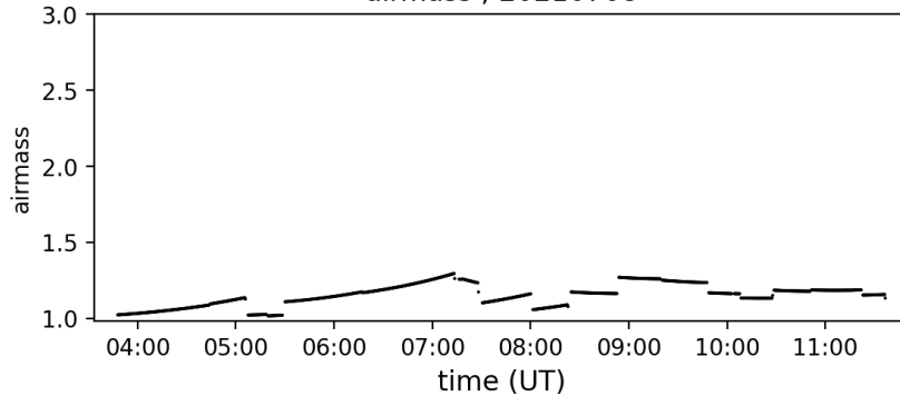
airmass ; 20210708
