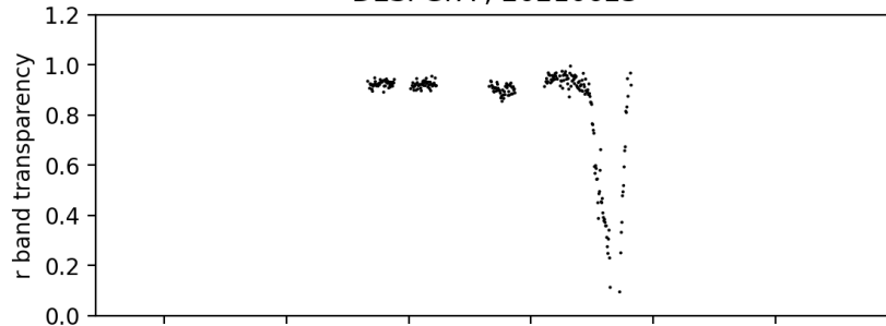
pointing camera zeropoint ; 20210623
