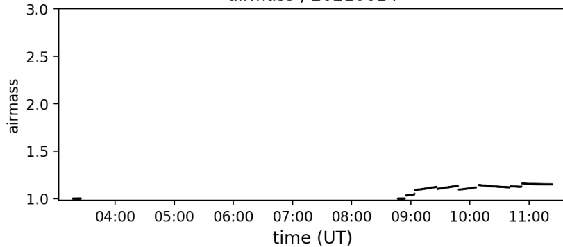
airmass ; 20210614
