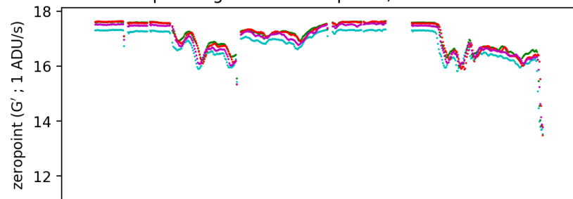
pointing camera sky brightness ; 20210709
