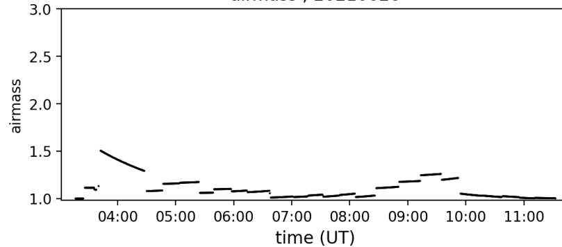
airmass ; 20210626
