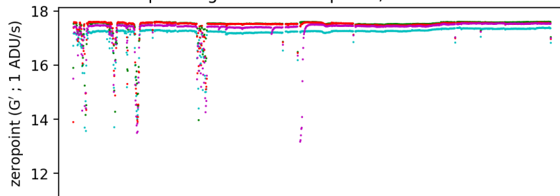
pointing camera sky brightness ; 20210708
