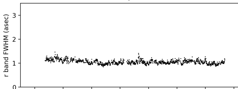
DESI GFA ; 20210616
