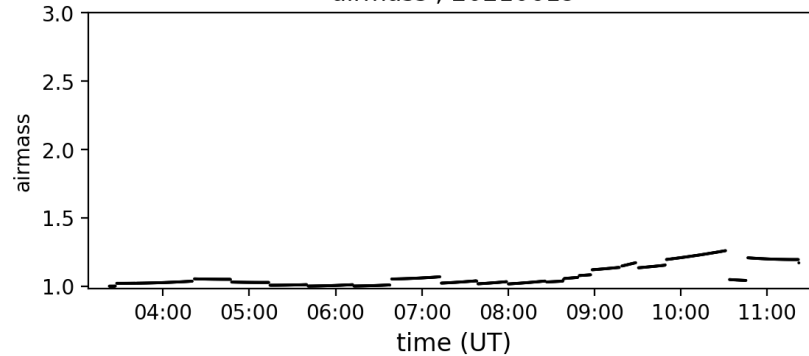
airmass ; 20210619
