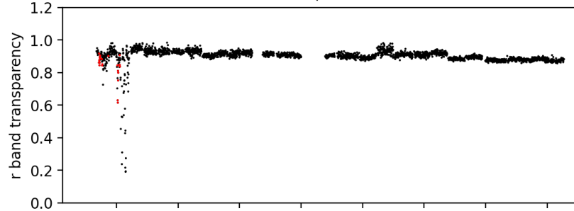
pointing camera zeropoint ; 20210617
