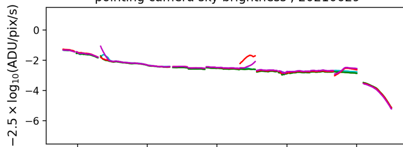
sky monitor sky brightness ; 20210629
