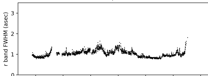
DESI GFA ; 20210627
