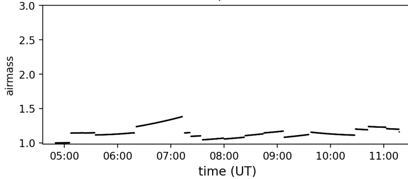
airmass ; 20210615
