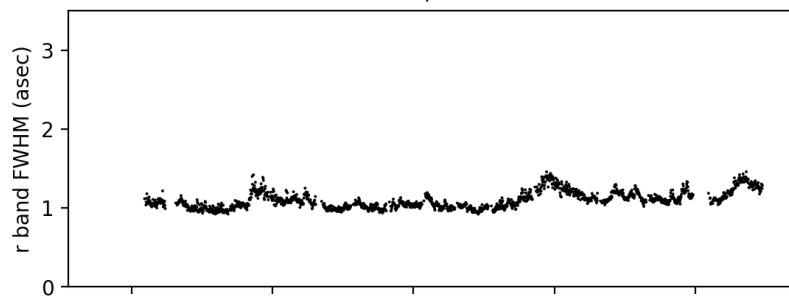
DESI GFA ; 20210629
