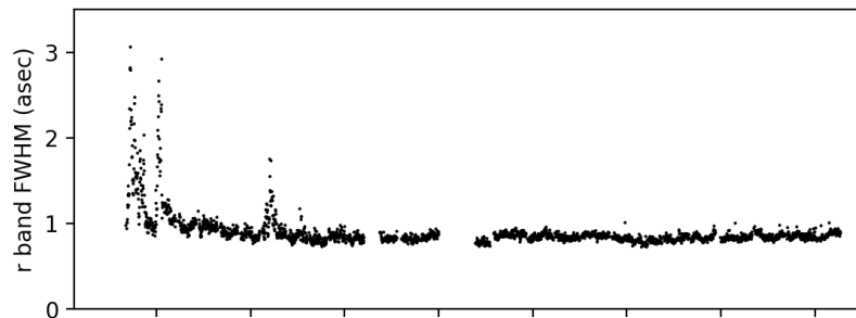
DESI GFA ; 20210617
