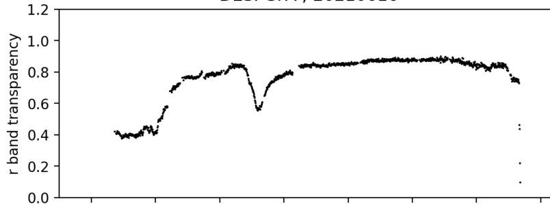
pointing camera zeropoint ; 20210616
