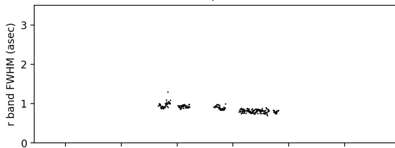
DESI GFA ; 20210623
