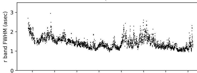
DESI GFA ; 20210628
