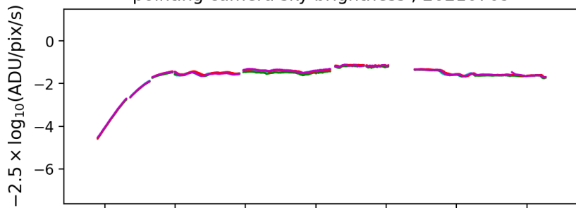
sky monitor sky brightness ; 20210709
