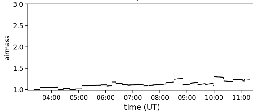
airmass ; 20210617
