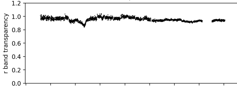
pointing camera zeropoint ; 20210612
