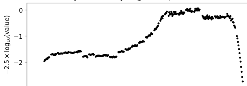
airmass ; 20210618
