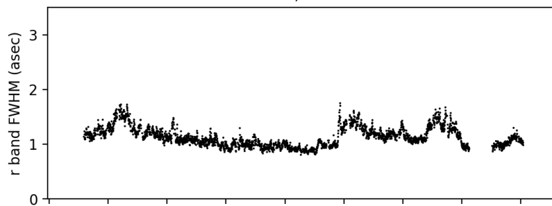
DESI GFA ; 20210612
