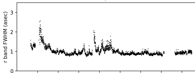
DESI GFA ; 20210613
