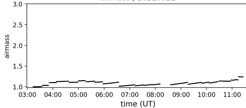
airmass ; 20210611
