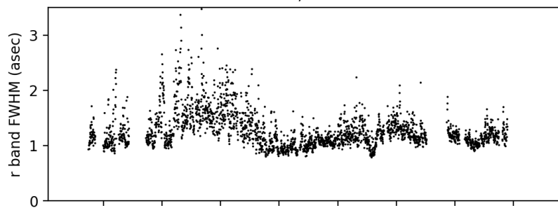
DESI GFA ; 20210705
