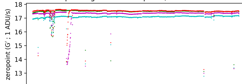
pointing camera sky brightness ; 20210617
