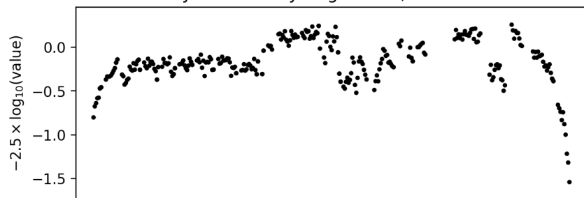
airmass ; 20210609
