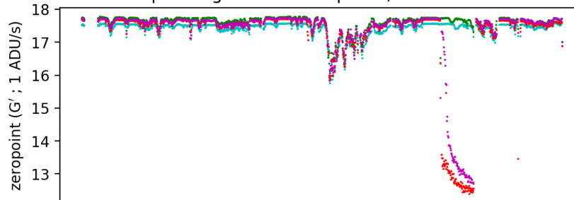
pointing camera sky brightness ; 20210609
