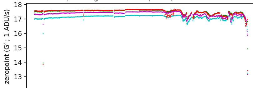
pointing camera sky brightness ; 20210615
