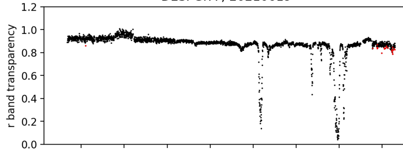
pointing camera zeropoint ; 20210619
