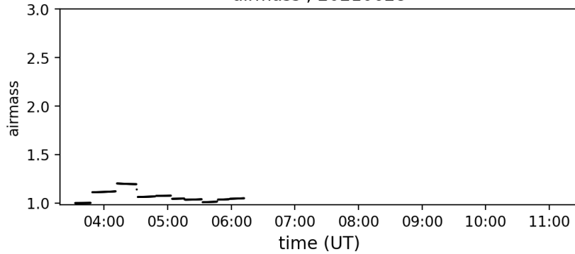
airmass ; 20210628
