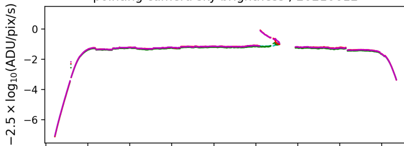
sky monitor sky brightness ; 20210612
