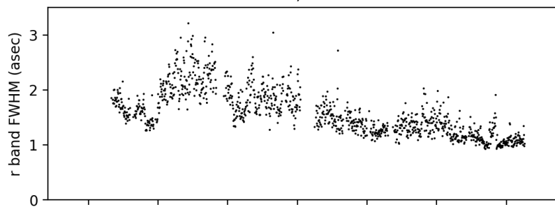
DESI GFA ; 20210709
