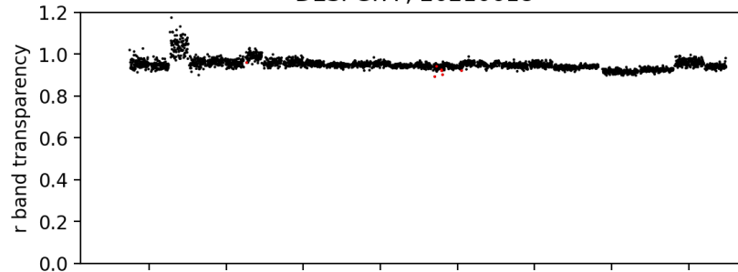
pointing camera zeropoint ; 20210618
