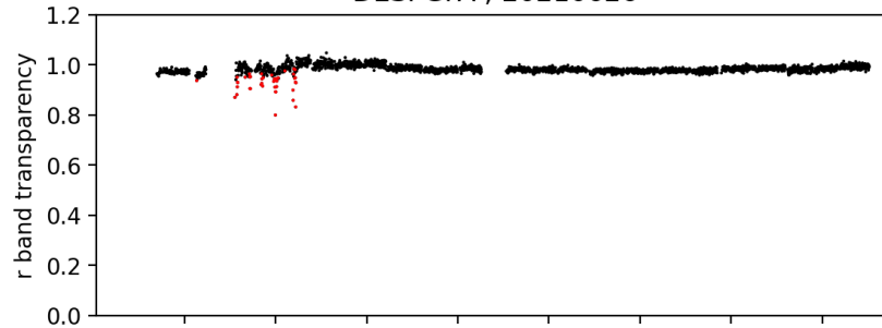
pointing camera zeropoint ; 20210626
