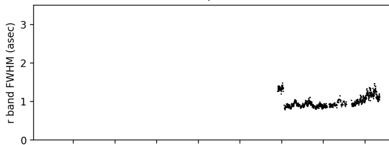
DESI GFA ; 20210614
