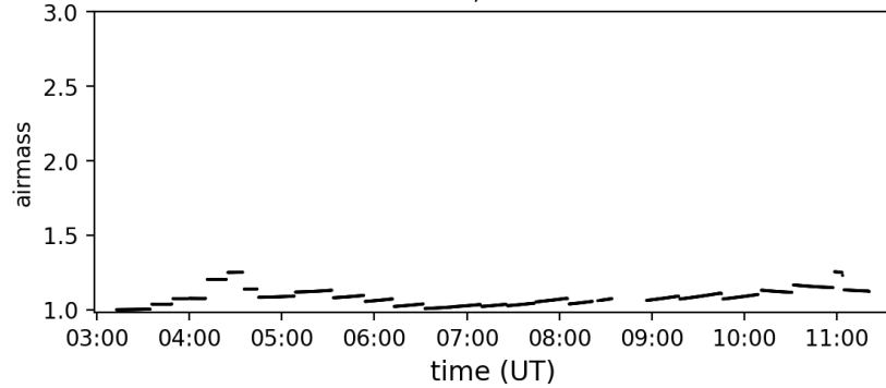
airmass ; 20210612
