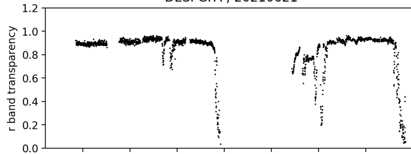
pointing camera zeropoint ; 20210621
