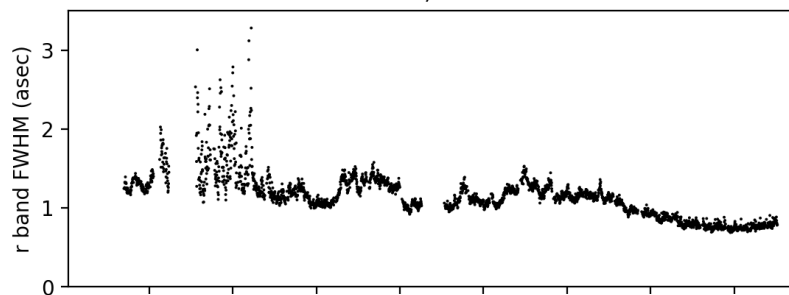
DESI GFA ; 20210626
