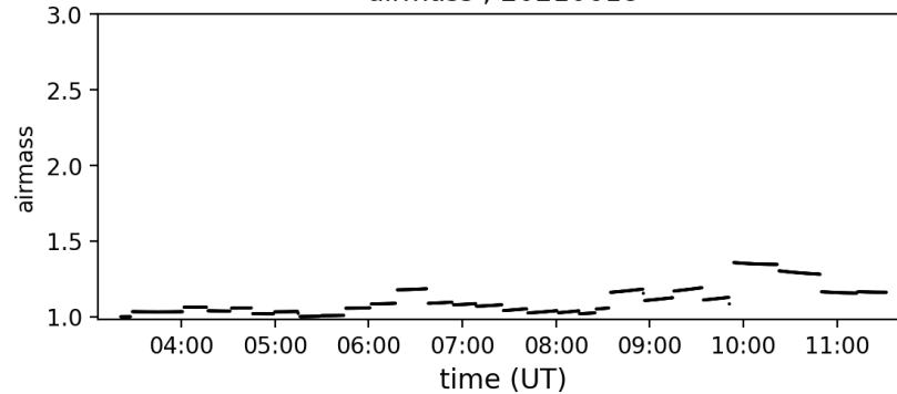
airmass ; 20210618
