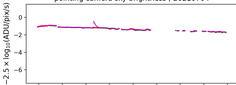
sky monitor sky brightness ; 20210704
