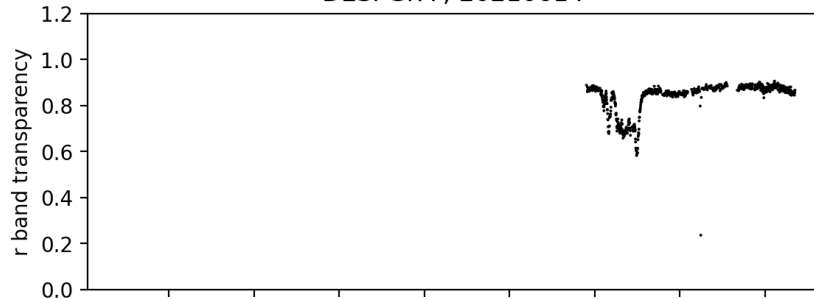
pointing camera zeropoint ; 20210614
