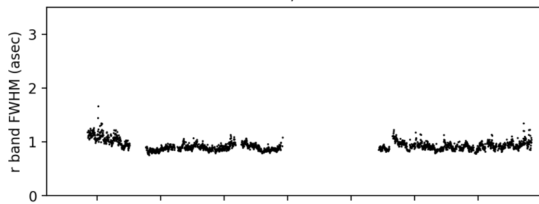
DESI GFA ; 20210621
