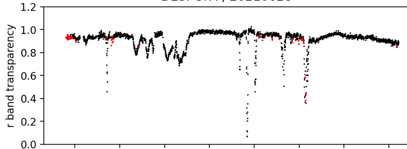
pointing camera zeropoint ; 20210628
