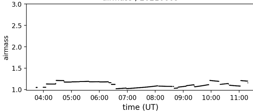
airmass ; 20210609
