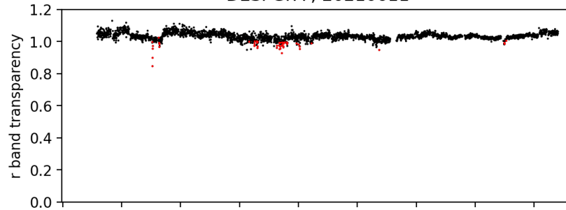
pointing camera zeropoint ; 20210611
