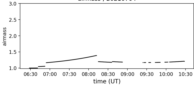
airmass ; 20210704
