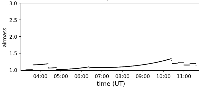
airmass ; 20210706
