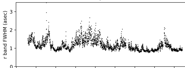
DESI GFA ; 20210611
