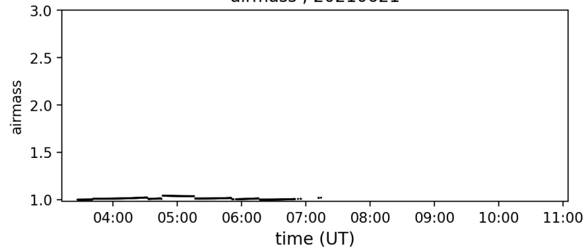
airmass ; 20210621
