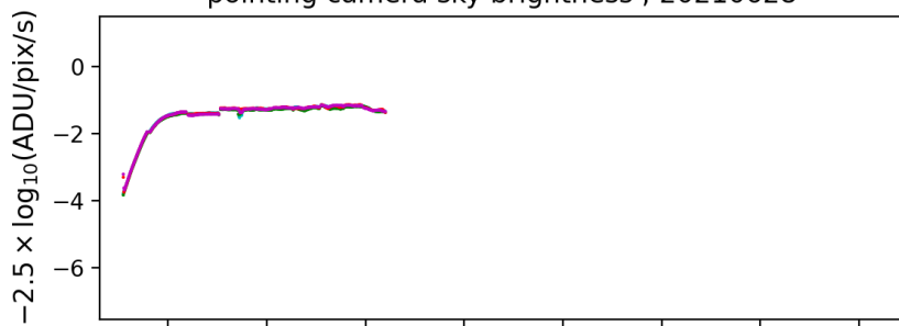
sky monitor sky brightness ; 20210628
