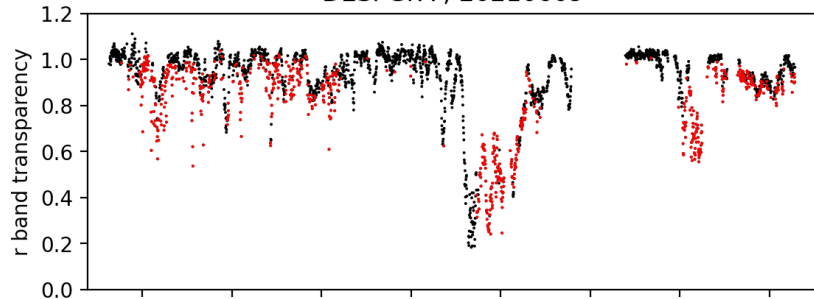
pointing camera zeropoint ; 20210609
