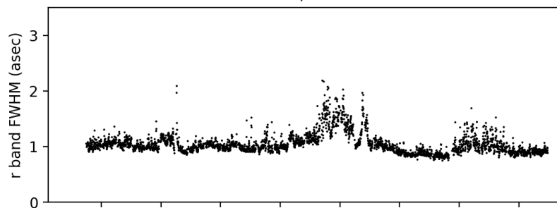
DESI GFA ; 20210618
