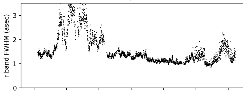
DESI GFA ; 20210615
