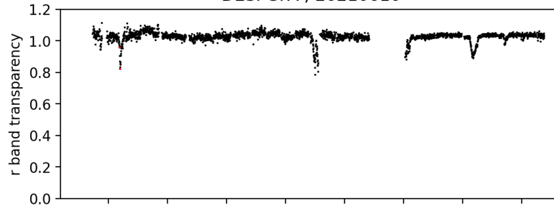
pointing camera zeropoint ; 20210610
