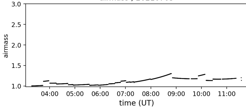
airmass ; 20210705
