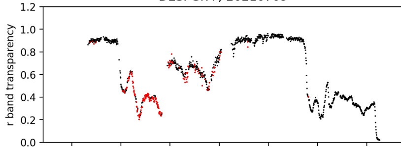
pointing camera zeropoint ; 20210709
