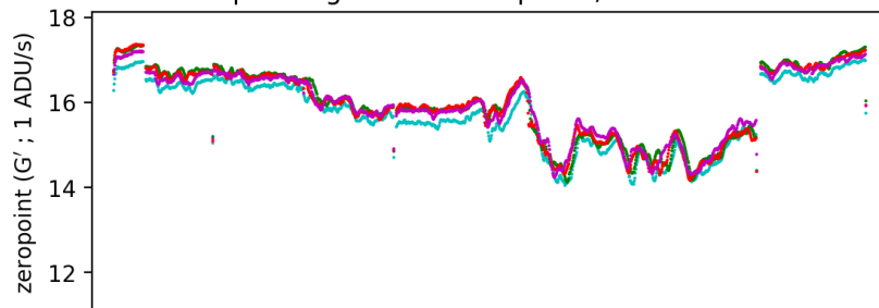
pointing camera sky brightness ; 20210706
