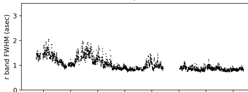
DESI GFA ; 20210610
