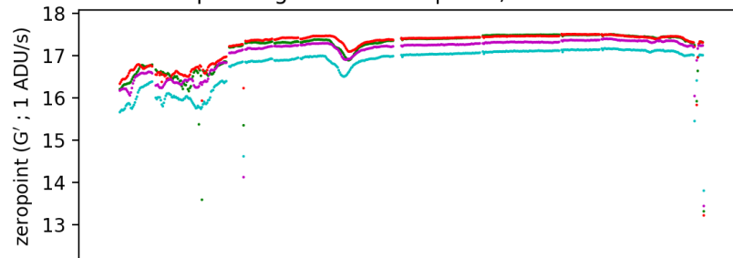
pointing camera sky brightness ; 20210616
