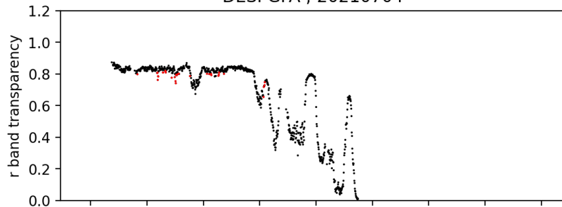
pointing camera zeropoint ; 20210704
