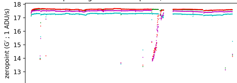
pointing camera sky brightness ; 20210612
