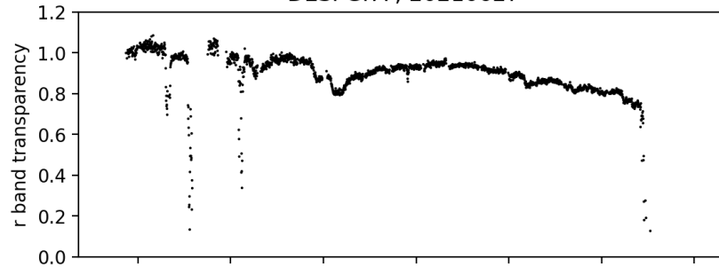
pointing camera zeropoint ; 20210627
