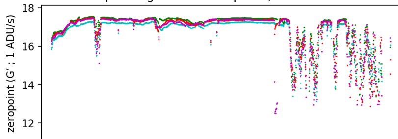
pointing camera sky brightness ; 20210705
