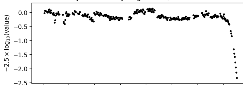
airmass ; 20210708
