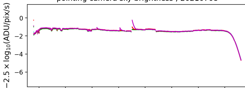
sky monitor sky brightness ; 20210708
