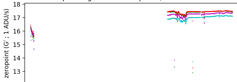
pointing camera sky brightness ; 20210614
