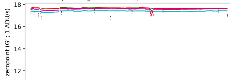
pointing camera sky brightness ; 20210626
