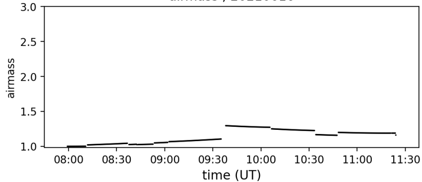
airmass ; 20210616
