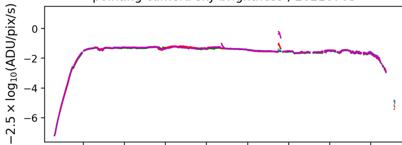
sky monitor sky brightness ; 20210705
