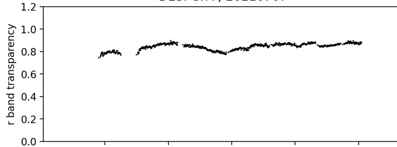
pointing camera zeropoint ; 20210707
