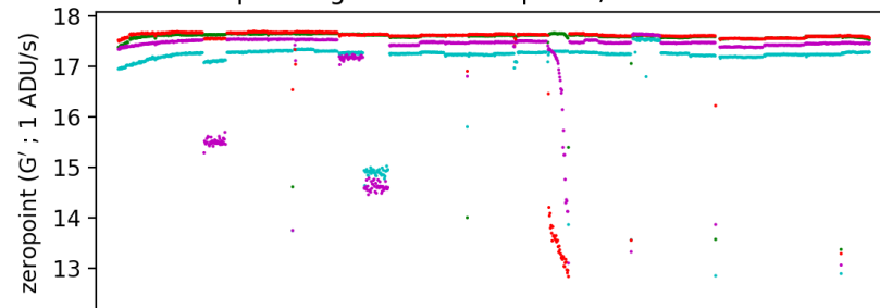
pointing camera sky brightness ; 20210618
