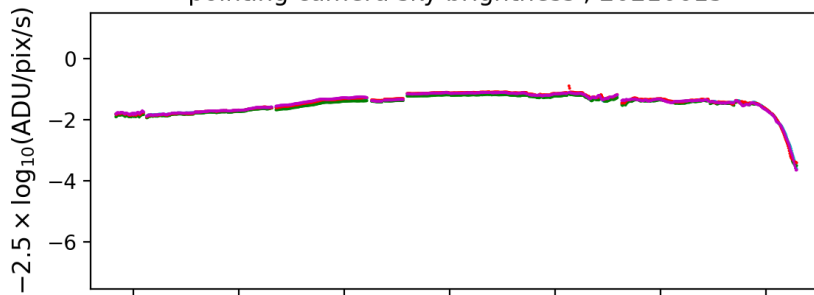
sky monitor sky brightness ; 20210615
