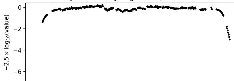
airmass ; 20210613
