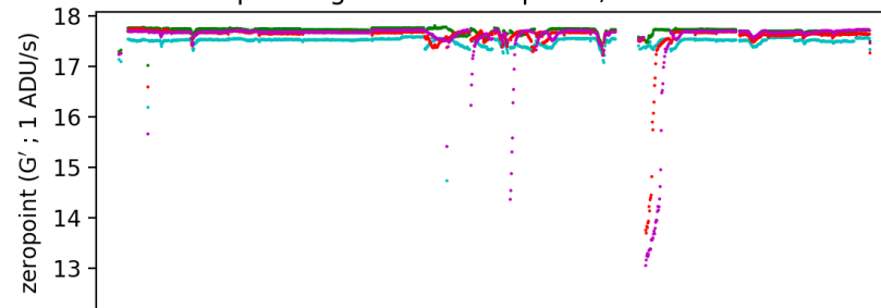
pointing camera sky brightness ; 20210610
