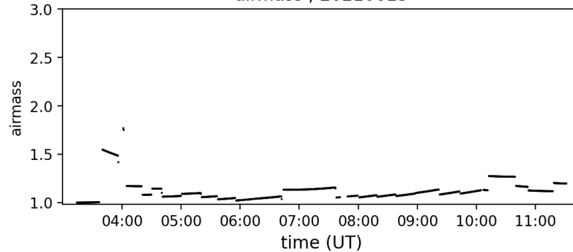
airmass ; 20210613
