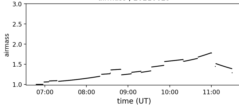
airmass ; 20210629
