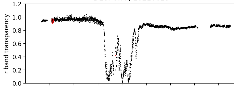
pointing camera zeropoint ; 20210613
