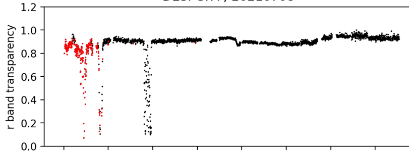
pointing camera zeropoint ; 20210708
