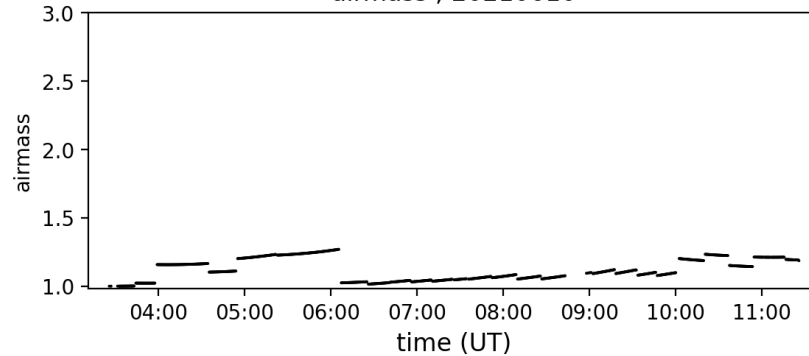
airmass ; 20210610
