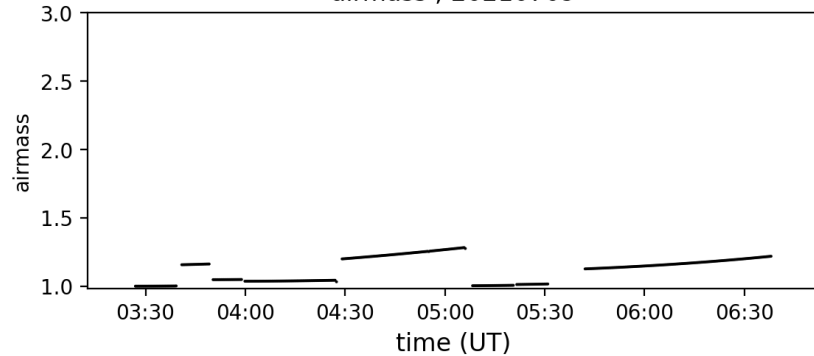
airmass ; 20210709
