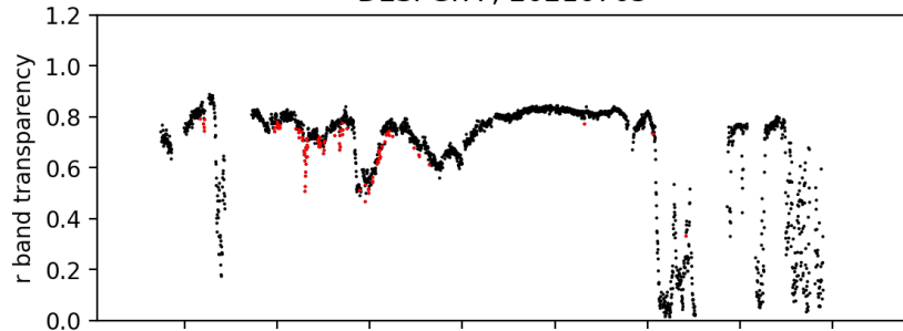
pointing camera zeropoint ; 20210705
