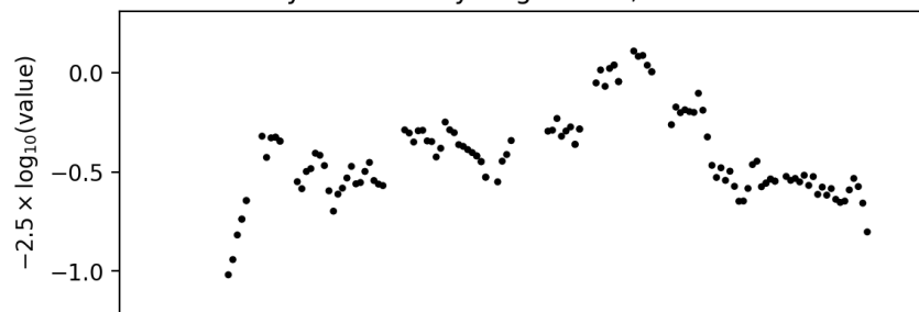
airmass ; 20210709
