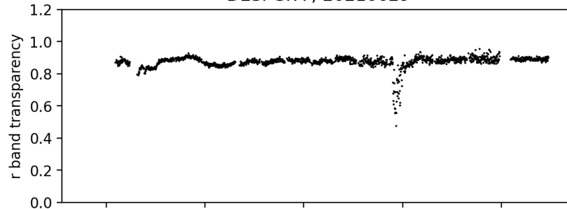
pointing camera zeropoint ; 20210629
