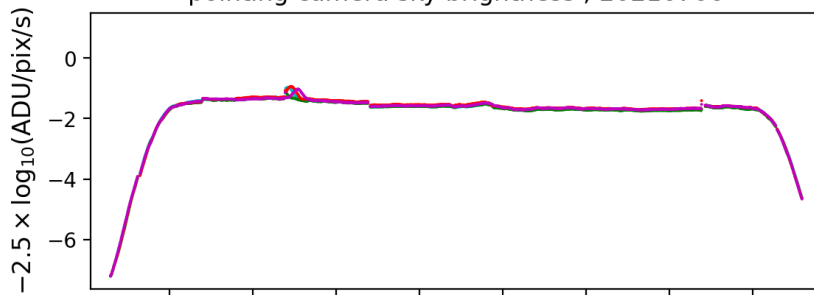
sky monitor sky brightness ; 20210706
