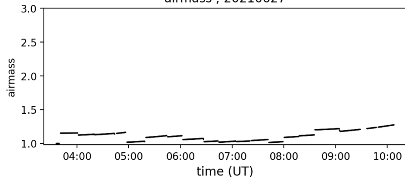
airmass ; 20210627
