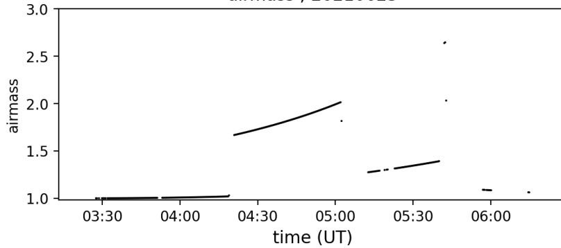
airmass ; 20210623
