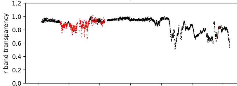
pointing camera zeropoint ; 20210615
