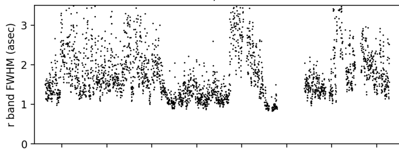
DESI GFA ; 20210609
