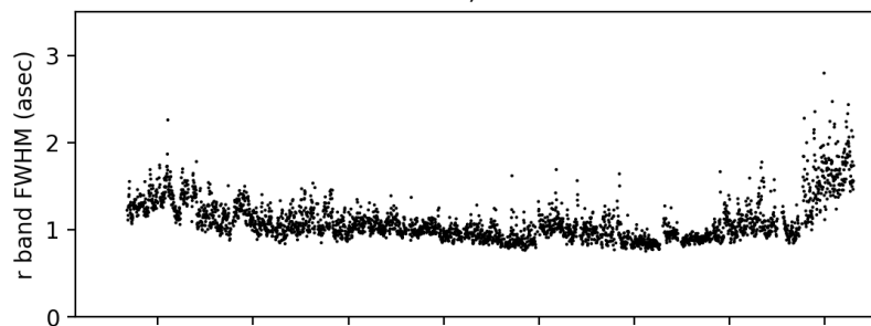
DESI GFA ; 20210619
