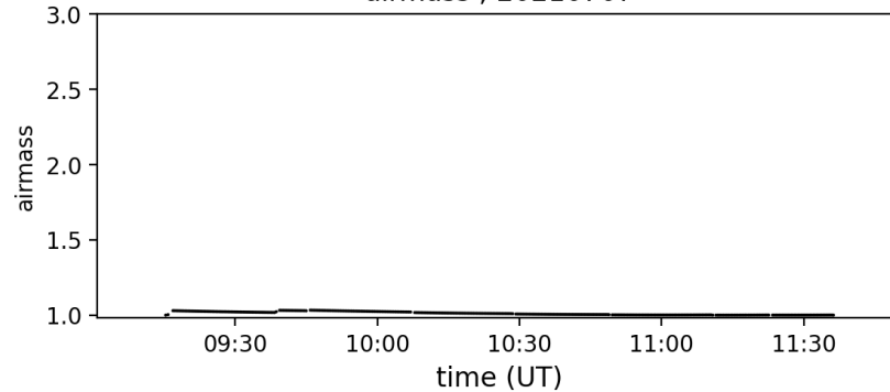
airmass ; 20210707
