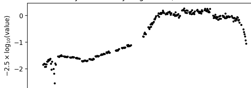
airmass ; 20210617
