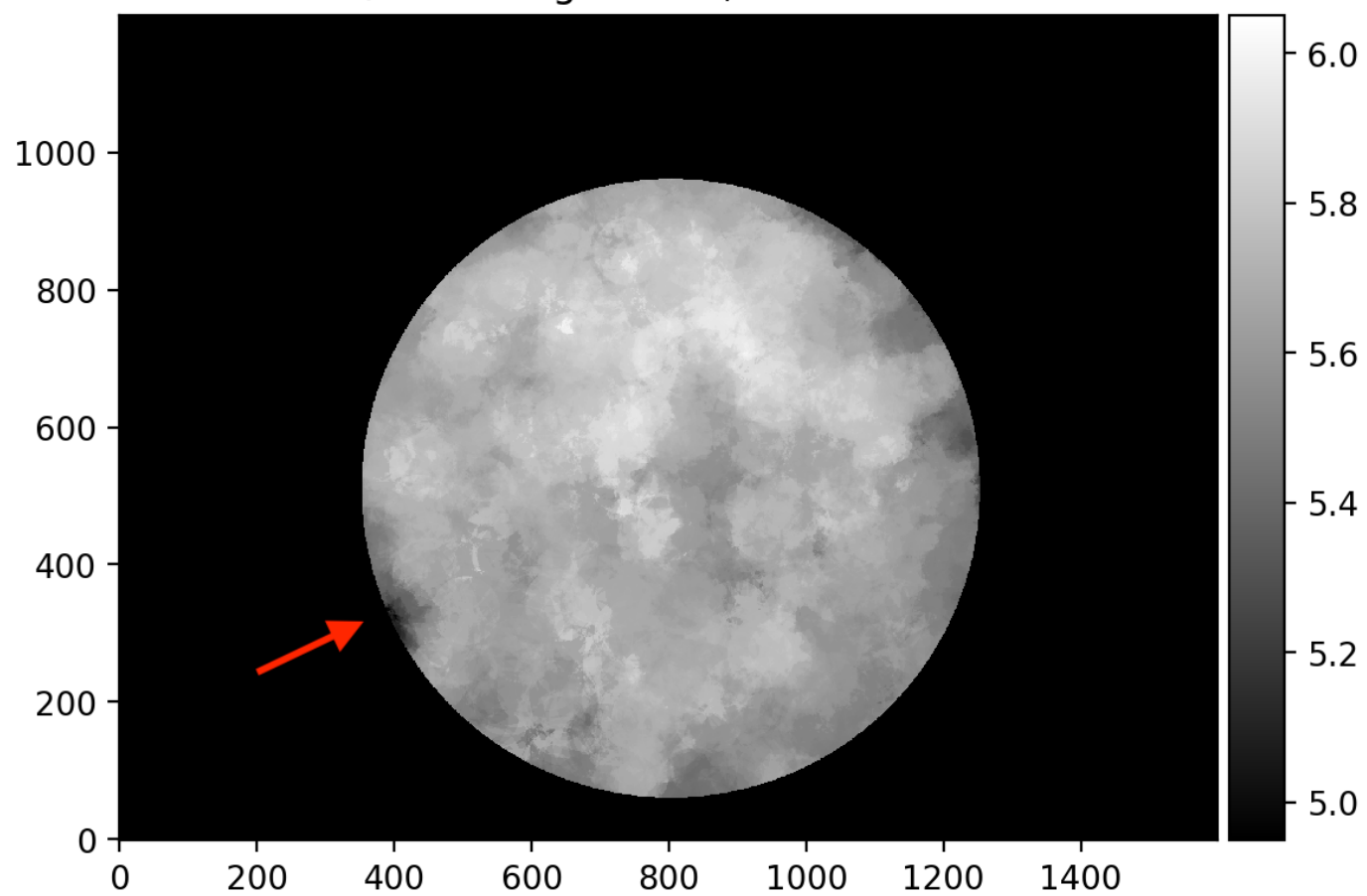
ZP w/in 7.1 deg radius ; median 25 stars
