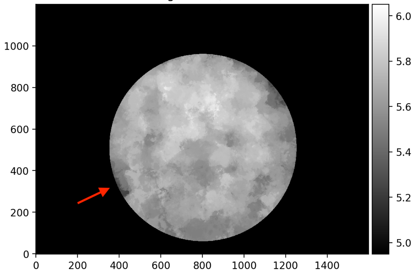
ZP w/in 7.1 deg radius ; median 26 stars
