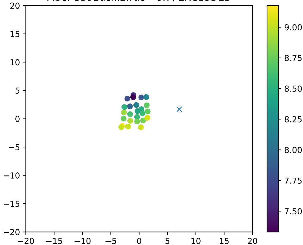
Fiber 3591dchi2frac= 0.7, EXCLUDED
