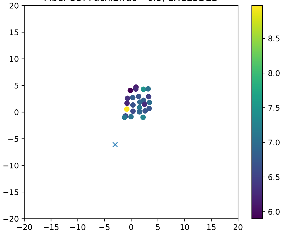
Fiber 3877dchi2frac= 0.5, EXCLUDED
