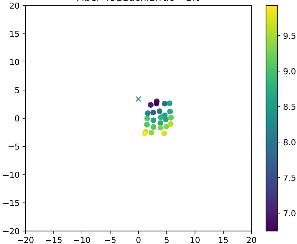
Fiber 4311dchi2frac= 1.0
