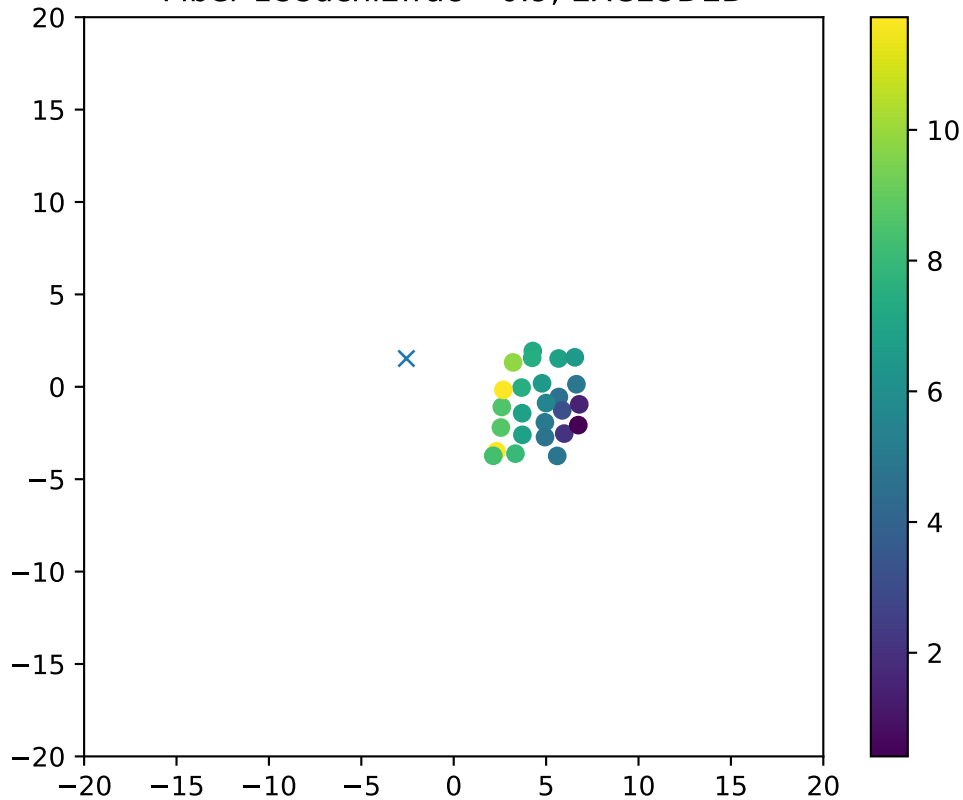
Fiber 188dchi2frac= 0.9, EXCLUDED
