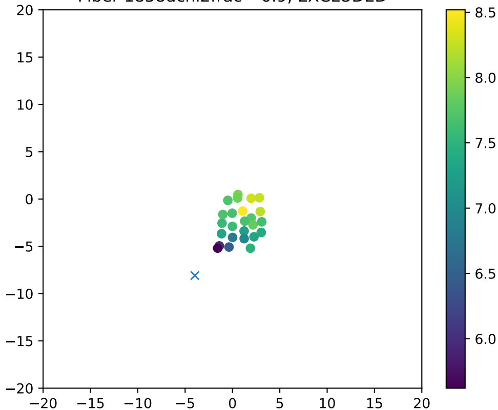
Fiber 1858dchi2frac= 0.9, EXCLUDED
