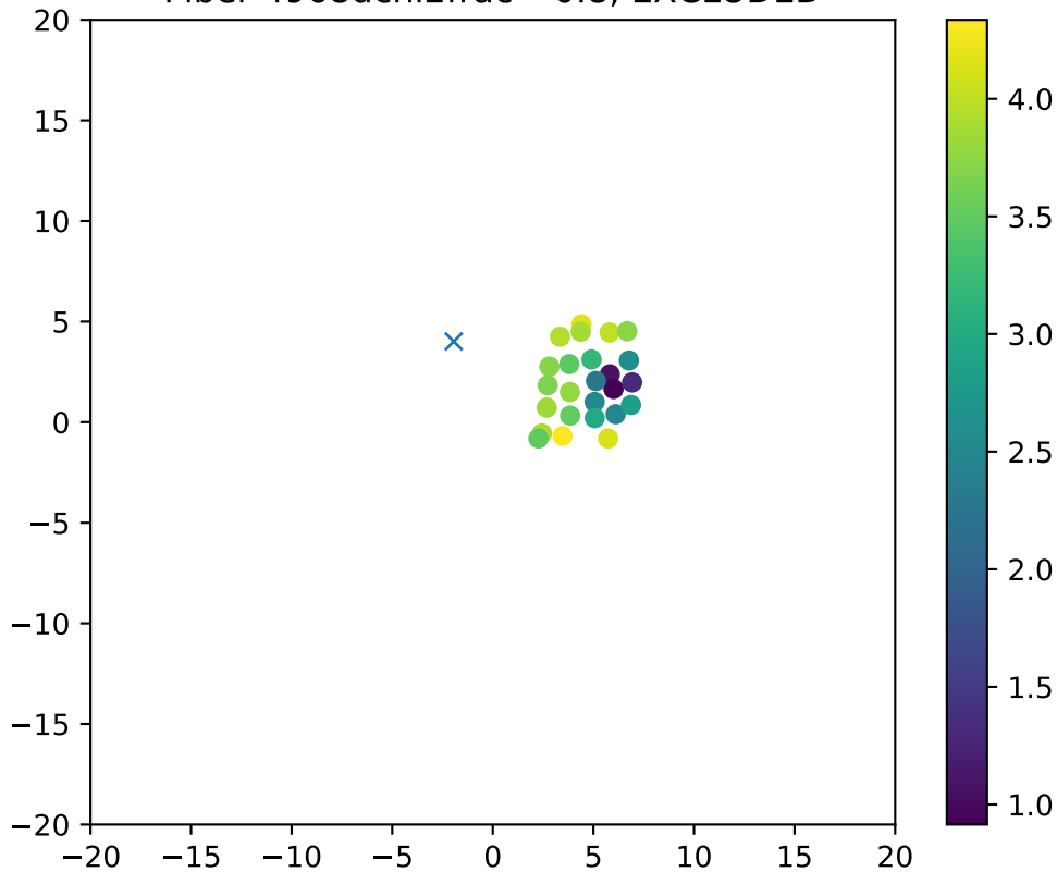
Fiber 4968dchi2frac= 0.8, EXCLUDED
