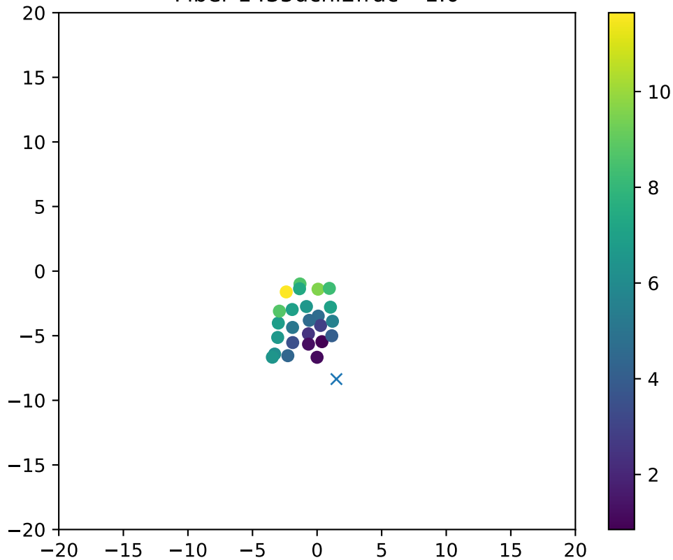
Fiber 1435dchi2frac= 1.0
