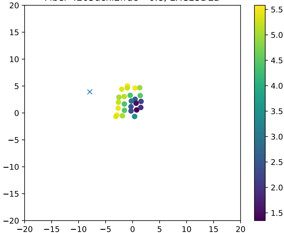
Fiber 4205dchi2frac= 0.8, EXCLUDED
