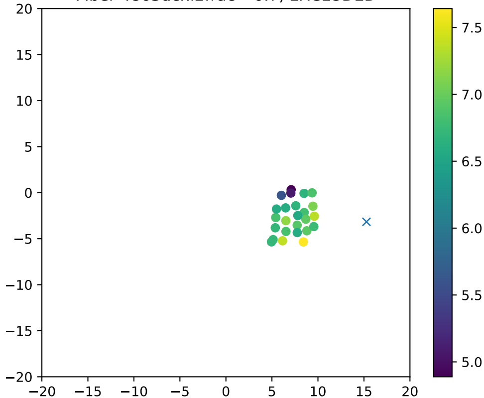
Fiber 4863dchi2frac= 0.7, EXCLUDED
