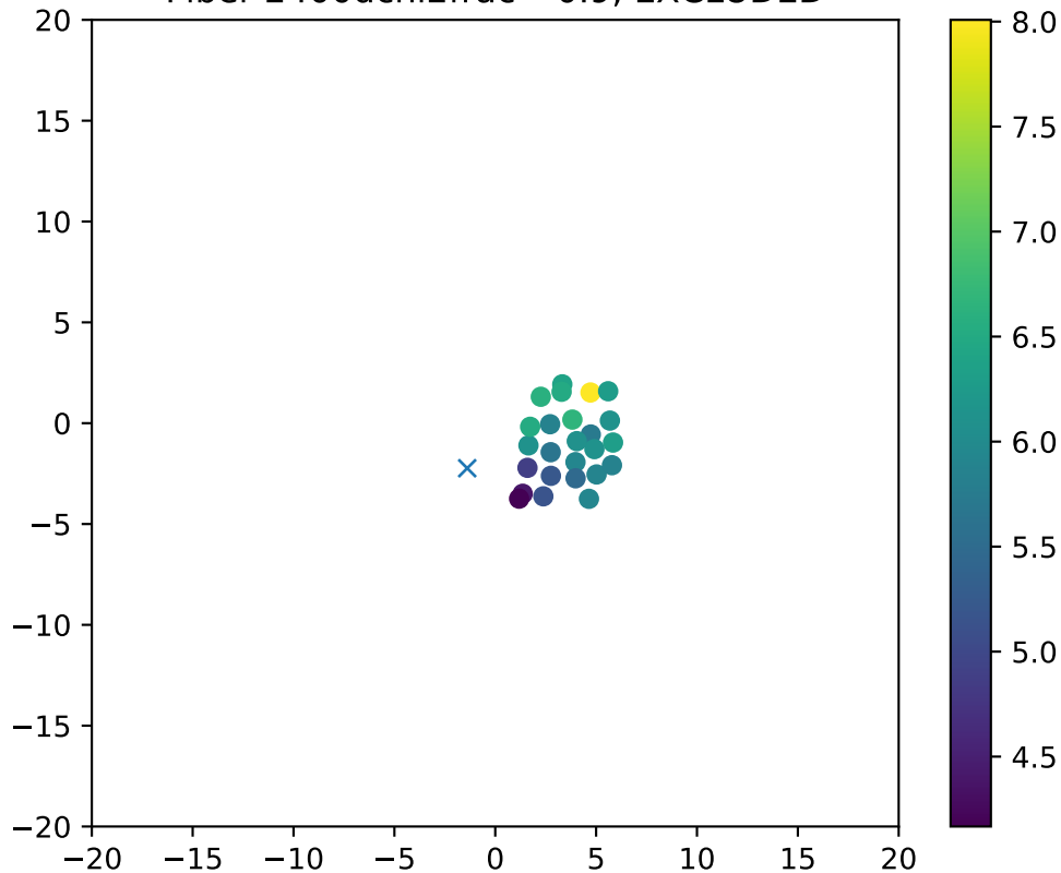
Fiber 2400dchi2frac= 0.9, EXCLUDED
