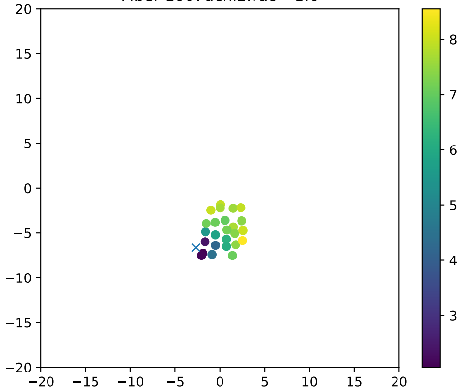
Fiber 1667dchi2frac= 1.0
