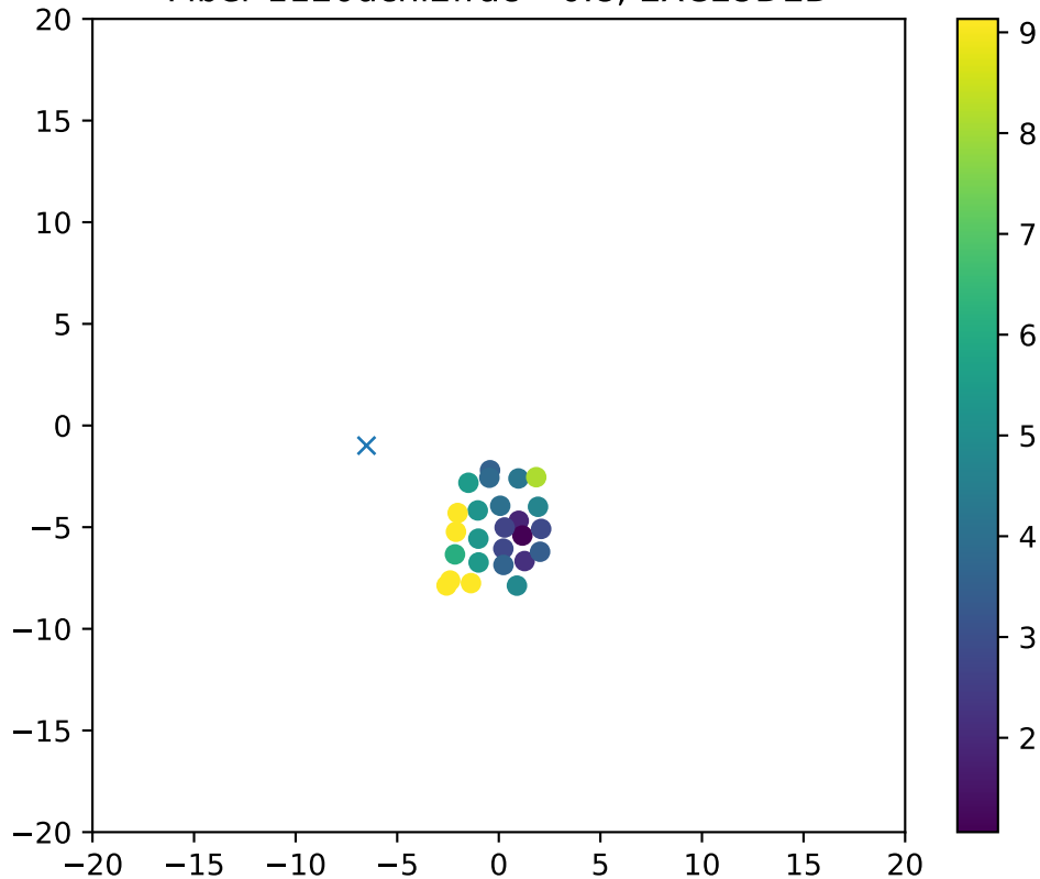
Fiber 1120dchi2frac= 0.8, EXCLUDED
