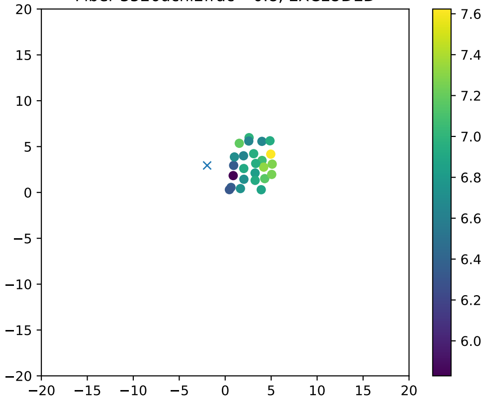
Fiber 3526dchi2frac= 0.8, EXCLUDED
