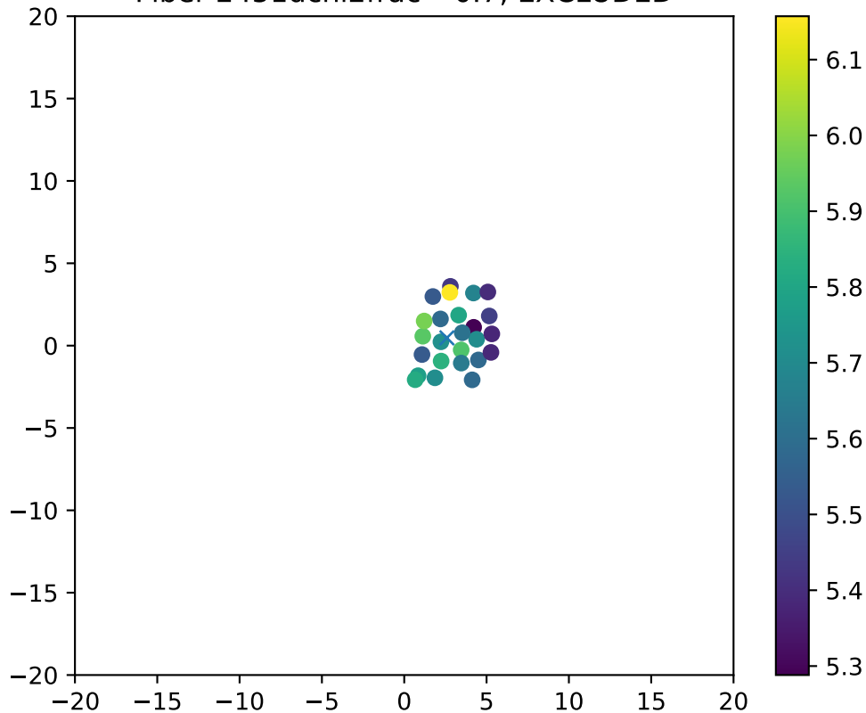
Fiber 2451dchi2frac= 0.7, EXCLUDED
