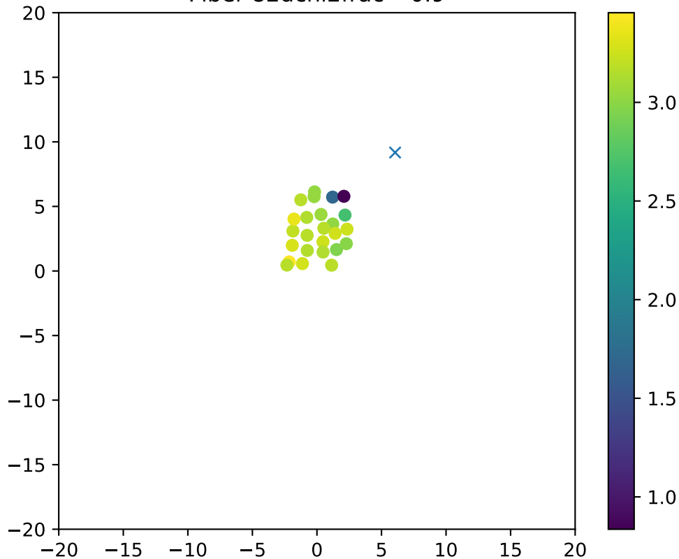
Fiber 82dchi2frac= 0.9
