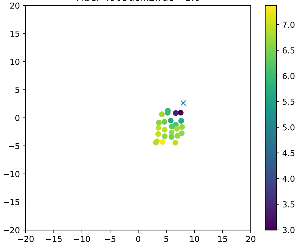
Fiber 4905dchi2frac= 1.0
