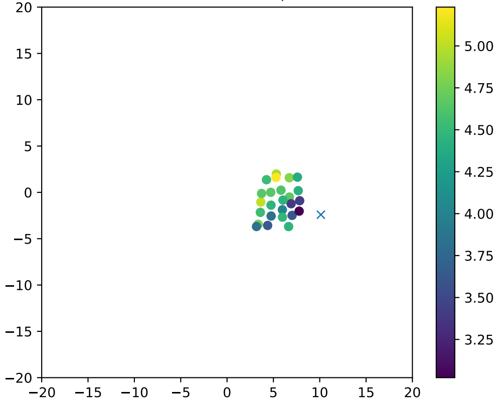
Fiber 1016dchi2frac= 0.8, EXCLUDED
