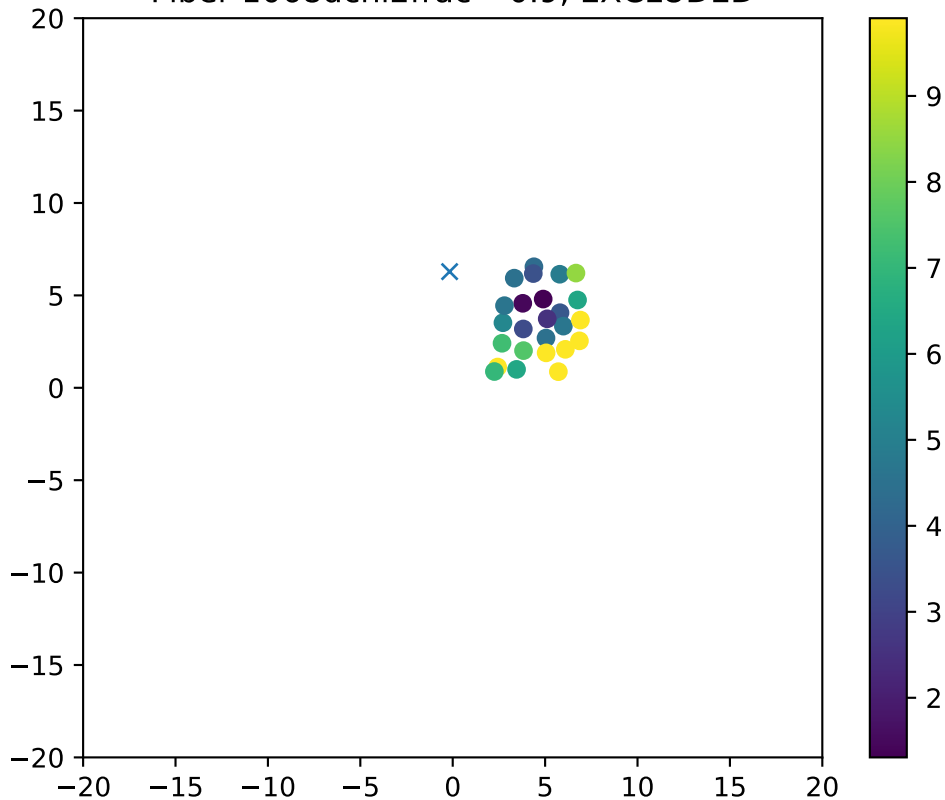
Fiber 1068dchi2frac= 0.9, EXCLUDED
