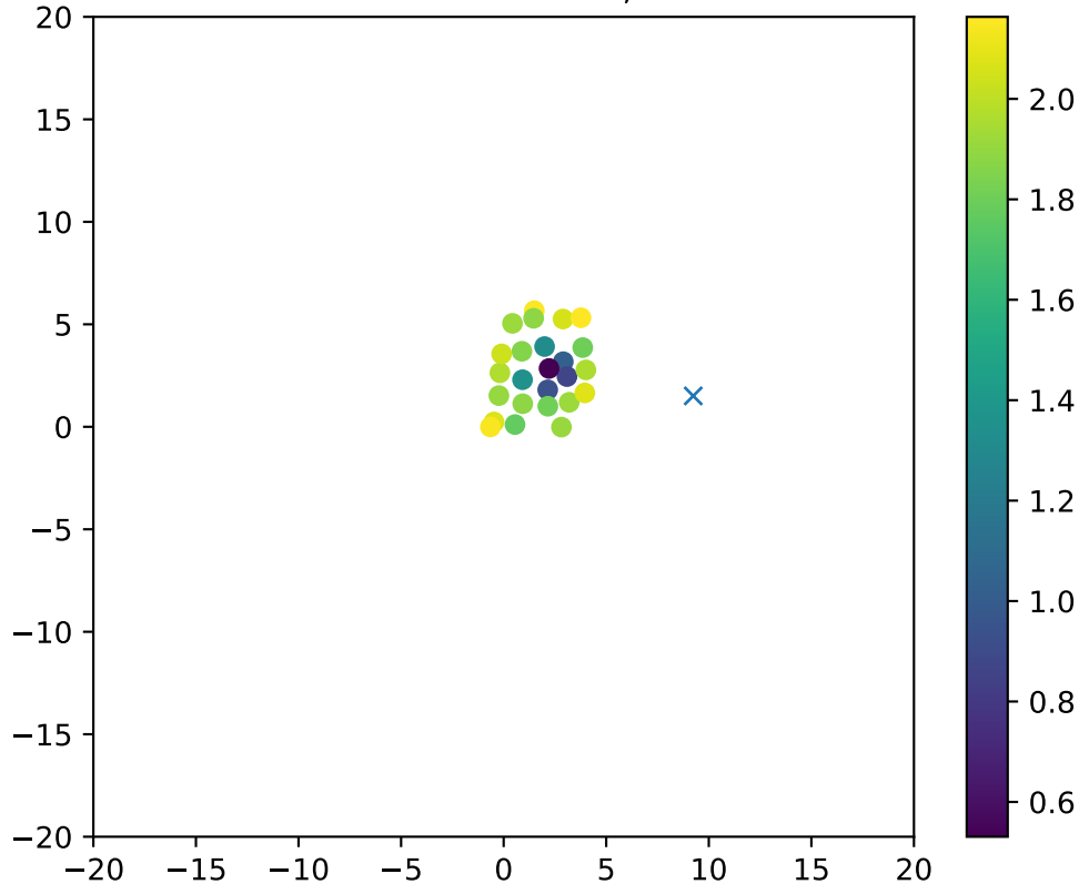
Fiber 4555dchi2frac= 0.8, EXCLUDED
