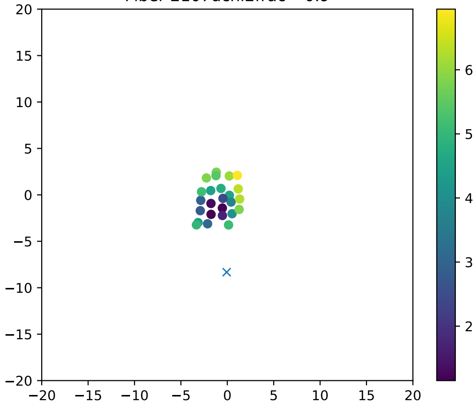
Fiber 2107dchi2frac= 0.9
