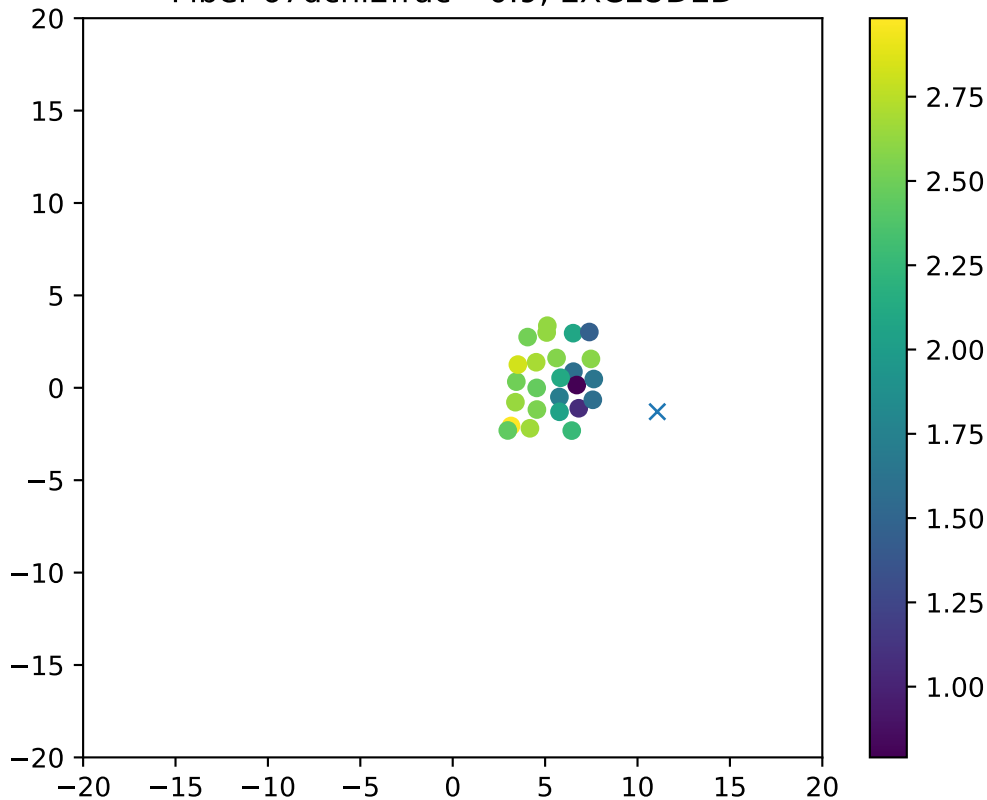
Fiber 67dchi2frac= 0.9, EXCLUDED
