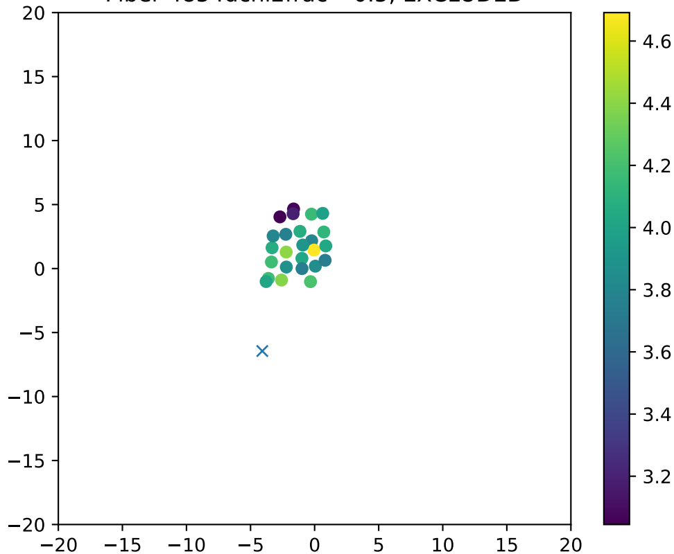
Fiber 4854dchi2frac= 0.5, EXCLUDED
