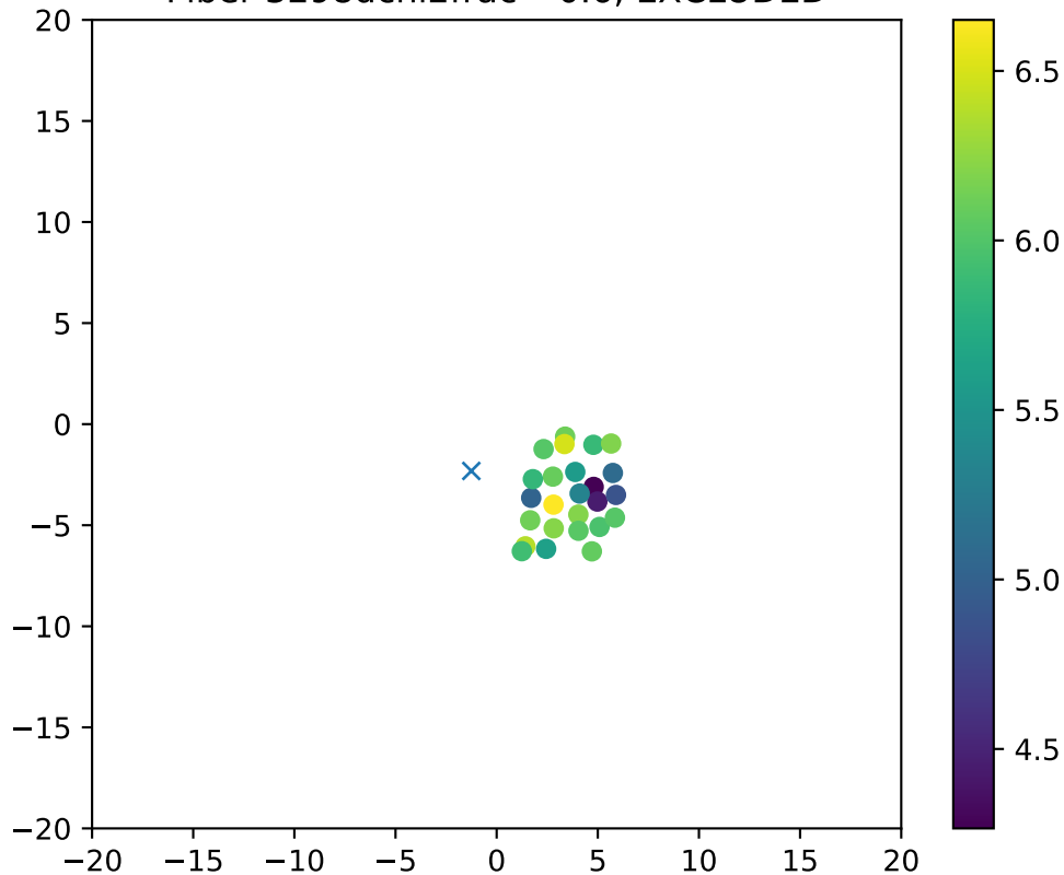
Fiber 3298dchi2frac= 0.6, EXCLUDED
