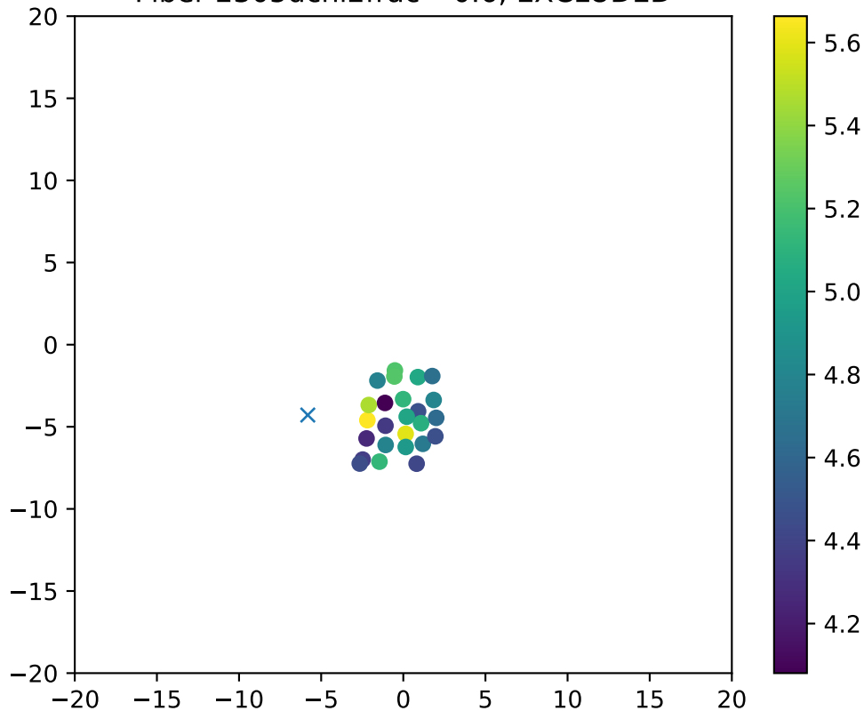
Fiber 2305dchi2frac= 0.6, EXCLUDED
