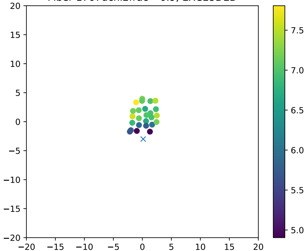
Fiber 1707dchi2frac= 0.9, EXCLUDED
