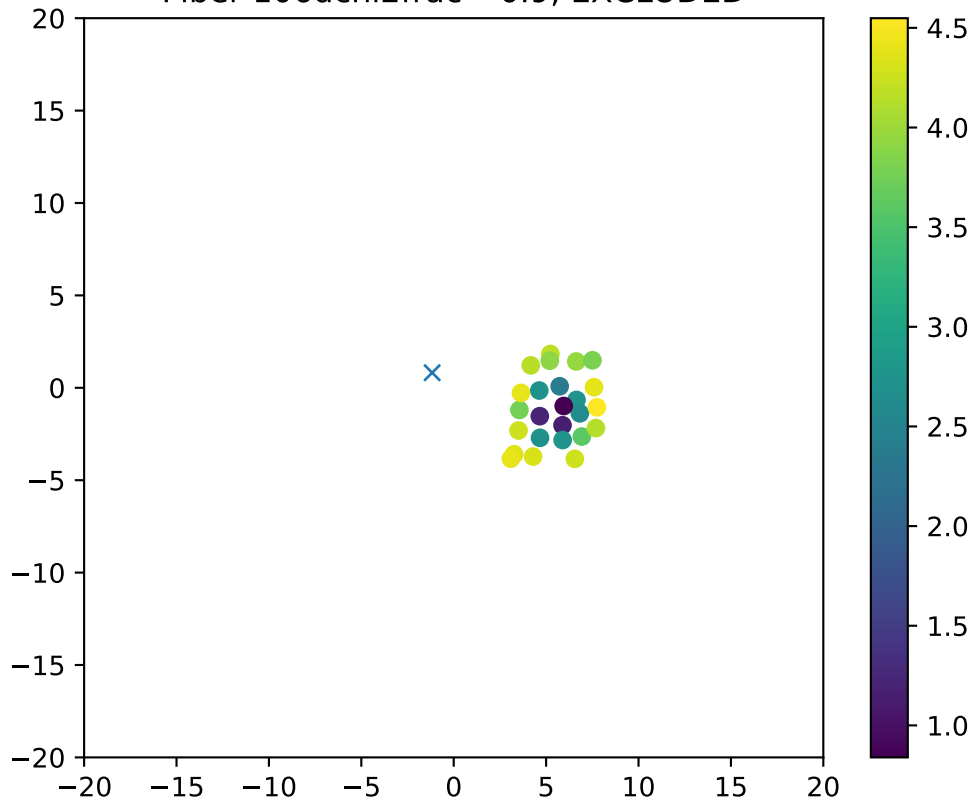
Fiber 106dchi2frac= 0.9, EXCLUDED
