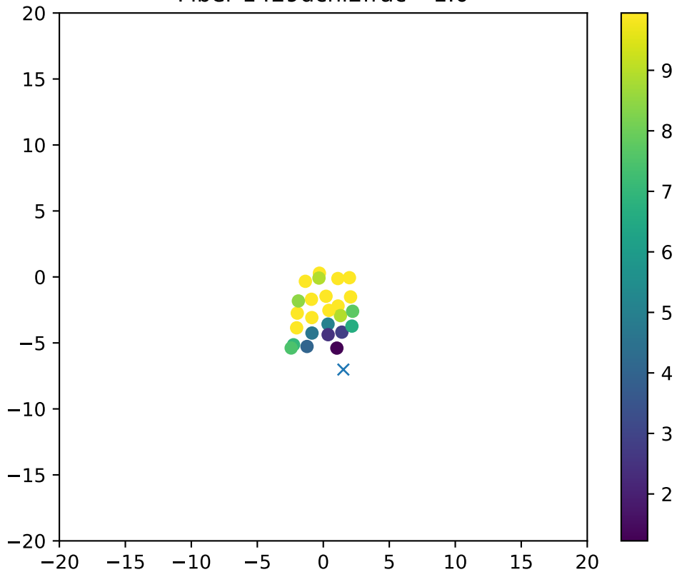
Fiber 1429dchi2frac= 1.0
