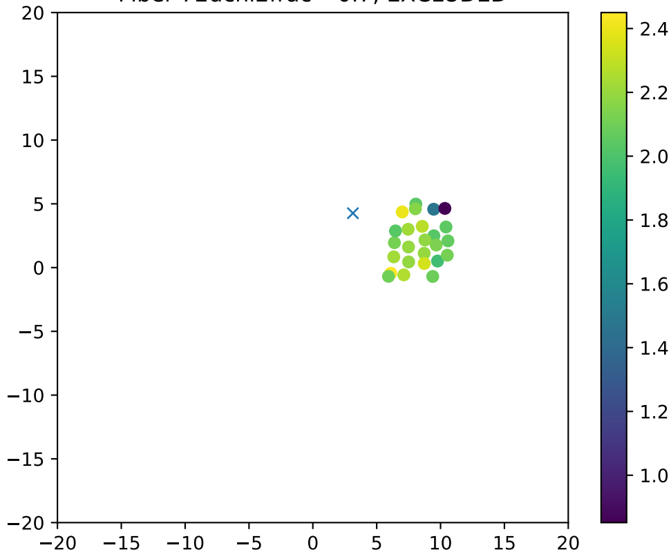
Fiber 72dchi2frac= 0.7, EXCLUDED
