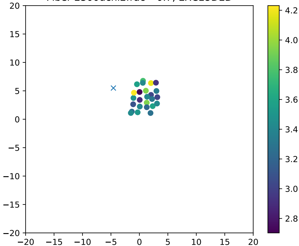
Fiber 2300dchi2frac= 0.7, EXCLUDED
