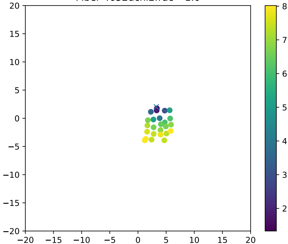
Fiber 4652dchi2frac= 1.0
