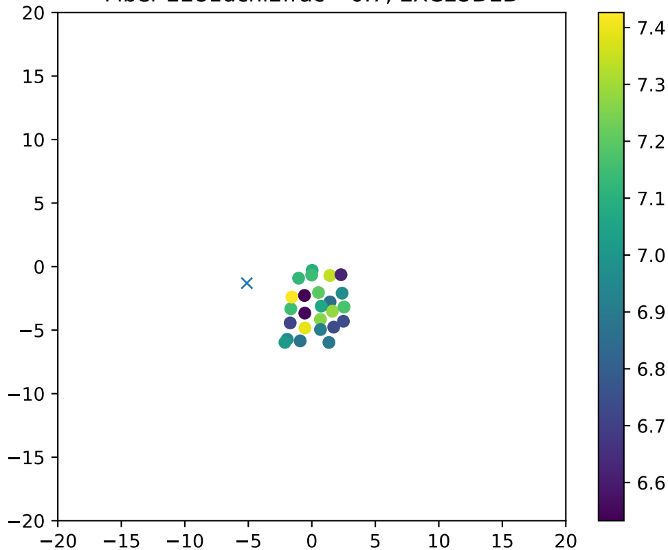
Fiber 2281dchi2frac= 0.7, EXCLUDED
