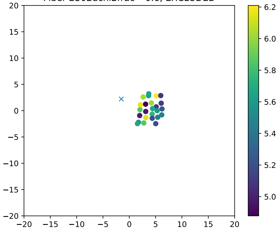
Fiber 2302dchi2frac= 0.6, EXCLUDED
