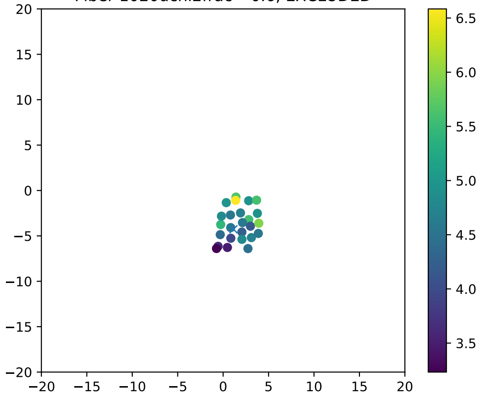
Fiber 1020dchi2frac= 0.6, EXCLUDED
