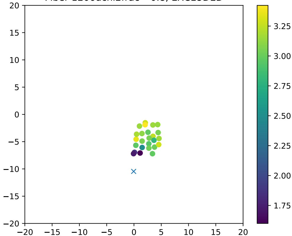
Fiber 1206dchi2frac= 0.8, EXCLUDED
