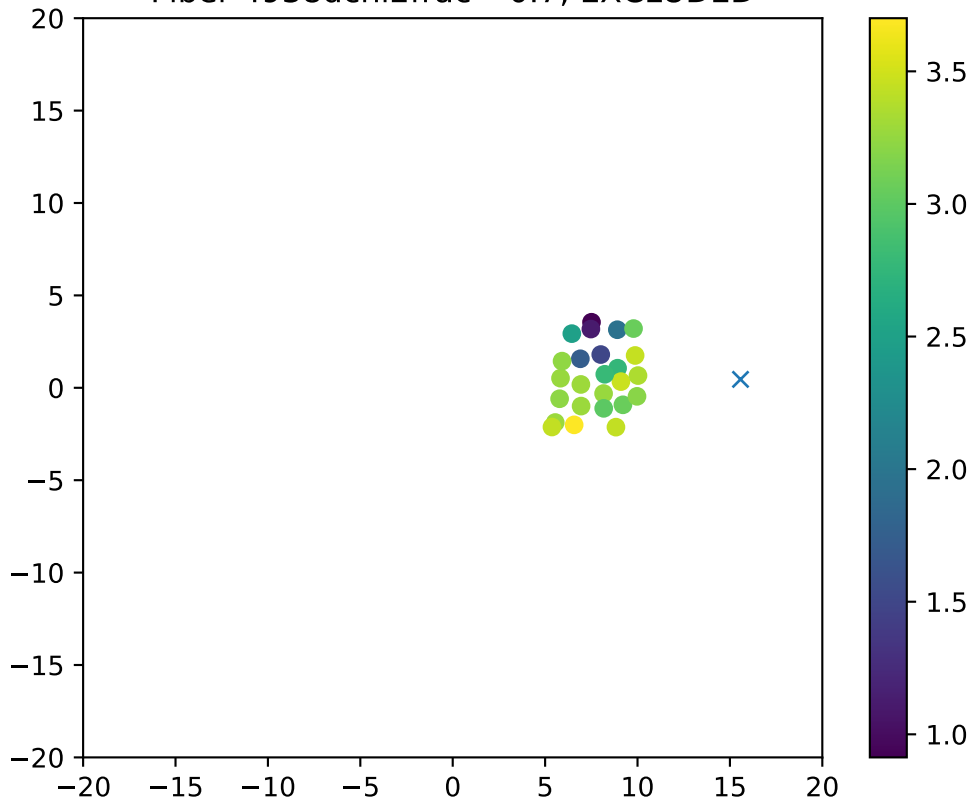
Fiber 4938dchi2frac= 0.7, EXCLUDED
