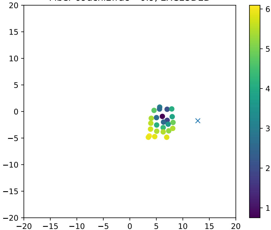
Fiber 69dchi2frac= 0.9, EXCLUDED
