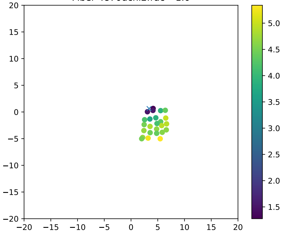
Fiber 4870dchi2frac= 1.0
