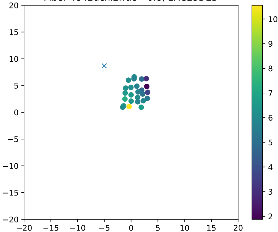
Fiber 4842dchi2frac= 0.8, EXCLUDED
