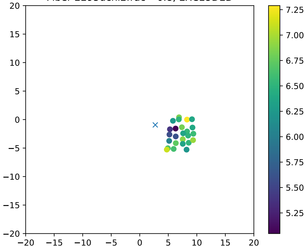
Fiber 2295dchi2frac= 0.8, EXCLUDED
