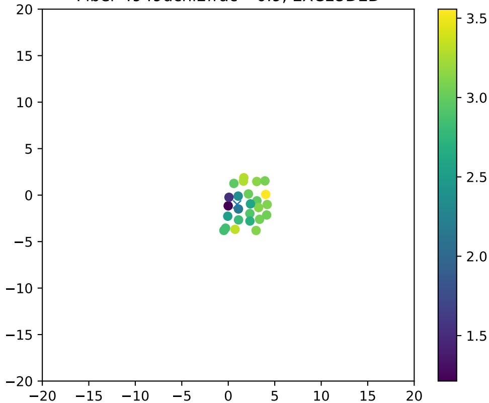
Fiber 4949dchi2frac= 0.9, EXCLUDED
