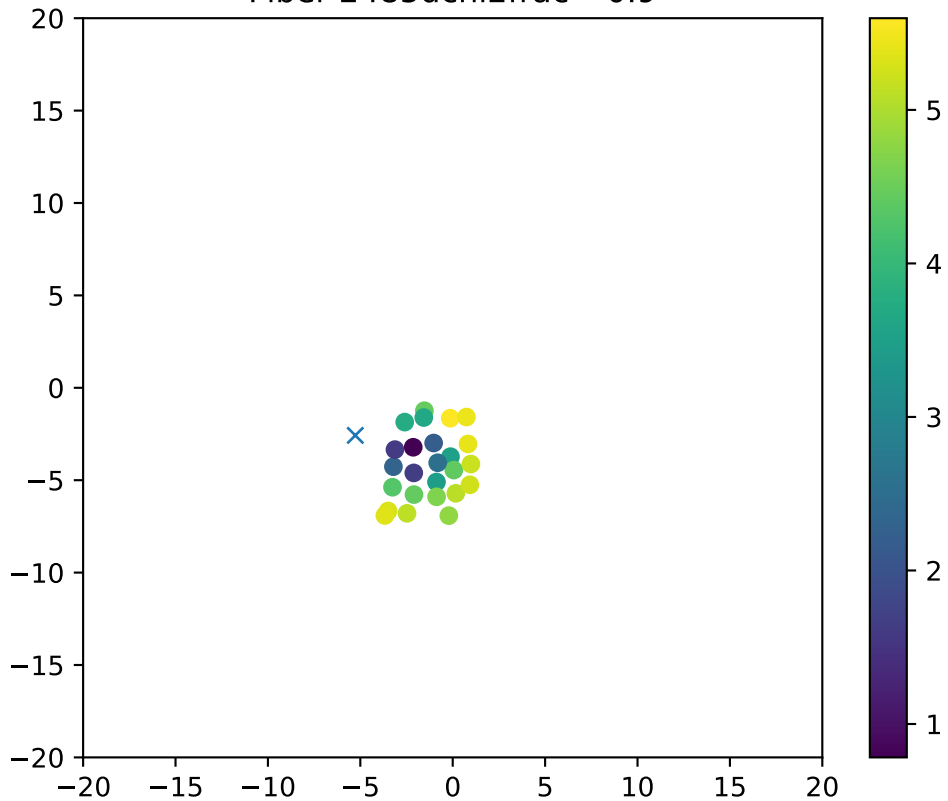
Fiber 2485dchi2frac= 0.9
