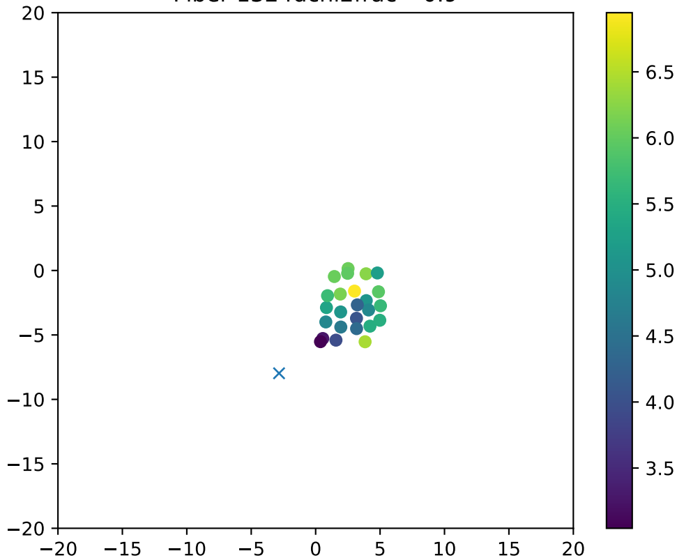
Fiber 1324dchi2frac= 0.9
