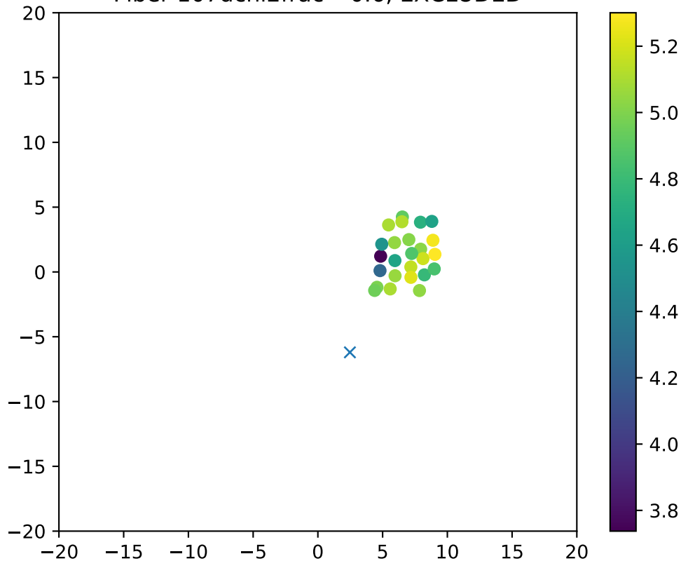
Fiber 107dchi2frac= 0.6, EXCLUDED
