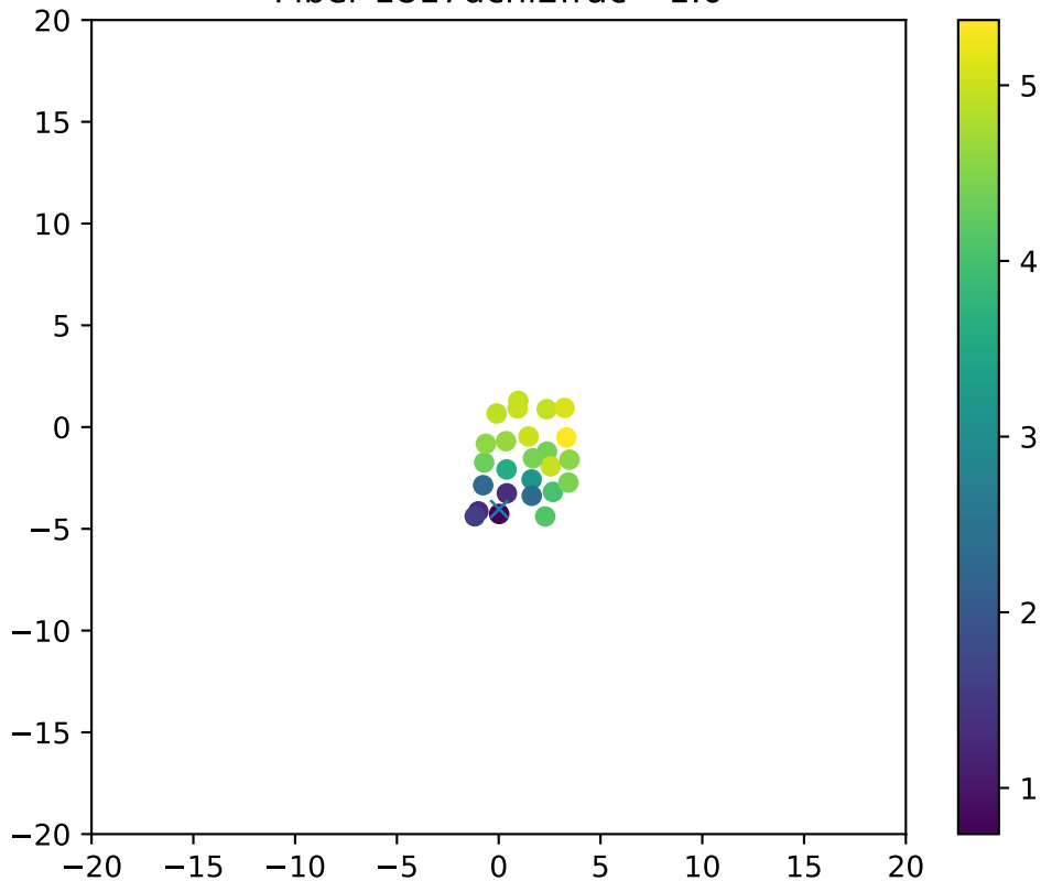
Fiber 1817dchi2frac= 1.0
