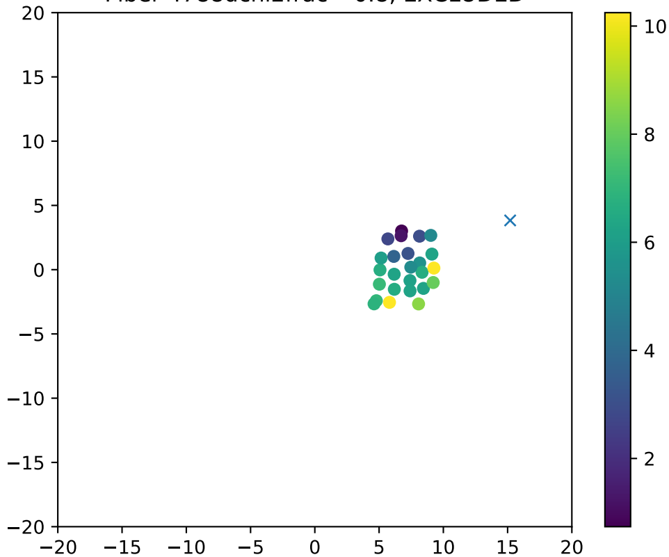
Fiber 4788dchi2frac= 0.8, EXCLUDED
