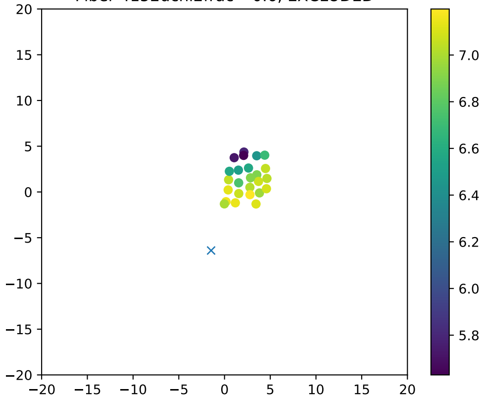
Fiber 4152dchi2frac= 0.6, EXCLUDED
