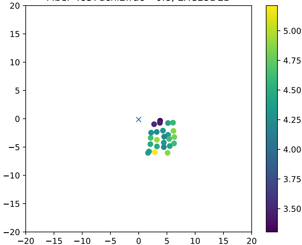
Fiber 4857dchi2frac= 0.8, EXCLUDED
