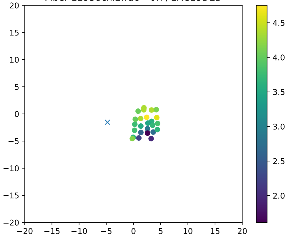
Fiber 1293dchi2frac= 0.7, EXCLUDED
