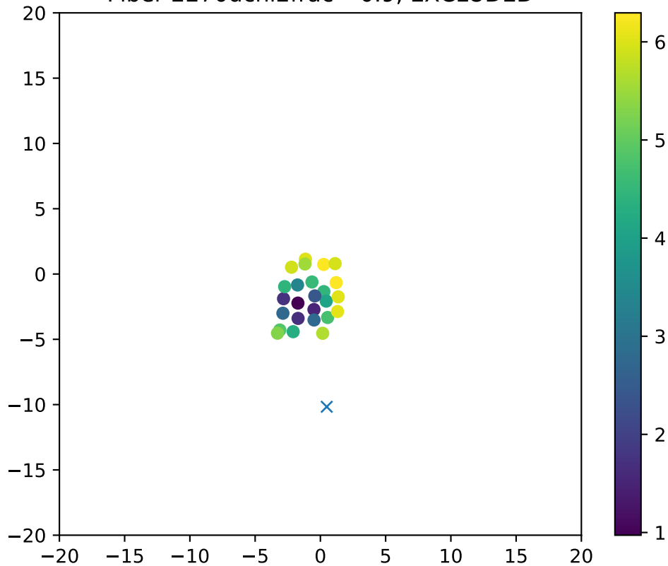
Fiber 2270dchi2frac= 0.9, EXCLUDED
