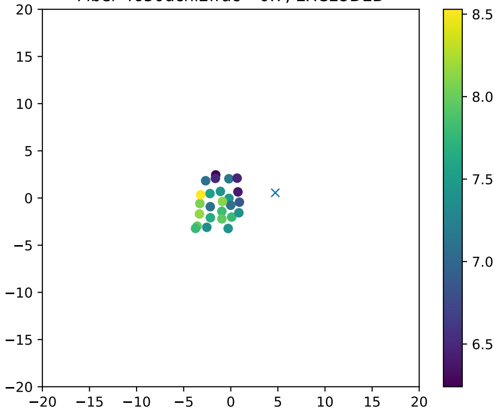
Fiber 4650dchi2frac= 0.7, EXCLUDED
