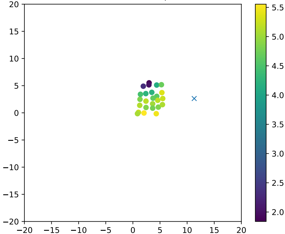
Fiber 4867dchi2frac= 0.8, EXCLUDED
