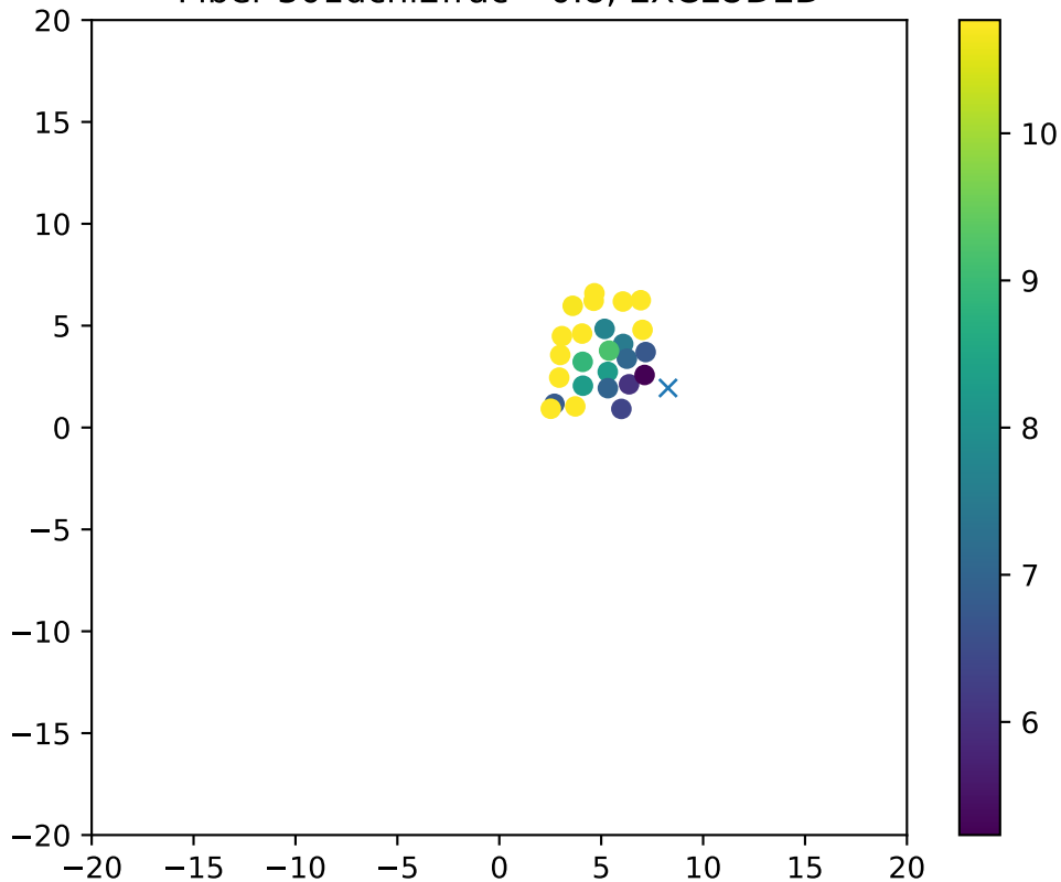
Fiber 301dchi2frac= 0.8, EXCLUDED
