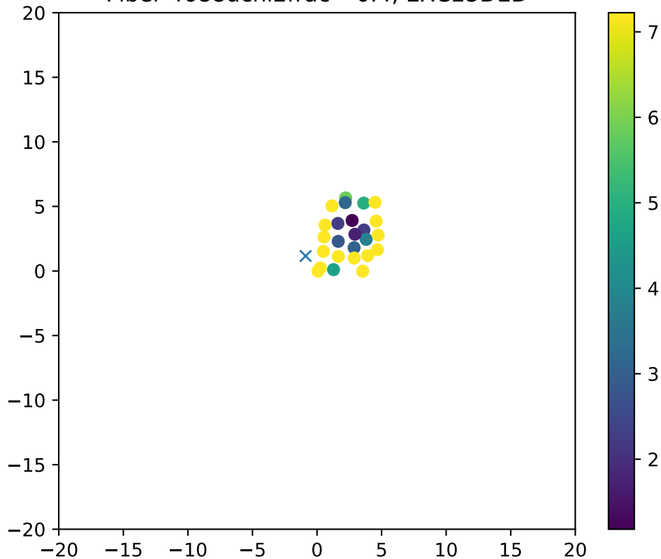
Fiber 4688dchi2frac= 0.4, EXCLUDED
