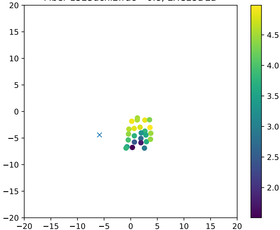
Fiber 1323dchi2frac= 0.8, EXCLUDED
