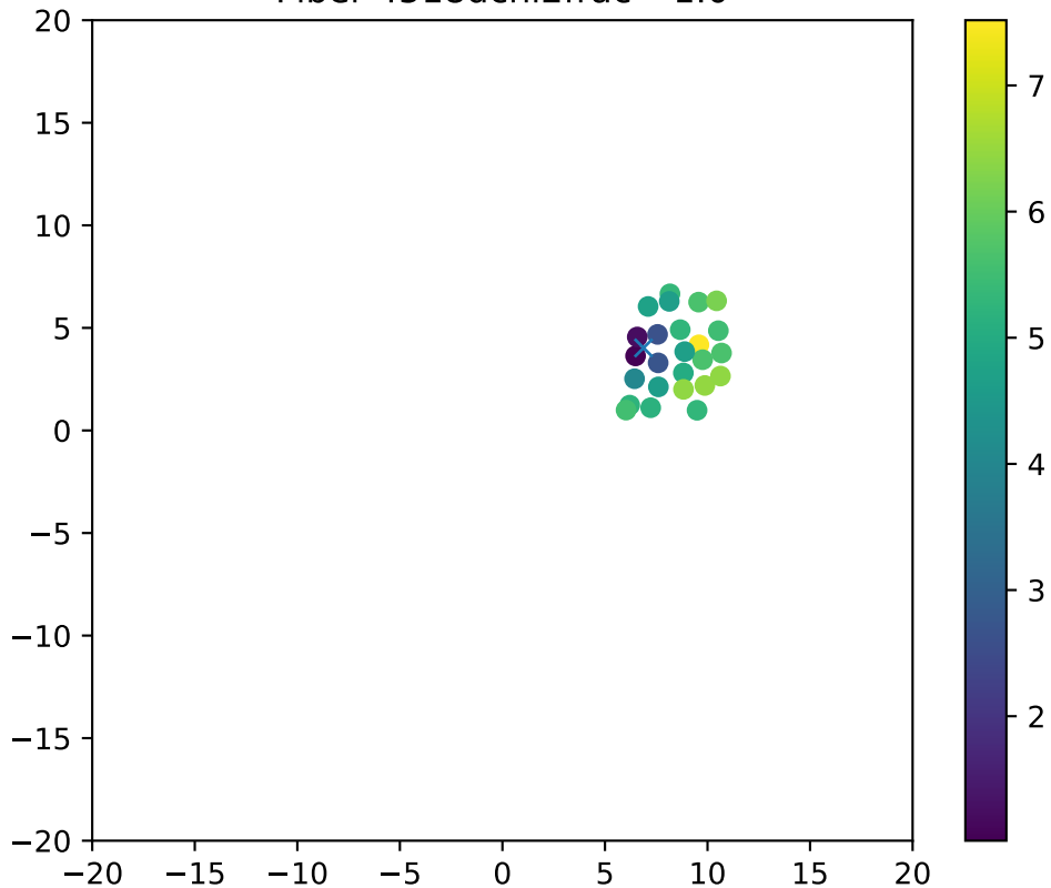
Fiber 4518dchi2frac= 1.0
