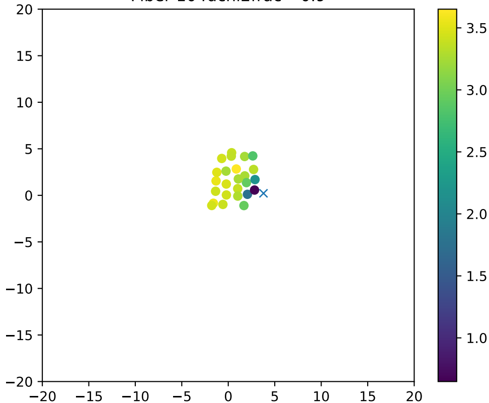
Fiber 104dchi2frac= 0.9
