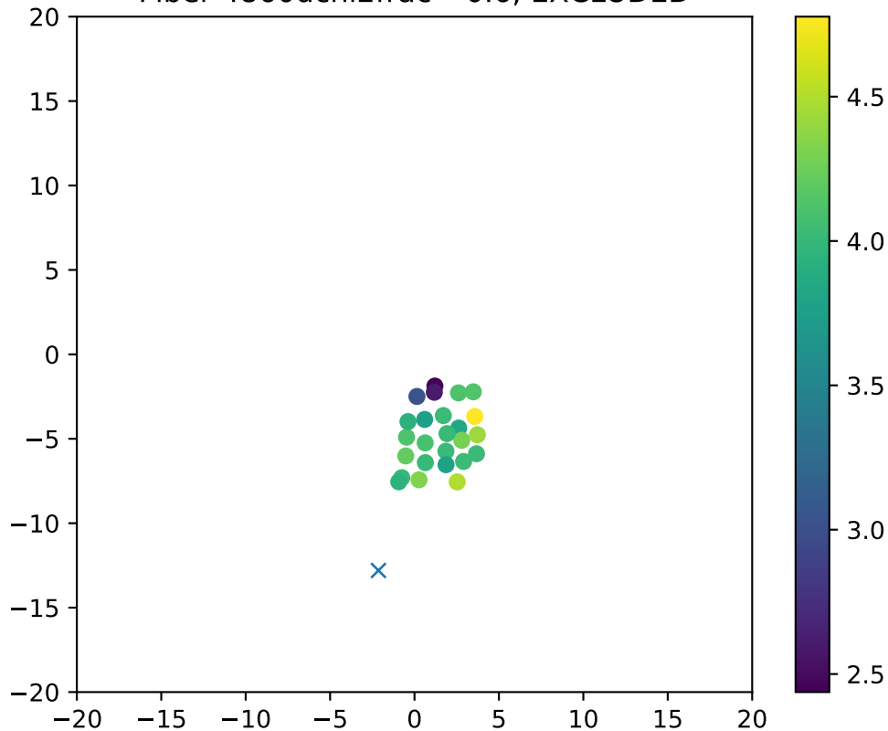
Fiber 4860dchi2frac= 0.6, EXCLUDED
