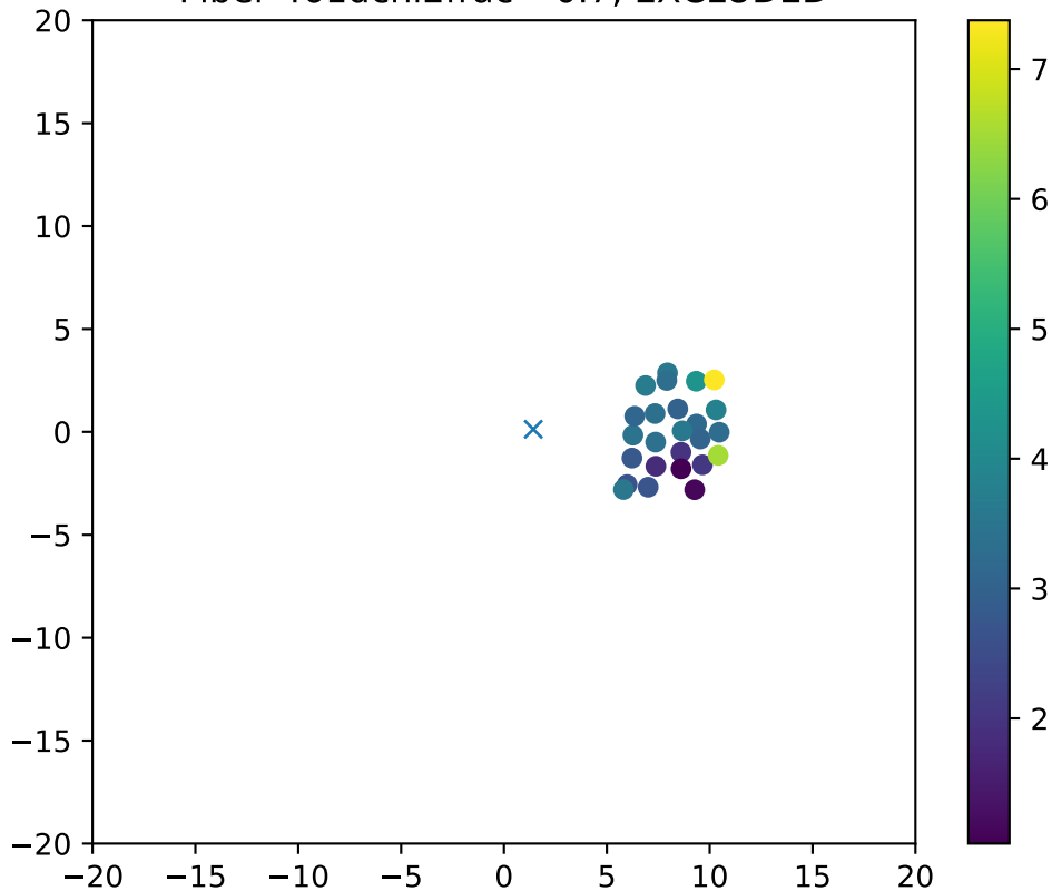
Fiber 461dchi2frac= 0.7, EXCLUDED
