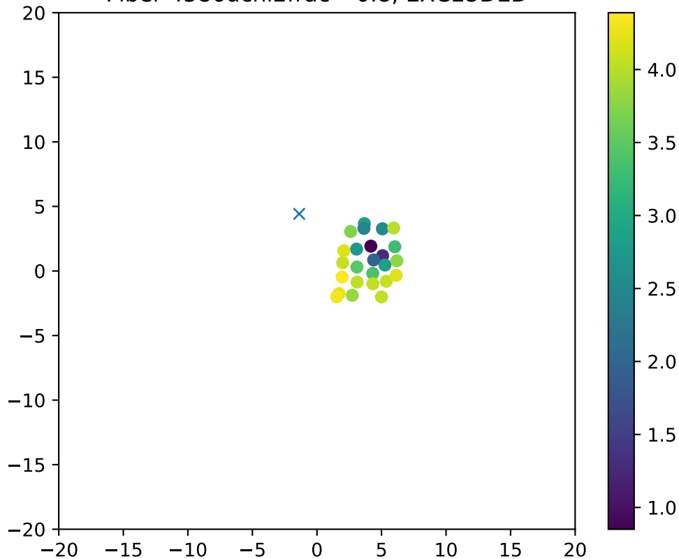
Fiber 4586dchi2frac= 0.8, EXCLUDED
