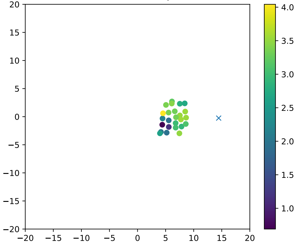
Fiber 120dchi2frac= 0.6, EXCLUDED
