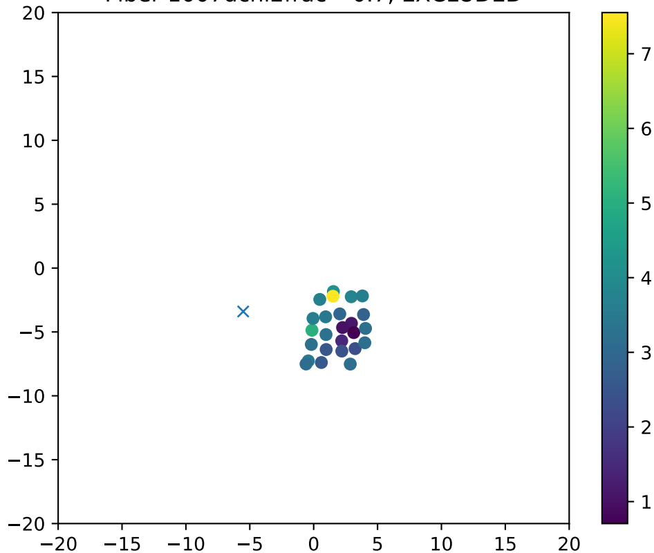
Fiber 1007dchi2frac= 0.7, EXCLUDED
