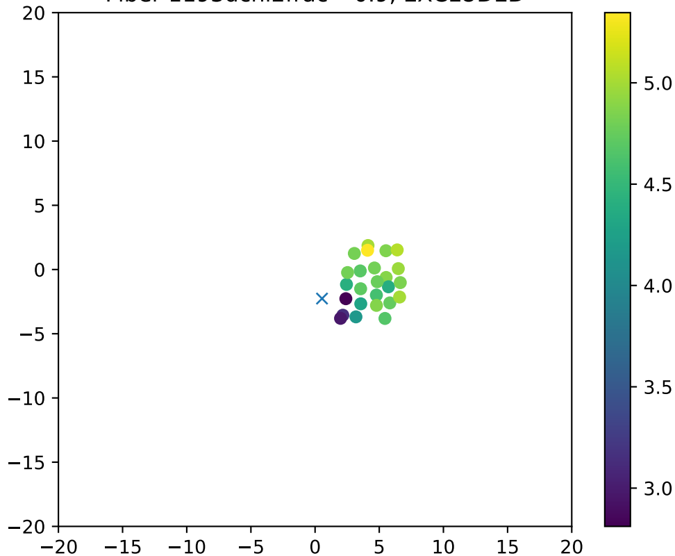
Fiber 1193dchi2frac= 0.9, EXCLUDED
