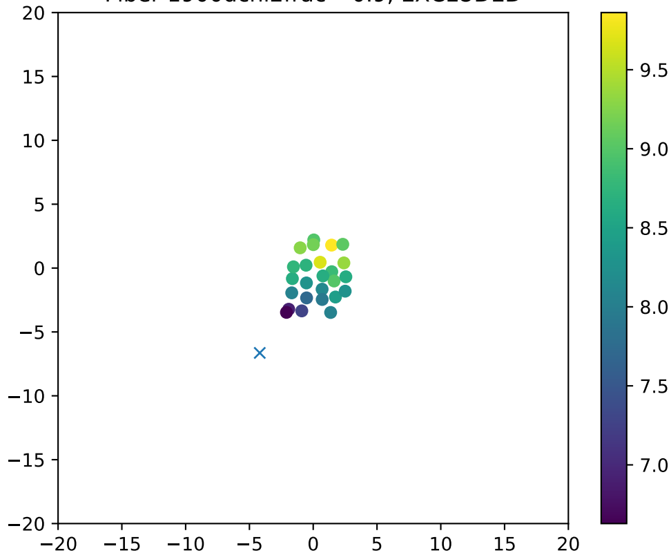
Fiber 1900dchi2frac= 0.9, EXCLUDED
