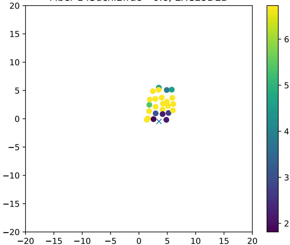
Fiber 143dchi2frac= 0.6, EXCLUDED
