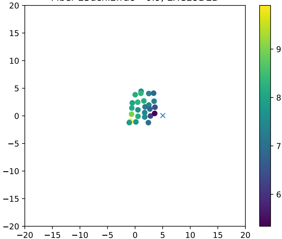
Fiber 23dchi2frac= 0.9, EXCLUDED
