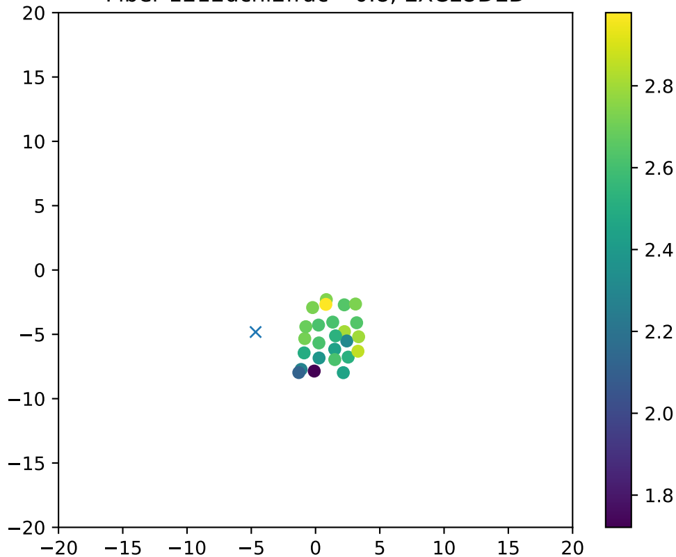
Fiber 1212dchi2frac= 0.8, EXCLUDED
