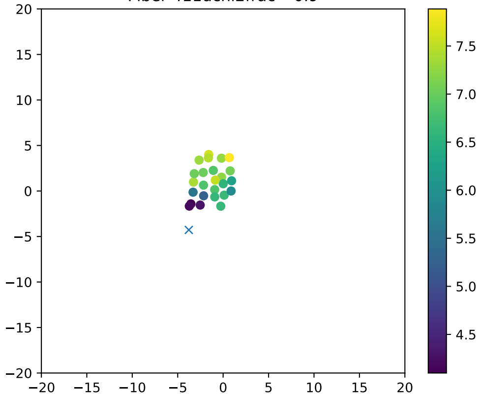
Fiber 411dchi2frac= 0.9
