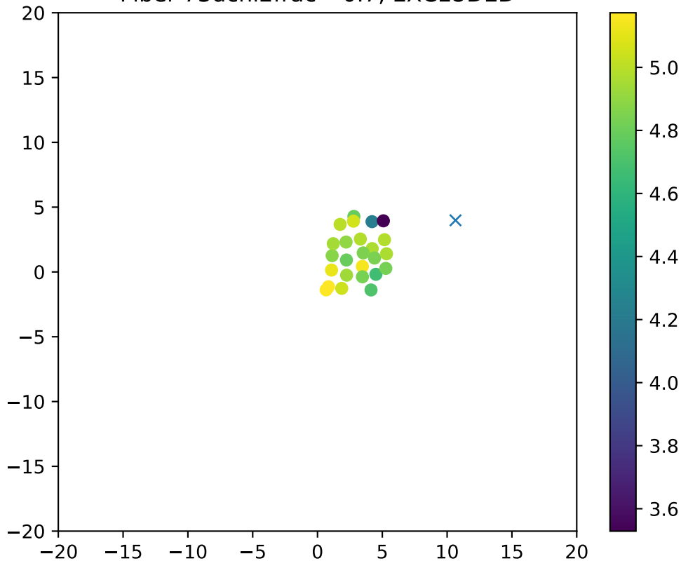
Fiber 73dchi2frac= 0.7, EXCLUDED
