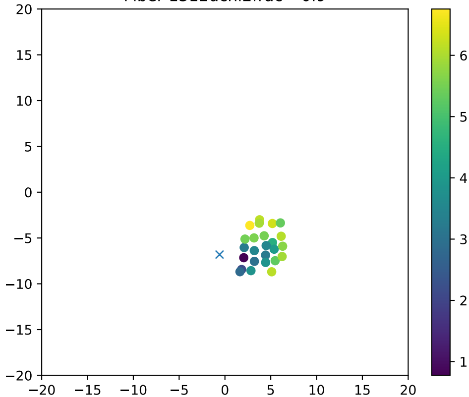
Fiber 1312dchi2frac= 0.9
