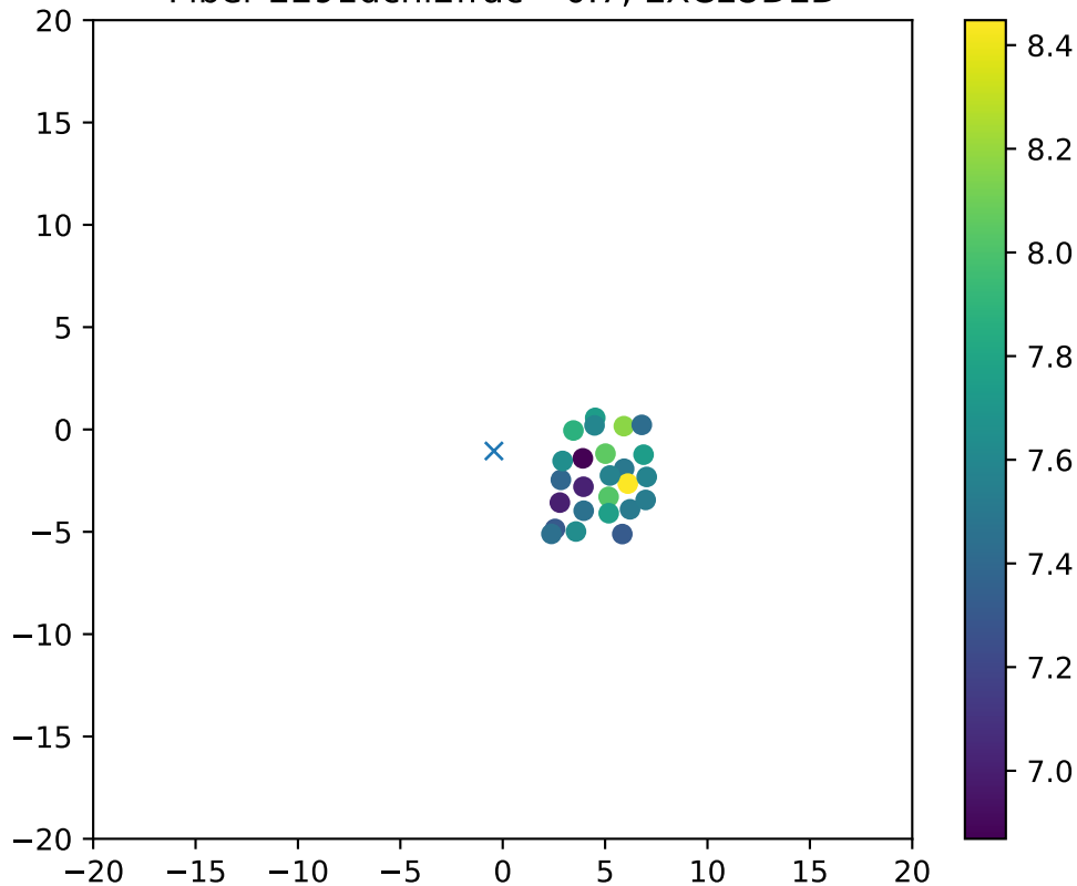
Fiber 2291dchi2frac= 0.7, EXCLUDED
