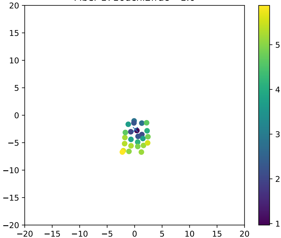
Fiber 1716dchi2frac= 1.0
