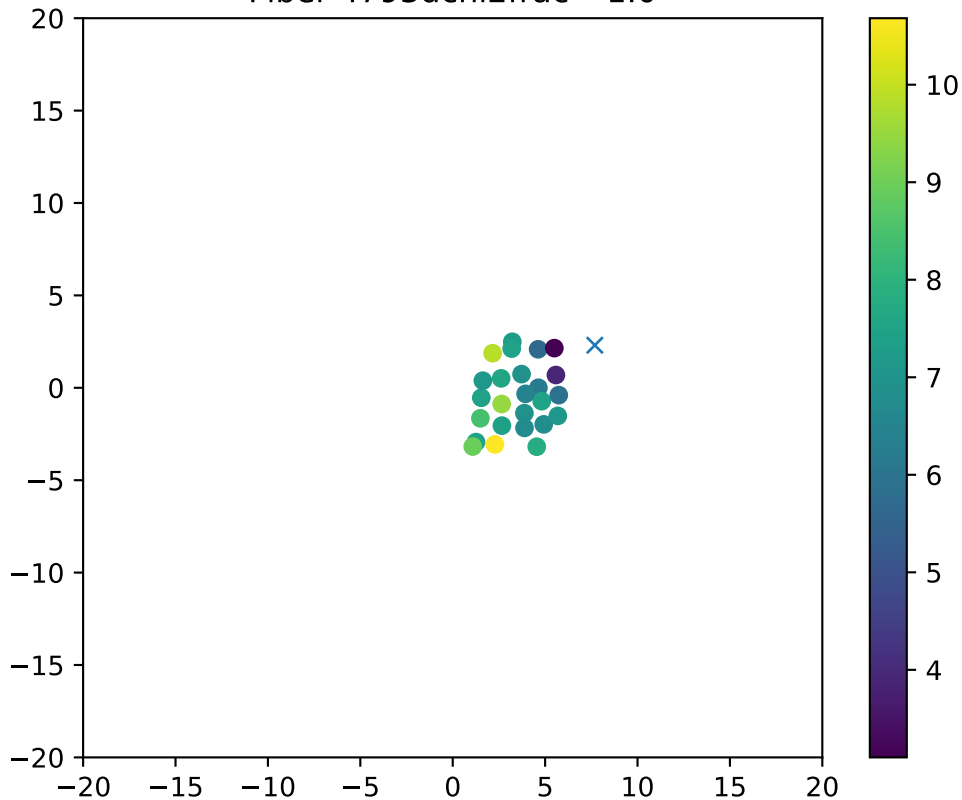
Fiber 4793dchi2frac= 1.0
