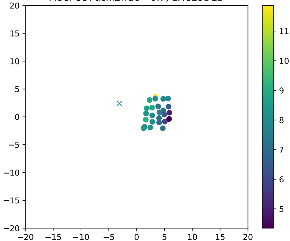
Fiber 337dchi2frac= 0.7, EXCLUDED
