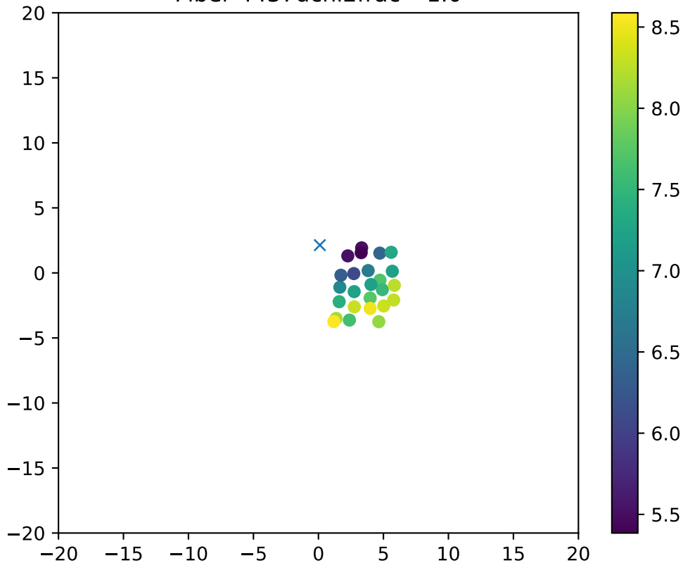
Fiber 4437dchi2frac= 1.0
