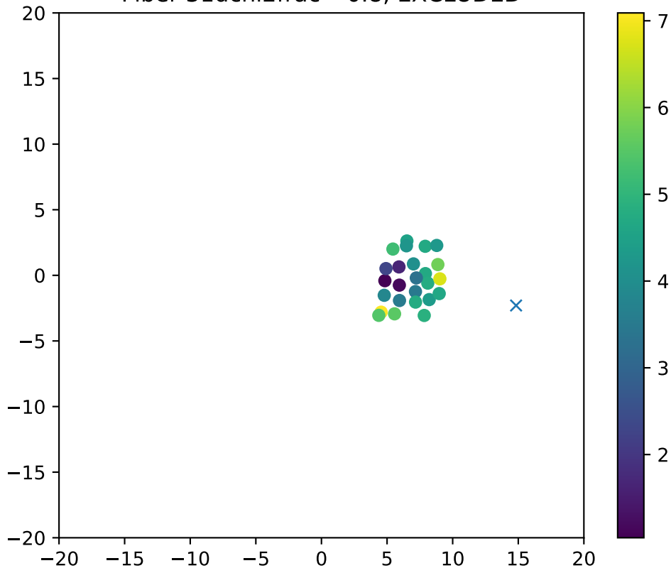
Fiber 31dchi2frac= 0.8, EXCLUDED
