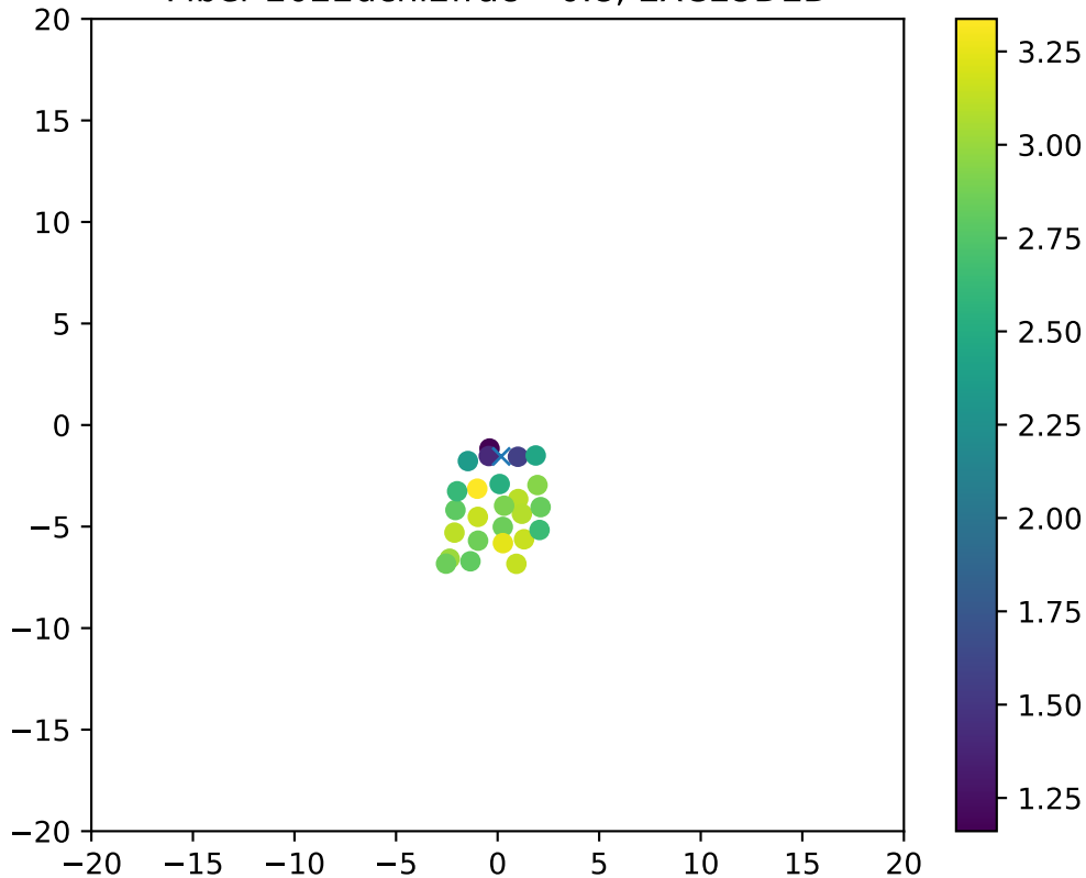
Fiber 2022dchi2frac= 0.8, EXCLUDED
