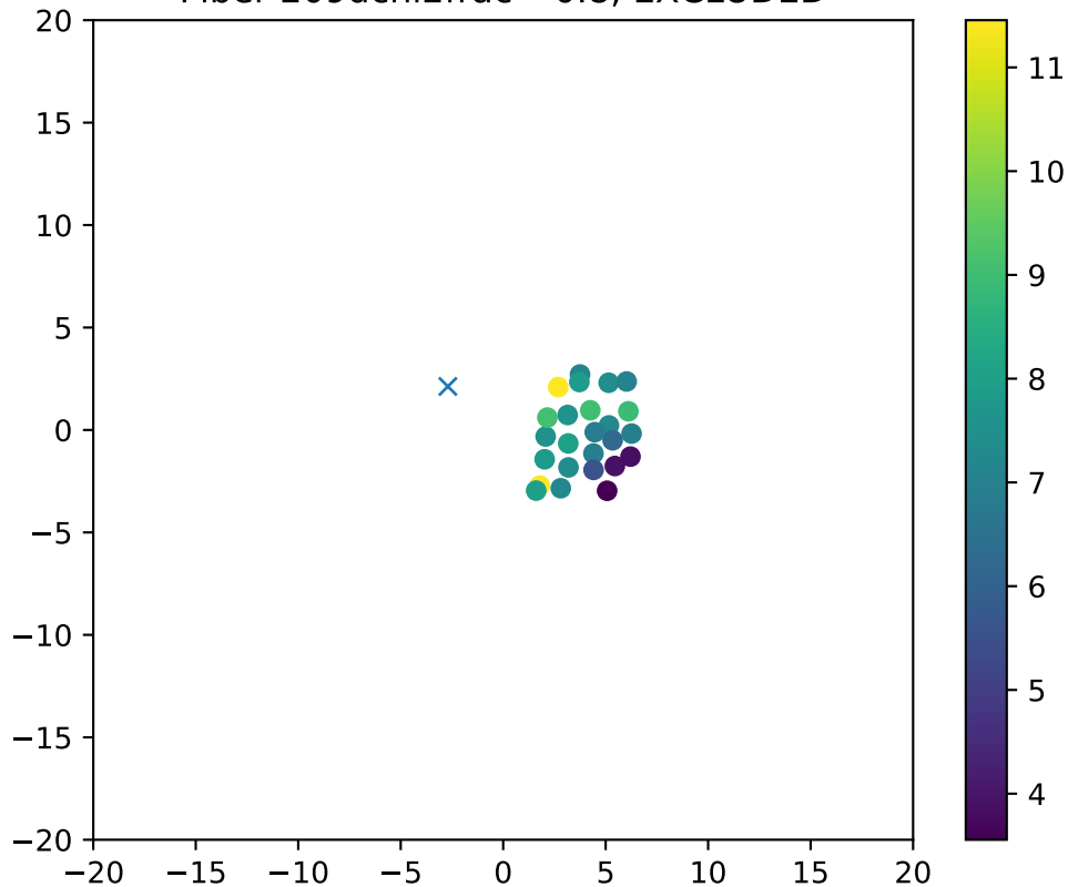
Fiber 209dchi2frac= 0.8, EXCLUDED
