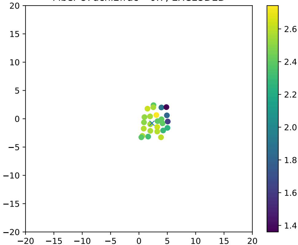
Fiber 87dchi2frac= 0.7, EXCLUDED
