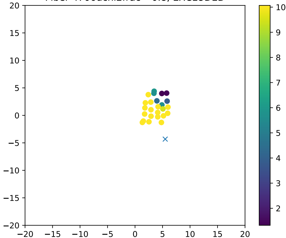
Fiber 4706dchi2frac= 0.8, EXCLUDED
