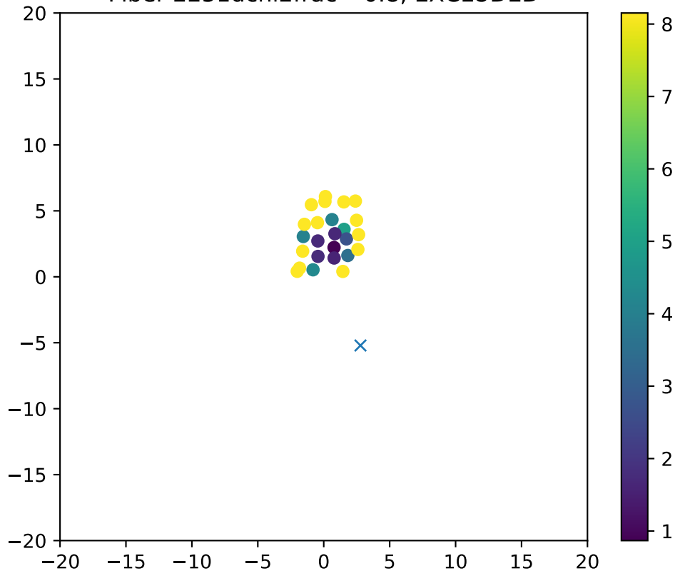
Fiber 2251dchi2frac= 0.8, EXCLUDED
