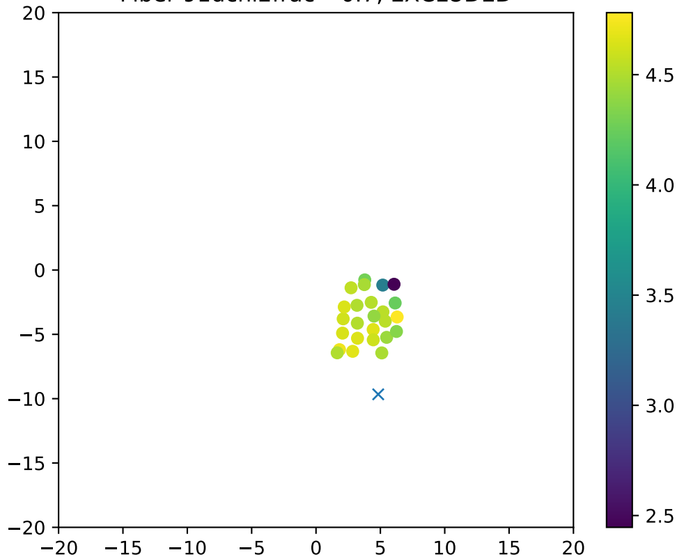
Fiber 91dchi2frac= 0.7, EXCLUDED
