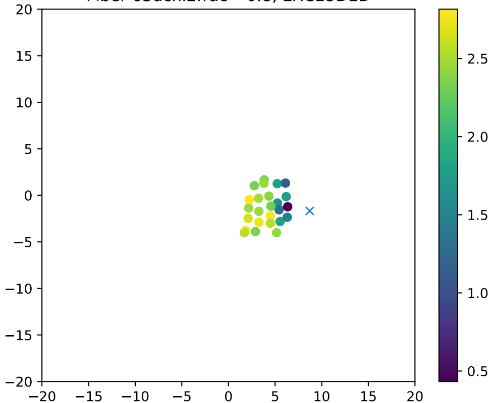
Fiber 63dchi2frac= 0.8, EXCLUDED
