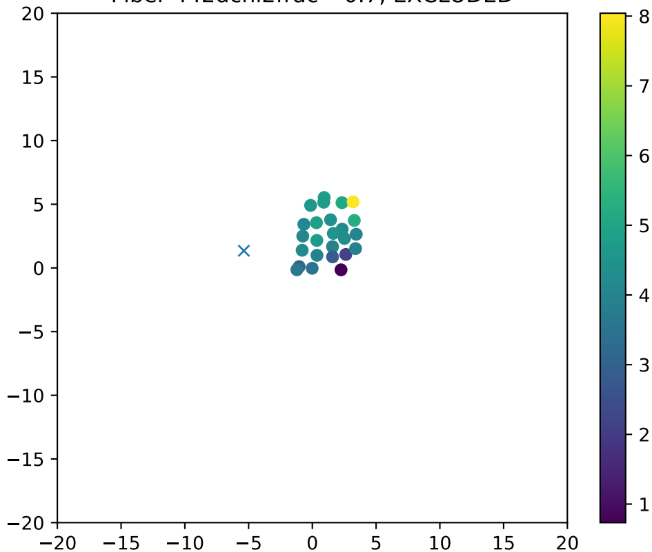
Fiber 442dchi2frac= 0.7, EXCLUDED
