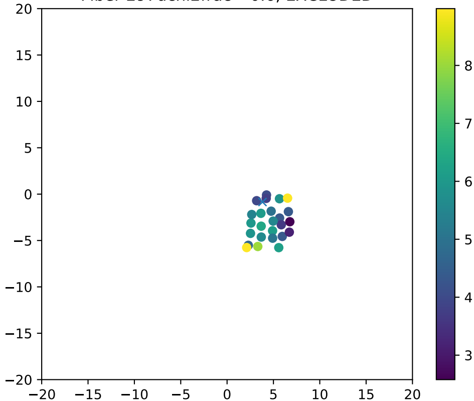
Fiber 297dchi2frac= 0.6, EXCLUDED
