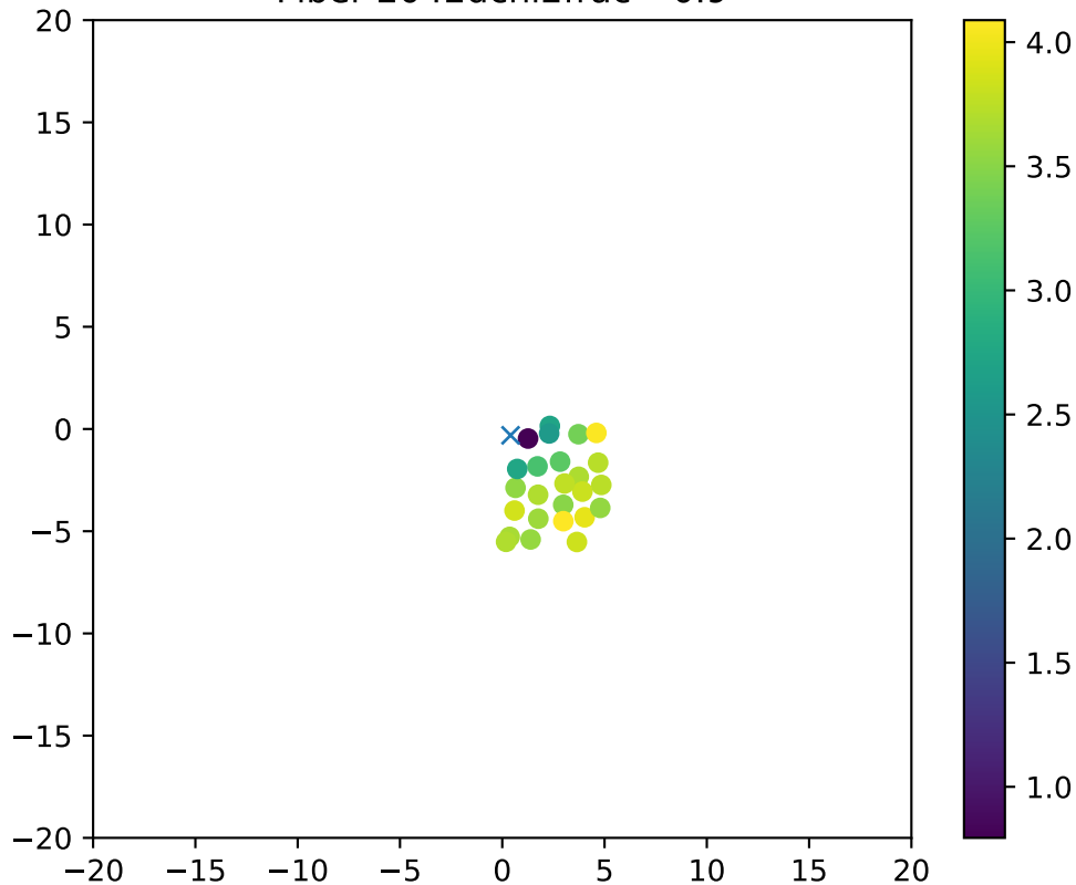
Fiber 2042dchi2frac= 0.9
