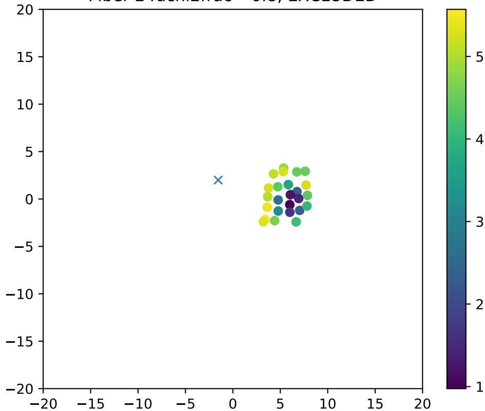
Fiber 24dchi2frac= 0.8, EXCLUDED
