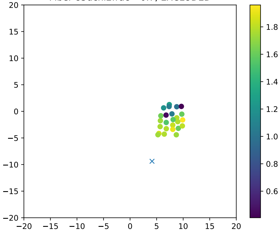
Fiber 85dchi2frac= 0.7, EXCLUDED
