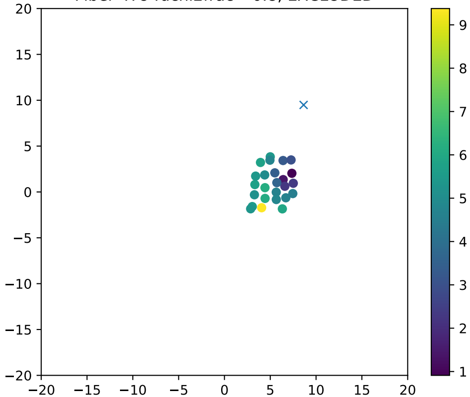
Fiber 4794dchi2frac= 0.8, EXCLUDED
