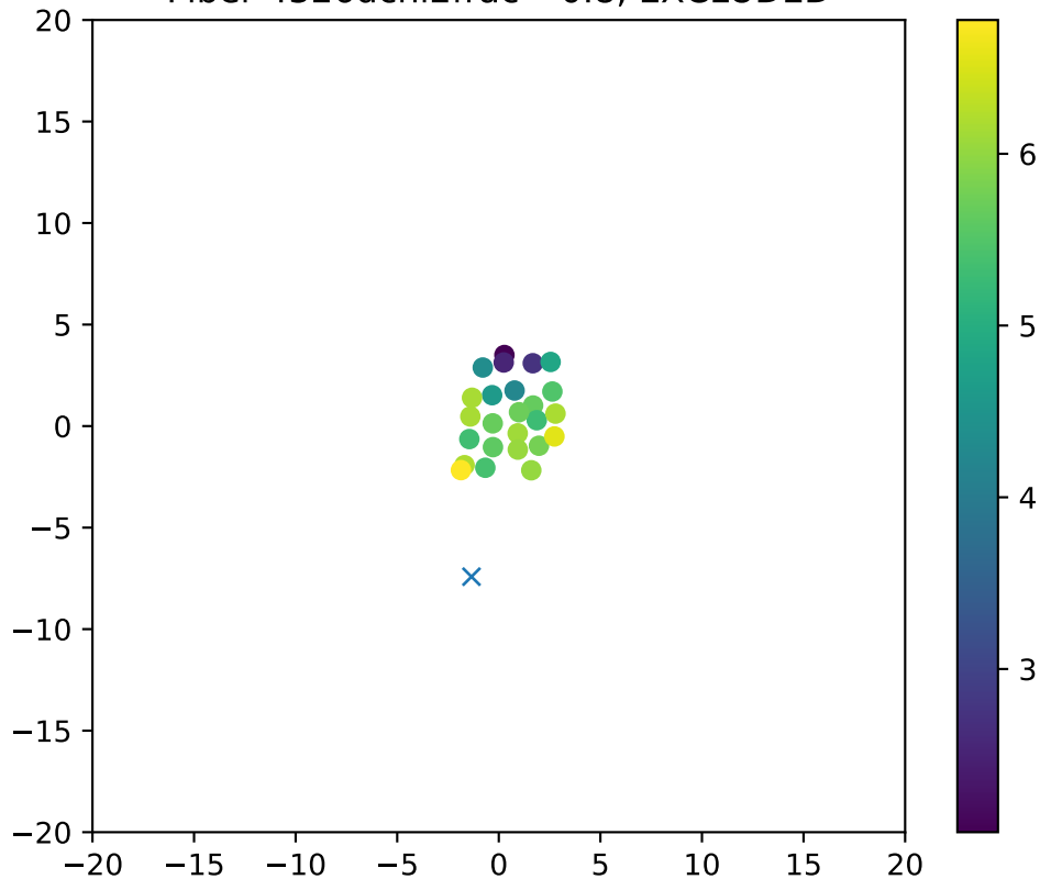
Fiber 4326dchi2frac= 0.8, EXCLUDED
