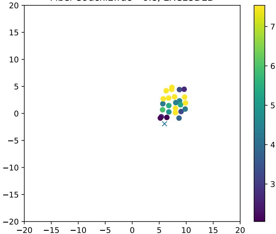
Fiber 39dchi2frac= 0.8, EXCLUDED
