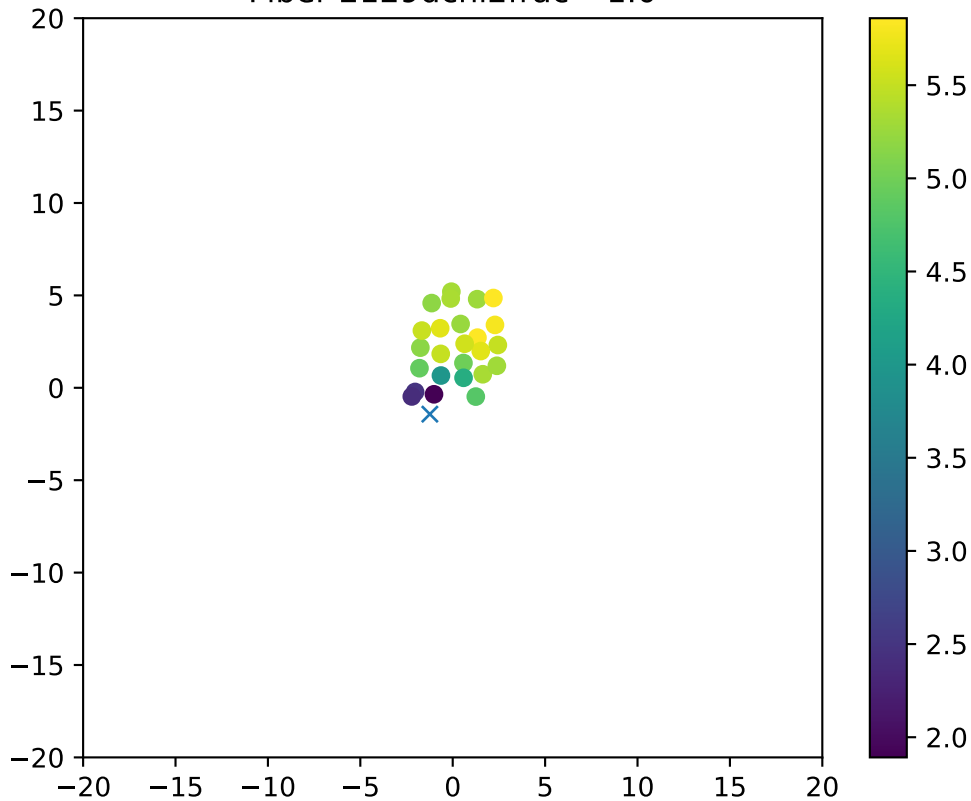
Fiber 2129dchi2frac= 1.0
