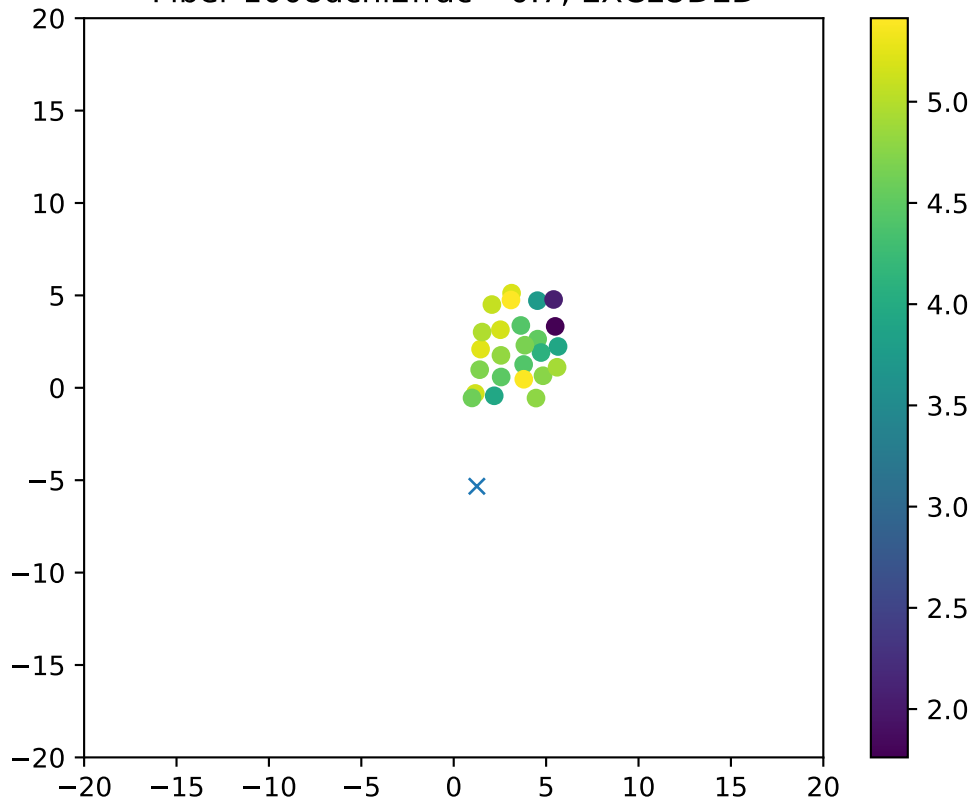
Fiber 1008dchi2frac= 0.7, EXCLUDED
