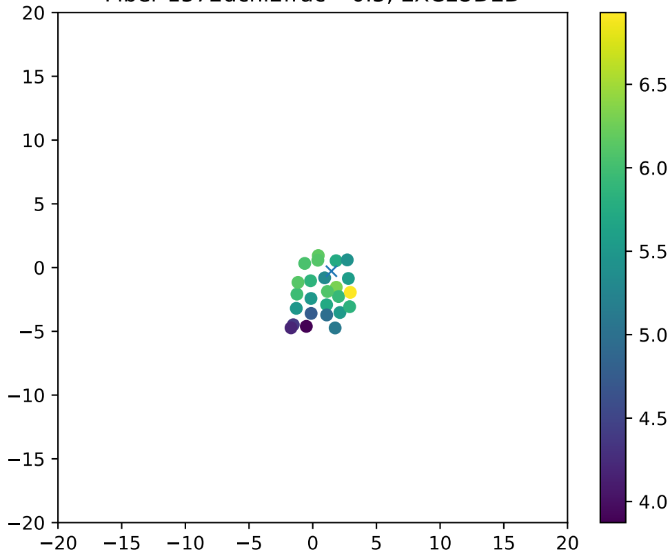
Fiber 1572dchi2frac= 0.5, EXCLUDED
