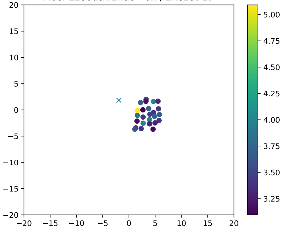
Fiber 2280dchi2frac= 0.7, EXCLUDED
