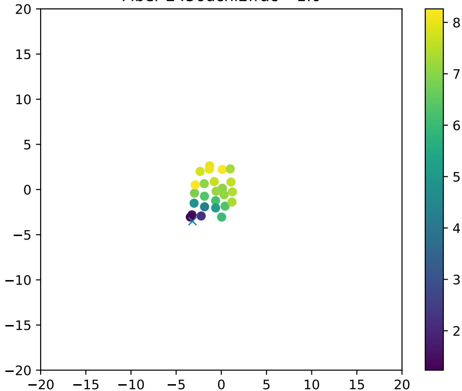
Fiber 2456dchi2frac= 1.0
