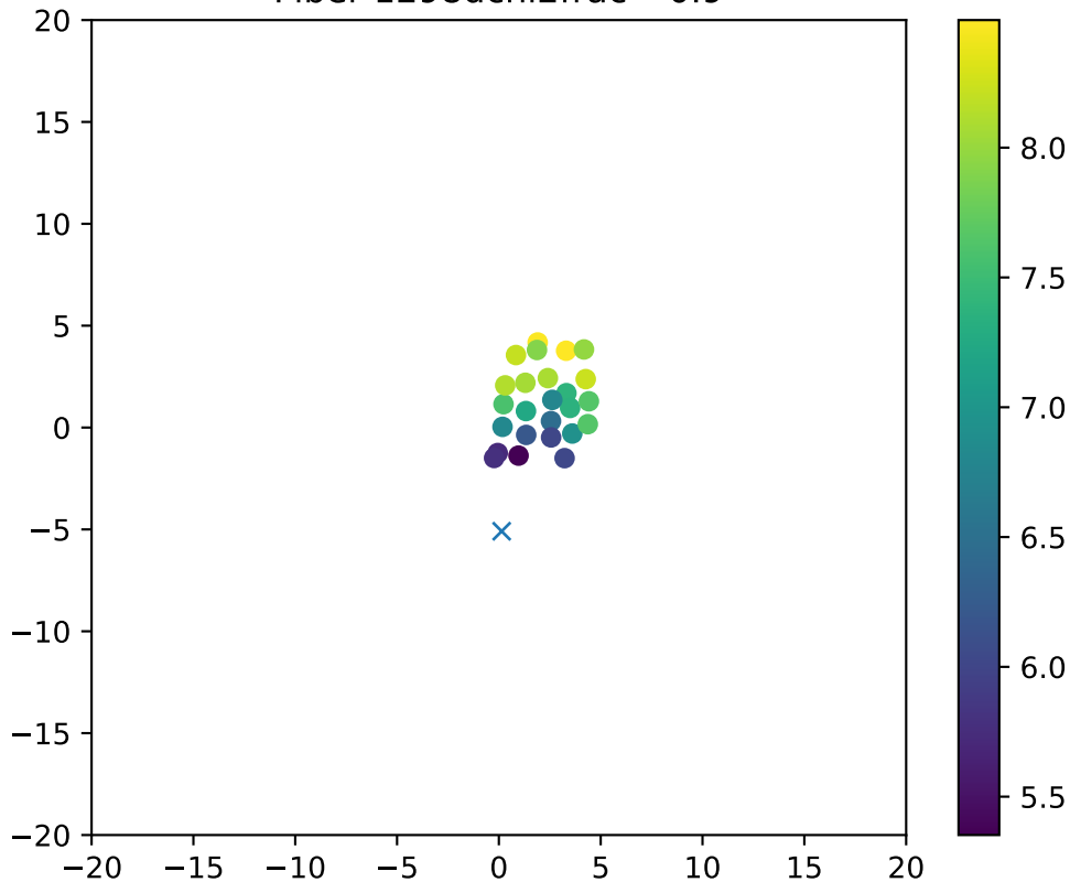
Fiber 1298dchi2frac= 0.9
