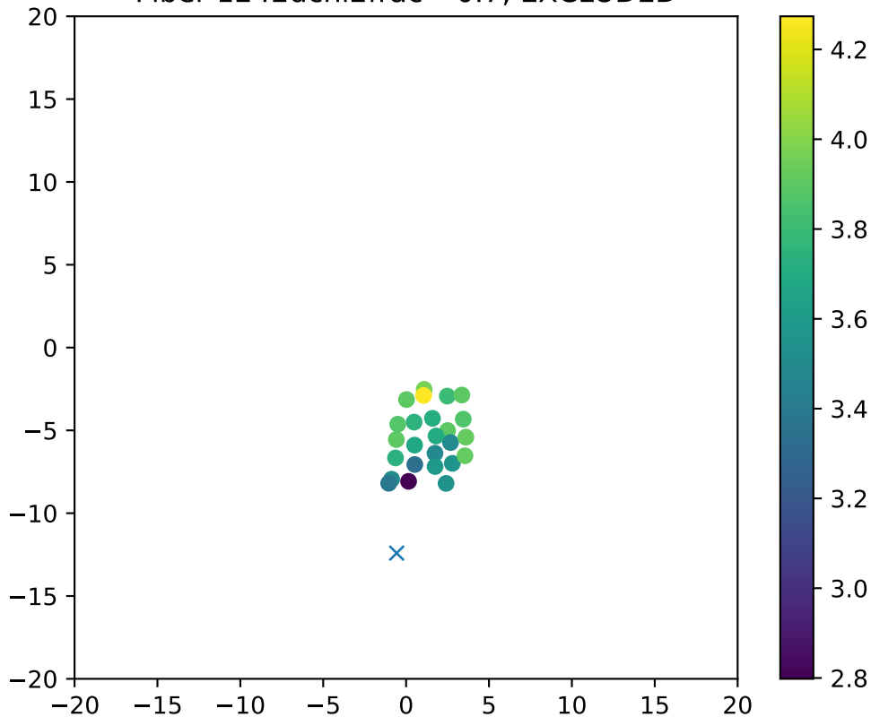
Fiber 1242dchi2frac= 0.7, EXCLUDED
