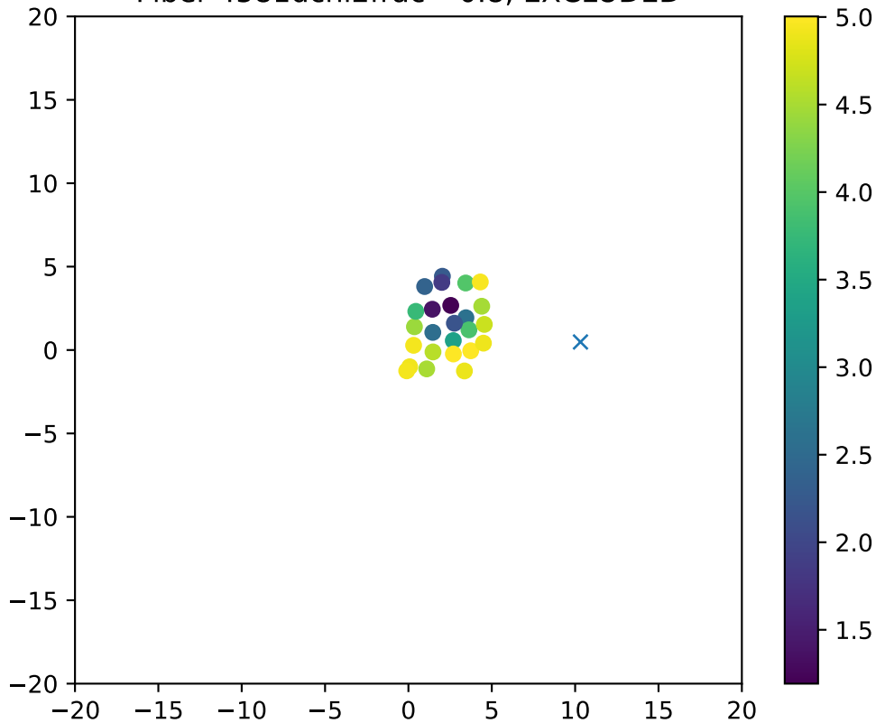
Fiber 4581dchi2frac= 0.8, EXCLUDED
