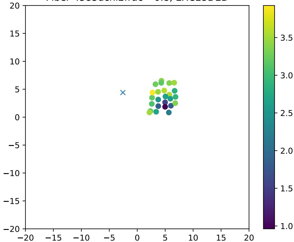
Fiber 4583dchi2frac= 0.8, EXCLUDED
