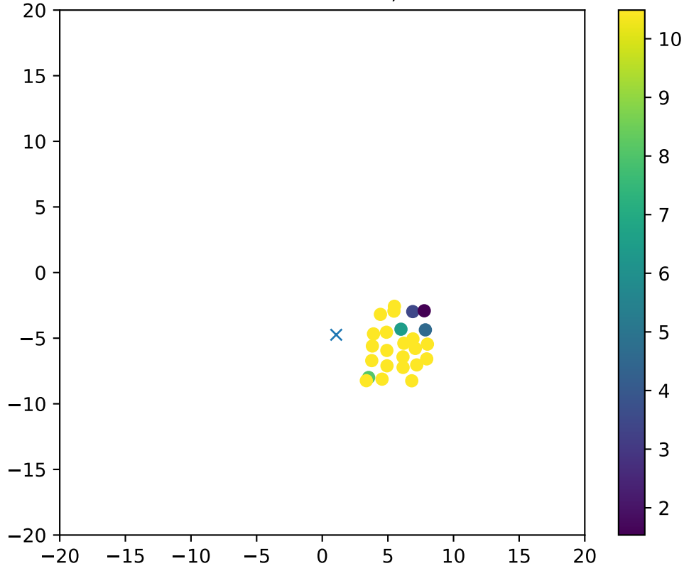
Fiber 496dchi2frac= 0.8, EXCLUDED
