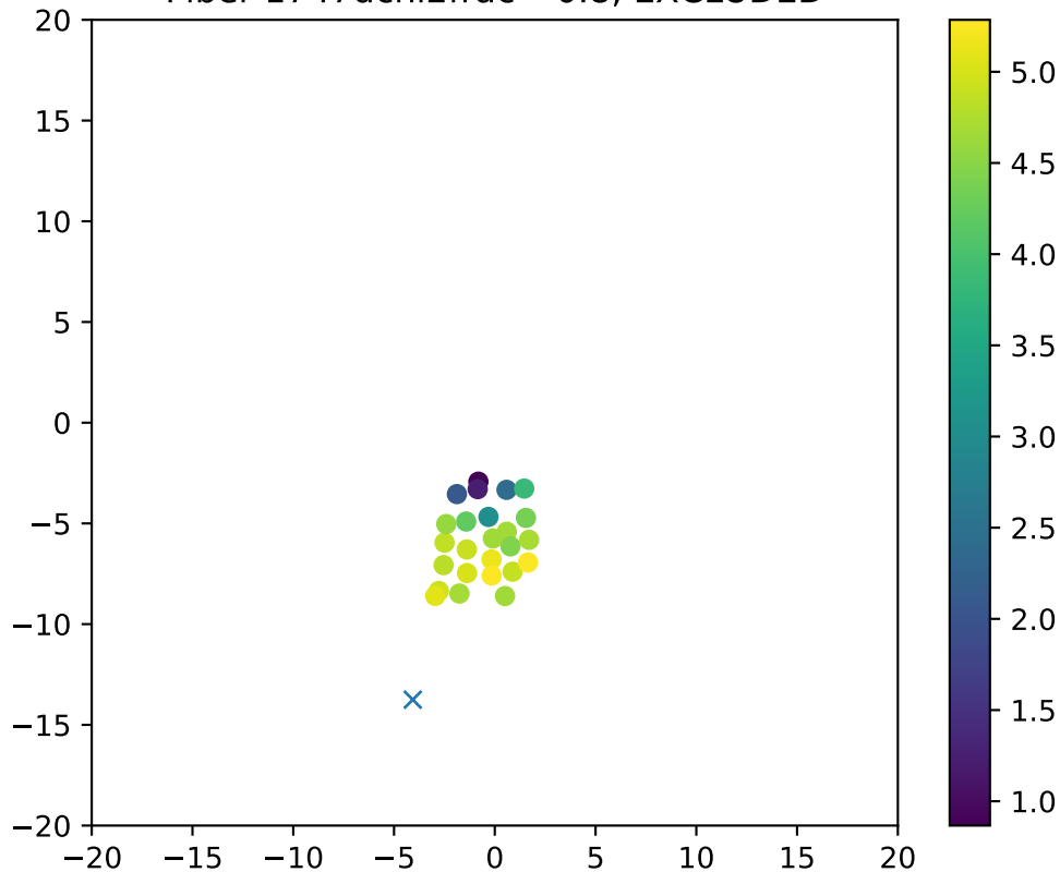
Fiber 1747dchi2frac= 0.8, EXCLUDED
