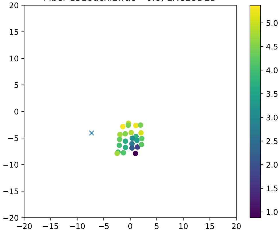
Fiber 1318dchi2frac= 0.8, EXCLUDED
