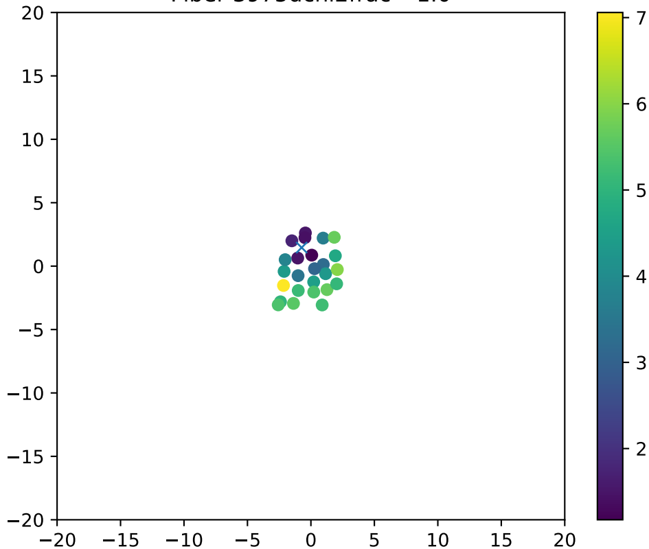
Fiber 3975dchi2frac= 1.0
