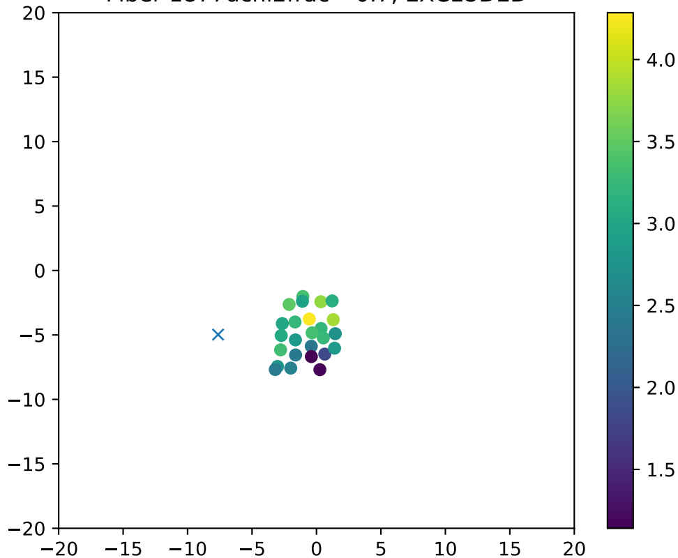
Fiber 1877dchi2frac= 0.7, EXCLUDED
