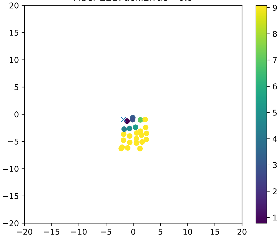
Fiber 2217dchi2frac= 0.9
