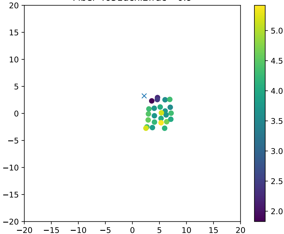
Fiber 4651dchi2frac= 0.9
