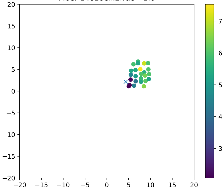
Fiber 1482dchi2frac= 1.0
