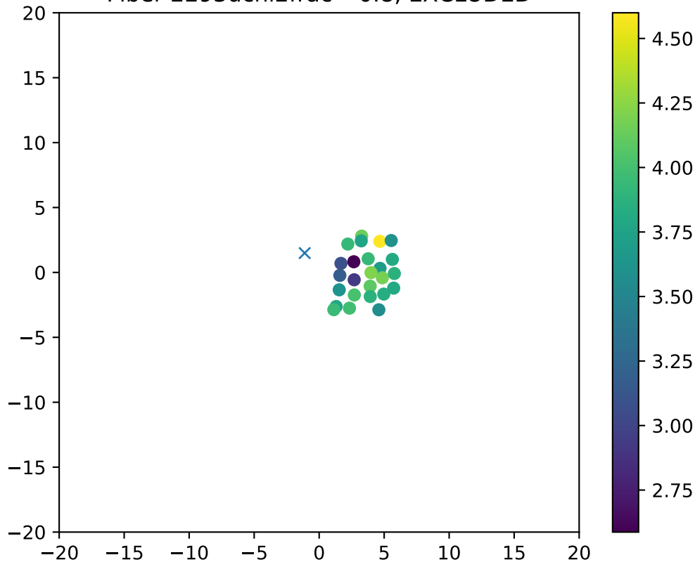
Fiber 2293dchi2frac= 0.8, EXCLUDED
