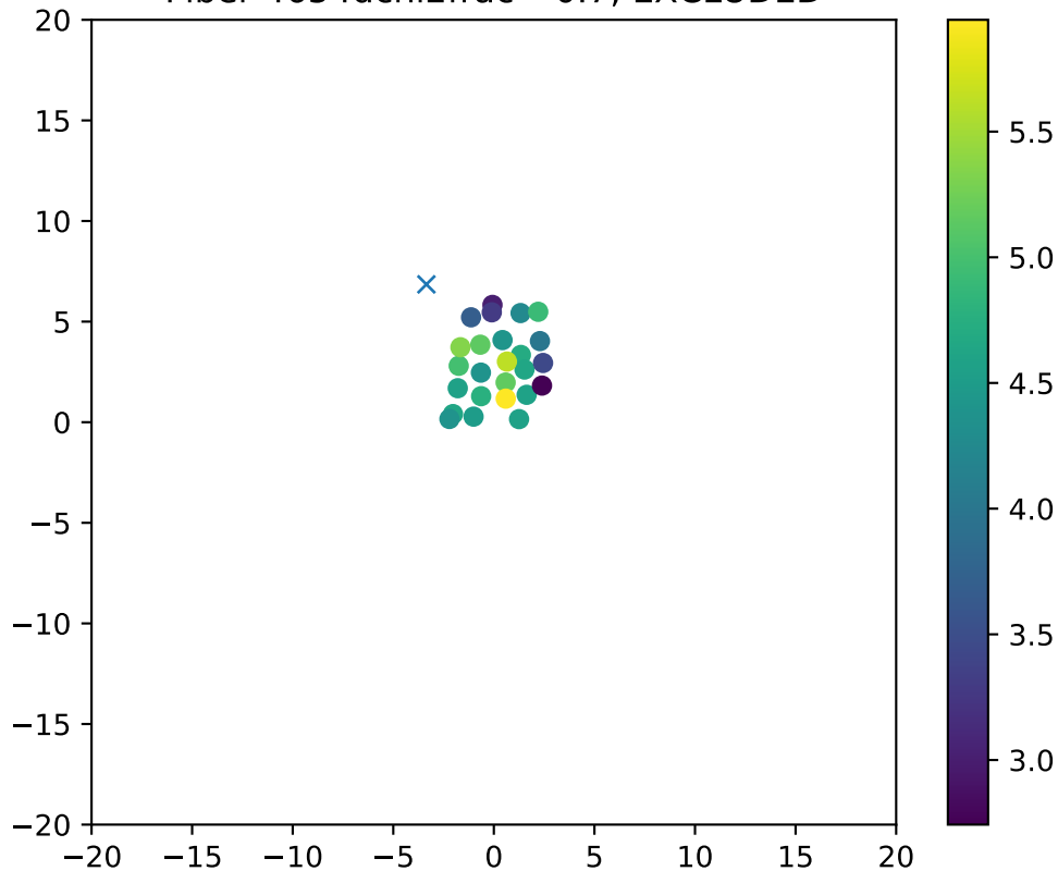
Fiber 4654dchi2frac= 0.7, EXCLUDED
