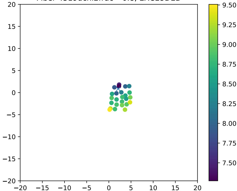
Fiber 4319dchi2frac= 0.8, EXCLUDED
