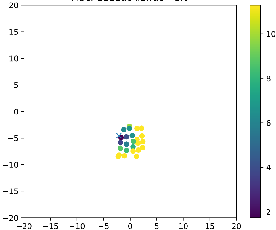
Fiber 2211dchi2frac= 1.0
