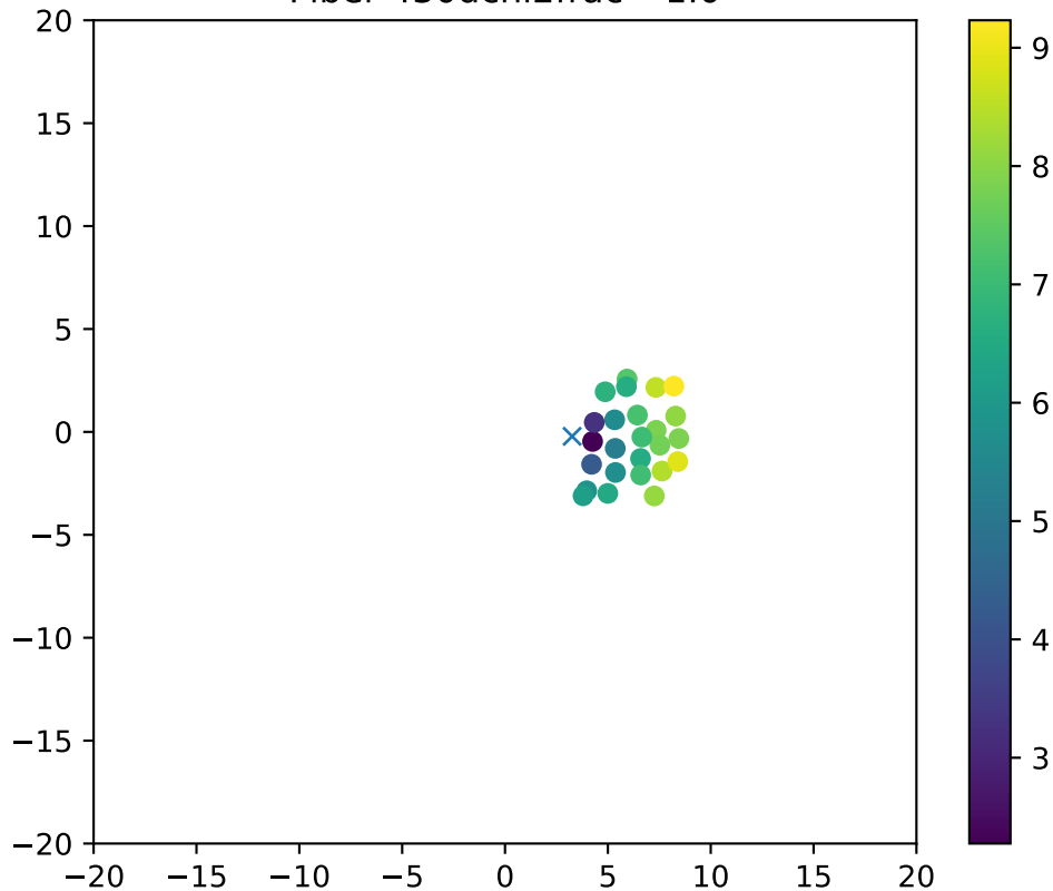
Fiber 430dchi2frac= 1.0
