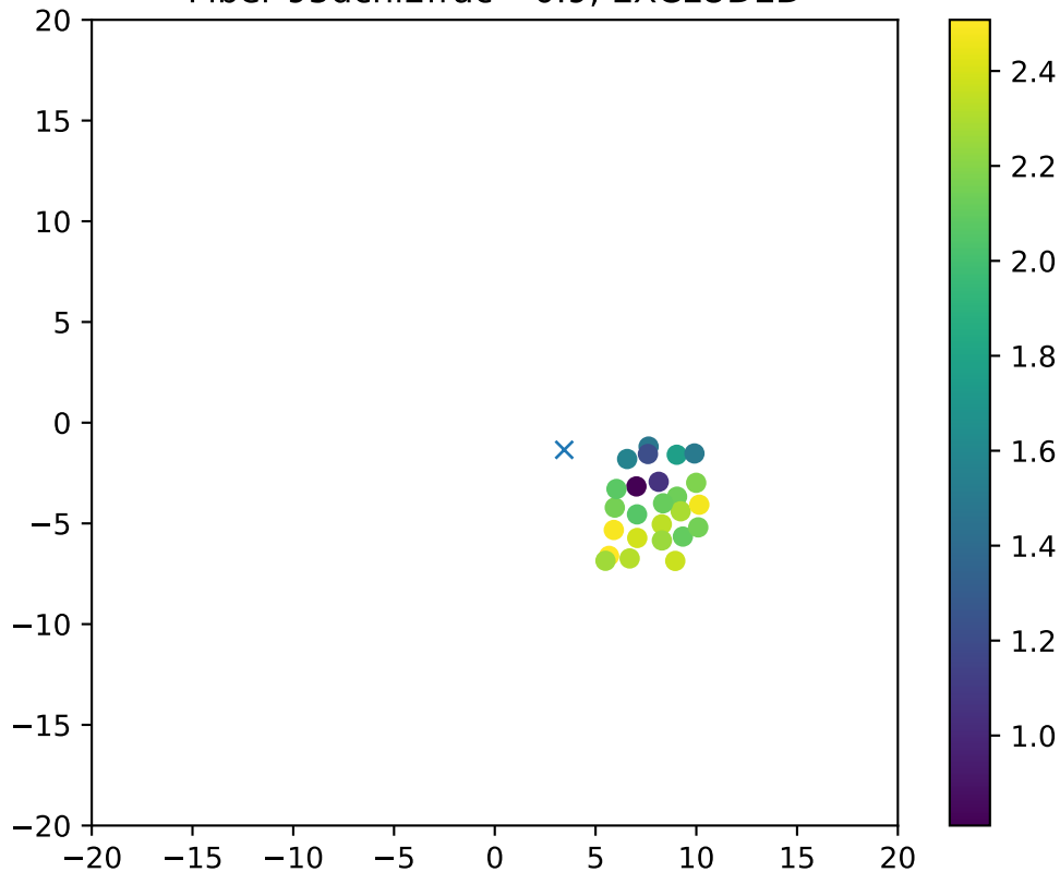
Fiber 95dchi2frac= 0.9, EXCLUDED
