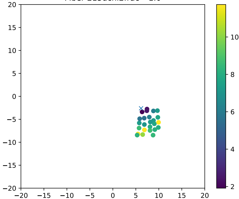
Fiber 213dchi2frac= 1.0
