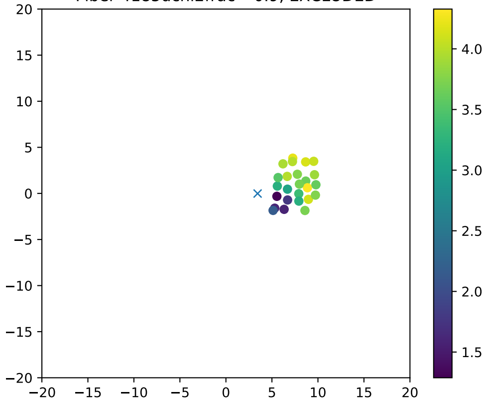
Fiber 4185dchi2frac= 0.9, EXCLUDED
