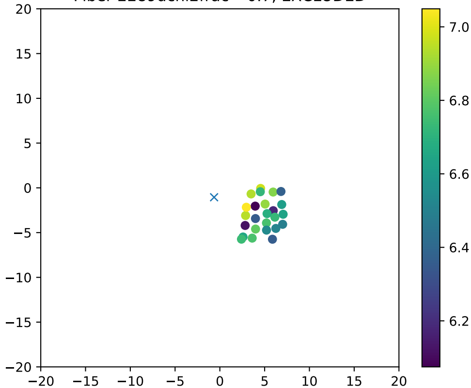
Fiber 2289dchi2frac= 0.7, EXCLUDED
