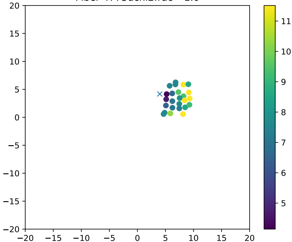
Fiber 4773dchi2frac= 1.0
