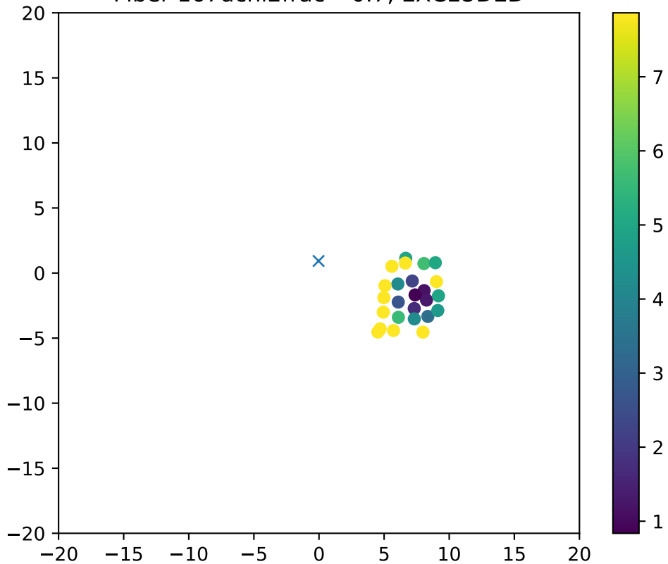
Fiber 167dchi2frac= 0.7, EXCLUDED
