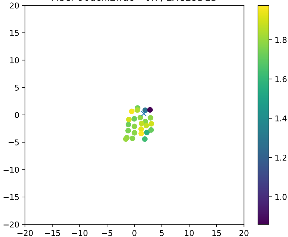
Fiber 90dchi2frac= 0.7, EXCLUDED
