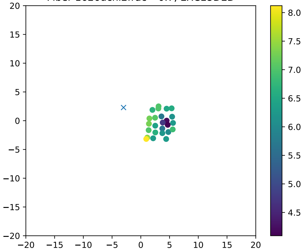
Fiber 1626dchi2frac= 0.7, EXCLUDED
