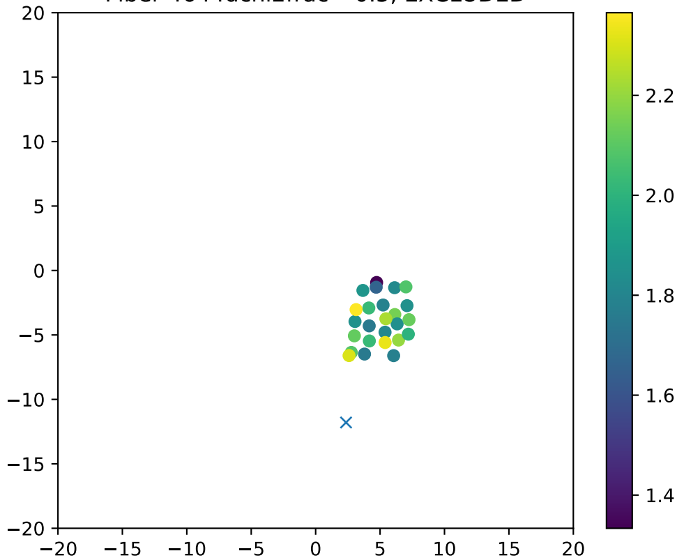
Fiber 4644dchi2frac= 0.5, EXCLUDED
