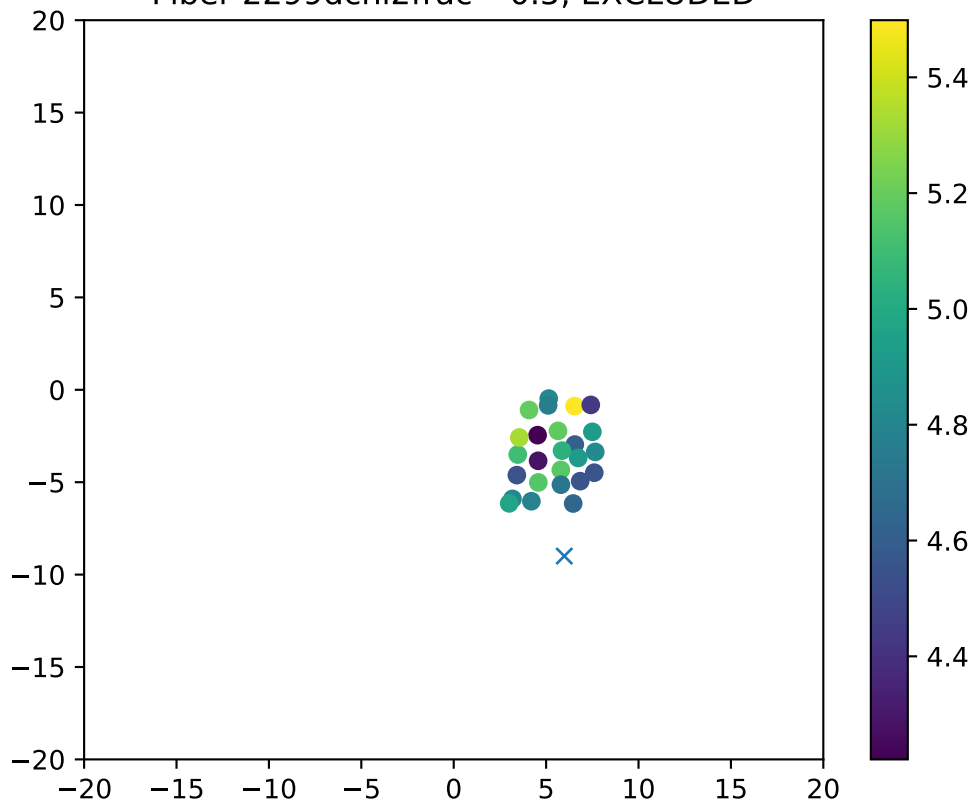
Fiber 2299dchi2frac= 0.5, EXCLUDED
