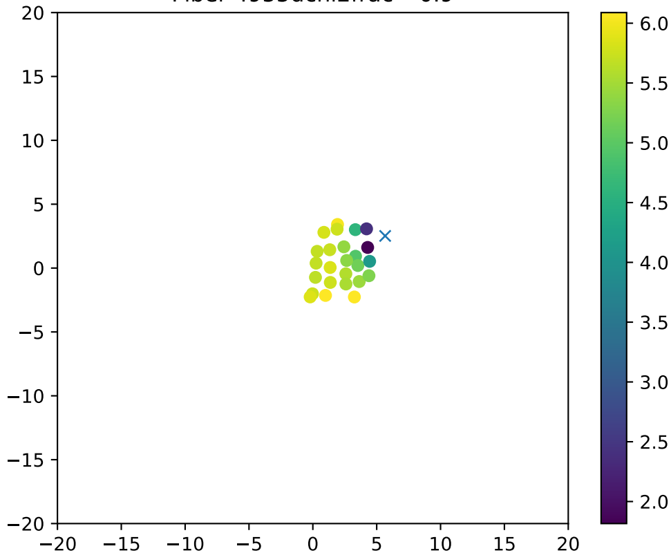
Fiber 4955dchi2frac= 0.9
