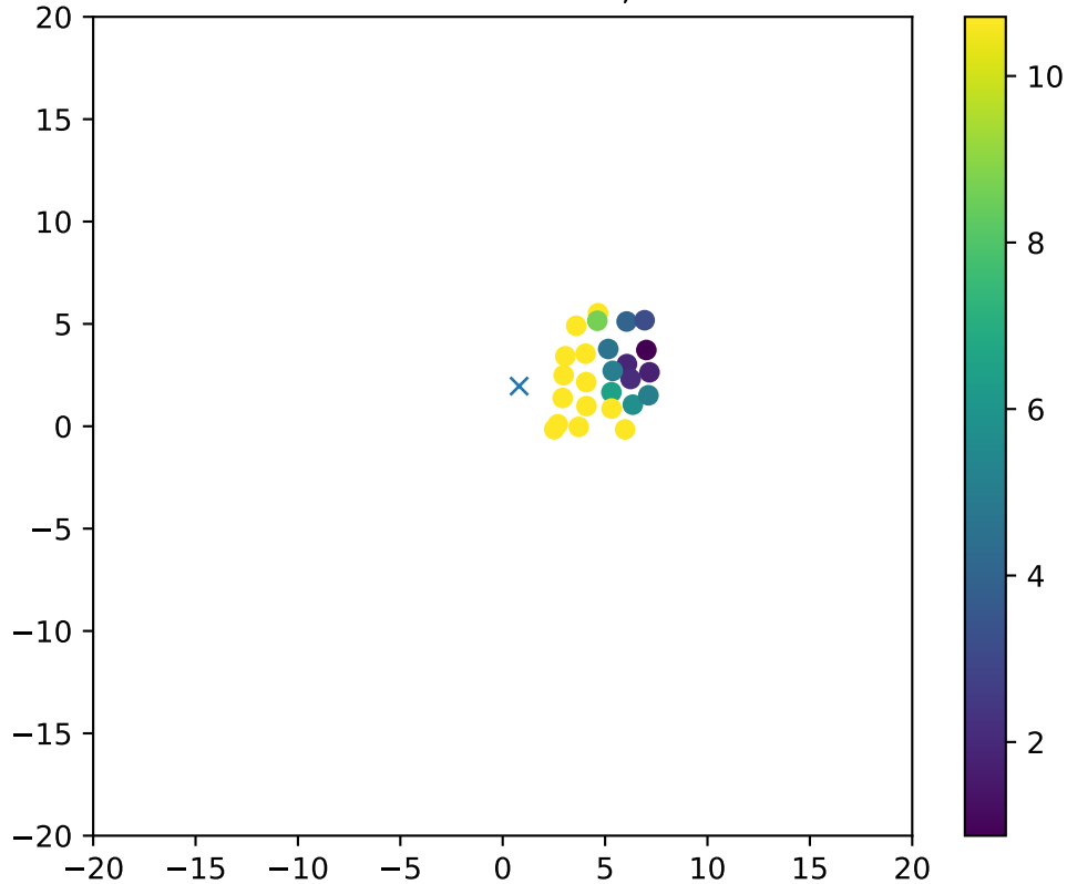
Fiber 4501dchi2frac= 0.8, EXCLUDED
