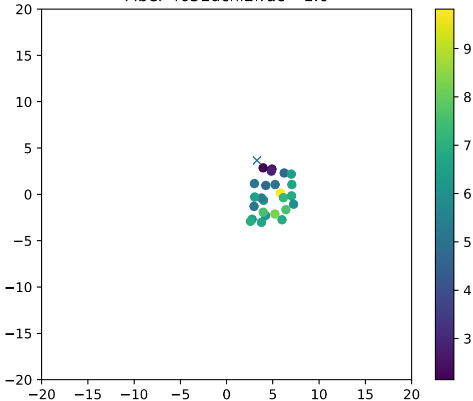
Fiber 4651dchi2frac= 1.0
