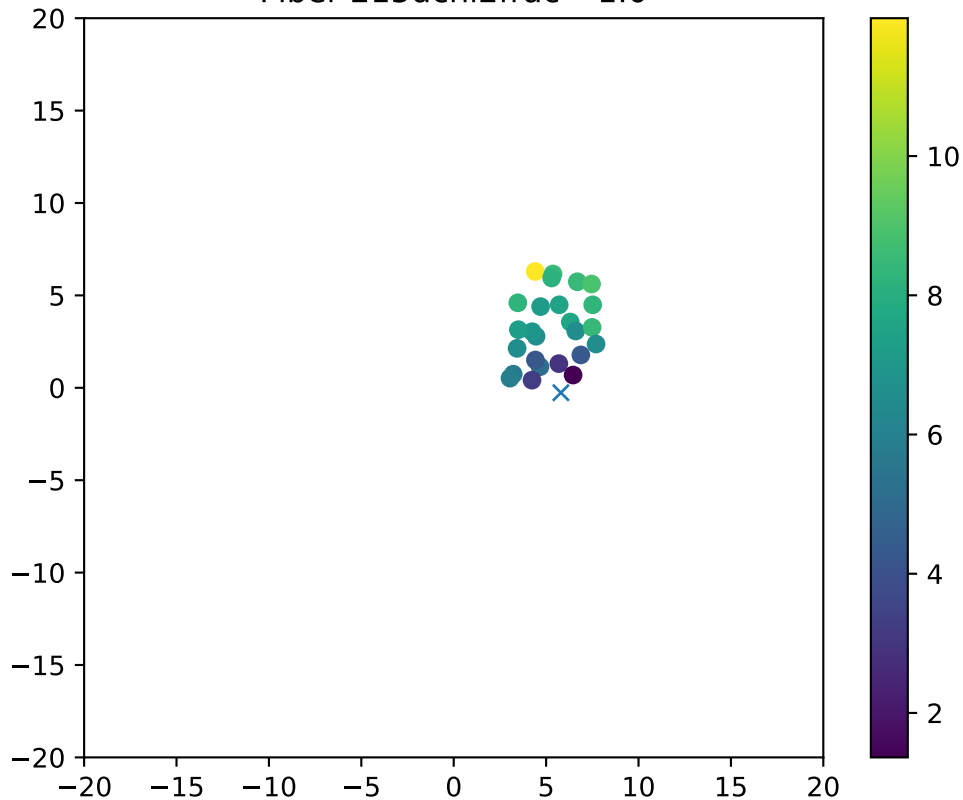
Fiber 215dchi2frac= 1.0
