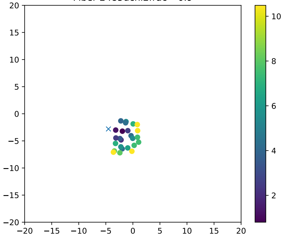
Fiber 2485dchi2frac= 0.9
