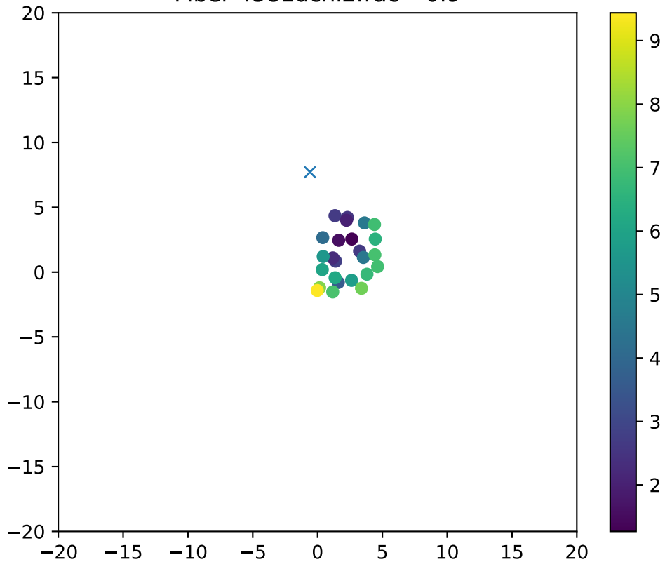
Fiber 4581dchi2frac= 0.9
