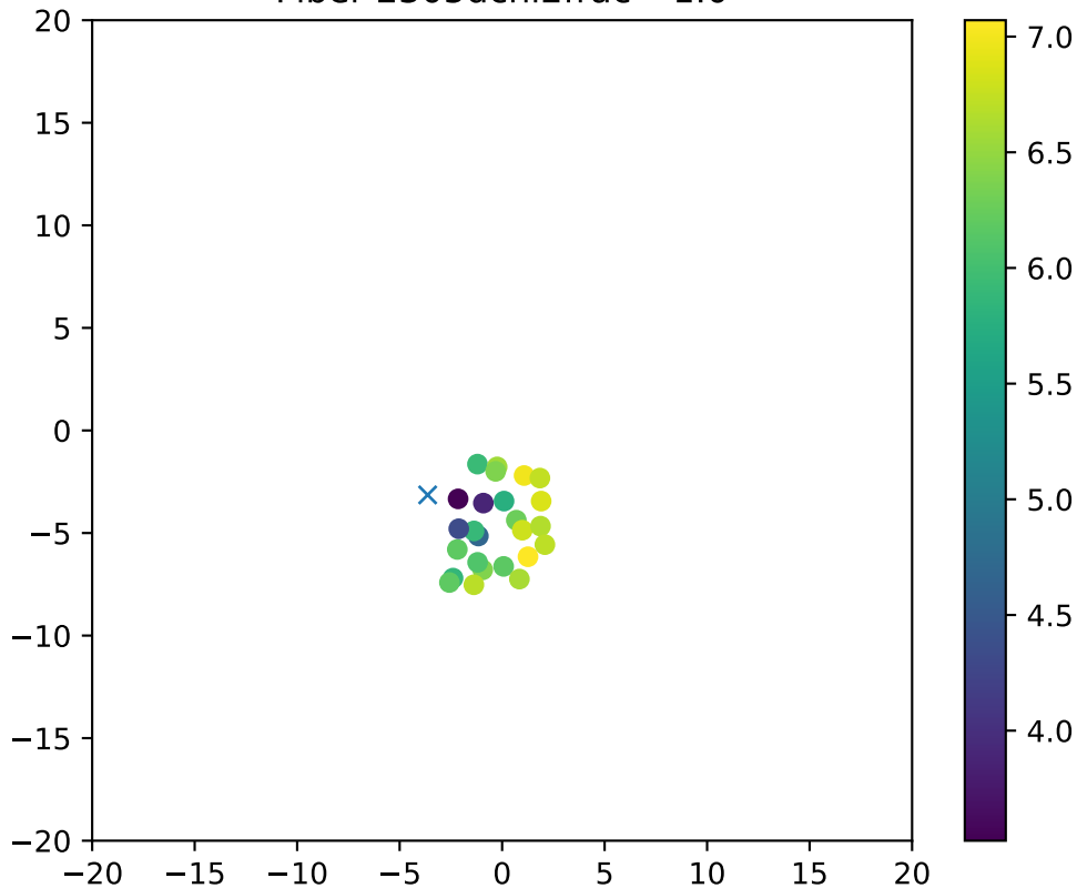
Fiber 2305dchi2frac= 1.0
