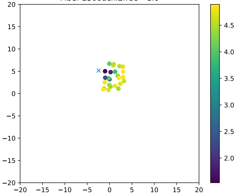
Fiber 2300dchi2frac= 1.0
