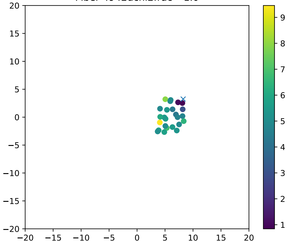
Fiber 4942dchi2frac= 1.0
