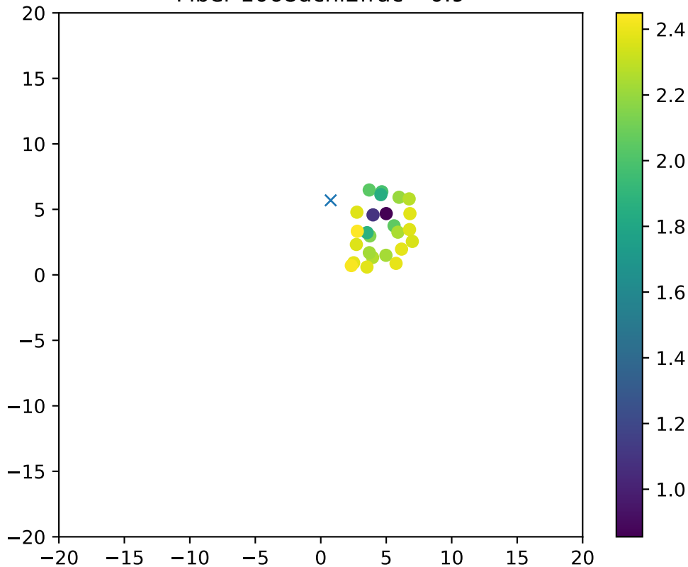
Fiber 1068dchi2frac= 0.9
