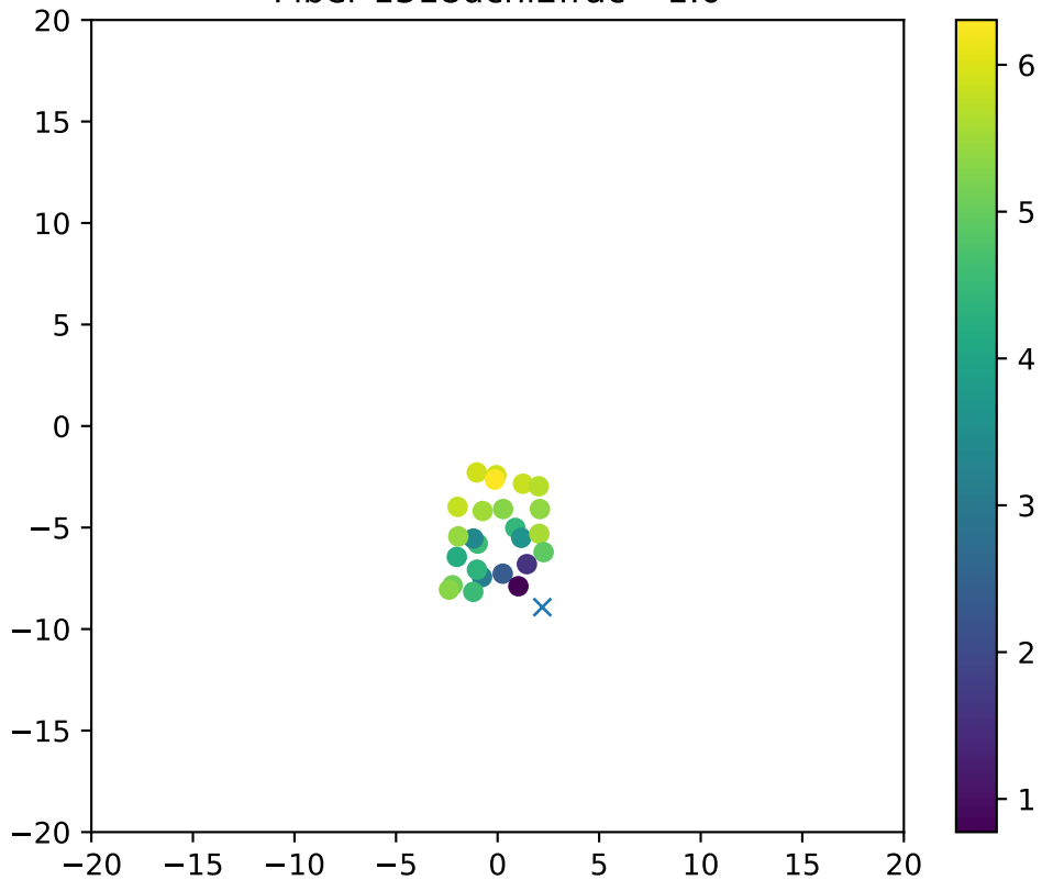
Fiber 1318dchi2frac= 1.0
