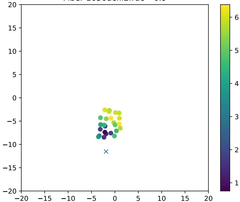
Fiber 1656dchi2frac= 0.9
