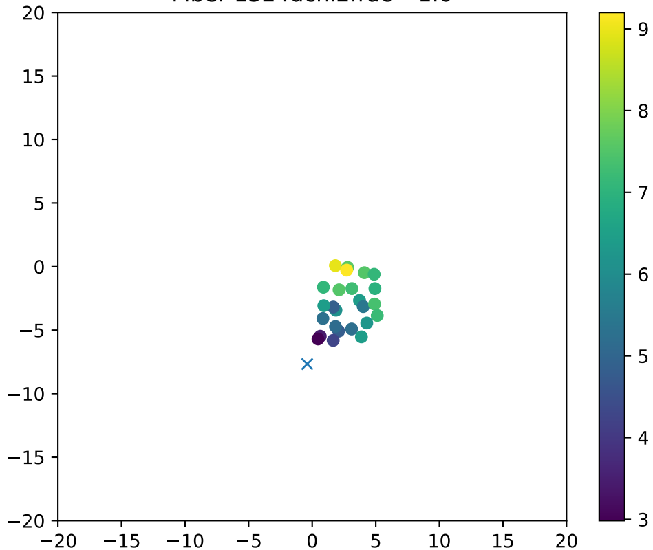
Fiber 1324dchi2frac= 1.0
