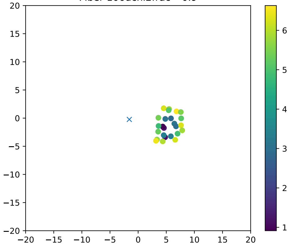
Fiber 106dchi2frac= 0.9
