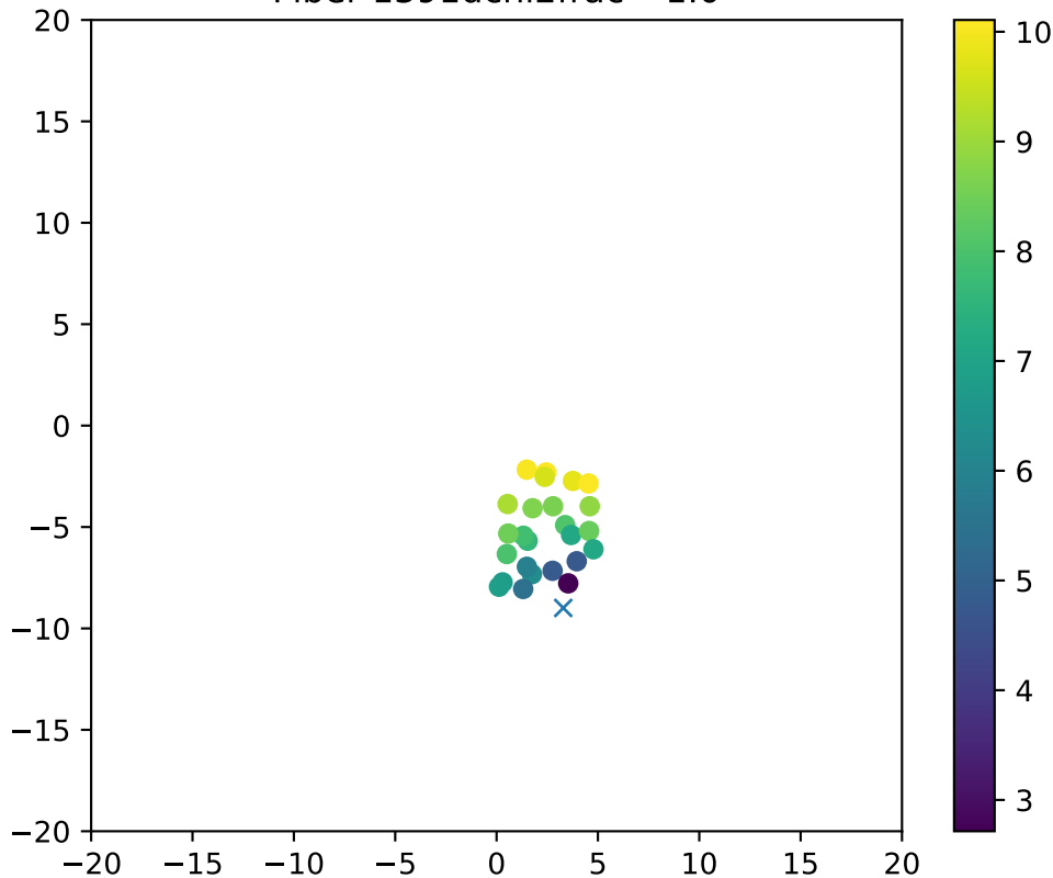
Fiber 1391dchi2frac= 1.0
