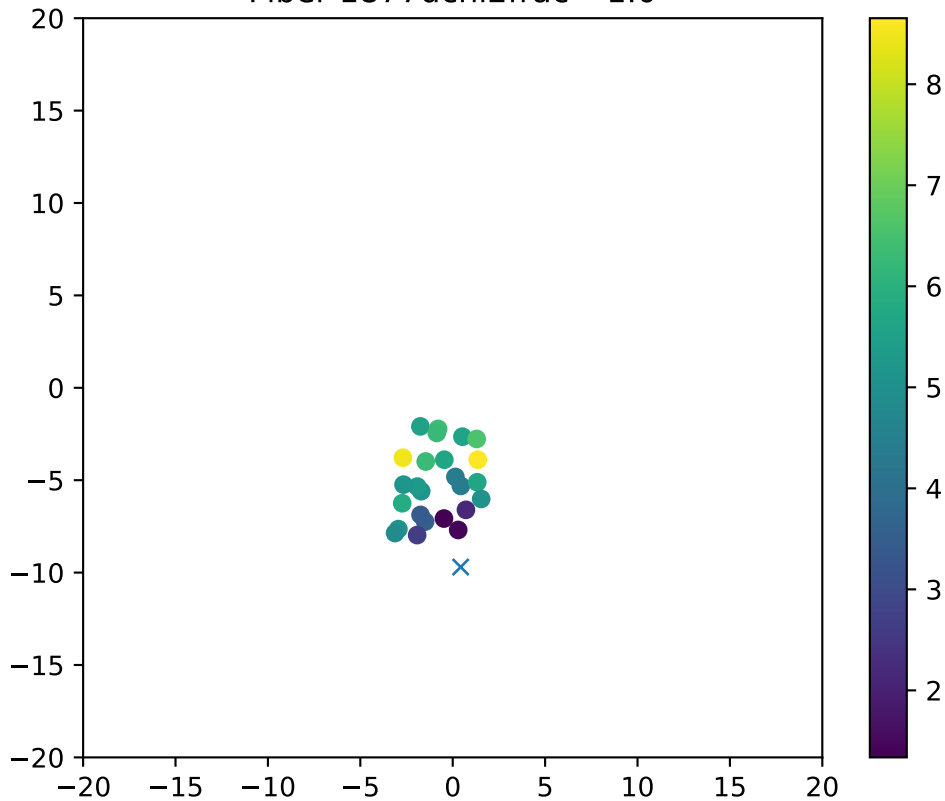
Fiber 1877dchi2frac= 1.0
