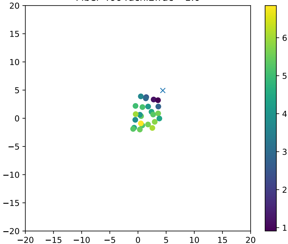
Fiber 4664dchi2frac= 1.0
