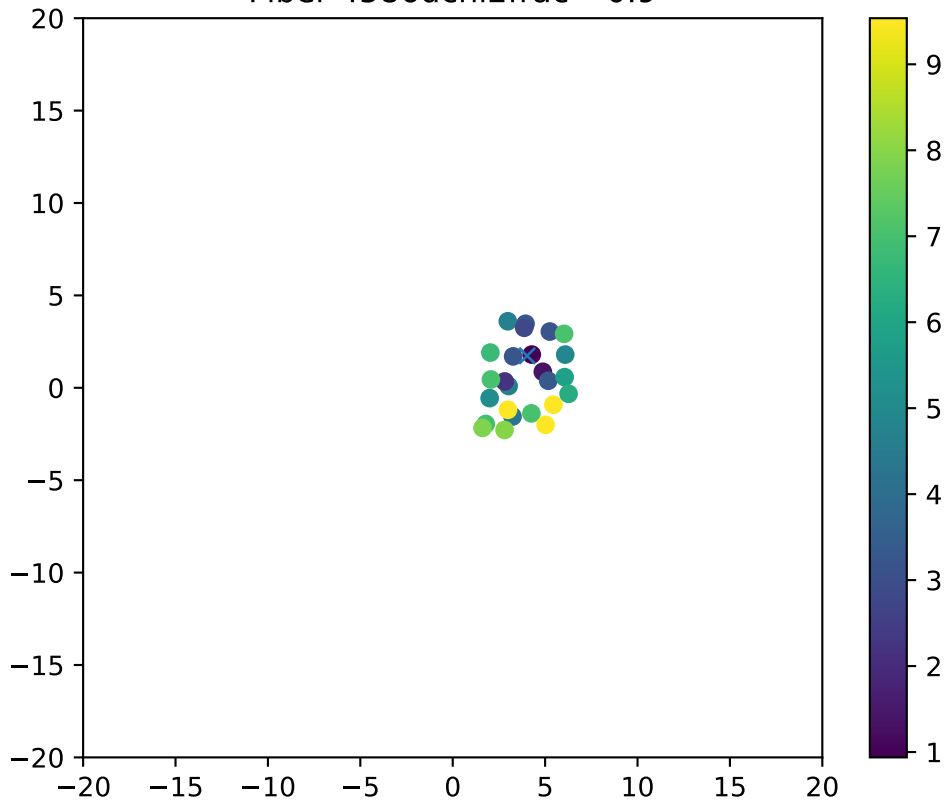
Fiber 4586dchi2frac= 0.9
