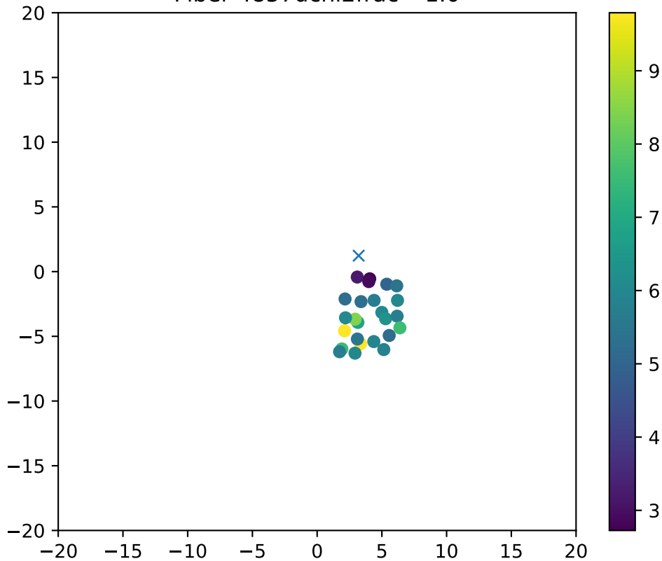
Fiber 4857dchi2frac= 1.0
