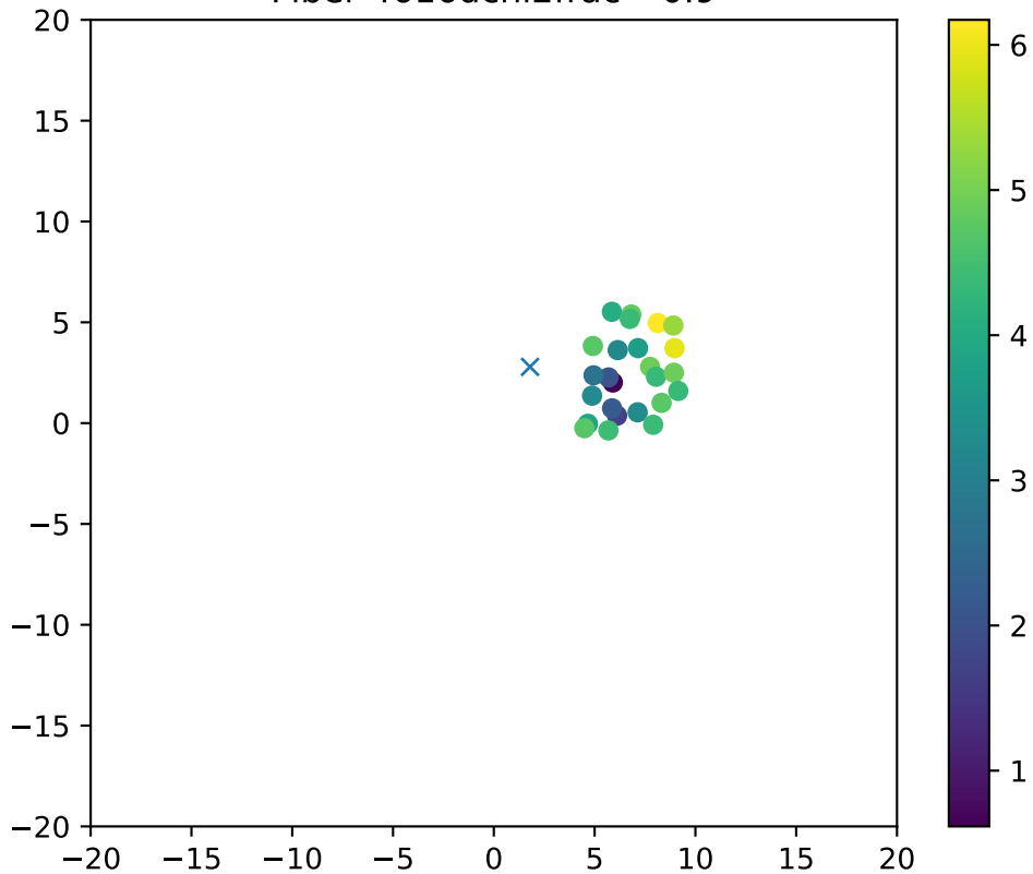
Fiber 4616dchi2frac= 0.9
