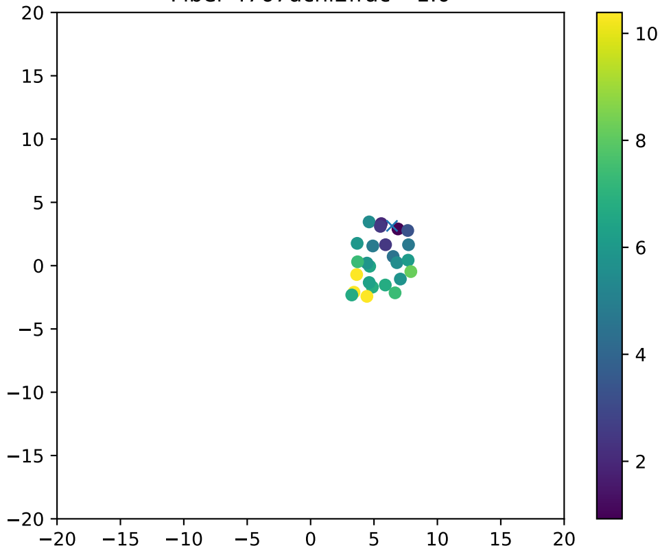
Fiber 4767dchi2frac= 1.0
