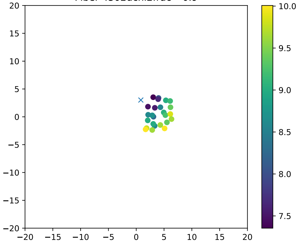
Fiber 4302dchi2frac= 0.9
