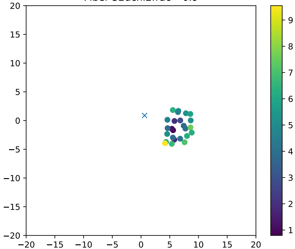
Fiber 32dchi2frac= 0.9
