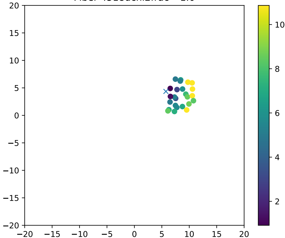
Fiber 4518dchi2frac= 1.0
