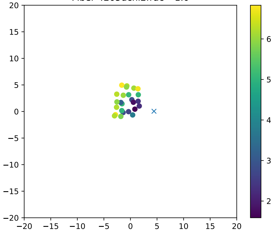
Fiber 4205dchi2frac= 1.0
