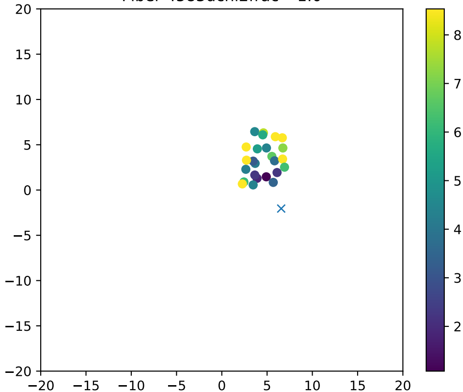
Fiber 4583dchi2frac= 1.0
