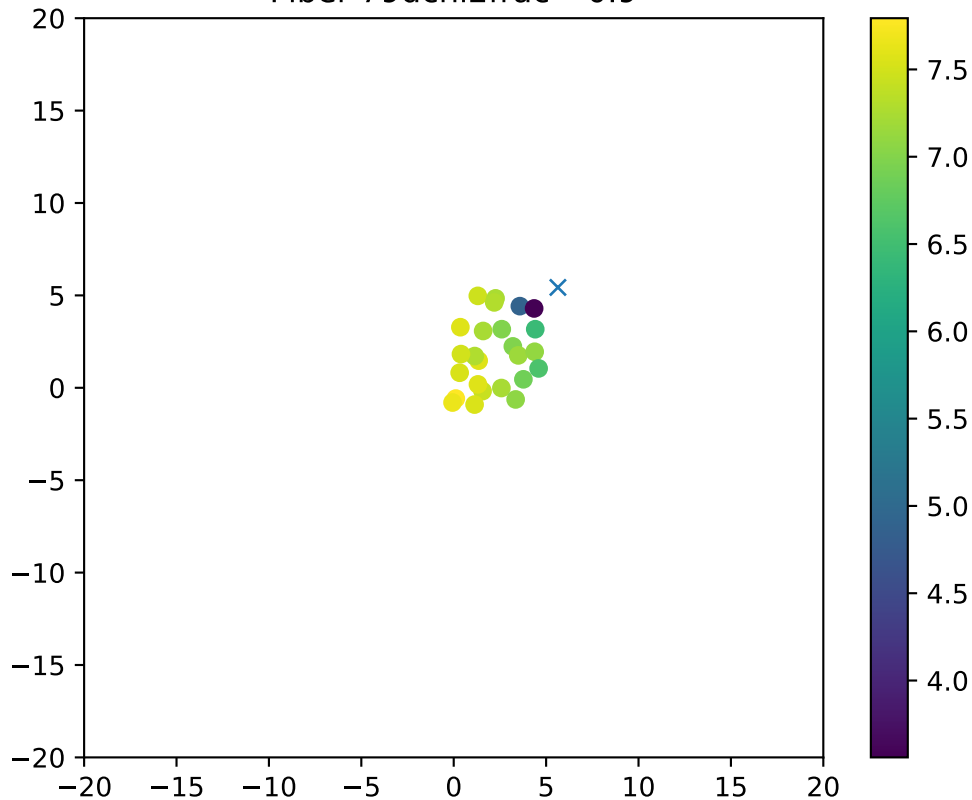
Fiber 79dchi2frac= 0.9
