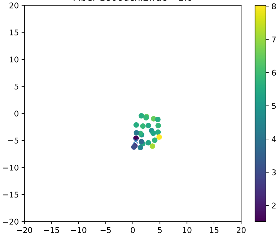
Fiber 1806dchi2frac= 1.0
