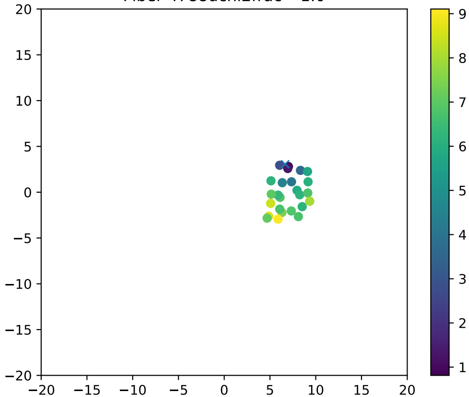
Fiber 4788dchi2frac= 1.0
