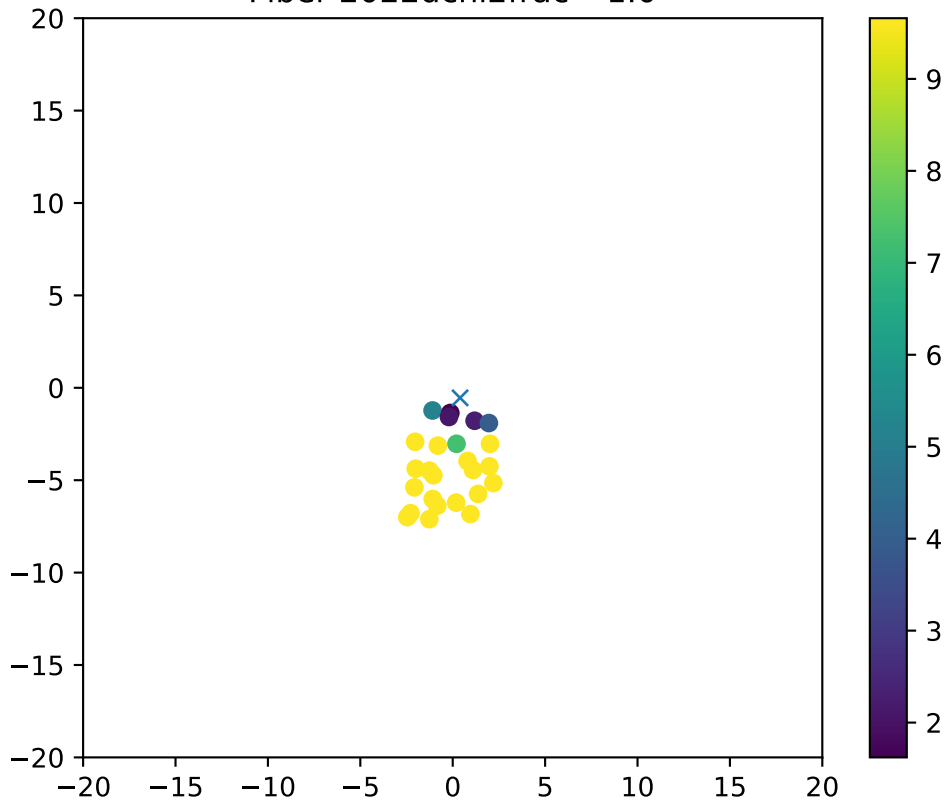
Fiber 2022dchi2frac= 1.0
