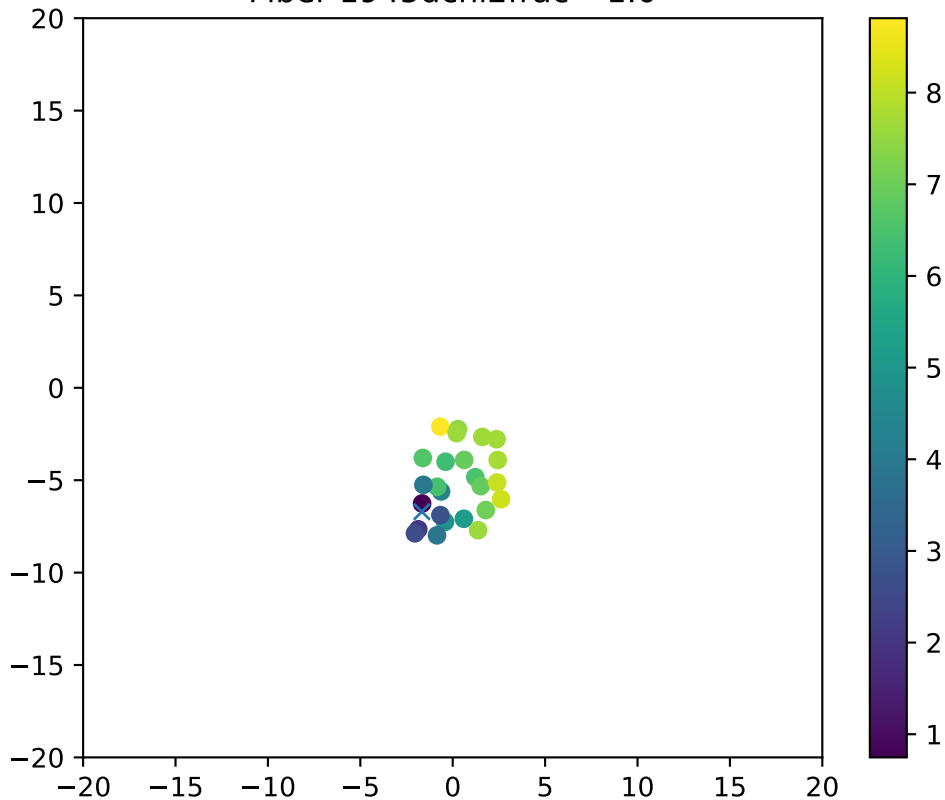
Fiber 1945dchi2frac= 1.0
