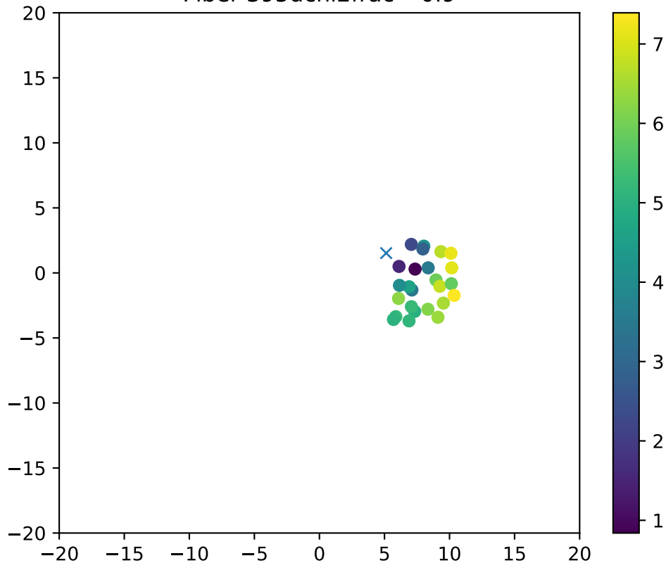
Fiber 395dchi2frac= 0.9
