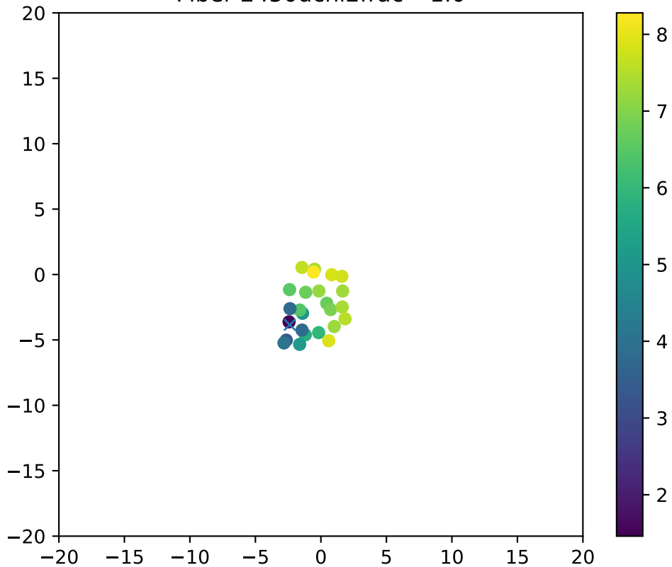
Fiber 2450dchi2frac= 1.0
