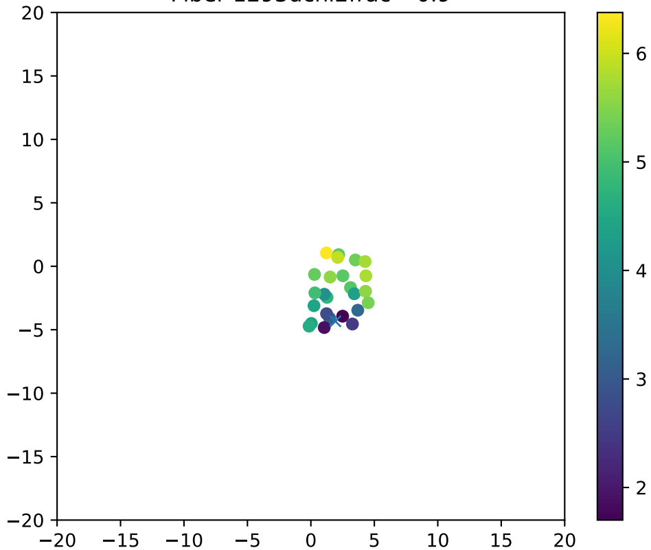
Fiber 1293dchi2frac= 0.9
