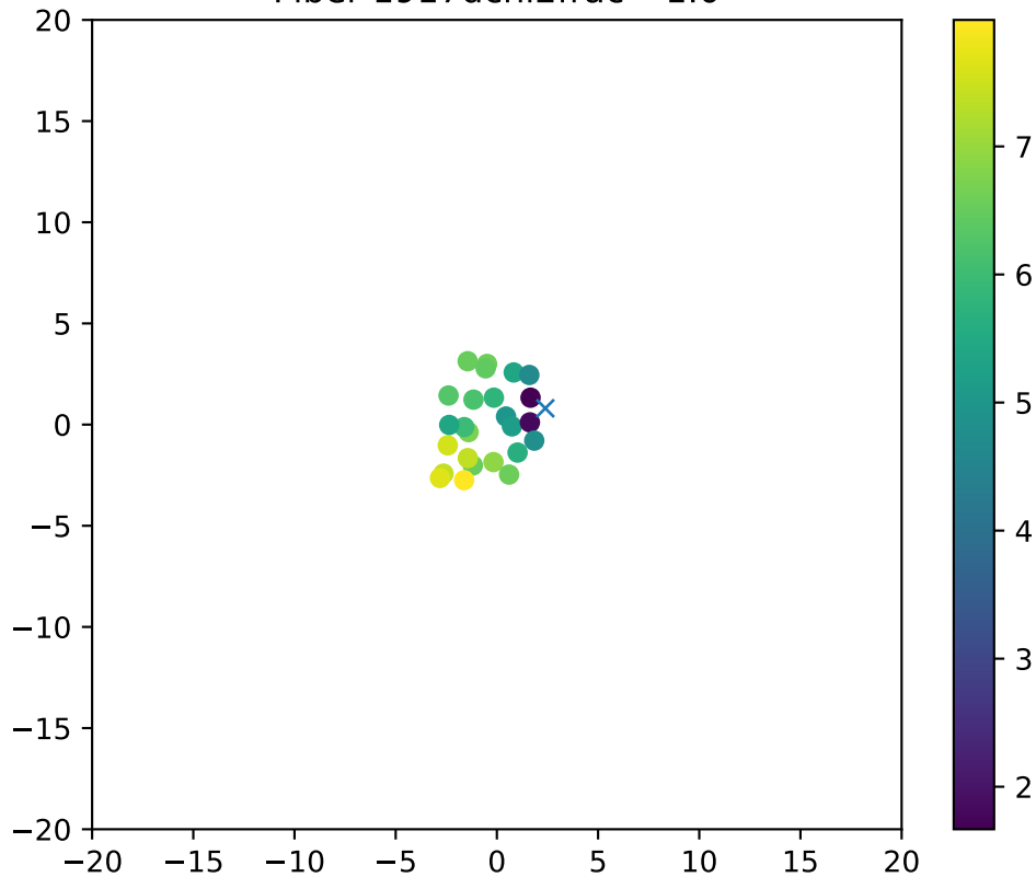
Fiber 1917dchi2frac= 1.0
