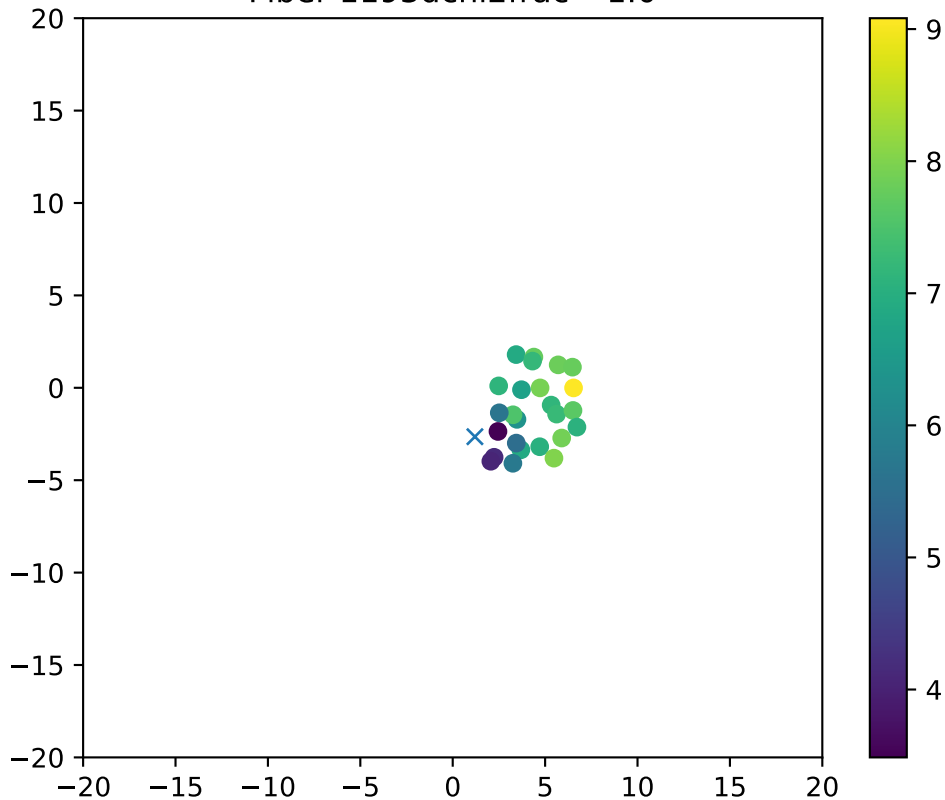
Fiber 1193dchi2frac= 1.0
