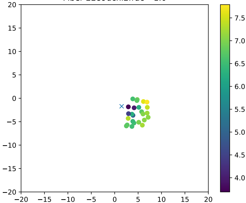
Fiber 2289dchi2frac= 1.0
