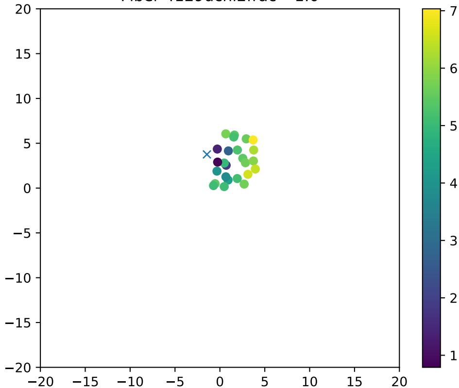
Fiber 4129dchi2frac= 1.0
