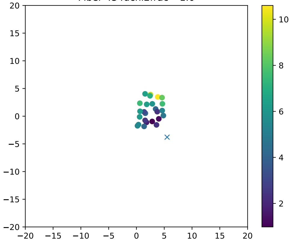
Fiber 434dchi2frac= 1.0
