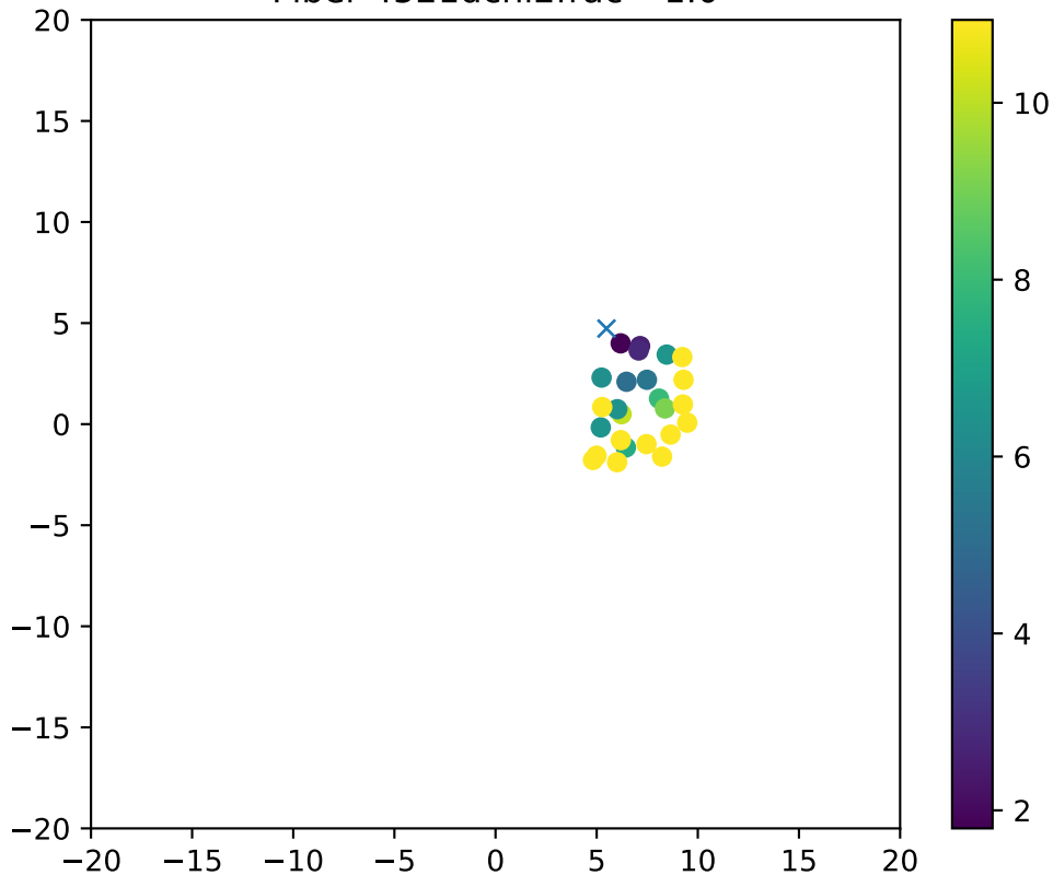
Fiber 4521dchi2frac= 1.0
