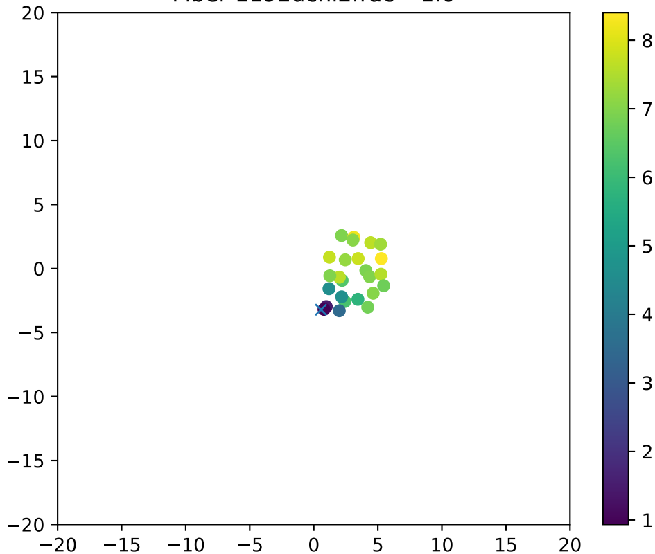
Fiber 1192dchi2frac= 1.0
