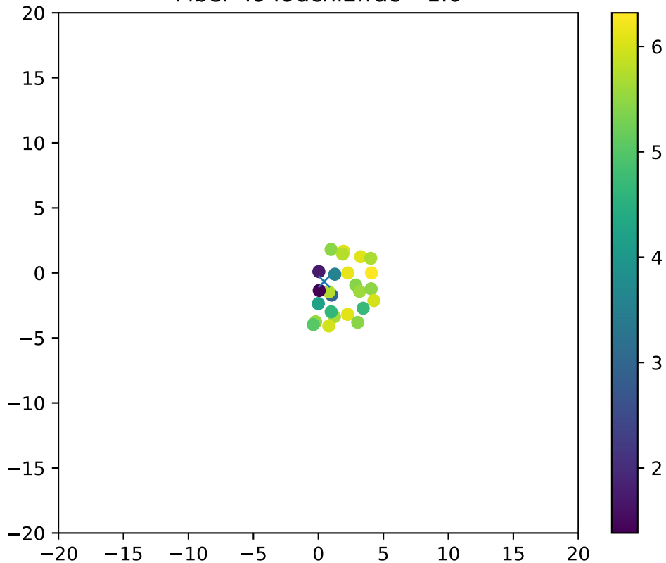
Fiber 4949dchi2frac= 1.0
