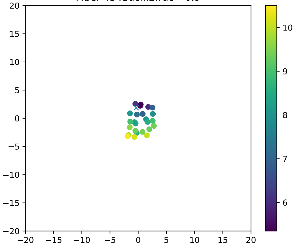
Fiber 4342dchi2frac= 0.9
