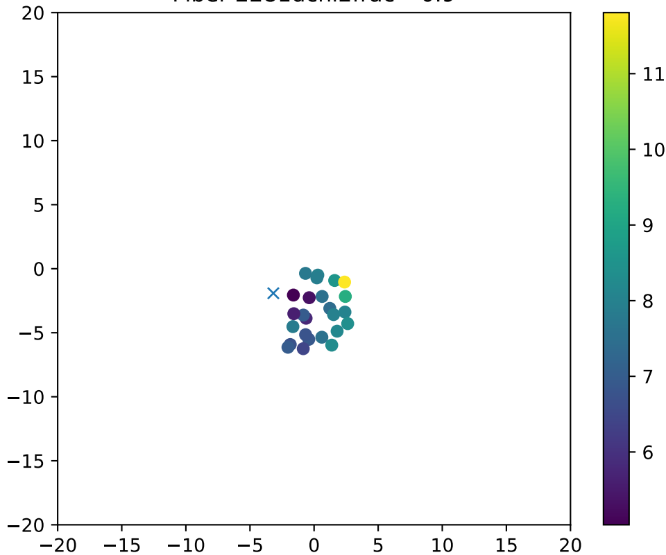
Fiber 2281dchi2frac= 0.9
