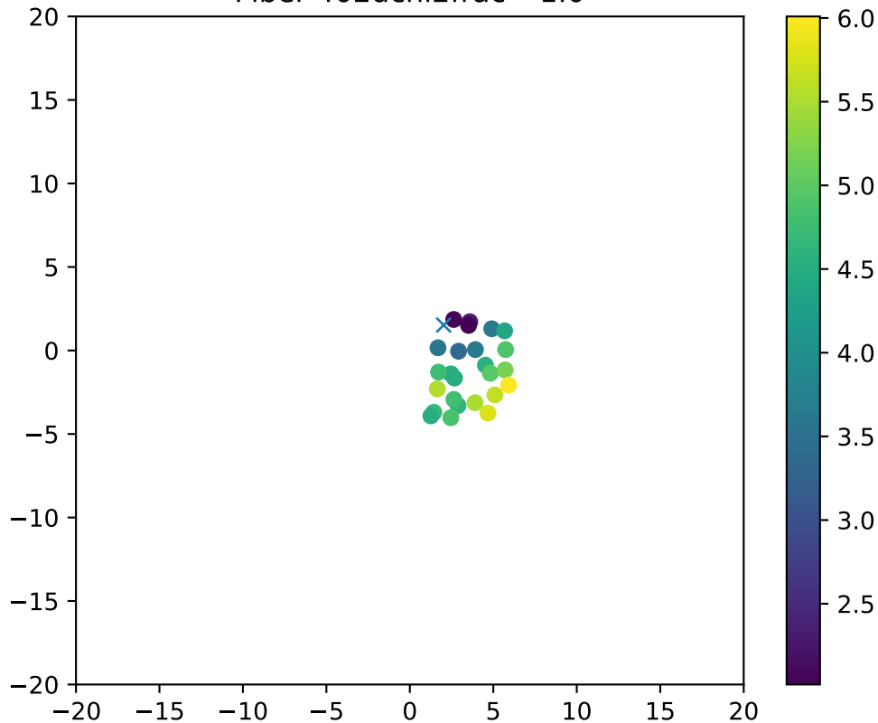
Fiber 402dchi2frac= 1.0
