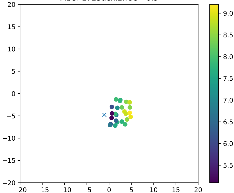
Fiber 1723dchi2frac= 0.9
