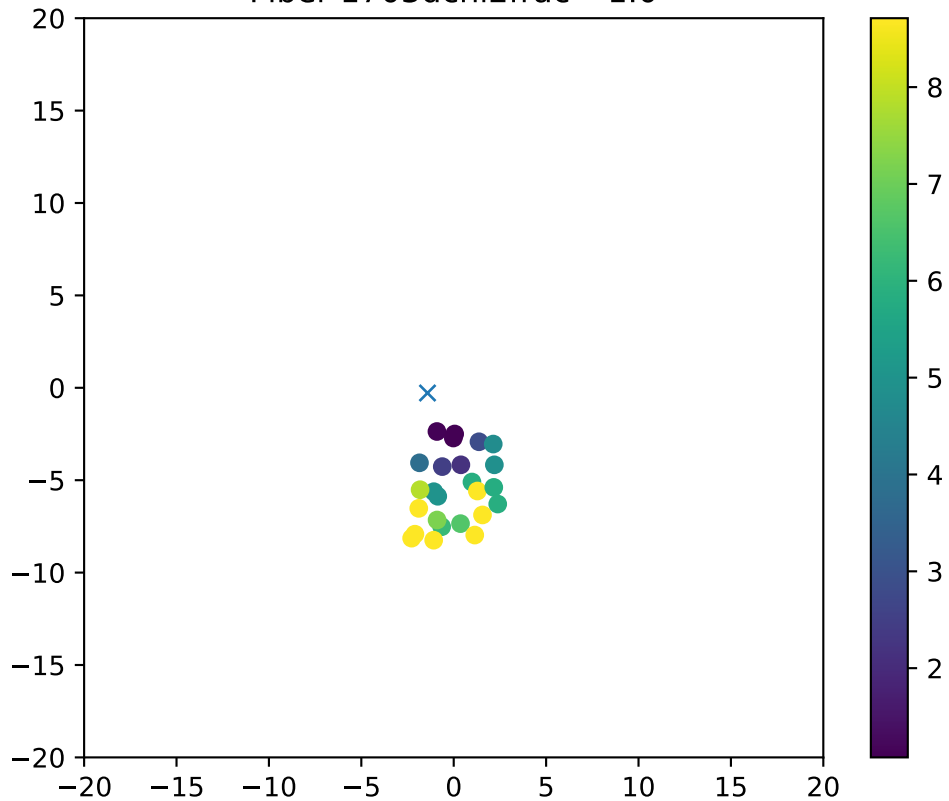
Fiber 1703dchi2frac= 1.0
