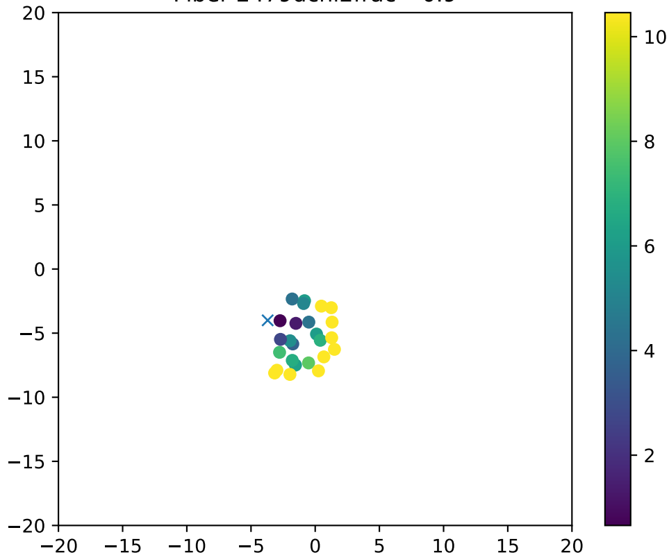
Fiber 2479dchi2frac= 0.9
