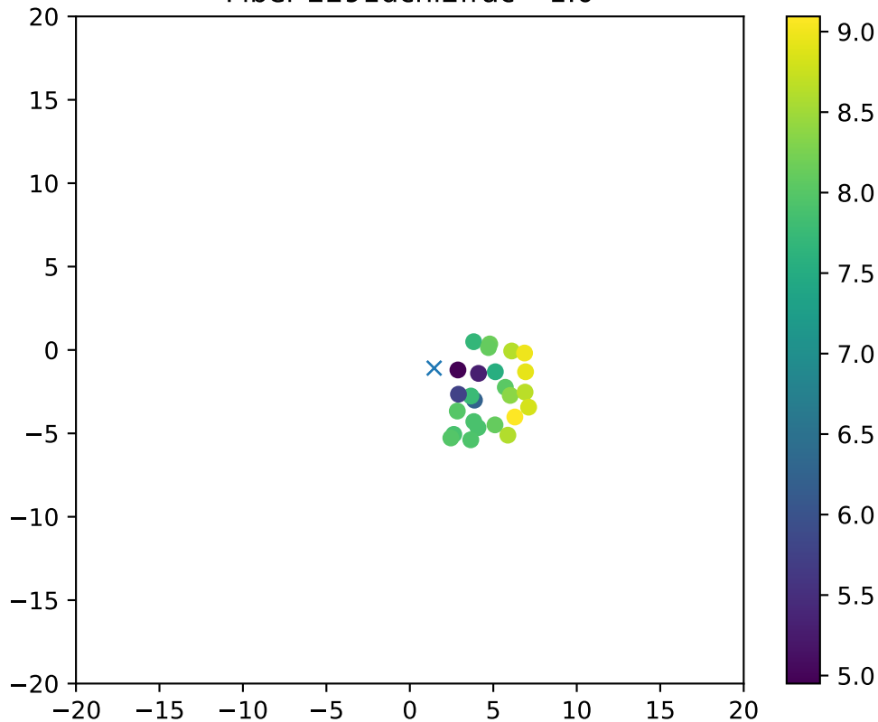
Fiber 2291dchi2frac= 1.0
