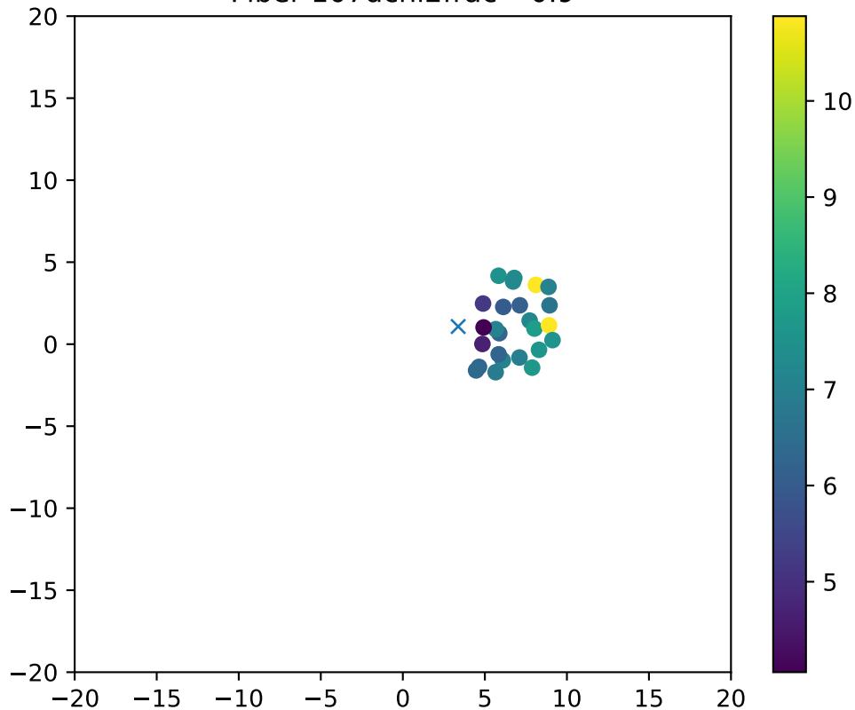
Fiber 107dchi2frac= 0.9
