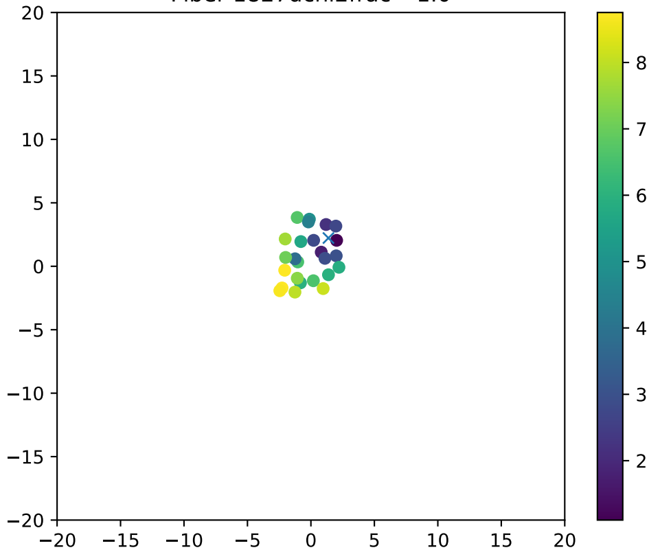
Fiber 1827dchi2frac= 1.0
