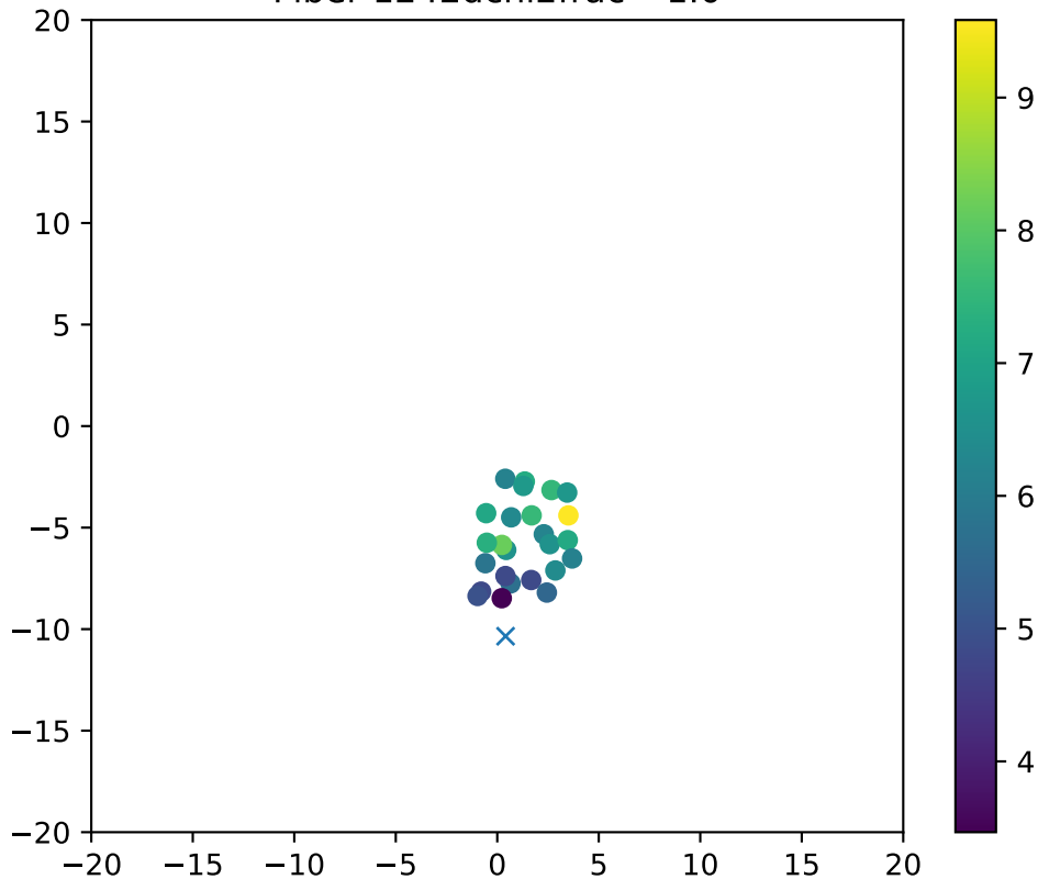
Fiber 1242dchi2frac= 1.0
