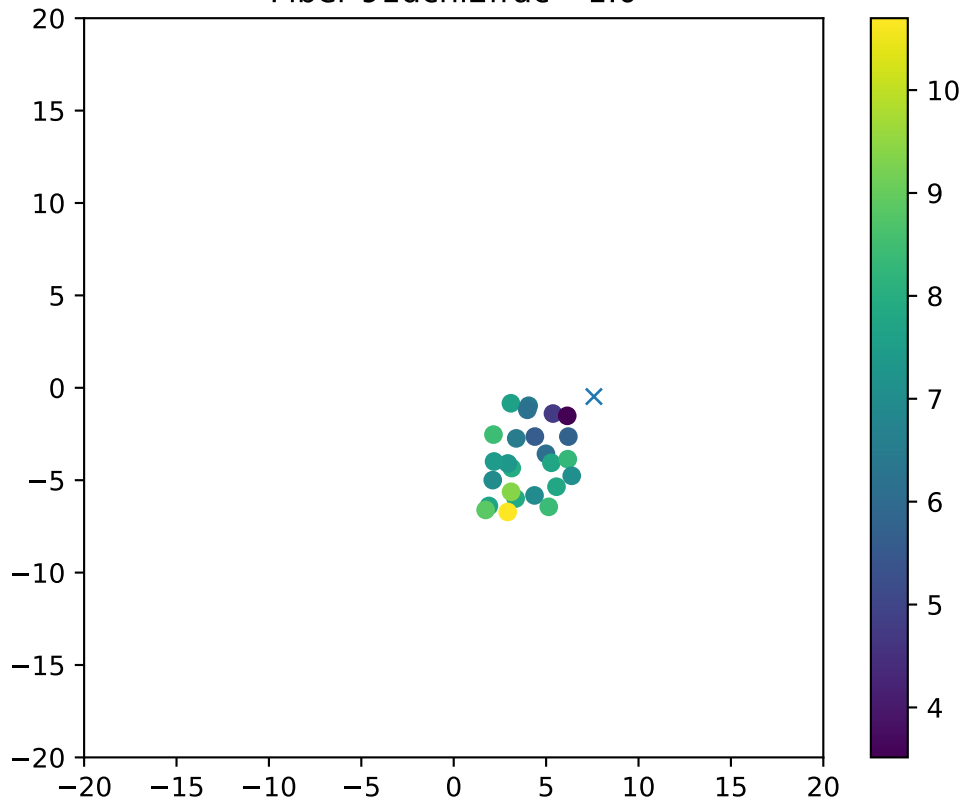
Fiber 91dchi2frac= 1.0
