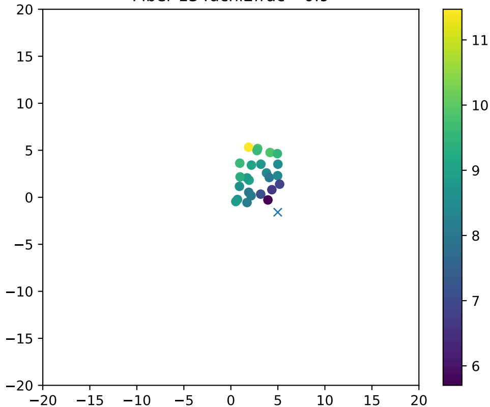
Fiber 134dchi2frac= 0.9
