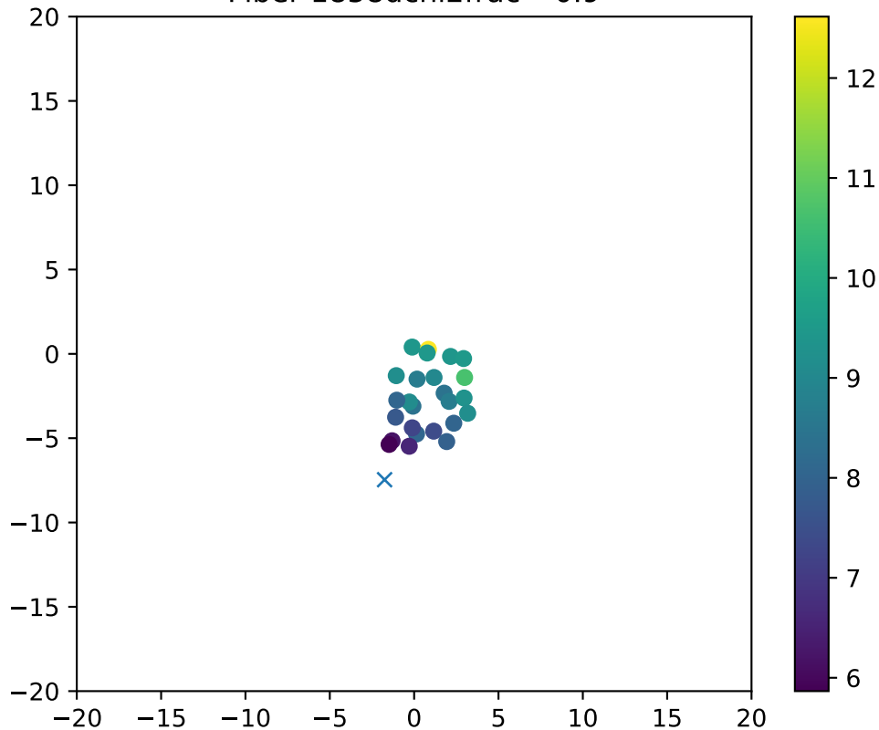
Fiber 1858dchi2frac= 0.9
