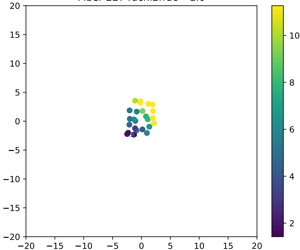
Fiber 2274dchi2frac= 1.0
