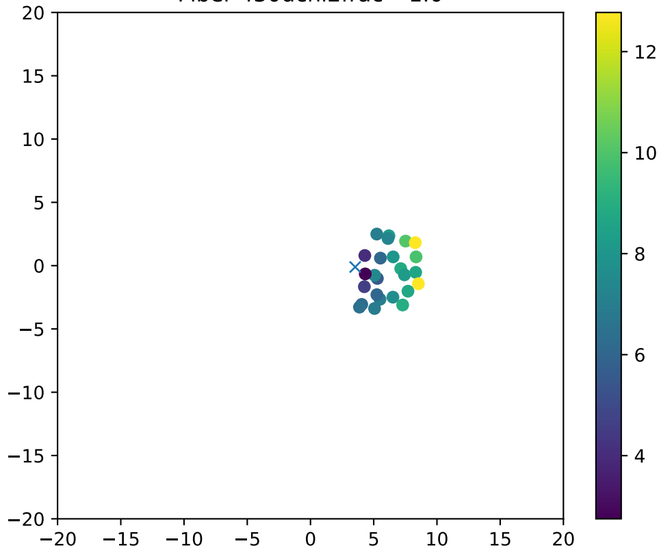
Fiber 430dchi2frac= 1.0
