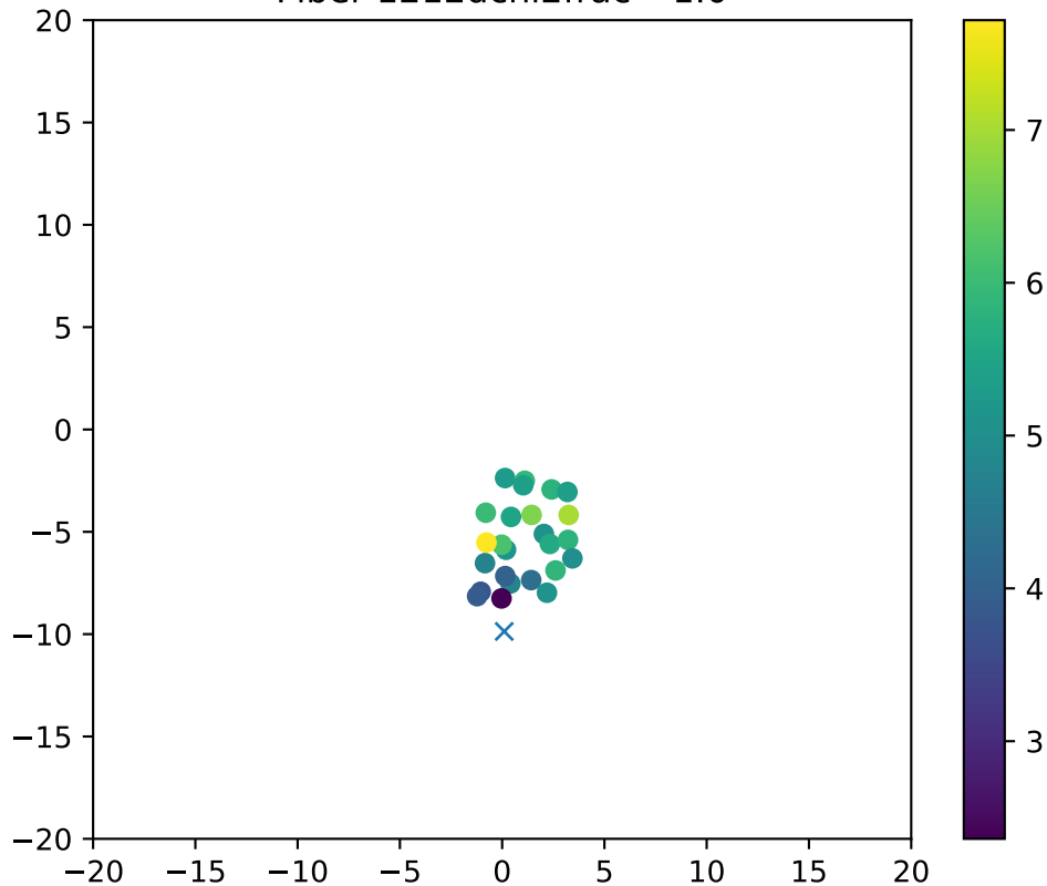
Fiber 1212dchi2frac= 1.0
