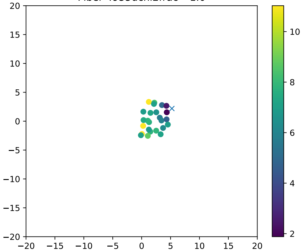
Fiber 4955dchi2frac= 1.0
