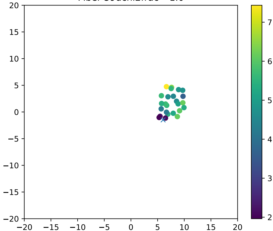
Fiber 39dchi2frac= 1.0
