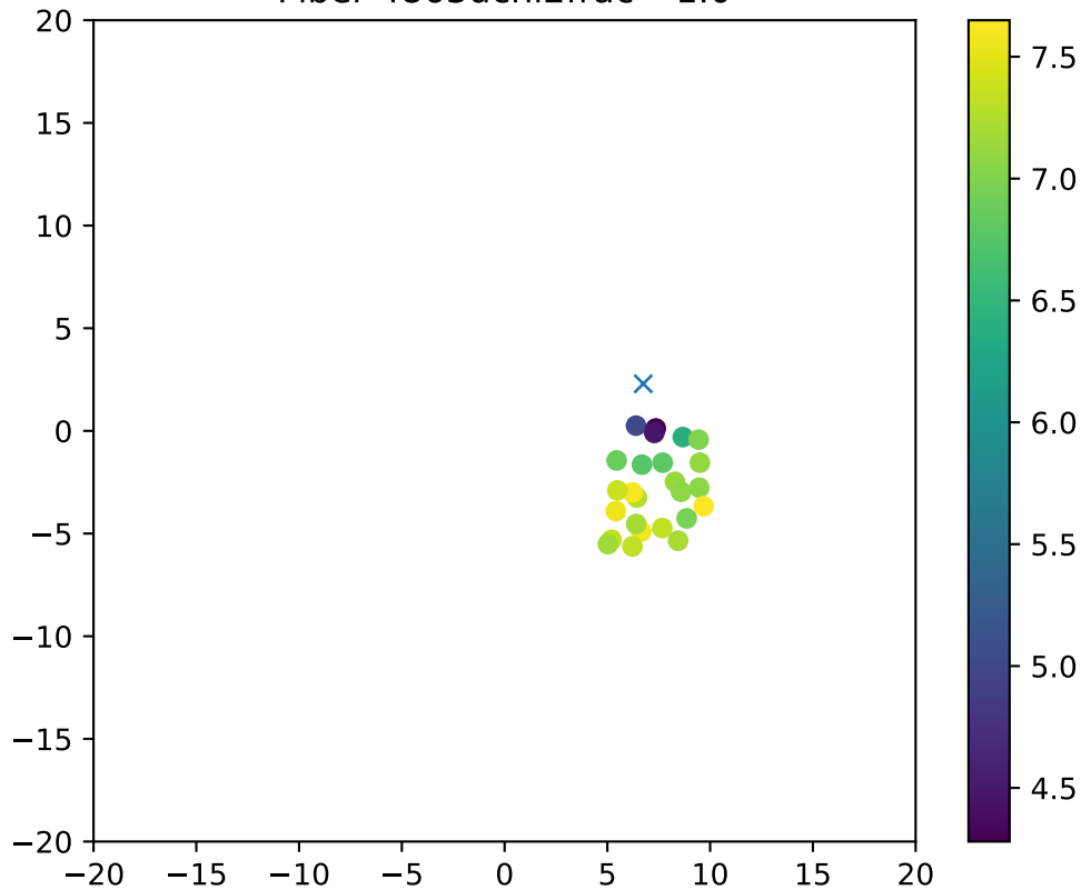
Fiber 4863dchi2frac= 1.0
