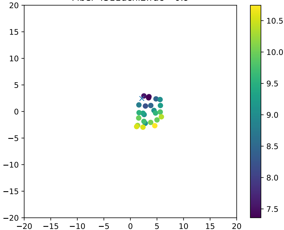
Fiber 4311dchi2frac= 0.9
