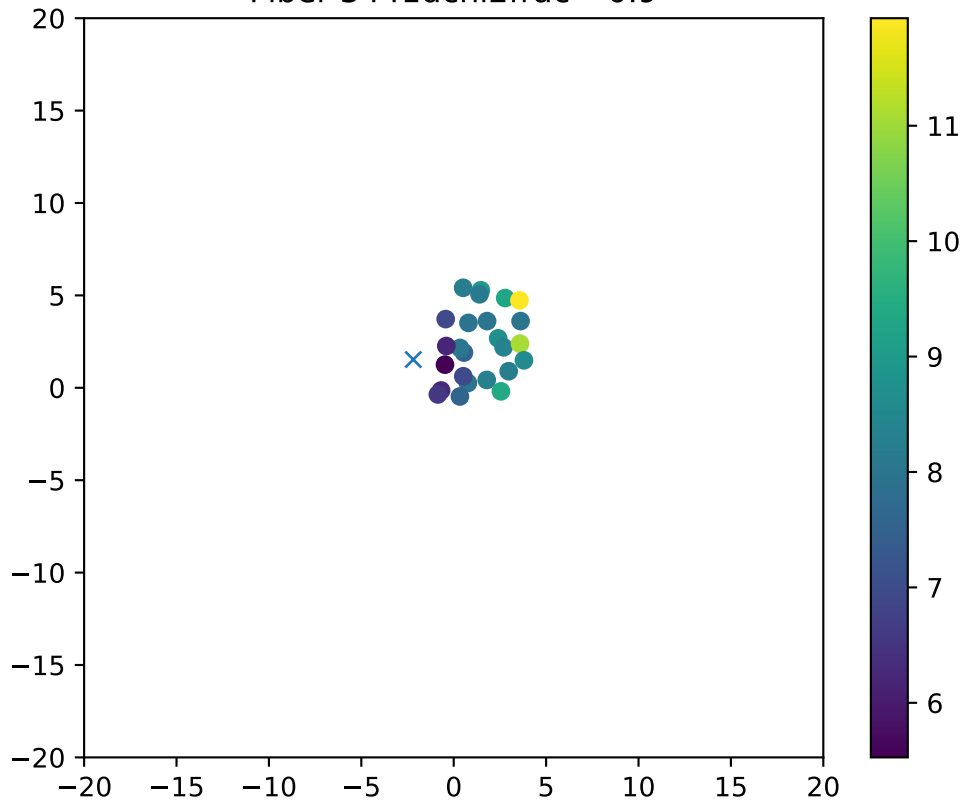
Fiber 3441dchi2frac= 0.9
