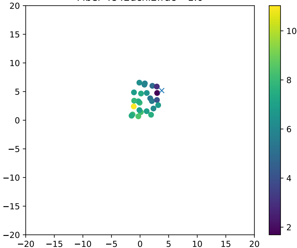
Fiber 4842dchi2frac= 1.0
