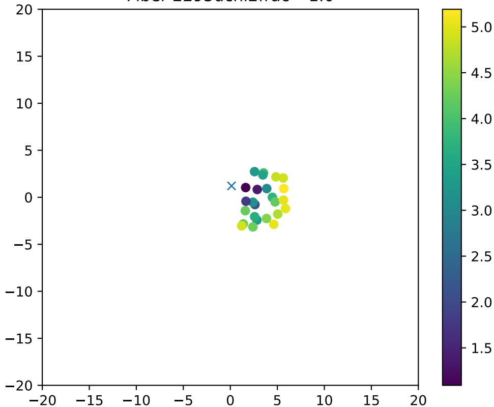
Fiber 2293dchi2frac= 1.0
