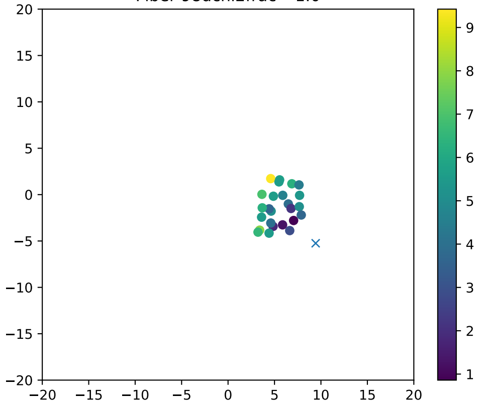
Fiber 98dchi2frac= 1.0
