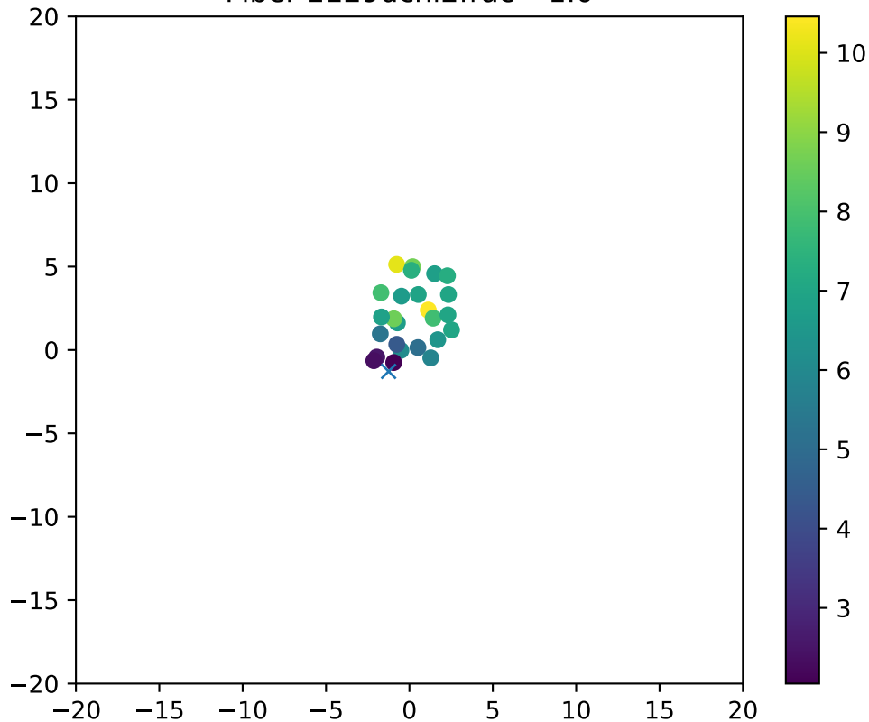
Fiber 2129dchi2frac= 1.0
