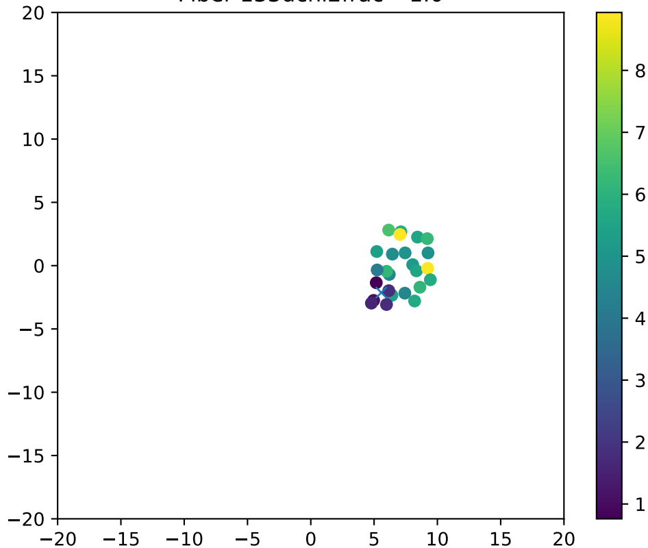
Fiber 133dchi2frac= 1.0
