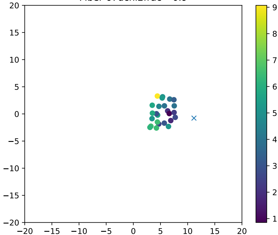
Fiber 67dchi2frac= 0.9
