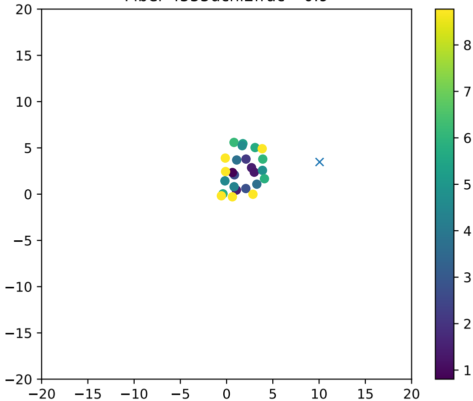
Fiber 4555dchi2frac= 0.9
