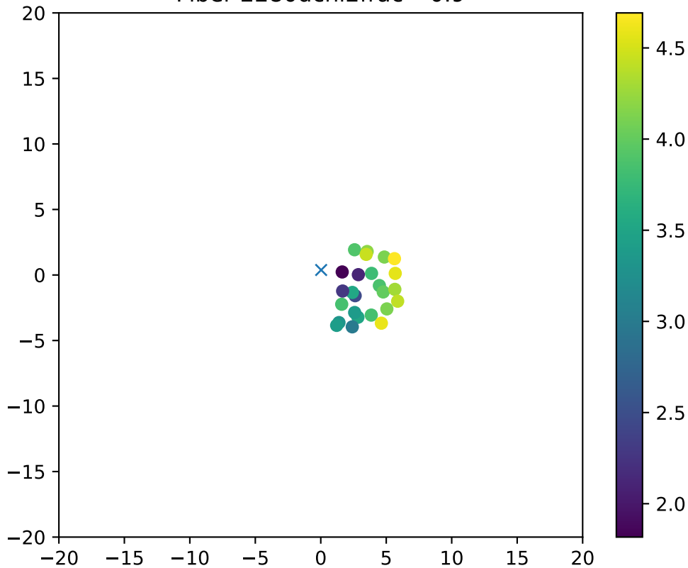
Fiber 2280dchi2frac= 0.9
