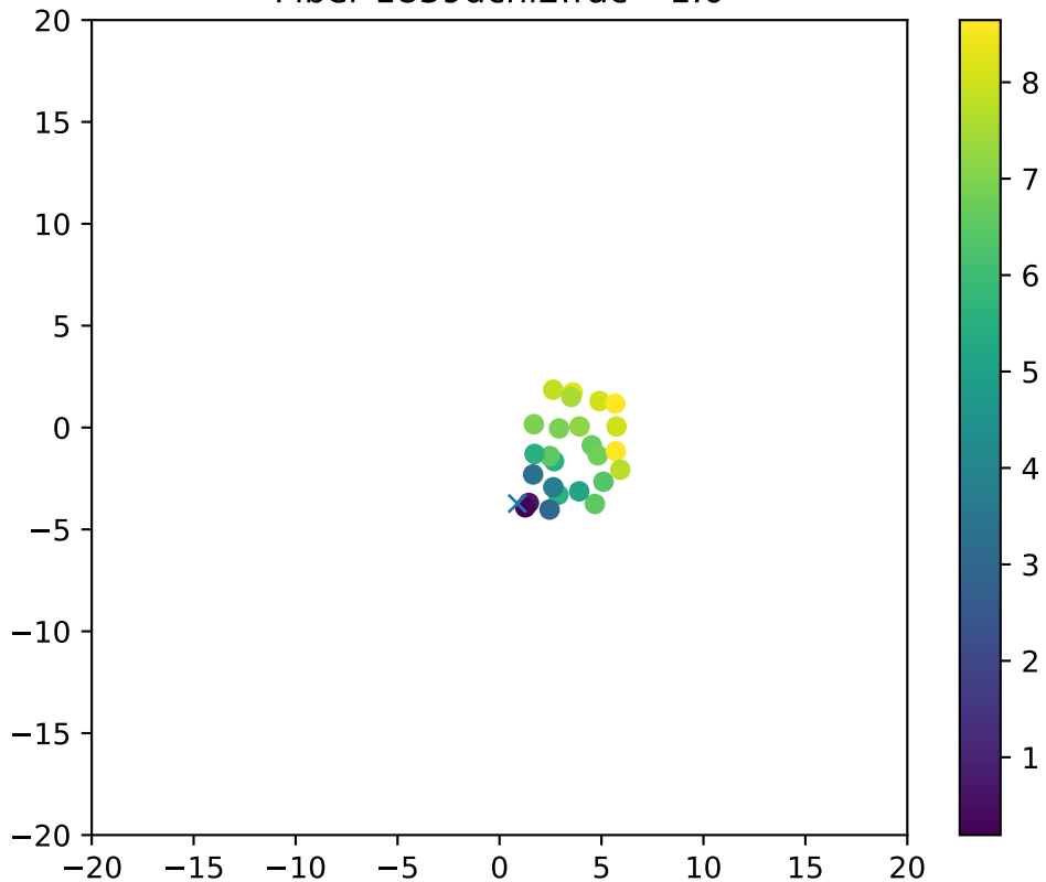
Fiber 1839dchi2frac= 1.0
