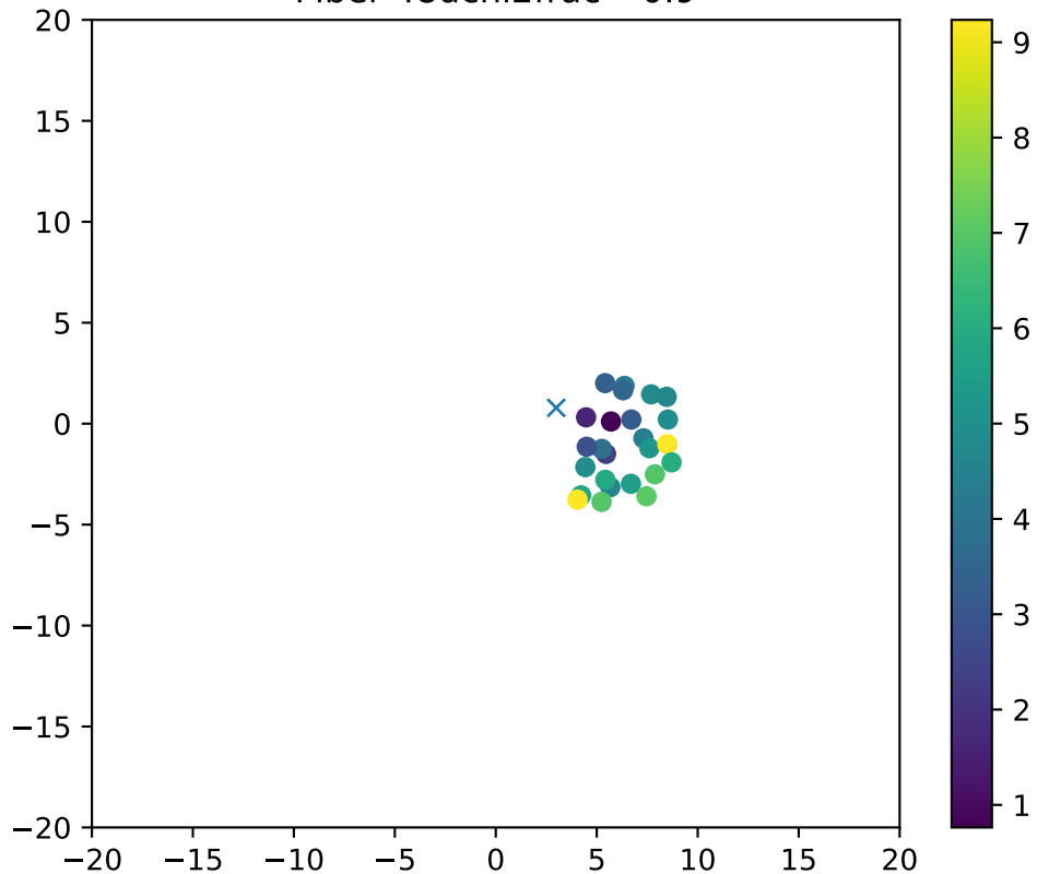
Fiber 48dchi2frac= 0.9
