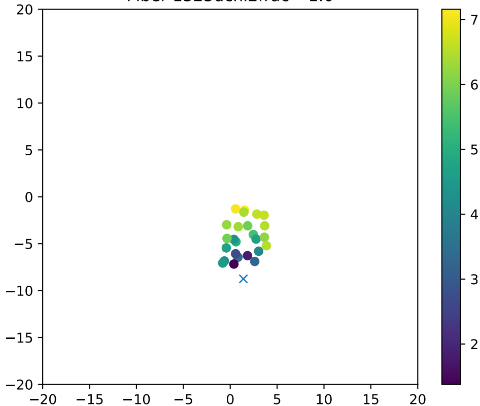
Fiber 1323dchi2frac= 1.0
