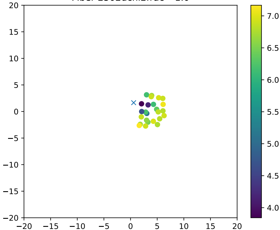
Fiber 2302dchi2frac= 1.0
