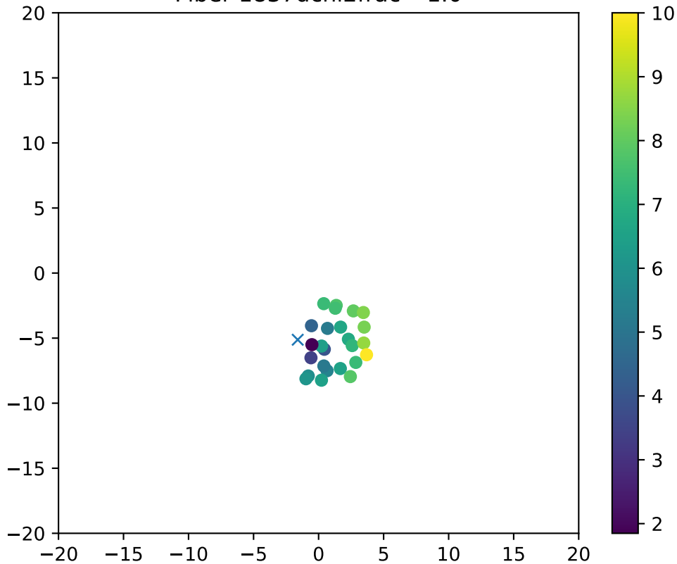
Fiber 1837dchi2frac= 1.0
