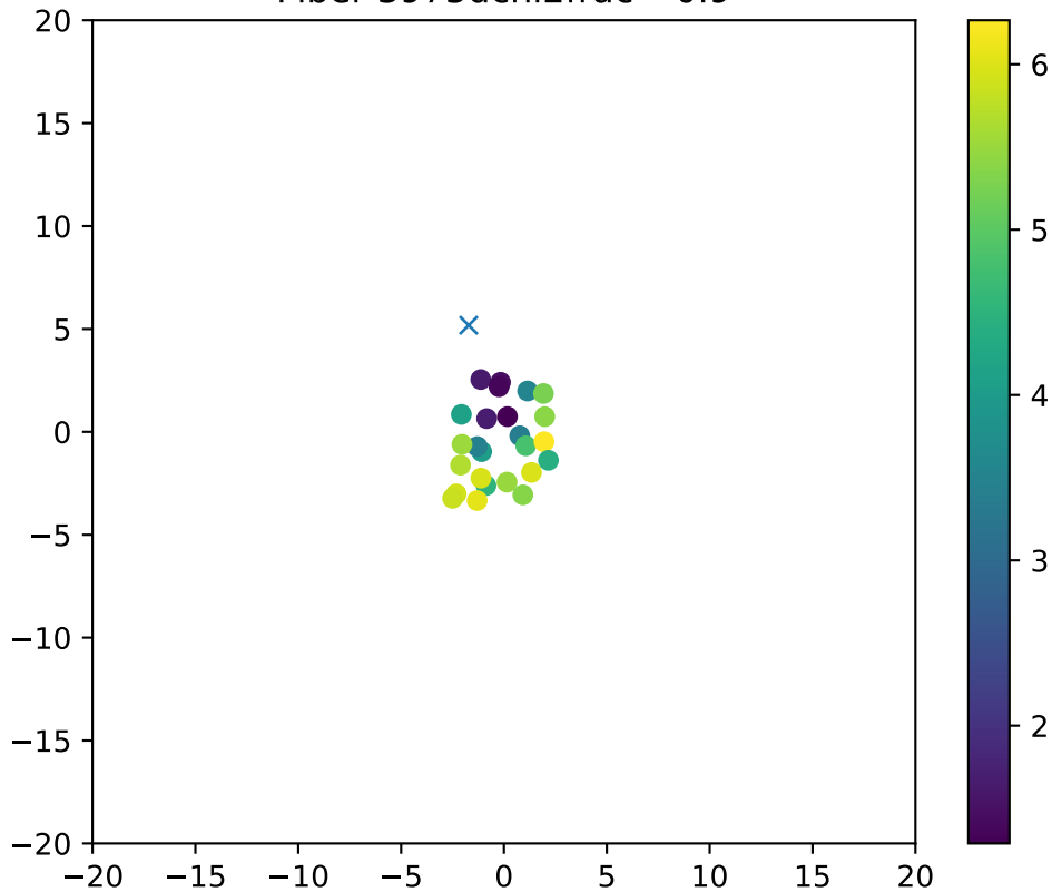
Fiber 3975dchi2frac= 0.9
