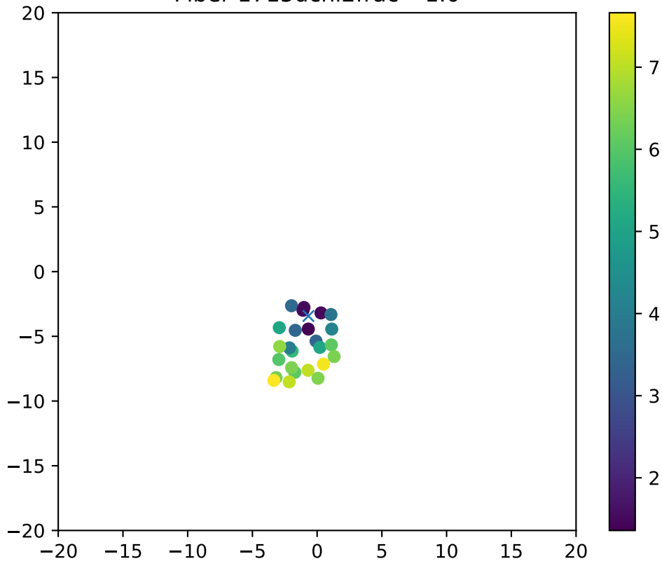
Fiber 1715dchi2frac= 1.0
