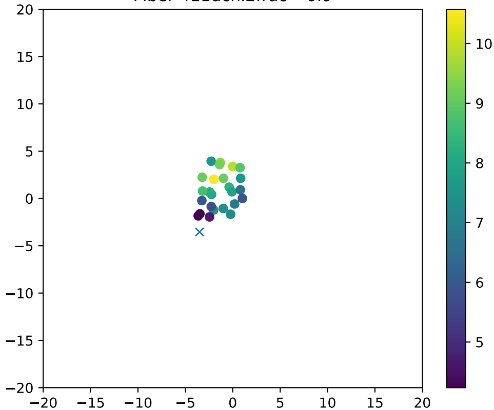
Fiber 411dchi2frac= 0.9
