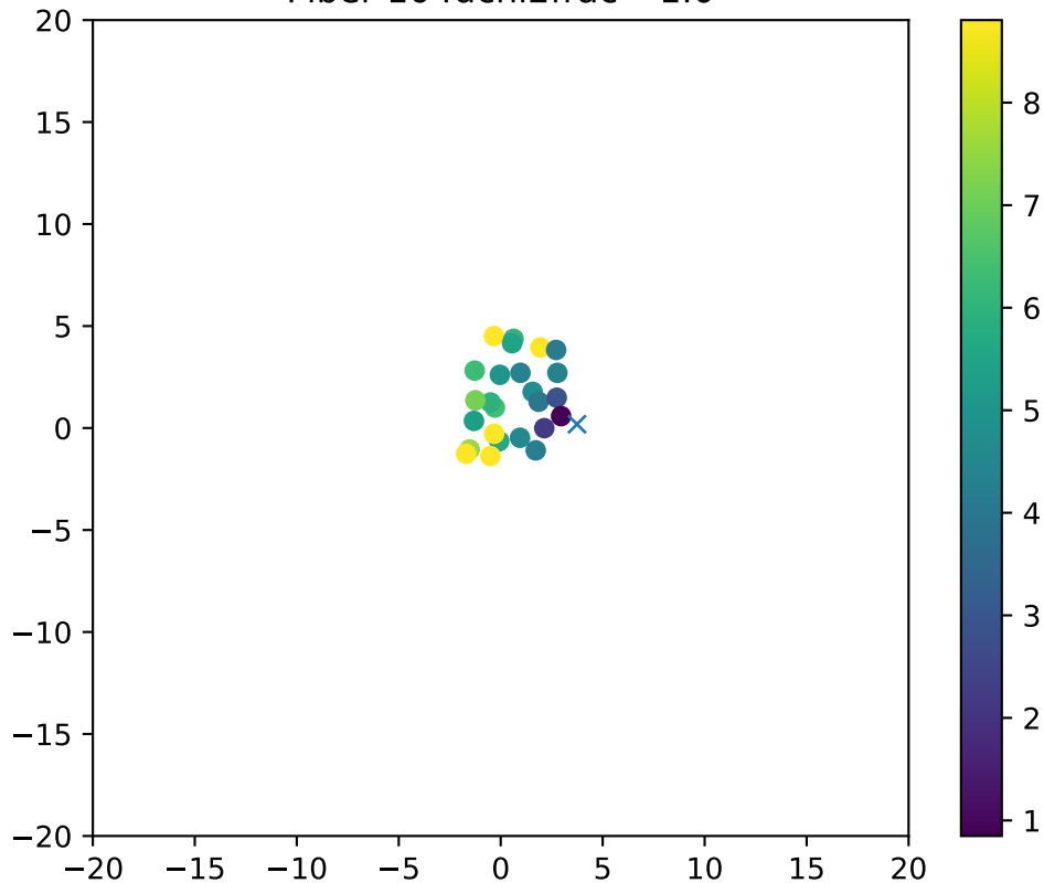
Fiber 104dchi2frac= 1.0
