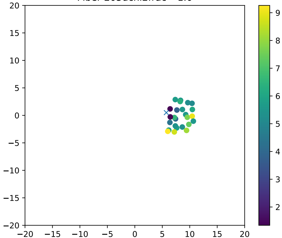
Fiber 203dchi2frac= 1.0
