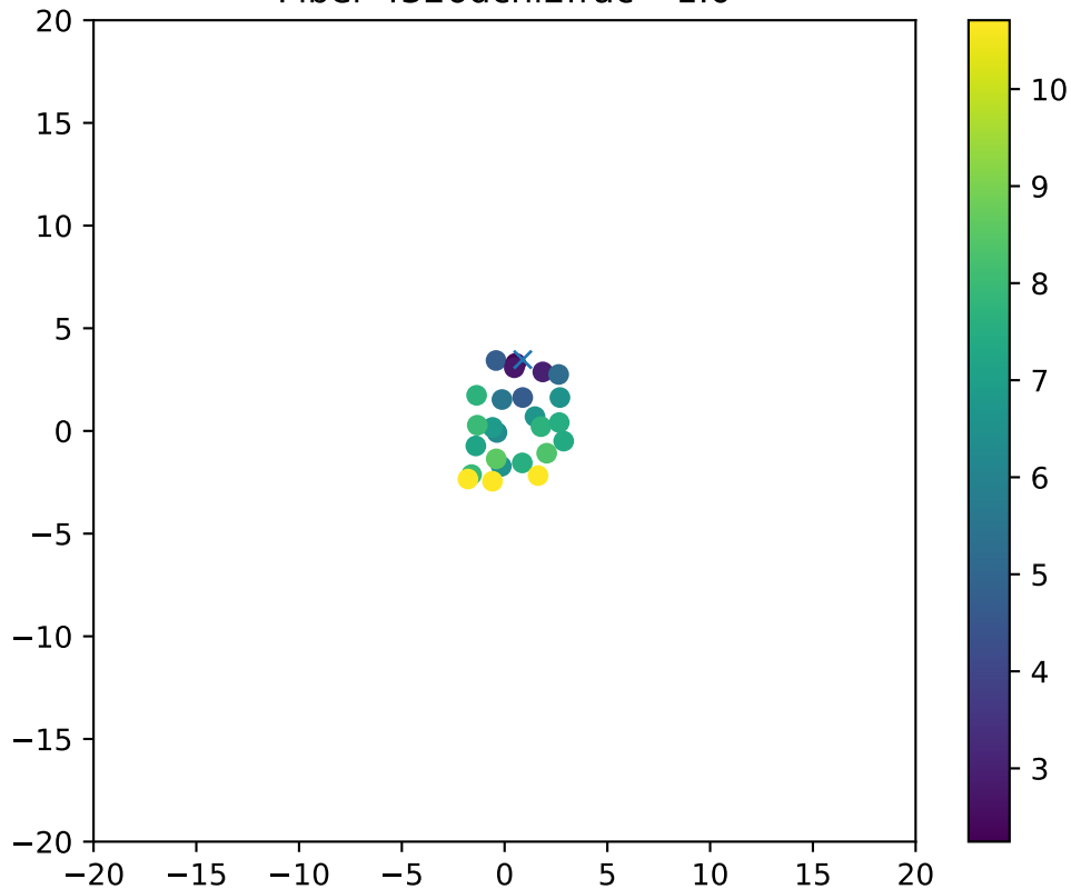
Fiber 4326dchi2frac= 1.0
