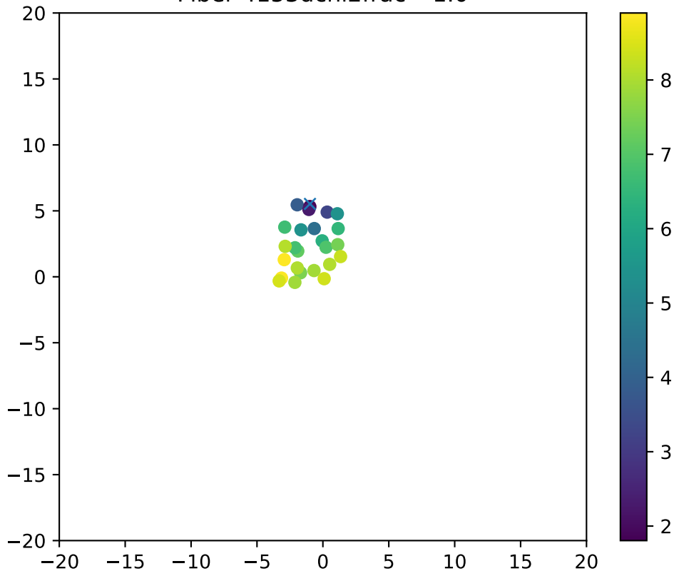
Fiber 4153dchi2frac= 1.0
