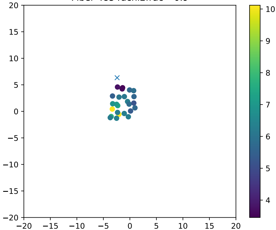
Fiber 4854dchi2frac= 0.9
