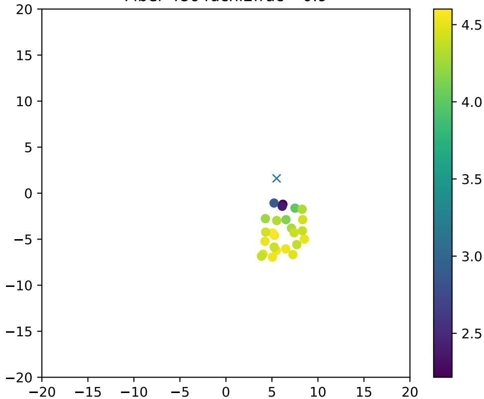
Fiber 4864dchi2frac= 0.9
