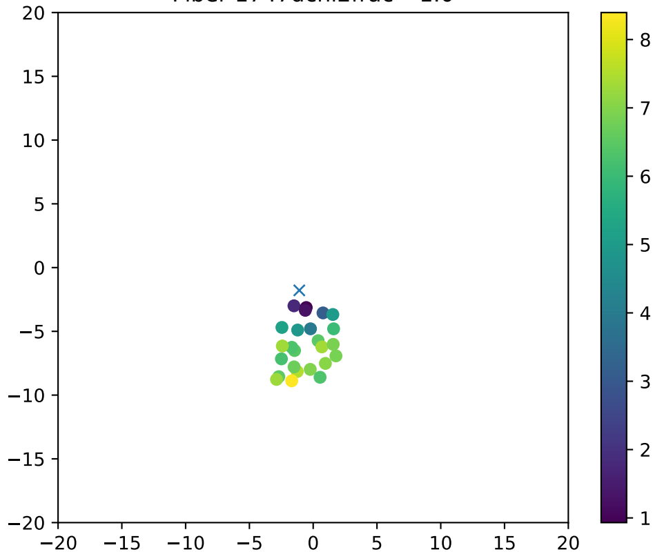
Fiber 1747dchi2frac= 1.0
