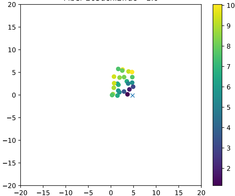
Fiber 265dchi2frac= 1.0
