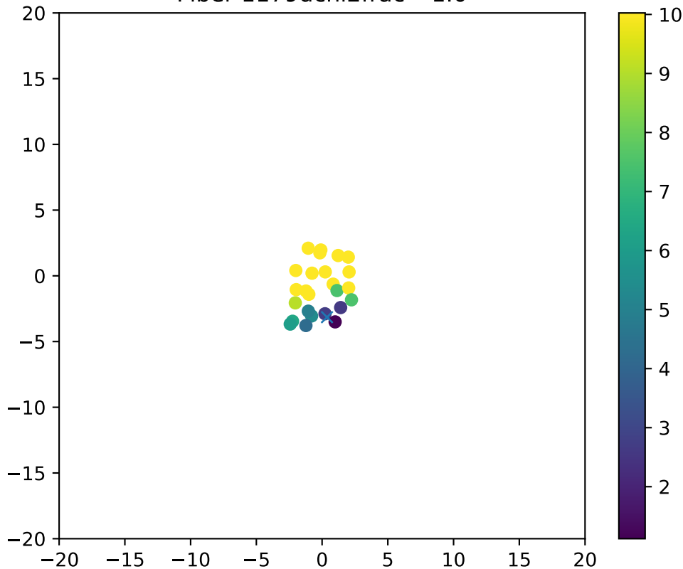
Fiber 1179dchi2frac= 1.0
