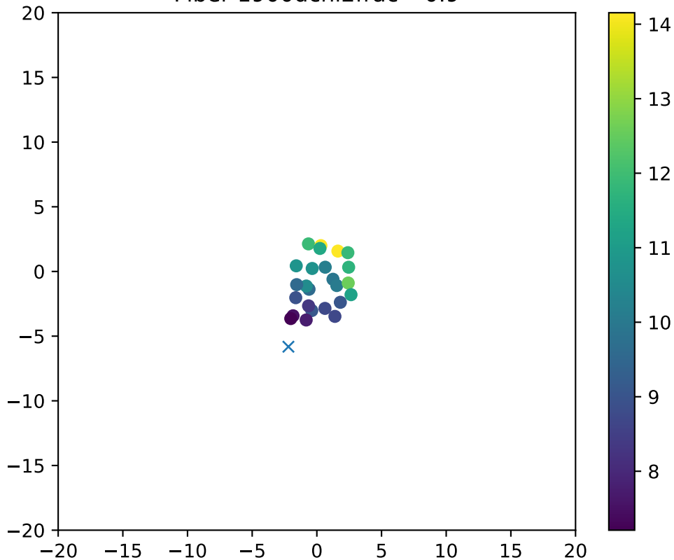
Fiber 1900dchi2frac= 0.9
