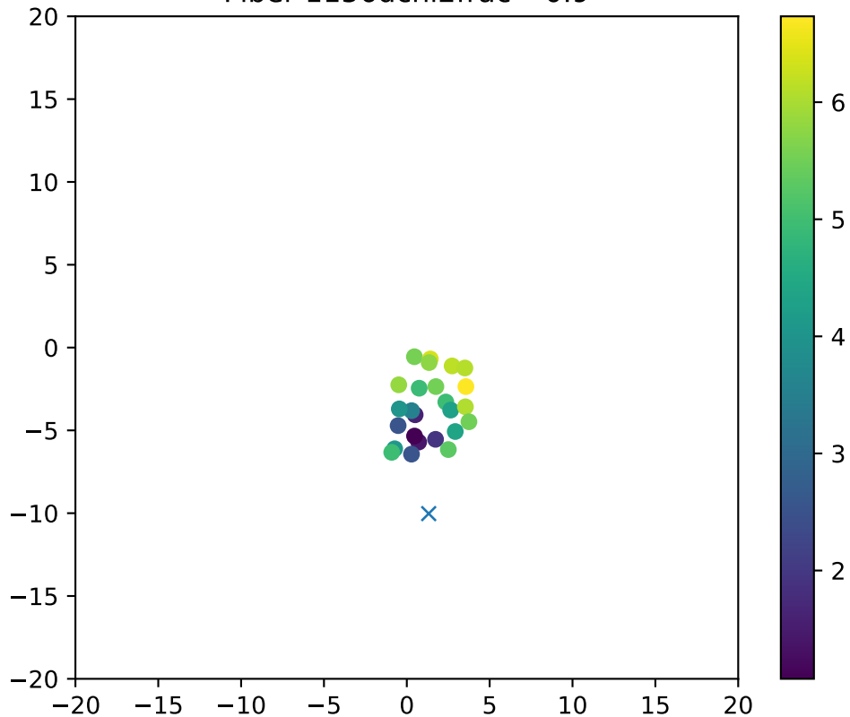
Fiber 1156dchi2frac= 0.9
