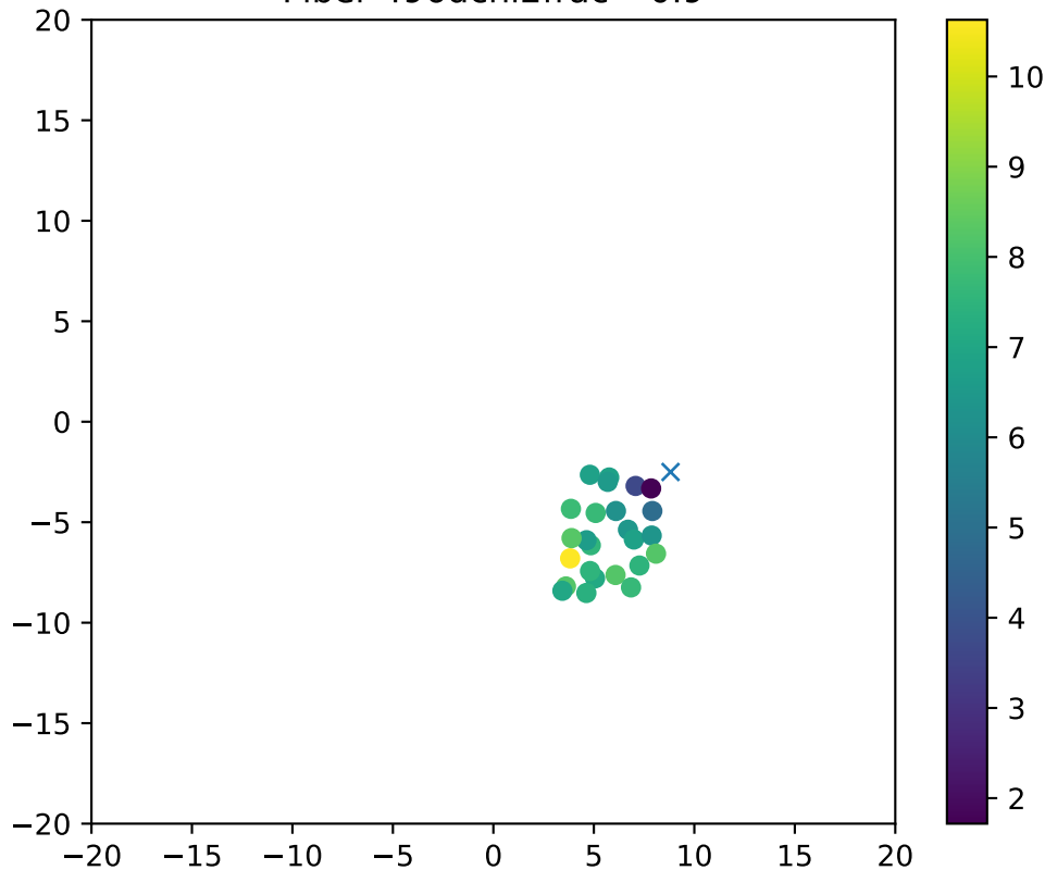
Fiber 496dchi2frac= 0.9
