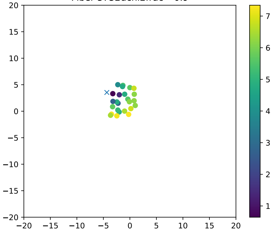
Fiber 3732dchi2frac= 0.9
