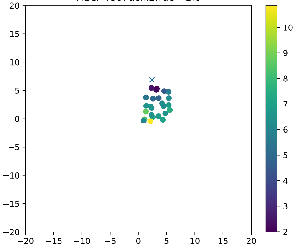
Fiber 4867dchi2frac= 1.0
