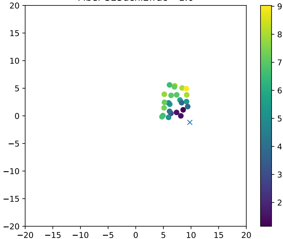
Fiber 325dchi2frac= 1.0
