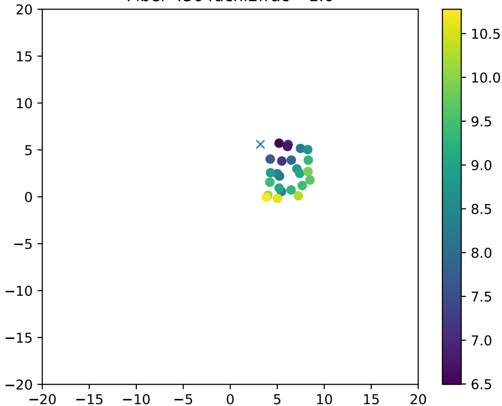
Fiber 4364dchi2frac= 1.0
