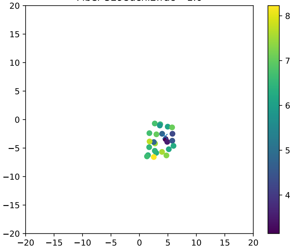
Fiber 3298dchi2frac= 1.0
