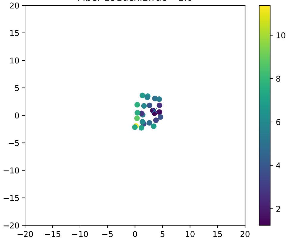
Fiber 291dchi2frac= 1.0
