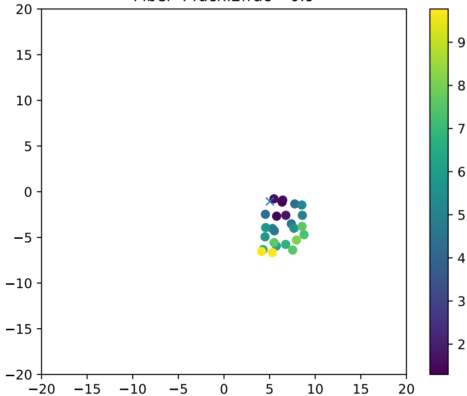
Fiber 44dchi2frac= 0.9
