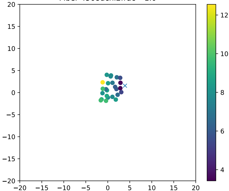
Fiber 4568dchi2frac= 1.0
