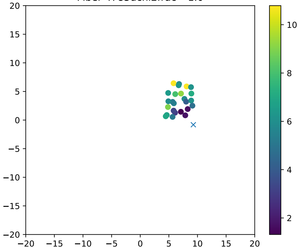
Fiber 4783dchi2frac= 1.0
