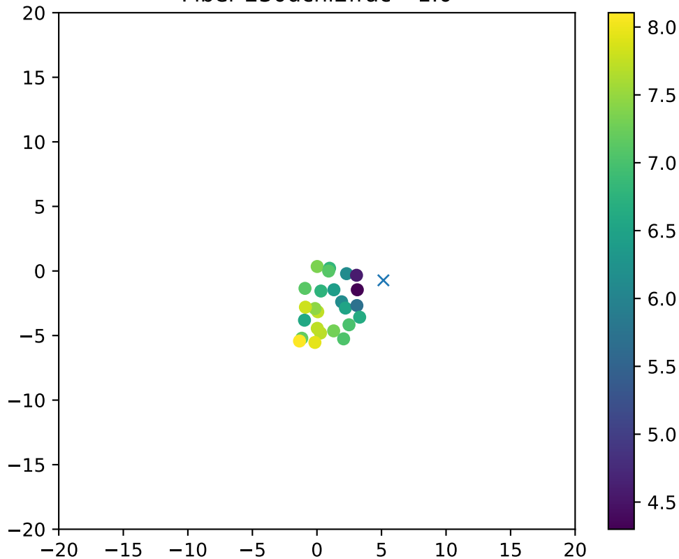
Fiber 230dchi2frac= 1.0
