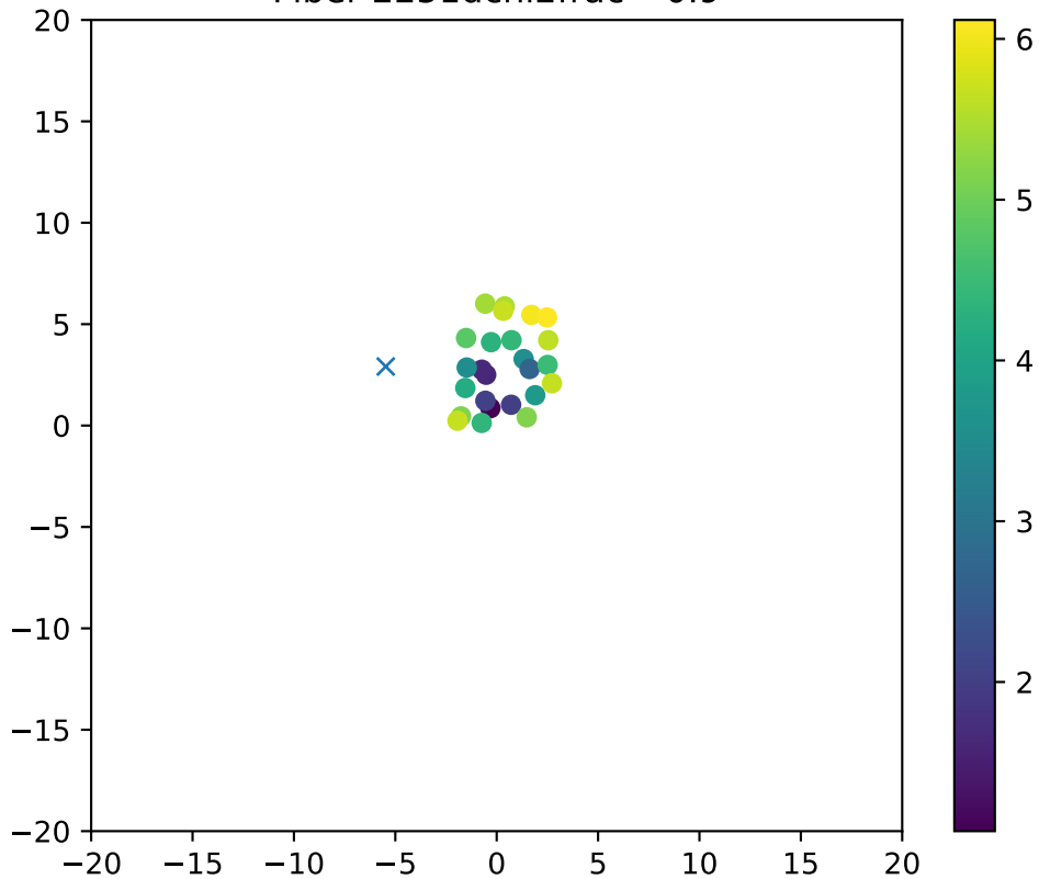
Fiber 2251dchi2frac= 0.9
