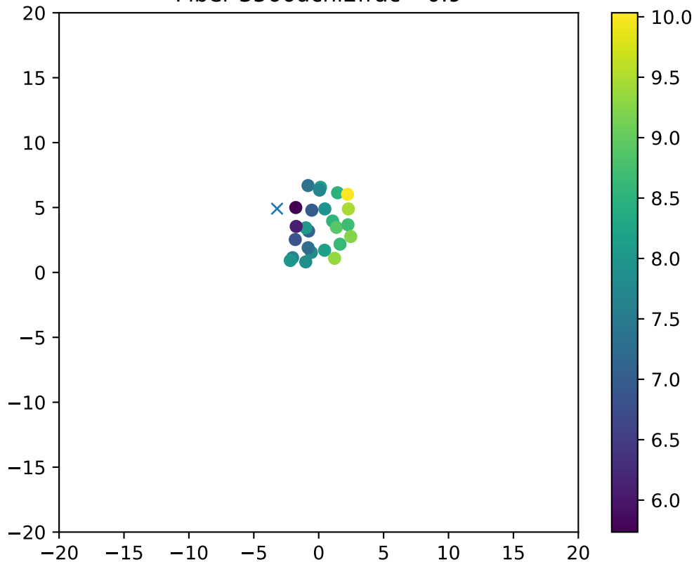
Fiber 3566dchi2frac= 0.9
