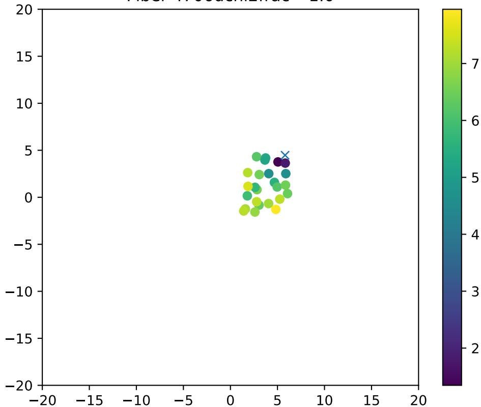
Fiber 4706dchi2frac= 1.0
