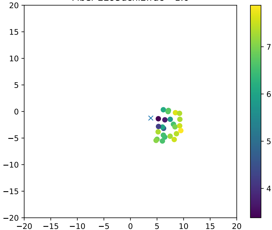
Fiber 2295dchi2frac= 1.0
