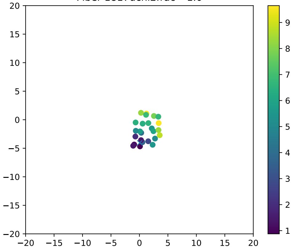
Fiber 1817dchi2frac= 1.0
