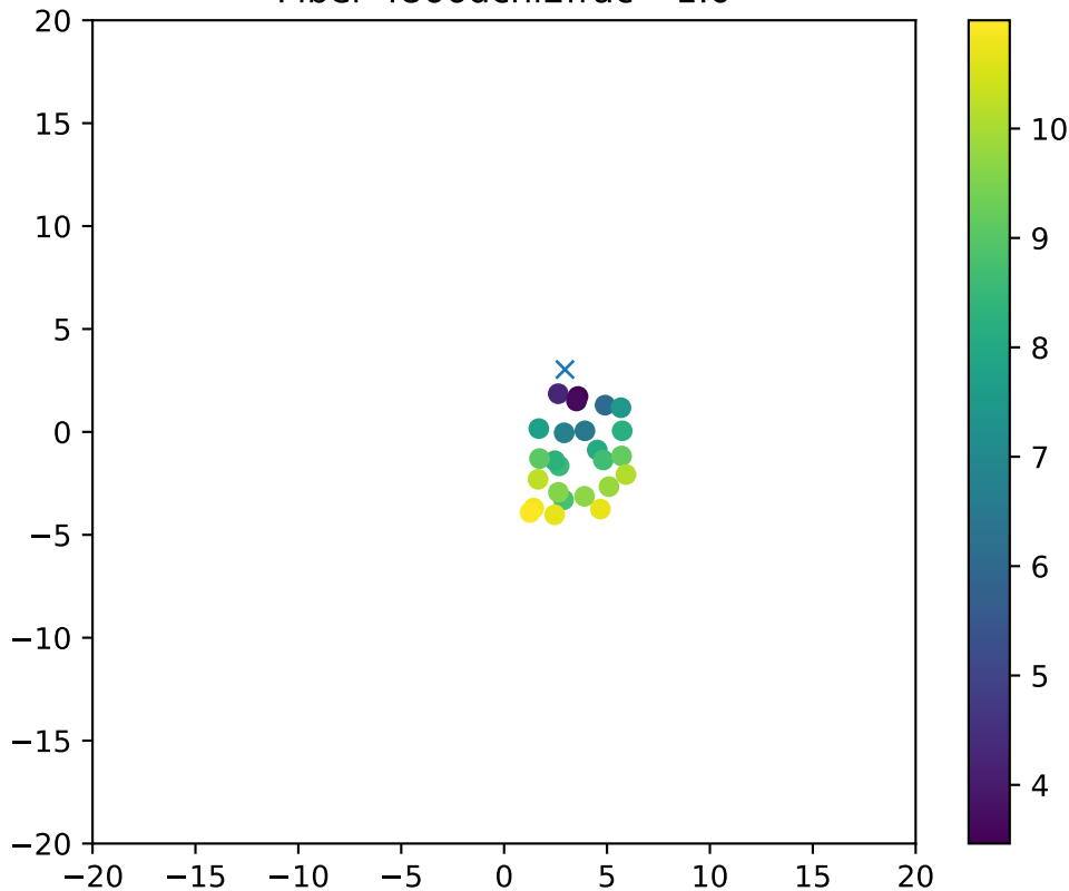
Fiber 4866dchi2frac= 1.0
