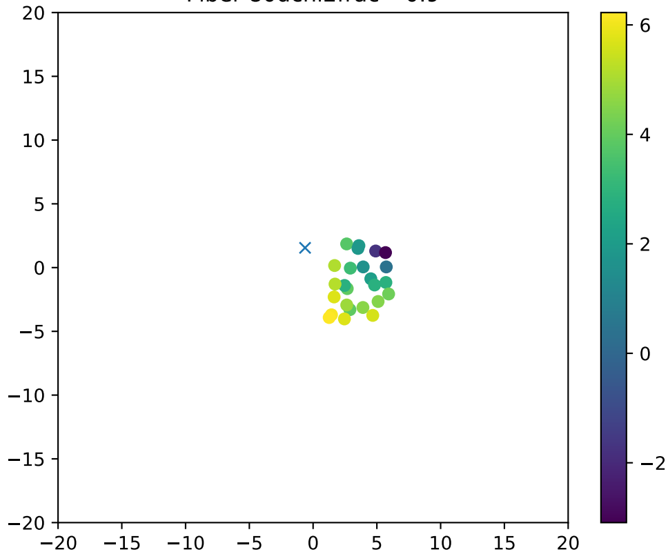
Fiber 80dchi2frac= 0.9
