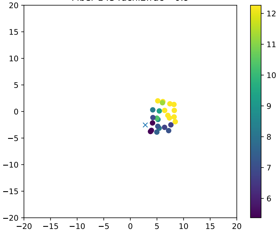
Fiber 1434dchi2frac= 0.9
