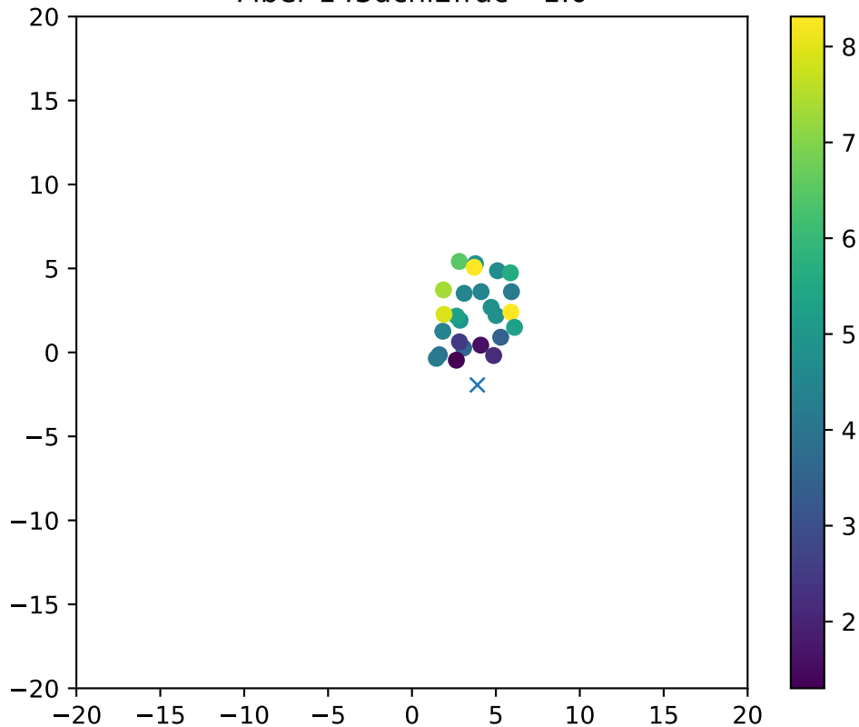
Fiber 143dchi2frac= 1.0
