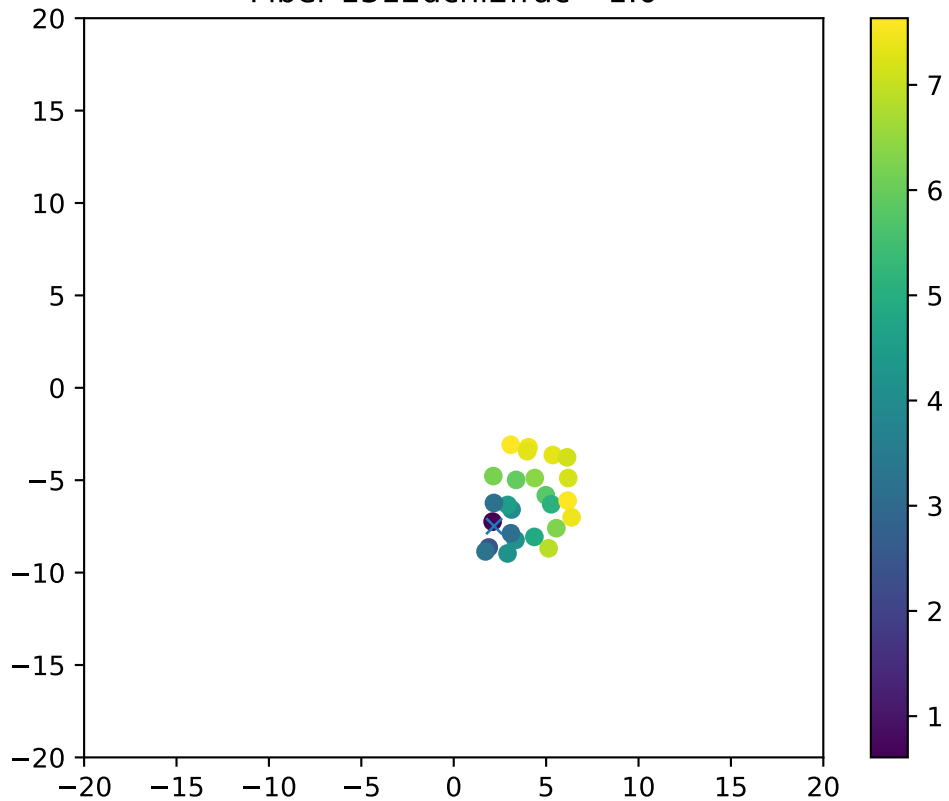
Fiber 1312dchi2frac= 1.0
