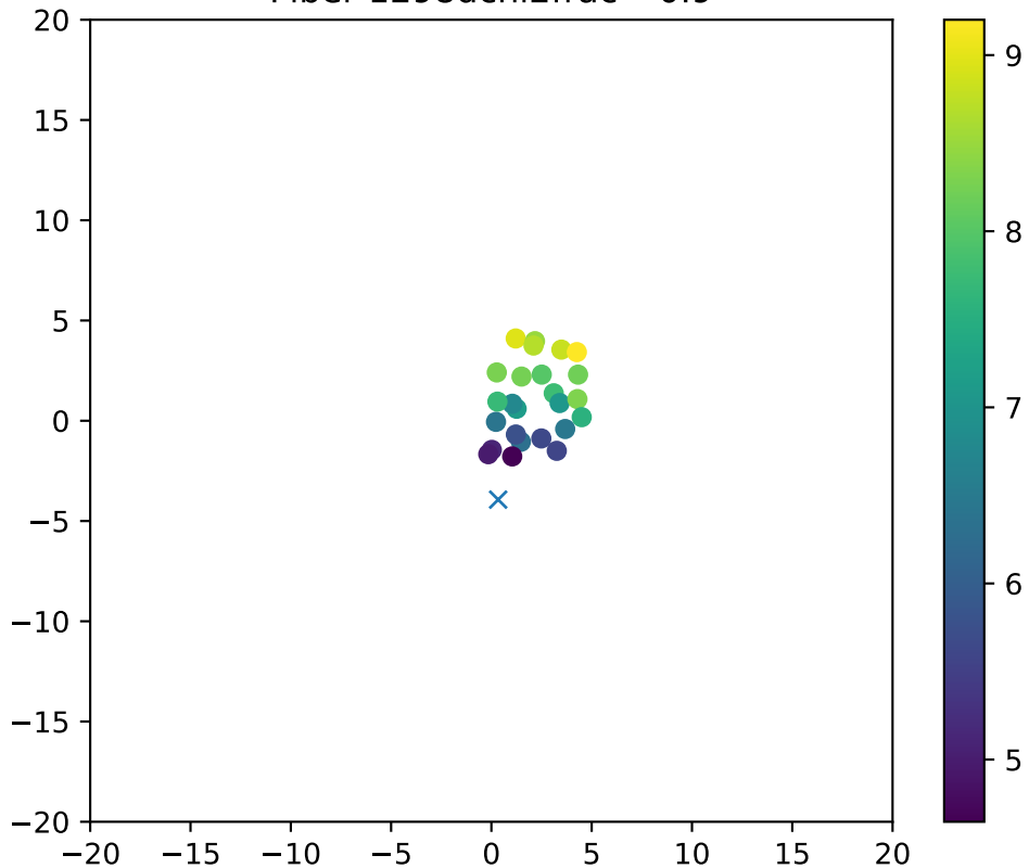
Fiber 1298dchi2frac= 0.9
