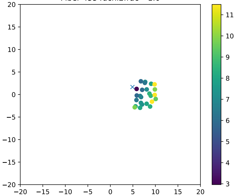
Fiber 4554dchi2frac= 1.0
