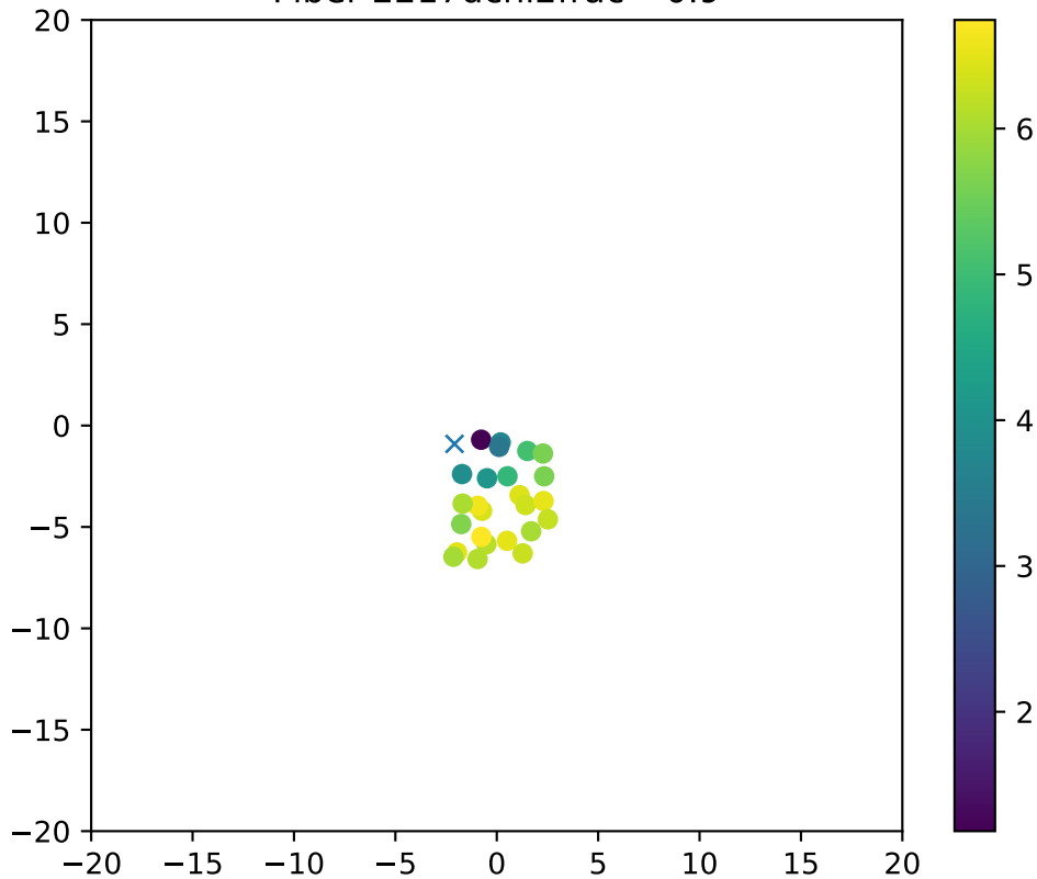
Fiber 2217dchi2frac= 0.9
