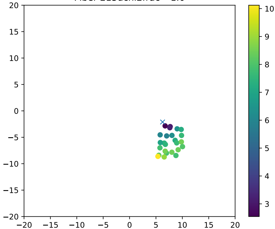
Fiber 213dchi2frac= 1.0
