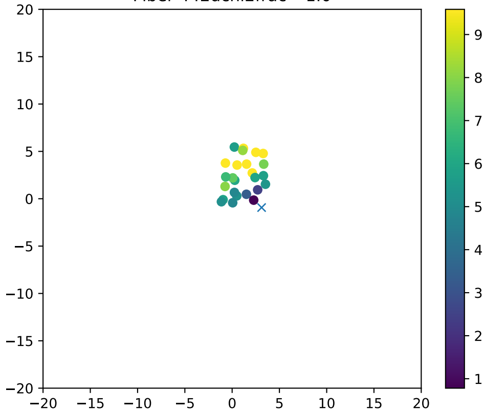
Fiber 442dchi2frac= 1.0
