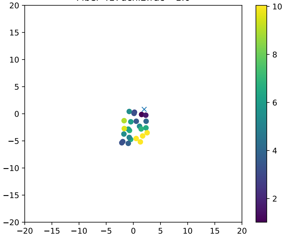
Fiber 417dchi2frac= 1.0
