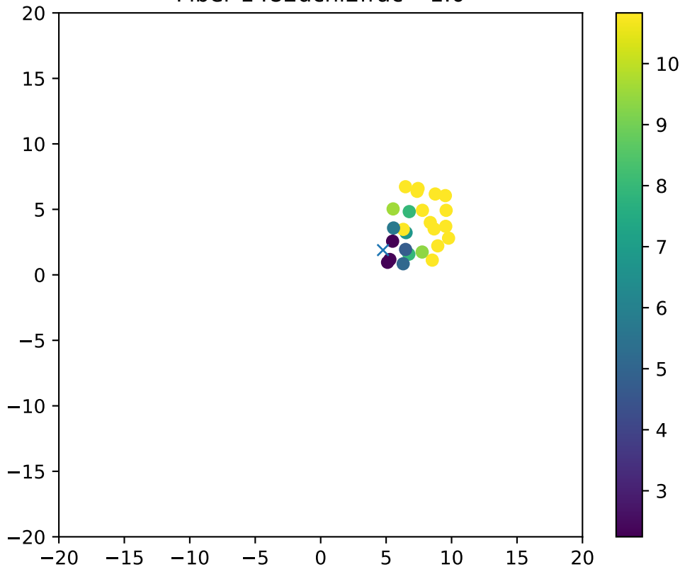
Fiber 1482dchi2frac= 1.0
