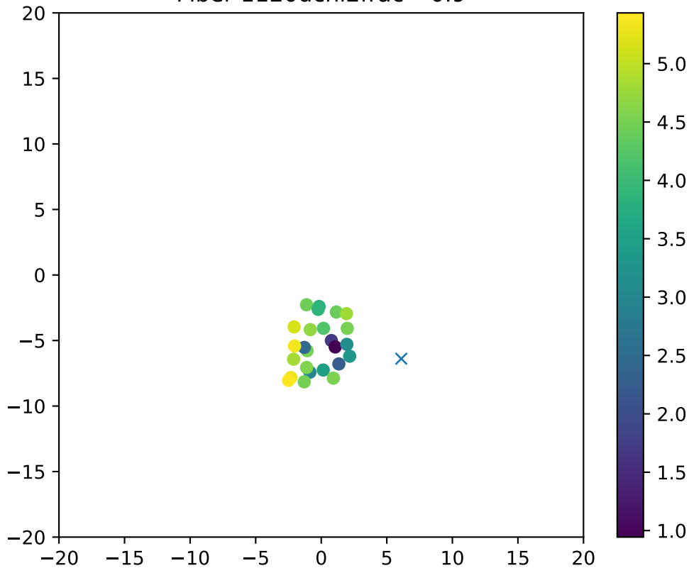
Fiber 1120dchi2frac= 0.9
