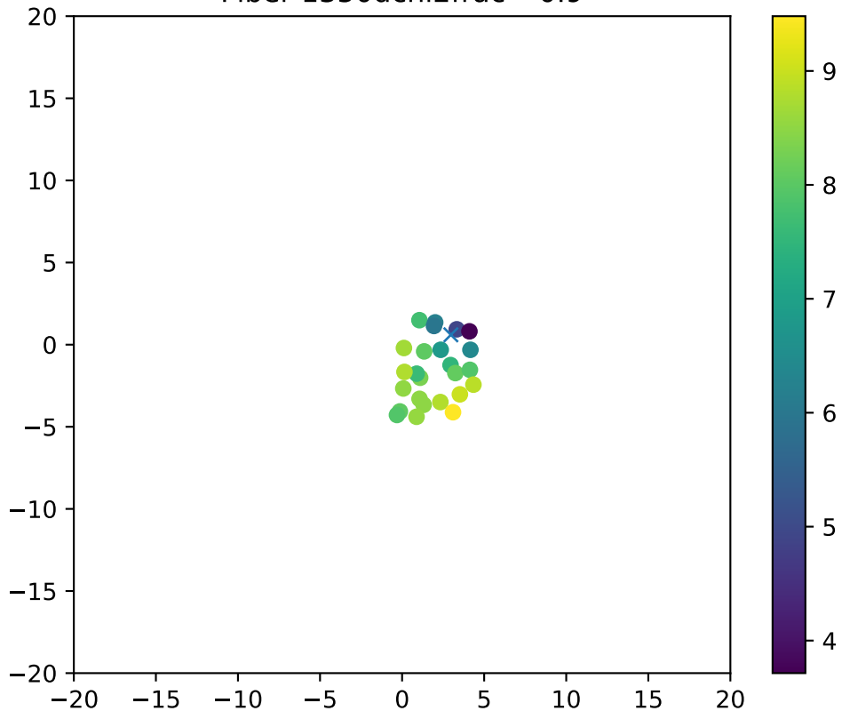
Fiber 1350dchi2frac= 0.9
