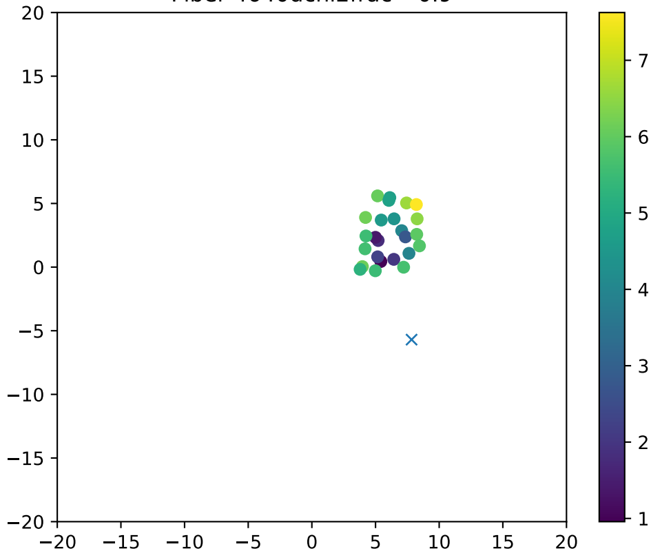
Fiber 4640dchi2frac= 0.9
