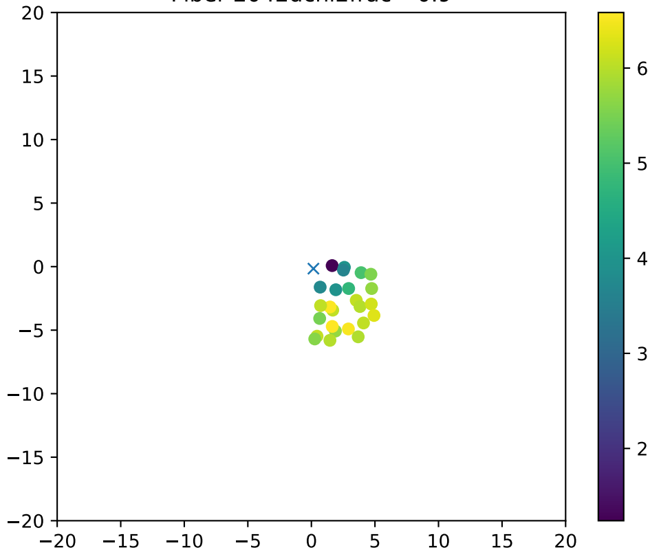
Fiber 2042dchi2frac= 0.9
