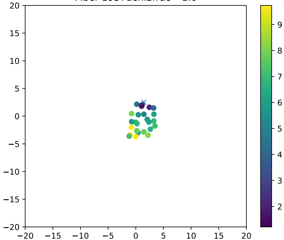
Fiber 1937dchi2frac= 1.0
