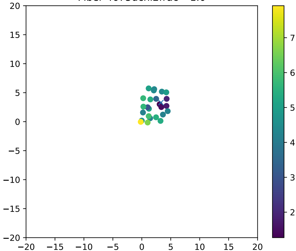
Fiber 4673dchi2frac= 1.0
