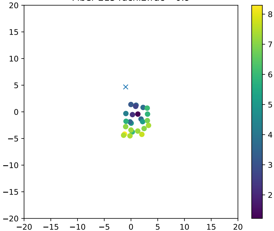
Fiber 2154dchi2frac= 0.9
