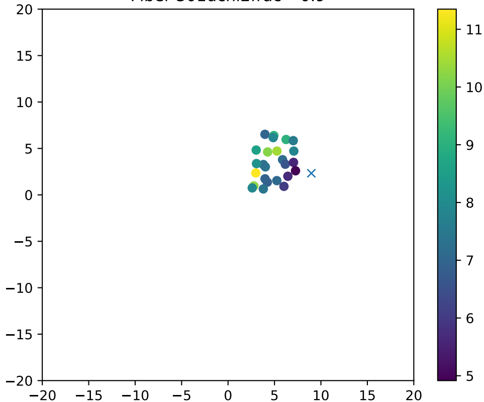
Fiber 301dchi2frac= 0.9
