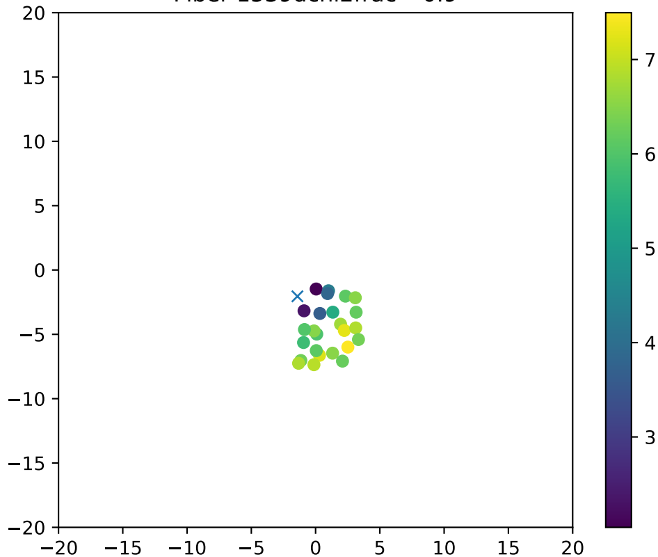
Fiber 1539dchi2frac= 0.9
