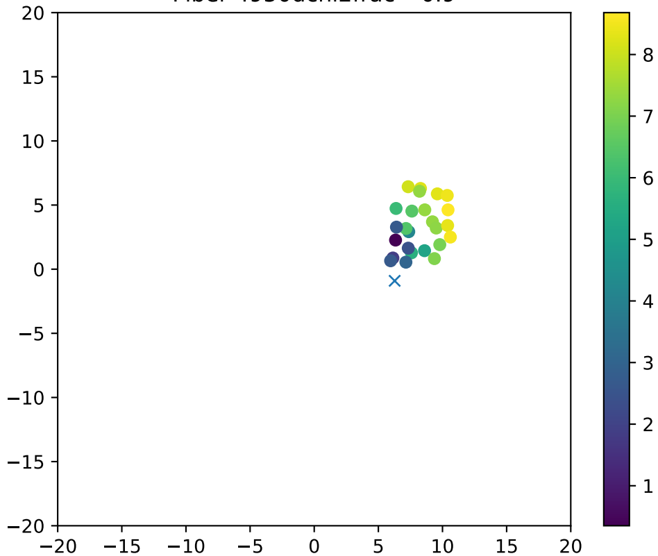
Fiber 4950dchi2frac= 0.9
