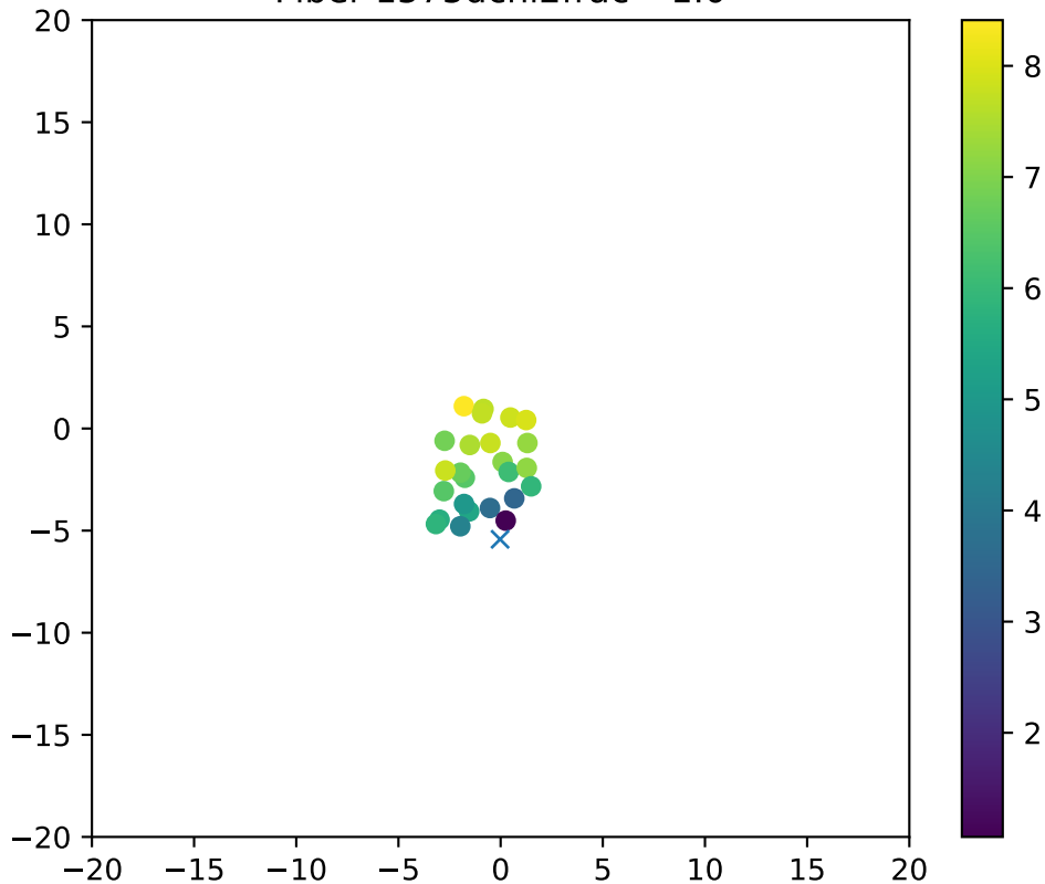
Fiber 1575dchi2frac= 1.0
