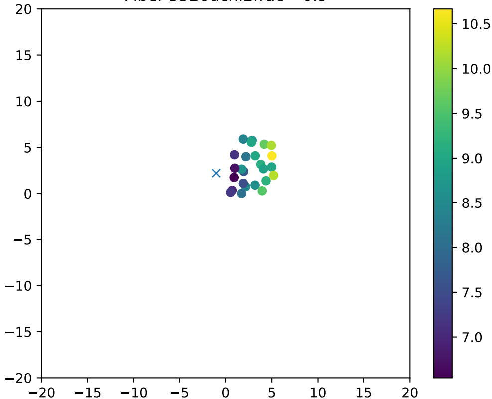
Fiber 3526dchi2frac= 0.9
