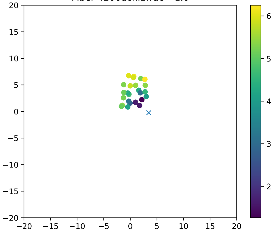
Fiber 4206dchi2frac= 1.0
