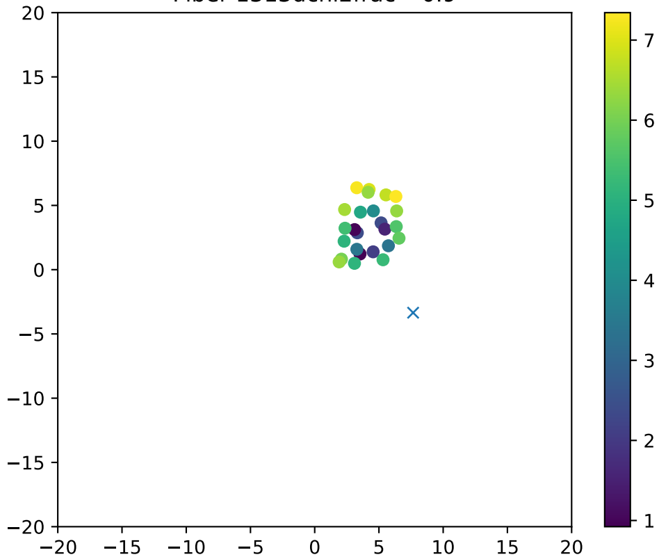
Fiber 1313dchi2frac= 0.9
