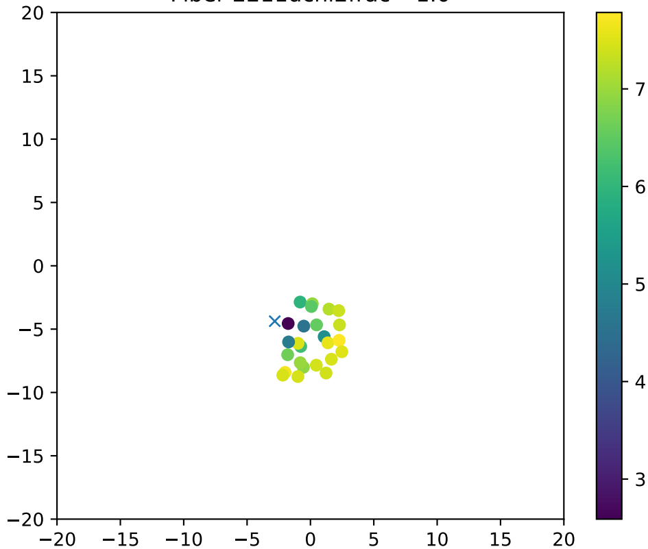
Fiber 2211dchi2frac= 1.0
