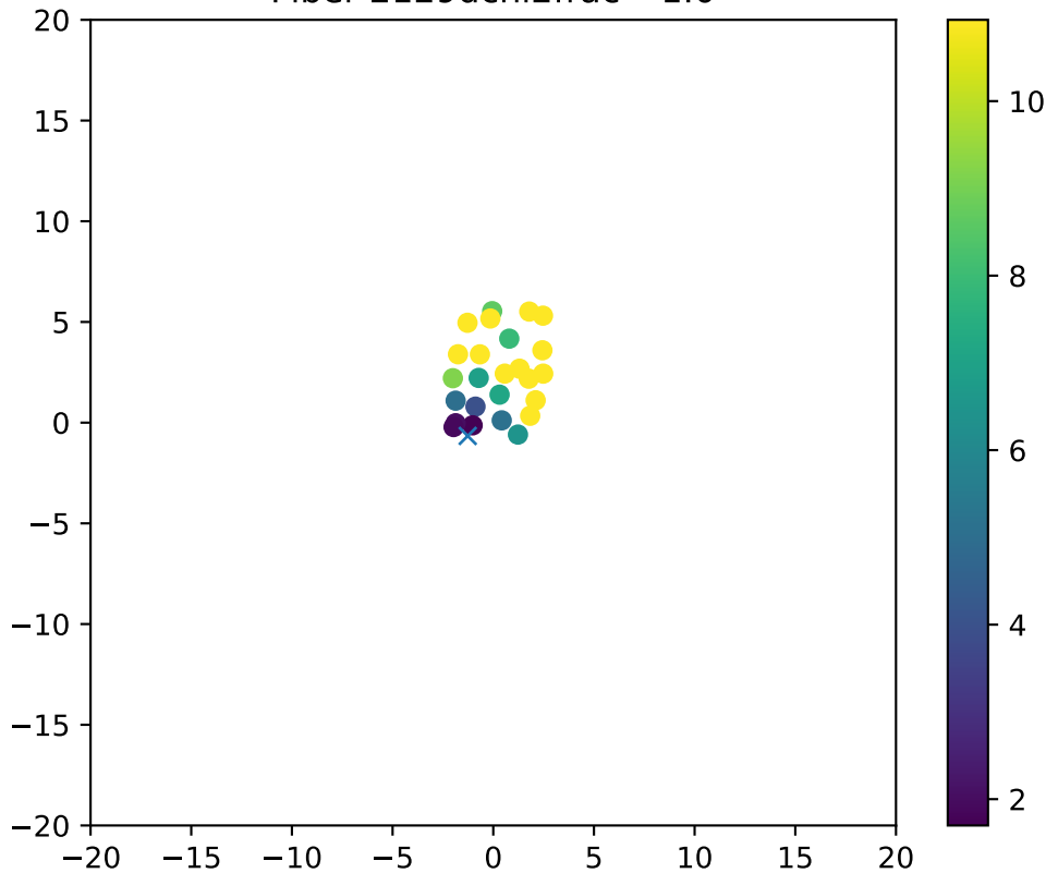
Fiber 2129dchi2frac= 1.0
