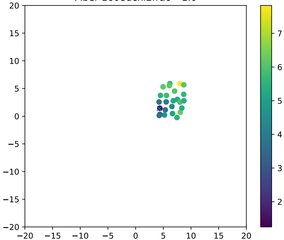
Fiber 1608dchi2frac= 1.0
