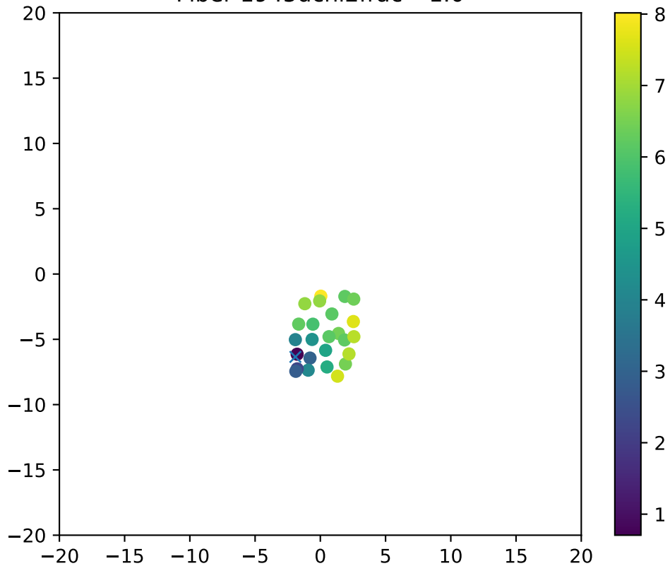
Fiber 1945dchi2frac= 1.0
