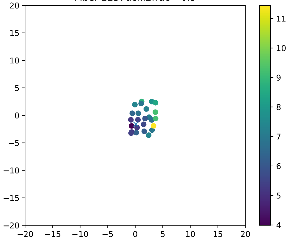
Fiber 2257dchi2frac= 0.9
