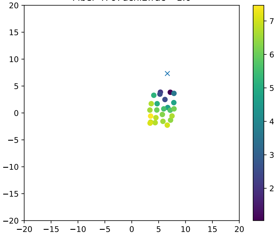
Fiber 4767dchi2frac= 1.0
