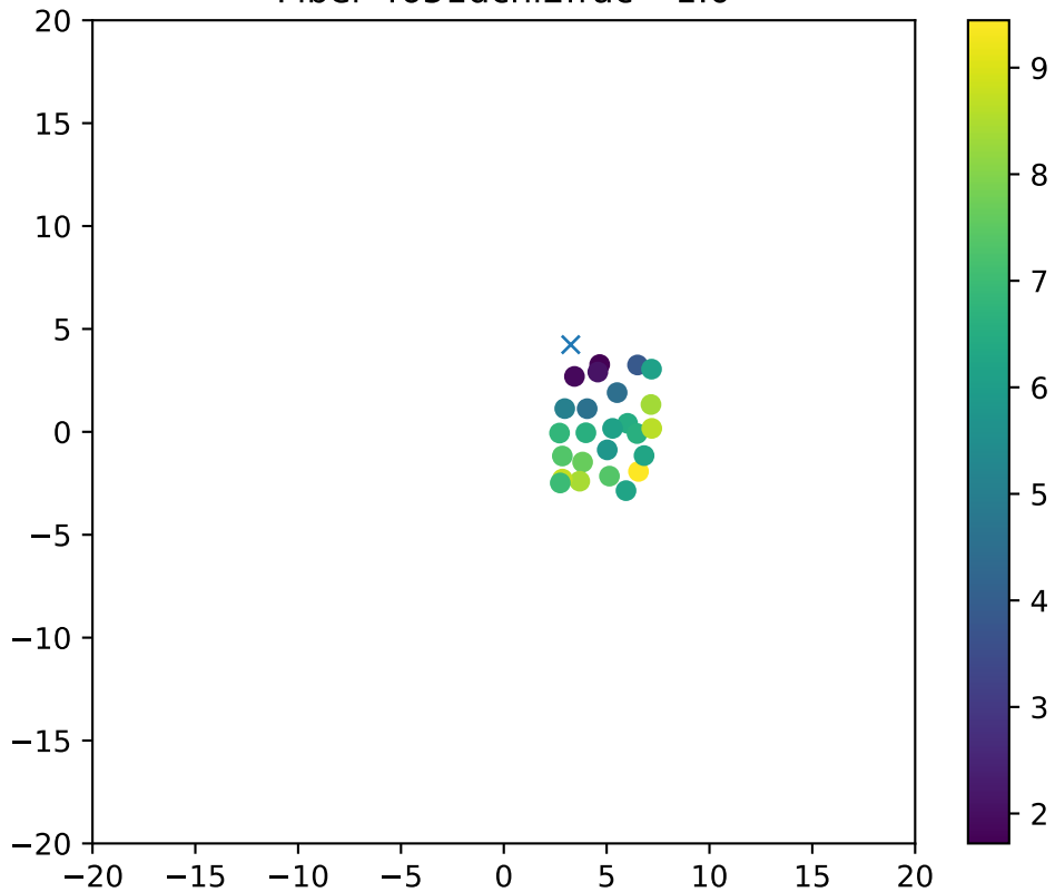
Fiber 4651dchi2frac= 1.0
