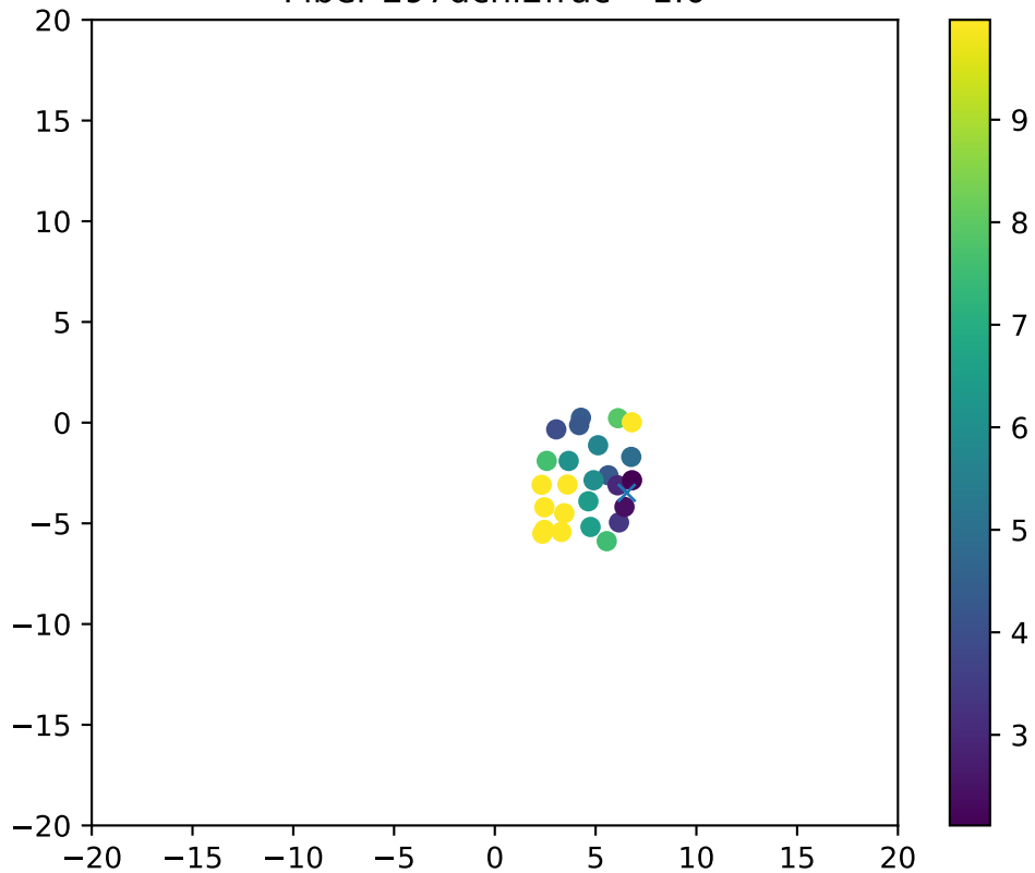
Fiber 297dchi2frac= 1.0
