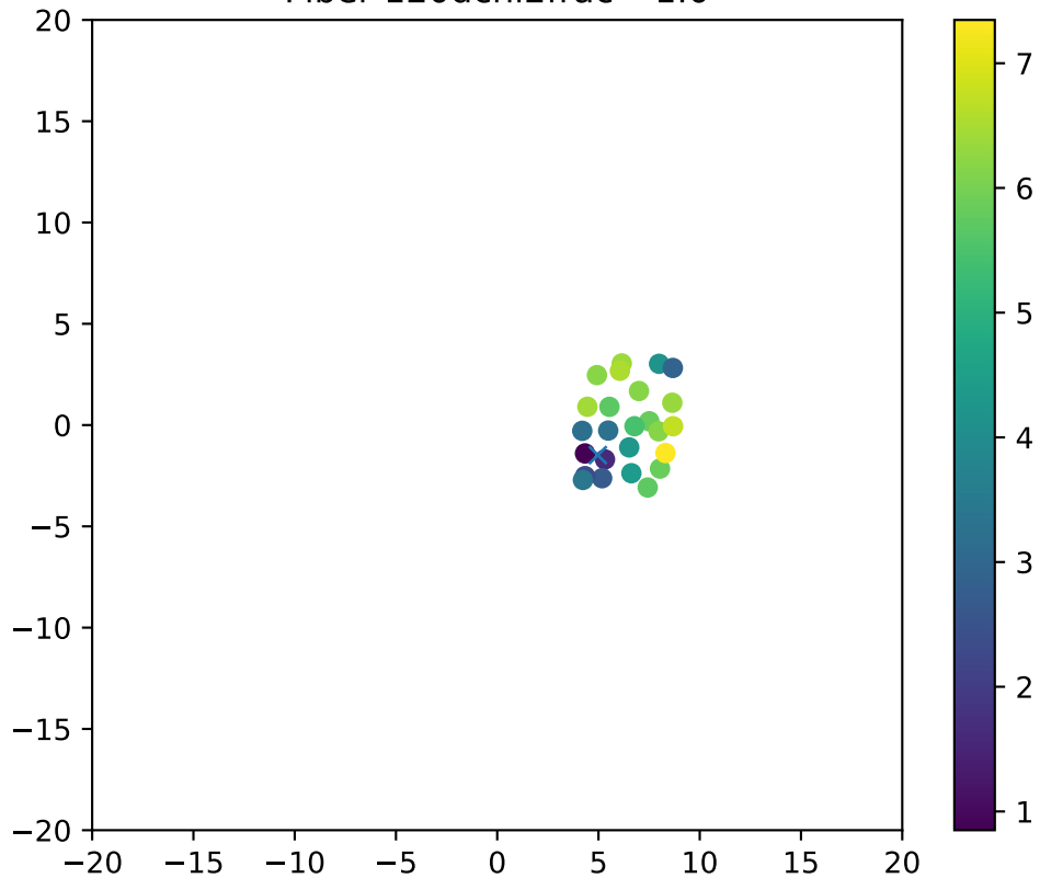
Fiber 120dchi2frac= 1.0
