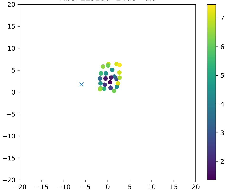
Fiber 2251dchi2frac= 0.9
