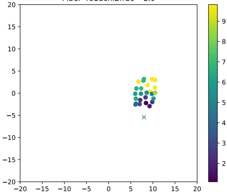
Fiber 461dchi2frac= 1.0
