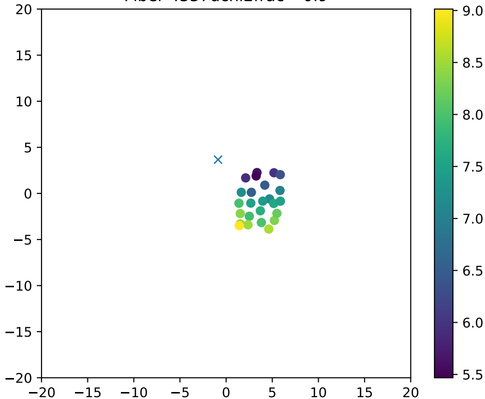
Fiber 4337dchi2frac= 0.9
