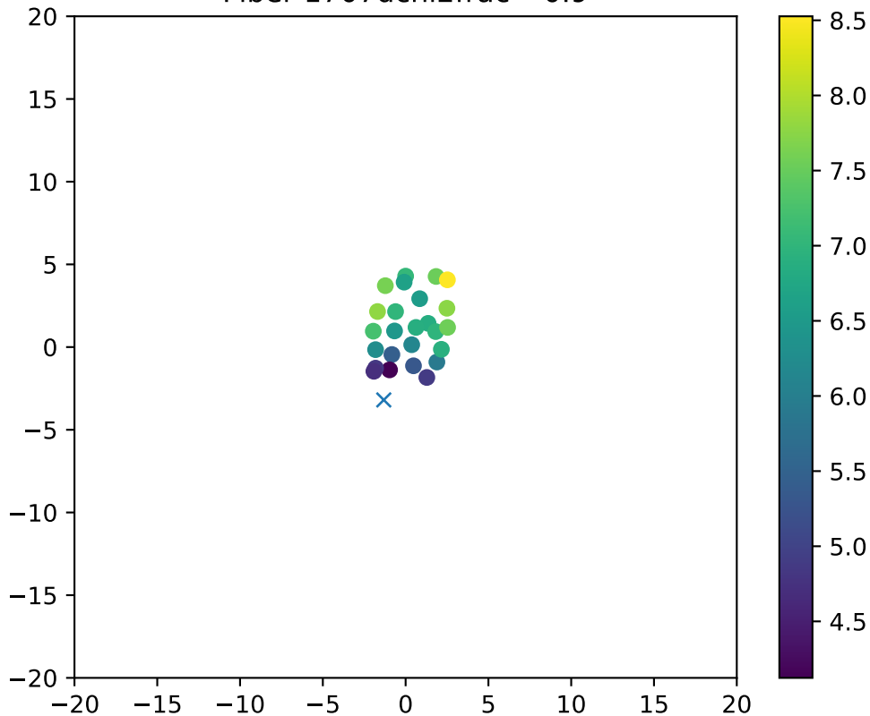
Fiber 1707dchi2frac= 0.9
