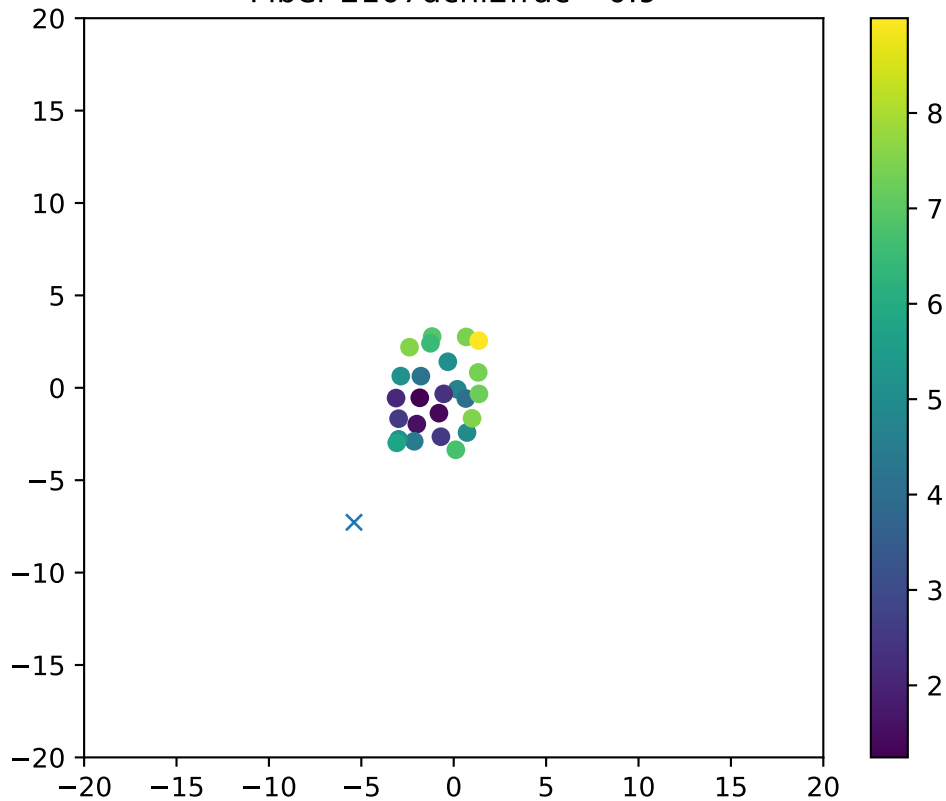
Fiber 2107dchi2frac= 0.9
