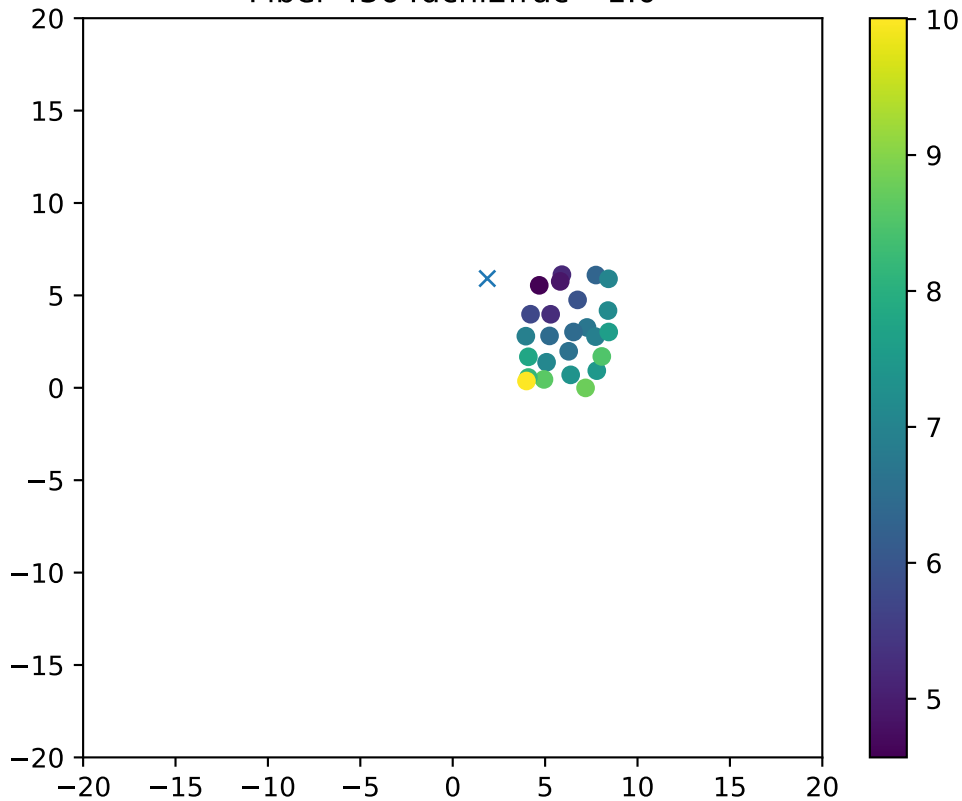
Fiber 4364dchi2frac= 1.0
