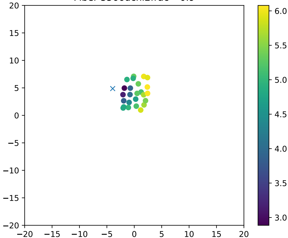
Fiber 3566dchi2frac= 0.9
