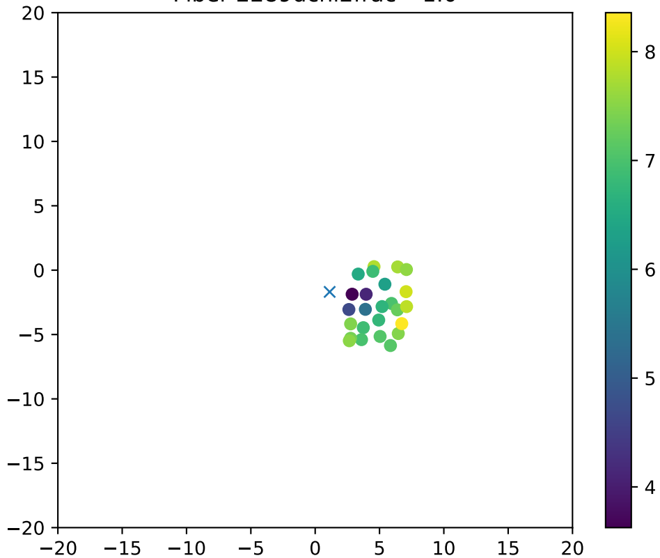
Fiber 2289dchi2frac= 1.0
