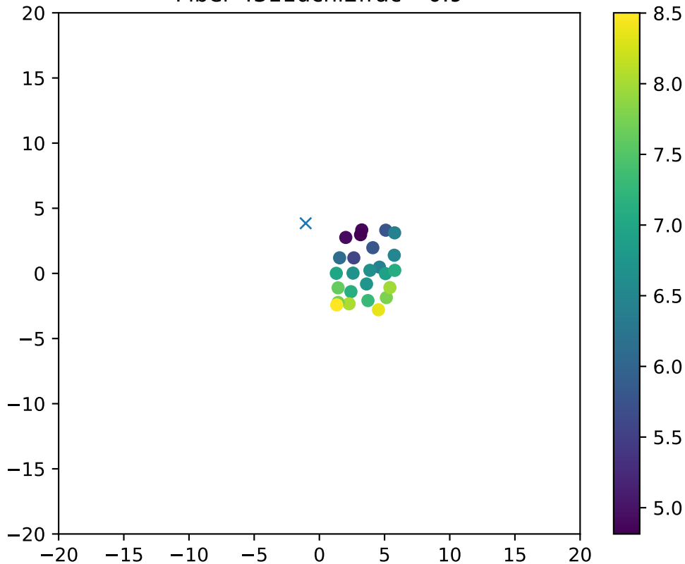
Fiber 4311dchi2frac= 0.9
