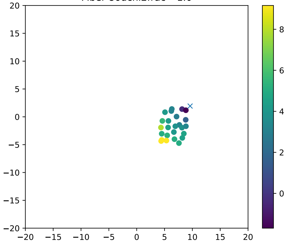
Fiber 86dchi2frac= 1.0
