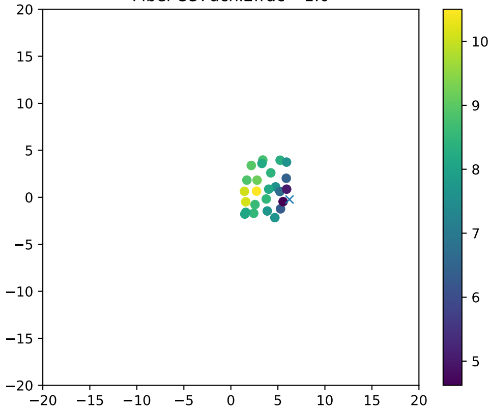
Fiber 337dchi2frac= 1.0
