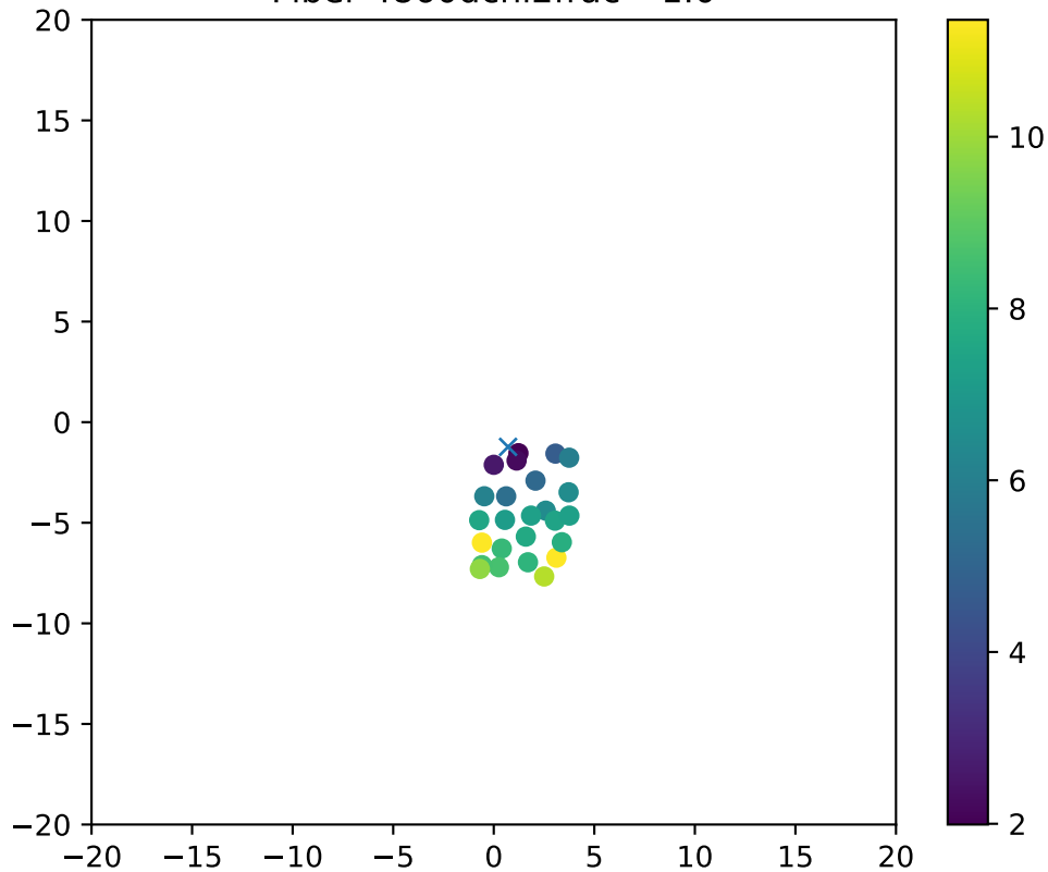
Fiber 4860dchi2frac= 1.0
