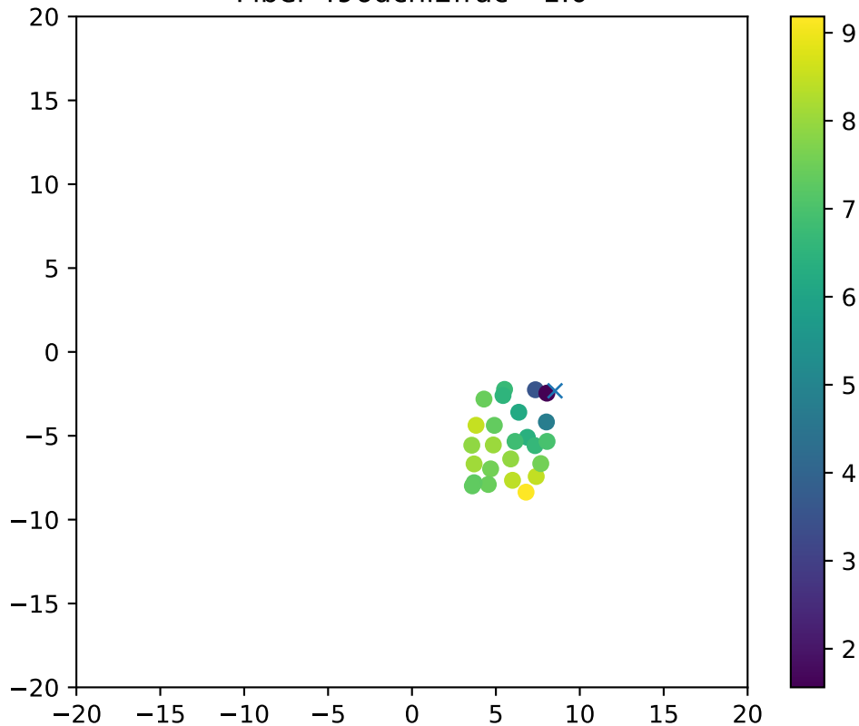
Fiber 496dchi2frac= 1.0
