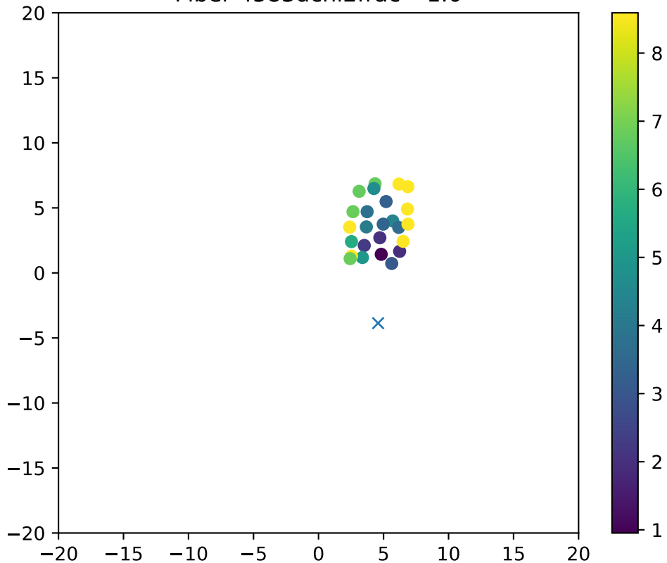
Fiber 4583dchi2frac= 1.0
