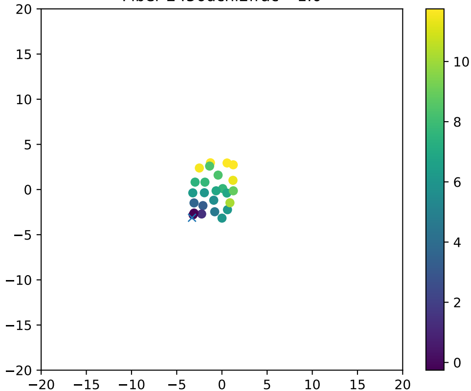
Fiber 2456dchi2frac= 1.0
