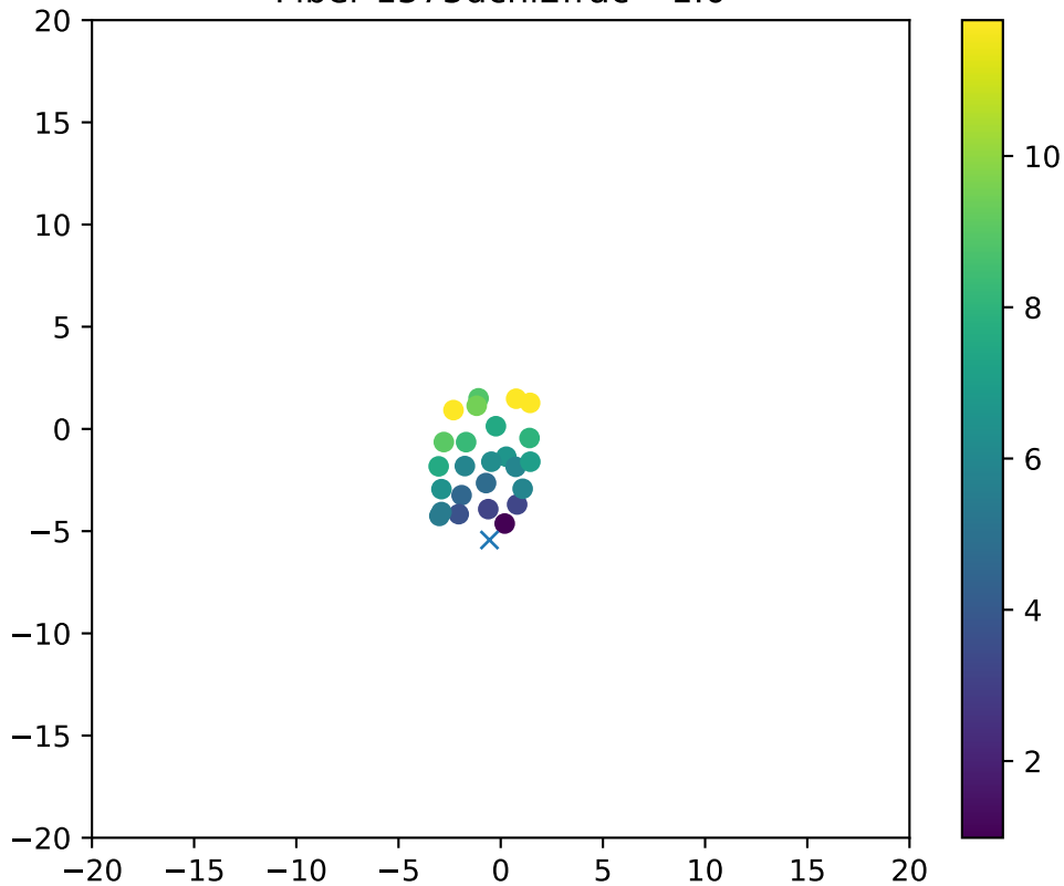
Fiber 1575dchi2frac= 1.0
