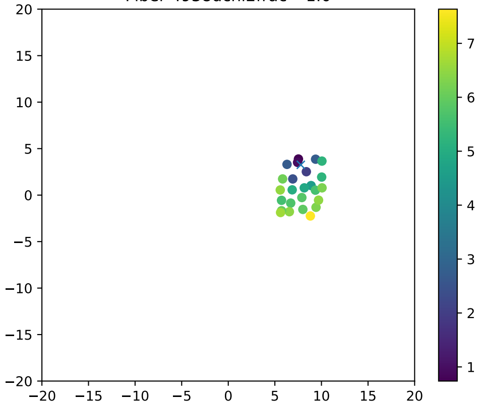
Fiber 4938dchi2frac= 1.0
