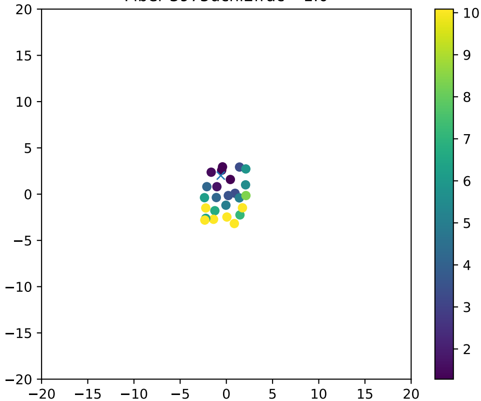
Fiber 3975dchi2frac= 1.0
