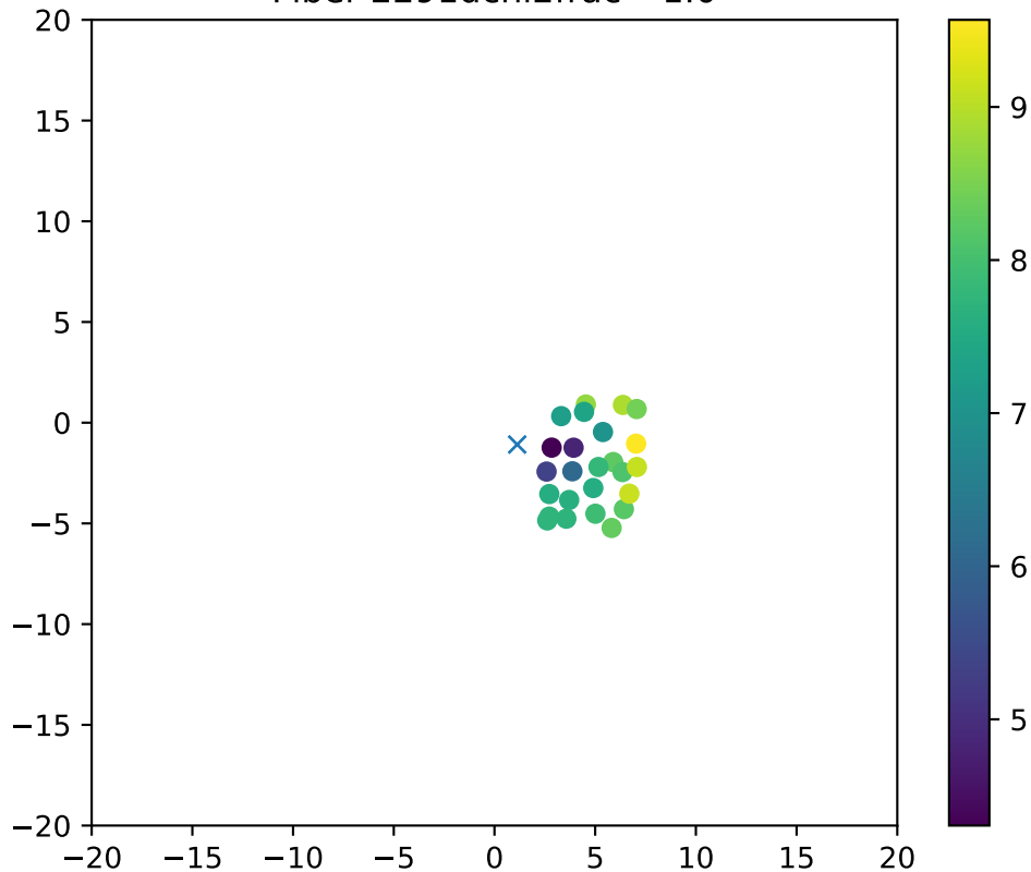
Fiber 2291dchi2frac= 1.0
