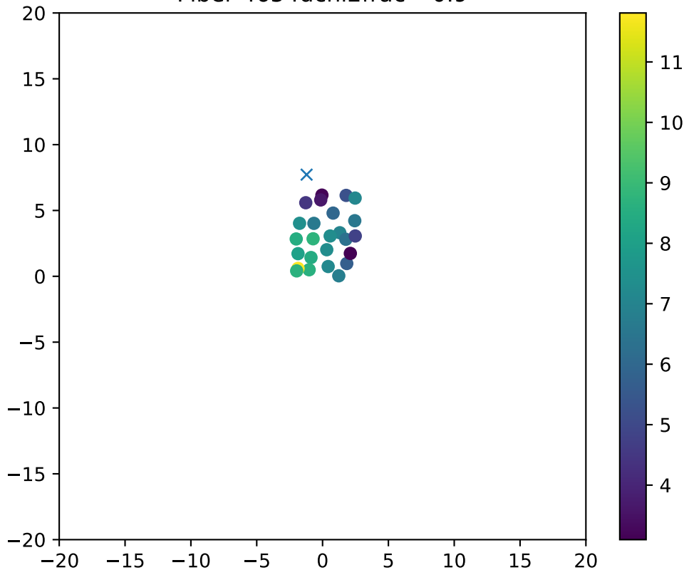
Fiber 4654dchi2frac= 0.9
