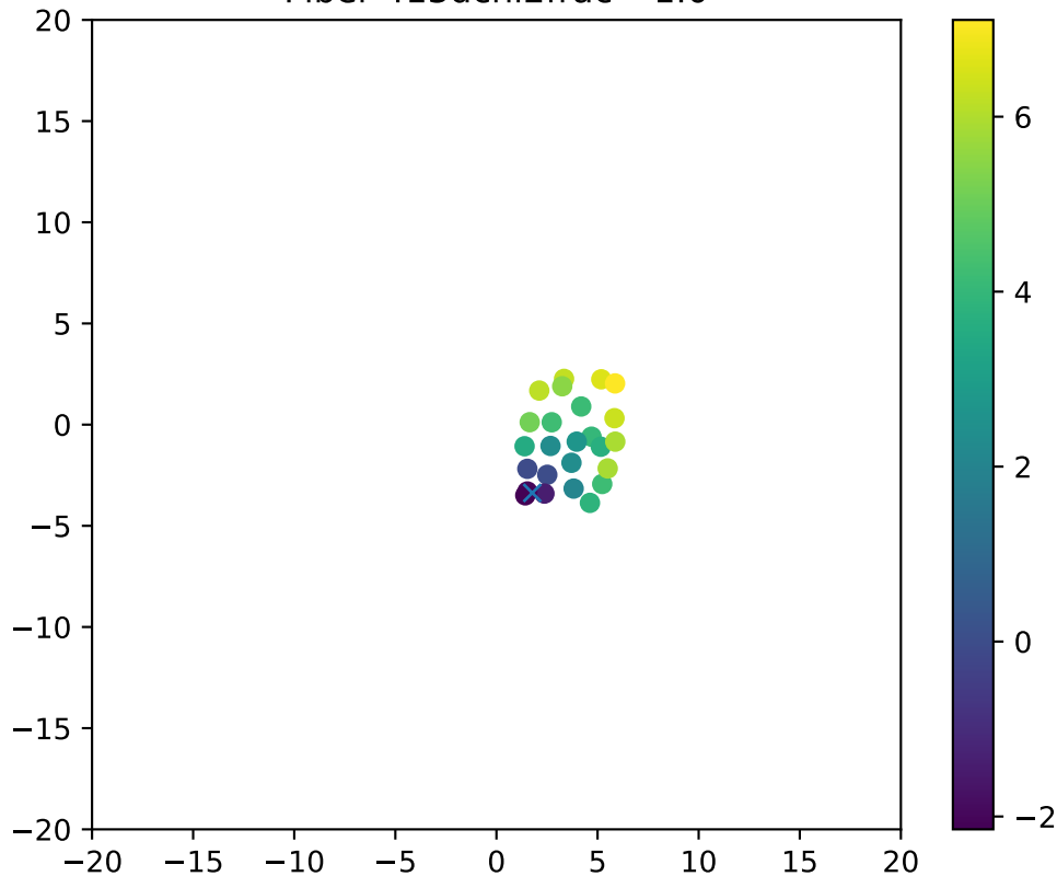
Fiber 413dchi2frac= 1.0
