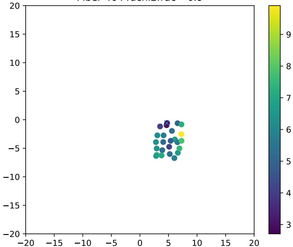
Fiber 4644dchi2frac= 0.9
