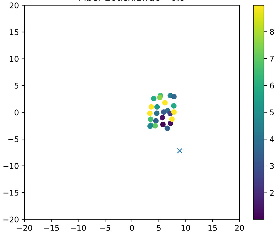
Fiber 20dchi2frac= 0.9
