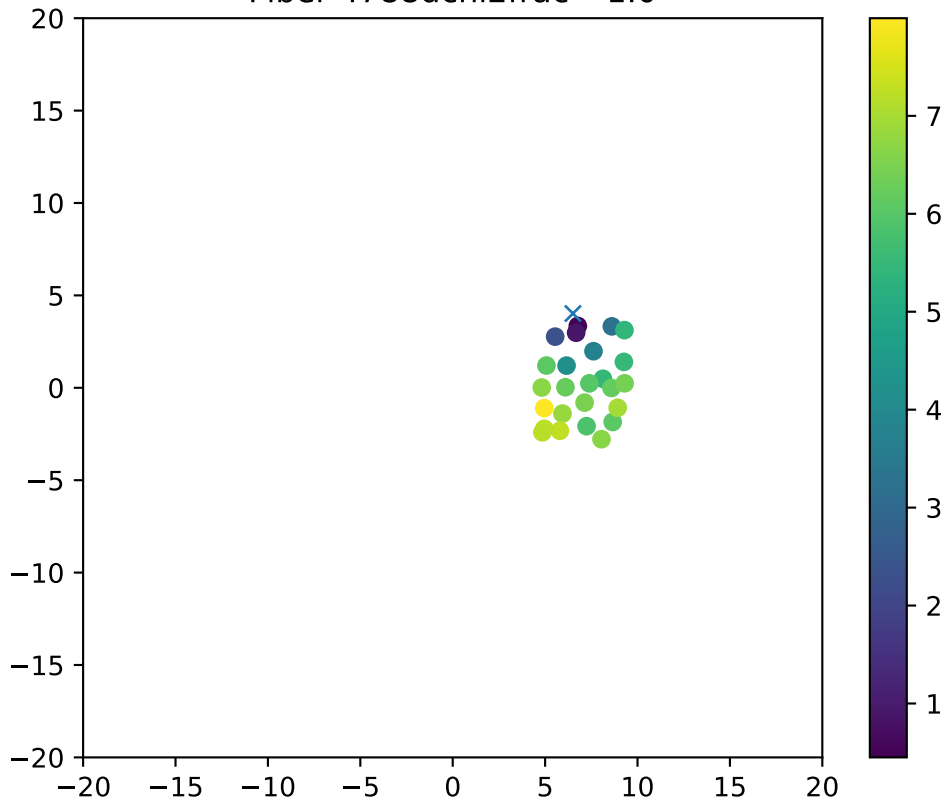
Fiber 4788dchi2frac= 1.0
