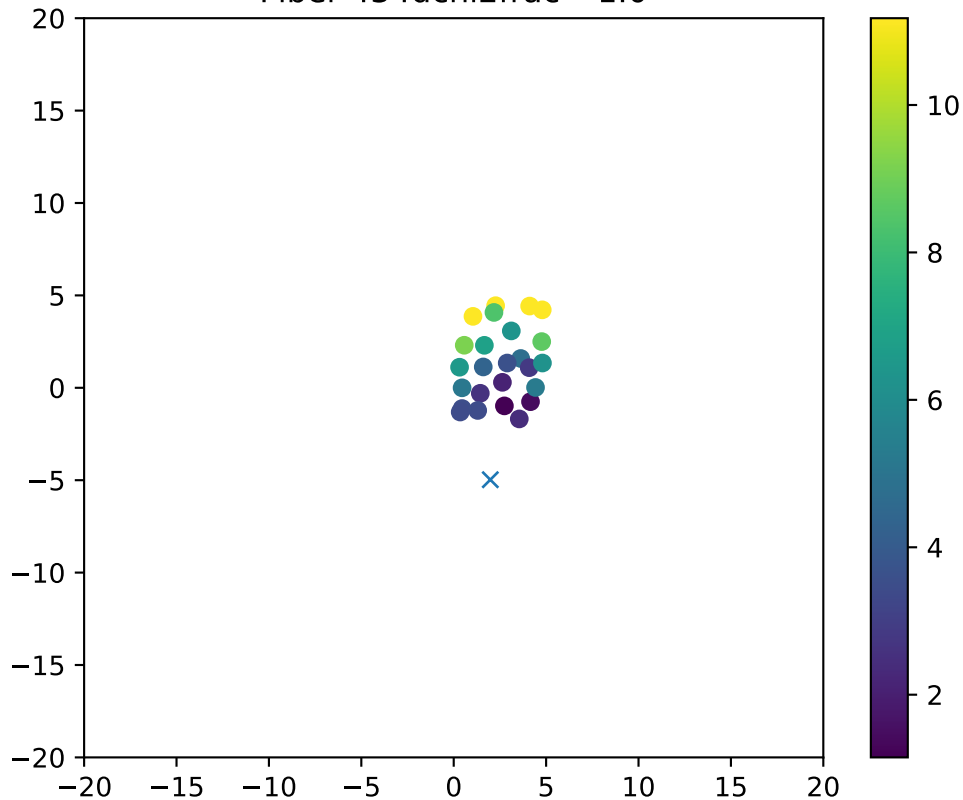
Fiber 434dchi2frac= 1.0
