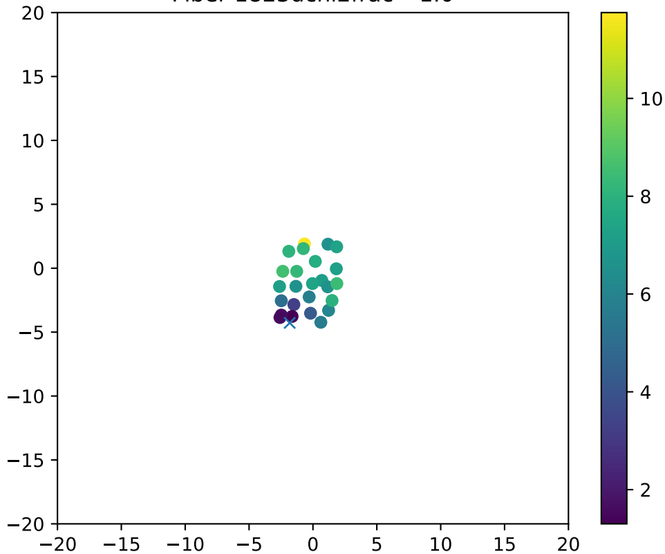
Fiber 1823dchi2frac= 1.0
