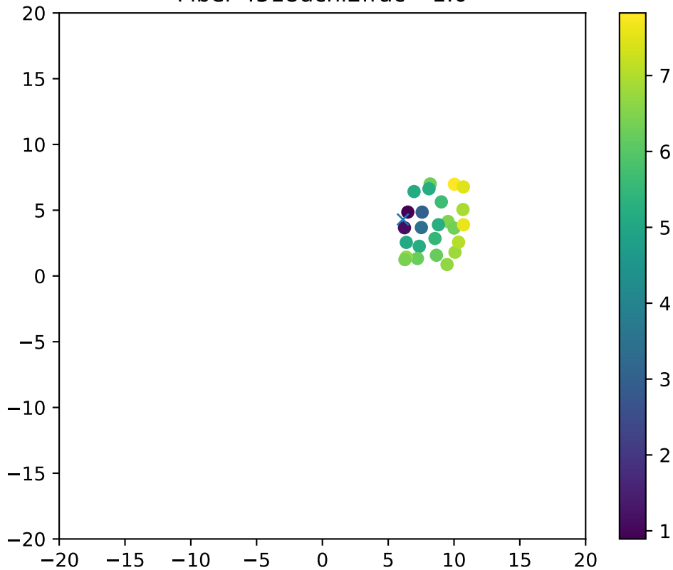
Fiber 4518dchi2frac= 1.0
