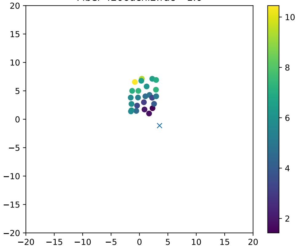
Fiber 4206dchi2frac= 1.0
