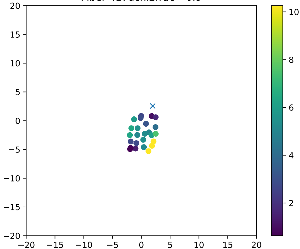
Fiber 417dchi2frac= 0.9
