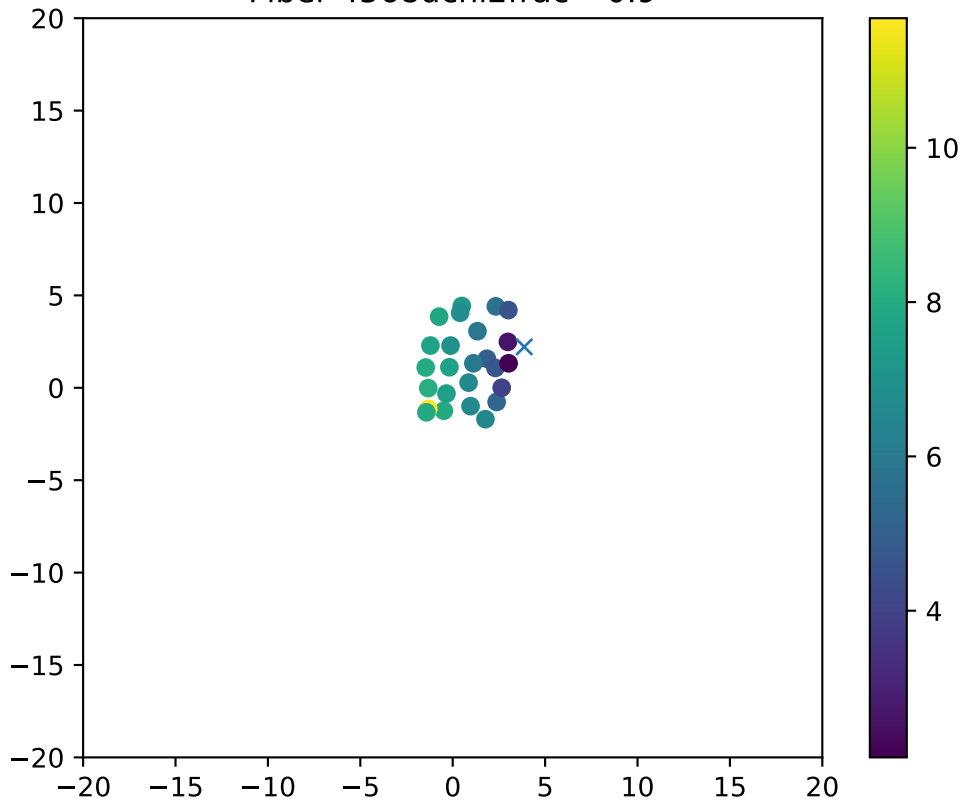
Fiber 4568dchi2frac= 0.9
