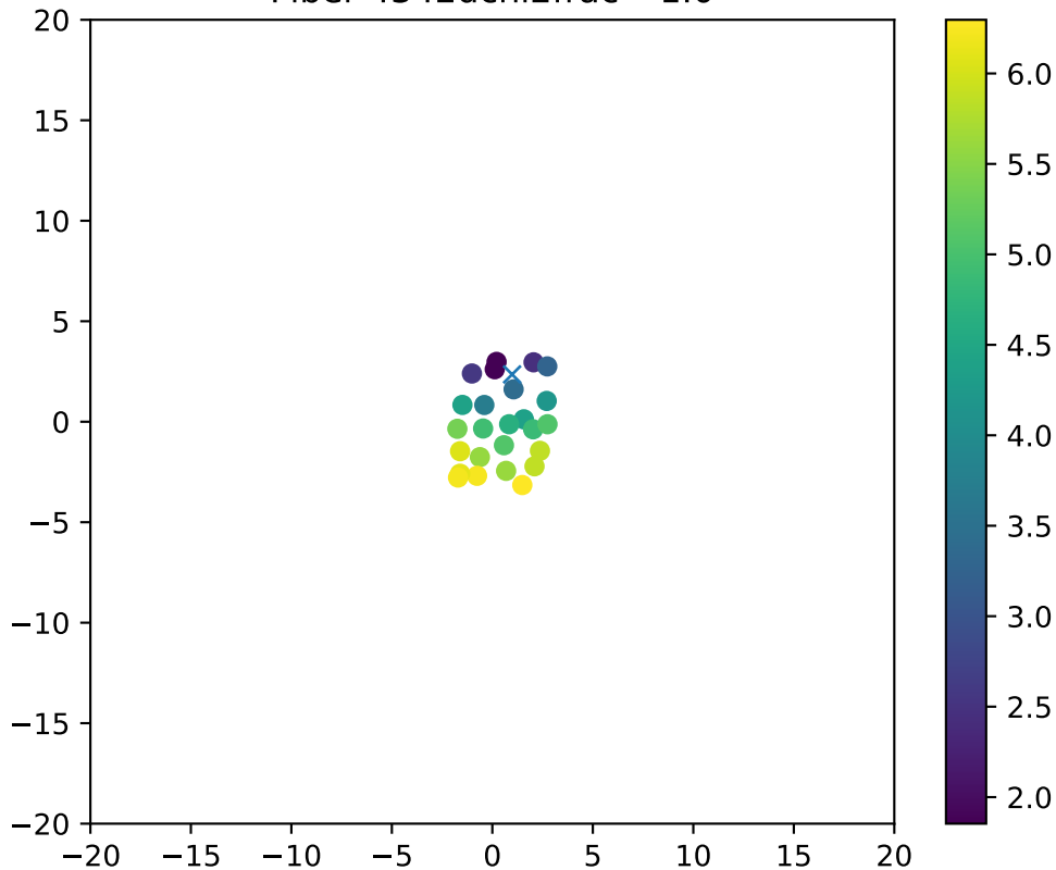
Fiber 4342dchi2frac= 1.0
