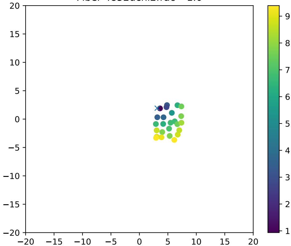
Fiber 4852dchi2frac= 1.0
