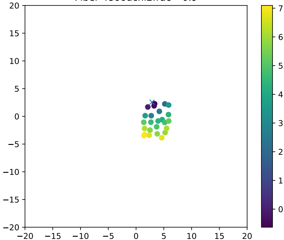
Fiber 4866dchi2frac= 0.9
