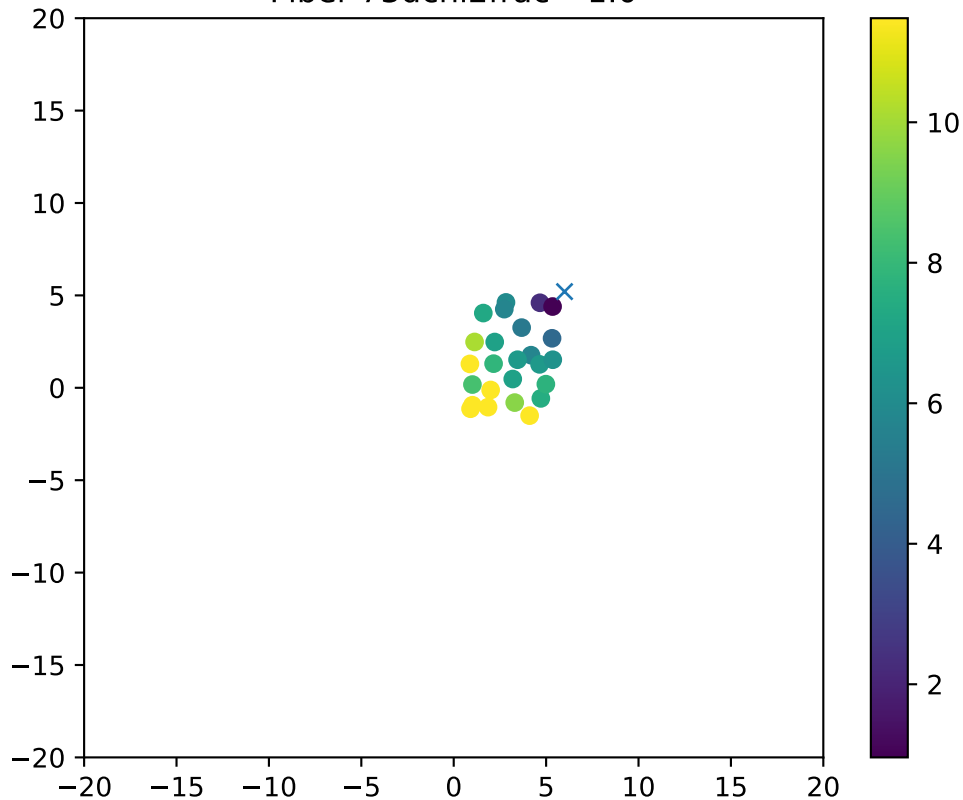
Fiber 73dchi2frac= 1.0
