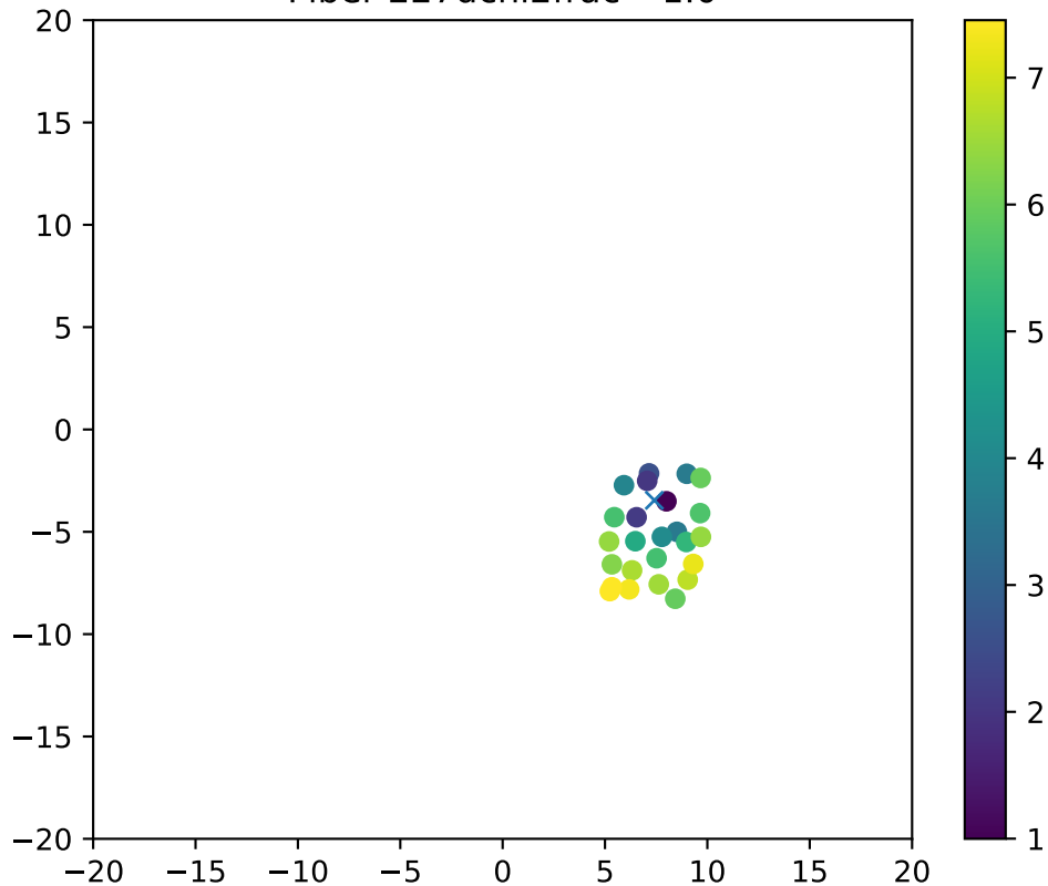
Fiber 227dchi2frac= 1.0
