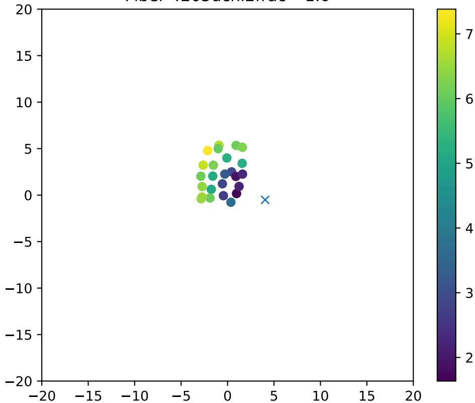
Fiber 4205dchi2frac= 1.0
