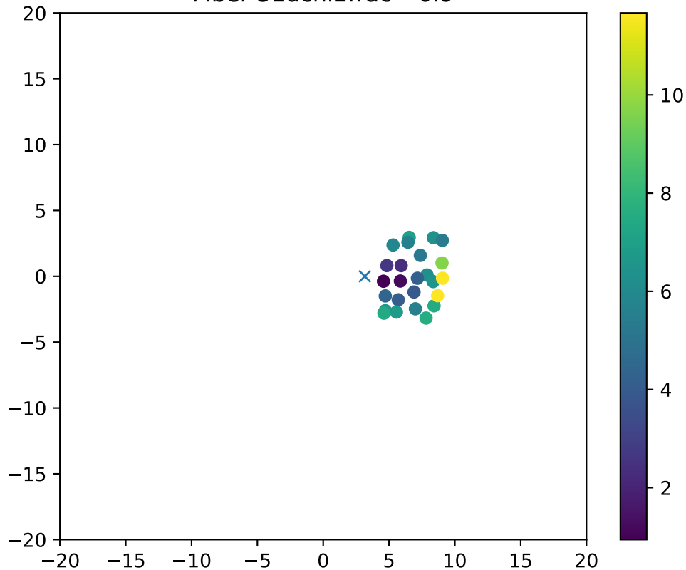
Fiber 31dchi2frac= 0.9
