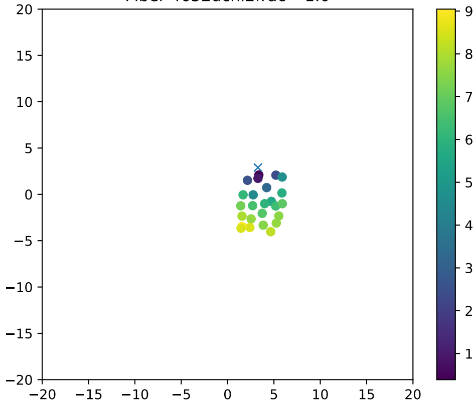
Fiber 4652dchi2frac= 1.0
