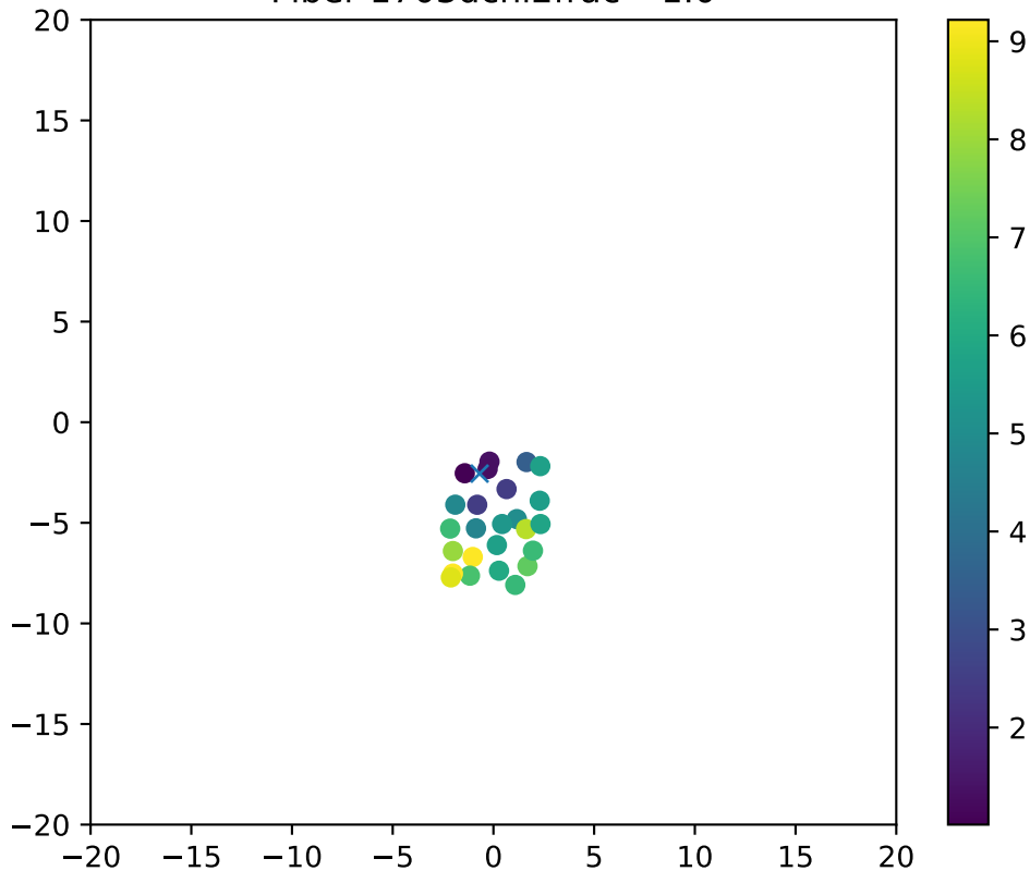
Fiber 1703dchi2frac= 1.0
