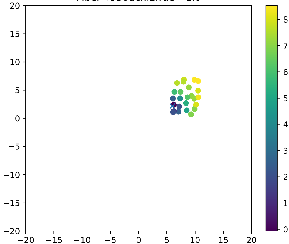
Fiber 4950dchi2frac= 1.0
