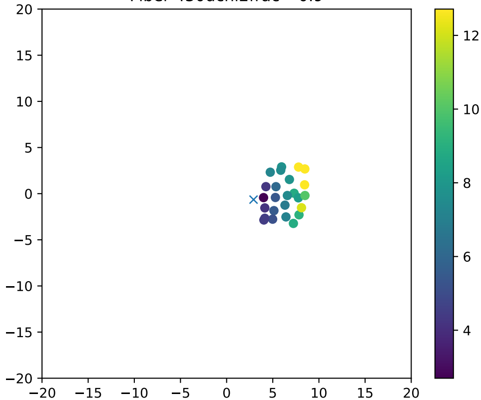
Fiber 430dchi2frac= 0.9
