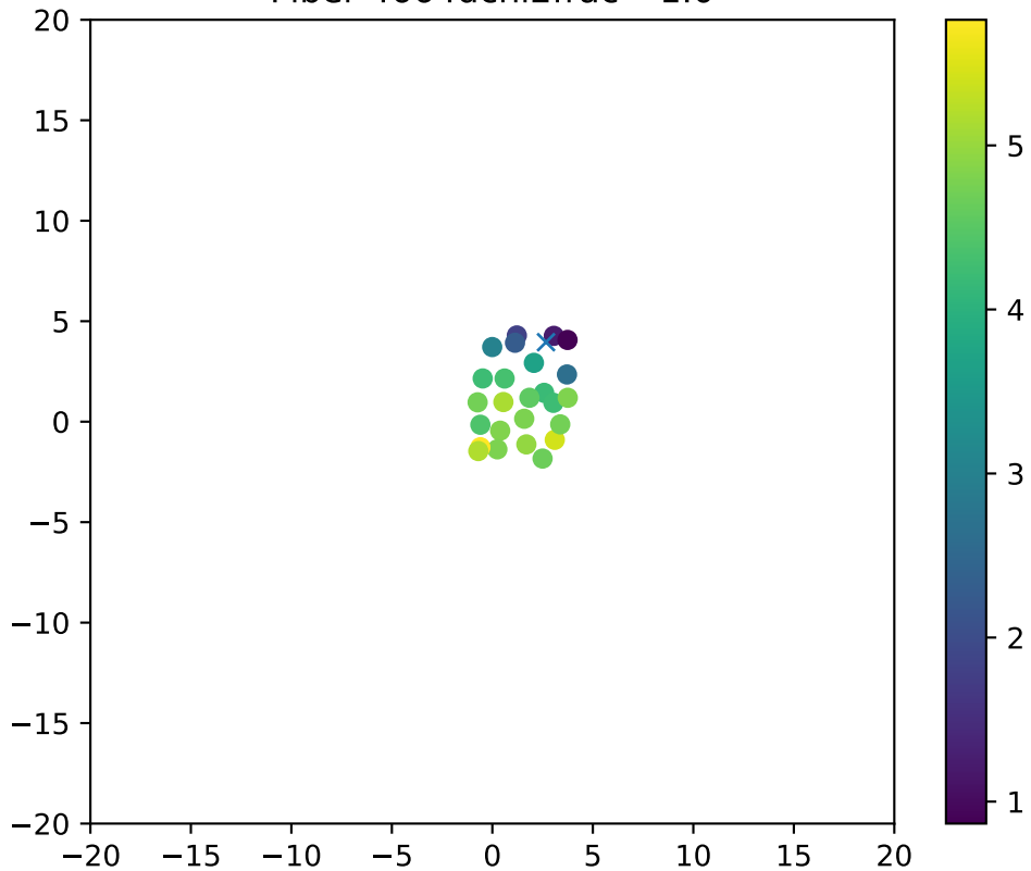
Fiber 4664dchi2frac= 1.0
