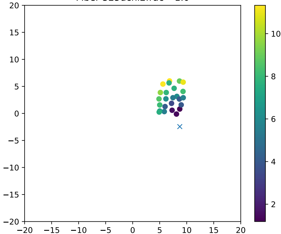
Fiber 325dchi2frac= 1.0
