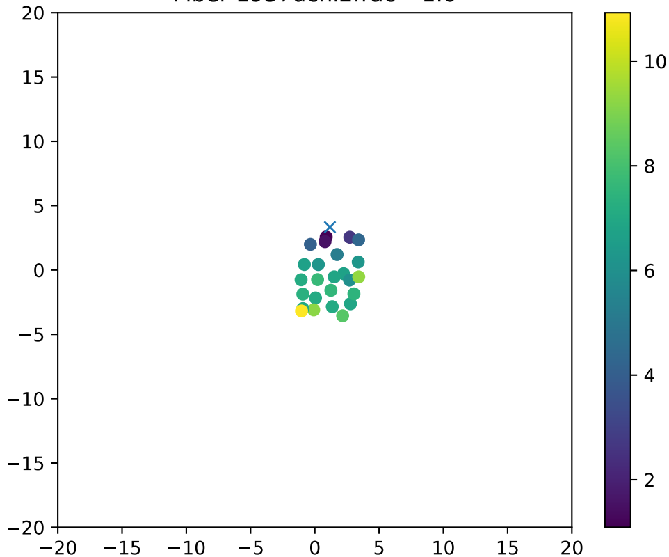
Fiber 1937dchi2frac= 1.0
