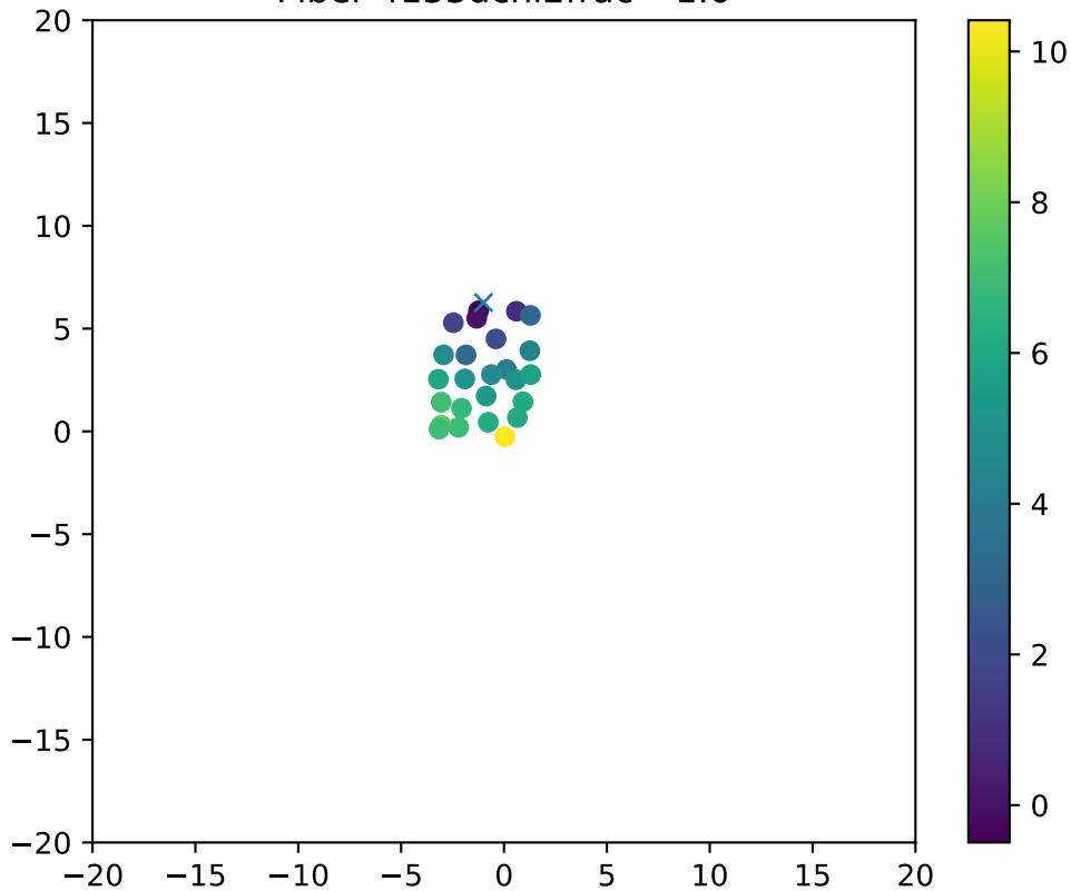
Fiber 4153dchi2frac= 1.0
