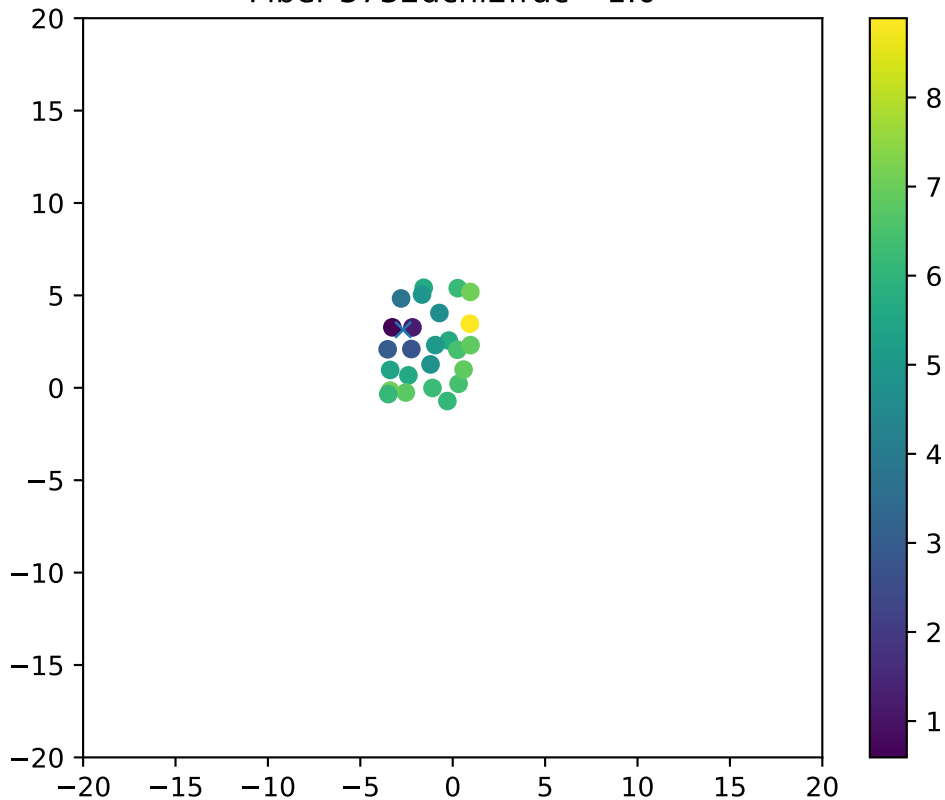
Fiber 3732dchi2frac= 1.0
