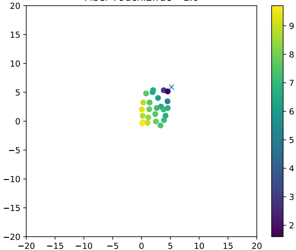
Fiber 79dchi2frac= 1.0
