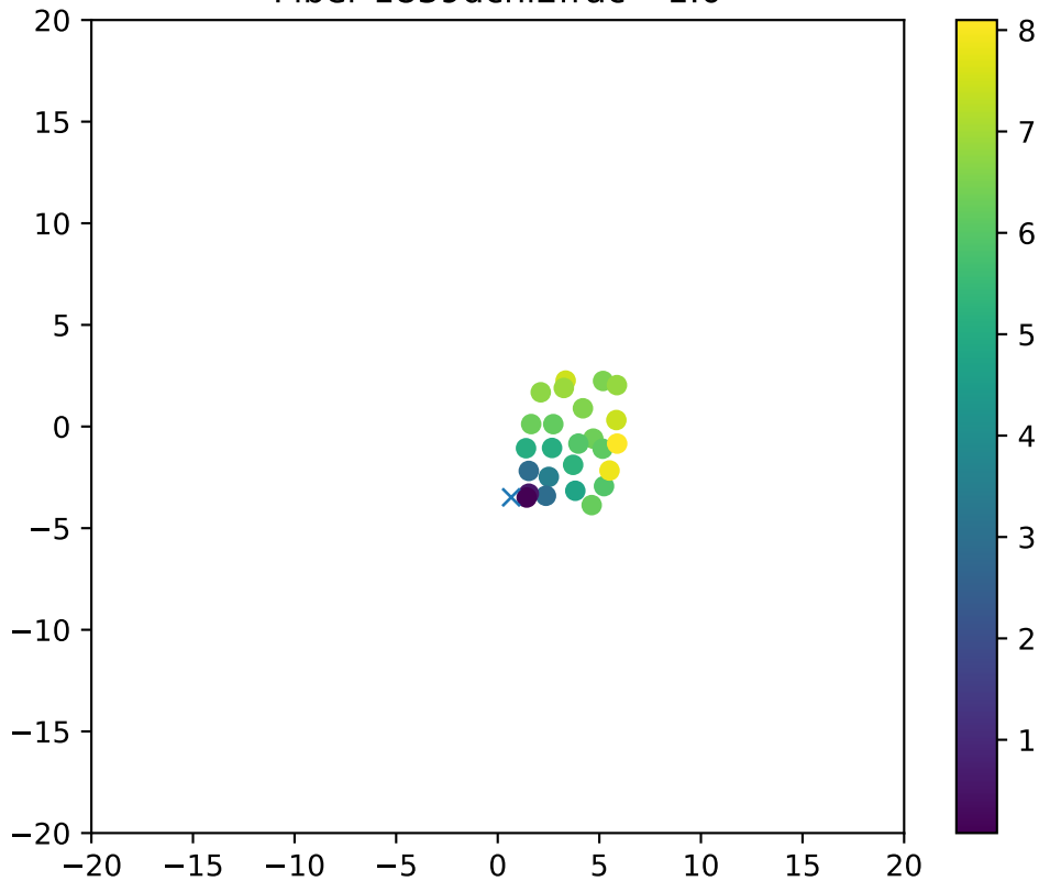
Fiber 1839dchi2frac= 1.0
