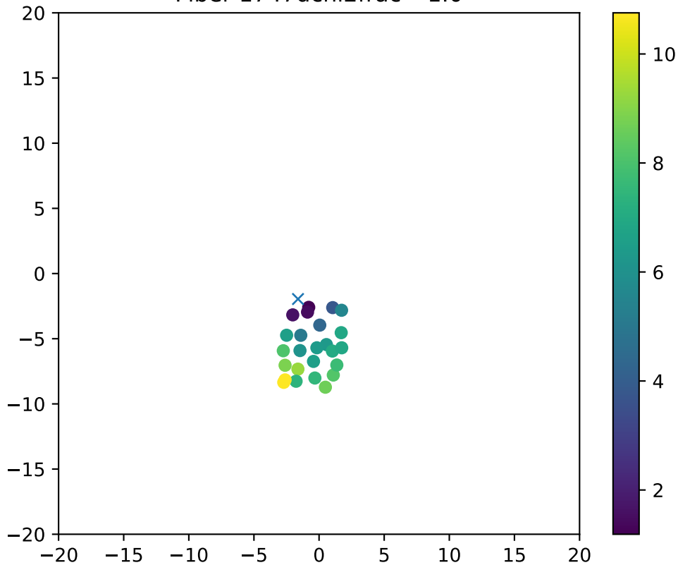
Fiber 1747dchi2frac= 1.0
