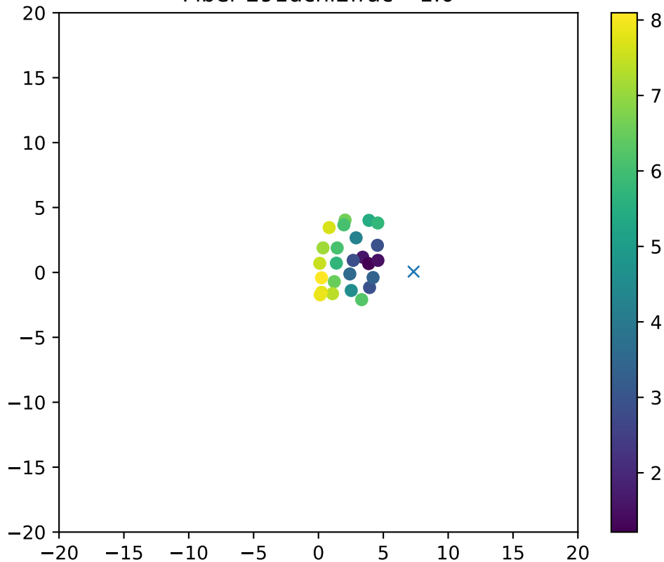
Fiber 291dchi2frac= 1.0
