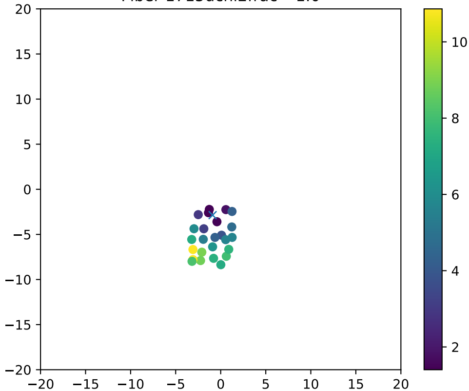
Fiber 1715dchi2frac= 1.0
