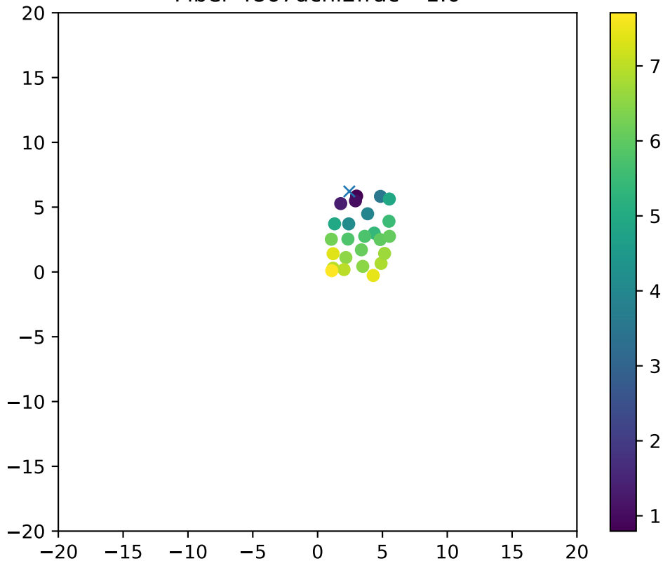
Fiber 4867dchi2frac= 1.0
