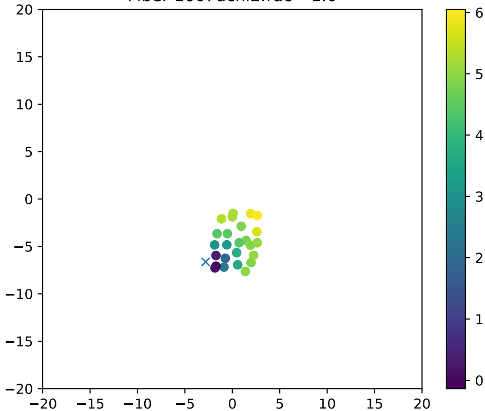
Fiber 1667dchi2frac= 1.0
