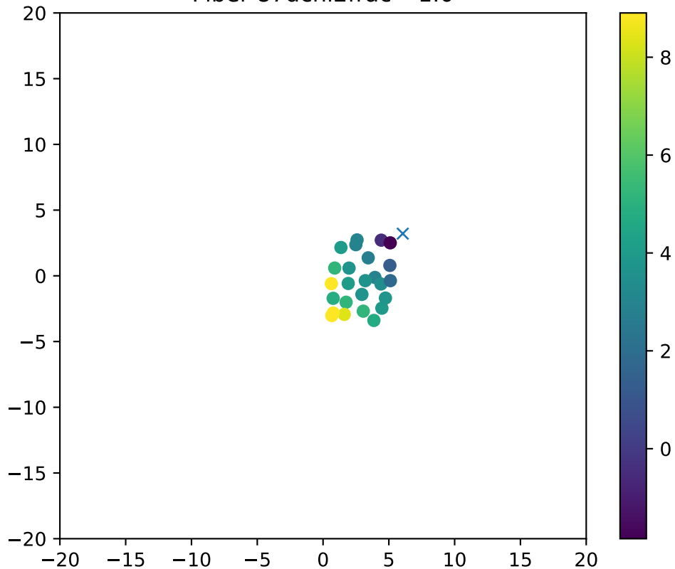
Fiber 87dchi2frac= 1.0
