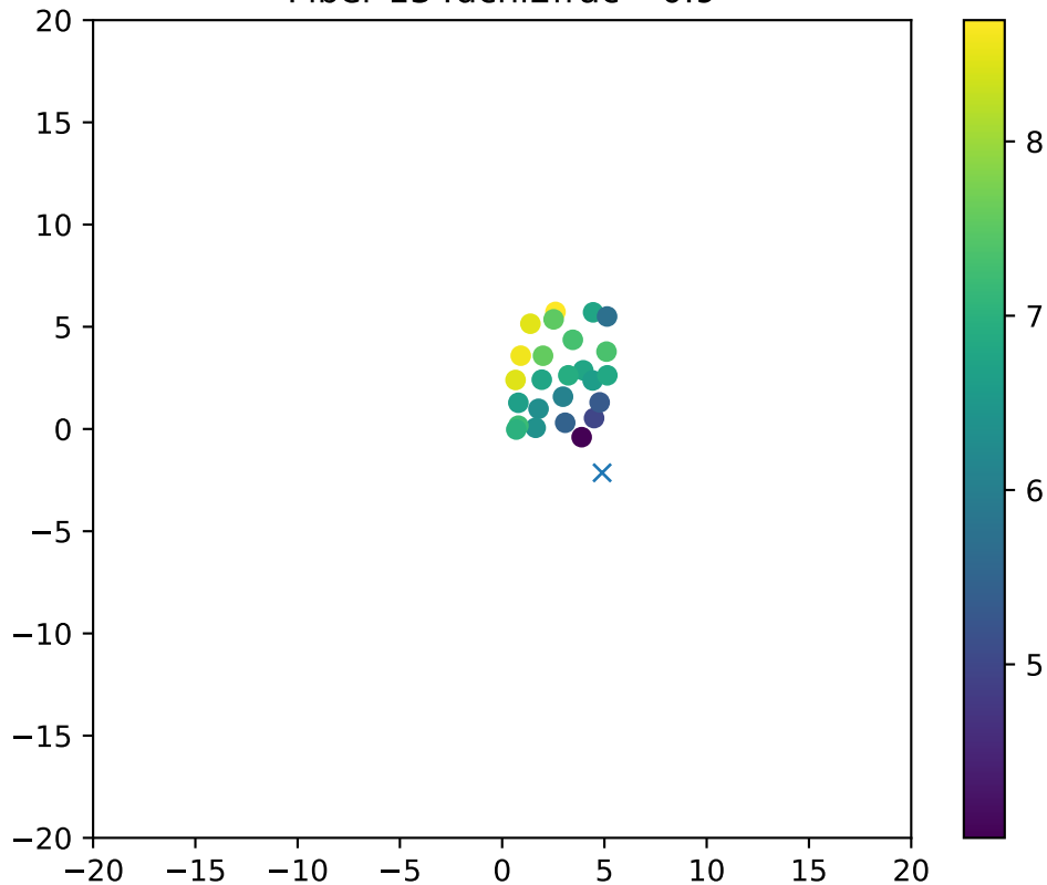
Fiber 134dchi2frac= 0.9
