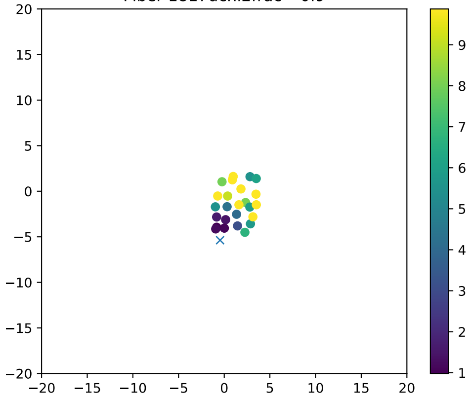
Fiber 1817dchi2frac= 0.9
