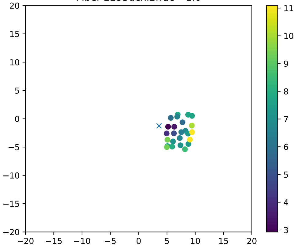
Fiber 2295dchi2frac= 1.0
