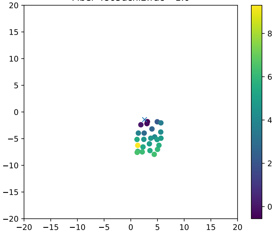
Fiber 4865dchi2frac= 1.0
