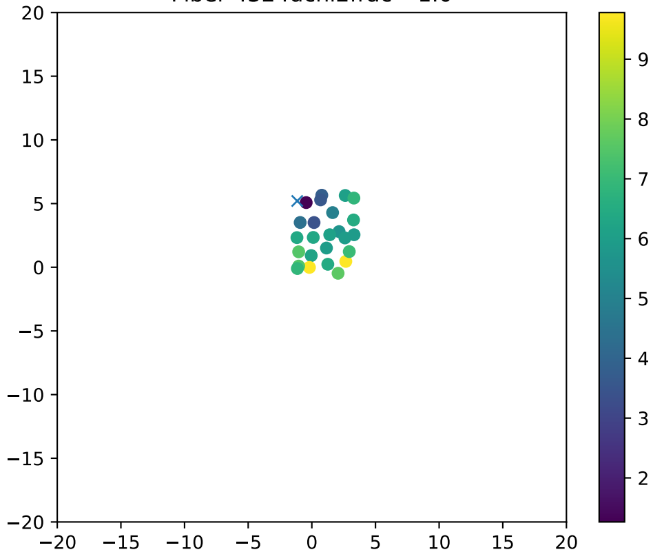
Fiber 4324dchi2frac= 1.0
