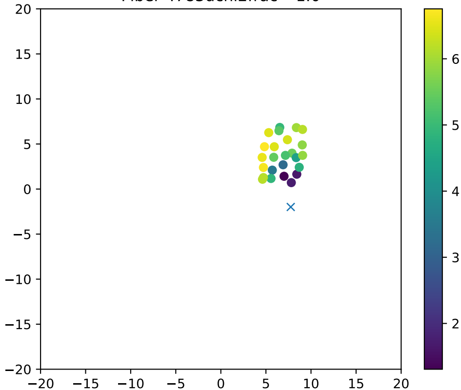
Fiber 4783dchi2frac= 1.0
