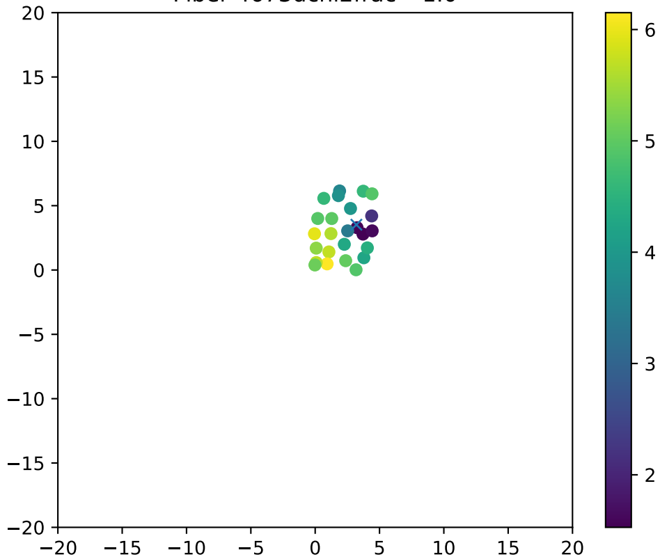
Fiber 4673dchi2frac= 1.0
