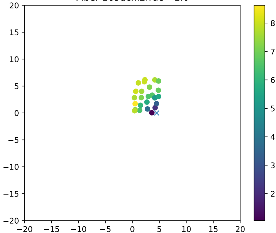
Fiber 265dchi2frac= 1.0
