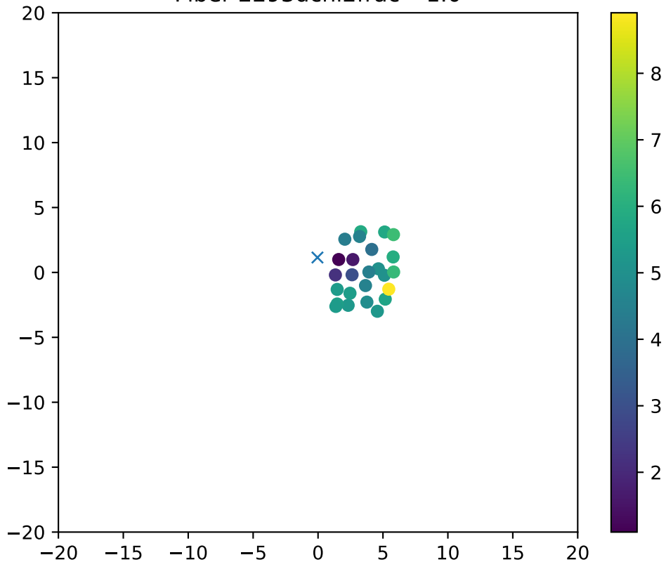
Fiber 2293dchi2frac= 1.0
