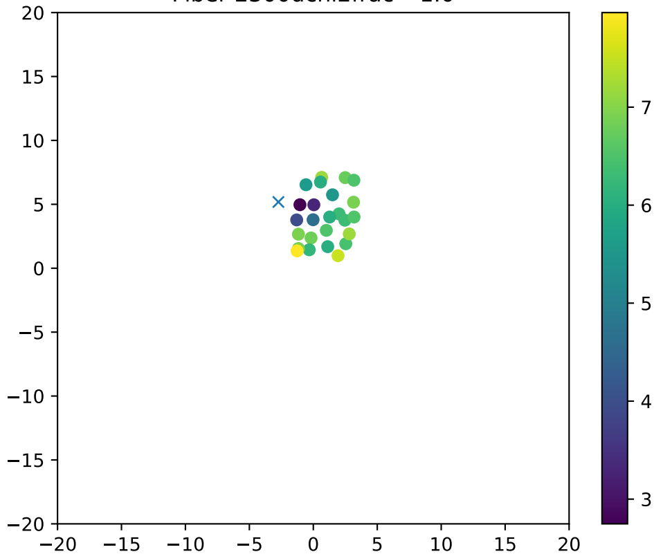
Fiber 2300dchi2frac= 1.0
