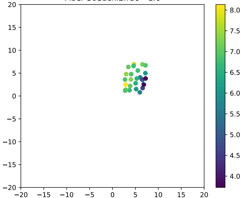
Fiber 301dchi2frac= 1.0
