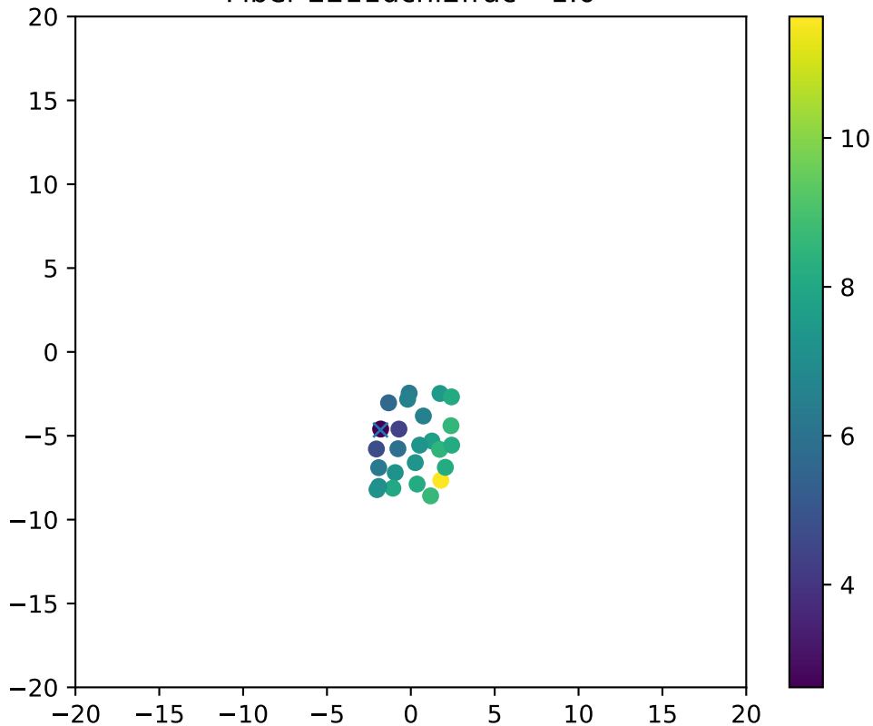
Fiber 2211dchi2frac= 1.0
