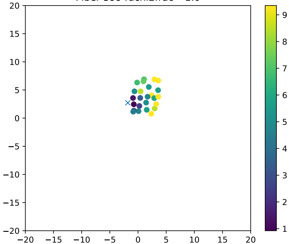
Fiber 3994dchi2frac= 1.0
