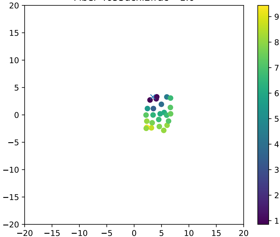
Fiber 4653dchi2frac= 1.0
