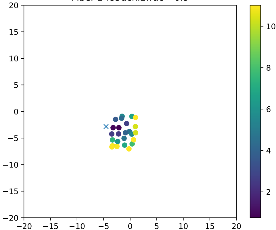
Fiber 2485dchi2frac= 0.9
