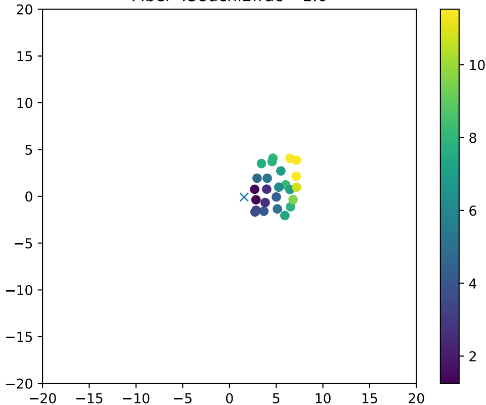
Fiber 438dchi2frac= 1.0
