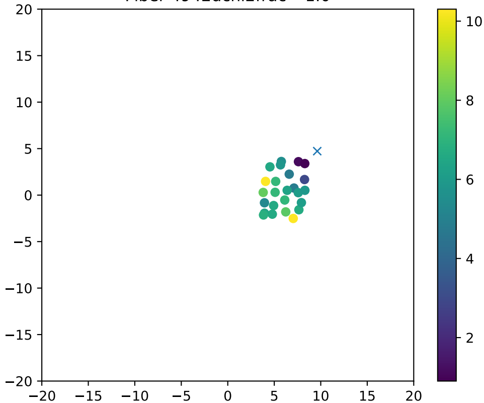
Fiber 4942dchi2frac= 1.0
