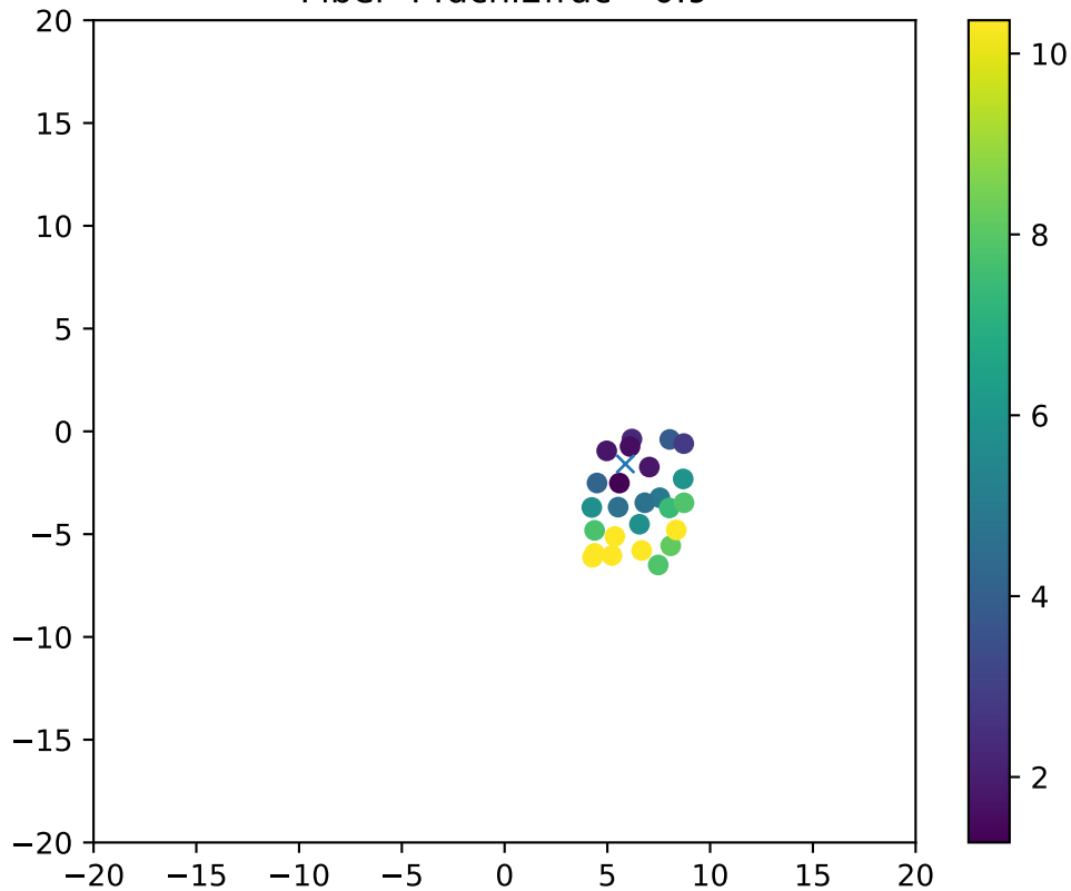
Fiber 44dchi2frac= 0.9
