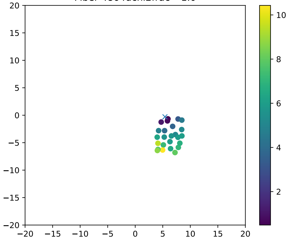
Fiber 4864dchi2frac= 1.0
