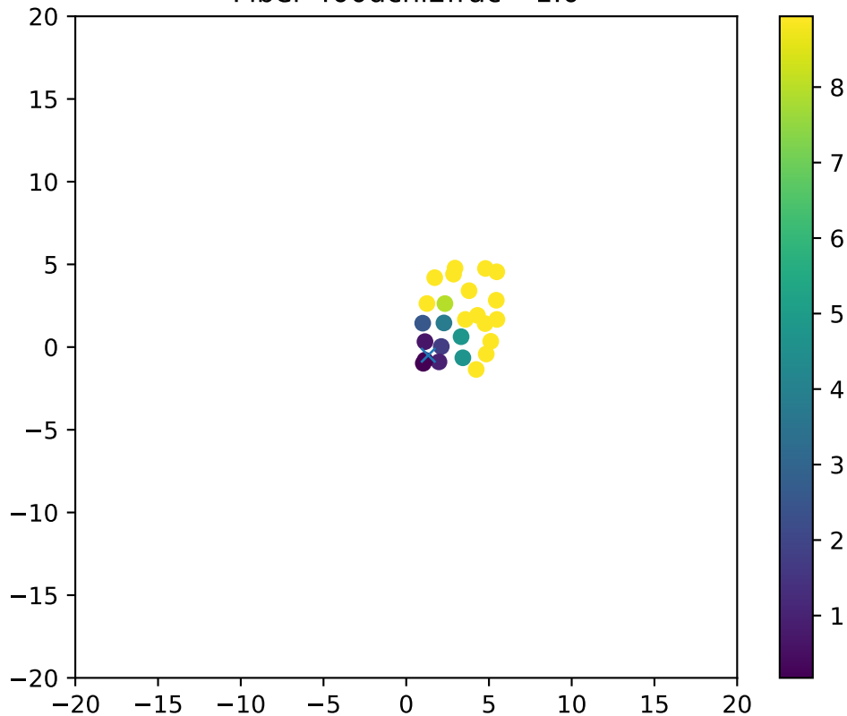
Fiber 400dchi2frac= 1.0
