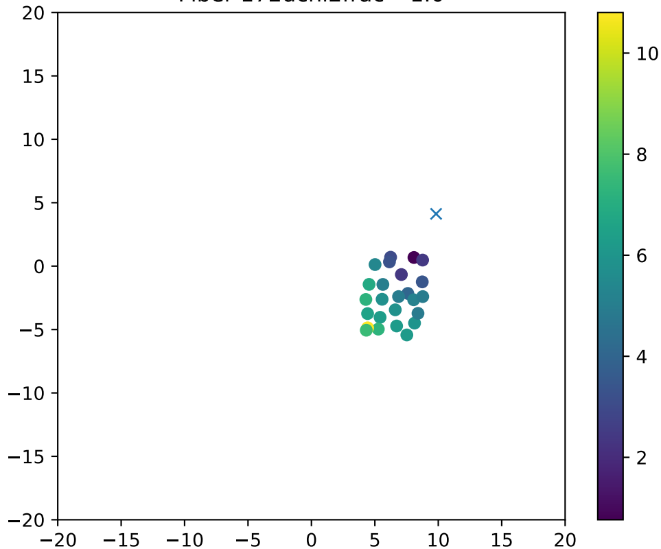
Fiber 172dchi2frac= 1.0
