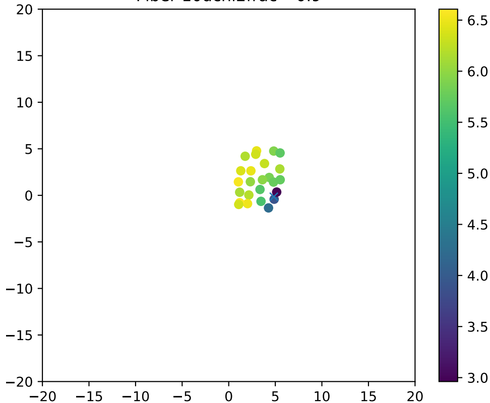
Fiber 10dchi2frac= 0.9
