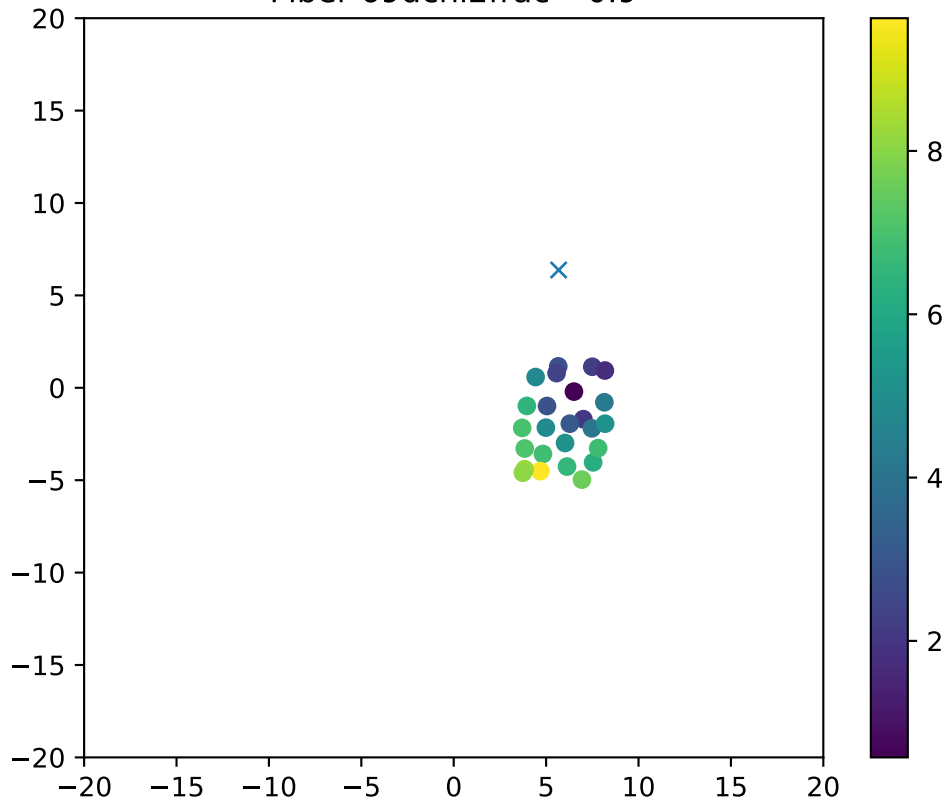
Fiber 69dchi2frac= 0.9
