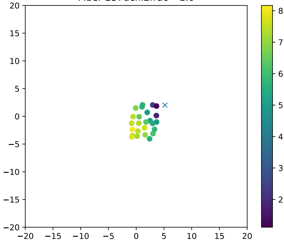
Fiber 257dchi2frac= 1.0
