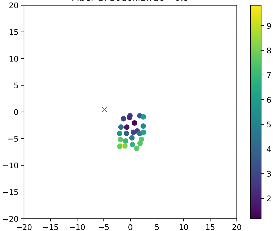
Fiber 1716dchi2frac= 0.9
