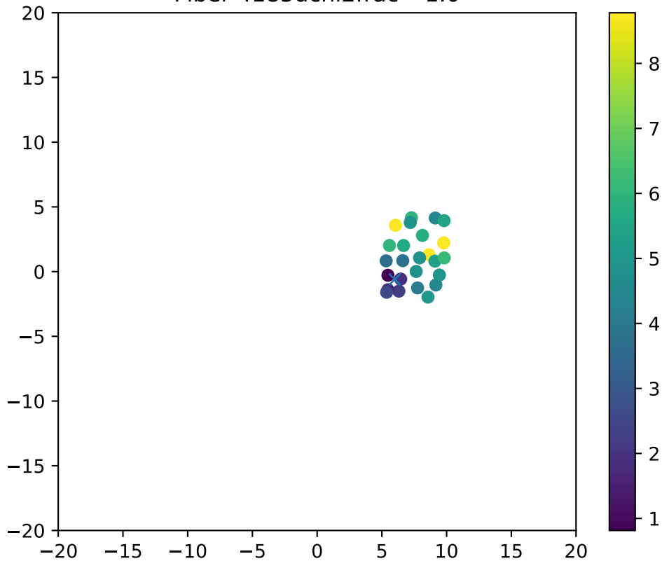
Fiber 4185dchi2frac= 1.0
