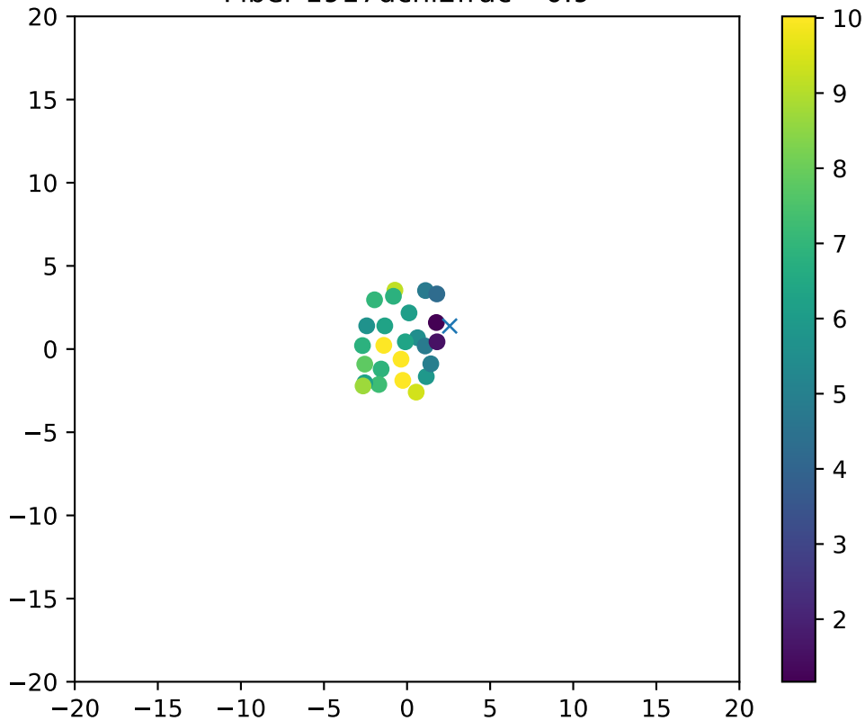
Fiber 1917dchi2frac= 0.9
