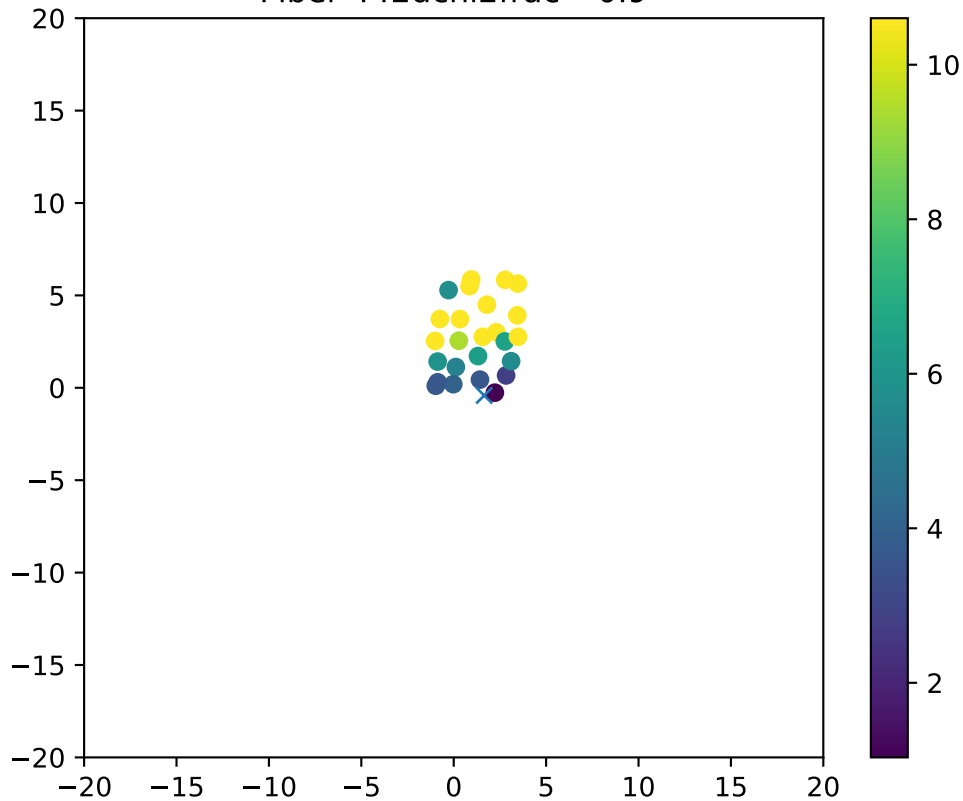
Fiber 442dchi2frac= 0.9
