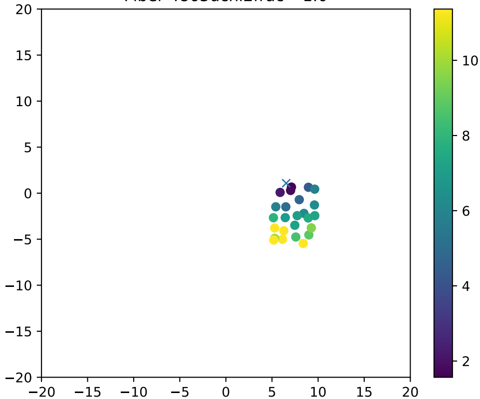
Fiber 4863dchi2frac= 1.0
