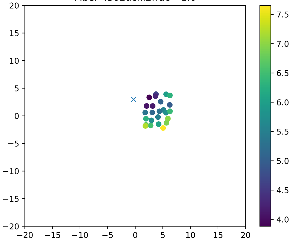
Fiber 4302dchi2frac= 1.0
