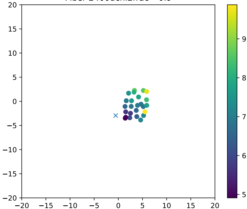
Fiber 2400dchi2frac= 0.9
