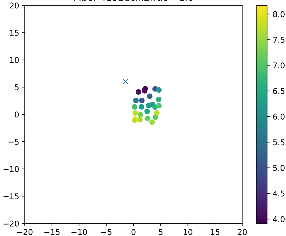
Fiber 4152dchi2frac= 1.0
