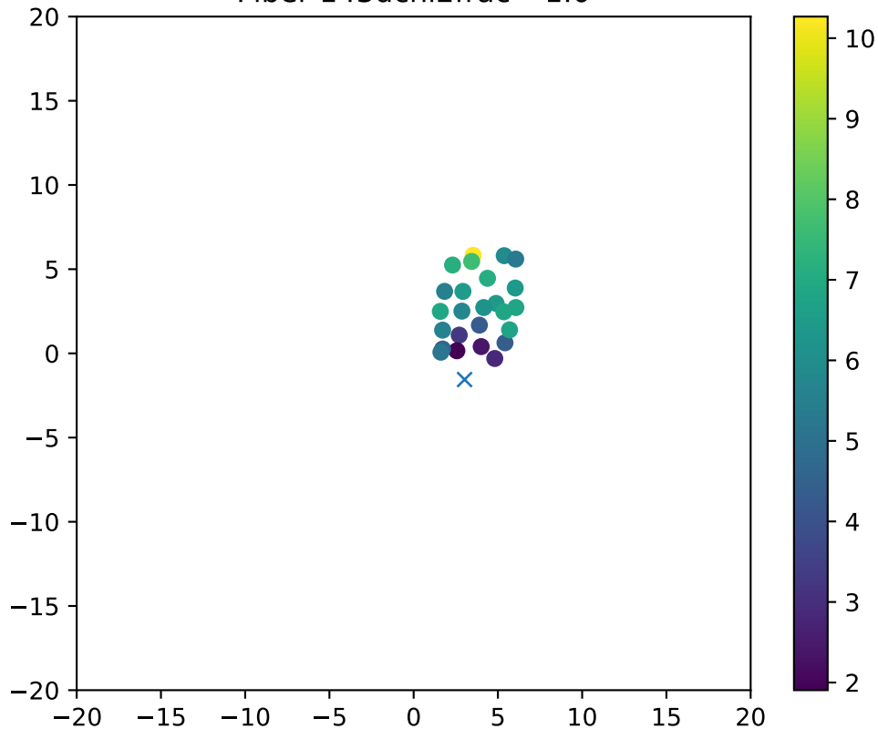
Fiber 143dchi2frac= 1.0
