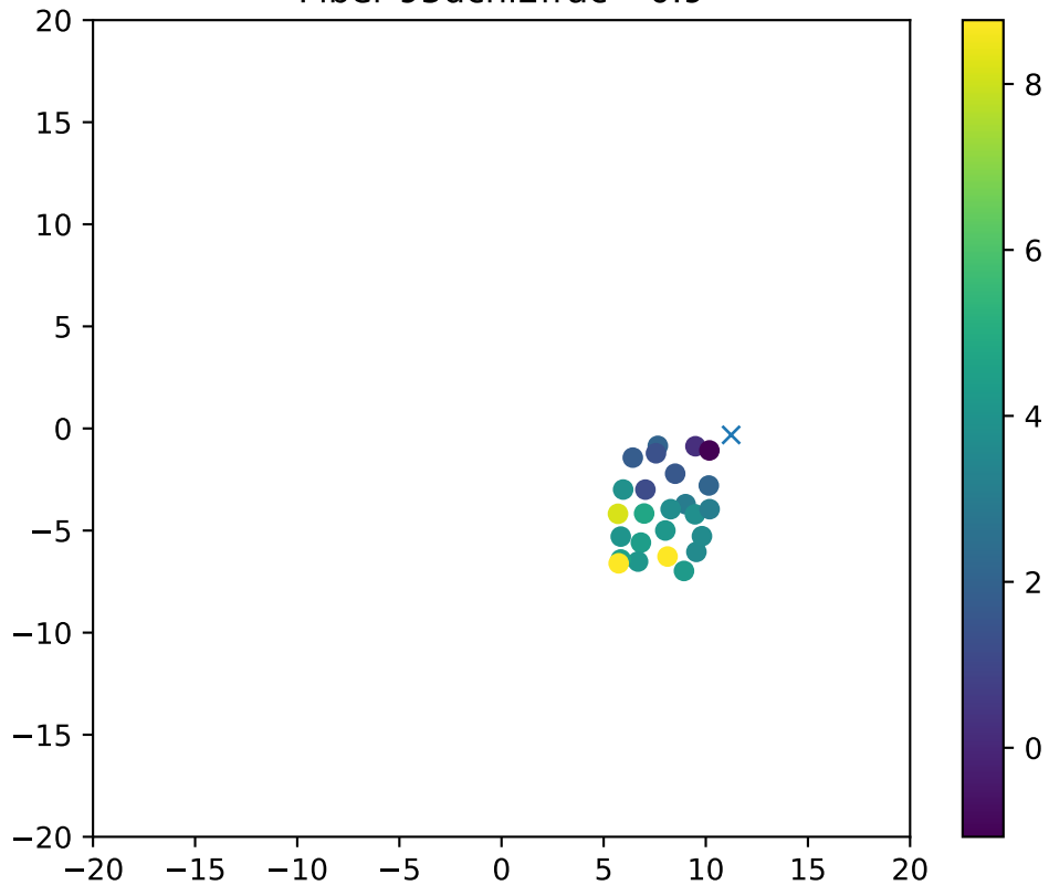
Fiber 95dchi2frac= 0.9
