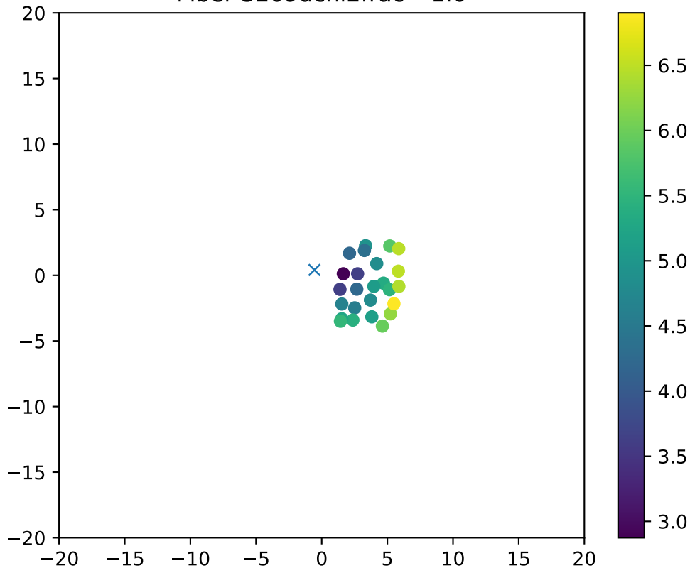
Fiber 3209dchi2frac= 1.0
