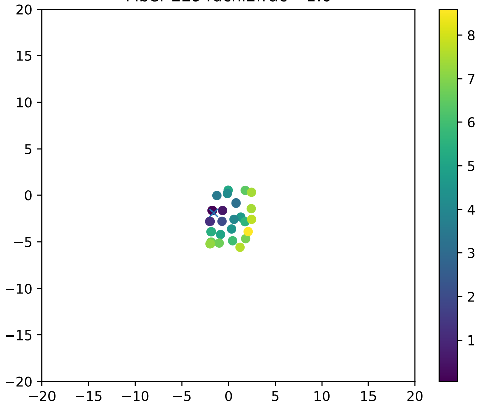
Fiber 2294dchi2frac= 1.0
