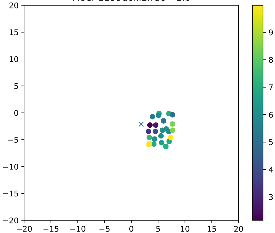
Fiber 2299dchi2frac= 1.0
