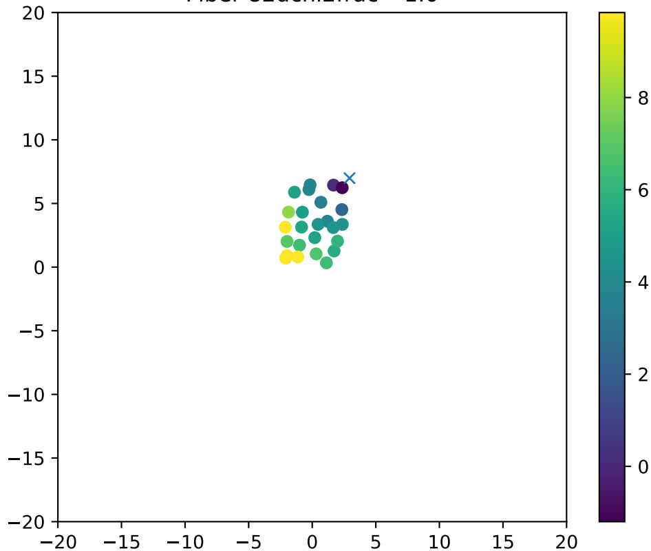
Fiber 82dchi2frac= 1.0
