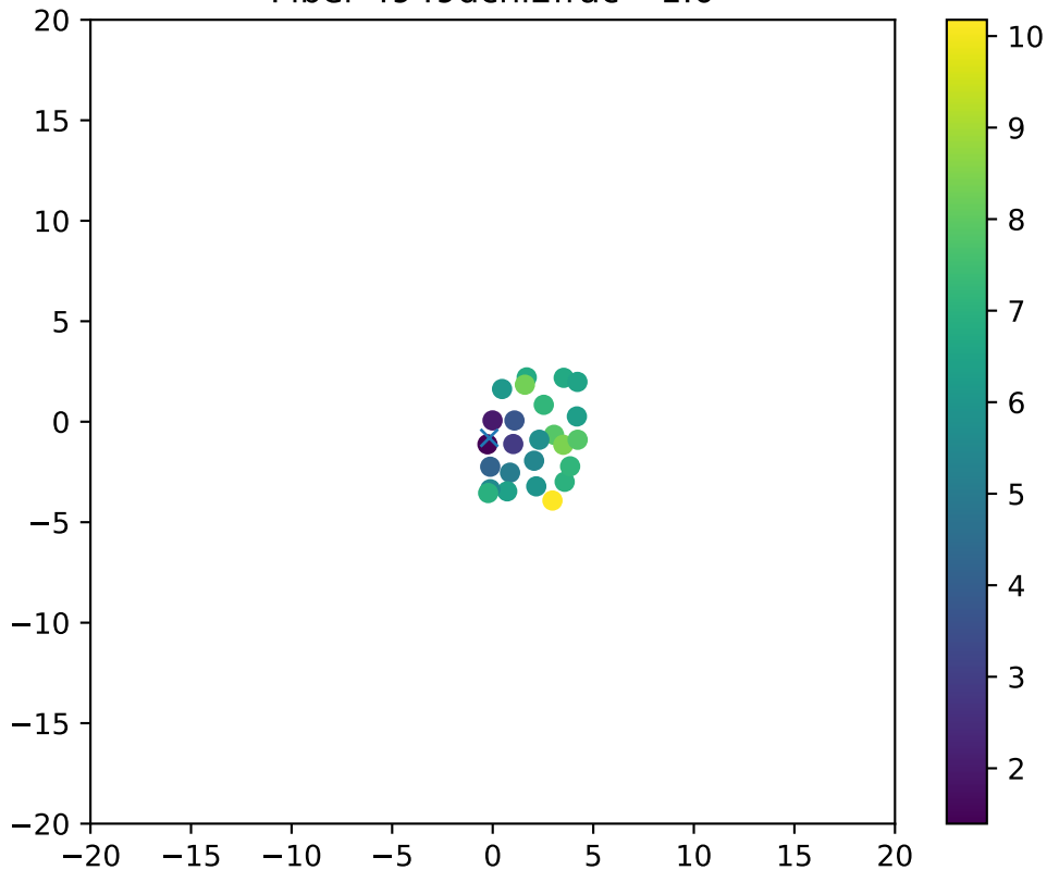
Fiber 4949dchi2frac= 1.0
