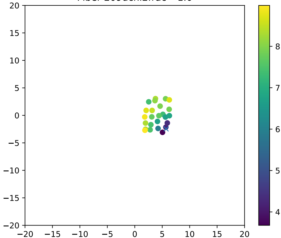
Fiber 209dchi2frac= 1.0
