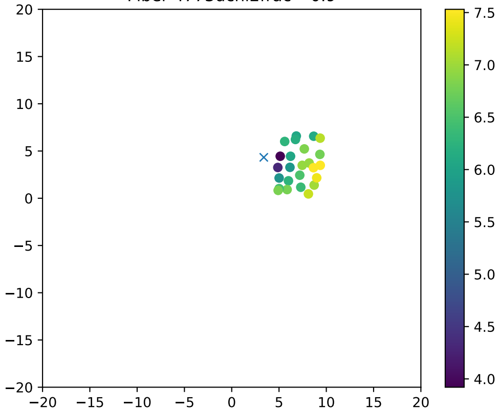
Fiber 4773dchi2frac= 0.9
