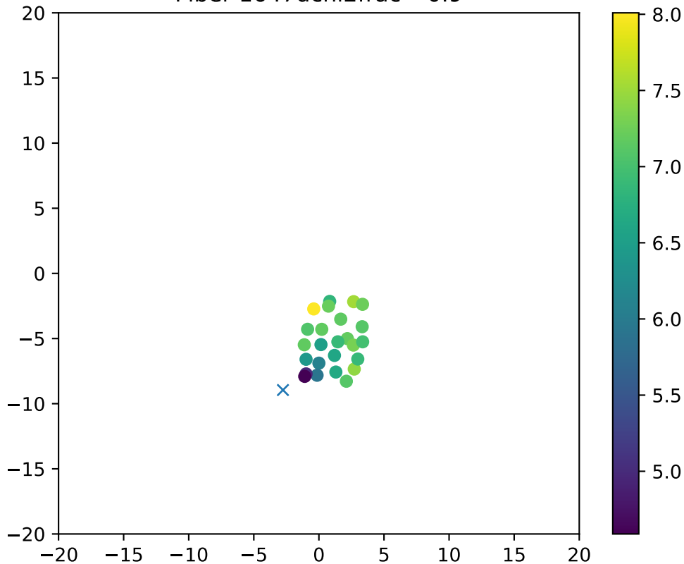
Fiber 1647dchi2frac= 0.9
