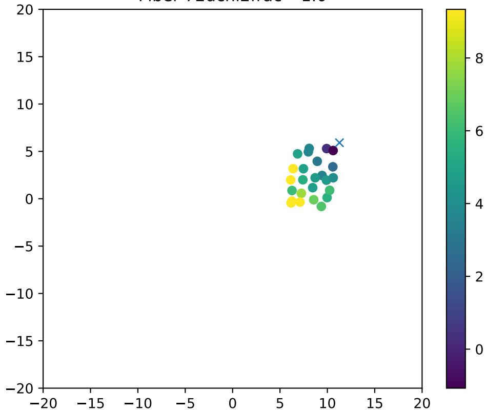
Fiber 72dchi2frac= 1.0
