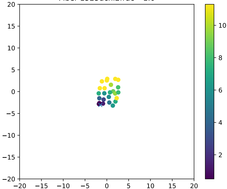
Fiber 1523dchi2frac= 1.0
