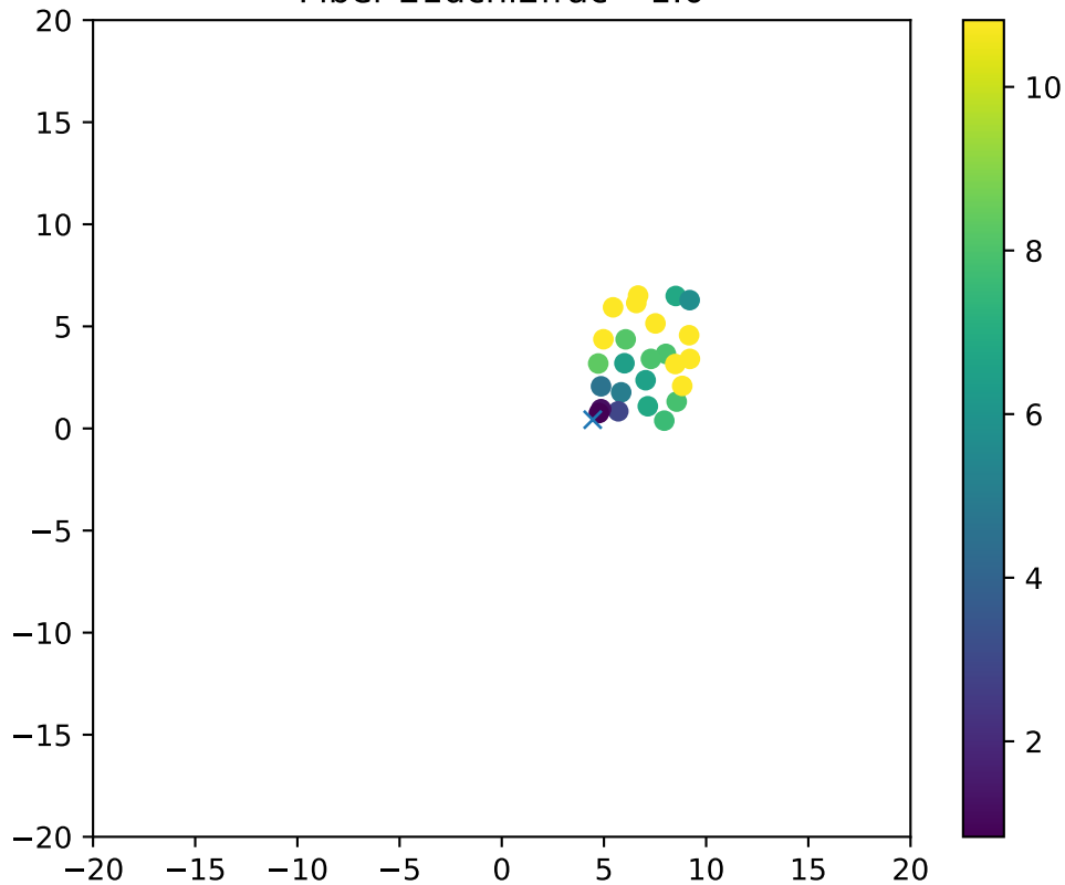
Fiber 21dchi2frac= 1.0
