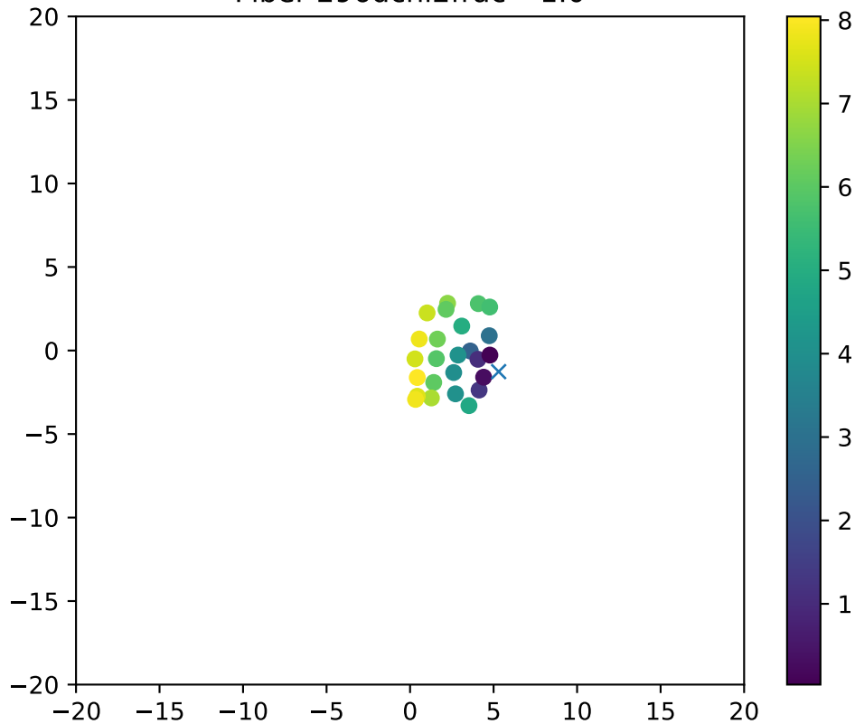
Fiber 296dchi2frac= 1.0
