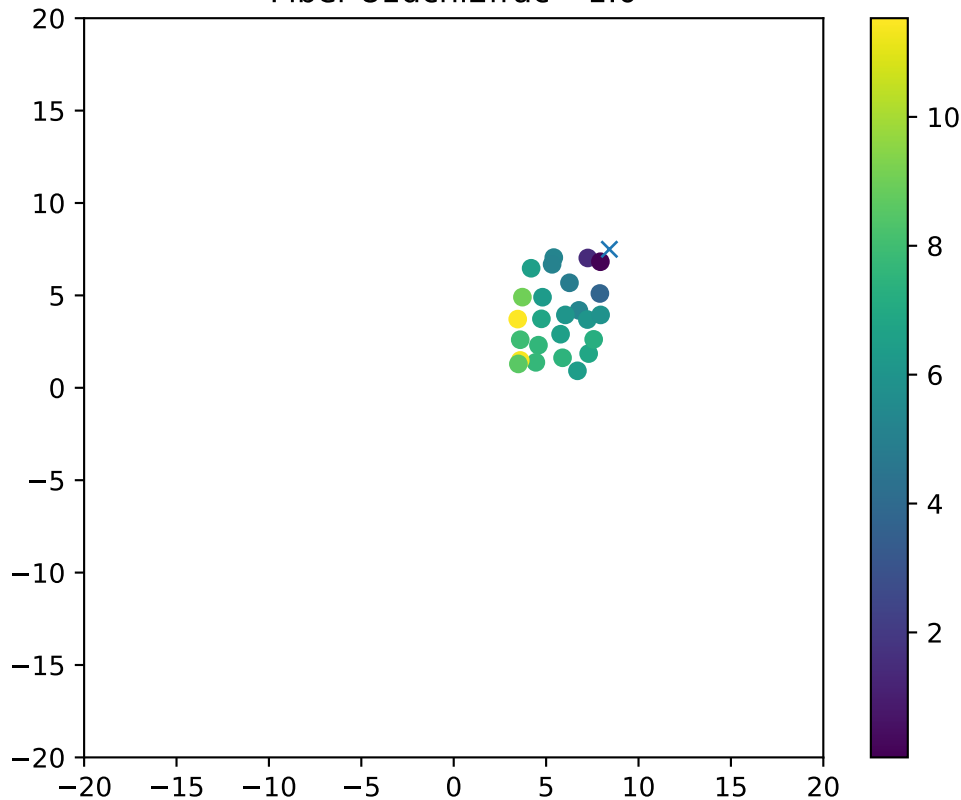
Fiber 81dchi2frac= 1.0
