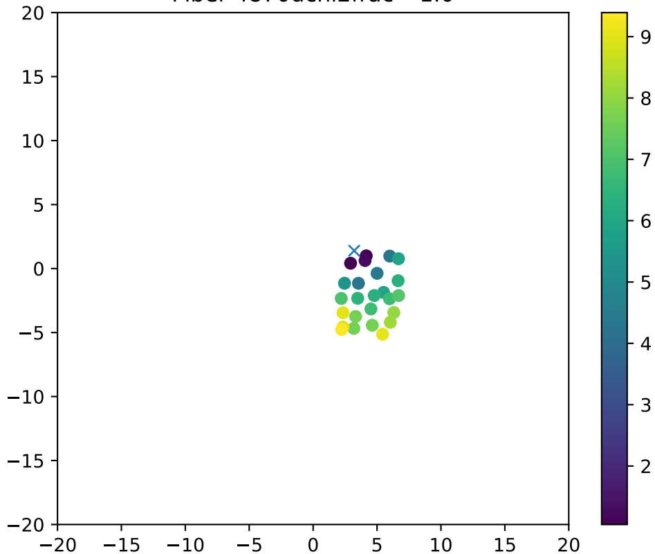
Fiber 4870dchi2frac= 1.0
