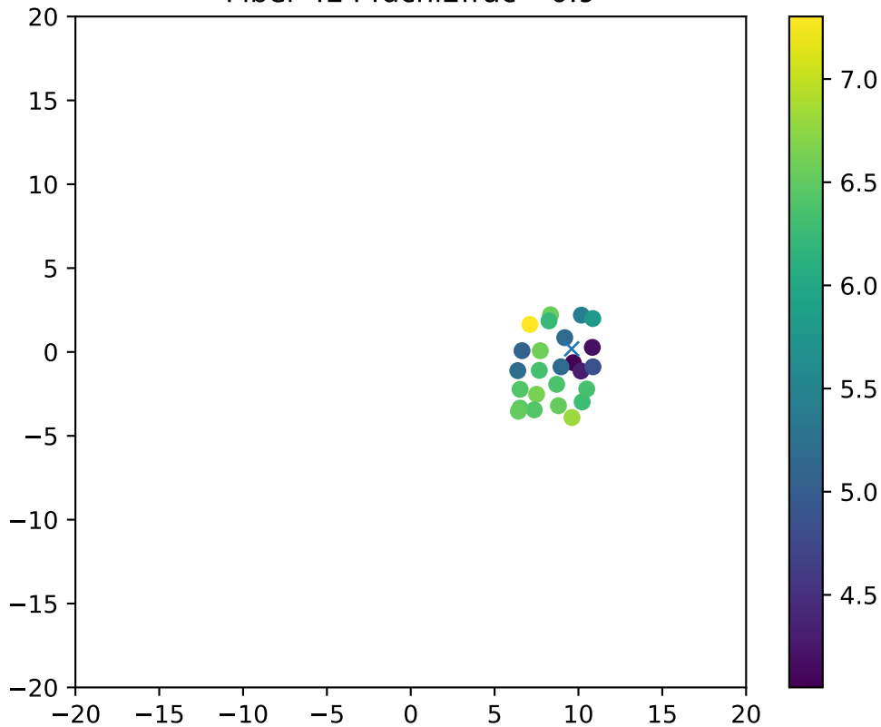
Fiber 4244dchi2frac= 0.9
