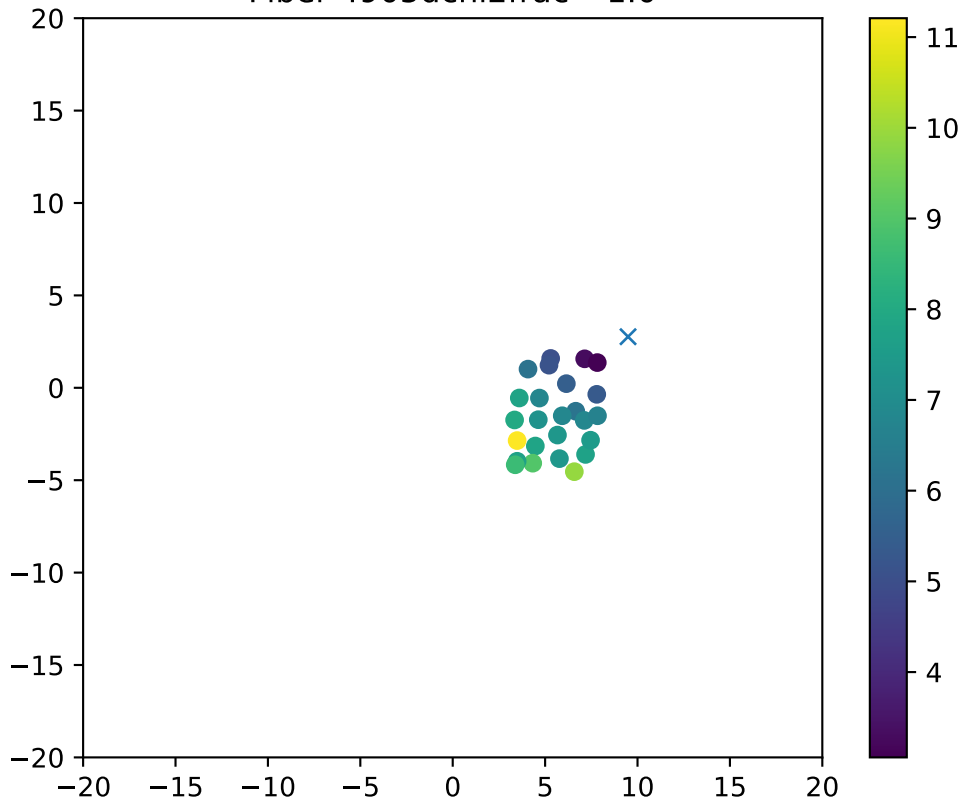
Fiber 4905dchi2frac= 1.0
