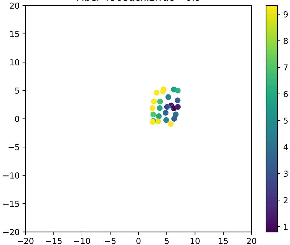
Fiber 4968dchi2frac= 0.9
