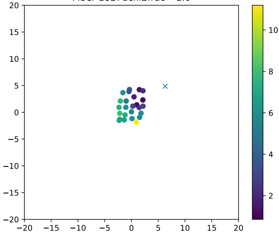
Fiber 1827dchi2frac= 1.0
