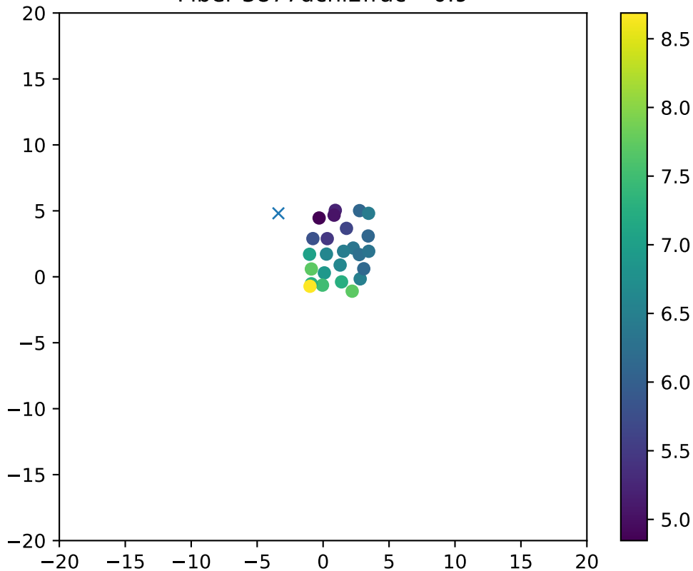
Fiber 3877dchi2frac= 0.9
