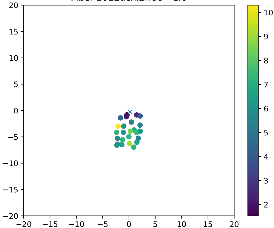
Fiber 2022dchi2frac= 1.0
