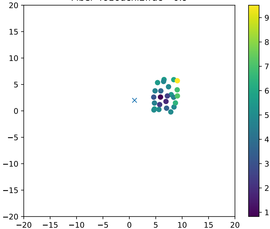
Fiber 4616dchi2frac= 0.9
