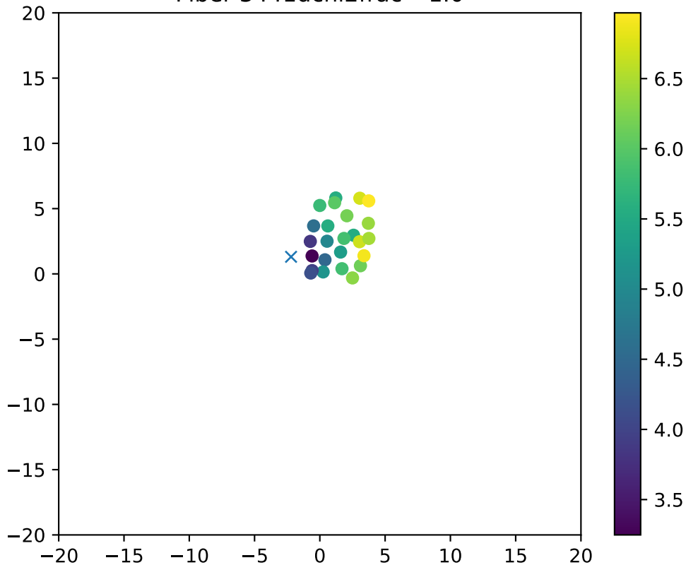
Fiber 3441dchi2frac= 1.0
