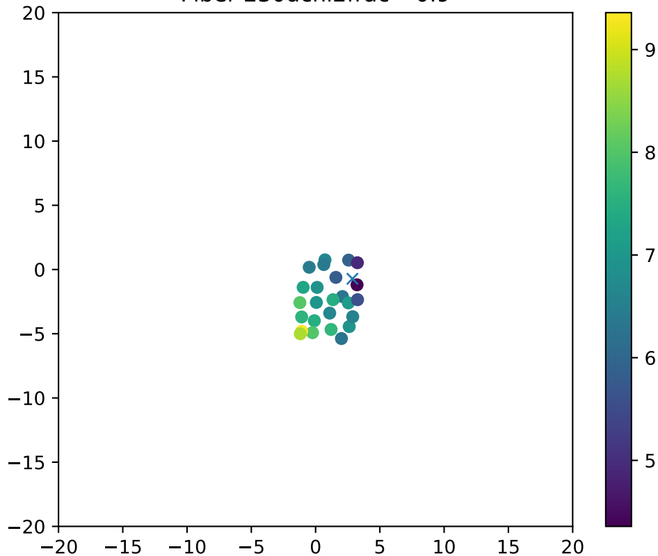
Fiber 230dchi2frac= 0.9
