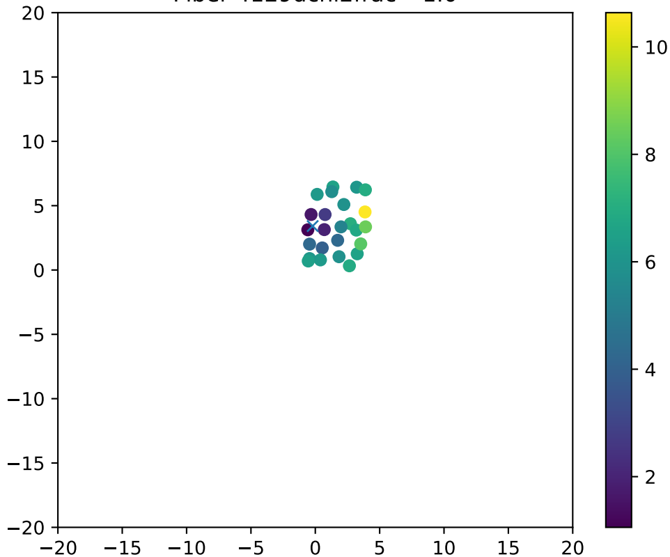
Fiber 4129dchi2frac= 1.0
