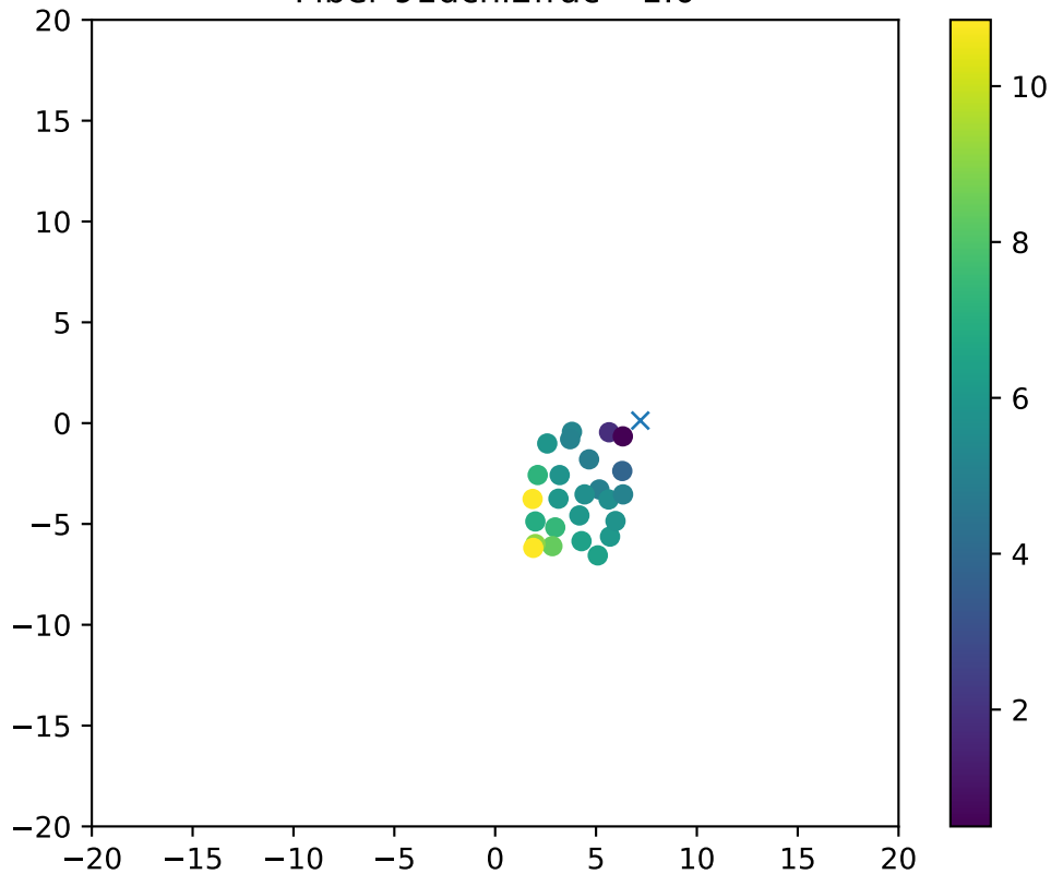
Fiber 91dchi2frac= 1.0
