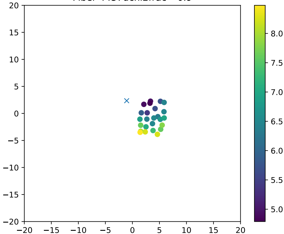
Fiber 4437dchi2frac= 0.9
