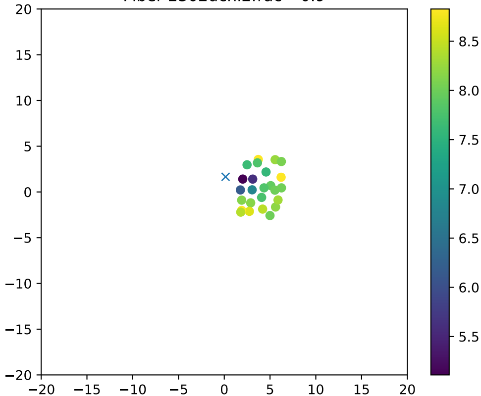
Fiber 2302dchi2frac= 0.9
