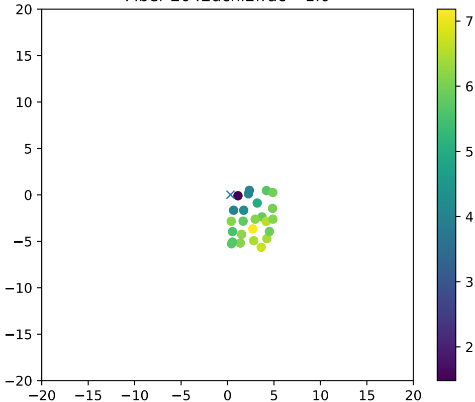
Fiber 2042dchi2frac= 1.0
