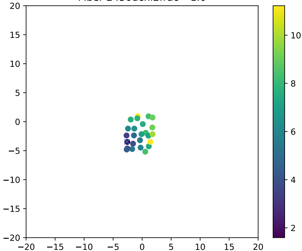
Fiber 2450dchi2frac= 1.0
