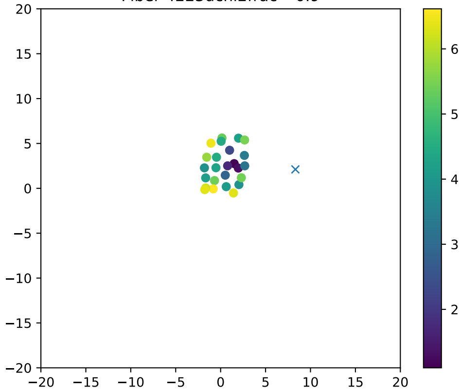
Fiber 4223dchi2frac= 0.9
