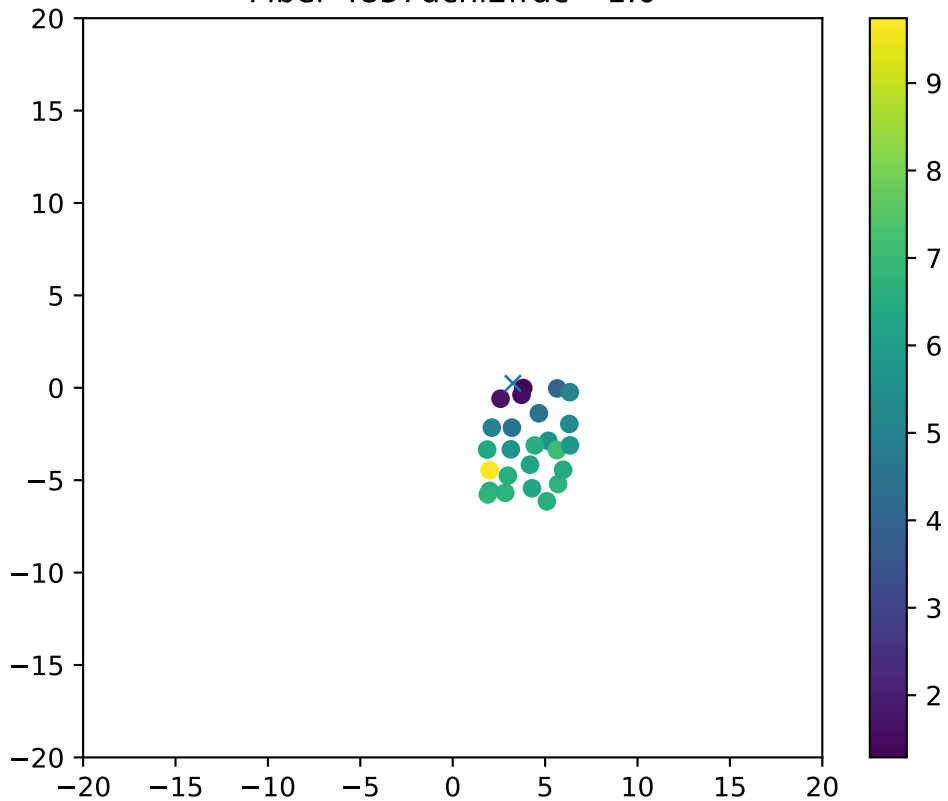
Fiber 4857dchi2frac= 1.0
