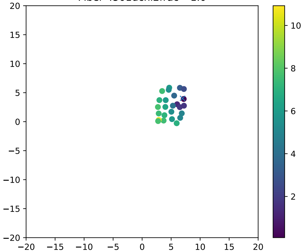
Fiber 4501dchi2frac= 1.0
