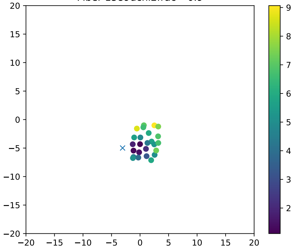
Fiber 1589dchi2frac= 0.9
