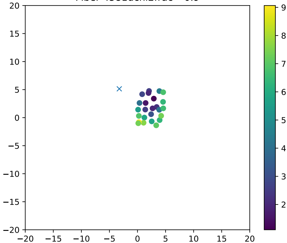
Fiber 4581dchi2frac= 0.9
