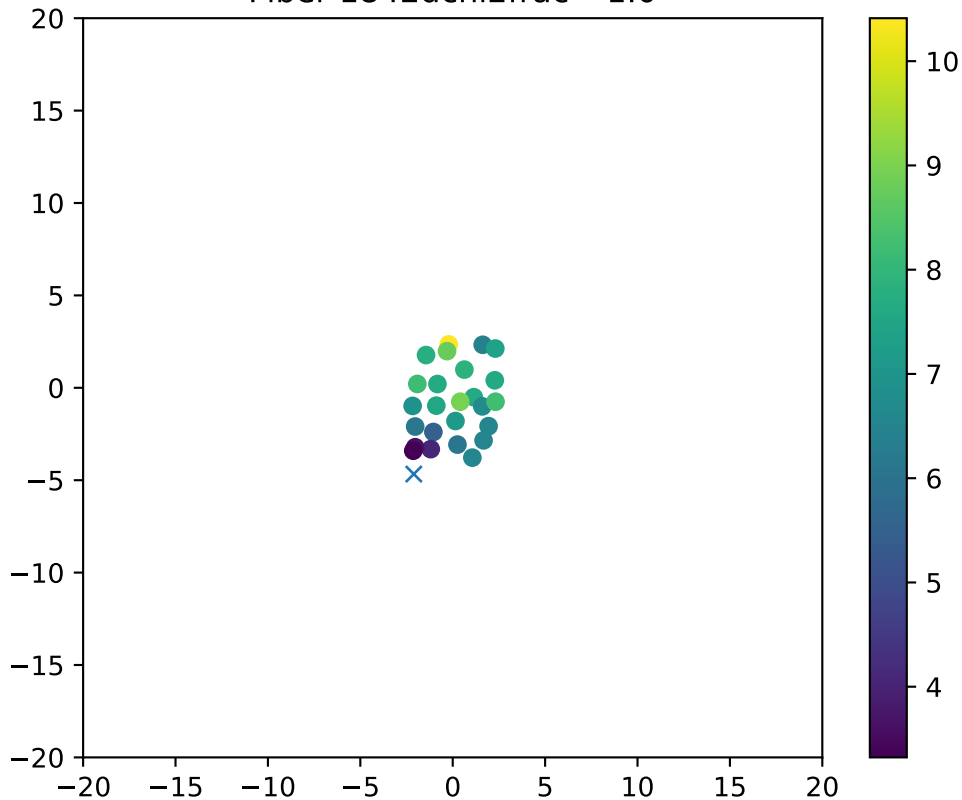
Fiber 1842dchi2frac= 1.0
