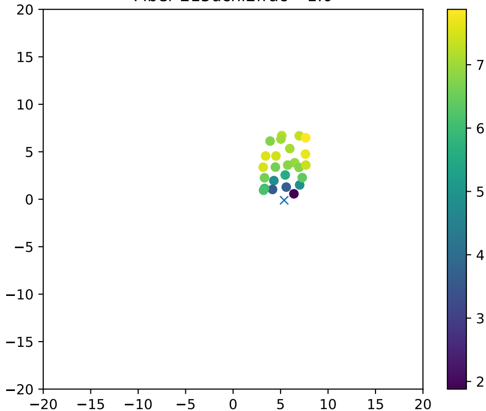
Fiber 215dchi2frac= 1.0
