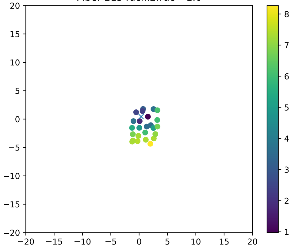
Fiber 2154dchi2frac= 1.0
