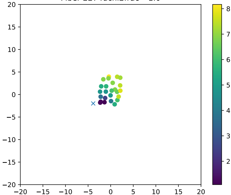
Fiber 2274dchi2frac= 1.0
