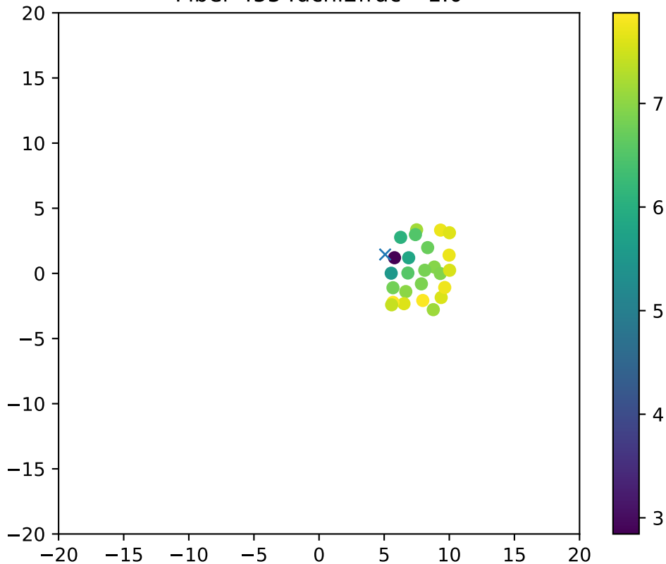
Fiber 4554dchi2frac= 1.0
