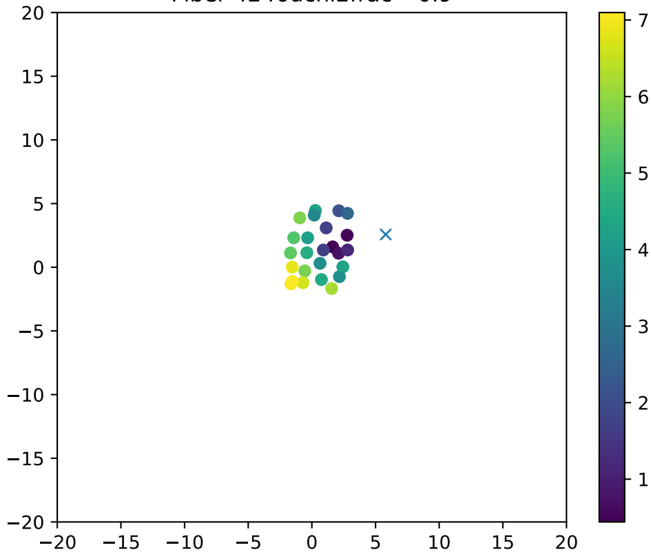
Fiber 4246dchi2frac= 0.9
