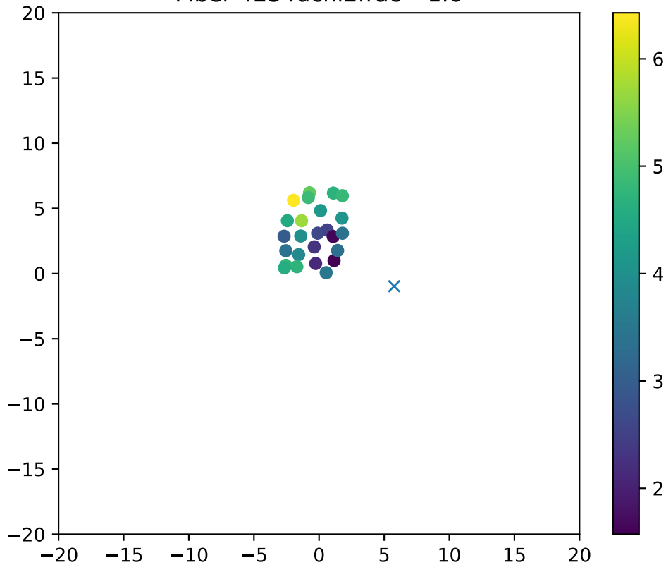
Fiber 4234dchi2frac= 1.0
