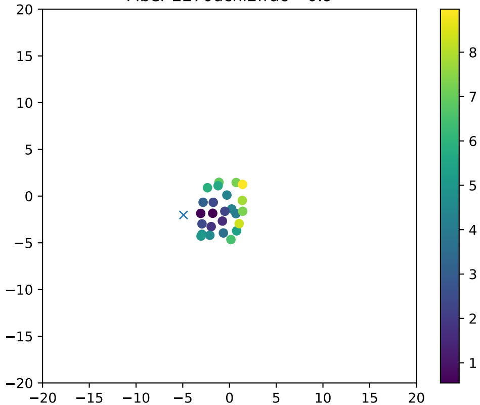
Fiber 2270dchi2frac= 0.9
