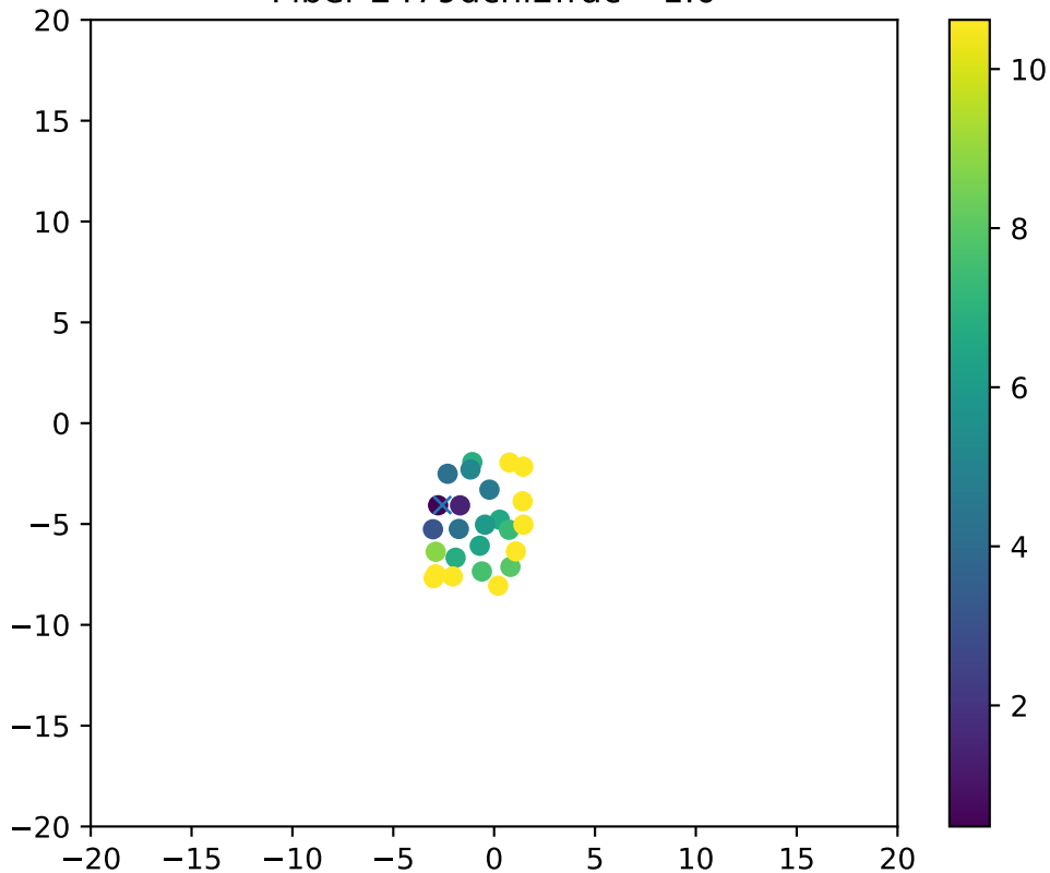
Fiber 2479dchi2frac= 1.0
