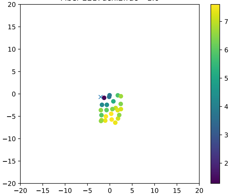
Fiber 2217dchi2frac= 1.0
