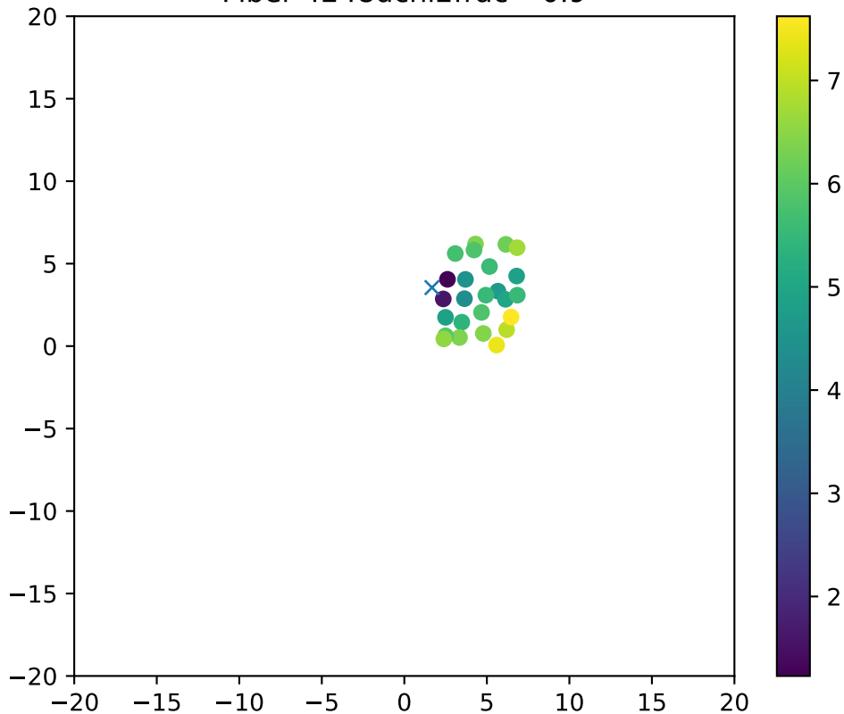
Fiber 4248dchi2frac= 0.9
