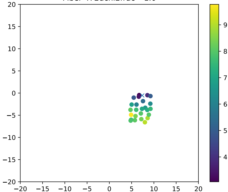
Fiber 472dchi2frac= 1.0
