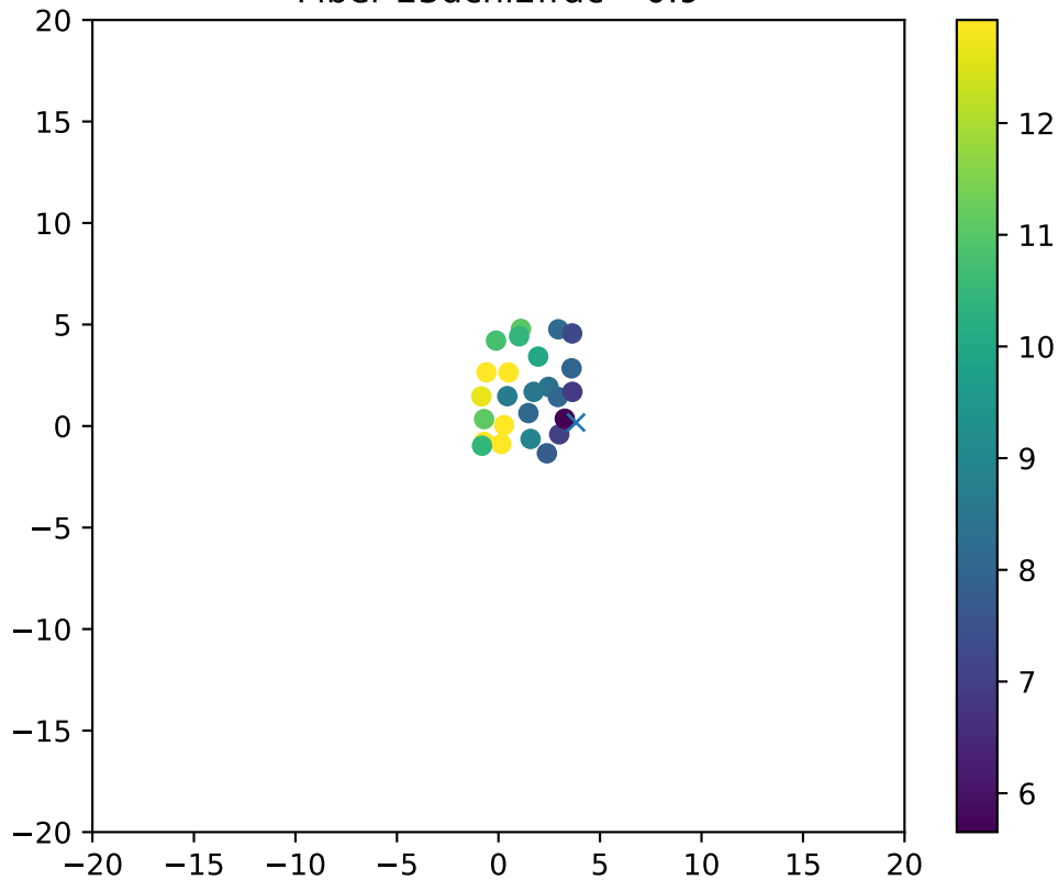
Fiber 23dchi2frac= 0.9
