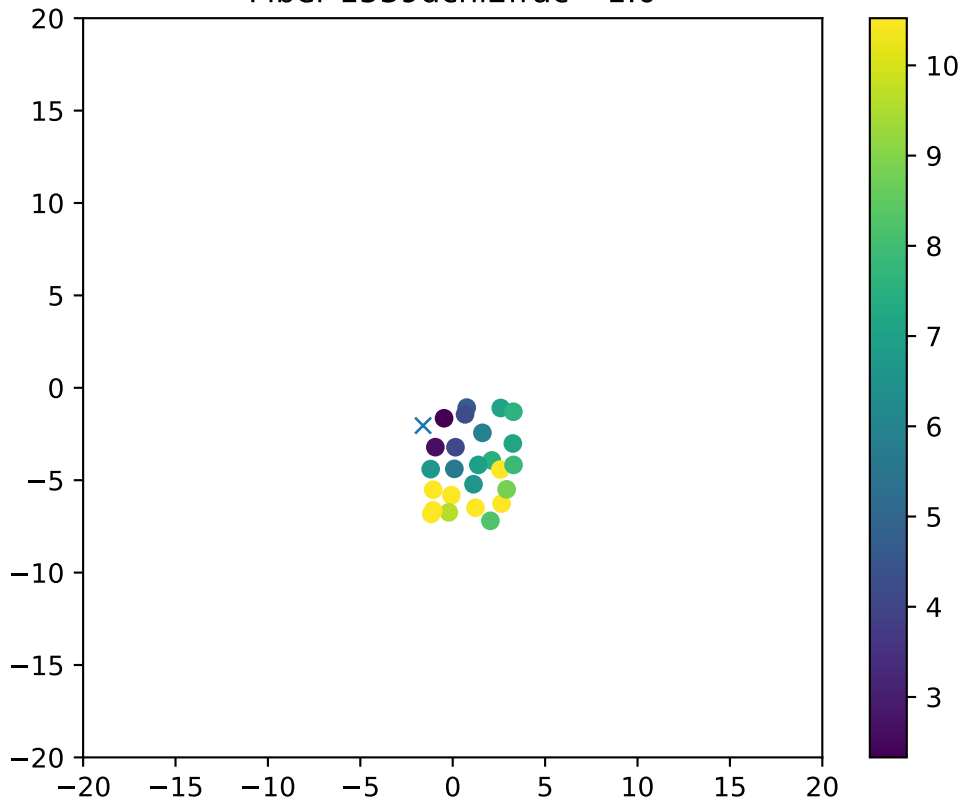
Fiber 1539dchi2frac= 1.0
