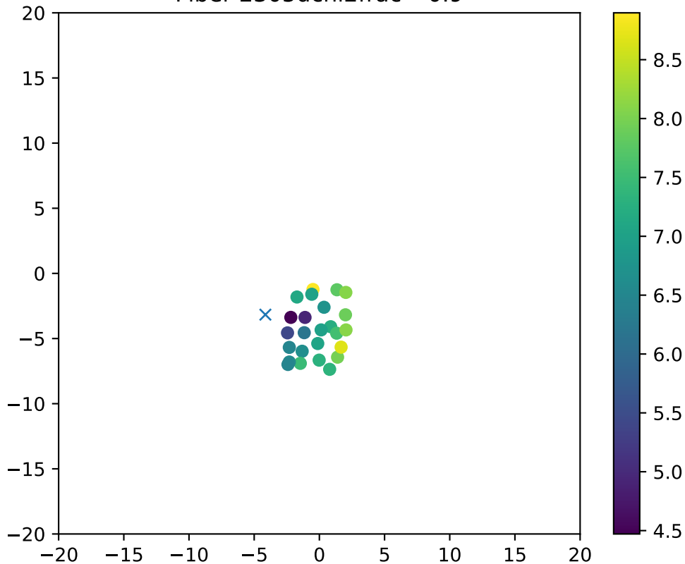
Fiber 2305dchi2frac= 0.9
