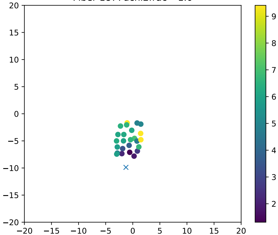
Fiber 1877dchi2frac= 1.0
