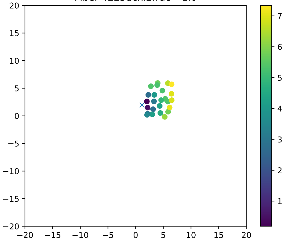
Fiber 4225dchi2frac= 1.0
