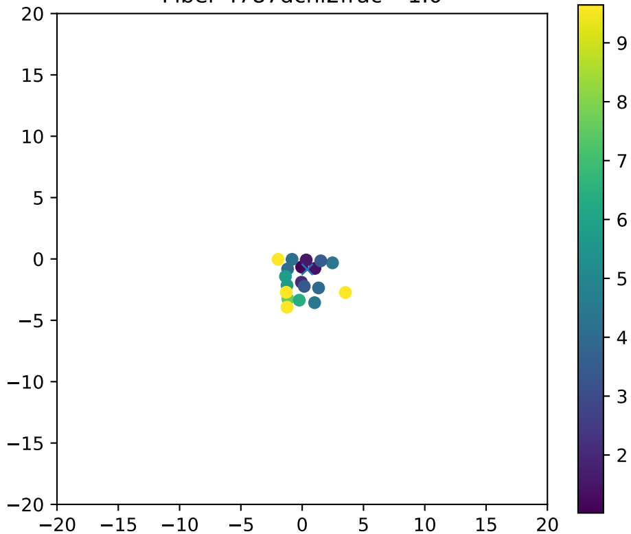
Fiber 4787dchi2frac= 1.0
