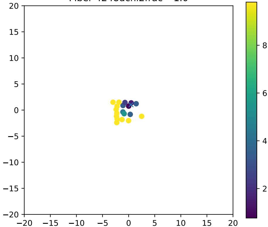
Fiber 4248dchi2frac= 1.0
