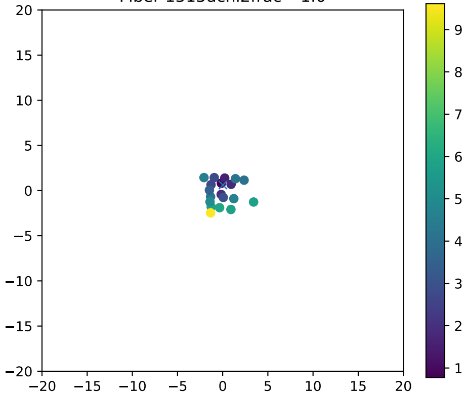
Fiber 1515dchi2frac= 1.0
