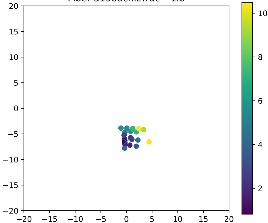
Fiber 3190dchi2frac= 1.0
