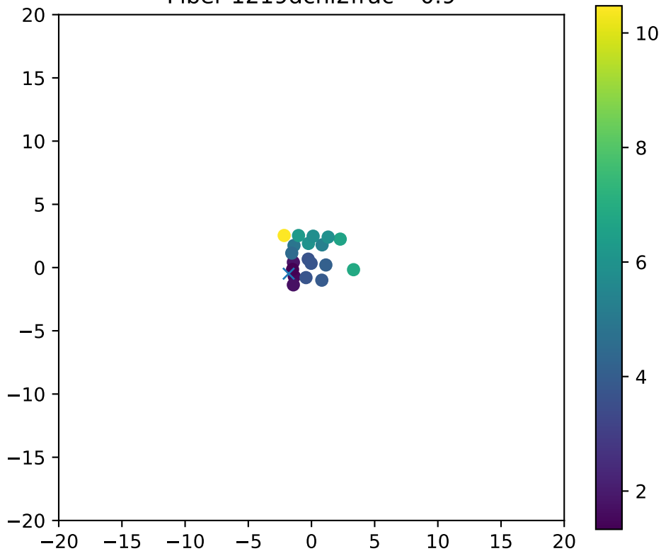
Fiber 1219dchi2frac= 0.9
