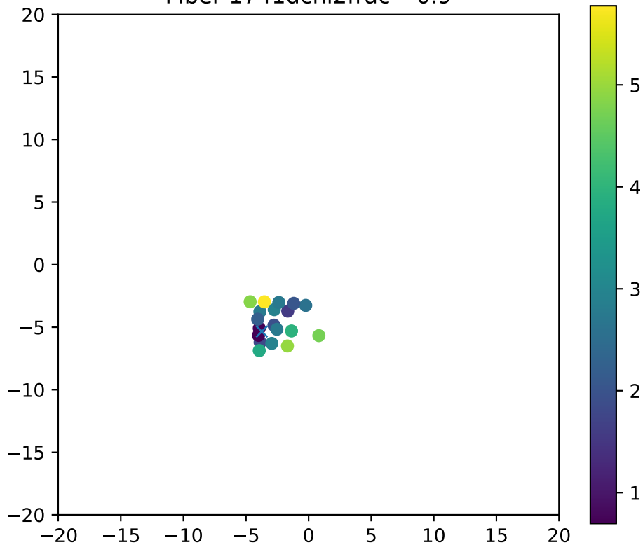
Fiber 1741dchi2frac= 0.9
