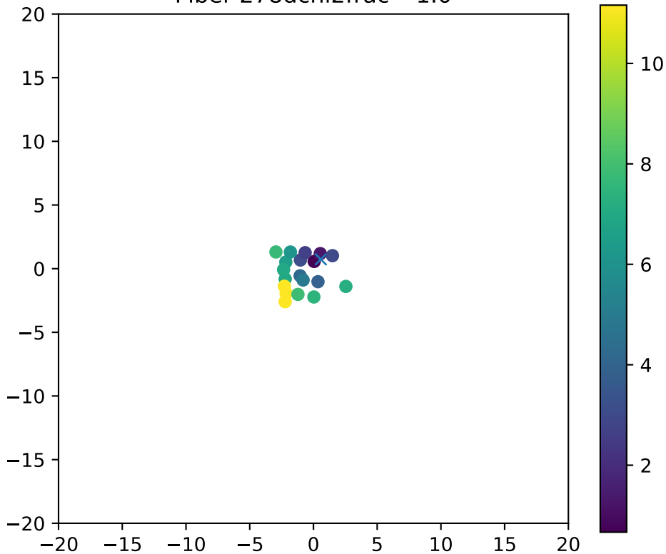
Fiber 278dchi2frac= 1.0
