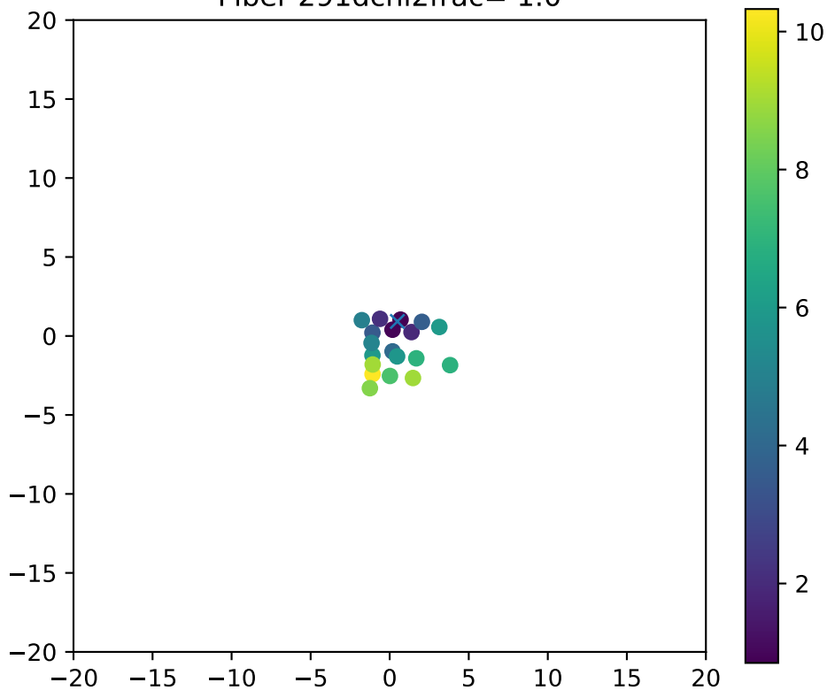
Fiber 291dchi2frac= 1.0
