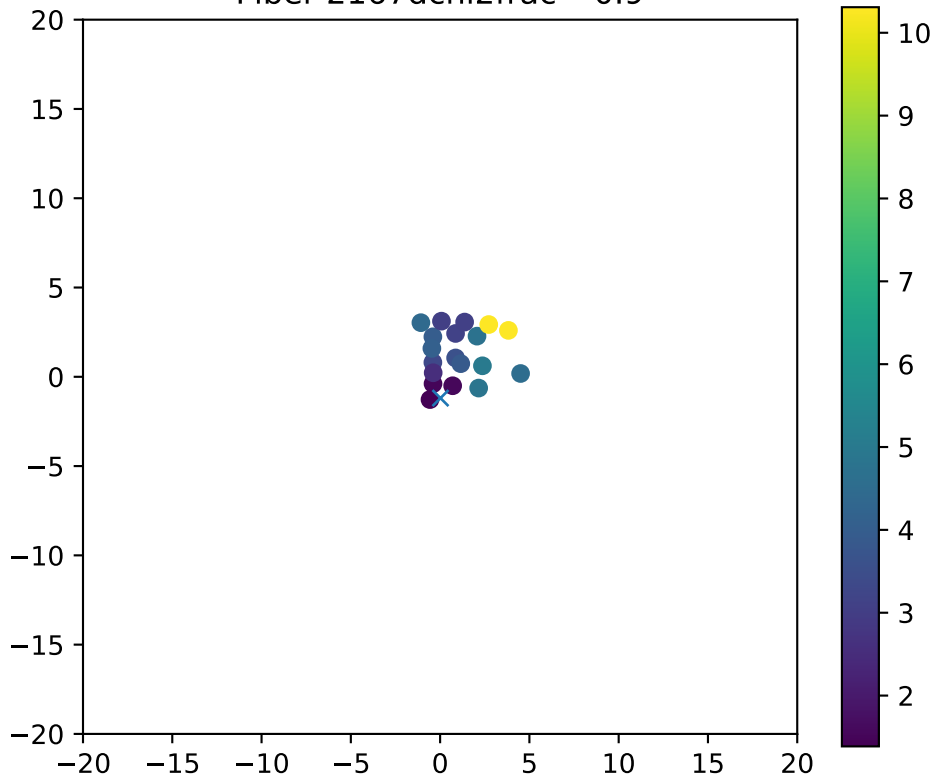
Fiber 2167dchi2frac= 0.9
