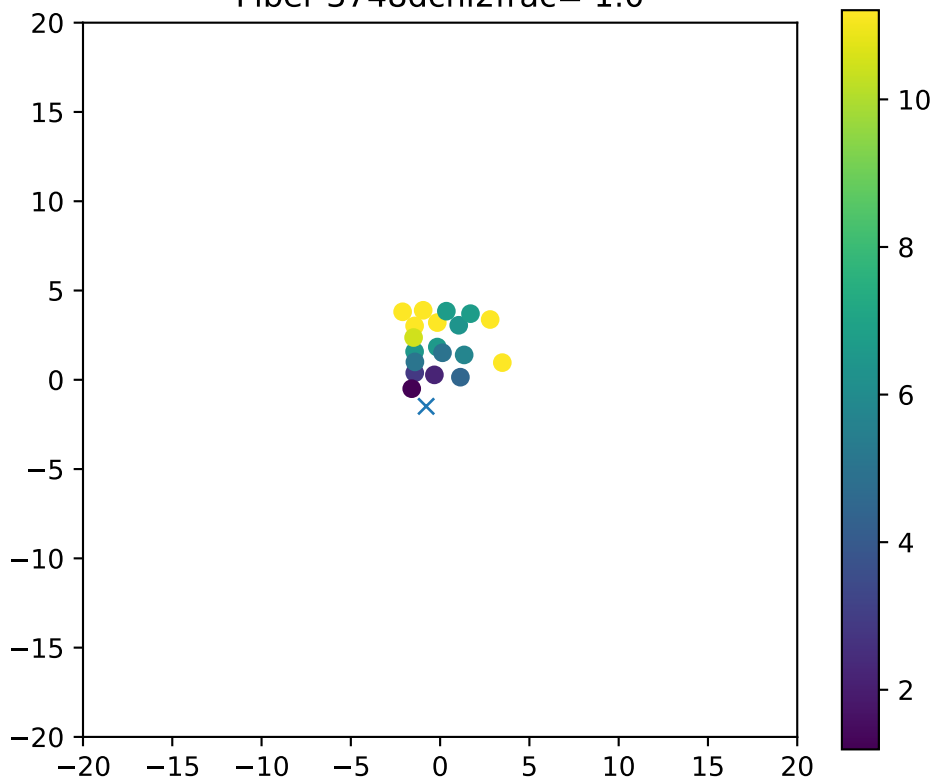
Fiber 3748dchi2frac= 1.0
