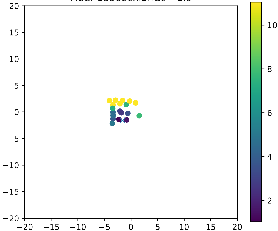
Fiber 1396dchi2frac= 1.0
