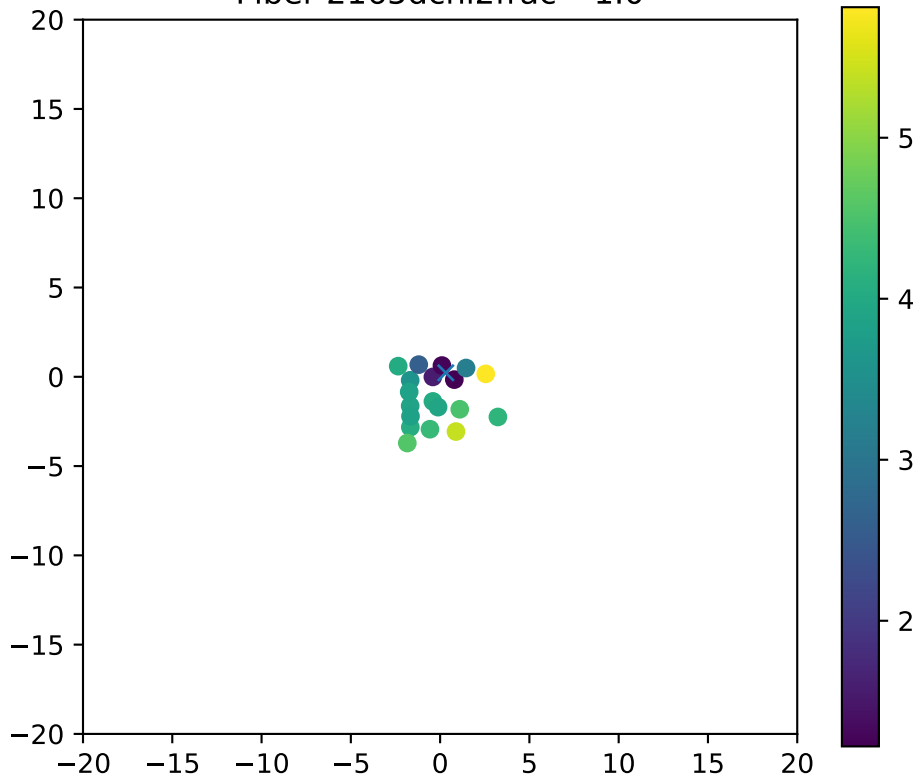
Fiber 2165dchi2frac= 1.0
