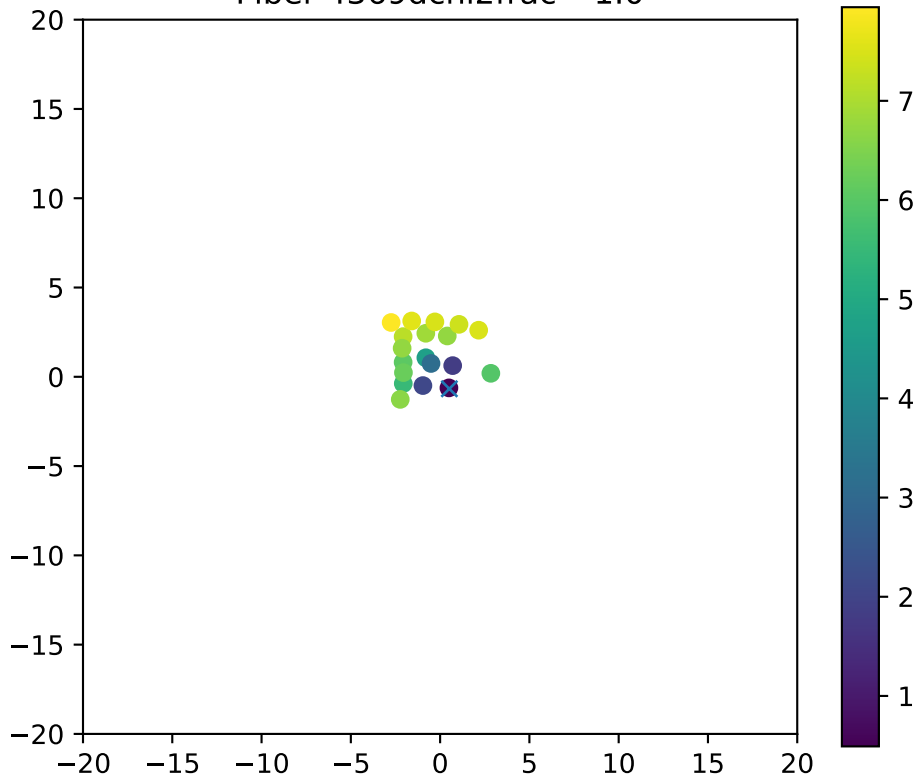
Fiber 4369dchi2frac= 1.0
