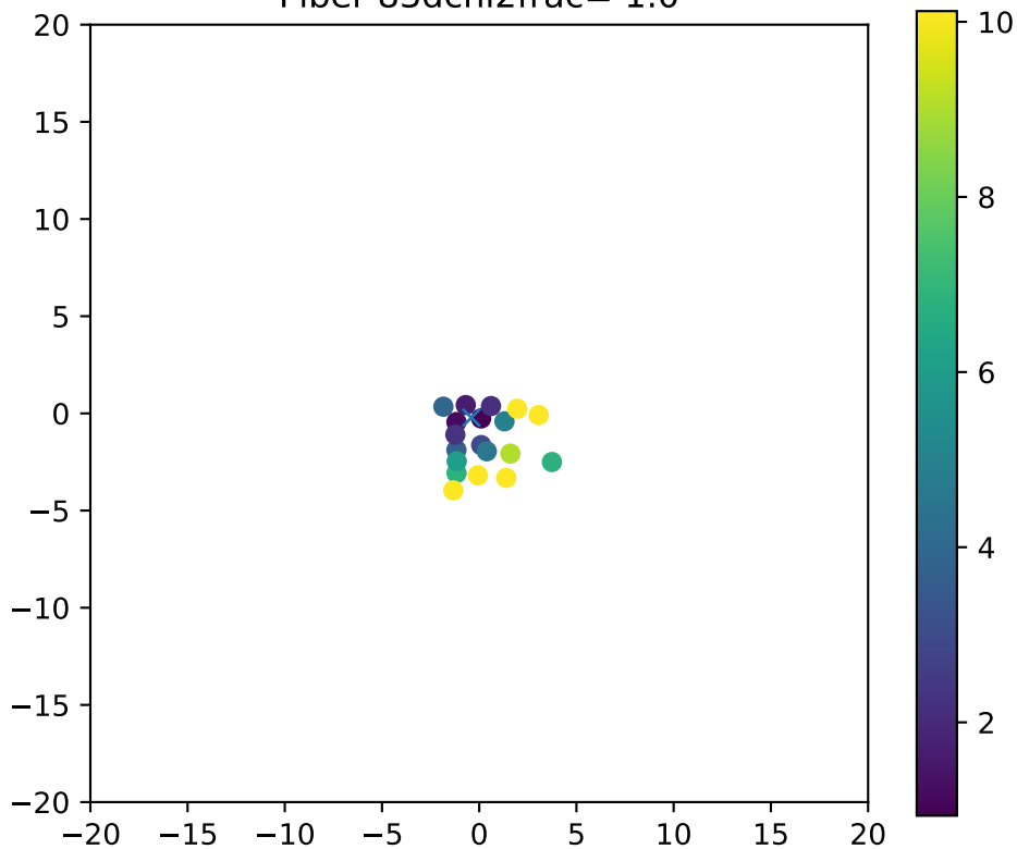
Fiber 83dchi2frac= 1.0
