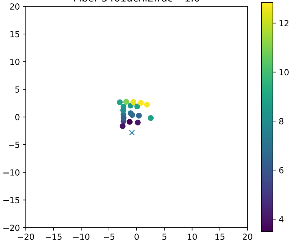
Fiber 3461dchi2frac= 1.0
