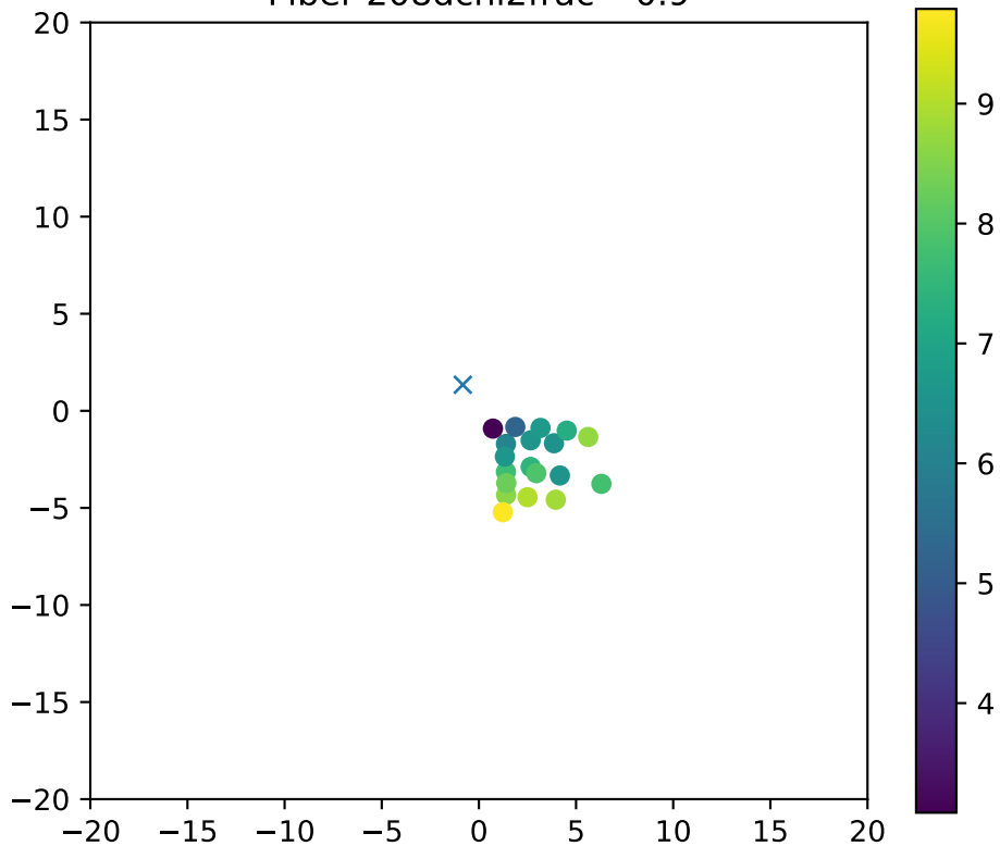
Fiber 208dchi2frac= 0.9
