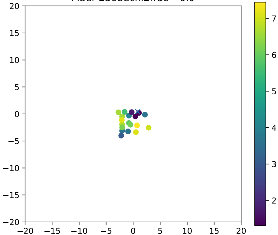
Fiber 2308dchi2frac= 0.9
