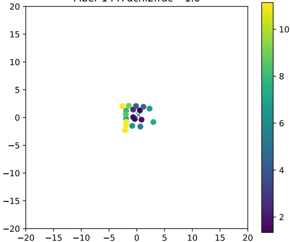
Fiber 1447dchi2frac= 1.0
