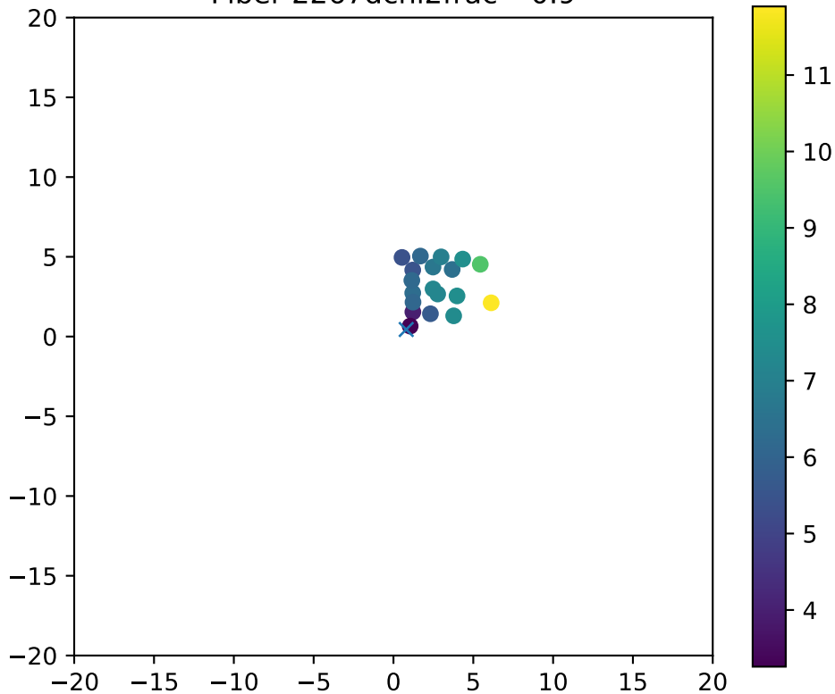
Fiber 2267dchi2frac= 0.9
