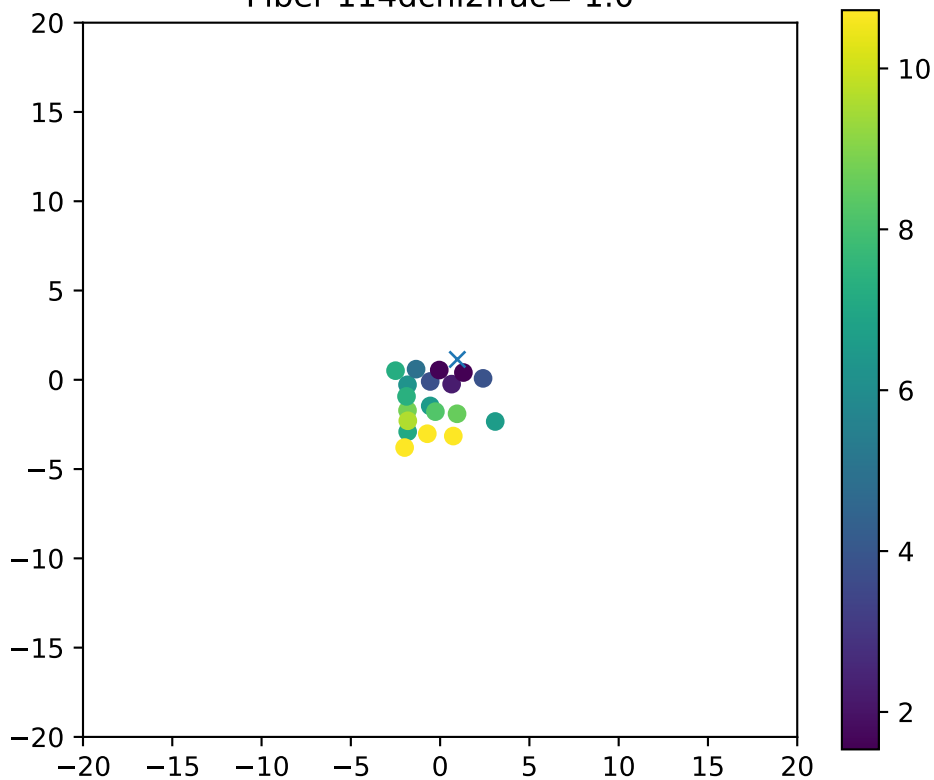
Fiber 114dchi2frac= 1.0
