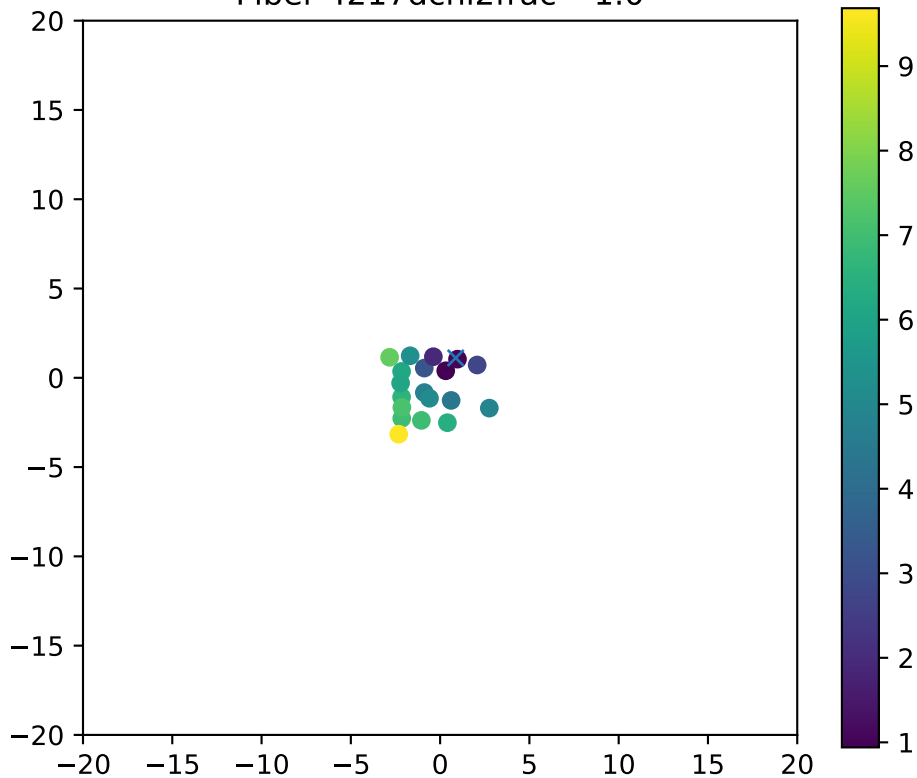
Fiber 4217dchi2frac= 1.0
