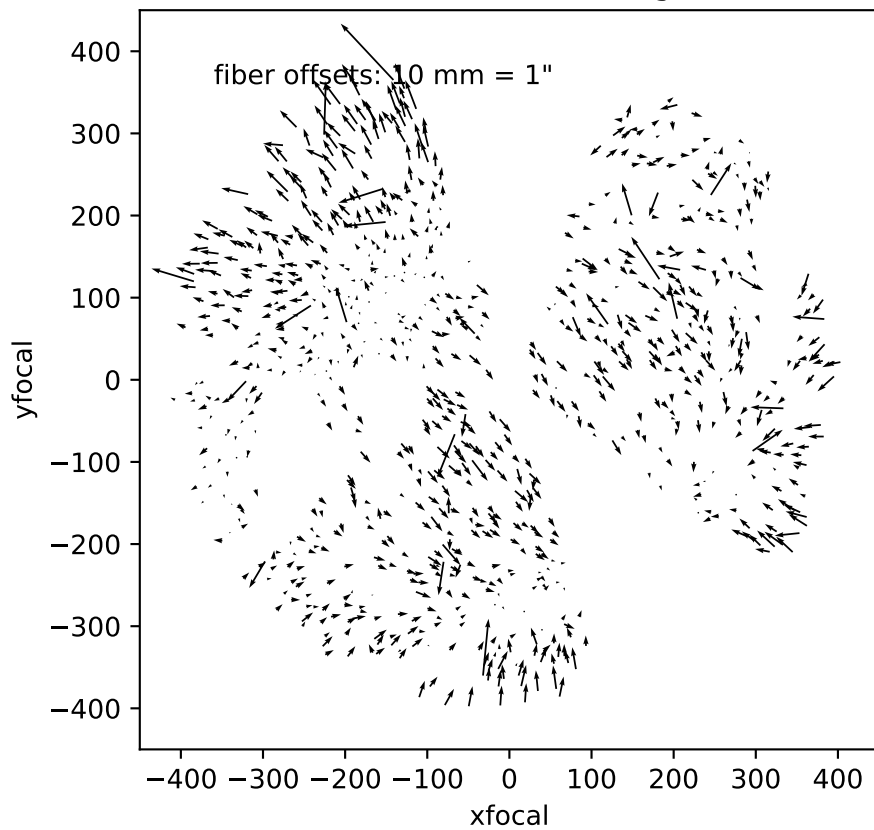
dither20200123-63076-highsnr-R
