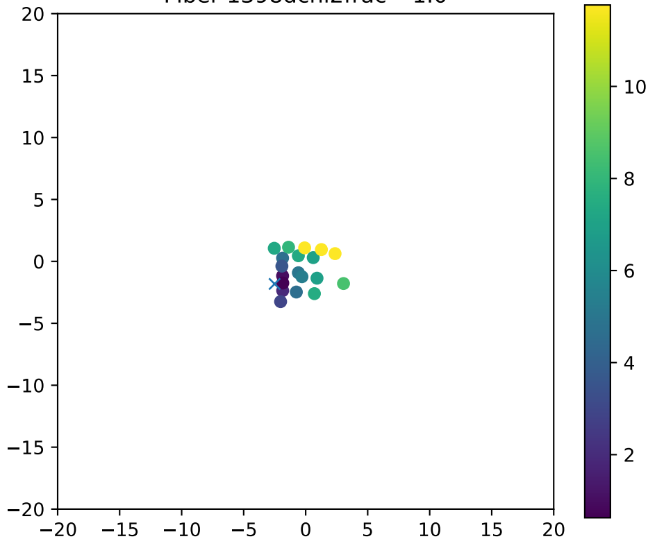
Fiber 1398dchi2frac= 1.0
