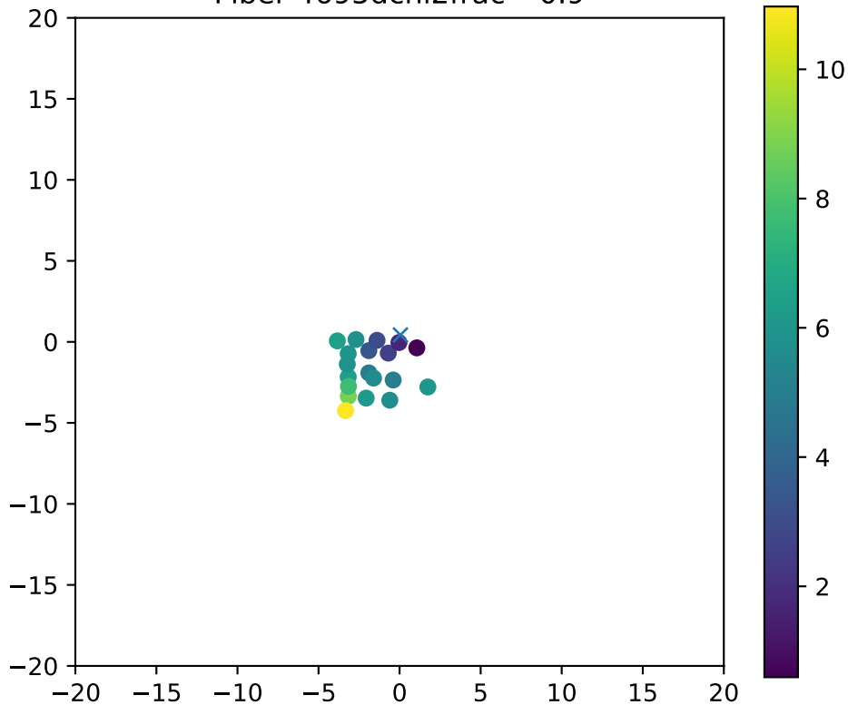
Fiber 4695dchi2frac= 0.9
