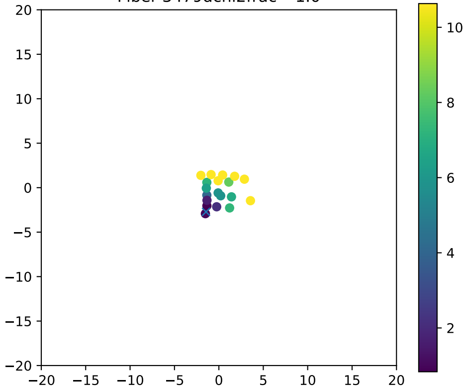
Fiber 3479dchi2frac= 1.0
