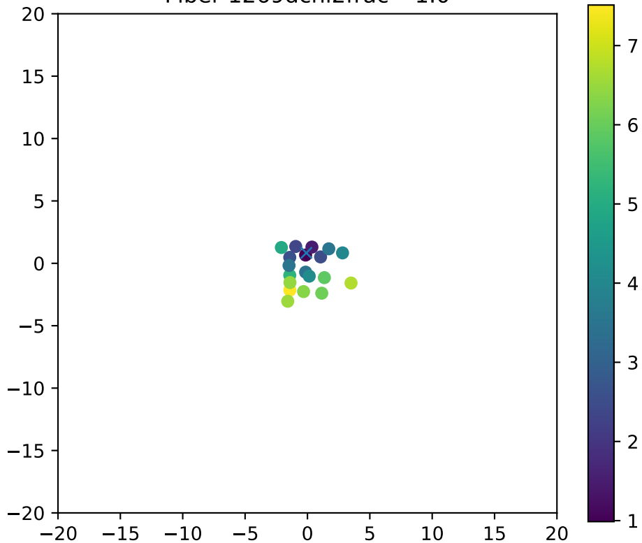
Fiber 1269dchi2frac= 1.0
