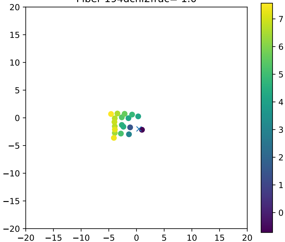
Fiber 194dchi2frac= 1.0
