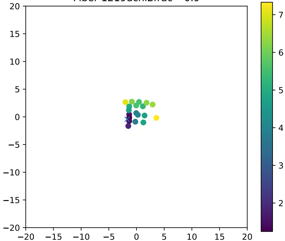
Fiber 1219dchi2frac= 0.9
