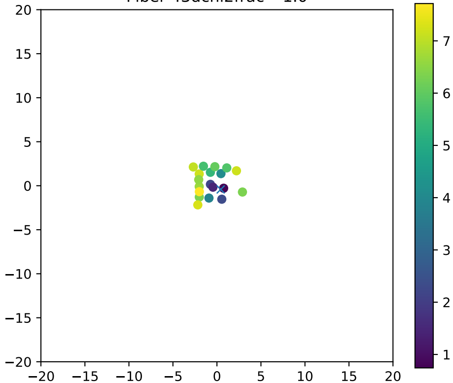
Fiber 43dchi2frac= 1.0
