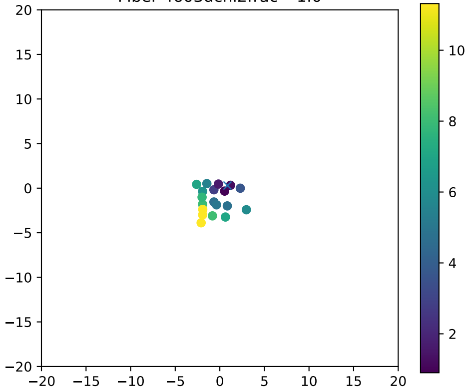
Fiber 4603dchi2frac= 1.0
