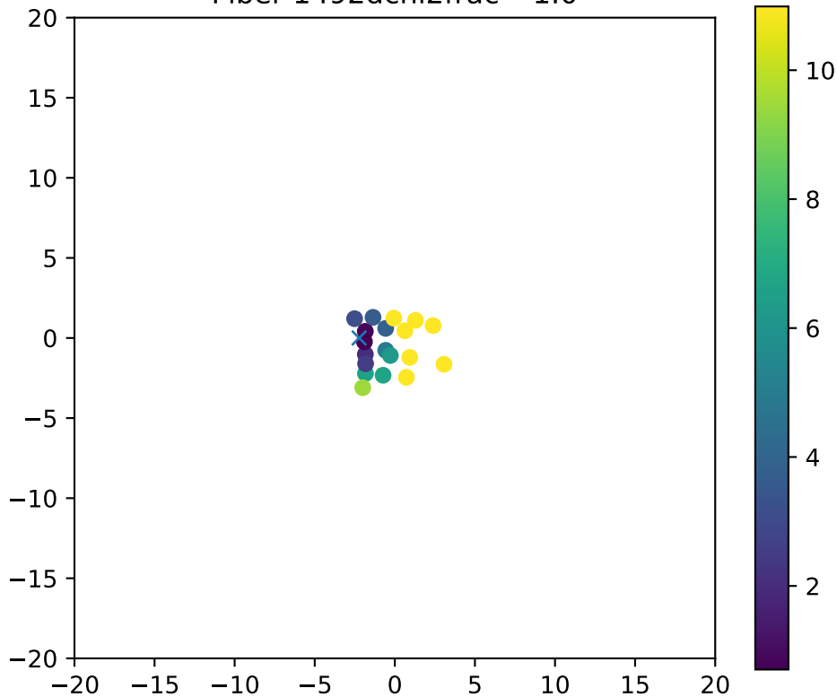
Fiber 1492dchi2frac= 1.0
