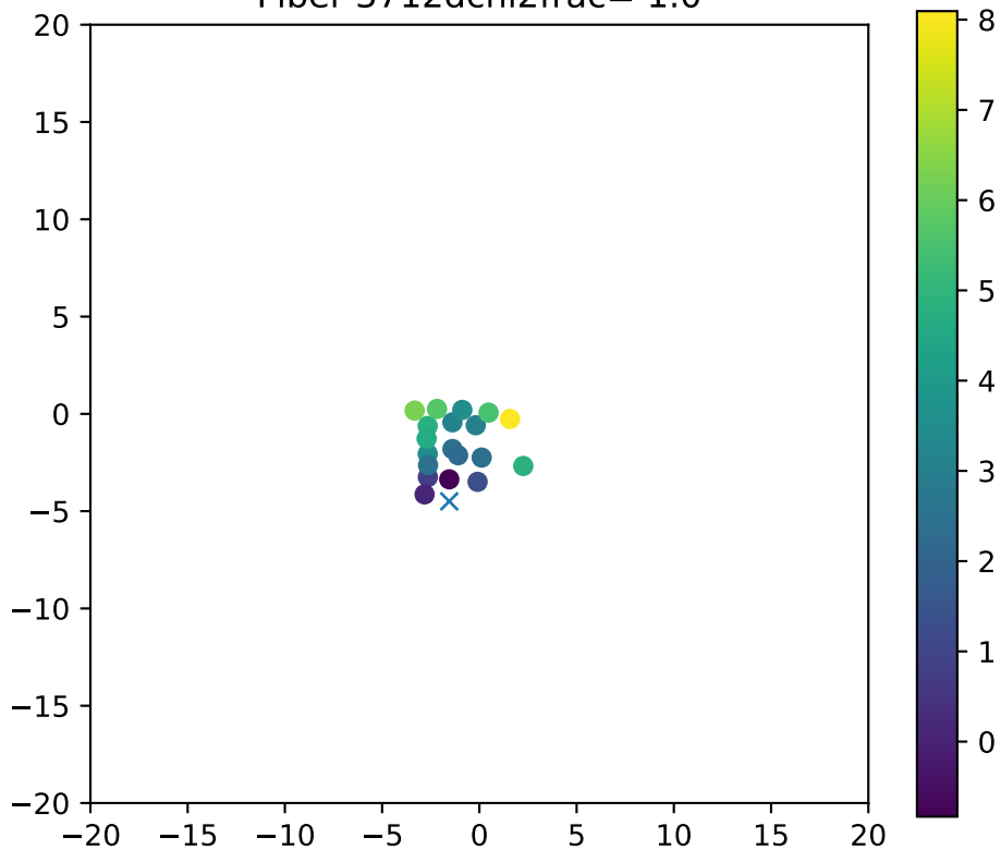
Fiber 3712dchi2frac= 1.0
