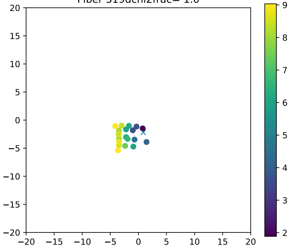
Fiber 319dchi2frac= 1.0
