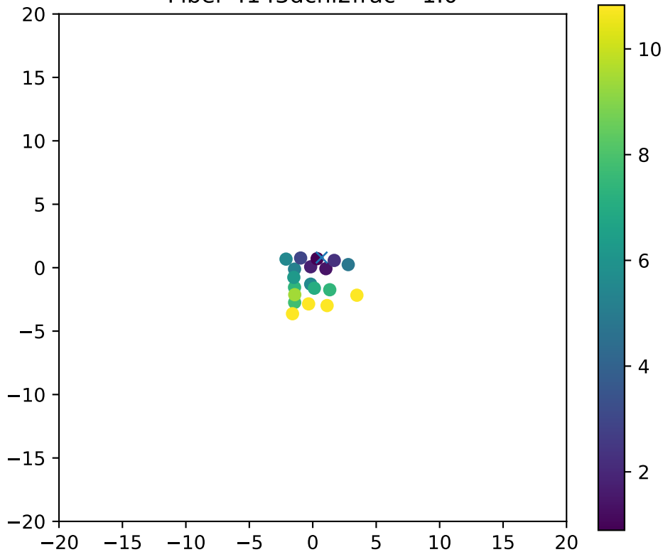
Fiber 4143dchi2frac= 1.0
