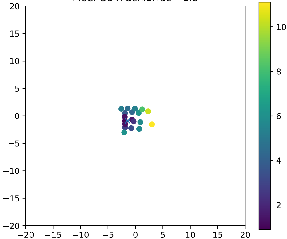
Fiber 3647dchi2frac= 1.0
