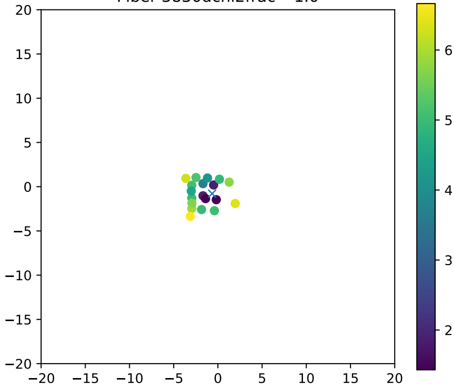
Fiber 3830dchi2frac= 1.0
