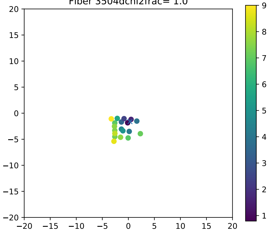
Fiber 3504dchi2frac= 1.0
