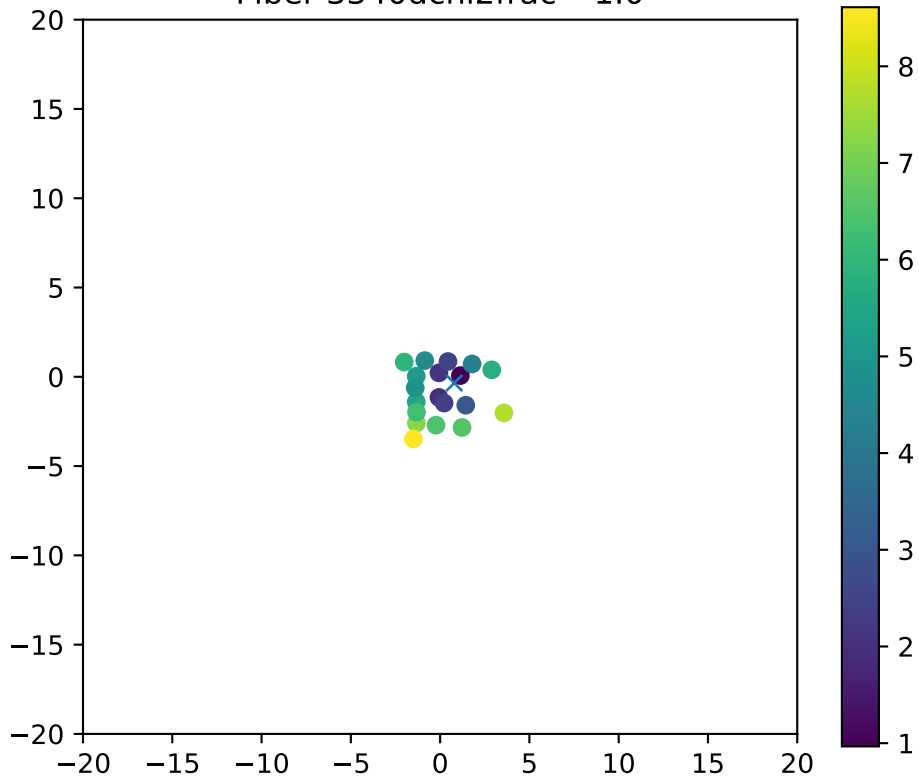
Fiber 3340dchi2frac= 1.0
