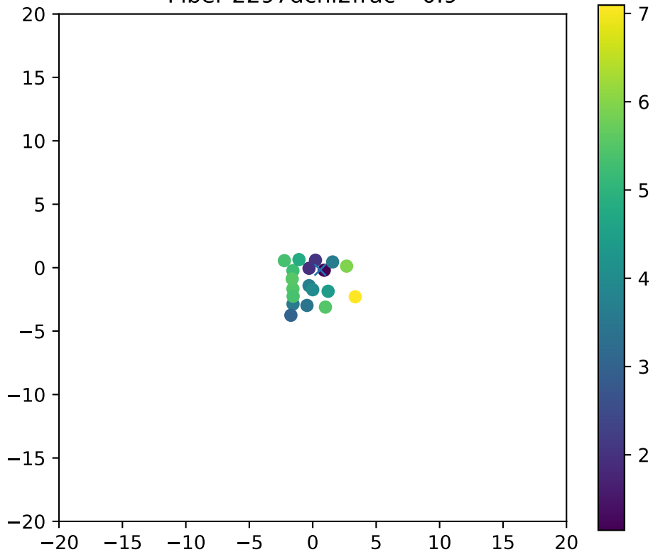
Fiber 2297dchi2frac= 0.9
