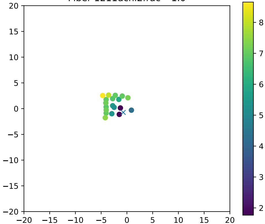
Fiber 1211dchi2frac= 1.0
