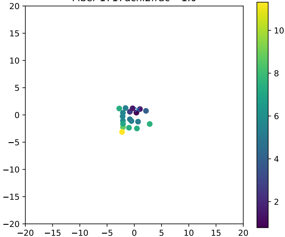
Fiber 1717dchi2frac= 1.0
