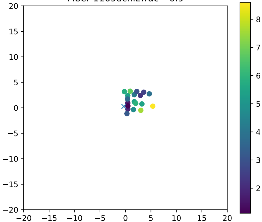
Fiber 1169dchi2frac= 0.9
