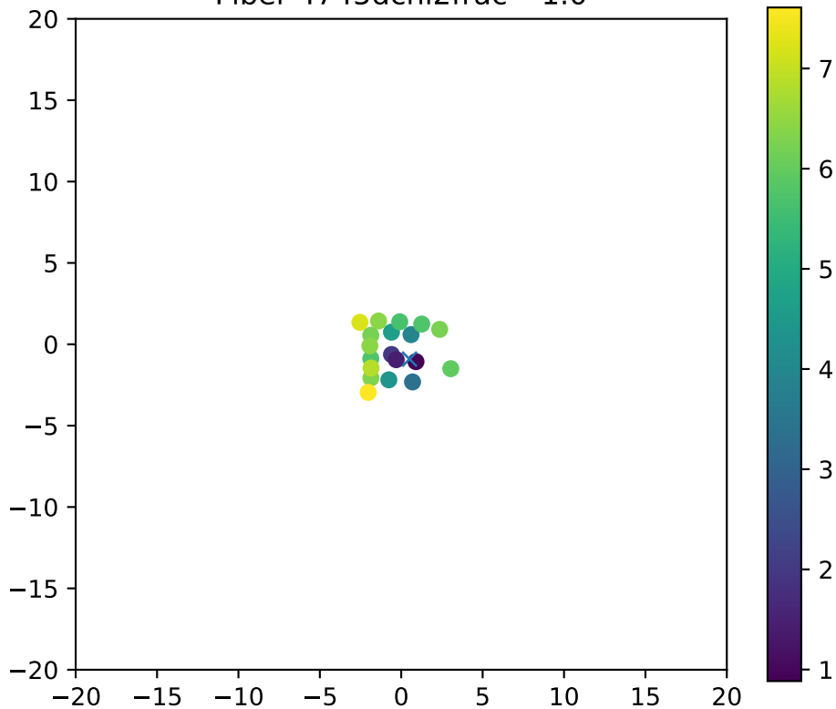
Fiber 4745dchi2frac= 1.0
