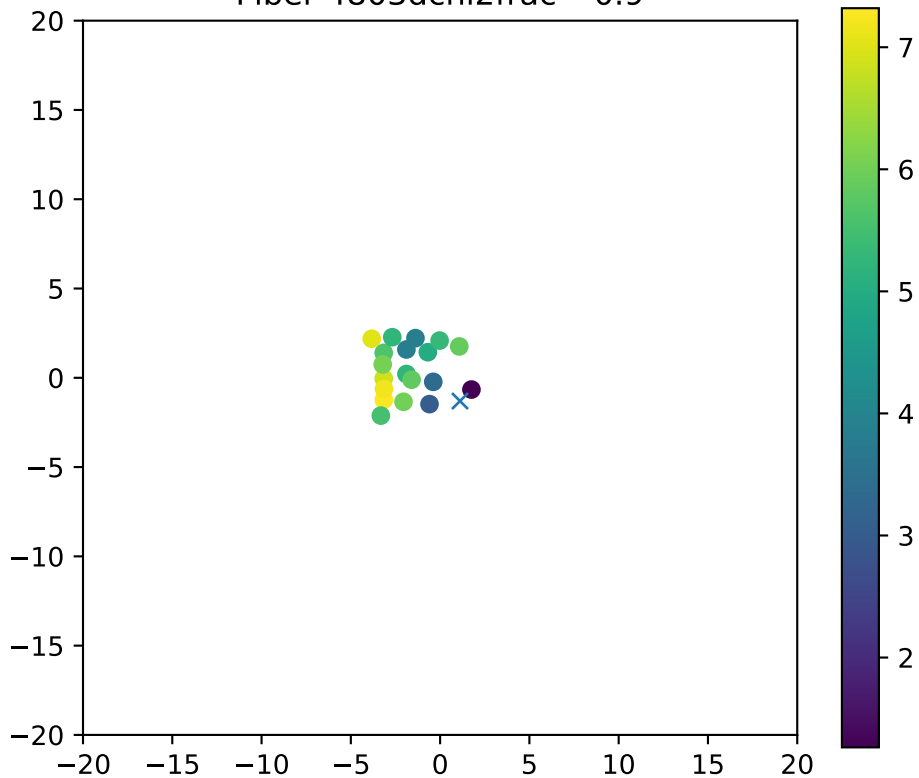
Fiber 4803dchi2frac= 0.9
