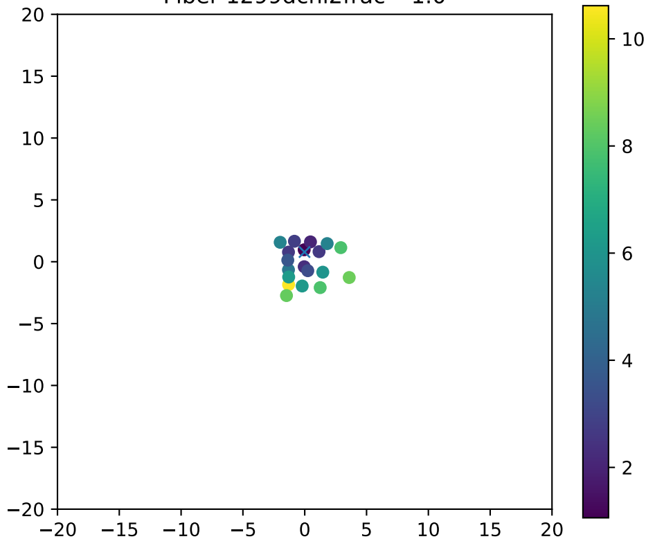
Fiber 1299dchi2frac= 1.0
