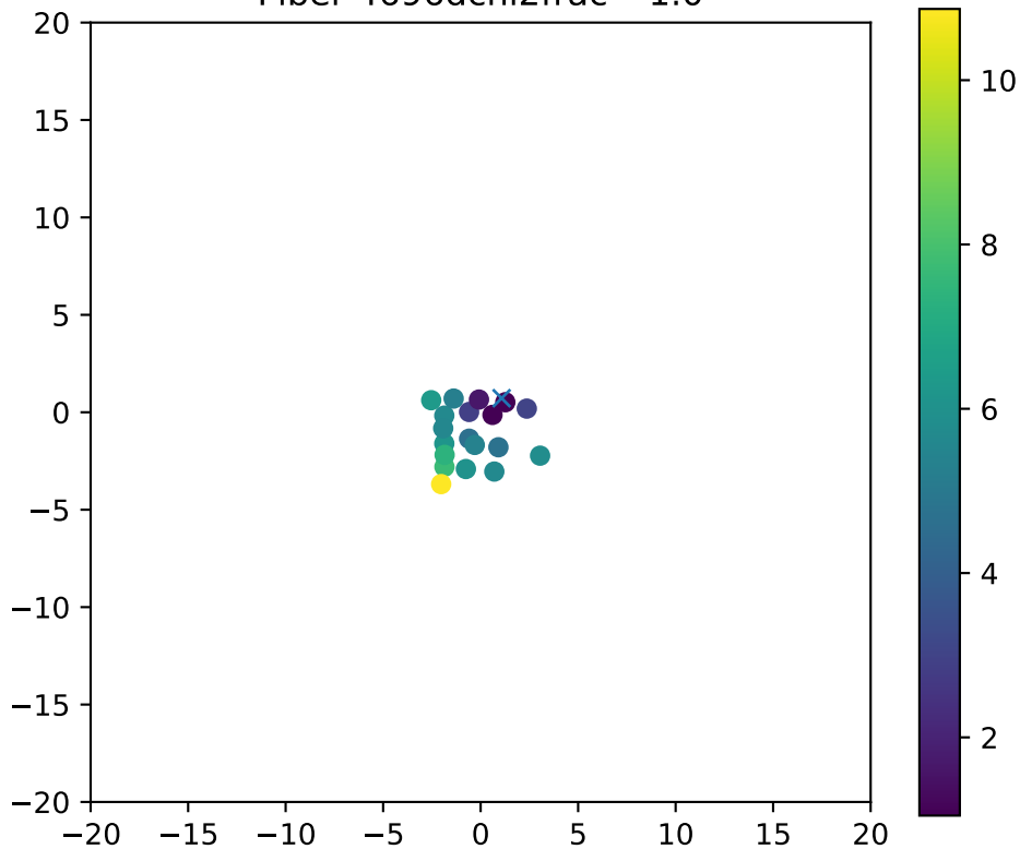
Fiber 4696dchi2frac= 1.0
