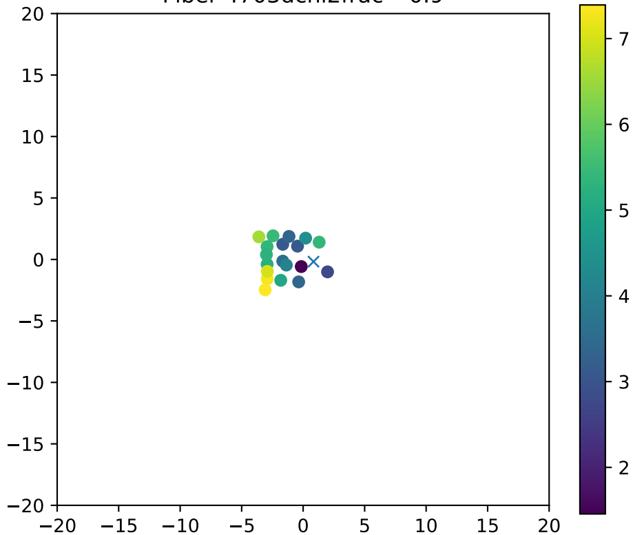
Fiber 4703dchi2frac= 0.9
