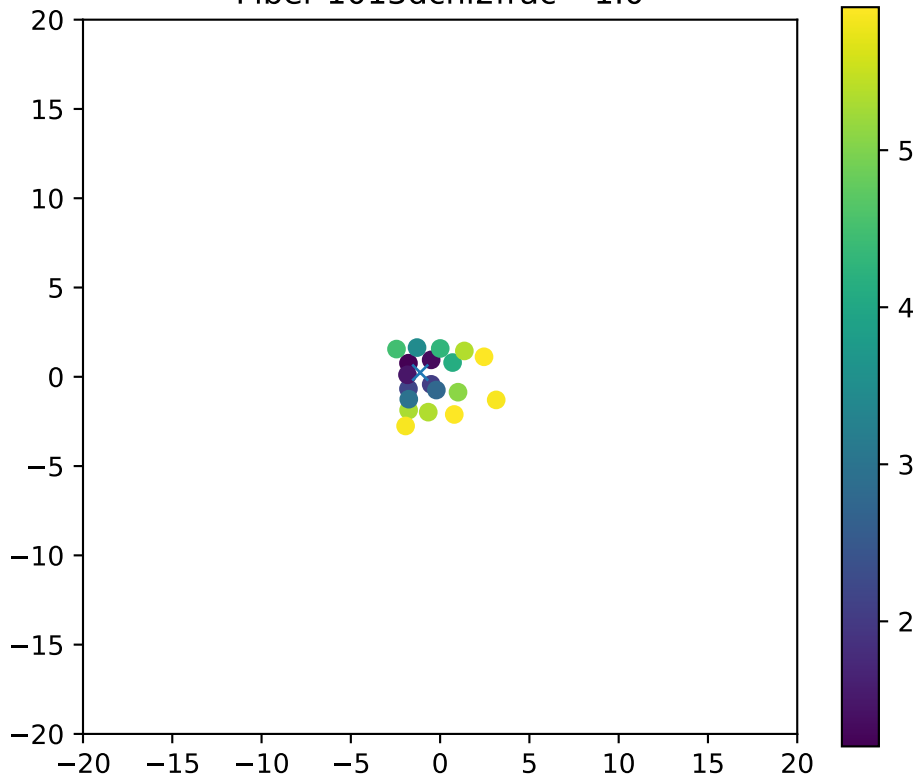
Fiber 1013dchi2frac= 1.0
