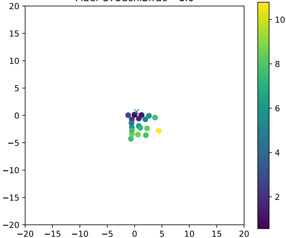
Fiber 375dchi2frac= 1.0
