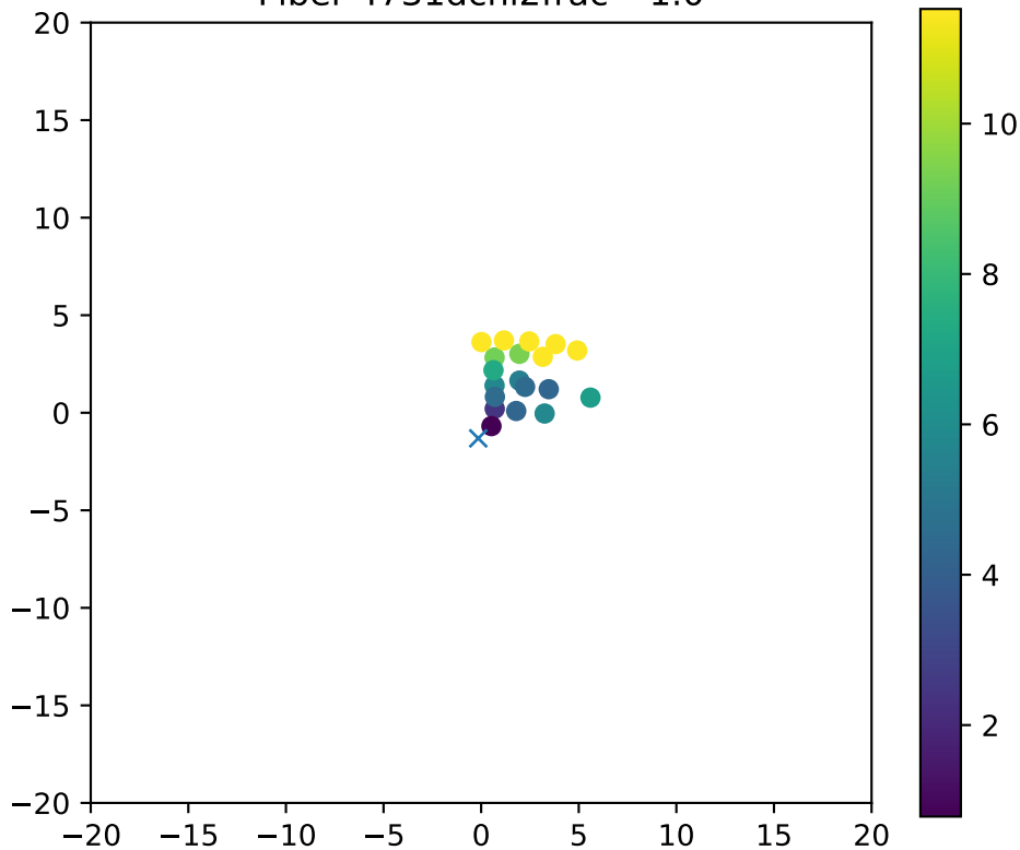
Fiber 4731dchi2frac= 1.0
