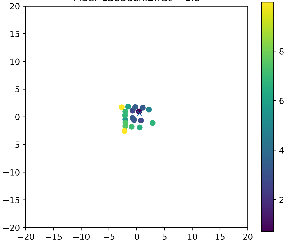
Fiber 1585dchi2frac= 1.0
