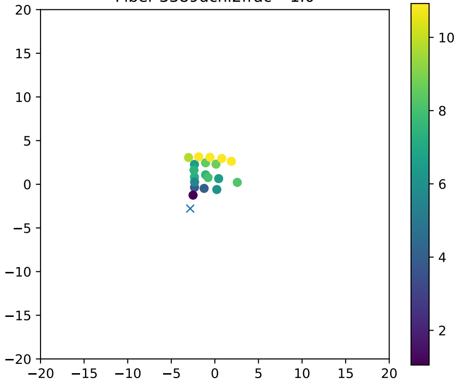
Fiber 3389dchi2frac= 1.0
