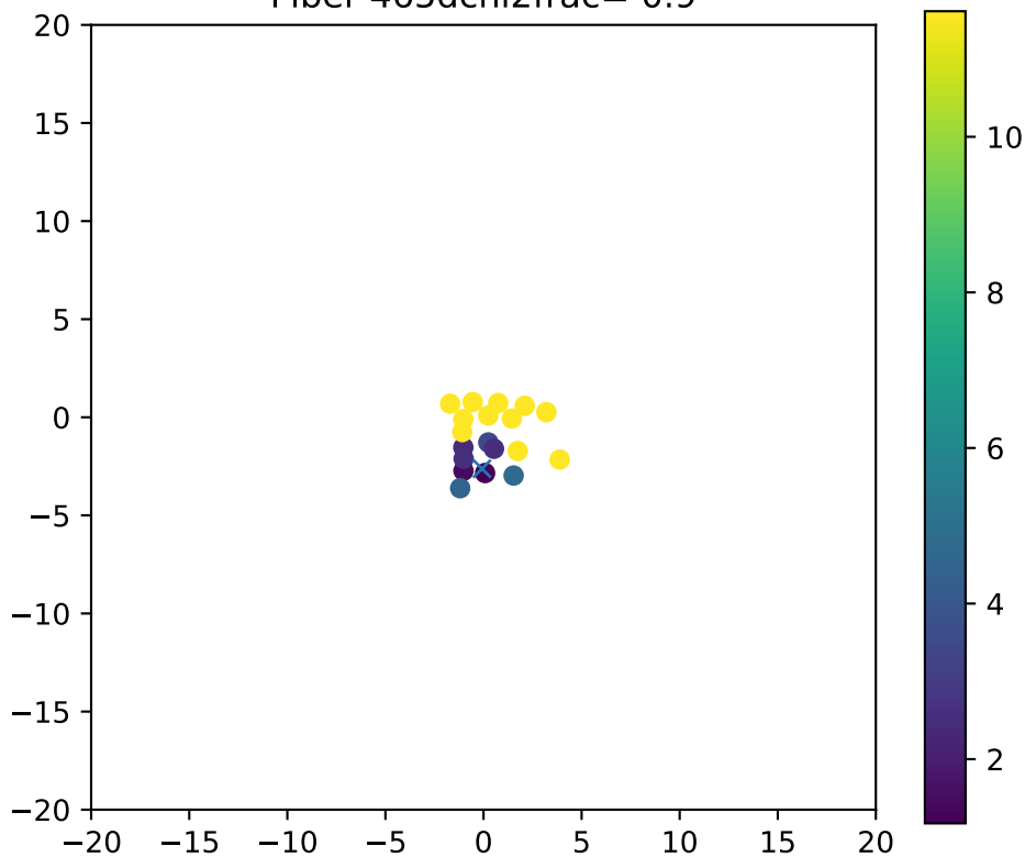
Fiber 465dchi2frac= 0.9
