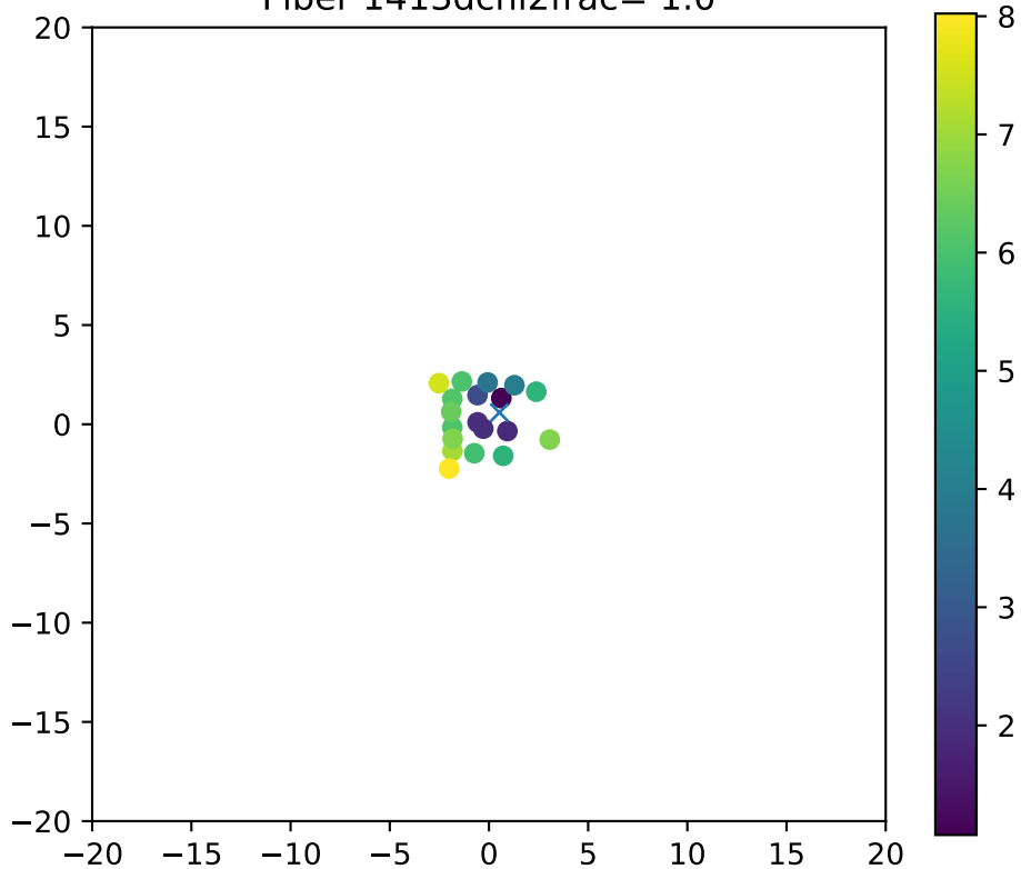
Fiber 1413dchi2frac= 1.0
