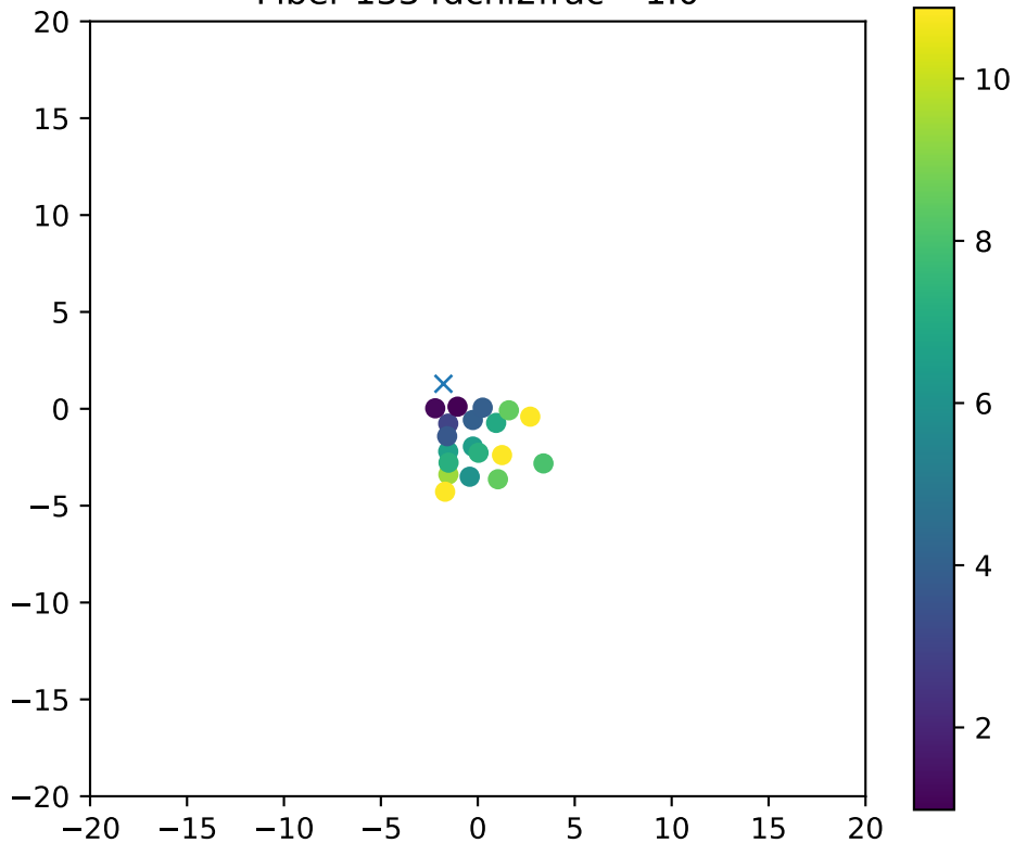
Fiber 1334dchi2frac= 1.0
