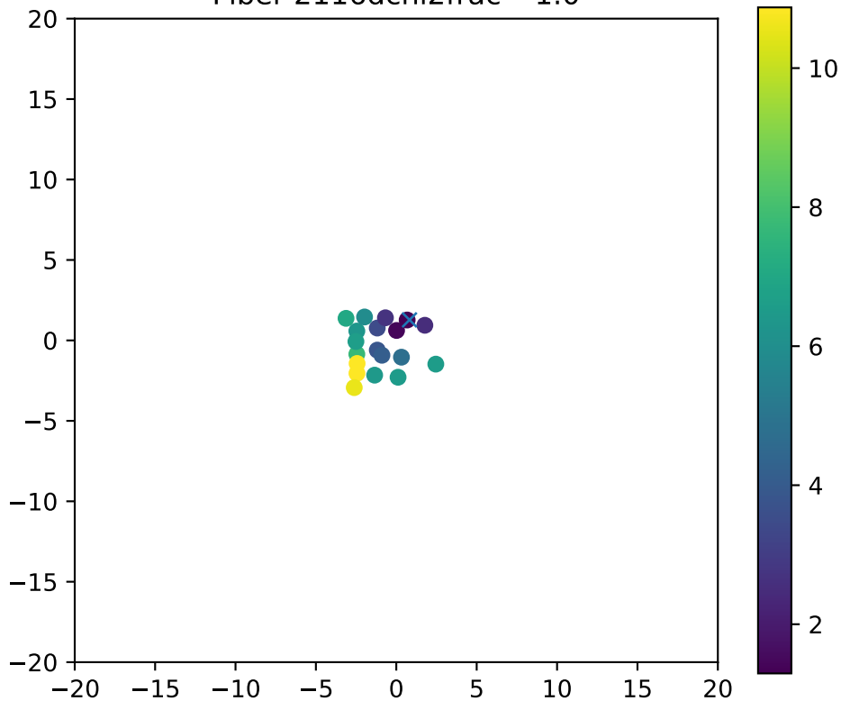
Fiber 2116dchi2frac= 1.0
