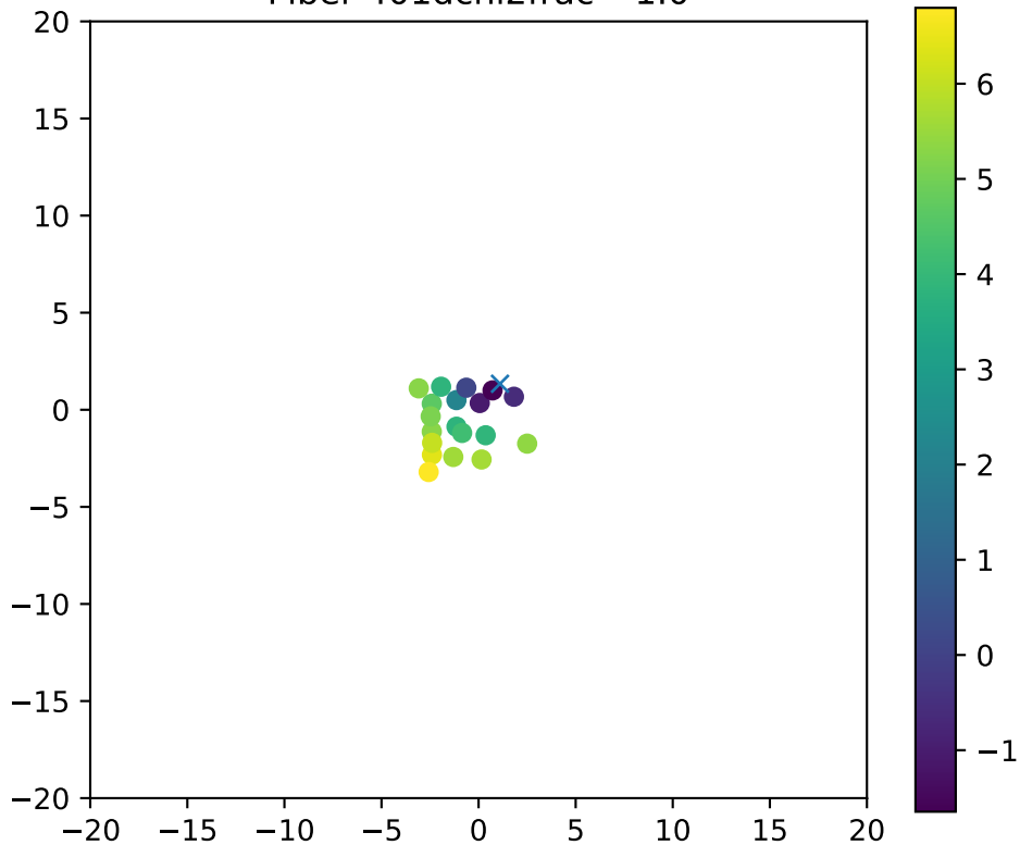
Fiber 401dchi2frac= 1.0
