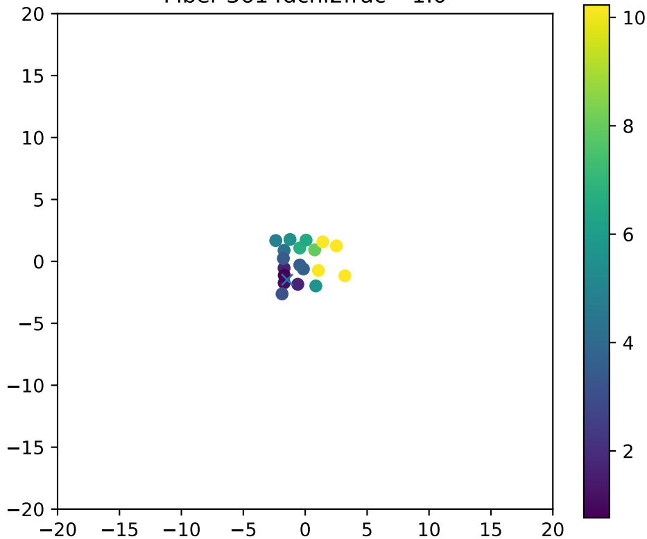
Fiber 3614dchi2frac= 1.0
