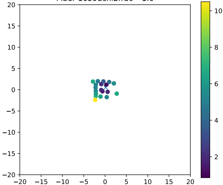
Fiber 1659dchi2frac= 1.0
