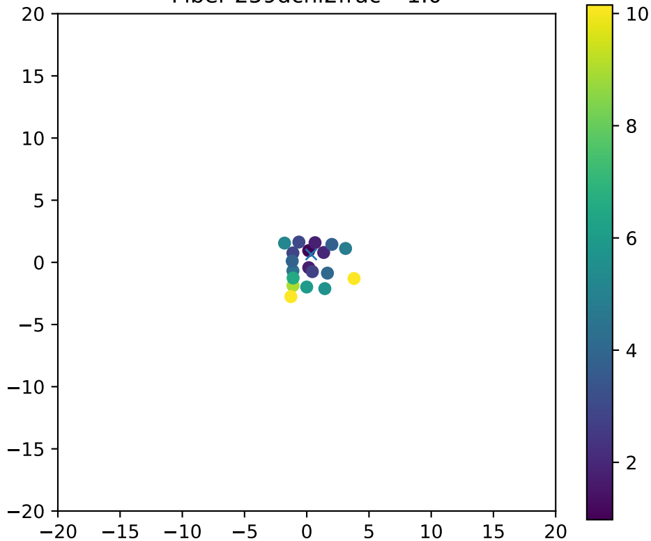
Fiber 259dchi2frac= 1.0
