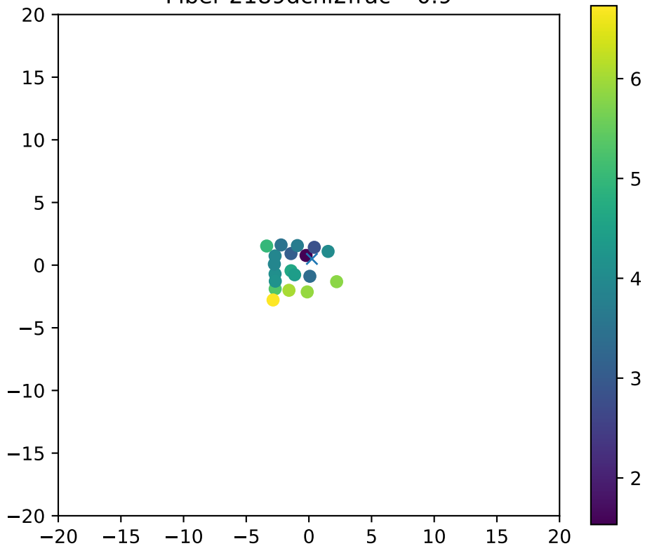
Fiber 2189dchi2frac= 0.9
