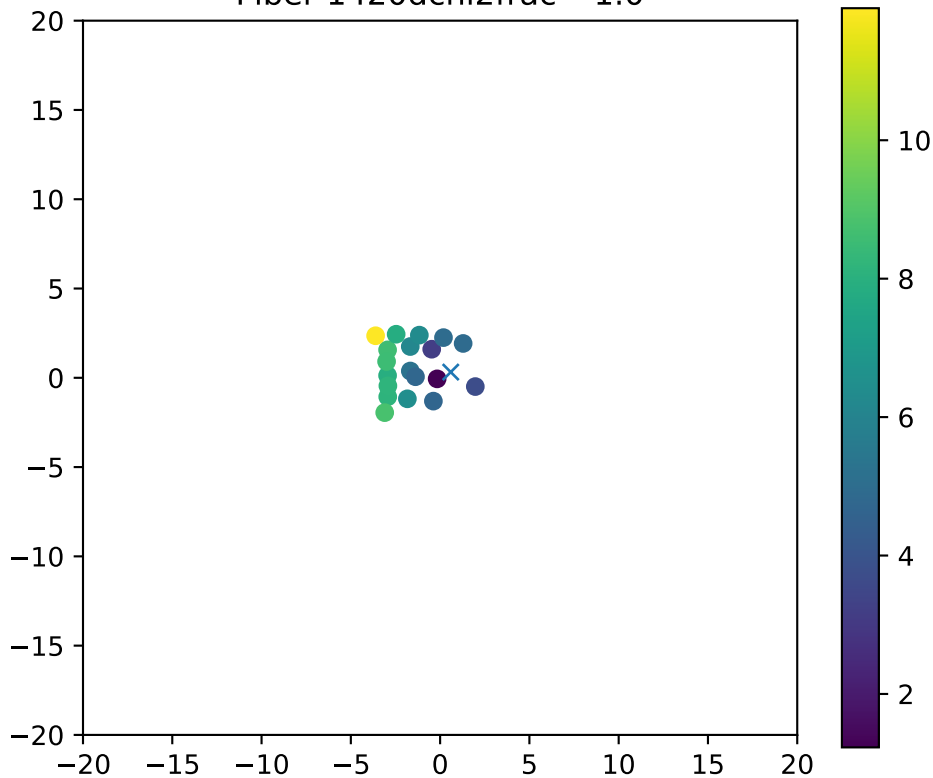
Fiber 1420dchi2frac= 1.0
