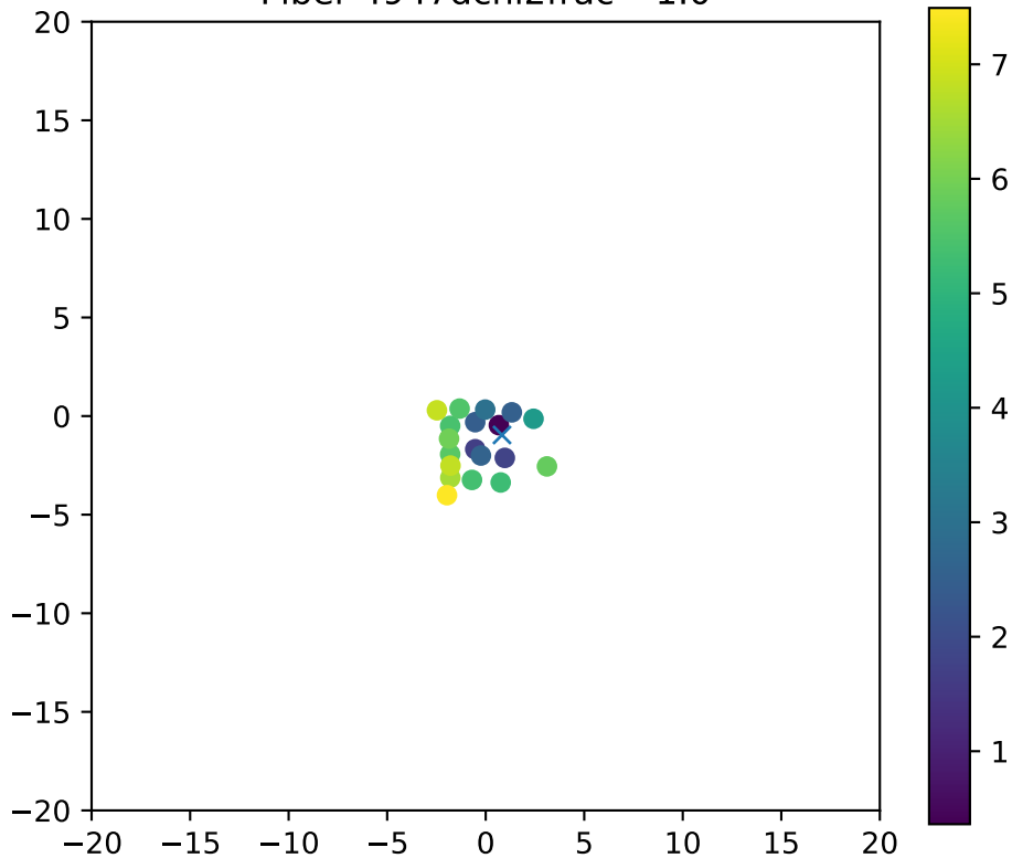
Fiber 4947dchi2frac= 1.0
