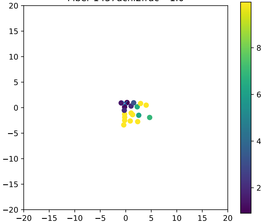
Fiber 1437dchi2frac= 1.0
