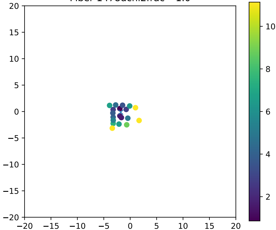
Fiber 1478dchi2frac= 1.0
