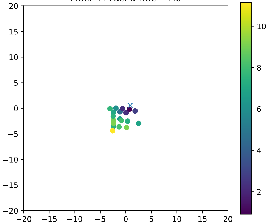
Fiber 117dchi2frac= 1.0
