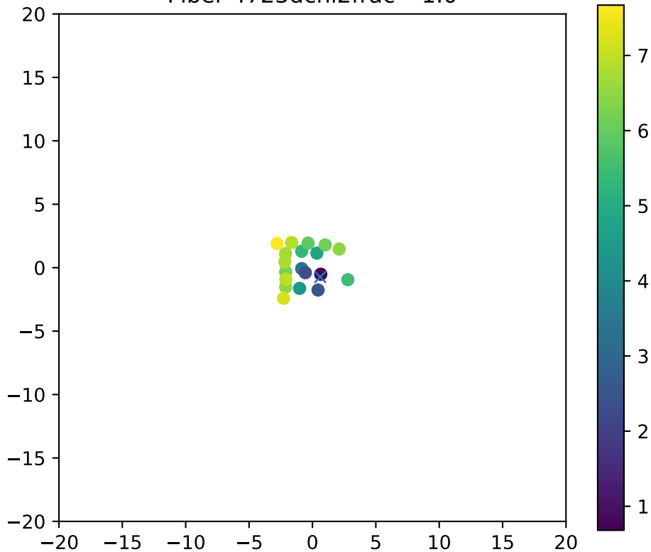
Fiber 4723dchi2frac= 1.0
