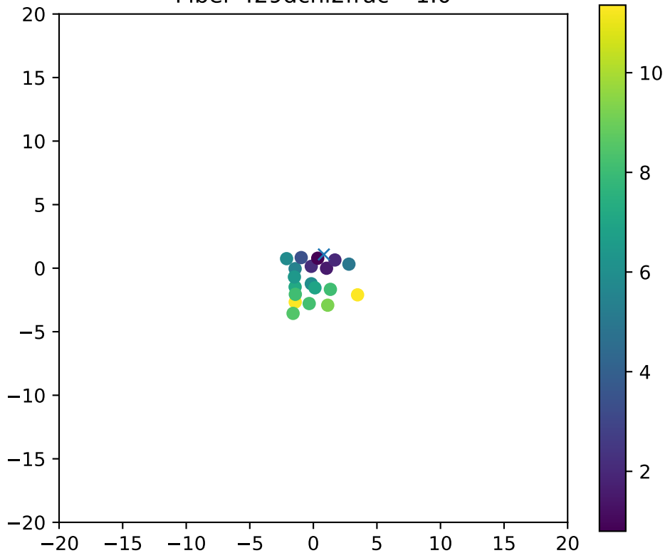
Fiber 429dchi2frac= 1.0
