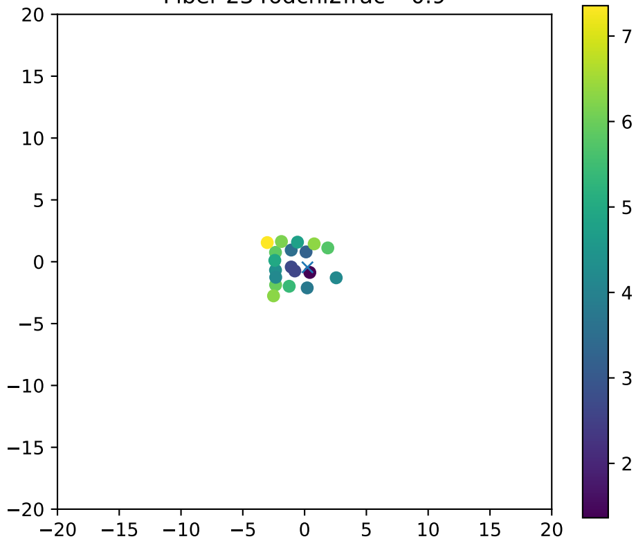
Fiber 2346dchi2frac= 0.9
