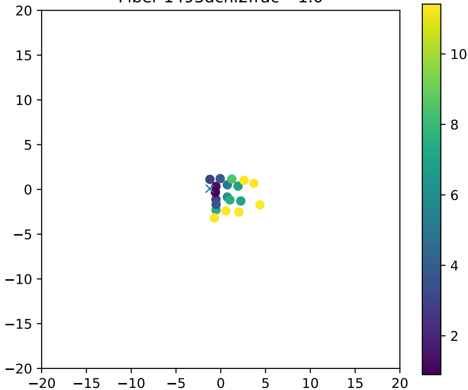
Fiber 1493dchi2frac= 1.0
