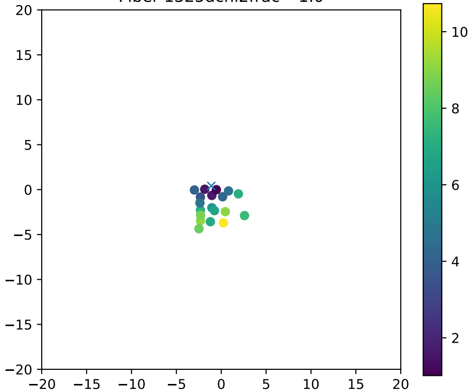
Fiber 1325dchi2frac= 1.0
