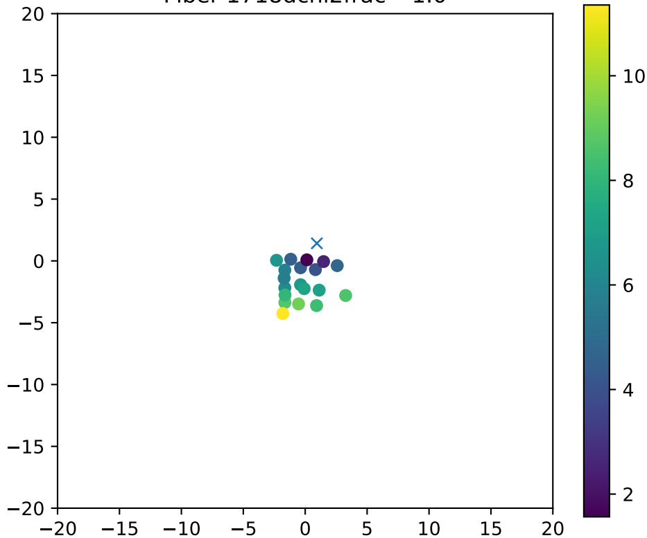
Fiber 1718dchi2frac= 1.0
