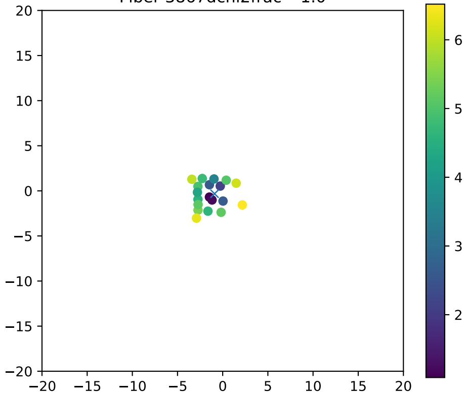
Fiber 3867dchi2frac= 1.0
