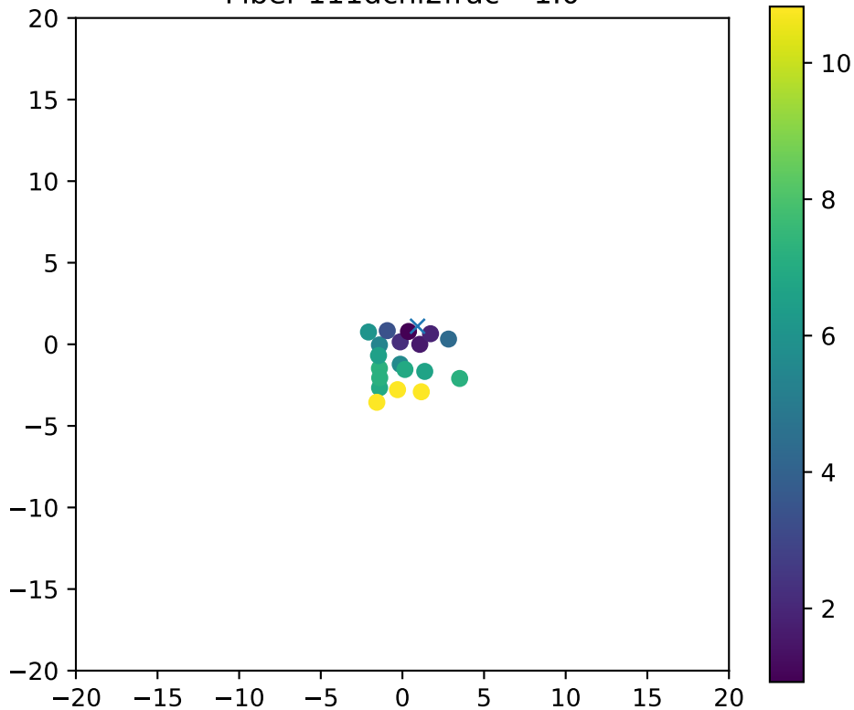
Fiber 111dchi2frac= 1.0
