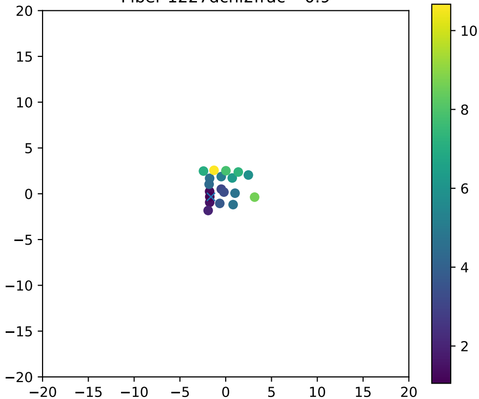
Fiber 1227dchi2frac= 0.9
