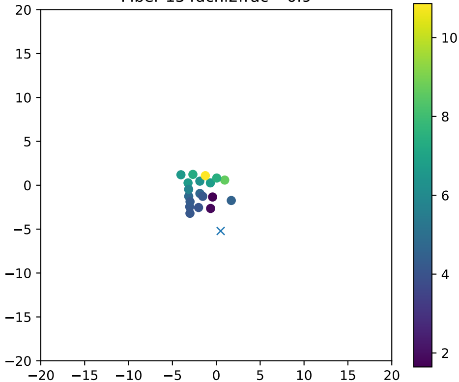
Fiber 154dchi2frac= 0.9
