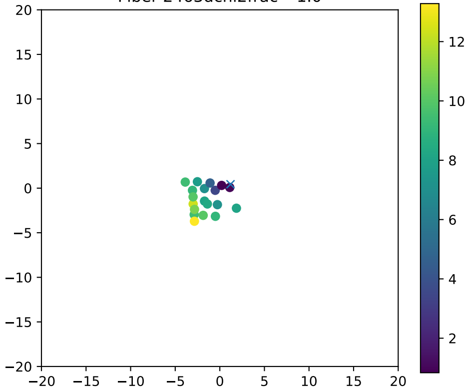
Fiber 2463dchi2frac= 1.0
