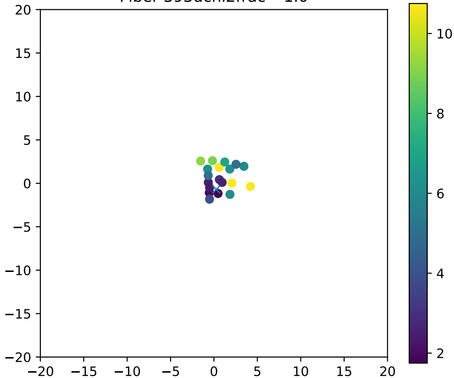
Fiber 393dchi2frac= 1.0
