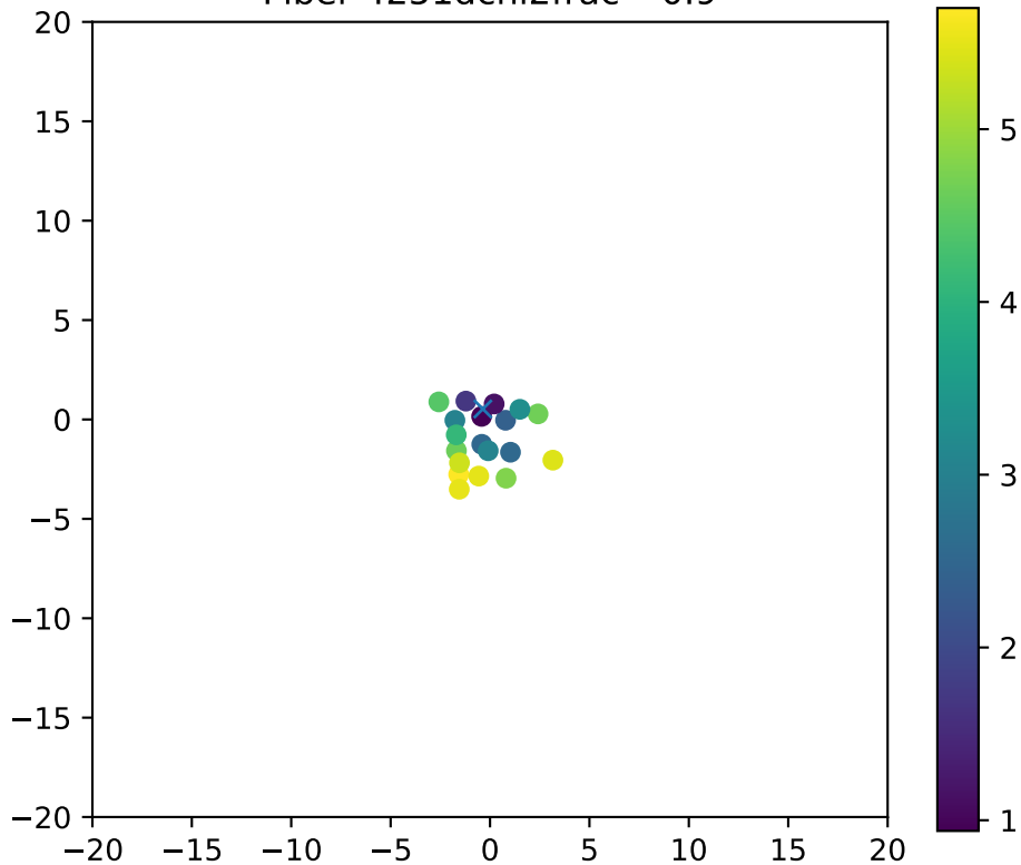
Fiber 4251dchi2frac= 0.9
