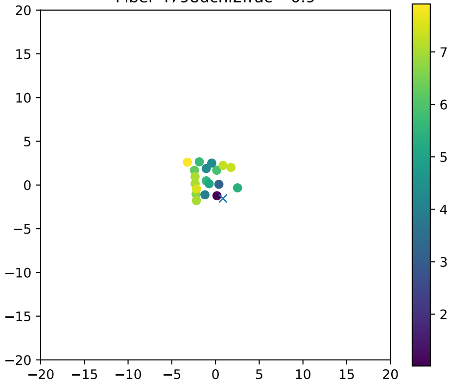
Fiber 4798dchi2frac= 0.9
