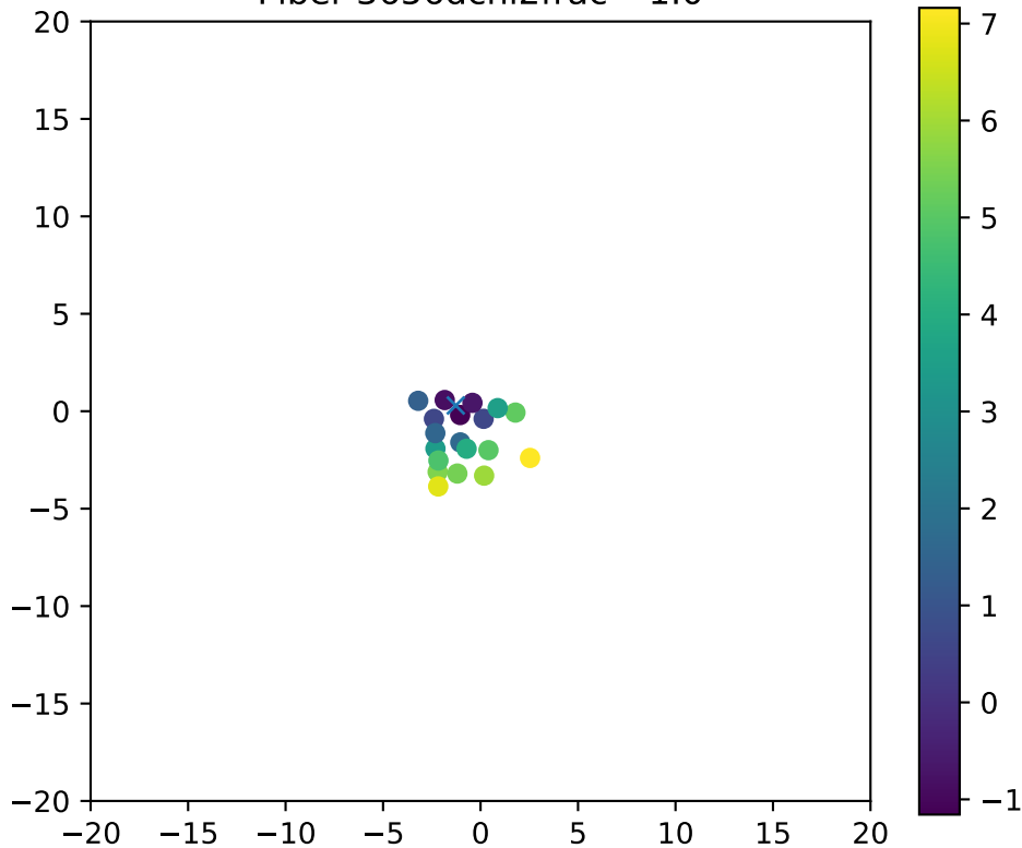
Fiber 3656dchi2frac= 1.0
