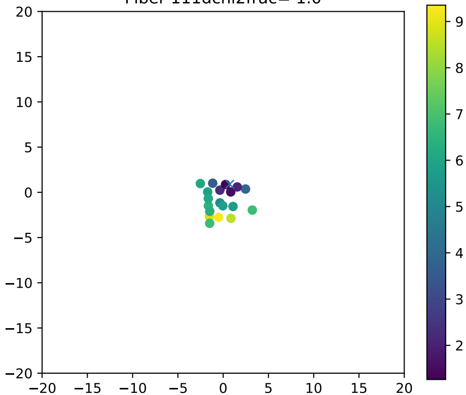
Fiber 111dchi2frac= 1.0
