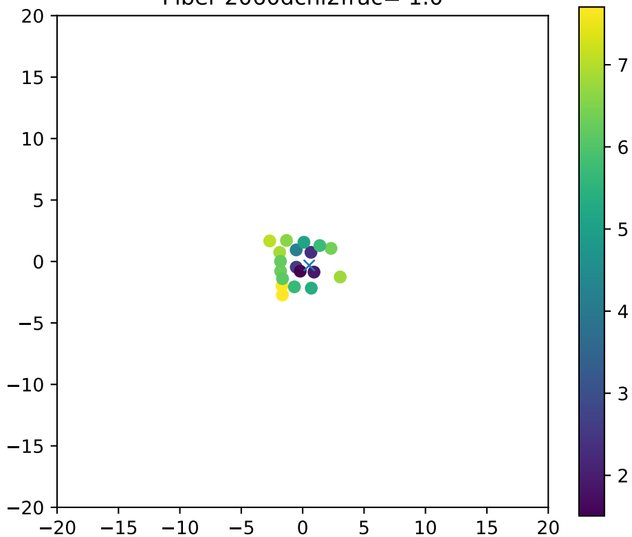
Fiber 2060dchi2frac= 1.0
