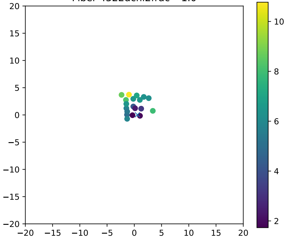
Fiber 4322dchi2frac= 1.0
