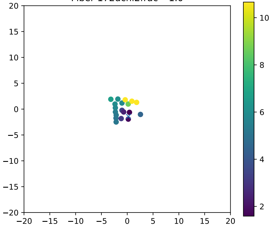
Fiber 172dchi2frac= 1.0
