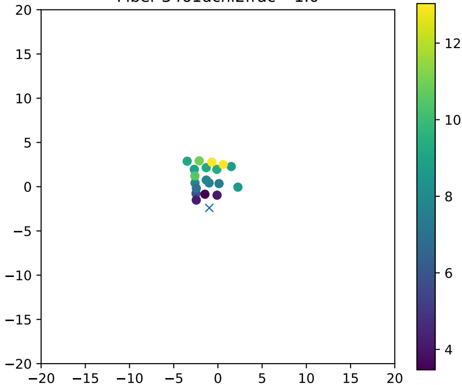
Fiber 3461dchi2frac= 1.0
