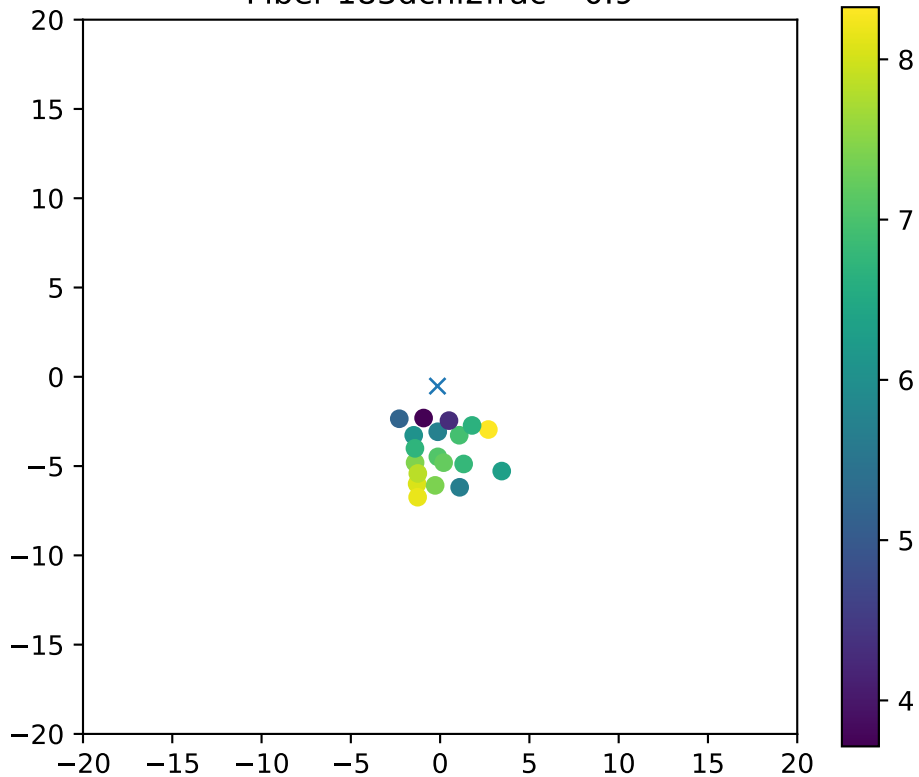
Fiber 183dchi2frac= 0.9
