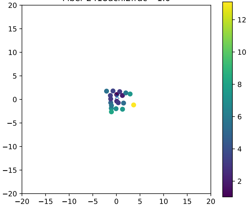
Fiber 2418dchi2frac= 1.0
