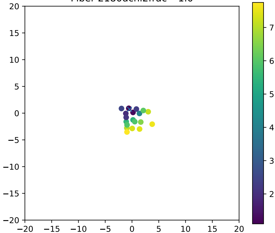
Fiber 2180dchi2frac= 1.0
