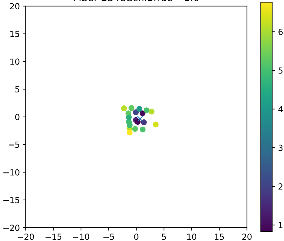
Fiber 2348dchi2frac= 1.0
