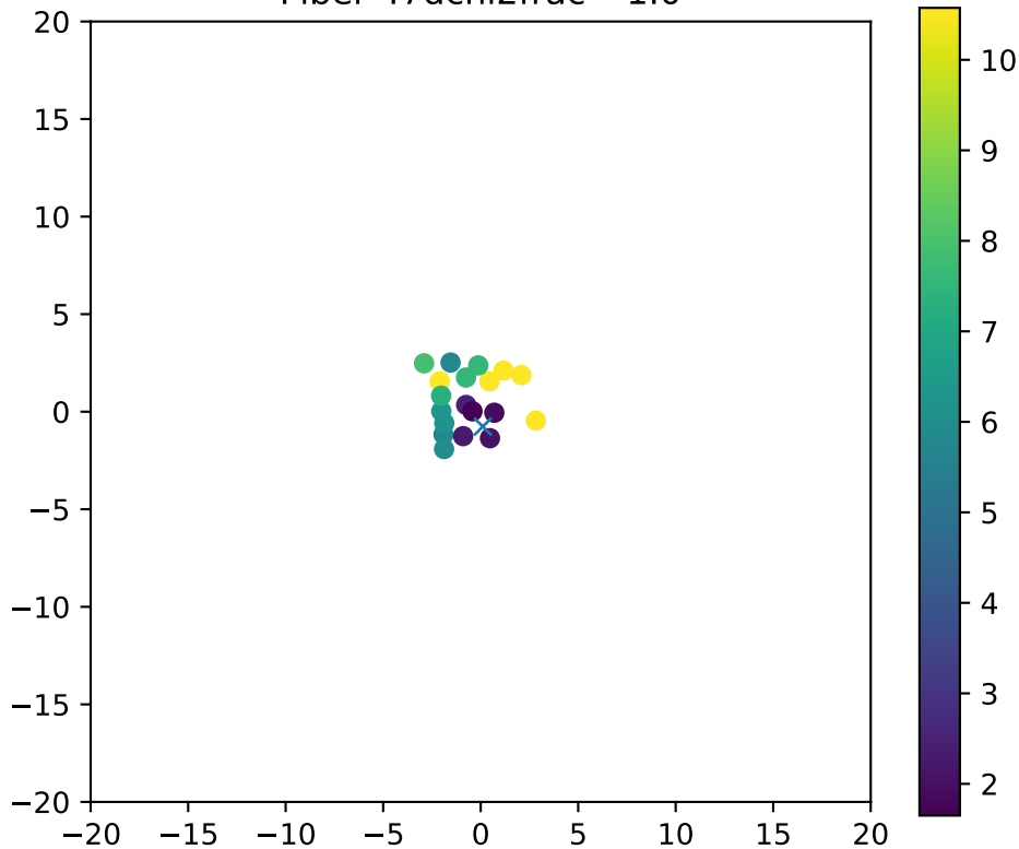
Fiber 47dchi2frac= 1.0
