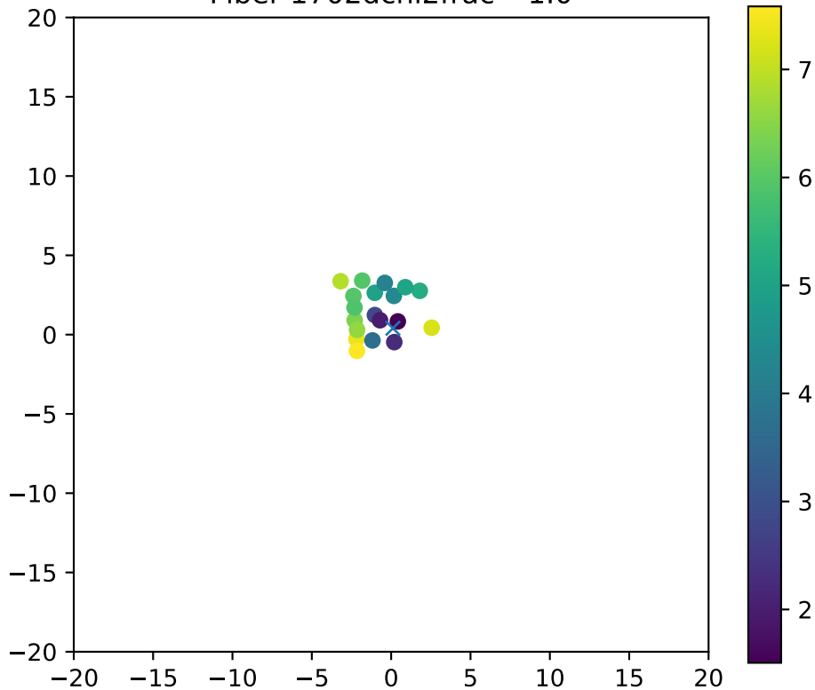
Fiber 1702dchi2frac= 1.0
