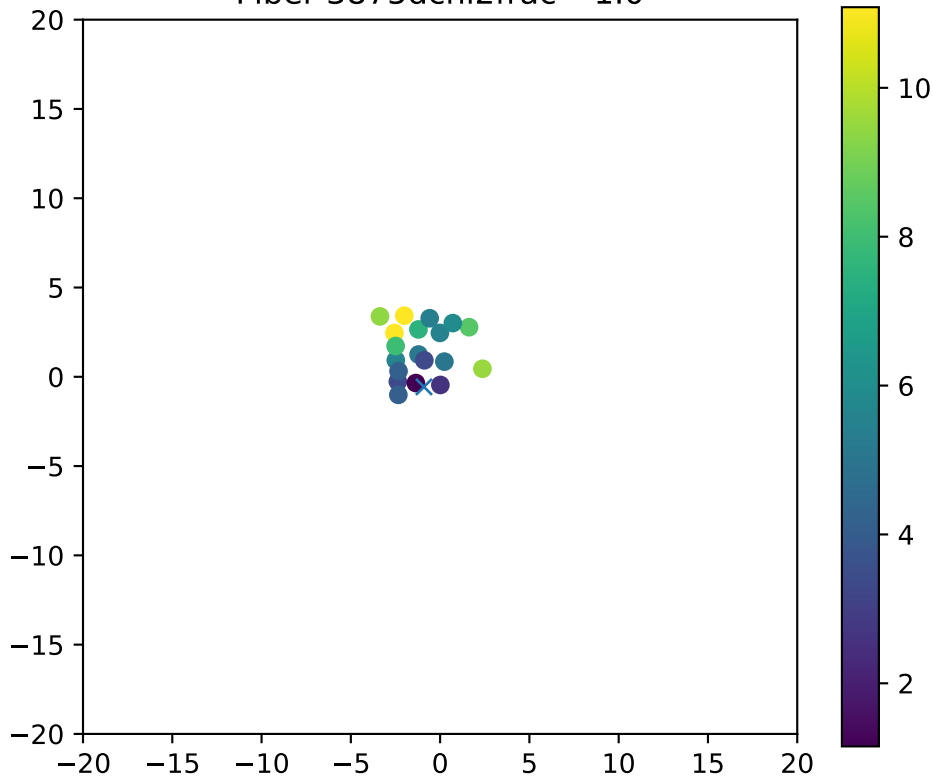
Fiber 3875dchi2frac= 1.0
