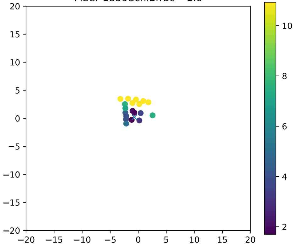
Fiber 1859dchi2frac= 1.0
