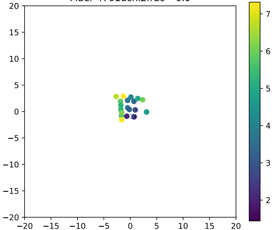
Fiber 4701dchi2frac= 0.9
