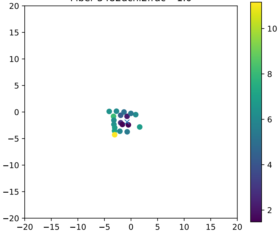
Fiber 3482dchi2frac= 1.0
