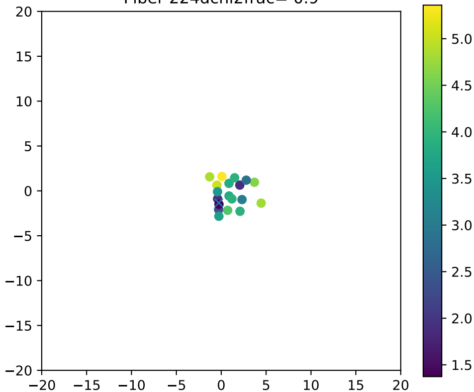
Fiber 224dchi2frac= 0.9
