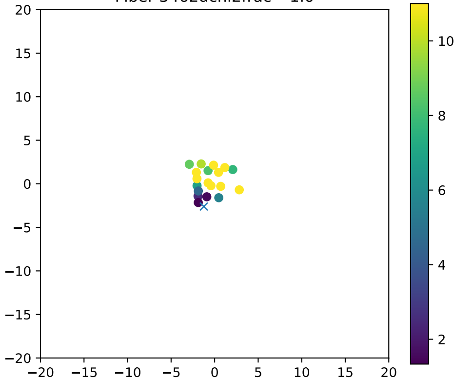
Fiber 3462dchi2frac= 1.0
