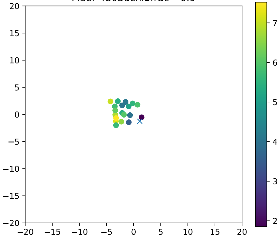
Fiber 4803dchi2frac= 0.9
