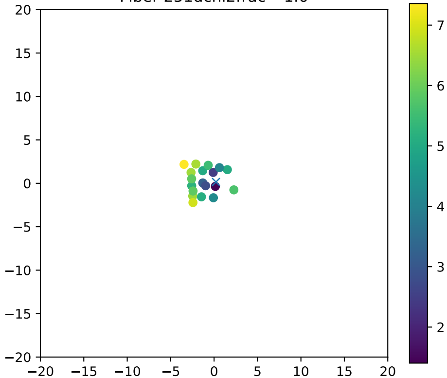
Fiber 251dchi2frac= 1.0
