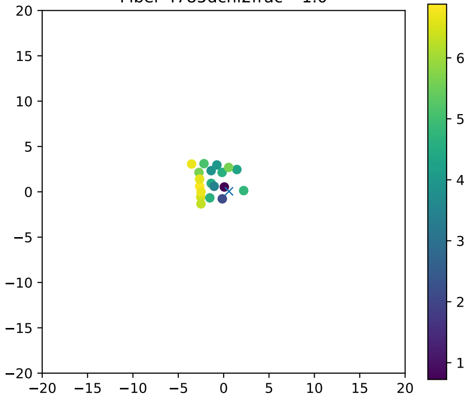
Fiber 4785dchi2frac= 1.0
