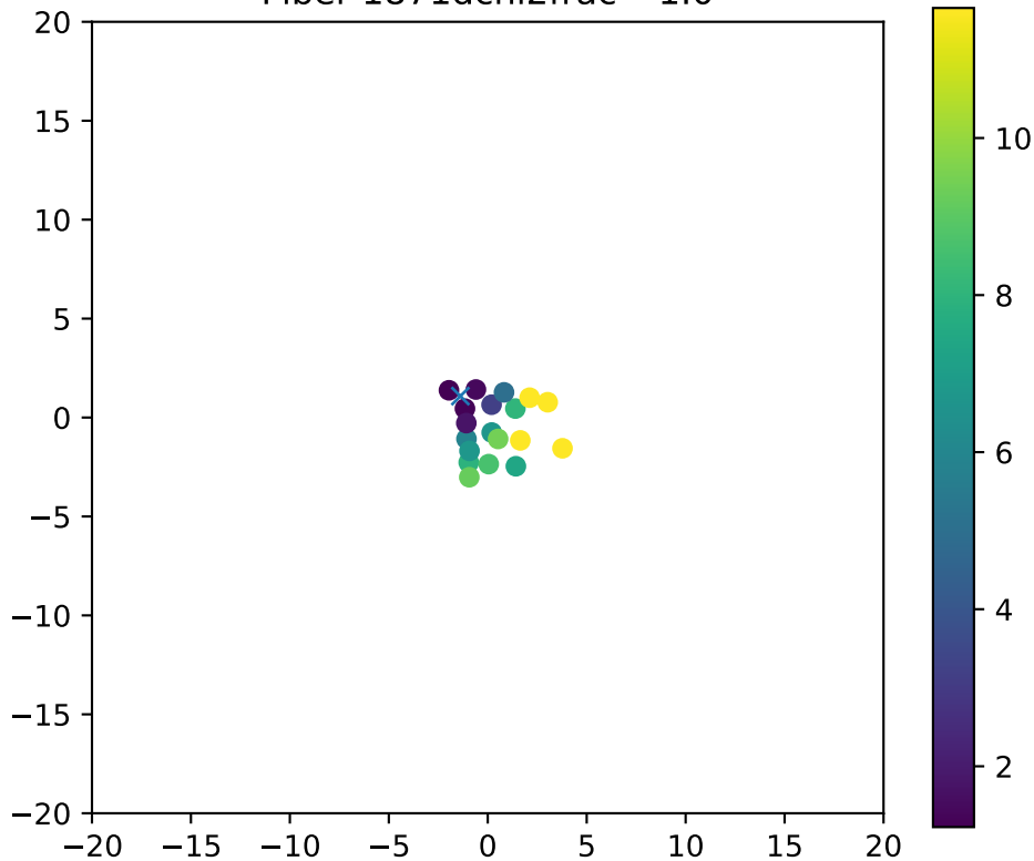
Fiber 1871dchi2frac= 1.0
