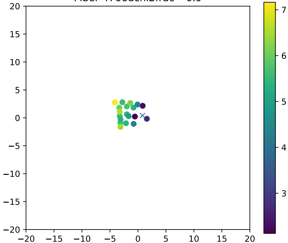
Fiber 4766dchi2frac= 0.9
