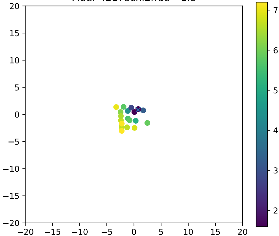
Fiber 4217dchi2frac= 1.0
