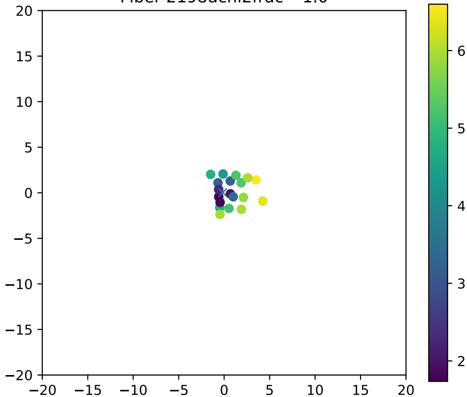
Fiber 2198dchi2frac= 1.0
