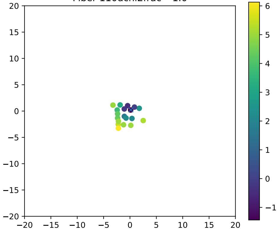
Fiber 110dchi2frac= 1.0
