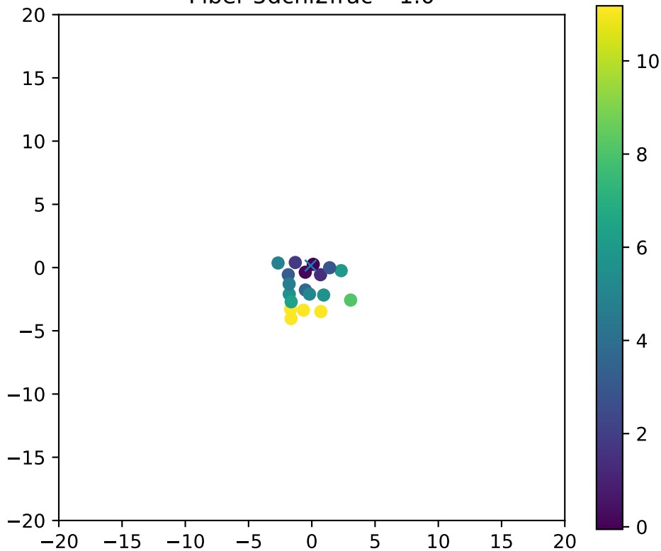
Fiber 5dchi2frac= 1.0
