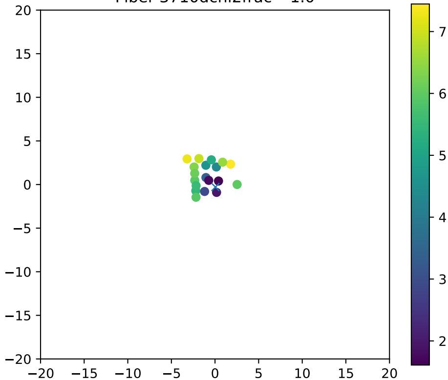
Fiber 3710dchi2frac= 1.0
