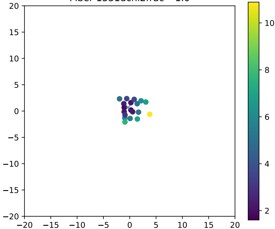
Fiber 1531dchi2frac= 1.0
