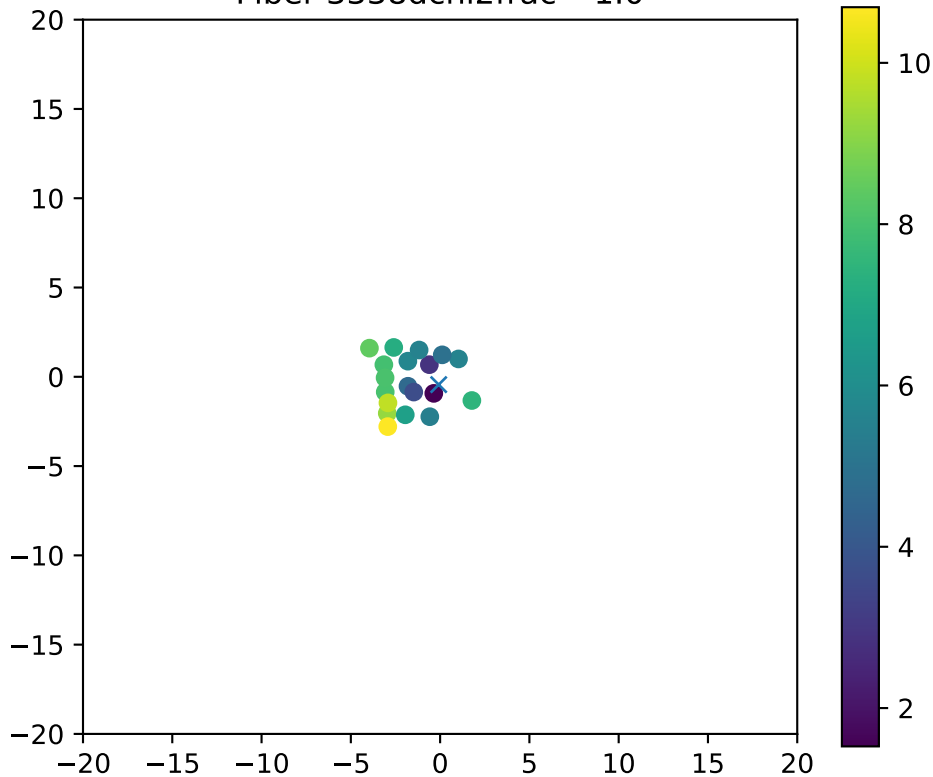
Fiber 3338dchi2frac= 1.0
