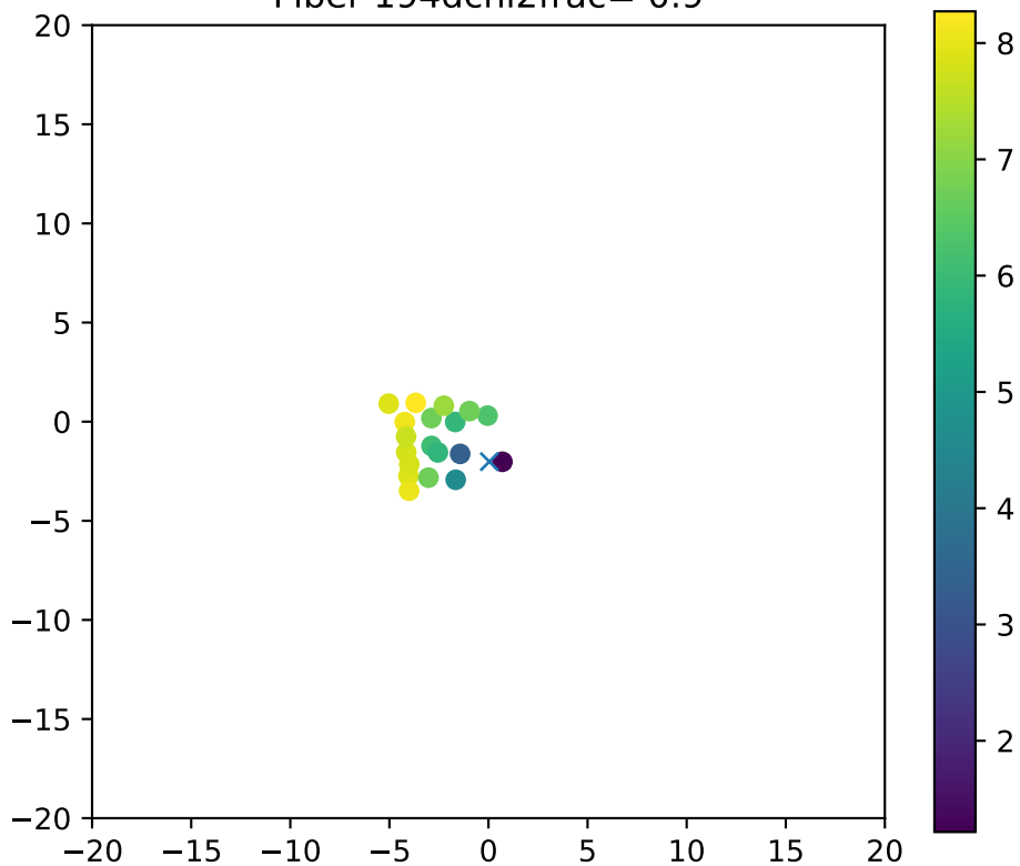
Fiber 194dchi2frac= 0.9
