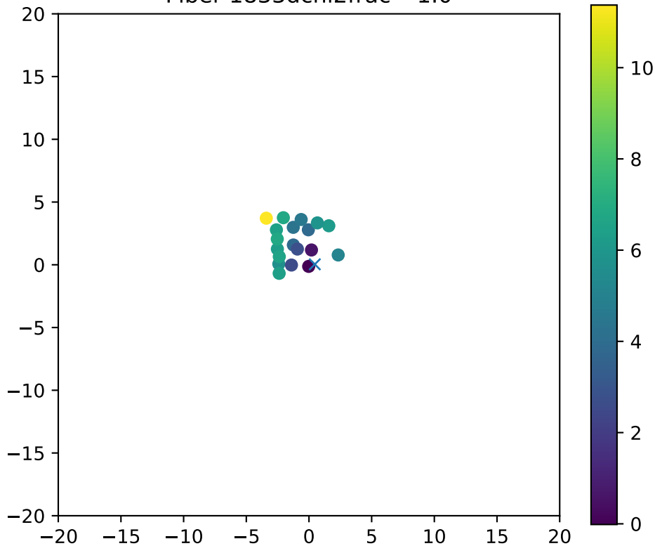
Fiber 1833dchi2frac= 1.0
