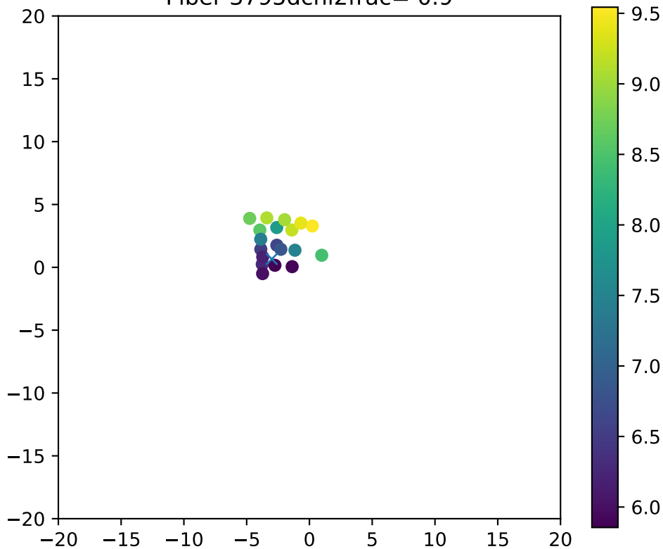
Fiber 3795dchi2frac= 0.9
