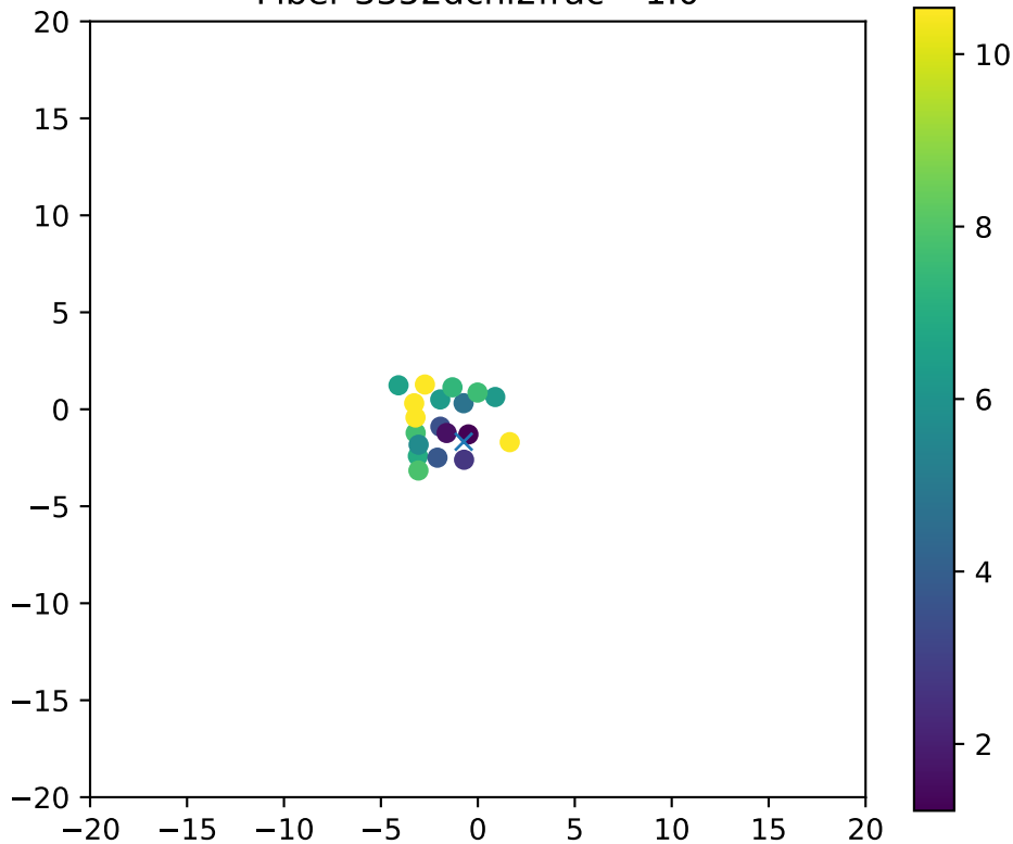
Fiber 3352dchi2frac= 1.0
