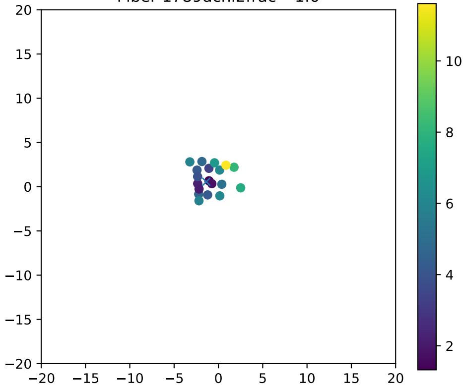
Fiber 1789dchi2frac= 1.0
