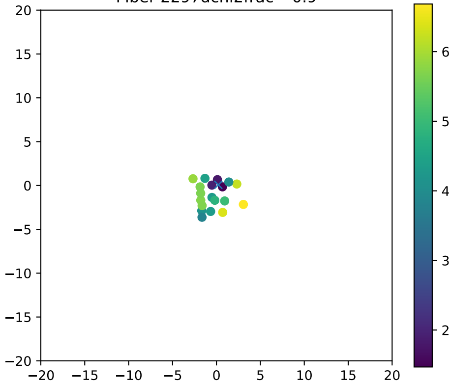
Fiber 2297dchi2frac= 0.9
