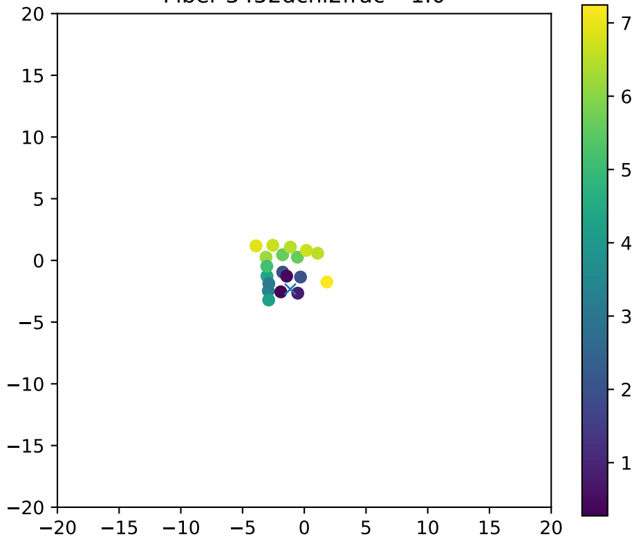
Fiber 3452dchi2frac= 1.0
