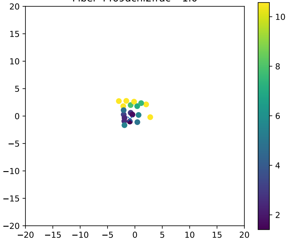
Fiber 4469dchi2frac= 1.0
