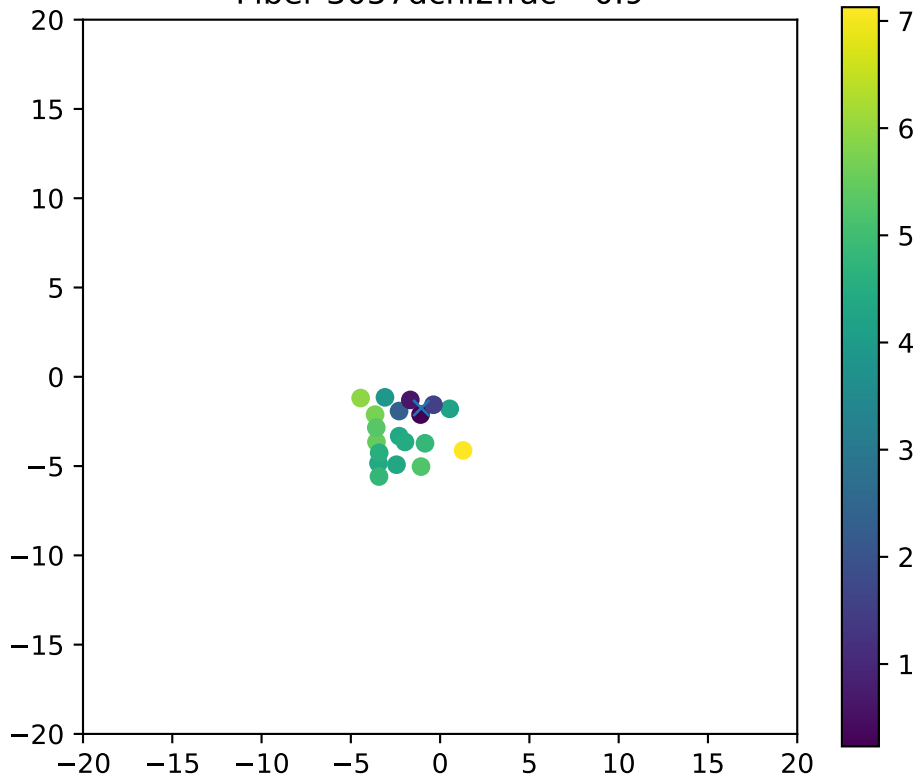
Fiber 3057dchi2frac= 0.9
