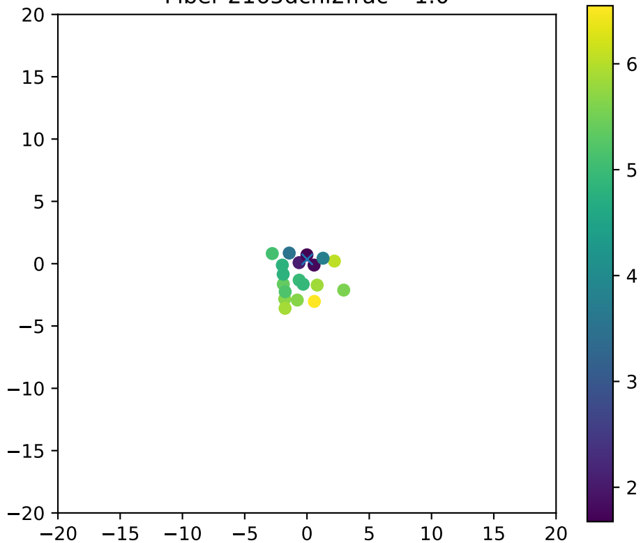
Fiber 2165dchi2frac= 1.0
