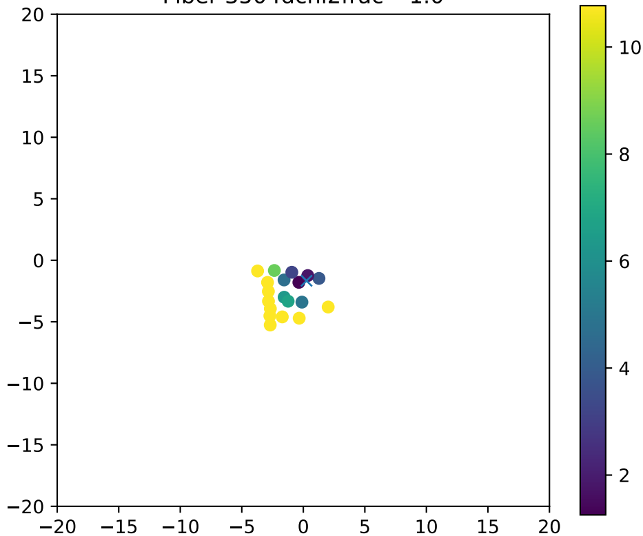
Fiber 3504dchi2frac= 1.0
