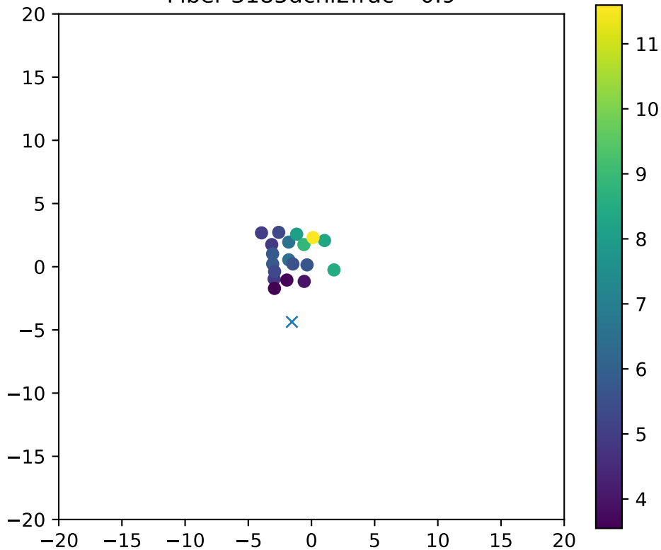
Fiber 3185dchi2frac= 0.9
