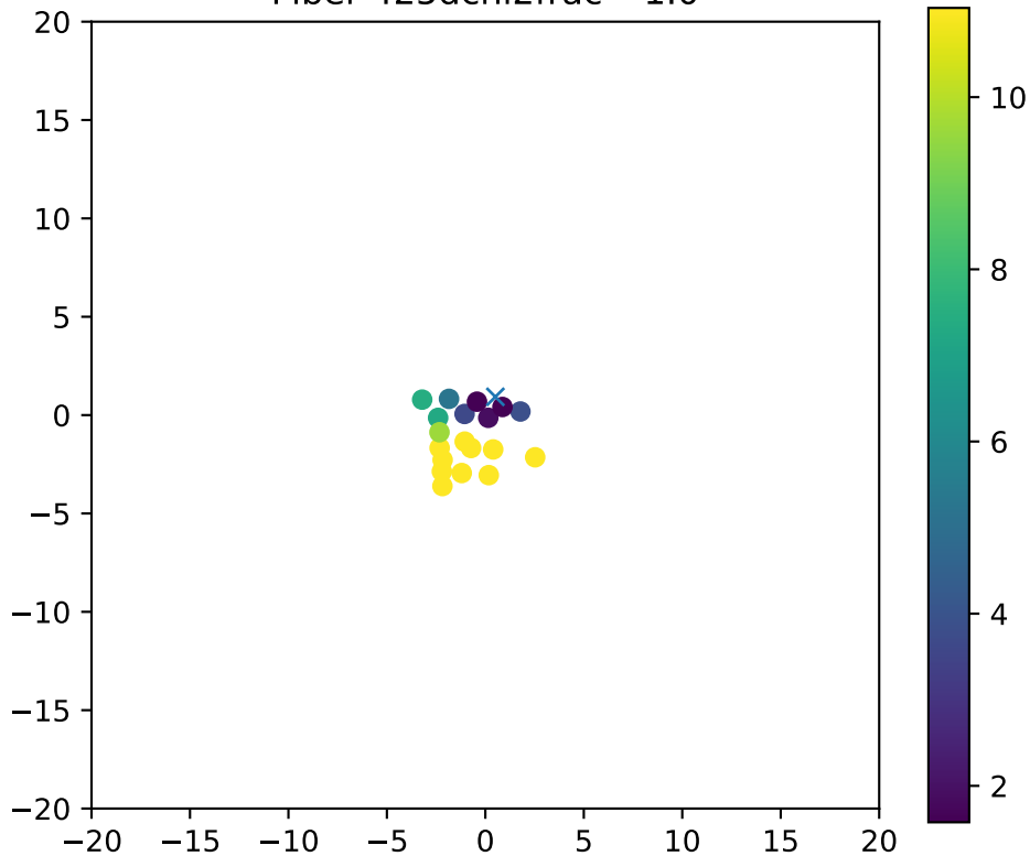
Fiber 425dchi2frac= 1.0
