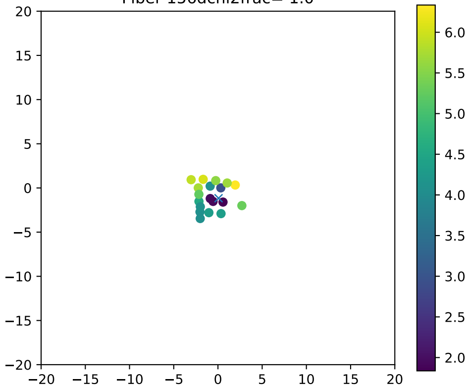
Fiber 156dchi2frac= 1.0
