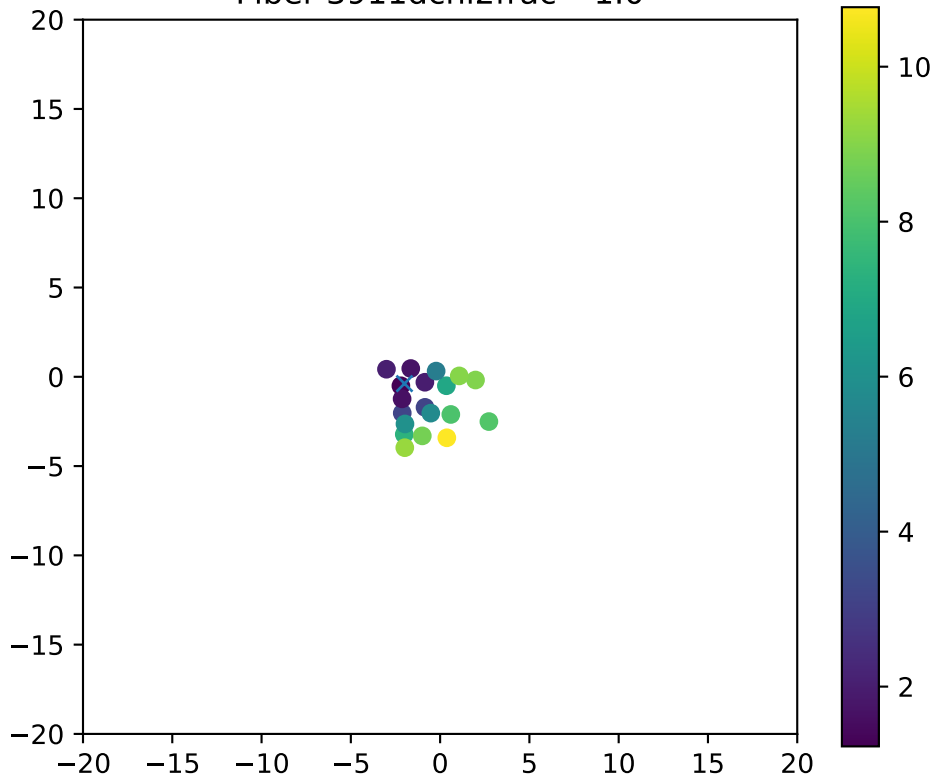
Fiber 3911dchi2frac= 1.0
