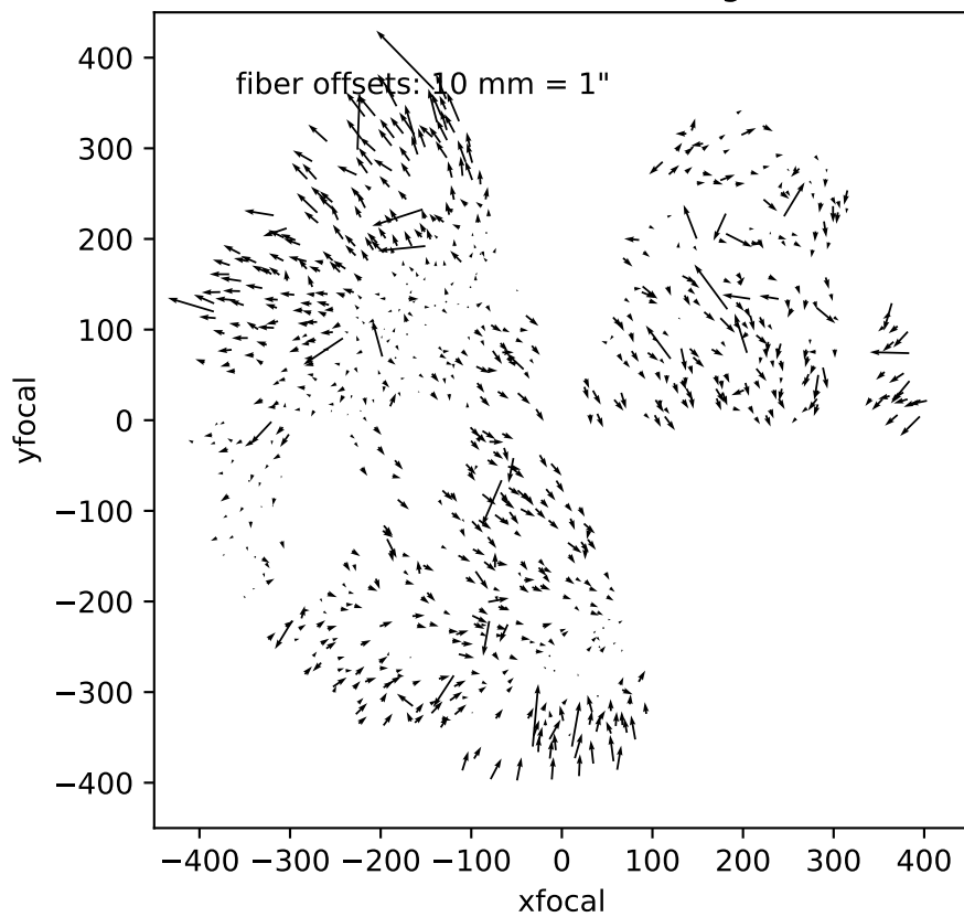
dither20200123-63076-highsnr-Z
