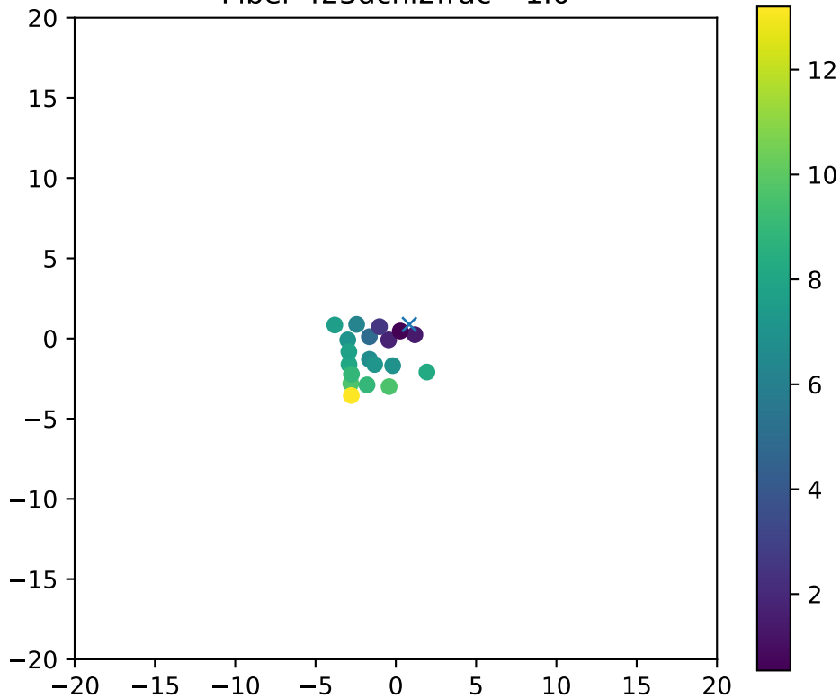
Fiber 423dchi2frac= 1.0
