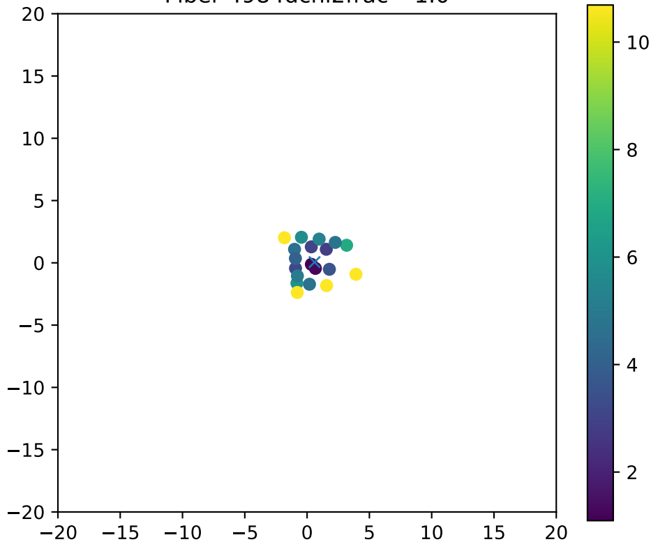
Fiber 4984dchi2frac= 1.0
