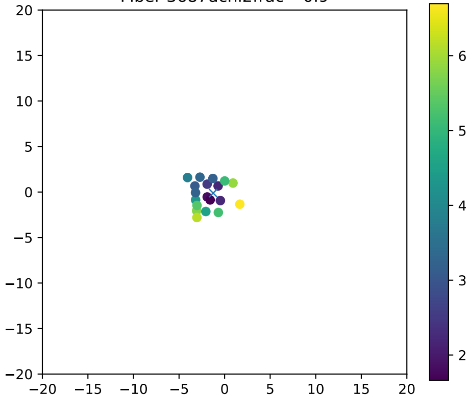
Fiber 3687dchi2frac= 0.9
