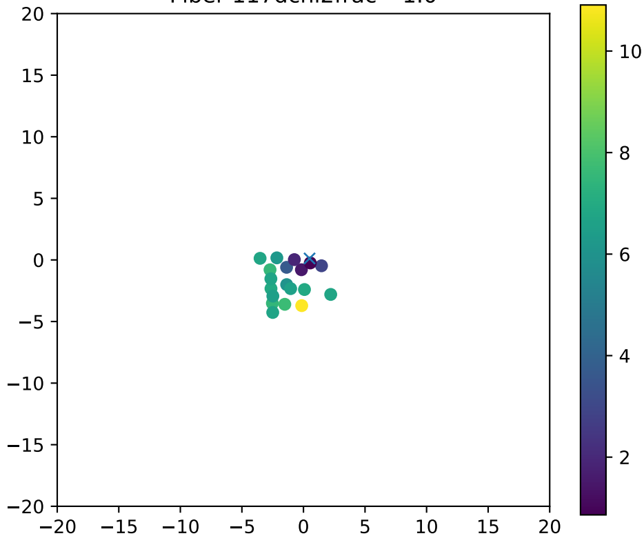
Fiber 117dchi2frac= 1.0
