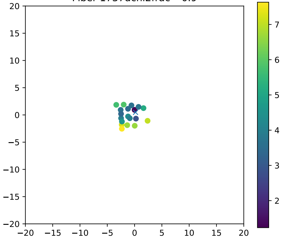
Fiber 1737dchi2frac= 0.9
