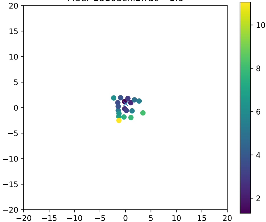
Fiber 1816dchi2frac= 1.0
