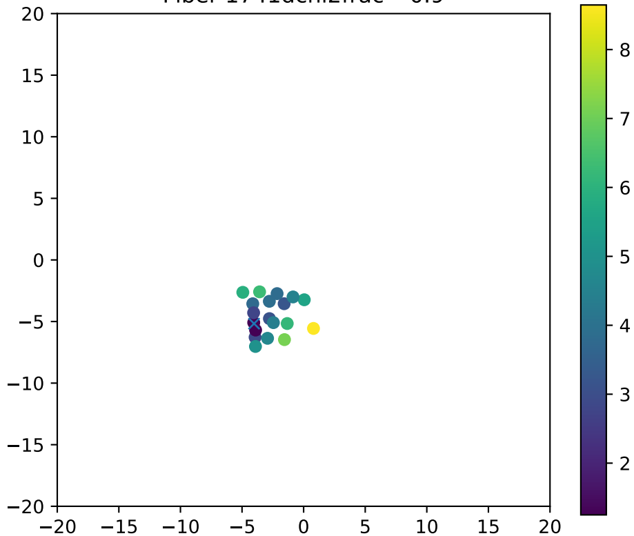
Fiber 1741dchi2frac= 0.9
