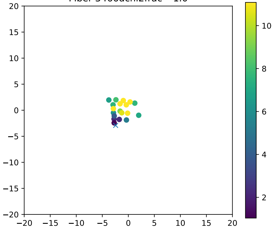
Fiber 3466dchi2frac= 1.0
