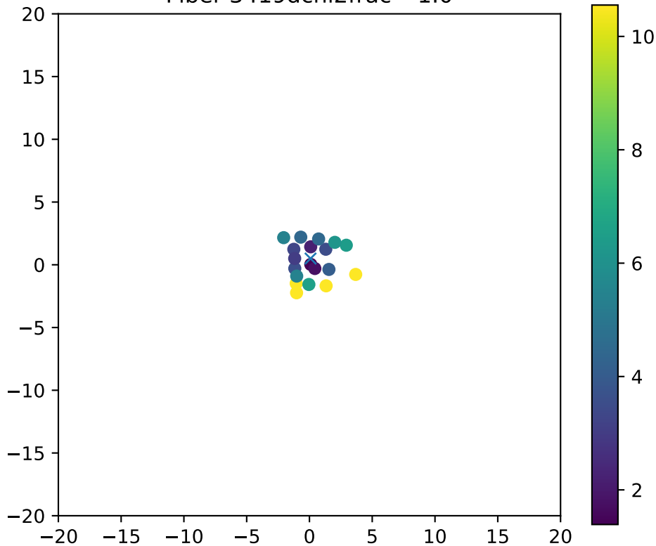
Fiber 3419dchi2frac= 1.0
