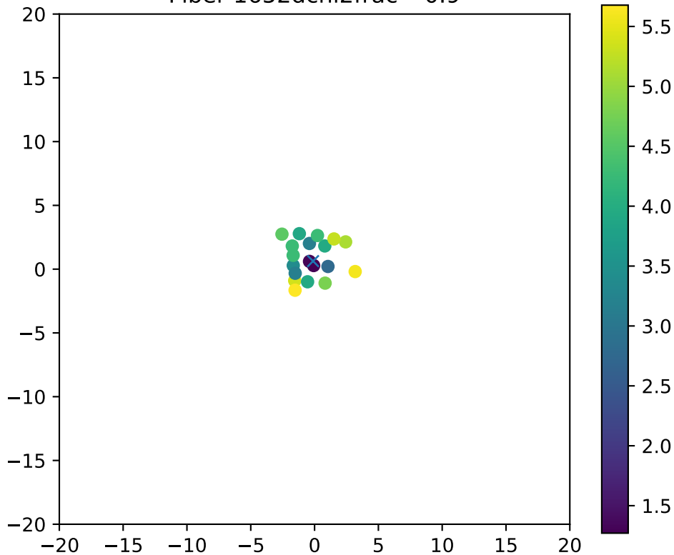
Fiber 1652dchi2frac= 0.9
