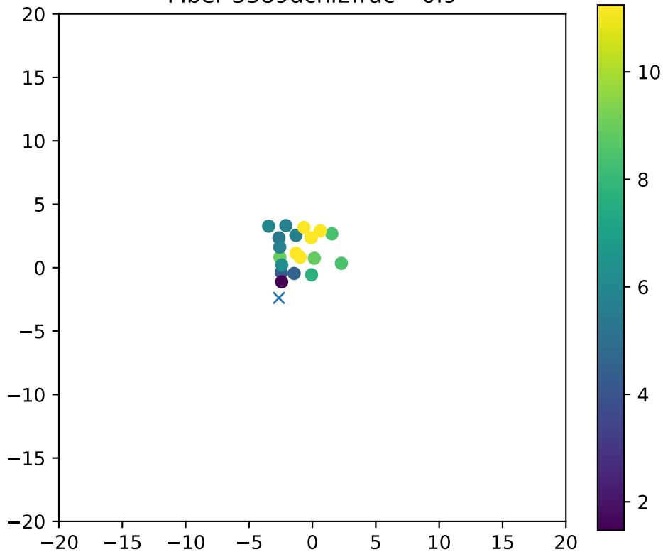
Fiber 3389dchi2frac= 0.9
