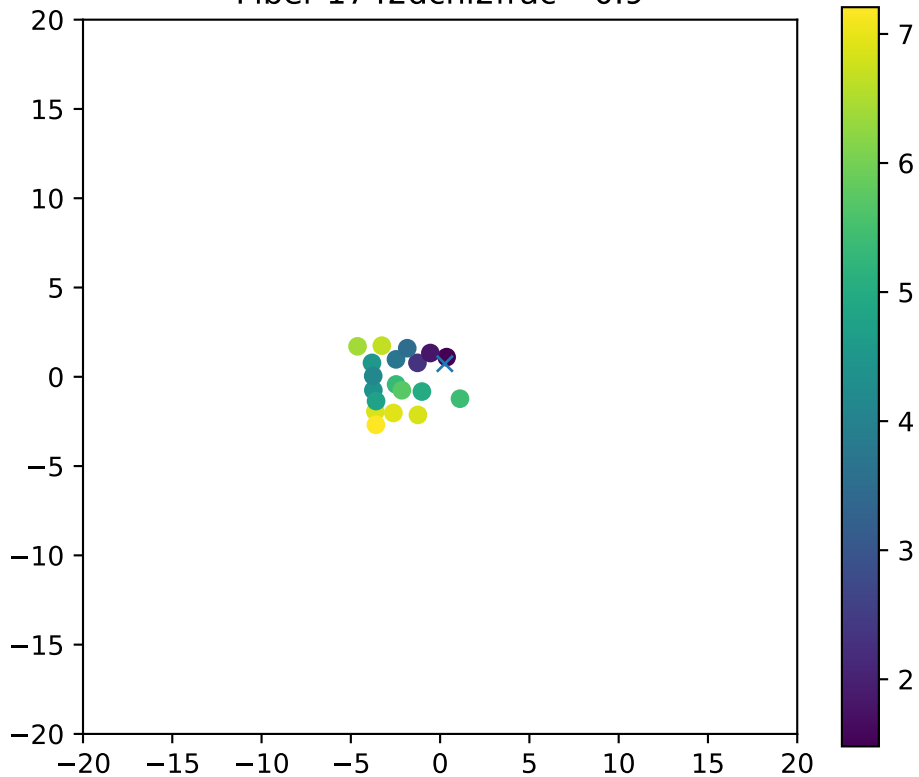
Fiber 1742dchi2frac= 0.9
