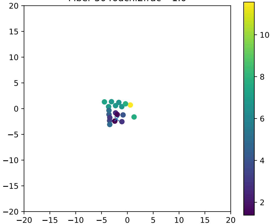
Fiber 3046dchi2frac= 1.0
