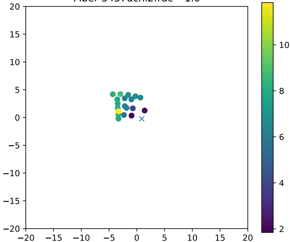
Fiber 3437dchi2frac= 1.0
