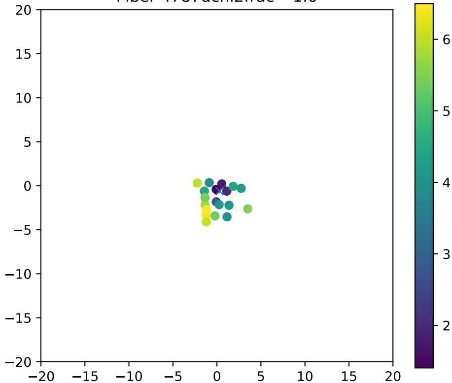
Fiber 4787dchi2frac= 1.0
