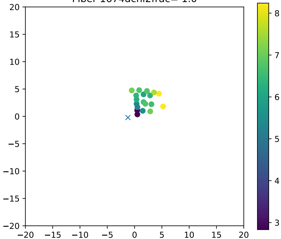
Fiber 1674dchi2frac= 1.0
