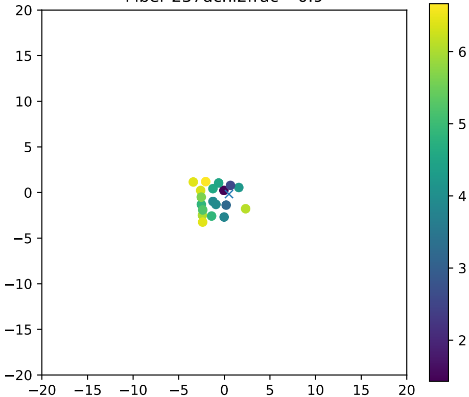
Fiber 237dchi2frac= 0.9
