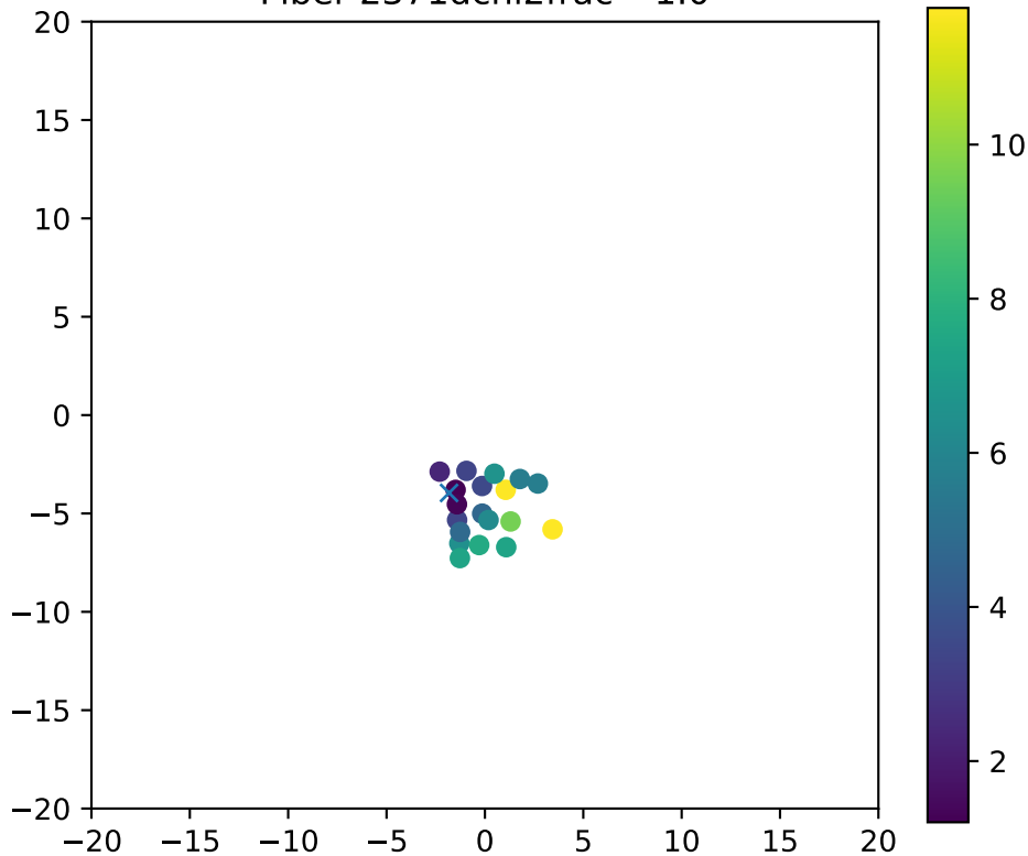
Fiber 2371dchi2frac= 1.0
