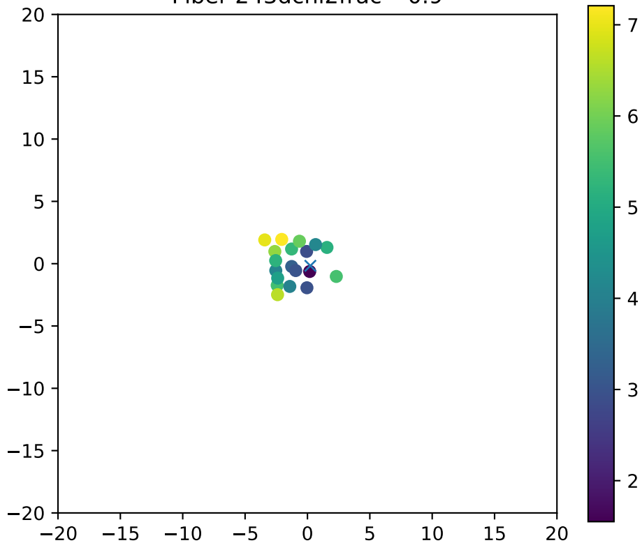
Fiber 243dchi2frac= 0.9
