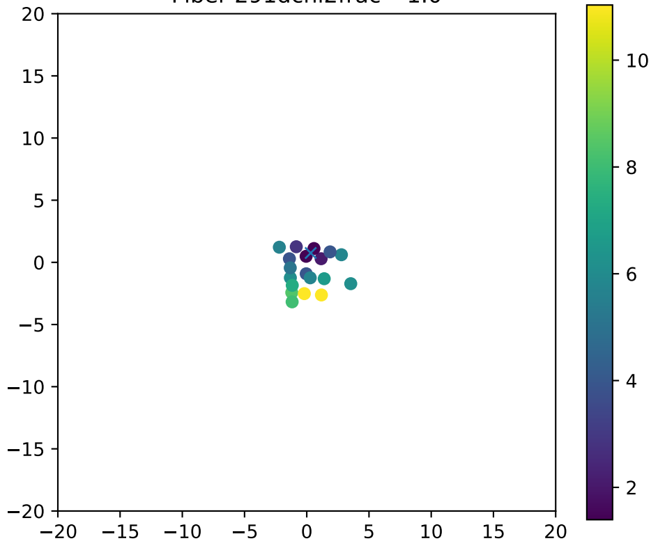
Fiber 291dchi2frac= 1.0
