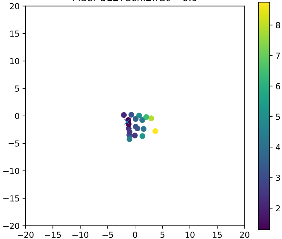
Fiber 3127dchi2frac= 0.9
