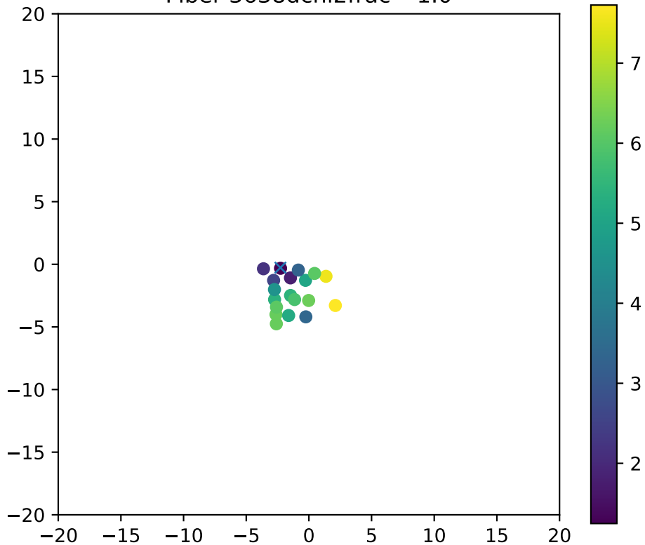
Fiber 3638dchi2frac= 1.0
