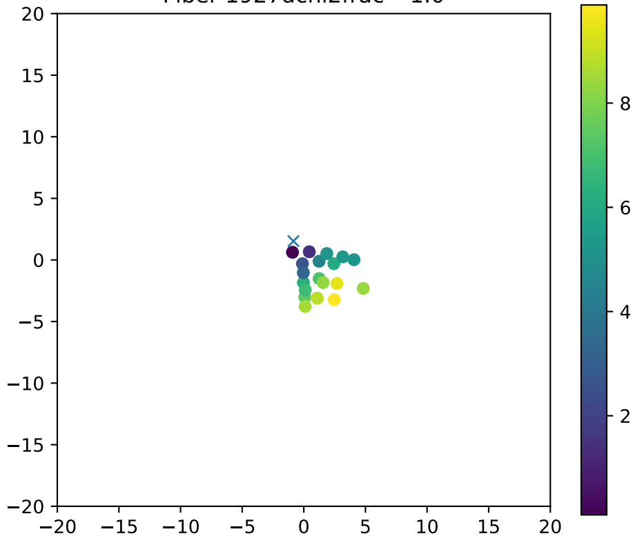
Fiber 1927dchi2frac= 1.0
