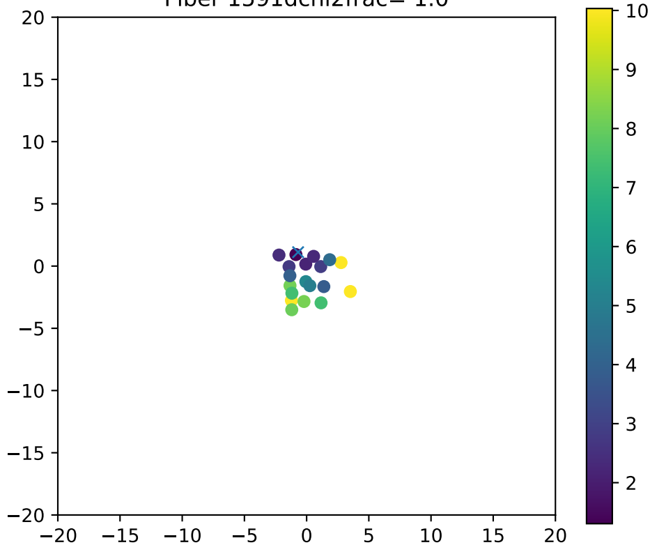
Fiber 1591dchi2frac= 1.0
