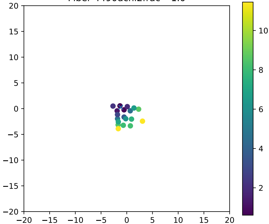
Fiber 4490dchi2frac= 1.0
