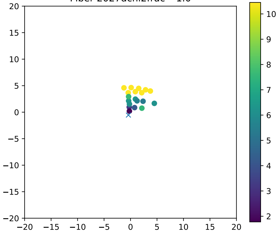
Fiber 2027dchi2frac= 1.0
