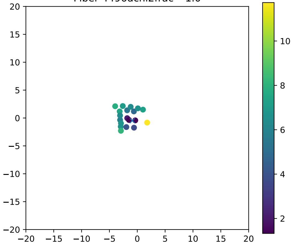
Fiber 4496dchi2frac= 1.0
