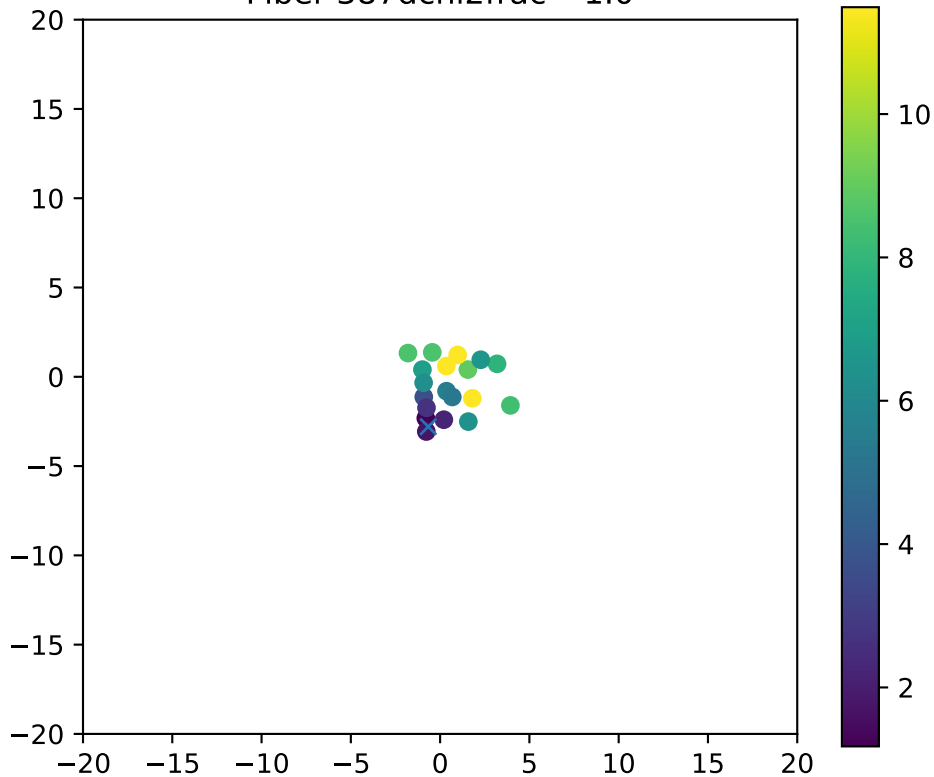
Fiber 387dchi2frac= 1.0
