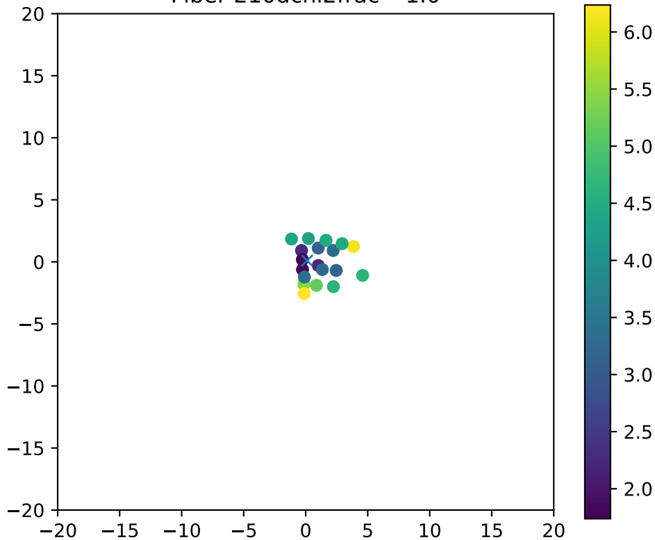
Fiber 210dchi2frac= 1.0
