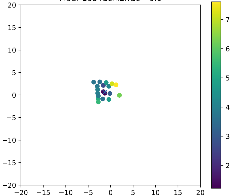
Fiber 1634dchi2frac= 0.9
