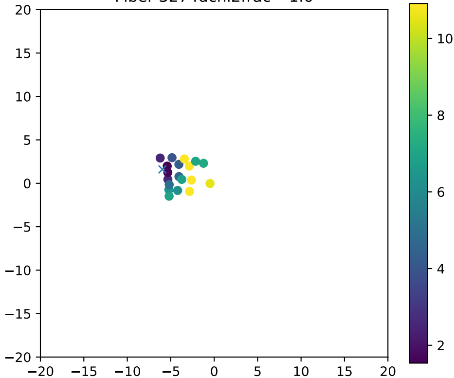
Fiber 3274dchi2frac= 1.0
