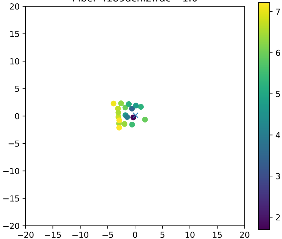
Fiber 4189dchi2frac= 1.0
