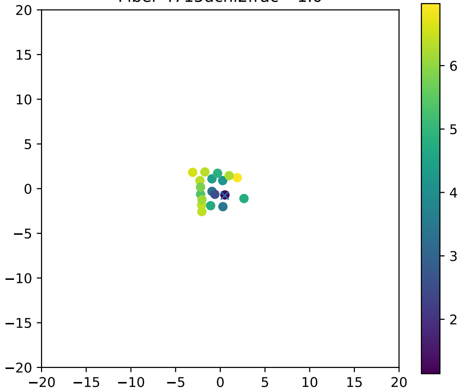
Fiber 4715dchi2frac= 1.0
