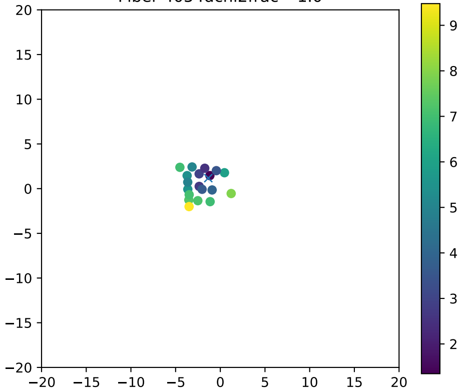
Fiber 4054dchi2frac= 1.0
