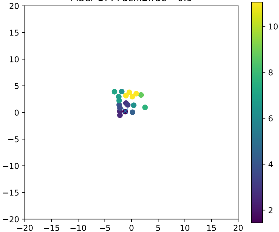
Fiber 1777dchi2frac= 0.9
