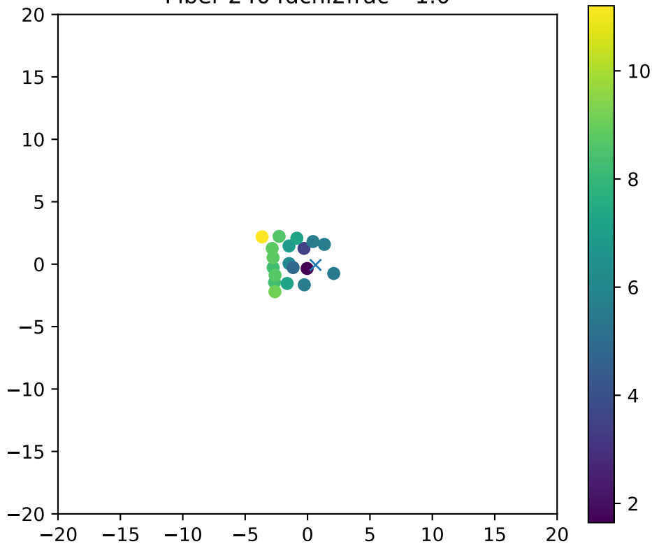
Fiber 2404dchi2frac= 1.0
