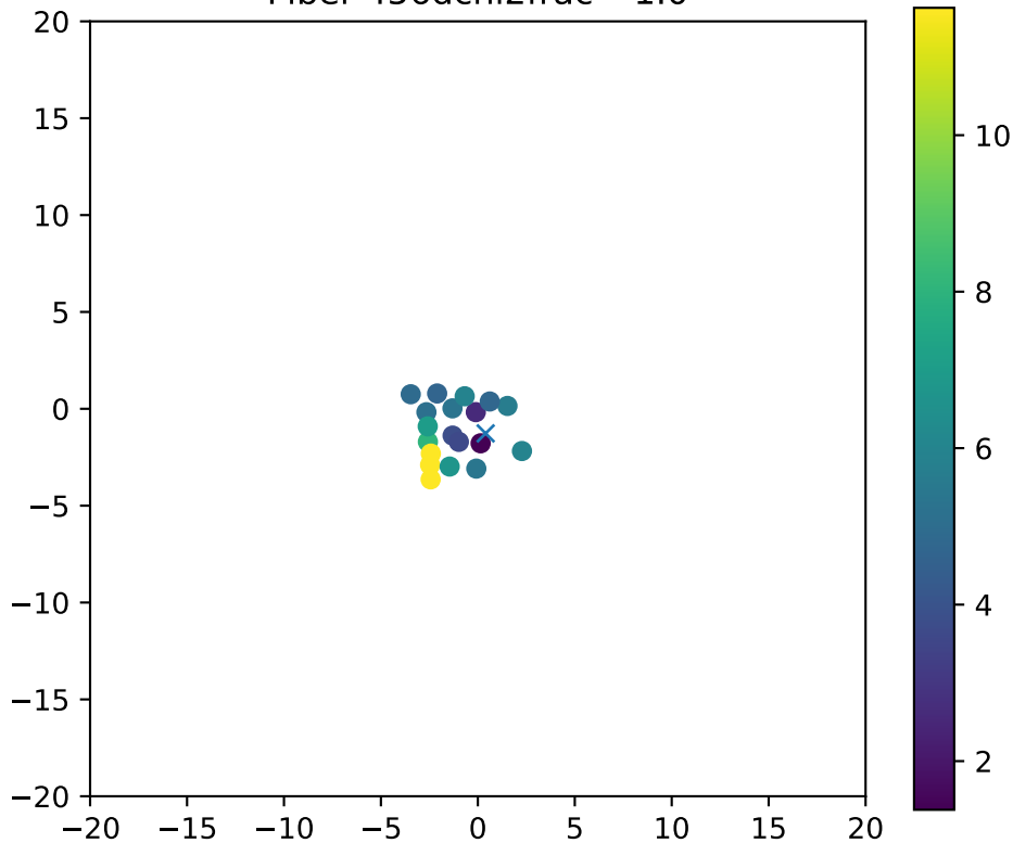
Fiber 456dchi2frac= 1.0
