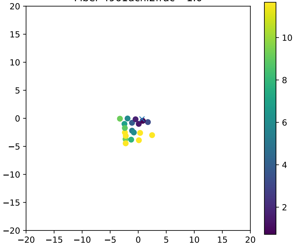
Fiber 4961dchi2frac= 1.0
