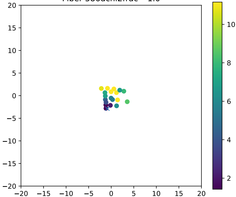
Fiber 386dchi2frac= 1.0
