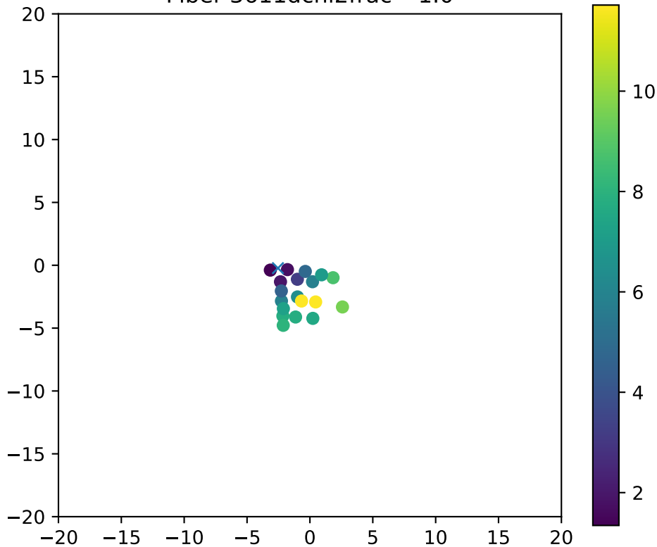
Fiber 3611dchi2frac= 1.0
