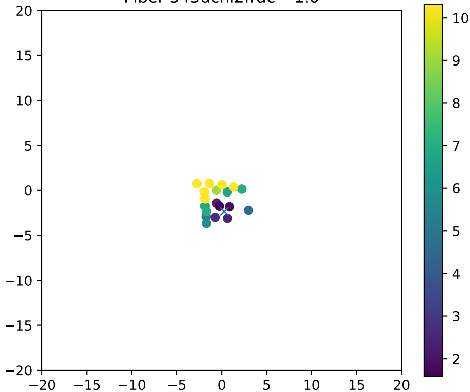
Fiber 343dchi2frac= 1.0
