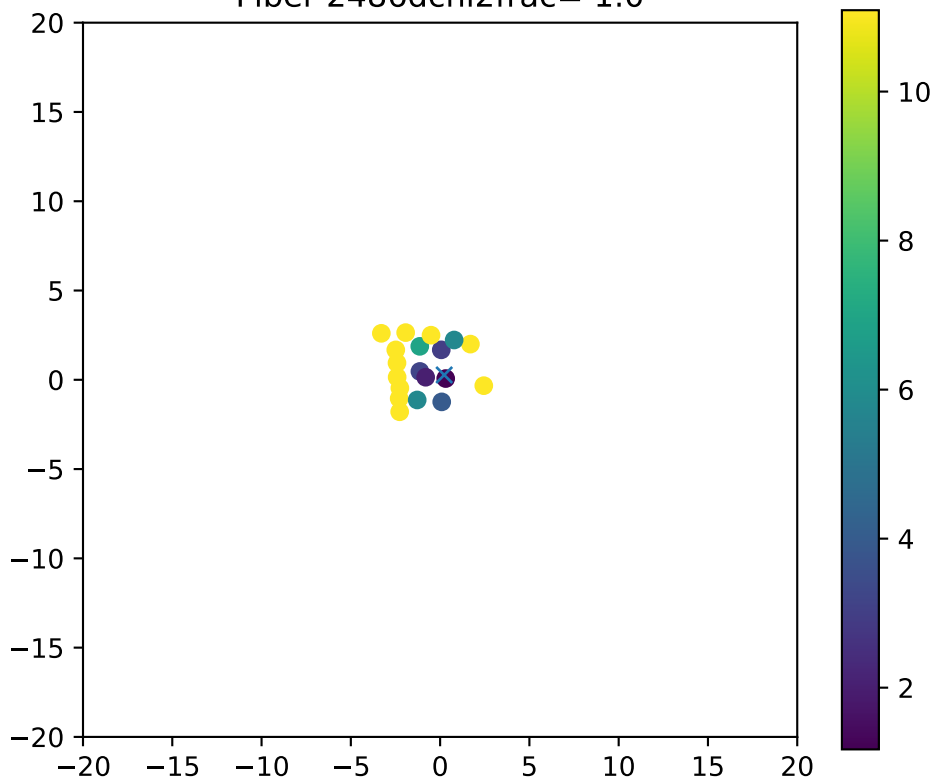
Fiber 2486dchi2frac= 1.0
