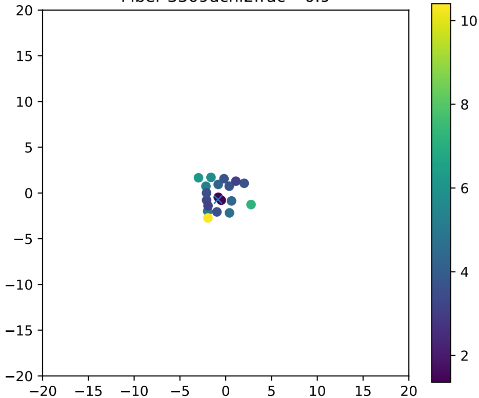
Fiber 3309dchi2frac= 0.9
