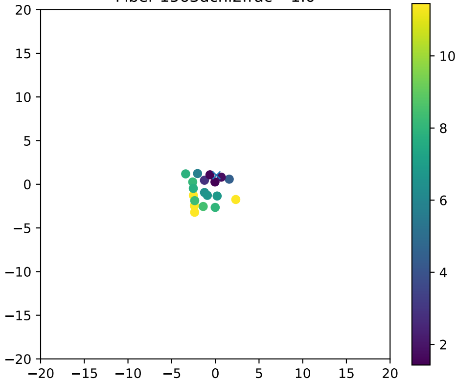
Fiber 1563dchi2frac= 1.0
