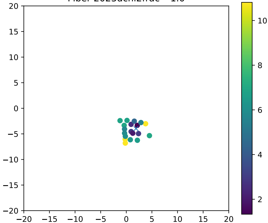
Fiber 2023dchi2frac= 1.0
