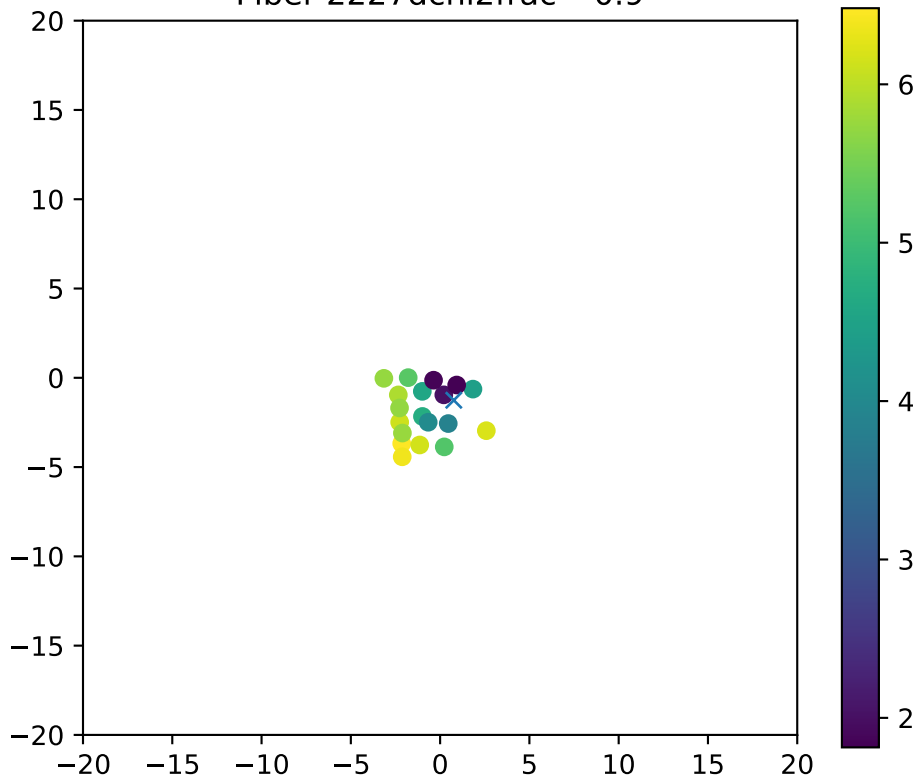
Fiber 2227dchi2frac= 0.9
