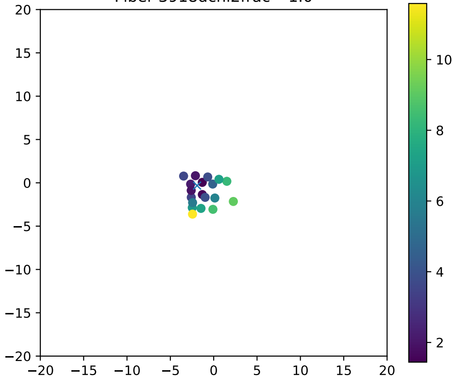
Fiber 3918dchi2frac= 1.0
