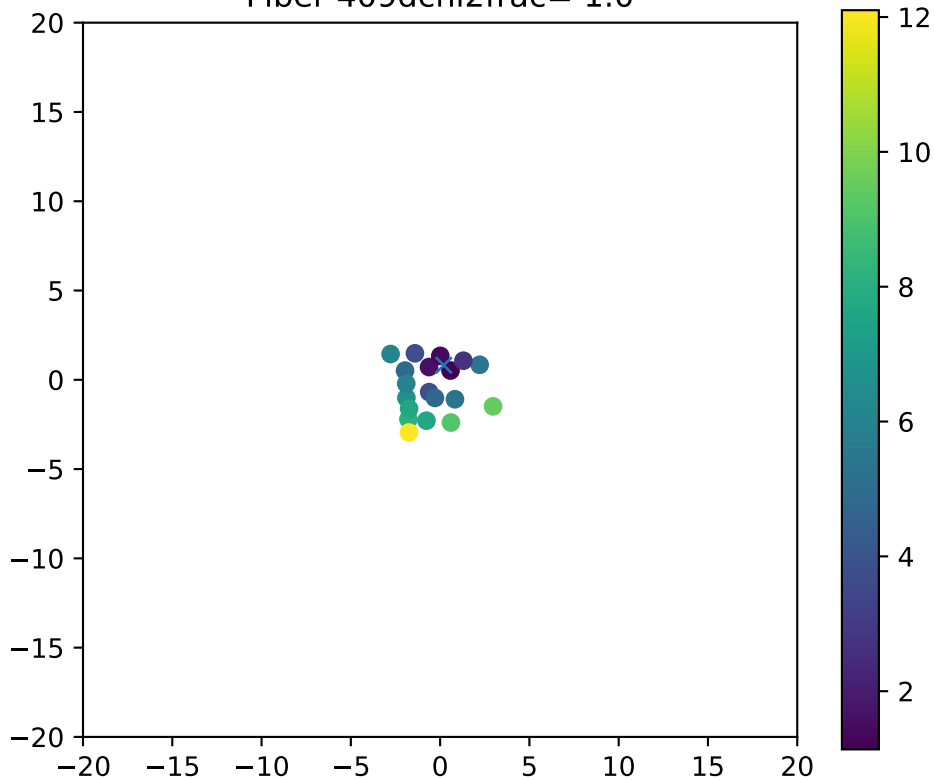
Fiber 409dchi2frac= 1.0
