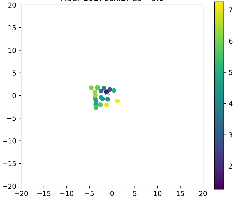
Fiber 1617dchi2frac= 0.9
