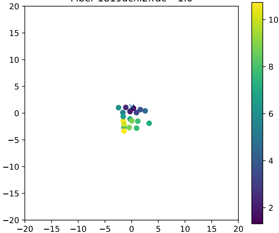
Fiber 1819dchi2frac= 1.0
