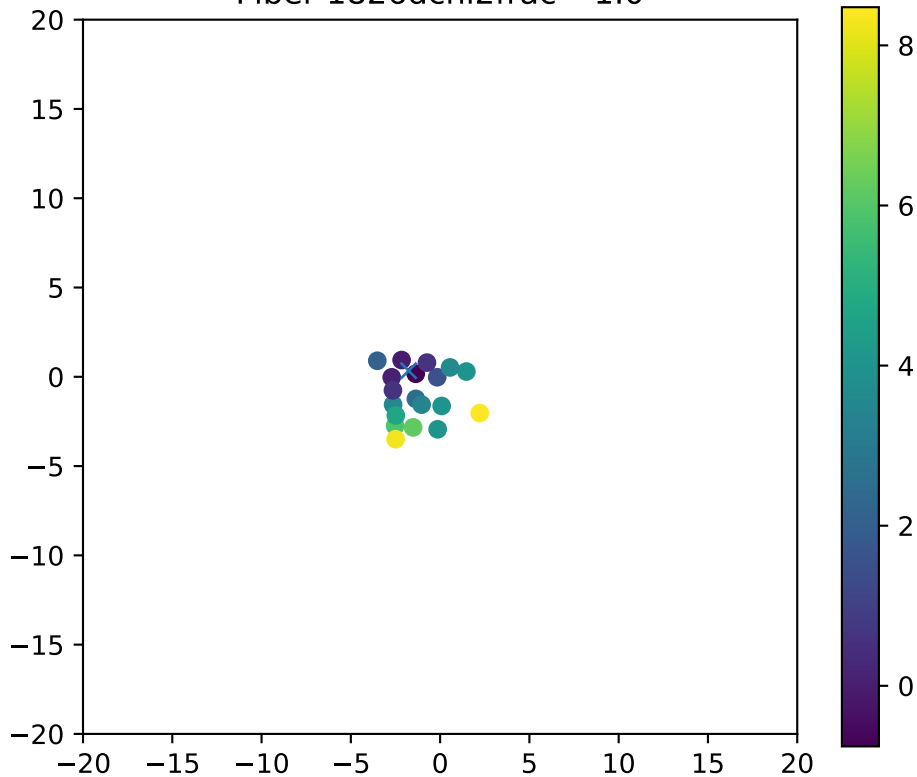
Fiber 1826dchi2frac= 1.0
