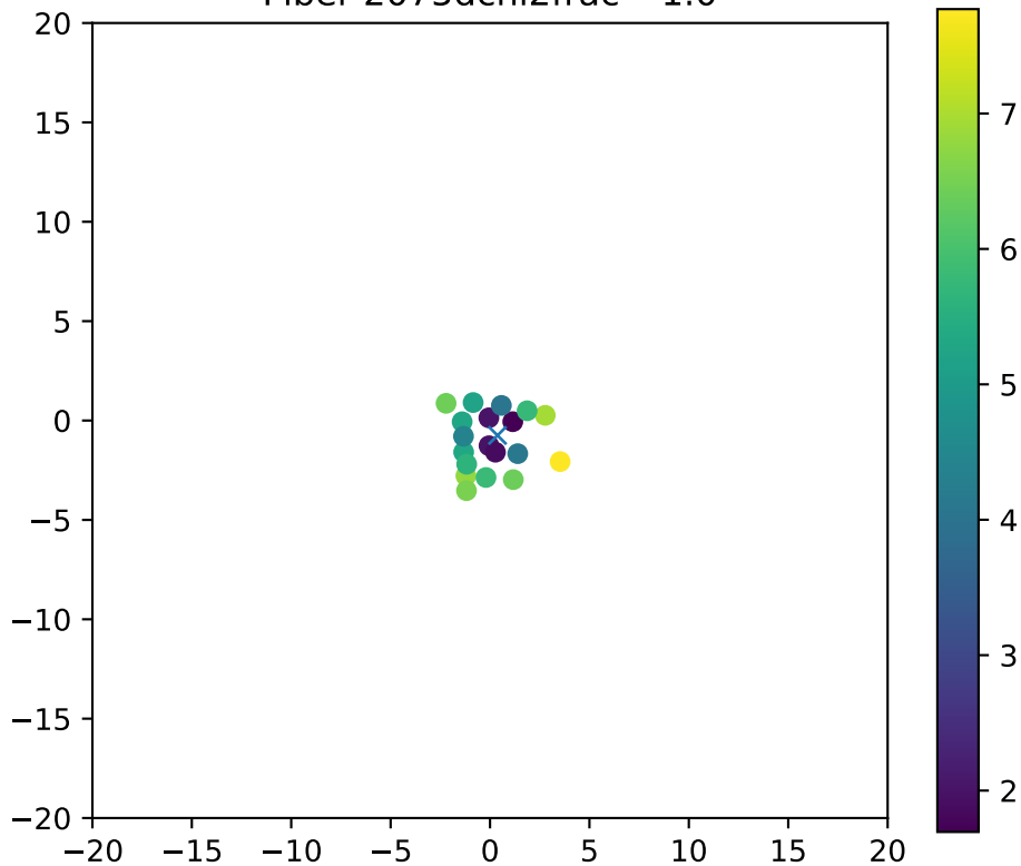
Fiber 2075dchi2frac= 1.0
