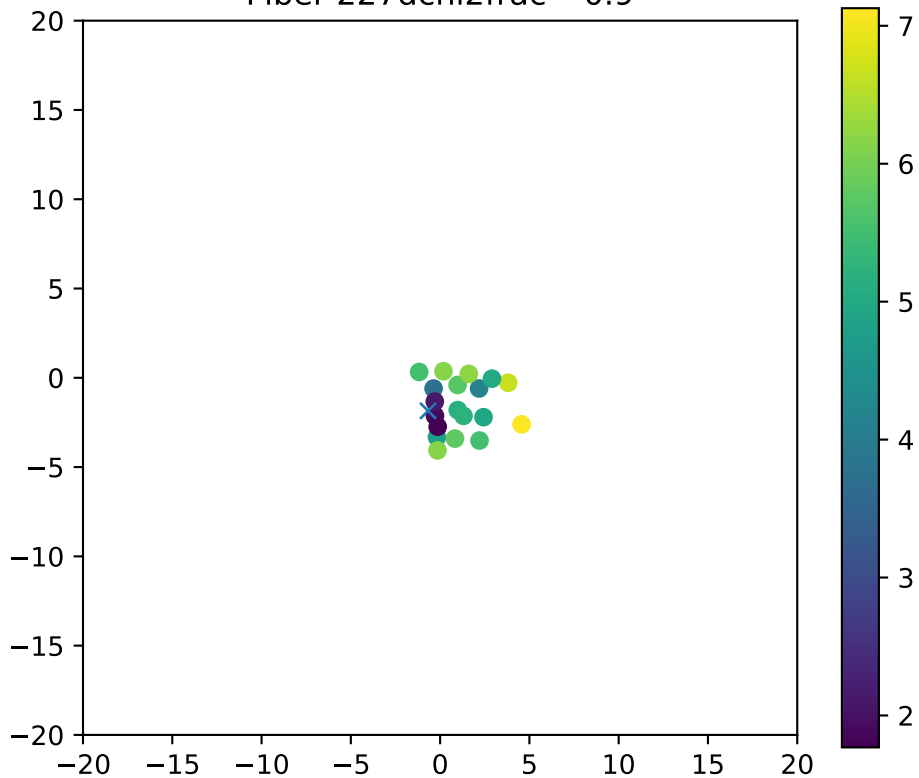
Fiber 227dchi2frac= 0.9
