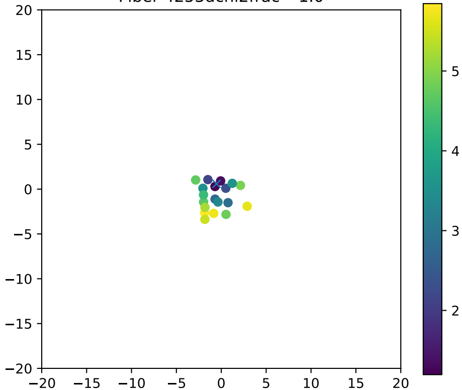
Fiber 4253dchi2frac= 1.0
