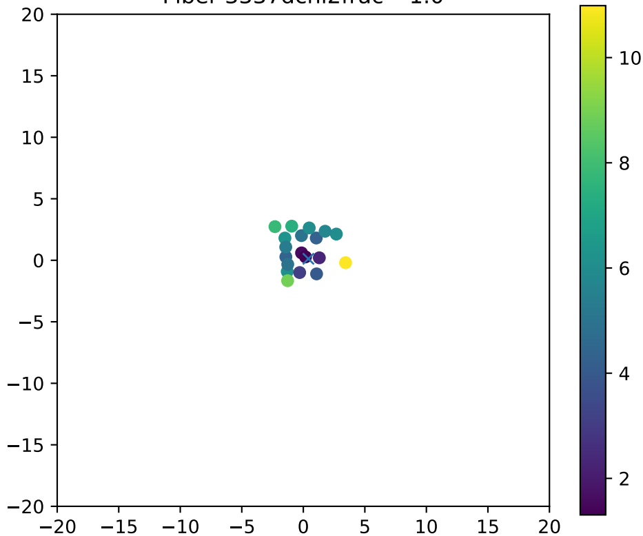
Fiber 3337dchi2frac= 1.0
