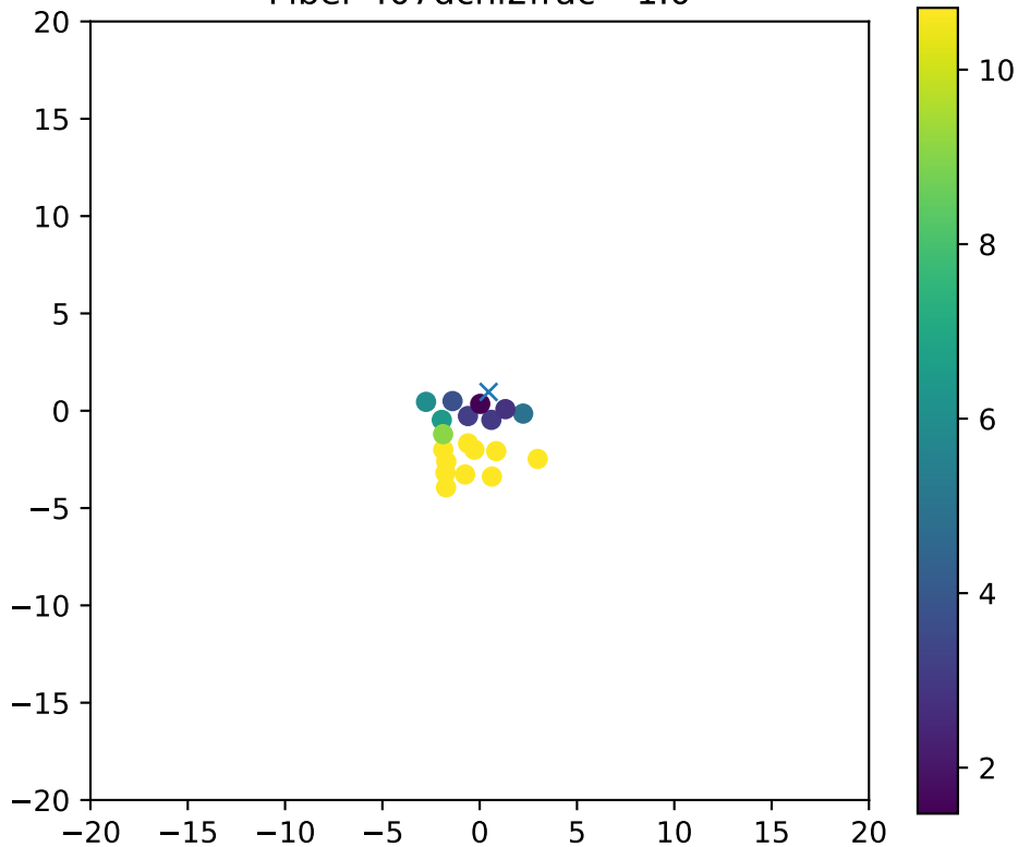
Fiber 407dchi2frac= 1.0
