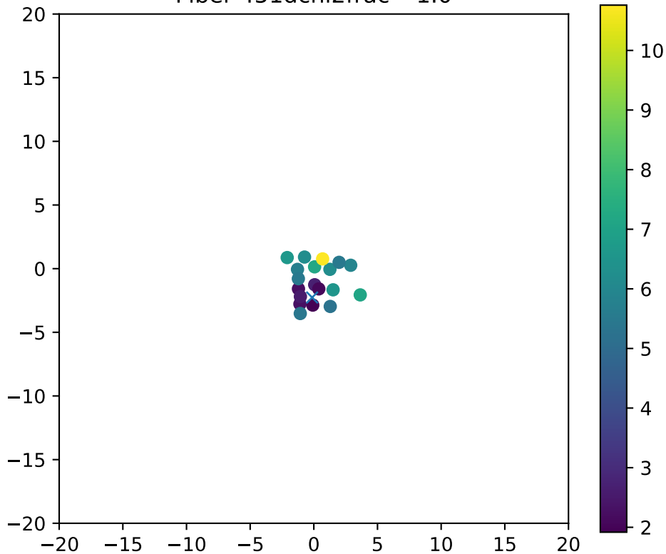
Fiber 451dchi2frac= 1.0
