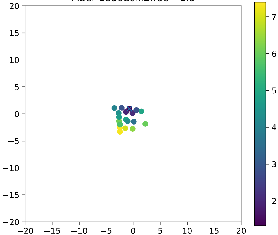
Fiber 1650dchi2frac= 1.0
