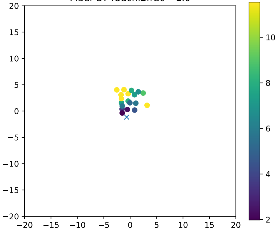
Fiber 3748dchi2frac= 1.0
