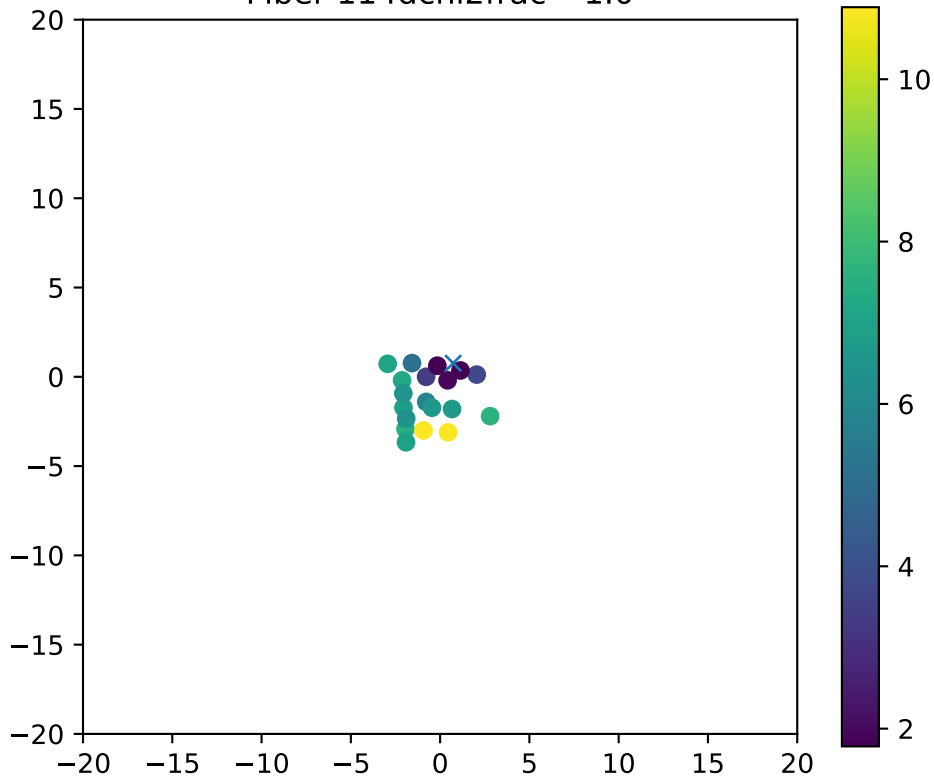
Fiber 114dchi2frac= 1.0
