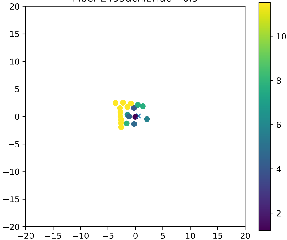
Fiber 2495dchi2frac= 0.9
