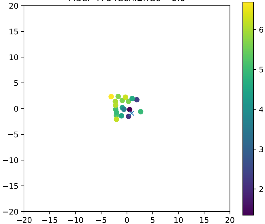
Fiber 4764dchi2frac= 0.9
