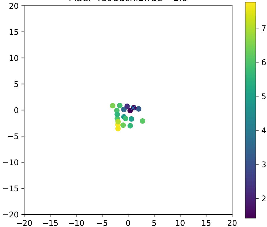
Fiber 4696dchi2frac= 1.0
