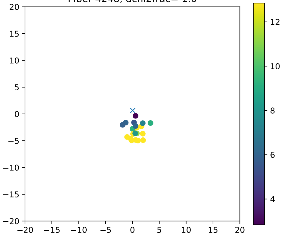
Fiber 4248, dchi2frac= 1.0
