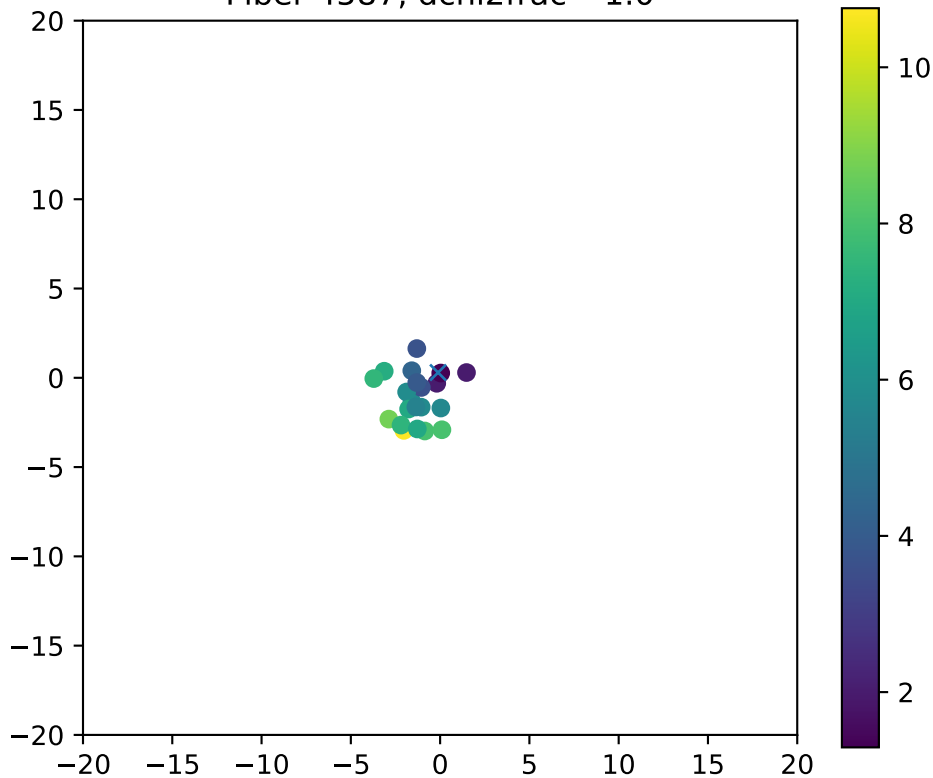
Fiber 4587, dchi2frac= 1.0
