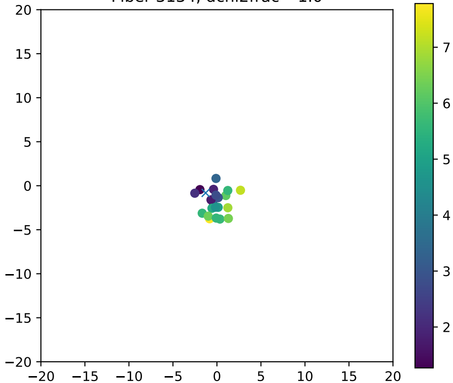
Fiber 3134, dchi2frac= 1.0
