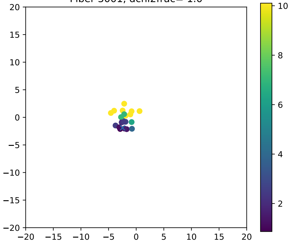
Fiber 3001, dchi2frac= 1.0
