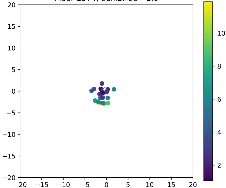
Fiber 1574, dchi2frac= 1.0
