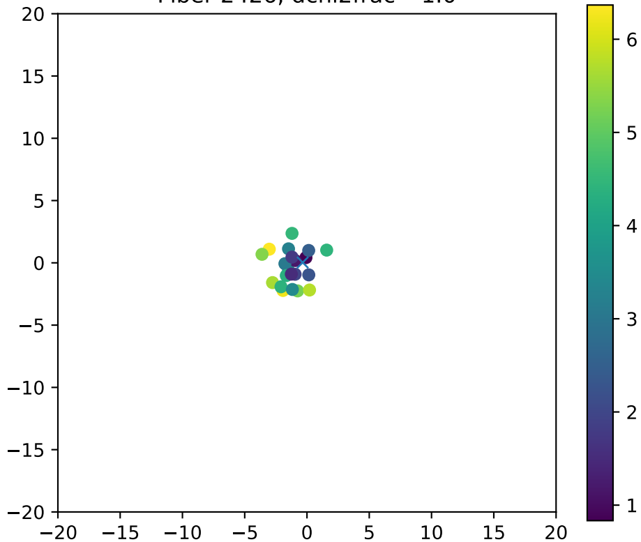
Fiber 2426, dchi2frac= 1.0
