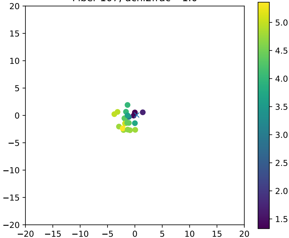
Fiber 107, dchi2frac= 1.0
