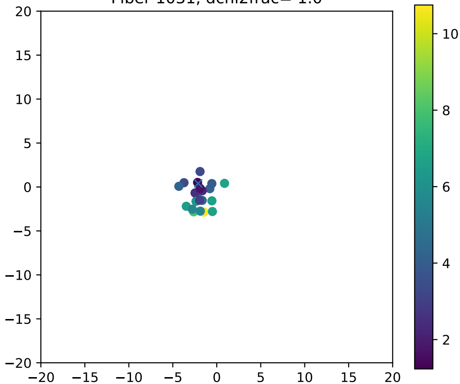
Fiber 1031, dchi2frac= 1.0
