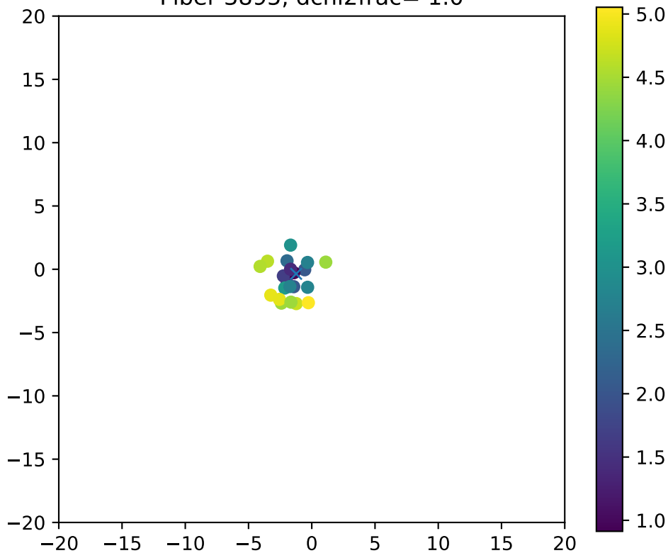
Fiber 3895, dchi2frac= 1.0
