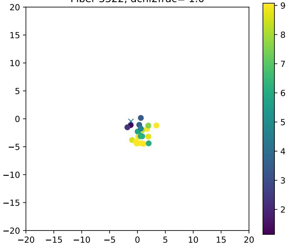
Fiber 3322, dchi2frac= 1.0
