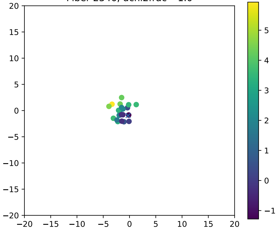
Fiber 2346, dchi2frac= 1.0
