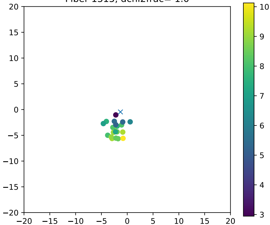
Fiber 1315, dchi2frac= 1.0
