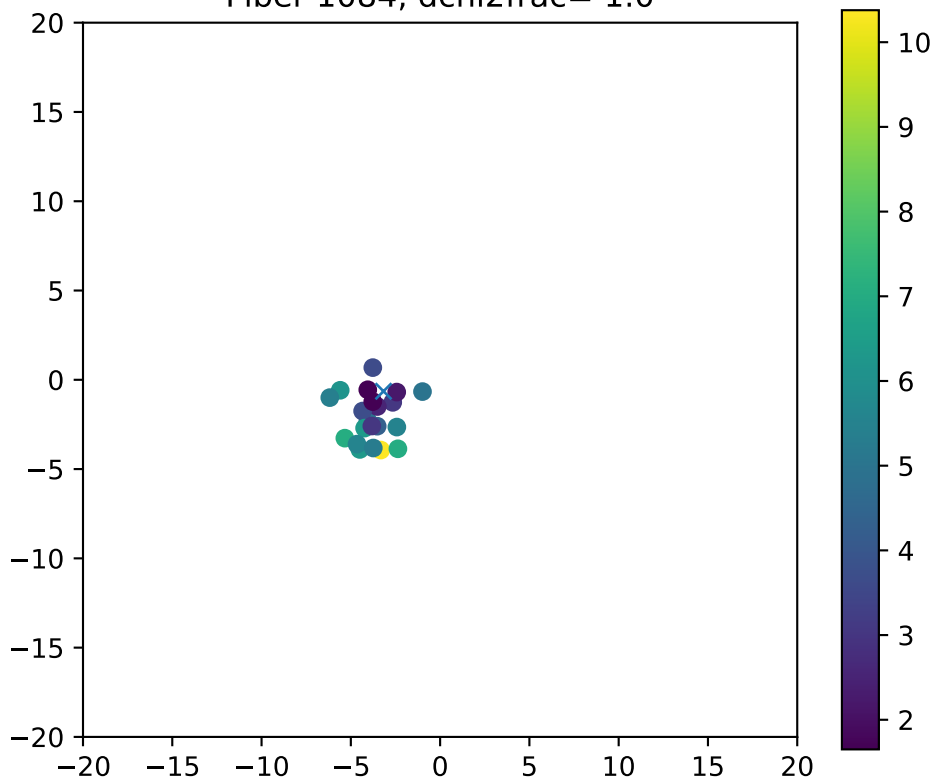
Fiber 1084, dchi2frac= 1.0
