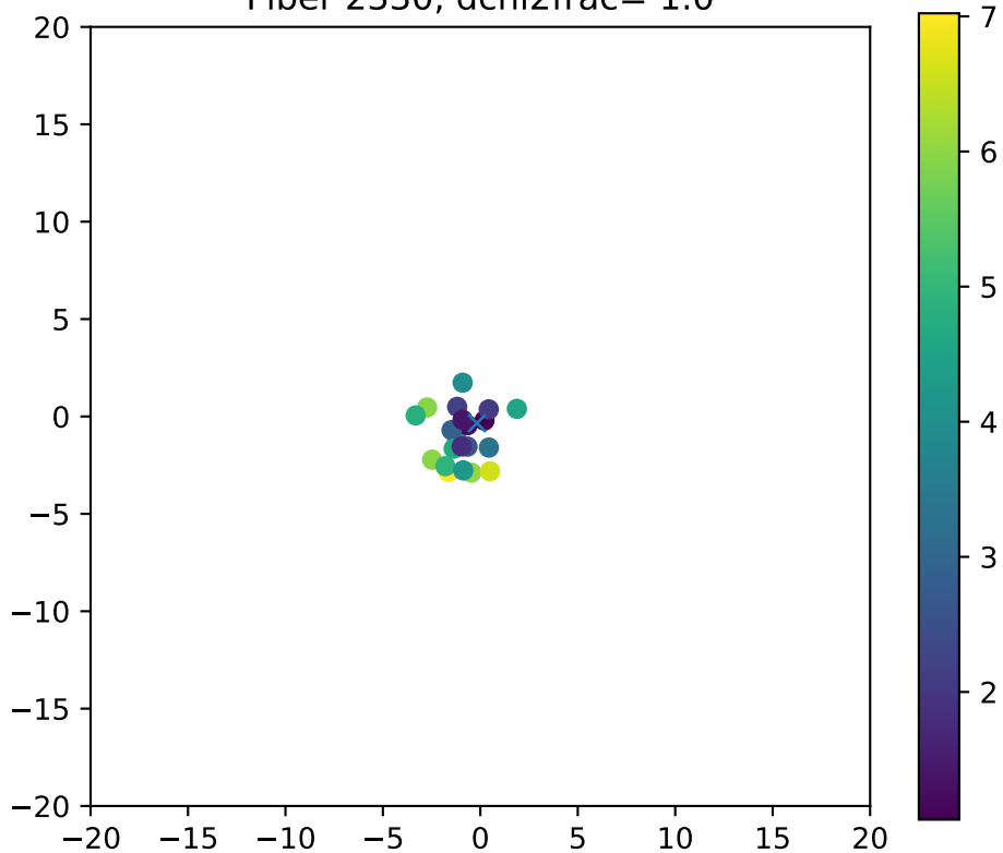
Fiber 2330, dchi2frac= 1.0
