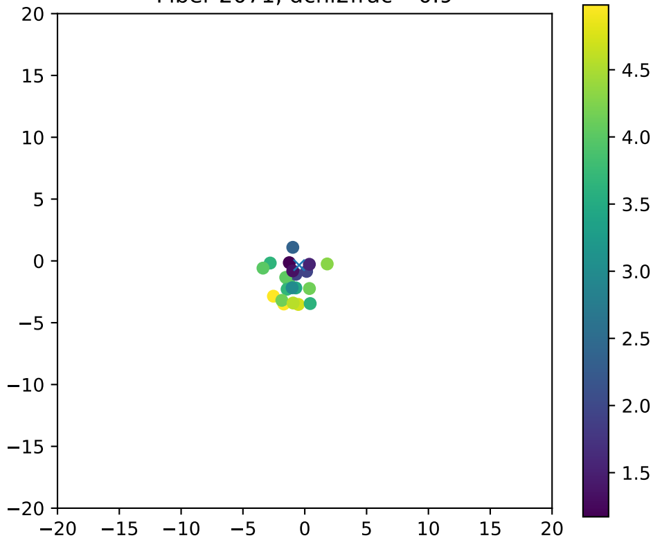
Fiber 2071, dchi2frac= 0.9
