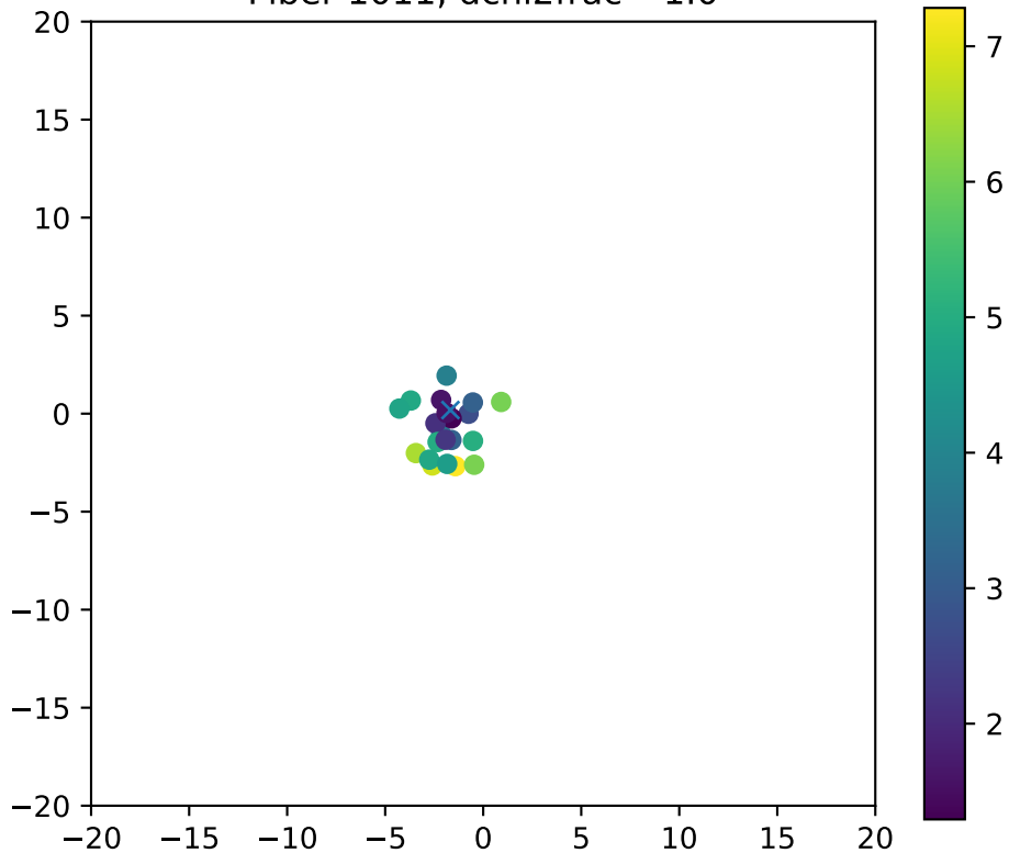
Fiber 1011, dchi2frac= 1.0
