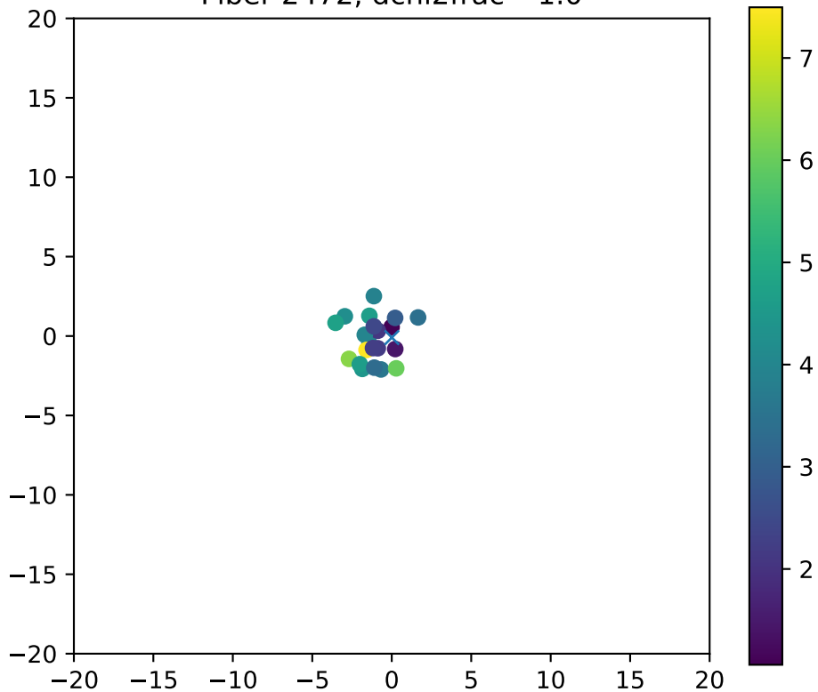
Fiber 2472, dchi2frac= 1.0
