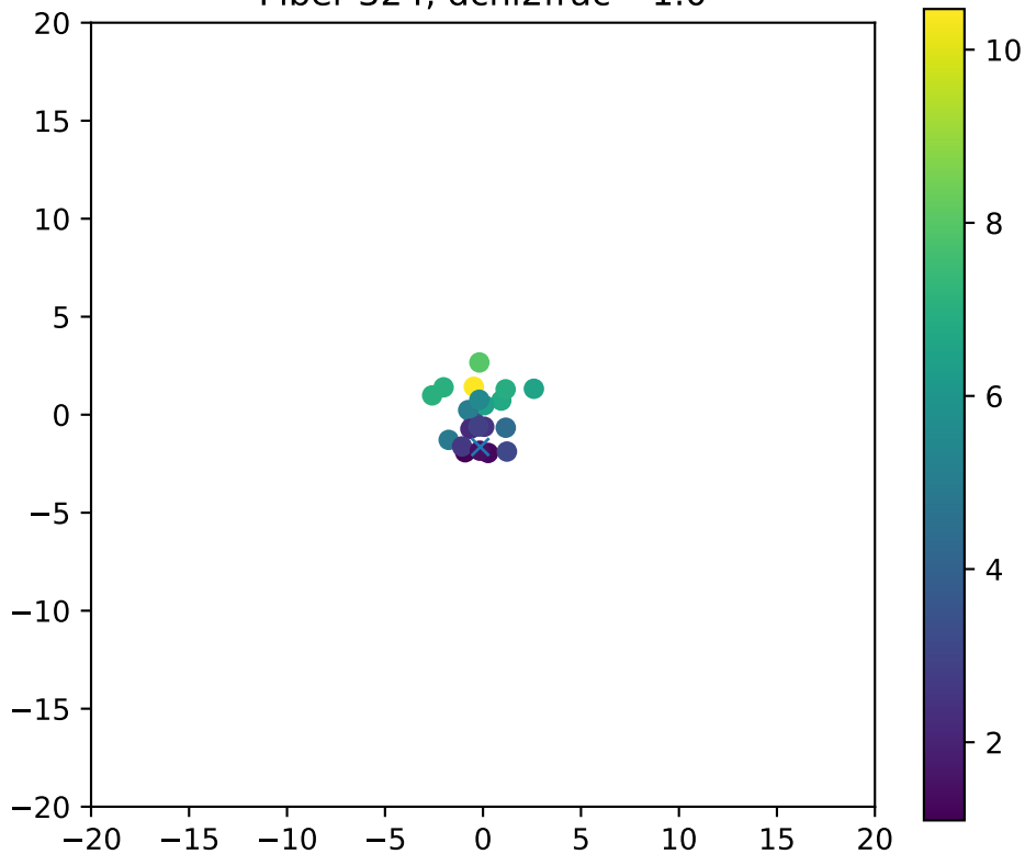
Fiber 324, dchi2frac= 1.0
