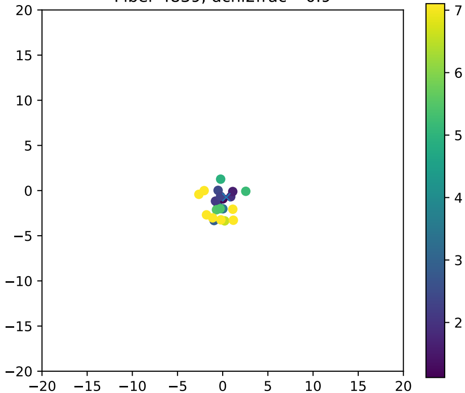
Fiber 4839, dchi2frac= 0.9
