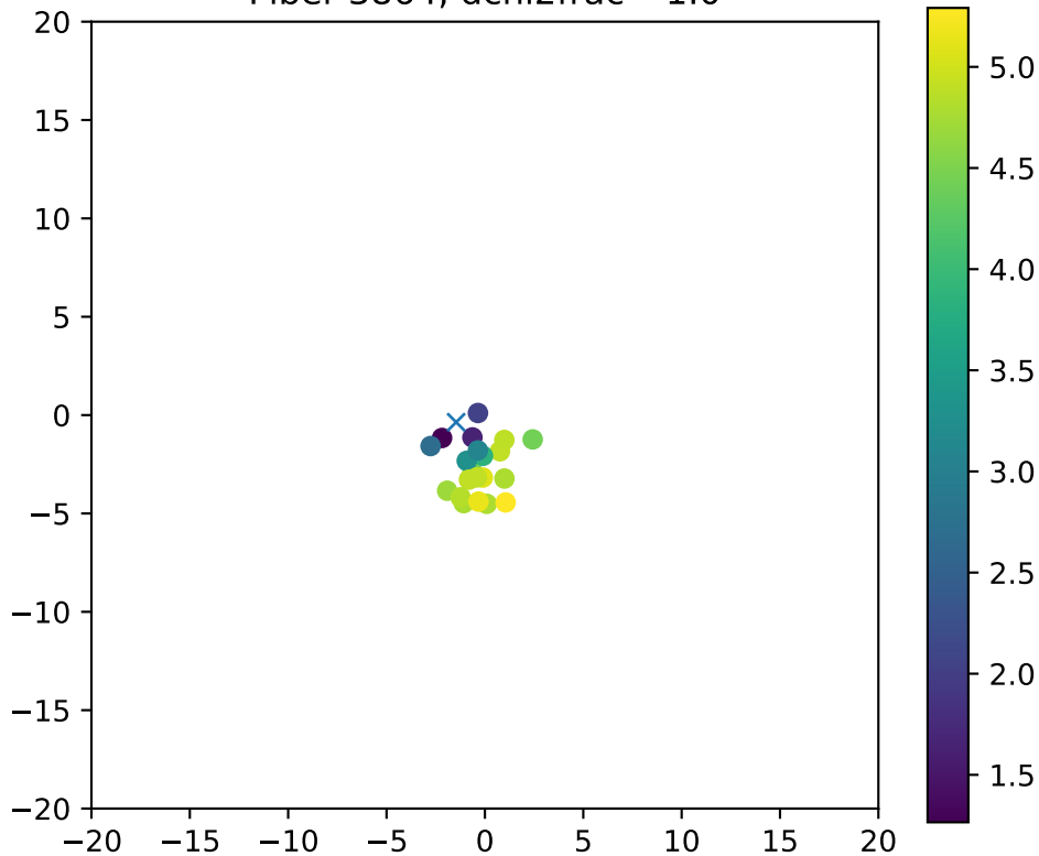
Fiber 3864, dchi2frac= 1.0
