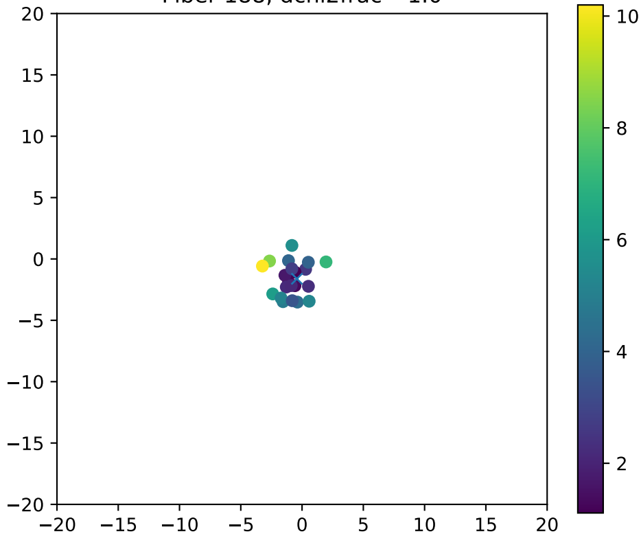
Fiber 188, dchi2frac= 1.0
