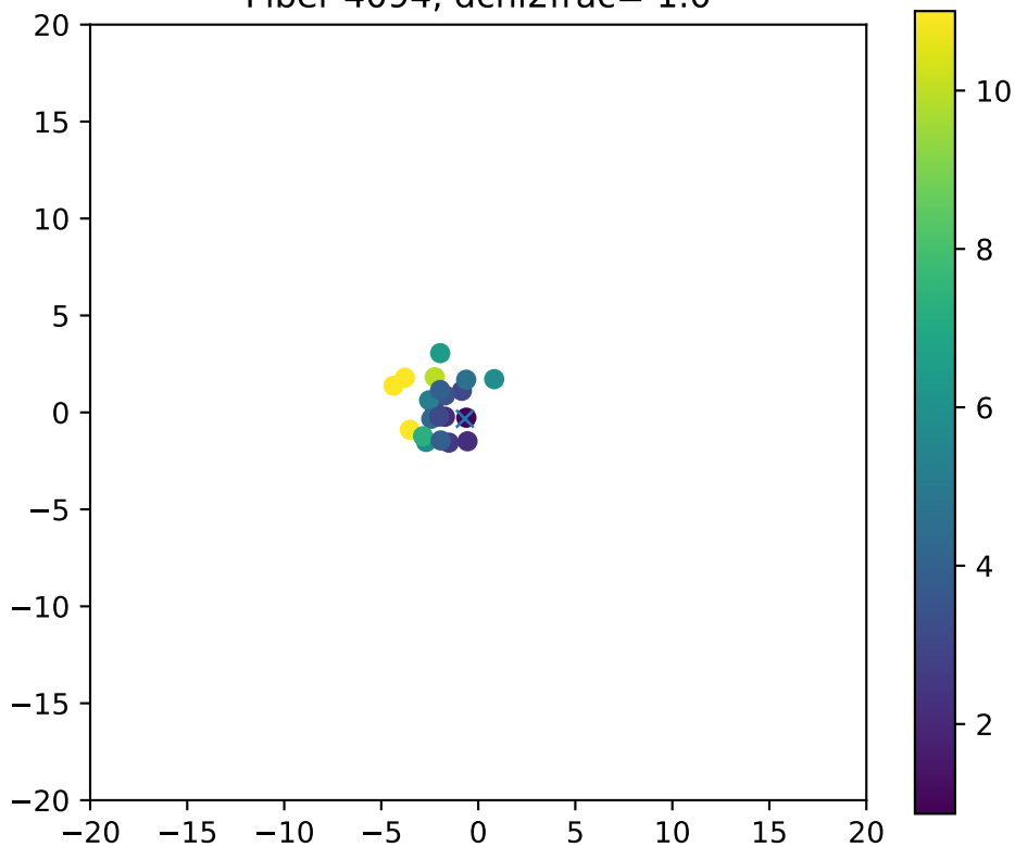
Fiber 4094, dchi2frac= 1.0
