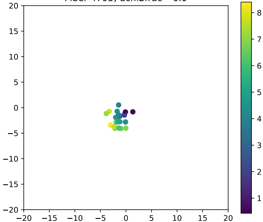
Fiber 4795, dchi2frac= 0.9
