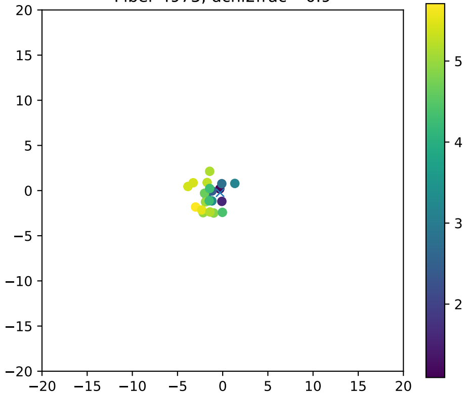
Fiber 4975, dchi2frac= 0.9
