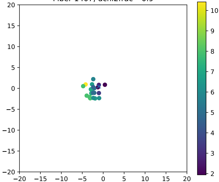
Fiber 1407, dchi2frac= 0.9
