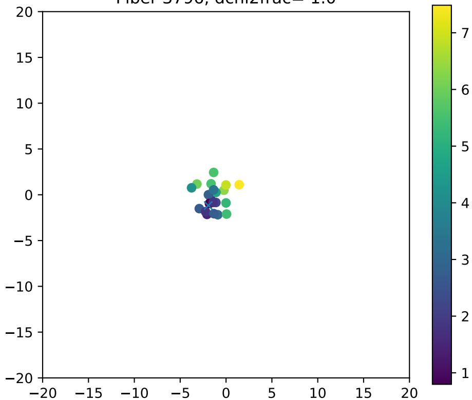
Fiber 3796, dchi2frac= 1.0
