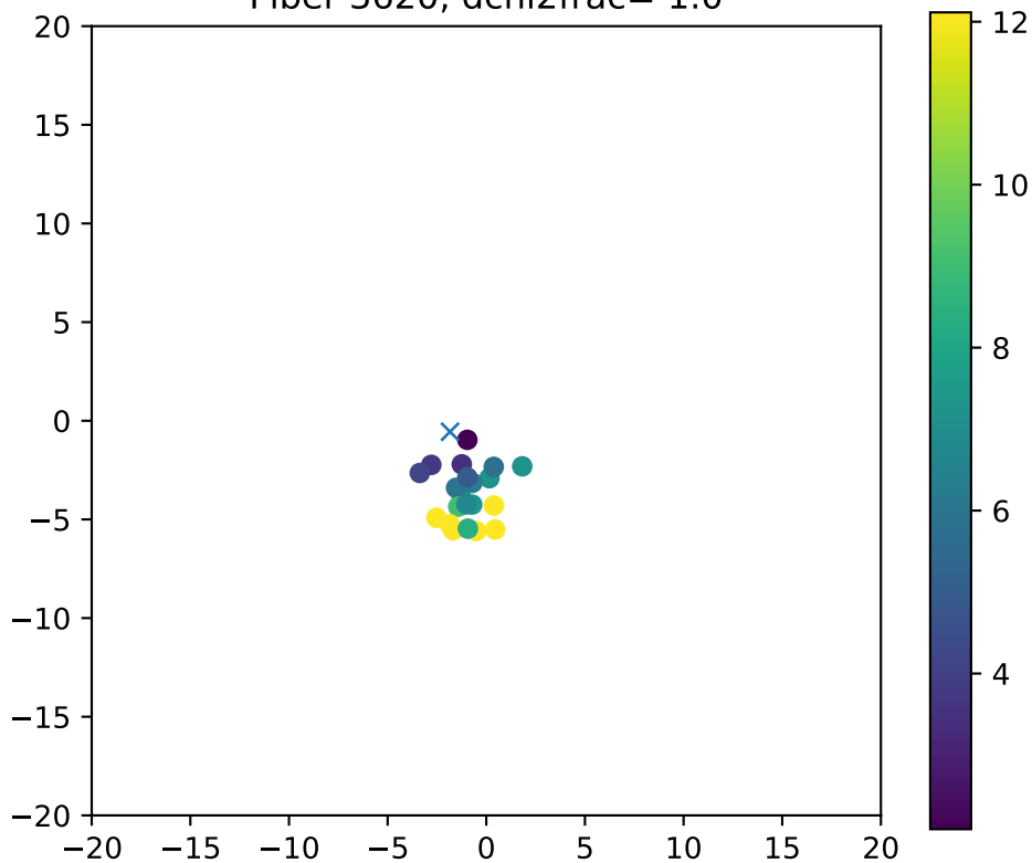
Fiber 3620, dchi2frac= 1.0
