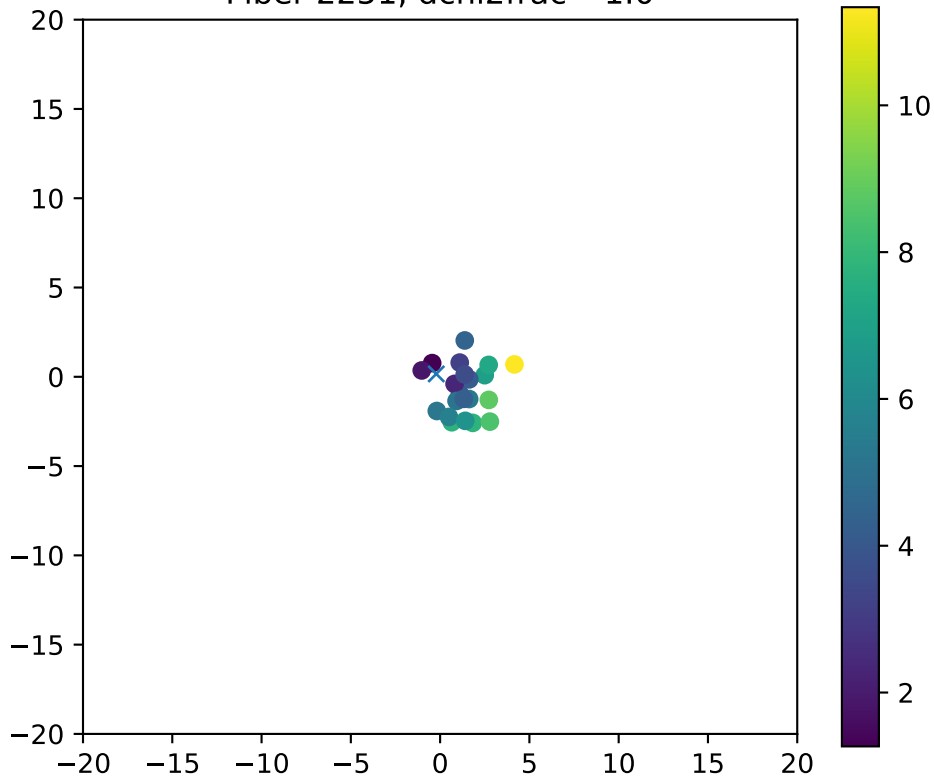
Fiber 2251, dchi2frac= 1.0
