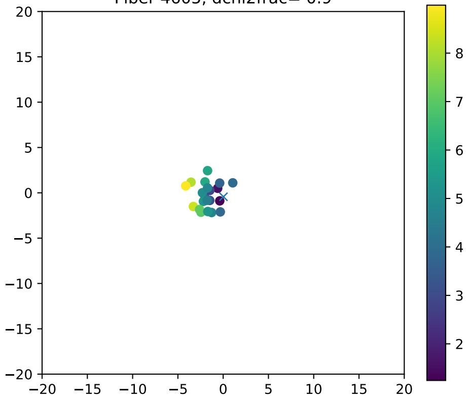
Fiber 4605, dchi2frac= 0.9
