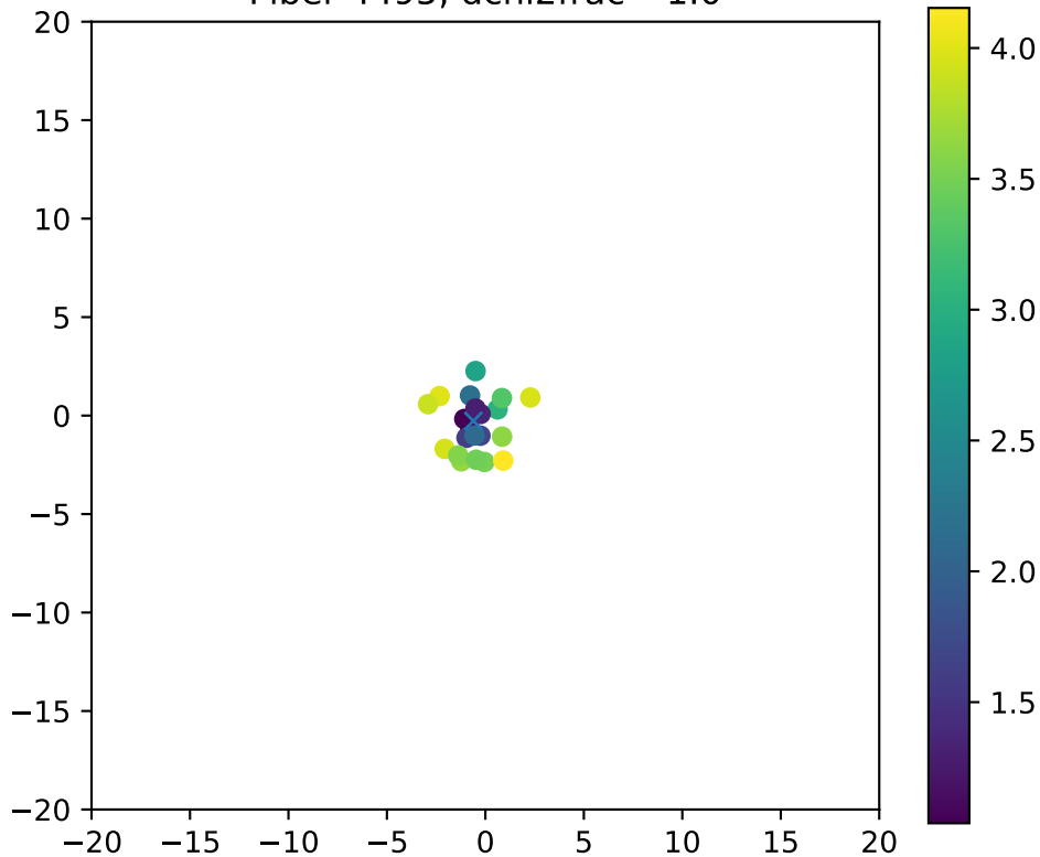
Fiber 4495, dchi2frac= 1.0
