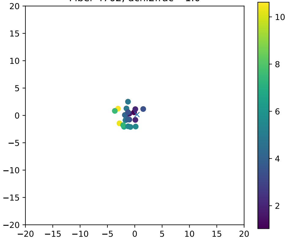
Fiber 4762, dchi2frac= 1.0
