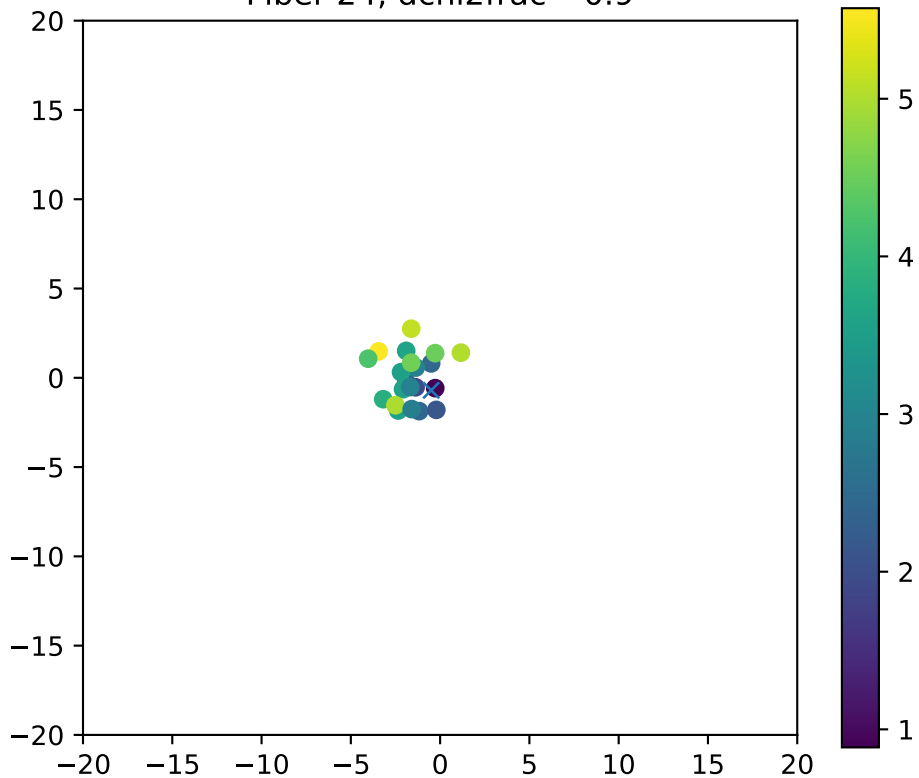
Fiber 24, dchi2frac= 0.9
