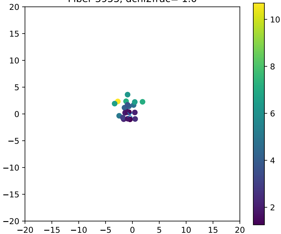
Fiber 3953, dchi2frac= 1.0
