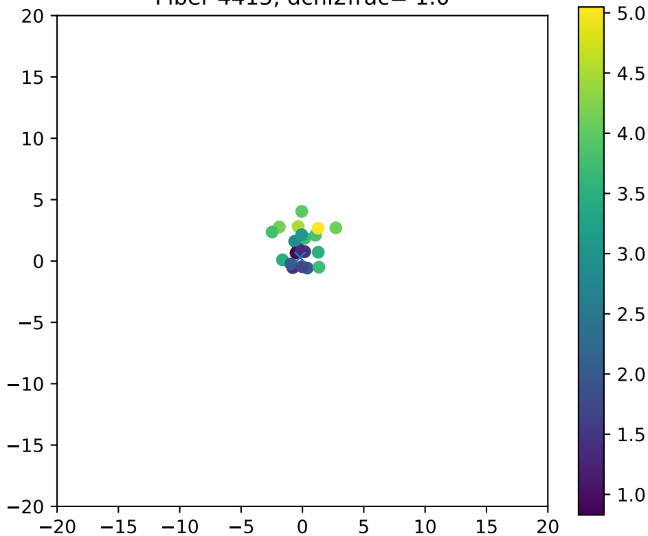
Fiber 4415, dchi2frac= 1.0
