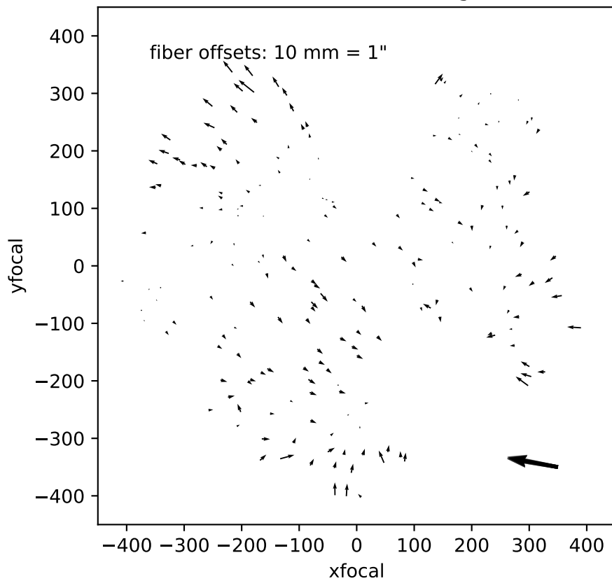
dither20200124-63074-highsnr-B
