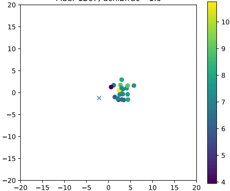
Fiber 1267, dchi2frac= 1.0
