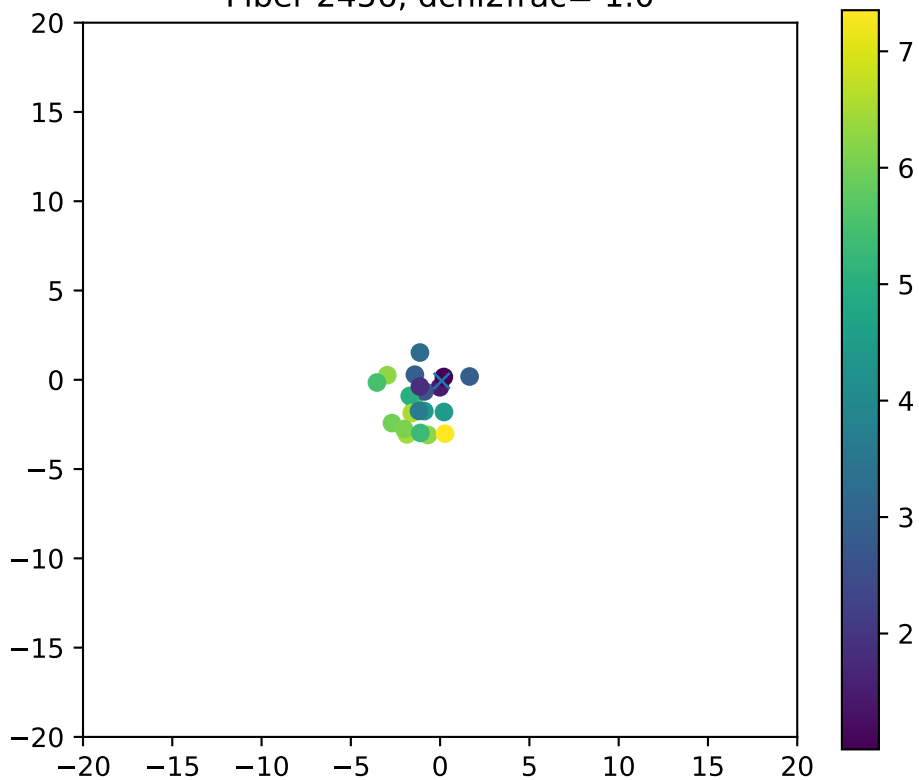
Fiber 2456, dchi2frac= 1.0
