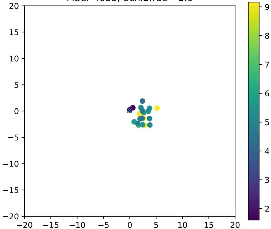
Fiber 4635, dchi2frac= 1.0
