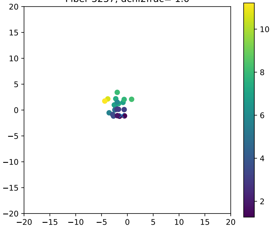
Fiber 3237, dchi2frac= 1.0
