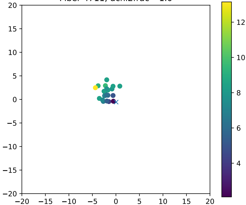
Fiber 4711, dchi2frac= 1.0
