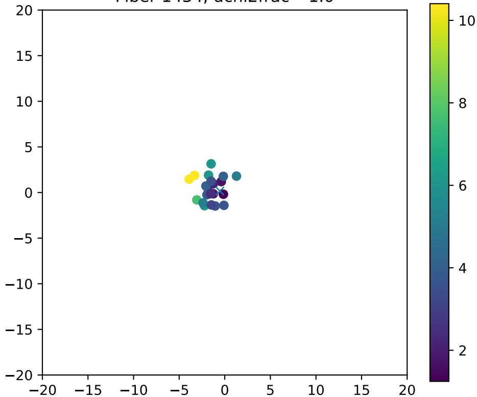
Fiber 1434, dchi2frac= 1.0
