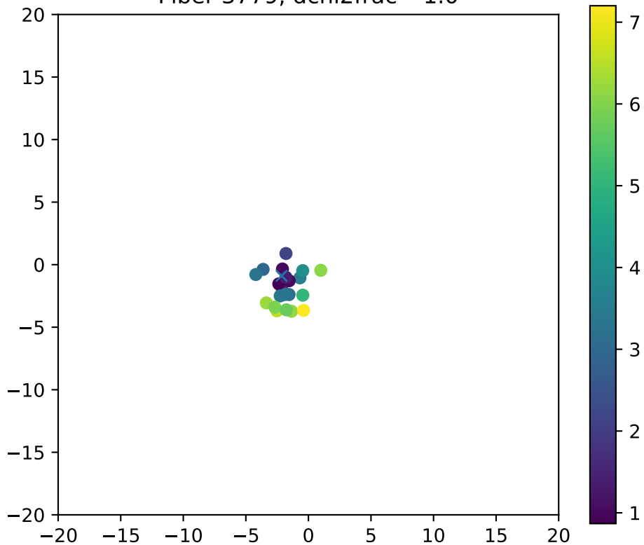
Fiber 3779, dchi2frac= 1.0
