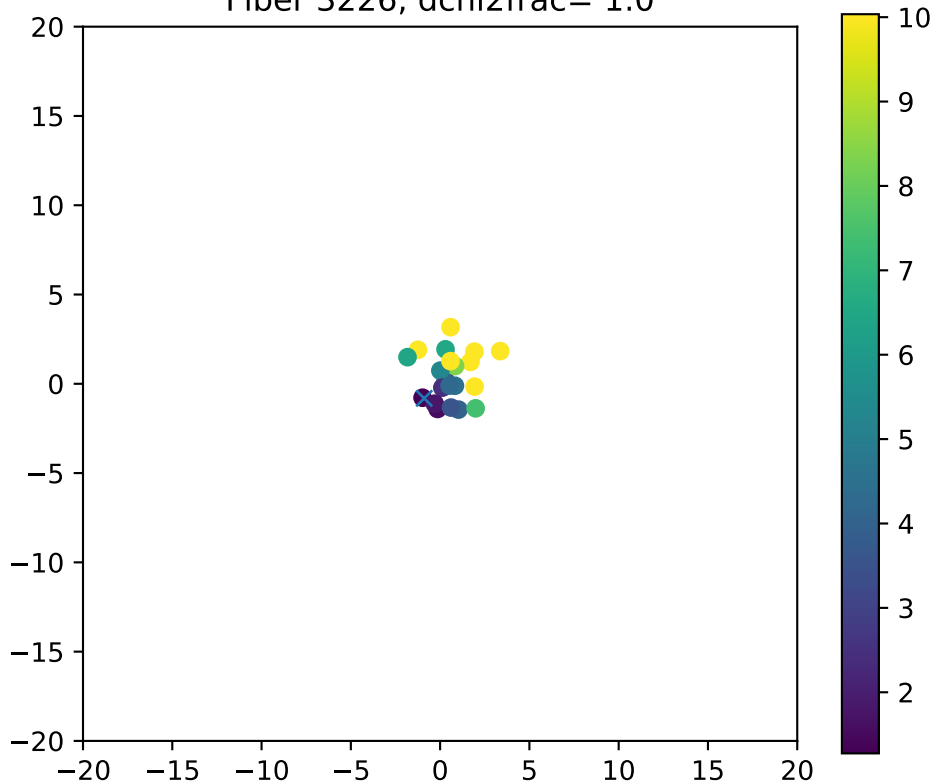
Fiber 3226, dchi2frac= 1.0
