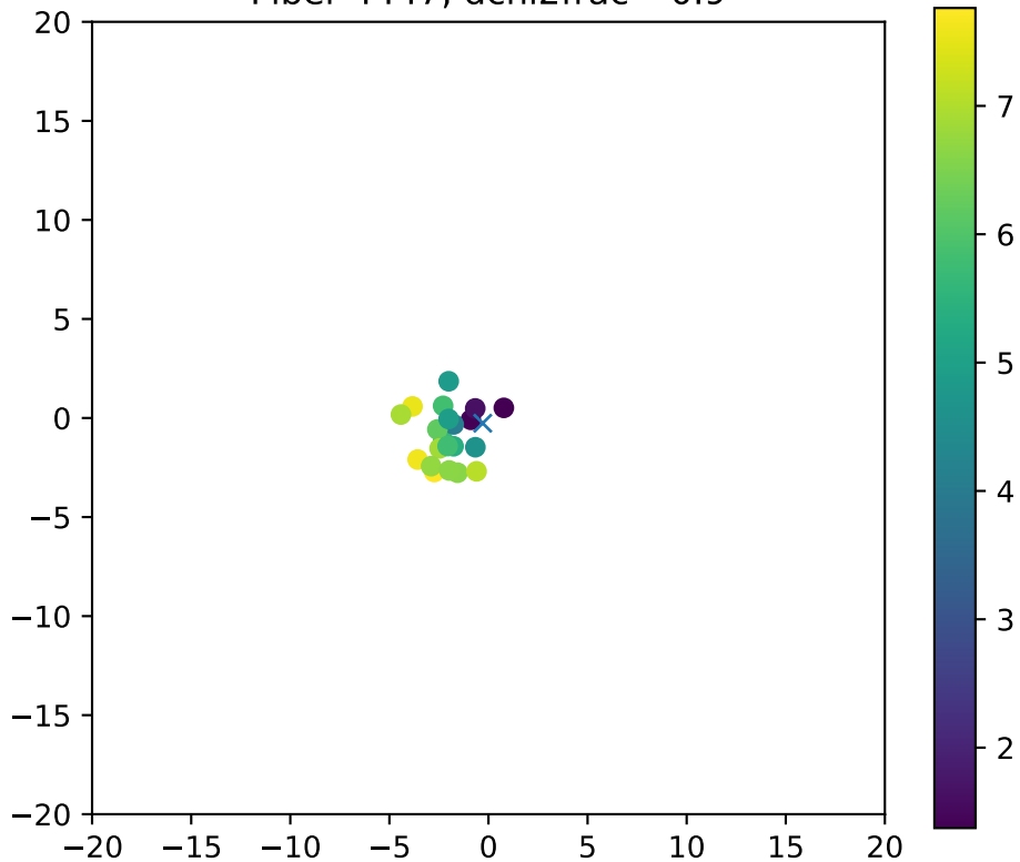
Fiber 4447, dchi2frac= 0.9
