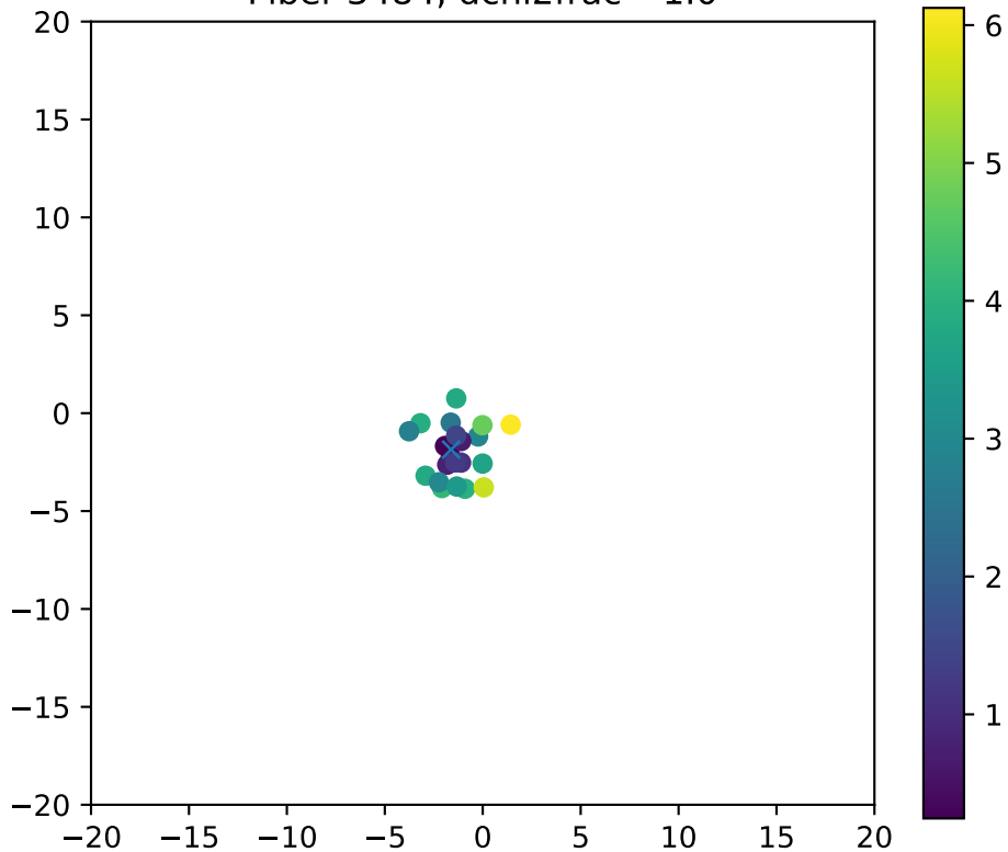
Fiber 3484, dchi2frac= 1.0
