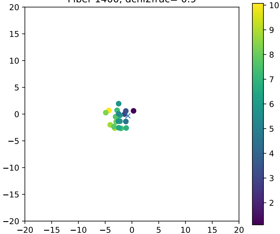
Fiber 1400, dchi2frac= 0.9
