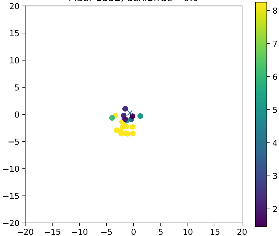
Fiber 1552, dchi2frac= 0.9
