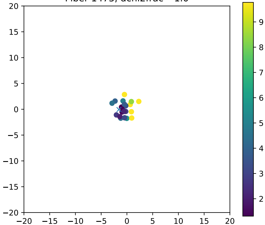
Fiber 1473, dchi2frac= 1.0
