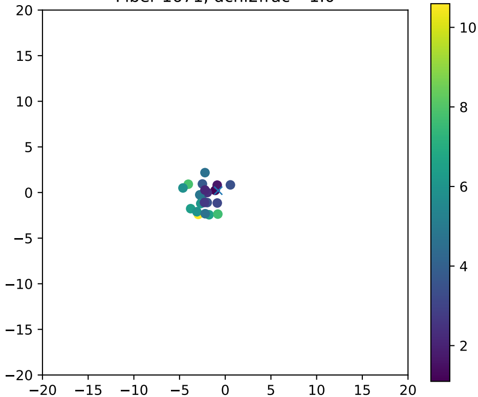
Fiber 1671, dchi2frac= 1.0
