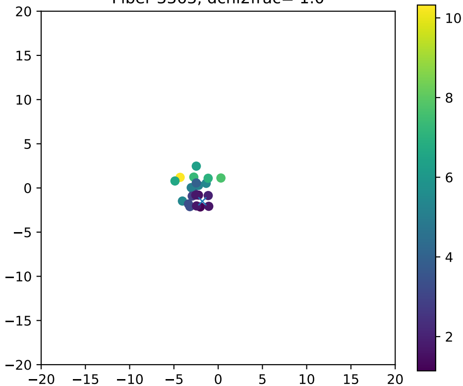
Fiber 3363, dchi2frac= 1.0
