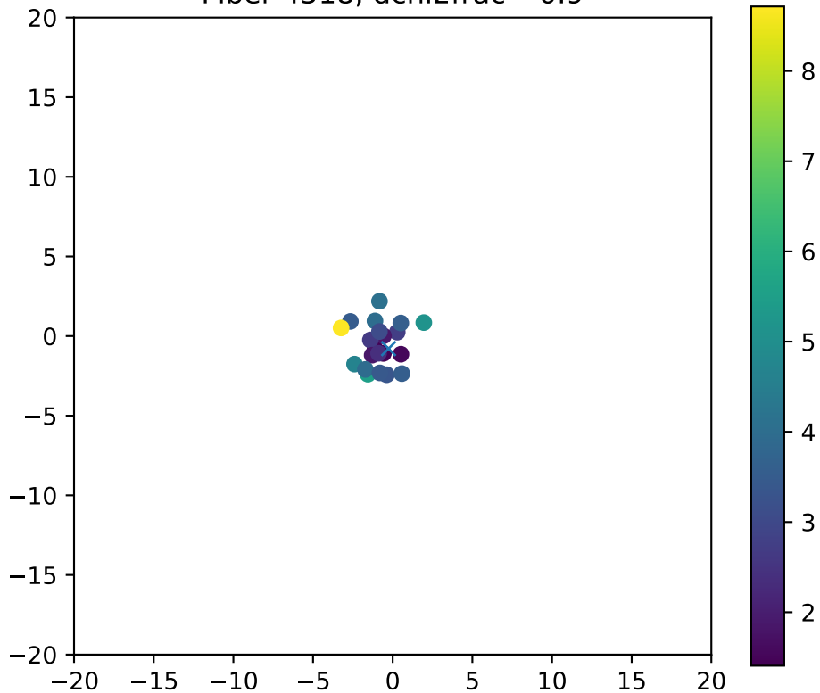
Fiber 4518, dchi2frac= 0.9
