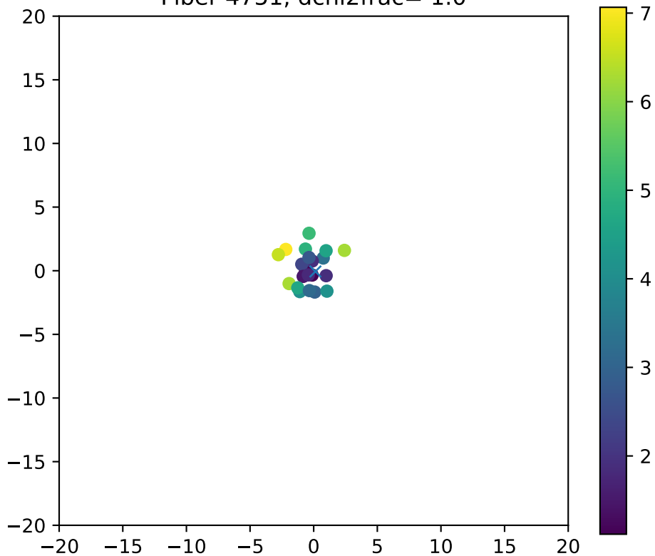
Fiber 4751, dchi2frac= 1.0
