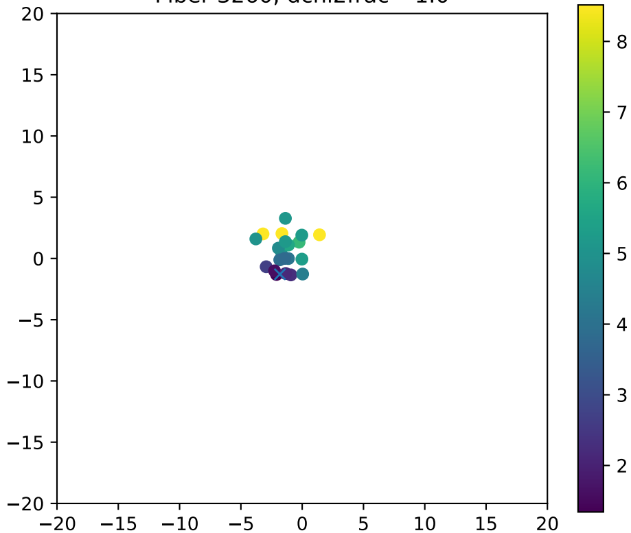
Fiber 3260, dchi2frac= 1.0
