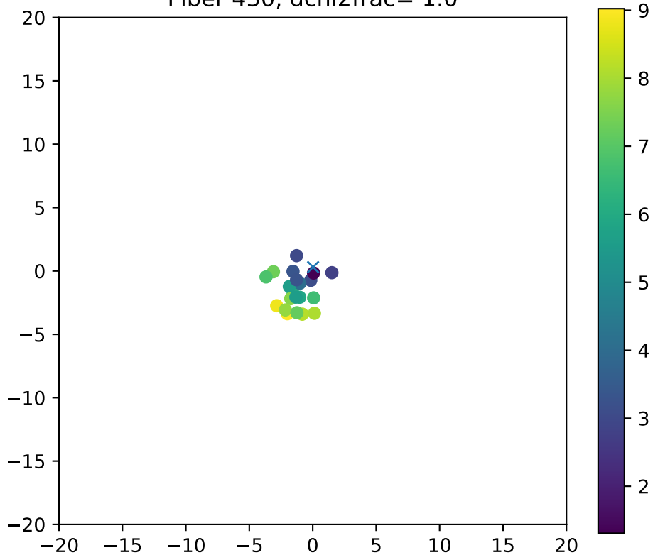
Fiber 430, dchi2frac= 1.0
