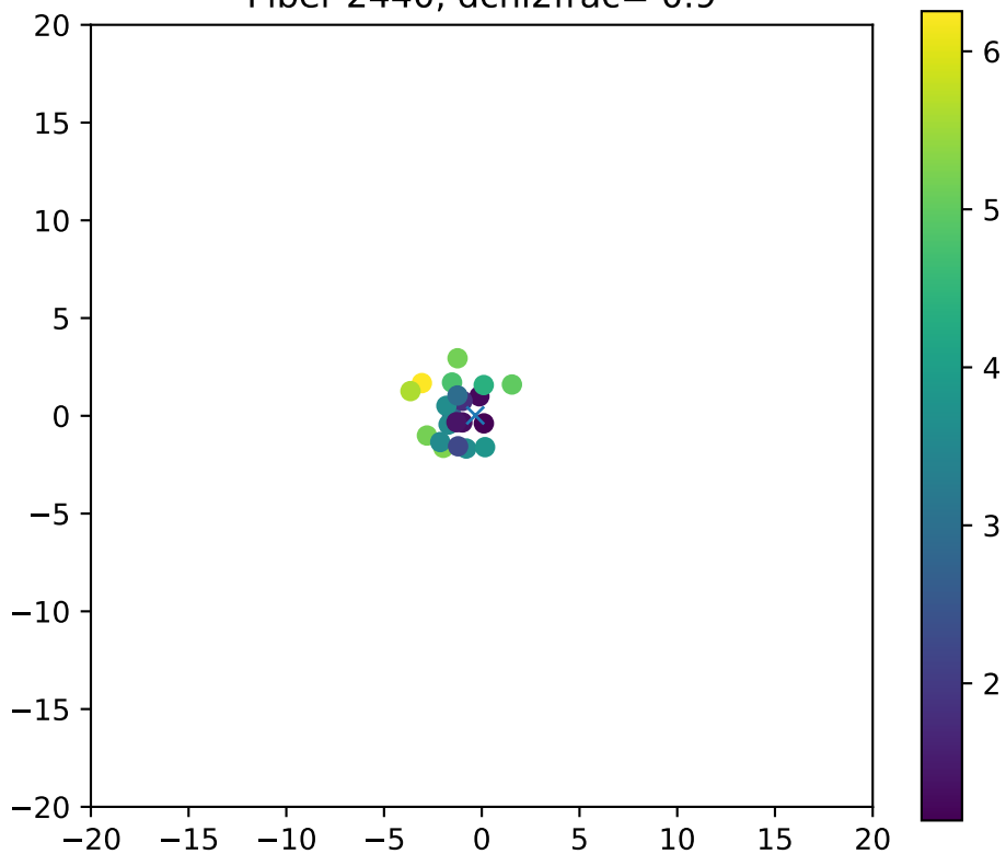
Fiber 2440, dchi2frac= 0.9
