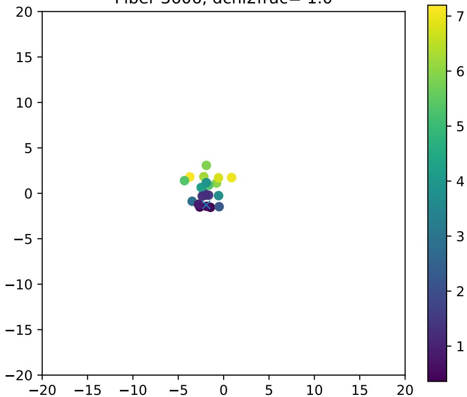
Fiber 3606, dchi2frac= 1.0
