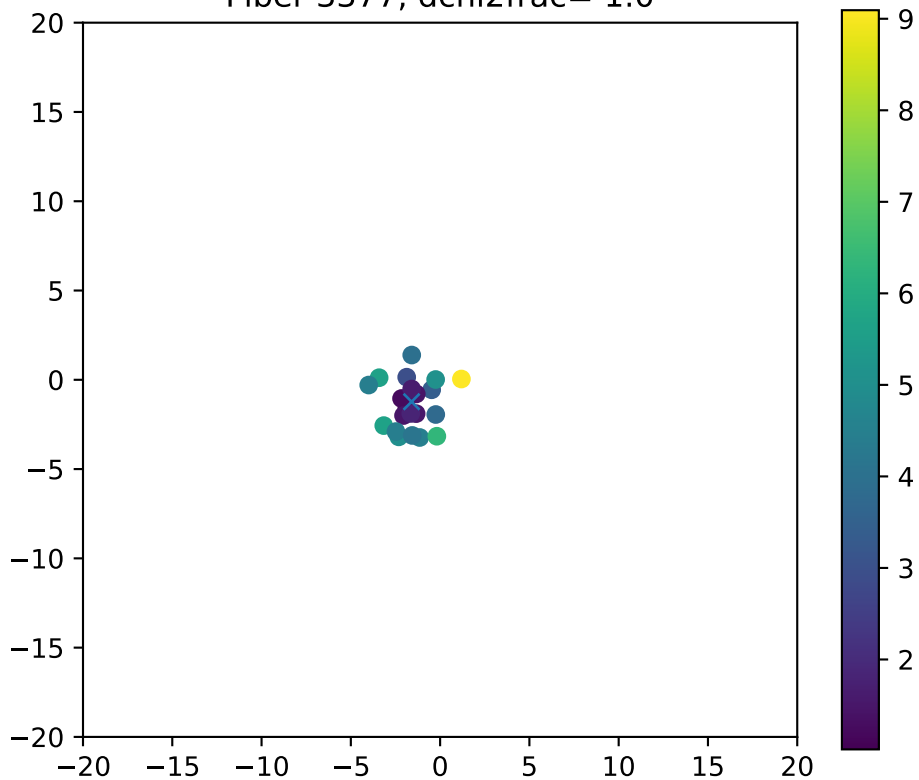
Fiber 3377, dchi2frac= 1.0
