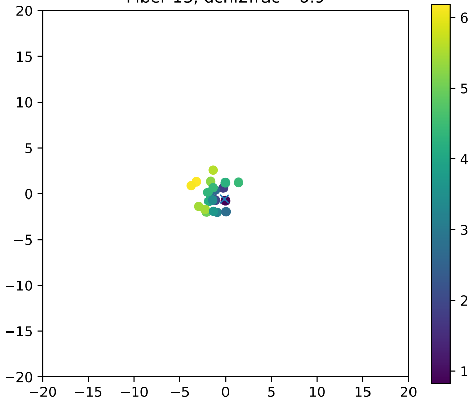
Fiber 13, dchi2frac= 0.9
