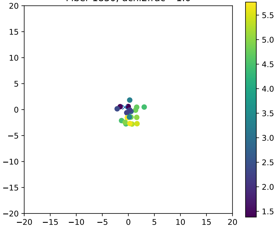
Fiber 1830, dchi2frac= 1.0
