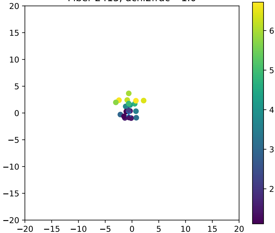
Fiber 2413, dchi2frac= 1.0
