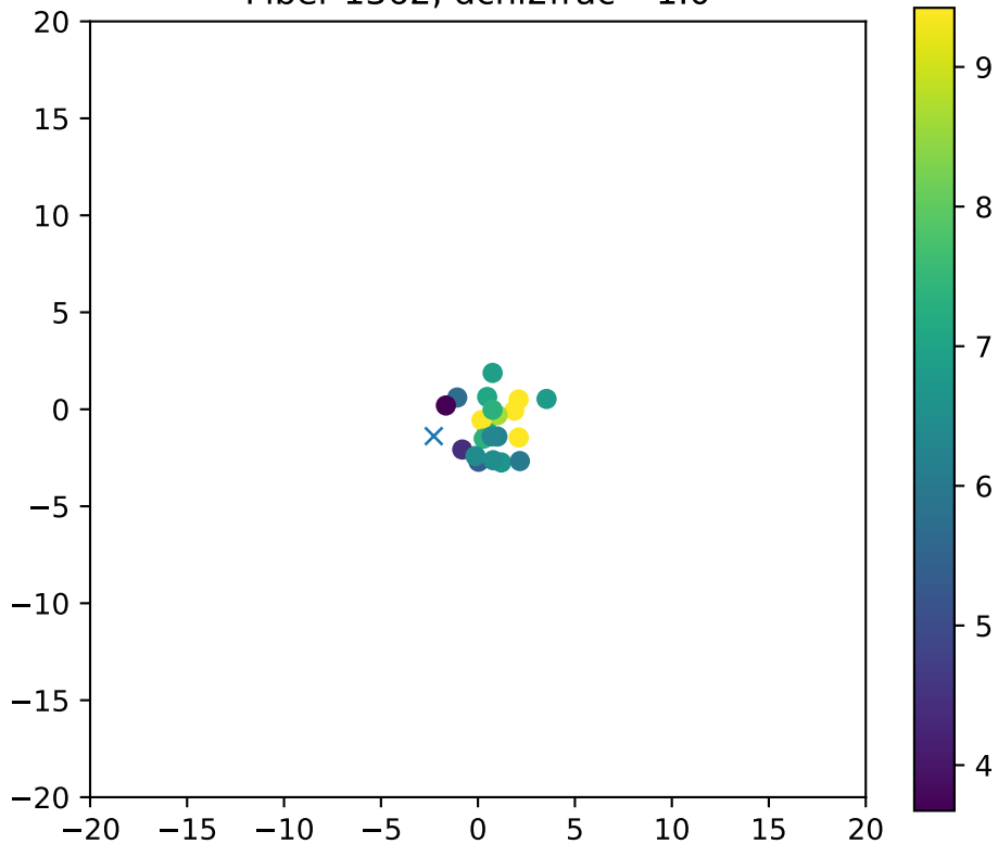
Fiber 1362, dchi2frac= 1.0
