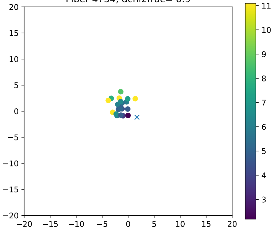
Fiber 4754, dchi2frac= 0.9
