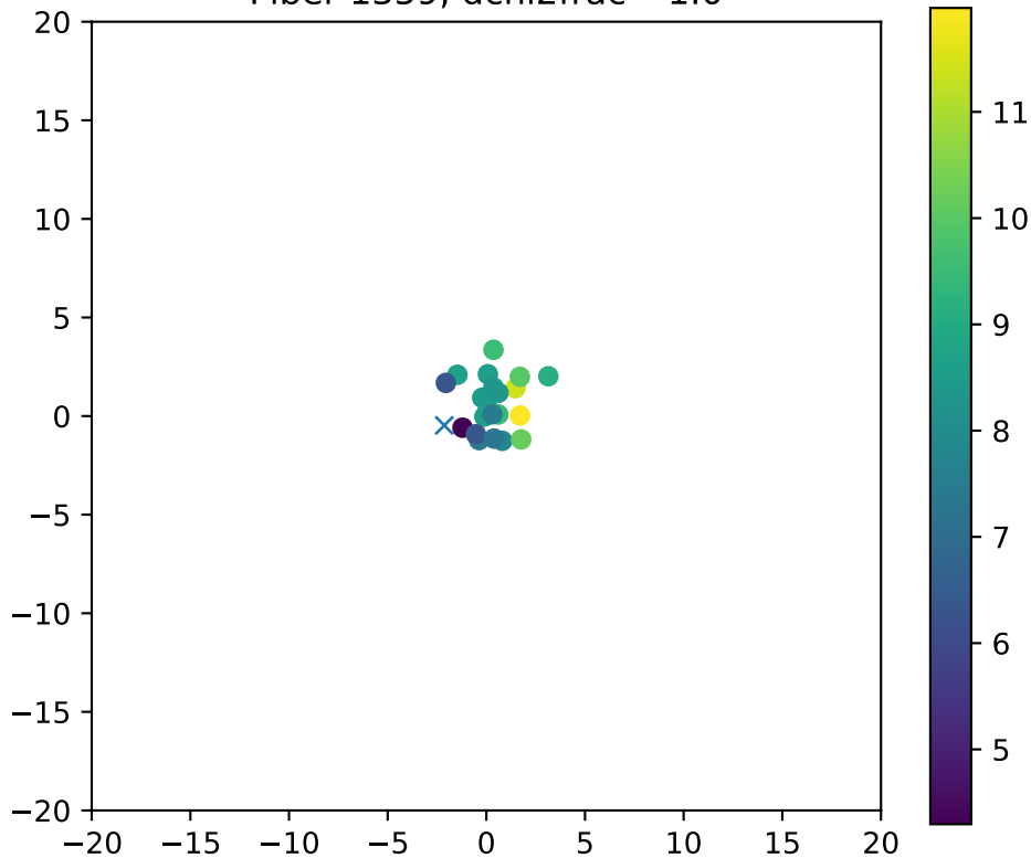
Fiber 1359, dchi2frac= 1.0
