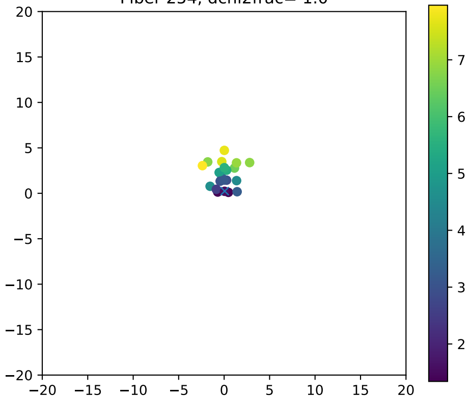
Fiber 254, dchi2frac= 1.0
