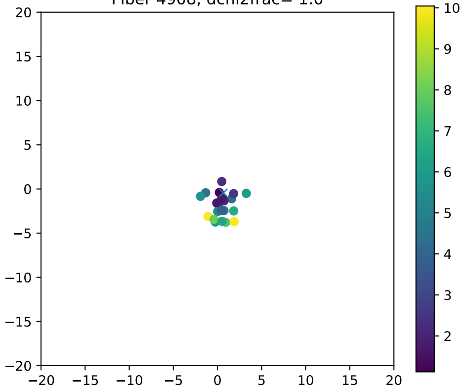
Fiber 4908, dchi2frac= 1.0
