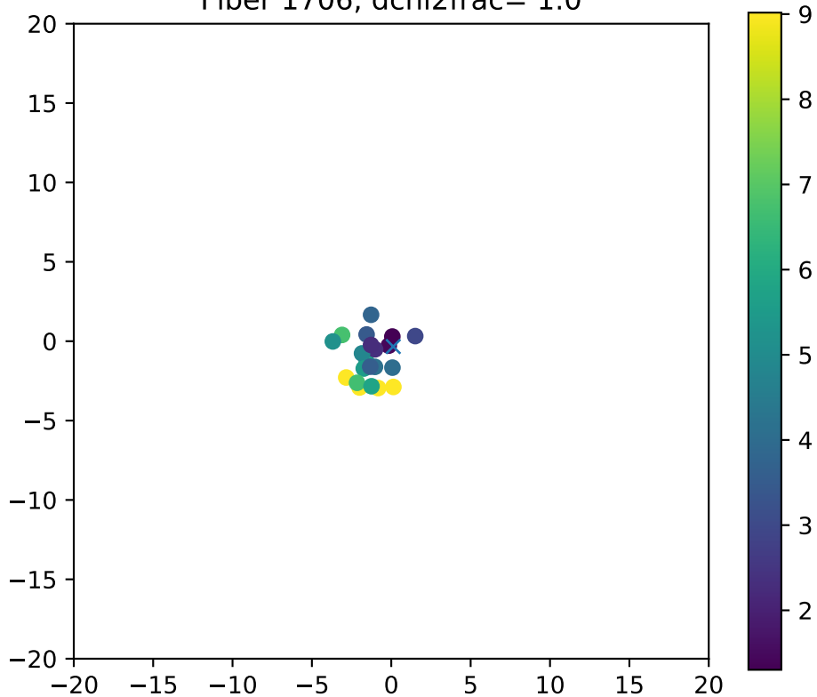
Fiber 1706, dchi2frac= 1.0
