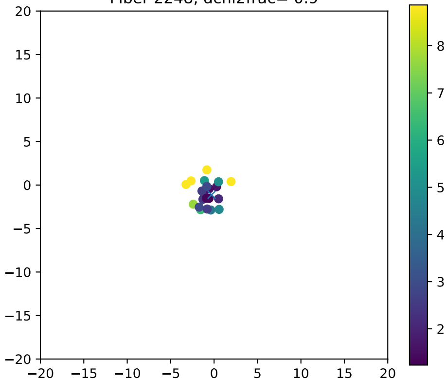
Fiber 2248, dchi2frac= 0.9
