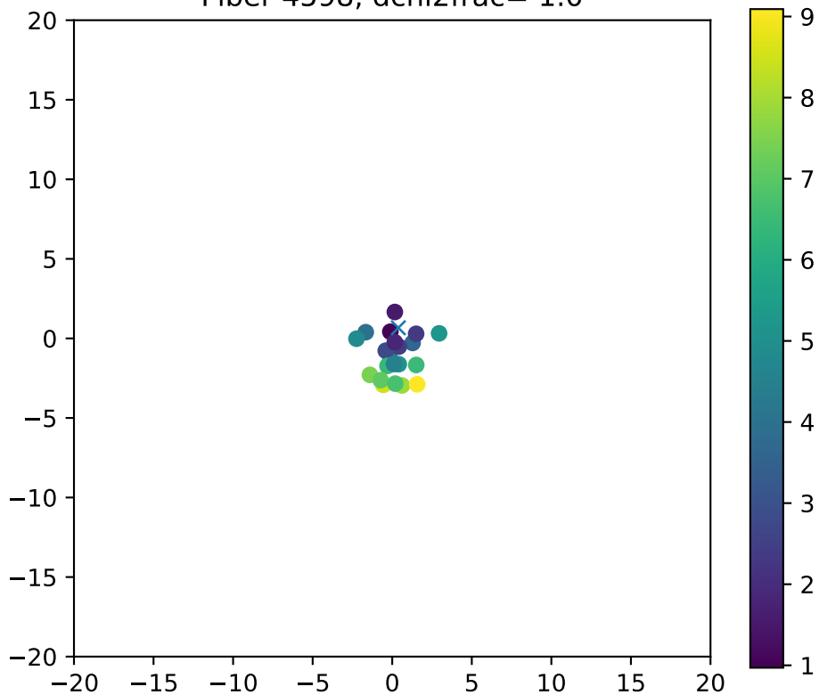
Fiber 4598, dchi2frac= 1.0
