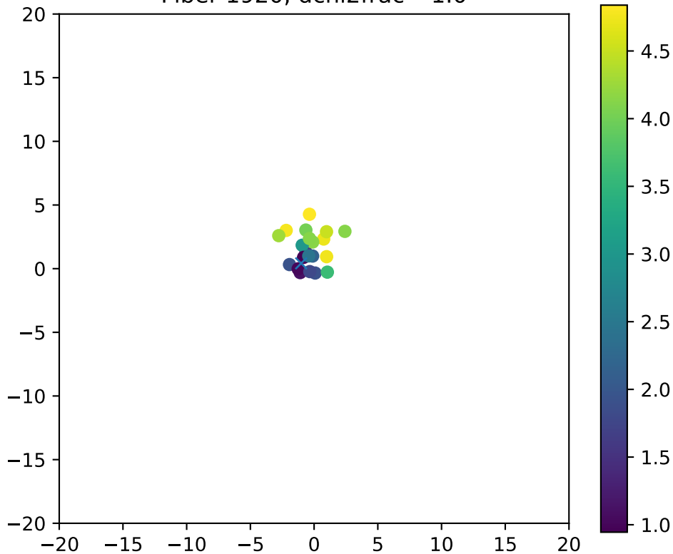
Fiber 1920, dchi2frac= 1.0
