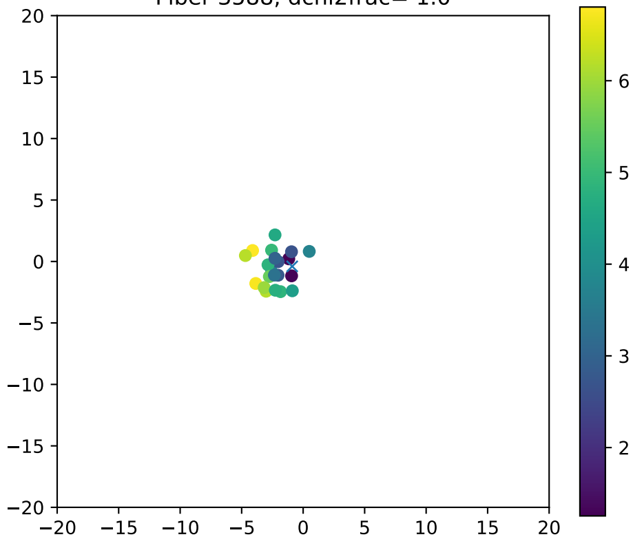
Fiber 3588, dchi2frac= 1.0
