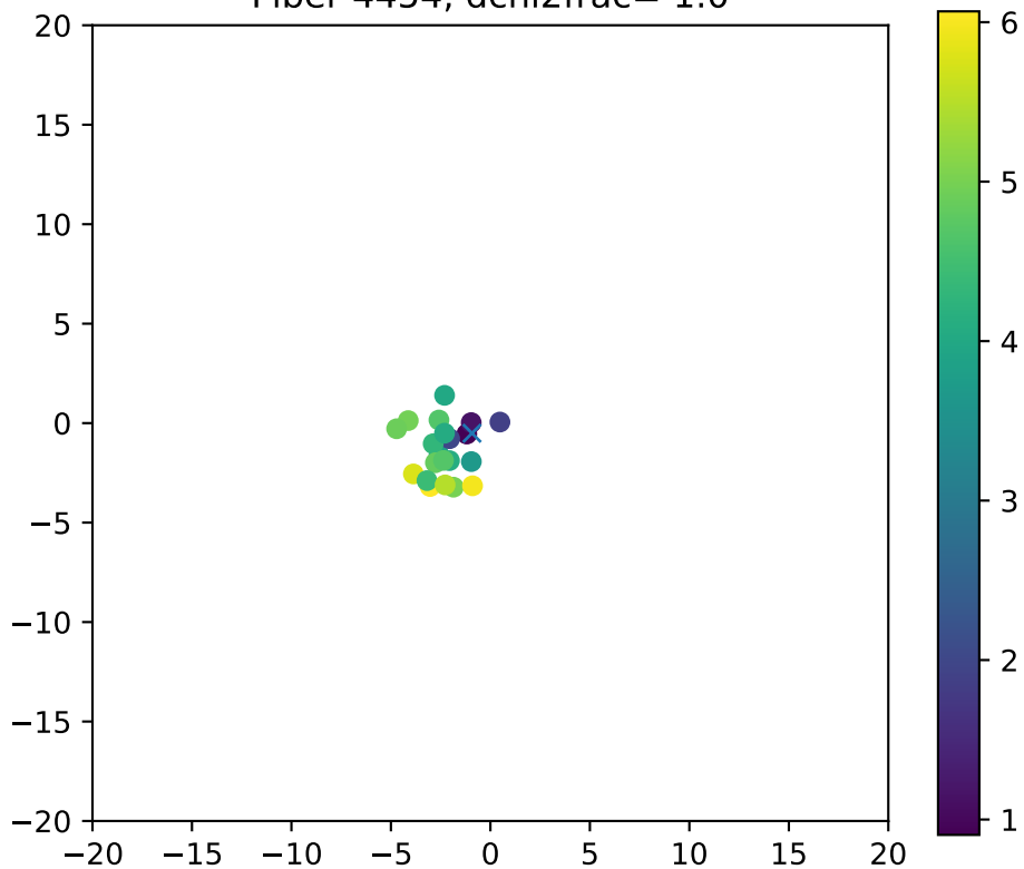
Fiber 4454, dchi2frac= 1.0
