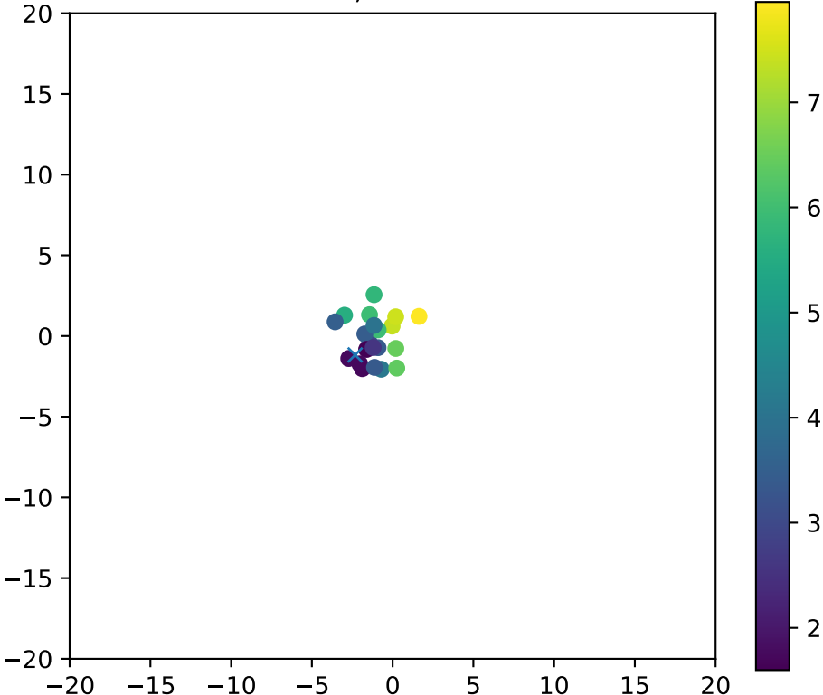
Fiber 3753, dchi2frac= 1.0
