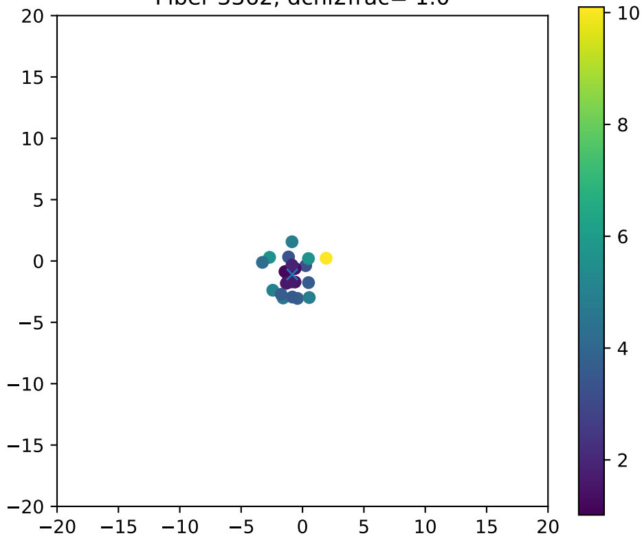
Fiber 3362, dchi2frac= 1.0
