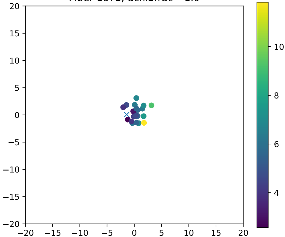
Fiber 1672, dchi2frac= 1.0
