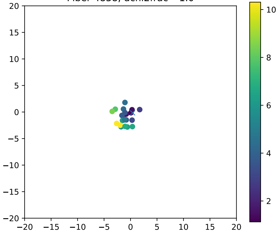
Fiber 4838, dchi2frac= 1.0
