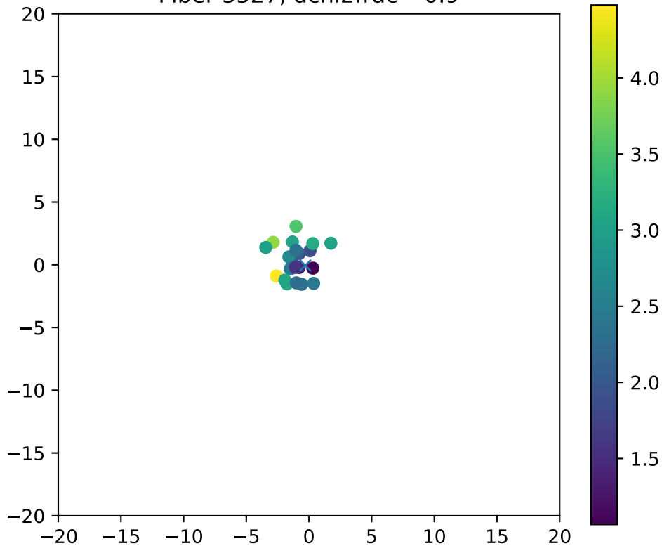
Fiber 3527, dchi2frac= 0.9
