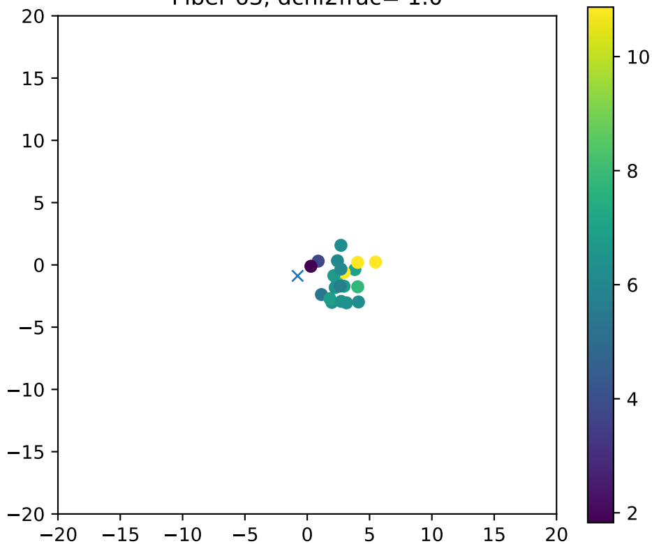
Fiber 63, dchi2frac= 1.0
