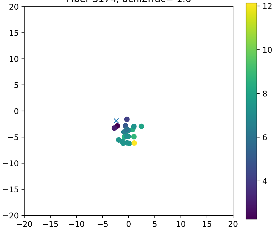
Fiber 3174, dchi2frac= 1.0
