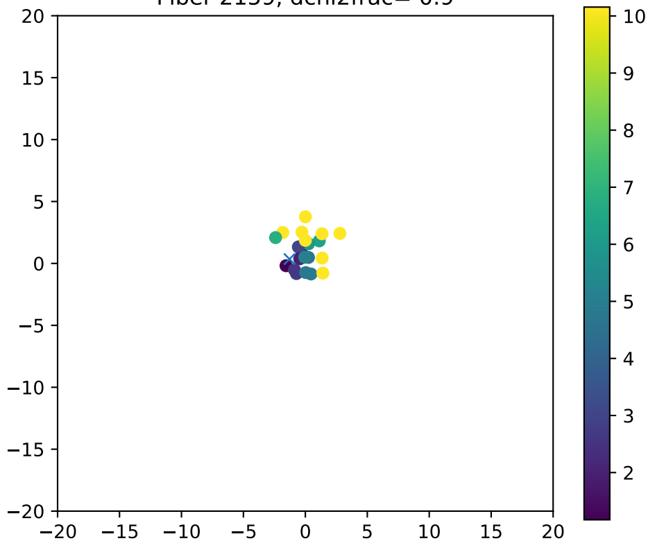
Fiber 2159, dchi2frac= 0.9
