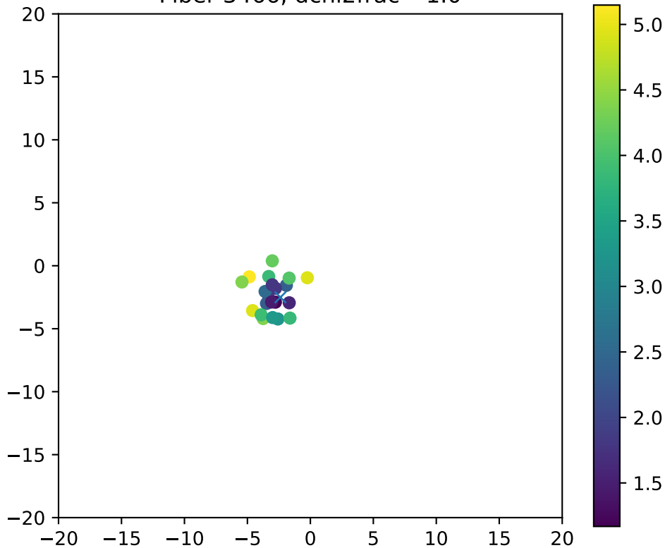
Fiber 3466, dchi2frac= 1.0
