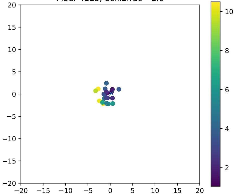
Fiber 4225, dchi2frac= 1.0
