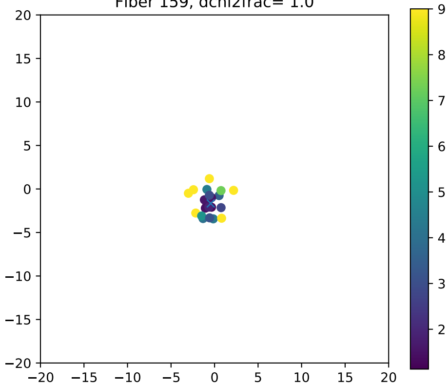
Fiber 159, dchi2frac= 1.0
