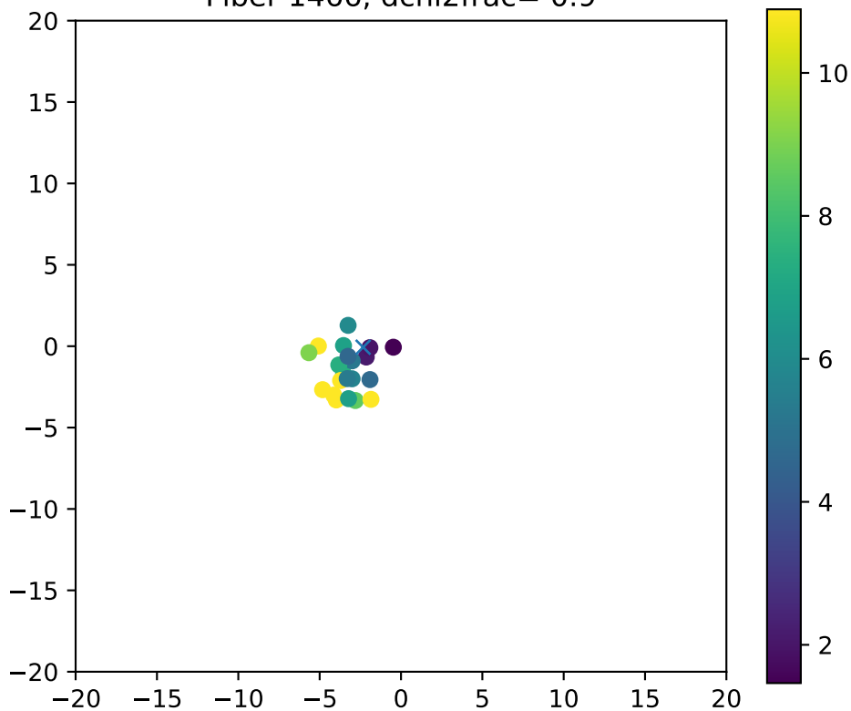
Fiber 1466, dchi2frac= 0.9
