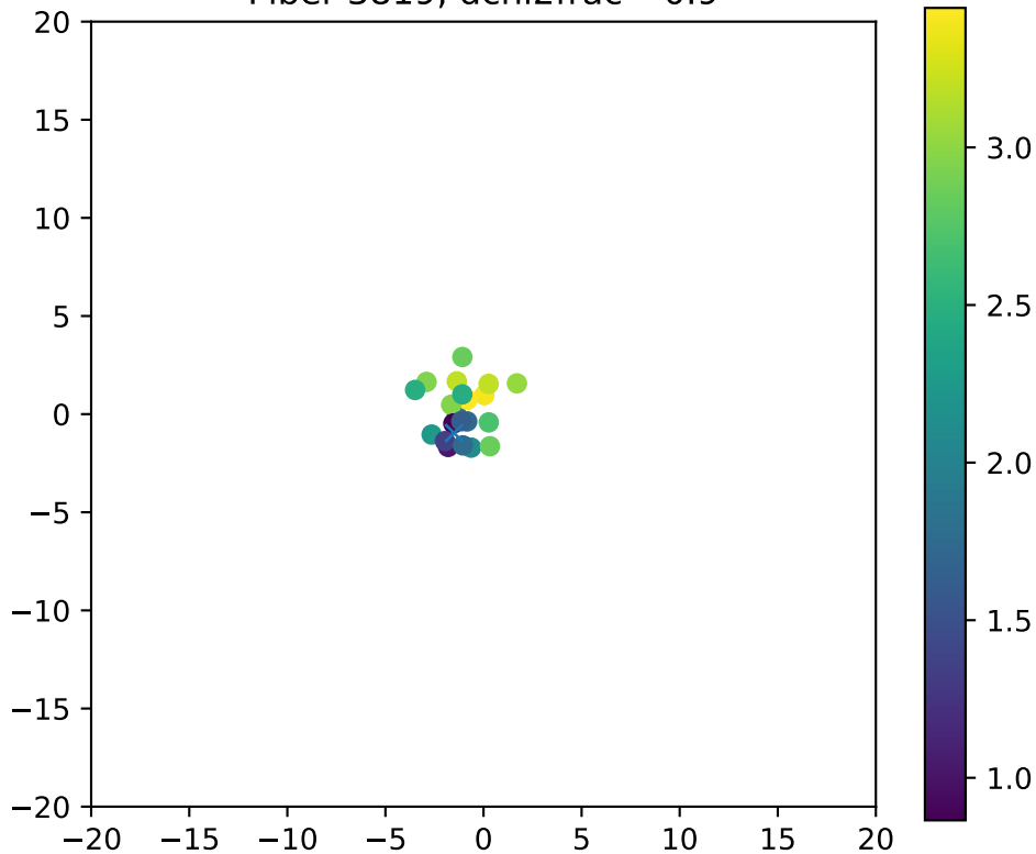
Fiber 3819, dchi2frac= 0.9
