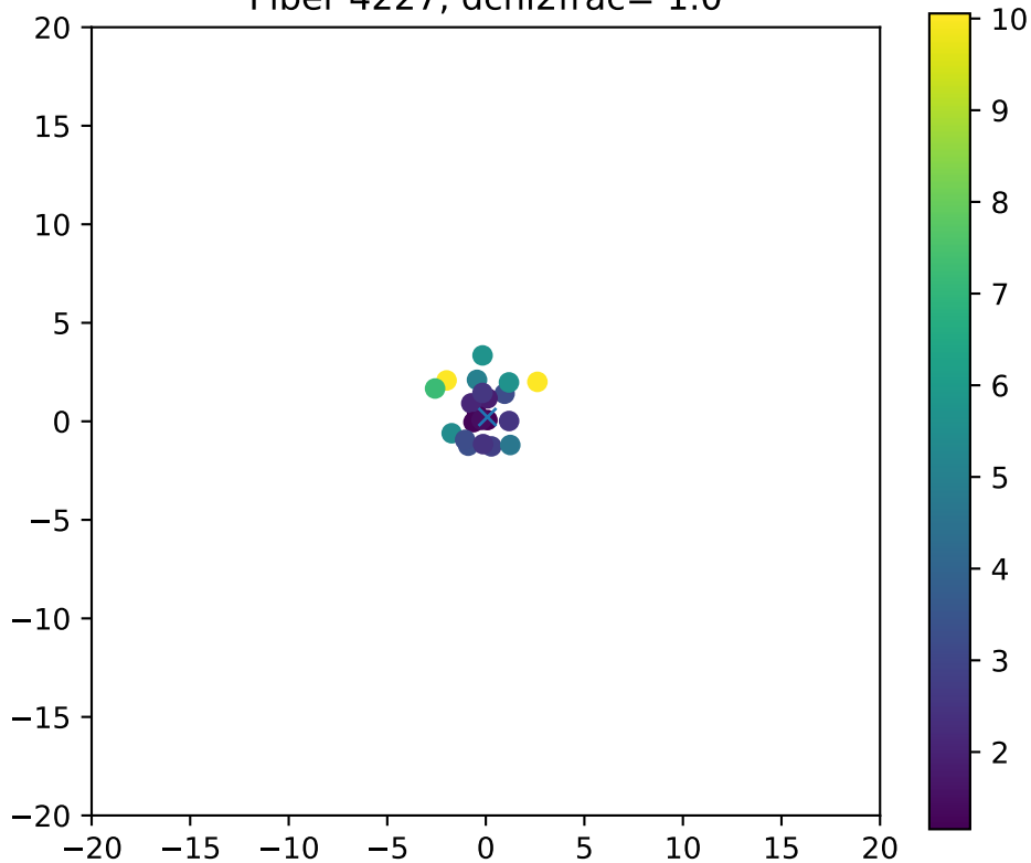
Fiber 4227, dchi2frac= 1.0
