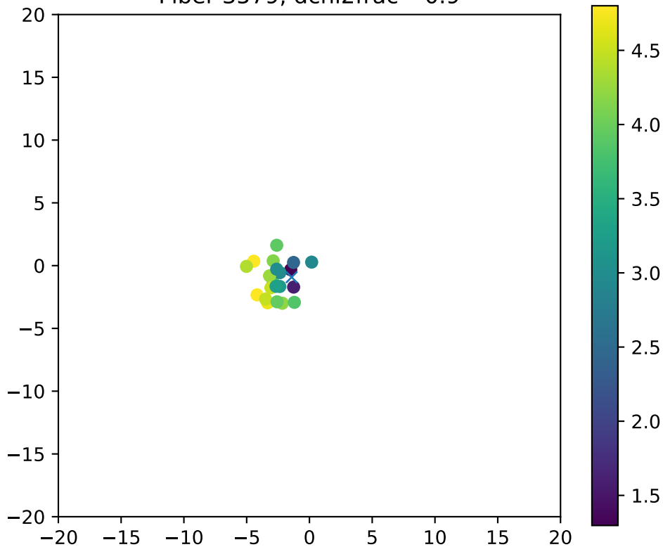
Fiber 3579, dchi2frac= 0.9
