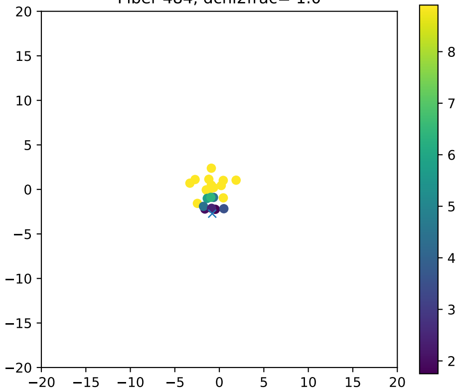
Fiber 484, dchi2frac= 1.0
