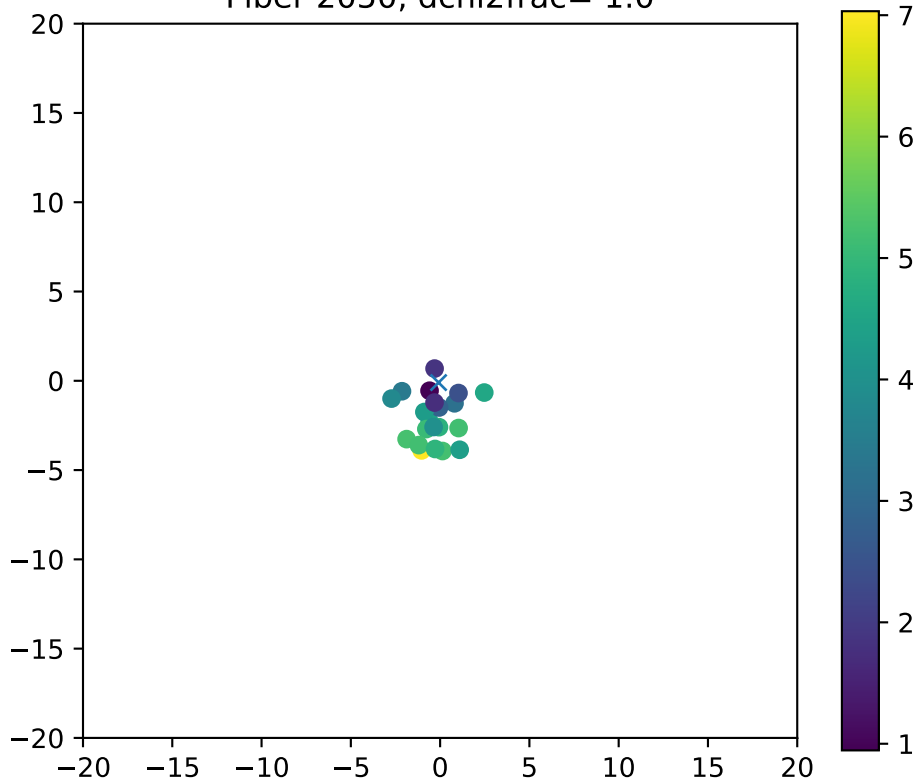
Fiber 2050, dchi2frac= 1.0
