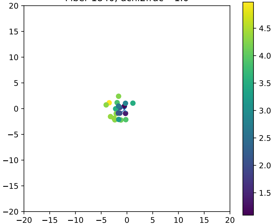
Fiber 1840, dchi2frac= 1.0
