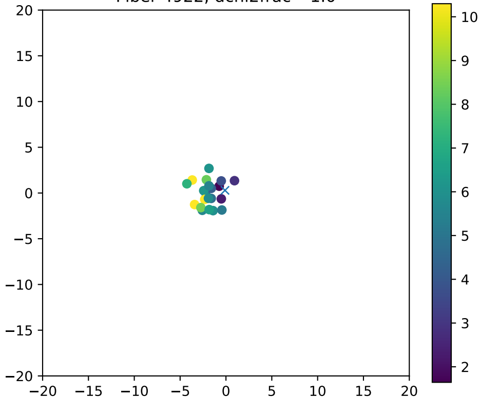
Fiber 4922, dchi2frac= 1.0
