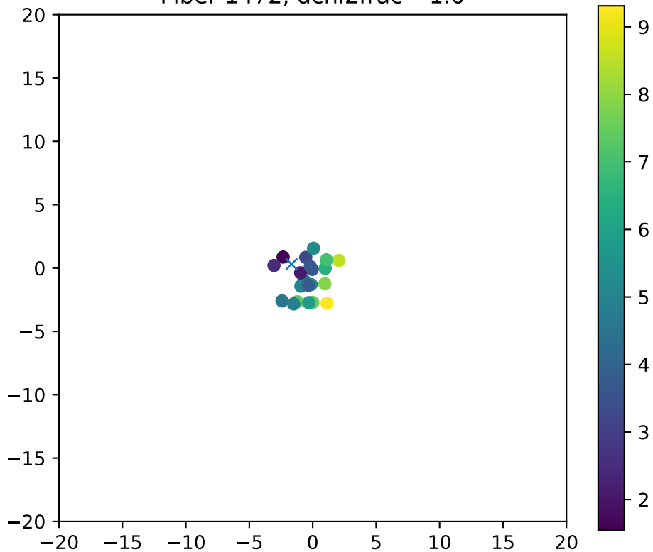
Fiber 1472, dchi2frac= 1.0
