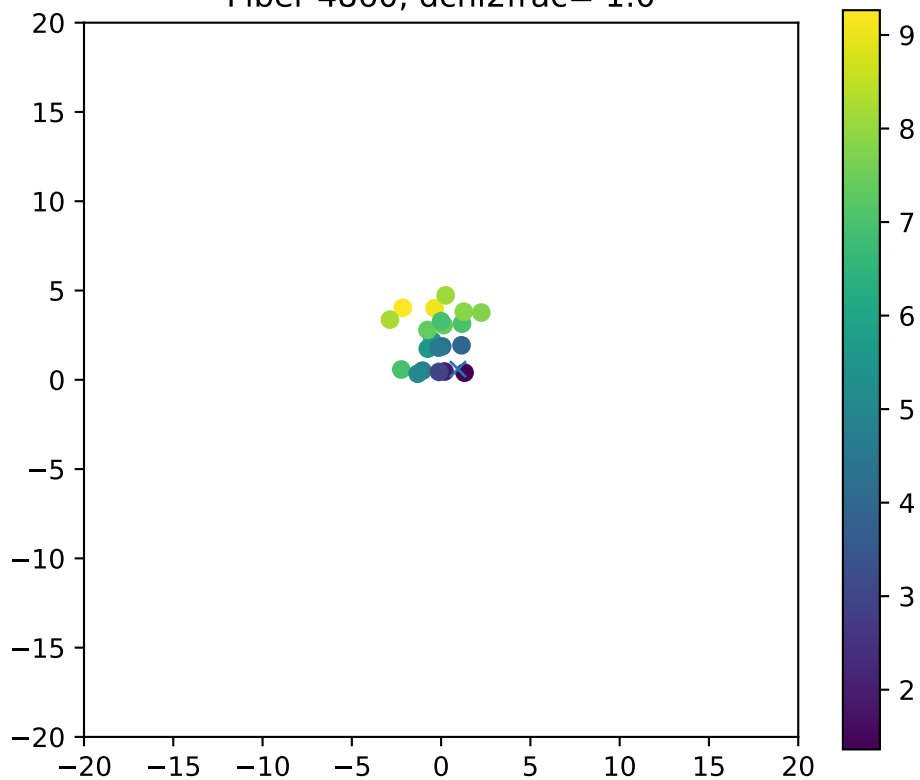
Fiber 4860, dchi2frac= 1.0
