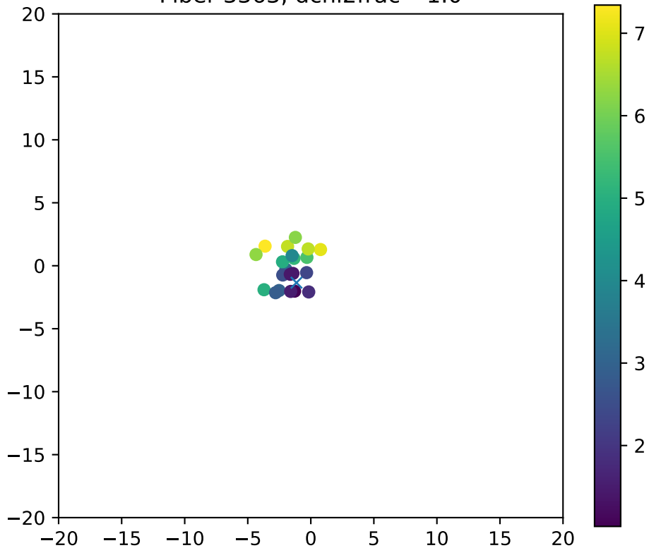
Fiber 3363, dchi2frac= 1.0
