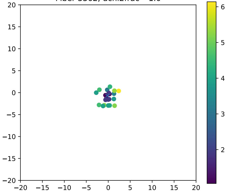
Fiber 3362, dchi2frac= 1.0
