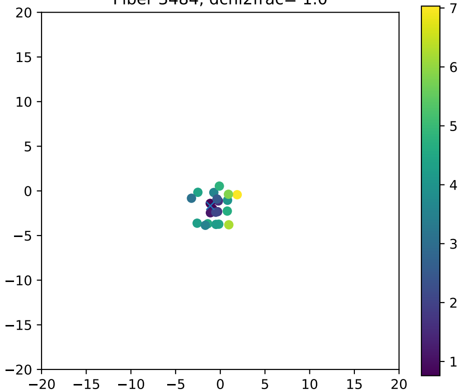
Fiber 3484, dchi2frac= 1.0
