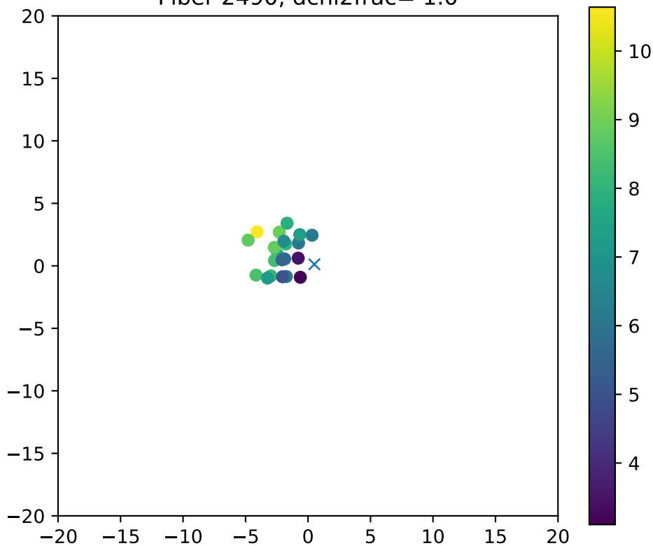
Fiber 2490, dchi2frac= 1.0
