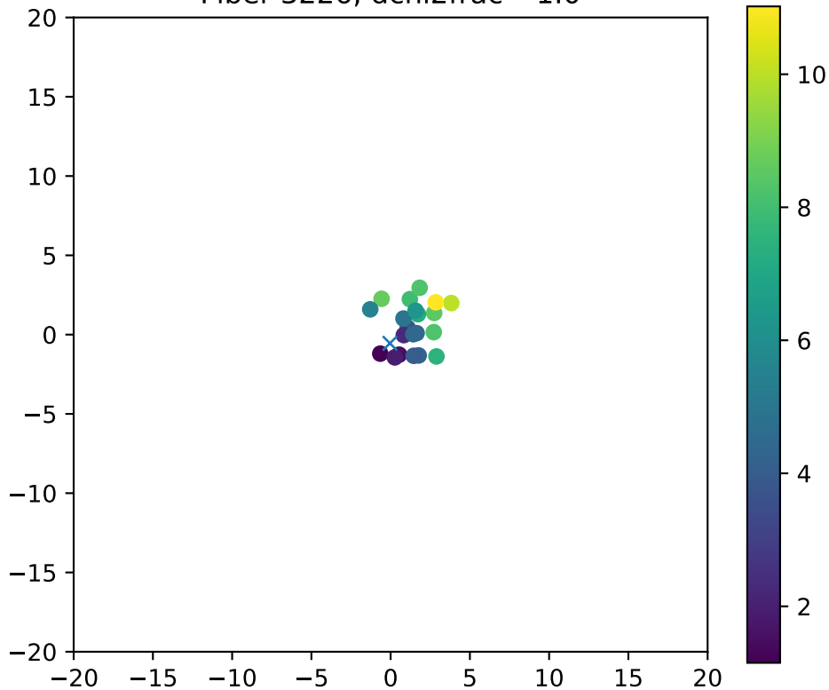
Fiber 3226, dchi2frac= 1.0
