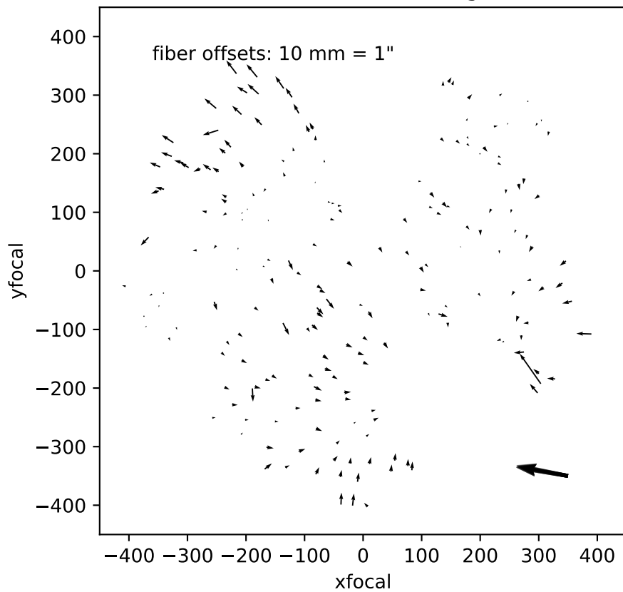
dither20200124-63074-highsnr-R
