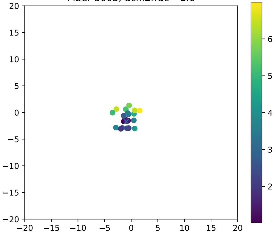
Fiber 3003, dchi2frac= 1.0
