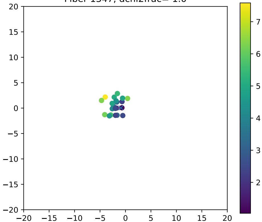
Fiber 1347, dchi2frac= 1.0
