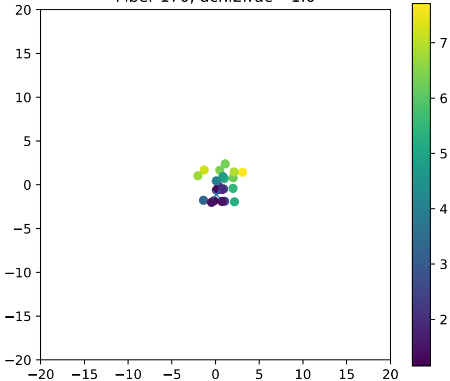
Fiber 170, dchi2frac= 1.0
