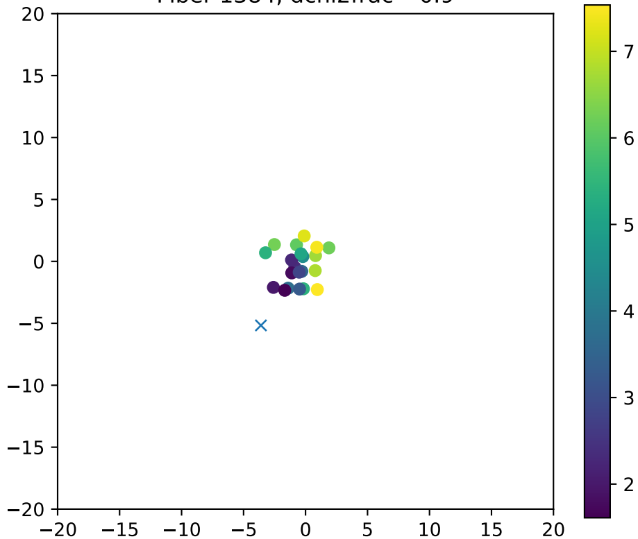
Fiber 1384, dchi2frac= 0.9
