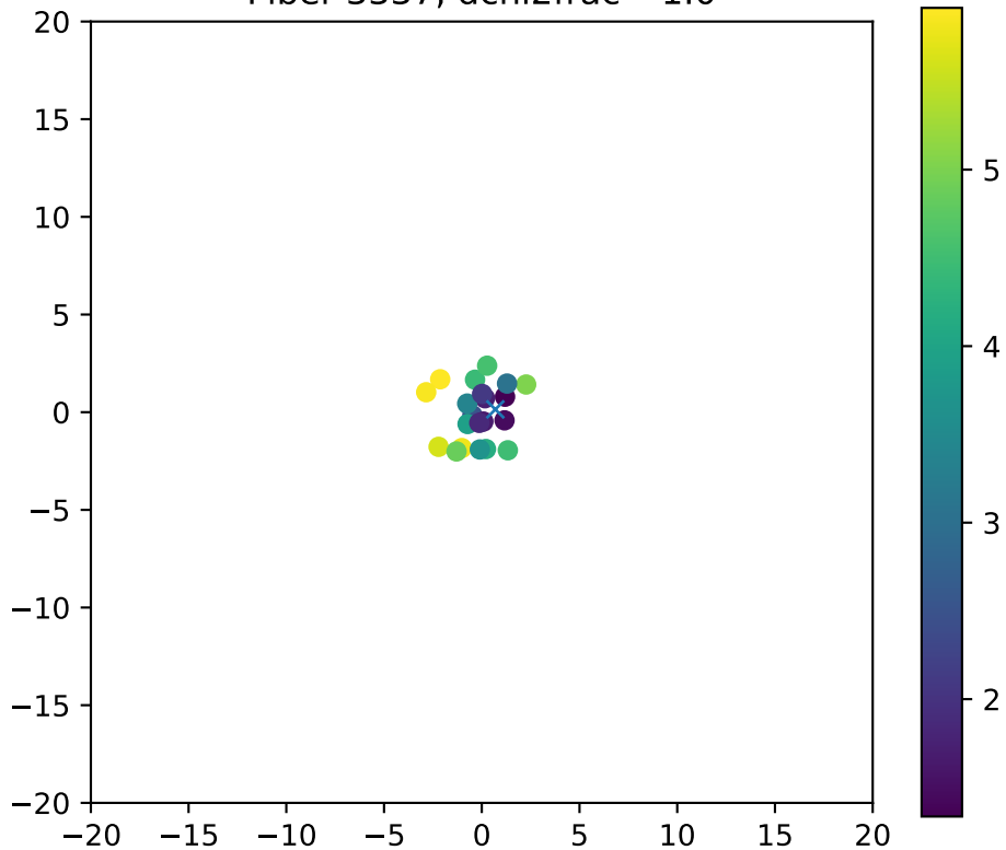
Fiber 3337, dchi2frac= 1.0
