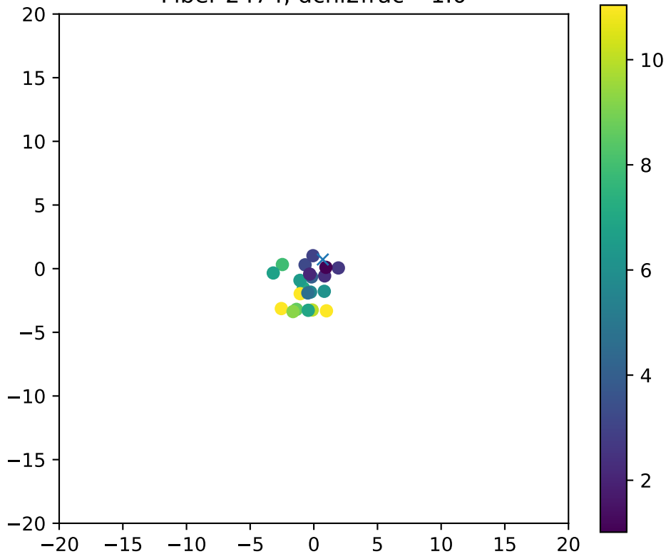
Fiber 2474, dchi2frac= 1.0
