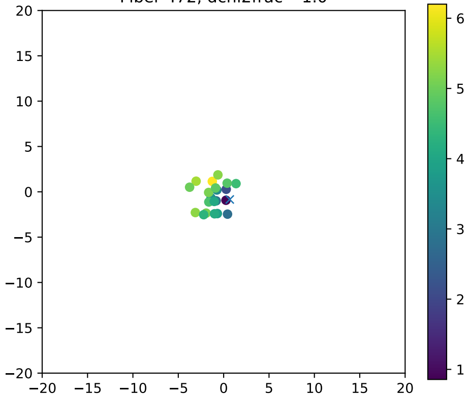
Fiber 472, dchi2frac= 1.0
