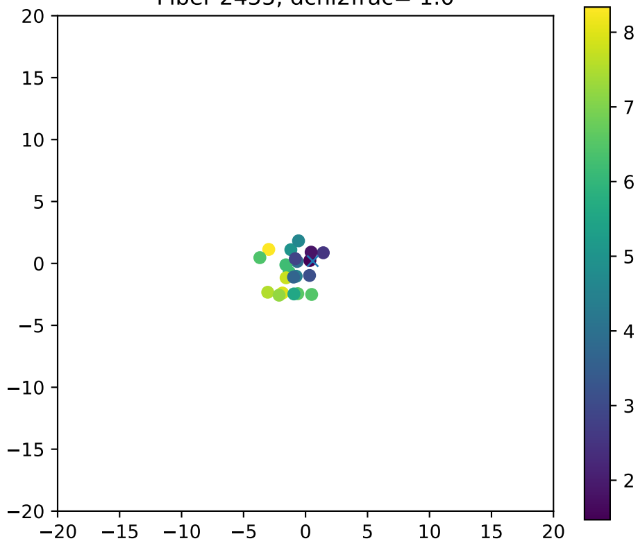
Fiber 2455, dchi2frac= 1.0
