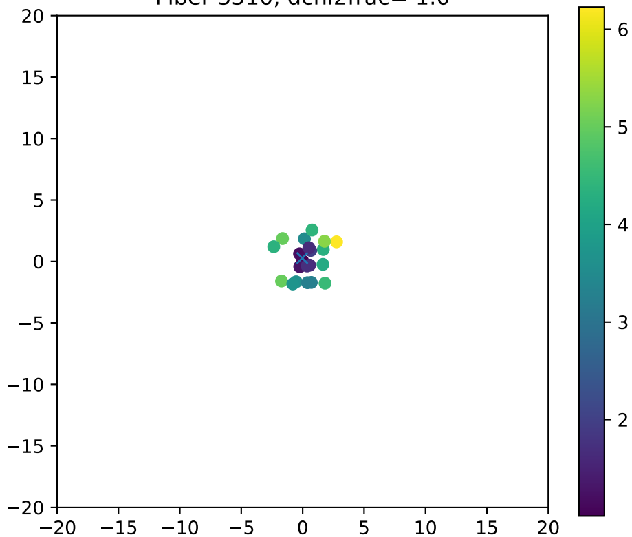
Fiber 3510, dchi2frac= 1.0
