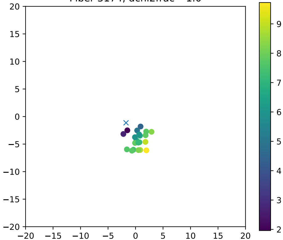
Fiber 3174, dchi2frac= 1.0
