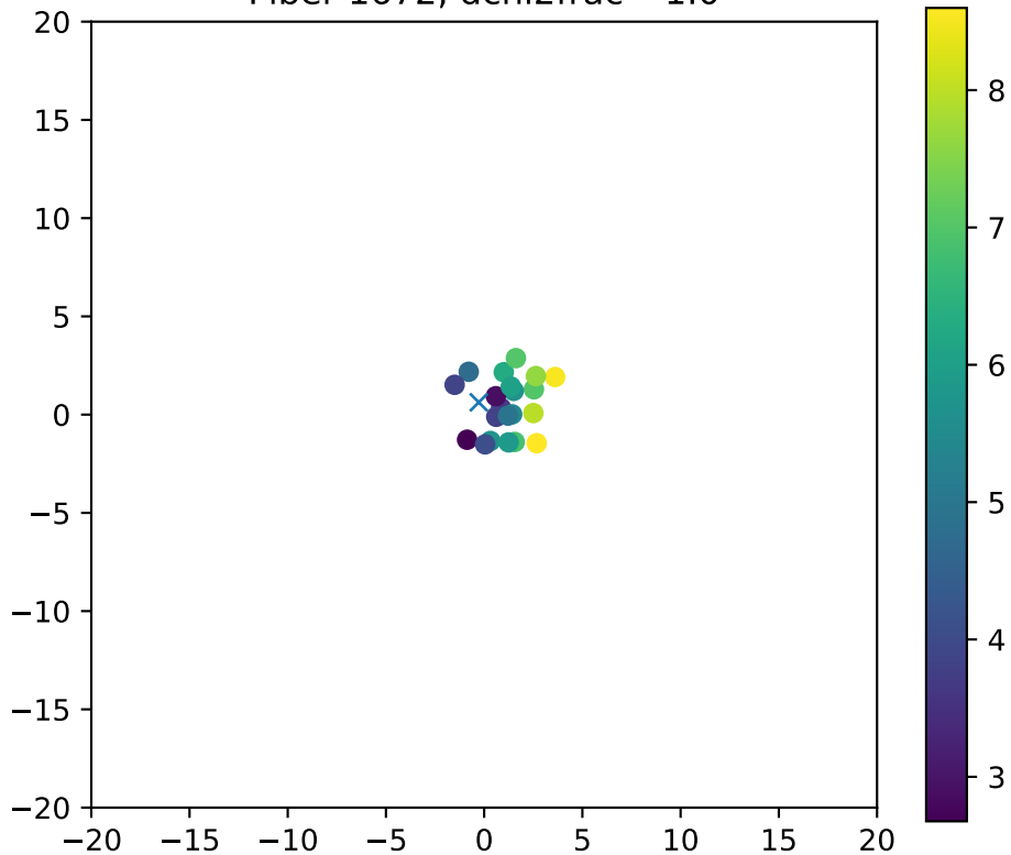
Fiber 1672, dchi2frac= 1.0
