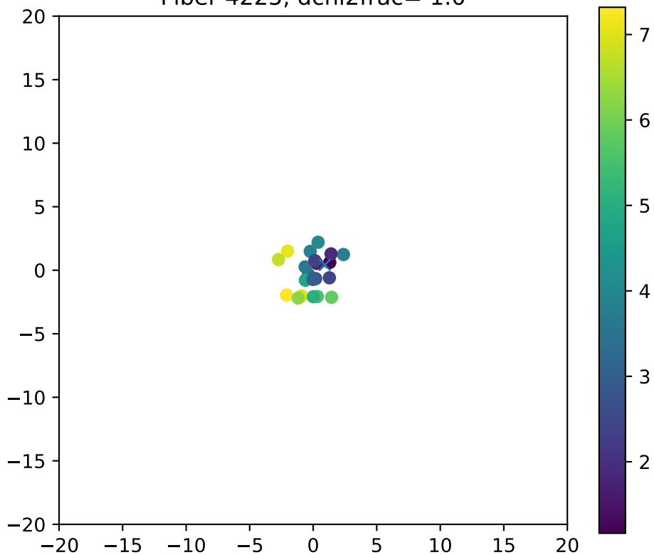
Fiber 4225, dchi2frac= 1.0
