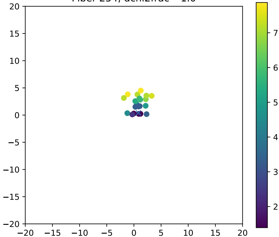
Fiber 254, dchi2frac= 1.0
