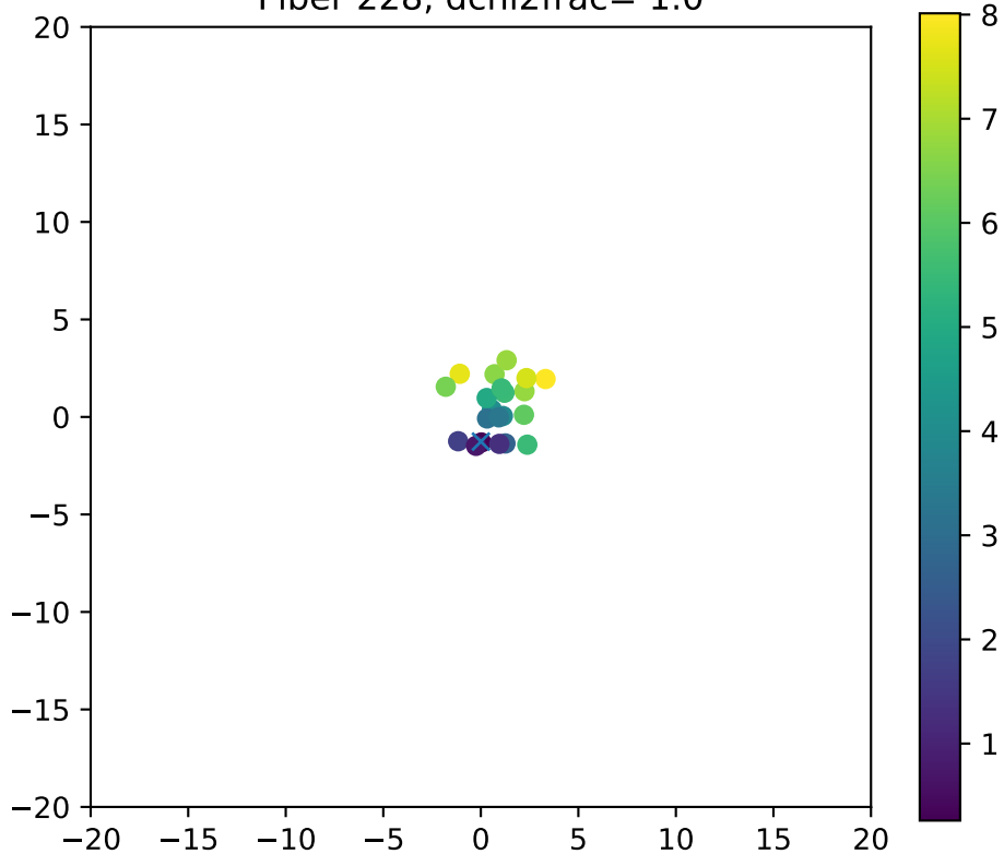
Fiber 228, dchi2frac= 1.0
