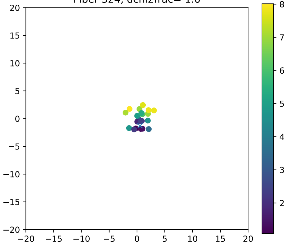
Fiber 324, dchi2frac= 1.0
