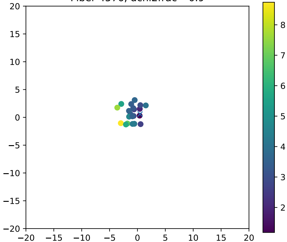
Fiber 4576, dchi2frac= 0.9
