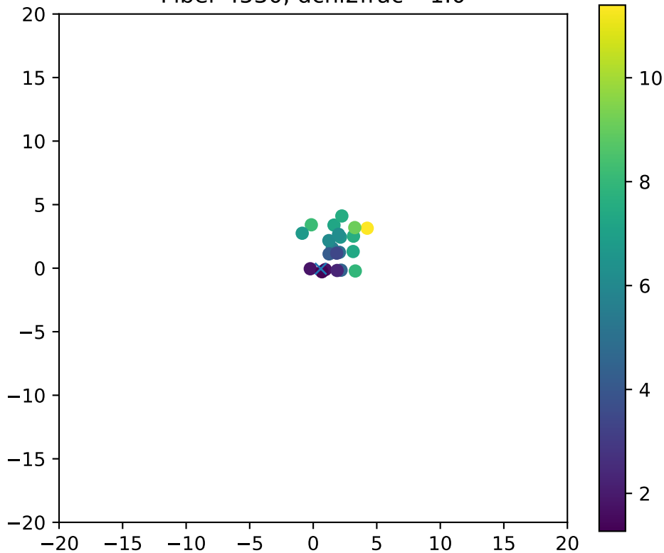
Fiber 4530, dchi2frac= 1.0
