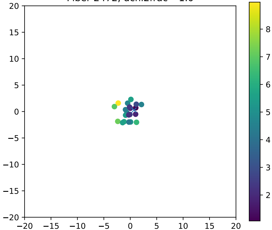
Fiber 2472, dchi2frac= 1.0
