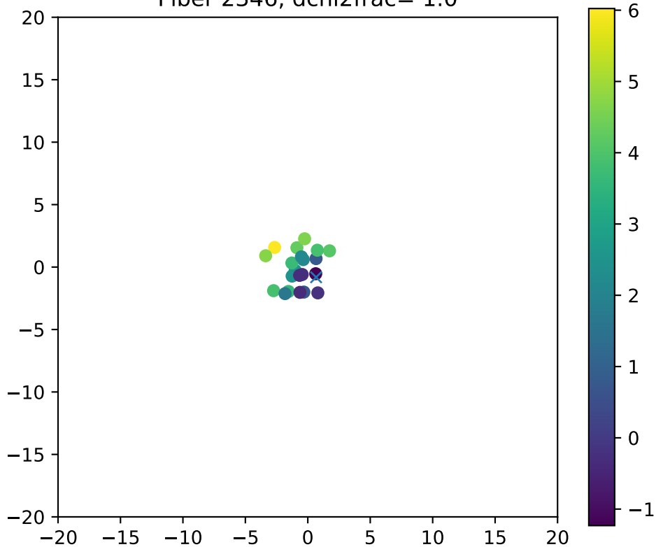
Fiber 2346, dchi2frac= 1.0
