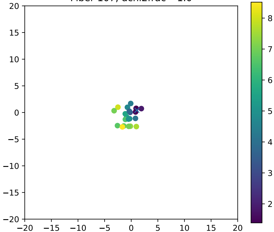
Fiber 107, dchi2frac= 1.0
