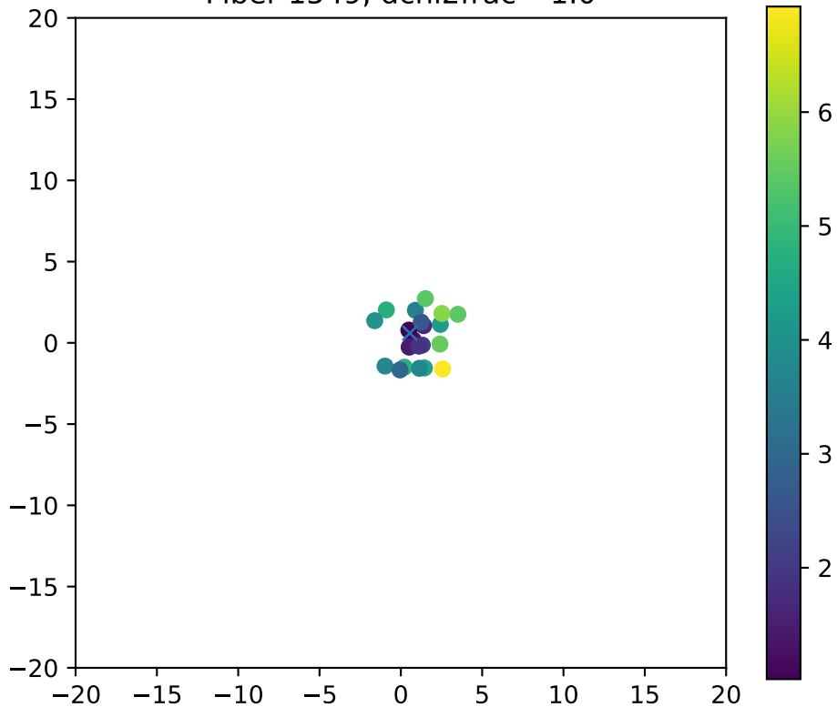
Fiber 1549, dchi2frac= 1.0
