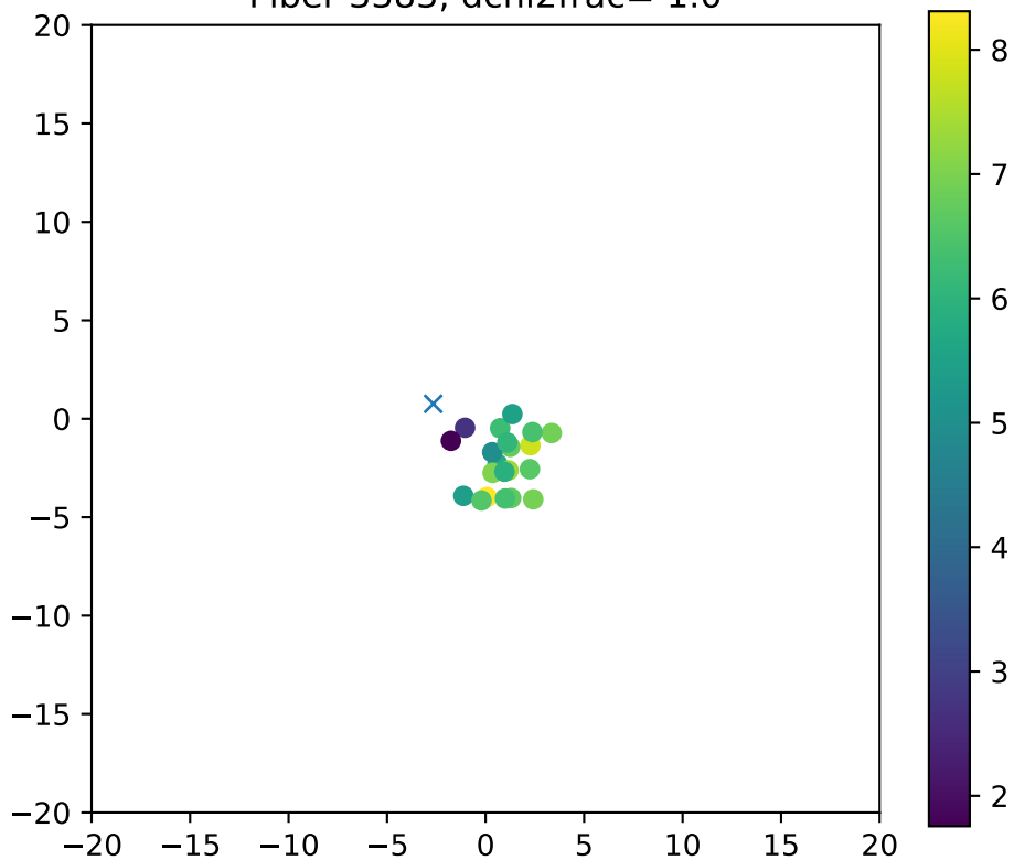
Fiber 3383, dchi2frac= 1.0
