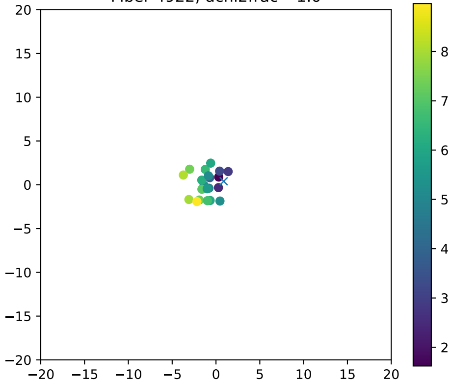
Fiber 4922, dchi2frac= 1.0
