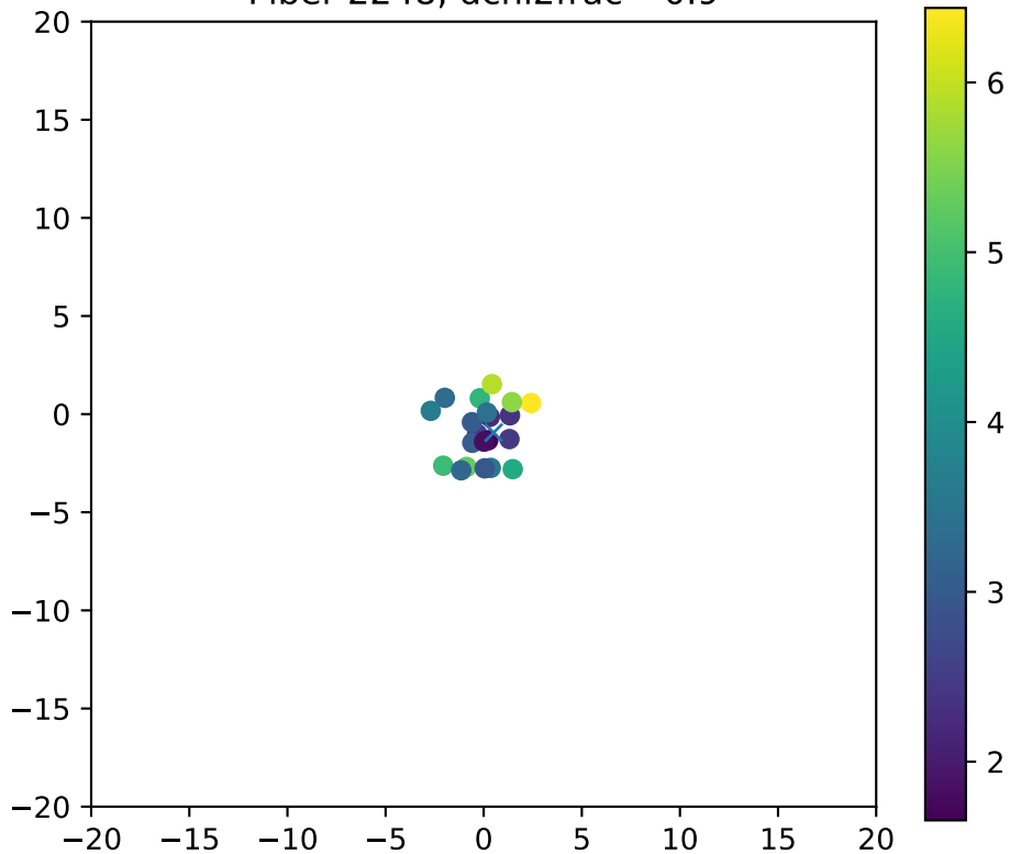
Fiber 2248, dchi2frac= 0.9
