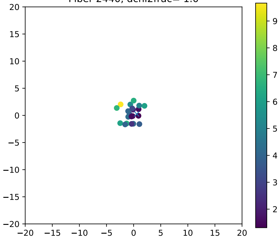
Fiber 2440, dchi2frac= 1.0
