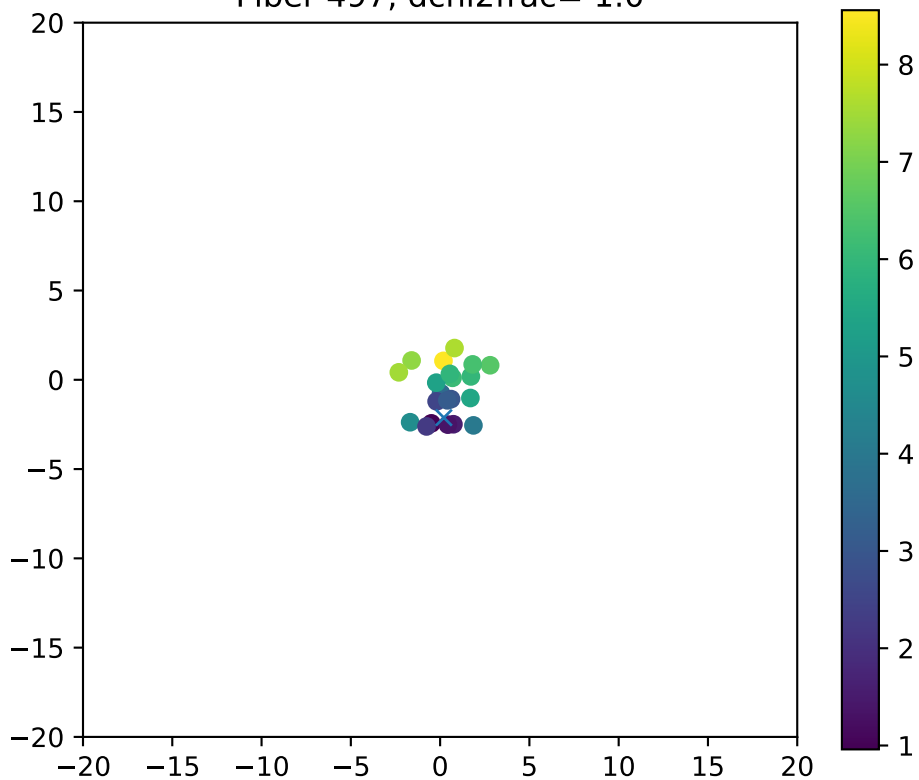
Fiber 497, dchi2frac= 1.0
