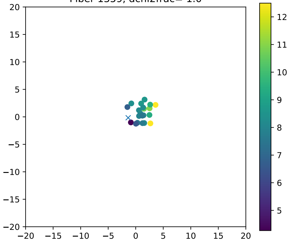
Fiber 1359, dchi2frac= 1.0
