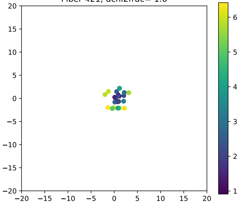
Fiber 421, dchi2frac= 1.0
