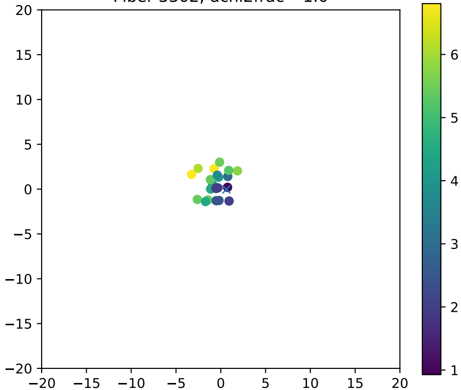
Fiber 3302, dchi2frac= 1.0
