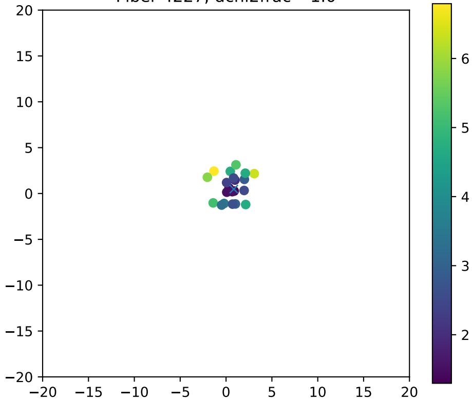
Fiber 4227, dchi2frac= 1.0
