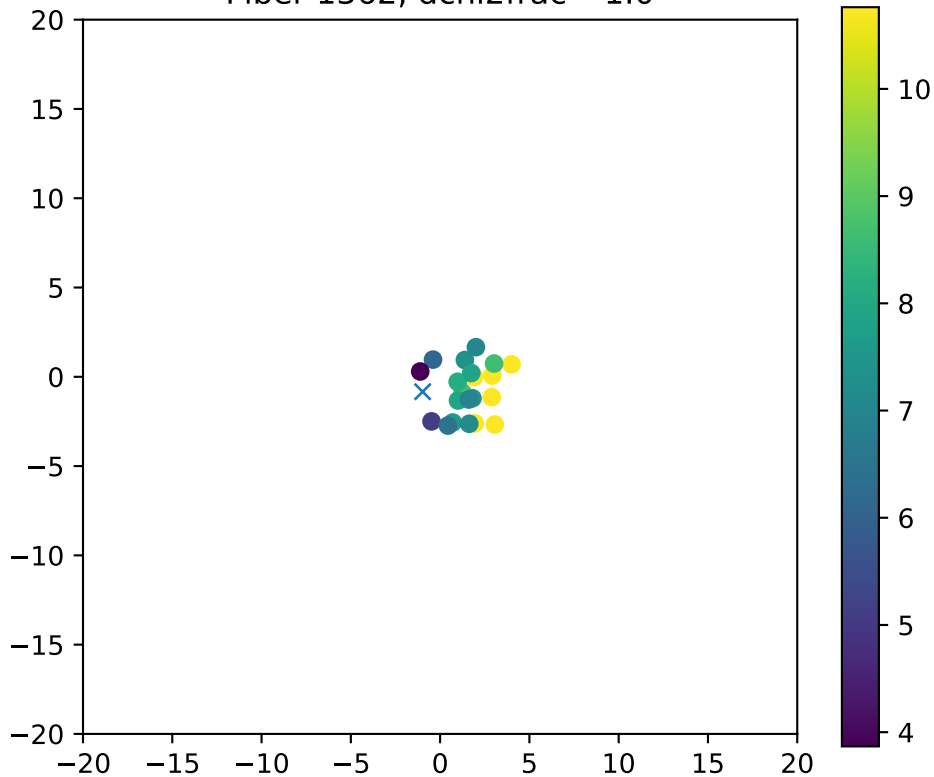
Fiber 1362, dchi2frac= 1.0
