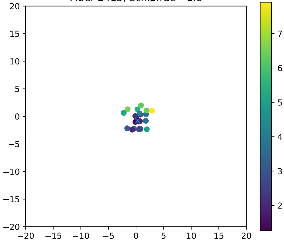
Fiber 2415, dchi2frac= 1.0
