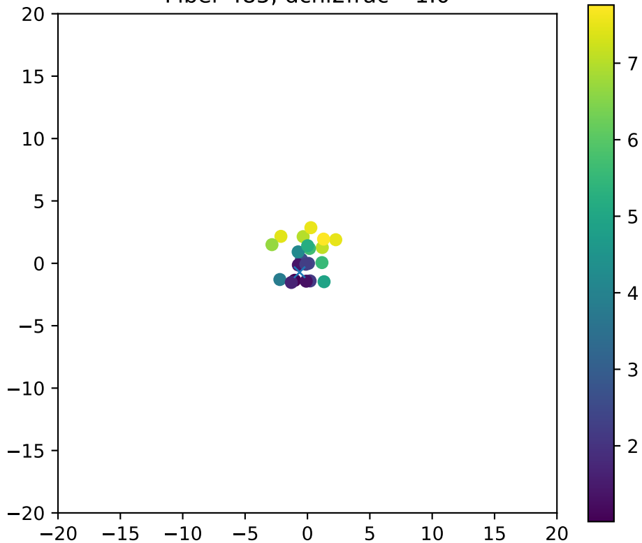
Fiber 485, dchi2frac= 1.0
