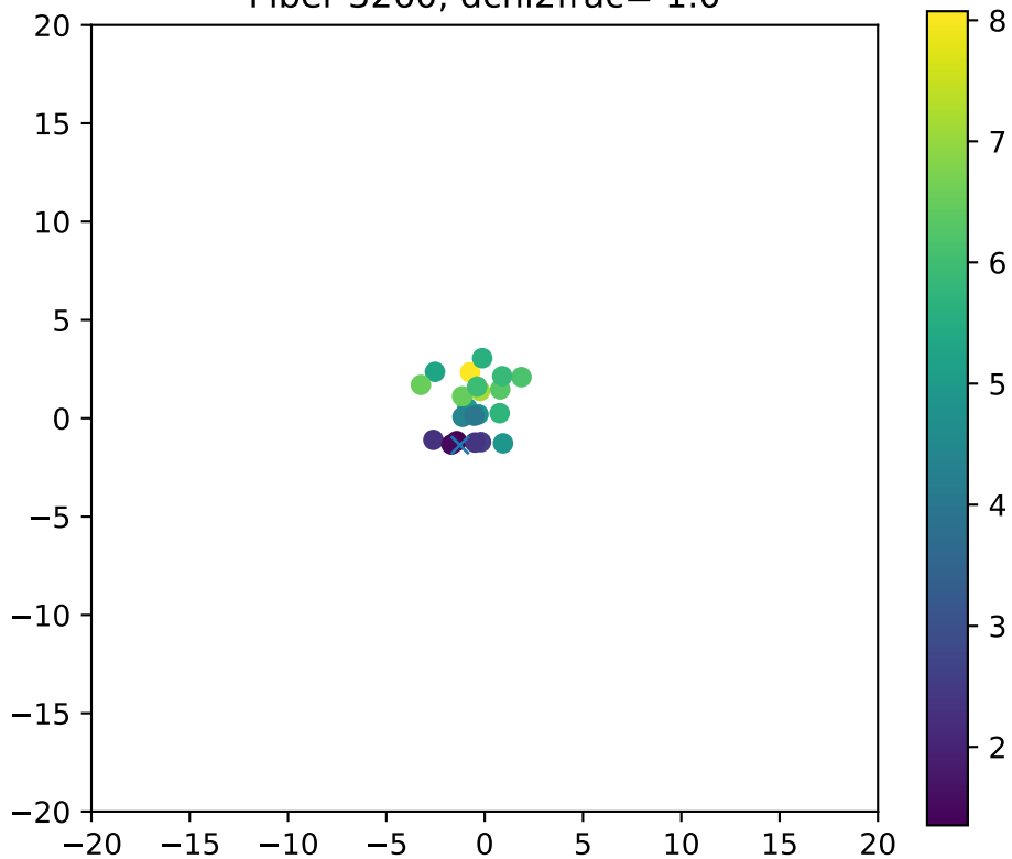
Fiber 3260, dchi2frac= 1.0
