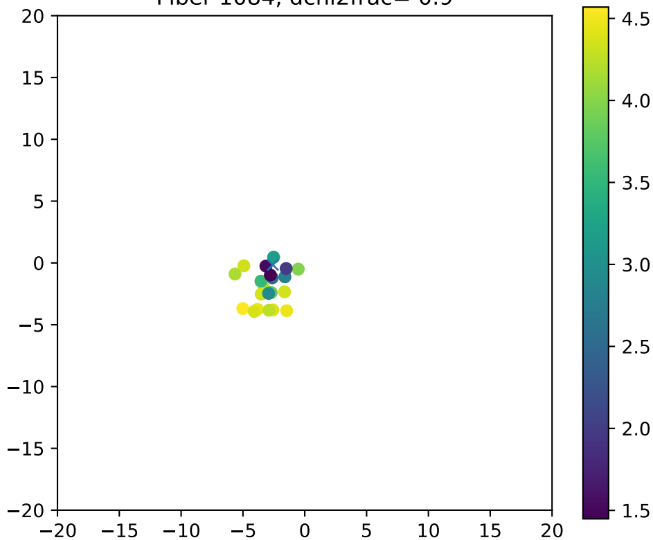
Fiber 1084, dchi2frac= 0.9
