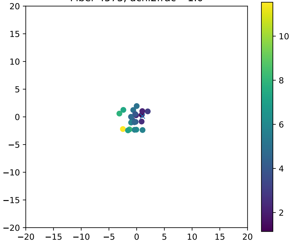
Fiber 4573, dchi2frac= 1.0
