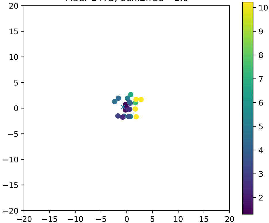
Fiber 1473, dchi2frac= 1.0
