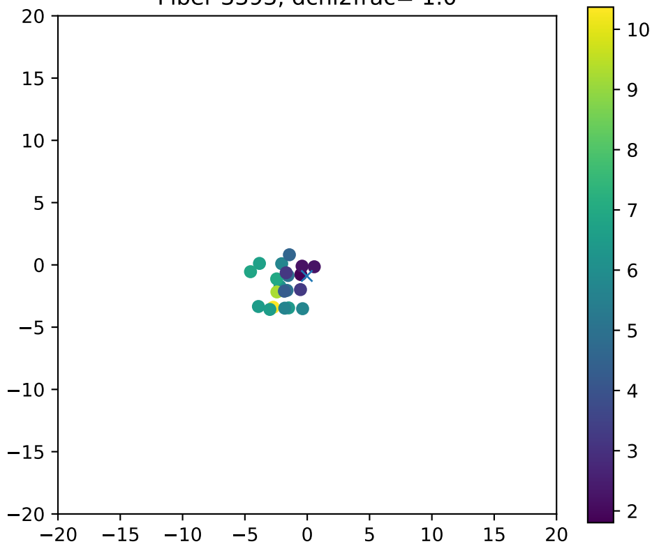
Fiber 3393, dchi2frac= 1.0
