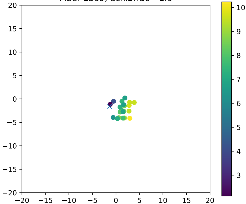
Fiber 1369, dchi2frac= 1.0
