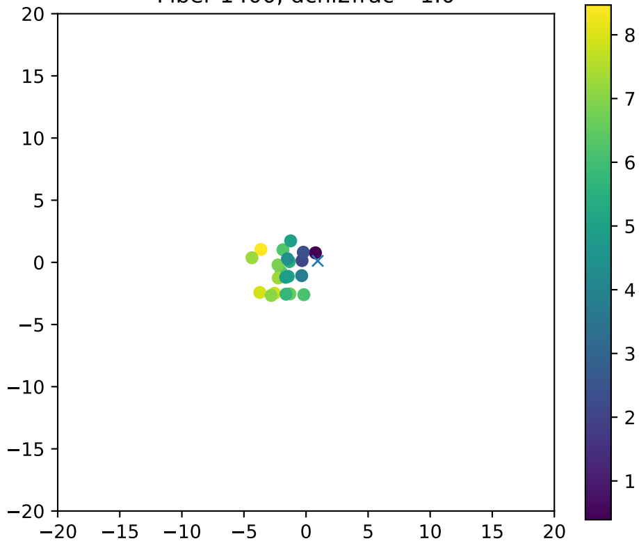
Fiber 1400, dchi2frac= 1.0
