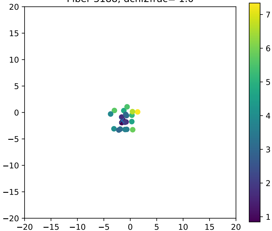
Fiber 3188, dchi2frac= 1.0
