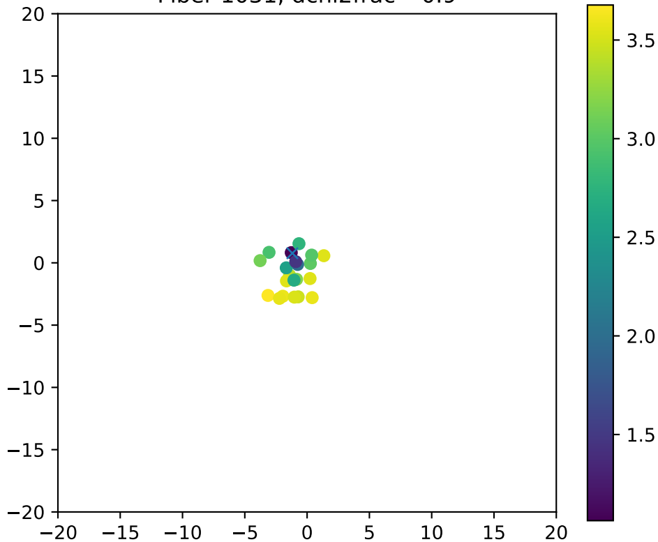
Fiber 1031, dchi2frac= 0.9
