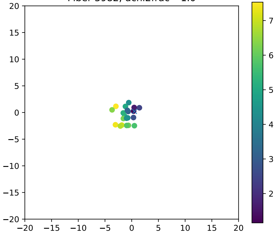
Fiber 3982, dchi2frac= 1.0
