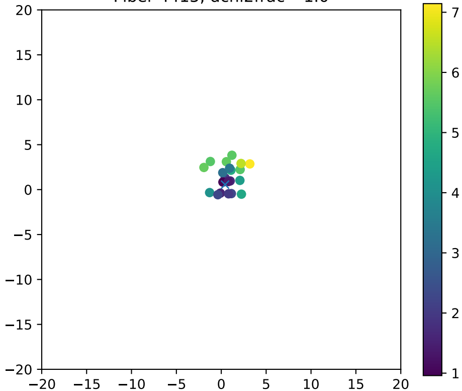
Fiber 4415, dchi2frac= 1.0
