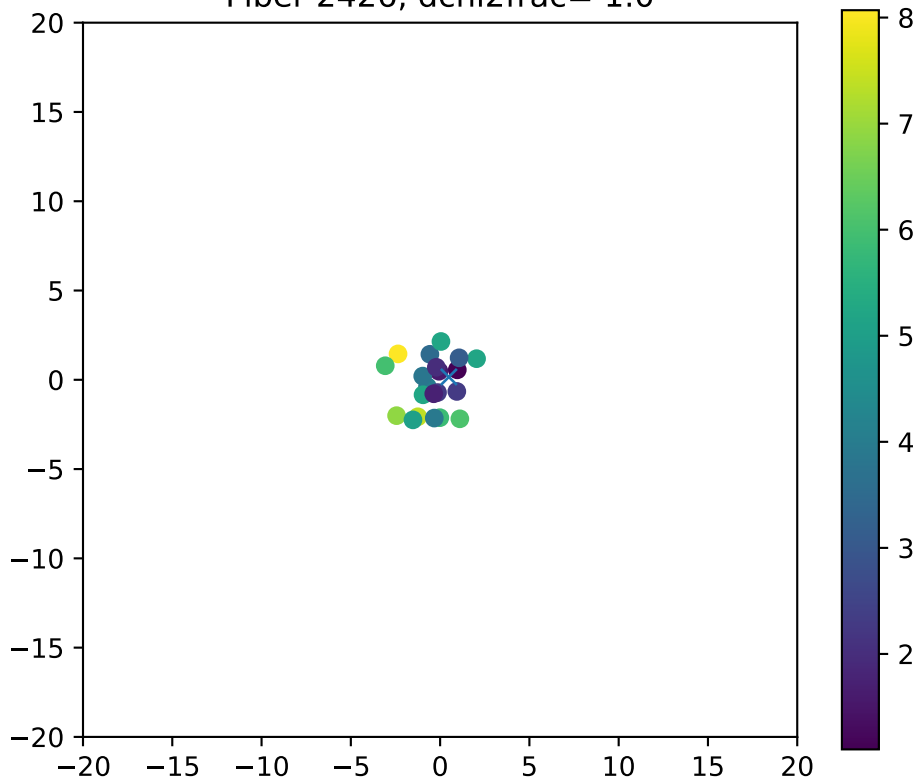
Fiber 2426, dchi2frac= 1.0
