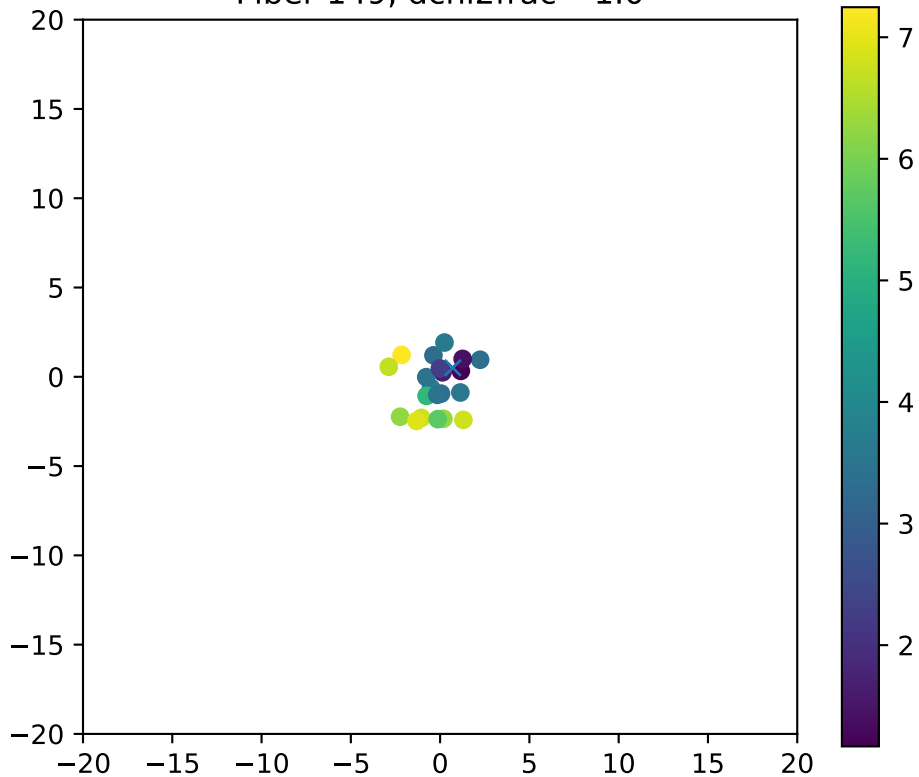
Fiber 149, dchi2frac= 1.0
