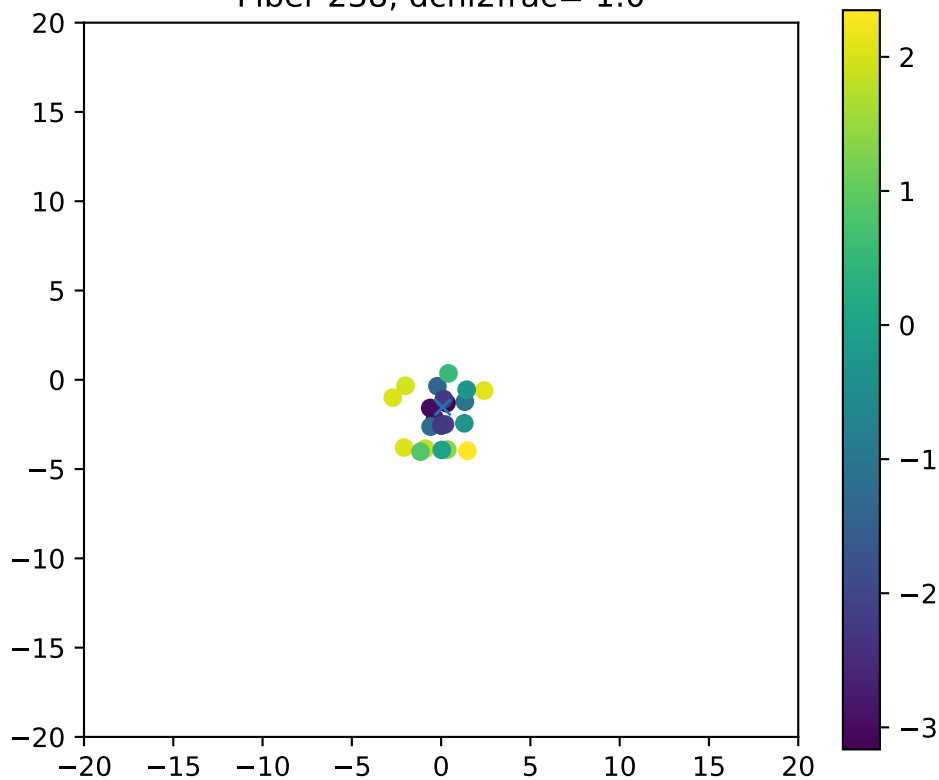
Fiber 238, dchi2frac= 1.0
