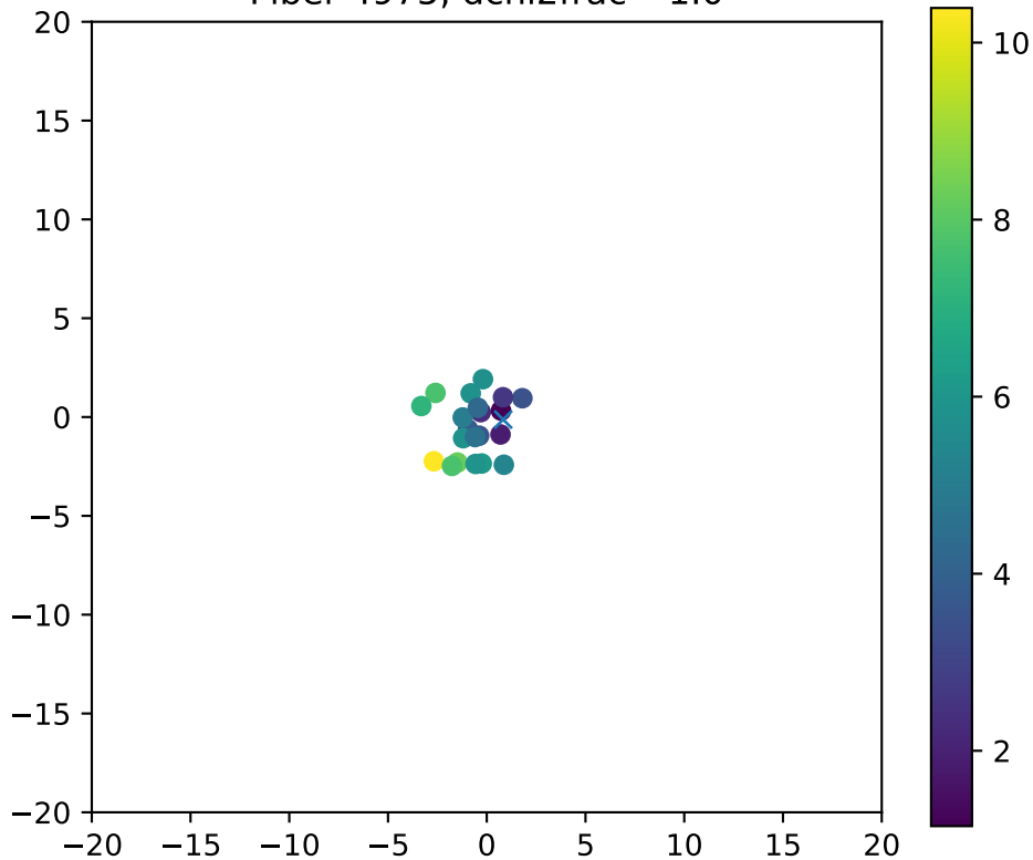
Fiber 4975, dchi2frac= 1.0
