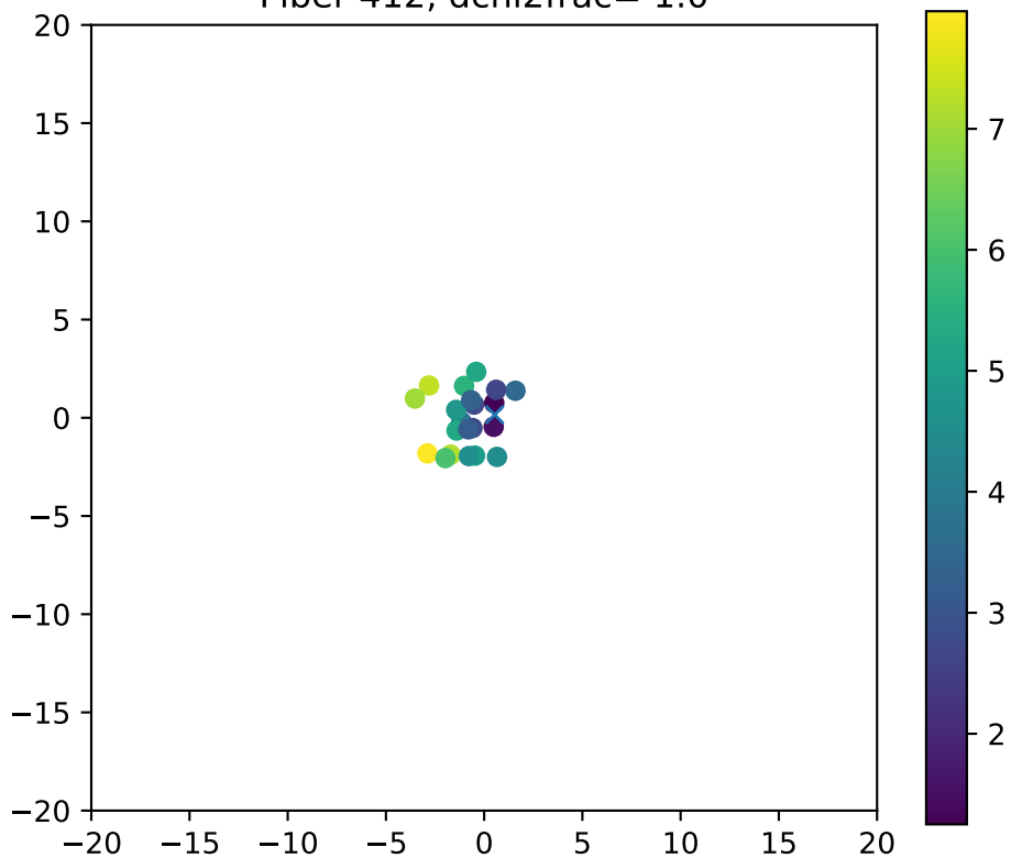
Fiber 412, dchi2frac= 1.0
