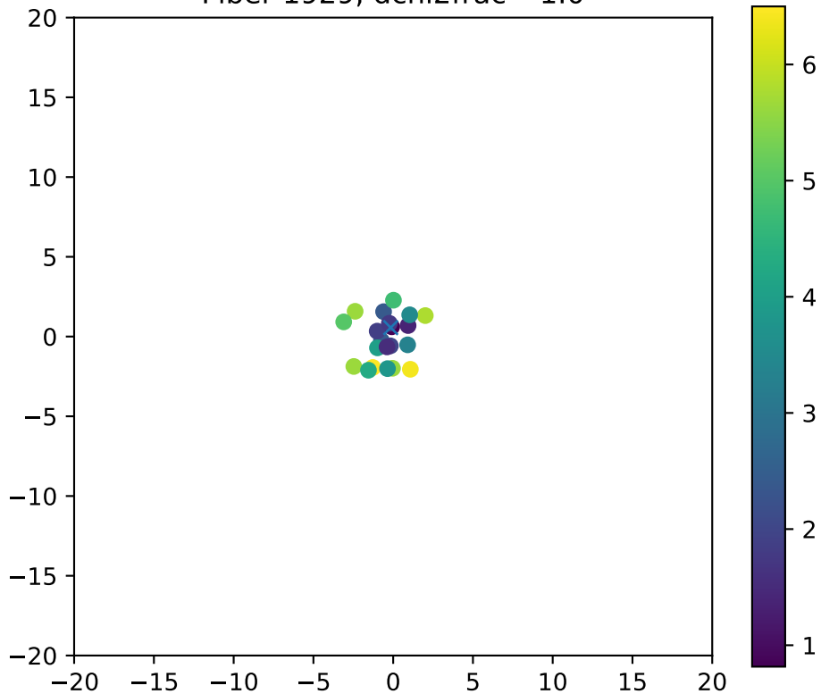
Fiber 1929, dchi2frac= 1.0
