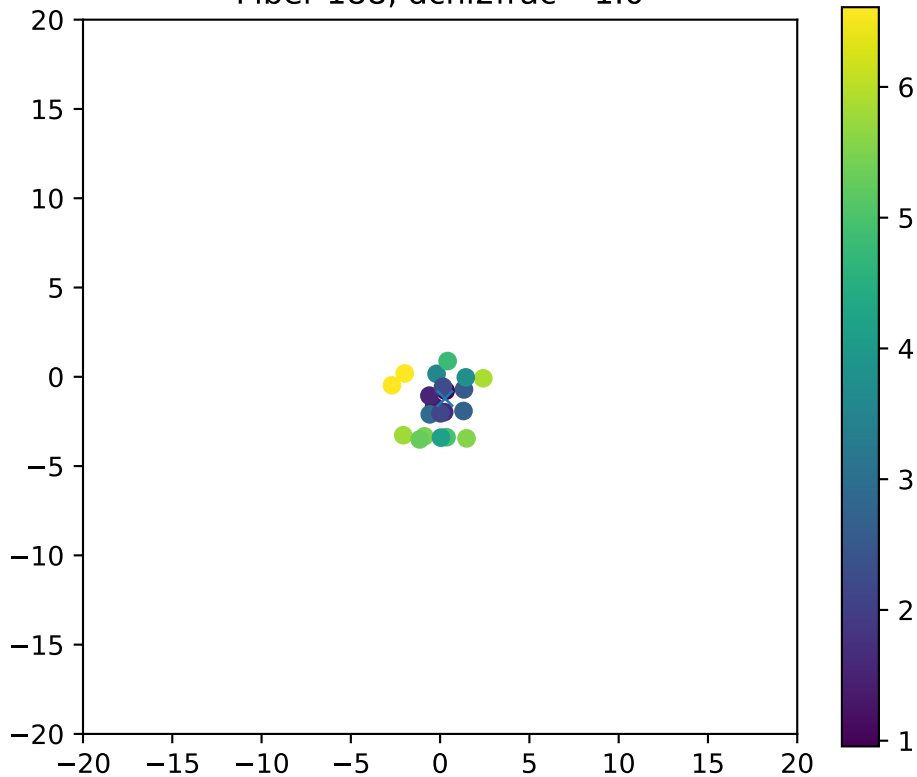
Fiber 188, dchi2frac= 1.0
