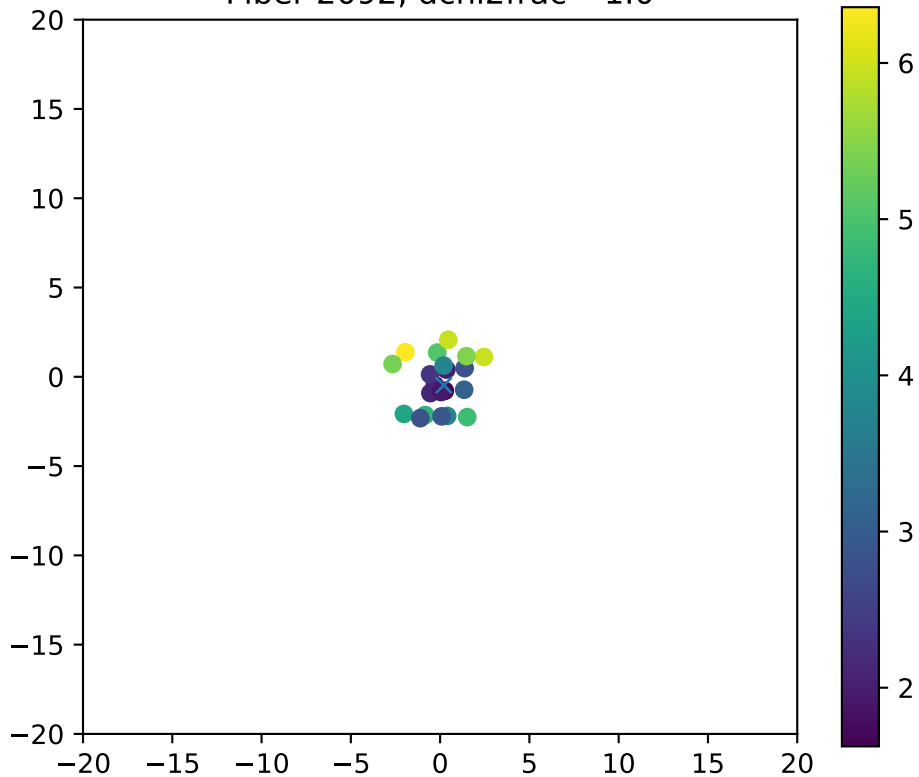
Fiber 2092, dchi2frac= 1.0
