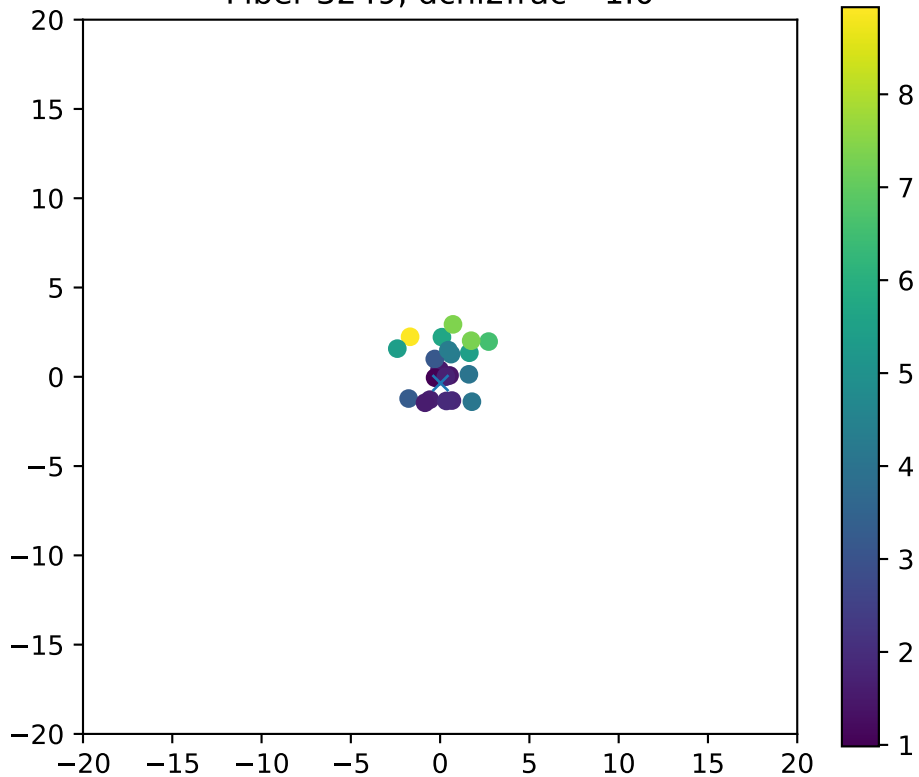
Fiber 3249, dchi2frac= 1.0
