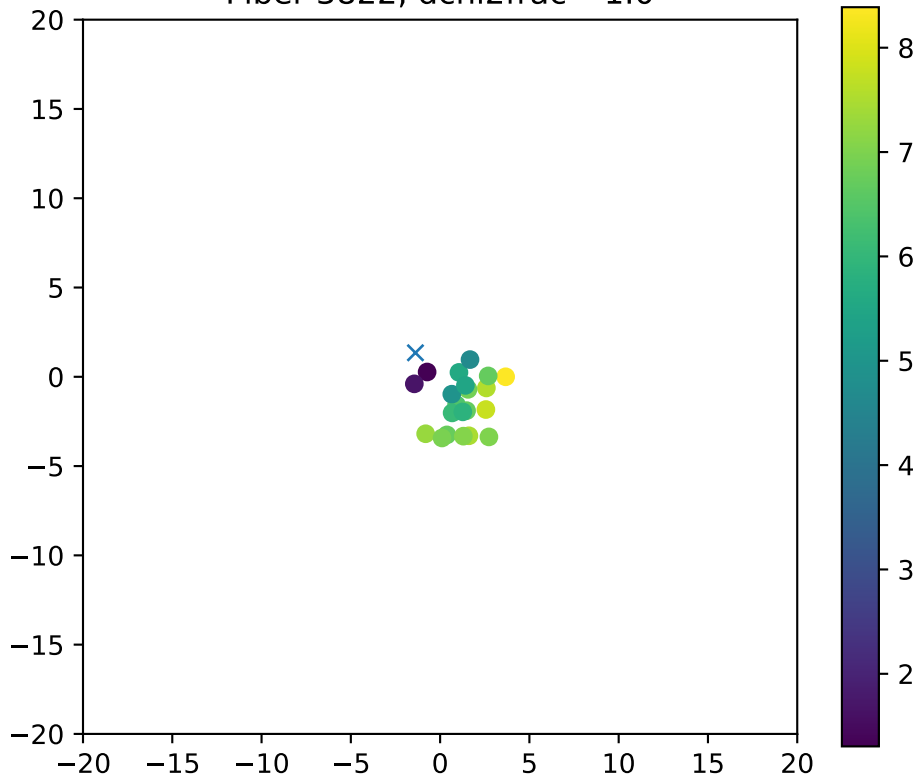
Fiber 3822, dchi2frac= 1.0
