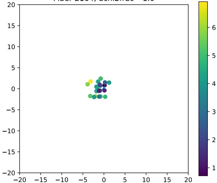
Fiber 2164, dchi2frac= 1.0
