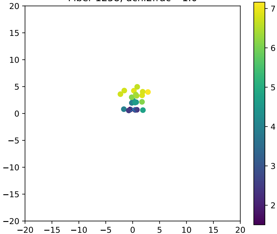
Fiber 1258, dchi2frac= 1.0
