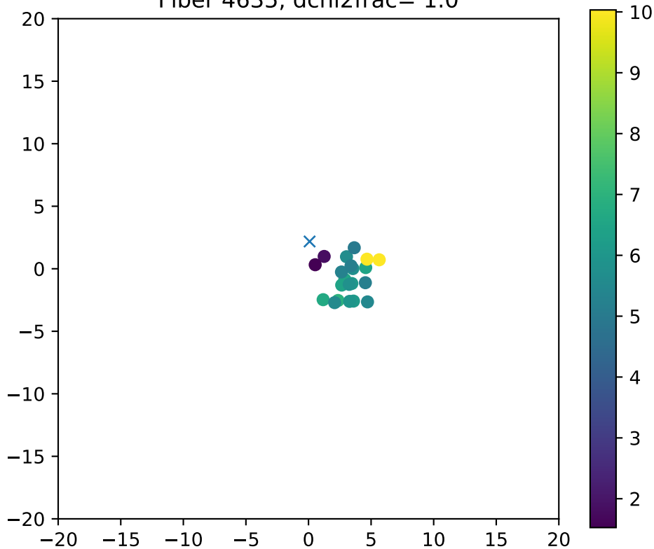
Fiber 4635, dchi2frac= 1.0
