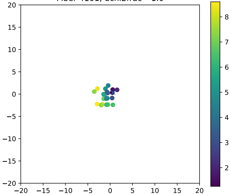
Fiber 4101, dchi2frac= 1.0
