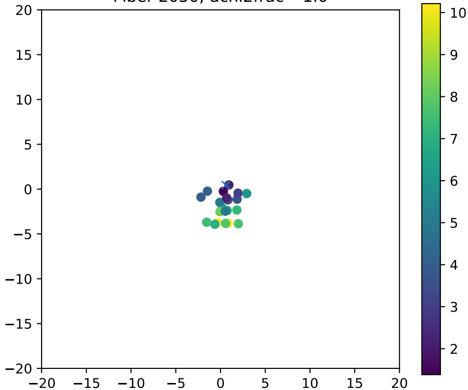
Fiber 2050, dchi2frac= 1.0
