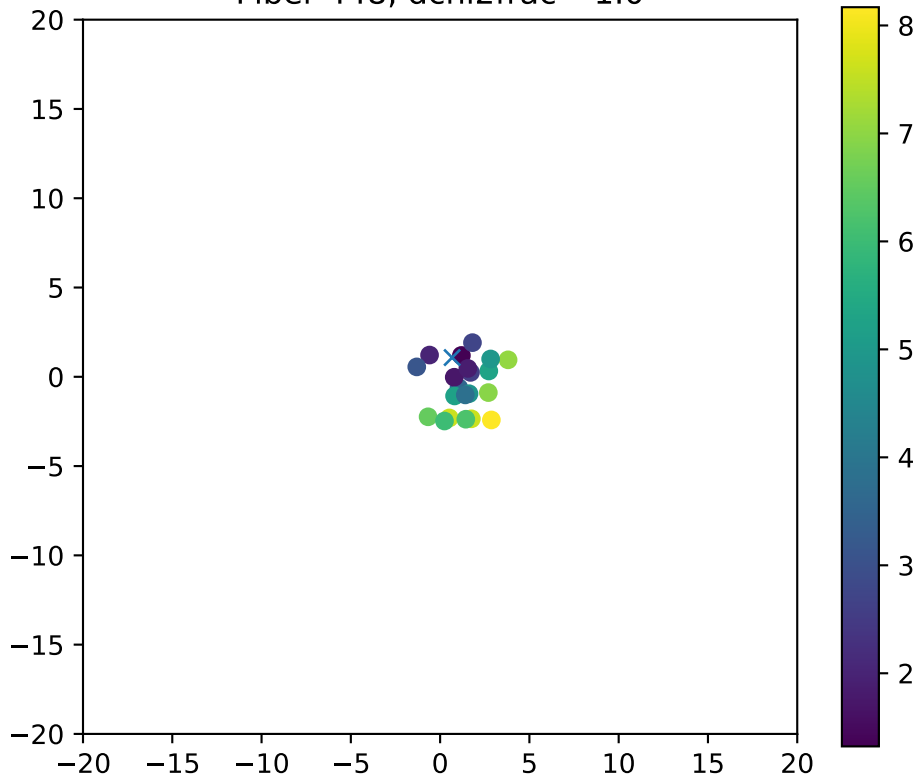
Fiber 448, dchi2frac= 1.0
