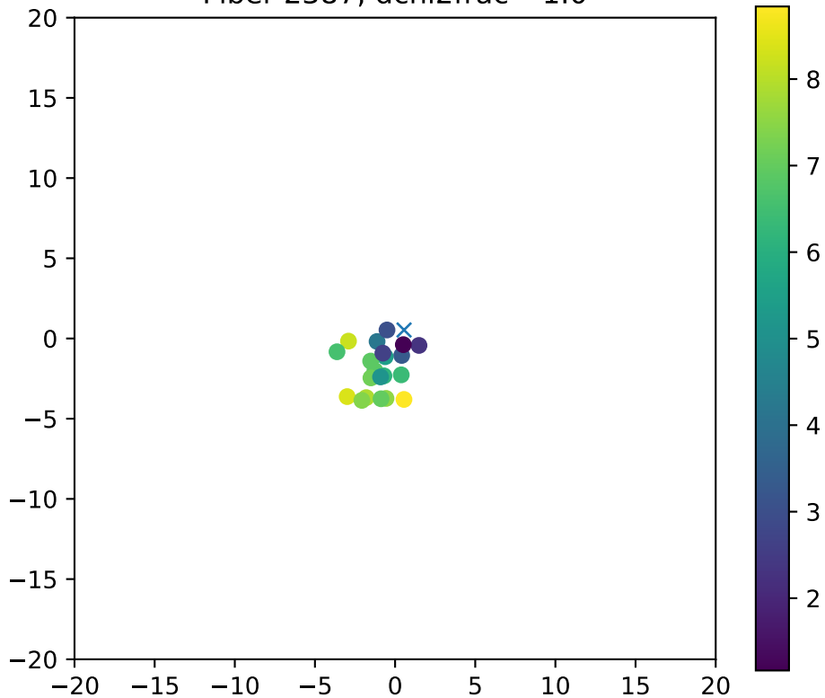
Fiber 2387, dchi2frac= 1.0
