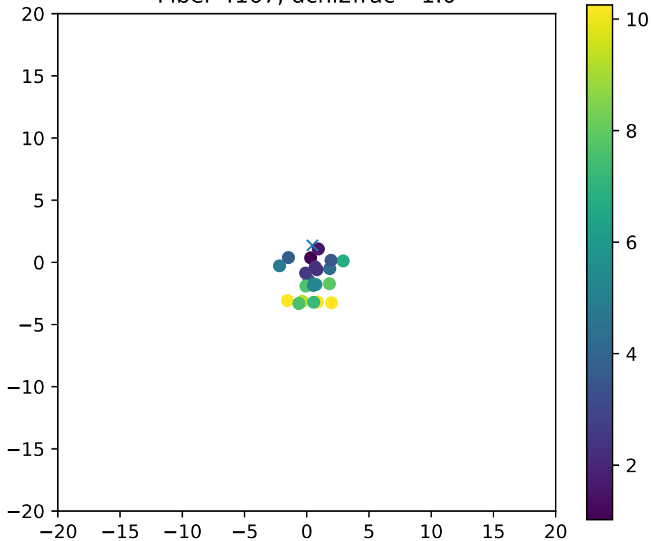
Fiber 4167, dchi2frac= 1.0
