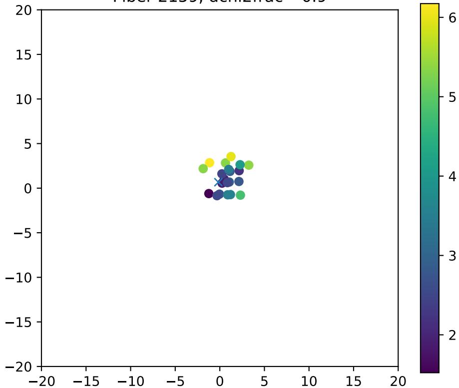
Fiber 2159, dchi2frac= 0.9
