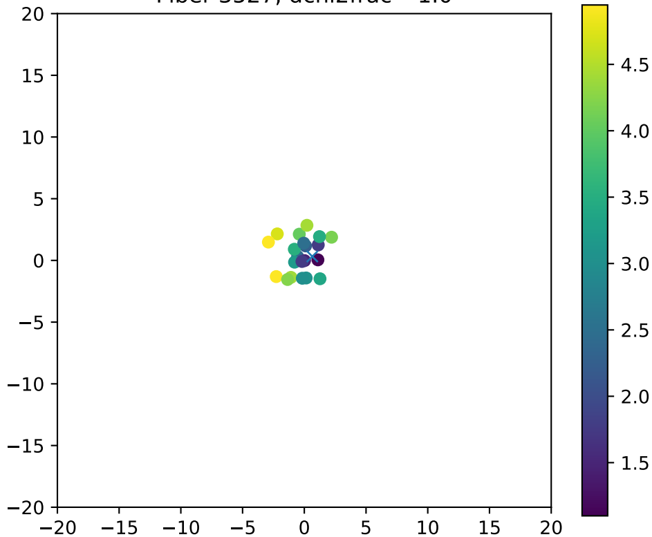
Fiber 3527, dchi2frac= 1.0
