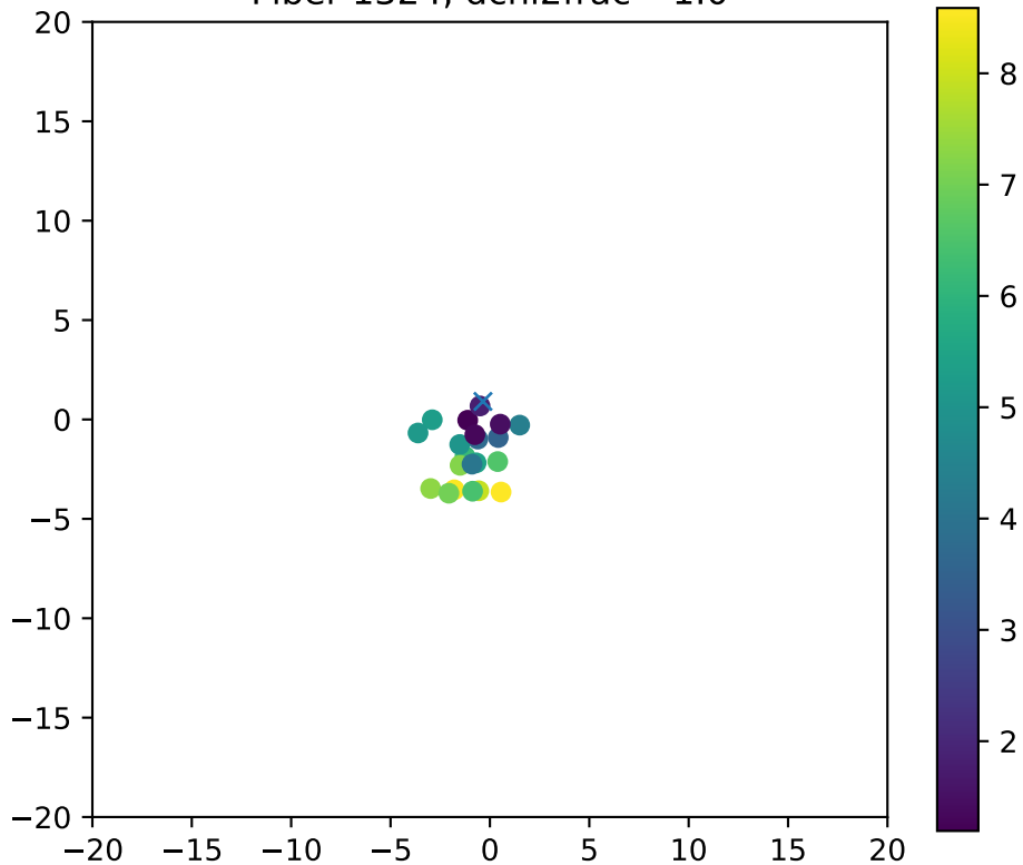
Fiber 1324, dchi2frac= 1.0
