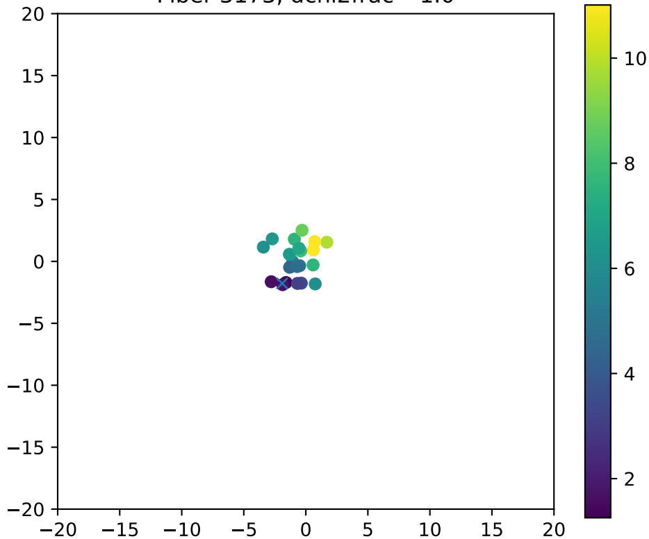
Fiber 3173, dchi2frac= 1.0
