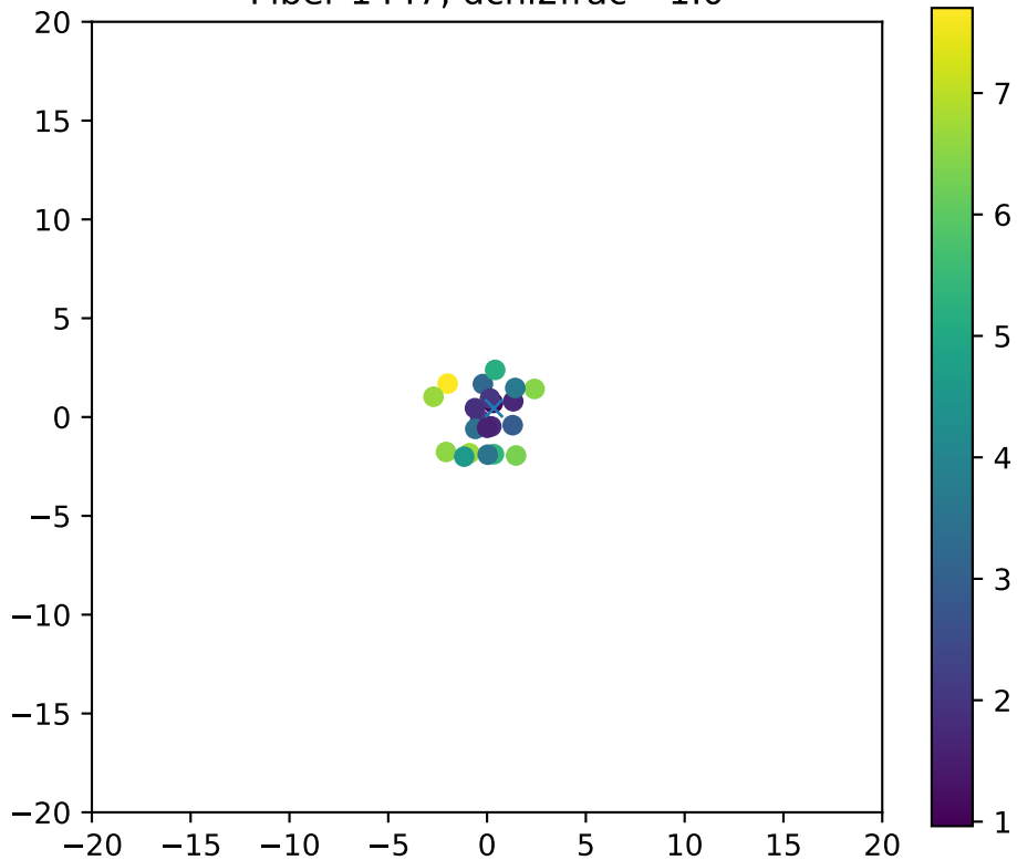
Fiber 1447, dchi2frac= 1.0
