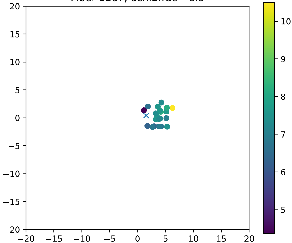
Fiber 1267, dchi2frac= 0.9
