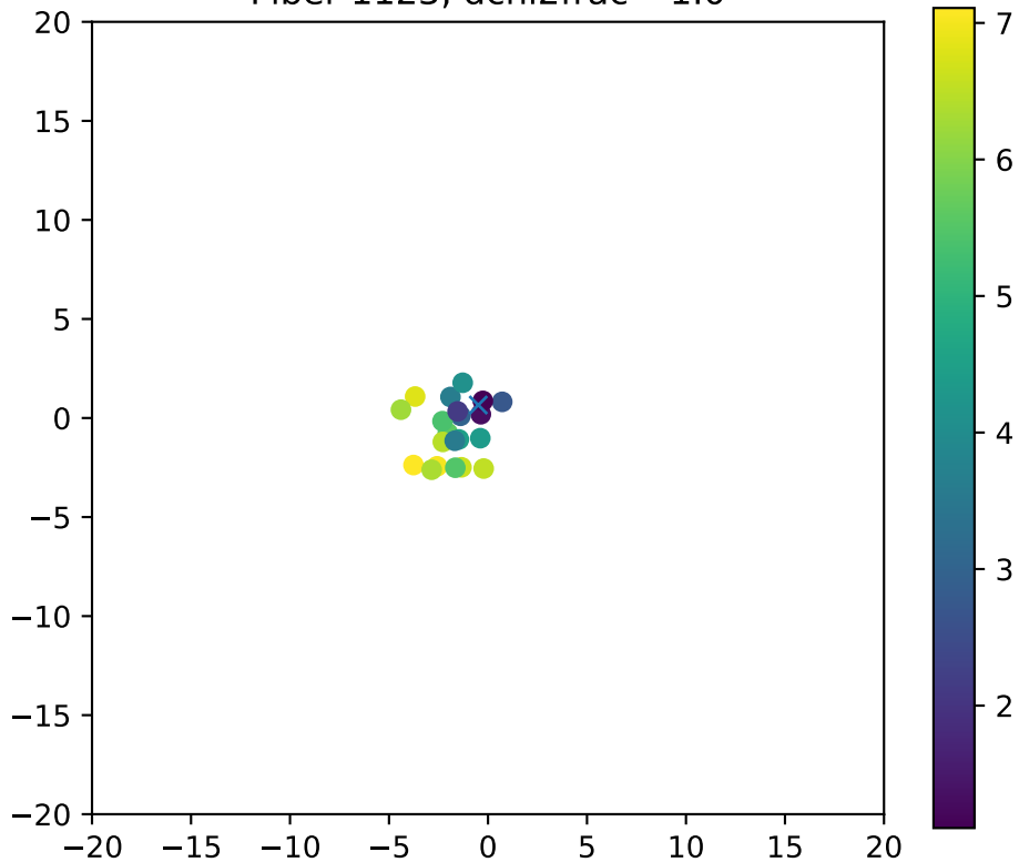
Fiber 1123, dchi2frac= 1.0
