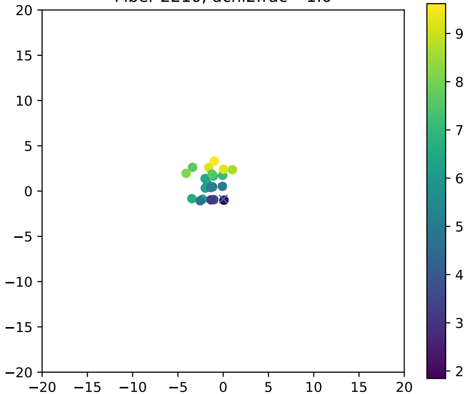
Fiber 2210, dchi2frac= 1.0
