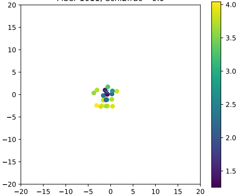
Fiber 1011, dchi2frac= 0.9
