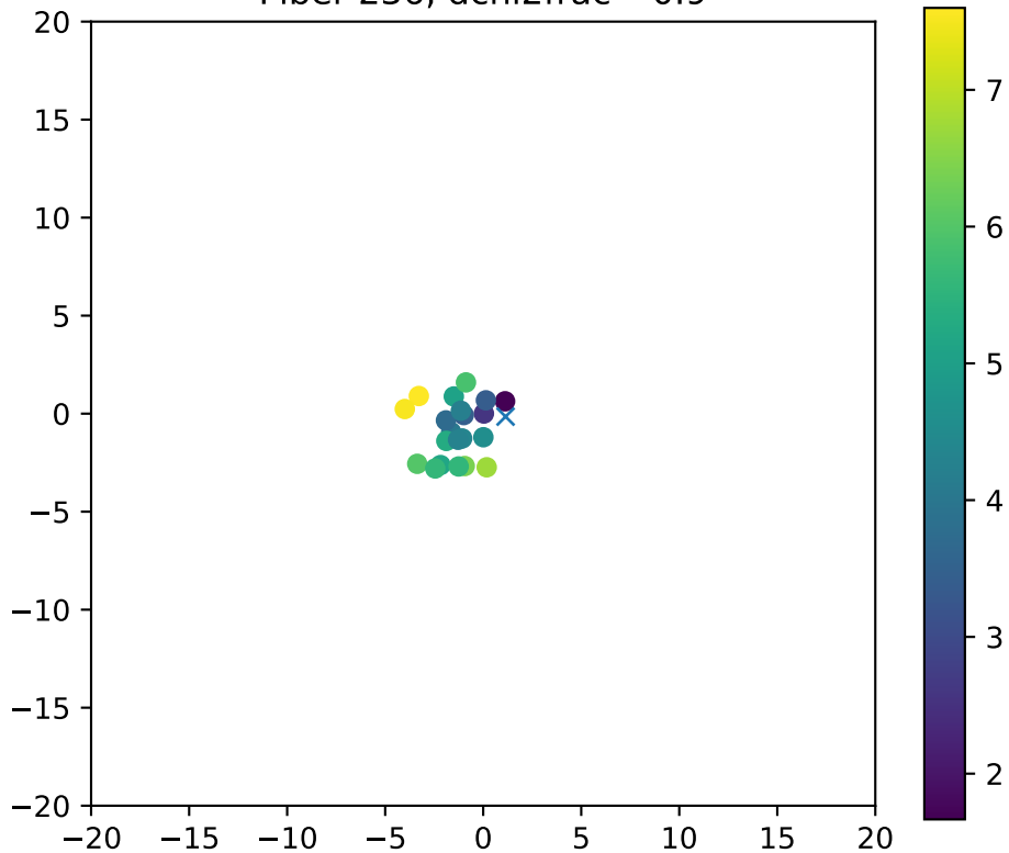
Fiber 236, dchi2frac= 0.9
