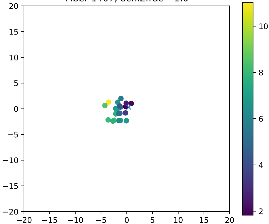
Fiber 1407, dchi2frac= 1.0
