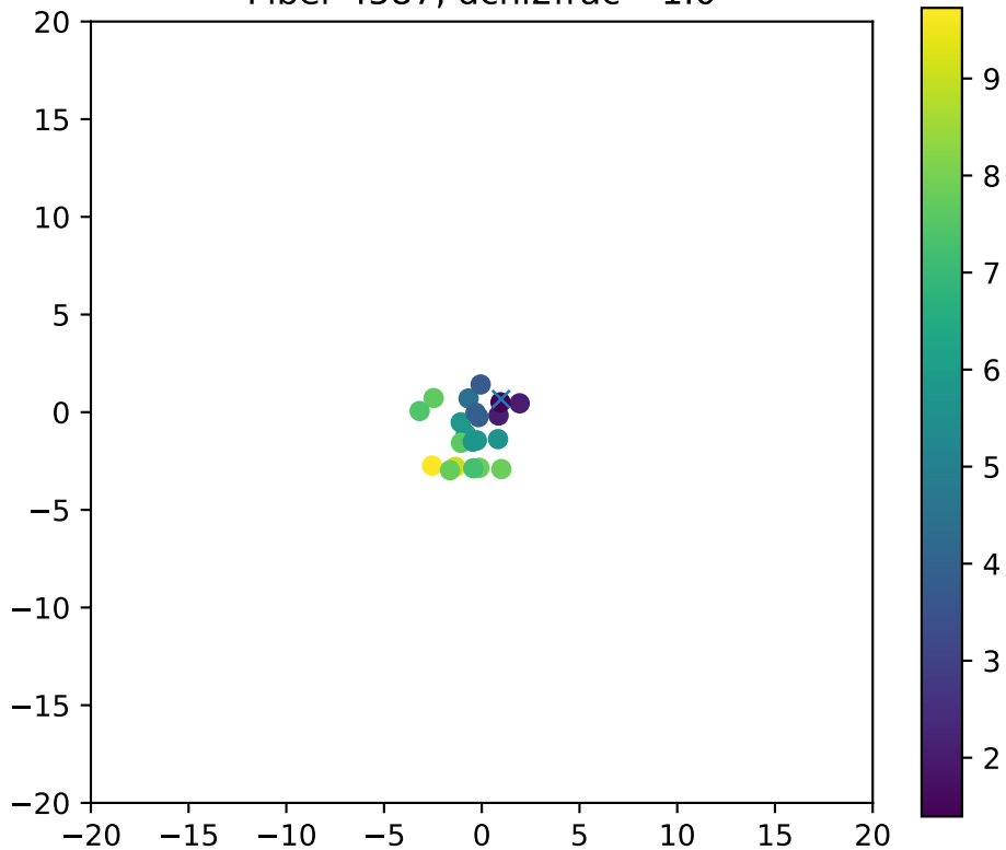
Fiber 4587, dchi2frac= 1.0
