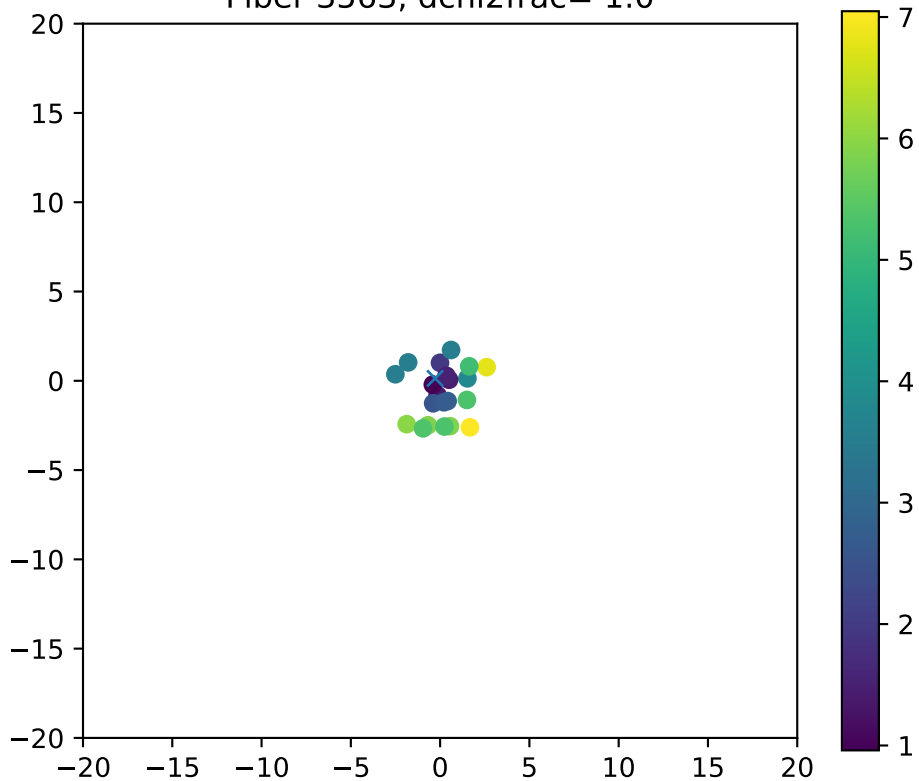
Fiber 3563, dchi2frac= 1.0
