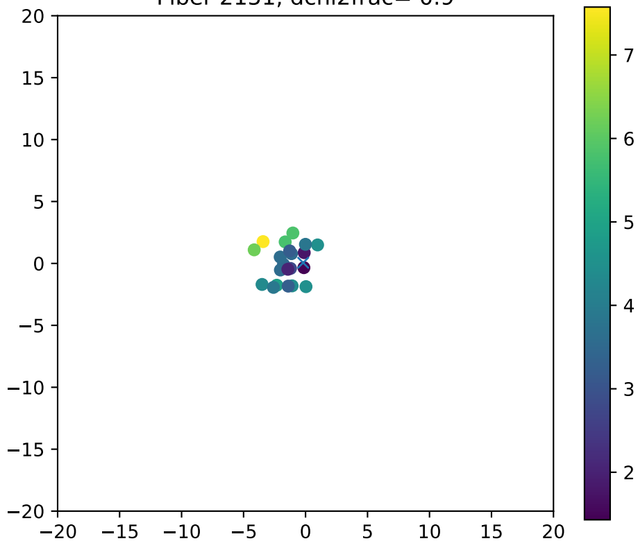
Fiber 2151, dchi2frac= 0.9
