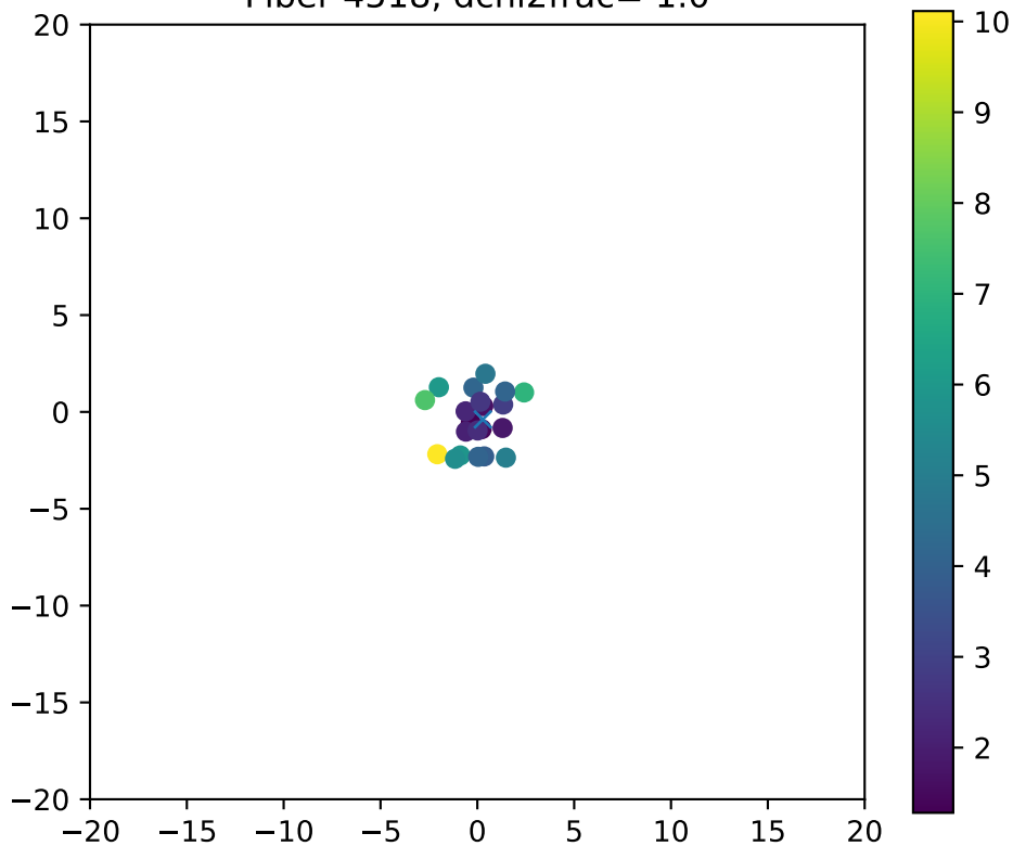
Fiber 4518, dchi2frac= 1.0
