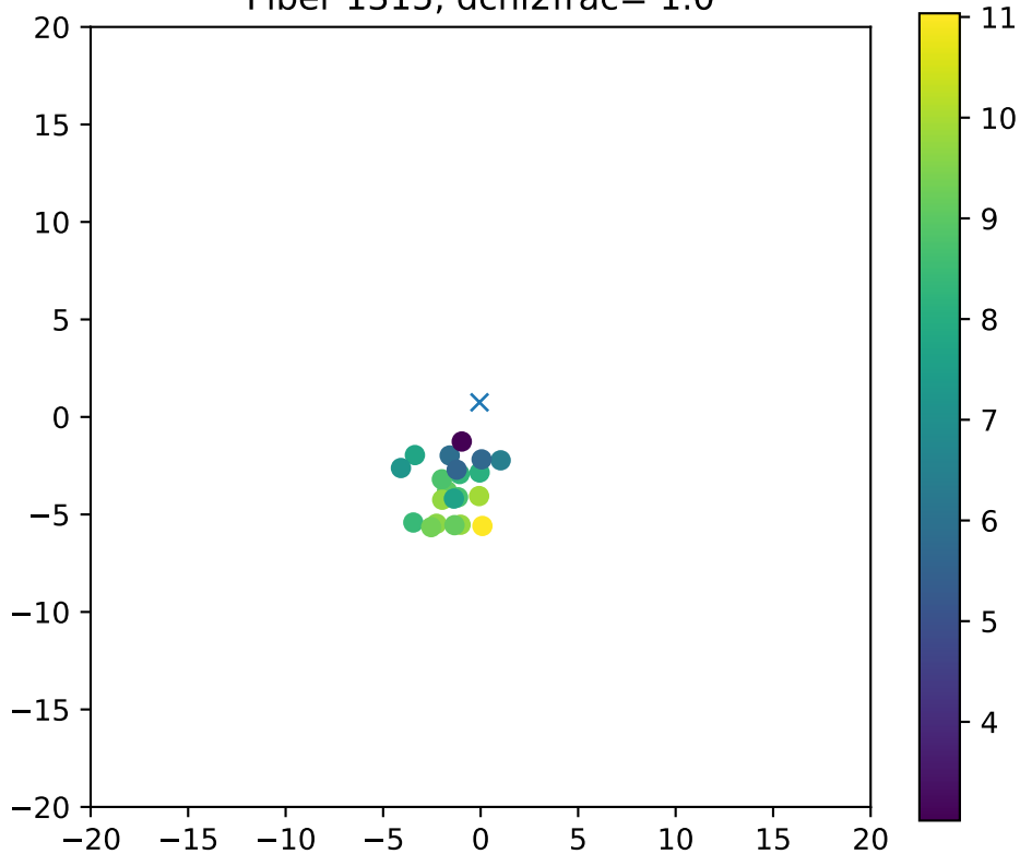
Fiber 1315, dchi2frac= 1.0
