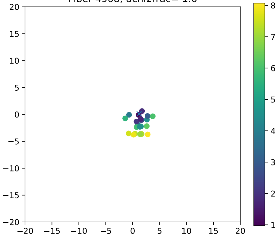
Fiber 4908, dchi2frac= 1.0
