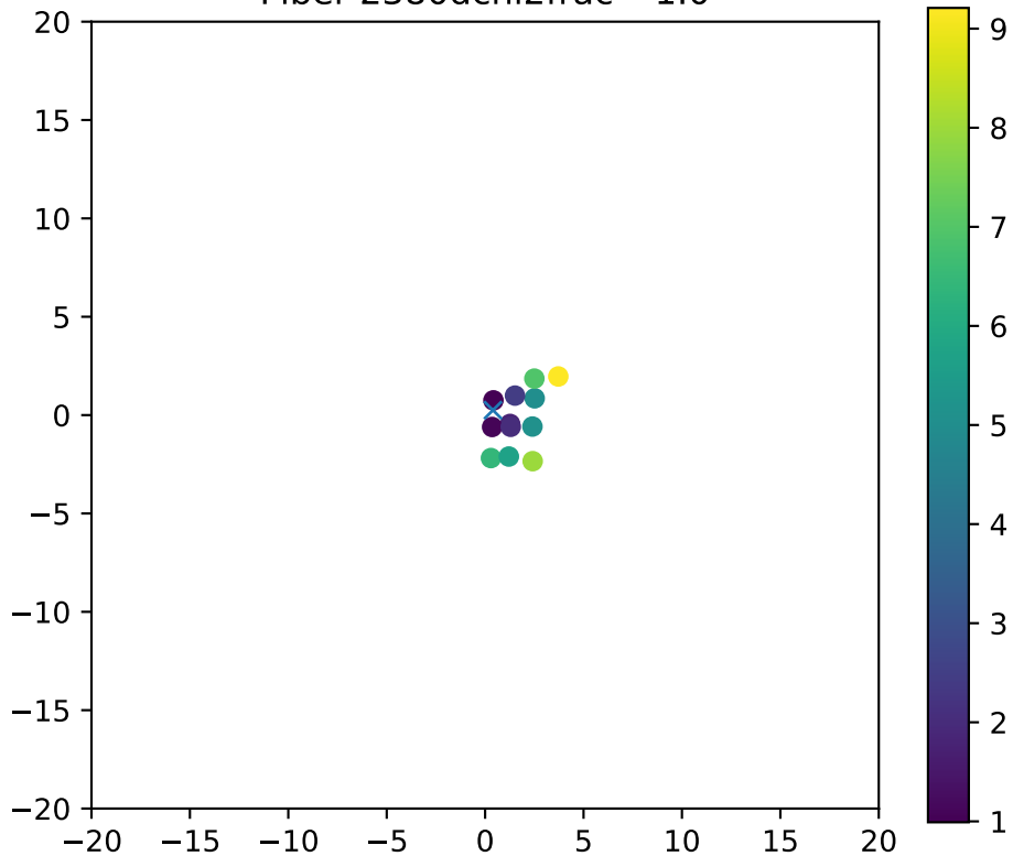
Fiber 2380dchi2frac= 1.0
