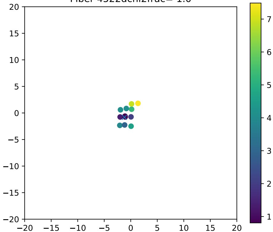
Fiber 4522dchi2frac= 1.0
