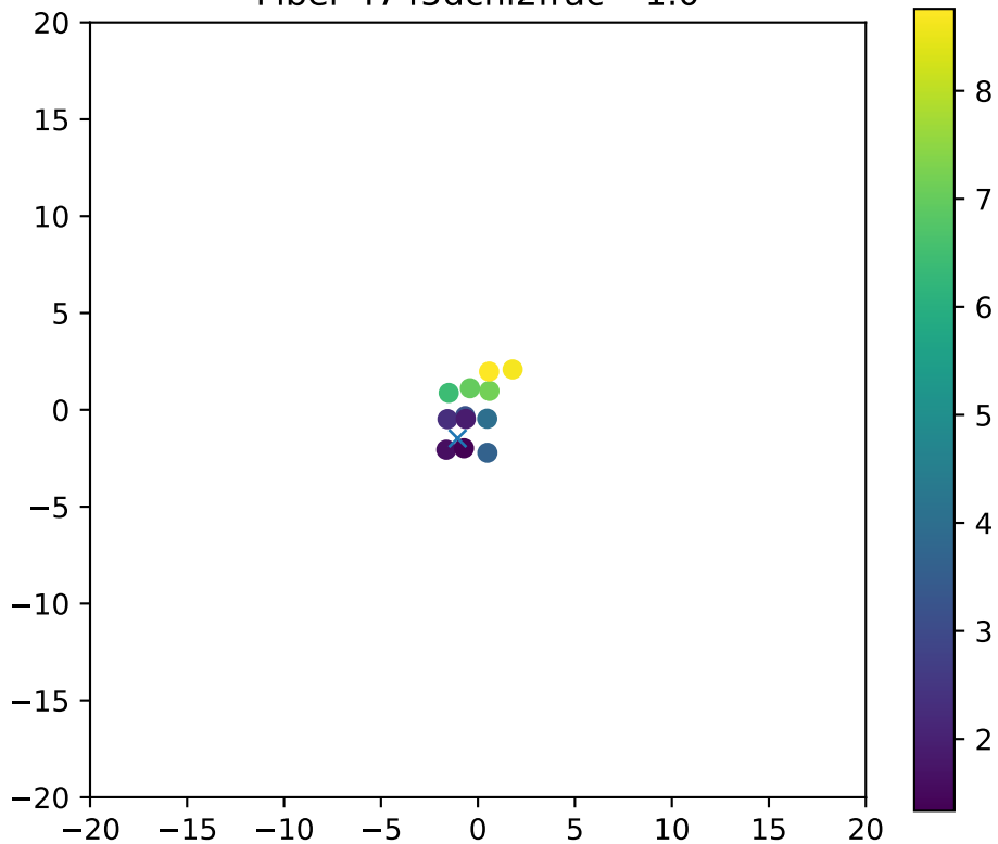
Fiber 4745dchi2frac= 1.0
