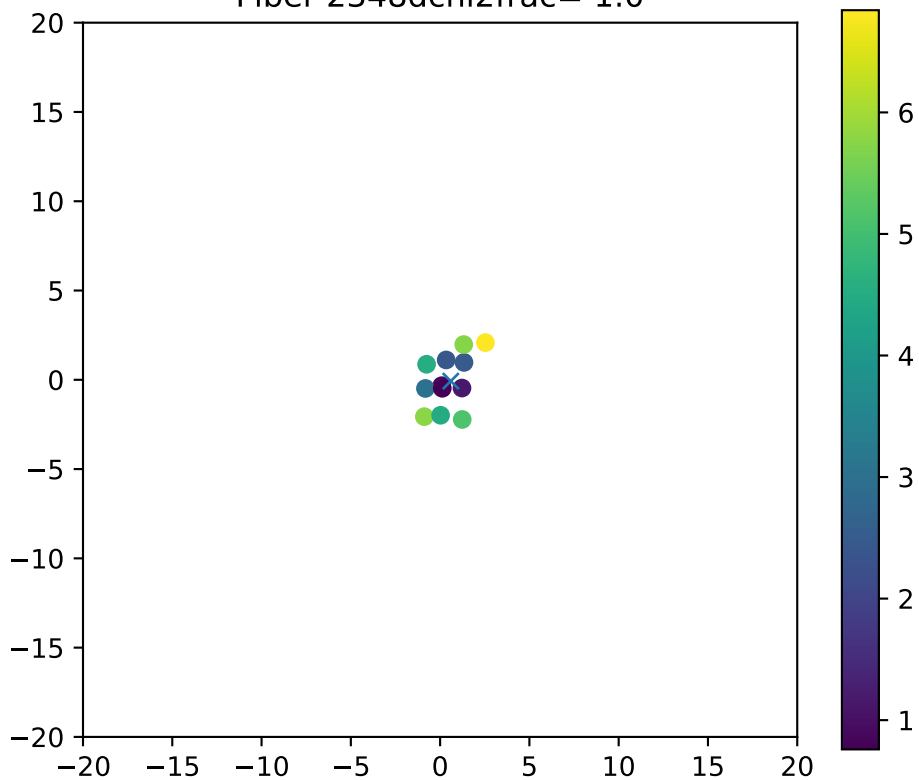
Fiber 2348dchi2frac= 1.0
