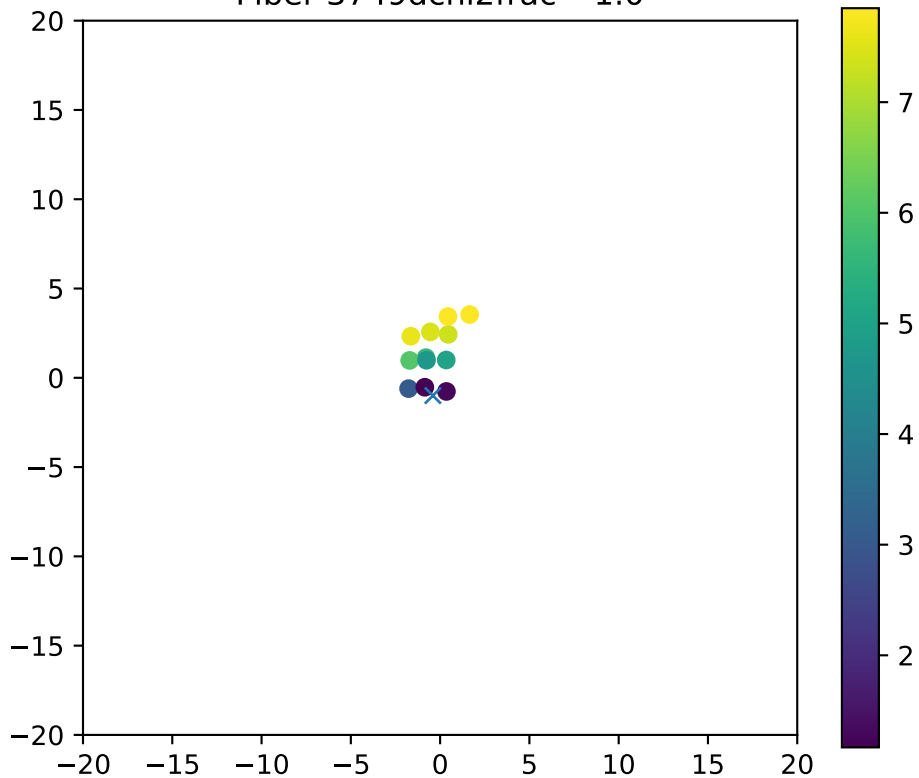
Fiber 3749dchi2frac= 1.0
