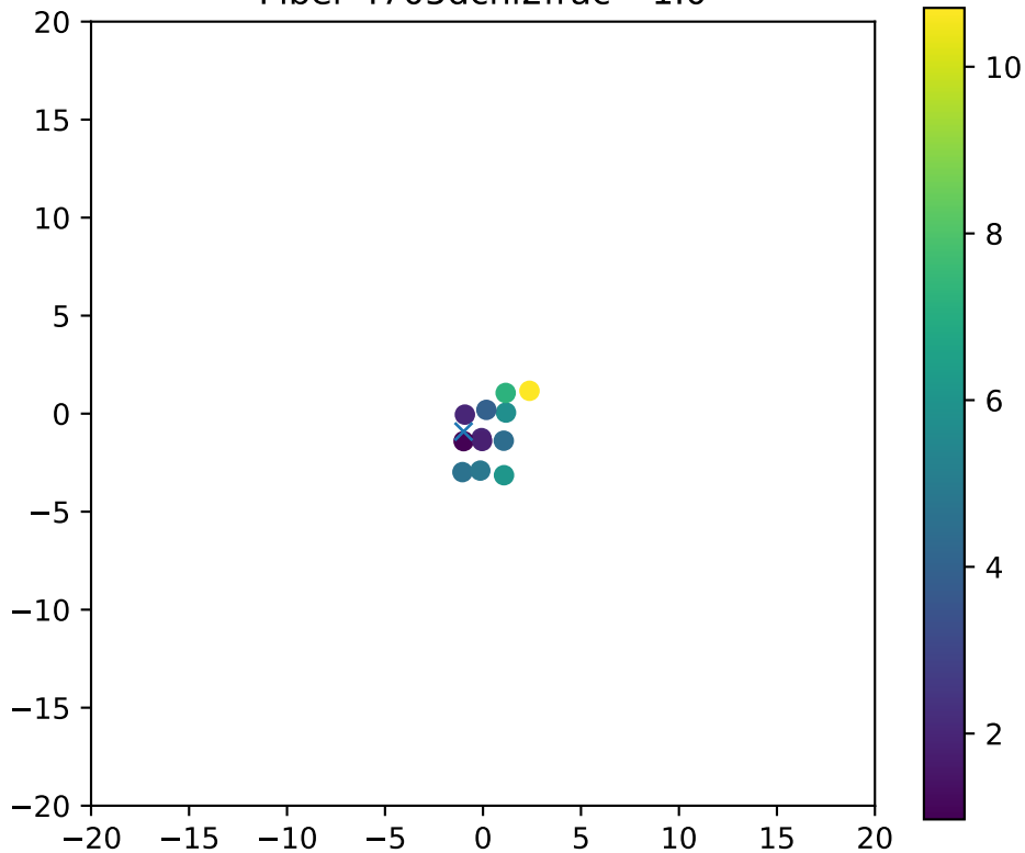
Fiber 4705dchi2frac= 1.0
