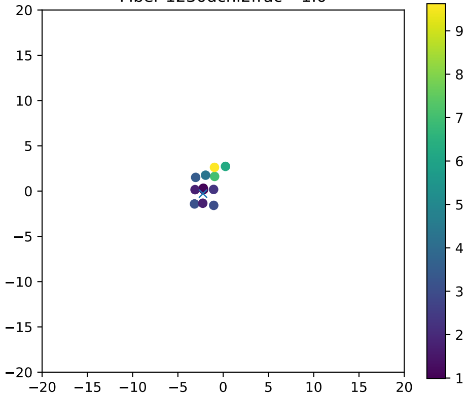
Fiber 1230dchi2frac= 1.0
