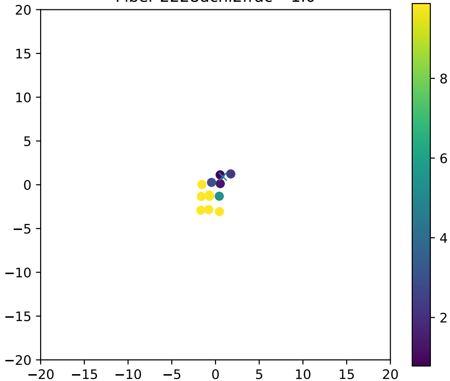
Fiber 2228dchi2frac= 1.0
