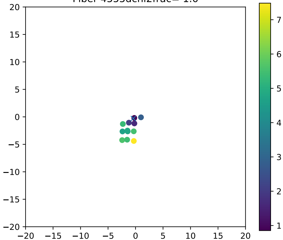
Fiber 4555dchi2frac= 1.0
