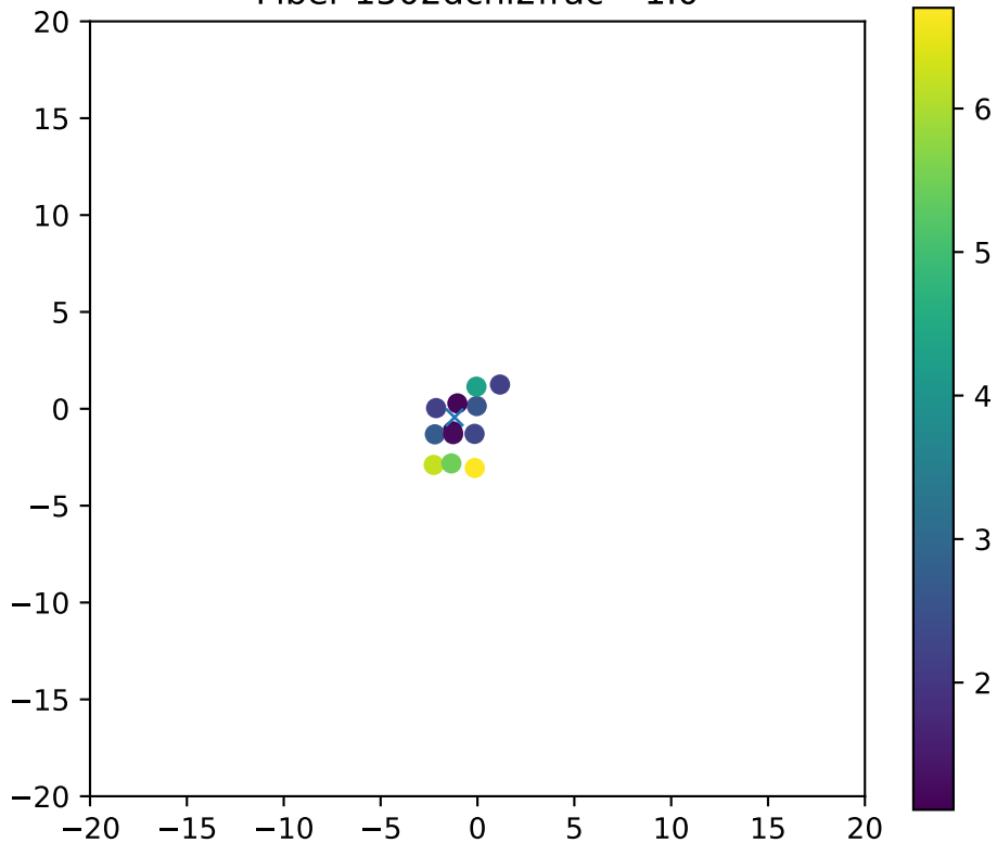
Fiber 1502dchi2frac= 1.0
