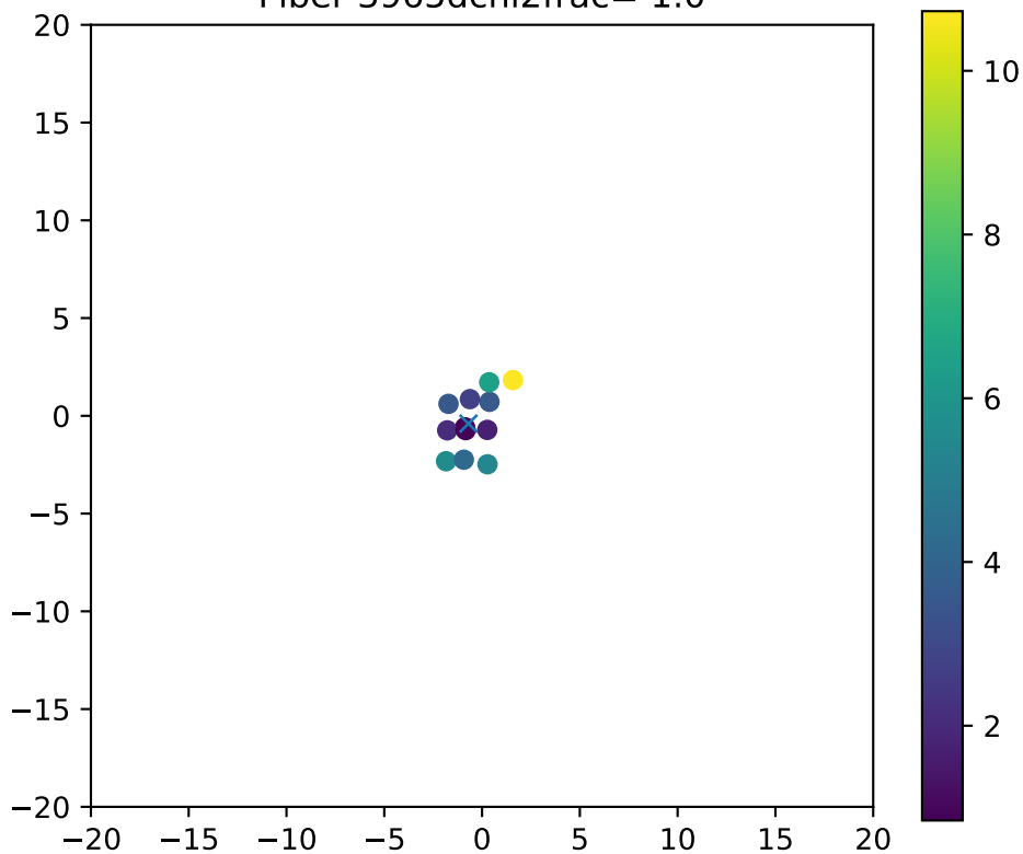
Fiber 3965dchi2frac= 1.0
