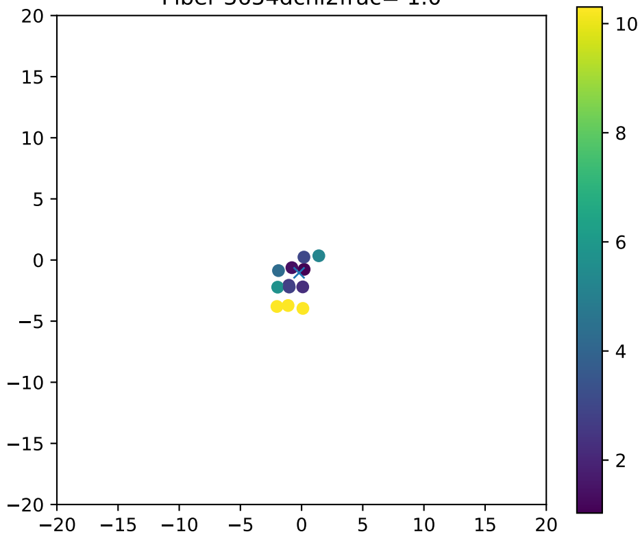
Fiber 3654dchi2frac= 1.0
