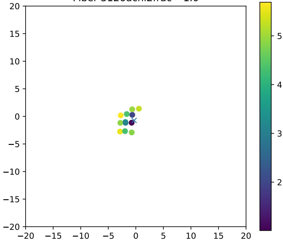
Fiber 3126dchi2frac= 1.0
