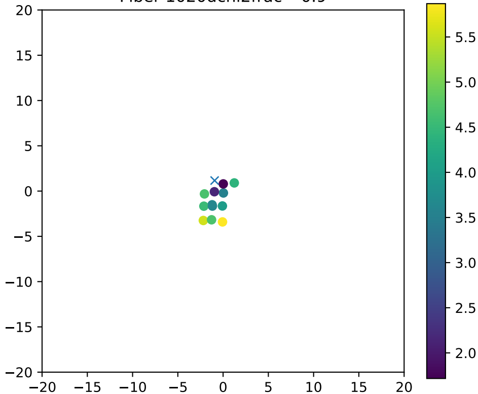
Fiber 1020dchi2frac= 0.9
