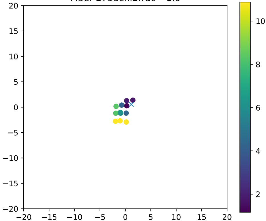
Fiber 279dchi2frac= 1.0
