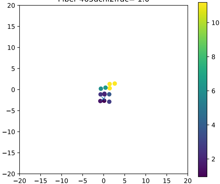
Fiber 465dchi2frac= 1.0
