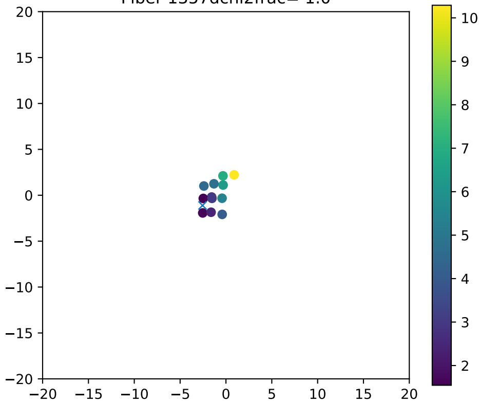
Fiber 1357dchi2frac= 1.0
