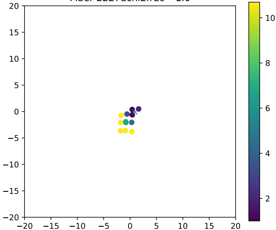
Fiber 2227dchi2frac= 1.0
