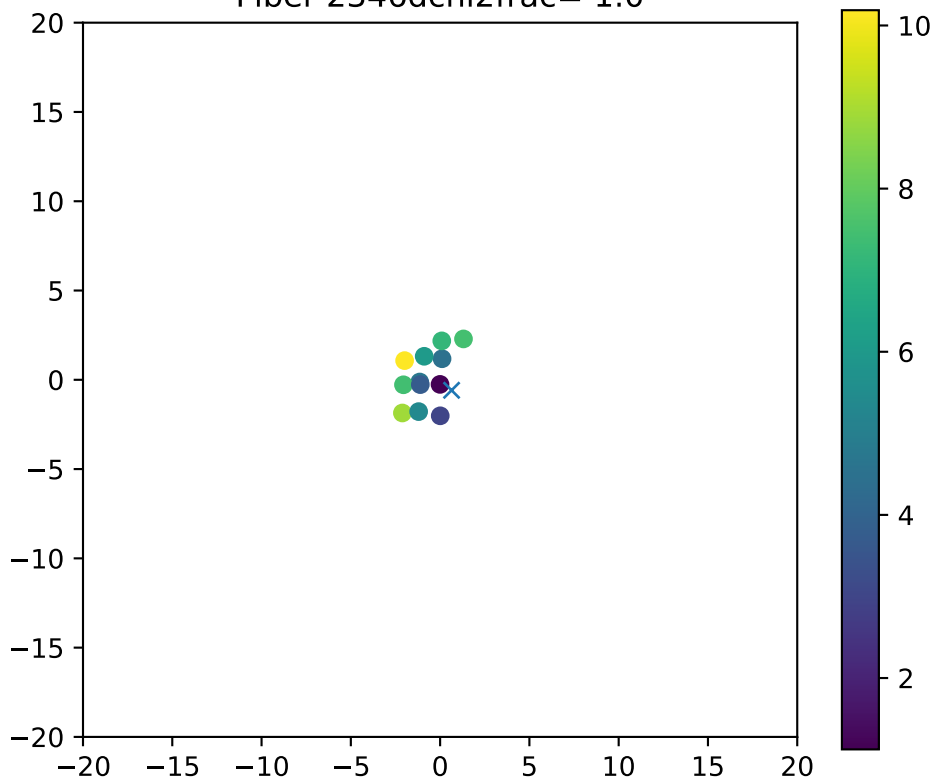
Fiber 2346dchi2frac= 1.0
