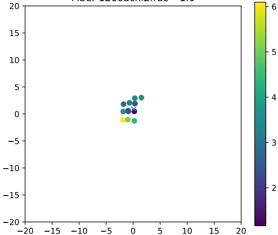
Fiber 1260dchi2frac= 1.0
