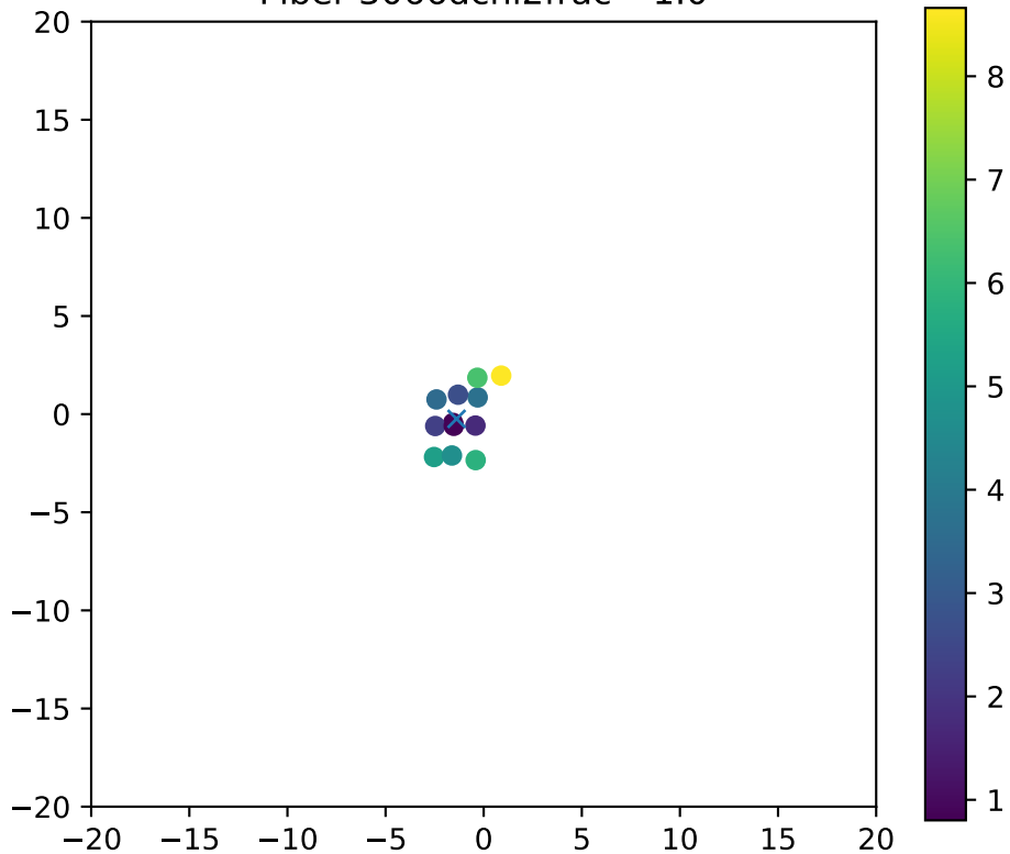
Fiber 3066dchi2frac= 1.0
