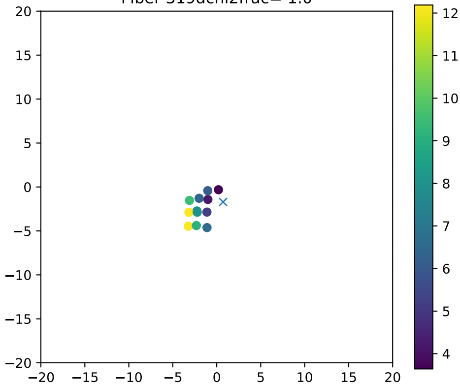
Fiber 319dchi2frac= 1.0
