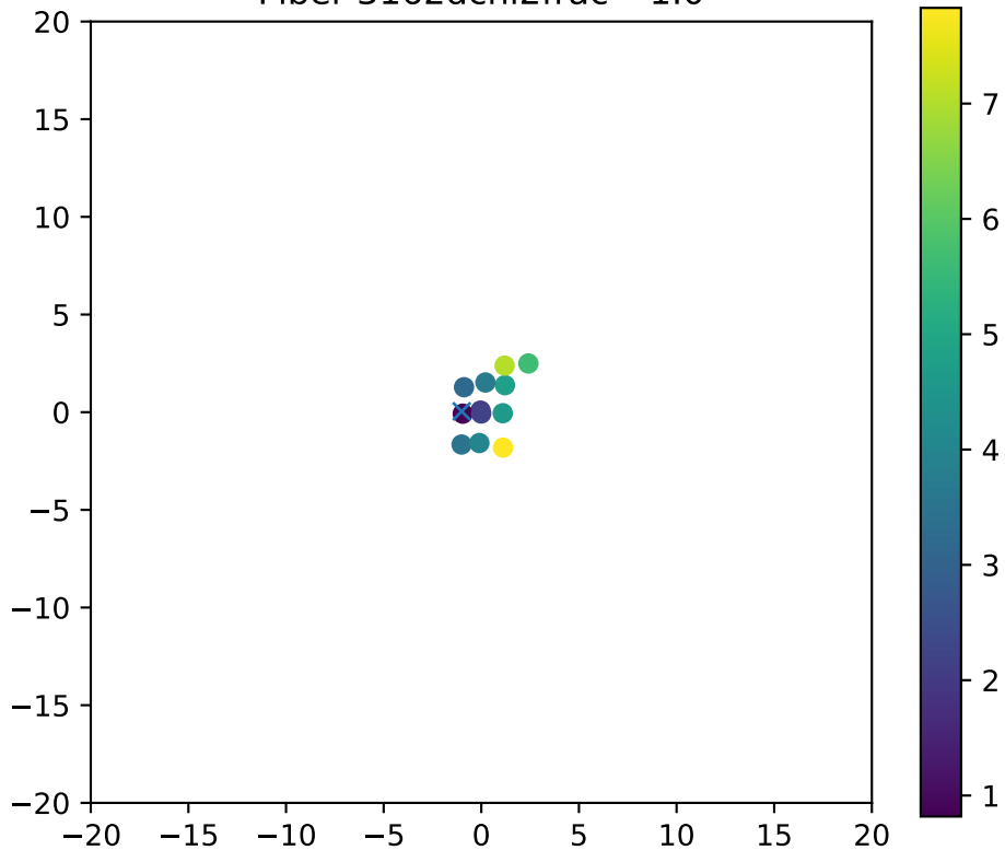
Fiber 3162dchi2frac= 1.0
