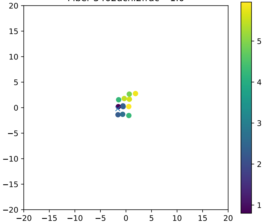
Fiber 3462dchi2frac= 1.0
