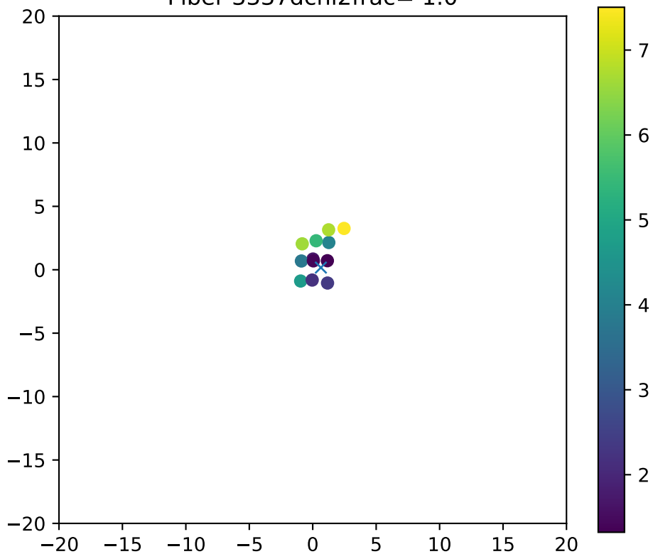
Fiber 3337dchi2frac= 1.0
