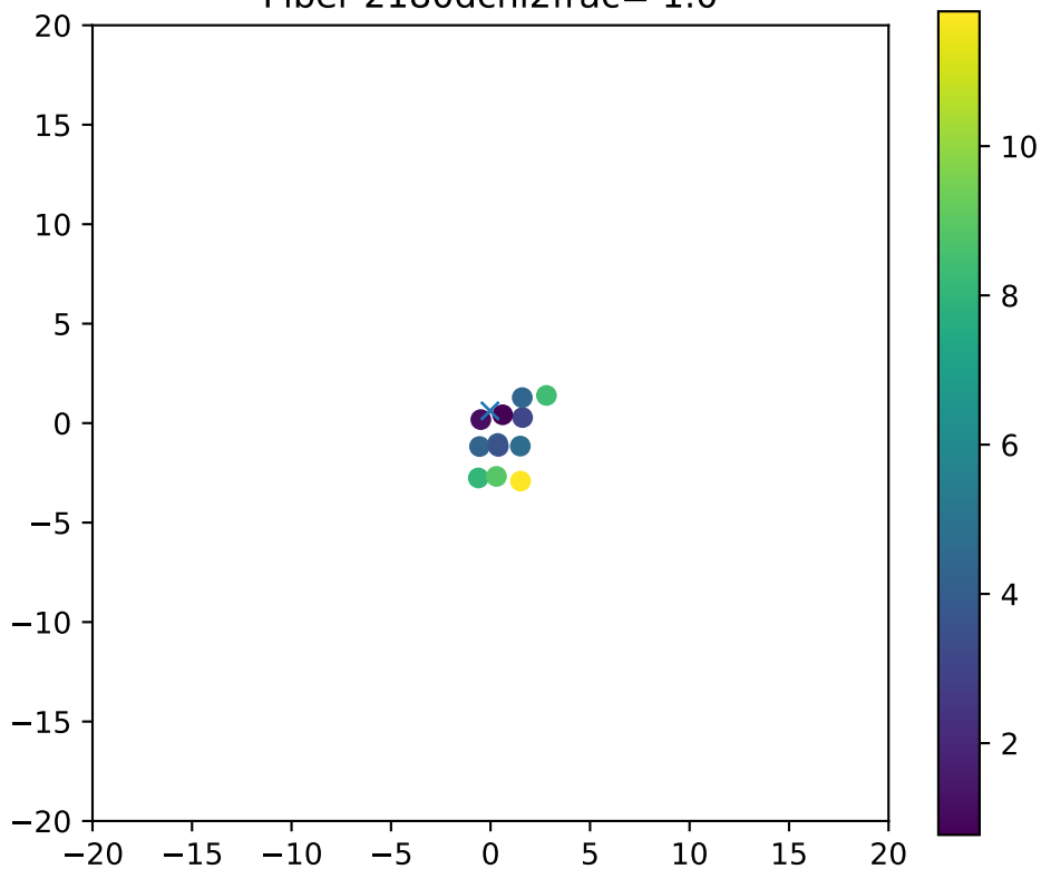
Fiber 2180dchi2frac= 1.0
