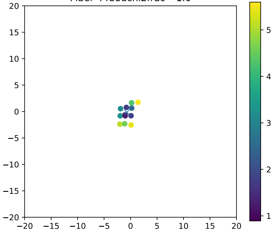
Fiber 4488dchi2frac= 1.0
