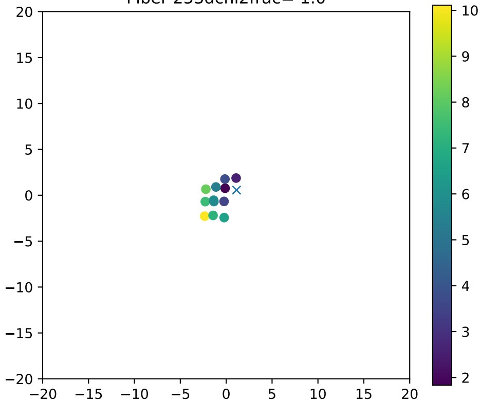
Fiber 253dchi2frac= 1.0
