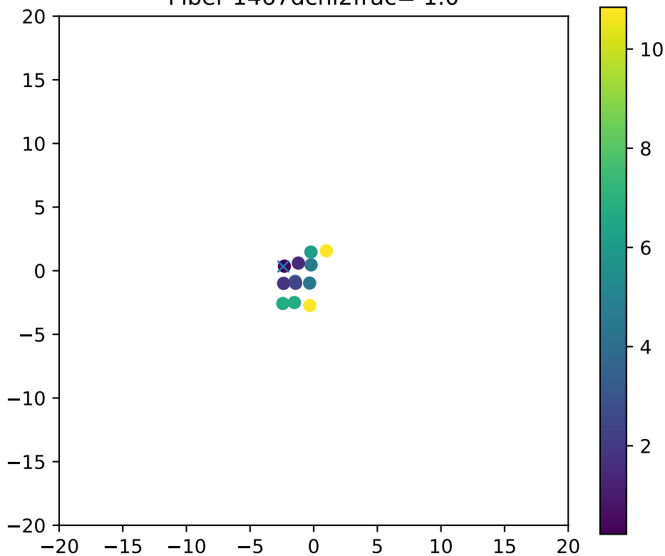
Fiber 1467dchi2frac= 1.0
