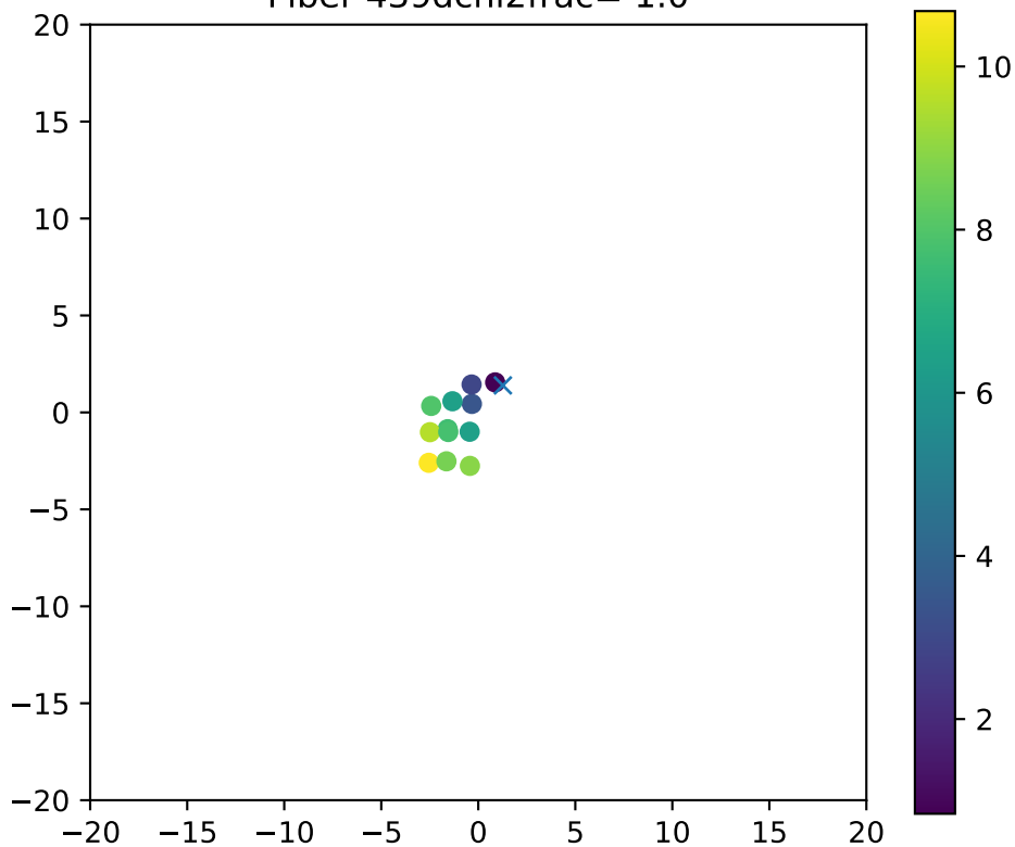
Fiber 439dchi2frac= 1.0
