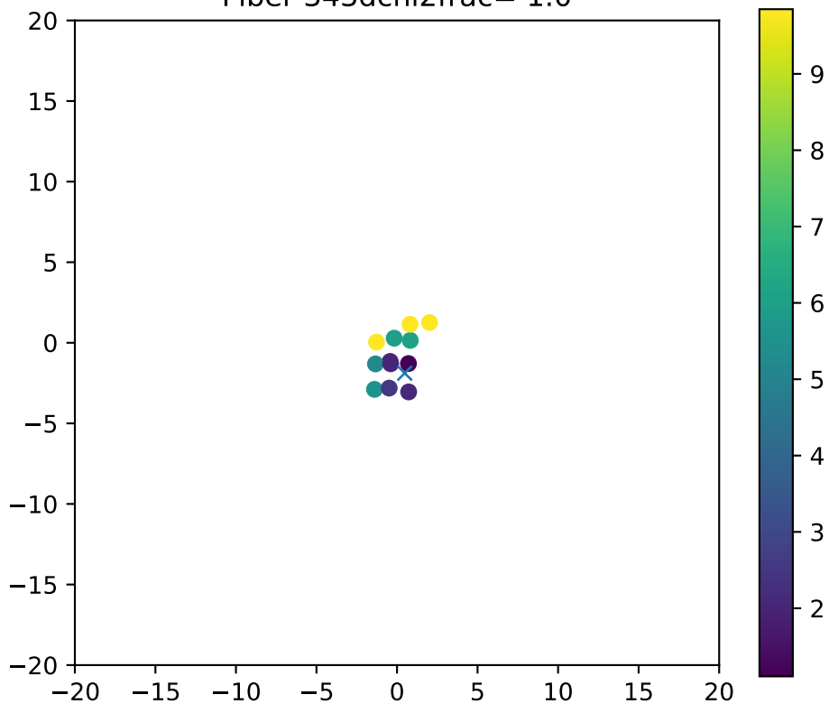
Fiber 343dchi2frac= 1.0
