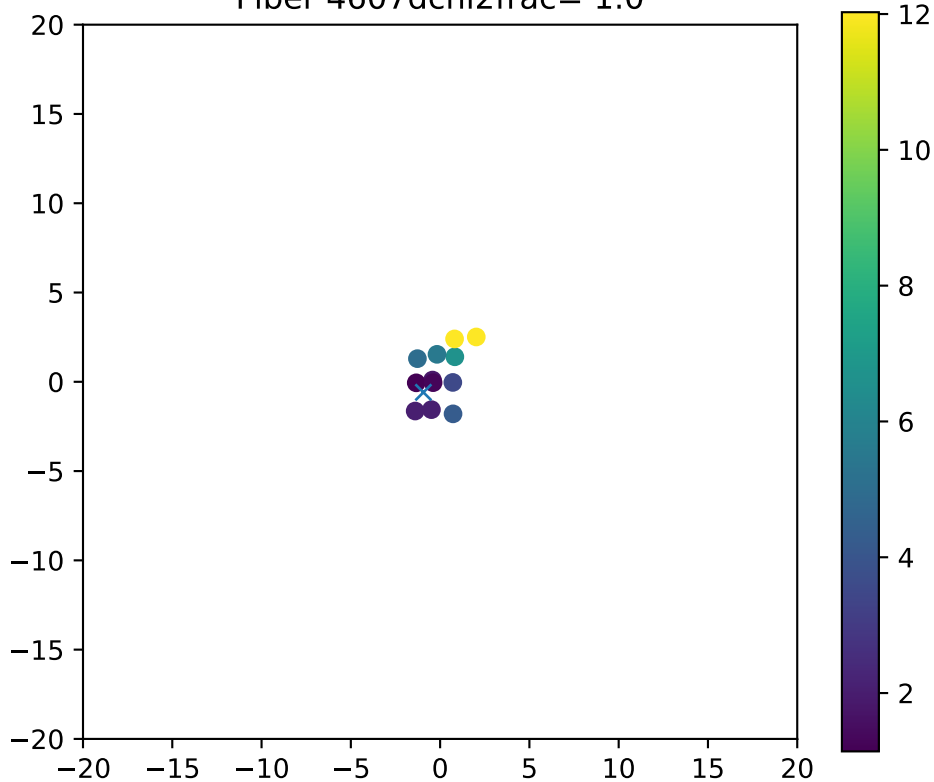
Fiber 4607dchi2frac= 1.0
