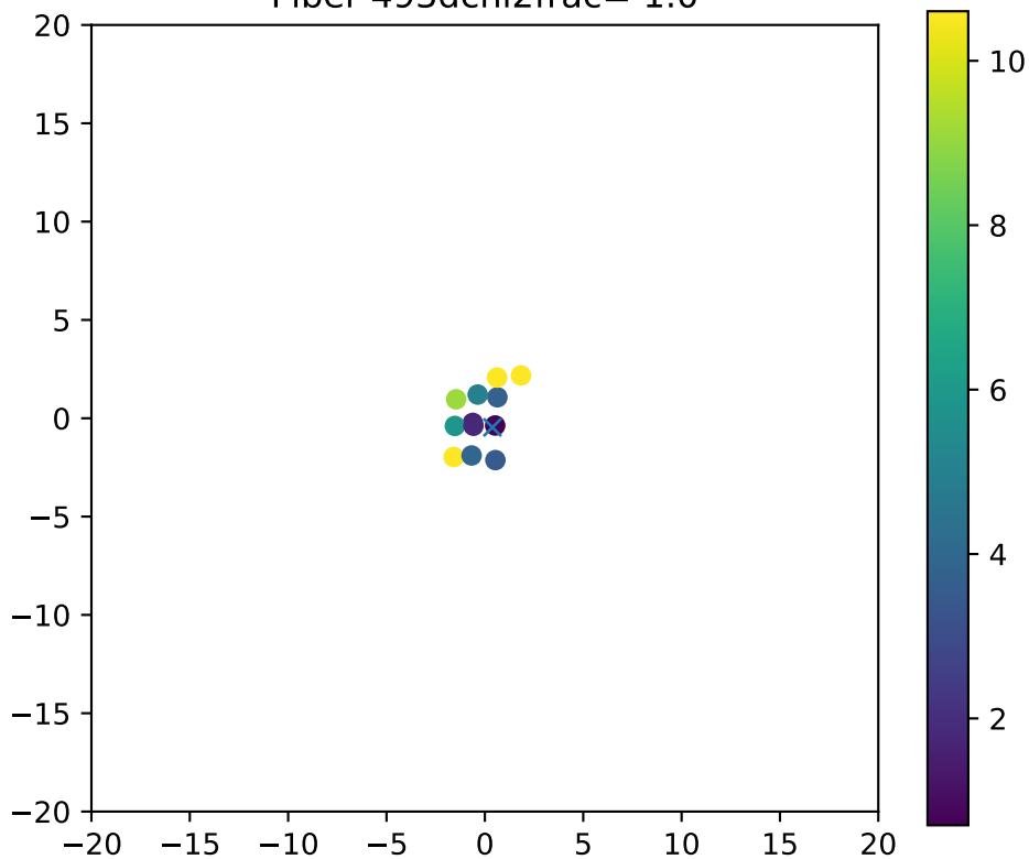
Fiber 493dchi2frac= 1.0
