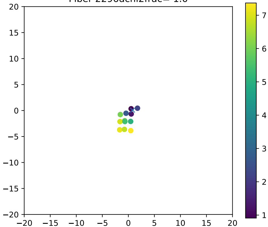
Fiber 2296dchi2frac= 1.0
