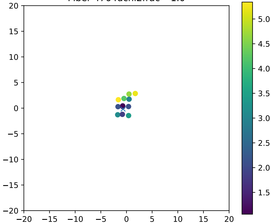
Fiber 4764dchi2frac= 1.0
