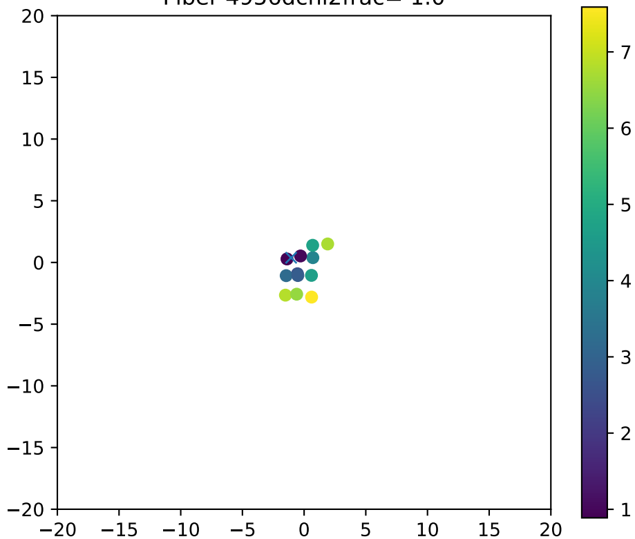
Fiber 4956dchi2frac= 1.0
