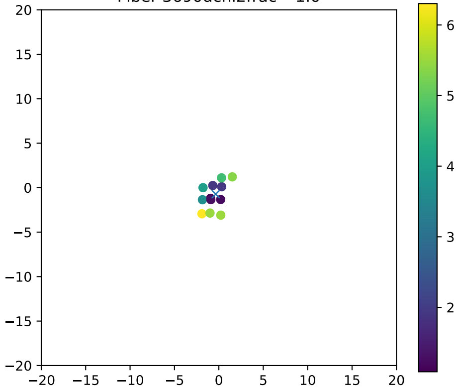
Fiber 3690dchi2frac= 1.0
