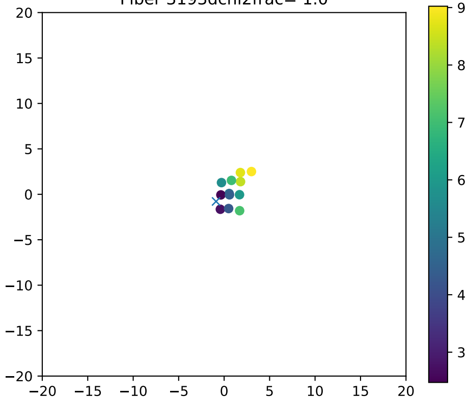
Fiber 3193dchi2frac= 1.0
