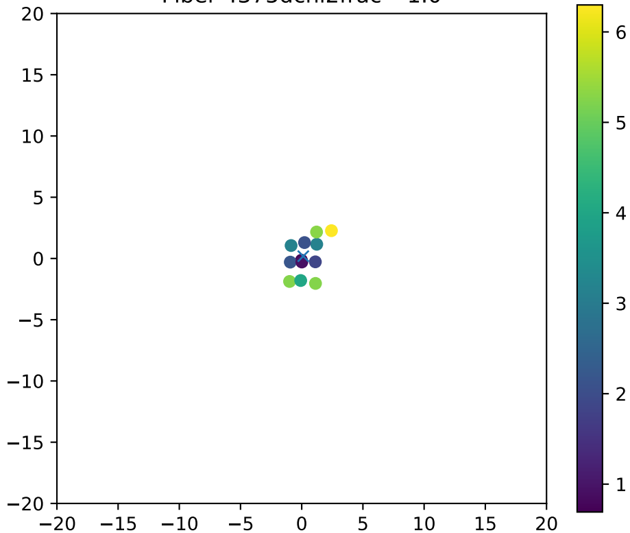
Fiber 4375dchi2frac= 1.0
