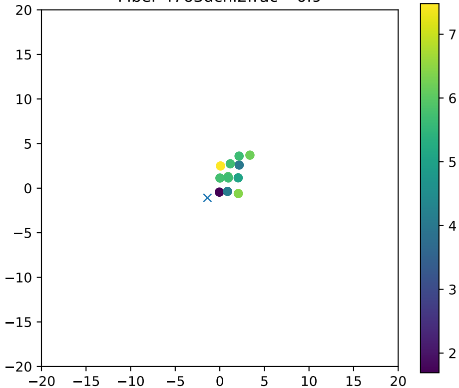
Fiber 4763dchi2frac= 0.9
