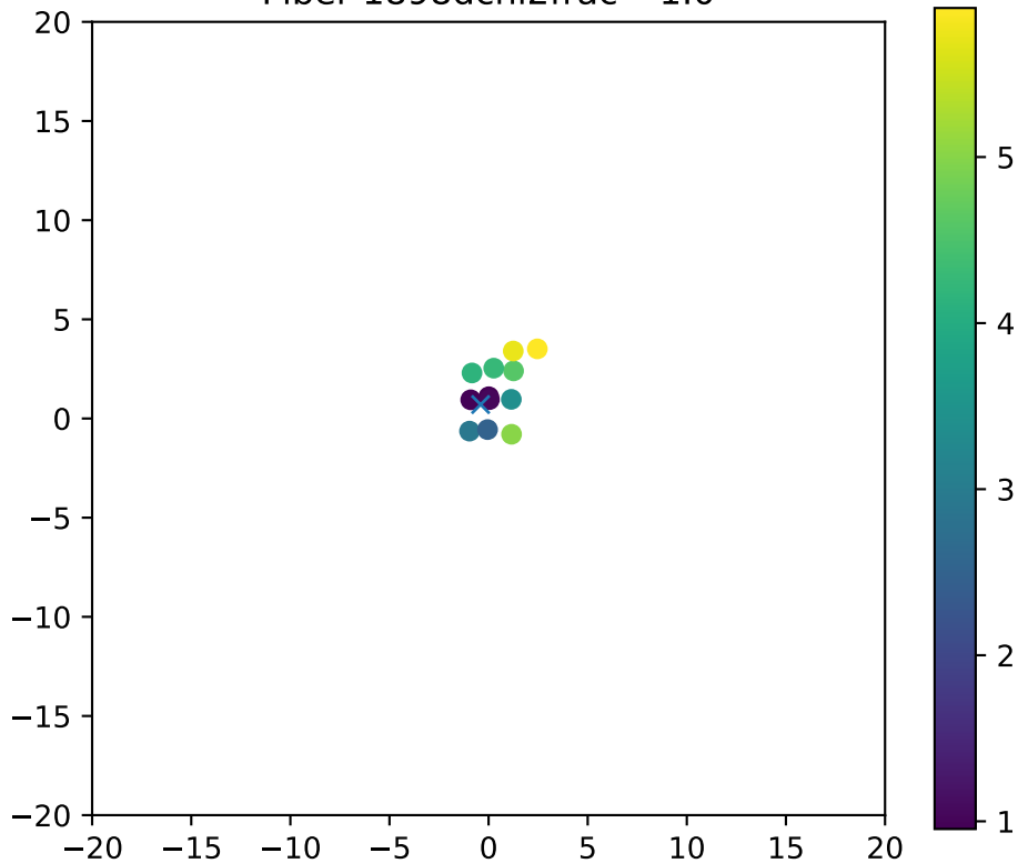
Fiber 1898dchi2frac= 1.0
