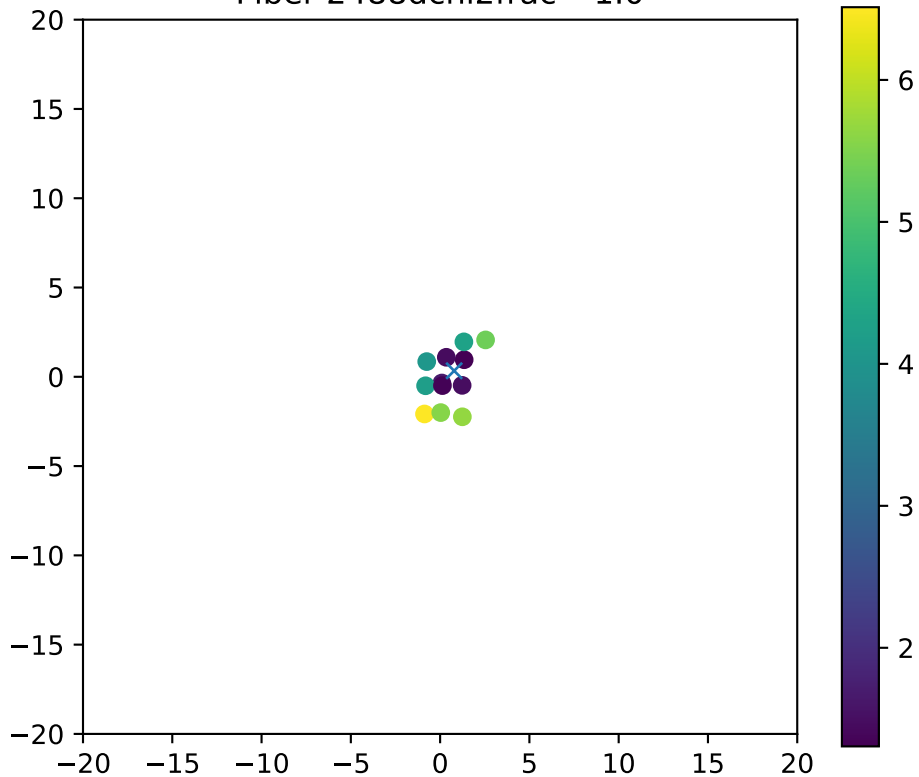
Fiber 2488dchi2frac= 1.0
