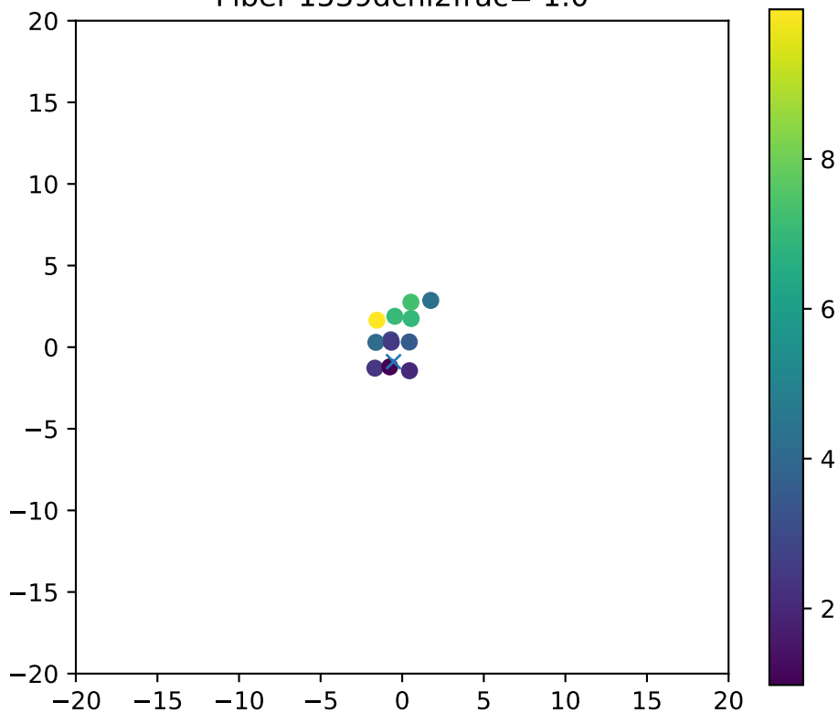
Fiber 1539dchi2frac= 1.0
