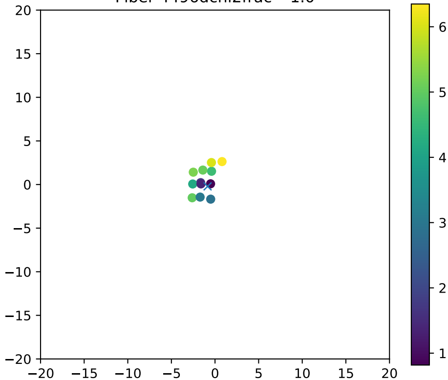
Fiber 4496dchi2frac= 1.0
