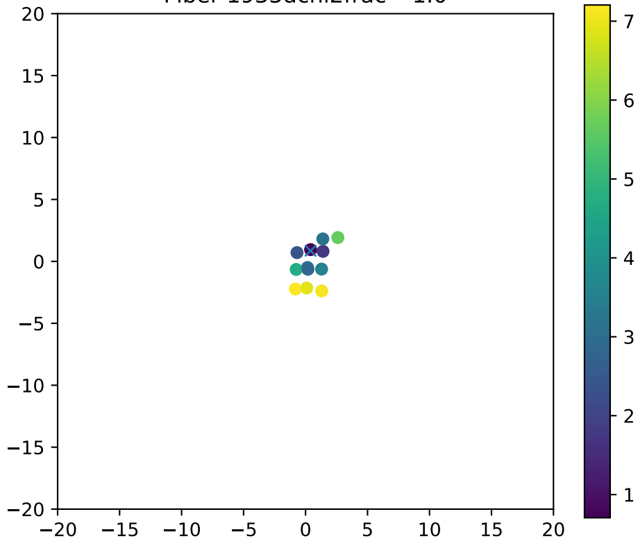
Fiber 1933dchi2frac= 1.0
