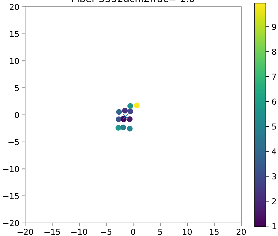
Fiber 3352dchi2frac= 1.0
