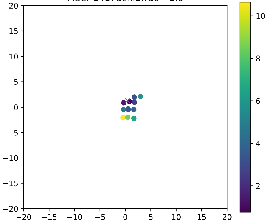
Fiber 1417dchi2frac= 1.0
