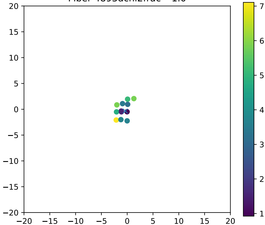
Fiber 4893dchi2frac= 1.0
