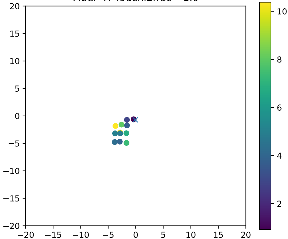
Fiber 4749dchi2frac= 1.0
