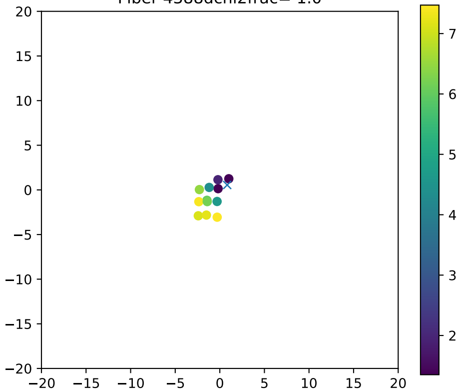
Fiber 4388dchi2frac= 1.0
