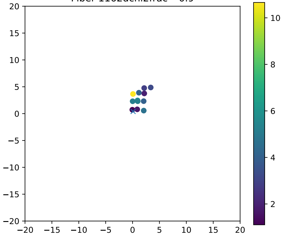
Fiber 1162dchi2frac= 0.9
