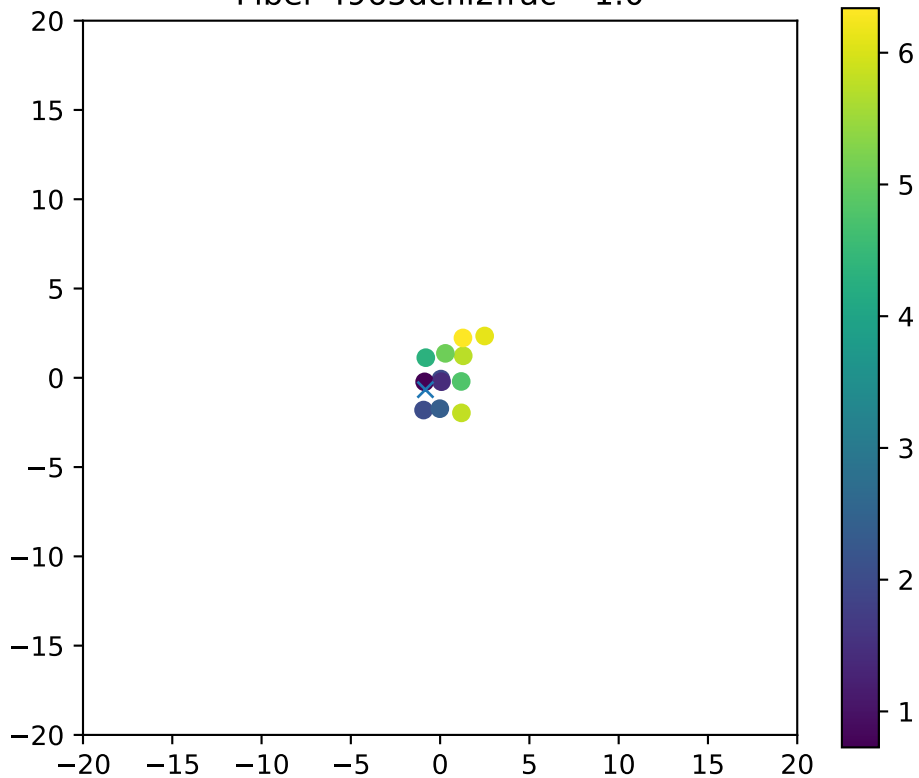
Fiber 4965dchi2frac= 1.0
