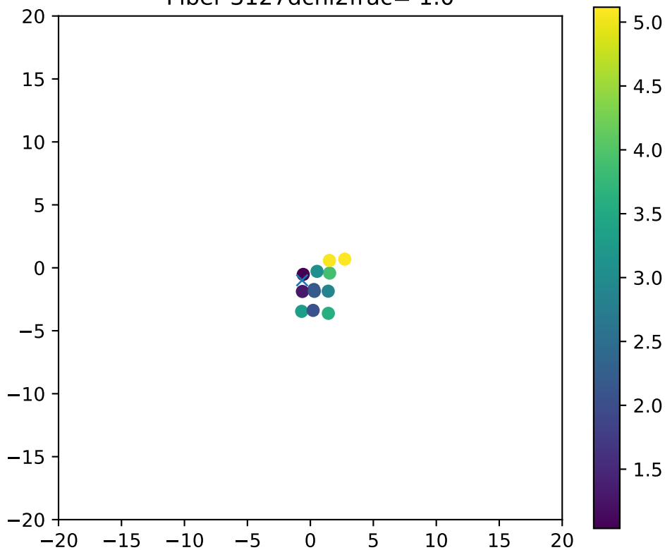
Fiber 3127dchi2frac= 1.0
