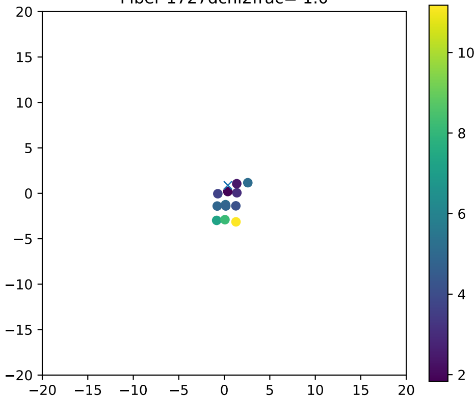
Fiber 1727dchi2frac= 1.0
