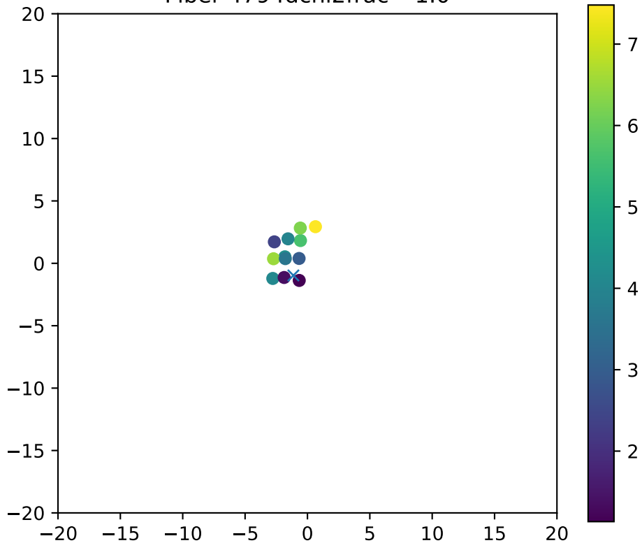
Fiber 4794dchi2frac= 1.0
