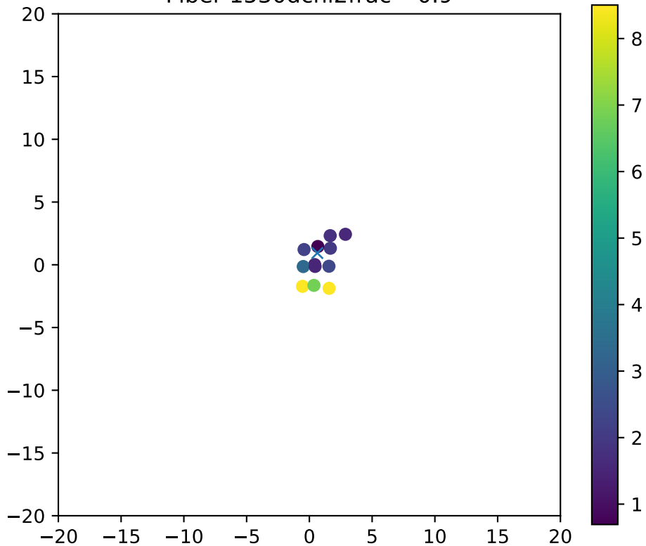
Fiber 1530dchi2frac= 0.9
