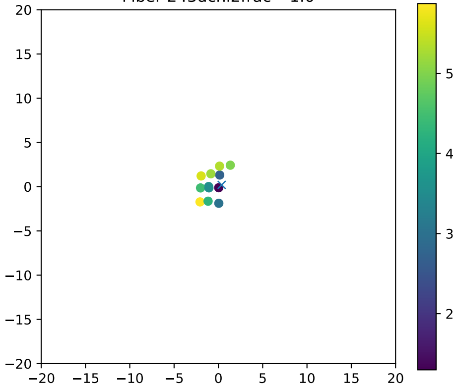
Fiber 243dchi2frac= 1.0
