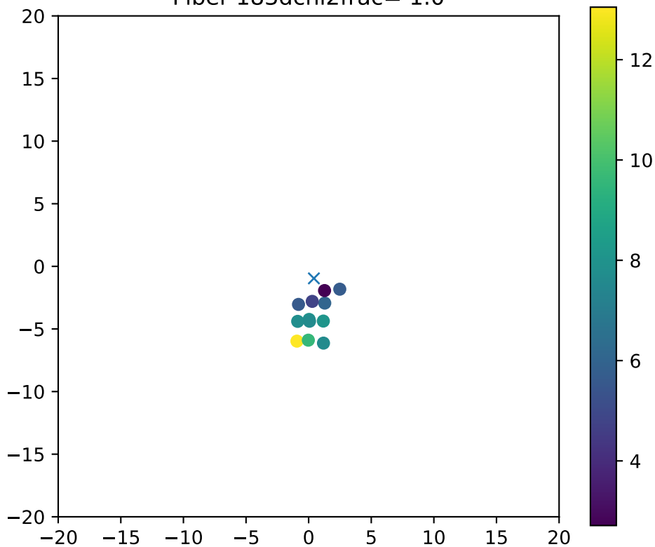
Fiber 183dchi2frac= 1.0
