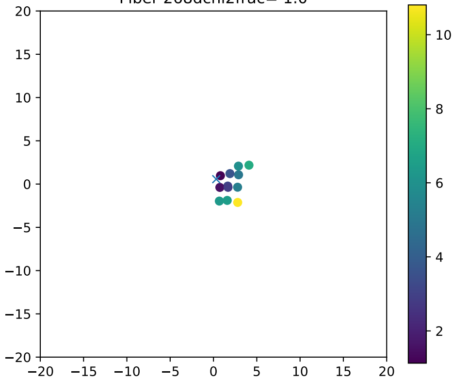
Fiber 268dchi2frac= 1.0
