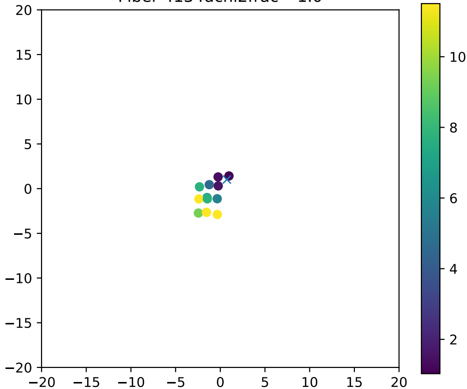
Fiber 4134dchi2frac= 1.0
