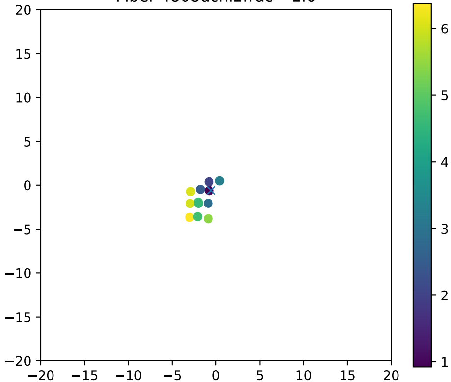
Fiber 4868dchi2frac= 1.0
