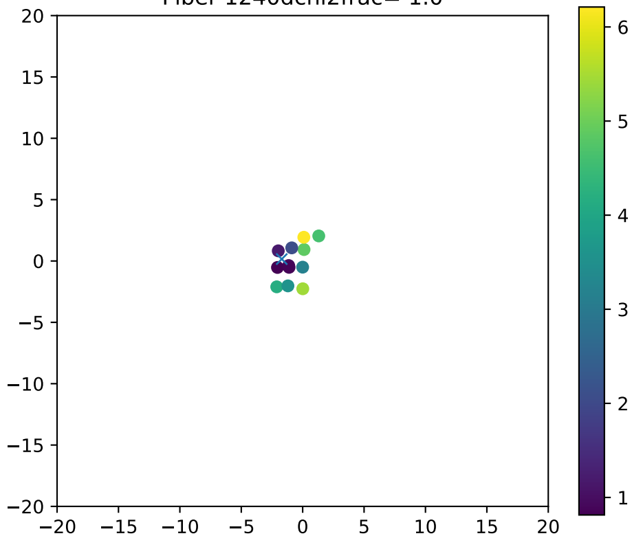
Fiber 1240dchi2frac= 1.0
