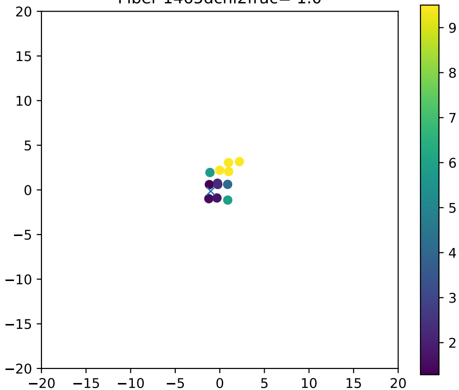
Fiber 1465dchi2frac= 1.0
