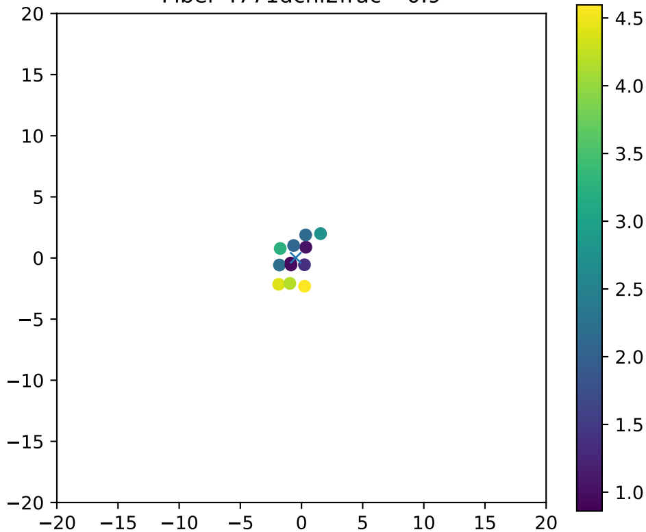
Fiber 4771dchi2frac= 0.9
