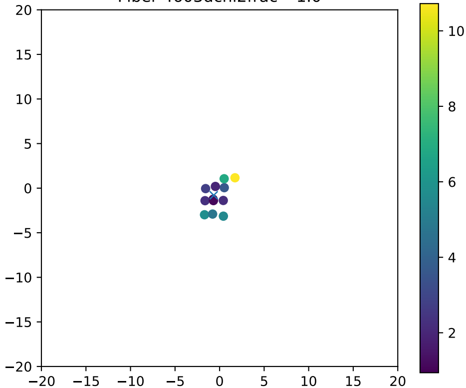
Fiber 4603dchi2frac= 1.0
