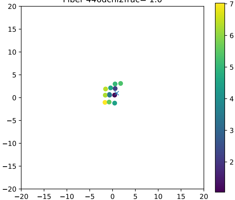
Fiber 446dchi2frac= 1.0
