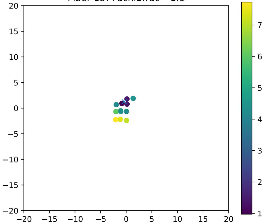
Fiber 1877dchi2frac= 1.0
