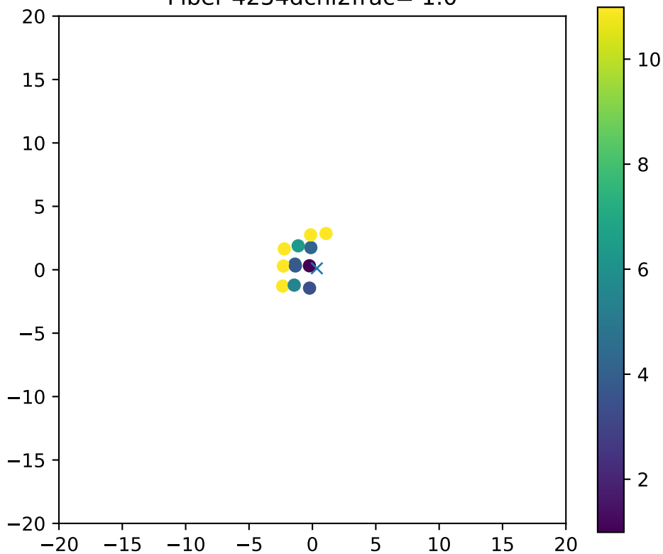
Fiber 4254dchi2frac= 1.0
