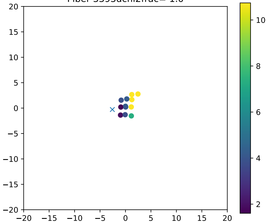
Fiber 3393dchi2frac= 1.0
