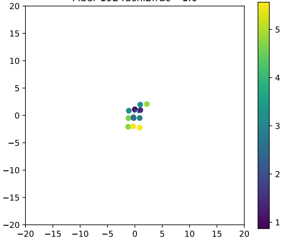
Fiber 1924dchi2frac= 1.0
