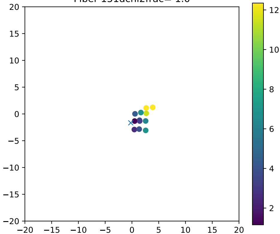
Fiber 151dchi2frac= 1.0
