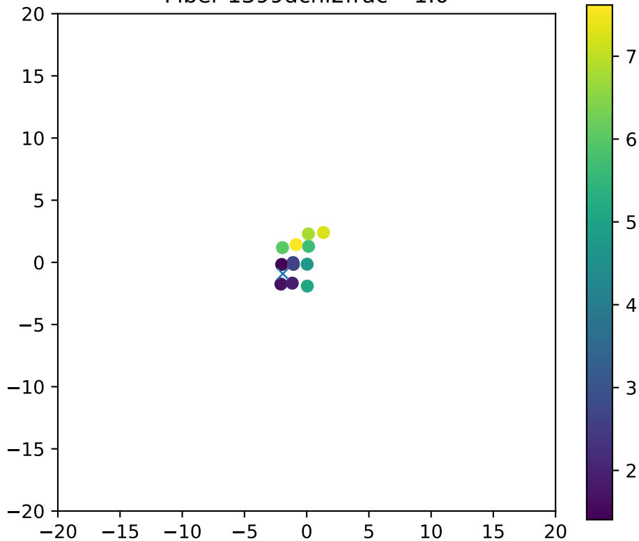
Fiber 1399dchi2frac= 1.0
