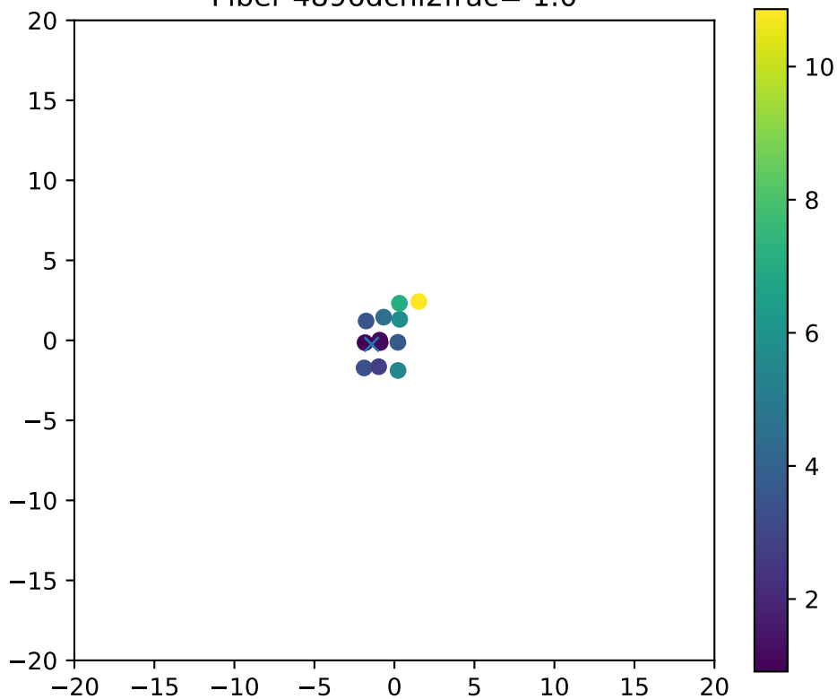
Fiber 4896dchi2frac= 1.0
