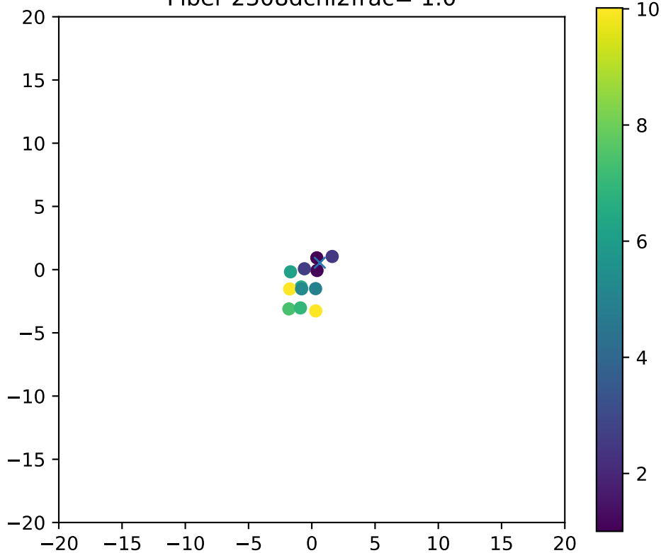
Fiber 2308dchi2frac= 1.0
