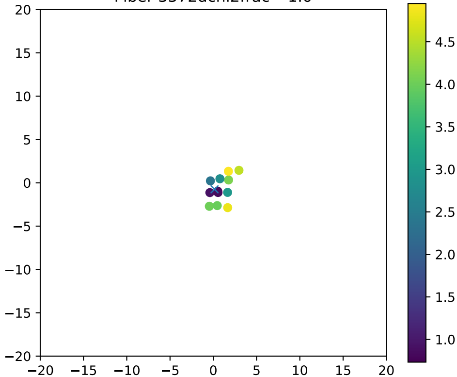
Fiber 3572dchi2frac= 1.0
