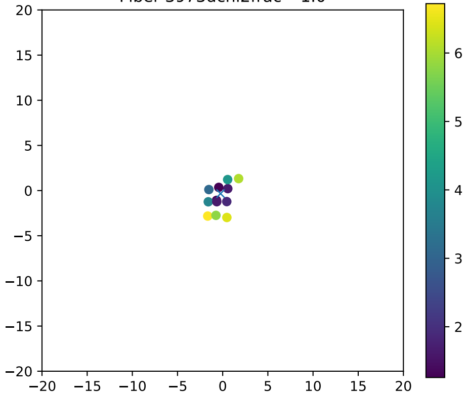
Fiber 3973dchi2frac= 1.0
