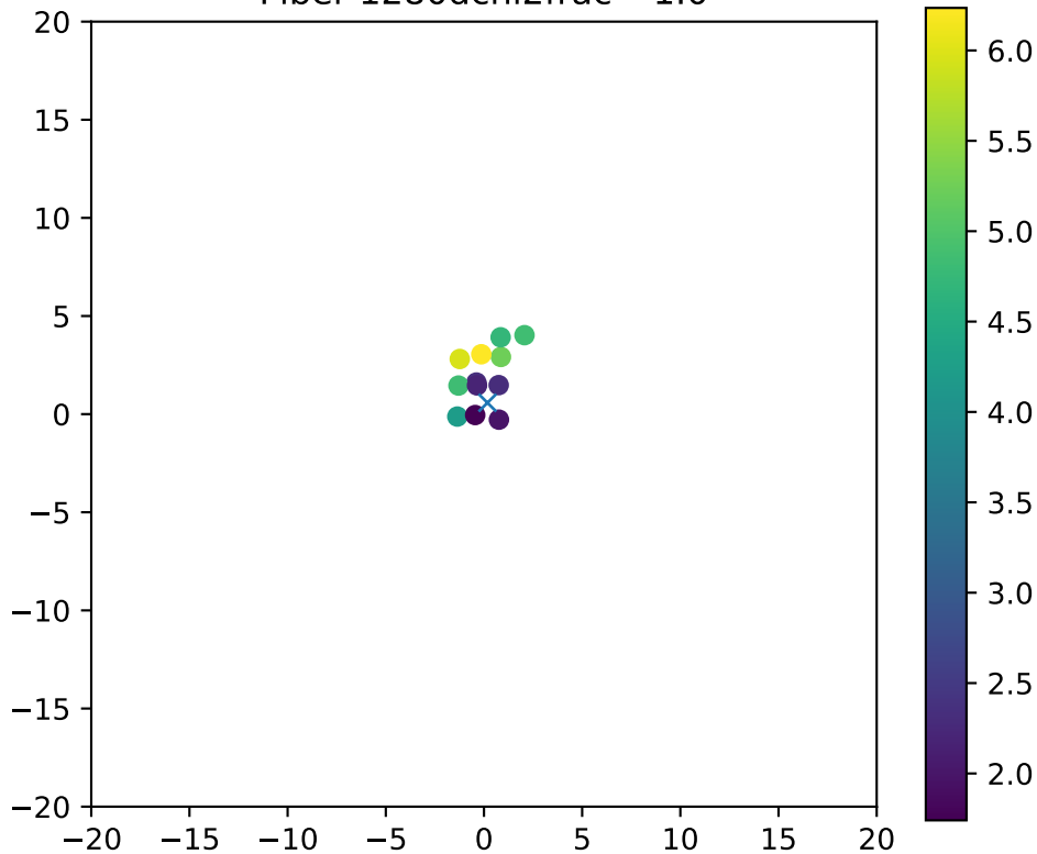
Fiber 1280dchi2frac= 1.0
