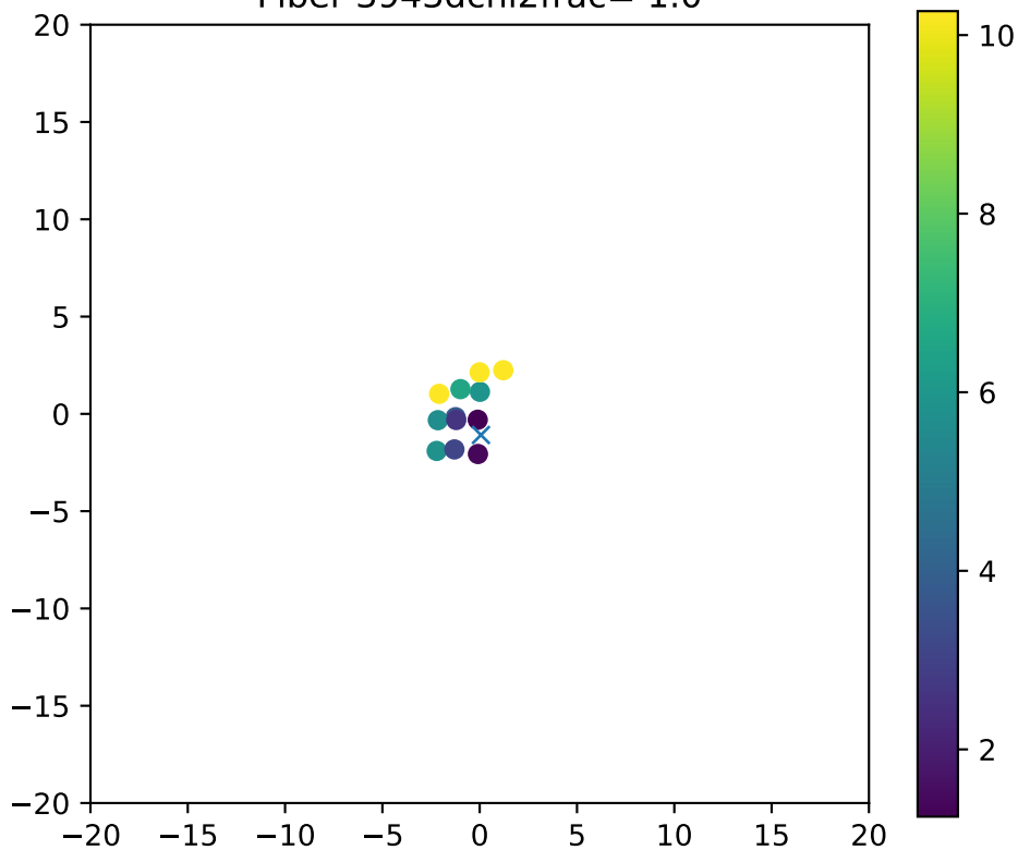
Fiber 3943dchi2frac= 1.0
