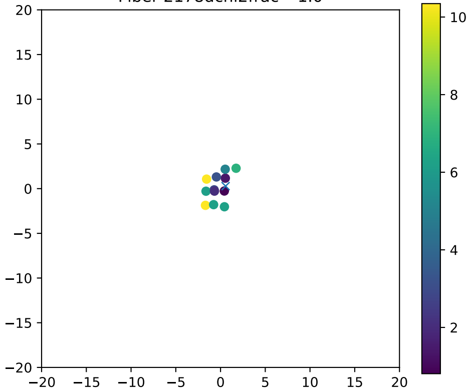
Fiber 2178dchi2frac= 1.0
