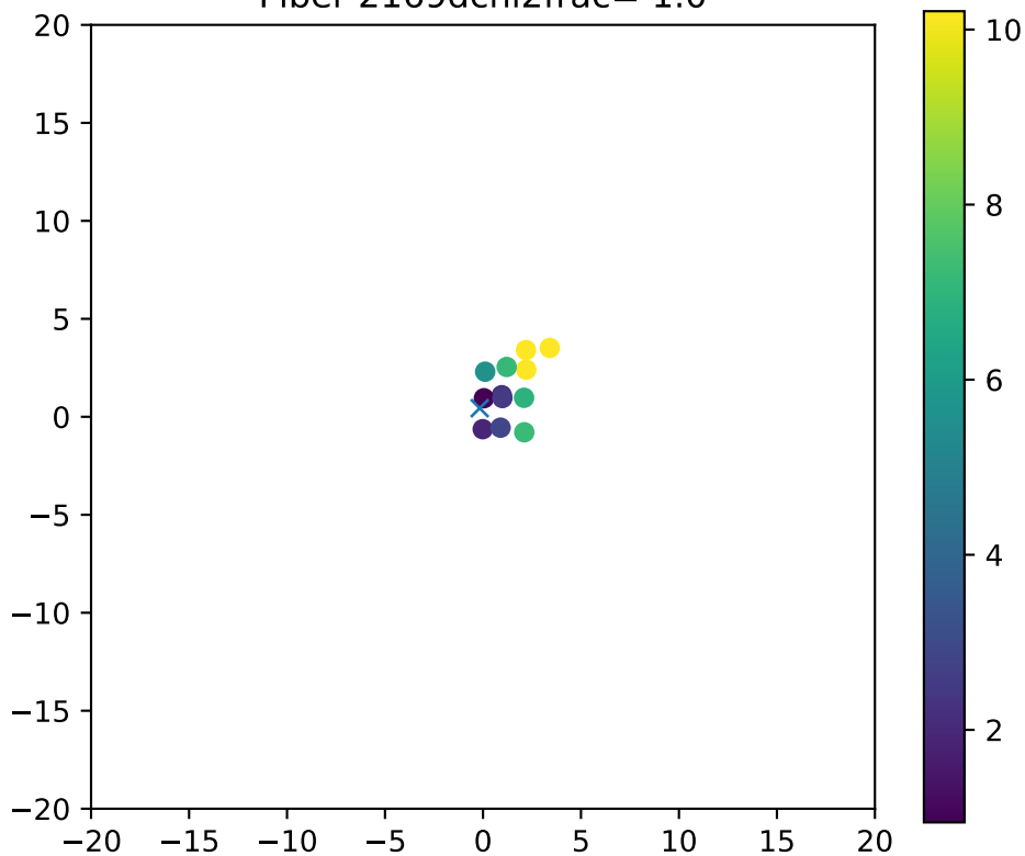
Fiber 2169dchi2frac= 1.0
