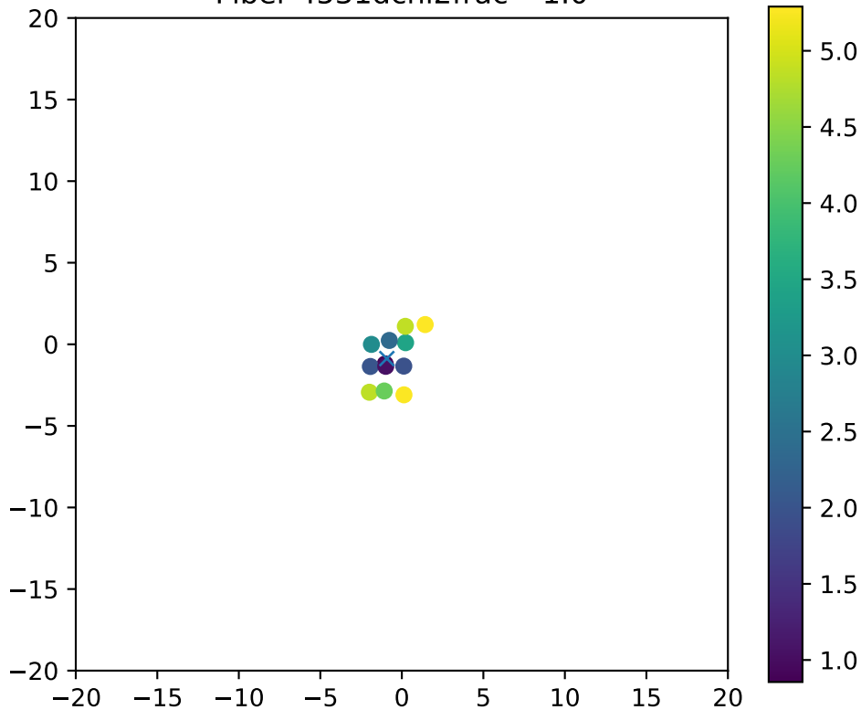
Fiber 4531dchi2frac= 1.0
