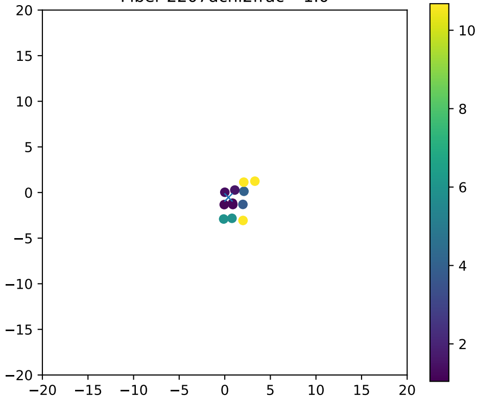
Fiber 2207dchi2frac= 1.0
