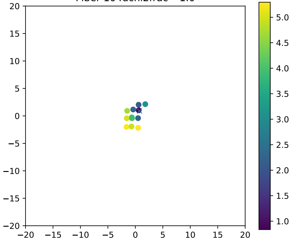
Fiber 104dchi2frac= 1.0
