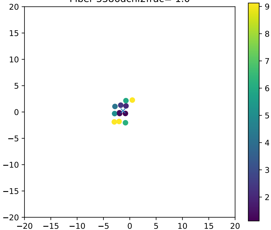
Fiber 3386dchi2frac= 1.0
