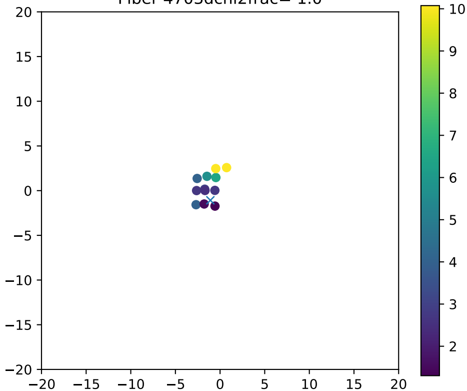
Fiber 4703dchi2frac= 1.0
