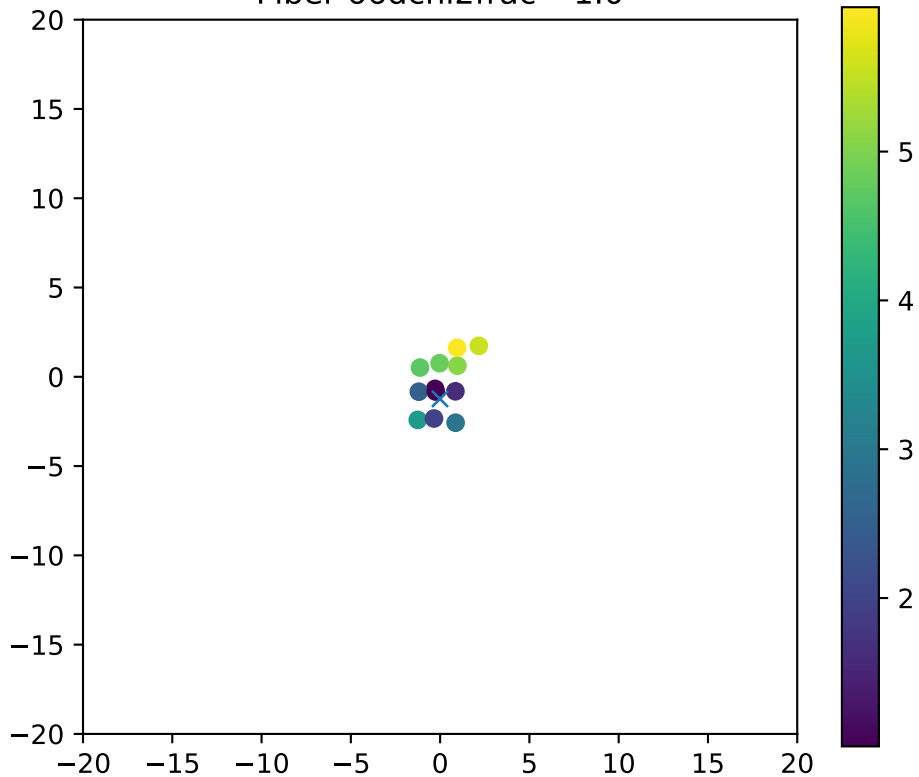
Fiber 66dchi2frac= 1.0
