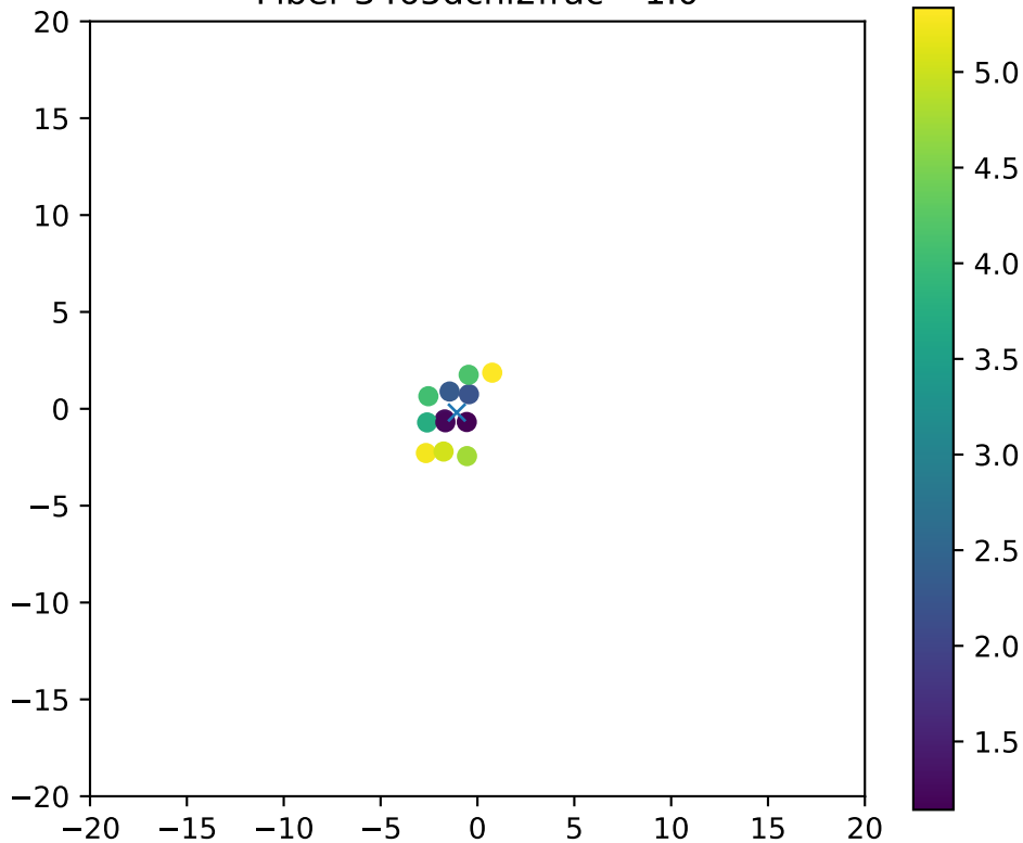
Fiber 3465dchi2frac= 1.0
