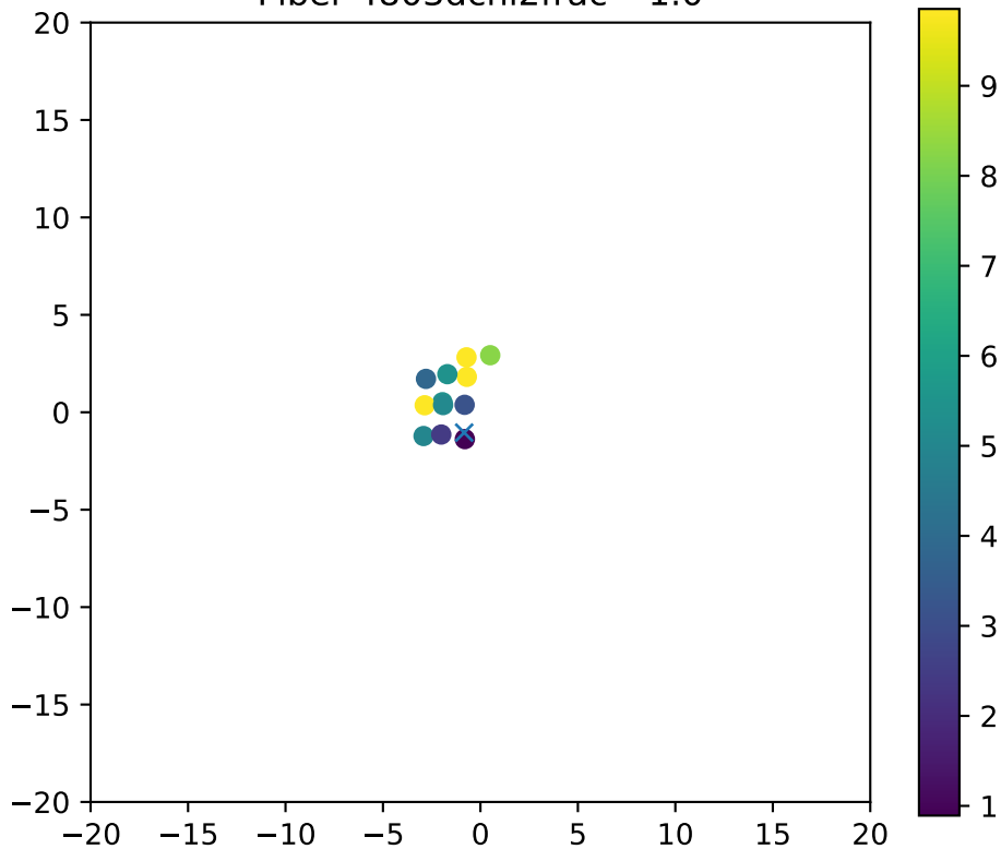
Fiber 4803dchi2frac= 1.0
