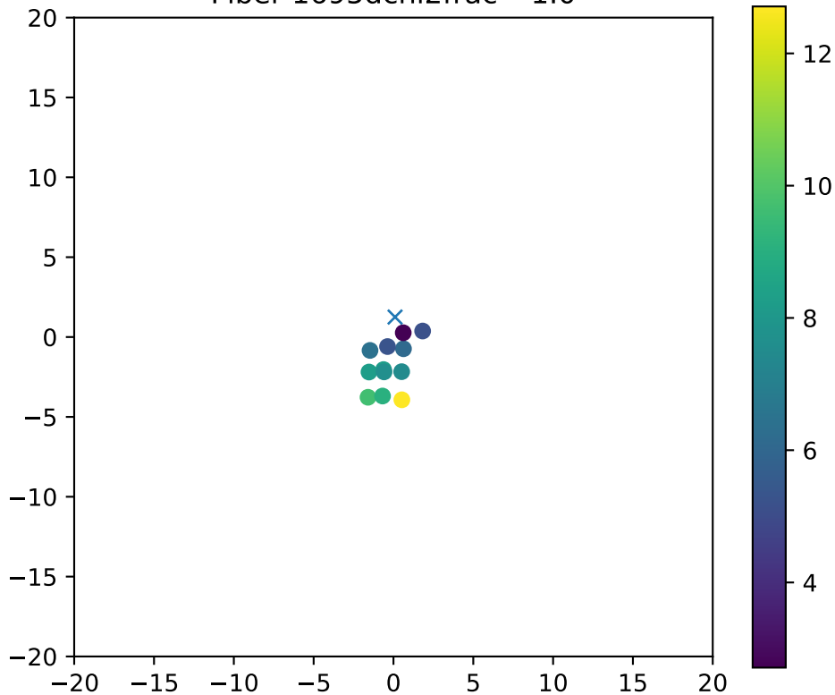
Fiber 1695dchi2frac= 1.0
