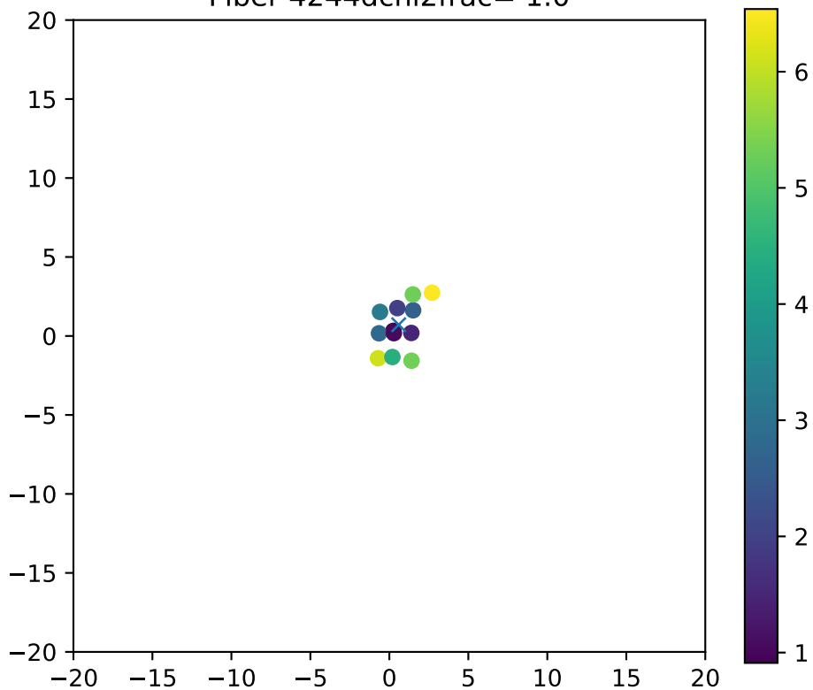
Fiber 4244dchi2frac= 1.0
