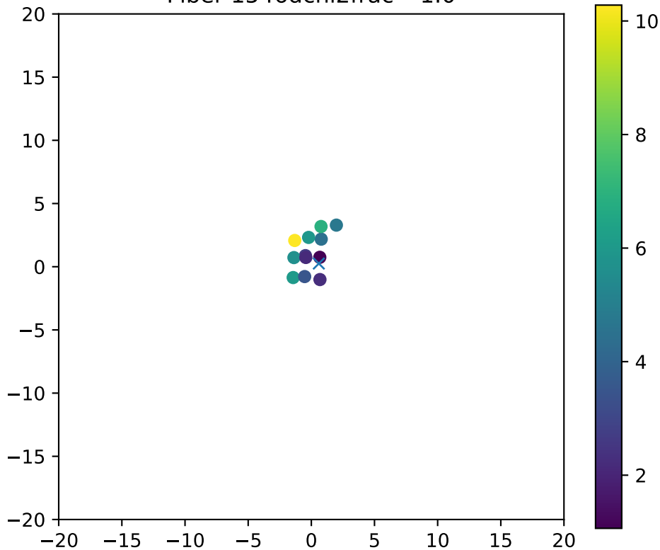
Fiber 1546dchi2frac= 1.0
