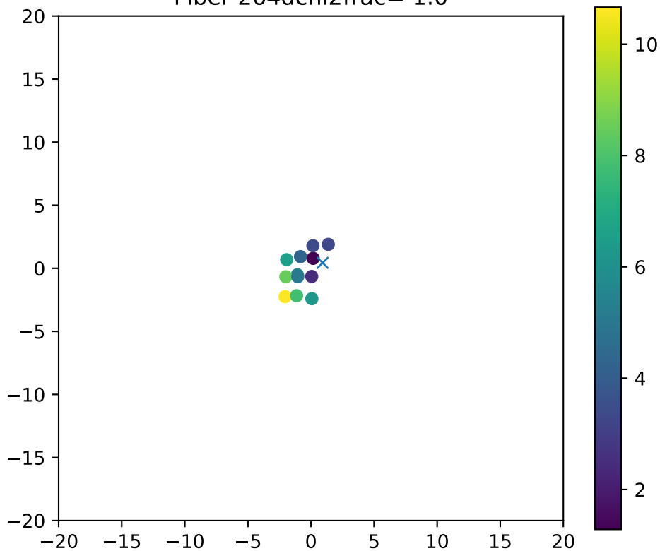
Fiber 264dchi2frac= 1.0
