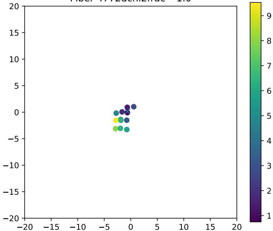
Fiber 4772dchi2frac= 1.0
