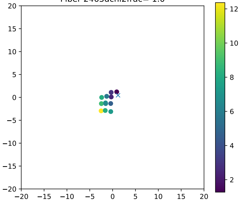
Fiber 2463dchi2frac= 1.0
