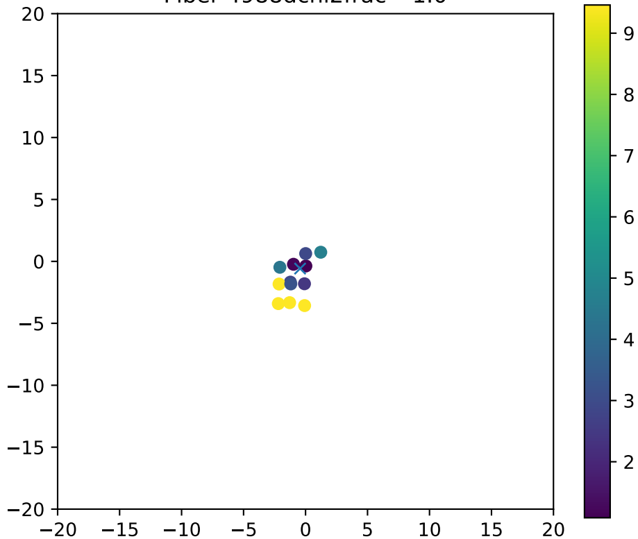
Fiber 4988dchi2frac= 1.0
