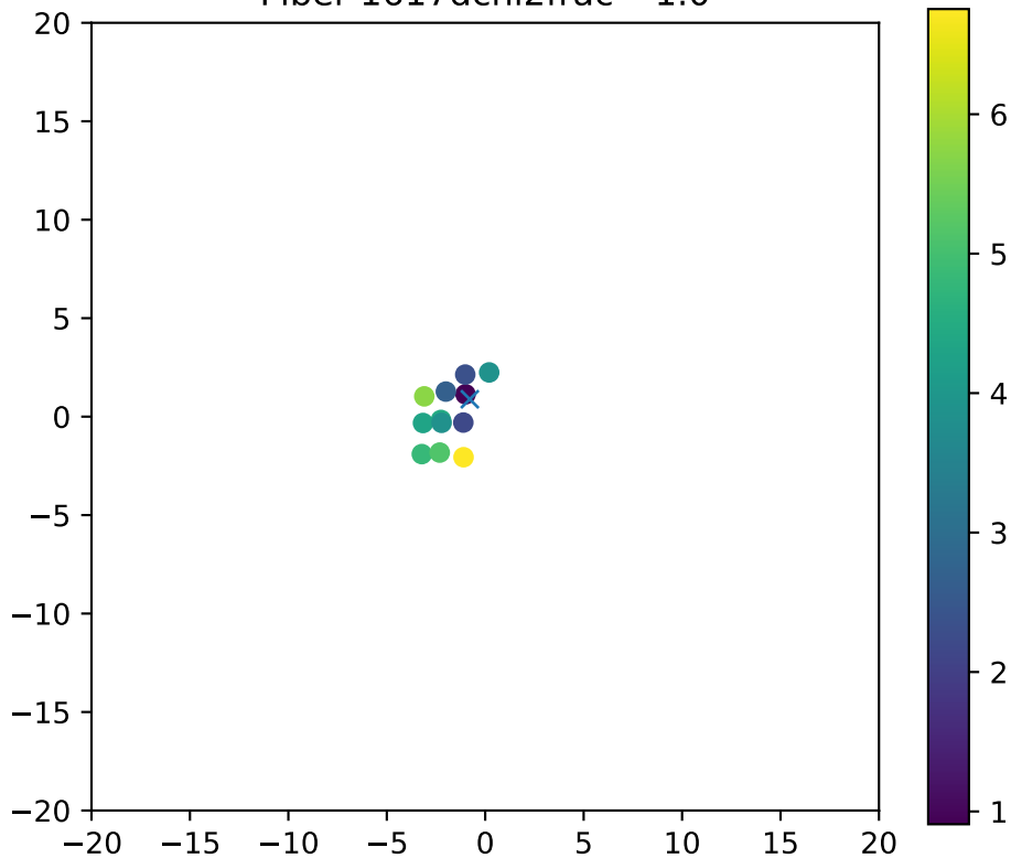
Fiber 1617dchi2frac= 1.0
