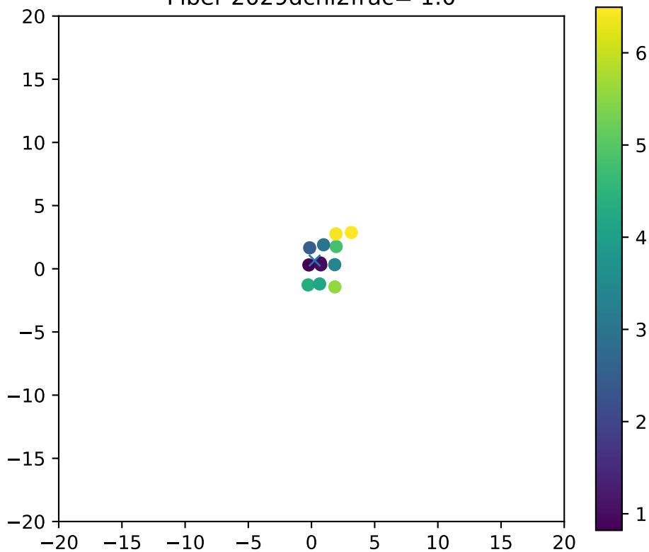
Fiber 2029dchi2frac= 1.0
