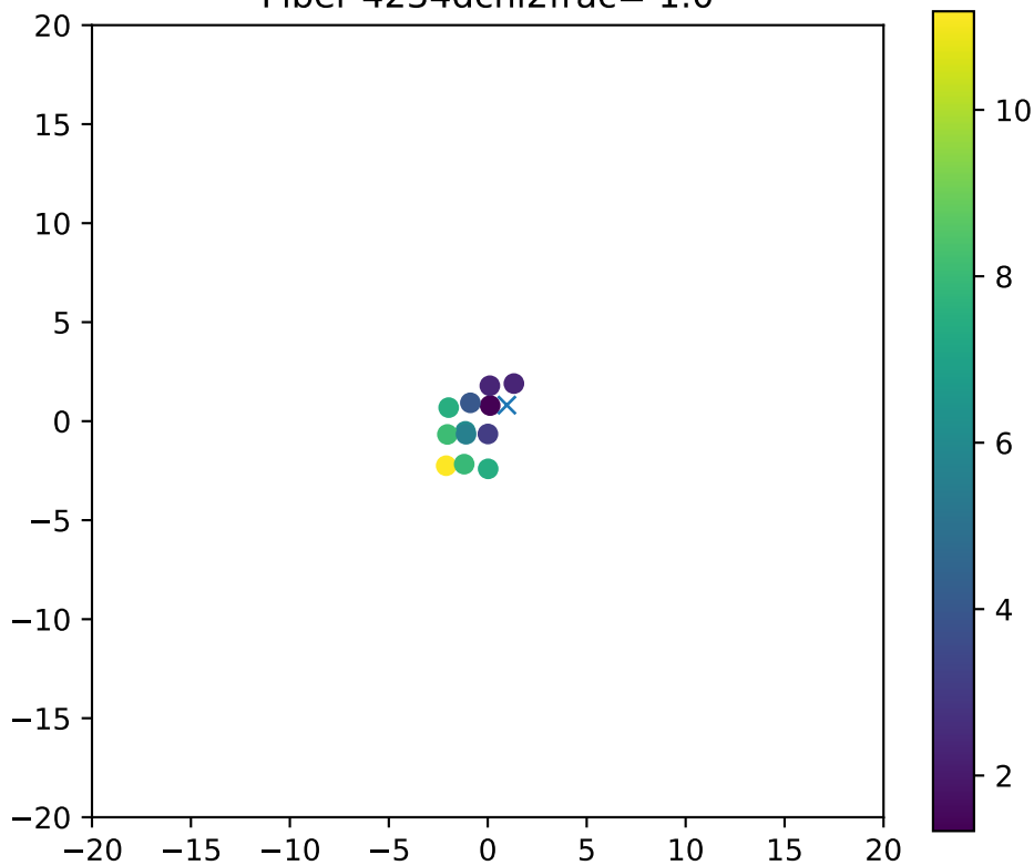
Fiber 4234dchi2frac= 1.0
