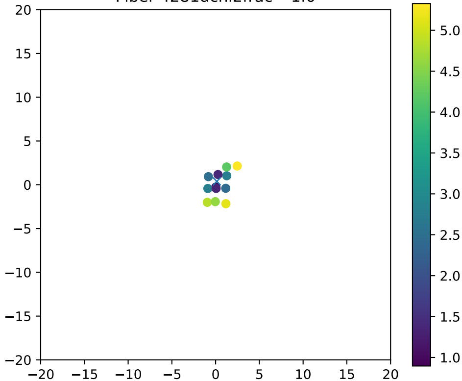
Fiber 4281dchi2frac= 1.0
