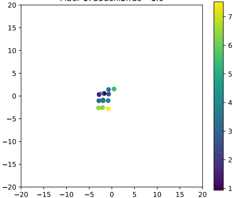
Fiber 1733dchi2frac= 1.0
