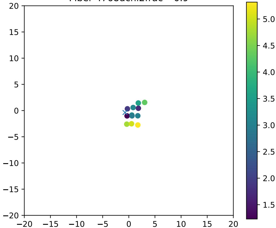
Fiber 4768dchi2frac= 0.9
