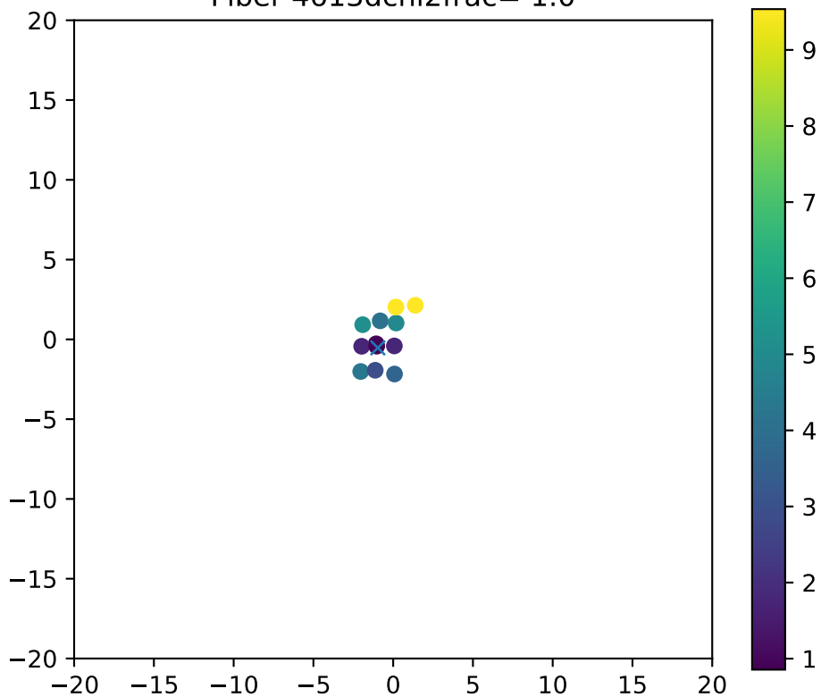
Fiber 4613dchi2frac= 1.0
