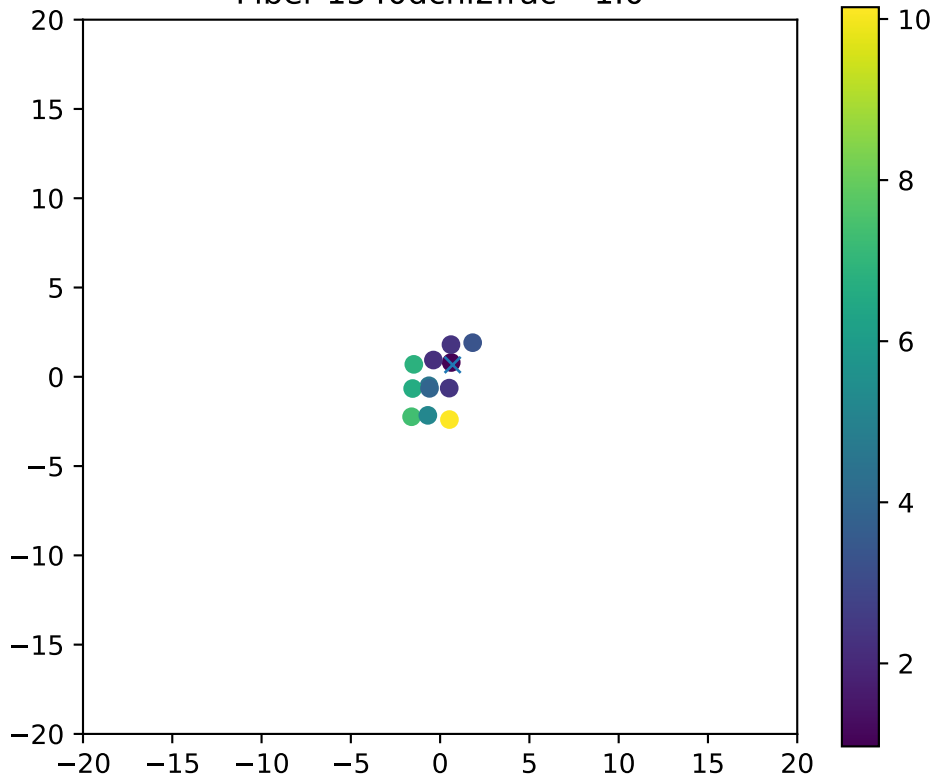
Fiber 1540dchi2frac= 1.0
