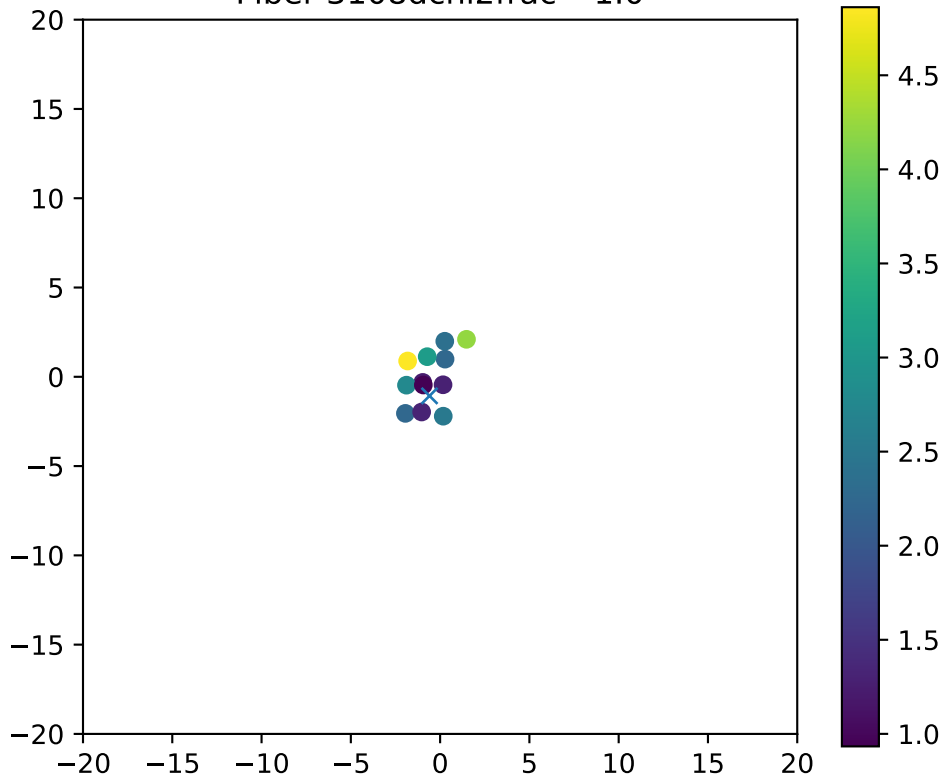
Fiber 3108dchi2frac= 1.0
