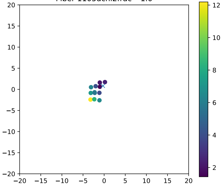
Fiber 1105dchi2frac= 1.0
