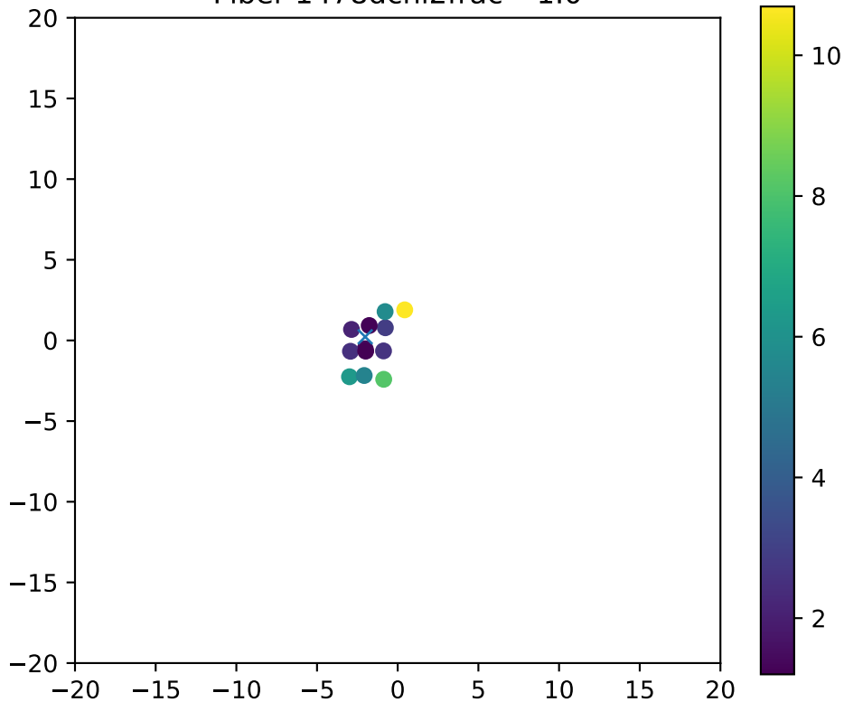
Fiber 1478dchi2frac= 1.0
