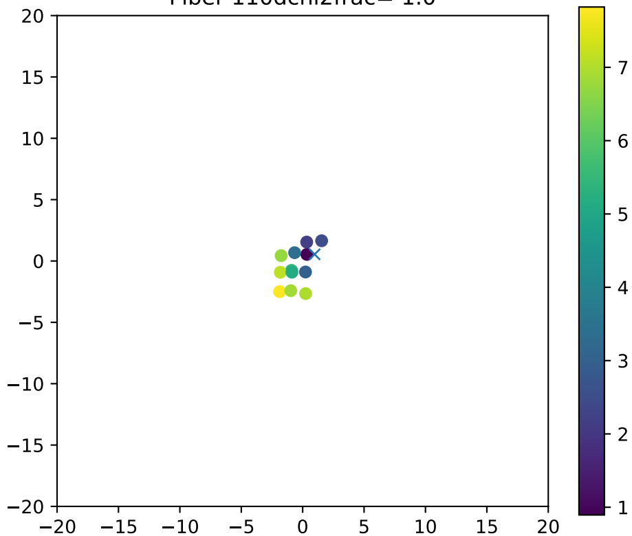
Fiber 110dchi2frac= 1.0
