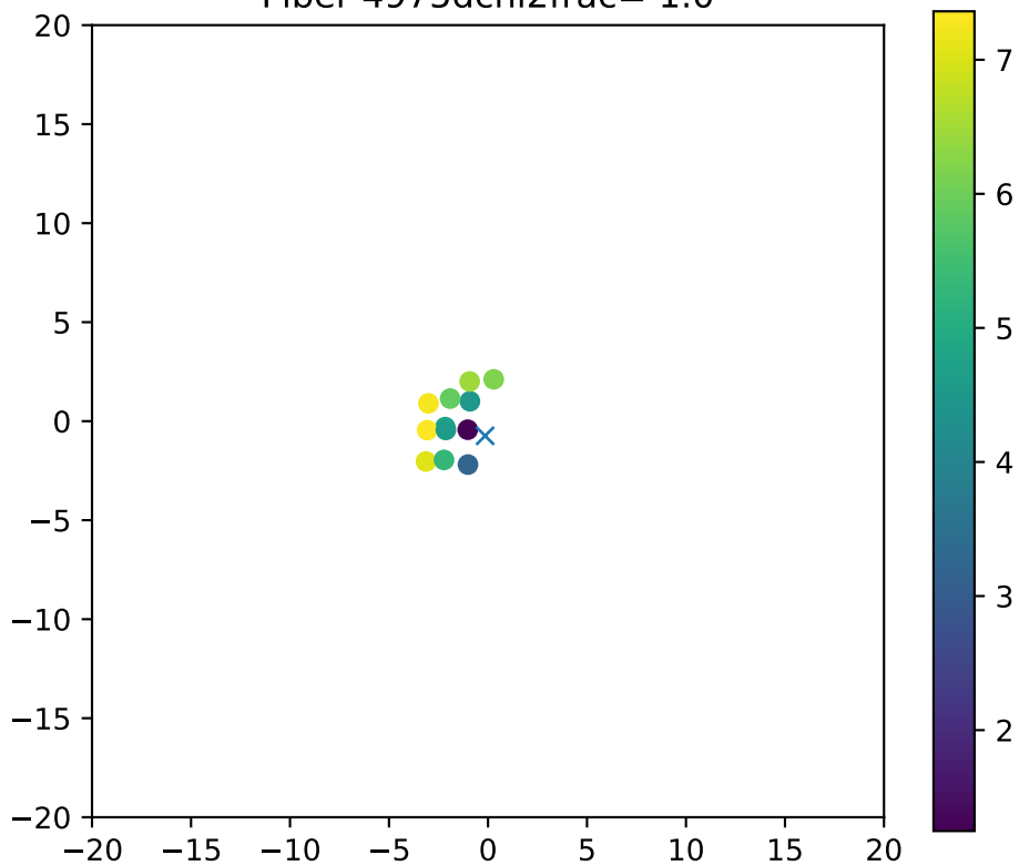
Fiber 4975dchi2frac= 1.0
