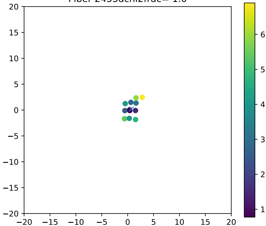
Fiber 2453dchi2frac= 1.0
