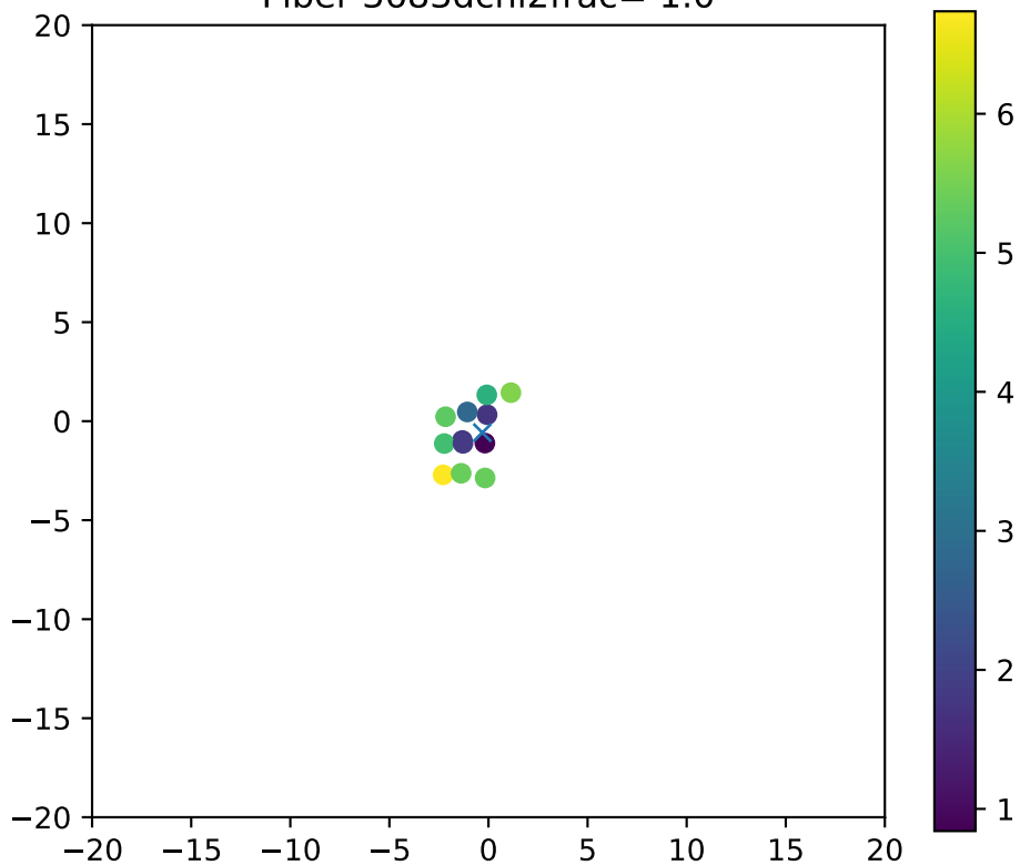
Fiber 3683dchi2frac= 1.0
