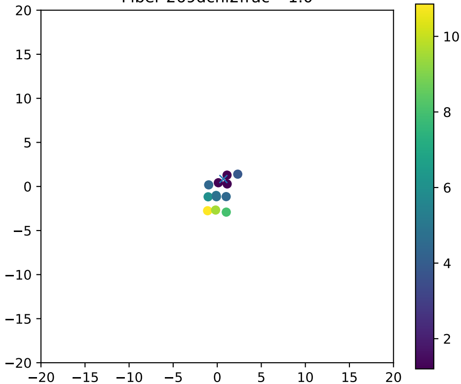
Fiber 269dchi2frac= 1.0
