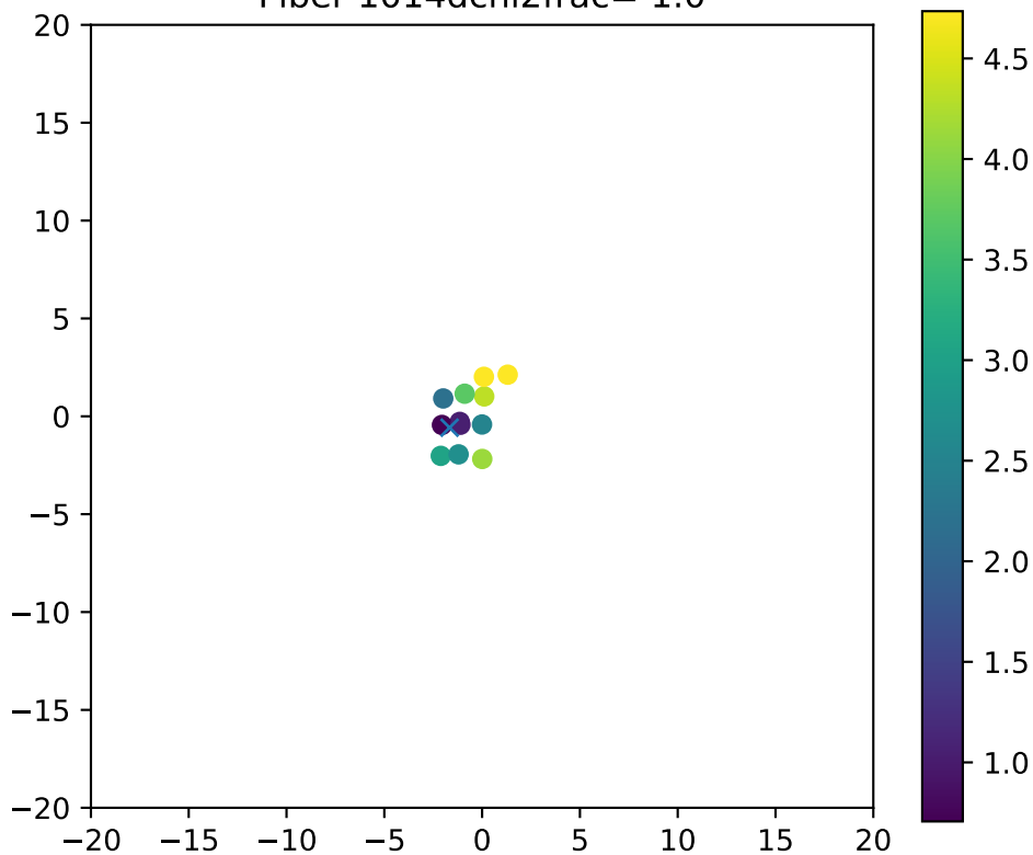
Fiber 1014dchi2frac= 1.0
