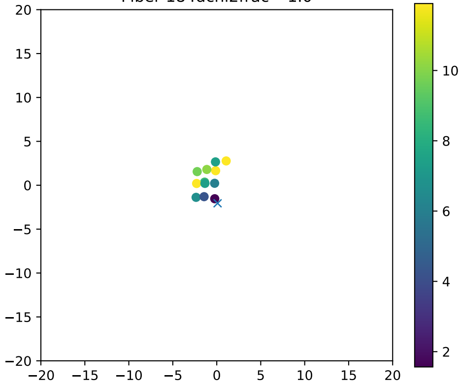
Fiber 184dchi2frac= 1.0
