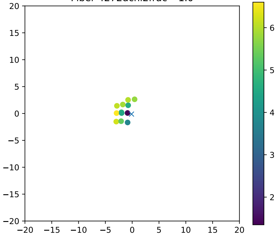
Fiber 4272dchi2frac= 1.0
