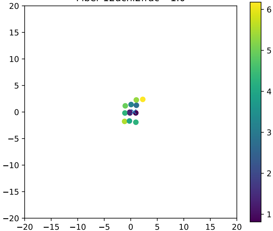
Fiber 12dchi2frac= 1.0
