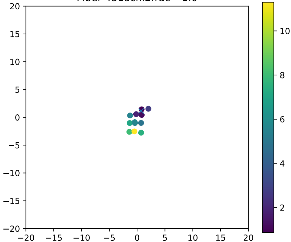
Fiber 431dchi2frac= 1.0
