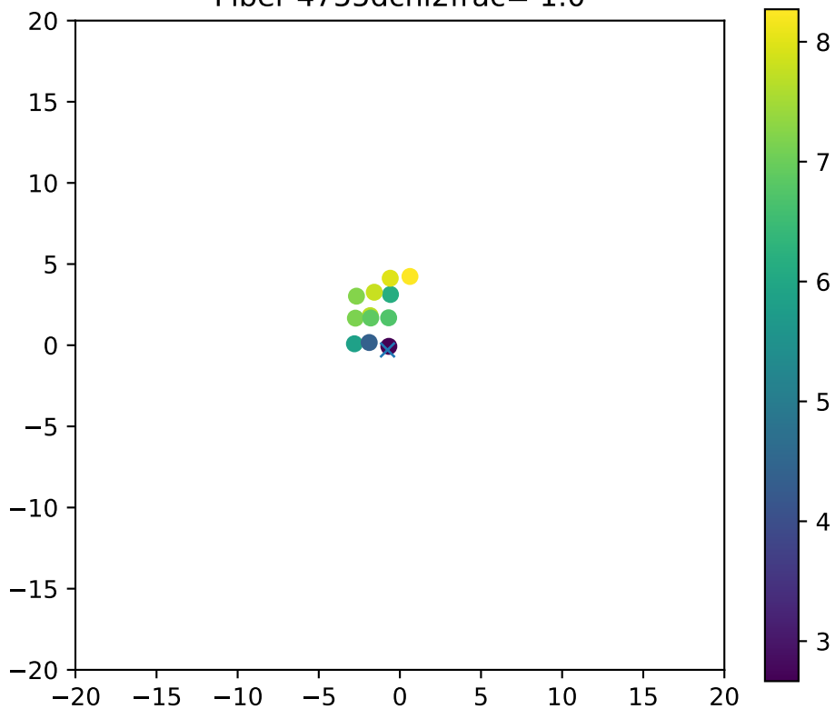
Fiber 4755dchi2frac= 1.0
