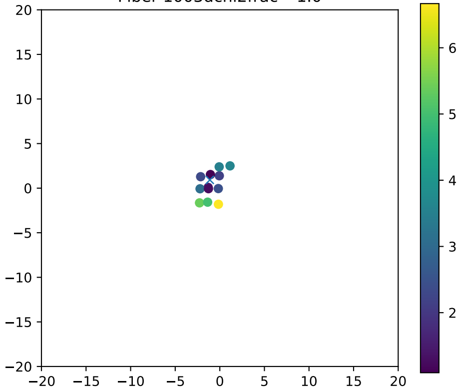
Fiber 1003dchi2frac= 1.0
