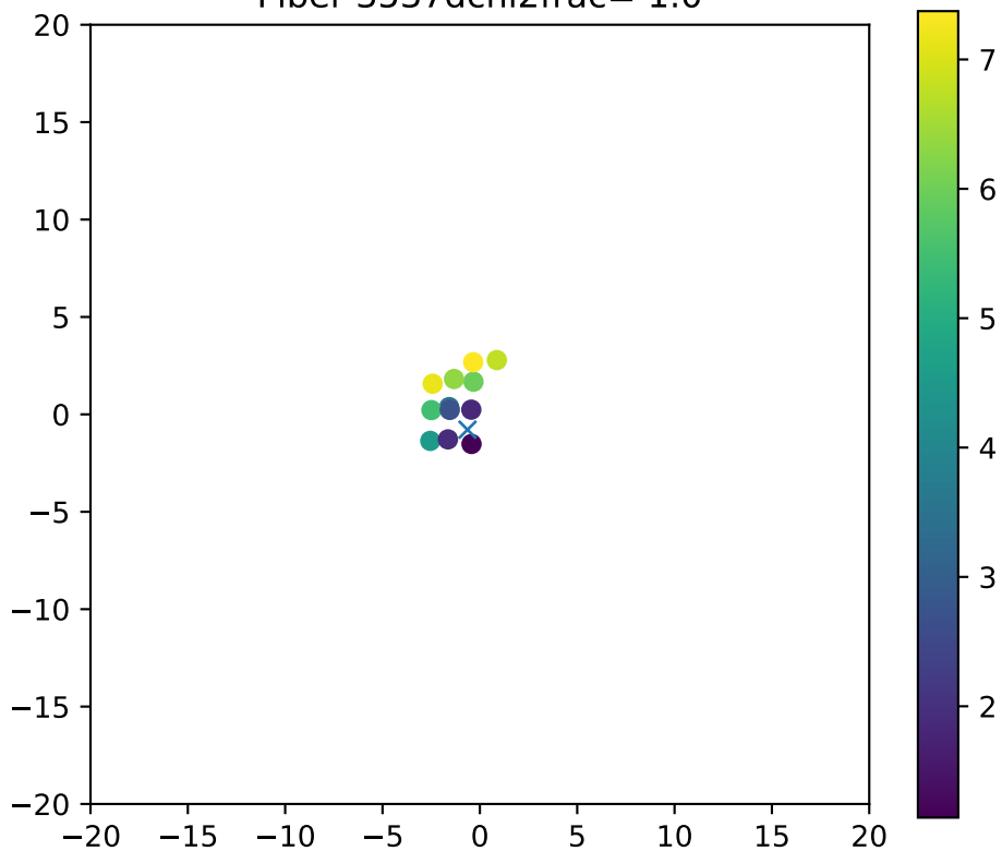
Fiber 3537dchi2frac= 1.0
