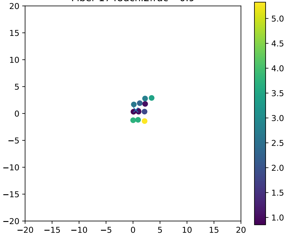
Fiber 1748dchi2frac= 0.9
