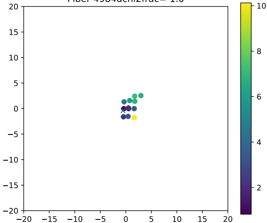
Fiber 4984dchi2frac= 1.0
