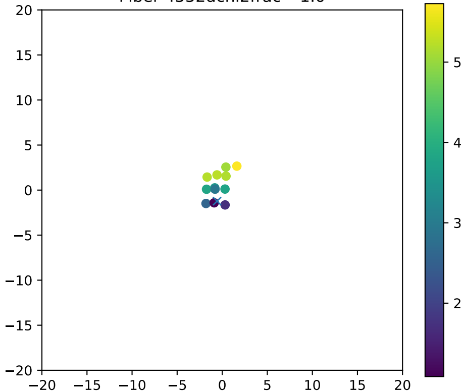
Fiber 4552dchi2frac= 1.0
