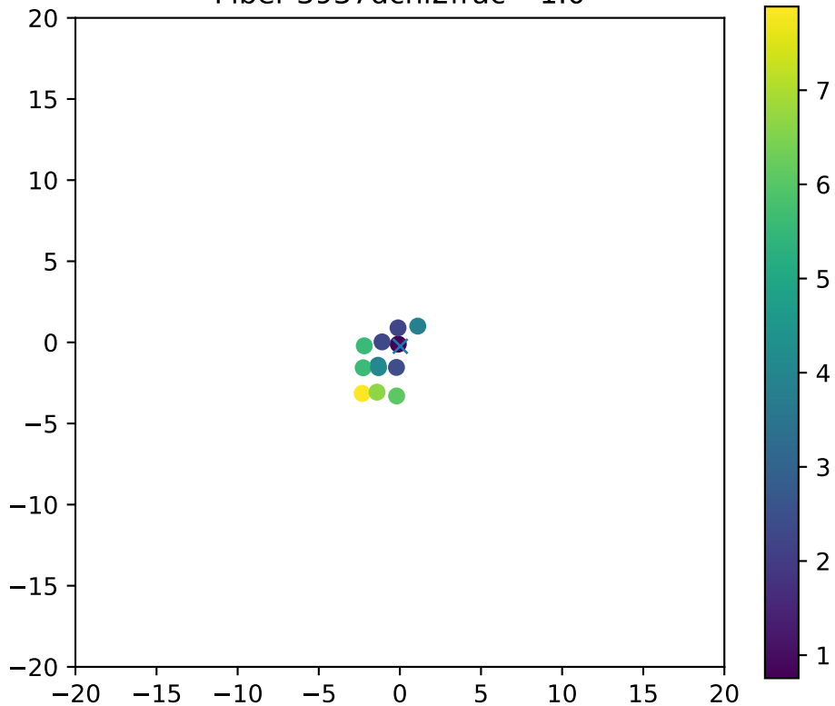
Fiber 3937dchi2frac= 1.0
