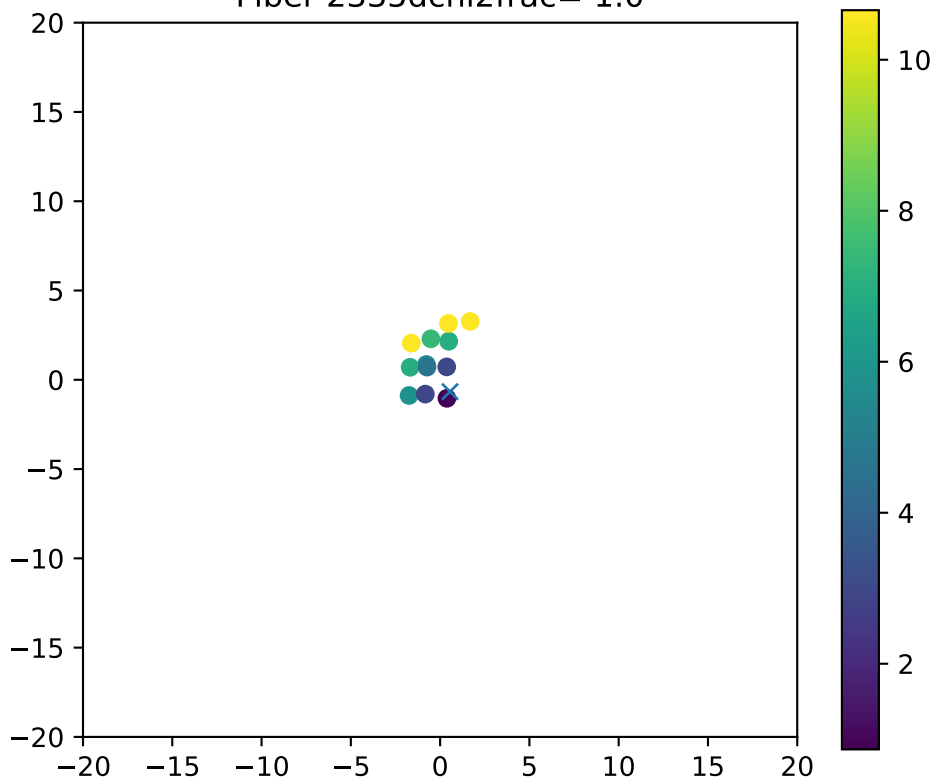
Fiber 2335dchi2frac= 1.0
