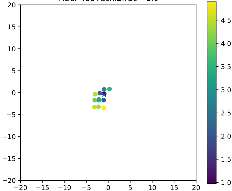
Fiber 4537dchi2frac= 1.0
