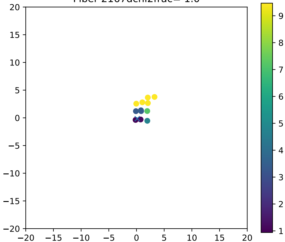
Fiber 2167dchi2frac= 1.0
