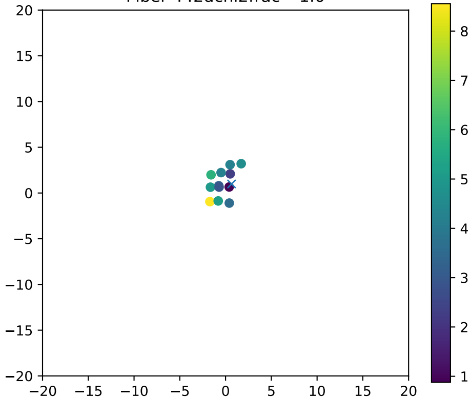
Fiber 442dchi2frac= 1.0
