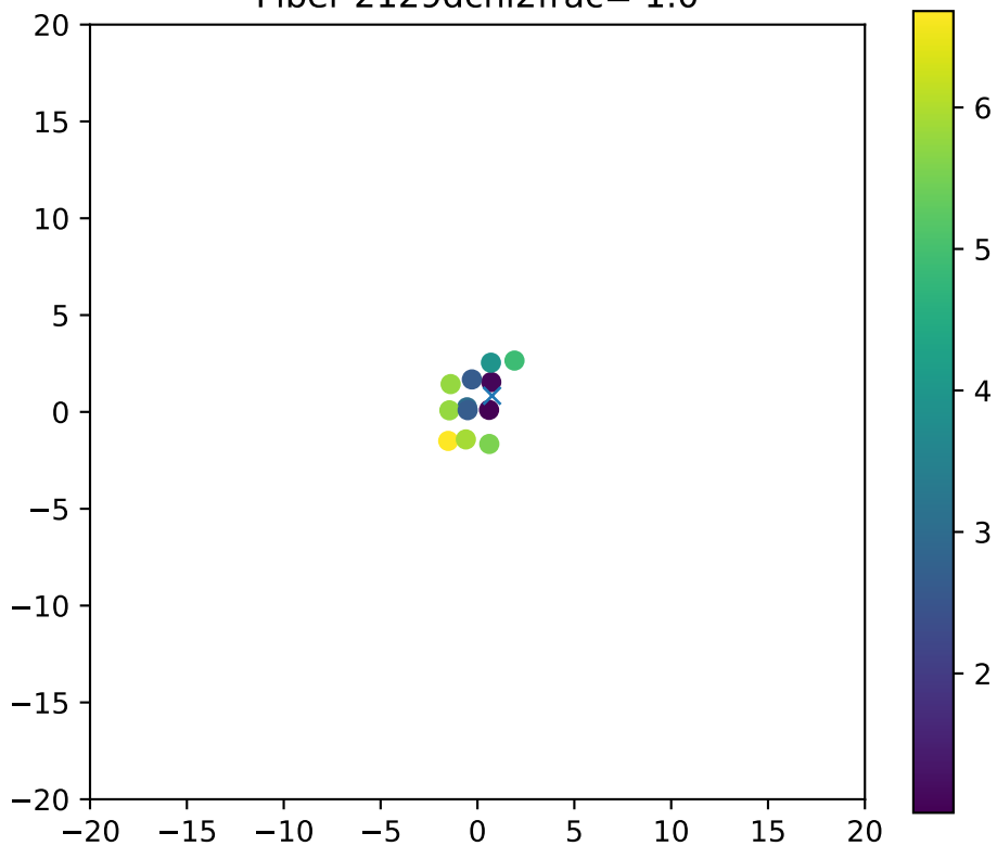
Fiber 2129dchi2frac= 1.0
