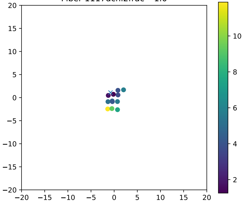
Fiber 1117dchi2frac= 1.0
