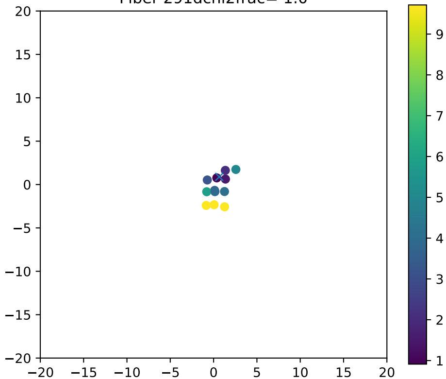
Fiber 291dchi2frac= 1.0
