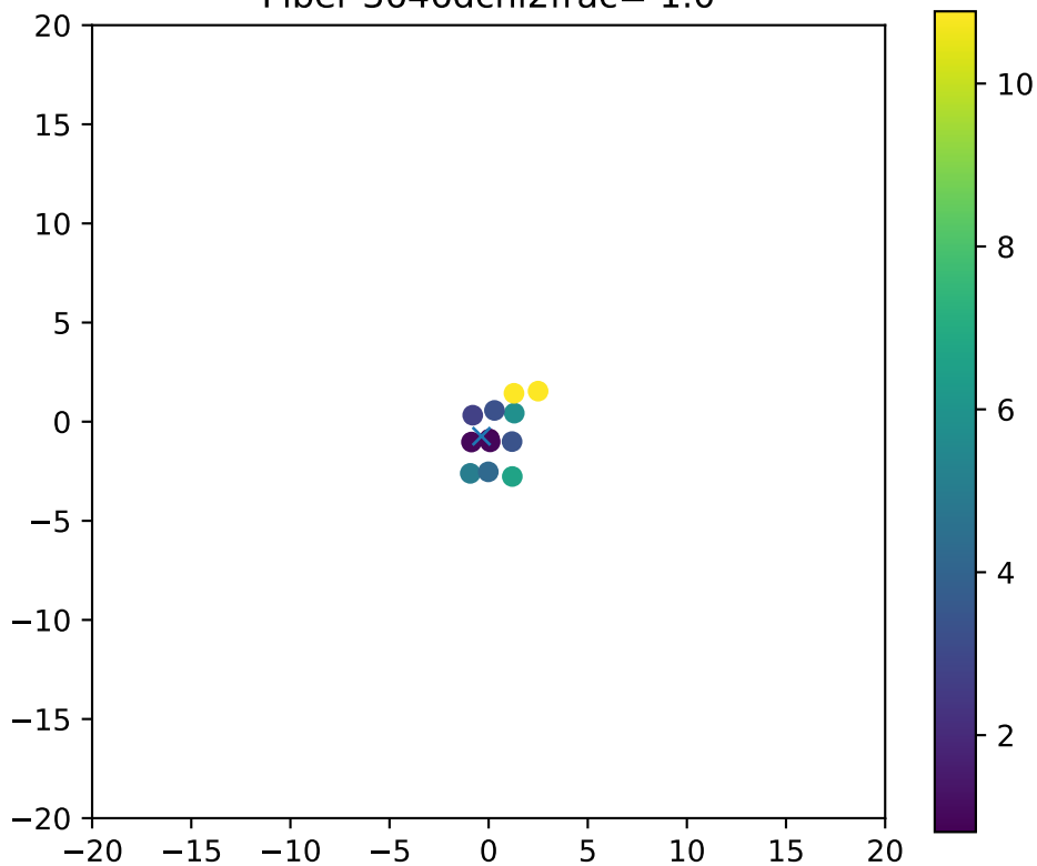
Fiber 3646dchi2frac= 1.0
