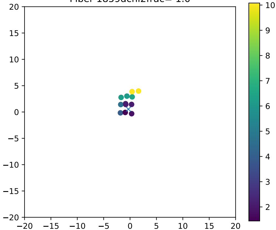
Fiber 1859dchi2frac= 1.0
