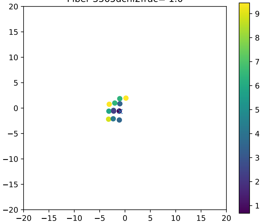
Fiber 3365dchi2frac= 1.0
