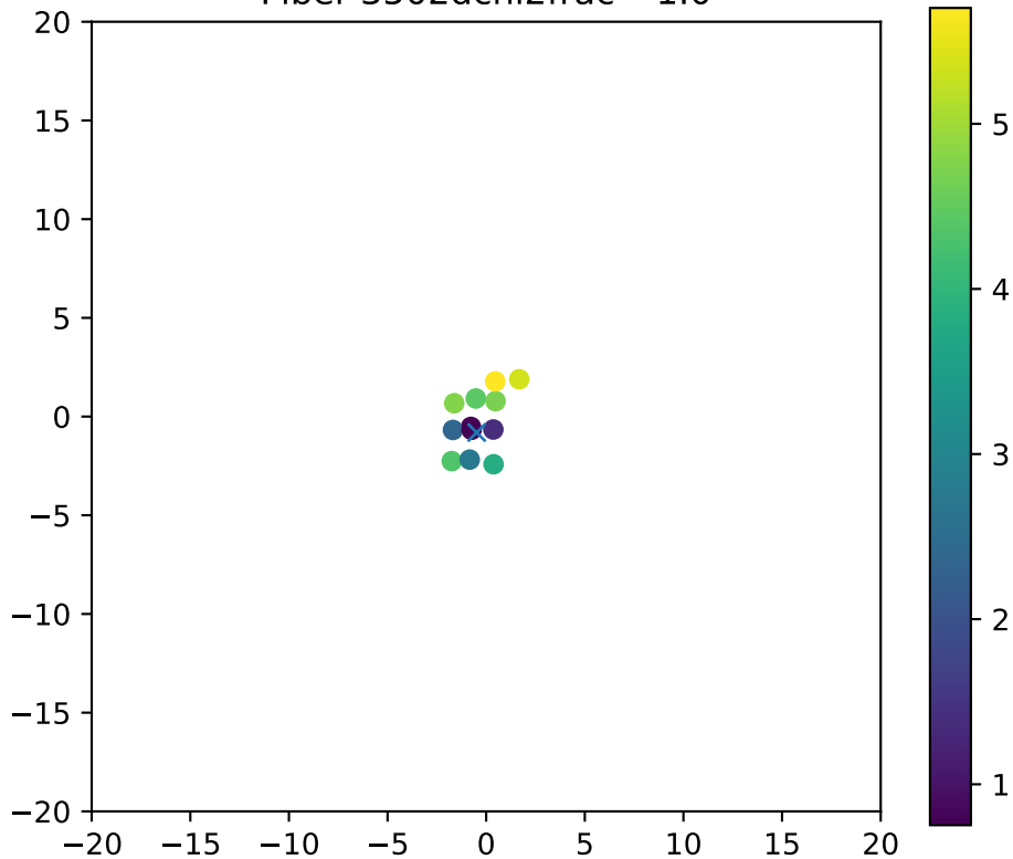
Fiber 3502dchi2frac= 1.0
