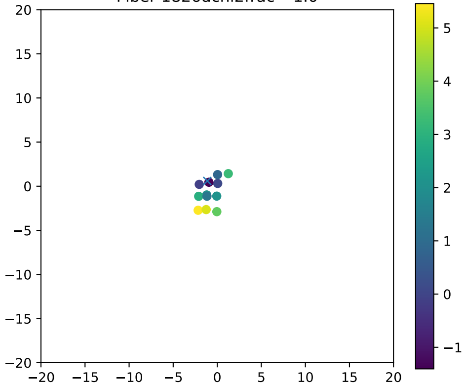
Fiber 1826dchi2frac= 1.0
