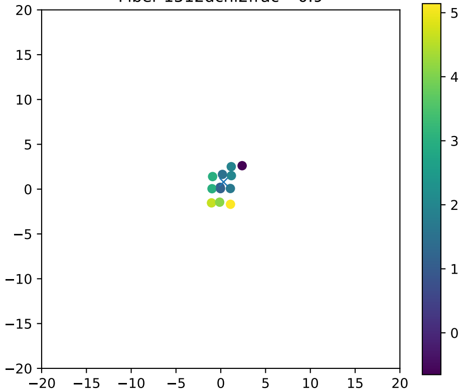
Fiber 1512dchi2frac= 0.9
