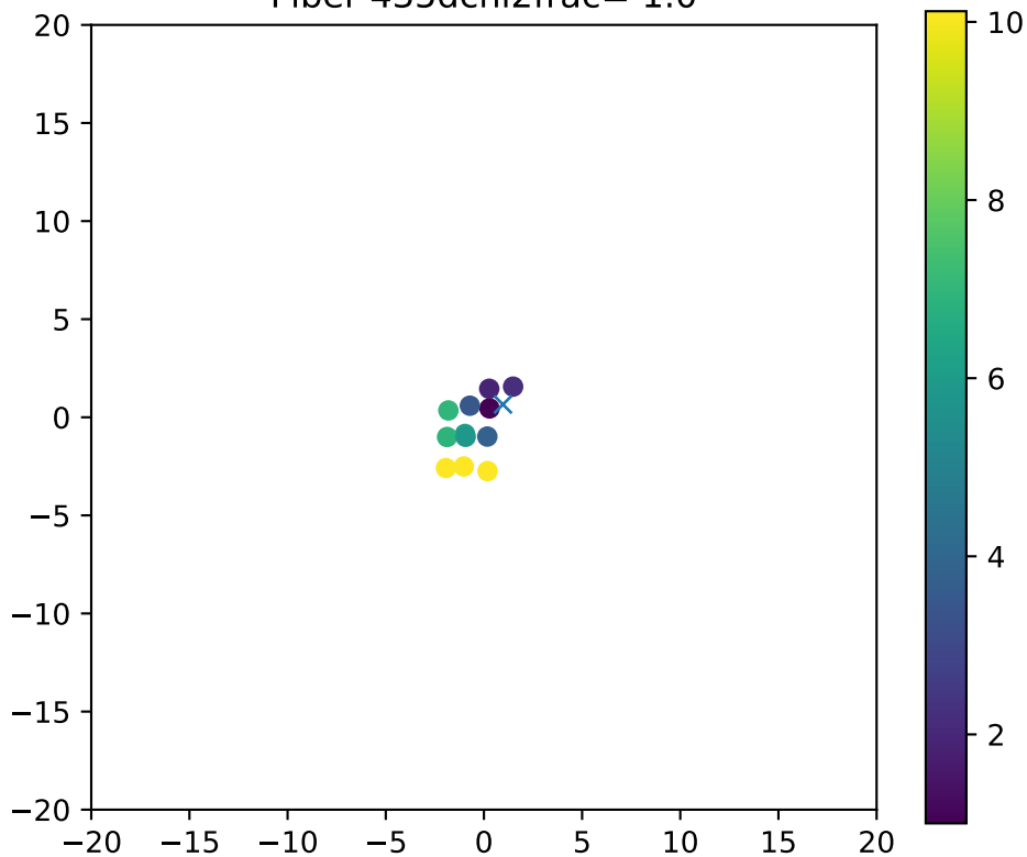
Fiber 435dchi2frac= 1.0
