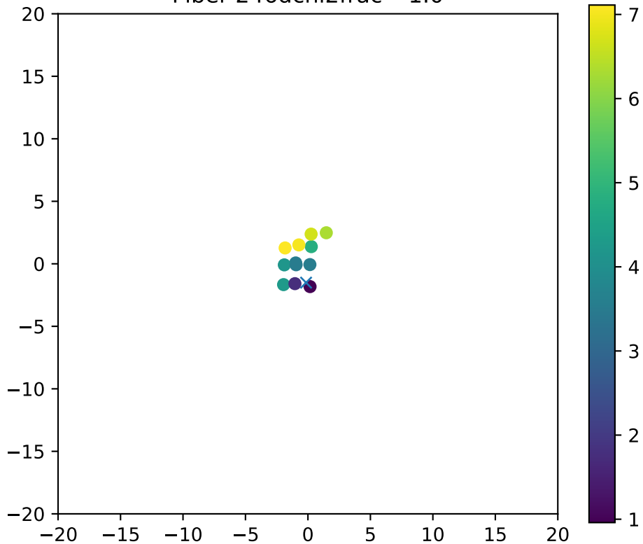
Fiber 246dchi2frac= 1.0
