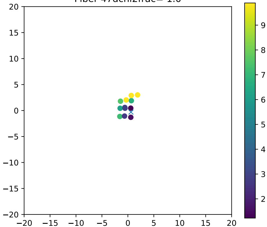
Fiber 47dchi2frac= 1.0
