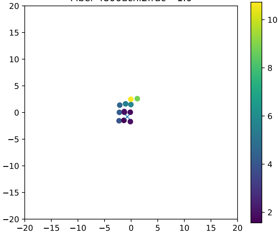
Fiber 4806dchi2frac= 1.0
