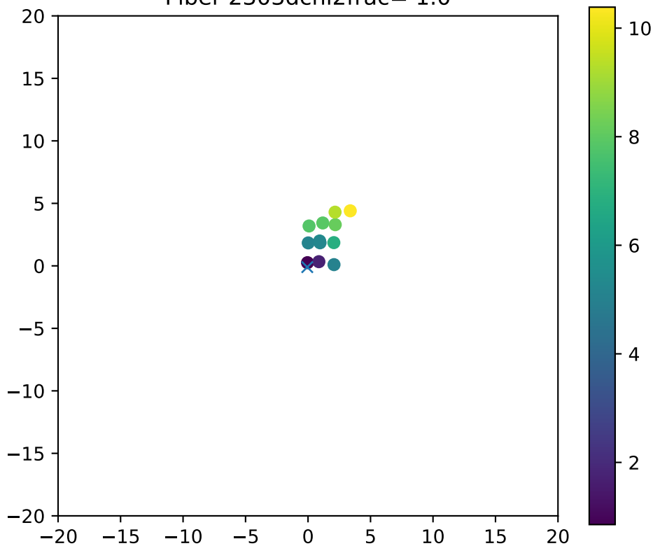
Fiber 2303dchi2frac= 1.0
