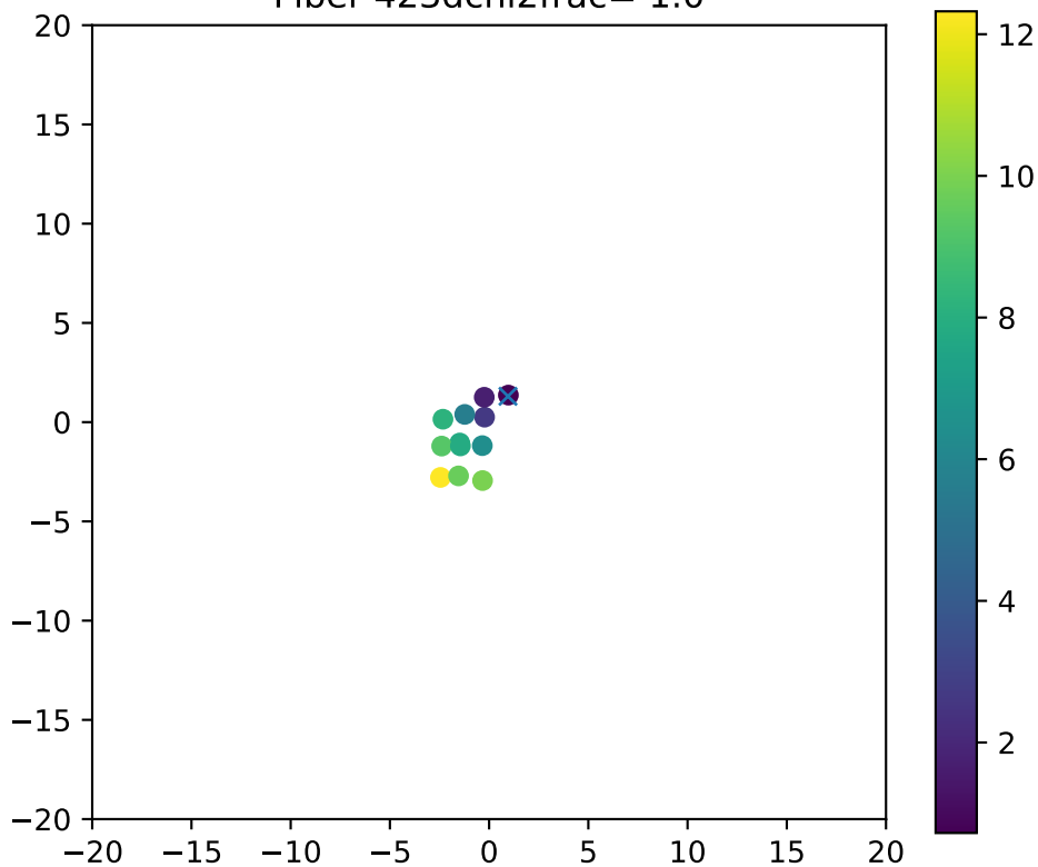
Fiber 423dchi2frac= 1.0
