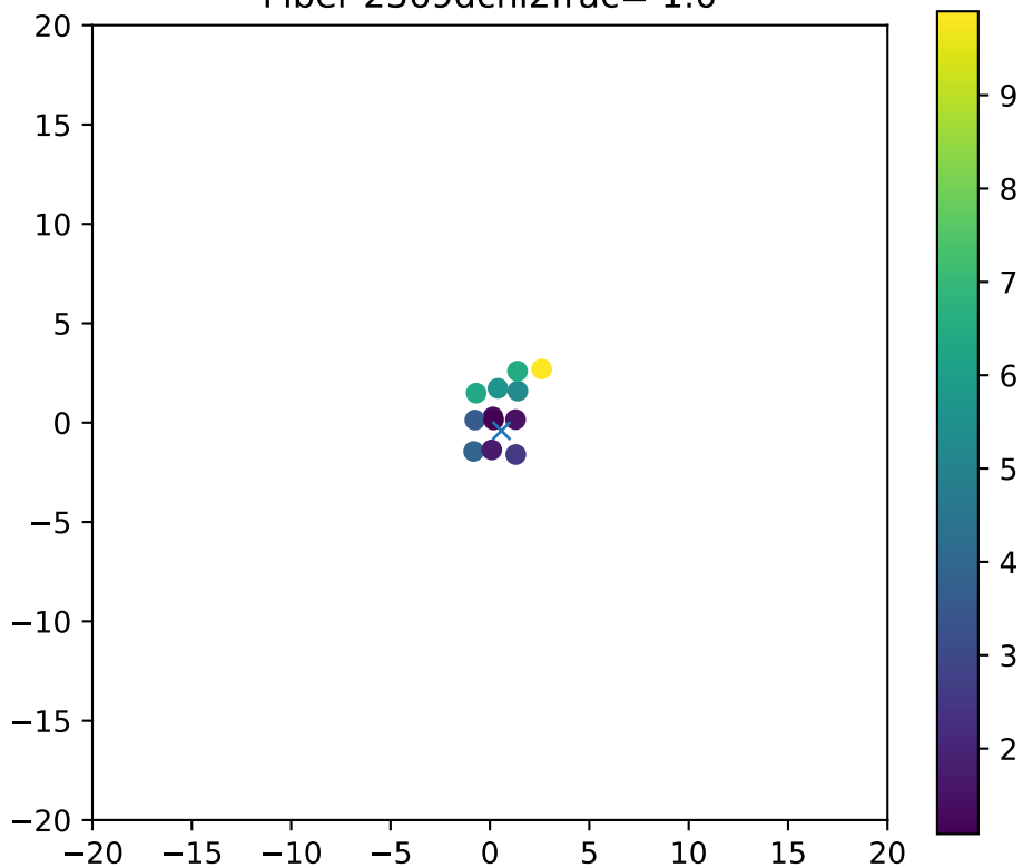
Fiber 2369dchi2frac= 1.0
