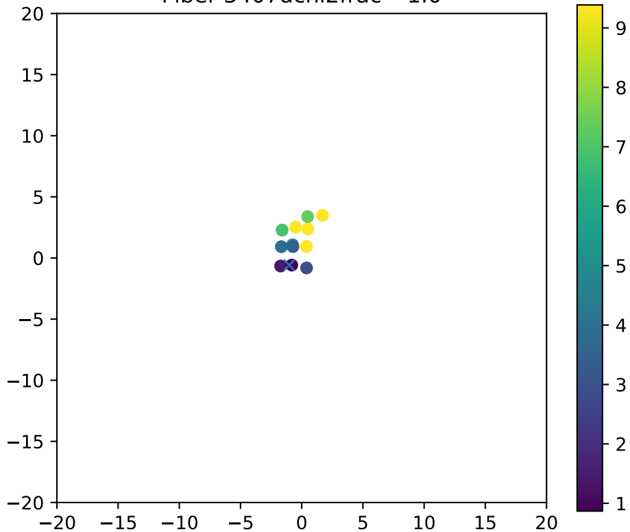
Fiber 3407dchi2frac= 1.0
