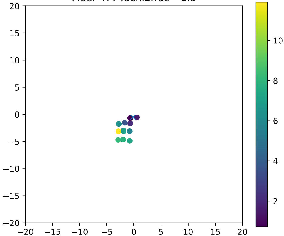
Fiber 4774dchi2frac= 1.0
