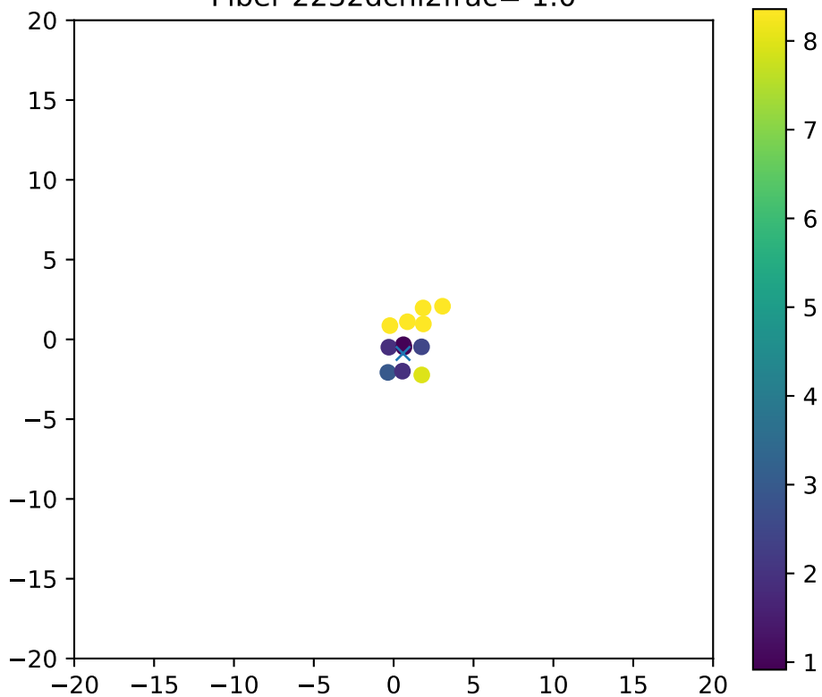
Fiber 2232dchi2frac= 1.0
