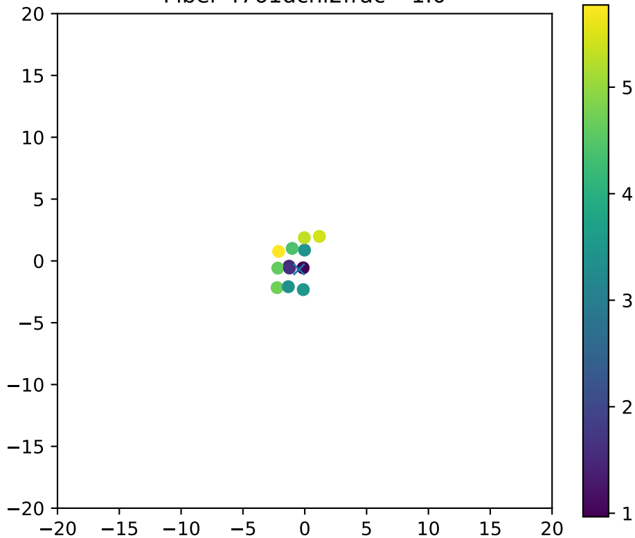
Fiber 4761dchi2frac= 1.0
