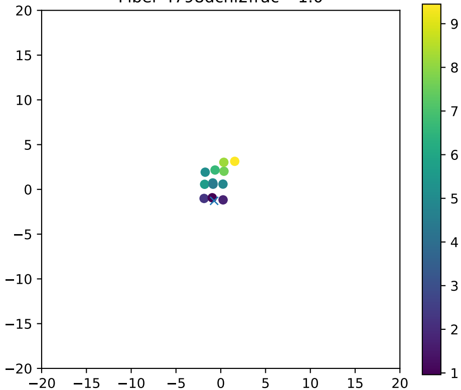
Fiber 4798dchi2frac= 1.0
