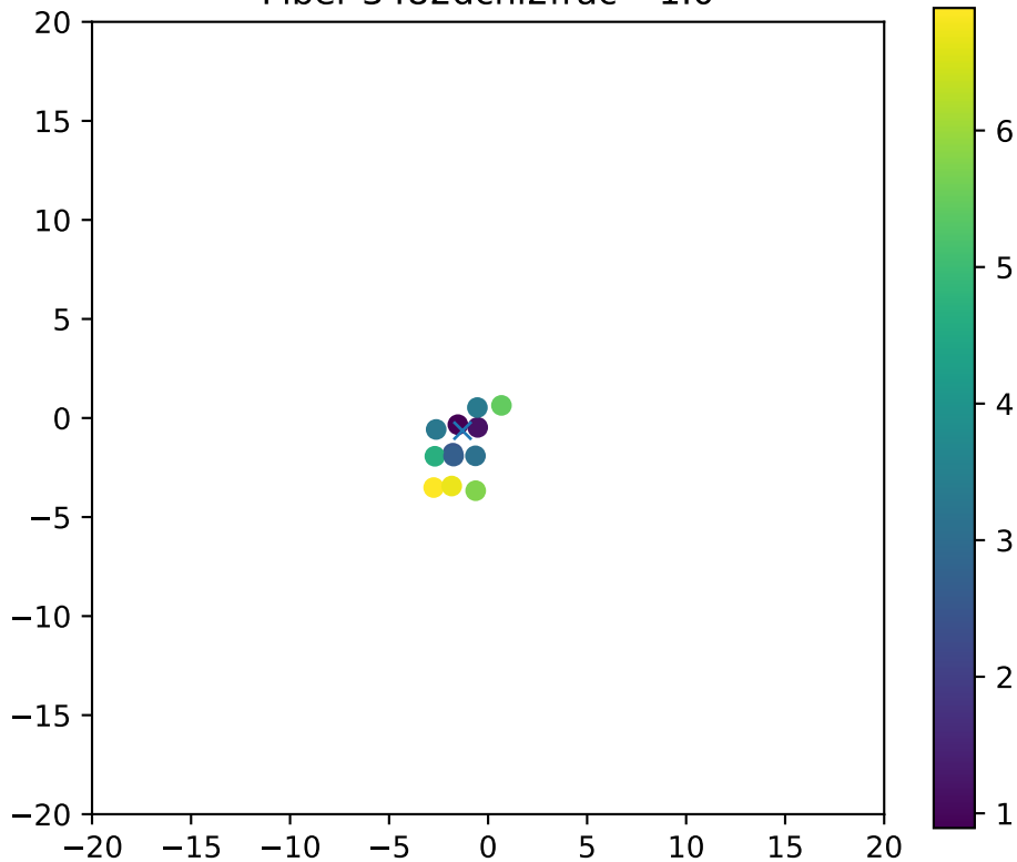
Fiber 3482dchi2frac= 1.0
