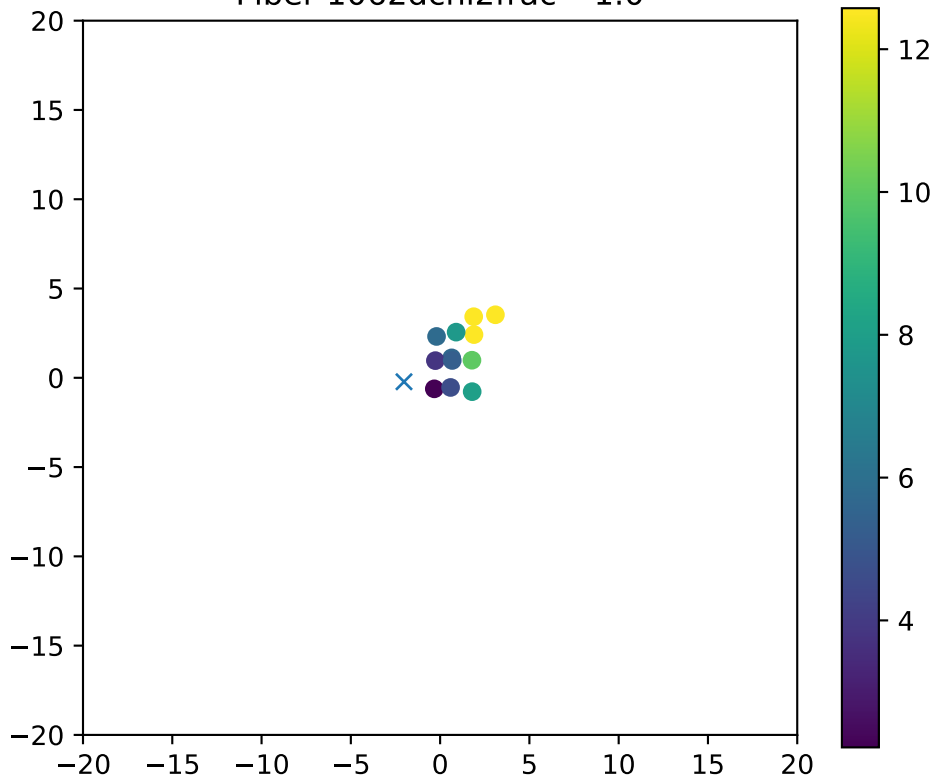
Fiber 1062dchi2frac= 1.0
