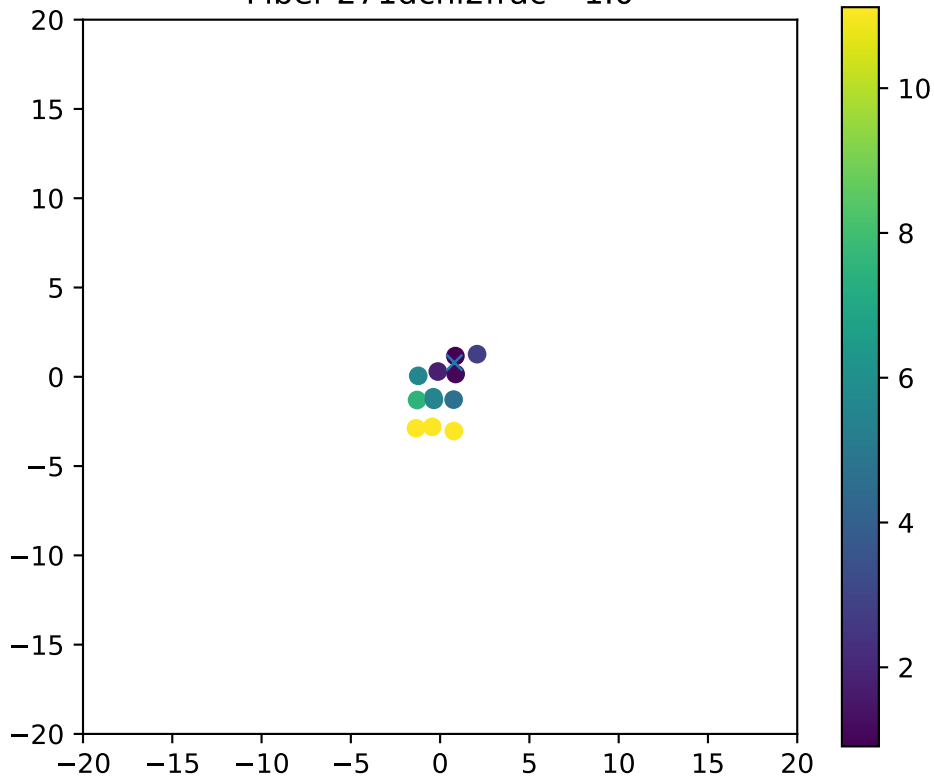
Fiber 271dchi2frac= 1.0
