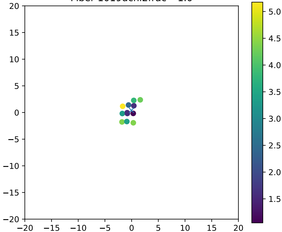
Fiber 1019dchi2frac= 1.0
