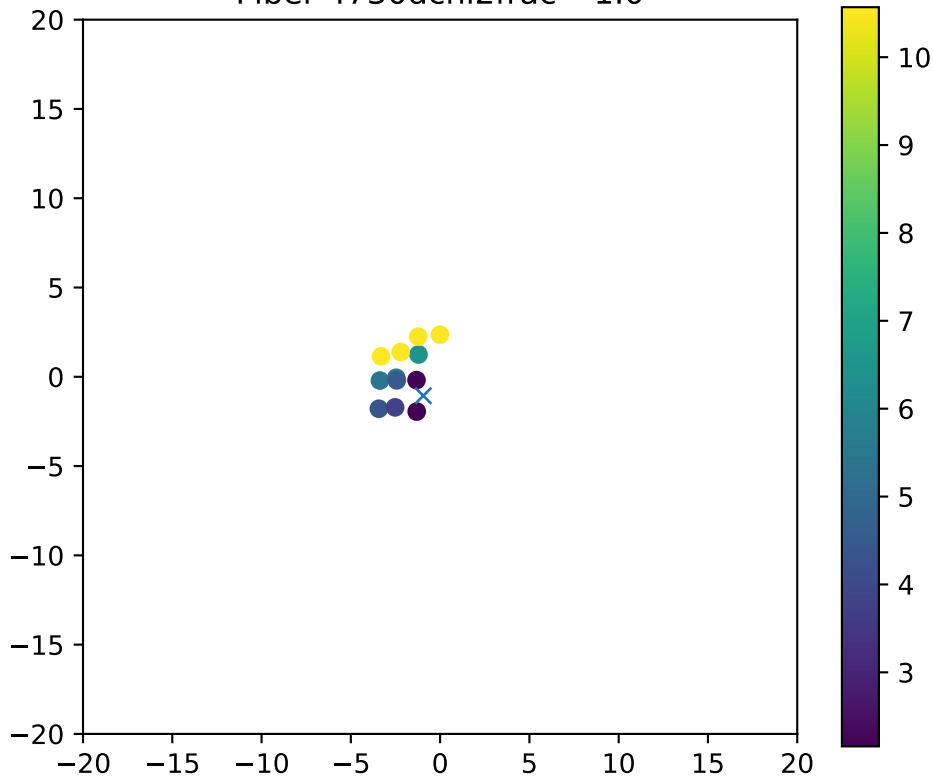
Fiber 4730dchi2frac= 1.0
