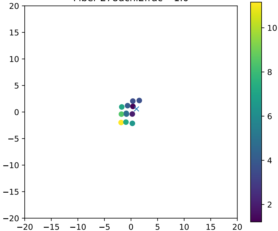
Fiber 278dchi2frac= 1.0
