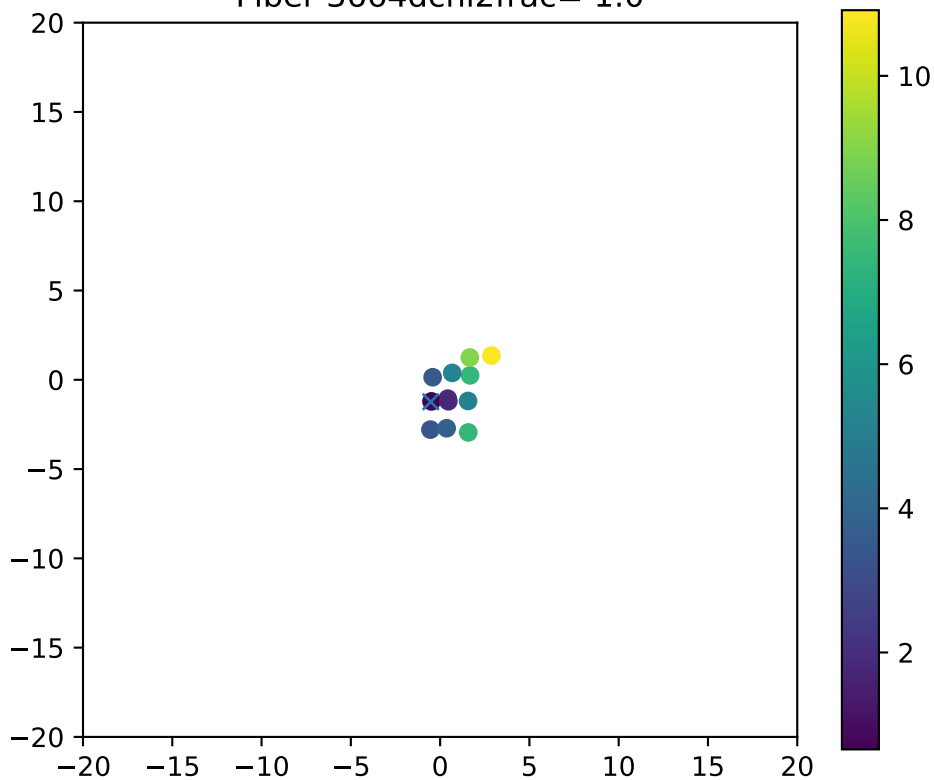
Fiber 3664dchi2frac= 1.0
