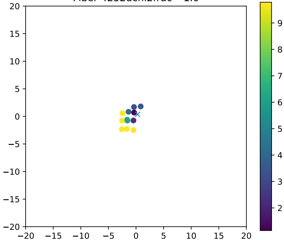
Fiber 4252dchi2frac= 1.0
