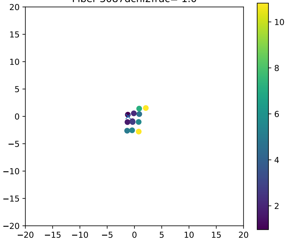
Fiber 3087dchi2frac= 1.0
