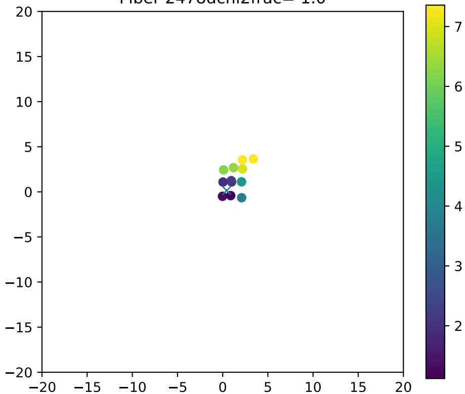
Fiber 2478dchi2frac= 1.0
