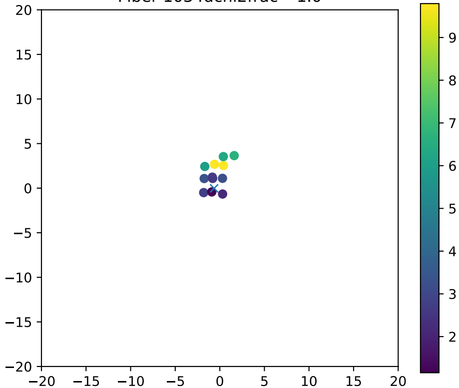
Fiber 1034dchi2frac= 1.0
