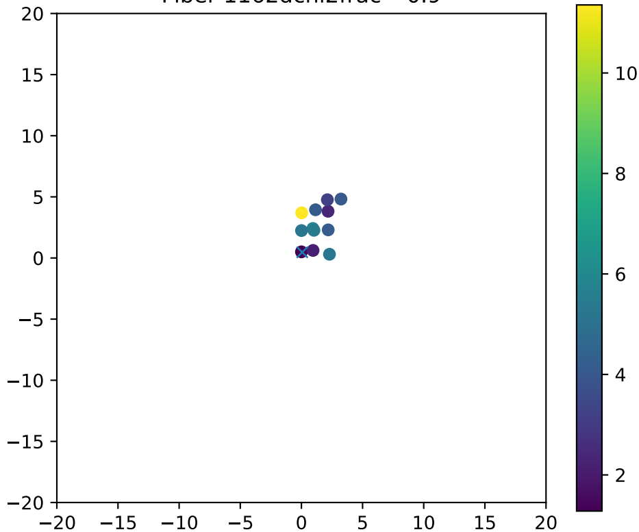
Fiber 1162dchi2frac= 0.9
