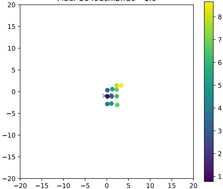
Fiber 3649dchi2frac= 1.0
