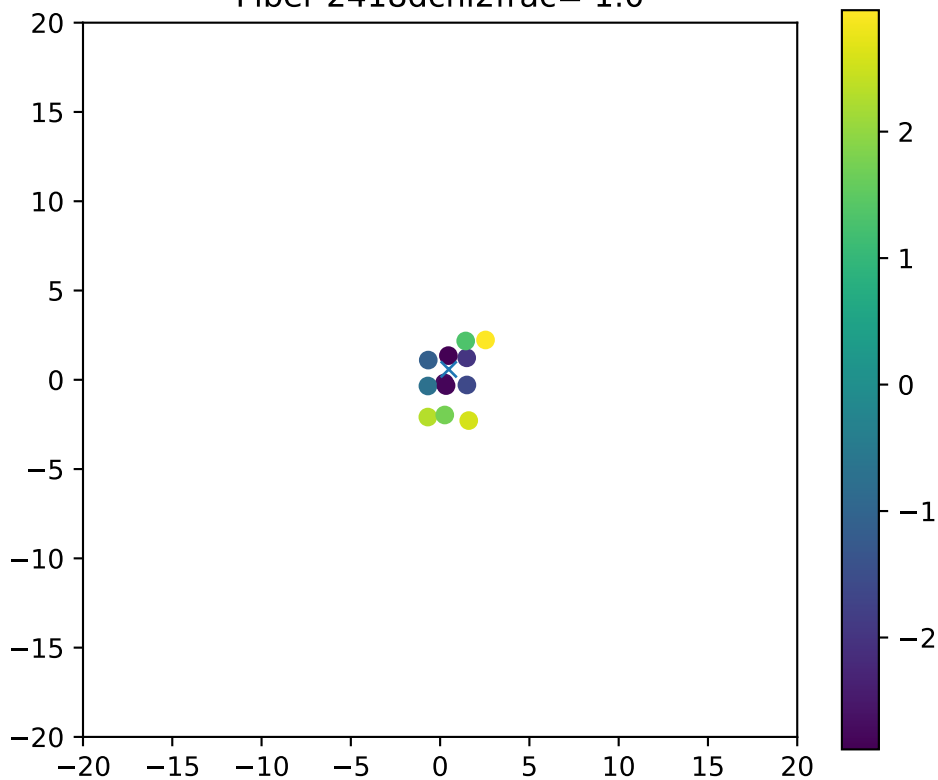
Fiber 2418dchi2frac= 1.0
