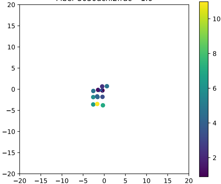
Fiber 3030dchi2frac= 1.0
