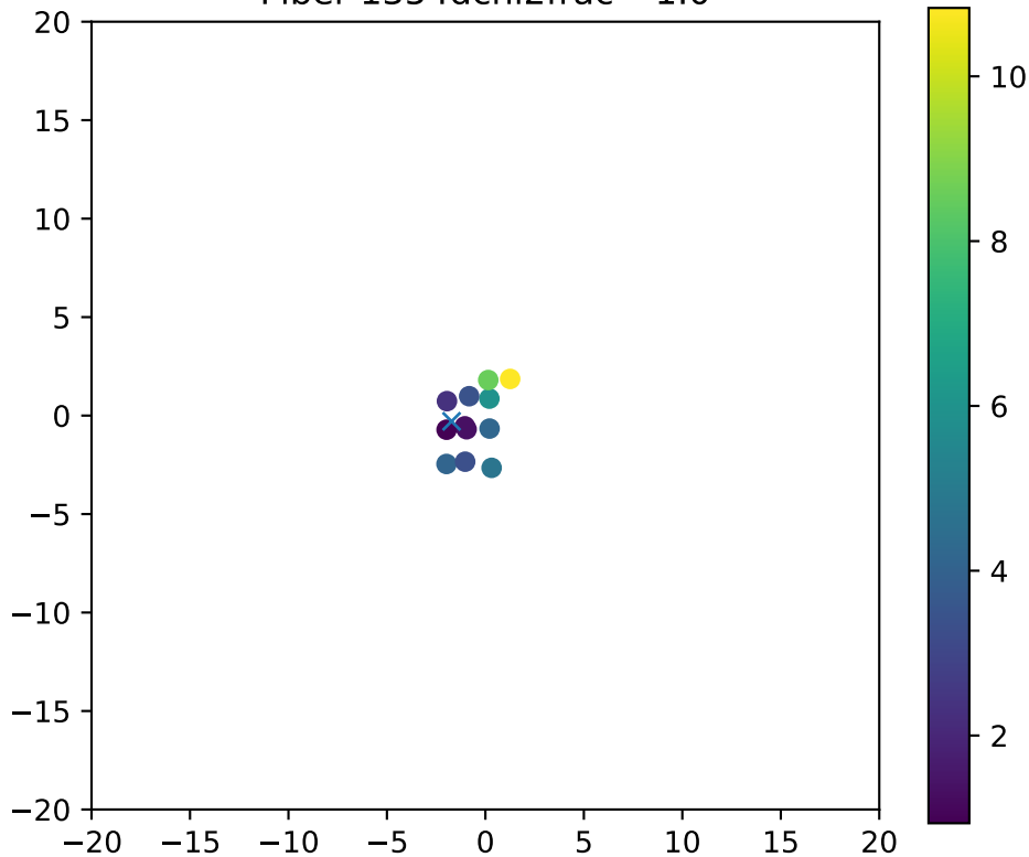
Fiber 1354dchi2frac= 1.0
