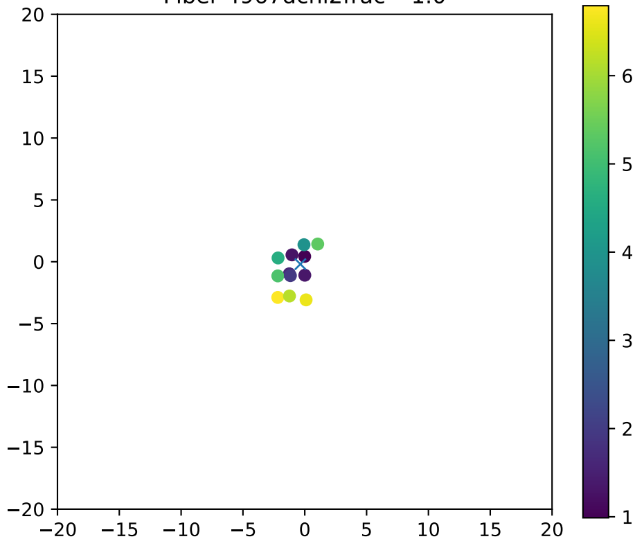
Fiber 4967dchi2frac= 1.0
