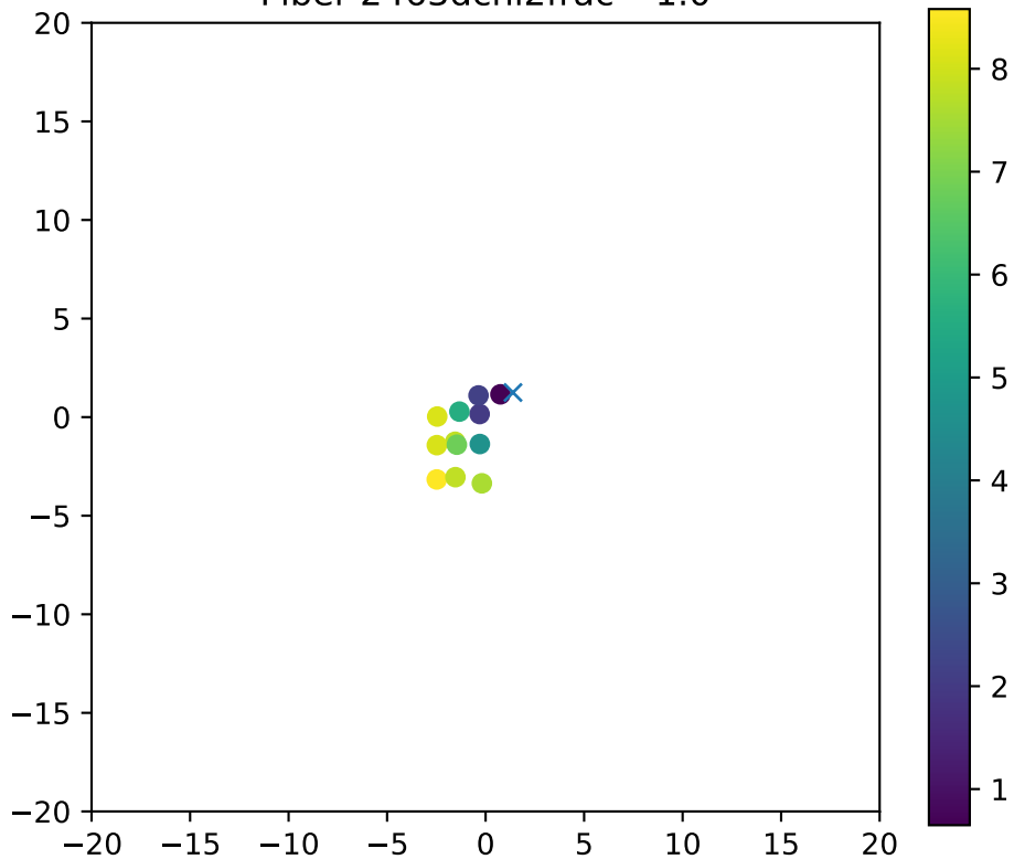
Fiber 2463dchi2frac= 1.0
