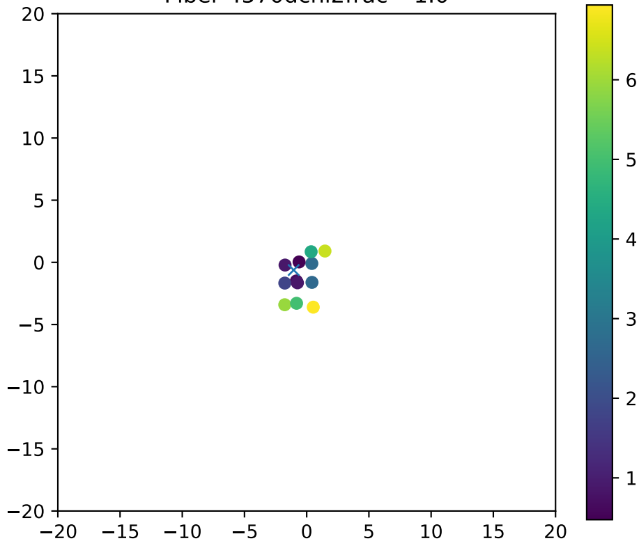
Fiber 4570dchi2frac= 1.0
