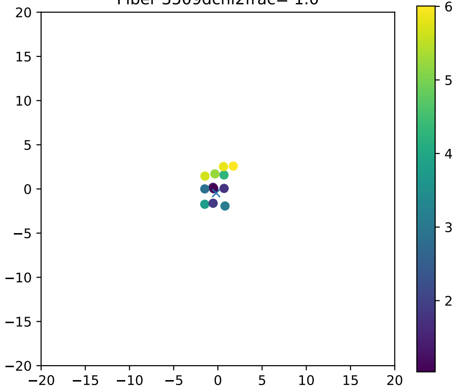
Fiber 3509dchi2frac= 1.0
