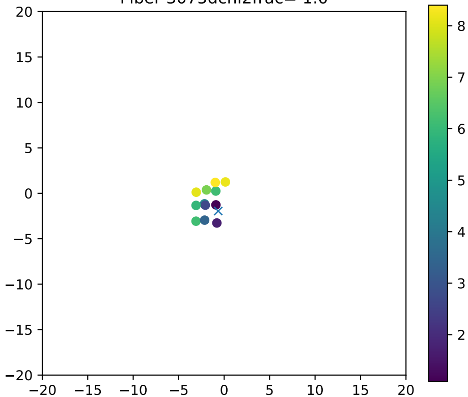
Fiber 3075dchi2frac= 1.0
