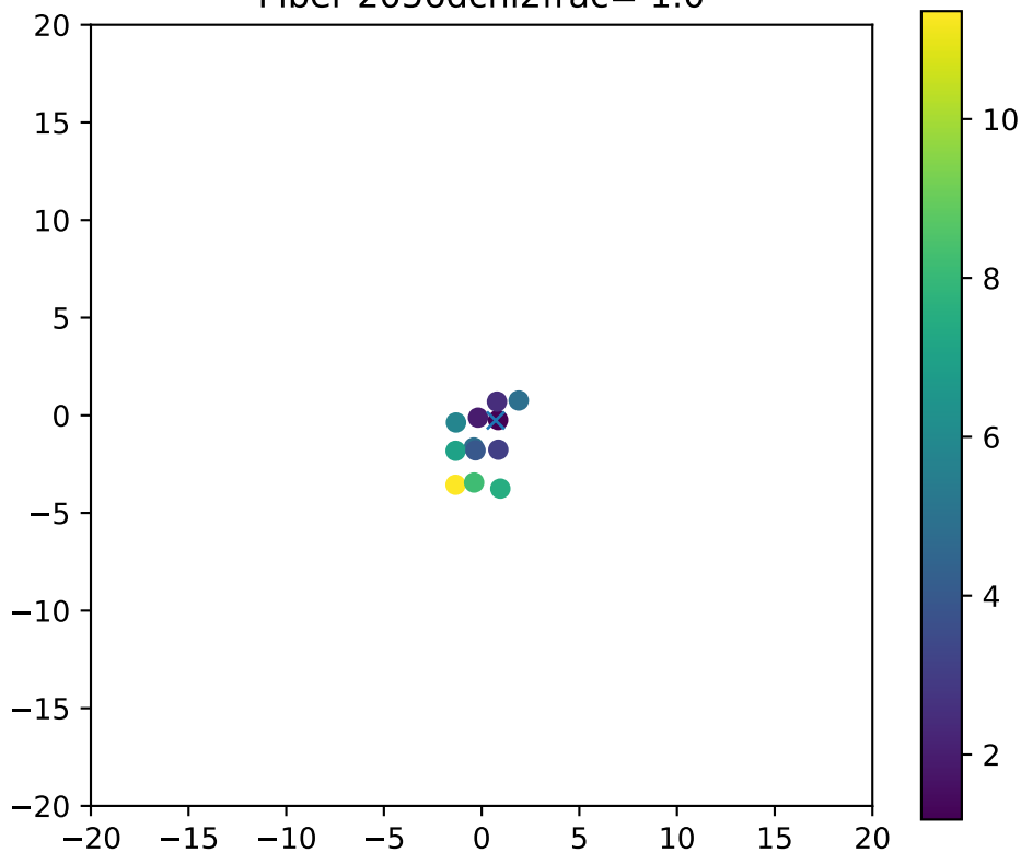
Fiber 2056dchi2frac= 1.0
