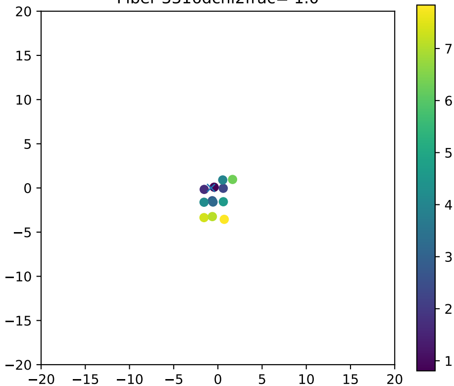
Fiber 3316dchi2frac= 1.0
