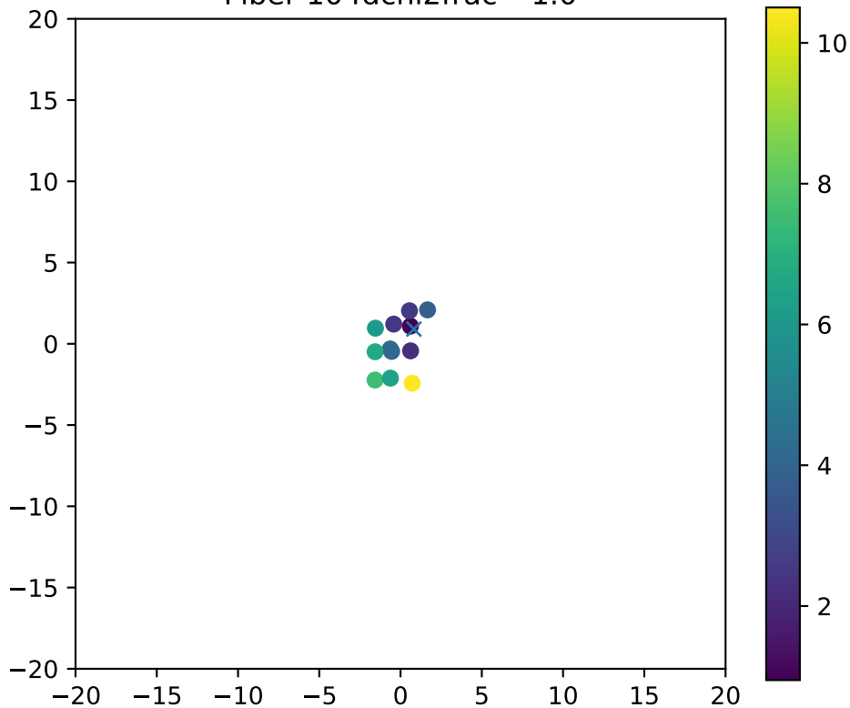
Fiber 104dchi2frac= 1.0
