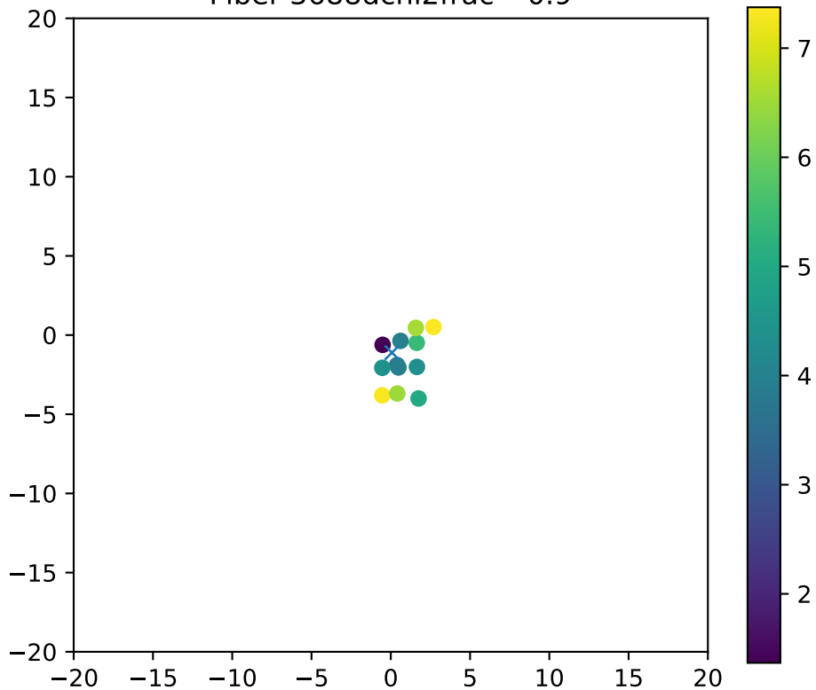
Fiber 3688dchi2frac= 0.9
