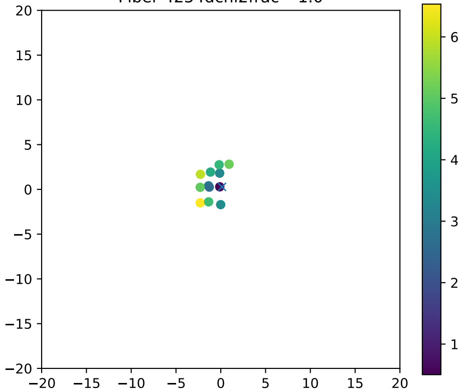
Fiber 4254dchi2frac= 1.0
