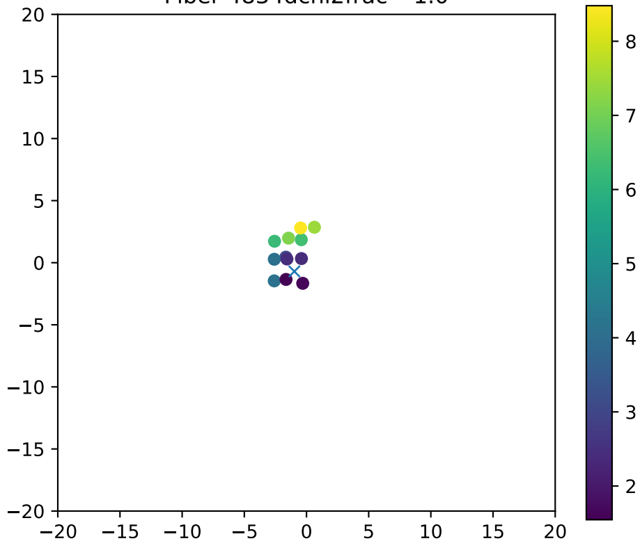
Fiber 4834dchi2frac= 1.0
