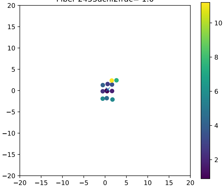
Fiber 2453dchi2frac= 1.0
