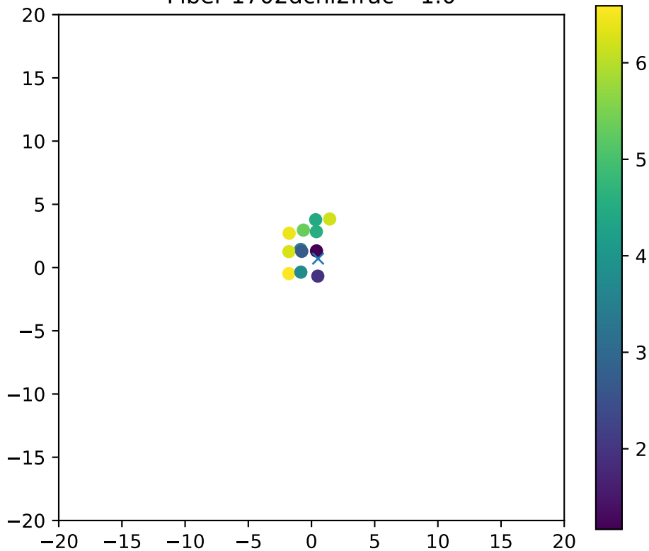
Fiber 1702dchi2frac= 1.0
