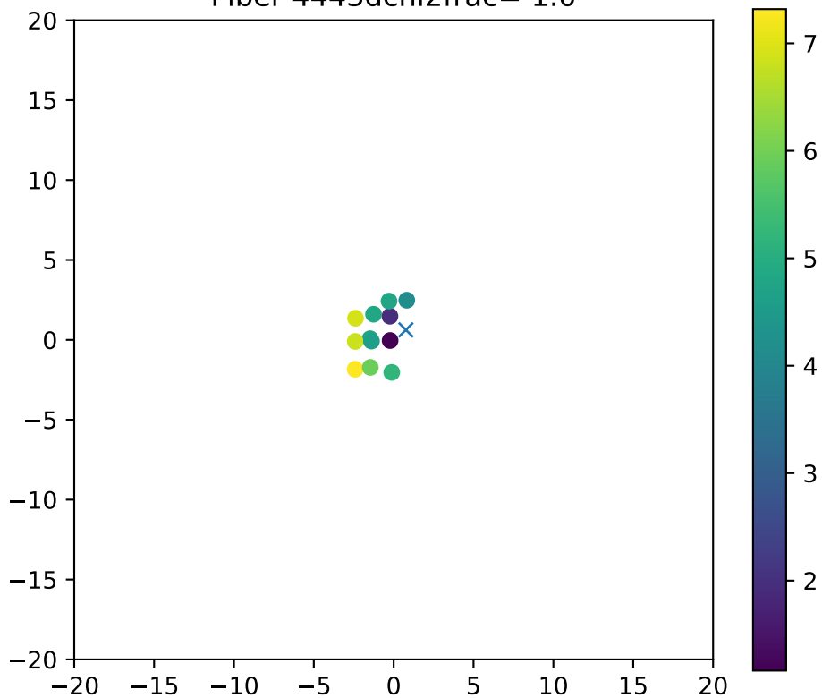
Fiber 4443dchi2frac= 1.0
