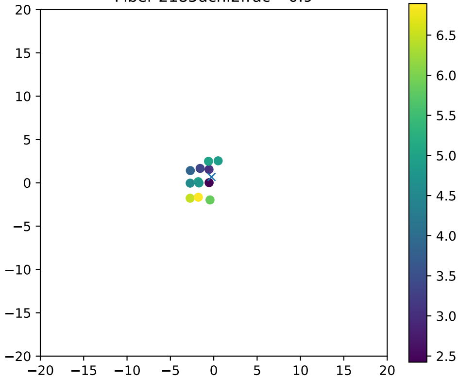
Fiber 2185dchi2frac= 0.9
