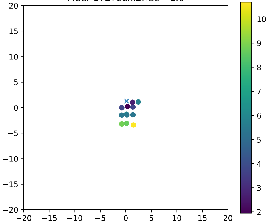
Fiber 1727dchi2frac= 1.0
