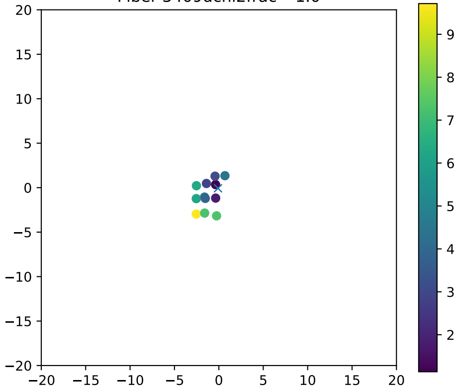
Fiber 3409dchi2frac= 1.0
