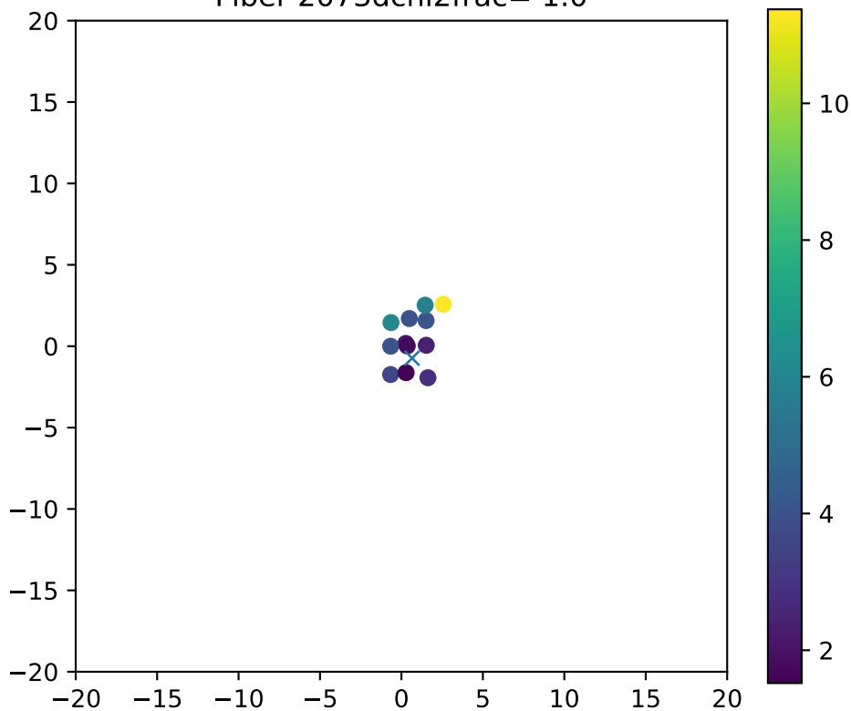
Fiber 2073dchi2frac= 1.0
