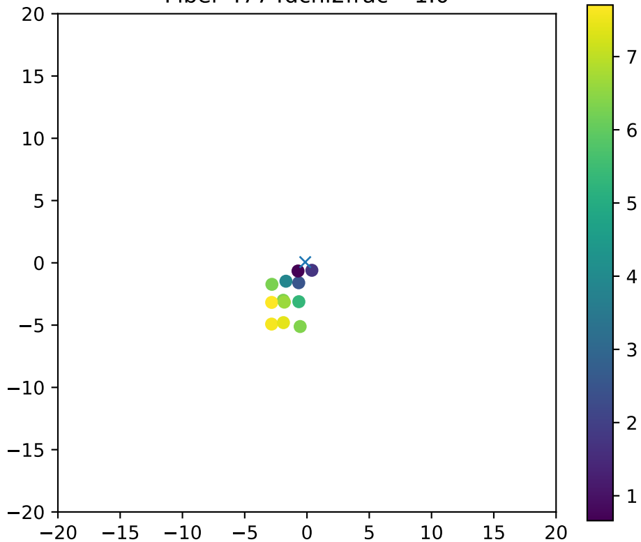
Fiber 4774dchi2frac= 1.0
