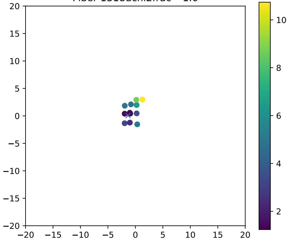
Fiber 1318dchi2frac= 1.0
