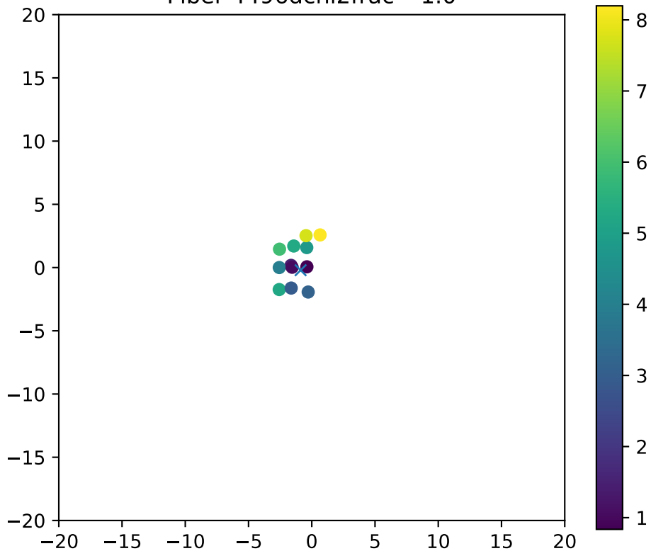
Fiber 4496dchi2frac= 1.0
