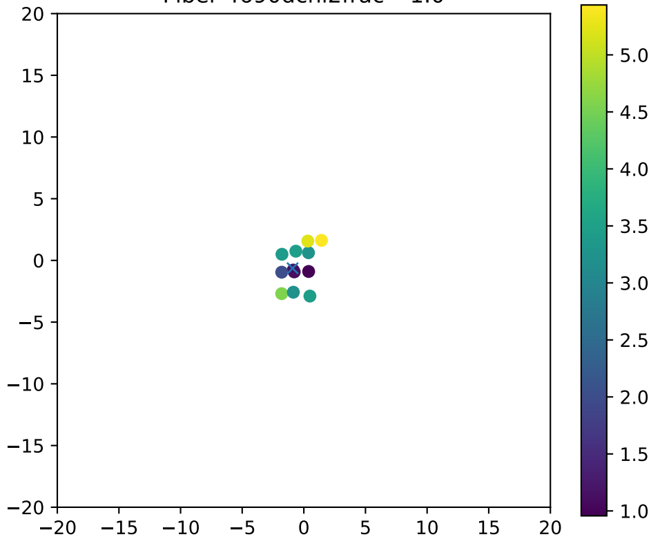
Fiber 4690dchi2frac= 1.0
