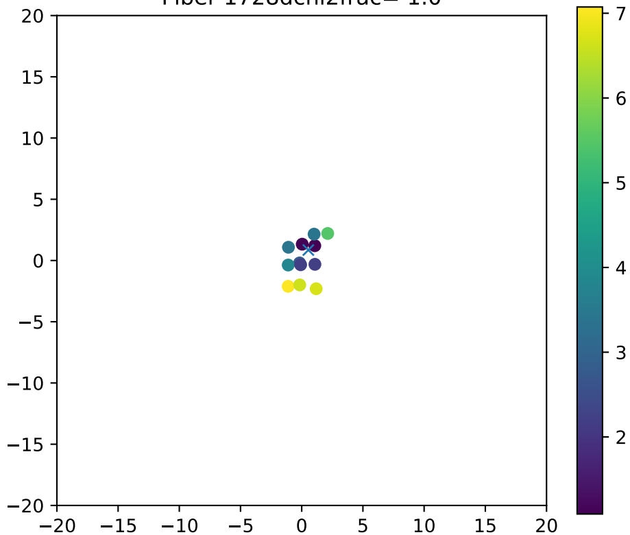
Fiber 1728dchi2frac= 1.0
