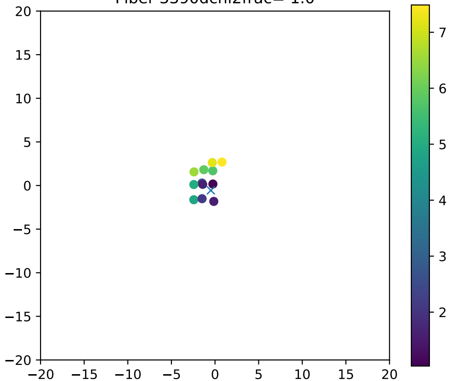
Fiber 3390dchi2frac= 1.0
