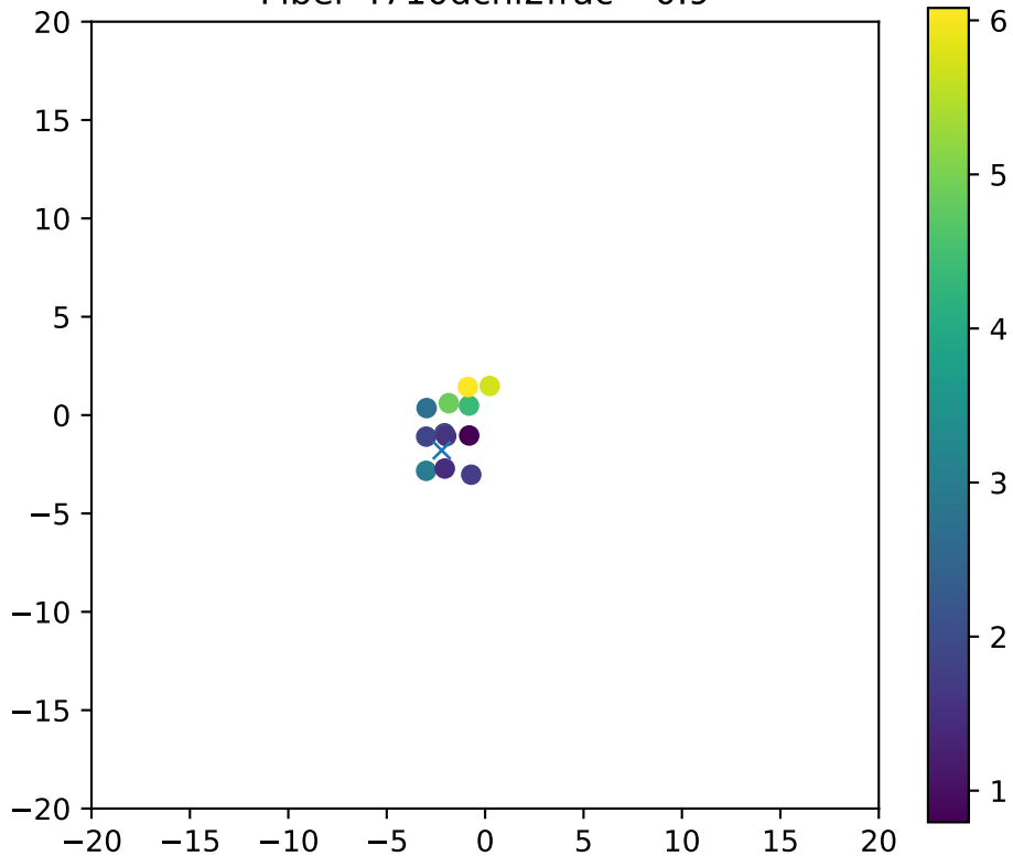
Fiber 4710dchi2frac= 0.9
