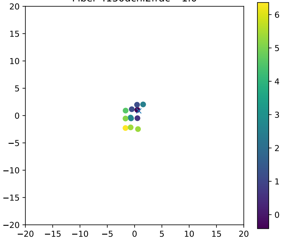
Fiber 4130dchi2frac= 1.0
