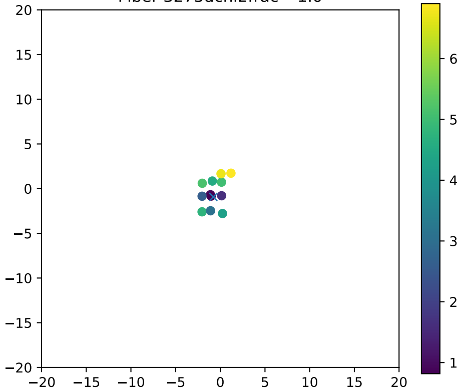
Fiber 3273dchi2frac= 1.0
