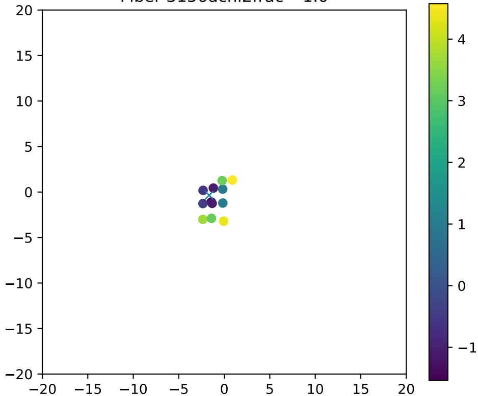
Fiber 3156dchi2frac= 1.0
