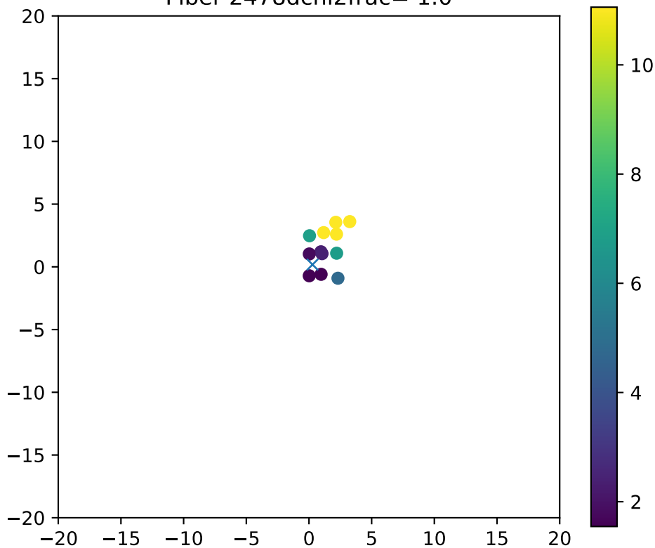
Fiber 2478dchi2frac= 1.0
