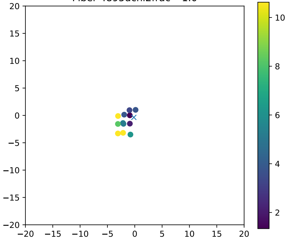
Fiber 4895dchi2frac= 1.0
