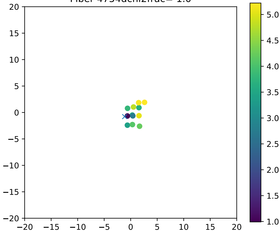
Fiber 4754dchi2frac= 1.0
