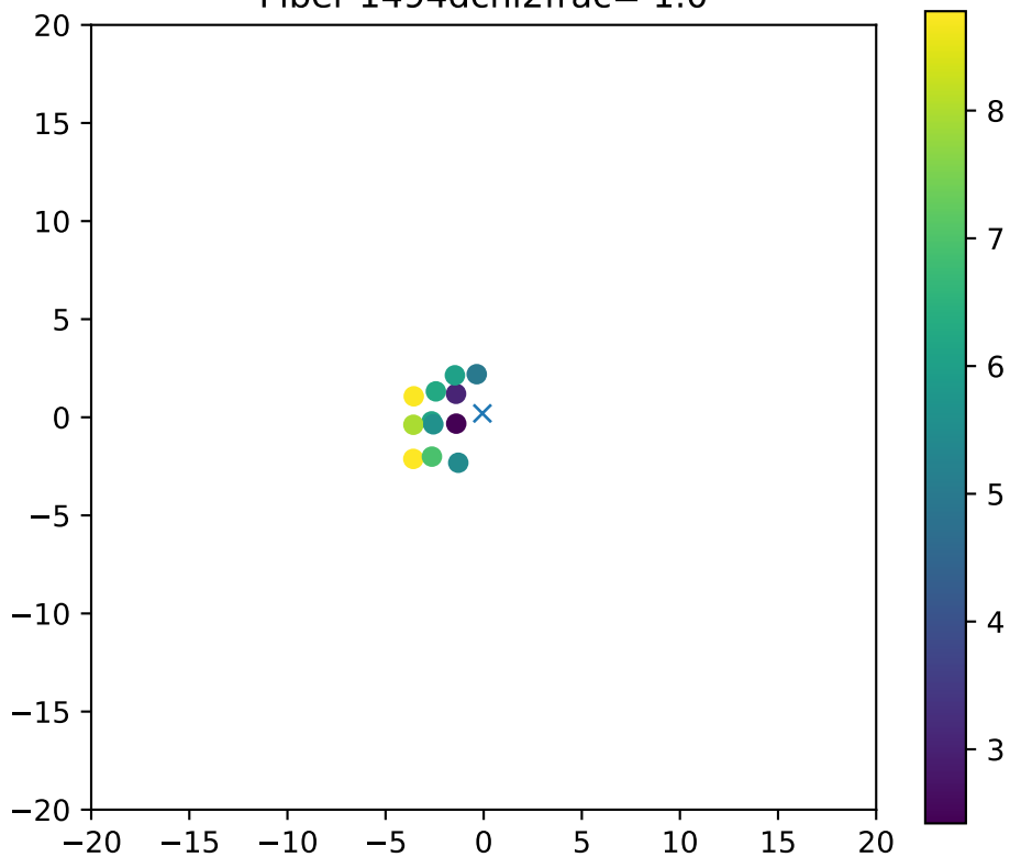
Fiber 1494dchi2frac= 1.0
