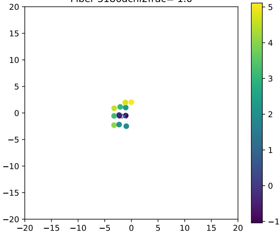
Fiber 3186dchi2frac= 1.0
