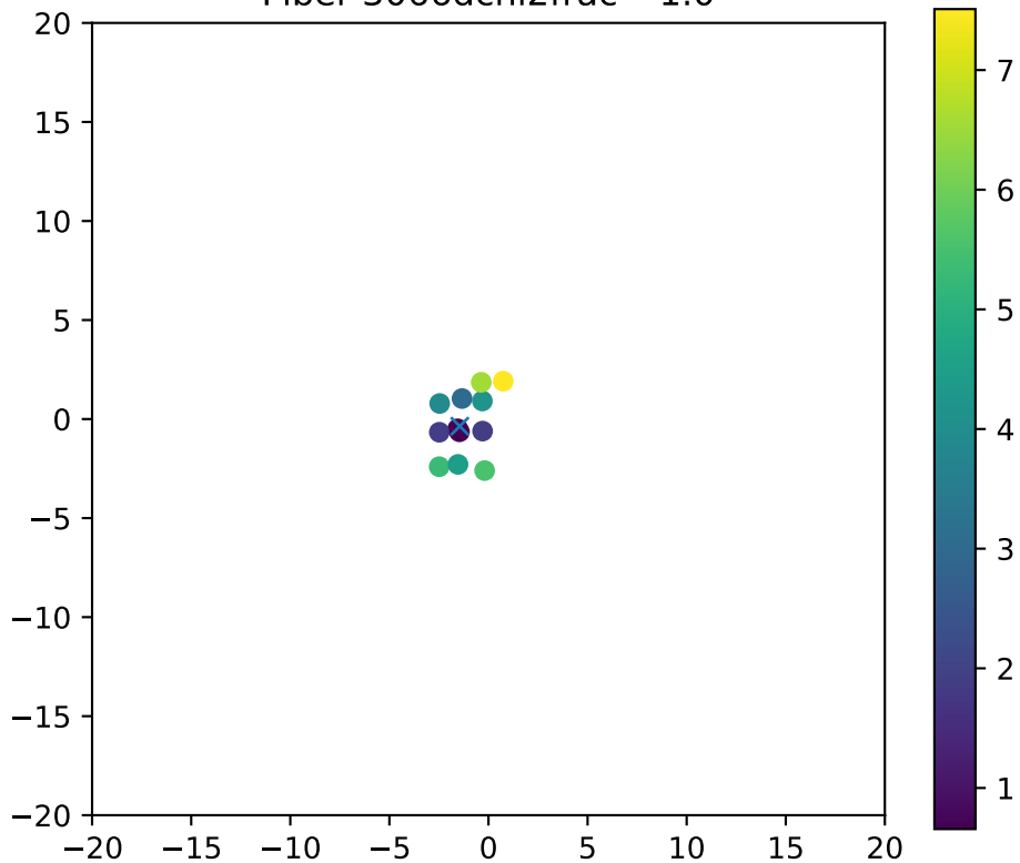
Fiber 3066dchi2frac= 1.0
