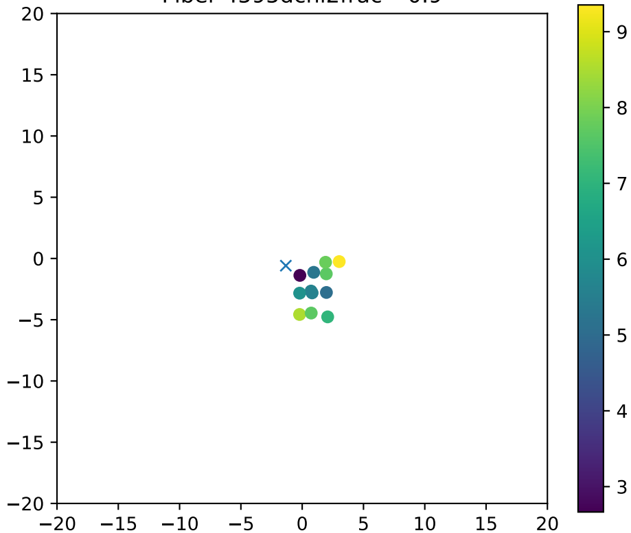
Fiber 4595dchi2frac= 0.9
