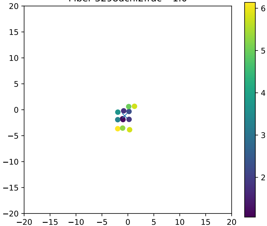
Fiber 3298dchi2frac= 1.0
