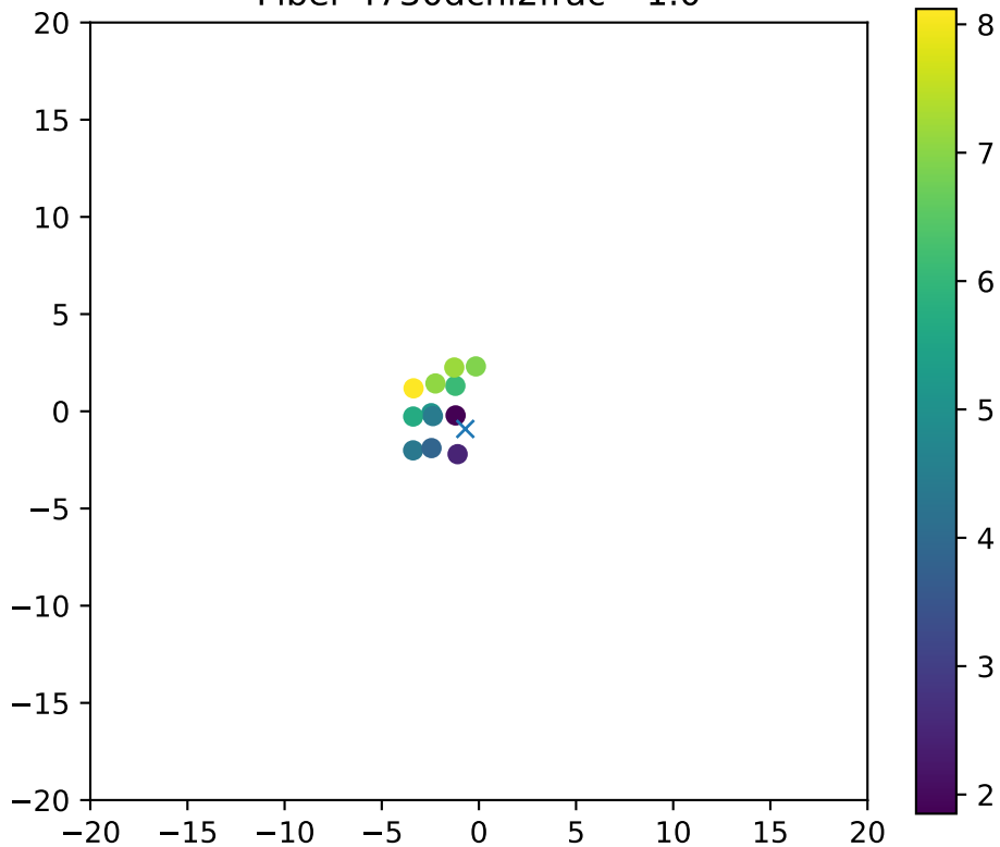
Fiber 4730dchi2frac= 1.0
