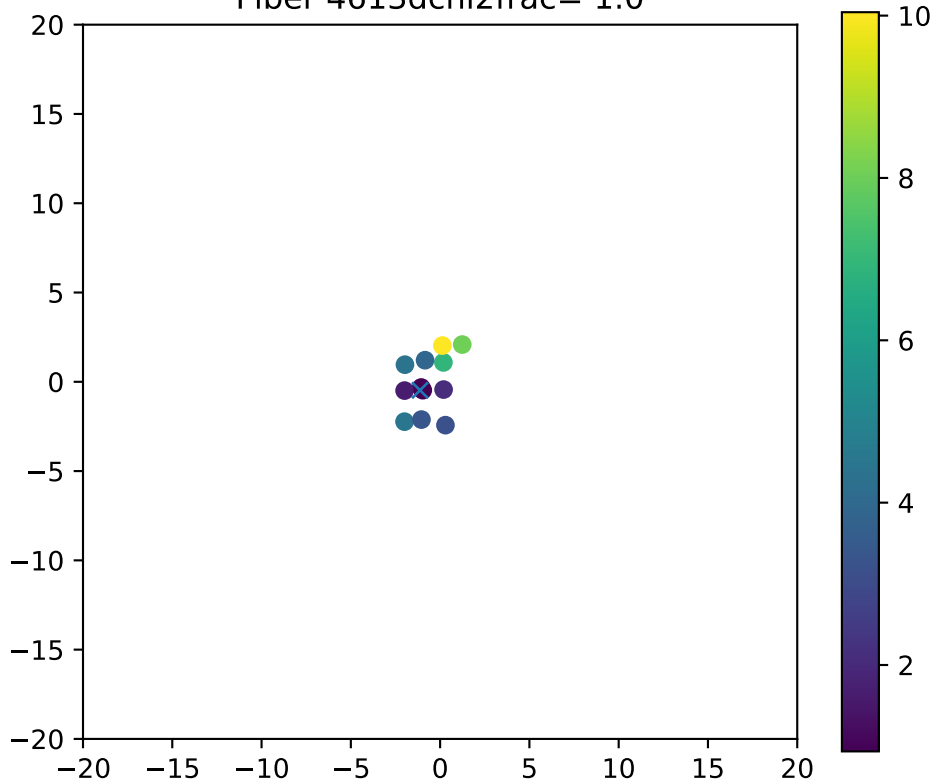
Fiber 4613dchi2frac= 1.0
