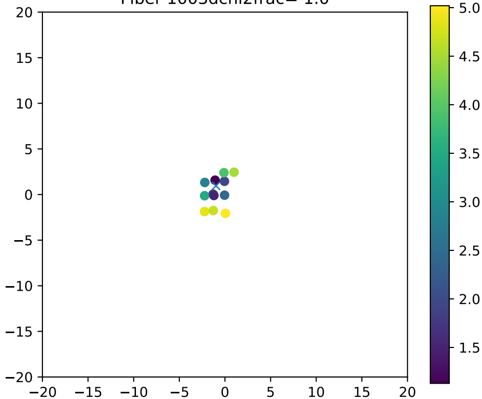
Fiber 1003dchi2frac= 1.0
