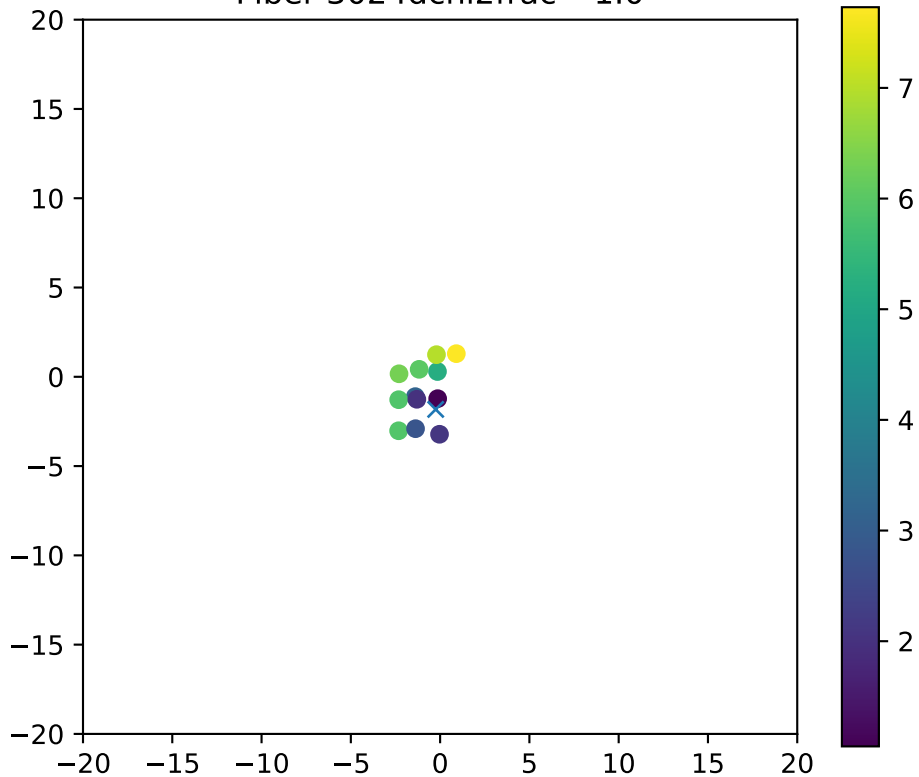
Fiber 3024dchi2frac= 1.0
