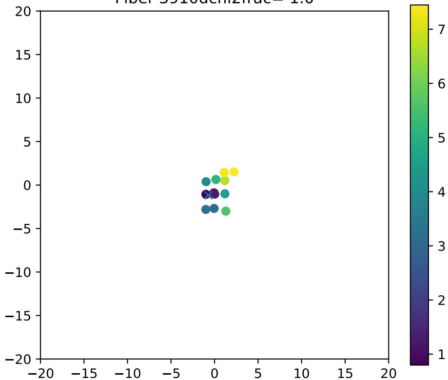
Fiber 3910dchi2frac= 1.0
