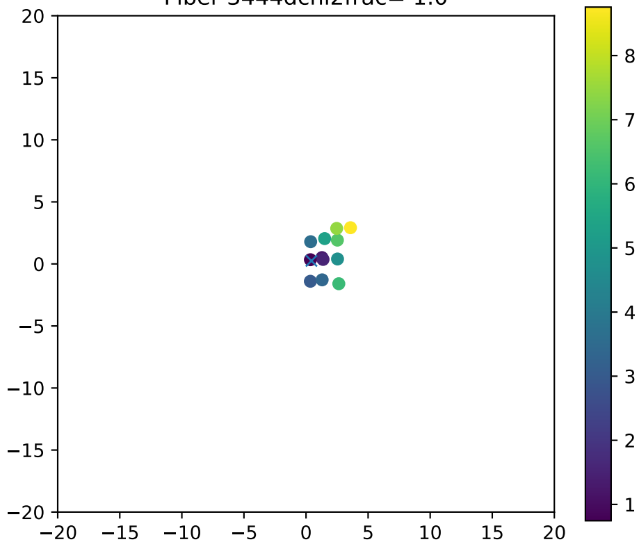
Fiber 3444dchi2frac= 1.0
