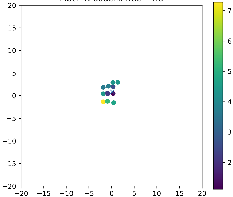
Fiber 1260dchi2frac= 1.0
