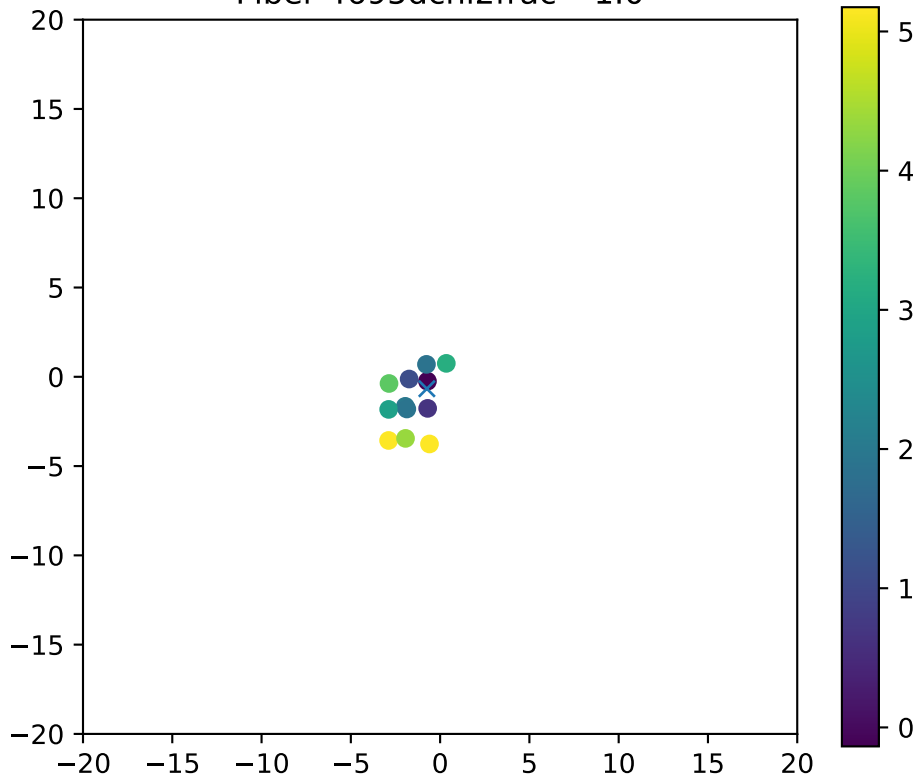
Fiber 4695dchi2frac= 1.0
