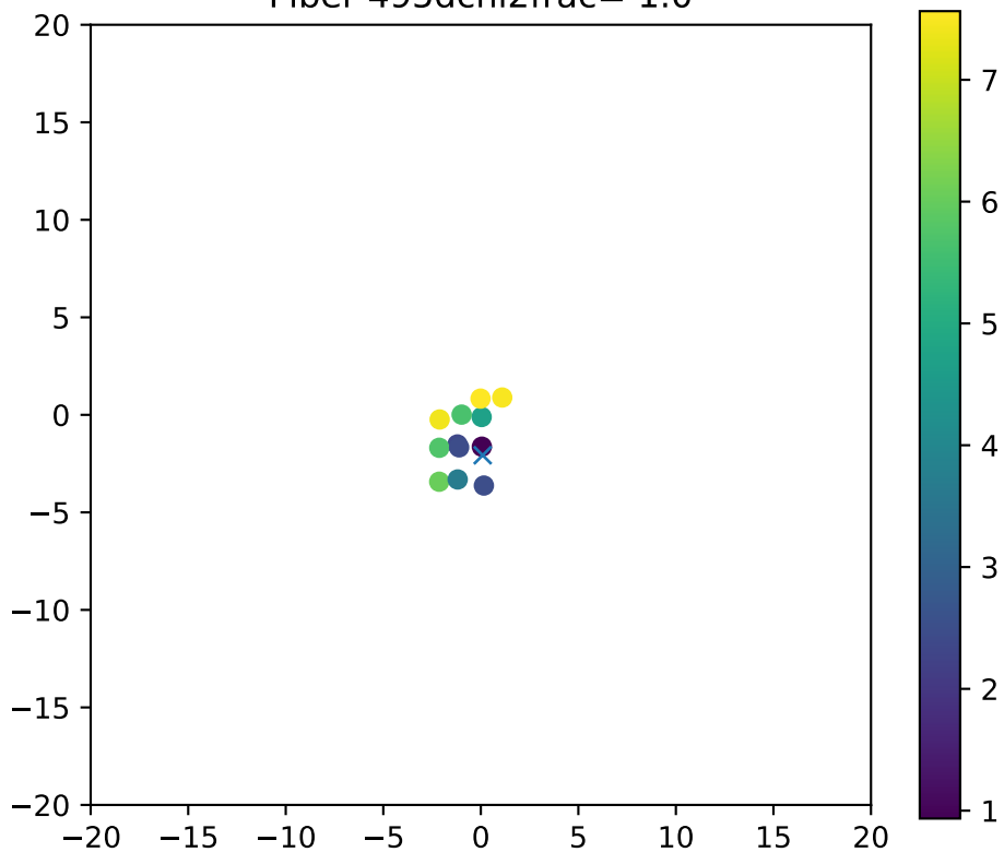
Fiber 495dchi2frac= 1.0
