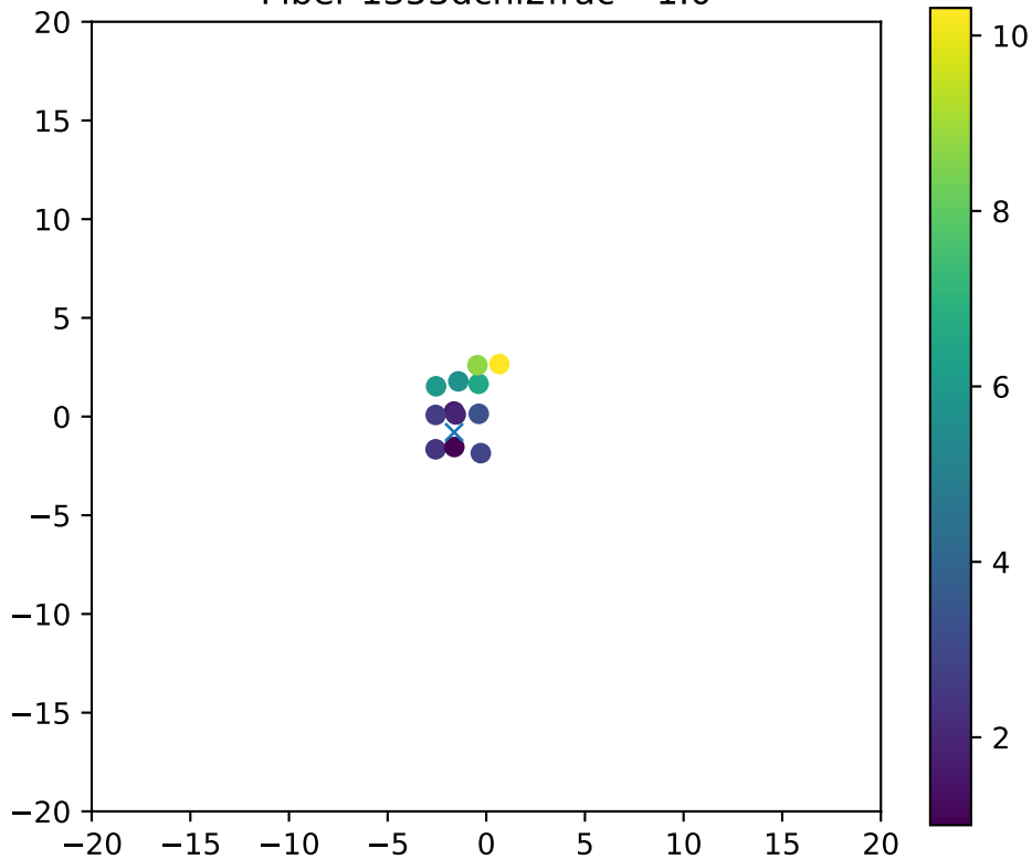
Fiber 1353dchi2frac= 1.0
