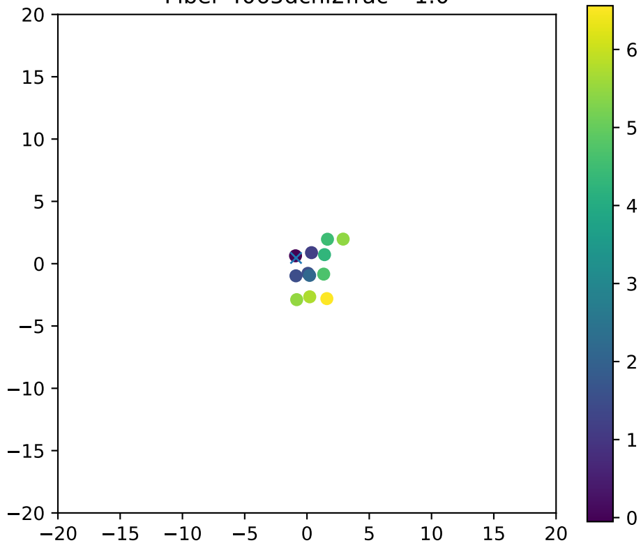
Fiber 4065dchi2frac= 1.0
