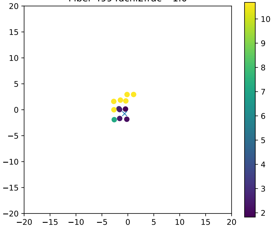
Fiber 4994dchi2frac= 1.0
