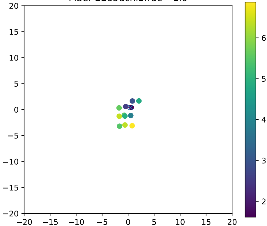
Fiber 2265dchi2frac= 1.0
