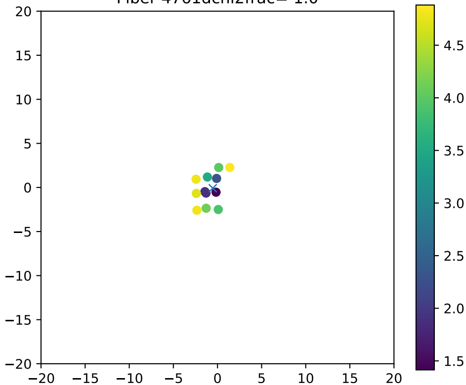
Fiber 4761dchi2frac= 1.0
