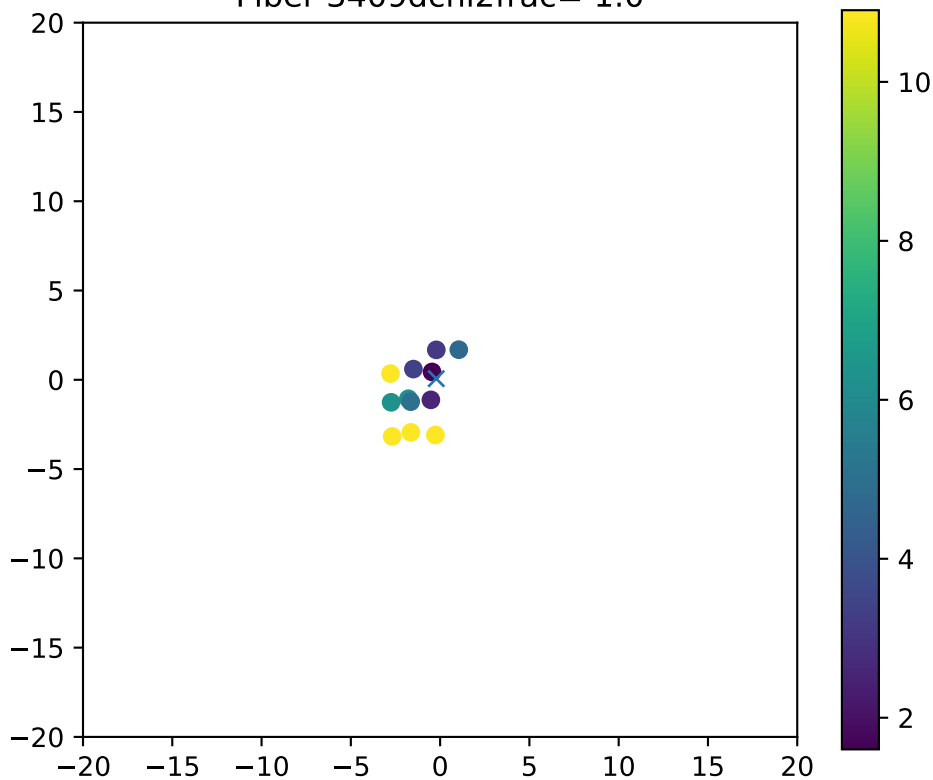
Fiber 3409dchi2frac= 1.0
