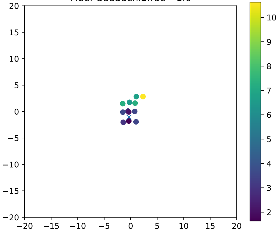
Fiber 3883dchi2frac= 1.0
