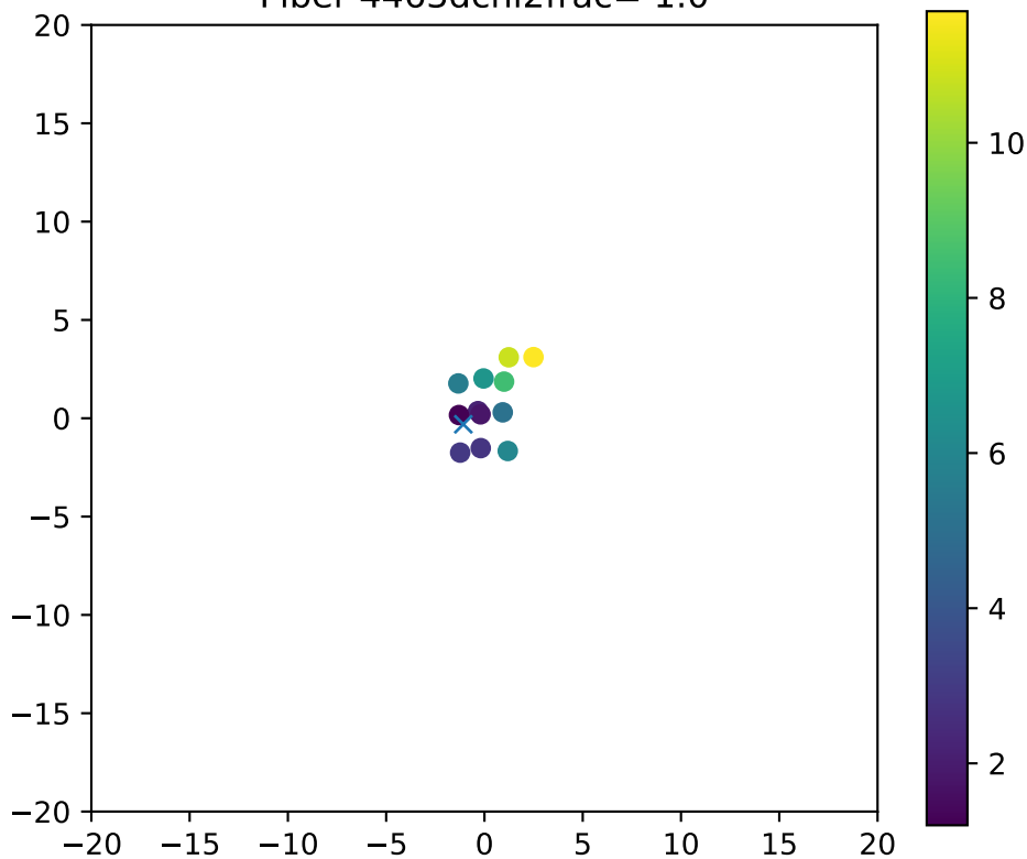
Fiber 4463dchi2frac= 1.0
