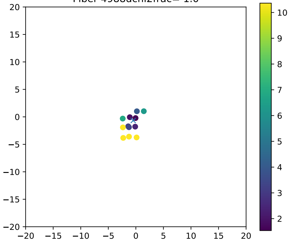
Fiber 4988dchi2frac= 1.0
