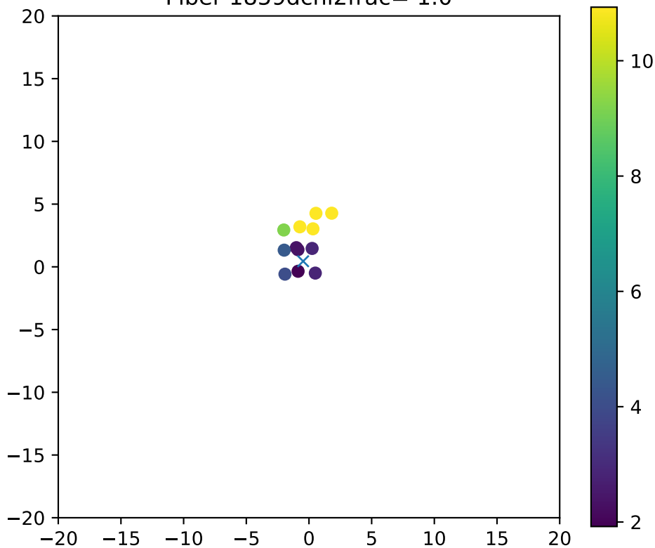
Fiber 1859dchi2frac= 1.0
