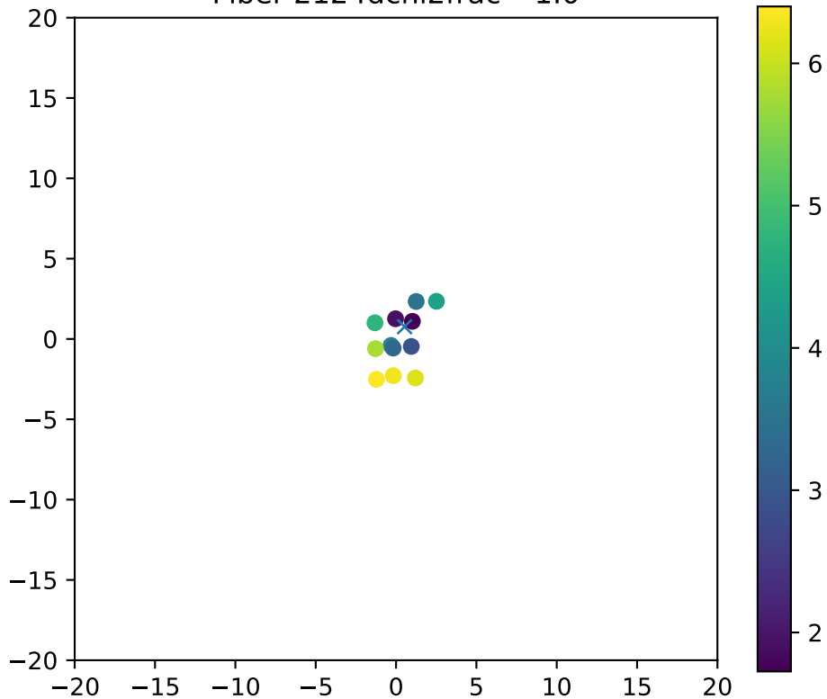
Fiber 2124dchi2frac= 1.0
