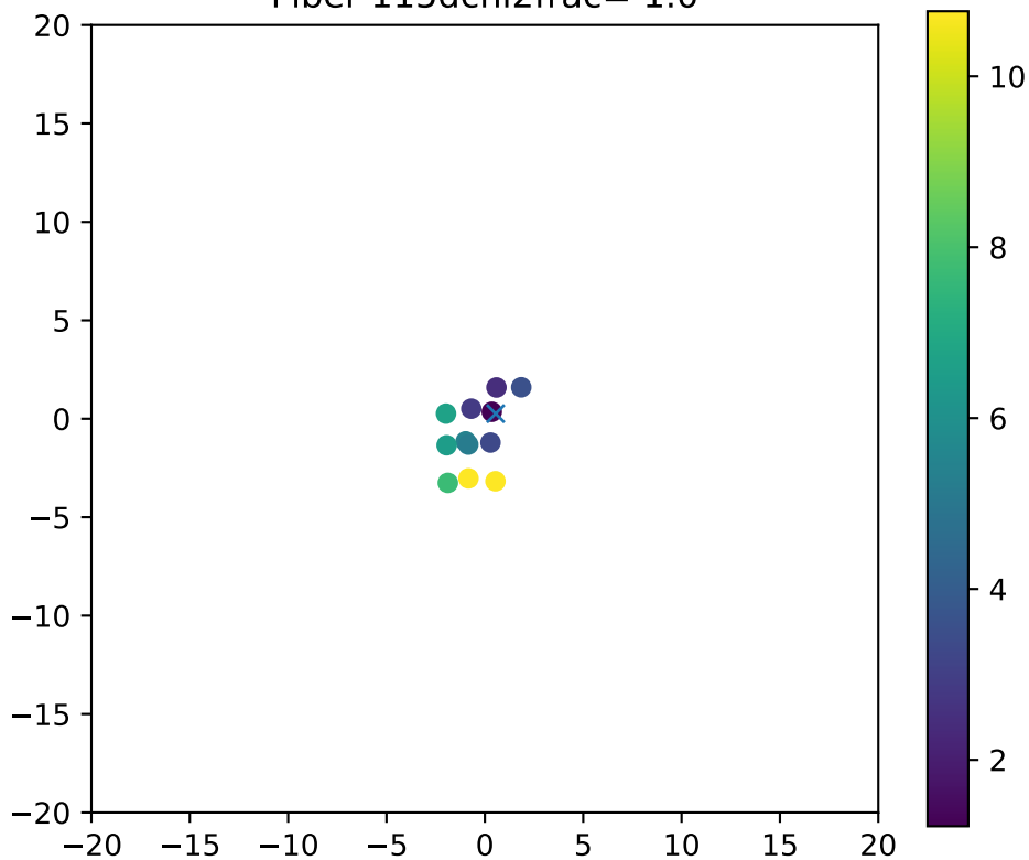
Fiber 115dchi2frac= 1.0
