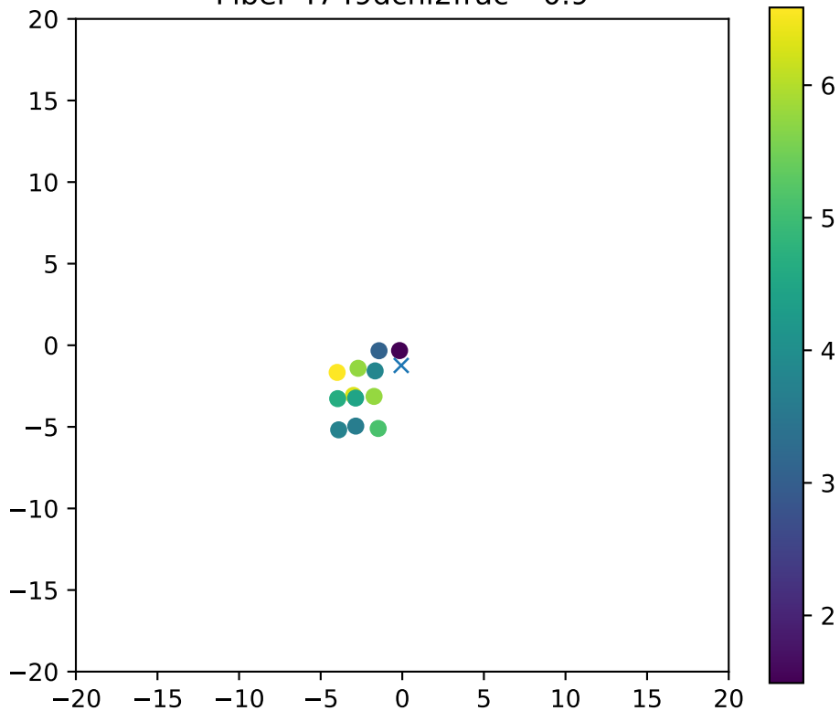
Fiber 4749dchi2frac= 0.9
