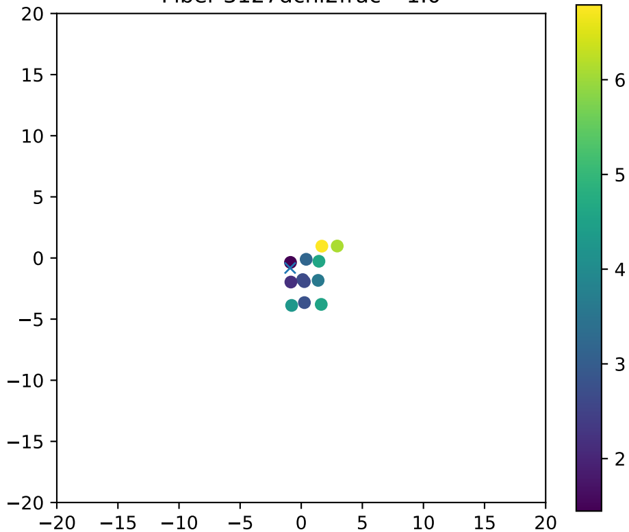
Fiber 3127dchi2frac= 1.0
