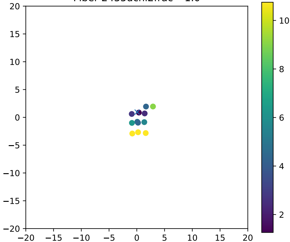
Fiber 2435dchi2frac= 1.0
