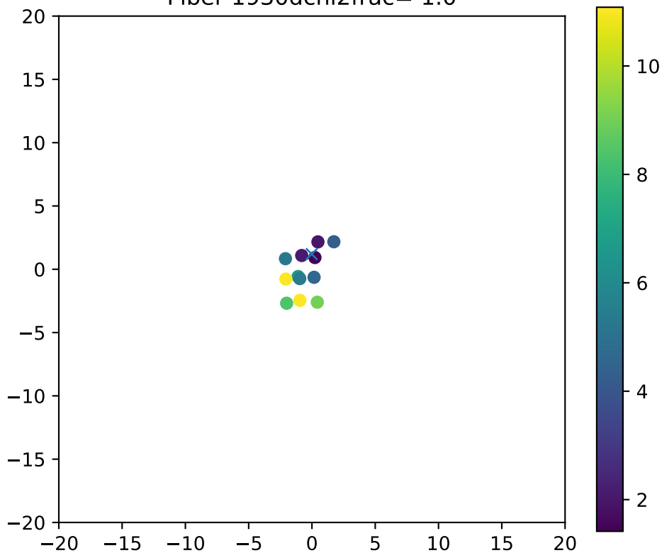
Fiber 1930dchi2frac= 1.0
