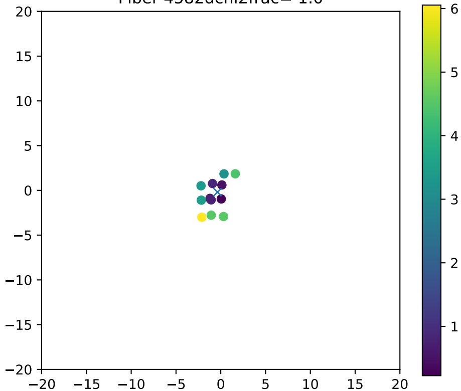
Fiber 4582dchi2frac= 1.0
