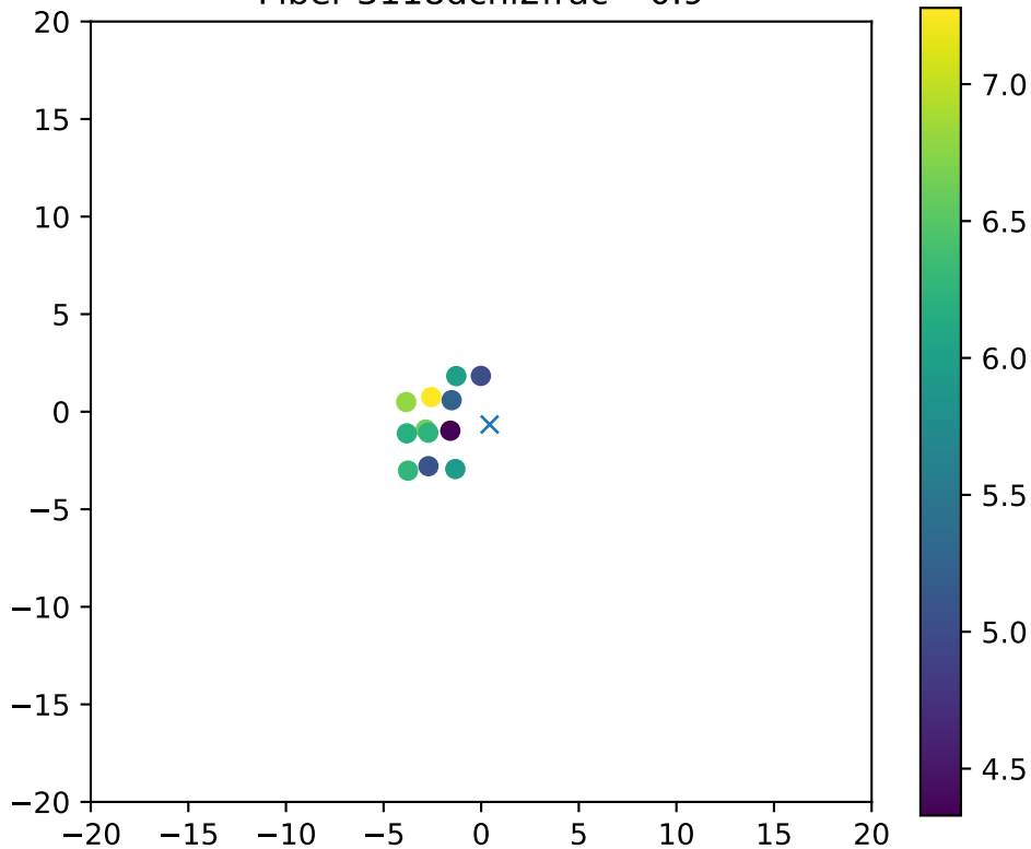
Fiber 3118dchi2frac= 0.9
