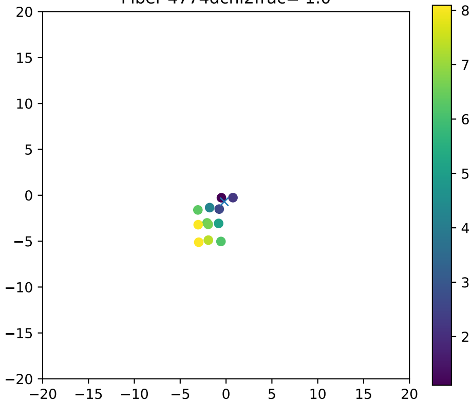
Fiber 4774dchi2frac= 1.0
