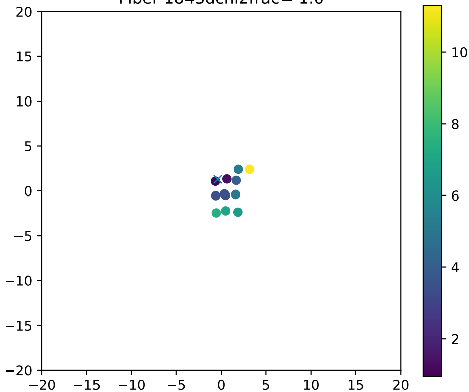
Fiber 1843dchi2frac= 1.0
