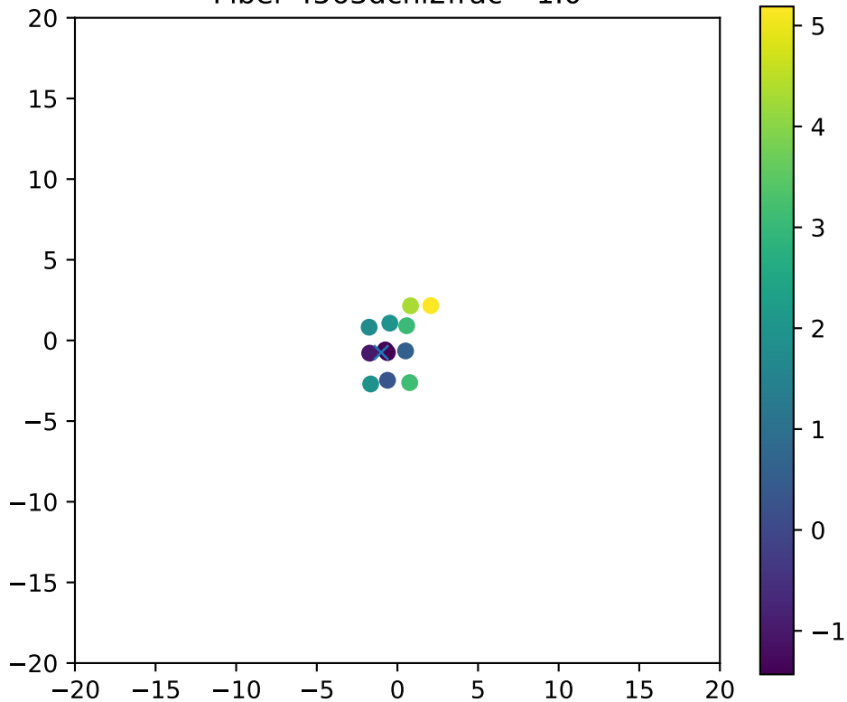
Fiber 4563dchi2frac= 1.0
