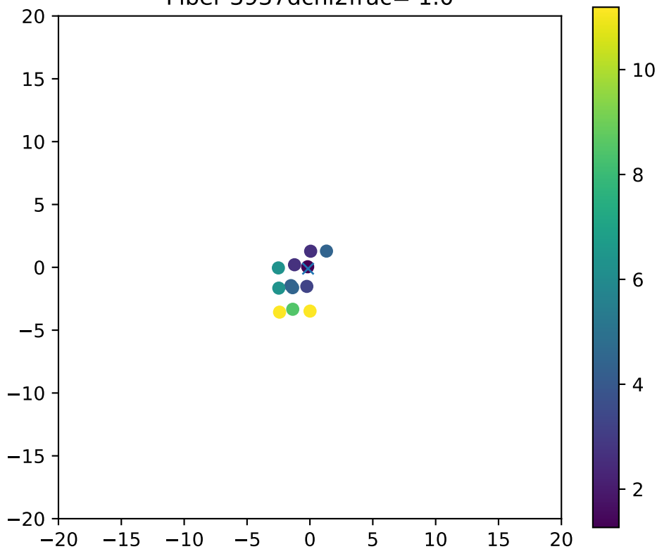
Fiber 3937dchi2frac= 1.0
