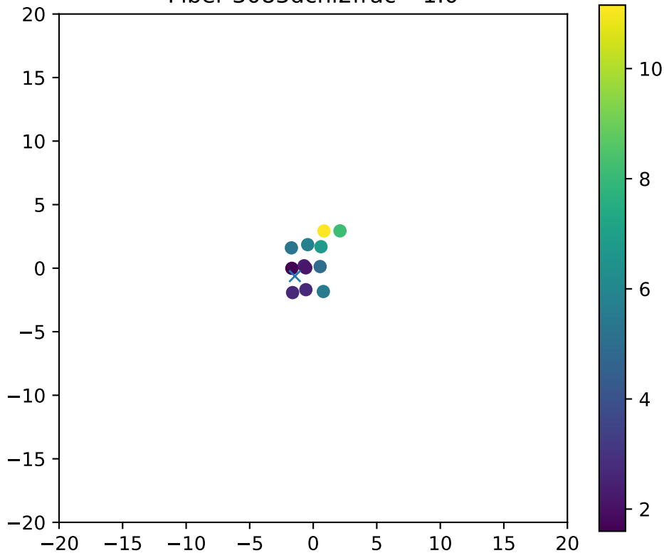
Fiber 3083dchi2frac= 1.0
