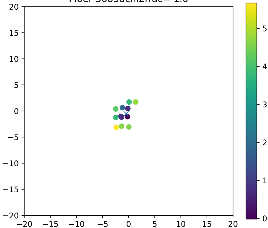
Fiber 3683dchi2frac= 1.0
