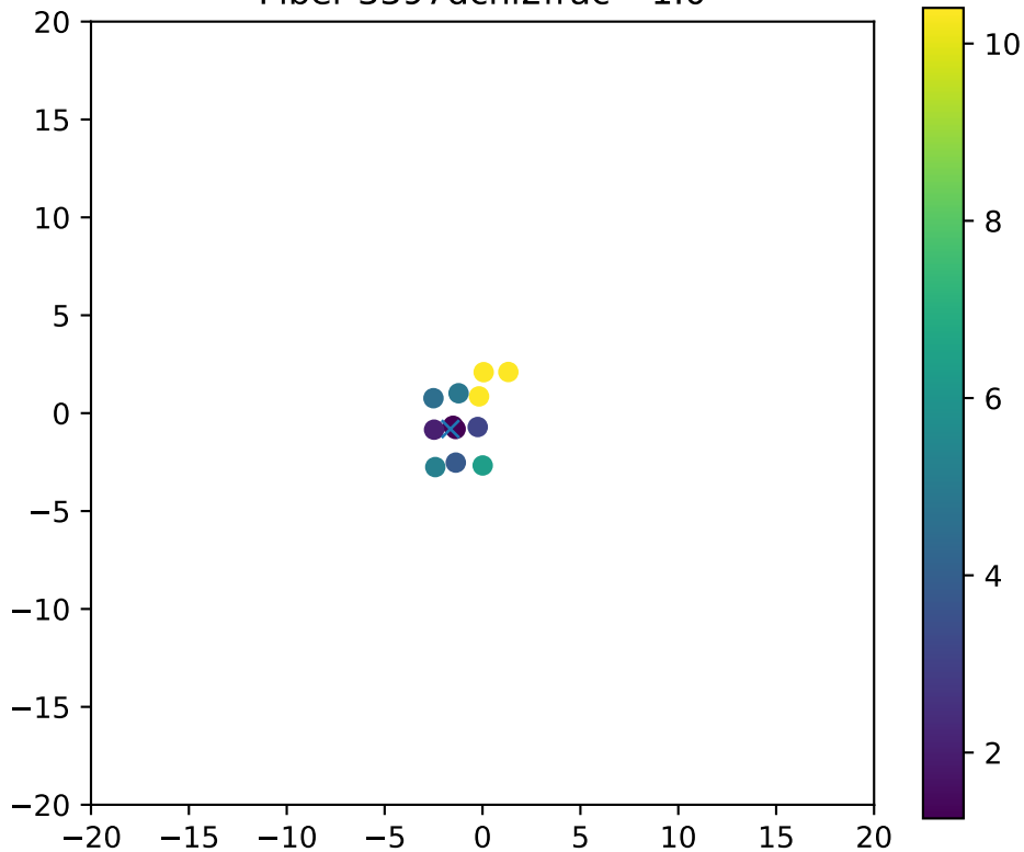
Fiber 3397dchi2frac= 1.0
