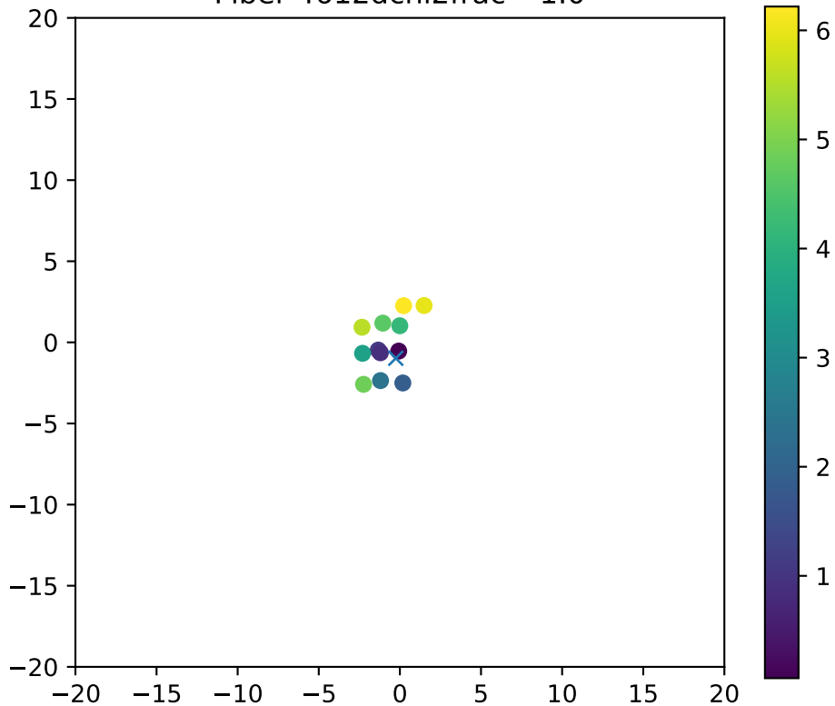
Fiber 4612dchi2frac= 1.0
