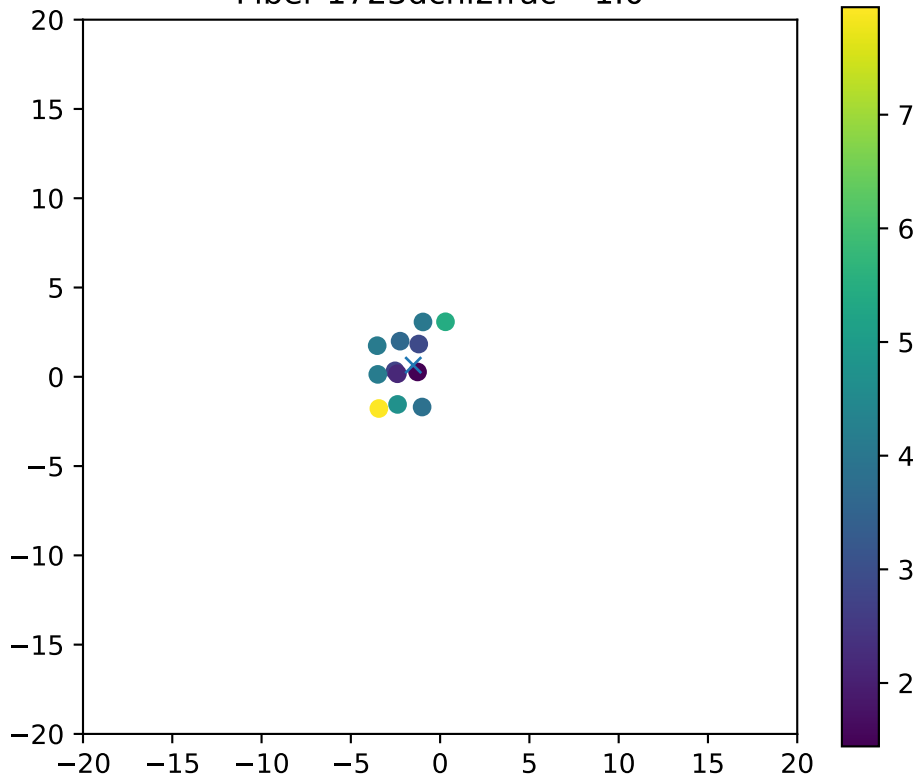
Fiber 1723dchi2frac= 1.0
