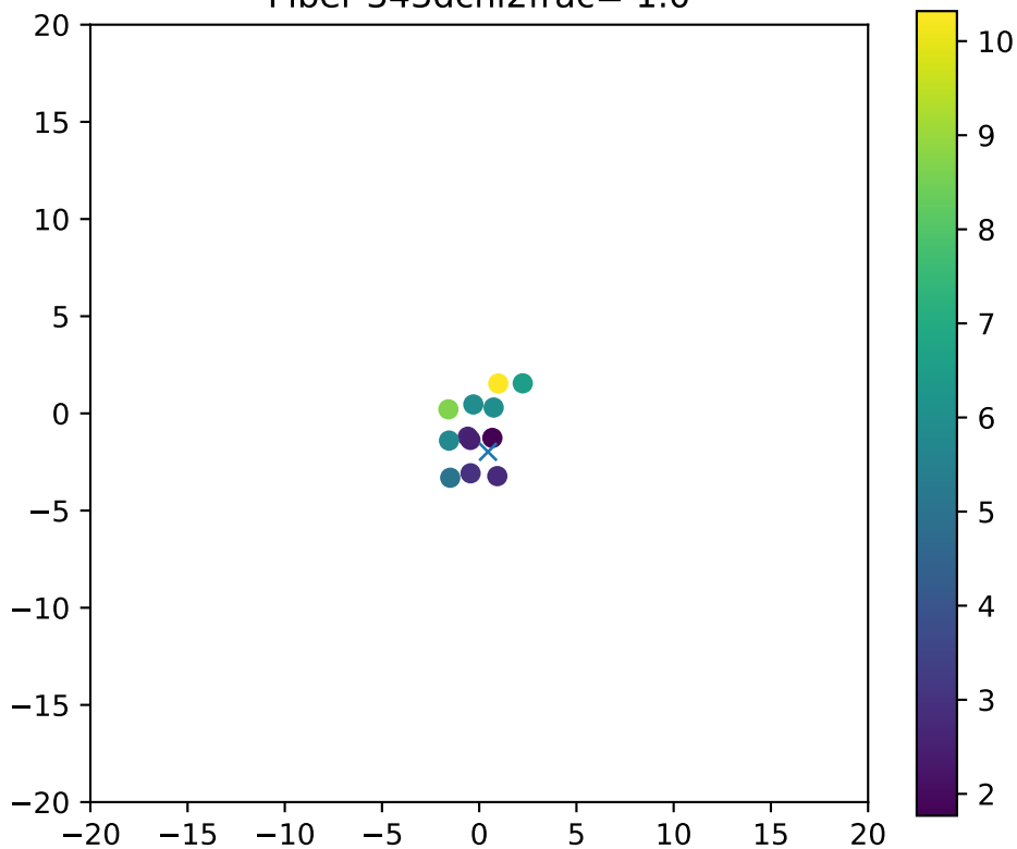
Fiber 343dchi2frac= 1.0
