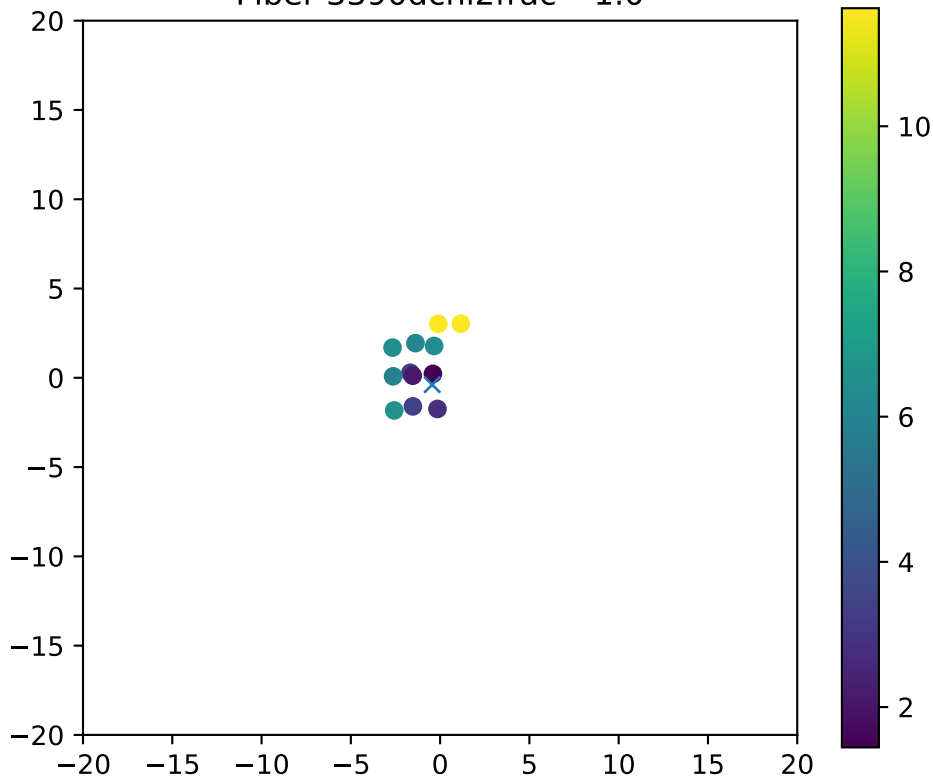
Fiber 3390dchi2frac= 1.0
