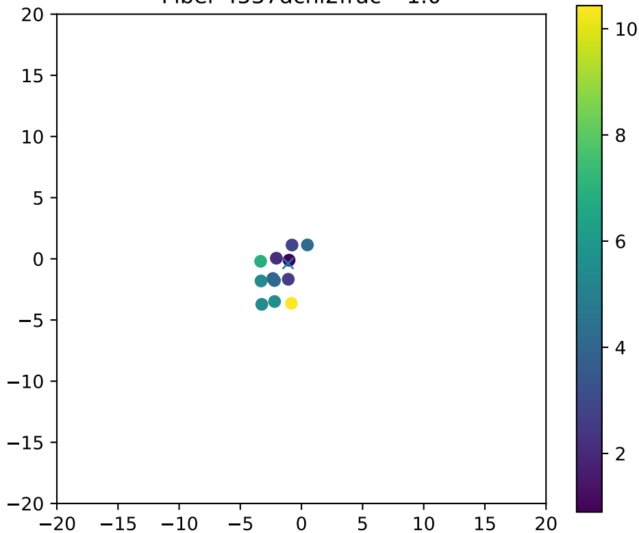
Fiber 4537dchi2frac= 1.0
