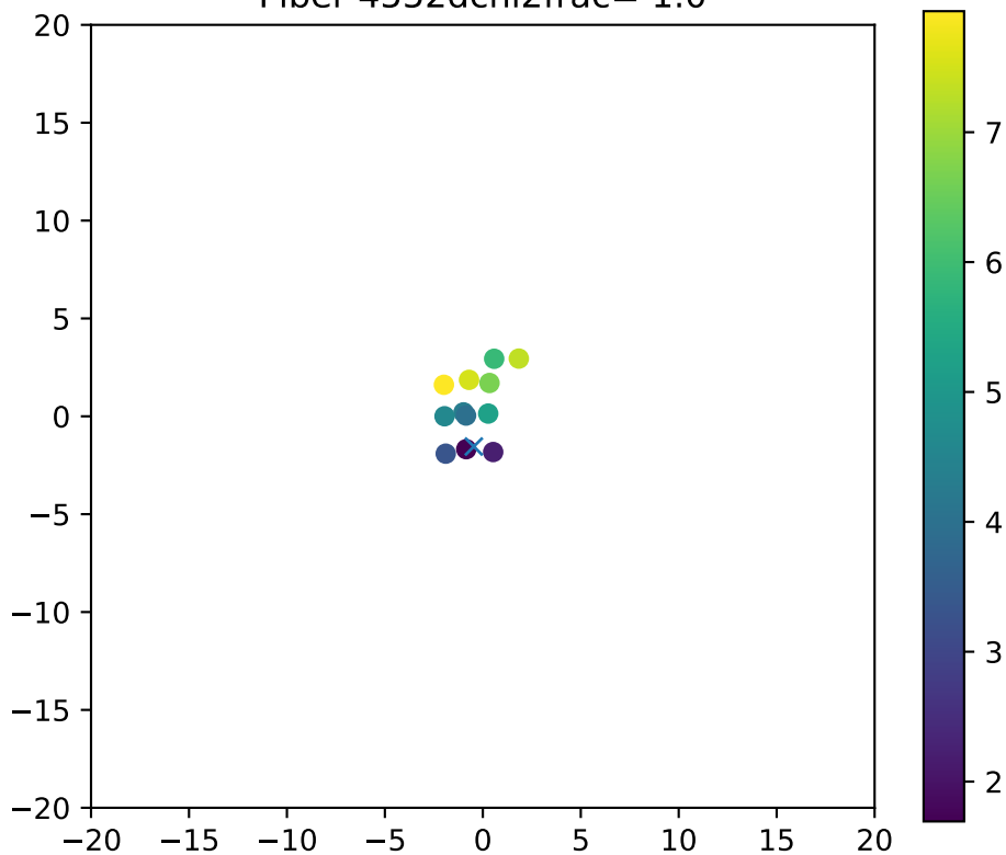
Fiber 4552dchi2frac= 1.0
