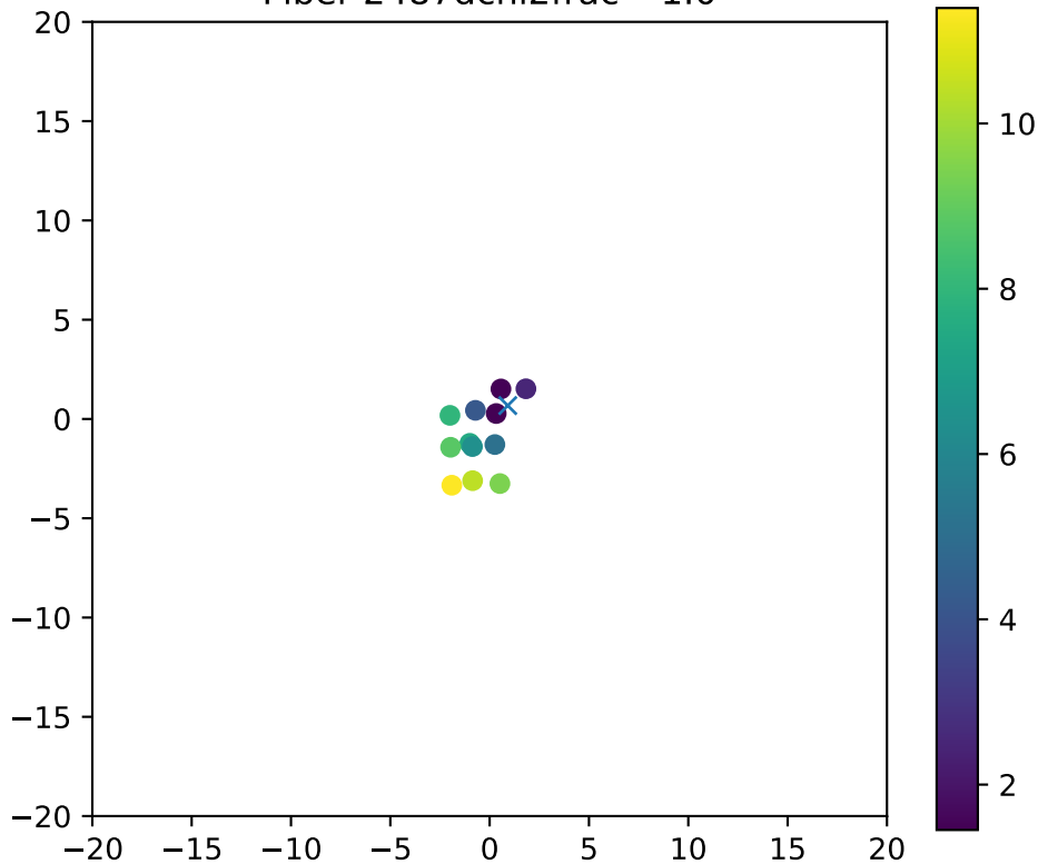
Fiber 2487dchi2frac= 1.0
