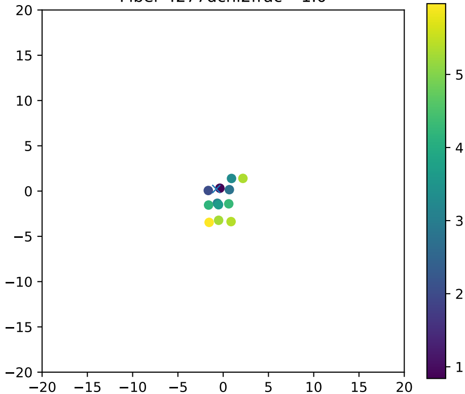
Fiber 4277dchi2frac= 1.0
