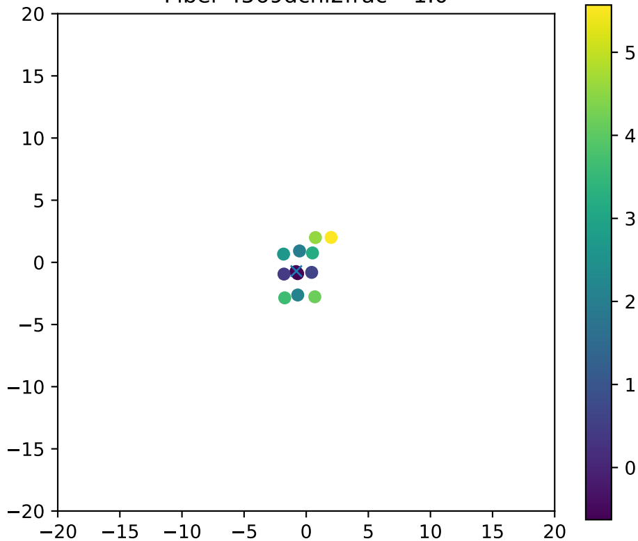
Fiber 4569dchi2frac= 1.0
