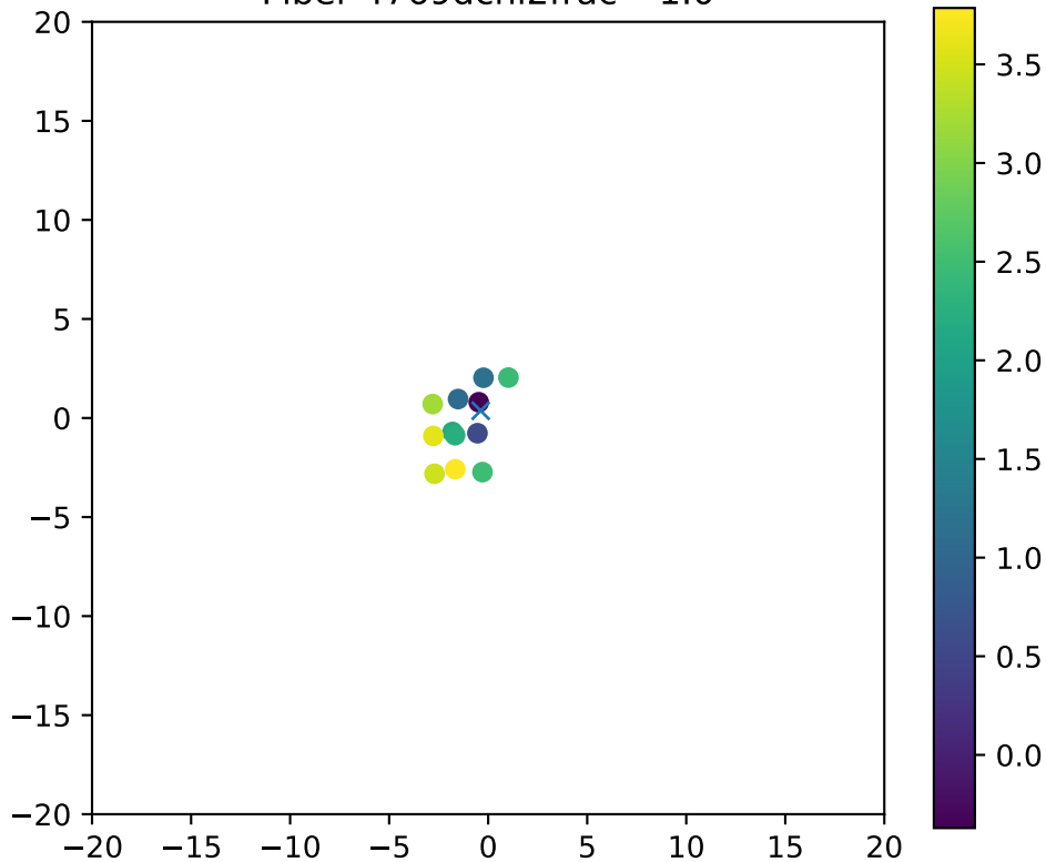
Fiber 4769dchi2frac= 1.0
