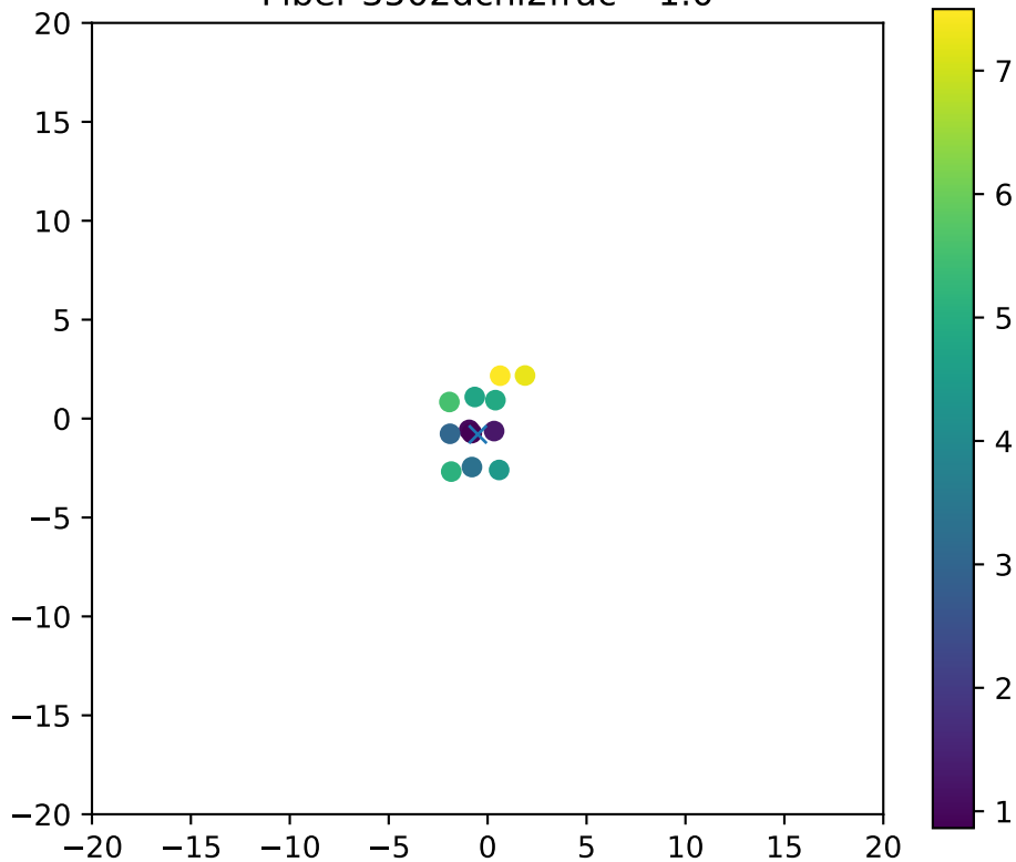
Fiber 3502dchi2frac= 1.0
