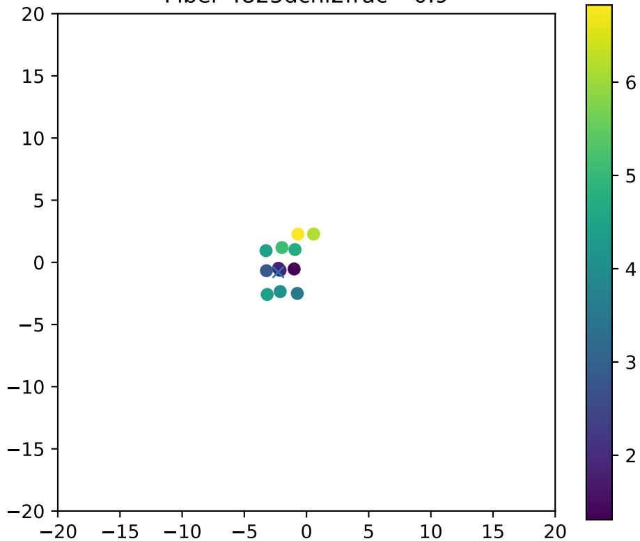
Fiber 4825dchi2frac= 0.9
