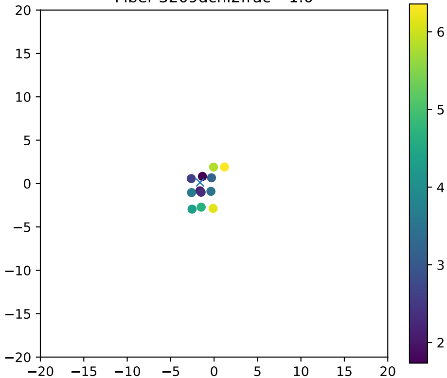
Fiber 3209dchi2frac= 1.0
