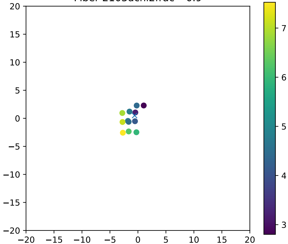
Fiber 2103dchi2frac= 0.9
