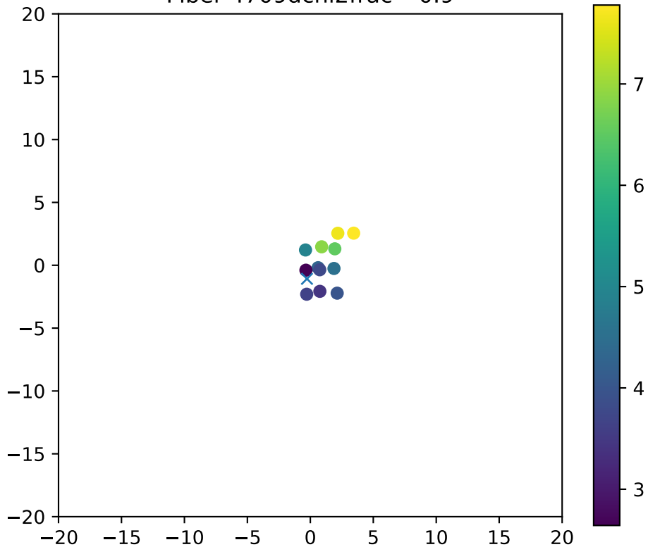
Fiber 4709dchi2frac= 0.9
