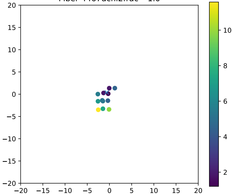
Fiber 4467dchi2frac= 1.0
