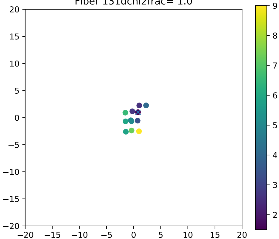
Fiber 131dchi2frac= 1.0
