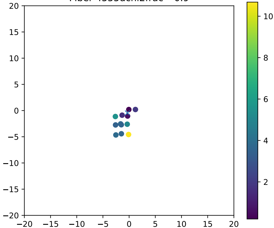
Fiber 4555dchi2frac= 0.9
