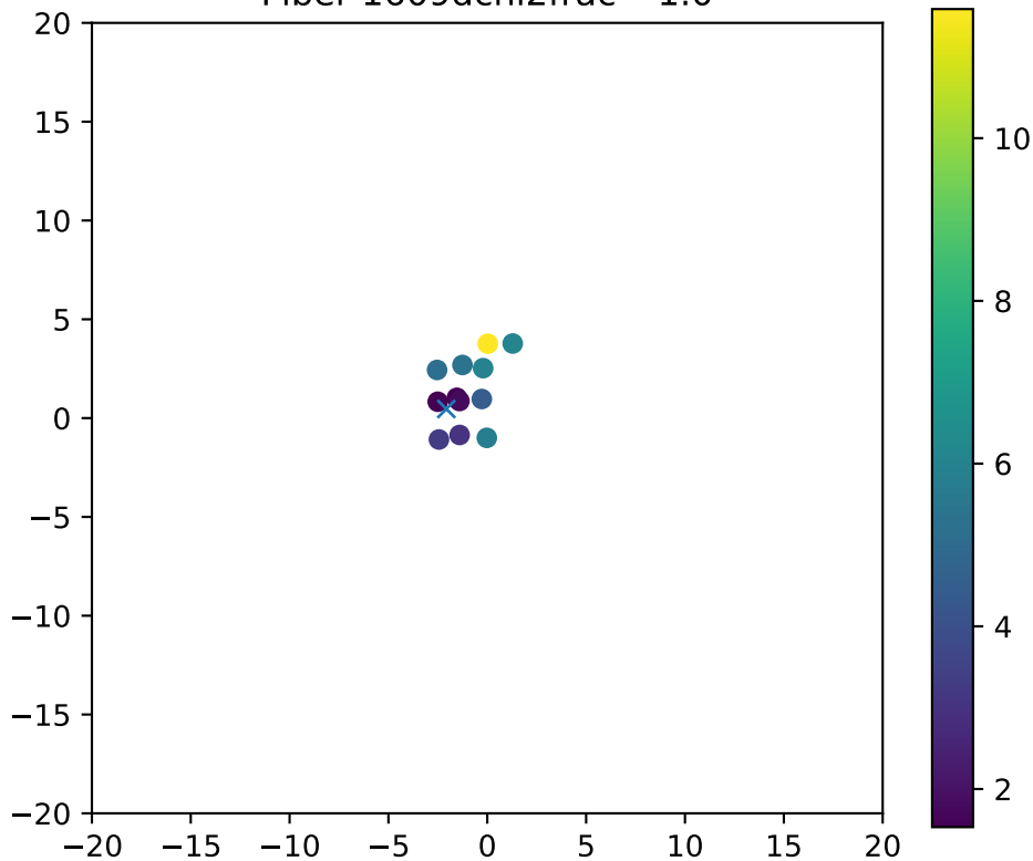
Fiber 1609dchi2frac= 1.0
