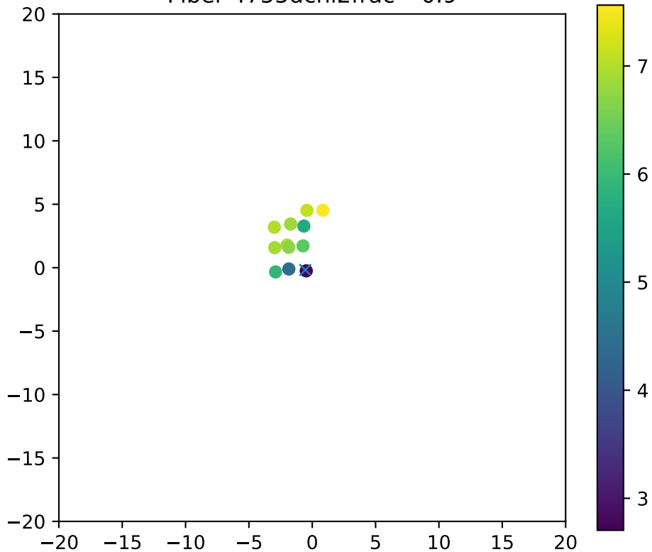
Fiber 4755dchi2frac= 0.9
