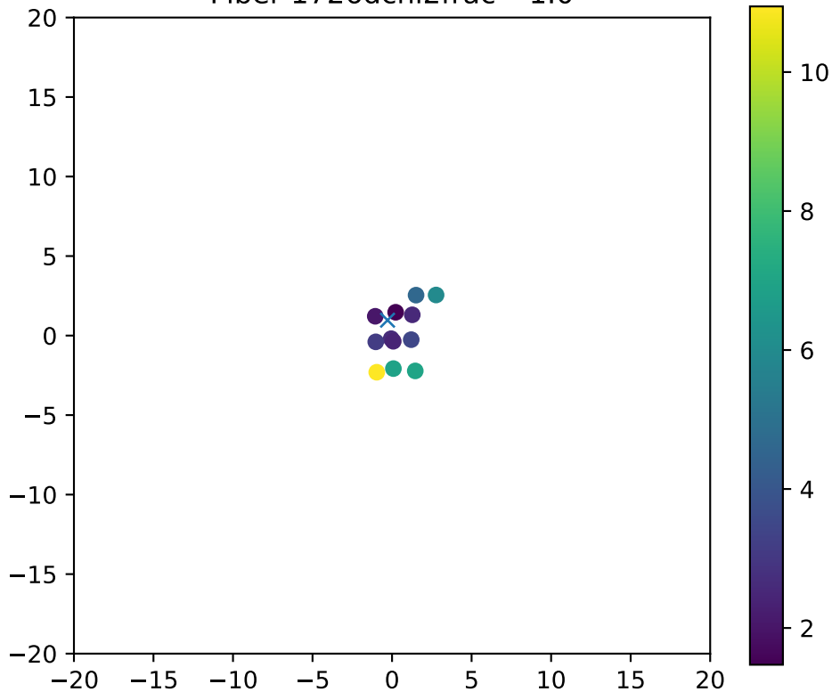
Fiber 1726dchi2frac= 1.0
