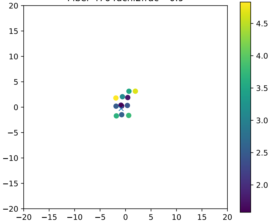
Fiber 4764dchi2frac= 0.9
