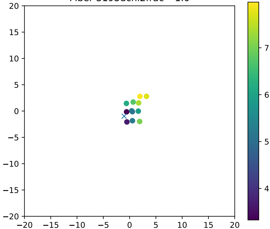
Fiber 3193dchi2frac= 1.0
