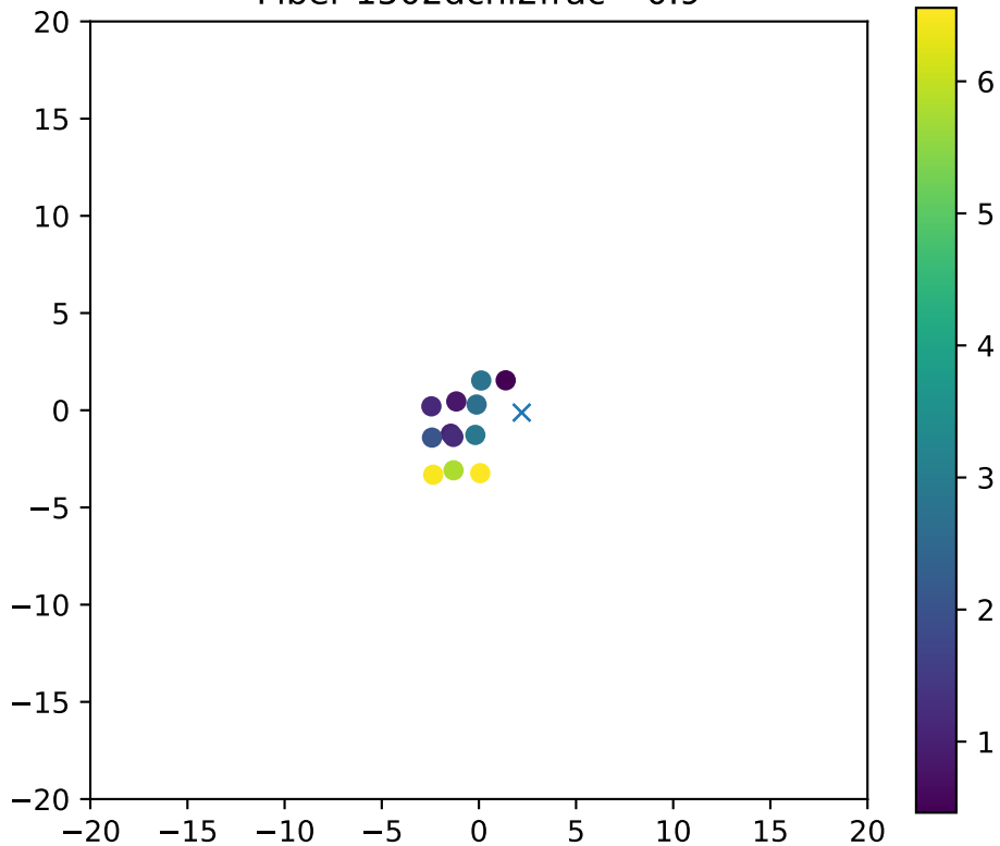
Fiber 1502dchi2frac= 0.9
