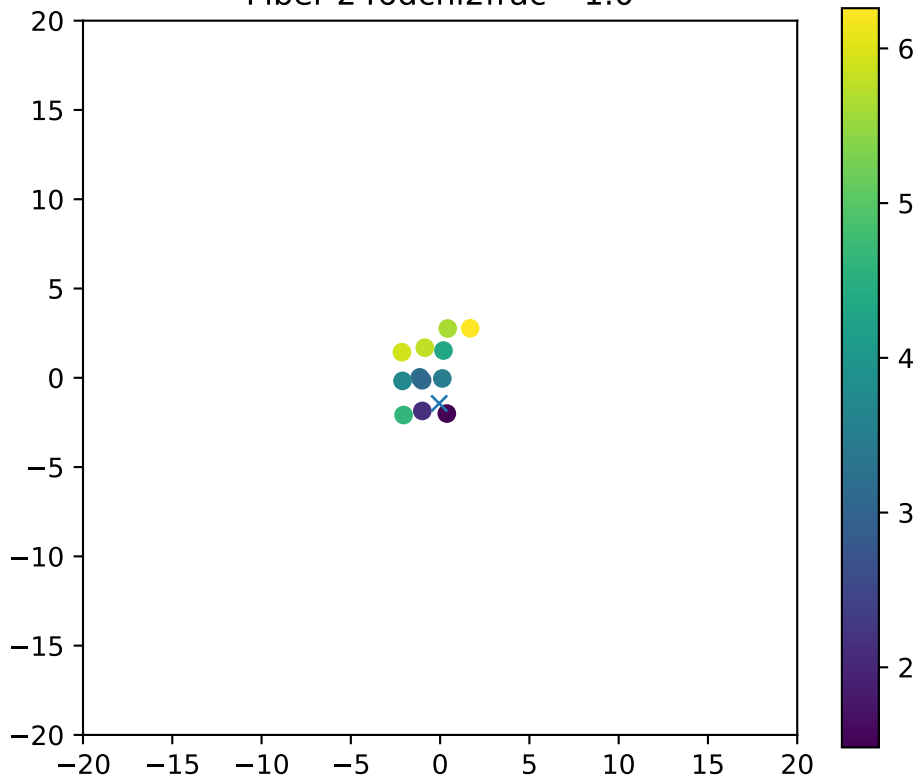
Fiber 246dchi2frac= 1.0
