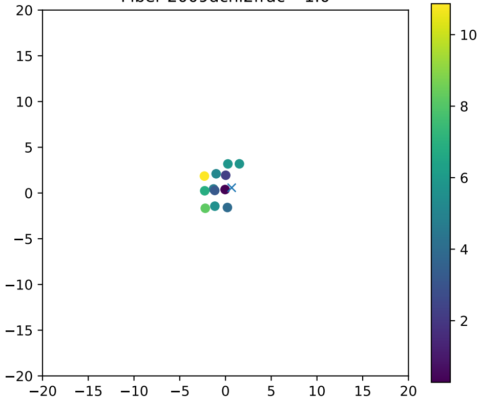
Fiber 2009dchi2frac= 1.0
