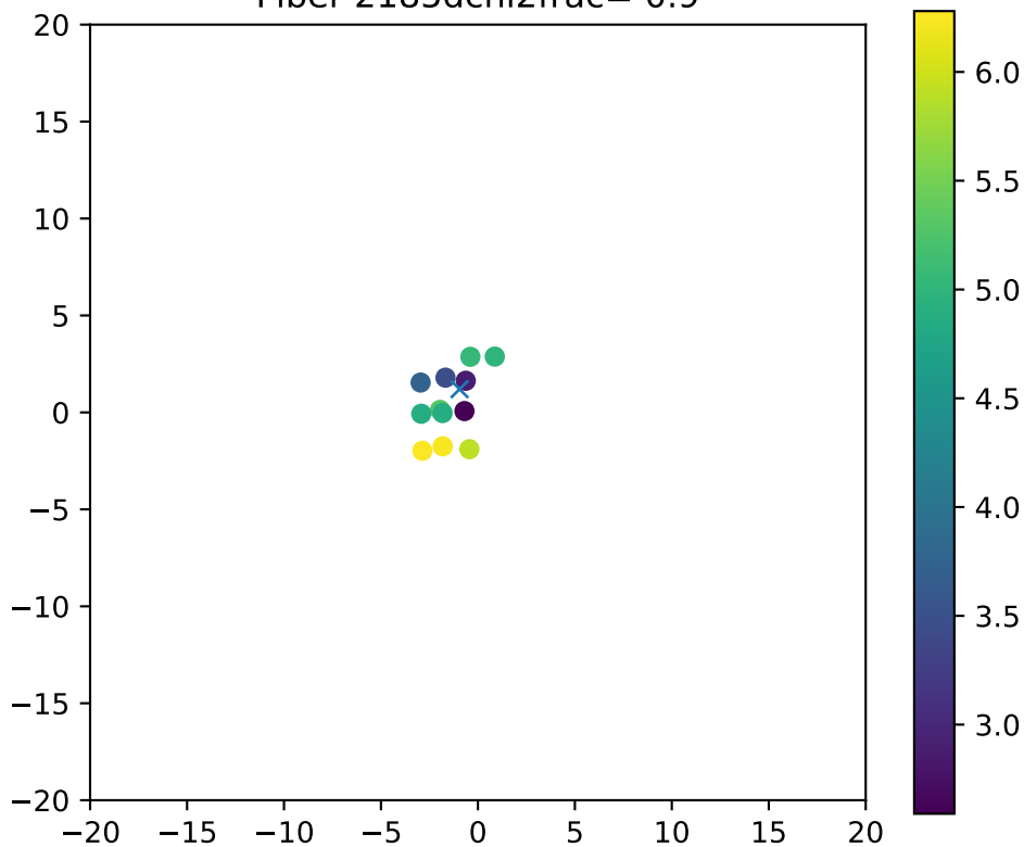
Fiber 2185dchi2frac= 0.9
