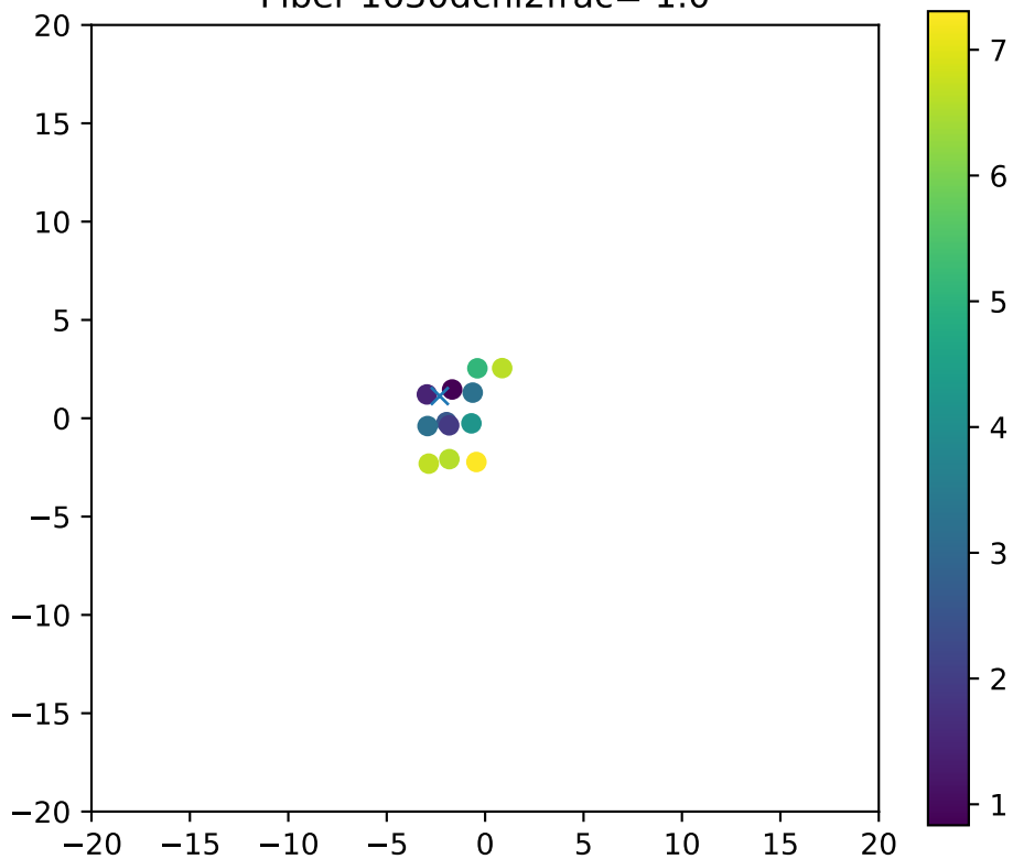
Fiber 1630dchi2frac= 1.0
