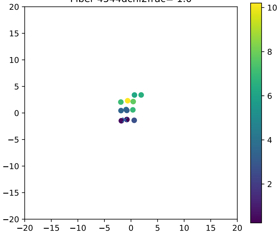
Fiber 4544dchi2frac= 1.0
