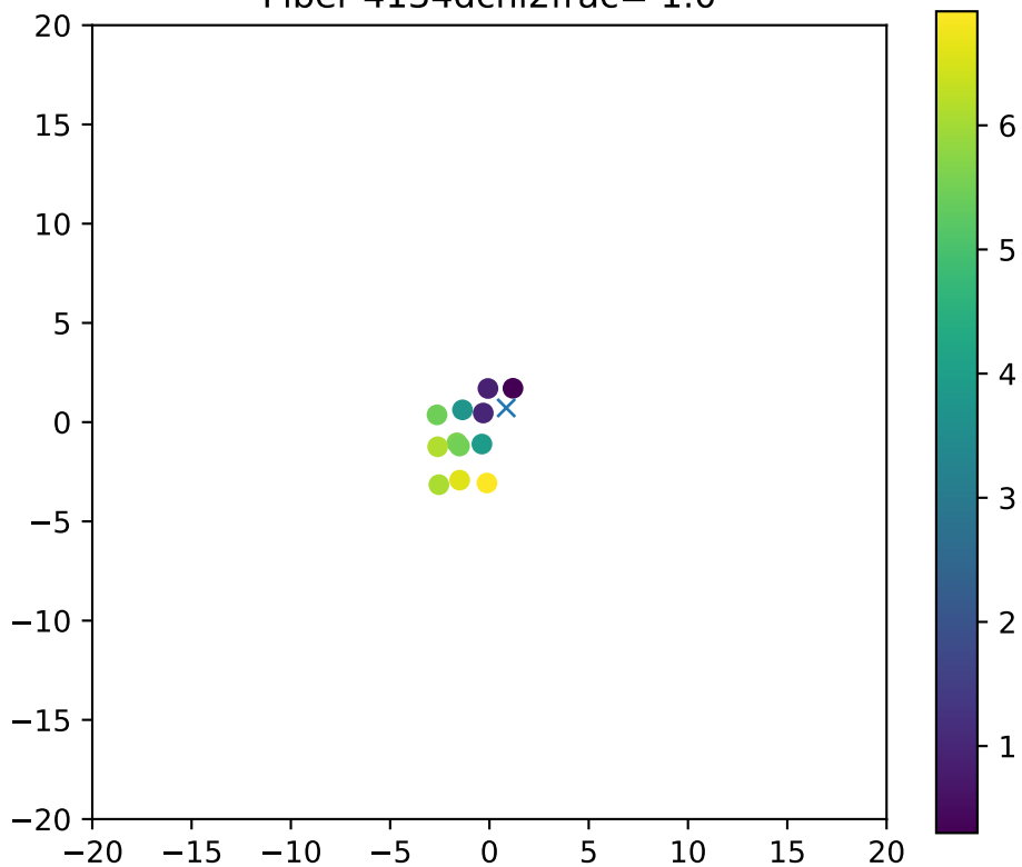
Fiber 4134dchi2frac= 1.0
