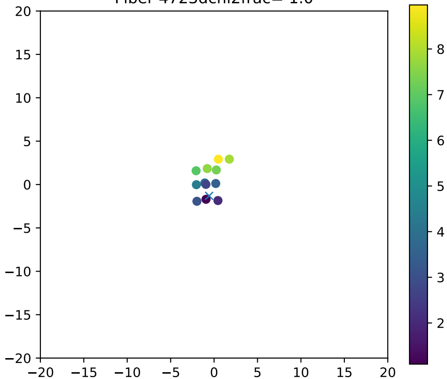
Fiber 4723dchi2frac= 1.0
