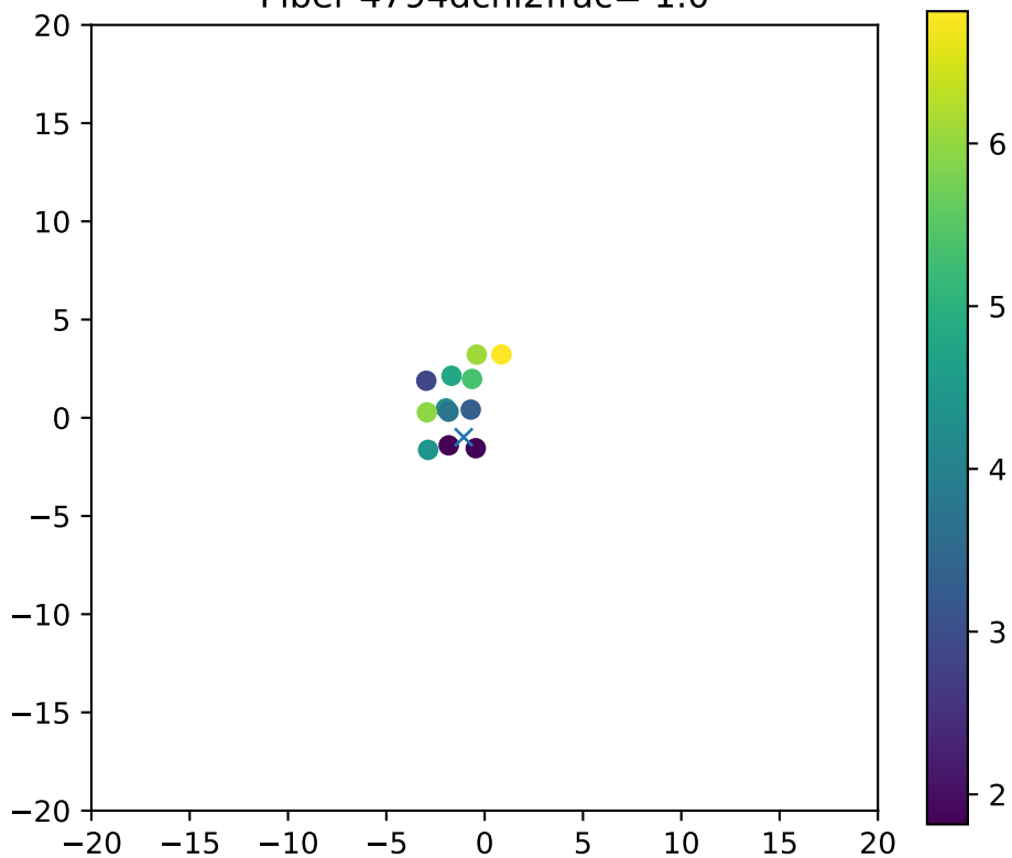
Fiber 4794dchi2frac= 1.0
