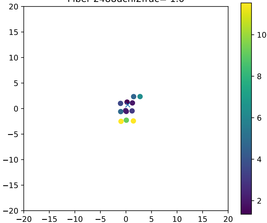
Fiber 2488dchi2frac= 1.0
