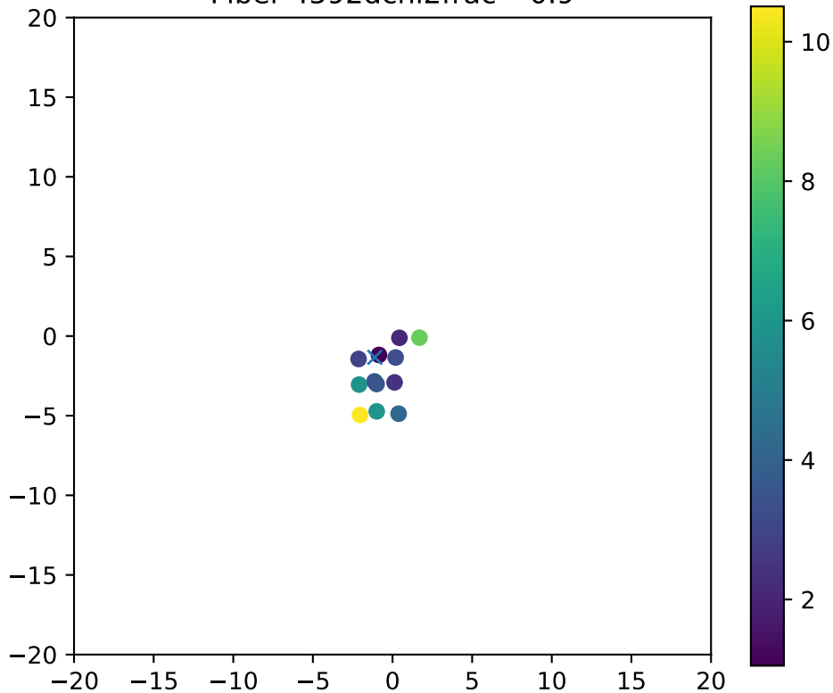
Fiber 4592dchi2frac= 0.9
