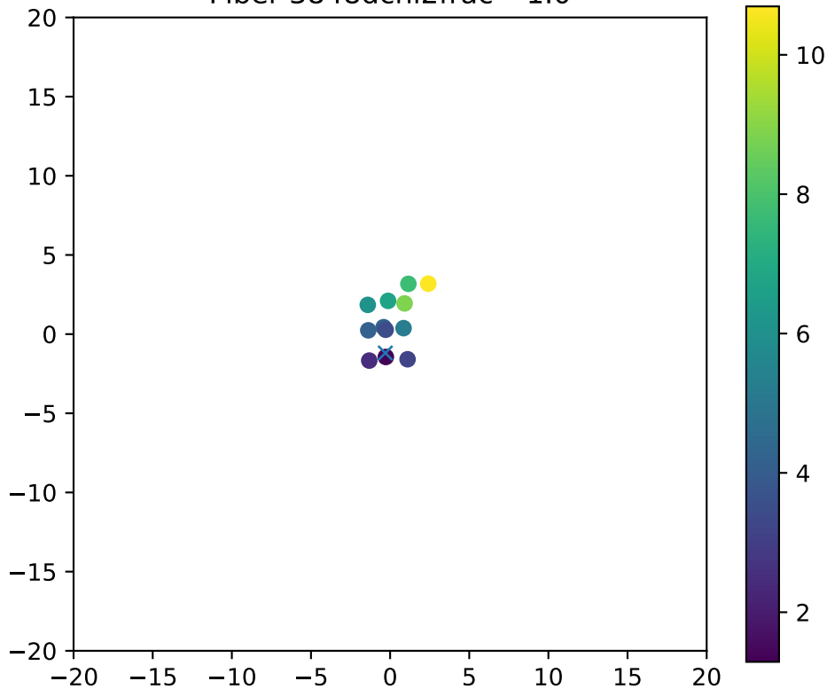
Fiber 3848dchi2frac= 1.0
