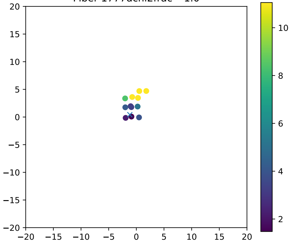
Fiber 1777dchi2frac= 1.0
