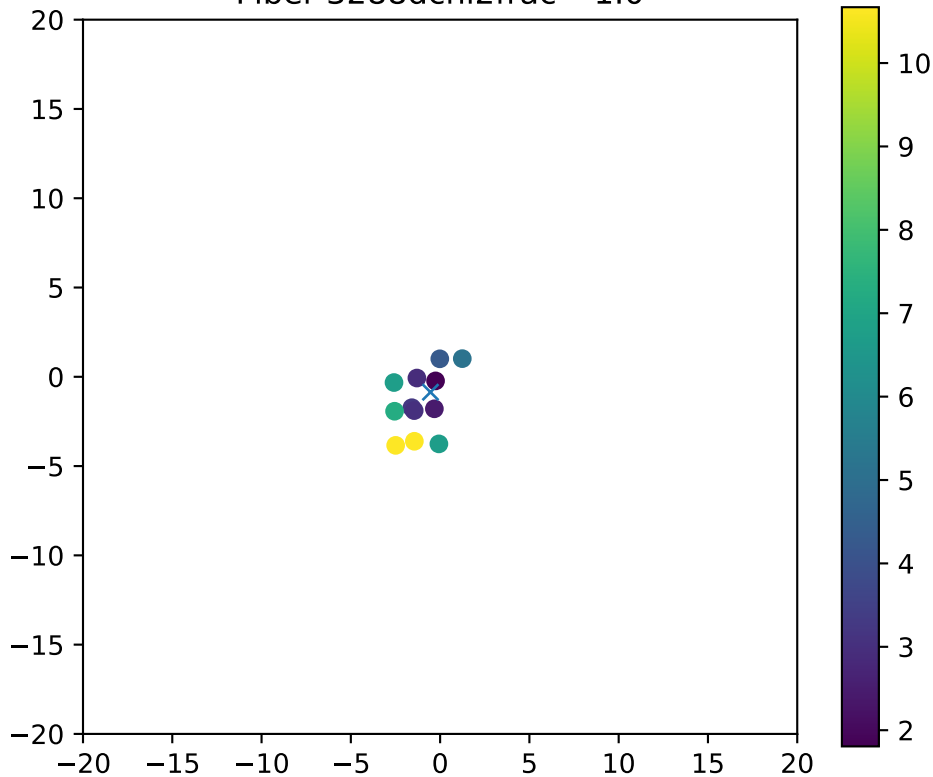
Fiber 3288dchi2frac= 1.0
