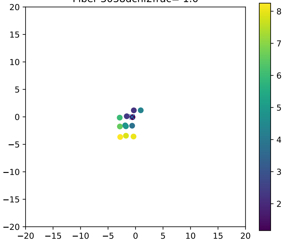
Fiber 3038dchi2frac= 1.0
