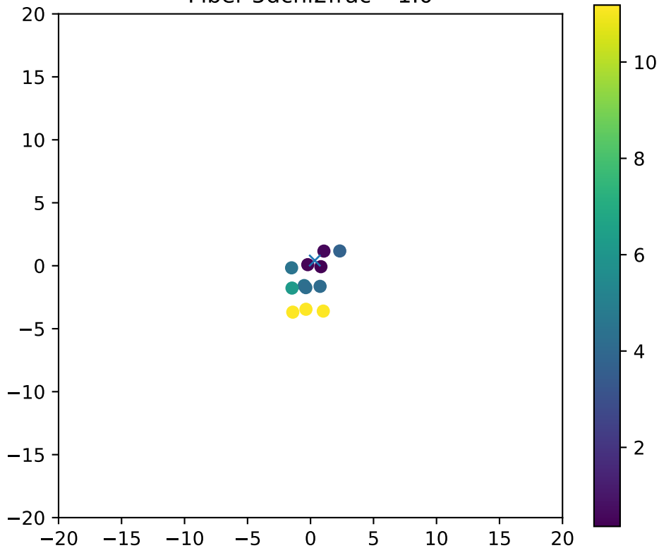
Fiber 5dchi2frac= 1.0
