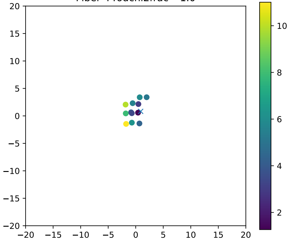
Fiber 446dchi2frac= 1.0
