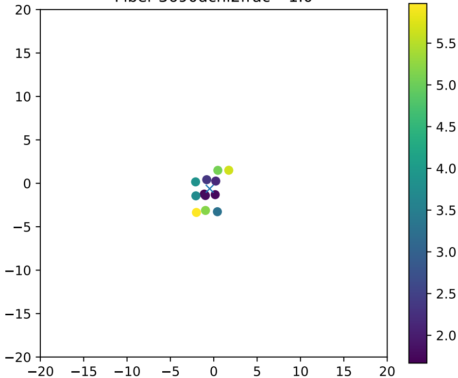
Fiber 3690dchi2frac= 1.0
