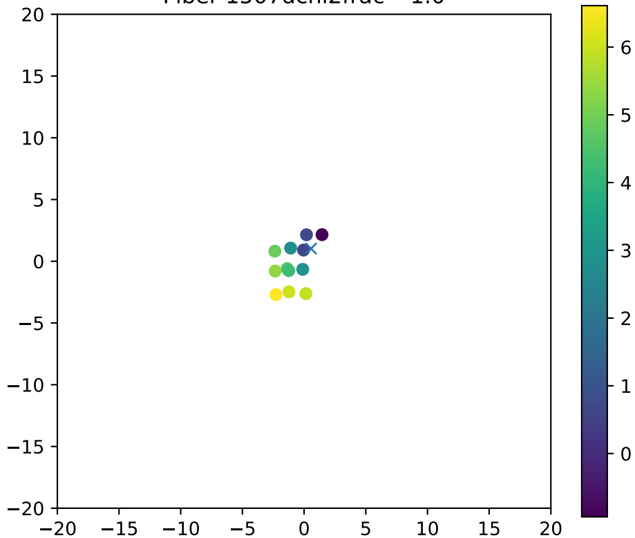
Fiber 1507dchi2frac= 1.0
