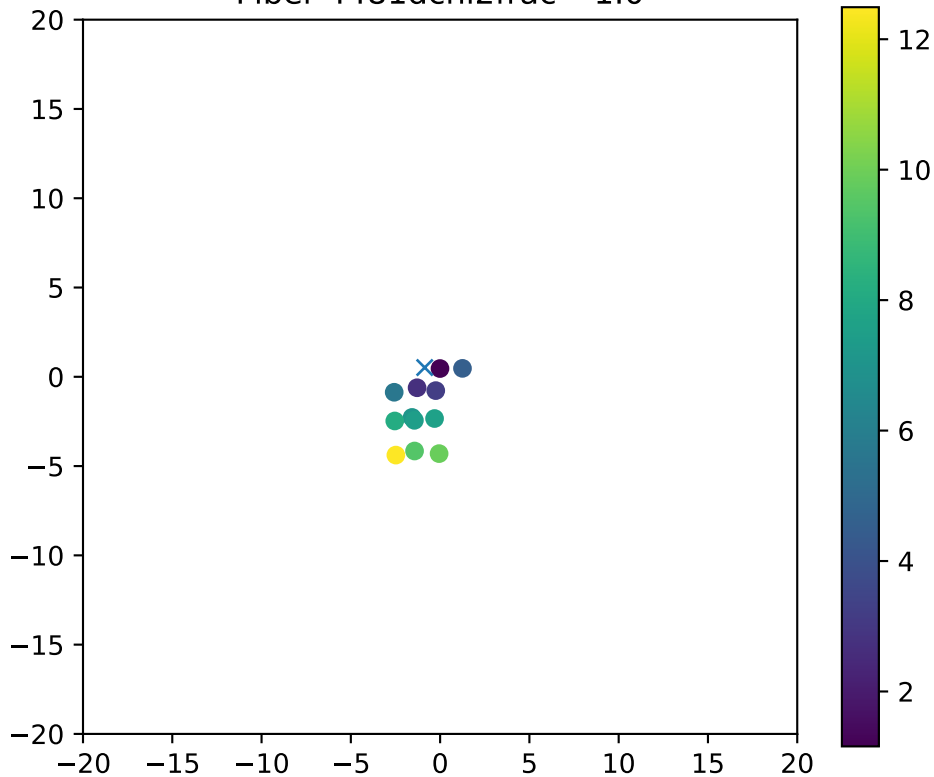
Fiber 4481dchi2frac= 1.0
