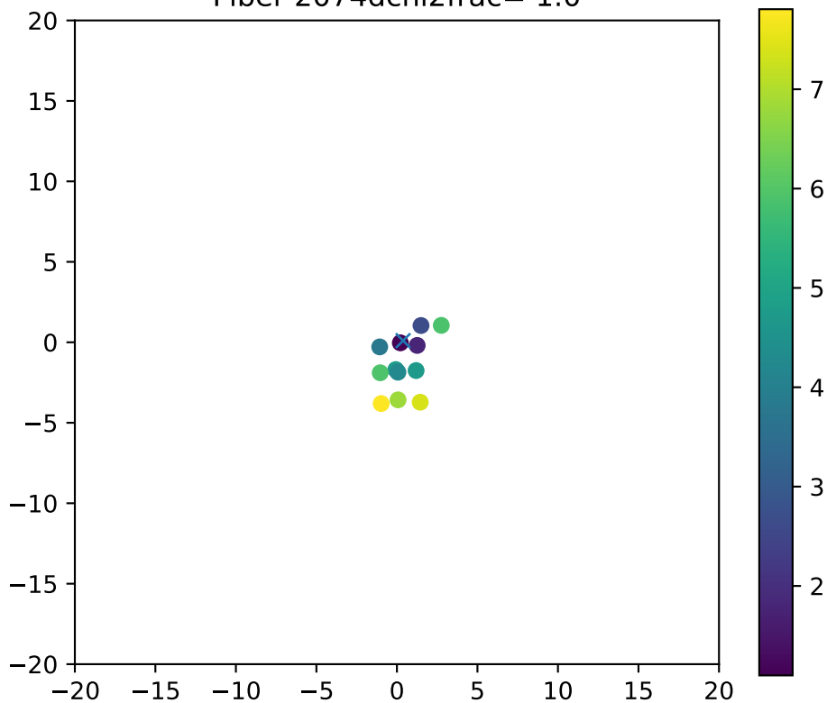
Fiber 2074dchi2frac= 1.0
