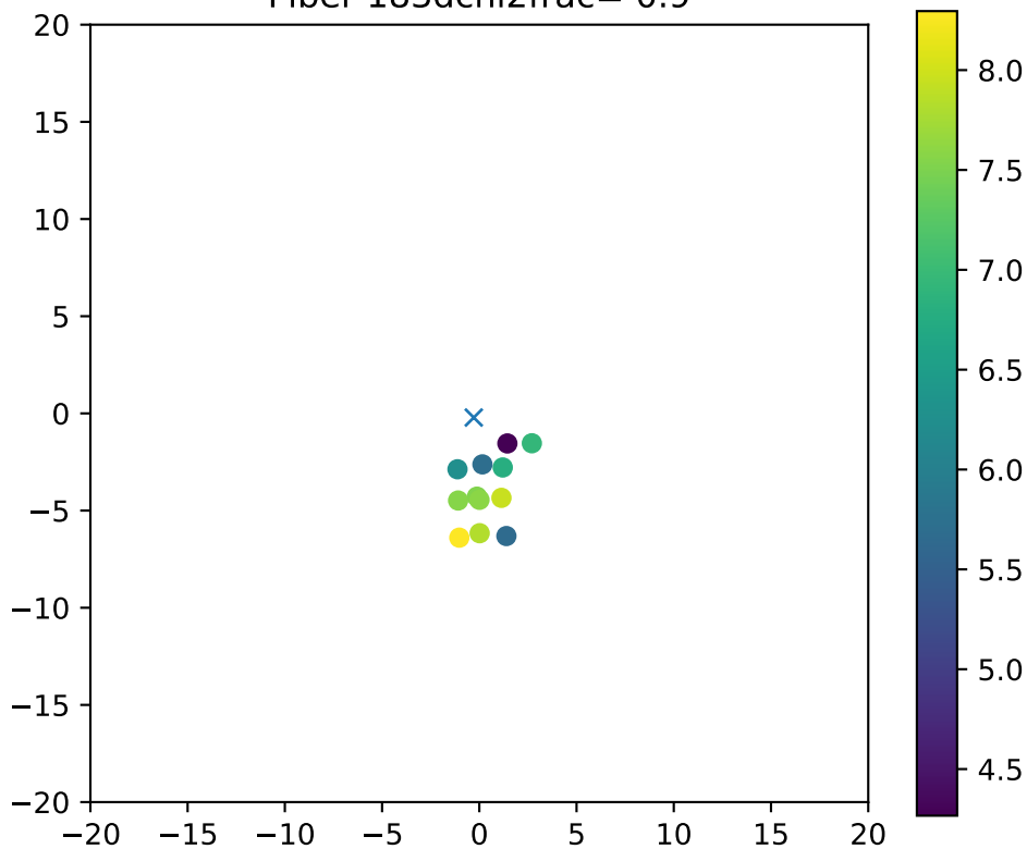
Fiber 183dchi2frac= 0.9
