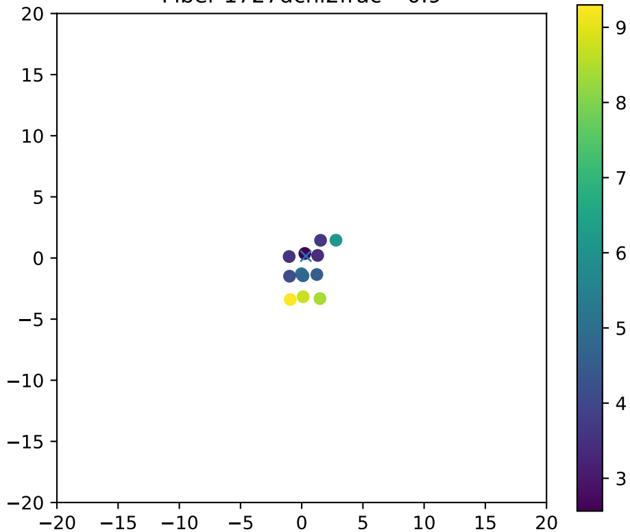
Fiber 1727dchi2frac= 0.9
