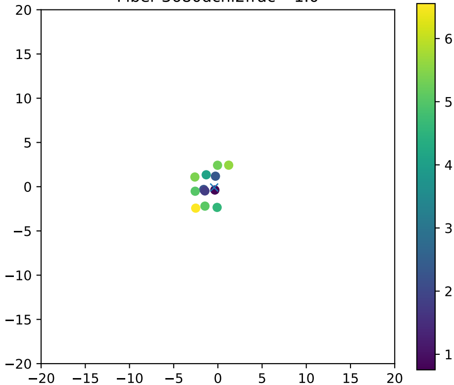
Fiber 3680dchi2frac= 1.0
