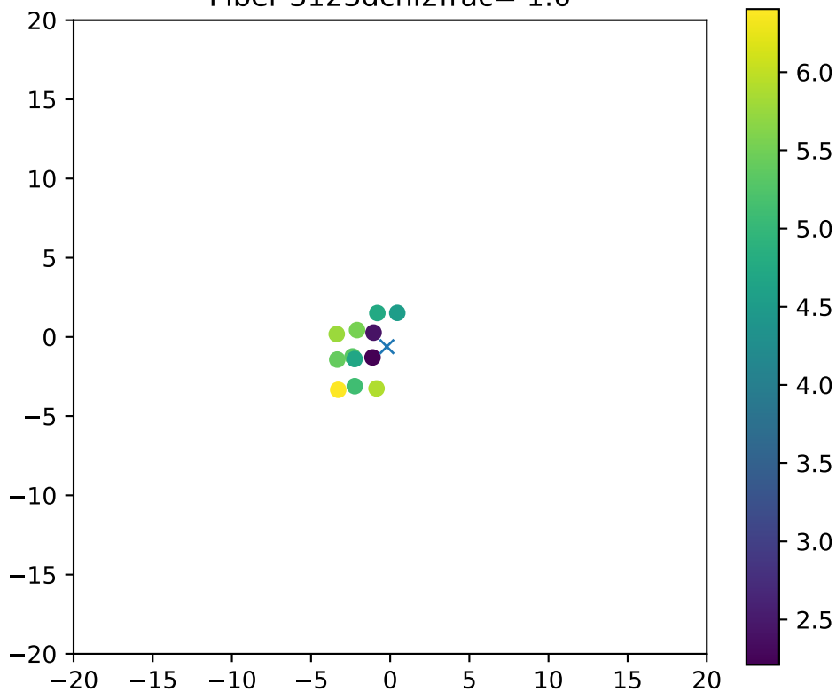
Fiber 3123dchi2frac= 1.0
