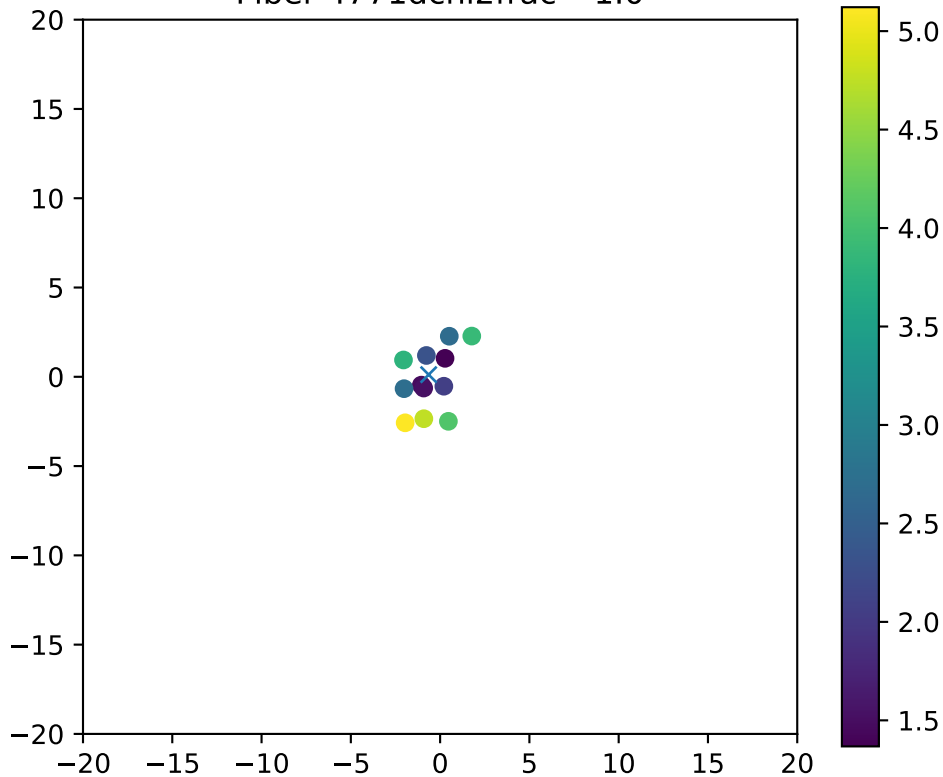
Fiber 4771dchi2frac= 1.0
