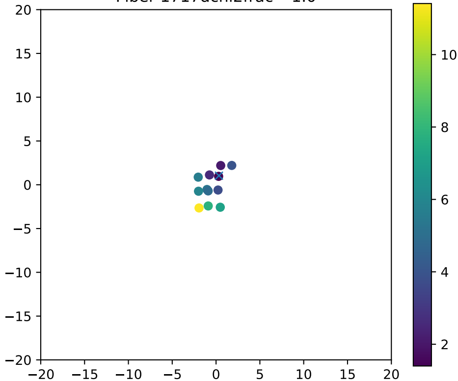
Fiber 1717dchi2frac= 1.0
