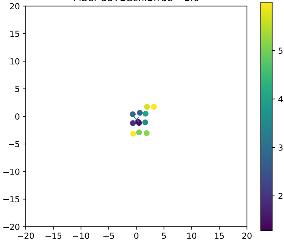
Fiber 3572dchi2frac= 1.0
