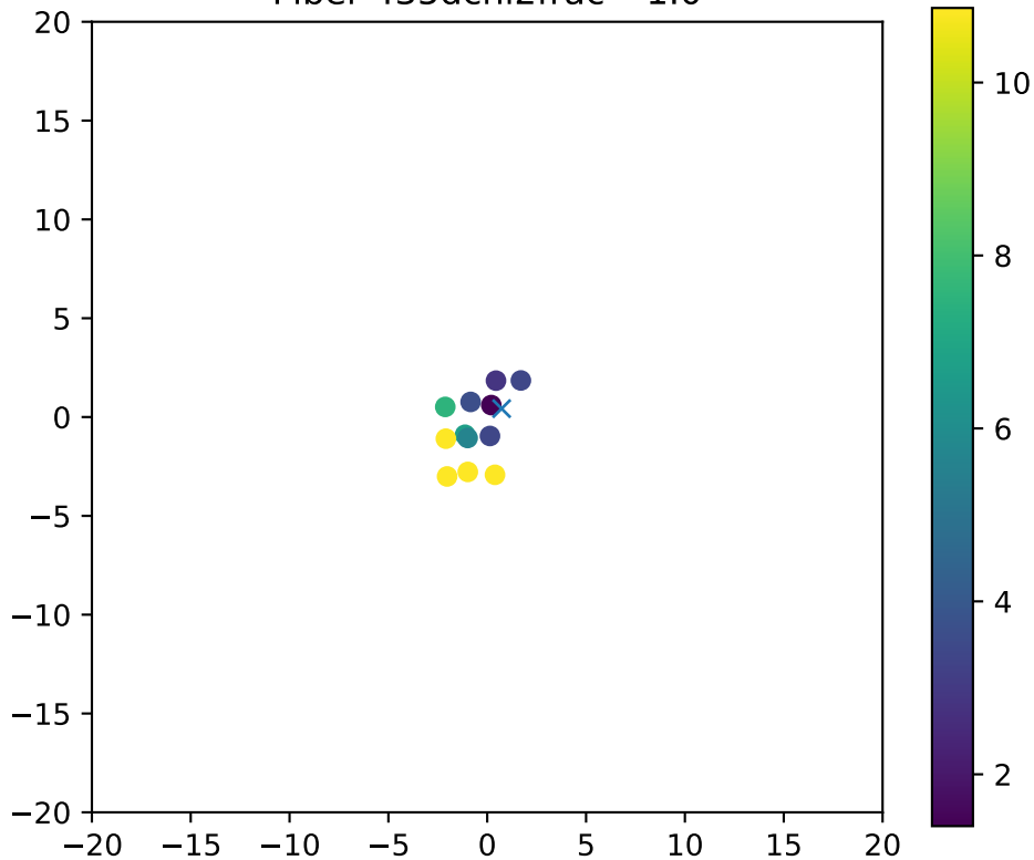
Fiber 435dchi2frac= 1.0
