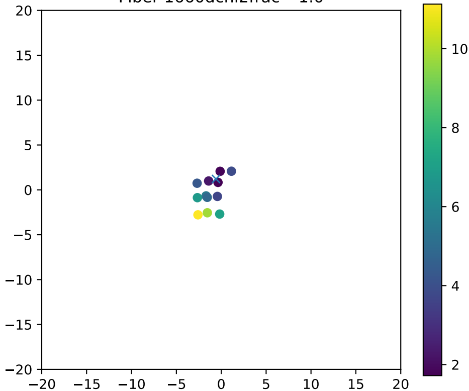
Fiber 1660dchi2frac= 1.0
