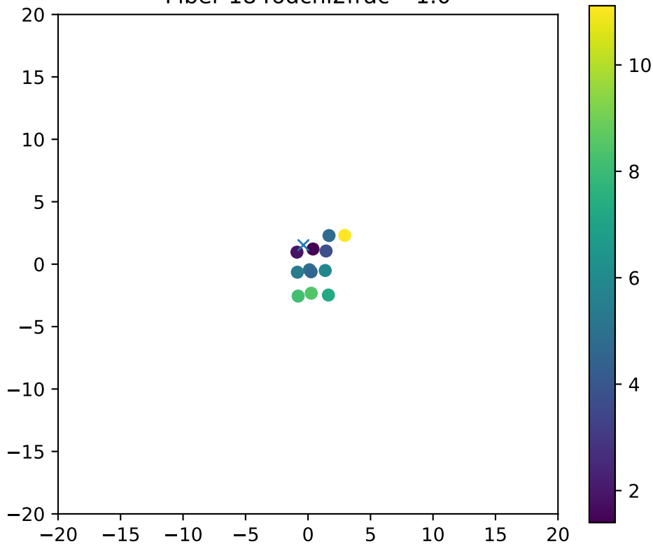
Fiber 1846dchi2frac= 1.0
