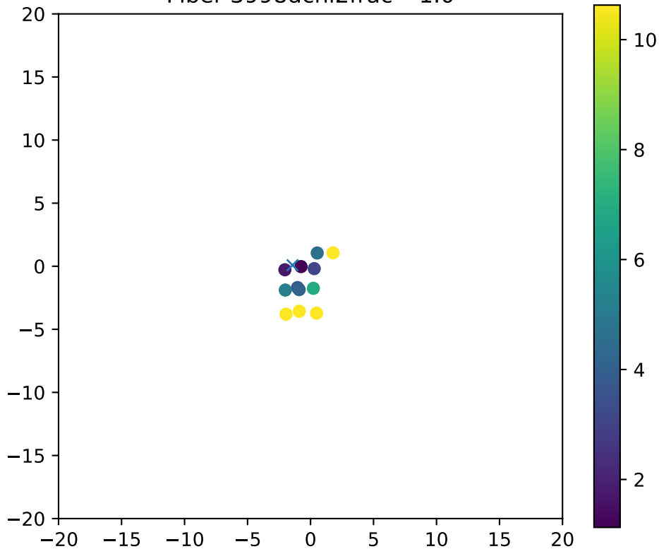
Fiber 3998dchi2frac= 1.0
