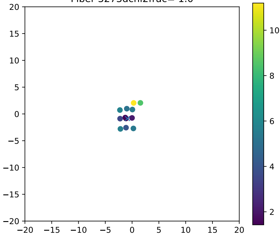
Fiber 3273dchi2frac= 1.0
