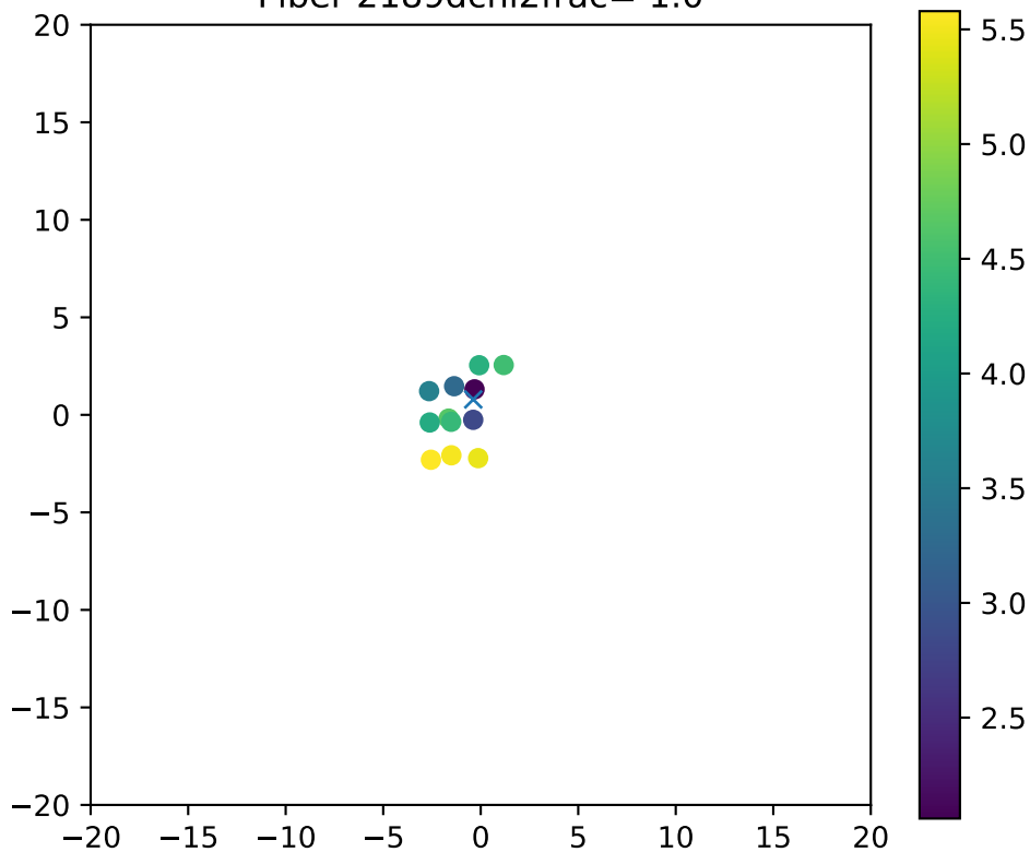
Fiber 2189dchi2frac= 1.0
