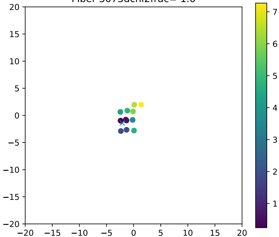
Fiber 3073dchi2frac= 1.0
