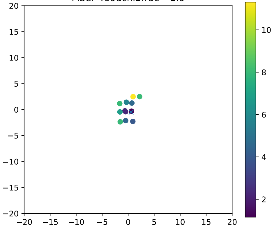
Fiber 460dchi2frac= 1.0
