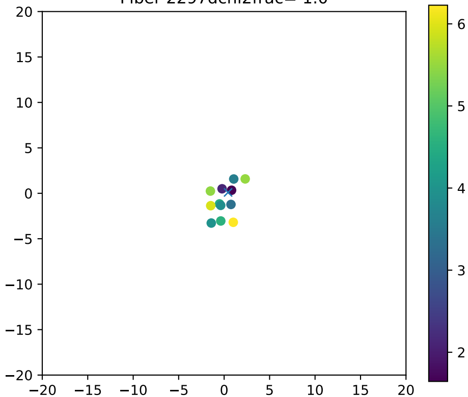
Fiber 2297dchi2frac= 1.0
