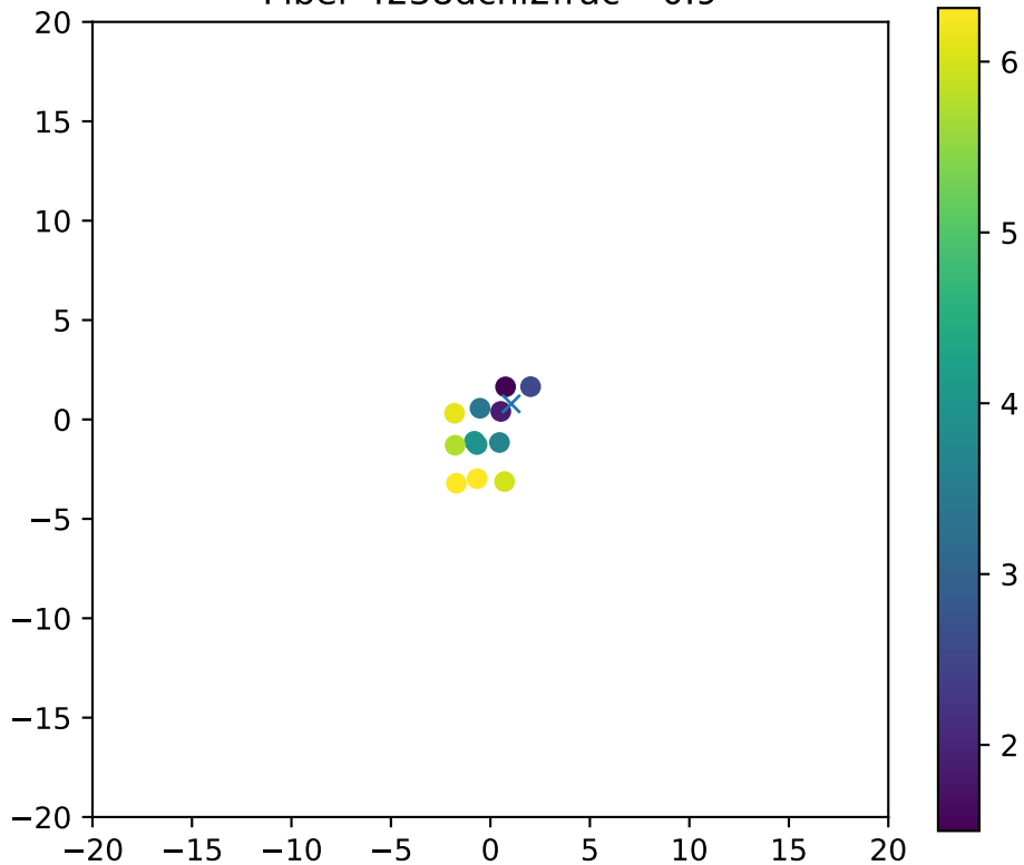
Fiber 4238dchi2frac= 0.9
