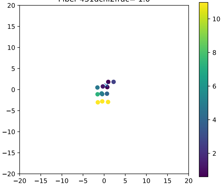
Fiber 431dchi2frac= 1.0
