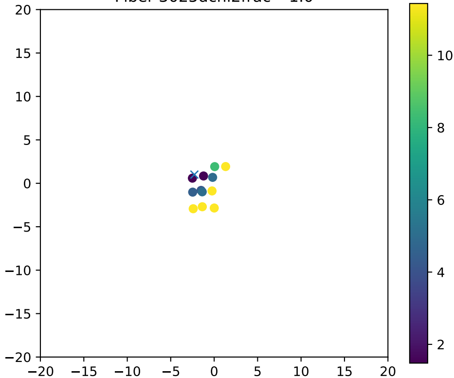
Fiber 3025dchi2frac= 1.0
