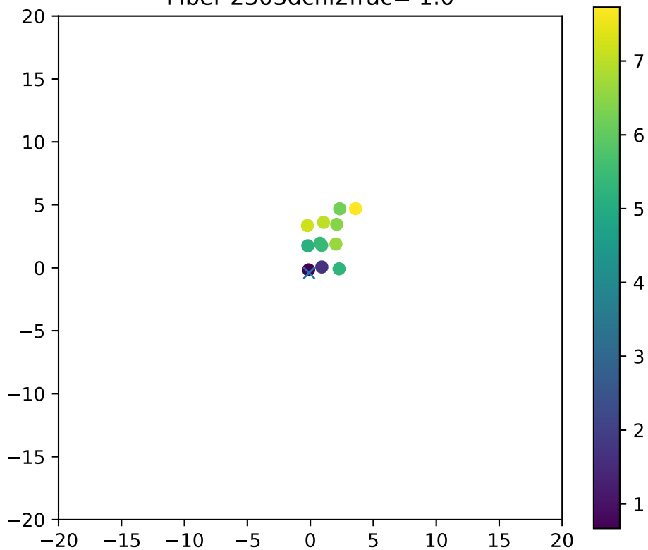
Fiber 2303dchi2frac= 1.0
