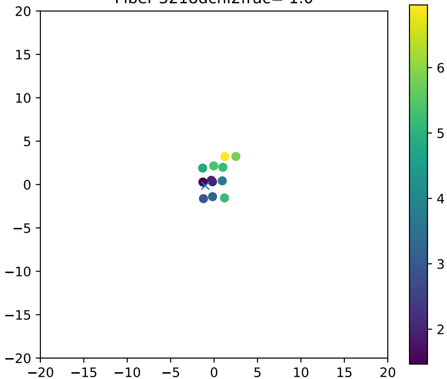
Fiber 3218dchi2frac= 1.0
