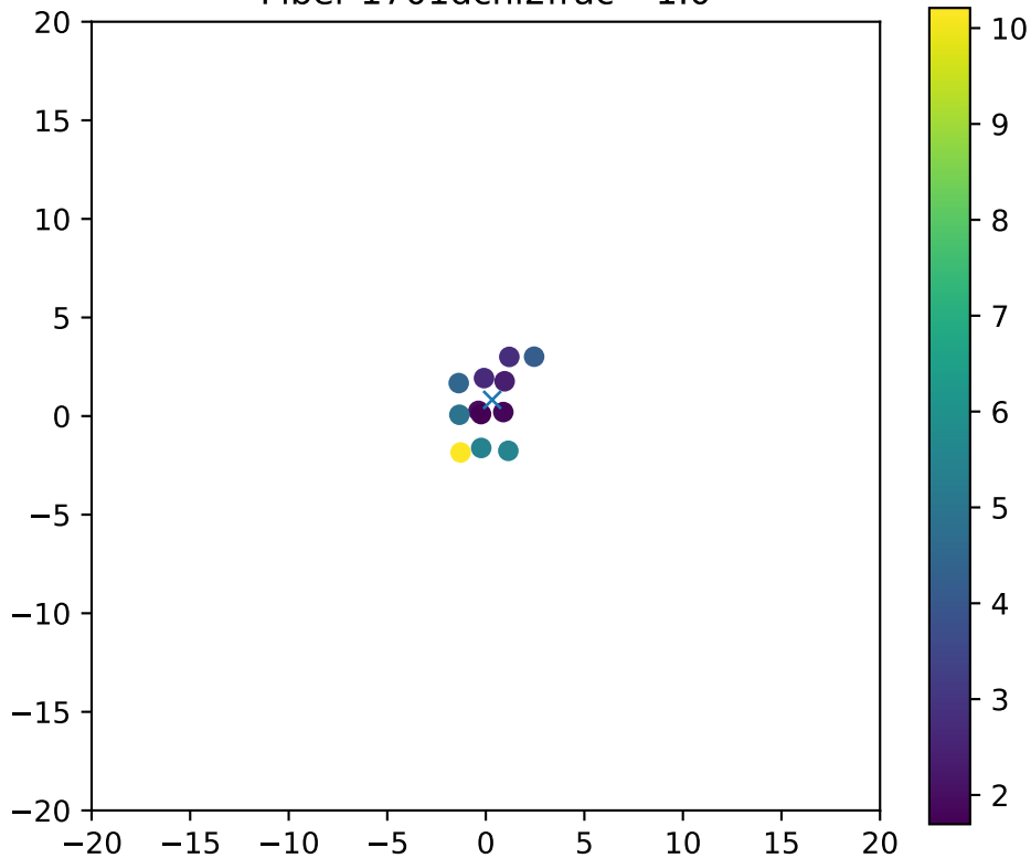
Fiber 1701dchi2frac= 1.0
