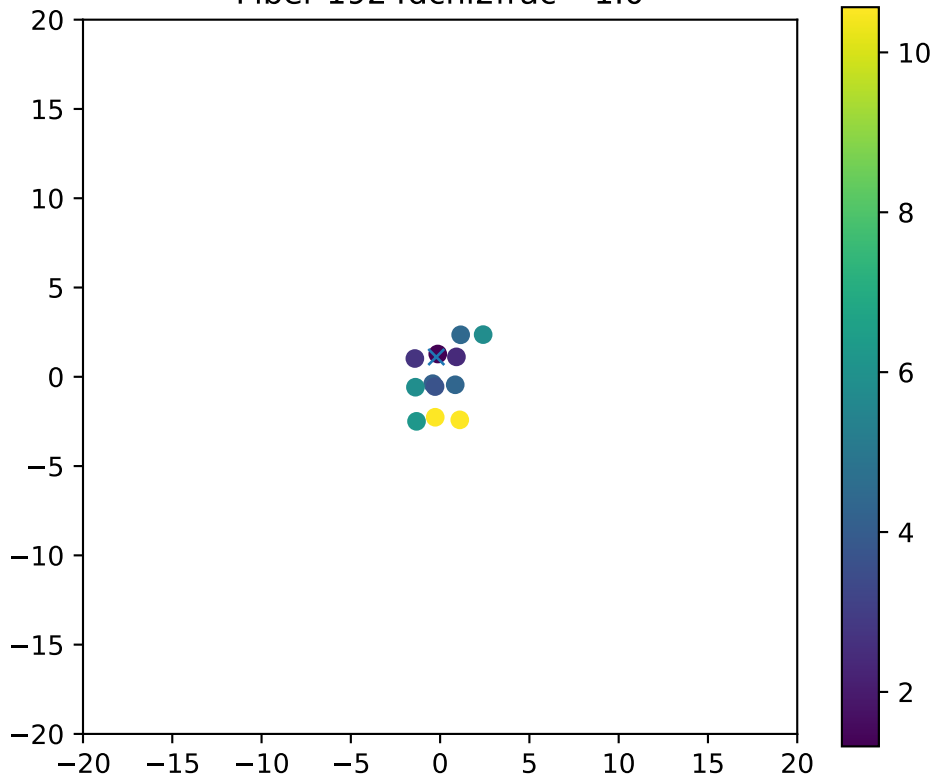
Fiber 1924dchi2frac= 1.0
