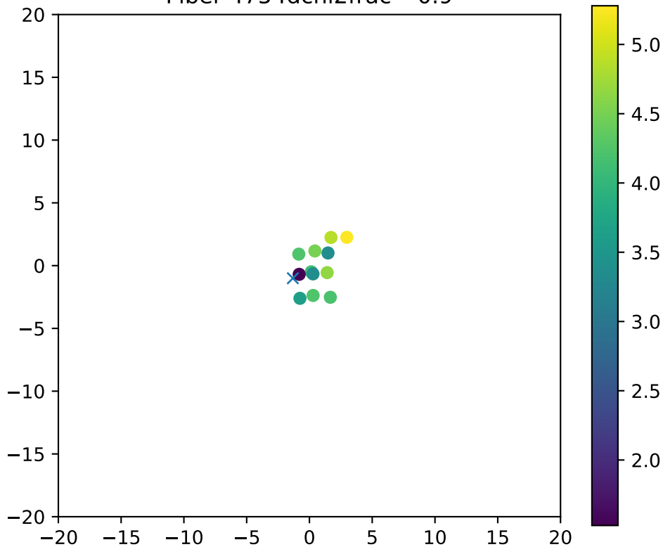
Fiber 4754dchi2frac= 0.9
