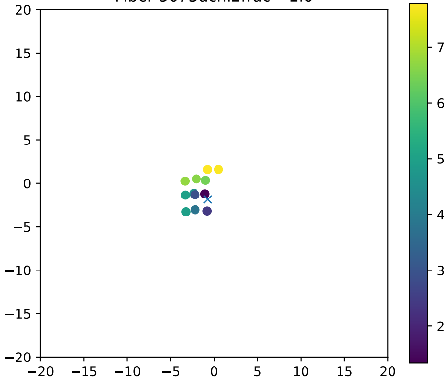
Fiber 3075dchi2frac= 1.0
