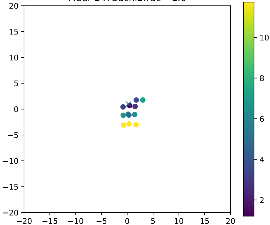
Fiber 2473dchi2frac= 1.0
