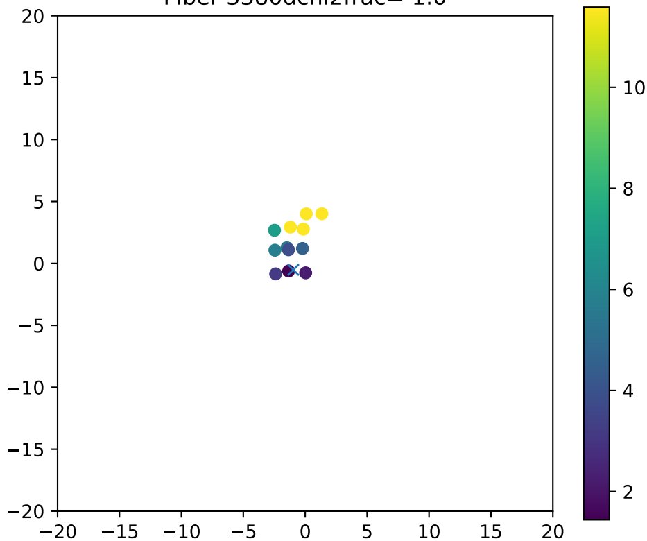
Fiber 3380dchi2frac= 1.0
