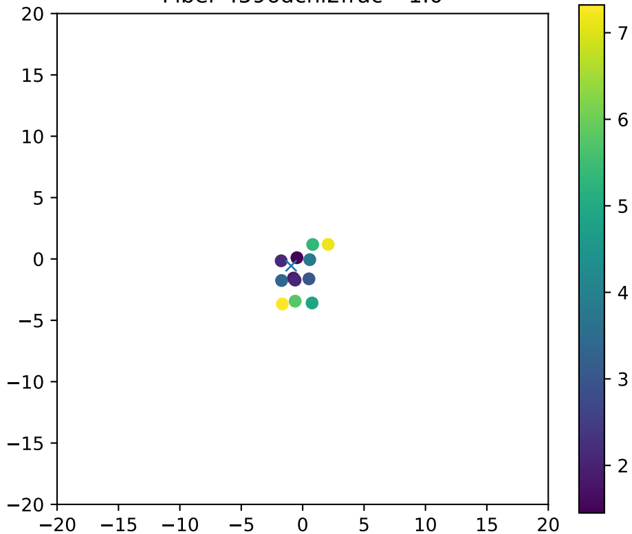
Fiber 4596dchi2frac= 1.0
