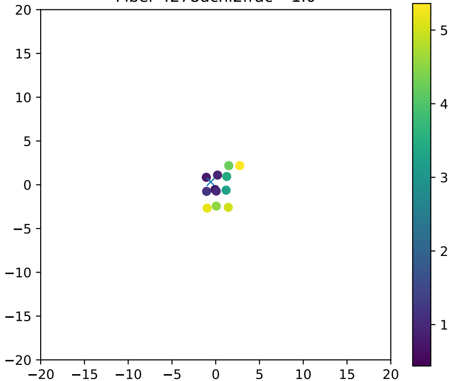
Fiber 4278dchi2frac= 1.0
