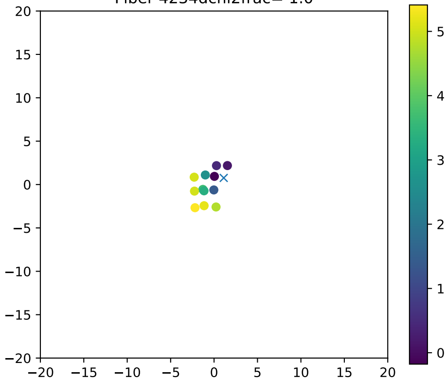
Fiber 4234dchi2frac= 1.0
