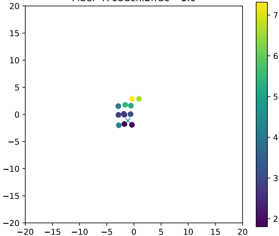
Fiber 4703dchi2frac= 1.0
