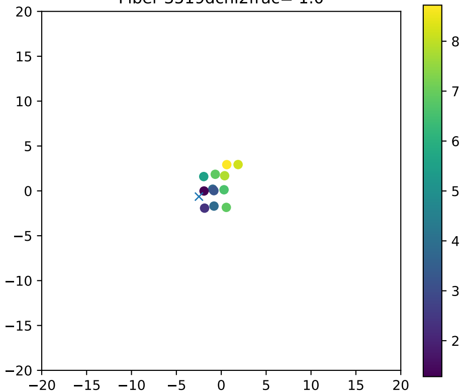
Fiber 3519dchi2frac= 1.0
