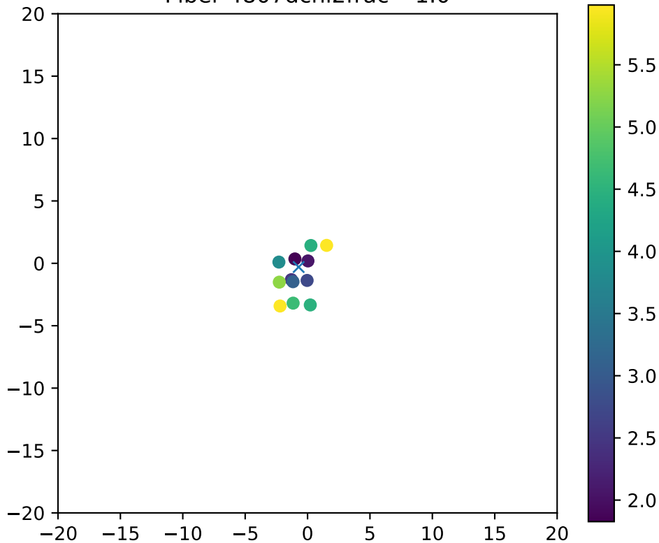
Fiber 4807dchi2frac= 1.0
