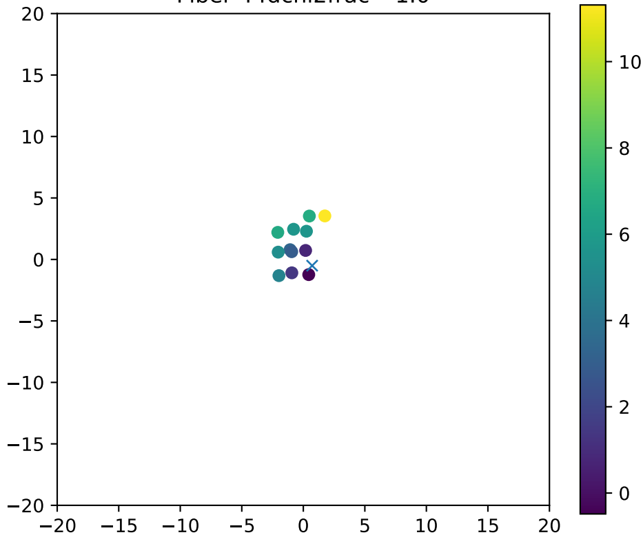
Fiber 44dchi2frac= 1.0
