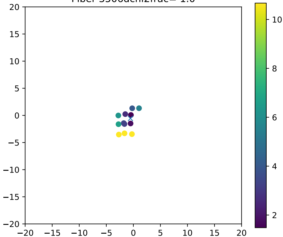
Fiber 3506dchi2frac= 1.0
