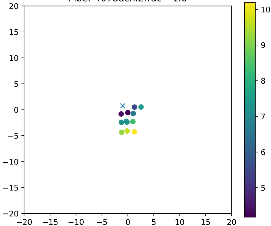
Fiber 4078dchi2frac= 1.0
