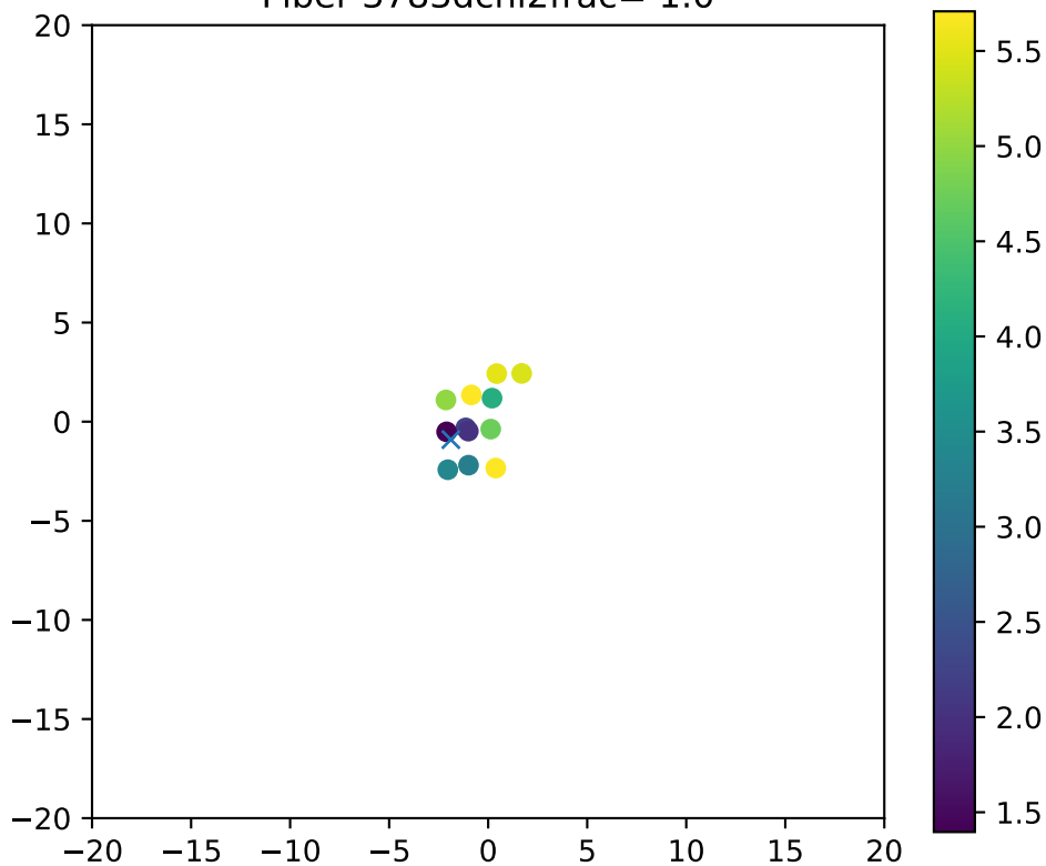
Fiber 3783dchi2frac= 1.0
