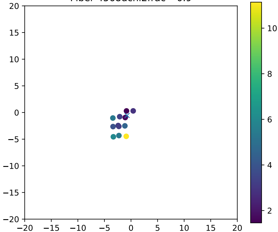
Fiber 4568dchi2frac= 0.9
