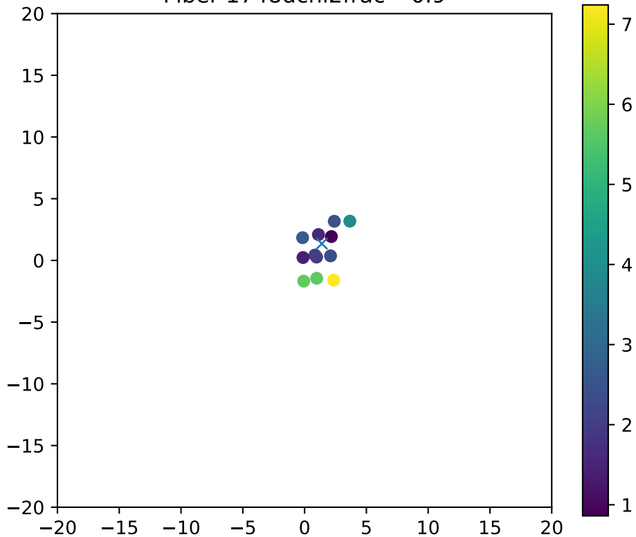
Fiber 1748dchi2frac= 0.9
