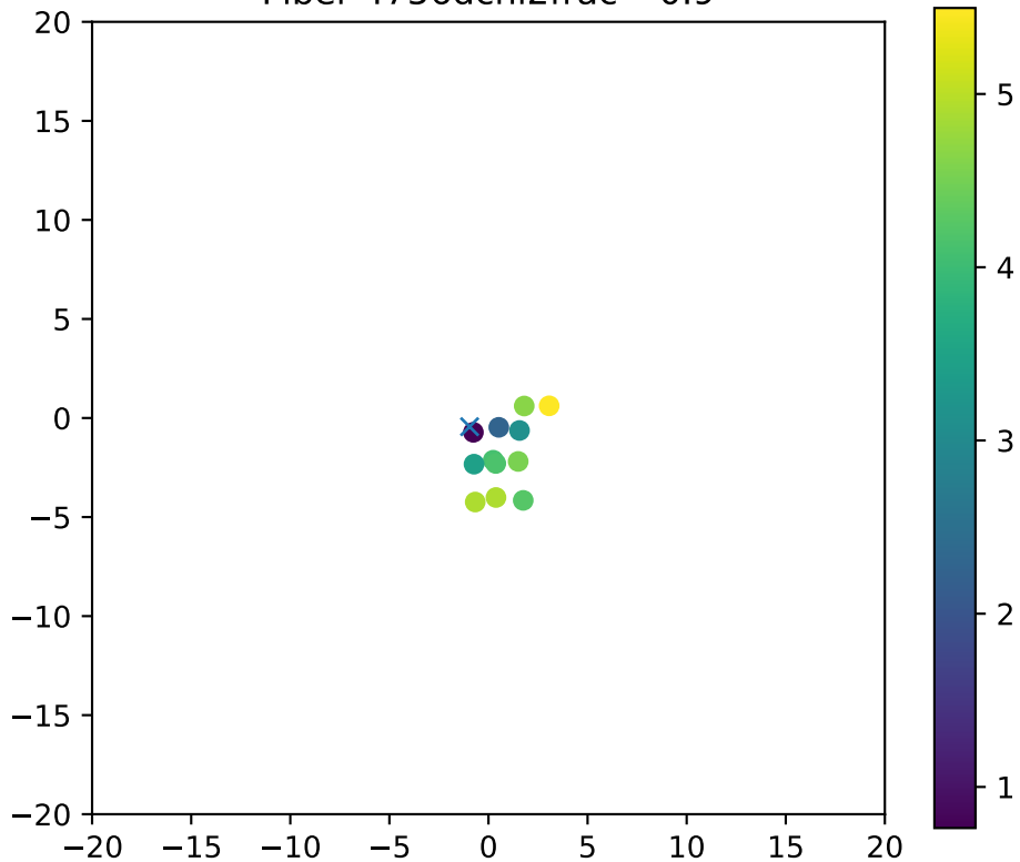
Fiber 4756dchi2frac= 0.9
