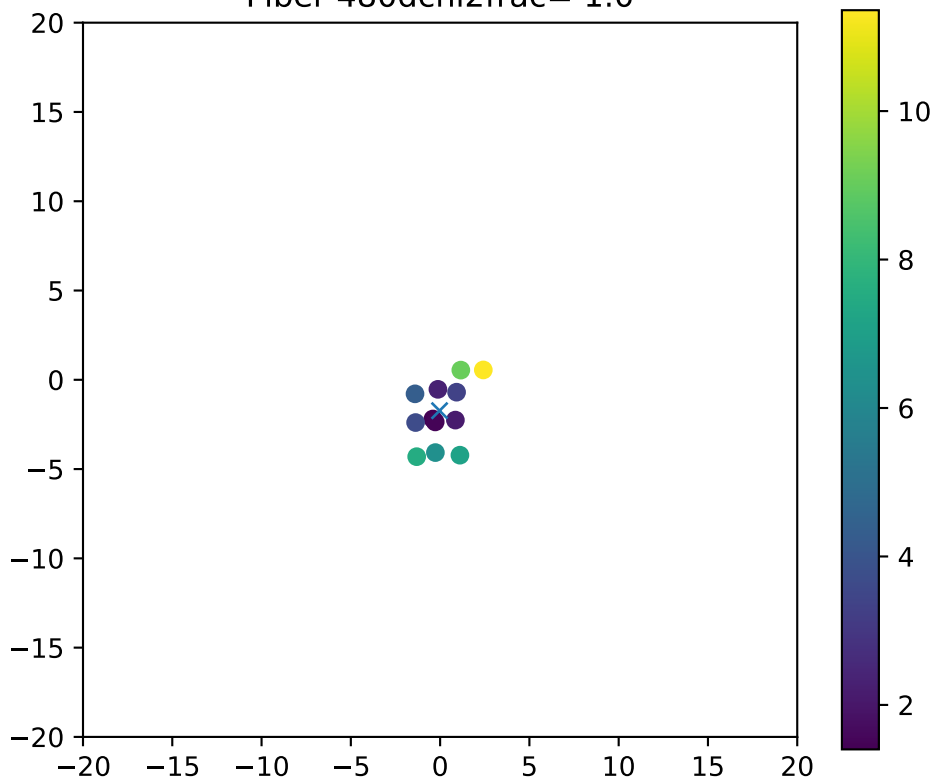
Fiber 480dchi2frac= 1.0
