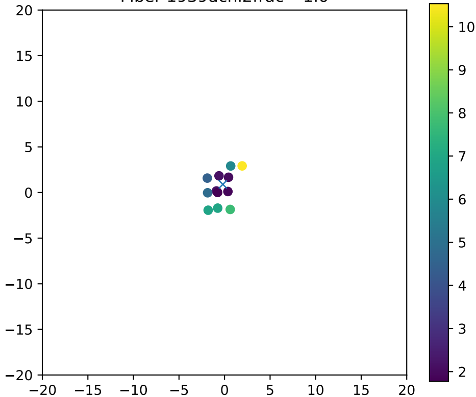
Fiber 1939dchi2frac= 1.0
