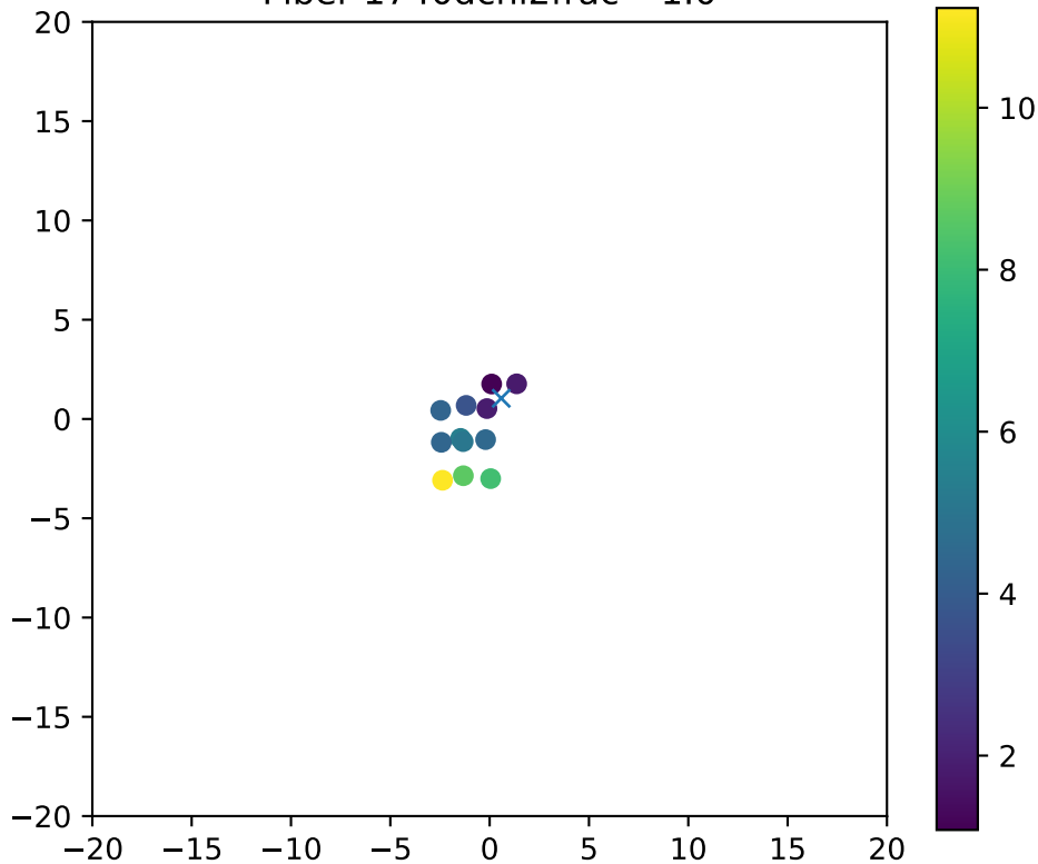
Fiber 1740dchi2frac= 1.0
