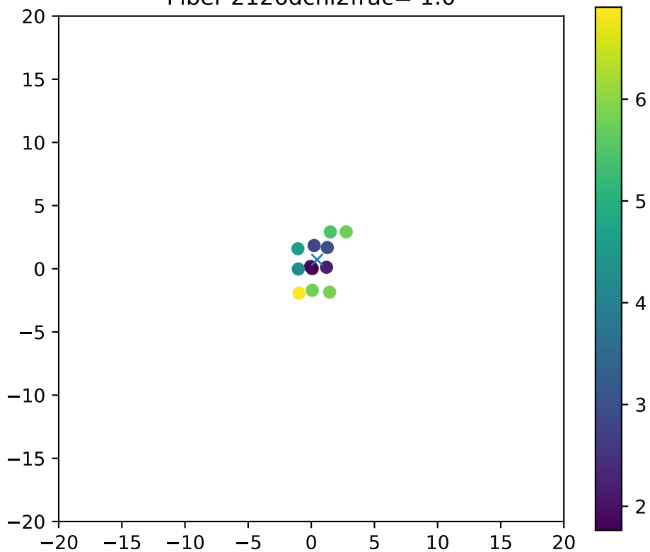
Fiber 2126dchi2frac= 1.0
