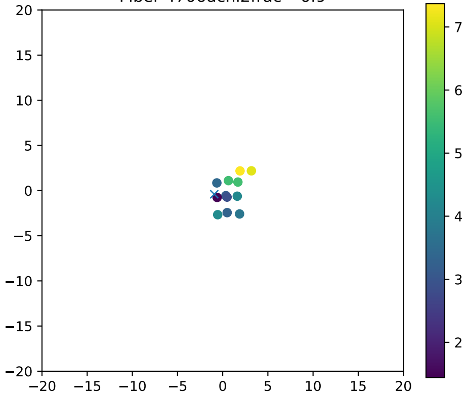
Fiber 4706dchi2frac= 0.9
