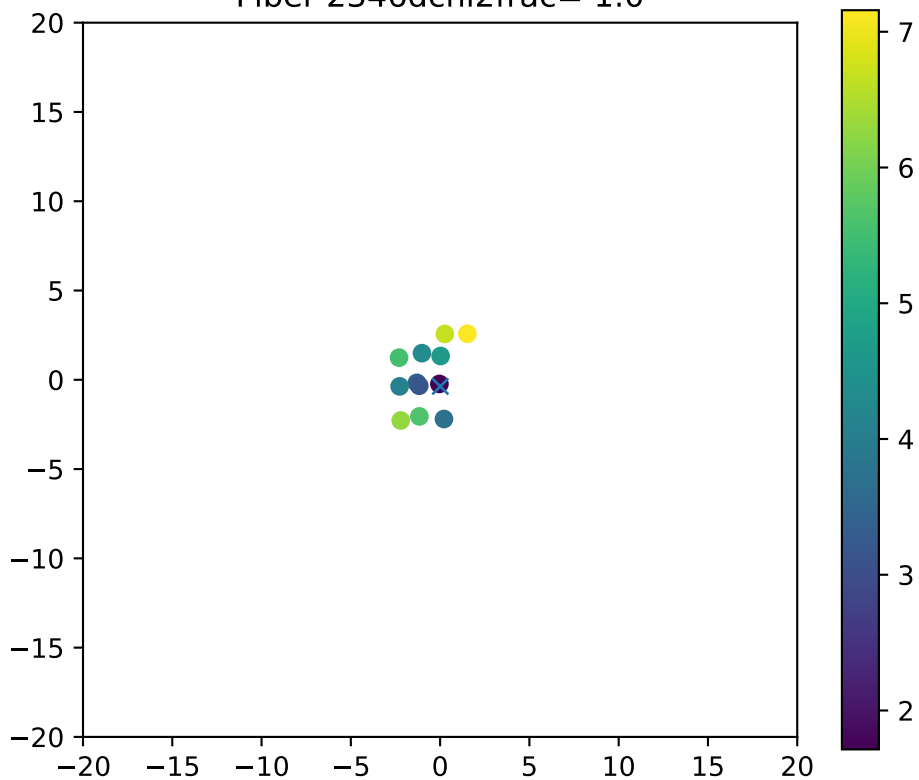
Fiber 2346dchi2frac= 1.0
