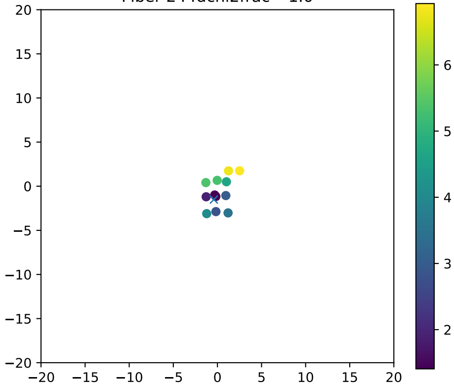
Fiber 244dchi2frac= 1.0
