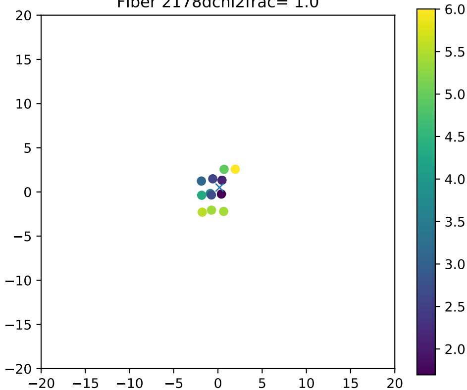
Fiber 2178dchi2frac= 1.0
