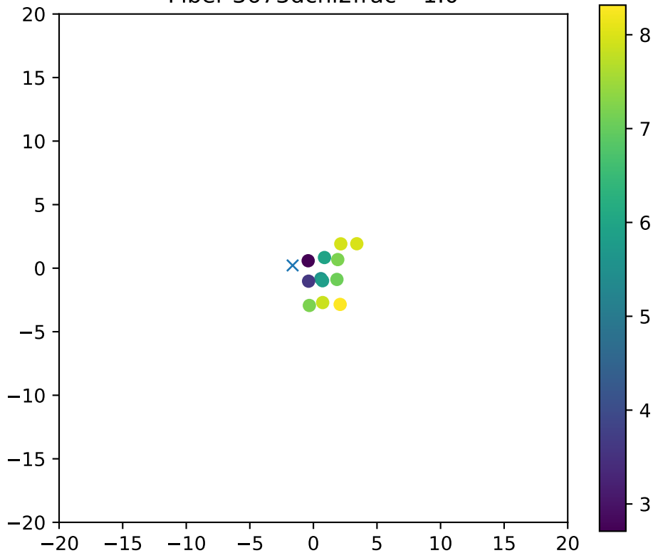
Fiber 3673dchi2frac= 1.0
