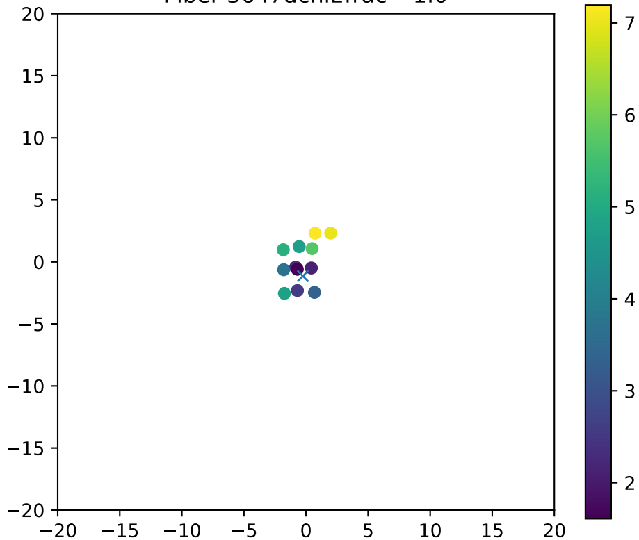
Fiber 3647dchi2frac= 1.0
