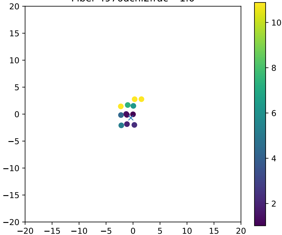
Fiber 4976dchi2frac= 1.0
