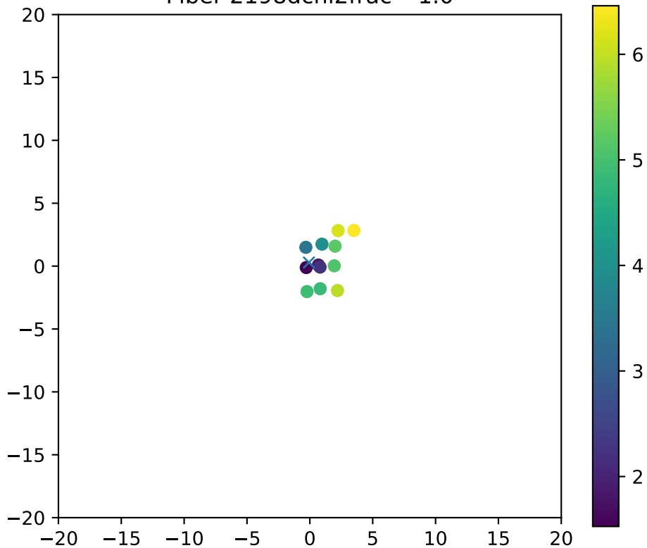
Fiber 2198dchi2frac= 1.0
