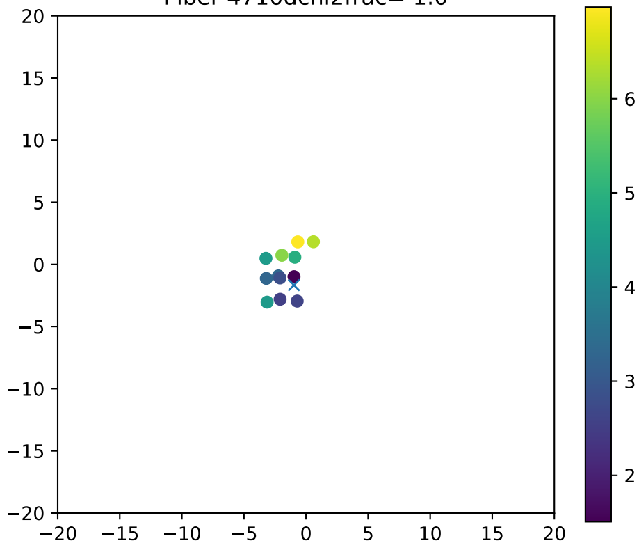
Fiber 4710dchi2frac= 1.0
