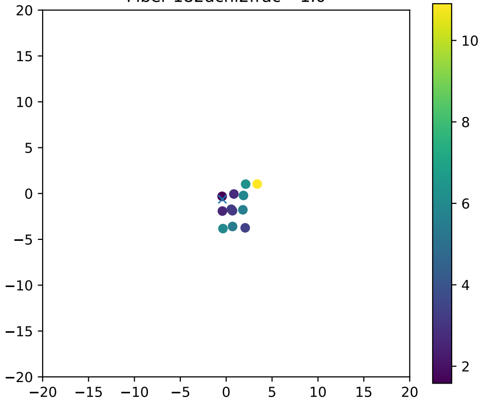
Fiber 182dchi2frac= 1.0
