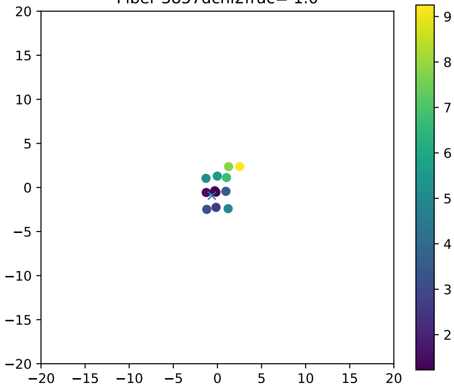
Fiber 3857dchi2frac= 1.0
