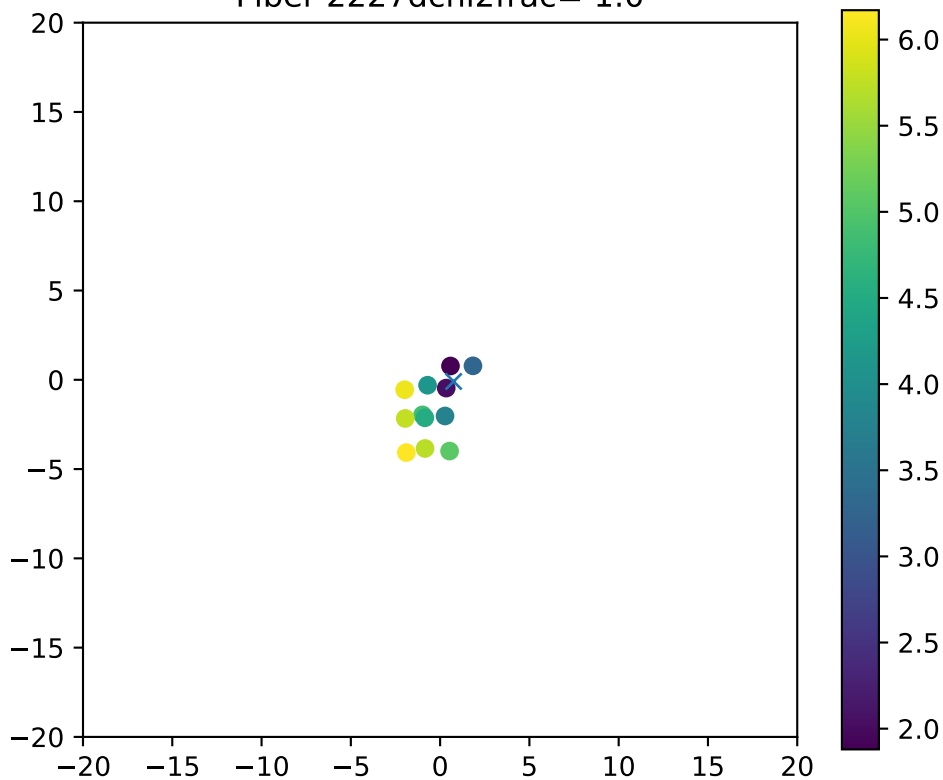
Fiber 2227dchi2frac= 1.0
