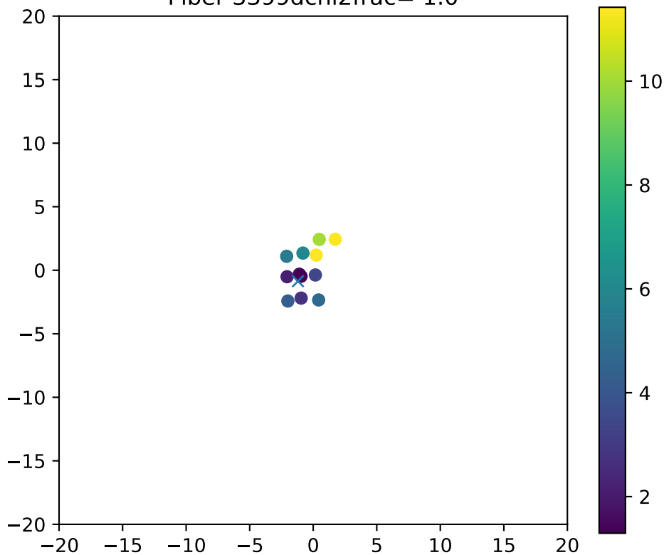
Fiber 3399dchi2frac= 1.0
