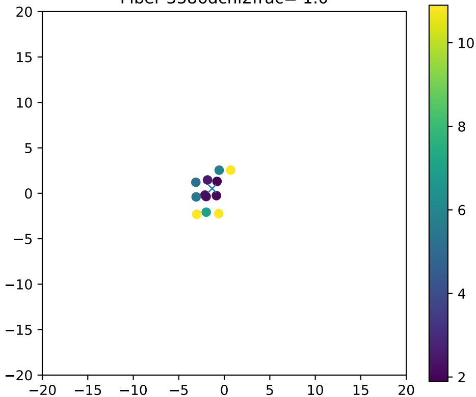
Fiber 3386dchi2frac= 1.0
