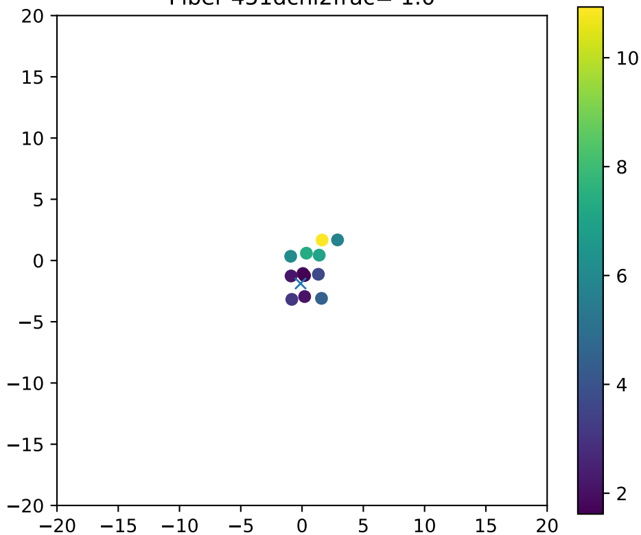
Fiber 451dchi2frac= 1.0
