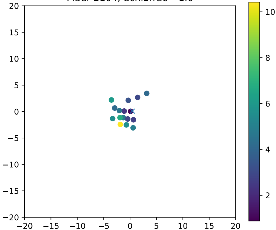
Fiber 2104, dchi2frac= 1.0
