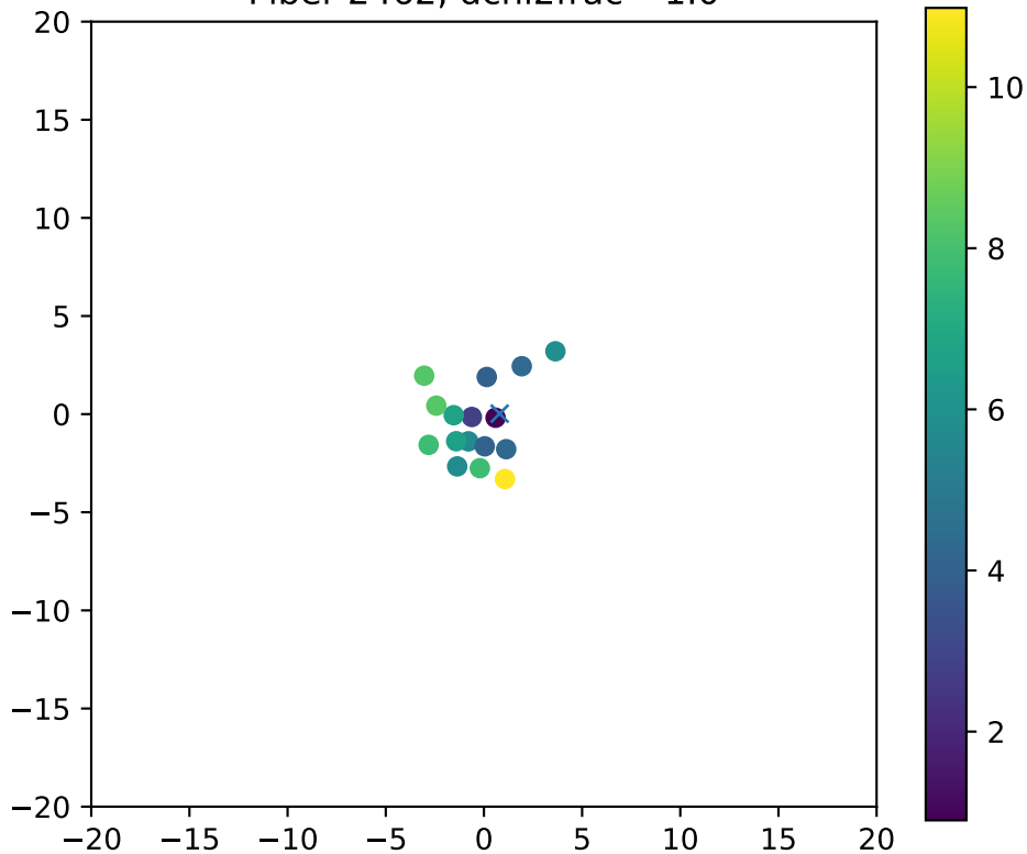
Fiber 2462, dchi2frac= 1.0
