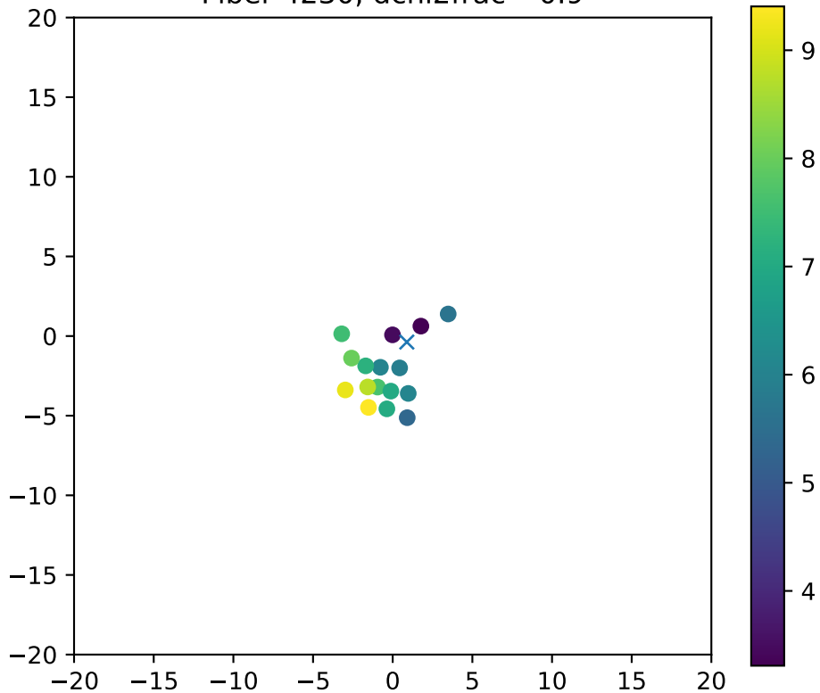
Fiber 4230, dchi2frac= 0.9
