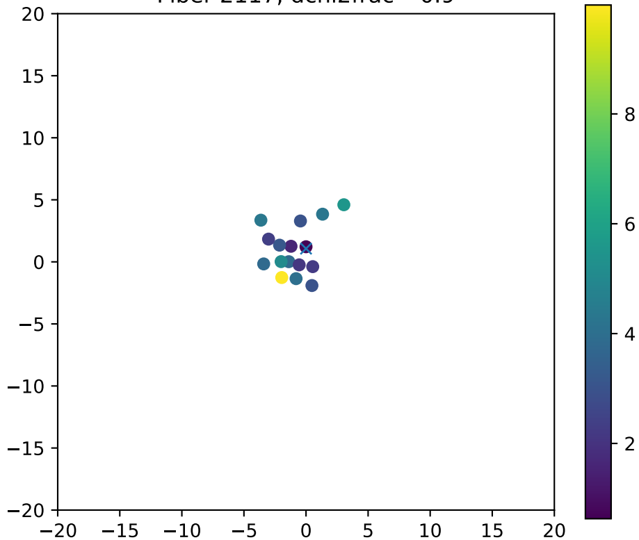
Fiber 2117, dchi2frac= 0.9
