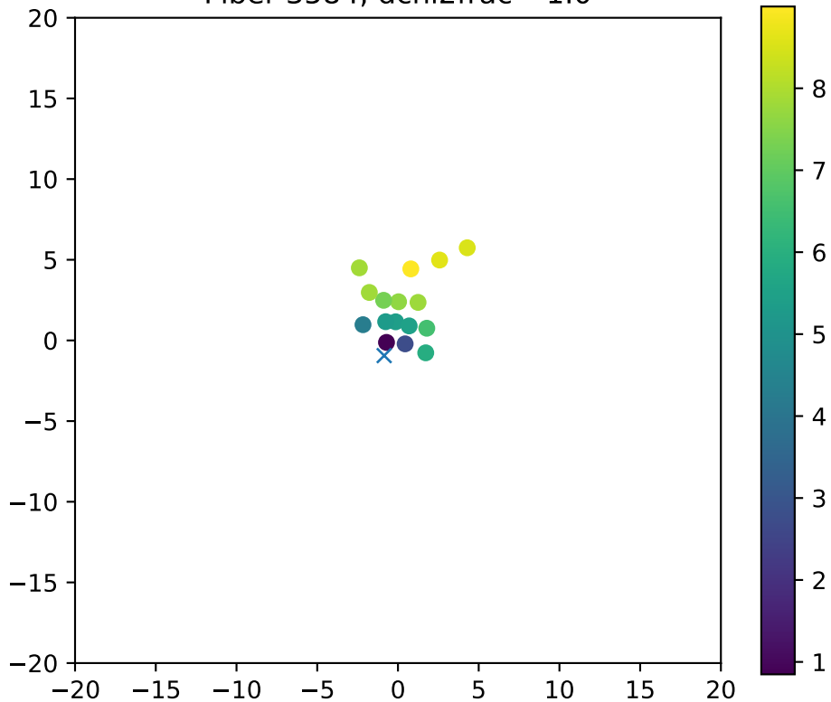
Fiber 3584, dchi2frac= 1.0
