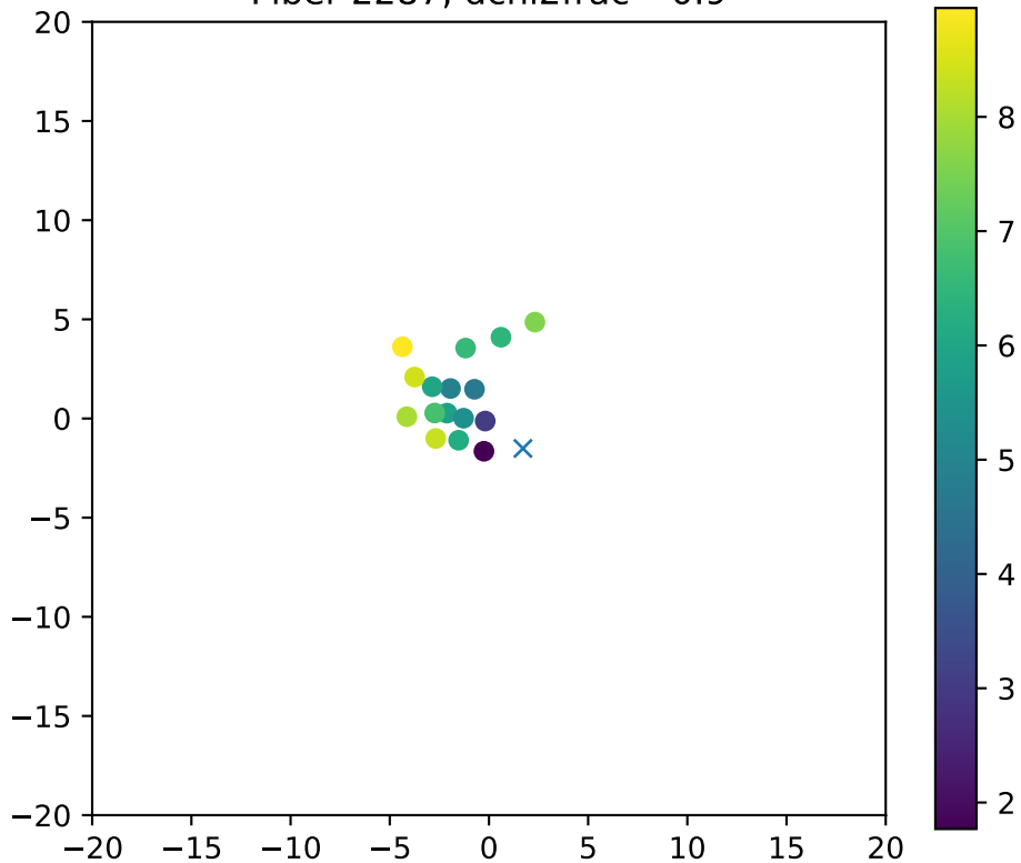
Fiber 2287, dchi2frac= 0.9
