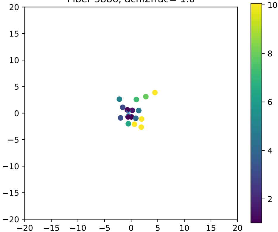
Fiber 3886, dchi2frac= 1.0
