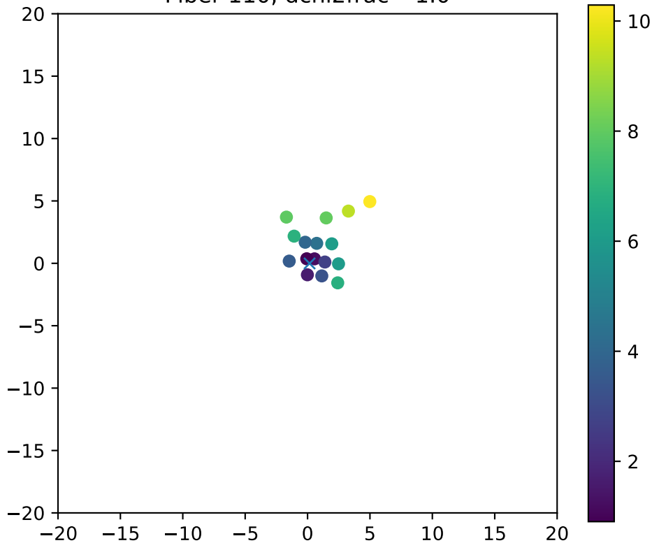
Fiber 110, dchi2frac= 1.0
