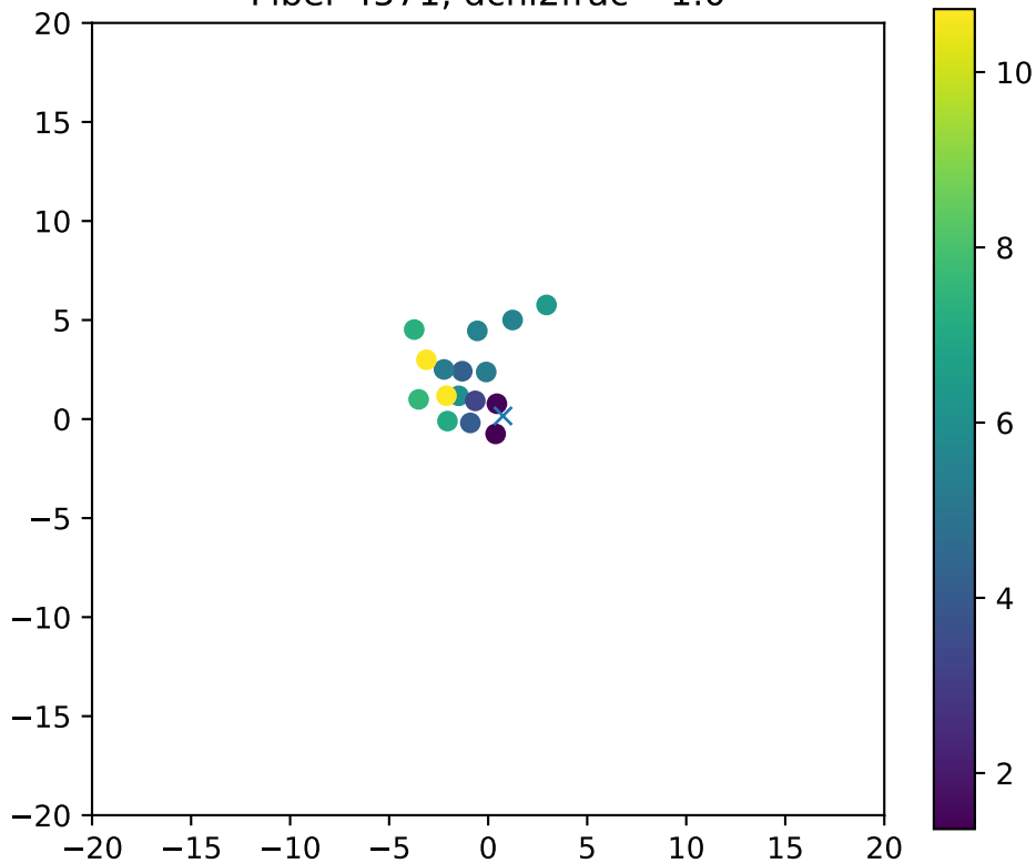
Fiber 4571, dchi2frac= 1.0
