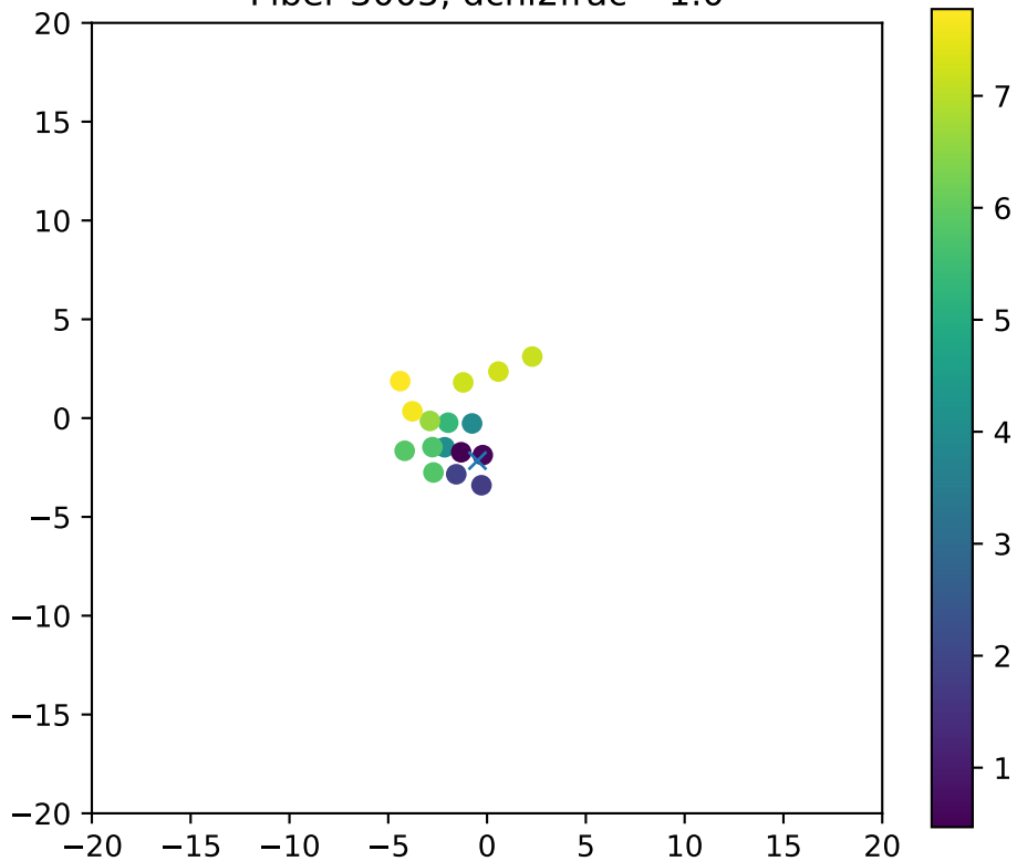
Fiber 3005, dchi2frac= 1.0
