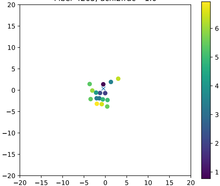
Fiber 4263, dchi2frac= 1.0
