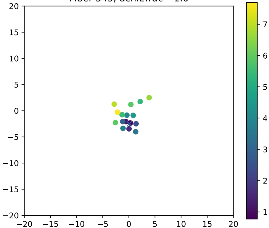
Fiber 345, dchi2frac= 1.0
