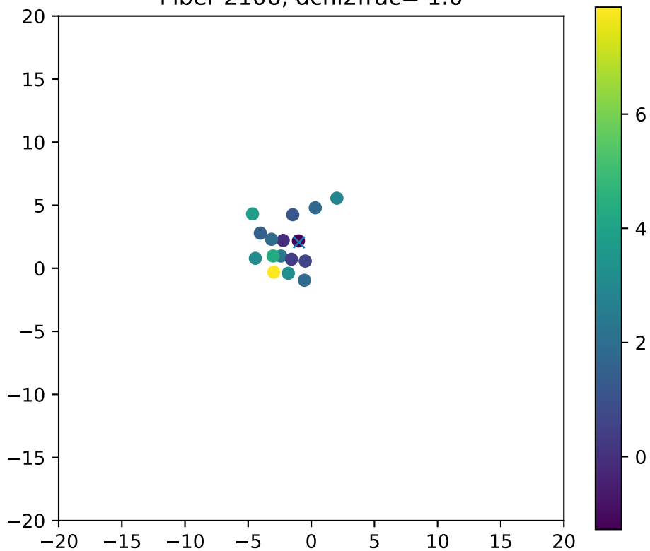
Fiber 2106, dchi2frac= 1.0
