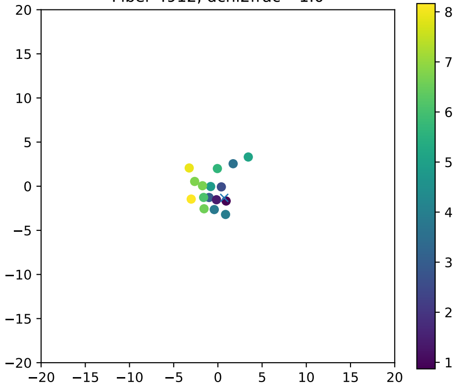
Fiber 4912, dchi2frac= 1.0
