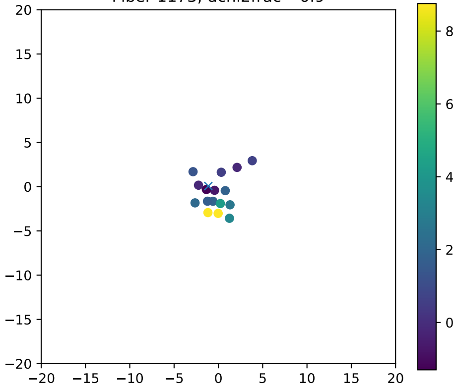
Fiber 1173, dchi2frac= 0.9
