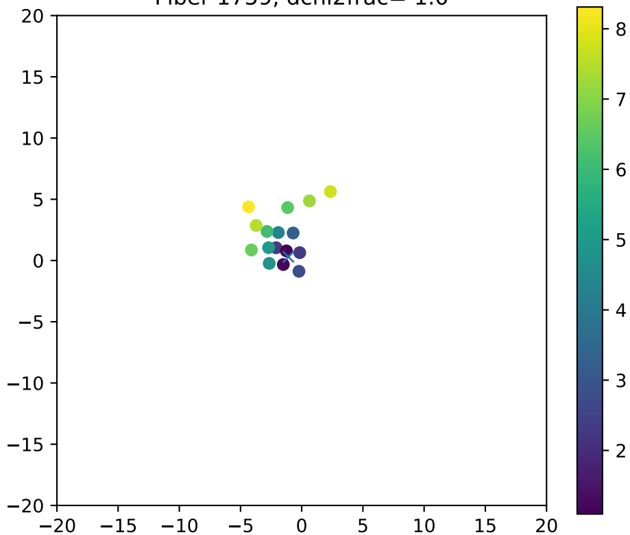
Fiber 1759, dchi2frac= 1.0
