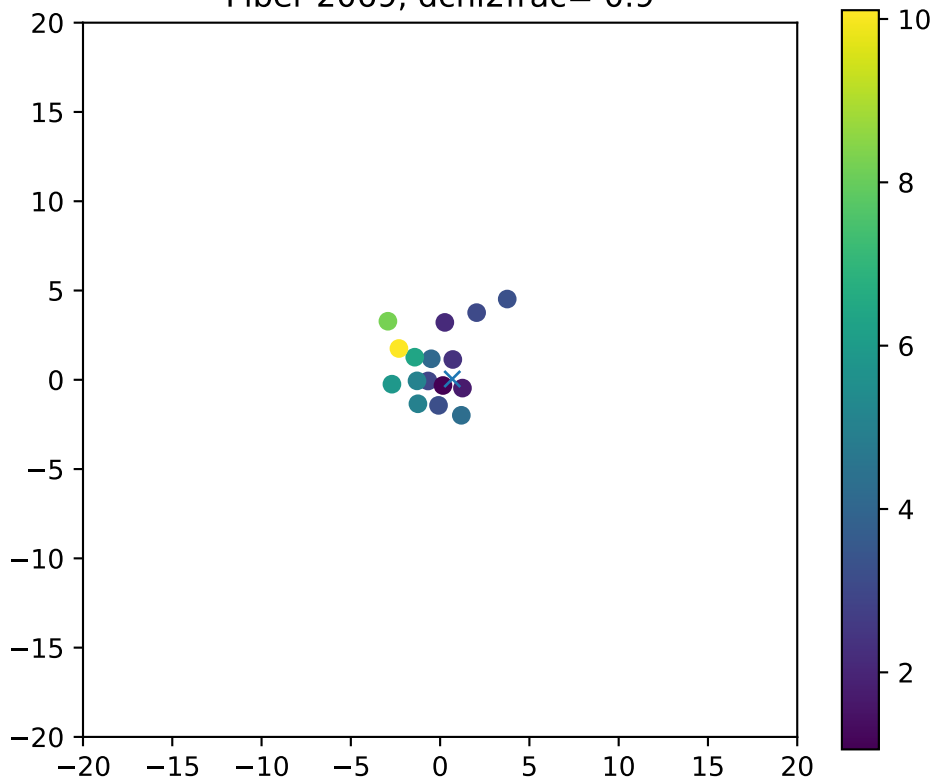
Fiber 2069, dchi2frac= 0.9
