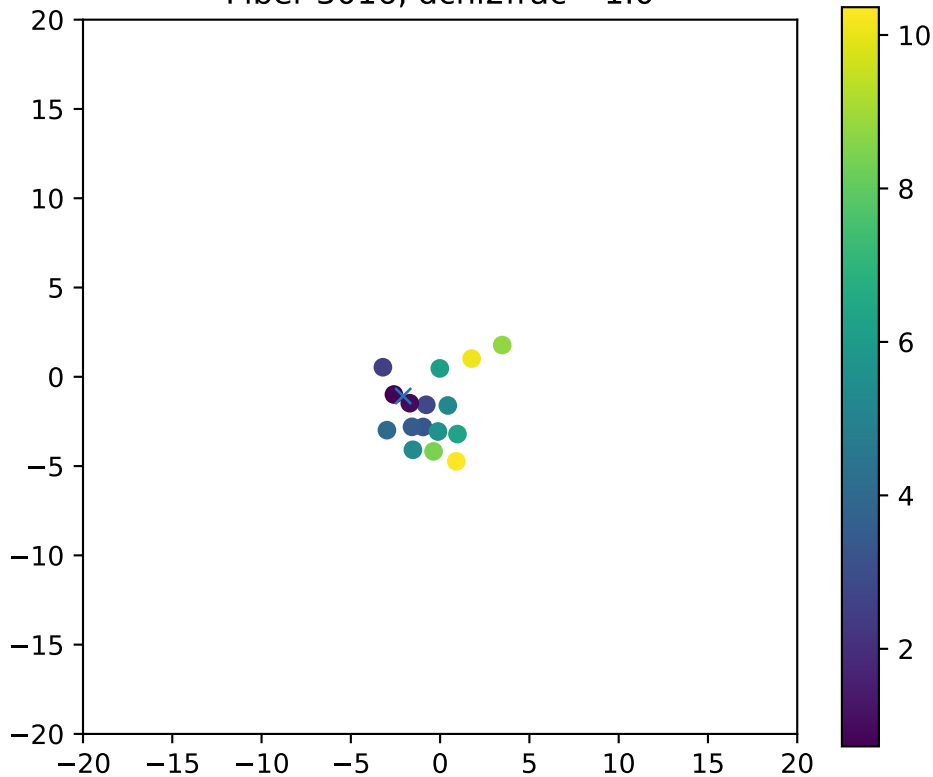
Fiber 3016, dchi2frac= 1.0
