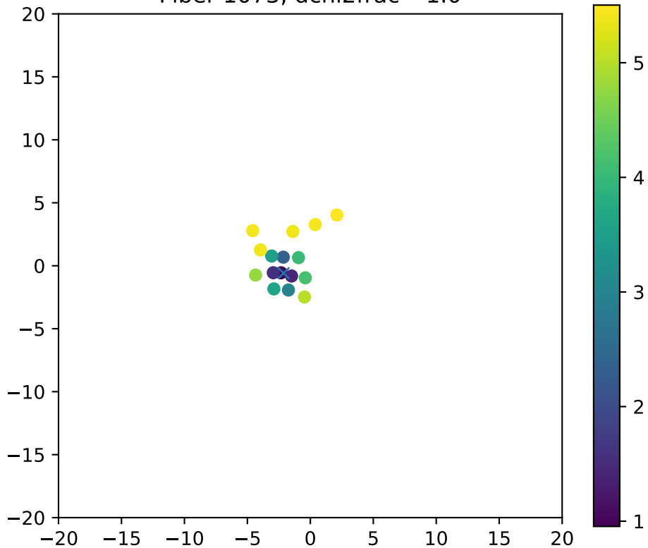
Fiber 1073, dchi2frac= 1.0
