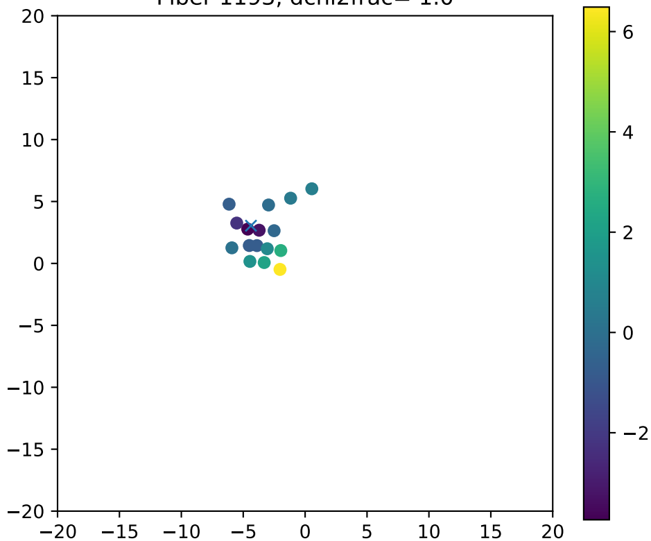
Fiber 1193, dchi2frac= 1.0
