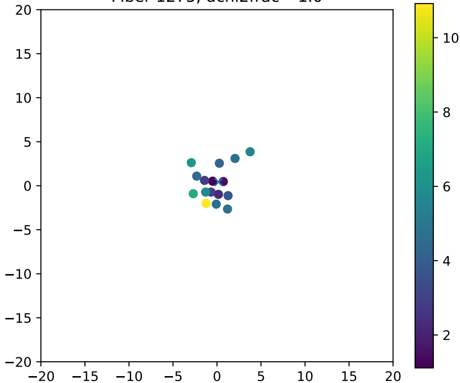
Fiber 1275, dchi2frac= 1.0
