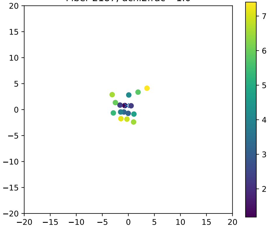
Fiber 2187, dchi2frac= 1.0
