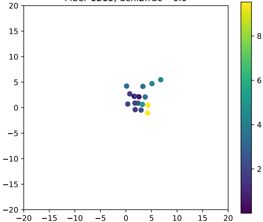
Fiber 1213, dchi2frac= 0.9
