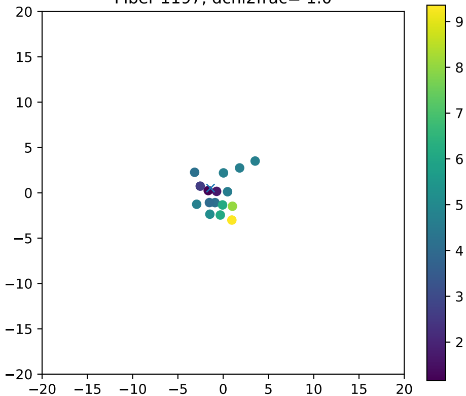
Fiber 1197, dchi2frac= 1.0
