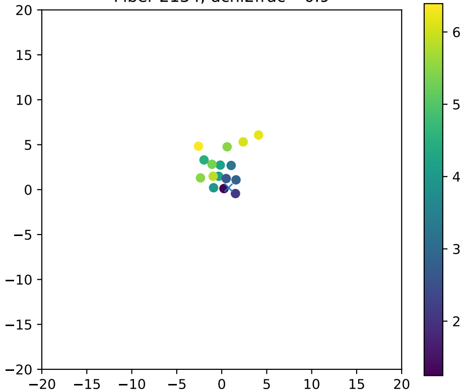
Fiber 2134, dchi2frac= 0.9
