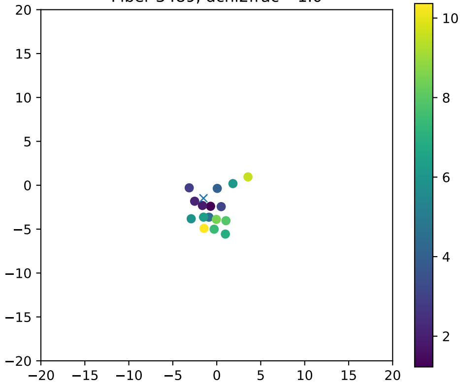
Fiber 3489, dchi2frac= 1.0
