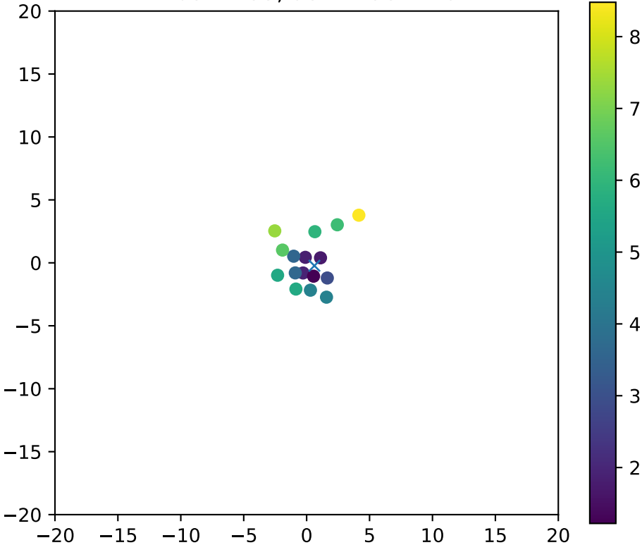
Fiber 2295, dchi2frac= 1.0
