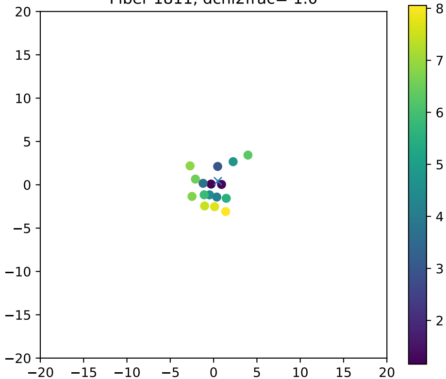
Fiber 1811, dchi2frac= 1.0
