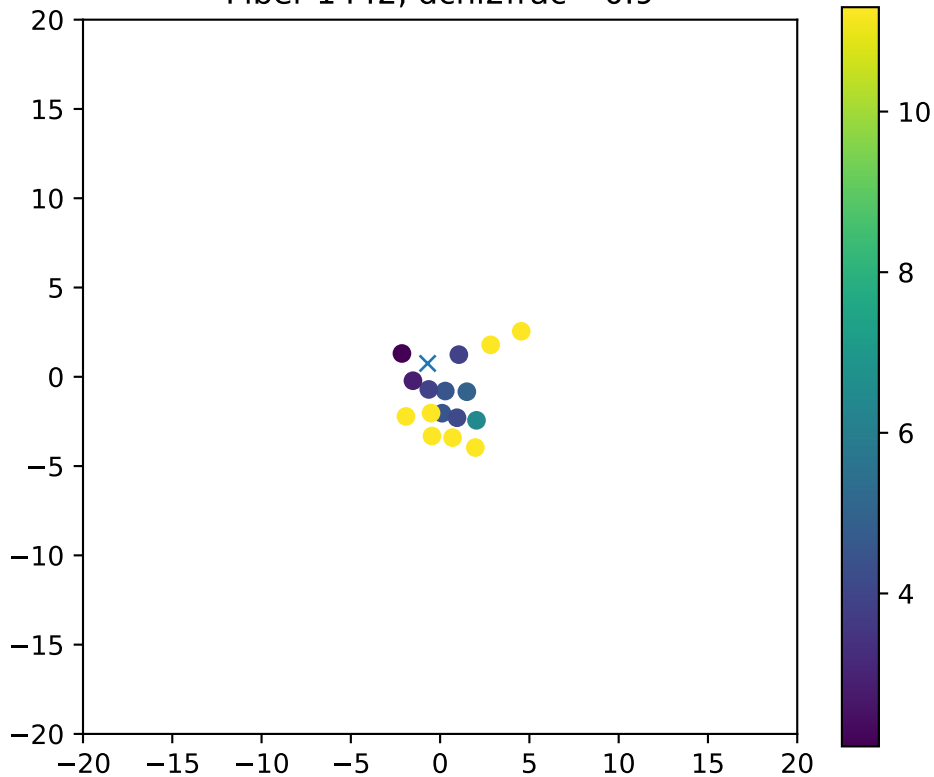
Fiber 1442, dchi2frac= 0.9
