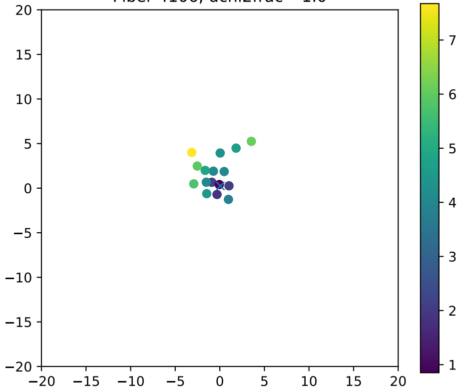
Fiber 4106, dchi2frac= 1.0
