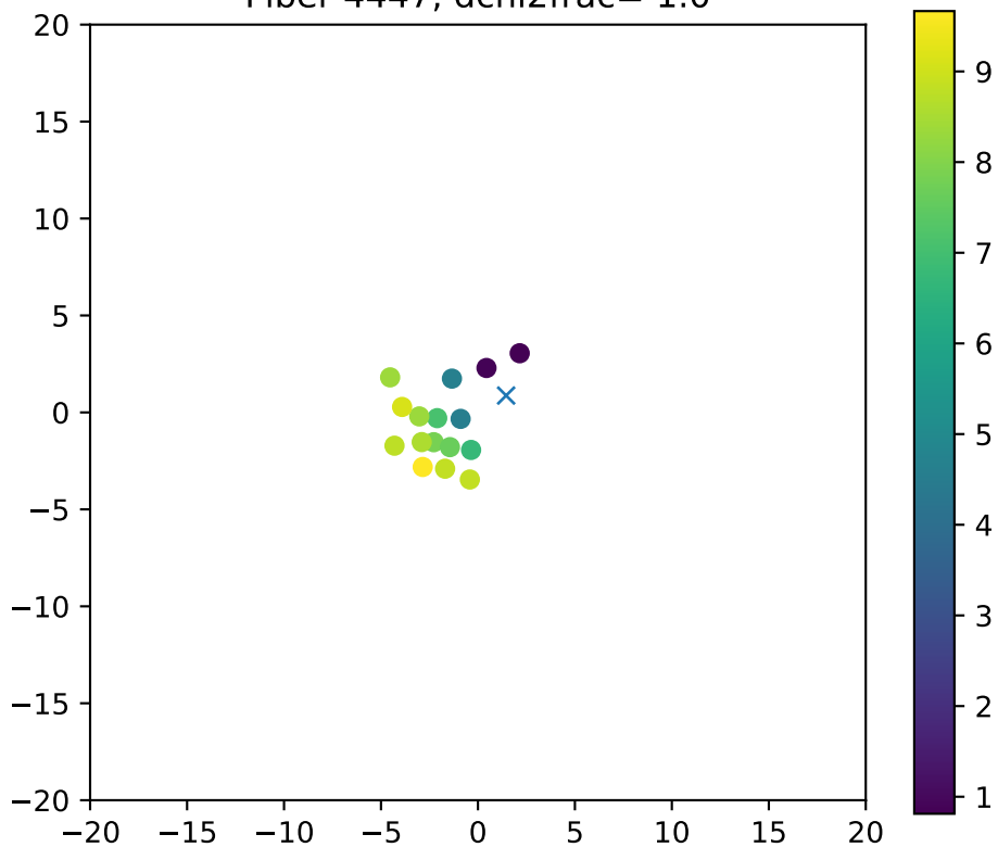
Fiber 4447, dchi2frac= 1.0
