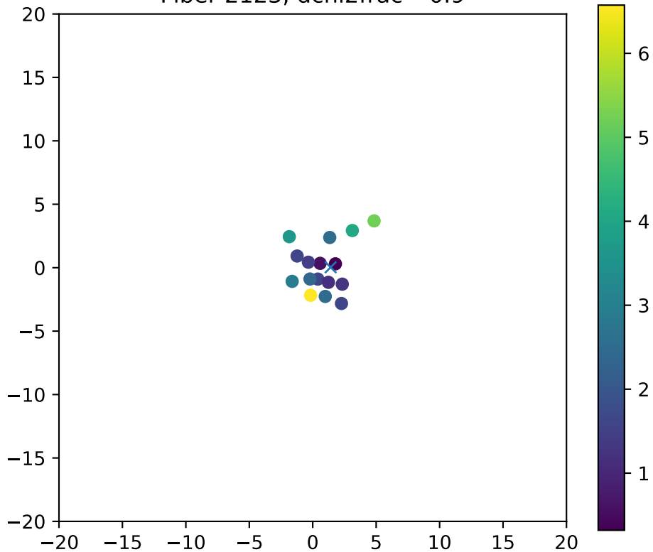
Fiber 2123, dchi2frac= 0.9
