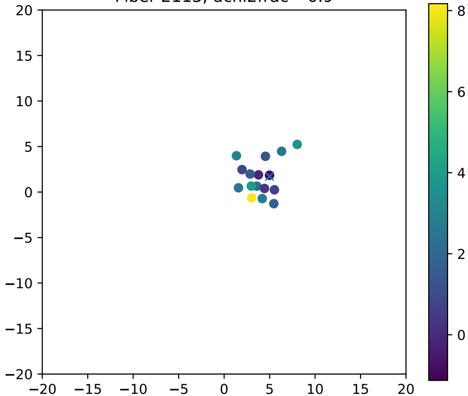
Fiber 2113, dchi2frac= 0.9
