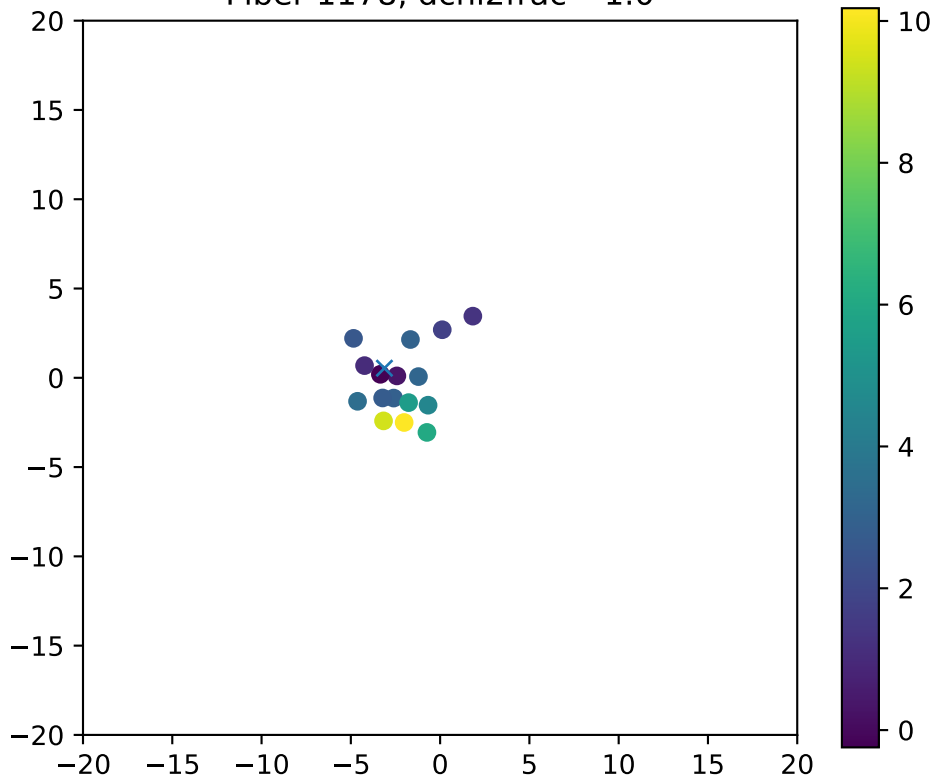
Fiber 1178, dchi2frac= 1.0
