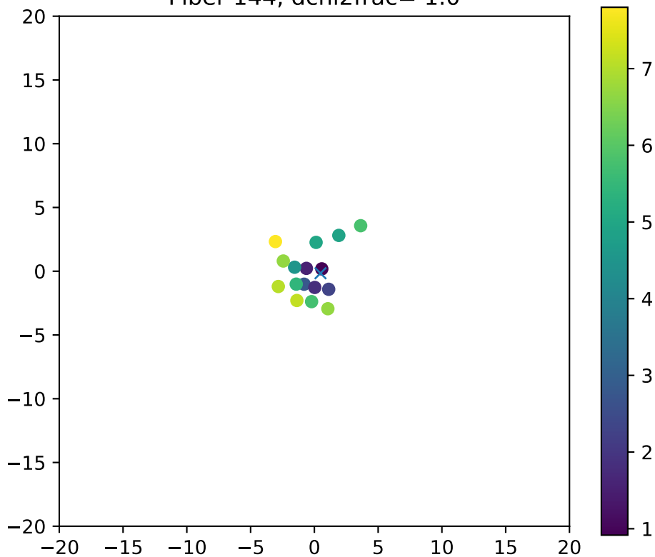
Fiber 144, dchi2frac= 1.0
