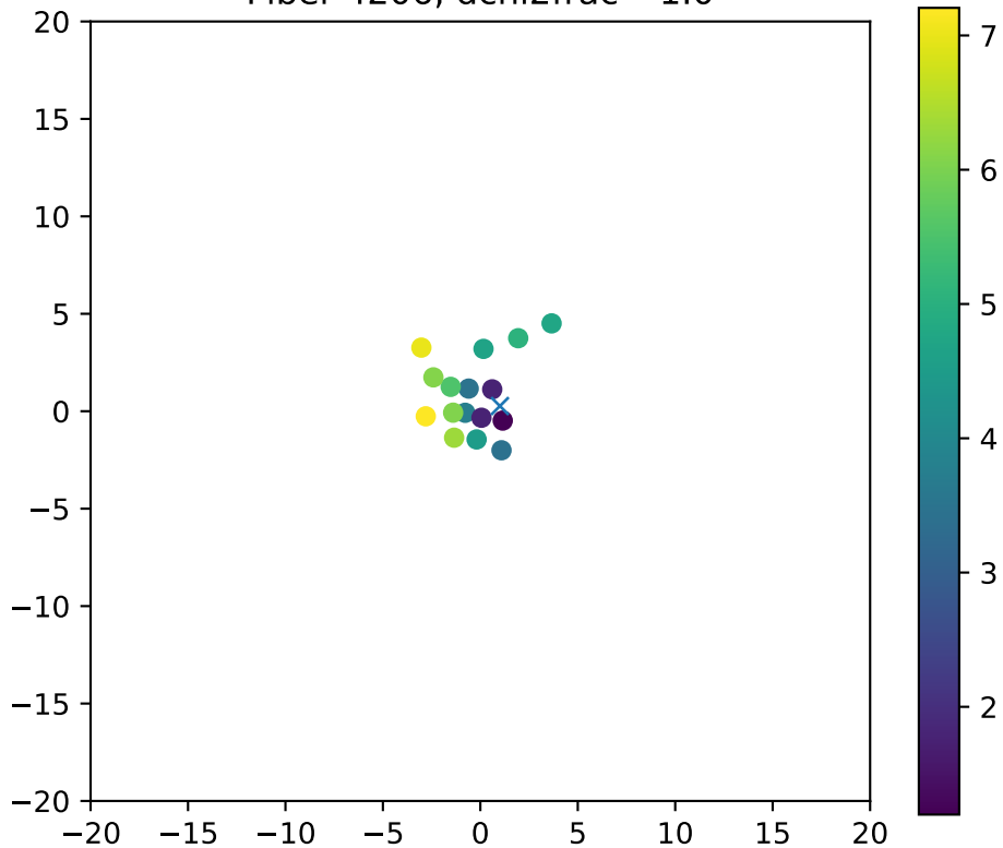
Fiber 4206, dchi2frac= 1.0
