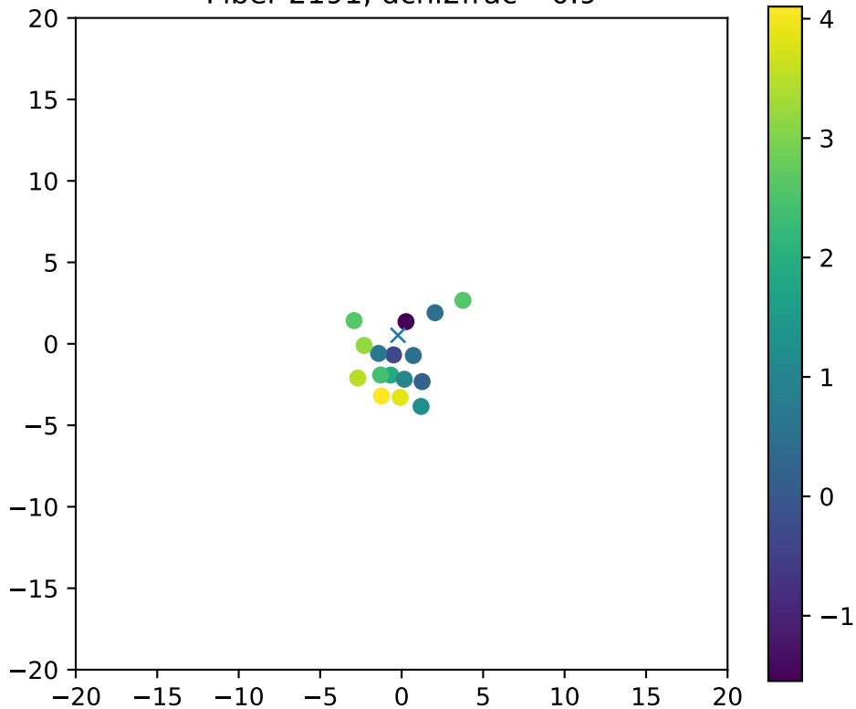
Fiber 2191, dchi2frac= 0.9
