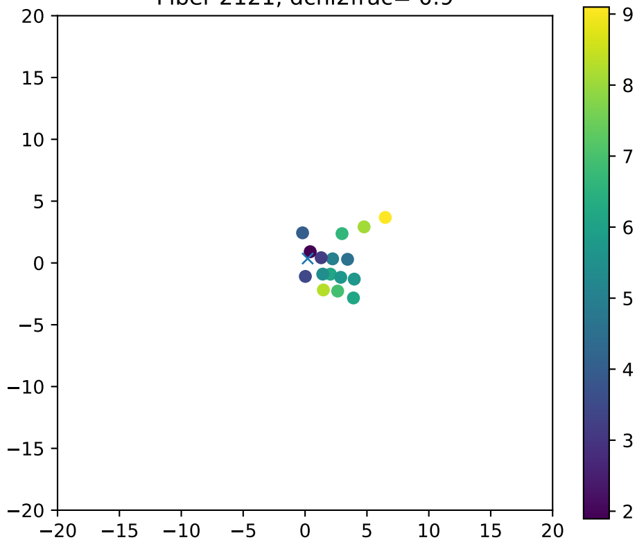
Fiber 2121, dchi2frac= 0.9
