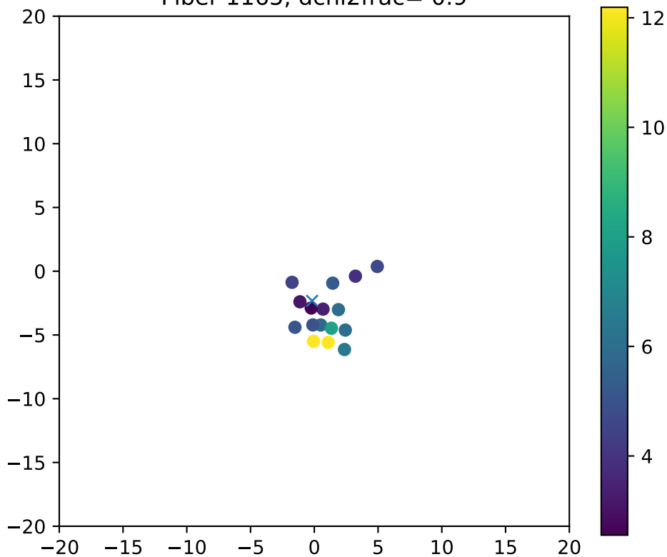
Fiber 1165, dchi2frac= 0.9
