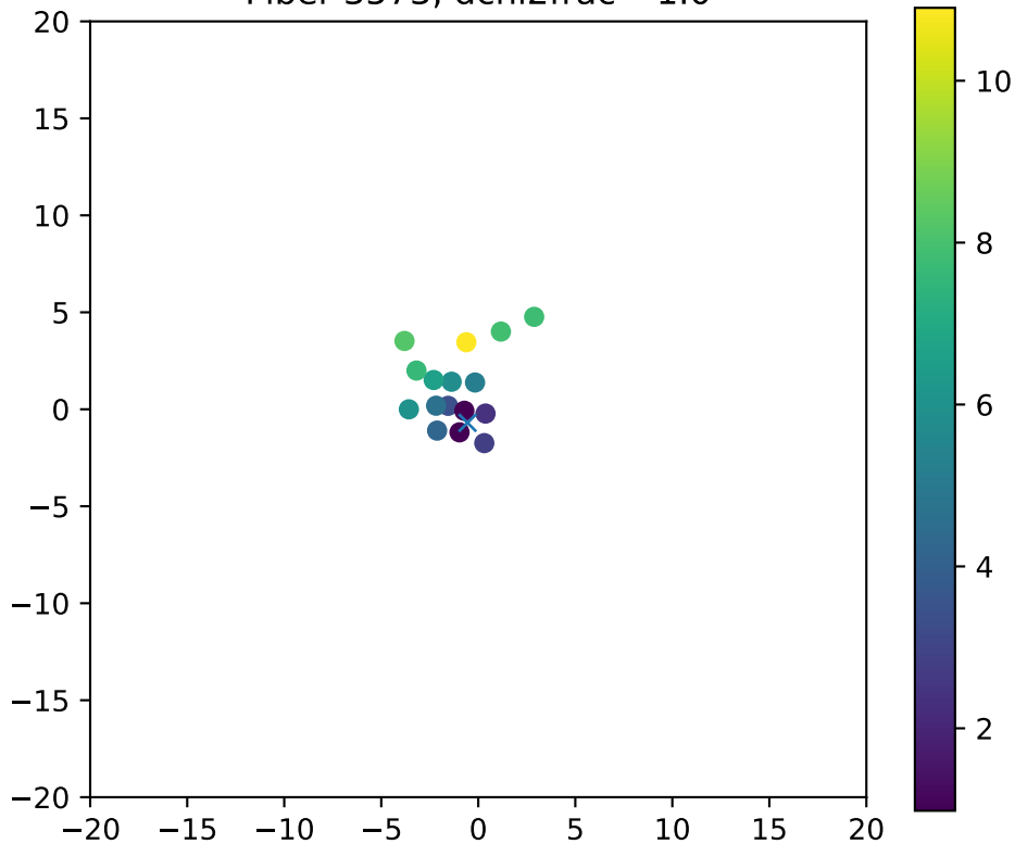
Fiber 3573, dchi2frac= 1.0
