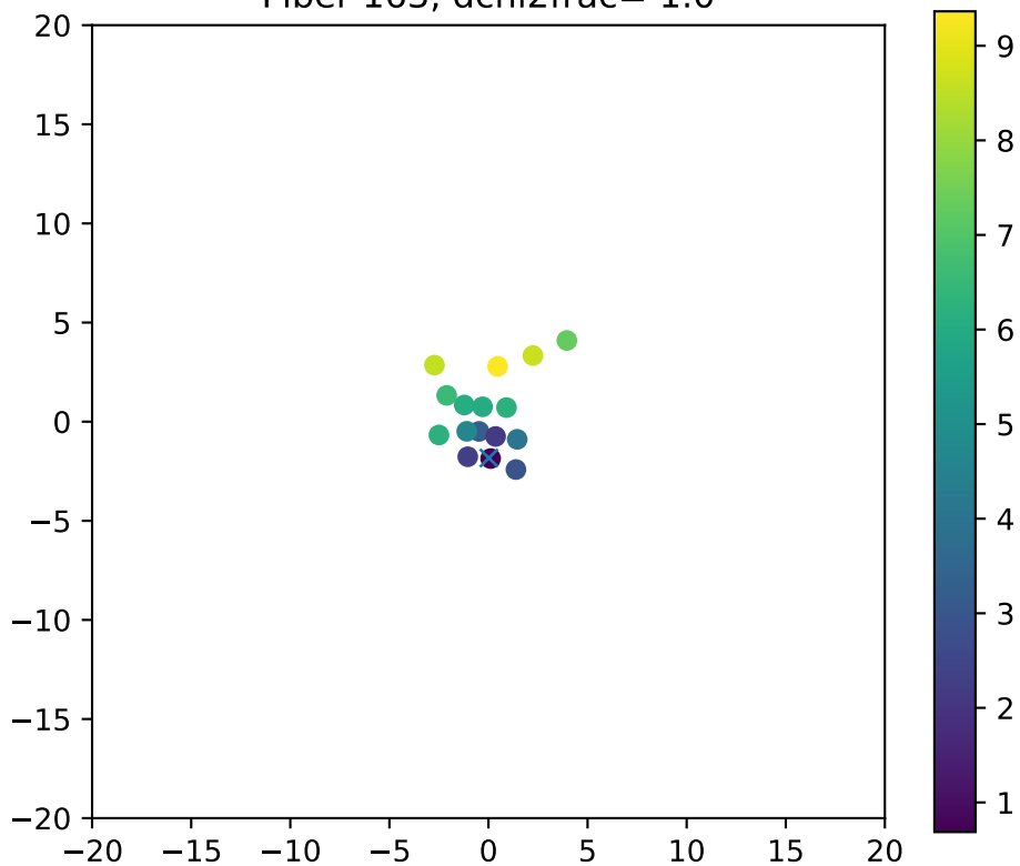
Fiber 163, dchi2frac= 1.0
