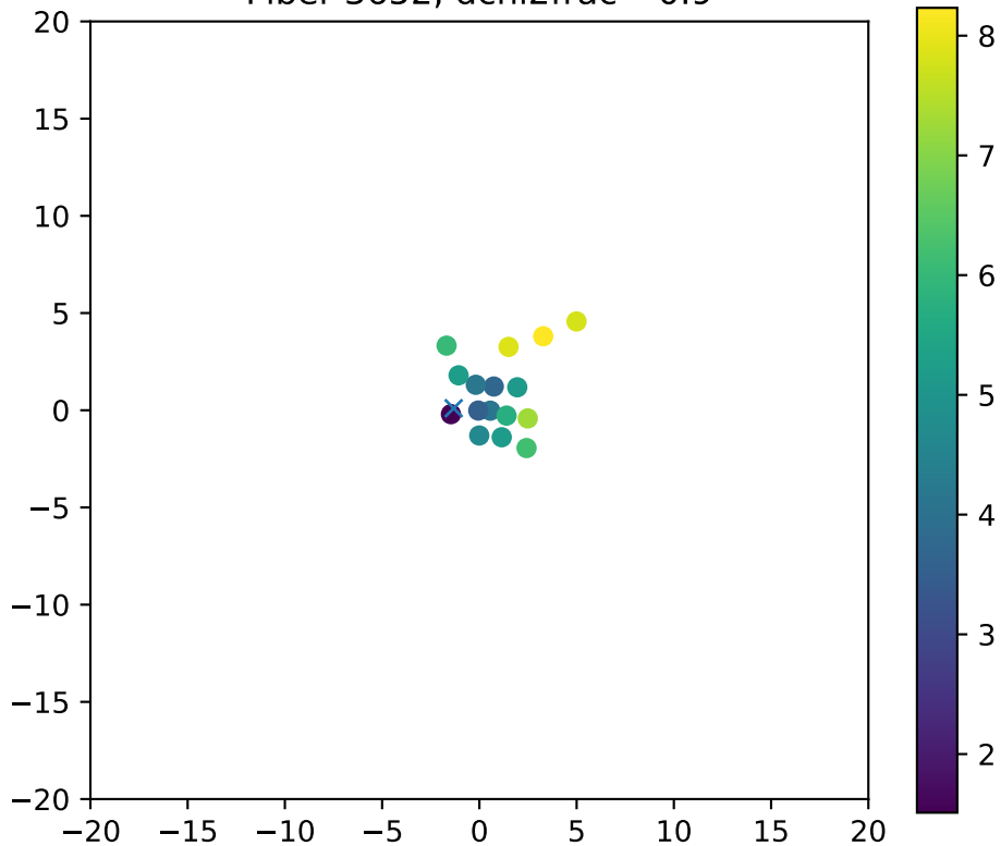
Fiber 3652, dchi2frac= 0.9
