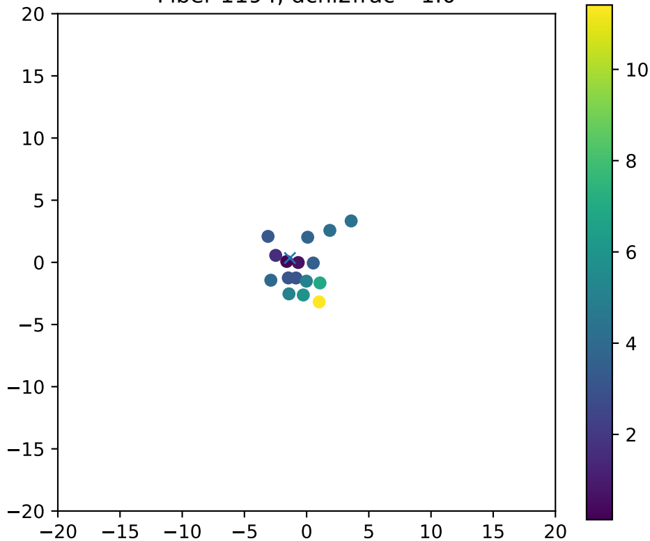
Fiber 1194, dchi2frac= 1.0
