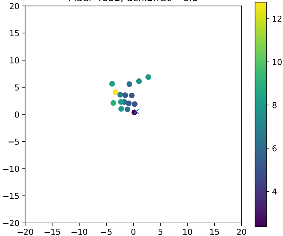
Fiber 4652, dchi2frac= 0.9
