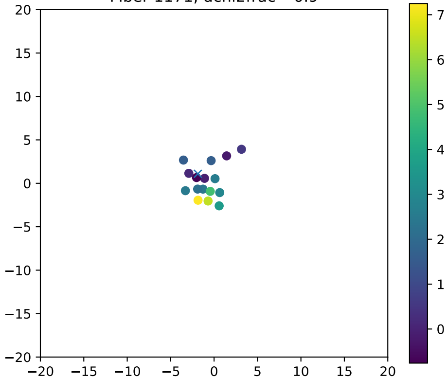
Fiber 1171, dchi2frac= 0.9
