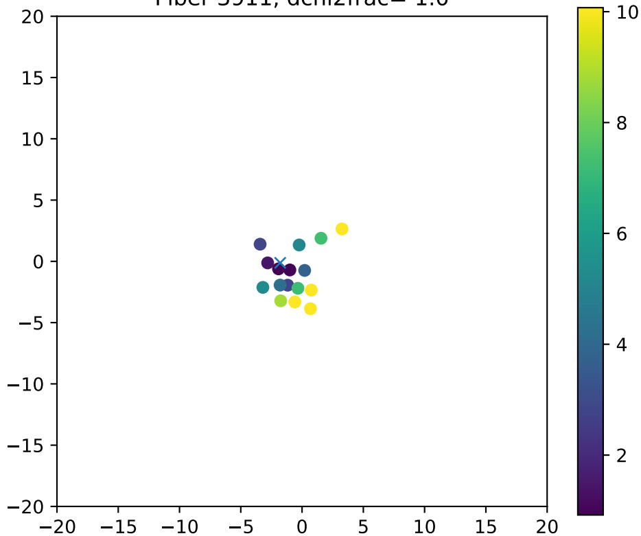
Fiber 3911, dchi2frac= 1.0
