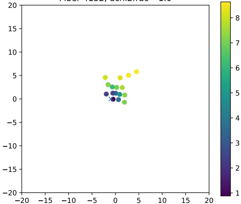
Fiber 4152, dchi2frac= 1.0
