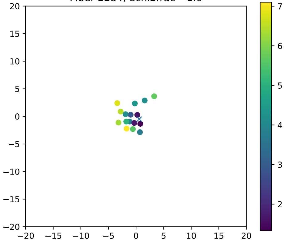
Fiber 2284, dchi2frac= 1.0
