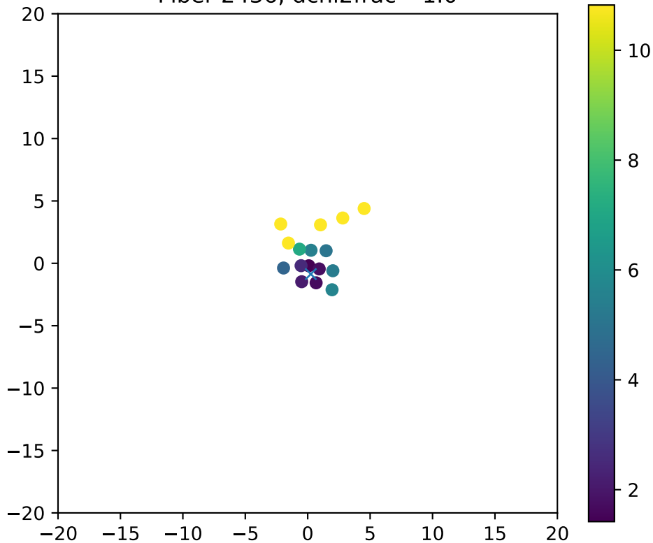
Fiber 2436, dchi2frac= 1.0
