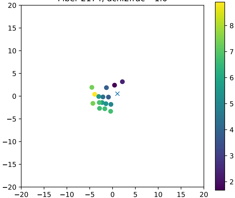
Fiber 2174, dchi2frac= 1.0
