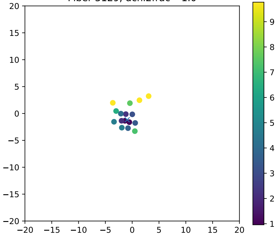
Fiber 3129, dchi2frac= 1.0
