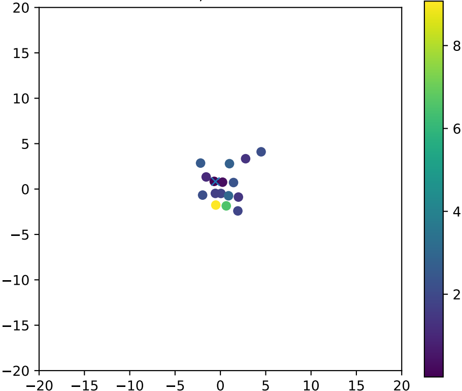
Fiber 1159, dchi2frac= 0.9
