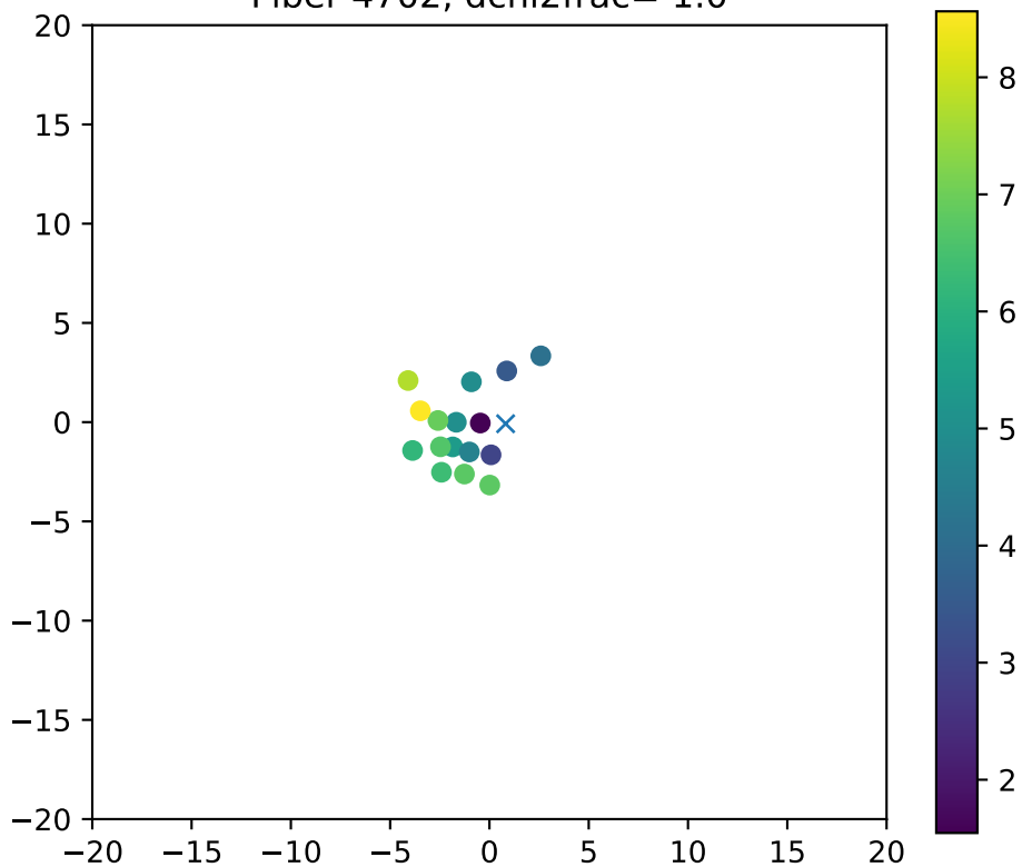
Fiber 4702, dchi2frac= 1.0
