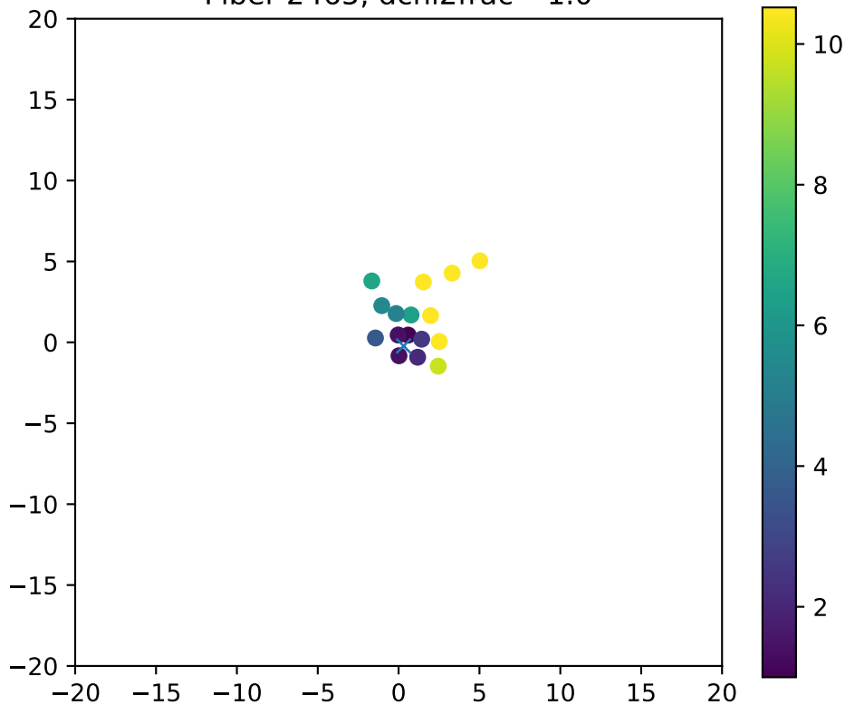
Fiber 2465, dchi2frac= 1.0
