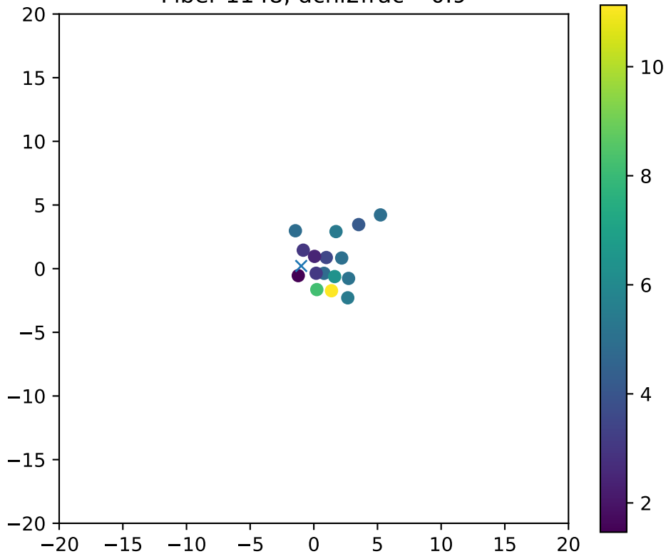
Fiber 1148, dchi2frac= 0.9
