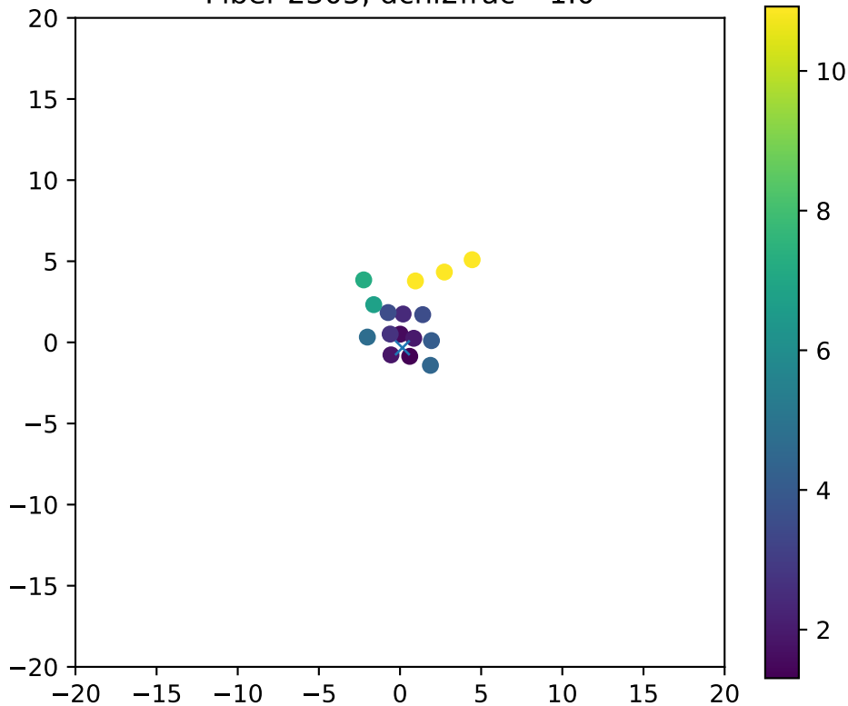
Fiber 2305, dchi2frac= 1.0
