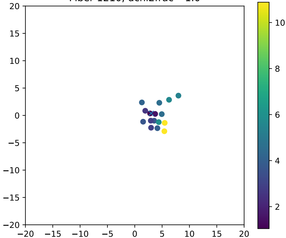
Fiber 1210, dchi2frac= 1.0
