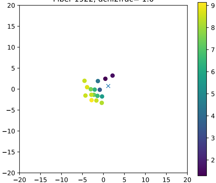
Fiber 1922, dchi2frac= 1.0
