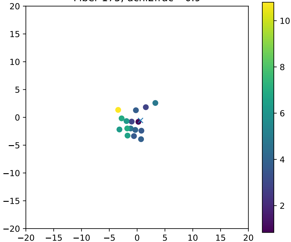
Fiber 175, dchi2frac= 0.9
