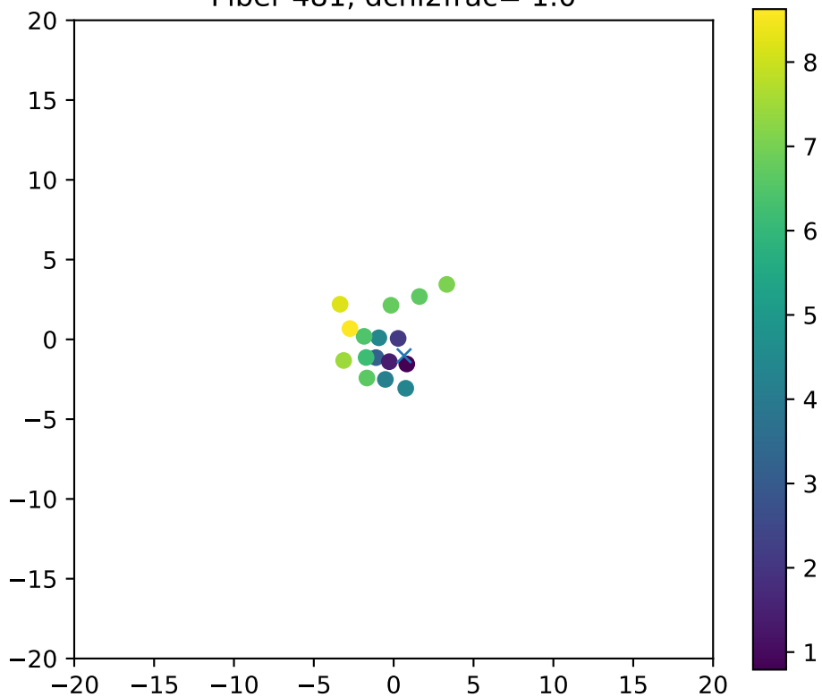
Fiber 481, dchi2frac= 1.0
