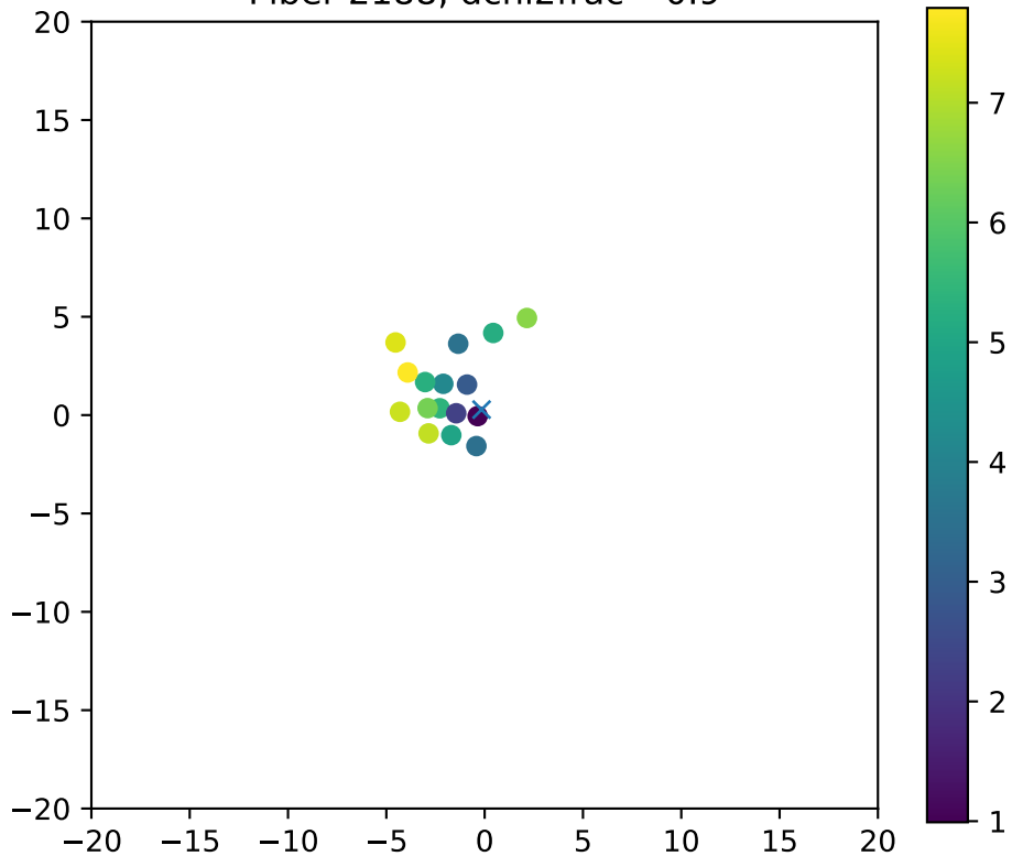
Fiber 2188, dchi2frac= 0.9
