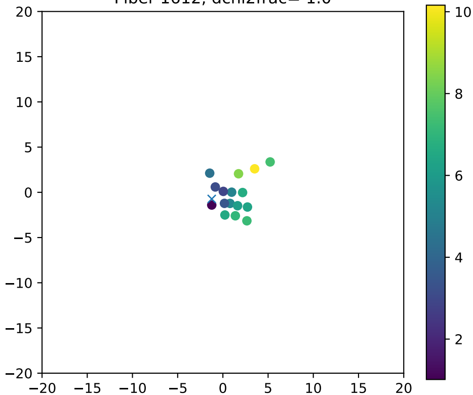
Fiber 1612, dchi2frac= 1.0
