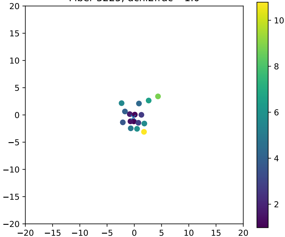
Fiber 3225, dchi2frac= 1.0
