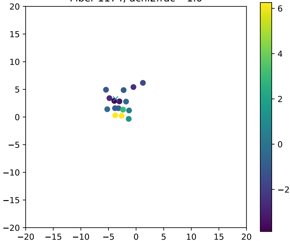
Fiber 1174, dchi2frac= 1.0
