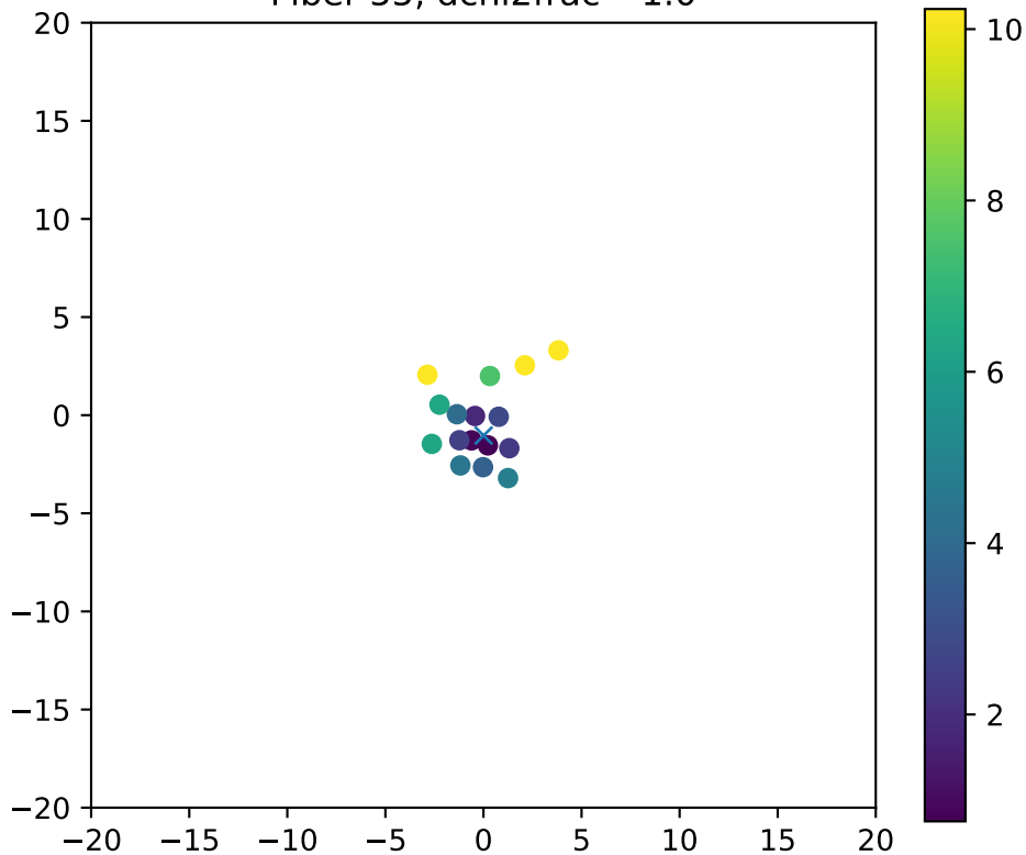
Fiber 55, dchi2frac= 1.0
