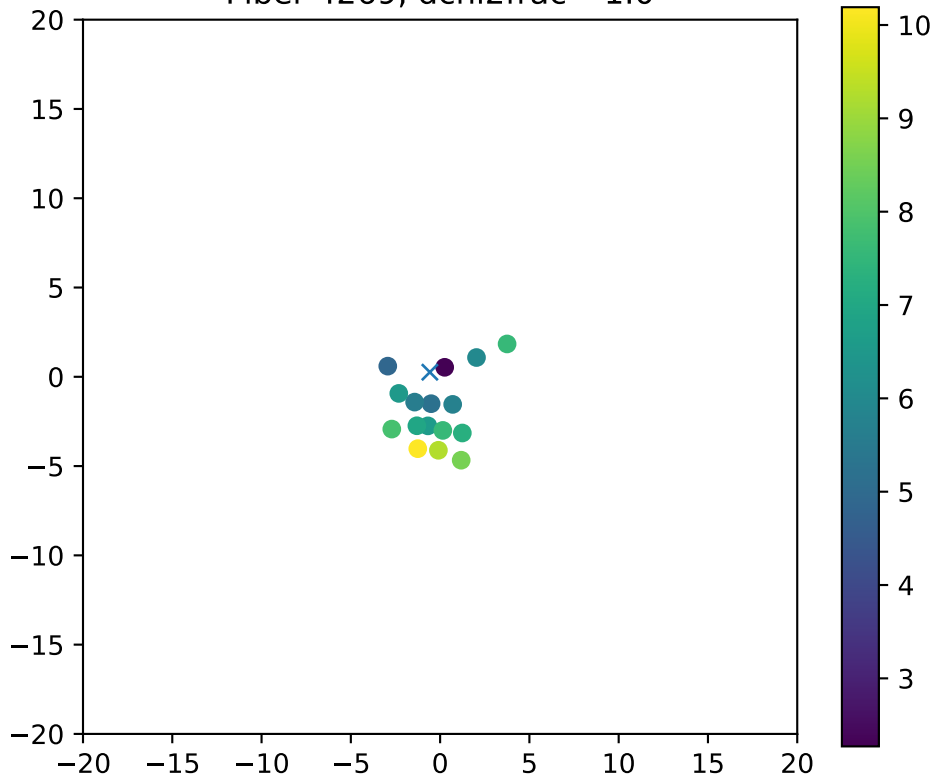
Fiber 4269, dchi2frac= 1.0
