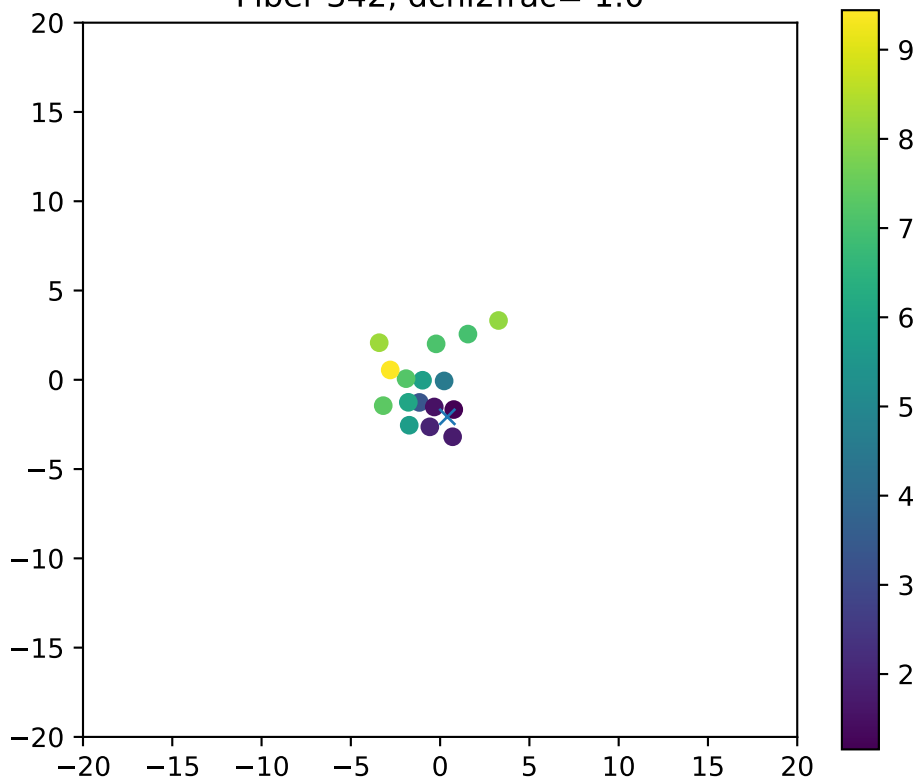
Fiber 342, dchi2frac= 1.0
