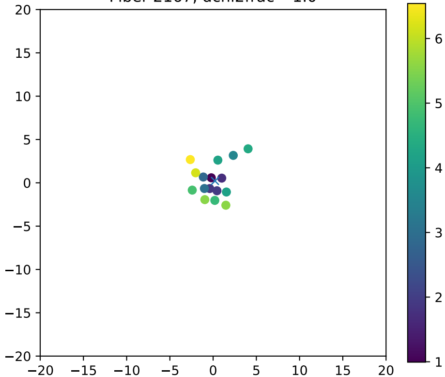
Fiber 2167, dchi2frac= 1.0
