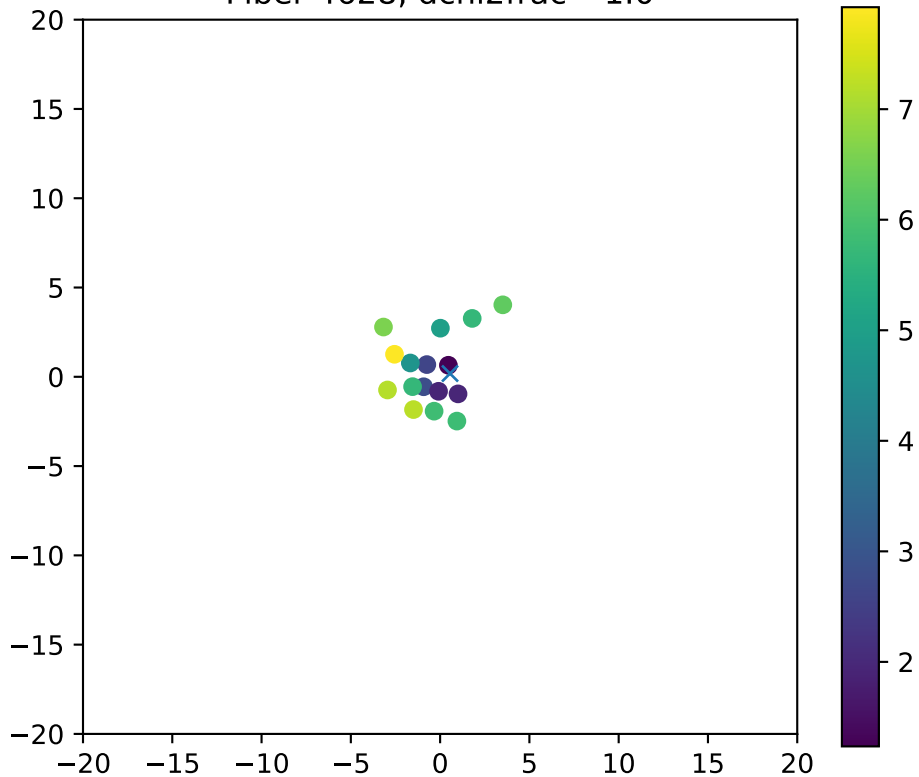
Fiber 4628, dchi2frac= 1.0
