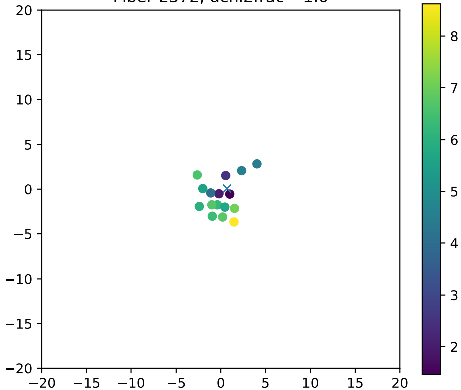
Fiber 2372, dchi2frac= 1.0
