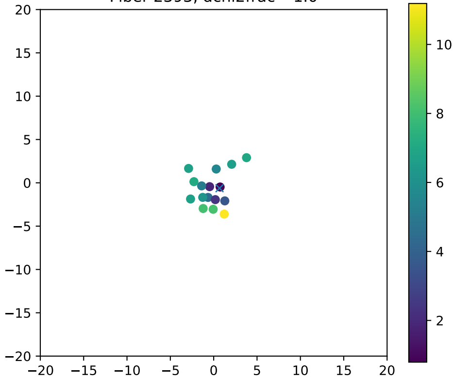
Fiber 2393, dchi2frac= 1.0
