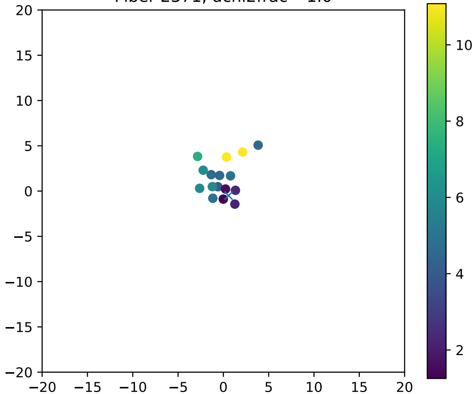
Fiber 2371, dchi2frac= 1.0
