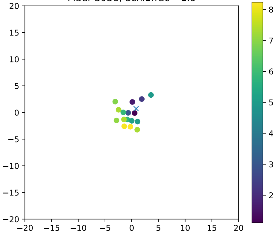
Fiber 3956, dchi2frac= 1.0
