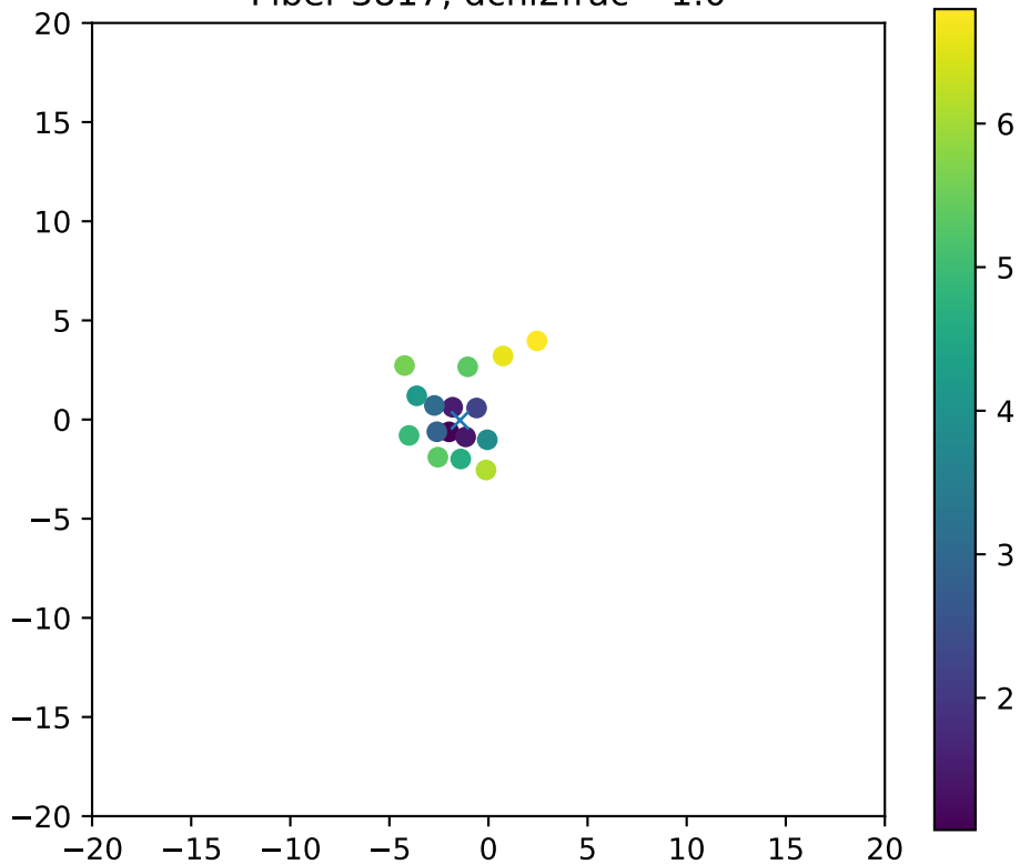
Fiber 3817, dchi2frac= 1.0
