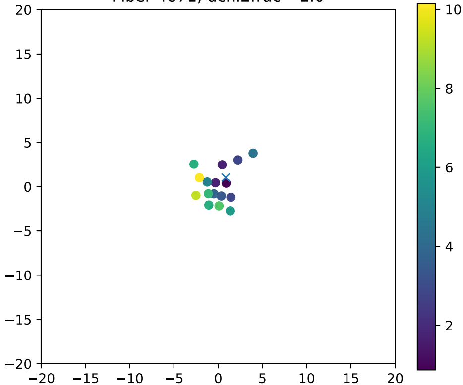
Fiber 4671, dchi2frac= 1.0
