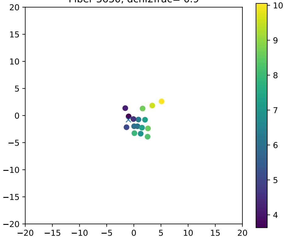
Fiber 3630, dchi2frac= 0.9
