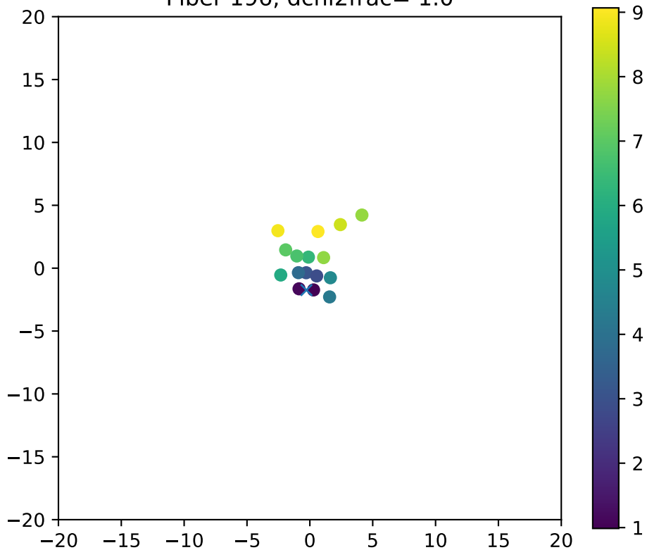
Fiber 196, dchi2frac= 1.0
