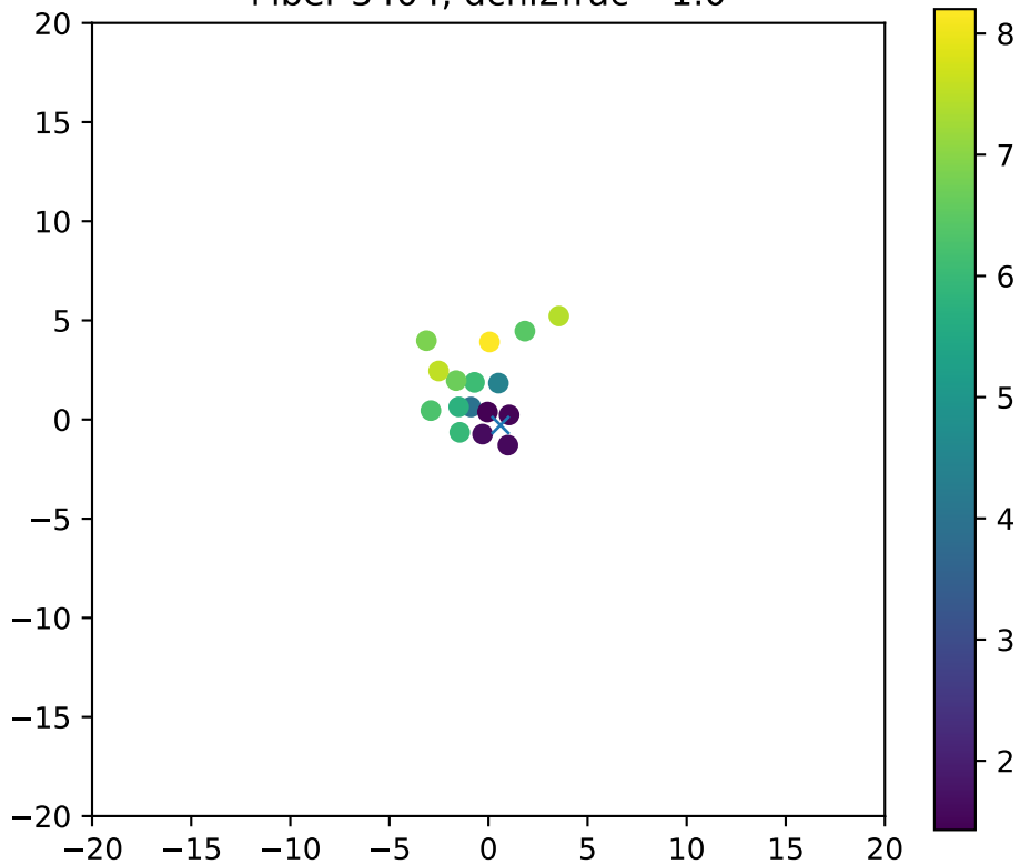
Fiber 3404, dchi2frac= 1.0
