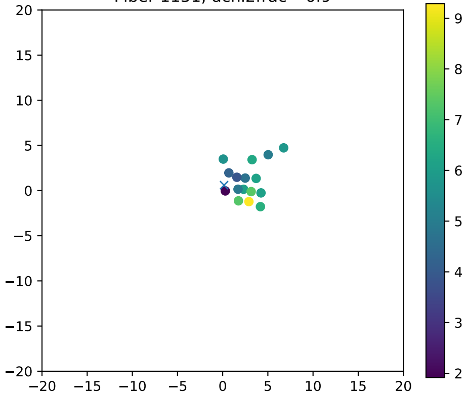
Fiber 1151, dchi2frac= 0.9
