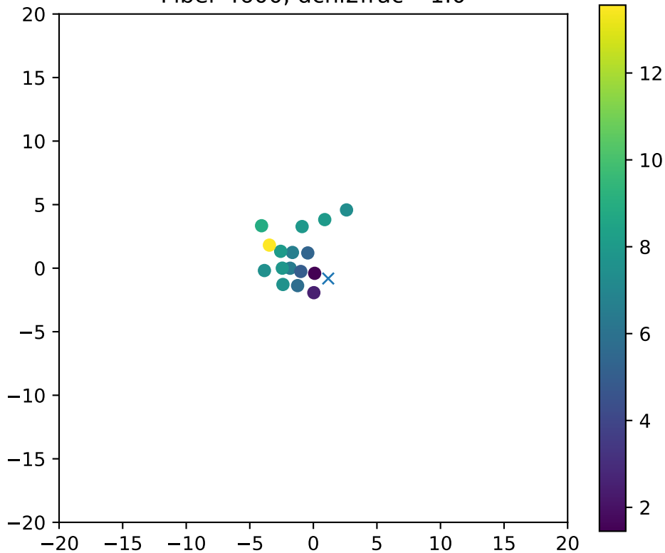
Fiber 4600, dchi2frac= 1.0
