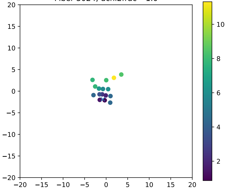
Fiber 3024, dchi2frac= 1.0
