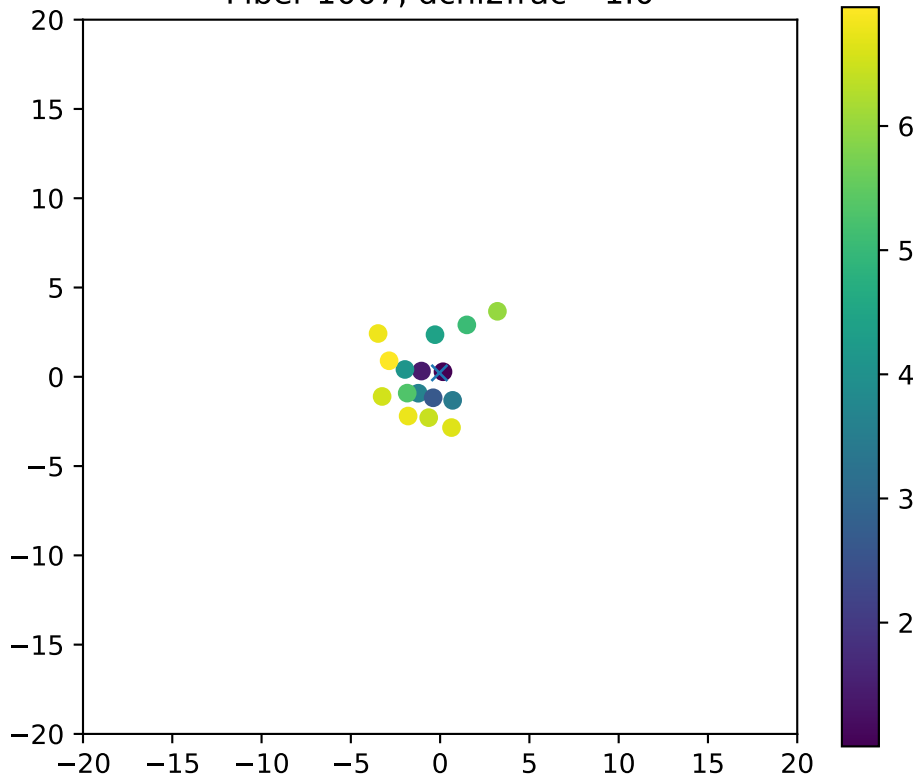
Fiber 1007, dchi2frac= 1.0
