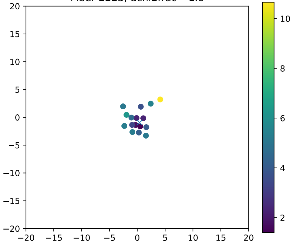
Fiber 2223, dchi2frac= 1.0
