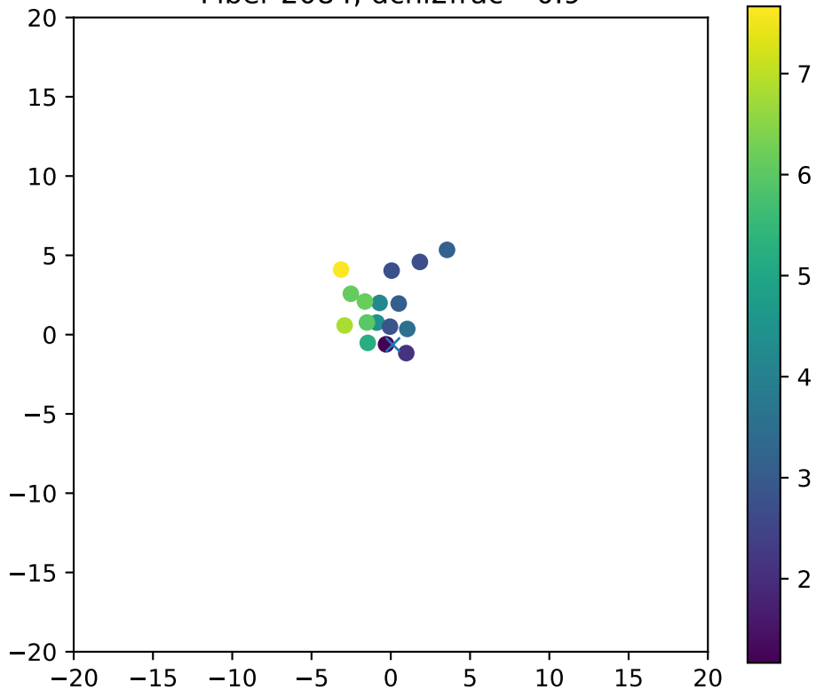
Fiber 2084, dchi2frac= 0.9
