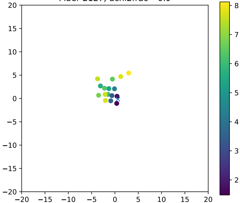
Fiber 2127, dchi2frac= 0.9
