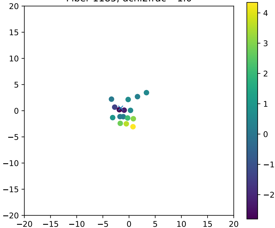
Fiber 1185, dchi2frac= 1.0
