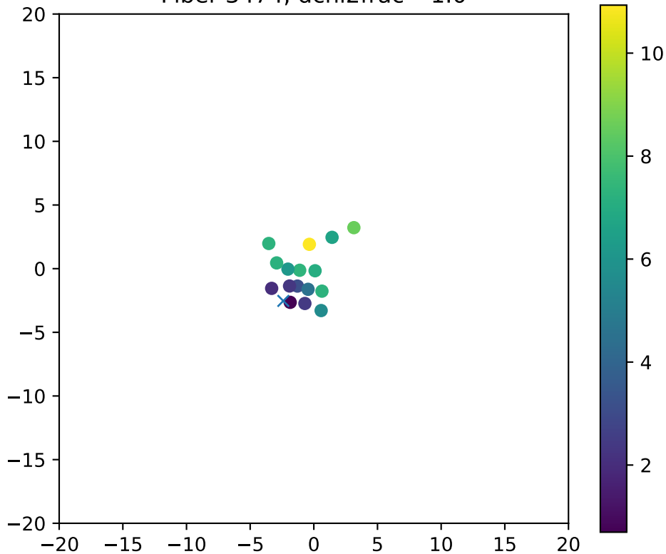
Fiber 3474, dchi2frac= 1.0
