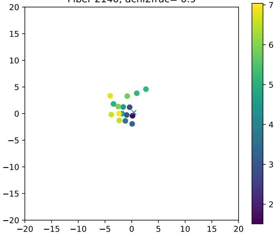
Fiber 2140, dchi2frac= 0.9
