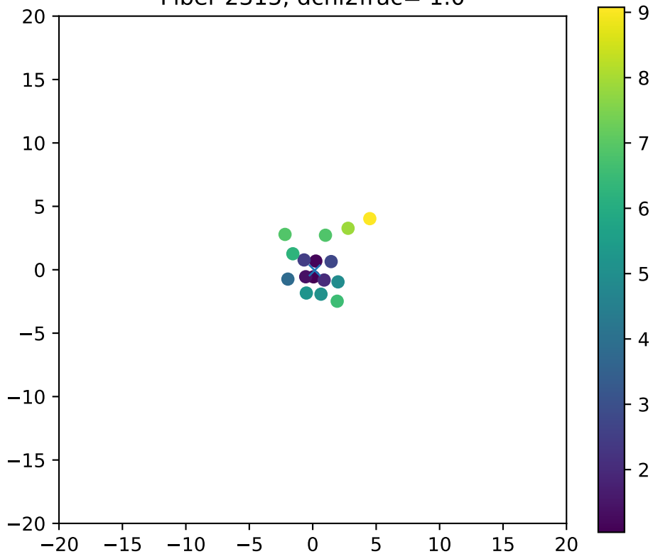
Fiber 2315, dchi2frac= 1.0
