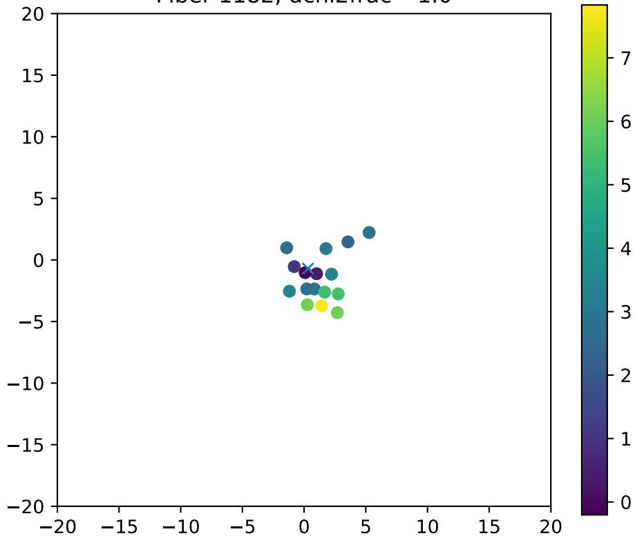
Fiber 1182, dchi2frac= 1.0
