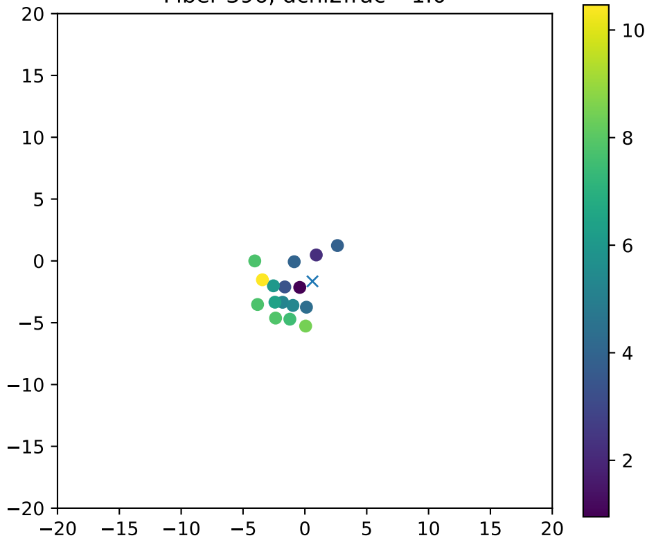
Fiber 396, dchi2frac= 1.0
