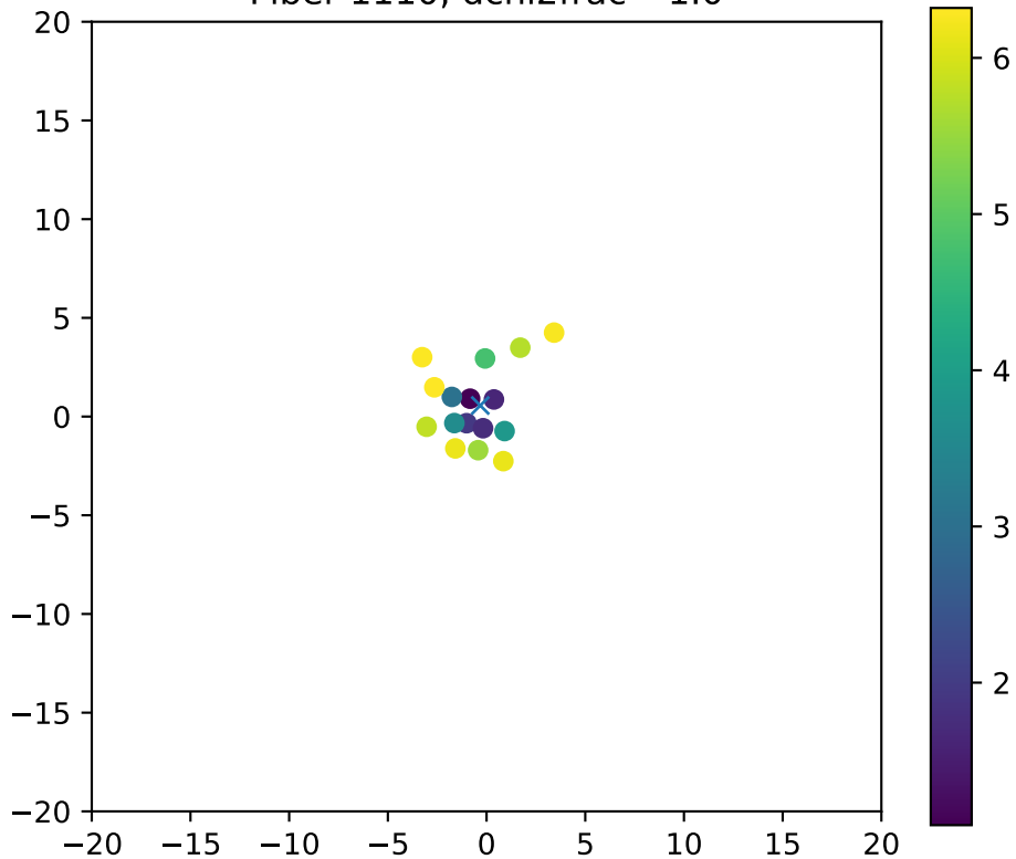
Fiber 1110, dchi2frac= 1.0
