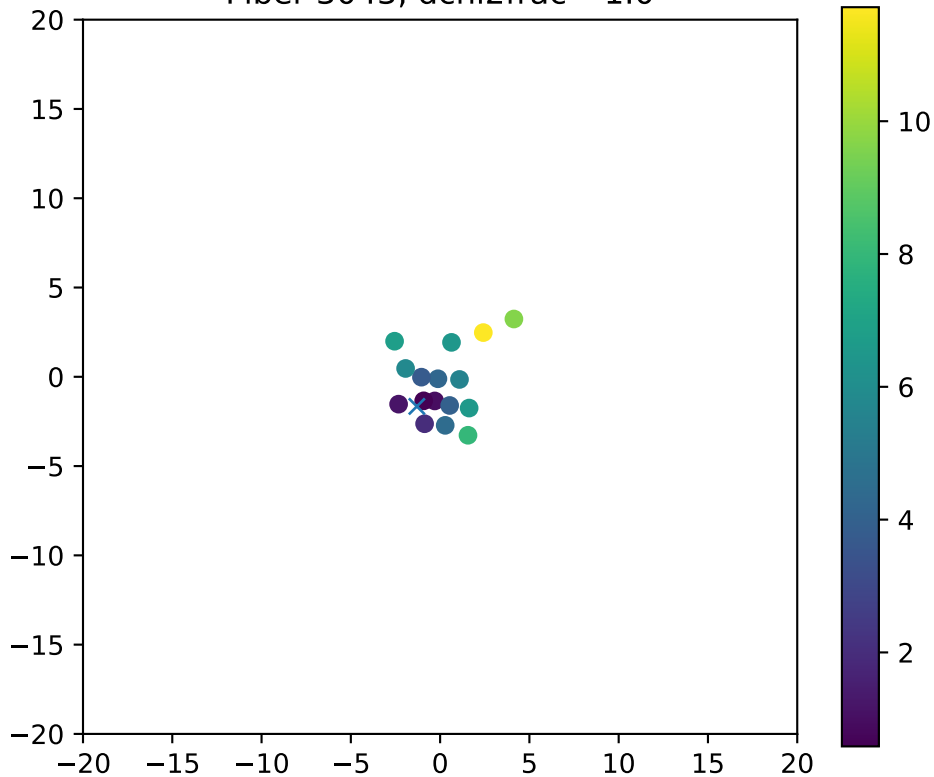
Fiber 3043, dchi2frac= 1.0
