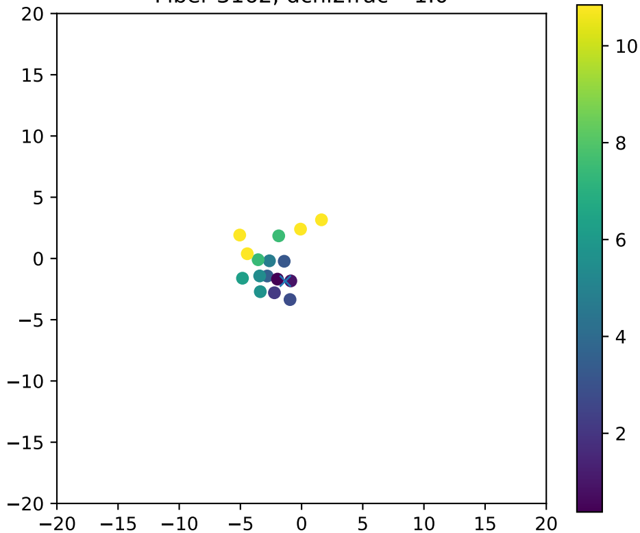
Fiber 3162, dchi2frac= 1.0
