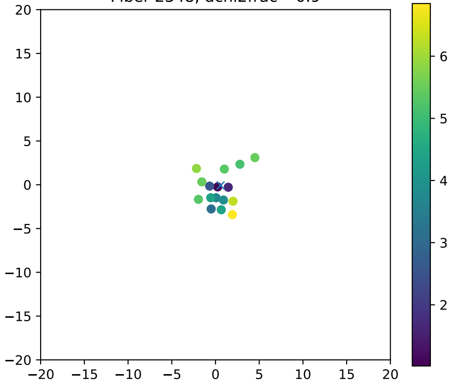
Fiber 2348, dchi2frac= 0.9
