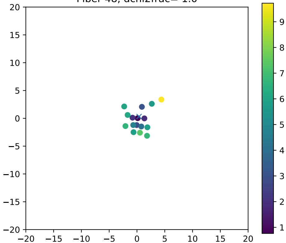
Fiber 48, dchi2frac= 1.0
