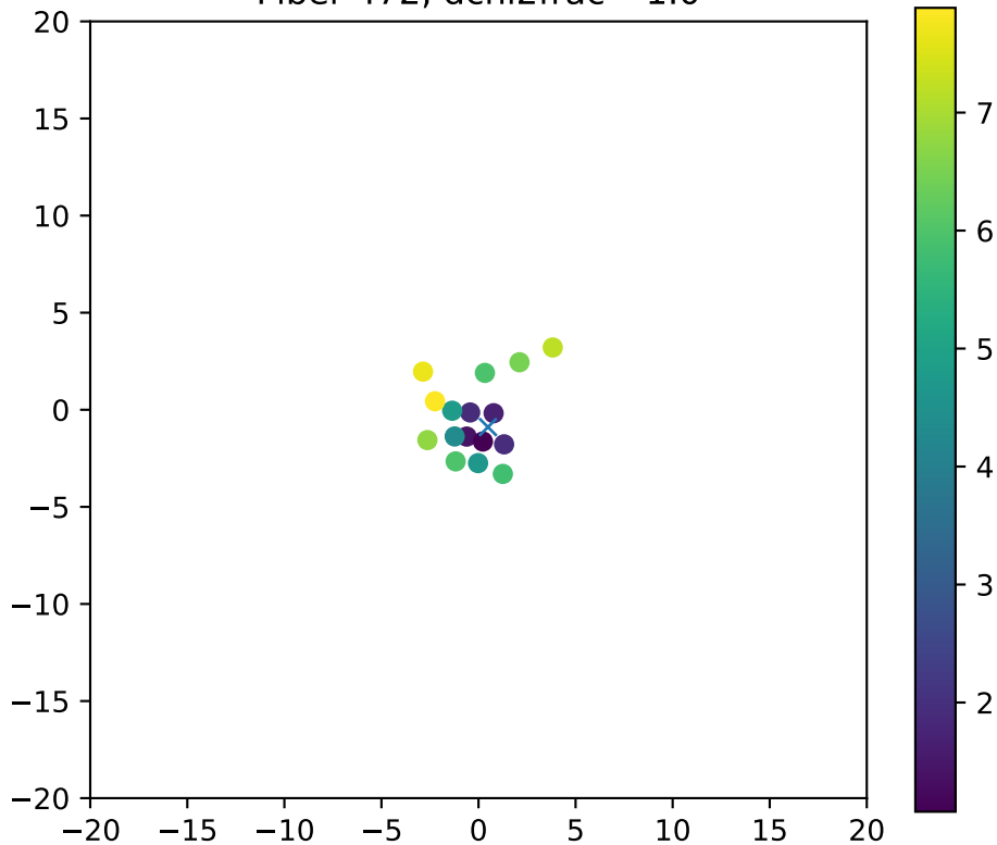
Fiber 472, dchi2frac= 1.0
