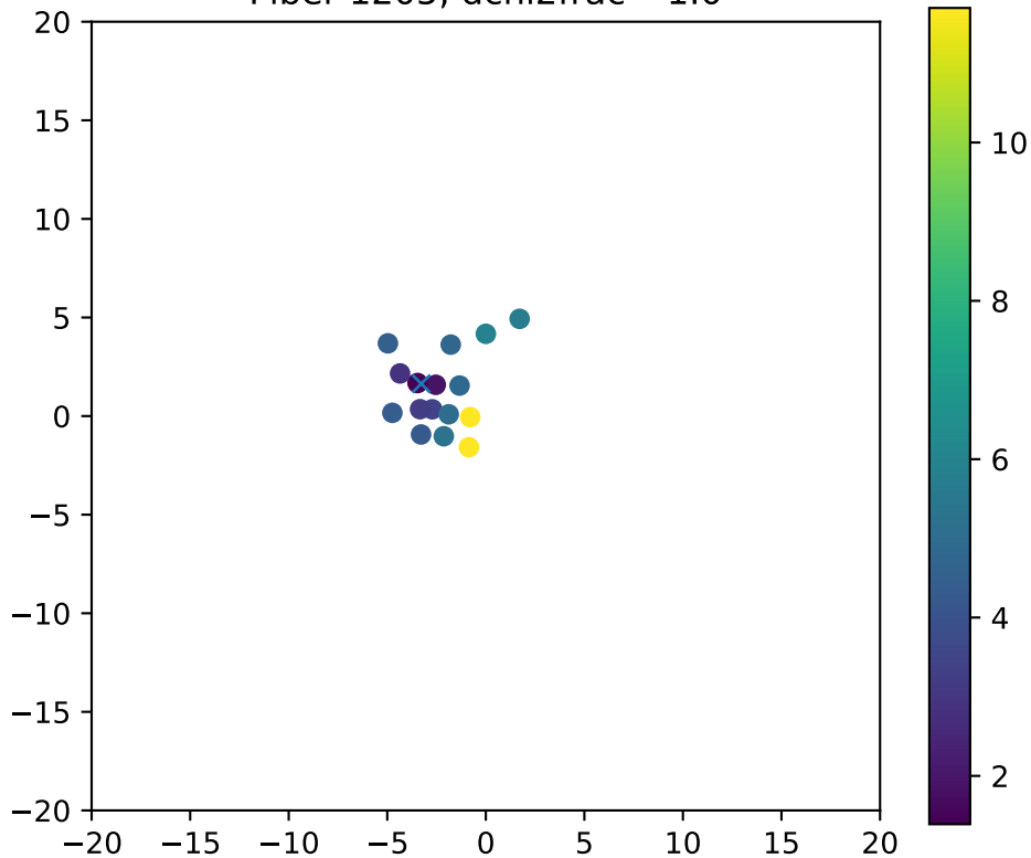
Fiber 1205, dchi2frac= 1.0
