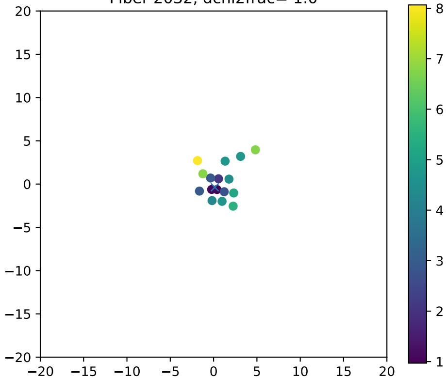
Fiber 2032, dchi2frac= 1.0
