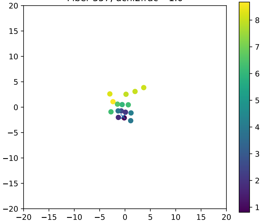
Fiber 357, dchi2frac= 1.0
