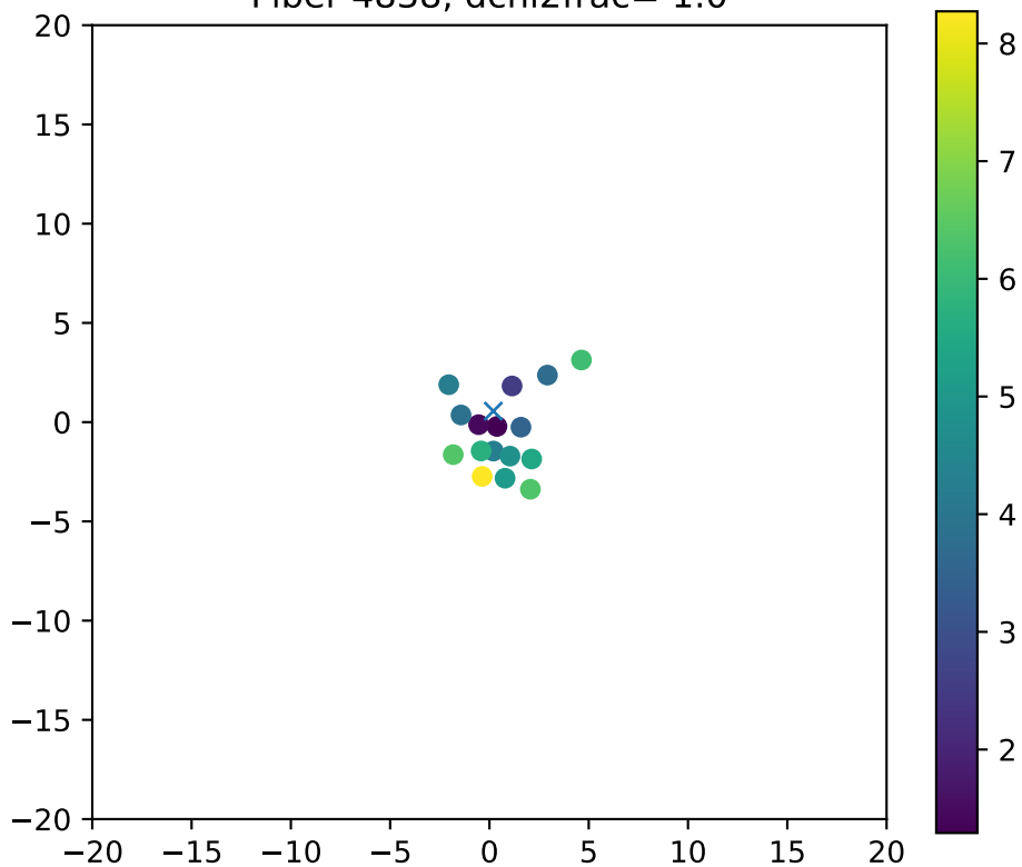
Fiber 4838, dchi2frac= 1.0
