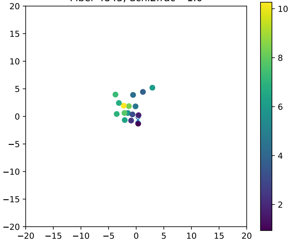
Fiber 4845, dchi2frac= 1.0
