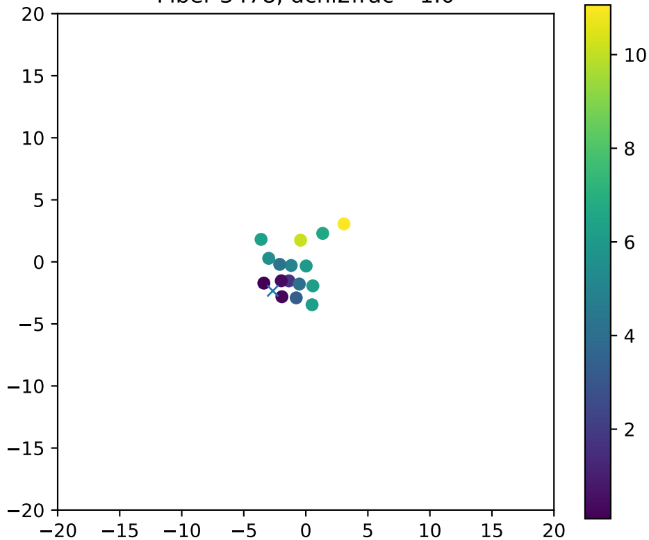
Fiber 3478, dchi2frac= 1.0
