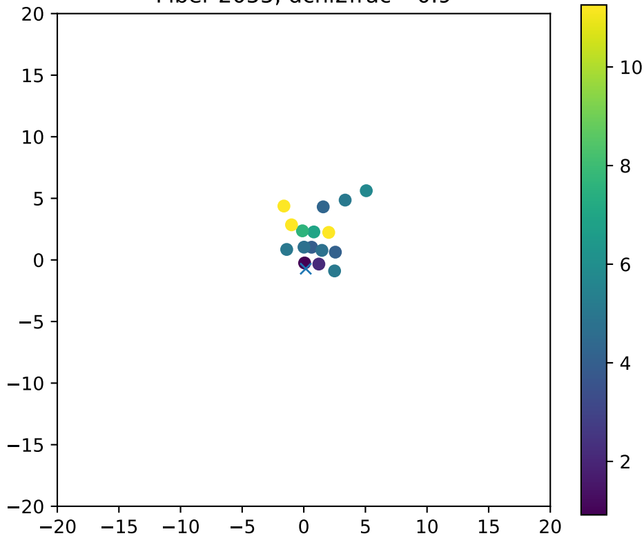
Fiber 2055, dchi2frac= 0.9
