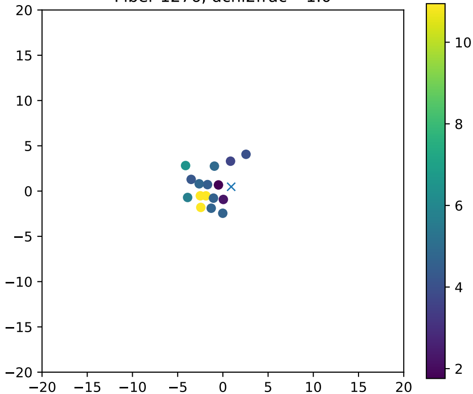
Fiber 1276, dchi2frac= 1.0
