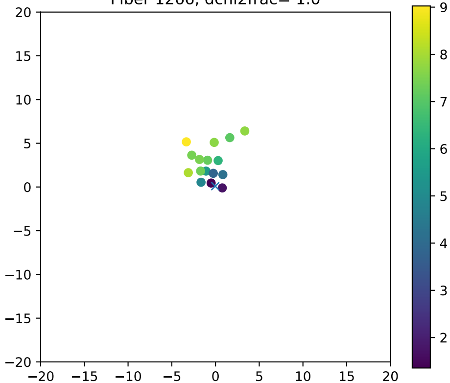
Fiber 1266, dchi2frac= 1.0
