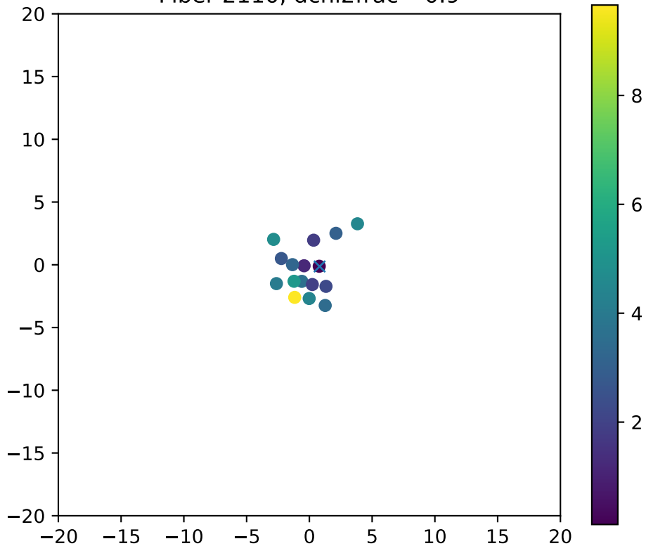
Fiber 2110, dchi2frac= 0.9
