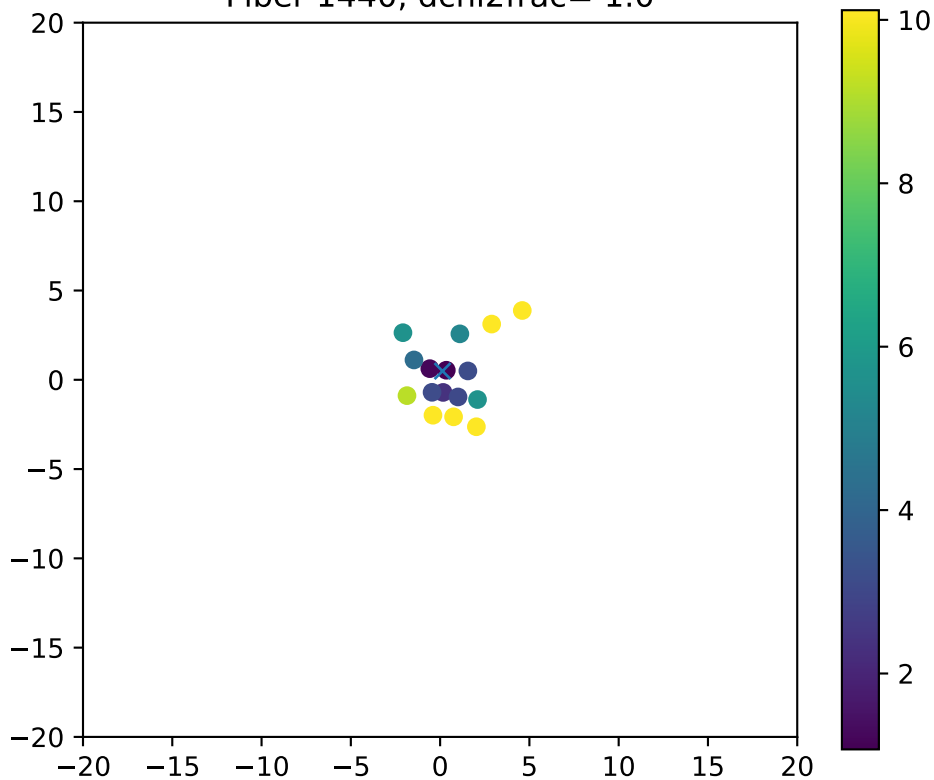
Fiber 1440, dchi2frac= 1.0
