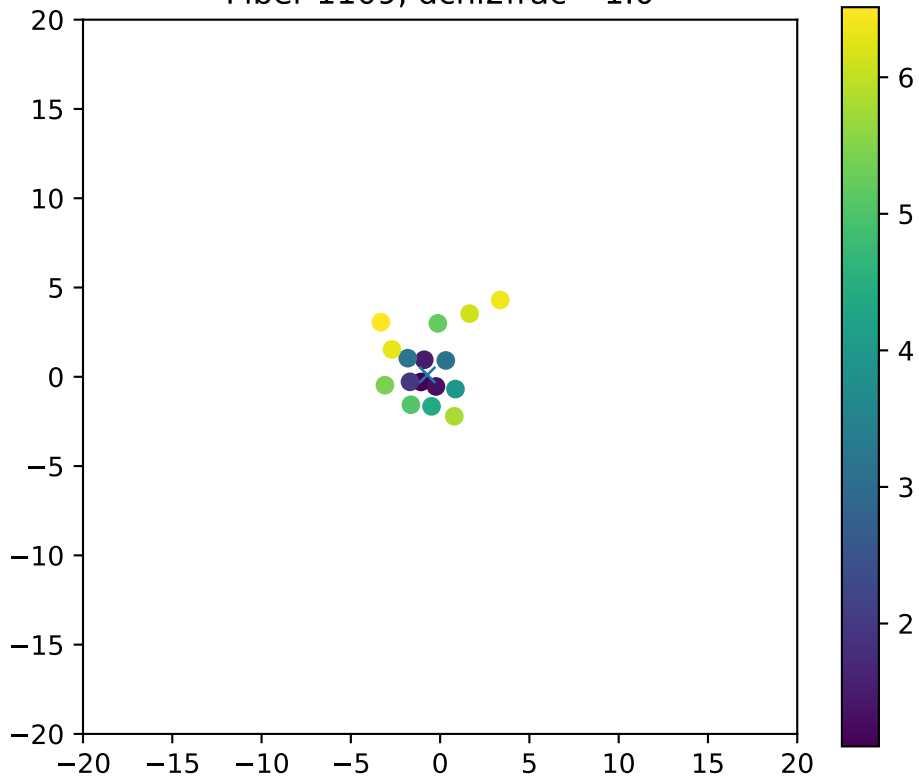
Fiber 1109, dchi2frac= 1.0
