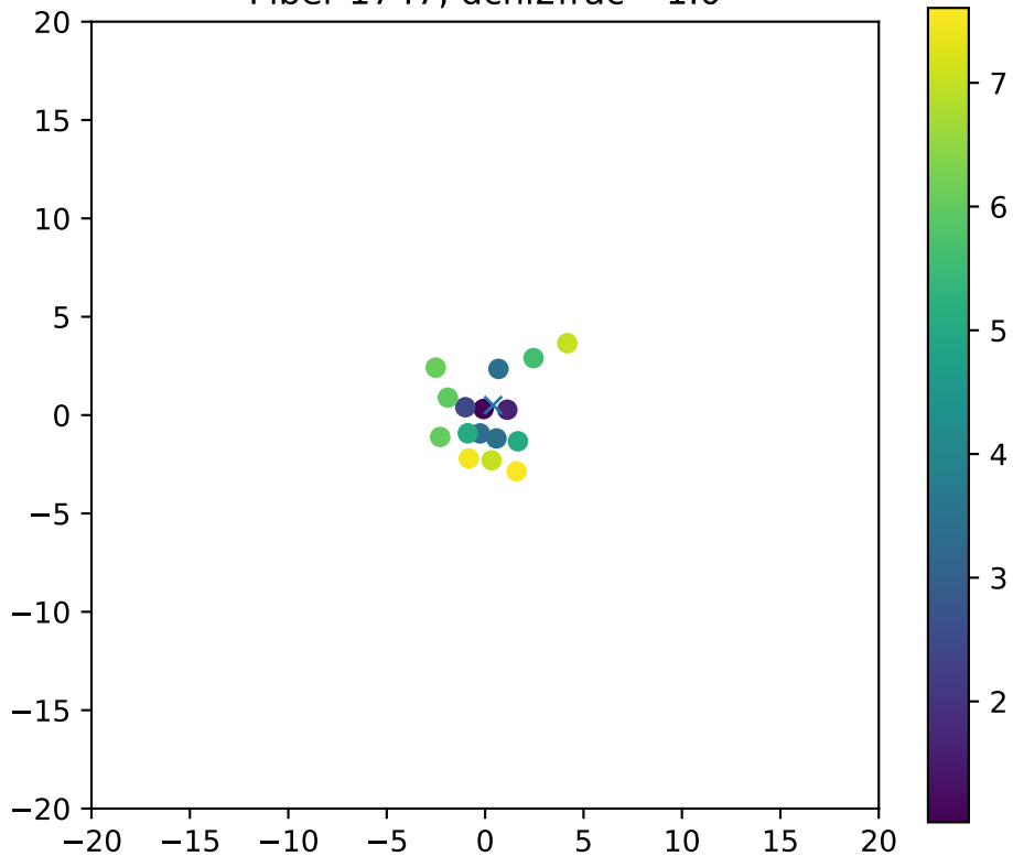
Fiber 1747, dchi2frac= 1.0
