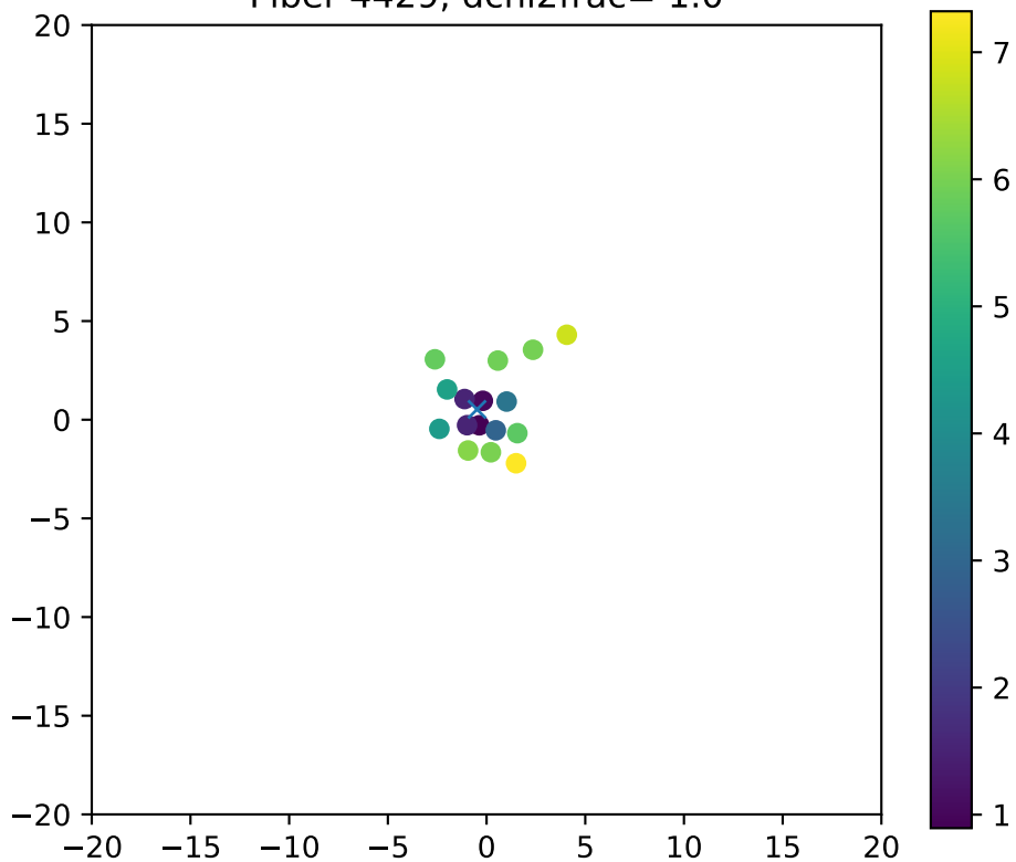
Fiber 4429, dchi2frac= 1.0
