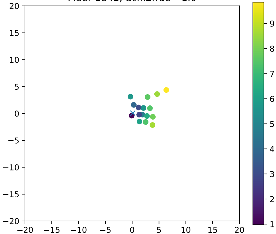
Fiber 1842, dchi2frac= 1.0
