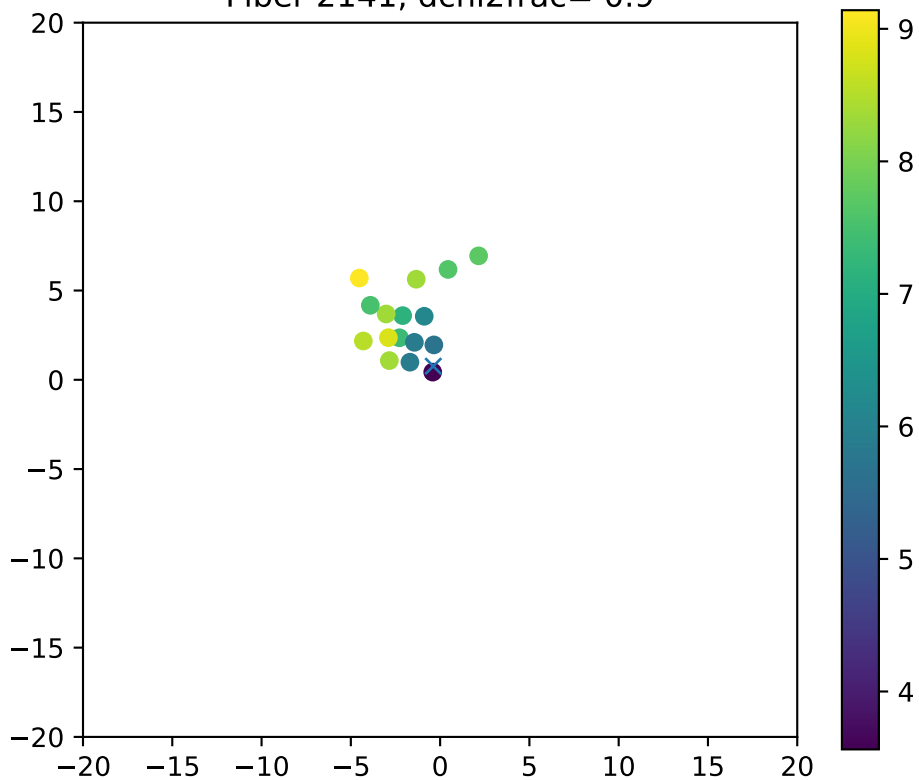
Fiber 2141, dchi2frac= 0.9
