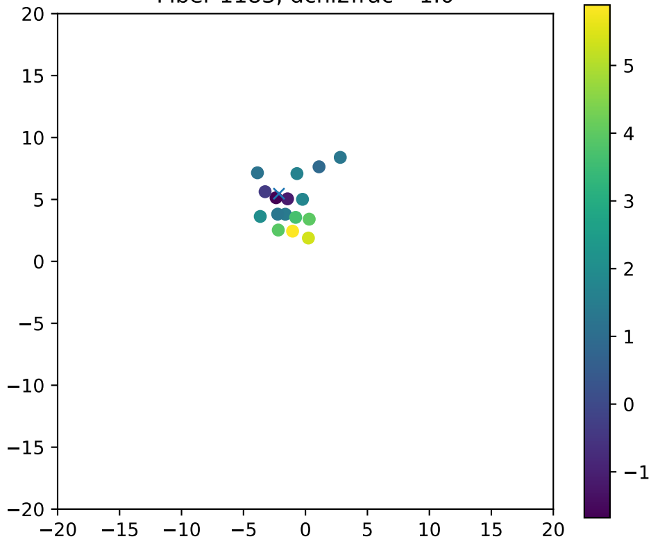
Fiber 1183, dchi2frac= 1.0
