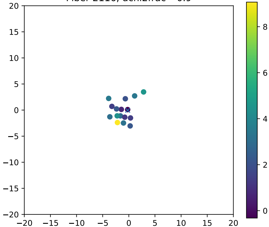
Fiber 2116, dchi2frac= 0.9
