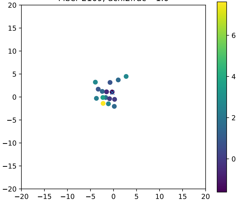
Fiber 2109, dchi2frac= 1.0
