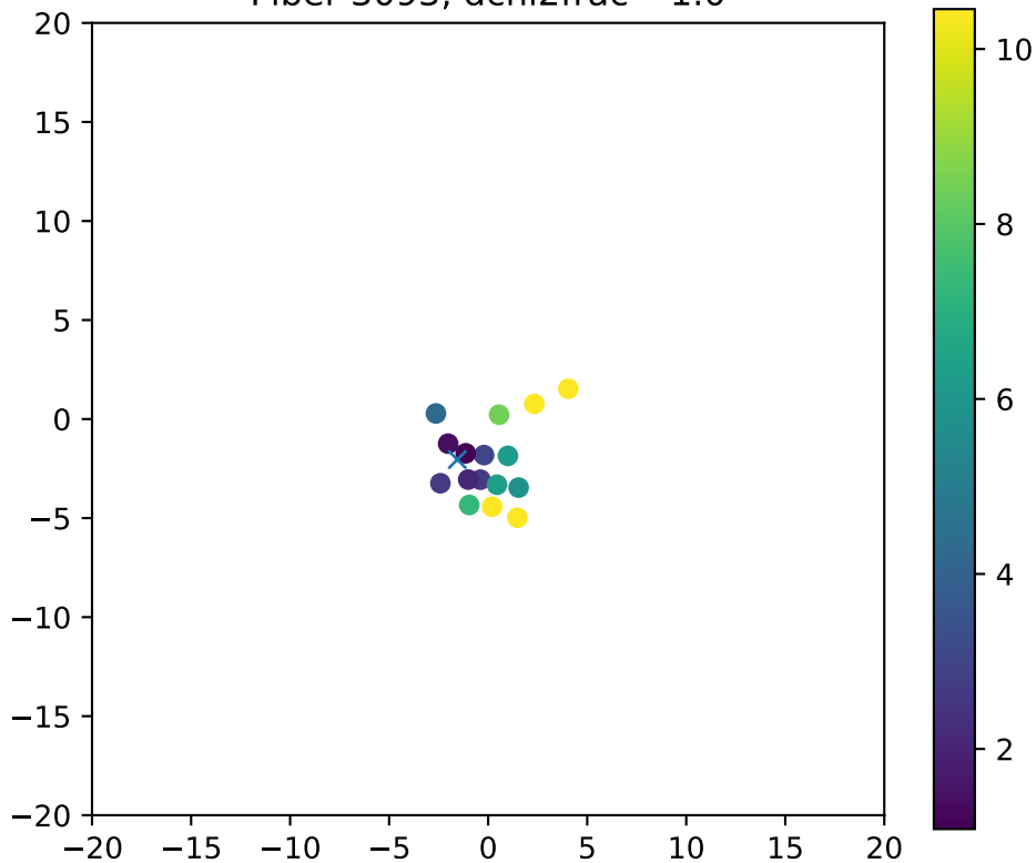
Fiber 3093, dchi2frac= 1.0
