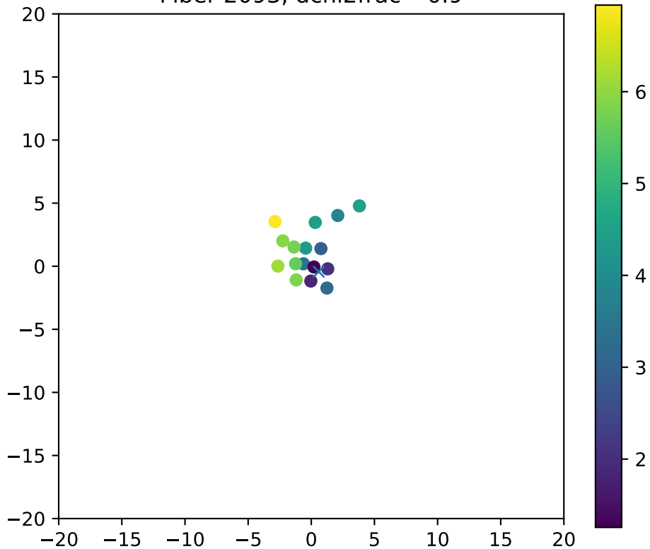
Fiber 2093, dchi2frac= 0.9
