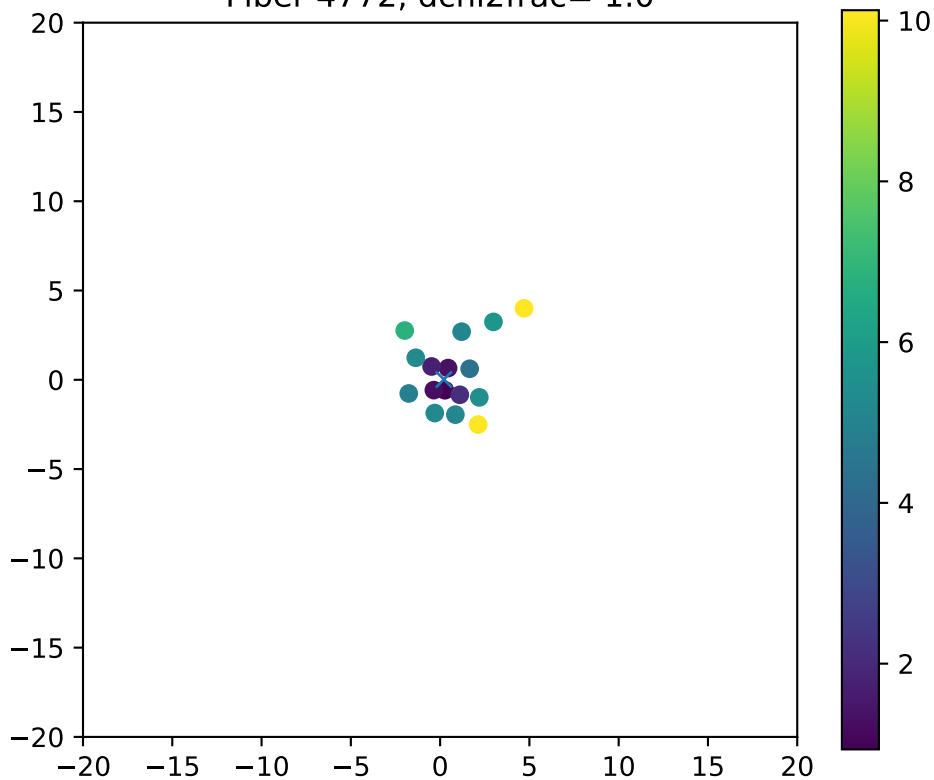
Fiber 4772, dchi2frac= 1.0
