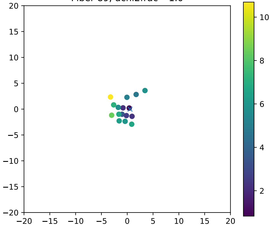
Fiber 89, dchi2frac= 1.0
