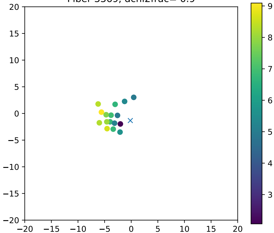
Fiber 3369, dchi2frac= 0.9
