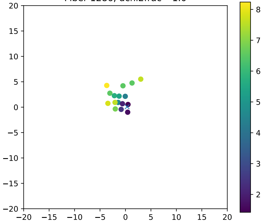
Fiber 1286, dchi2frac= 1.0
