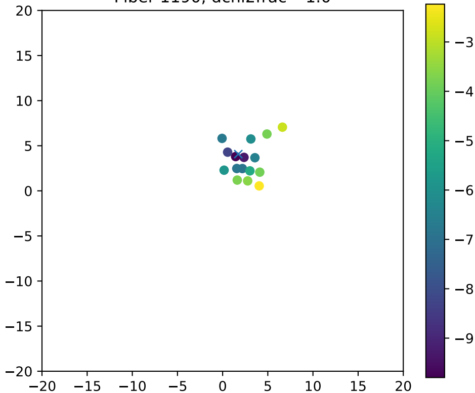
Fiber 1190, dchi2frac= 1.0
