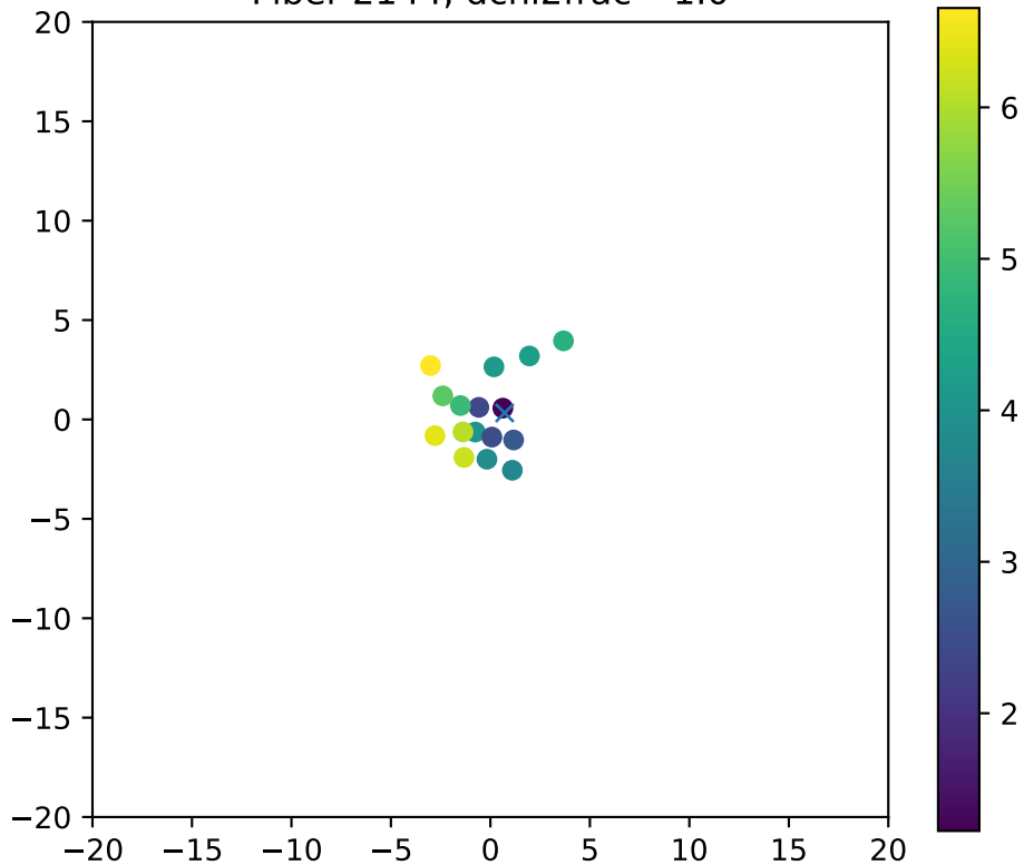
Fiber 2144, dchi2frac= 1.0
