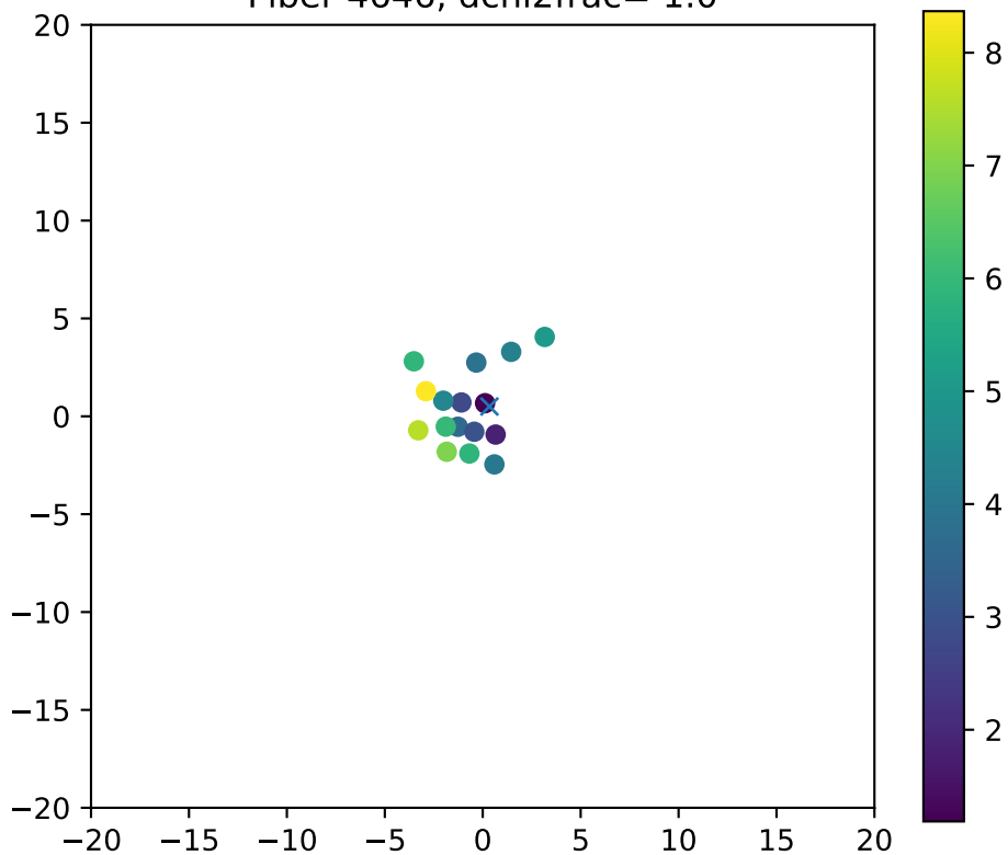
Fiber 4646, dchi2frac= 1.0
