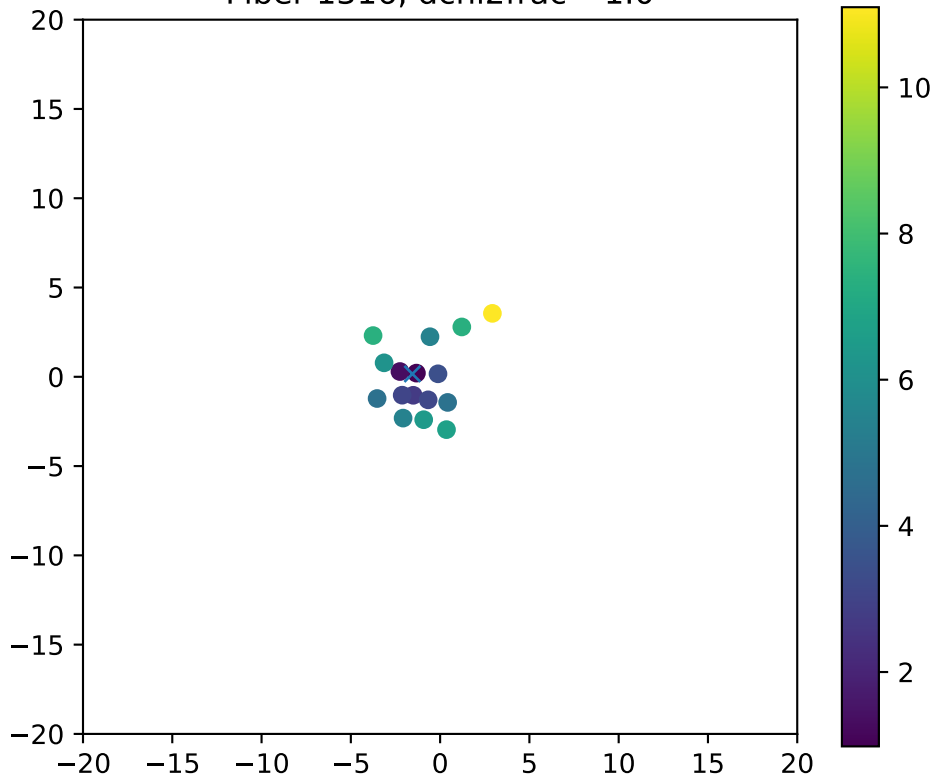
Fiber 1316, dchi2frac= 1.0
