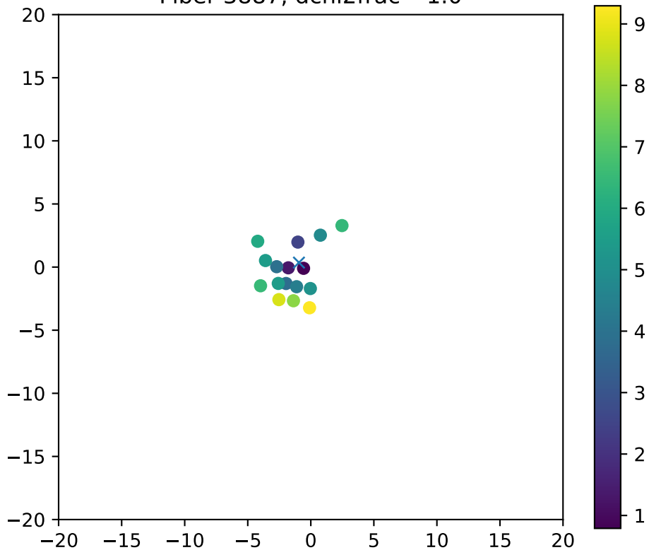
Fiber 3887, dchi2frac= 1.0
