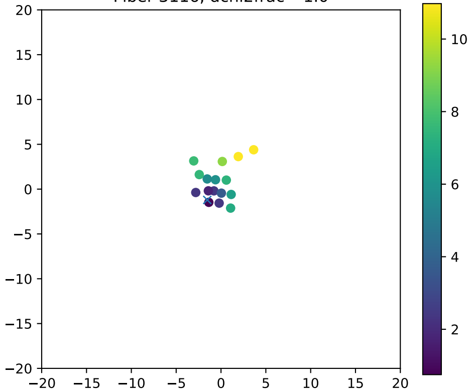
Fiber 3116, dchi2frac= 1.0
