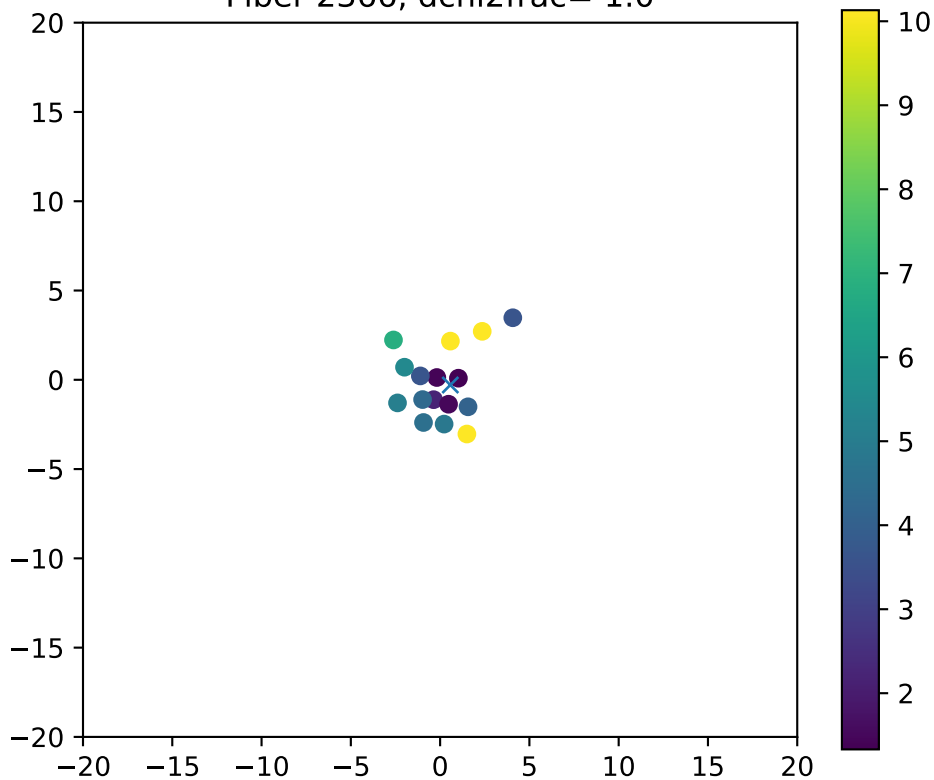
Fiber 2366, dchi2frac= 1.0
