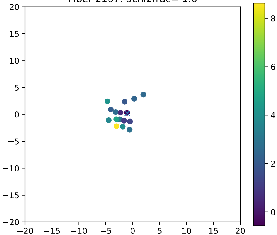
Fiber 2107, dchi2frac= 1.0
