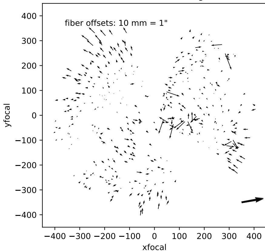
dither20200125-63070-highsnr-R
