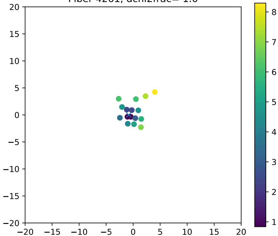
Fiber 4261, dchi2frac= 1.0
