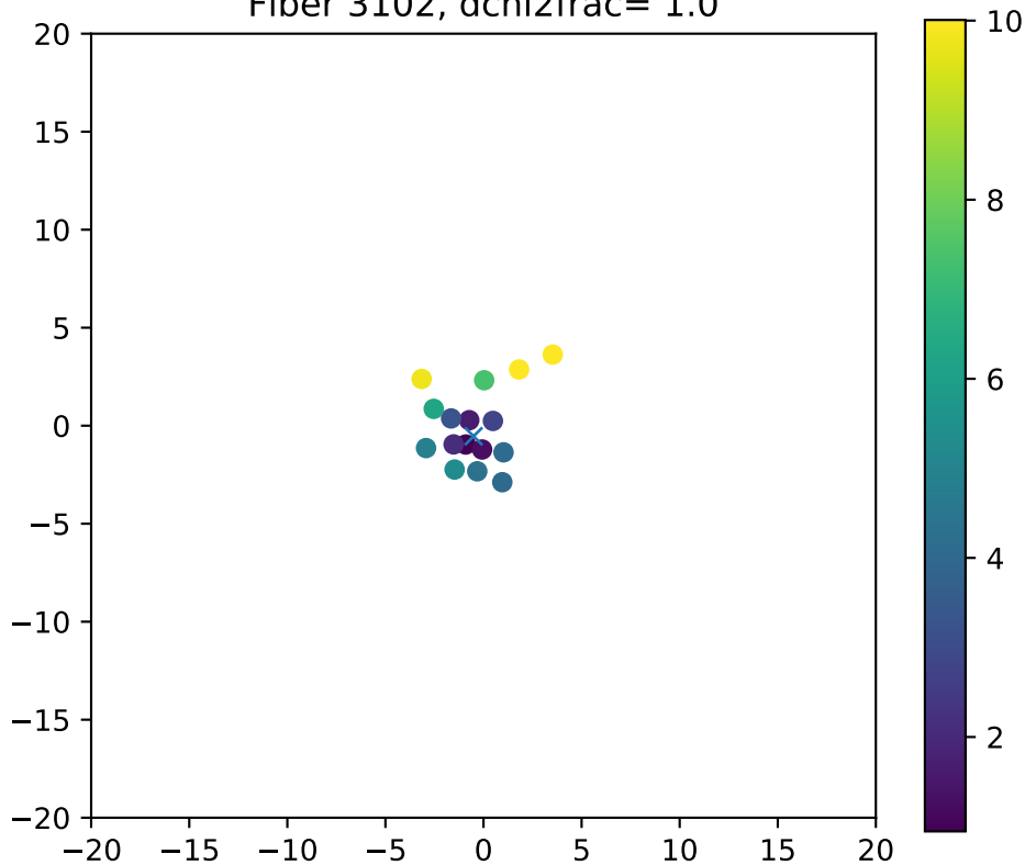
Fiber 3102, dchi2frac= 1.0
