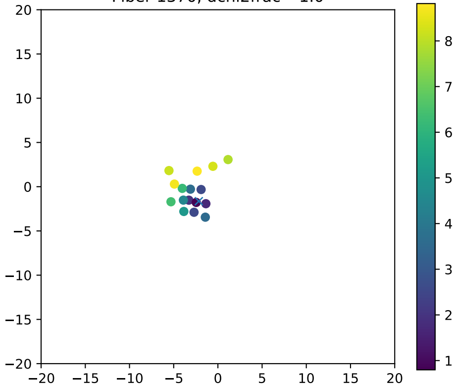
Fiber 1370, dchi2frac= 1.0
