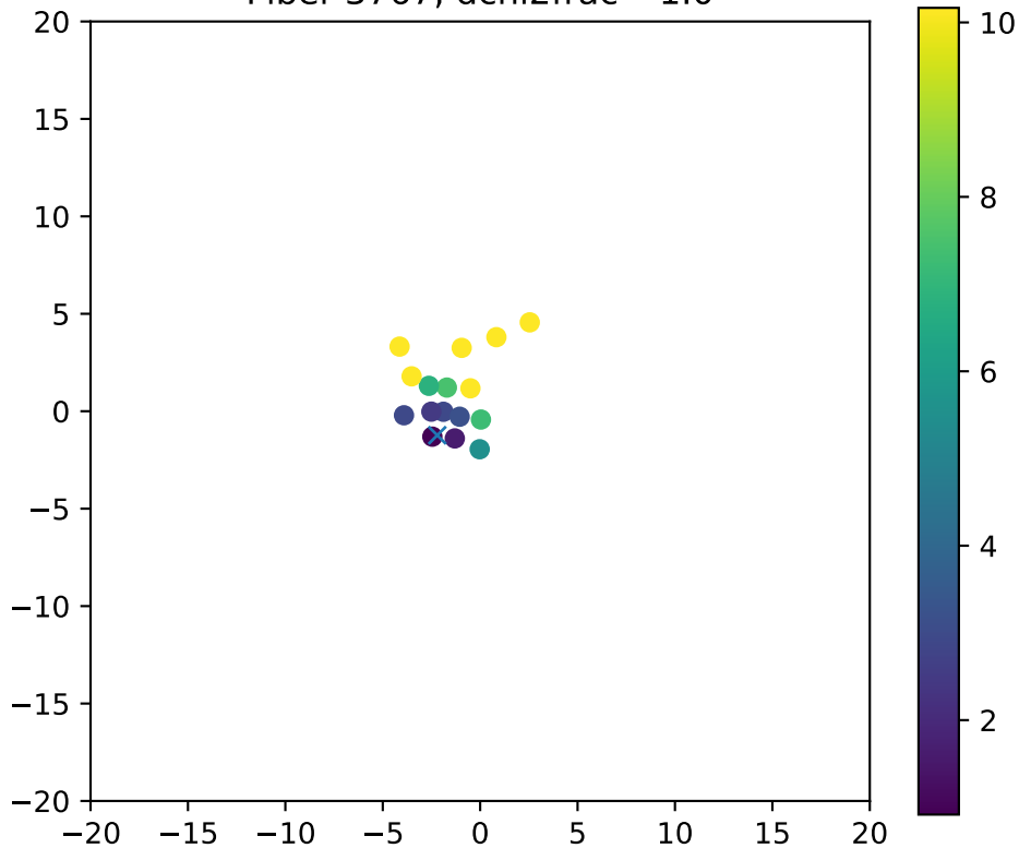
Fiber 3767, dchi2frac= 1.0
