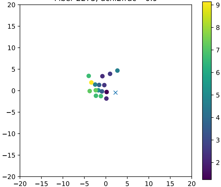
Fiber 2273, dchi2frac= 0.9
