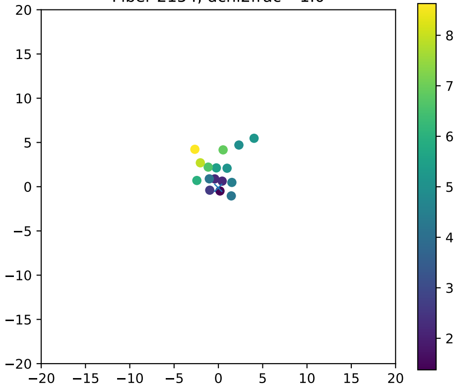
Fiber 2154, dchi2frac= 1.0
