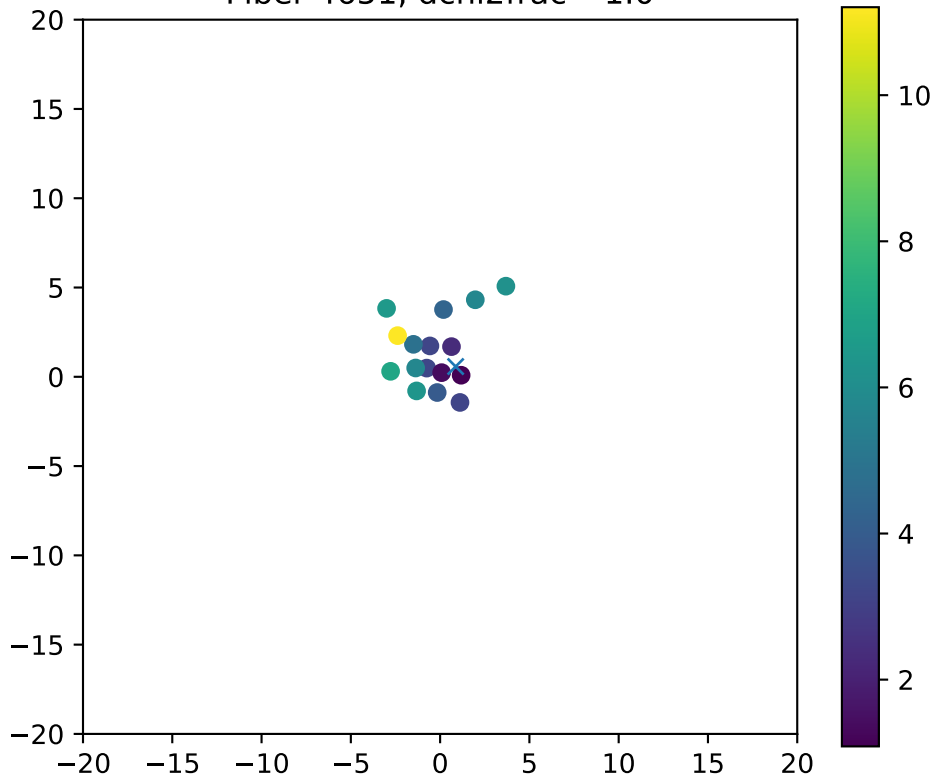
Fiber 4651, dchi2frac= 1.0
