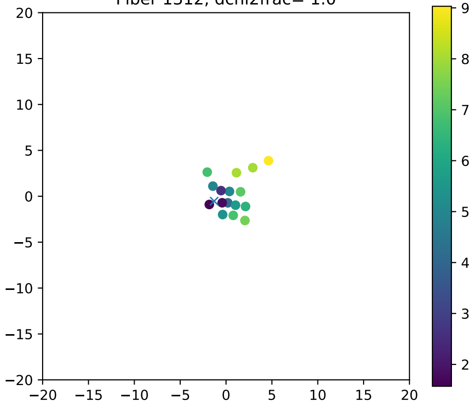
Fiber 1312, dchi2frac= 1.0
