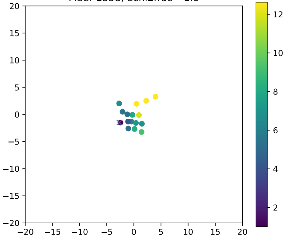
Fiber 1358, dchi2frac= 1.0
