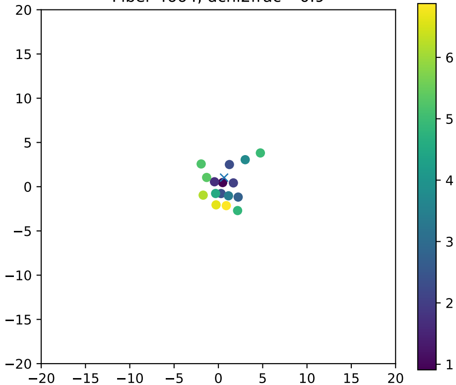
Fiber 4664, dchi2frac= 0.9
