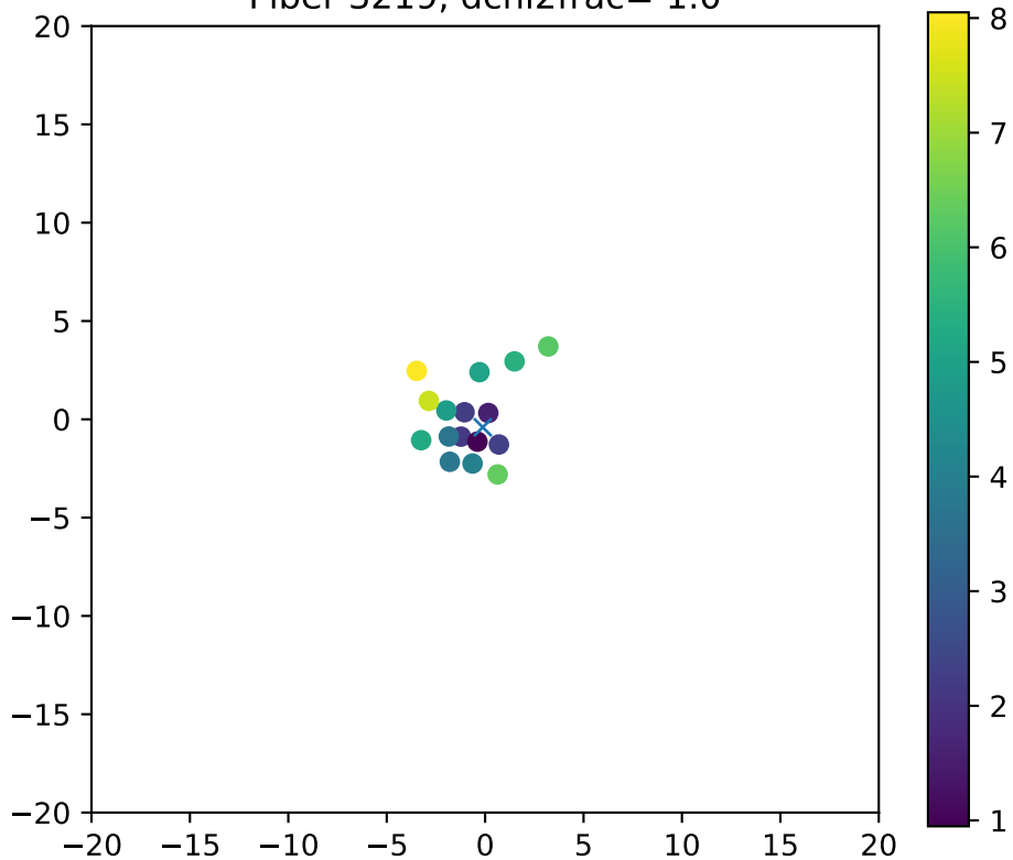
Fiber 3219, dchi2frac= 1.0
