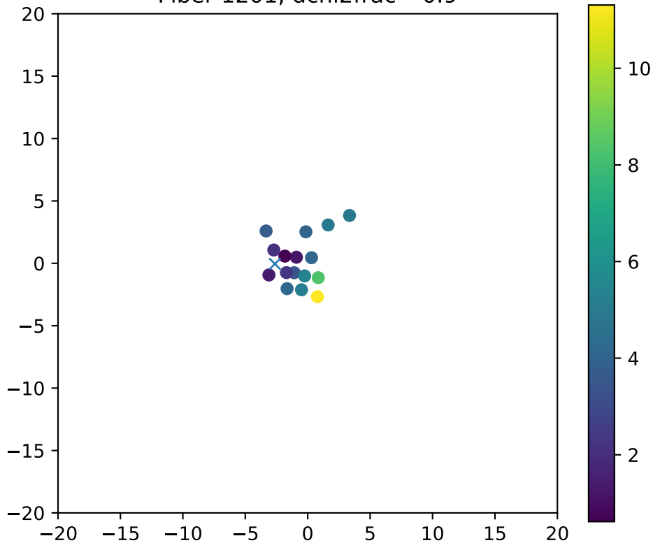
Fiber 1201, dchi2frac= 0.9
