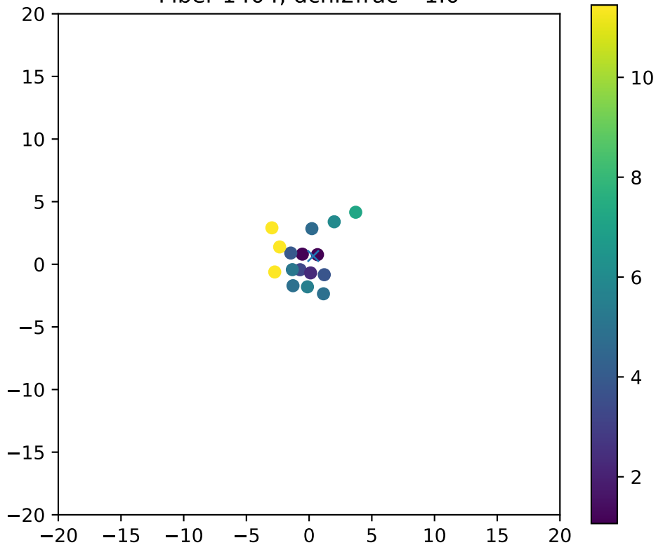
Fiber 1404, dchi2frac= 1.0
