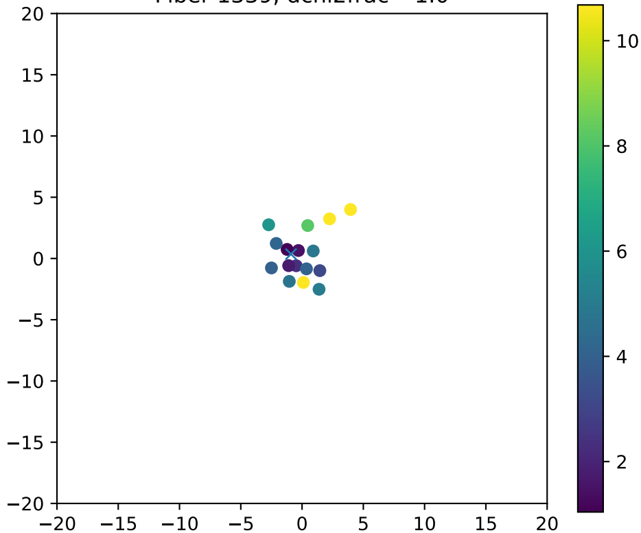
Fiber 1339, dchi2frac= 1.0
