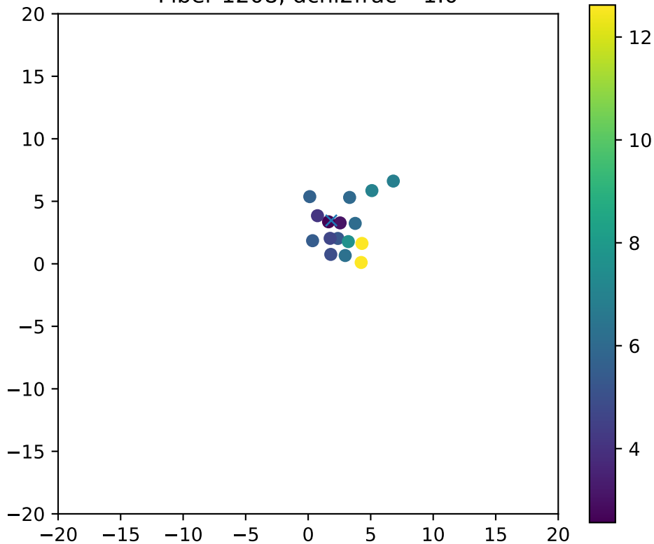
Fiber 1208, dchi2frac= 1.0
