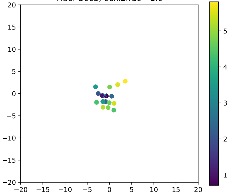
Fiber 3663, dchi2frac= 1.0
