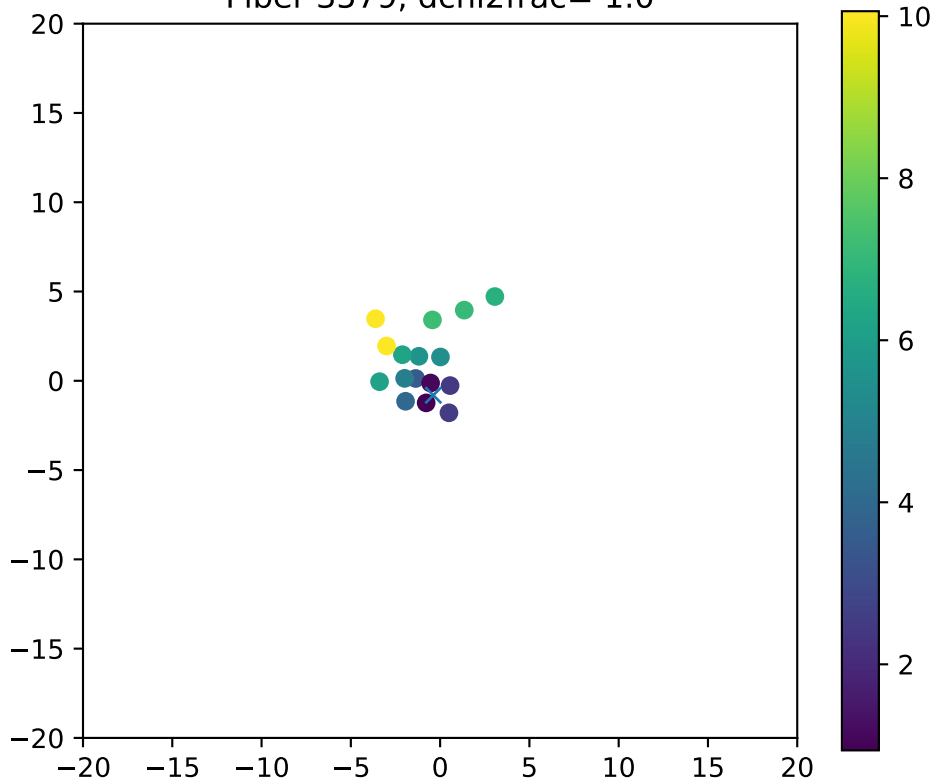
Fiber 3579, dchi2frac= 1.0
