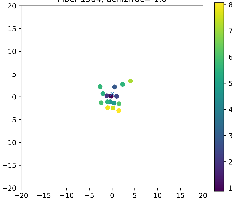
Fiber 1564, dchi2frac= 1.0
