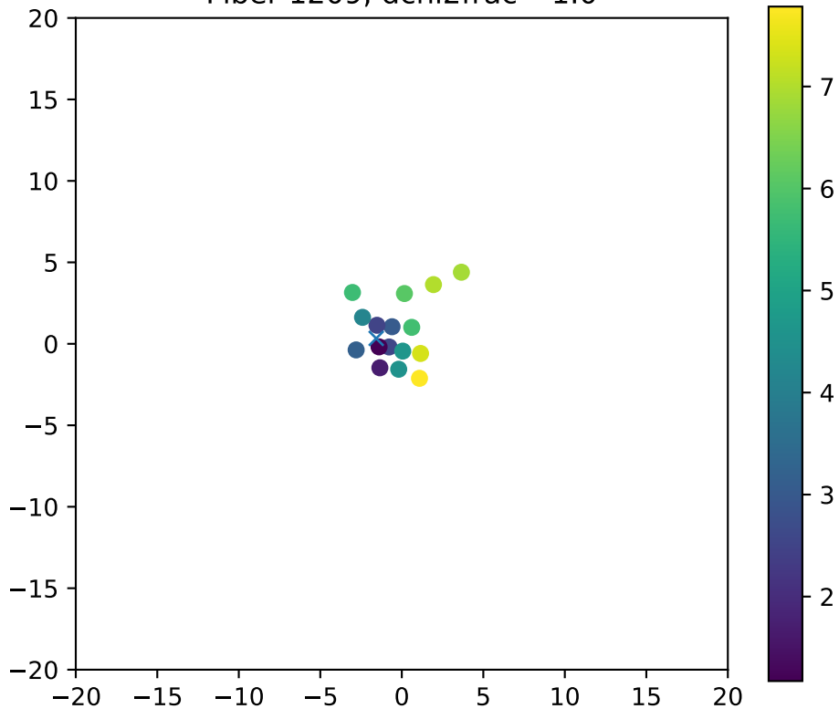
Fiber 1209, dchi2frac= 1.0
