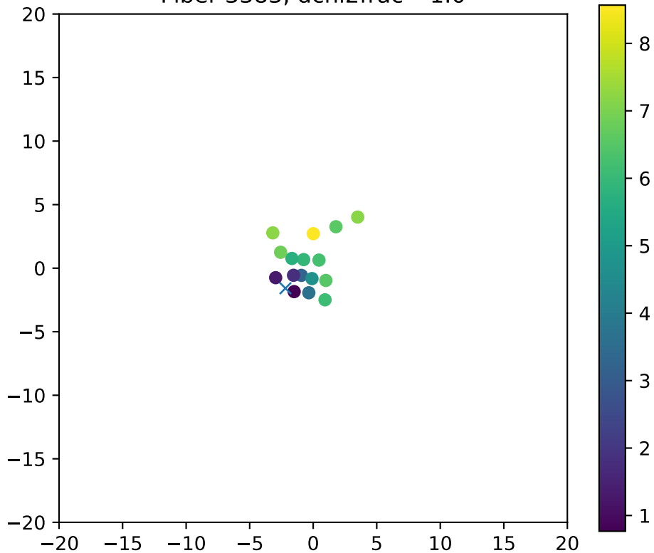
Fiber 3383, dchi2frac= 1.0
