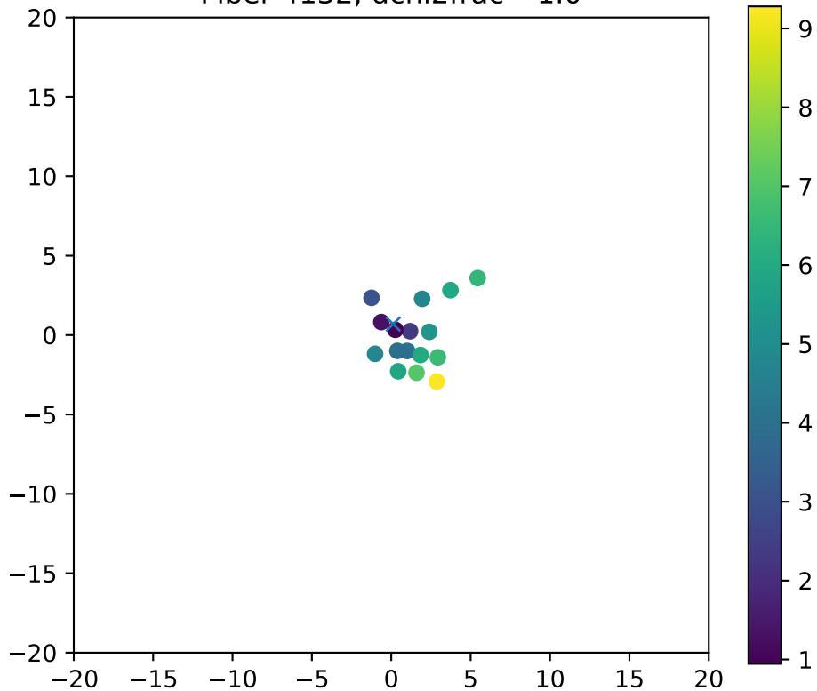
Fiber 4132, dchi2frac= 1.0
