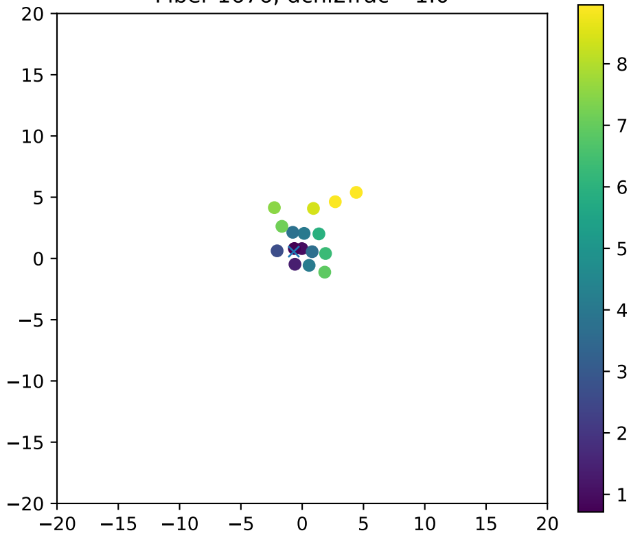
Fiber 1676, dchi2frac= 1.0
