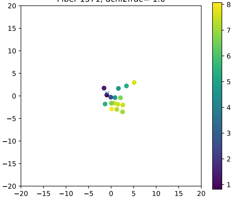
Fiber 1571, dchi2frac= 1.0
