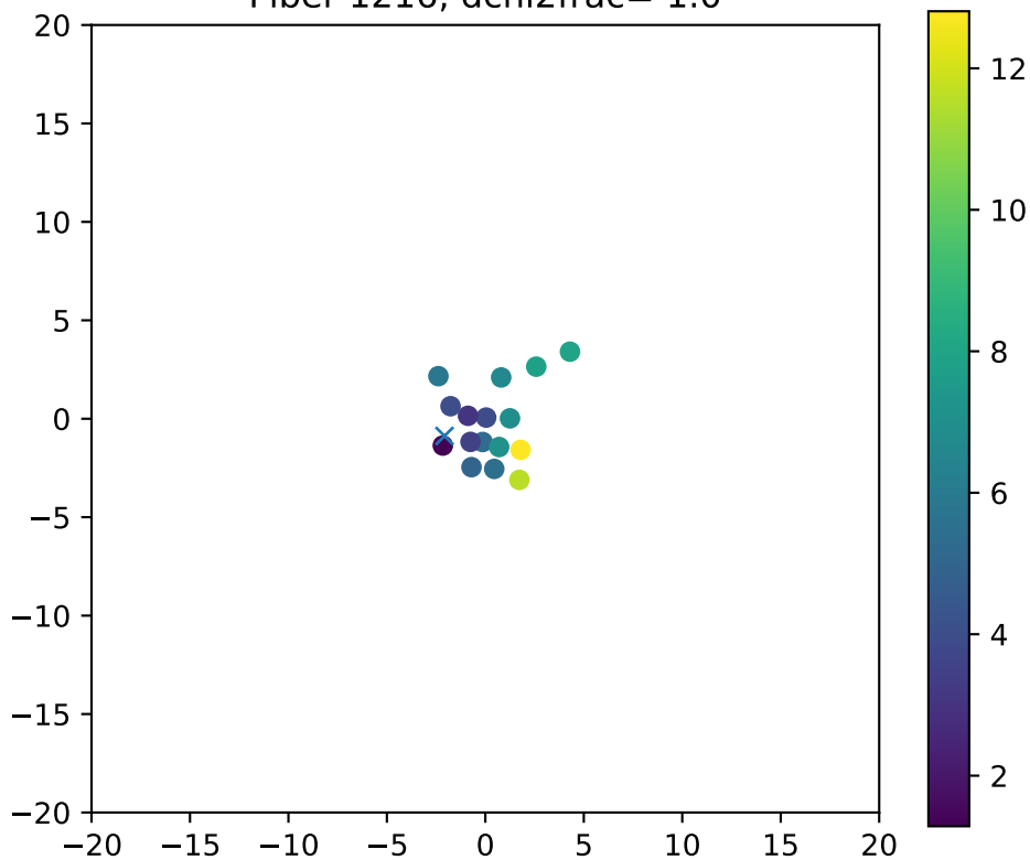
Fiber 1216, dchi2frac= 1.0
