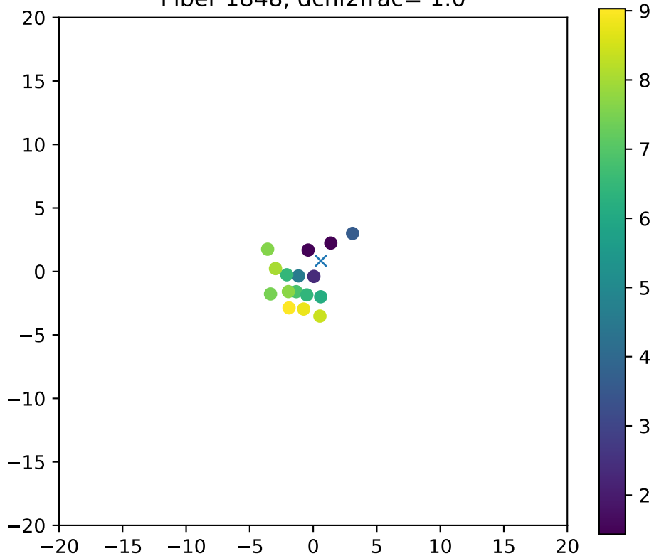
Fiber 1848, dchi2frac= 1.0
