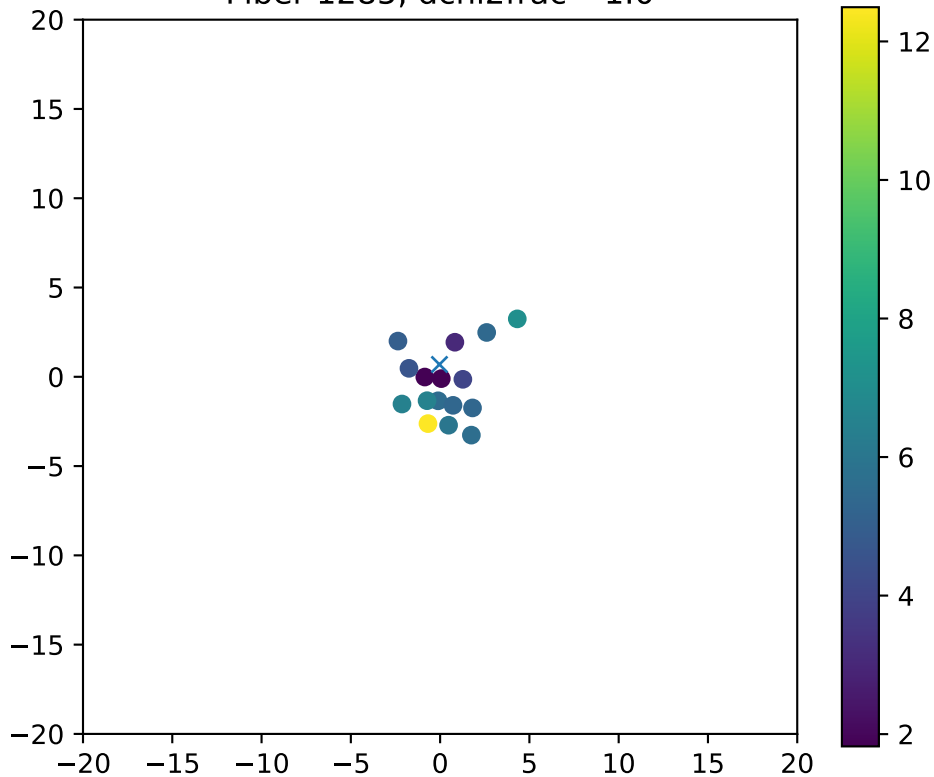
Fiber 1285, dchi2frac= 1.0
