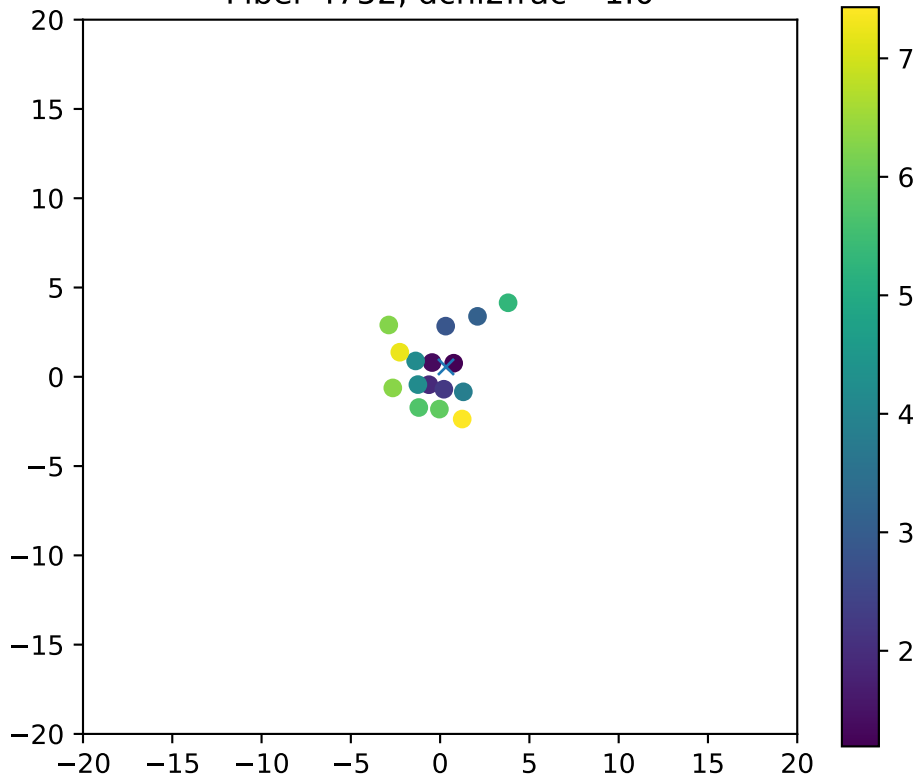
Fiber 4752, dchi2frac= 1.0
