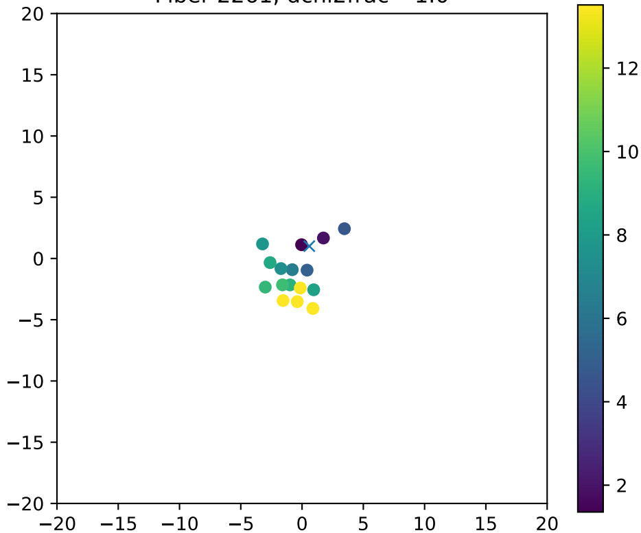
Fiber 2261, dchi2frac= 1.0
