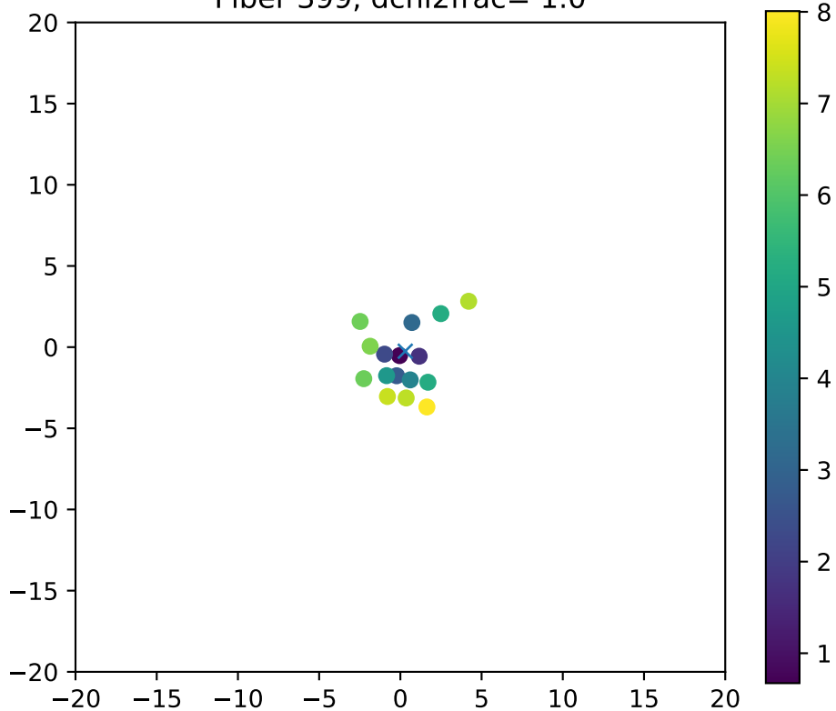
Fiber 399, dchi2frac= 1.0
