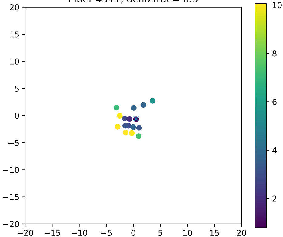
Fiber 4511, dchi2frac= 0.9
