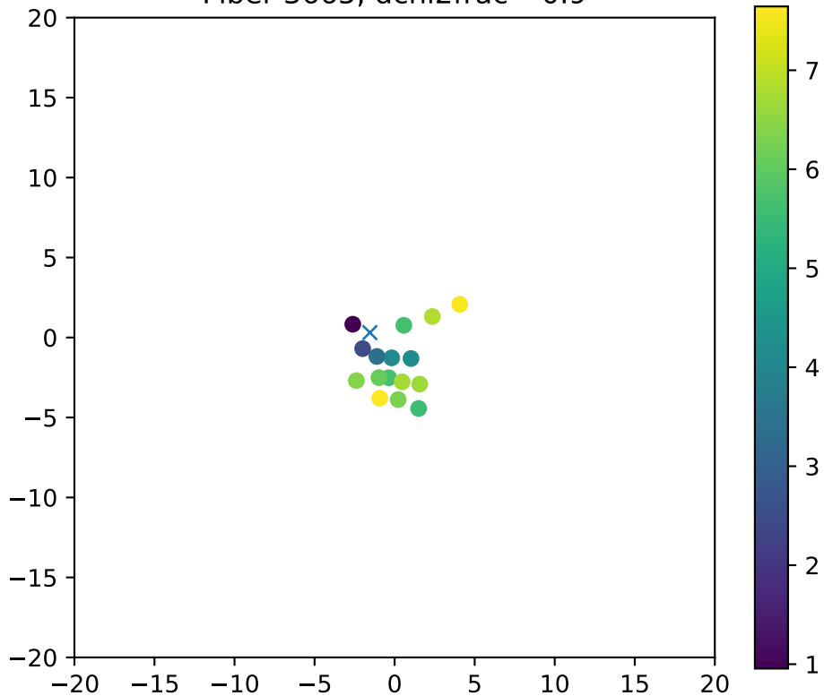
Fiber 3665, dchi2frac= 0.9
