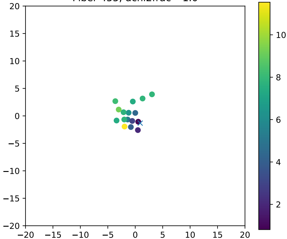
Fiber 455, dchi2frac= 1.0
