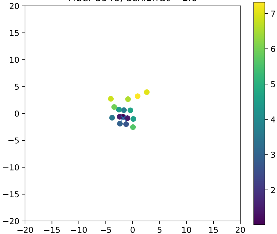
Fiber 3946, dchi2frac= 1.0
