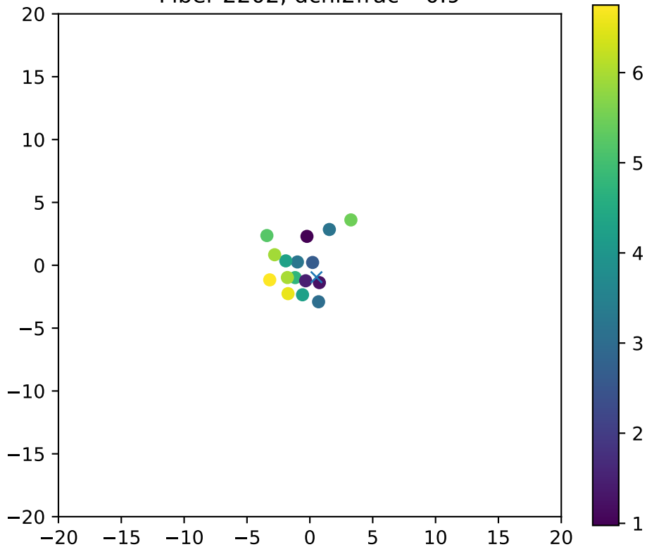
Fiber 2202, dchi2frac= 0.9
