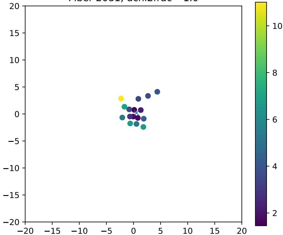
Fiber 2081, dchi2frac= 1.0
