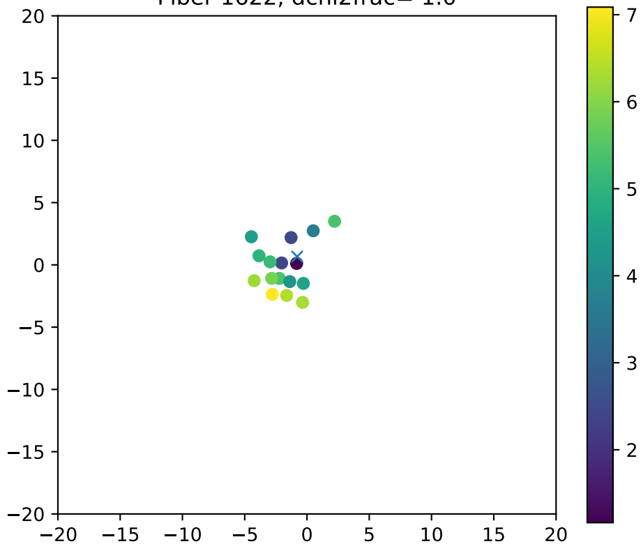
Fiber 1622, dchi2frac= 1.0
