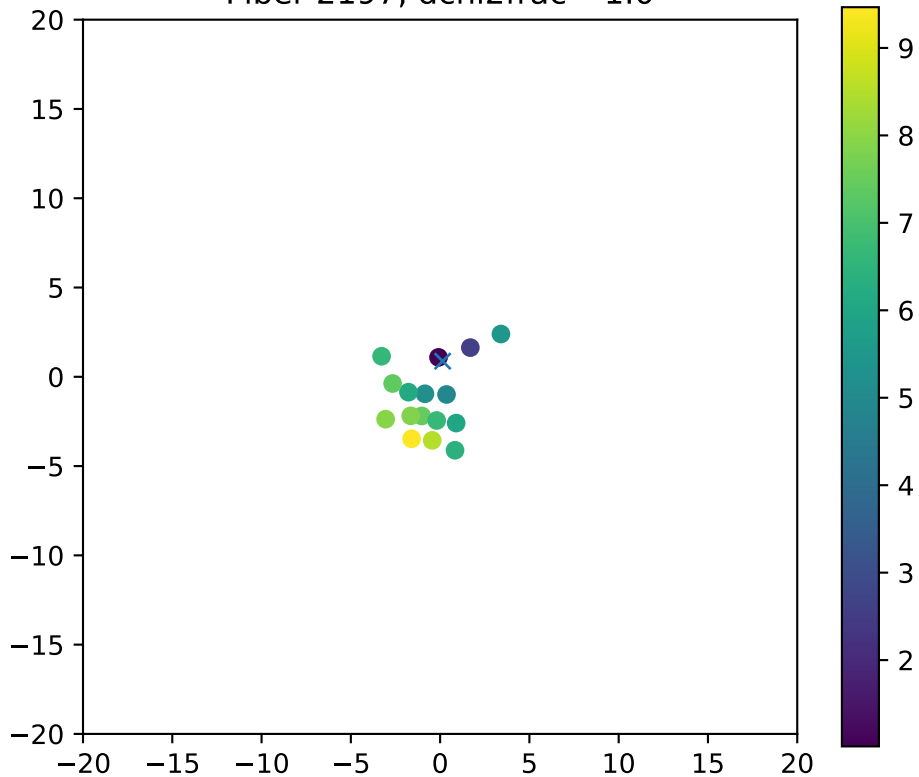
Fiber 2197, dchi2frac= 1.0
