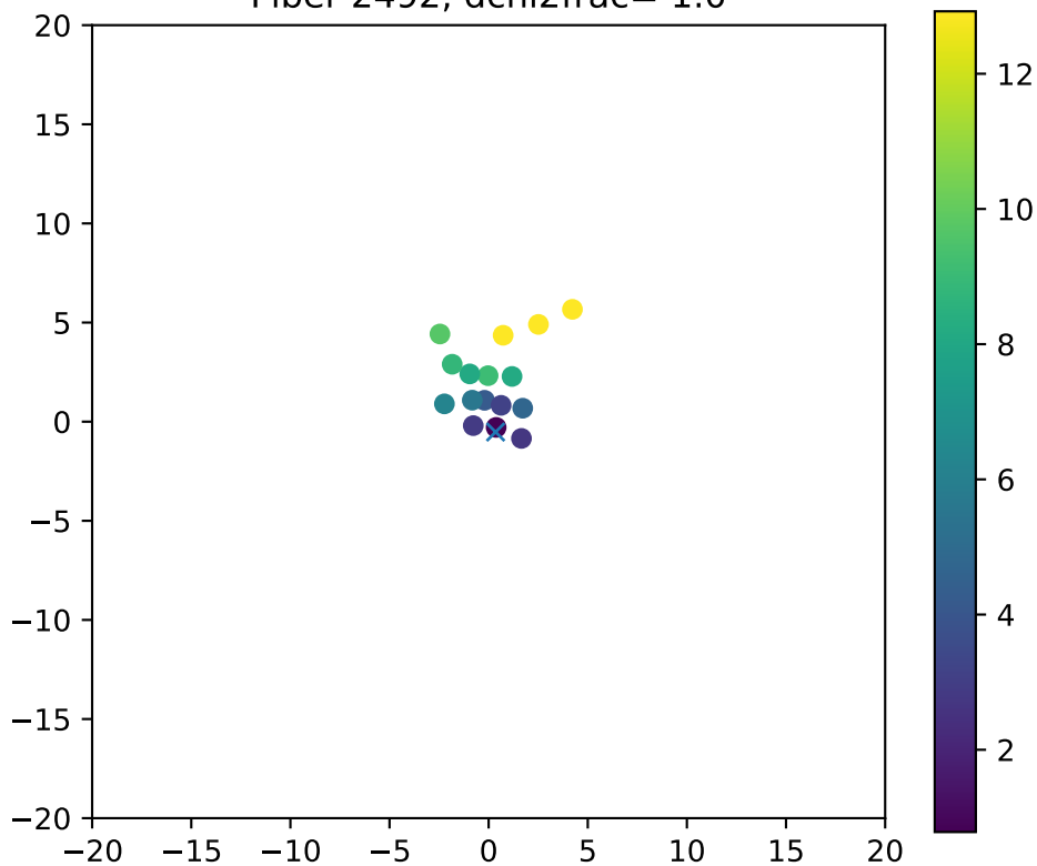
Fiber 2492, dchi2frac= 1.0
