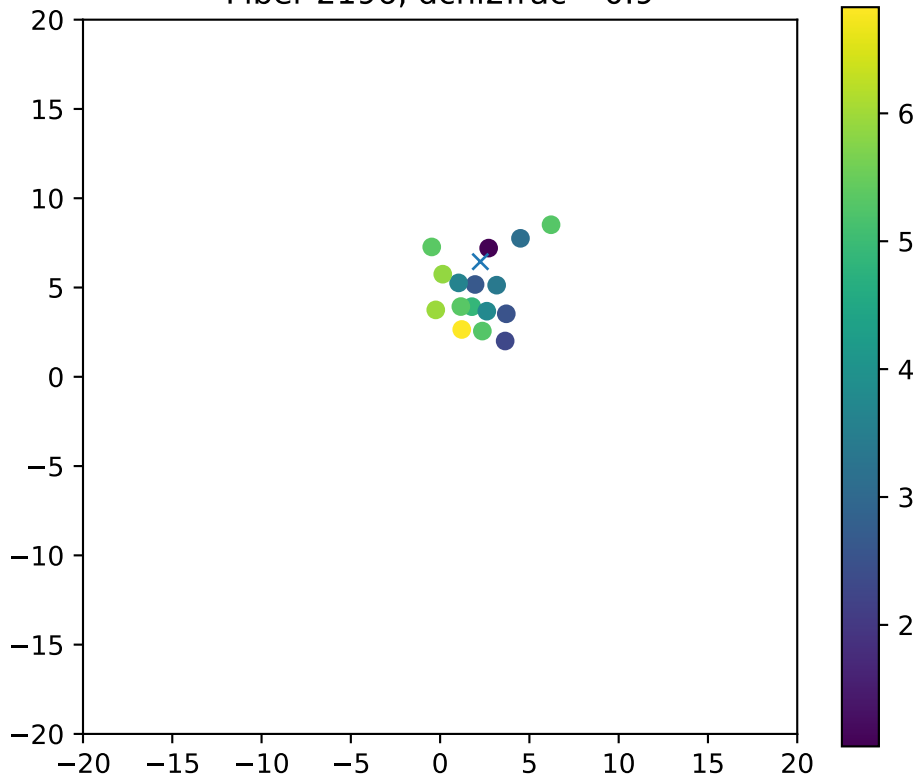
Fiber 2196, dchi2frac= 0.9
