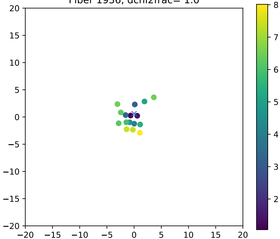
Fiber 1936, dchi2frac= 1.0
