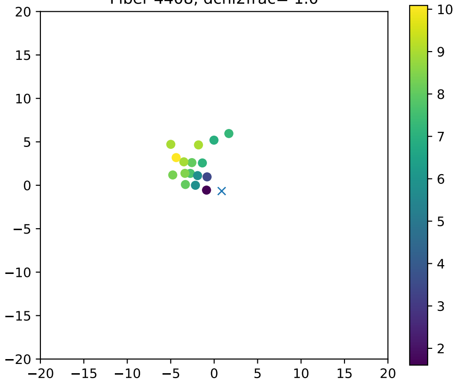
Fiber 4408, dchi2frac= 1.0
