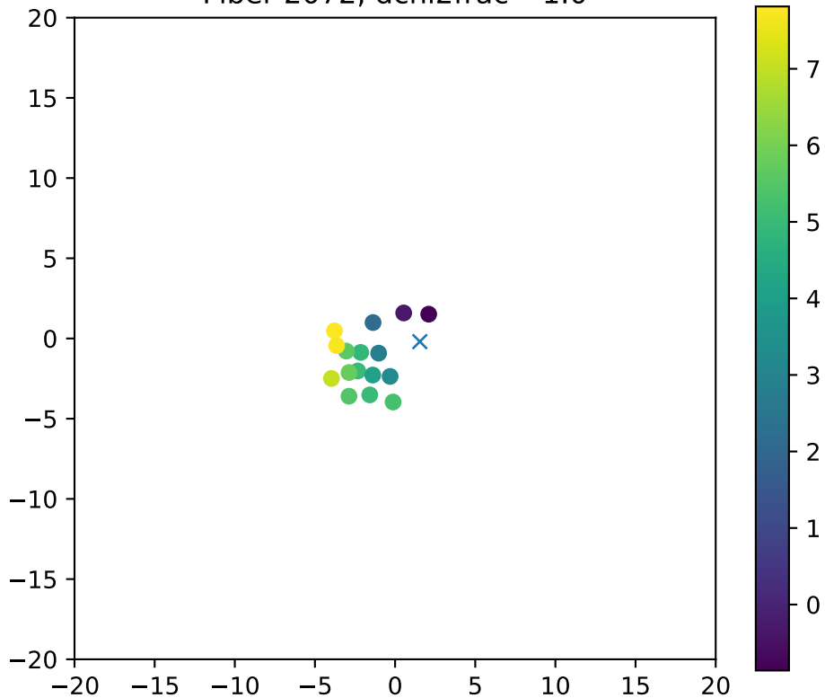
Fiber 2072, dchi2frac= 1.0
