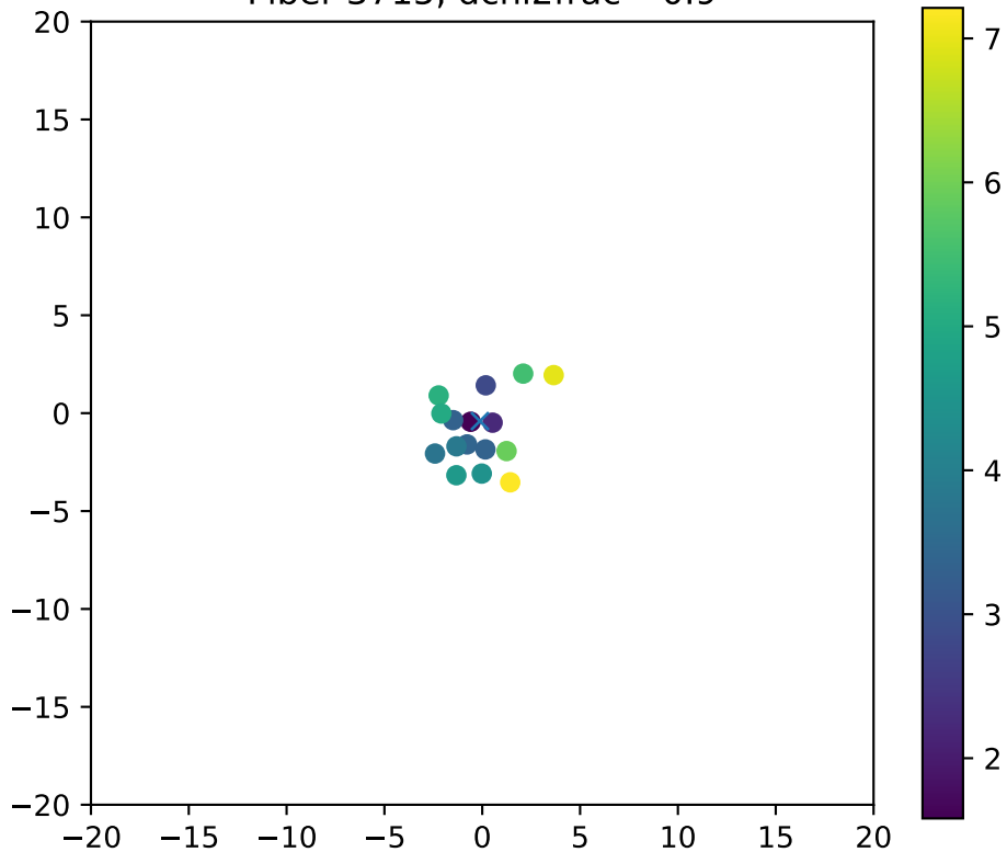
Fiber 3715, dchi2frac= 0.9
