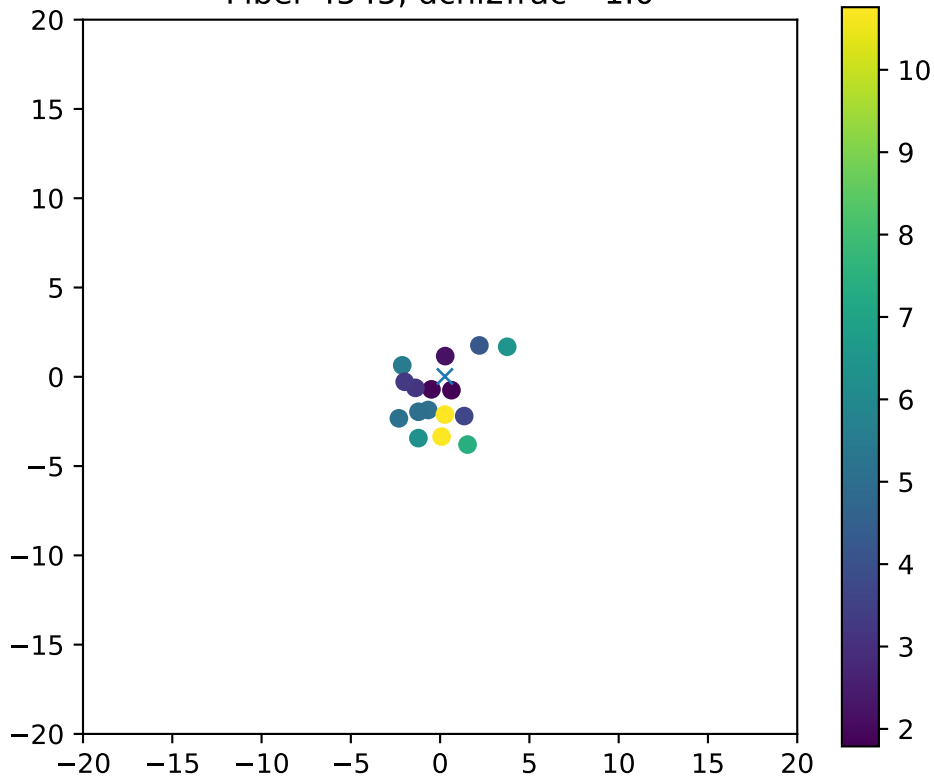
Fiber 4545, dchi2frac= 1.0
