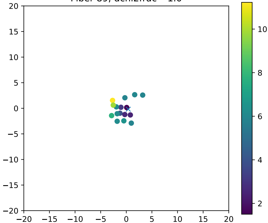
Fiber 89, dchi2frac= 1.0
