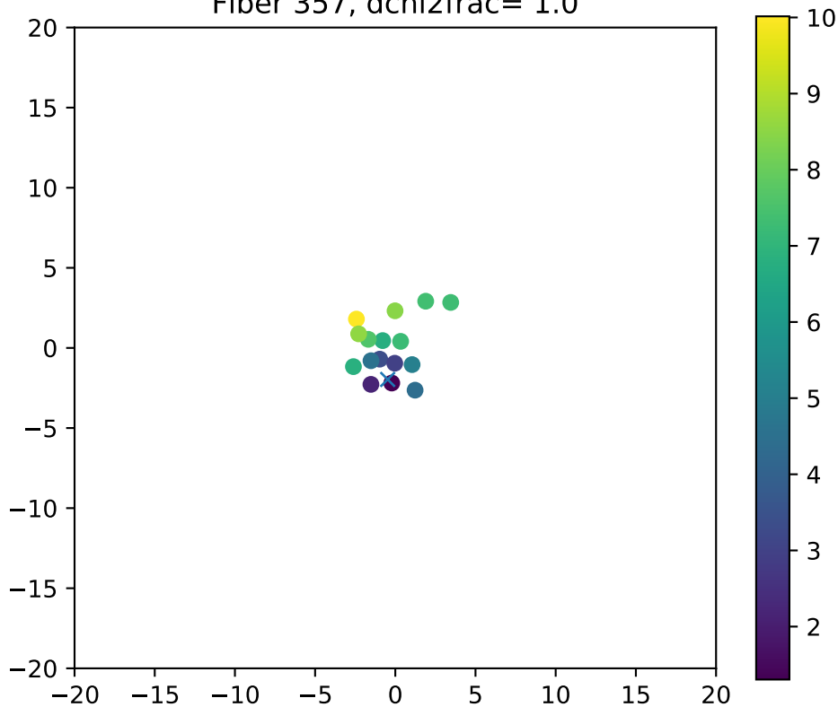
Fiber 357, dchi2frac= 1.0
