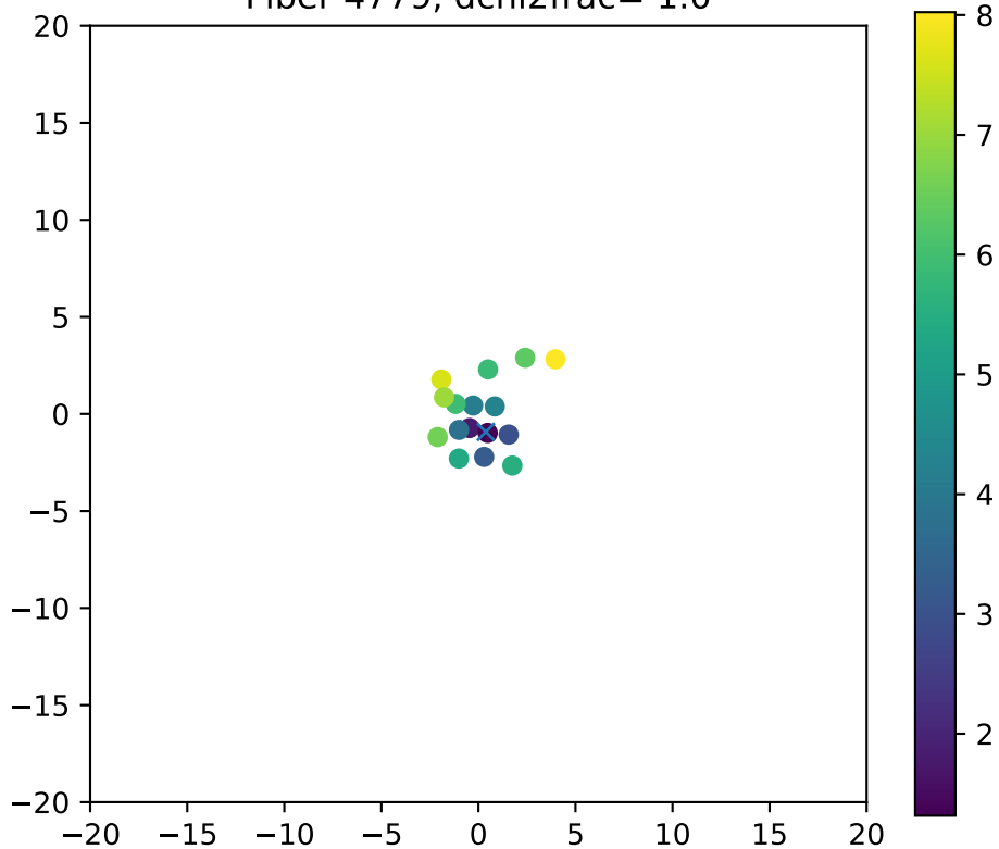
Fiber 4779, dchi2frac= 1.0
