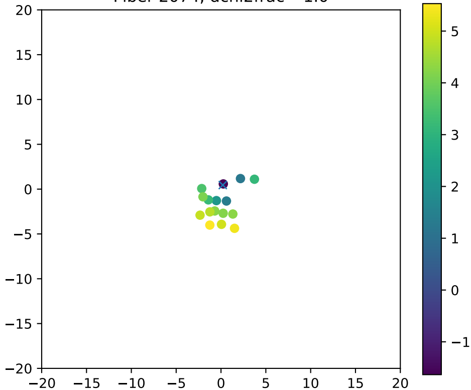
Fiber 2074, dchi2frac= 1.0
