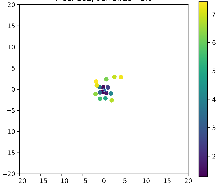
Fiber 382, dchi2frac= 1.0
