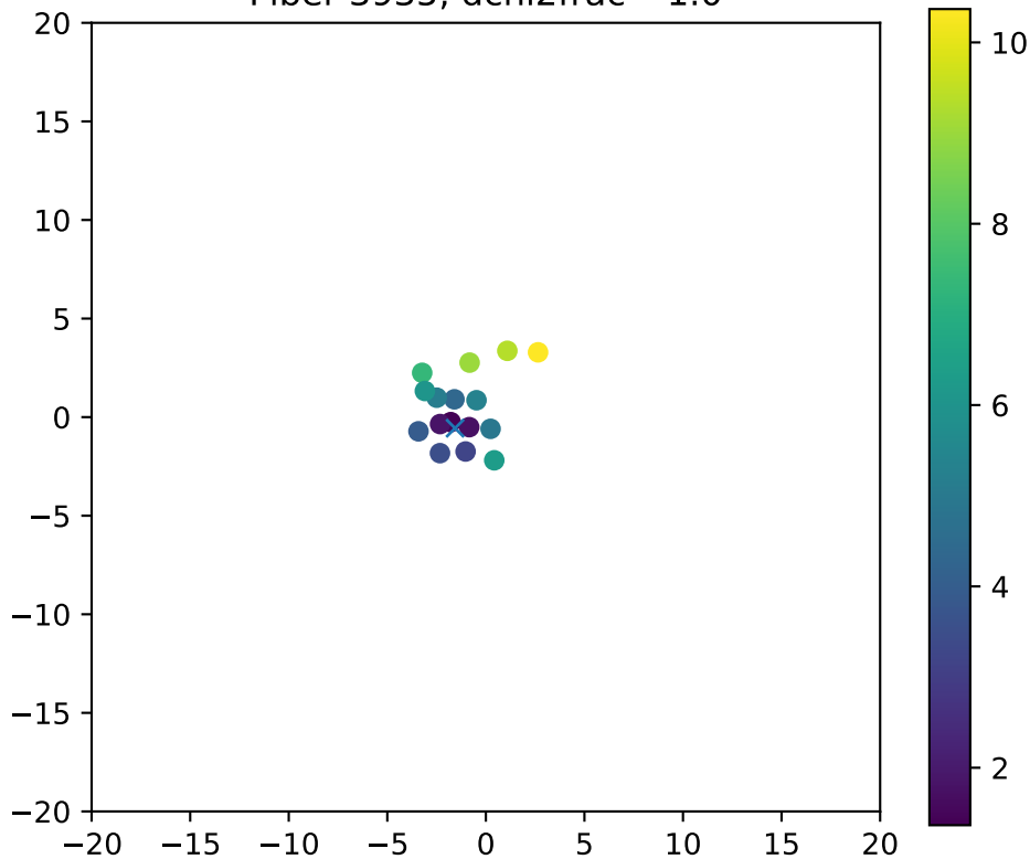
Fiber 3935, dchi2frac= 1.0
