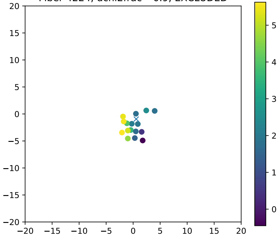
Fiber 4224, dchi2frac= 0.9, EXCLUDED
