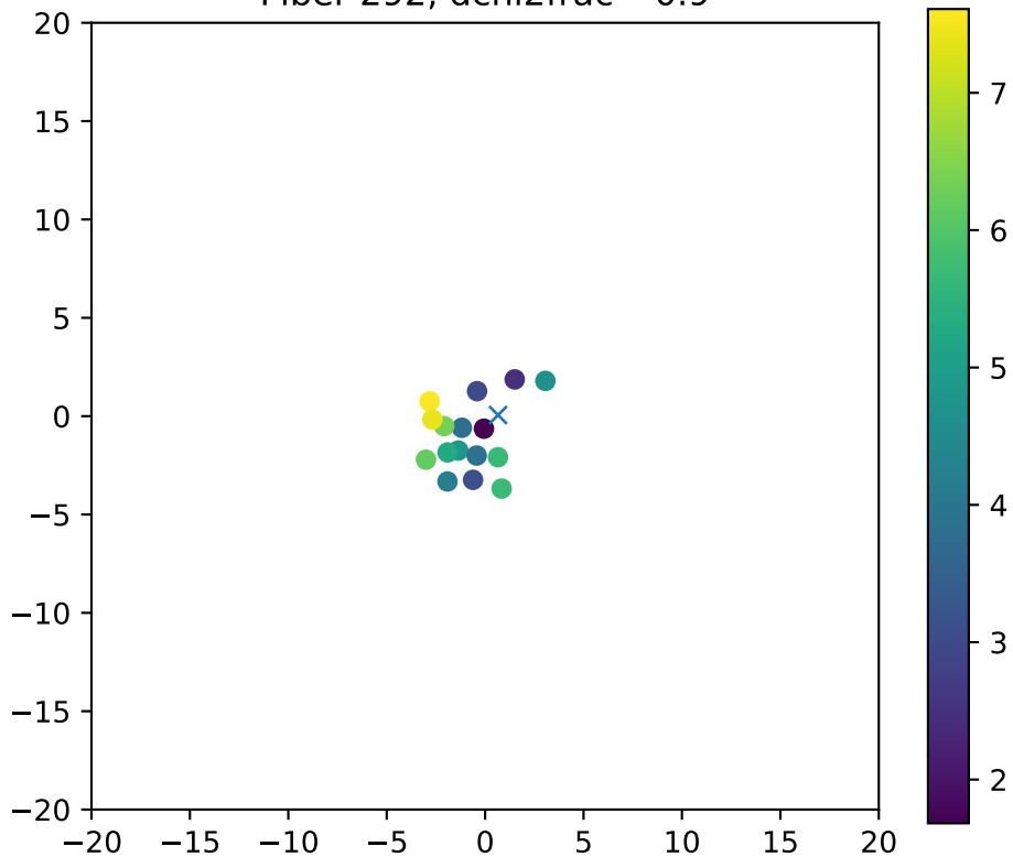
Fiber 292, dchi2frac= 0.9
