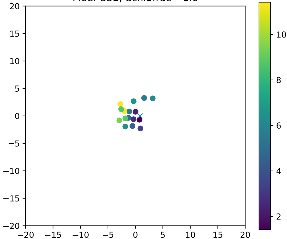
Fiber 352, dchi2frac= 1.0
