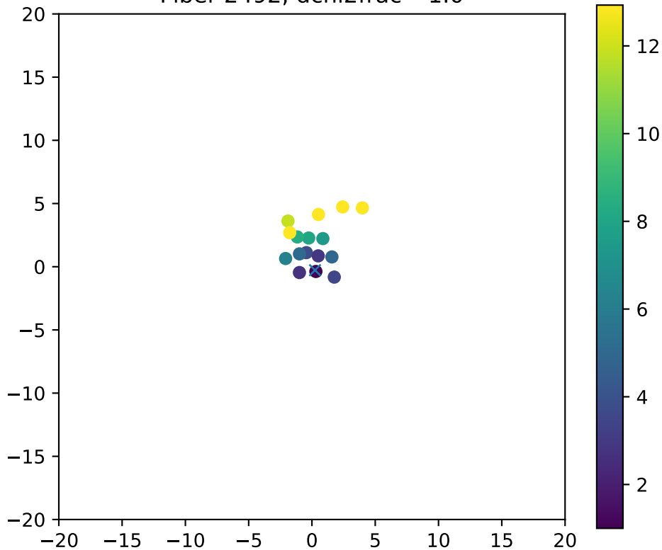
Fiber 2492, dchi2frac= 1.0
