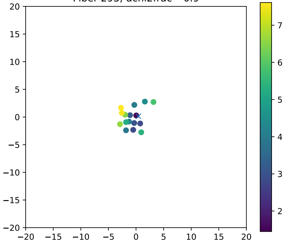
Fiber 293, dchi2frac= 0.9
