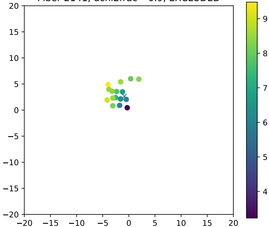
Fiber 2141, dchi2frac= 0.9, EXCLUDED
