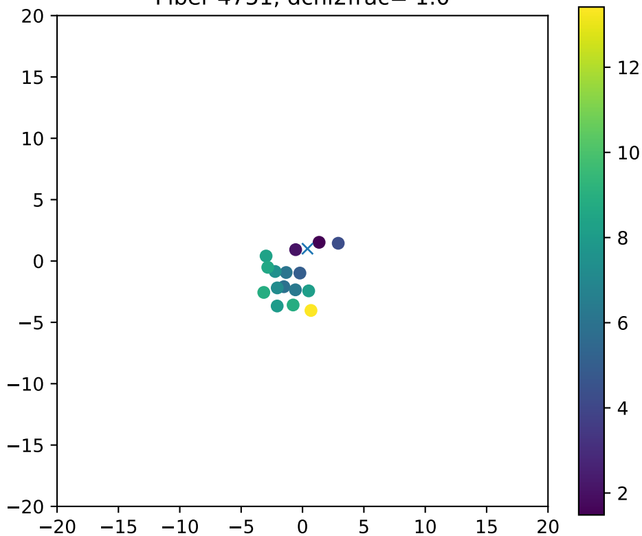
Fiber 4751, dchi2frac= 1.0
