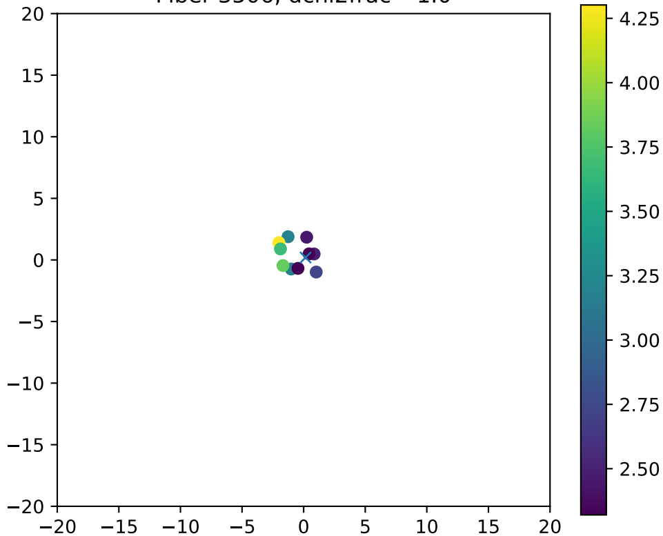
Fiber 3506, dchi2frac= 1.0
