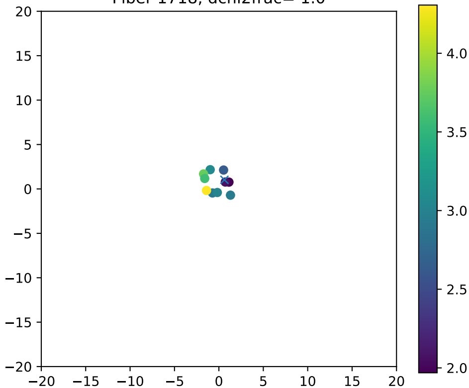
Fiber 1718, dchi2frac= 1.0
