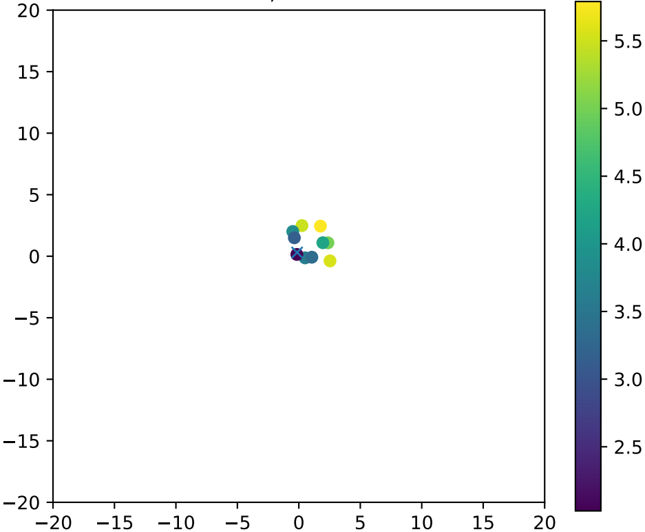
Fiber 1496, dchi2frac= 1.0
