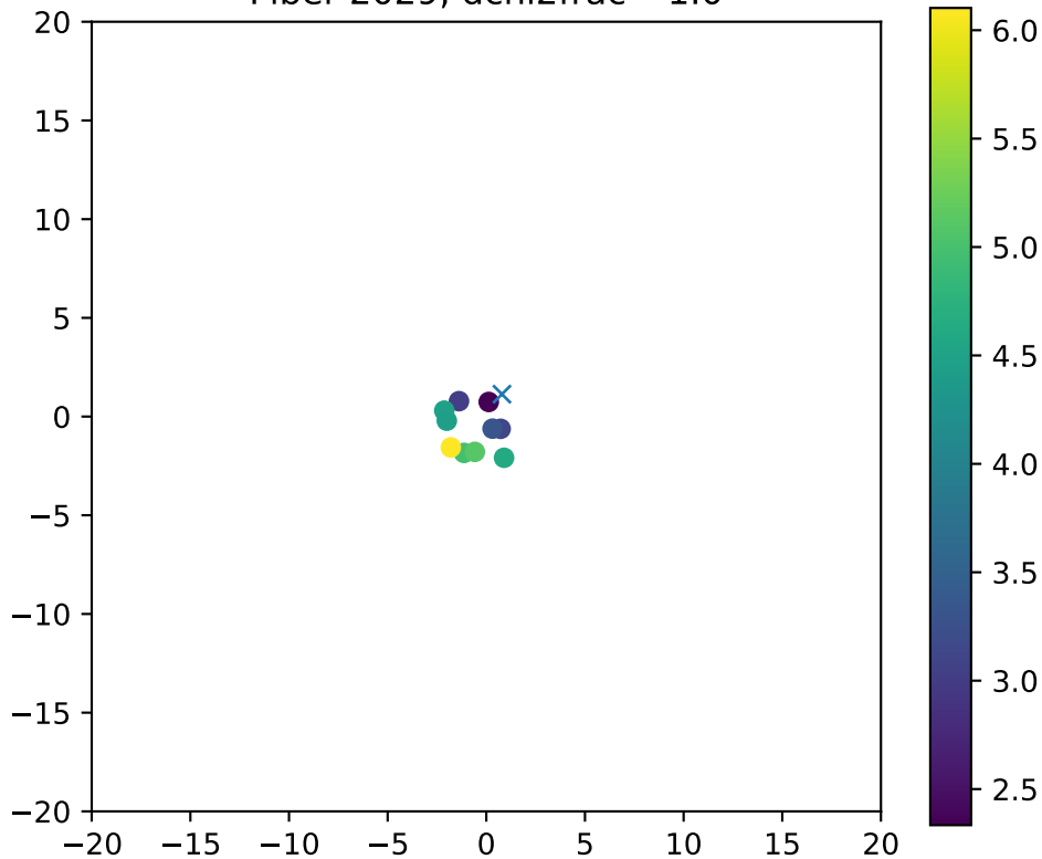
Fiber 2029, dchi2frac= 1.0
