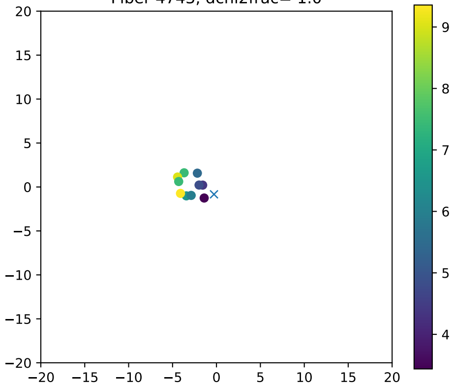
Fiber 4743, dchi2frac= 1.0
