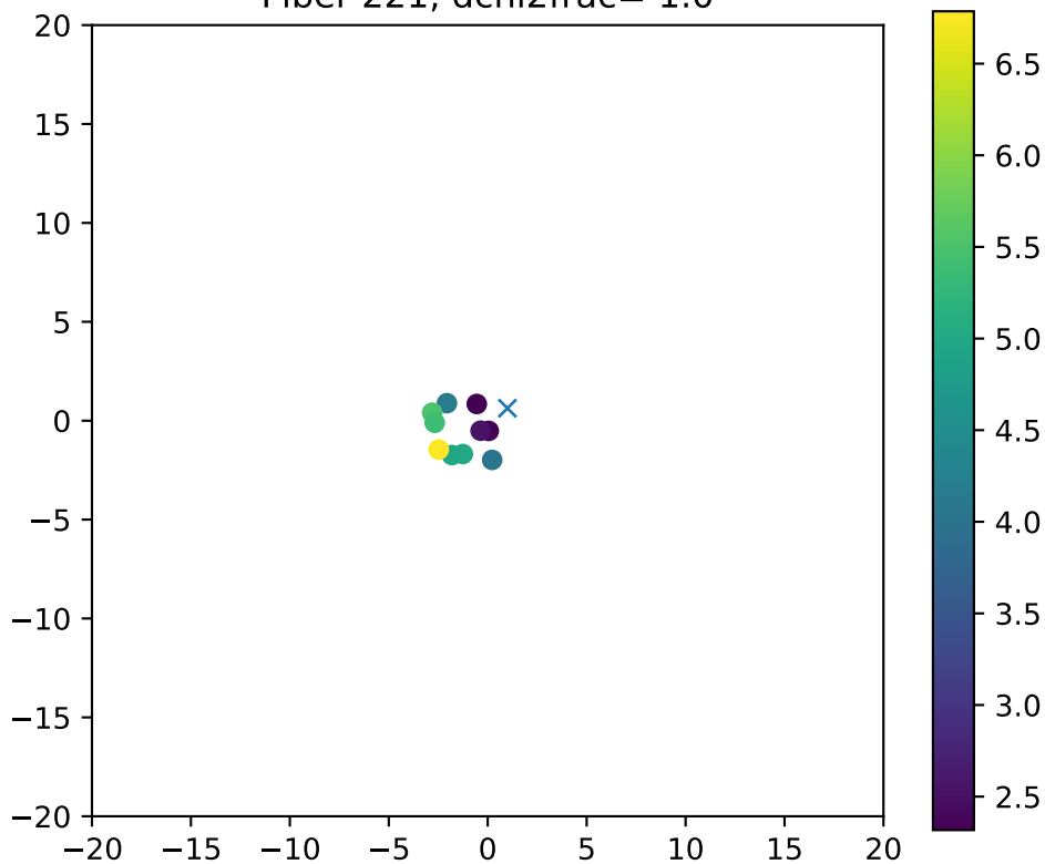
Fiber 221, dchi2frac= 1.0
