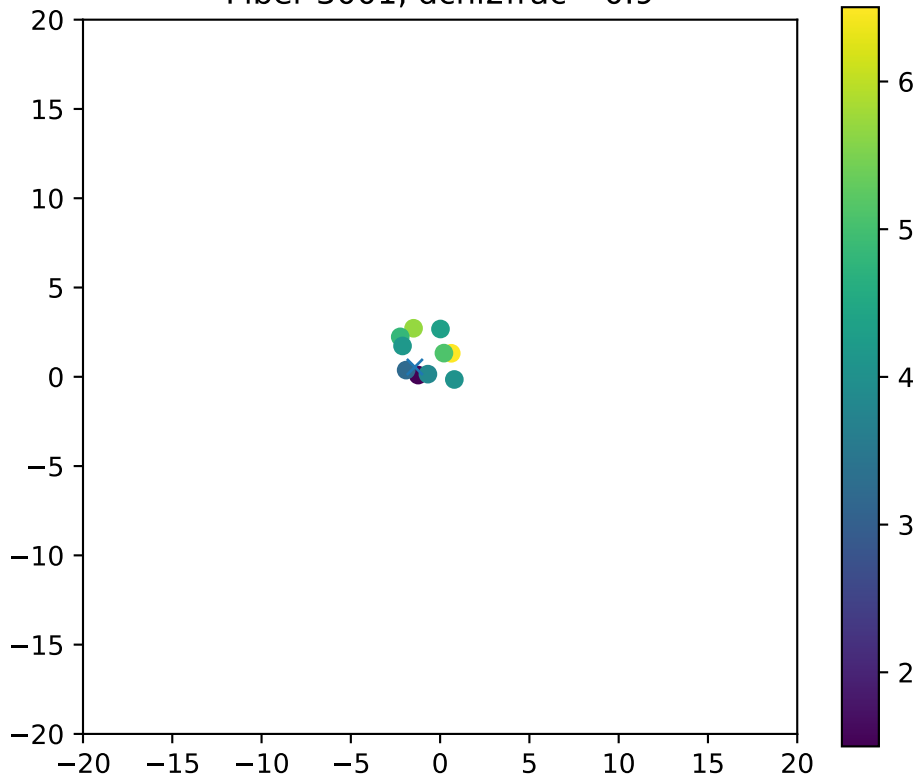
Fiber 3001, dchi2frac= 0.9
