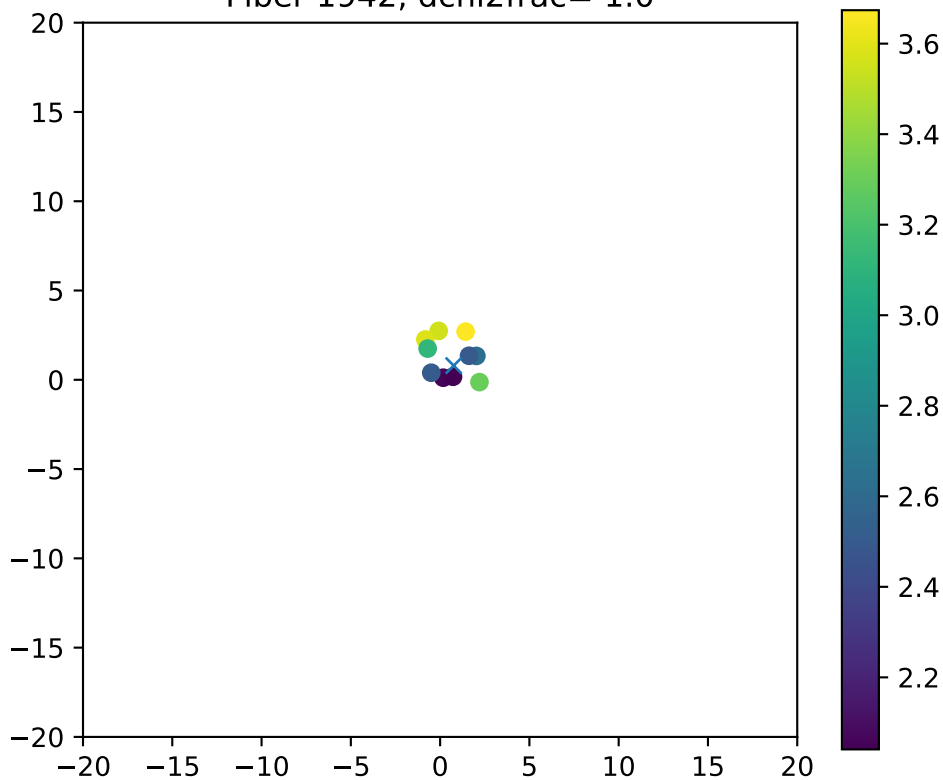
Fiber 1942, dchi2frac= 1.0
