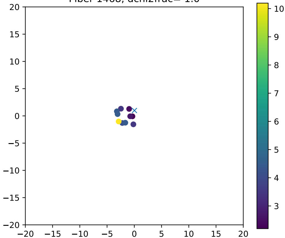
Fiber 1468, dchi2frac= 1.0
