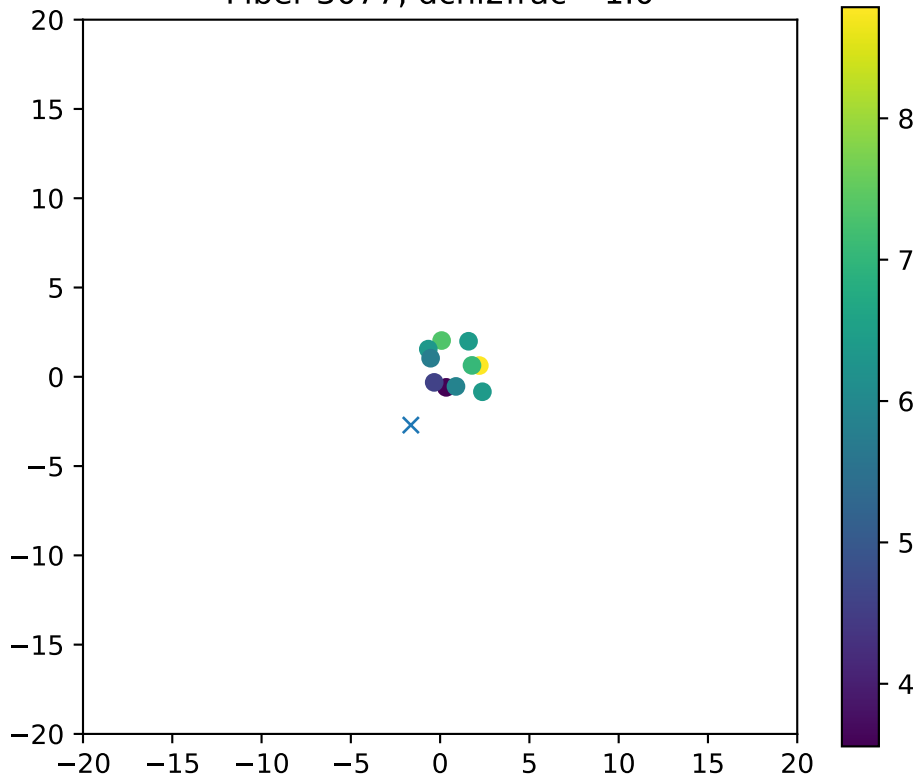
Fiber 3077, dchi2frac= 1.0
