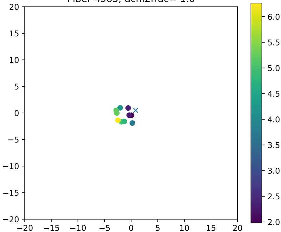
Fiber 4965, dchi2frac= 1.0
