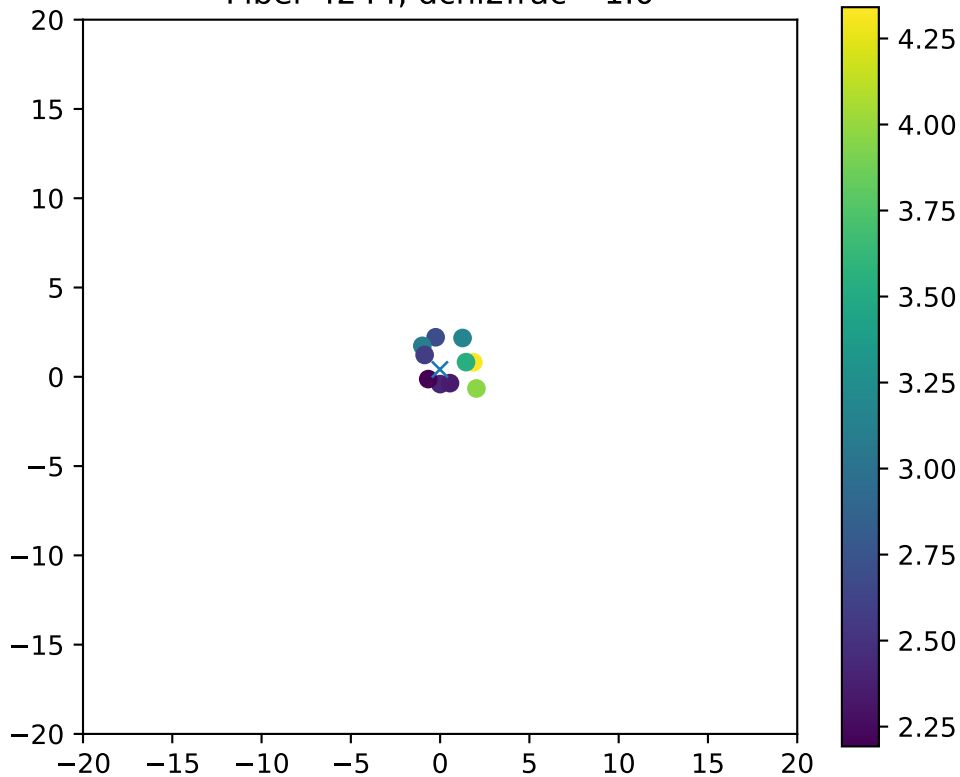
Fiber 4244, dchi2frac= 1.0
