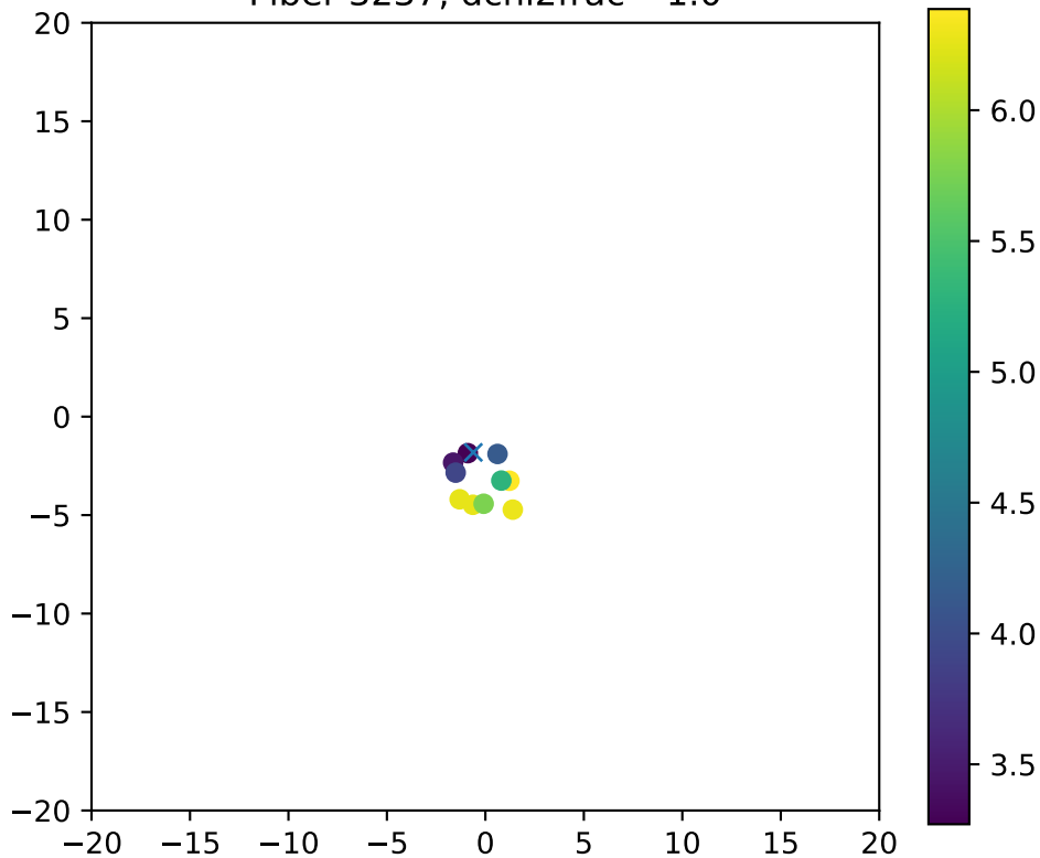
Fiber 3237, dchi2frac= 1.0
