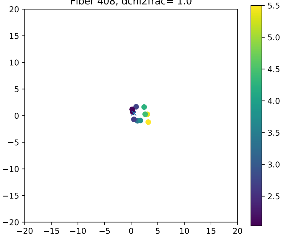
Fiber 408, dchi2frac= 1.0
