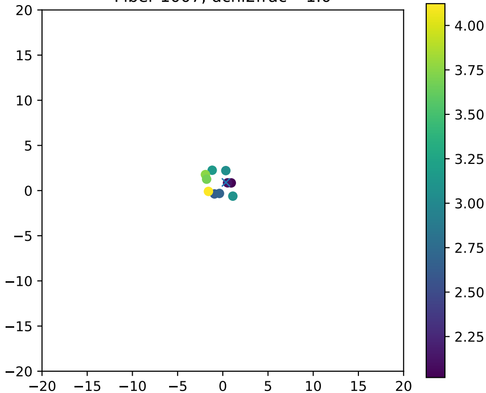
Fiber 1007, dchi2frac= 1.0
