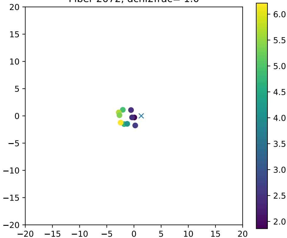
Fiber 2072, dchi2frac= 1.0
