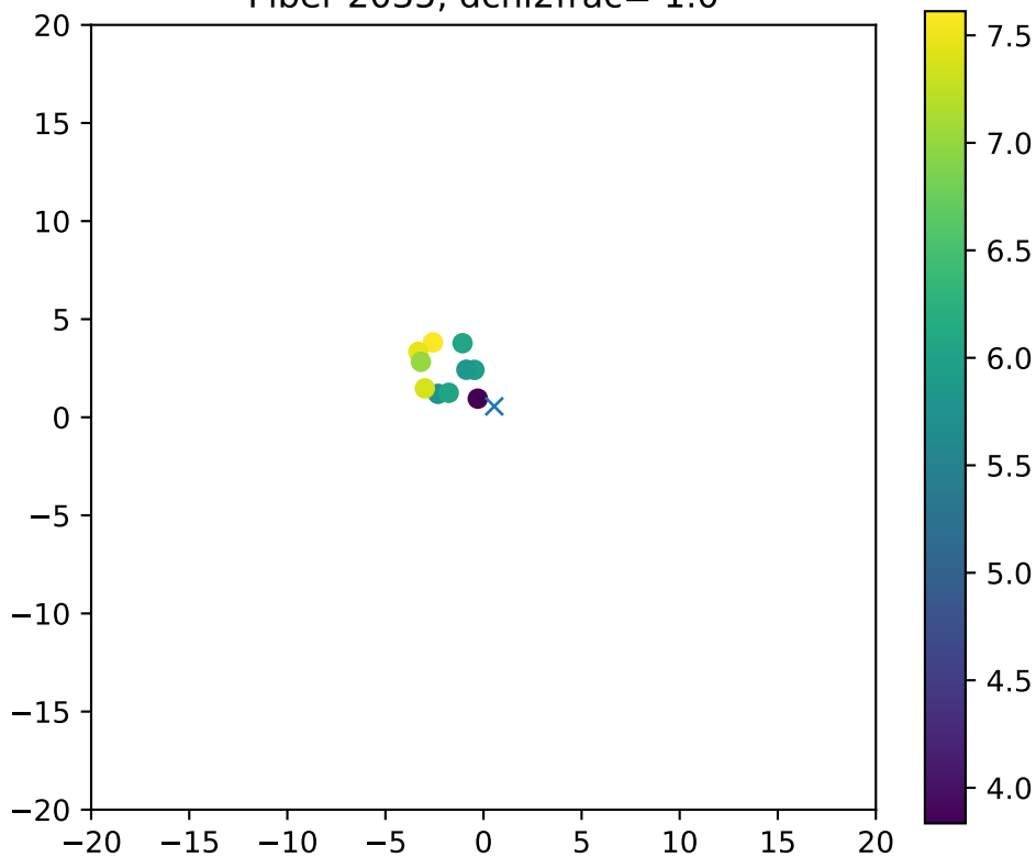
Fiber 2035, dchi2frac= 1.0
