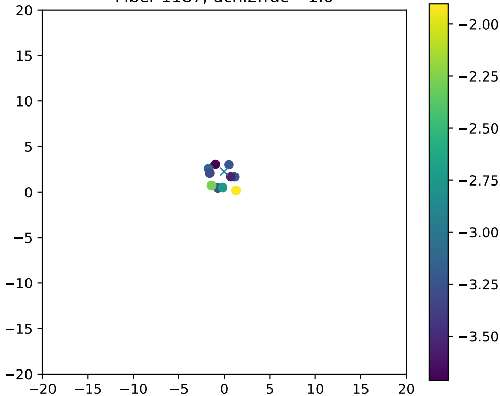
Fiber 1187, dchi2frac= 1.0
