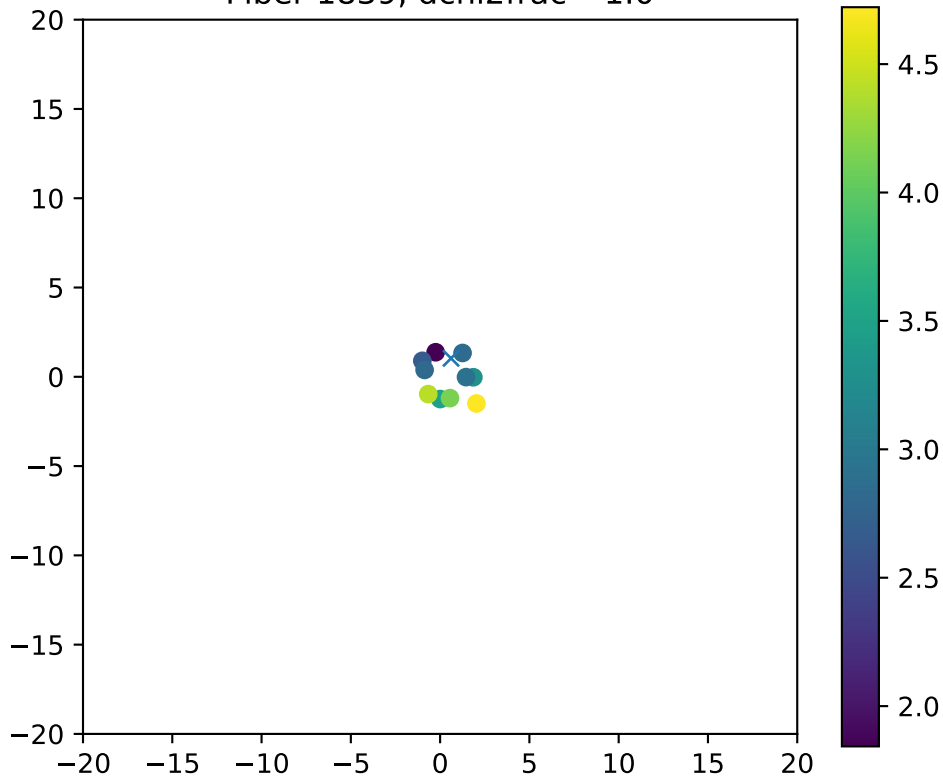
Fiber 1839, dchi2frac= 1.0
