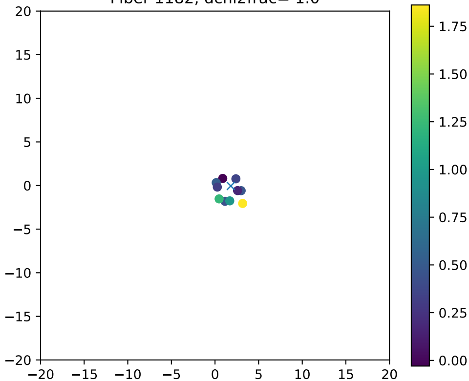
Fiber 1182, dchi2frac= 1.0
