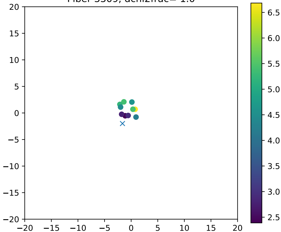
Fiber 3309, dchi2frac= 1.0
