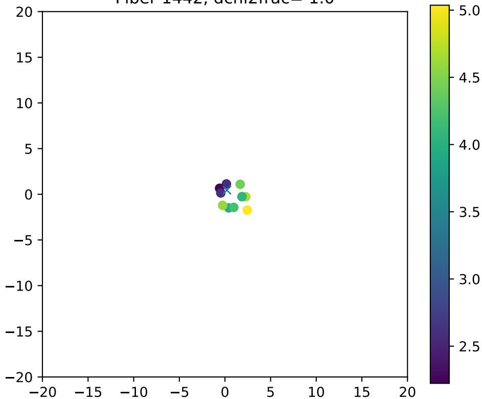
Fiber 1442, dchi2frac= 1.0
