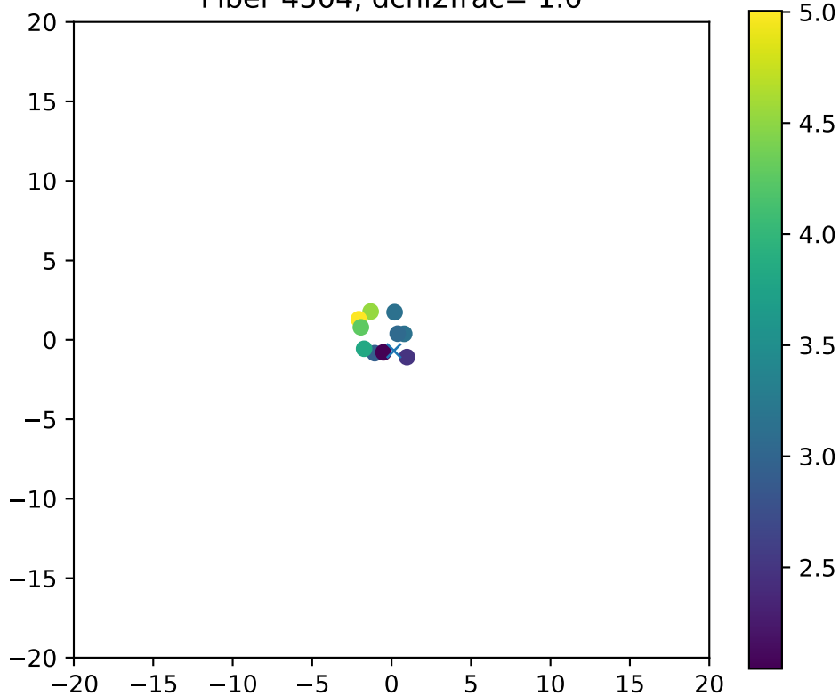
Fiber 4504, dchi2frac= 1.0
