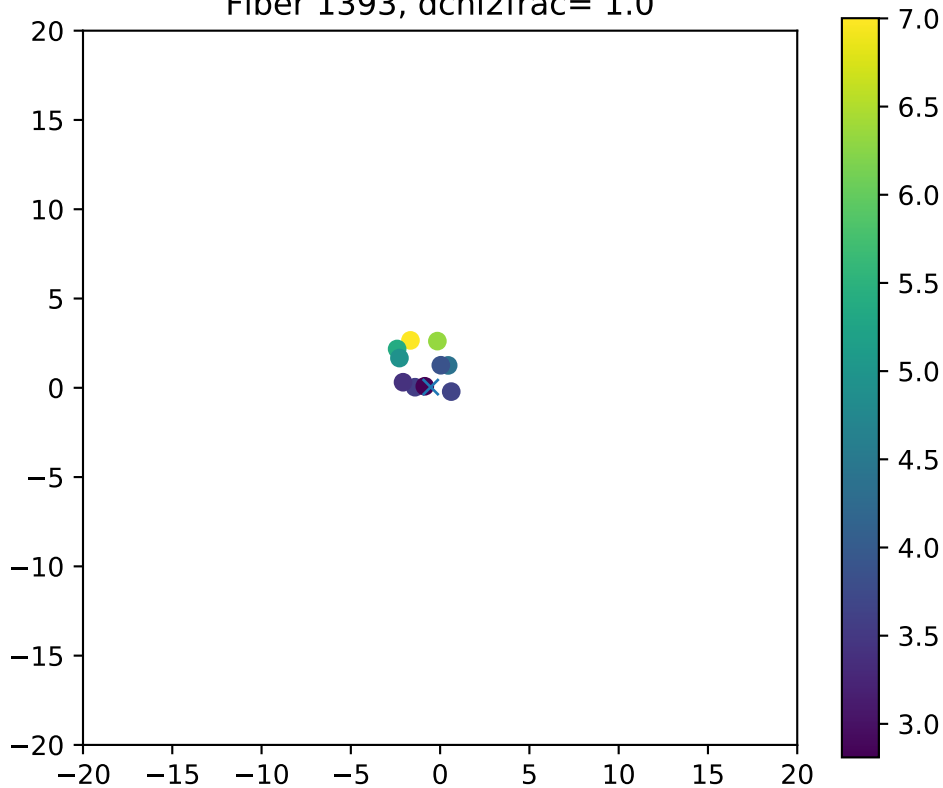
Fiber 1393, dchi2frac= 1.0
