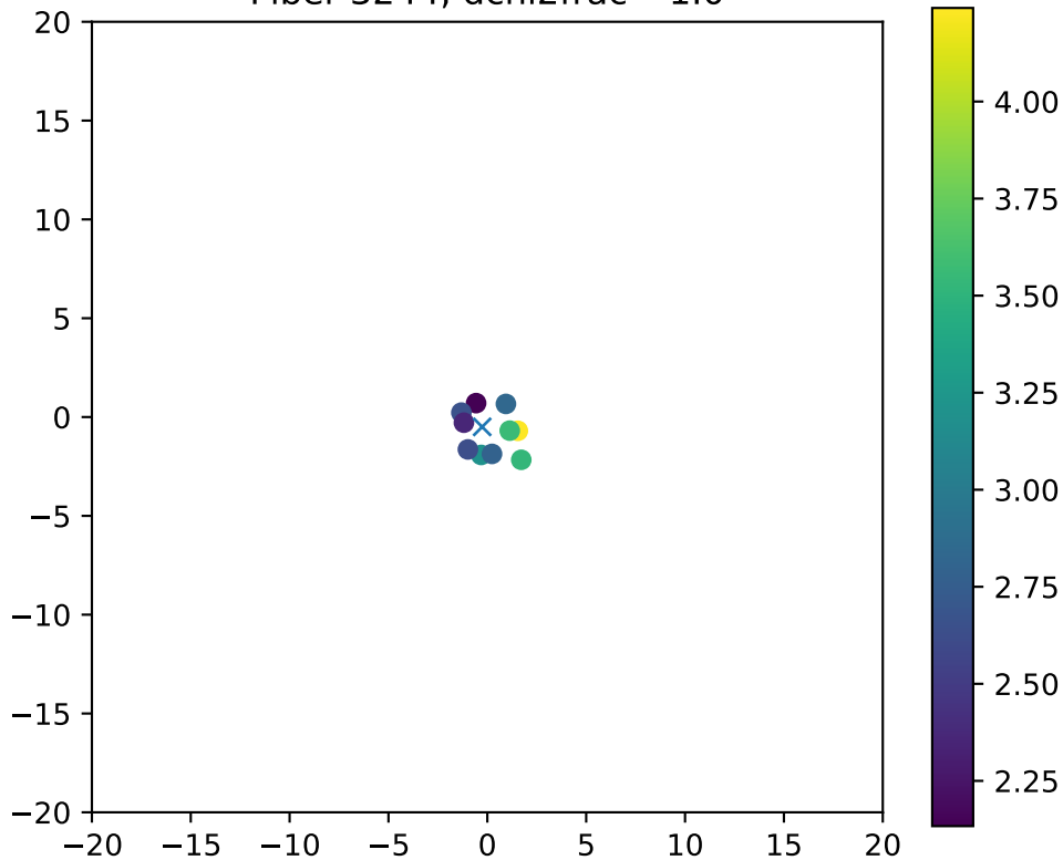
Fiber 3244, dchi2frac= 1.0
