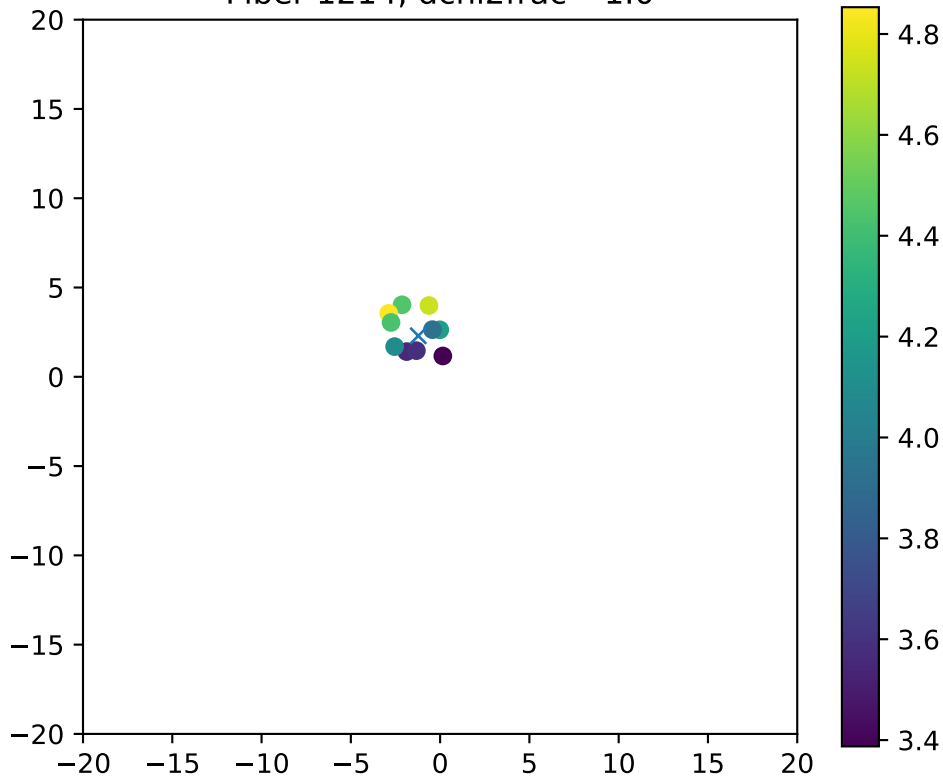
Fiber 1214, dchi2frac= 1.0
