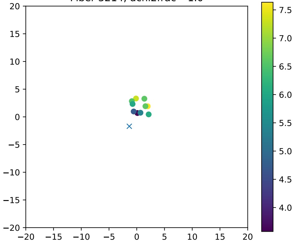
Fiber 3214, dchi2frac= 1.0
