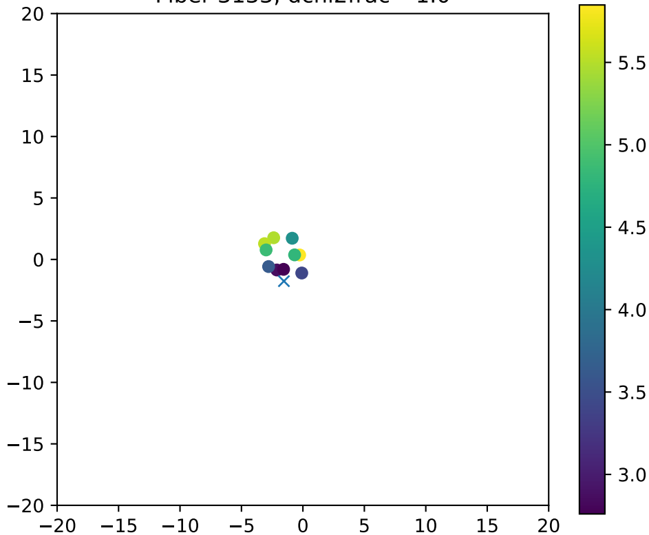
Fiber 3133, dchi2frac= 1.0
