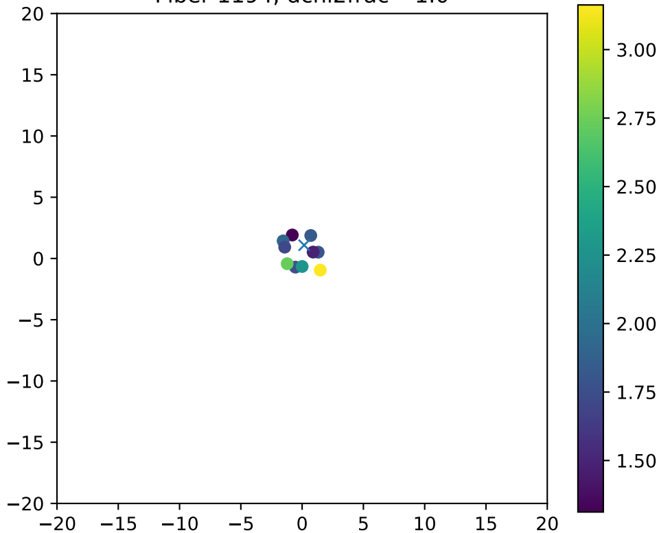
Fiber 1194, dchi2frac= 1.0
