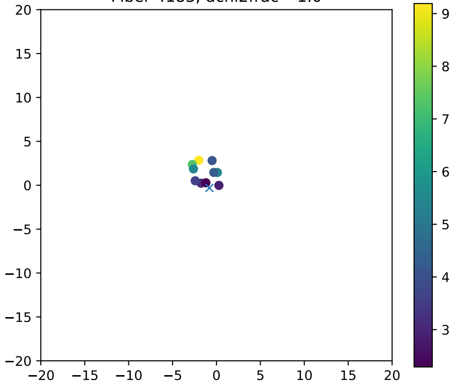
Fiber 4183, dchi2frac= 1.0
