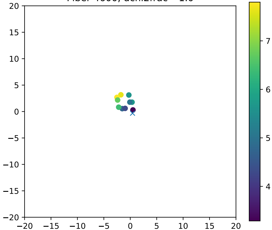
Fiber 4600, dchi2frac= 1.0
