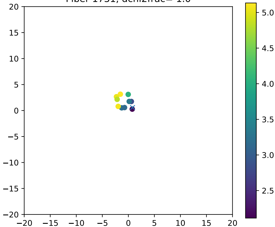
Fiber 1731, dchi2frac= 1.0
