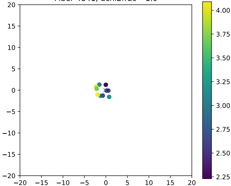
Fiber 4841, dchi2frac= 1.0
