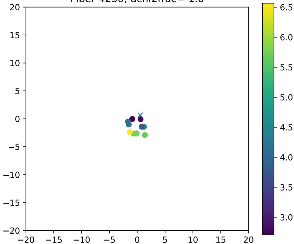
Fiber 4230, dchi2frac= 1.0
