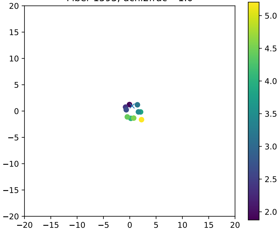
Fiber 1593, dchi2frac= 1.0
