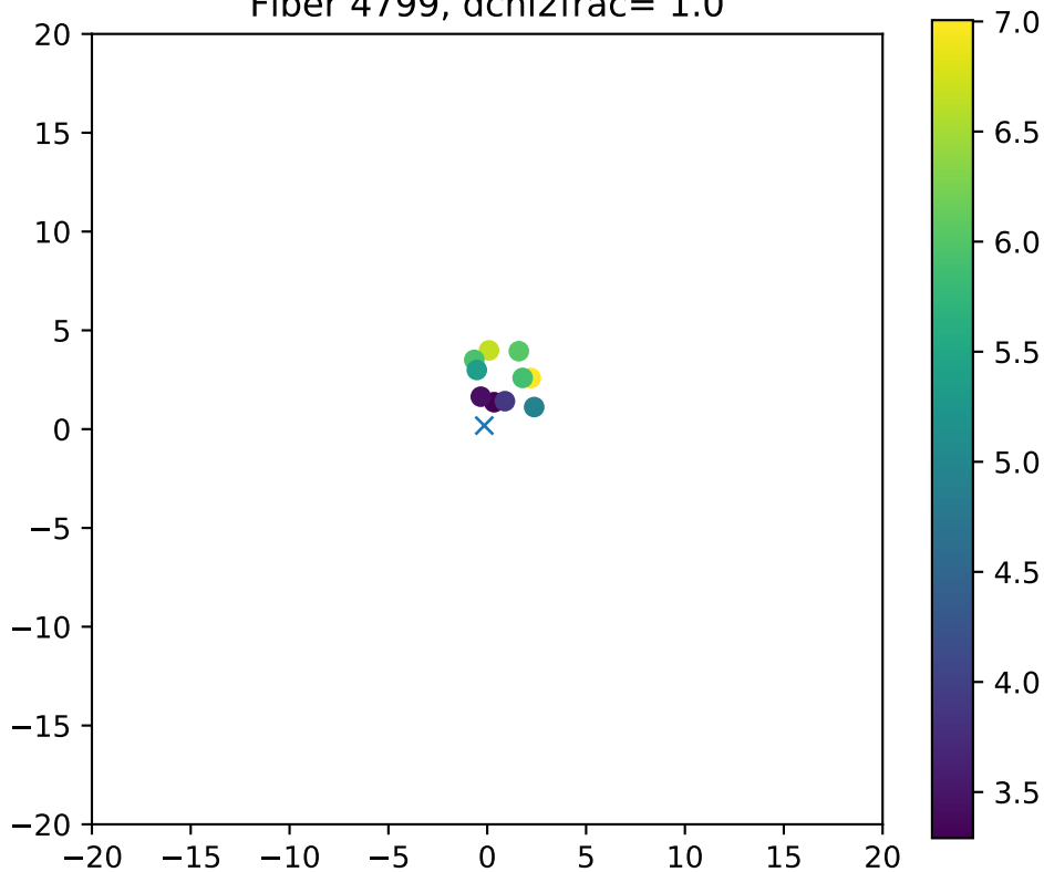
Fiber 4799, dchi2frac= 1.0
