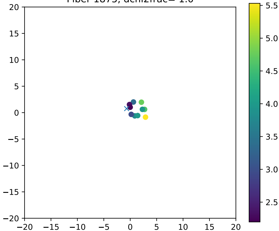
Fiber 1875, dchi2frac= 1.0
