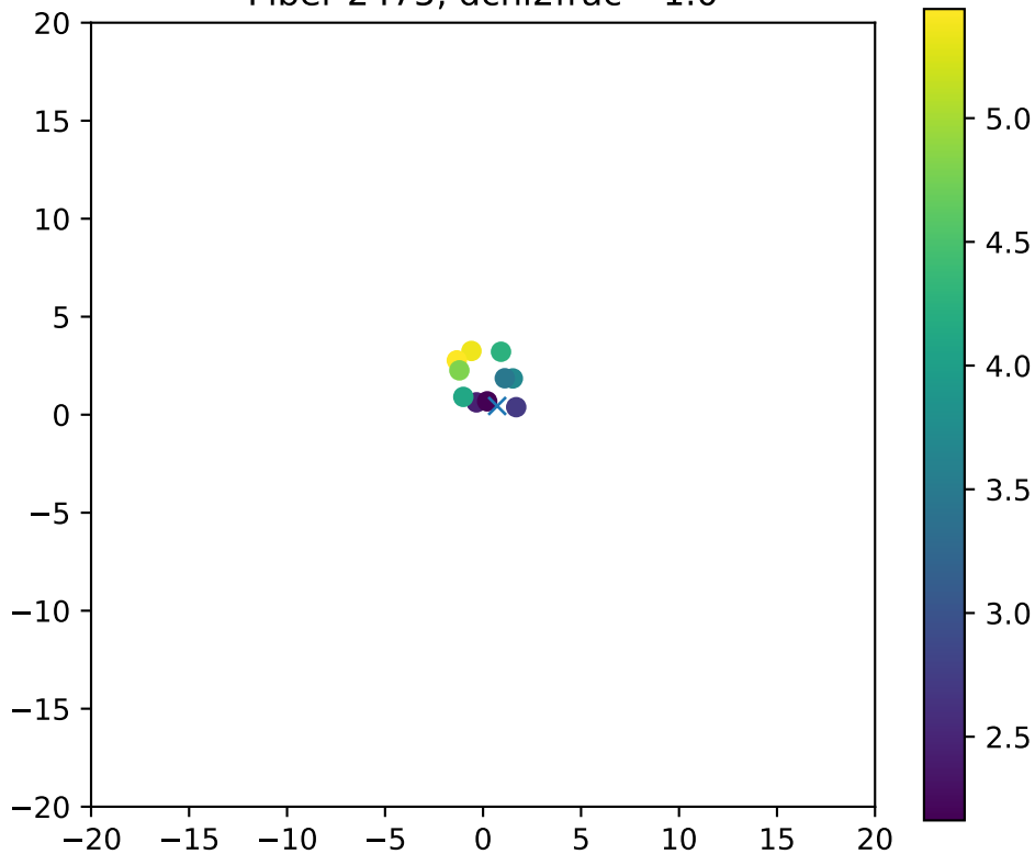
Fiber 2475, dchi2frac= 1.0
