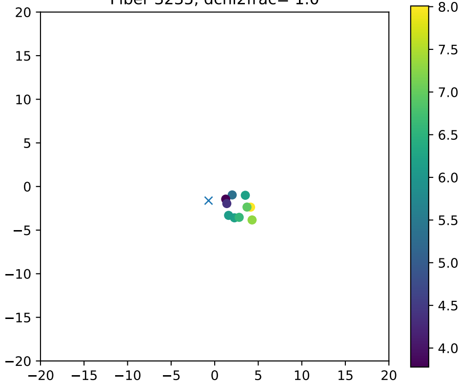
Fiber 3235, dchi2frac= 1.0
