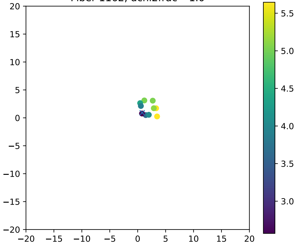
Fiber 1162, dchi2frac= 1.0
