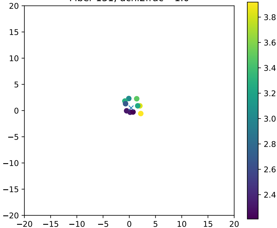
Fiber 131, dchi2frac= 1.0
