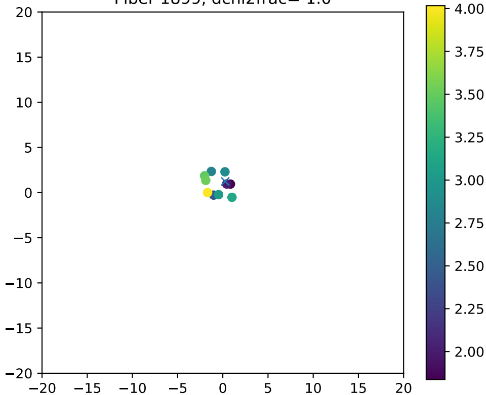
Fiber 1899, dchi2frac= 1.0
