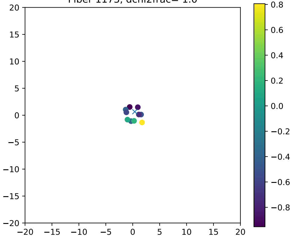
Fiber 1173, dchi2frac= 1.0
