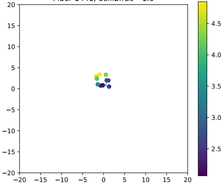
Fiber 1441, dchi2frac= 1.0
