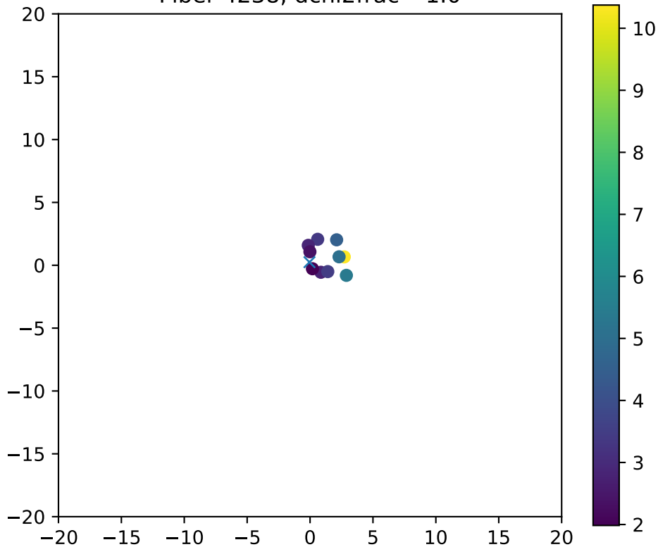
Fiber 4238, dchi2frac= 1.0
