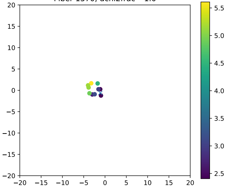
Fiber 1370, dchi2frac= 1.0
