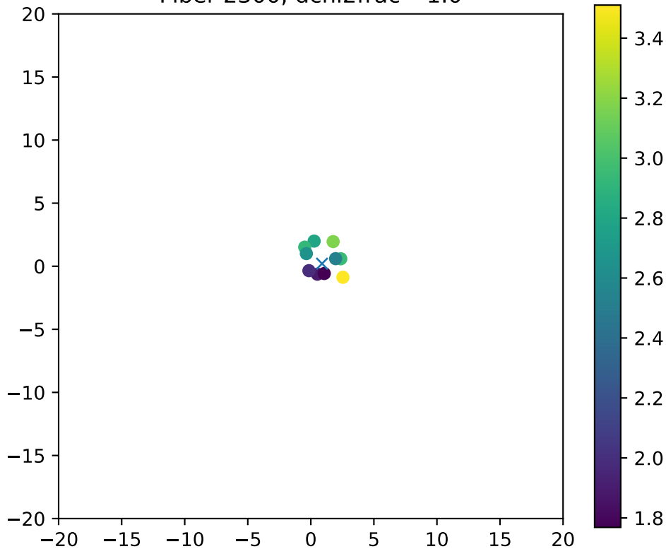
Fiber 2300, dchi2frac= 1.0
