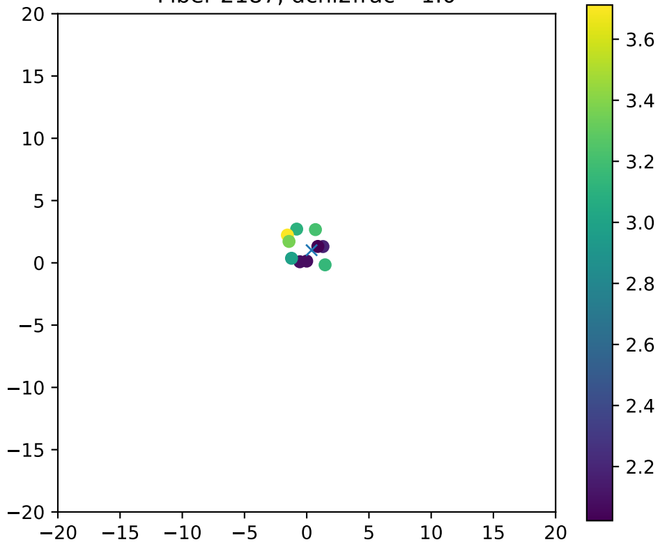
Fiber 2187, dchi2frac= 1.0
