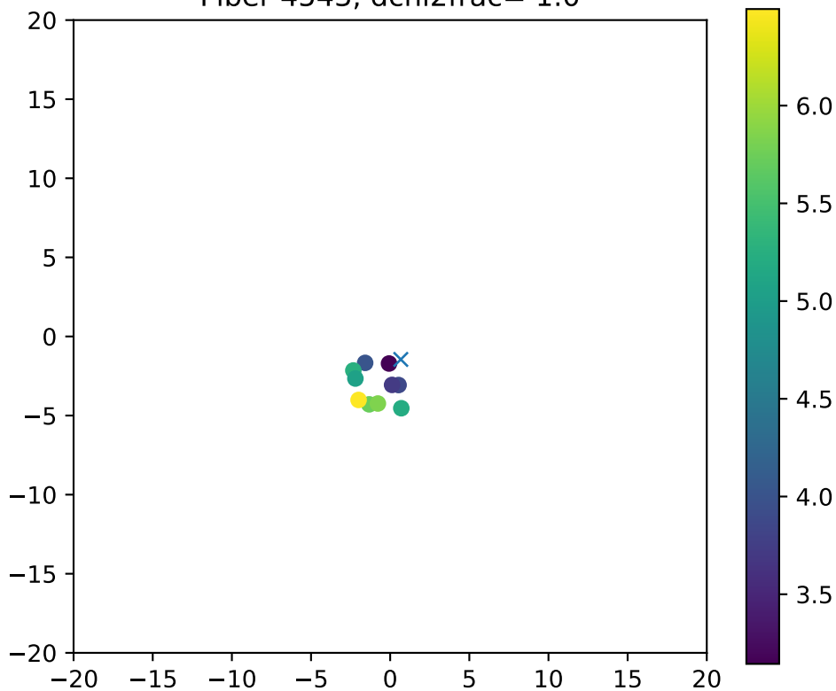
Fiber 4543, dchi2frac= 1.0
