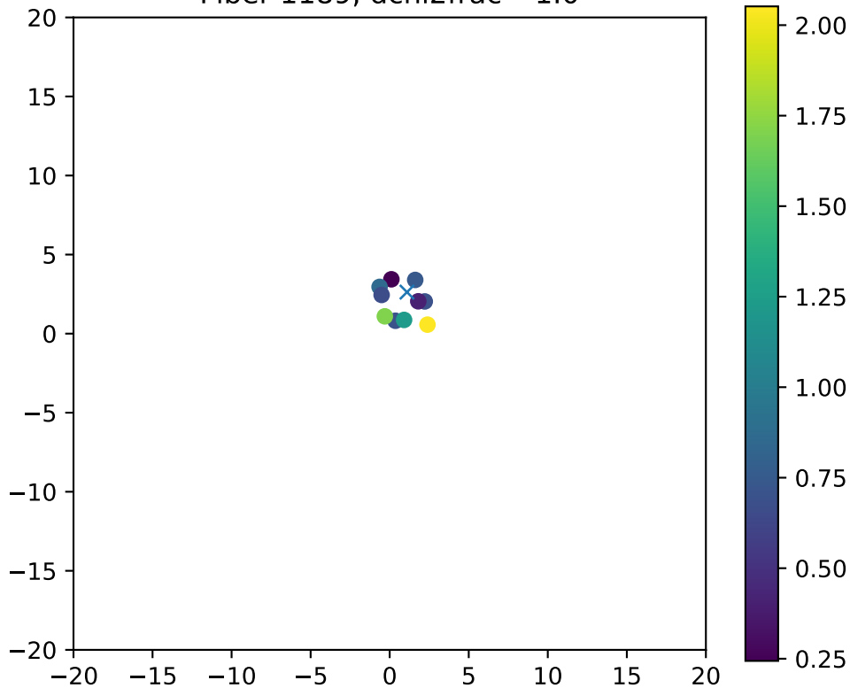
Fiber 1189, dchi2frac= 1.0
