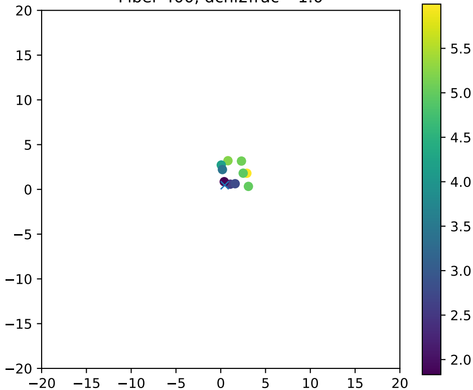
Fiber 400, dchi2frac= 1.0
