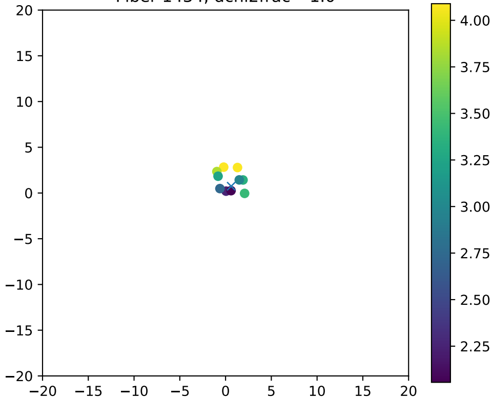
Fiber 1434, dchi2frac= 1.0
