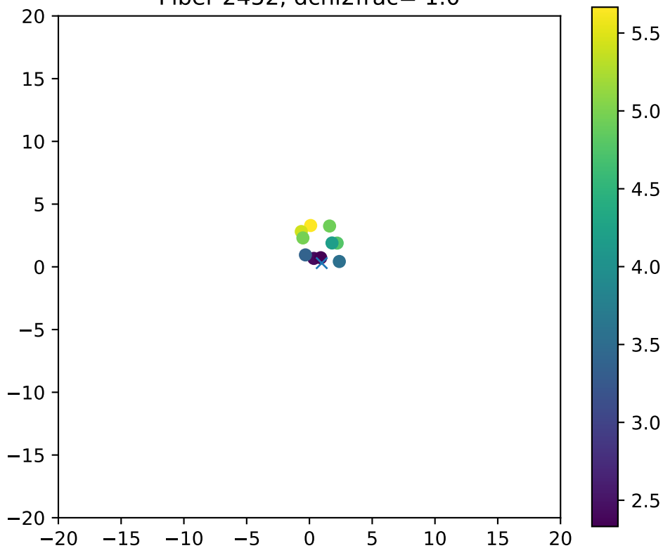
Fiber 2452, dchi2frac= 1.0
