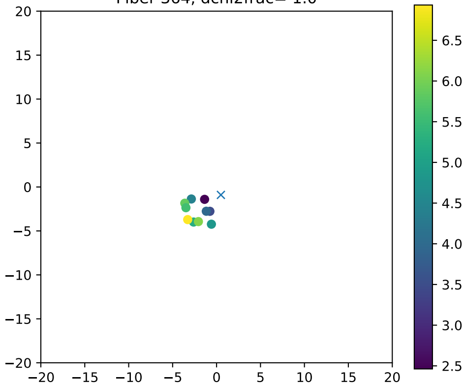
Fiber 364, dchi2frac= 1.0
