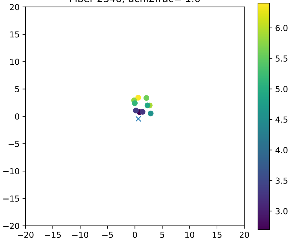
Fiber 2346, dchi2frac= 1.0
