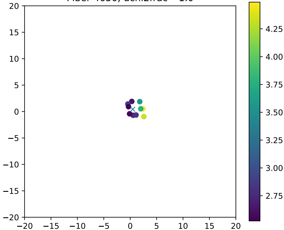
Fiber 4650, dchi2frac= 1.0
