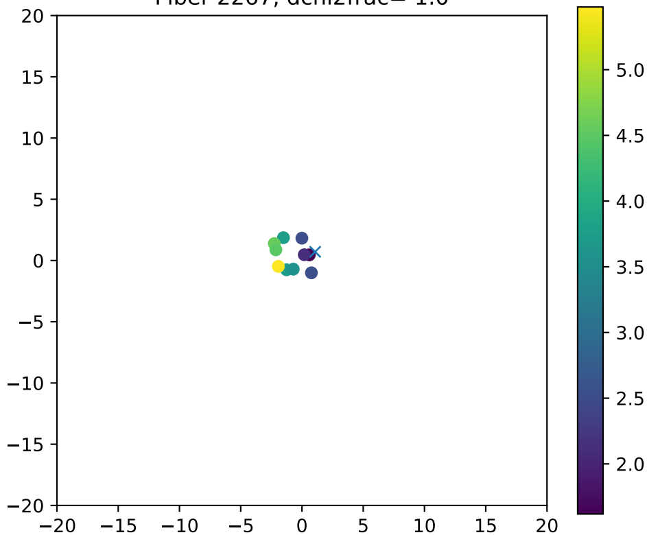
Fiber 2267, dchi2frac= 1.0
