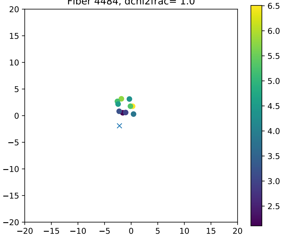
Fiber 4484, dchi2frac= 1.0
