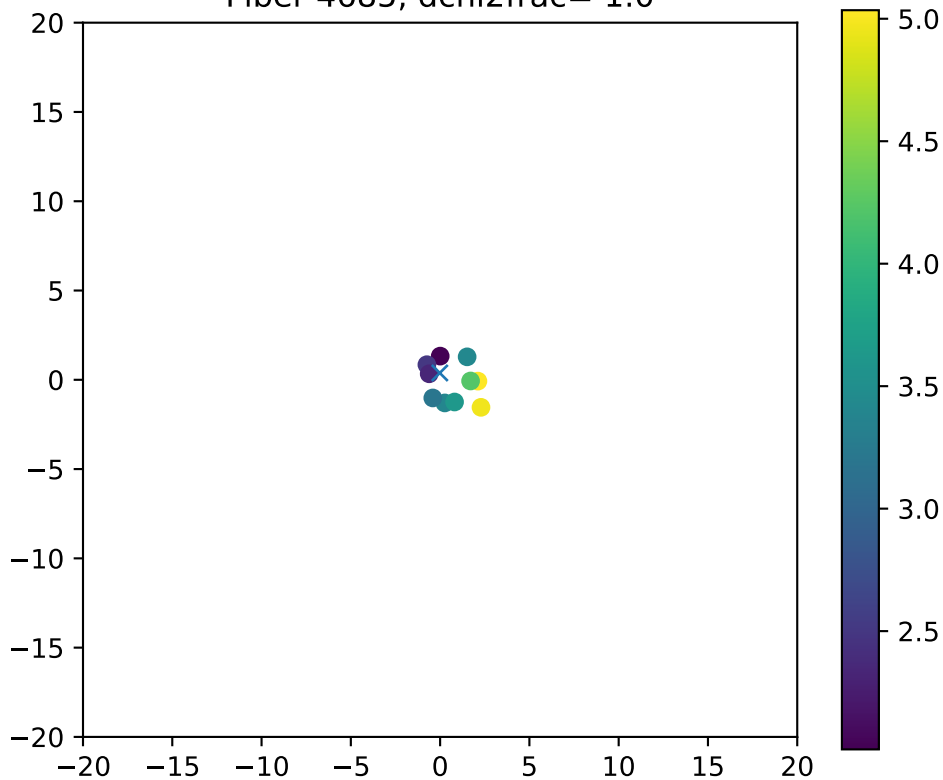
Fiber 4685, dchi2frac= 1.0
