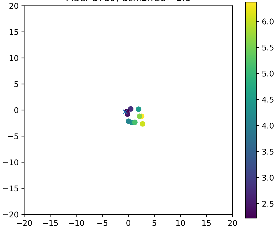
Fiber 3739, dchi2frac= 1.0
