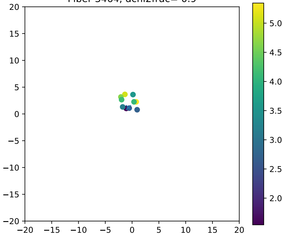
Fiber 3464, dchi2frac= 0.9
