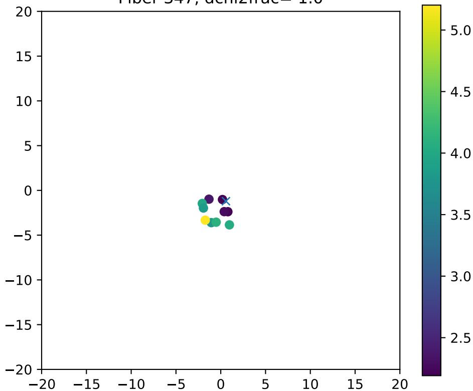
Fiber 347, dchi2frac= 1.0
