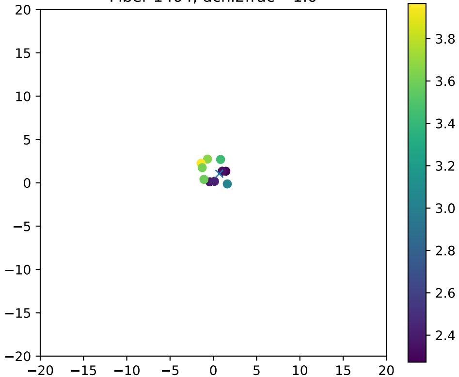
Fiber 1404, dchi2frac= 1.0
