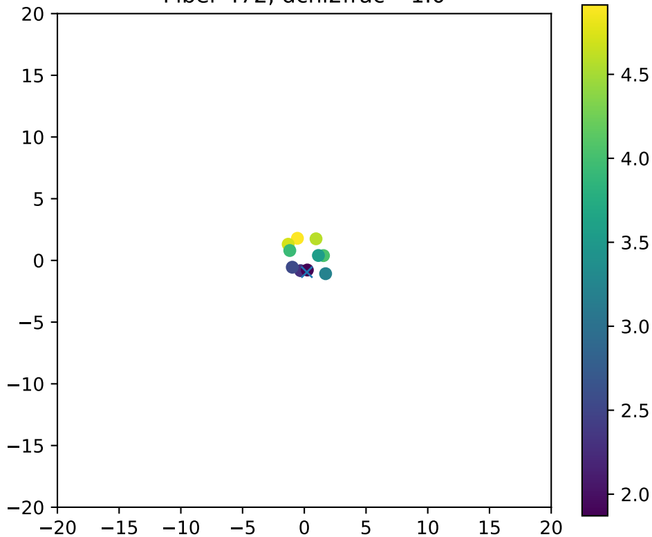
Fiber 472, dchi2frac= 1.0
