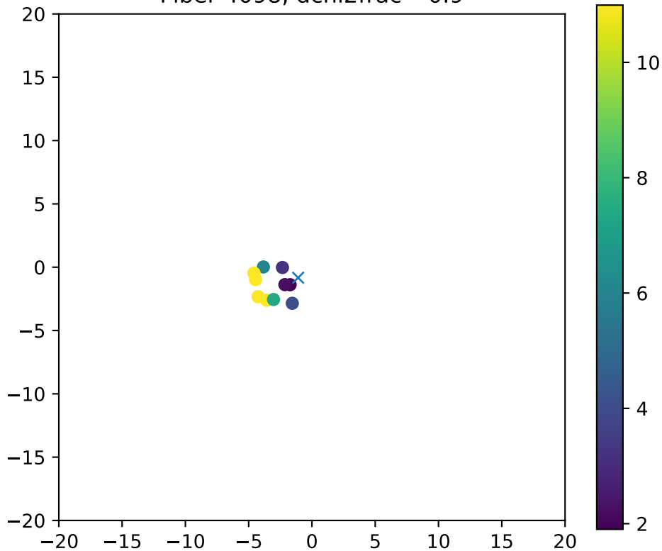
Fiber 4098, dchi2frac= 0.9
