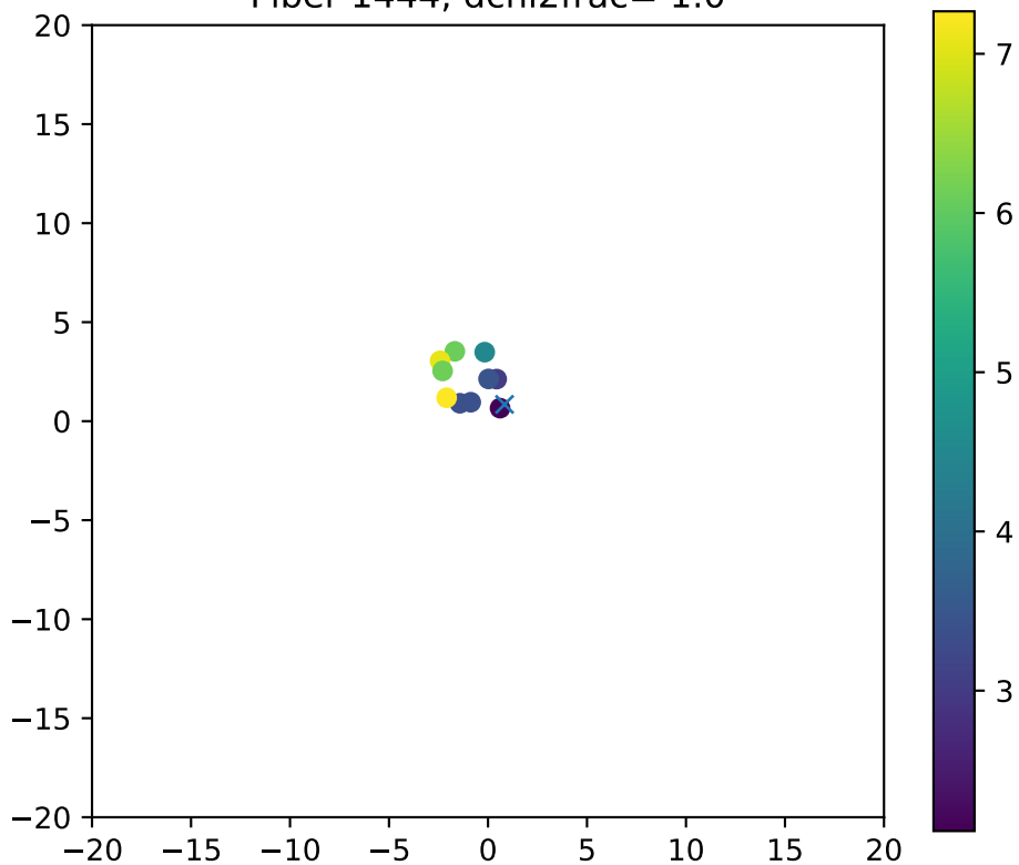
Fiber 1444, dchi2frac= 1.0
