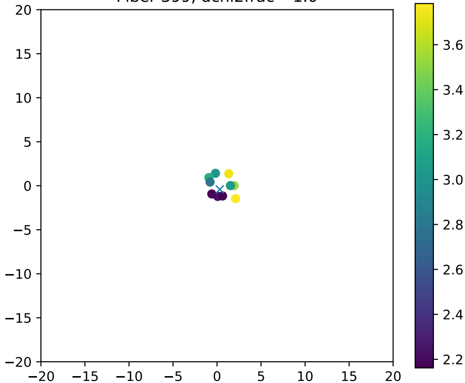
Fiber 399, dchi2frac= 1.0
