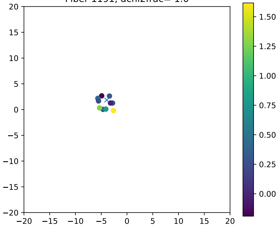
Fiber 1191, dchi2frac= 1.0
