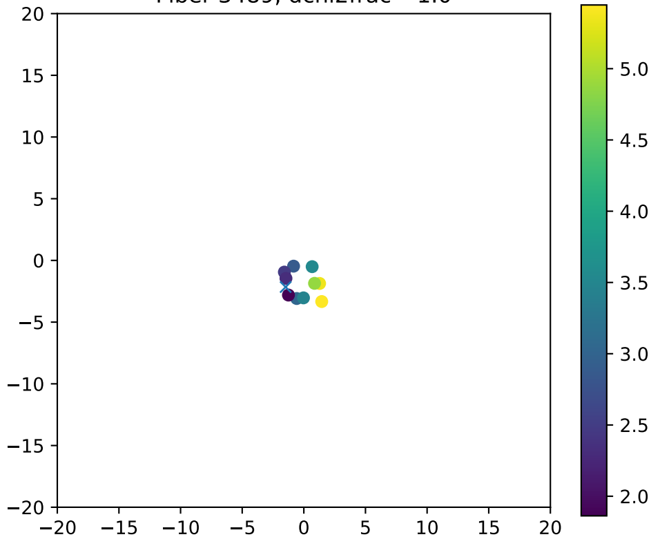
Fiber 3489, dchi2frac= 1.0
