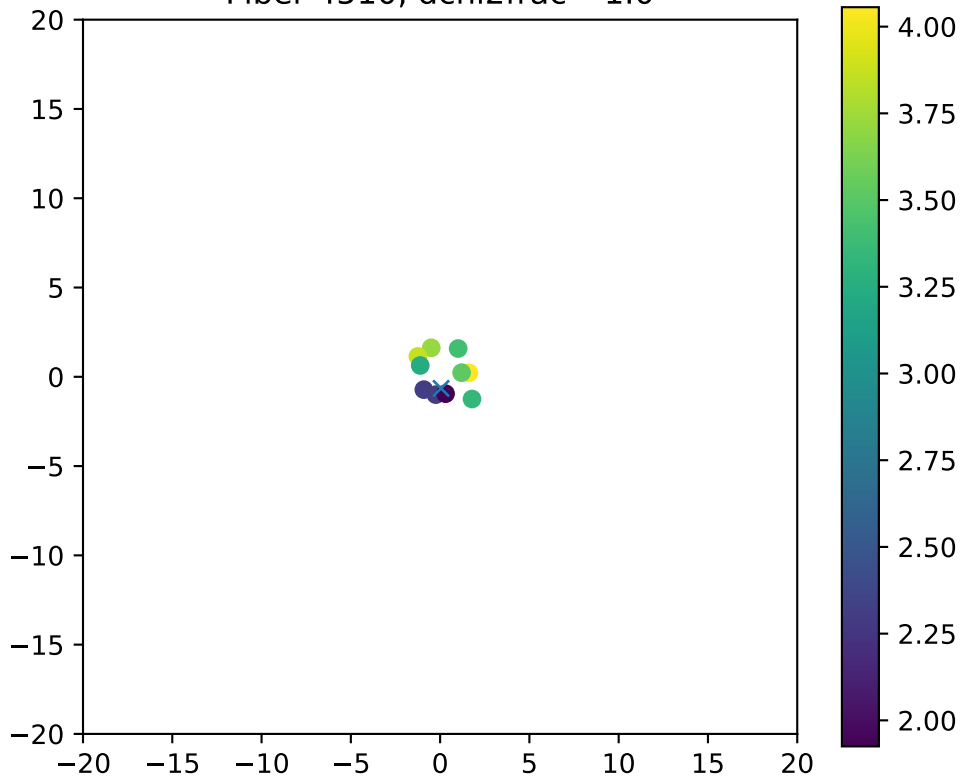
Fiber 4510, dchi2frac= 1.0
