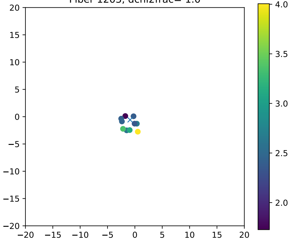
Fiber 1203, dchi2frac= 1.0
