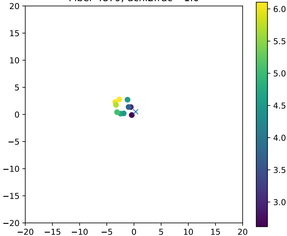
Fiber 4879, dchi2frac= 1.0
