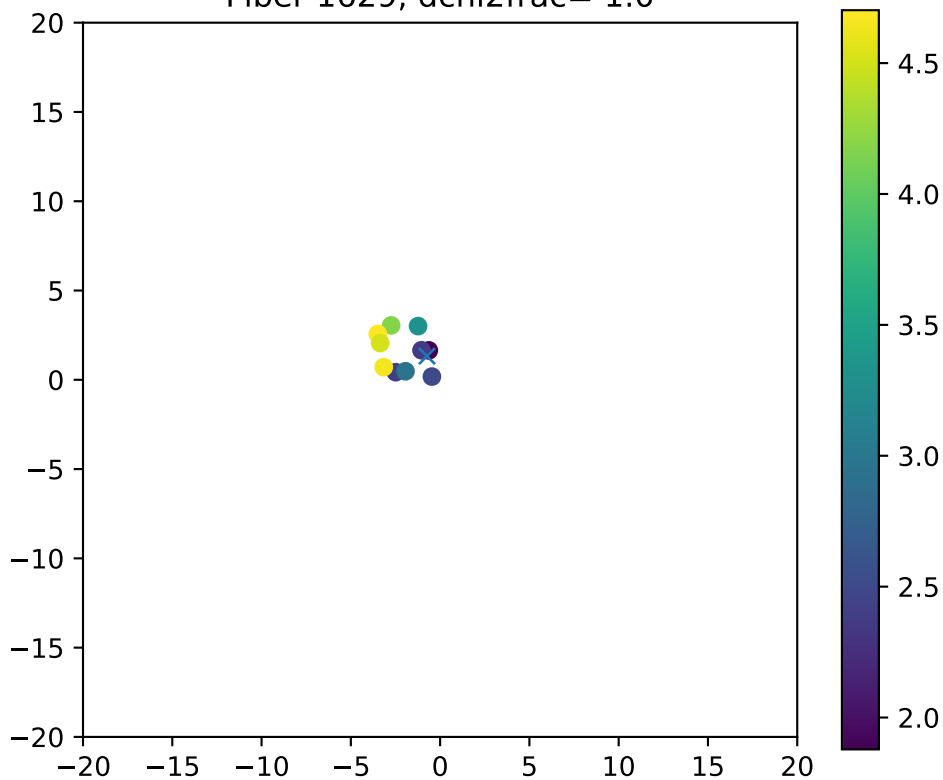
Fiber 1629, dchi2frac= 1.0
