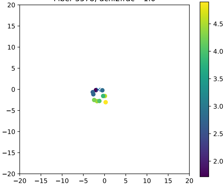
Fiber 3578, dchi2frac= 1.0
