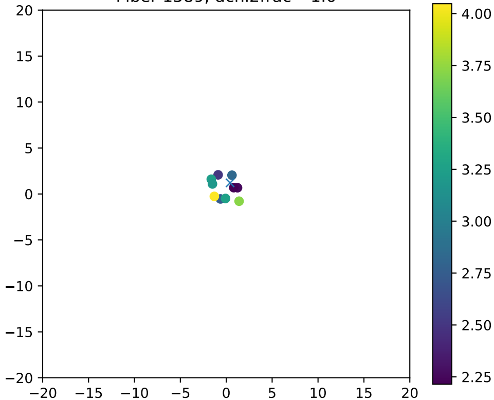
Fiber 1589, dchi2frac= 1.0
