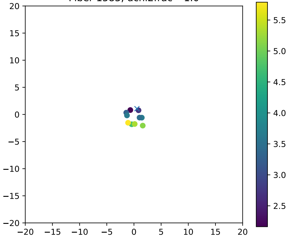
Fiber 1583, dchi2frac= 1.0
