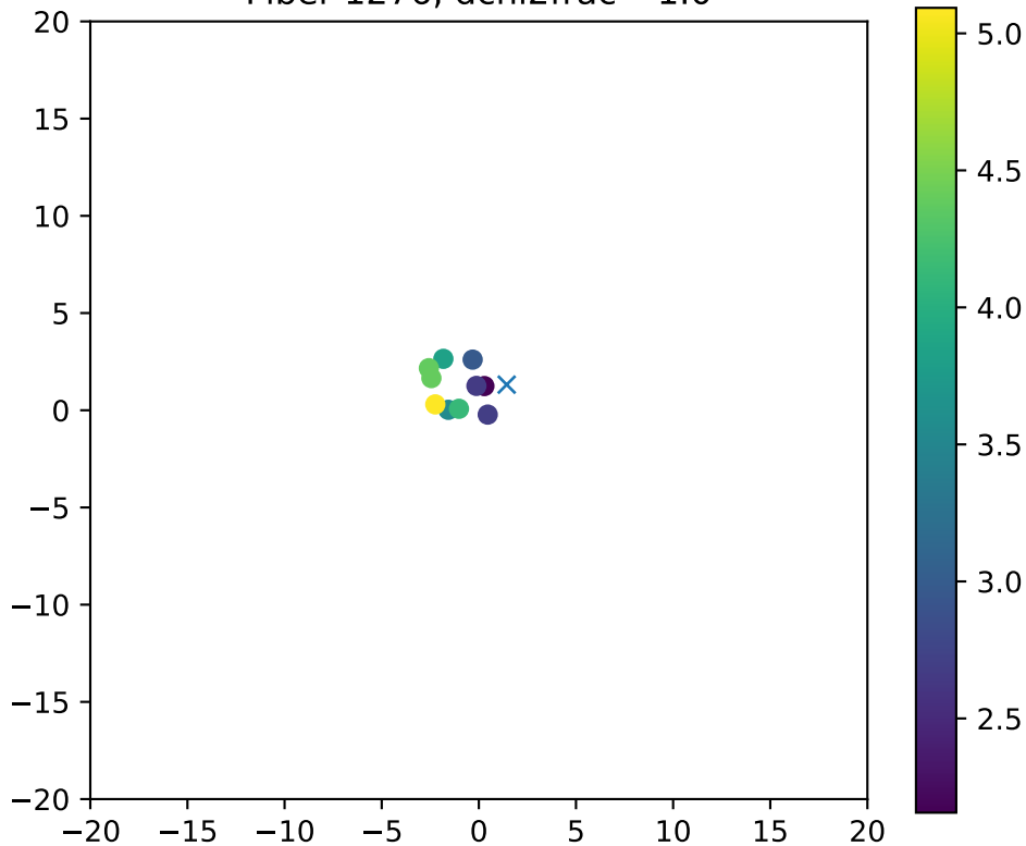
Fiber 1276, dchi2frac= 1.0
