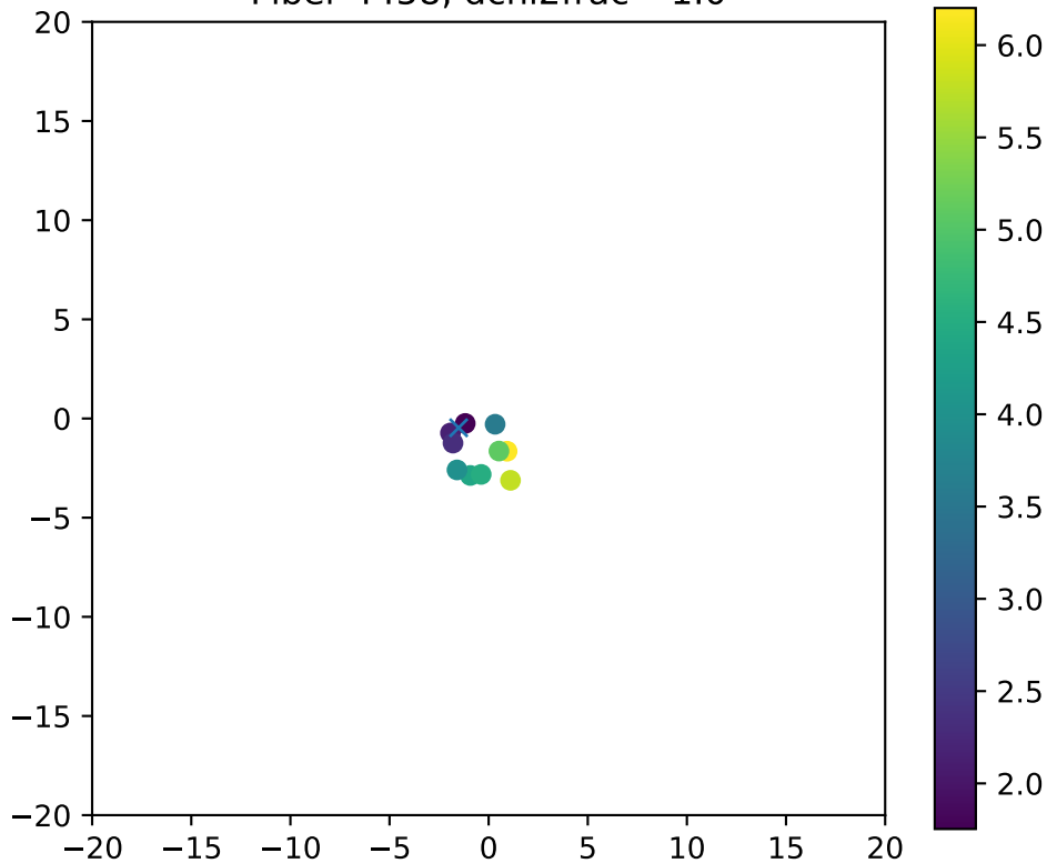
Fiber 4458, dchi2frac= 1.0
