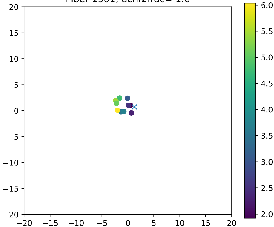
Fiber 1501, dchi2frac= 1.0
