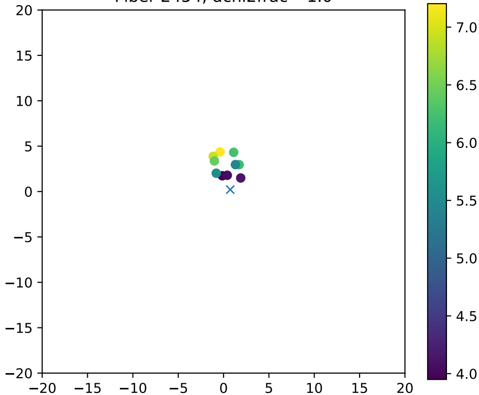
Fiber 2454, dchi2frac= 1.0
