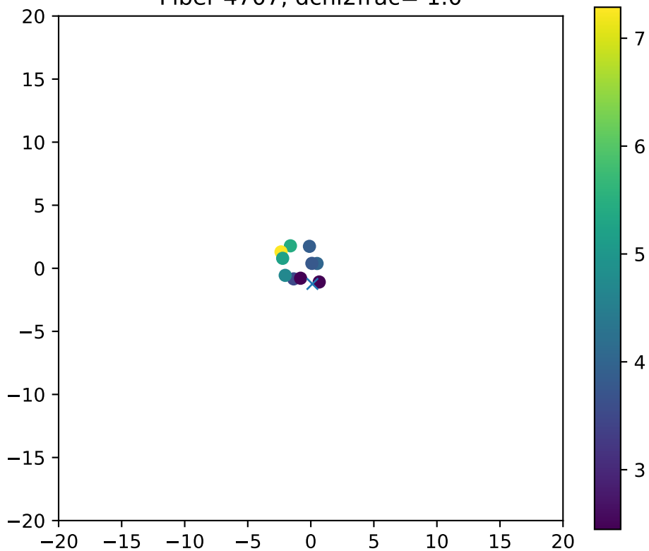
Fiber 4707, dchi2frac= 1.0
