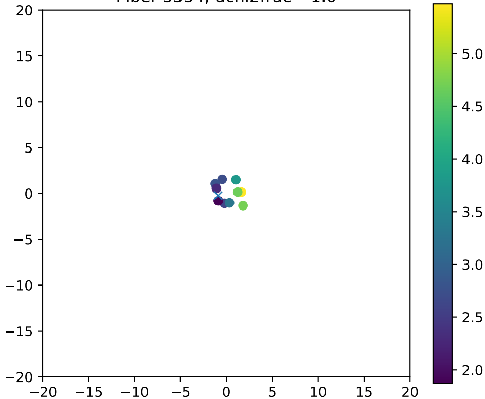
Fiber 3534, dchi2frac= 1.0
