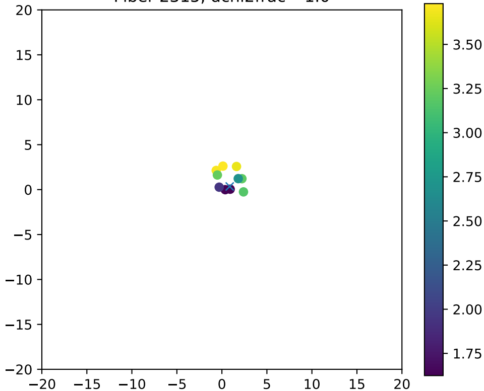
Fiber 2315, dchi2frac= 1.0
