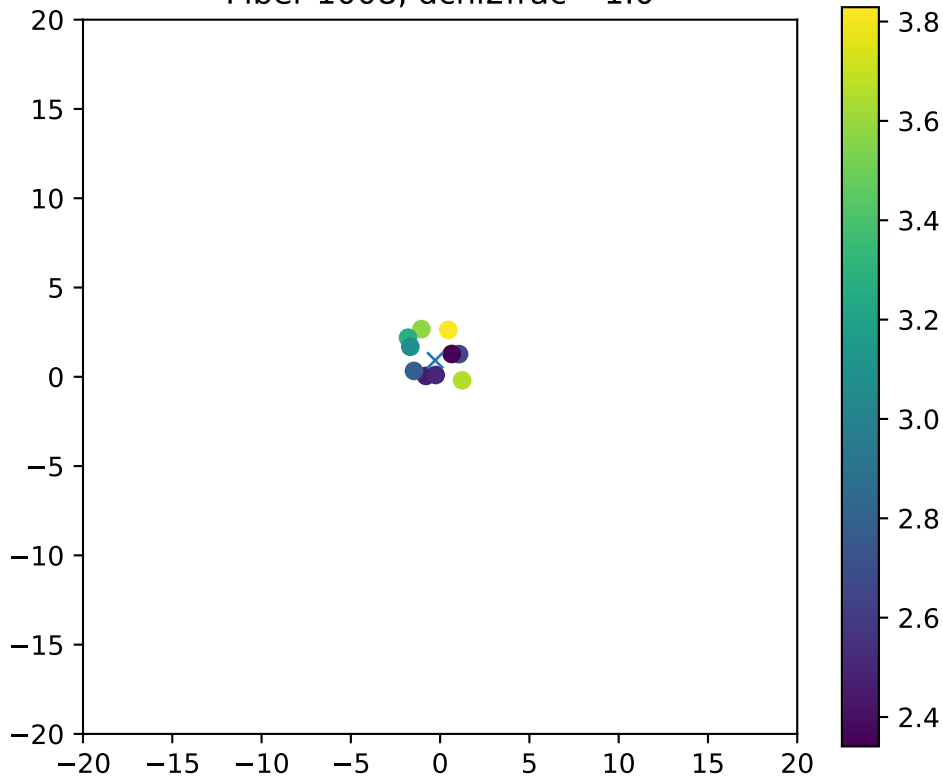
Fiber 1008, dchi2frac= 1.0
