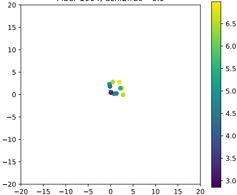
Fiber 1064, dchi2frac= 0.9
