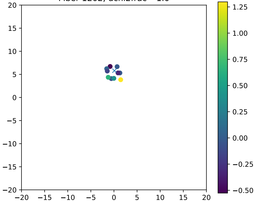
Fiber 1202, dchi2frac= 1.0
