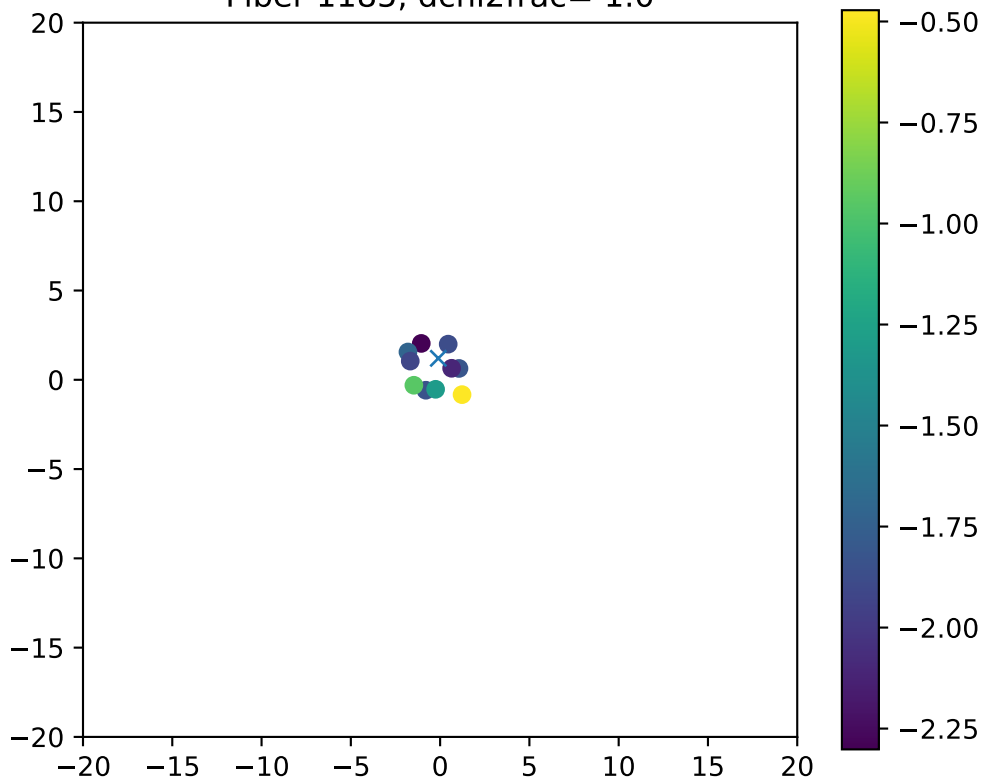
Fiber 1185, dchi2frac= 1.0
