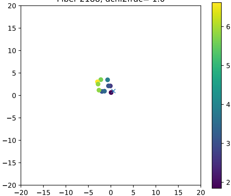
Fiber 2188, dchi2frac= 1.0
