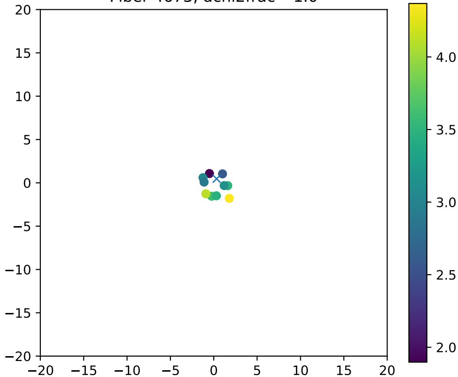
Fiber 4673, dchi2frac= 1.0
