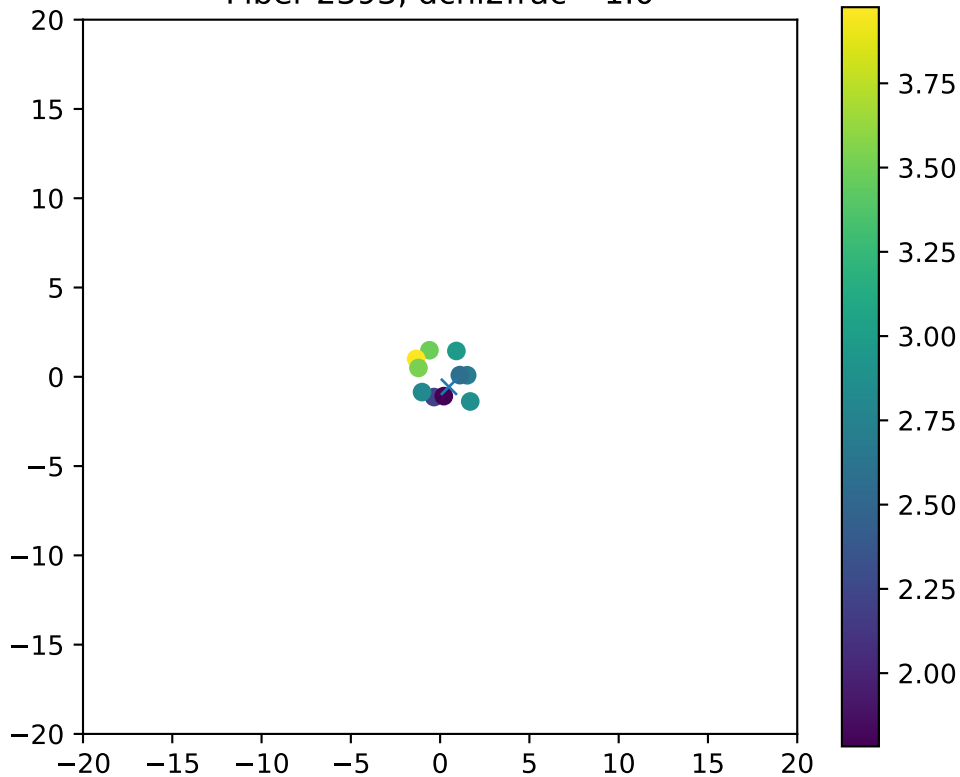
Fiber 2393, dchi2frac= 1.0
