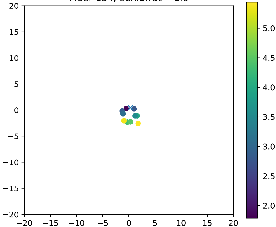
Fiber 134, dchi2frac= 1.0
