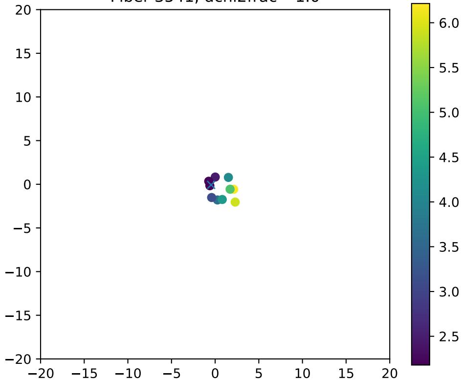
Fiber 3541, dchi2frac= 1.0
