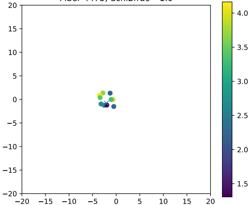
Fiber 4475, dchi2frac= 1.0
