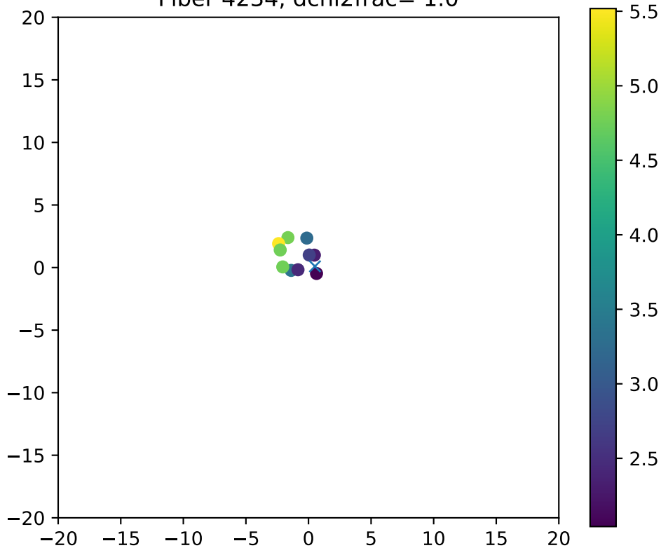
Fiber 4234, dchi2frac= 1.0
