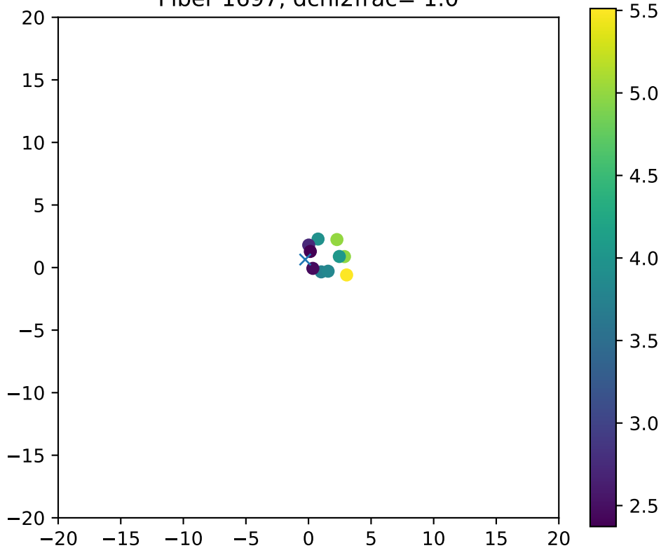
Fiber 1697, dchi2frac= 1.0
