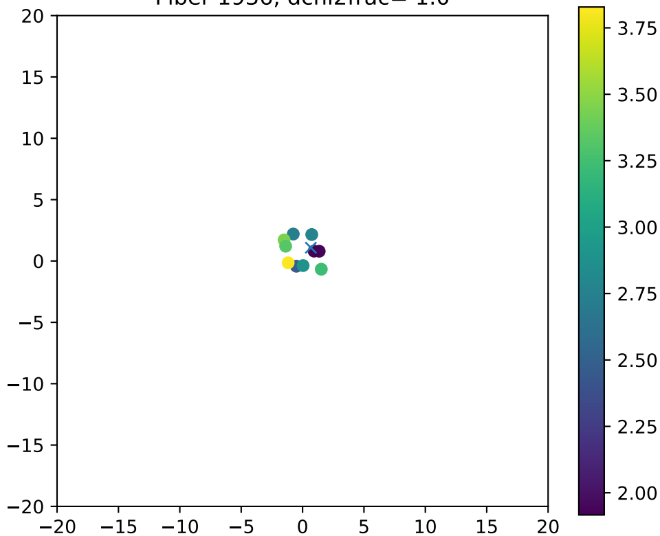
Fiber 1936, dchi2frac= 1.0
