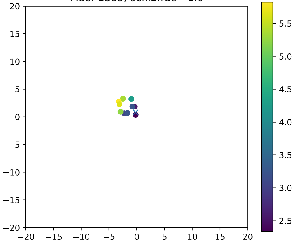
Fiber 1303, dchi2frac= 1.0
