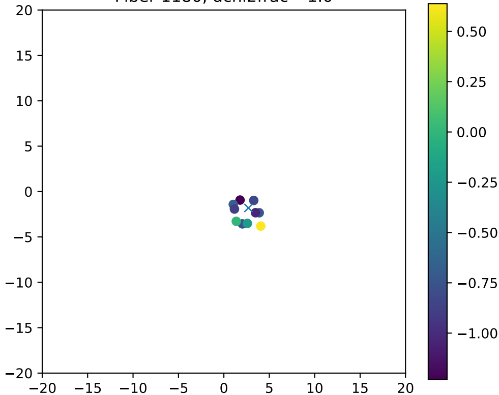
Fiber 1180, dchi2frac= 1.0
