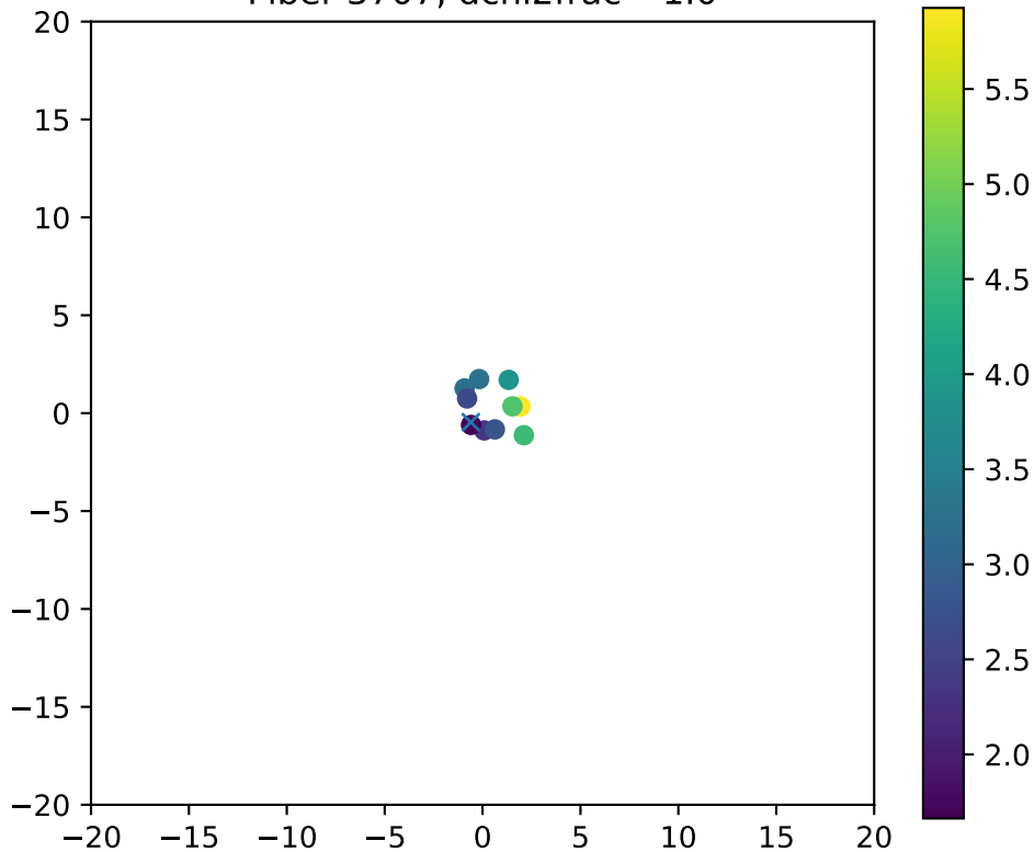
Fiber 3707, dchi2frac= 1.0
