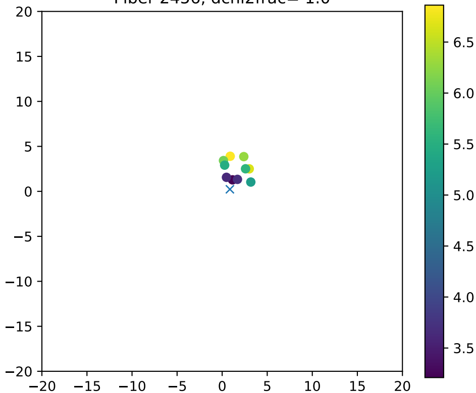
Fiber 2456, dchi2frac= 1.0
