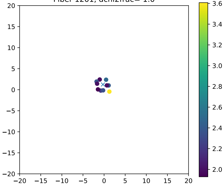
Fiber 1201, dchi2frac= 1.0
