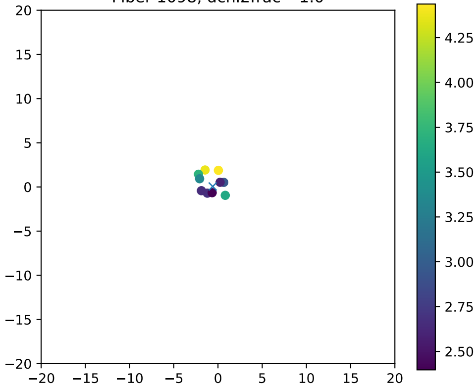
Fiber 1098, dchi2frac= 1.0
