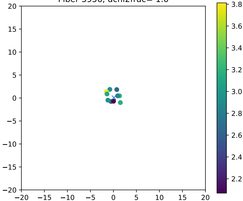
Fiber 3956, dchi2frac= 1.0
