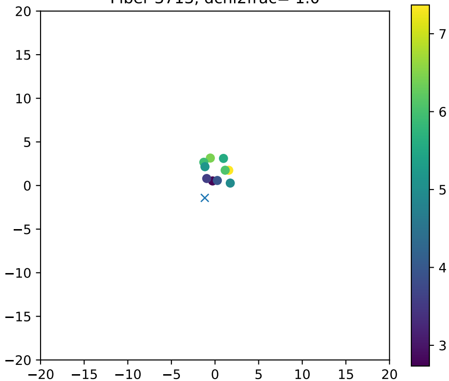
Fiber 3713, dchi2frac= 1.0
