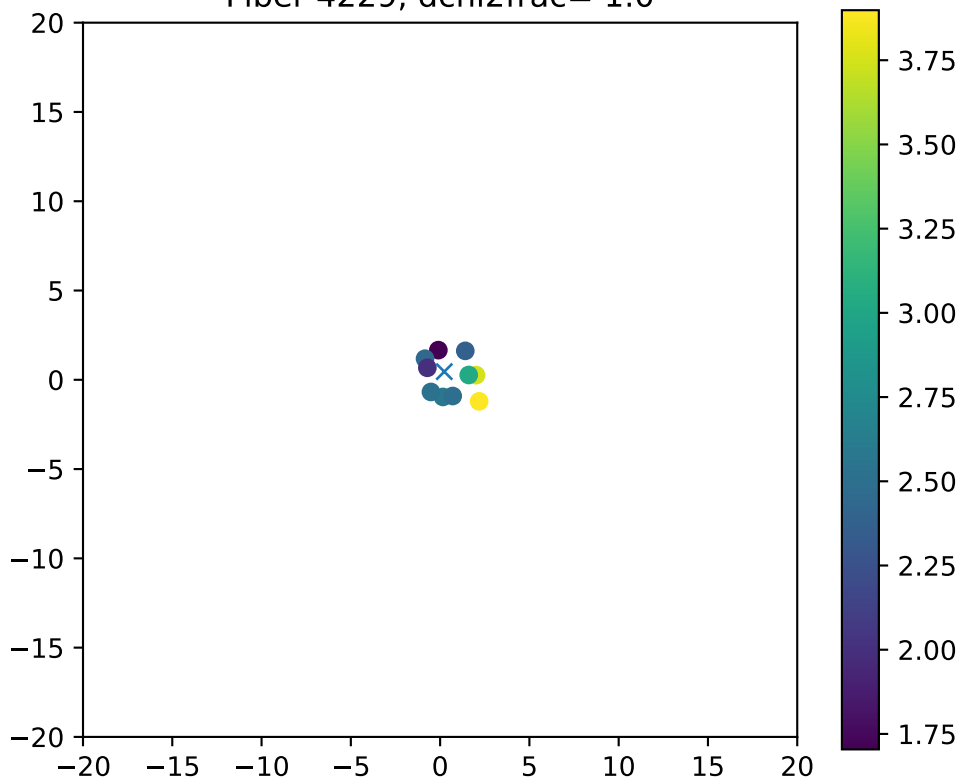
Fiber 4229, dchi2frac= 1.0
