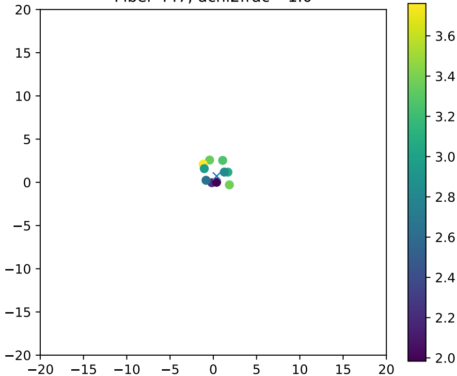
Fiber 447, dchi2frac= 1.0
