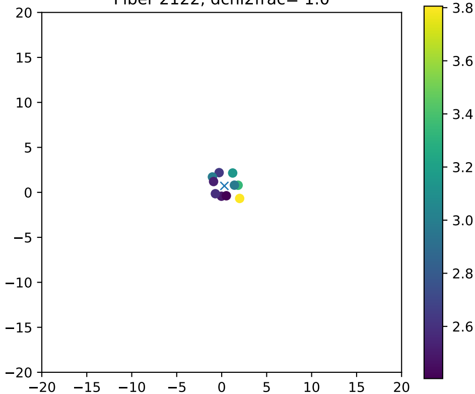
Fiber 2122, dchi2frac= 1.0
