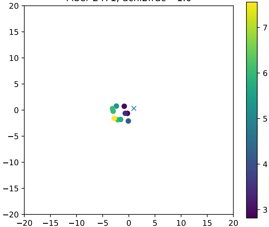
Fiber 2471, dchi2frac= 1.0
