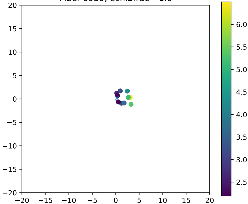
Fiber 3959, dchi2frac= 1.0
