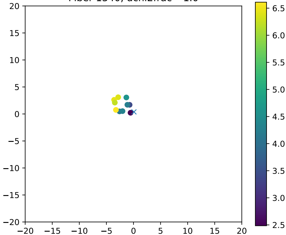
Fiber 1340, dchi2frac= 1.0
