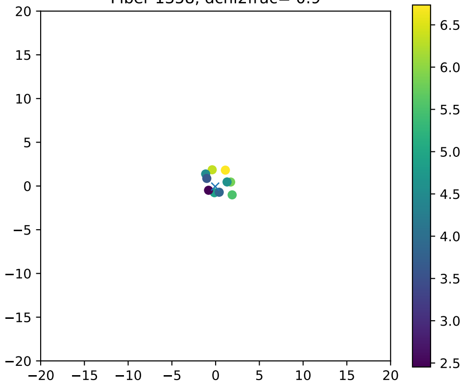
Fiber 1358, dchi2frac= 0.9
