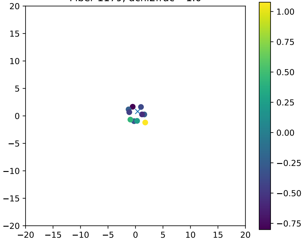
Fiber 1179, dchi2frac= 1.0
