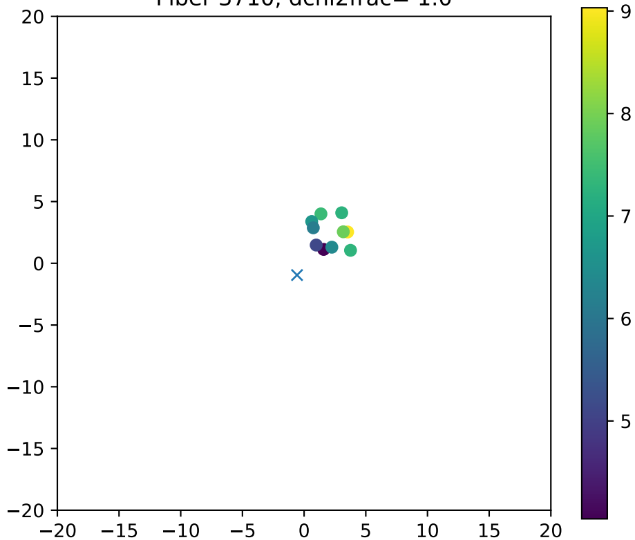
Fiber 3710, dchi2frac= 1.0
