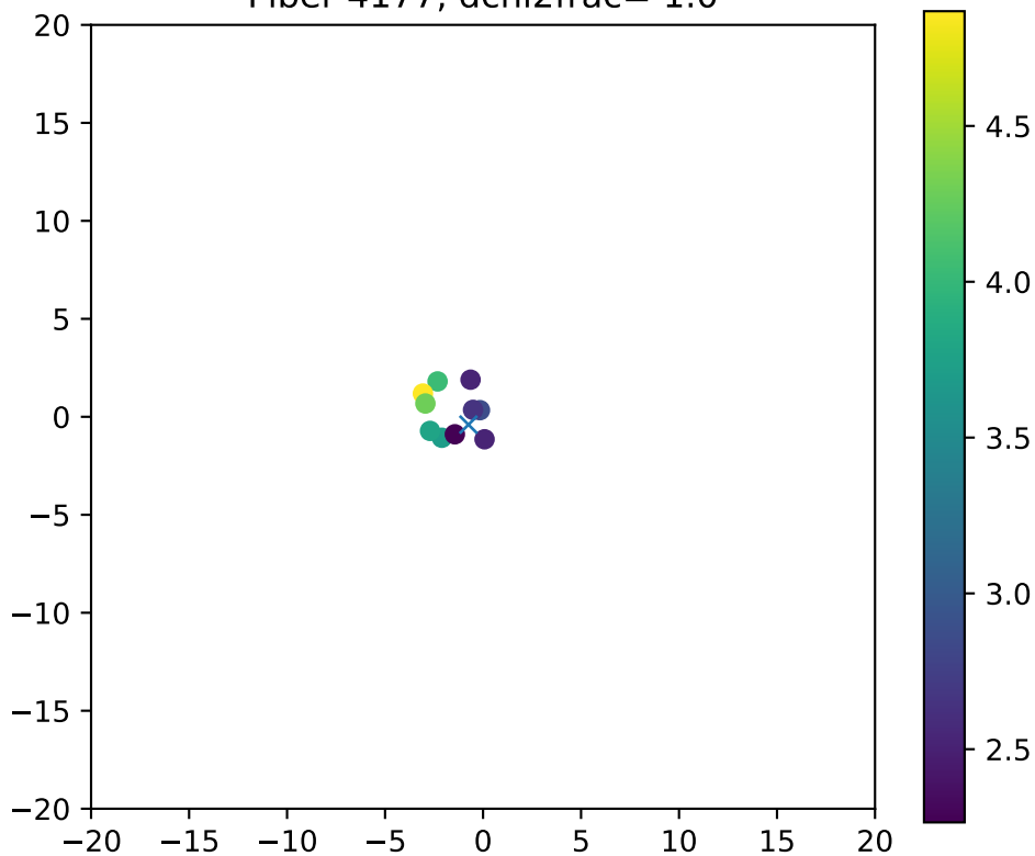
Fiber 4177, dchi2frac= 1.0
