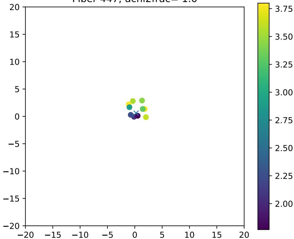
Fiber 447, dchi2frac= 1.0
