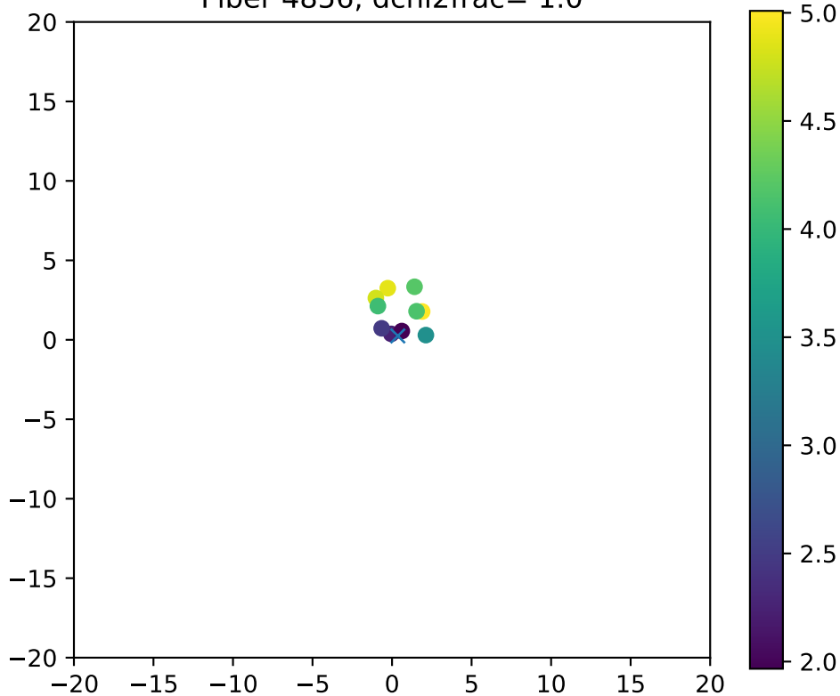
Fiber 4856, dchi2frac= 1.0
