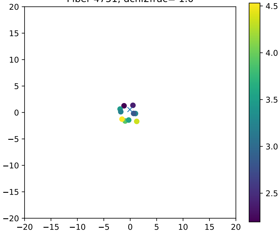
Fiber 4751, dchi2frac= 1.0
