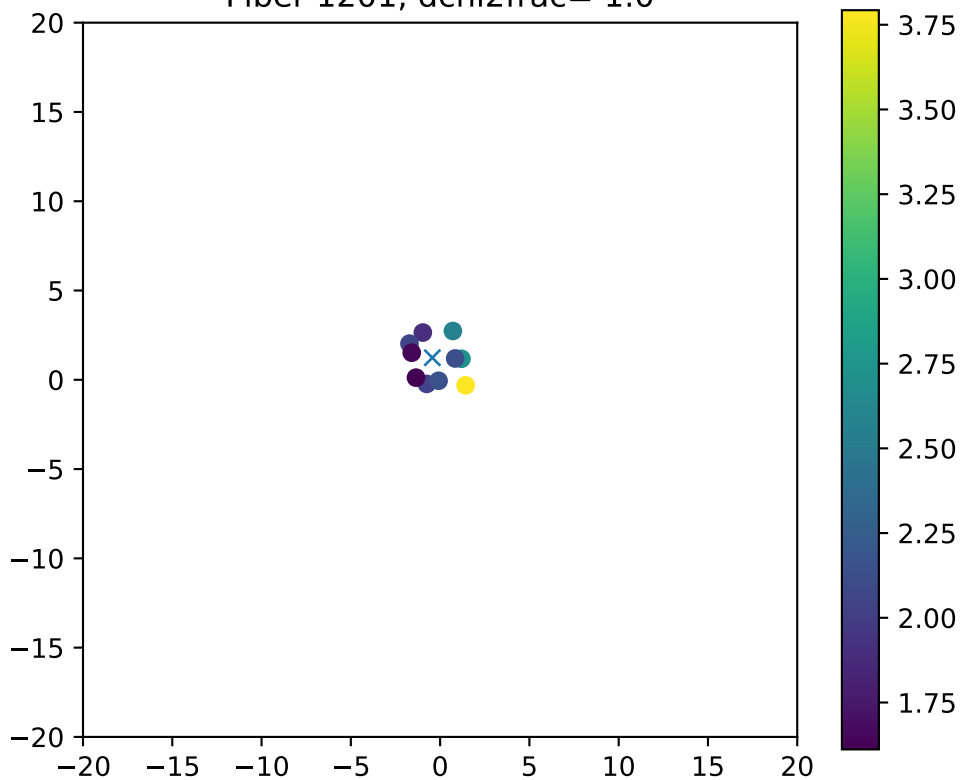
Fiber 1201, dchi2frac= 1.0
