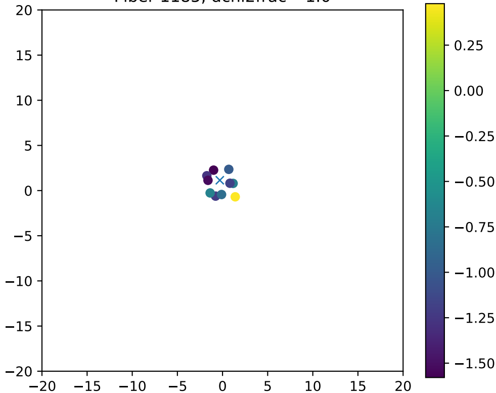
Fiber 1185, dchi2frac= 1.0
