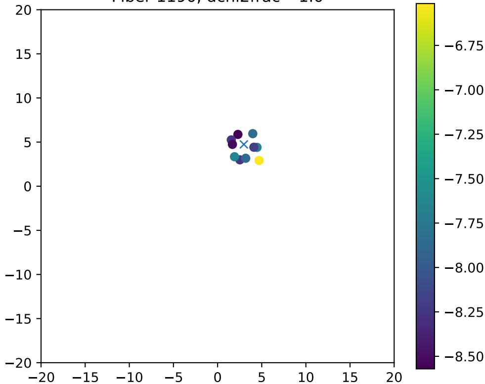
Fiber 1190, dchi2frac= 1.0
