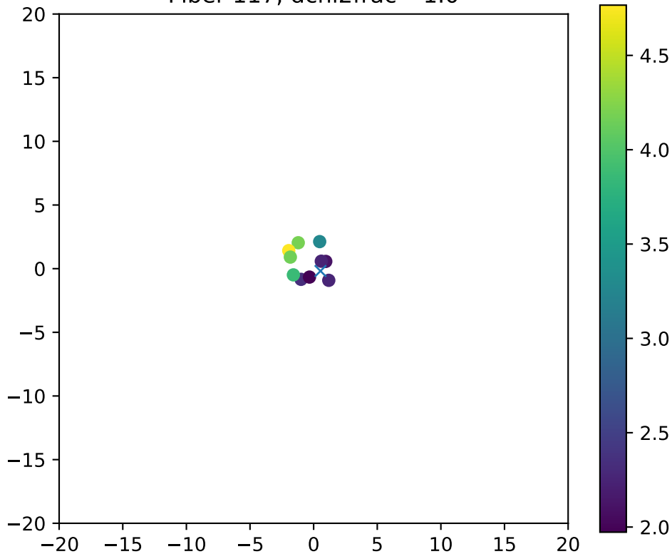
Fiber 117, dchi2frac= 1.0
