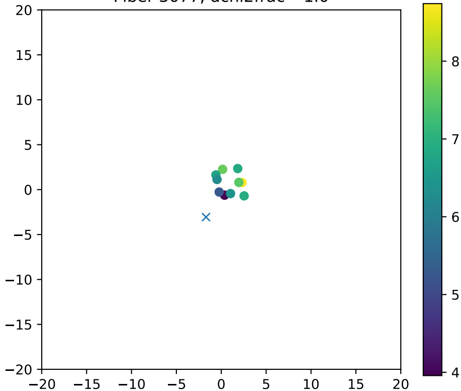
Fiber 3077, dchi2frac= 1.0
