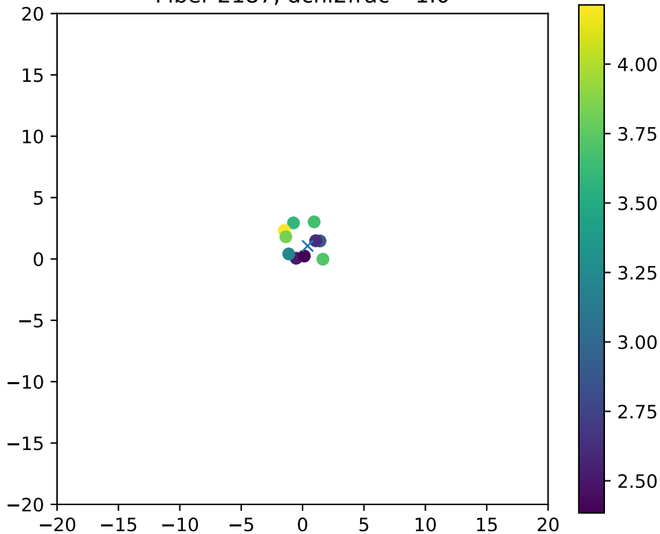
Fiber 2187, dchi2frac= 1.0
