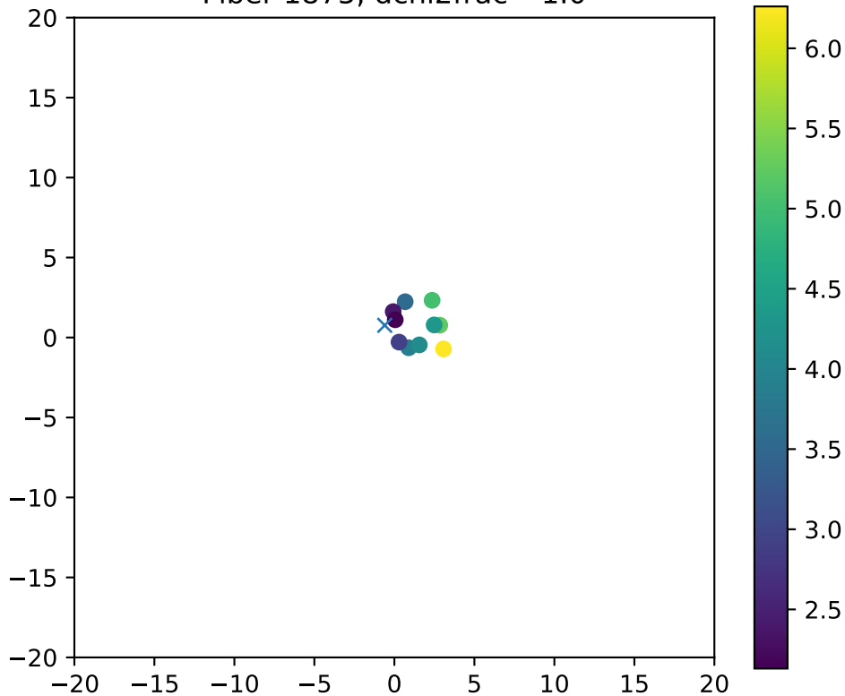
Fiber 1875, dchi2frac= 1.0
