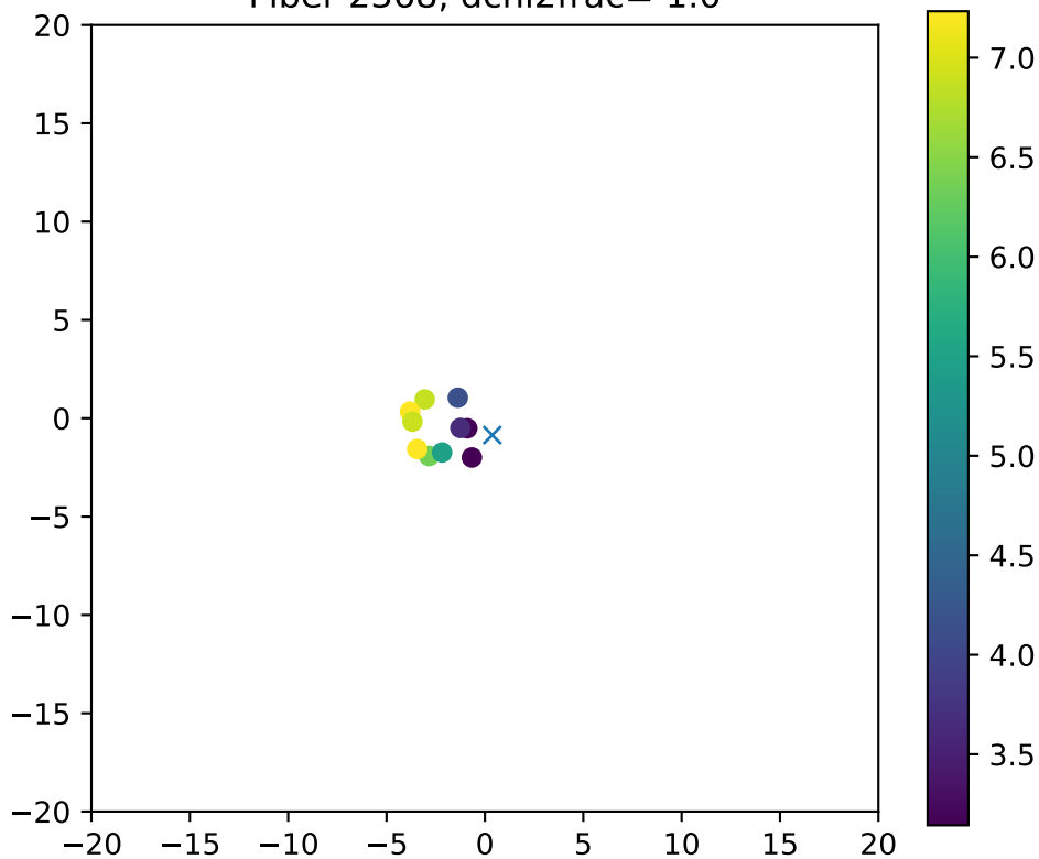
Fiber 2368, dchi2frac= 1.0
