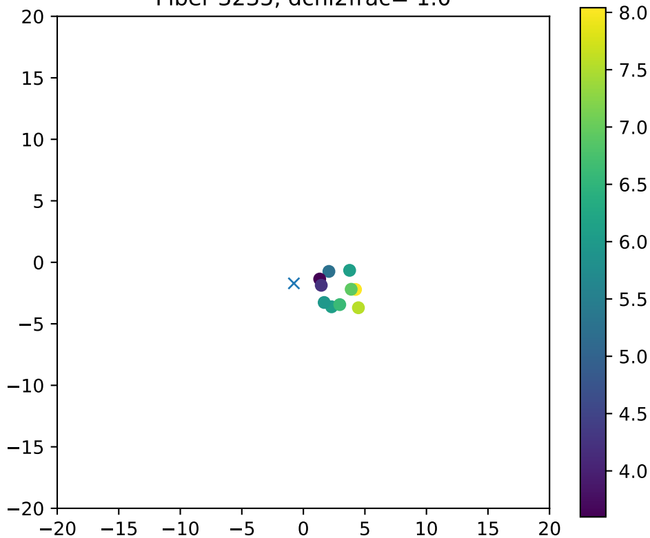
Fiber 3235, dchi2frac= 1.0
