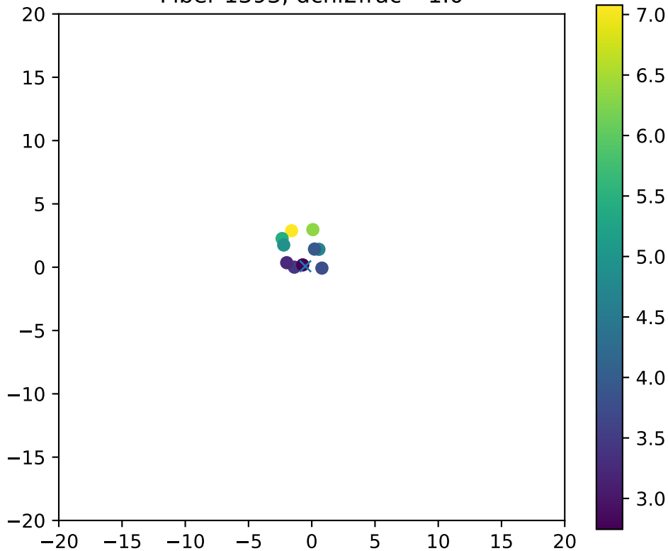
Fiber 1393, dchi2frac= 1.0
