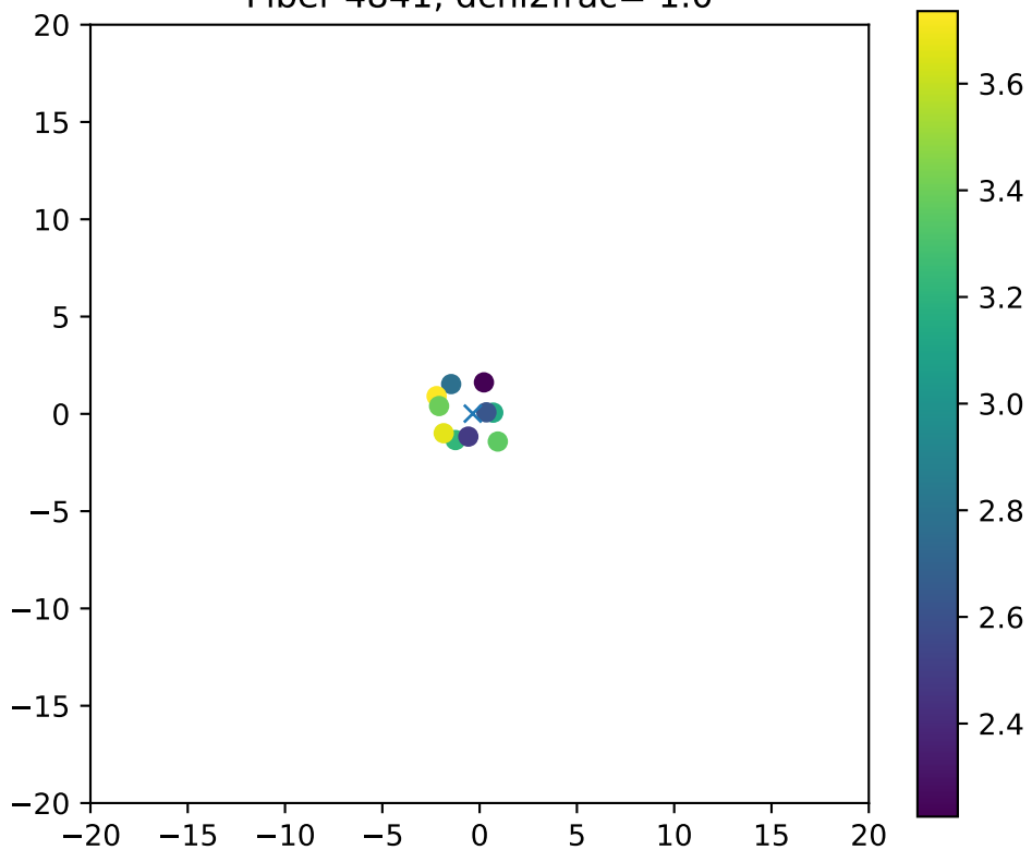
Fiber 4841, dchi2frac= 1.0
