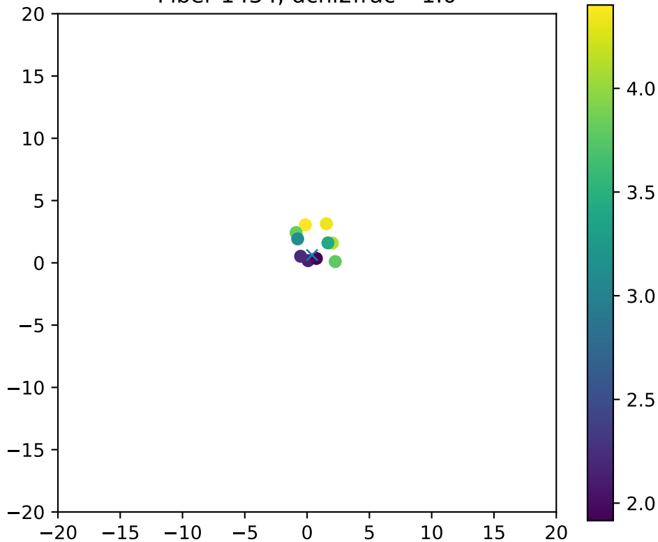
Fiber 1434, dchi2frac= 1.0
