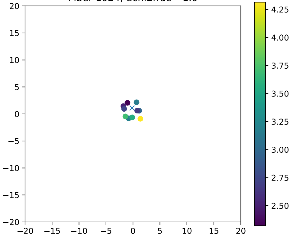
Fiber 1024, dchi2frac= 1.0
