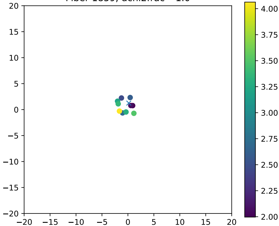
Fiber 1859, dchi2frac= 1.0
