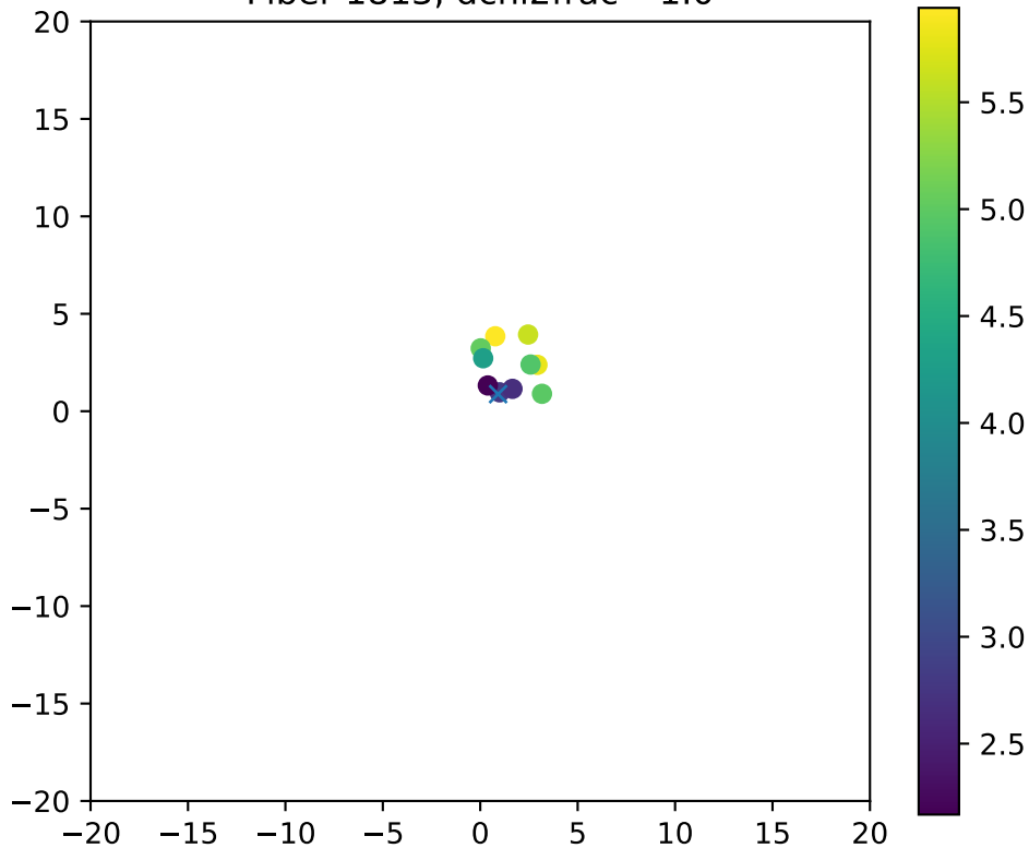
Fiber 1813, dchi2frac= 1.0
