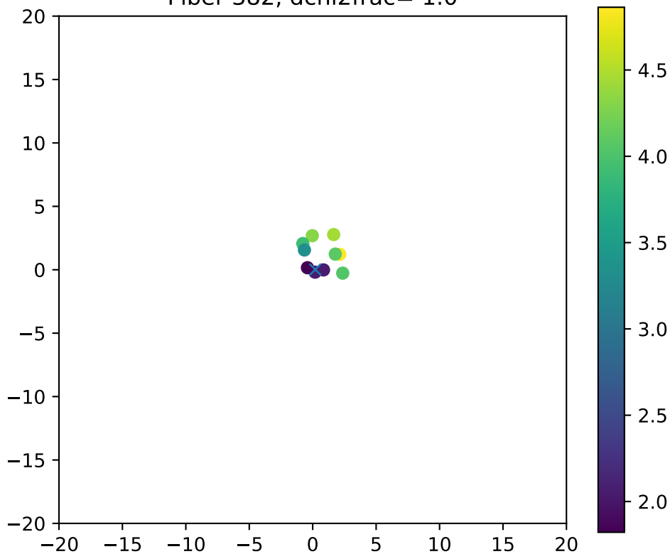
Fiber 382, dchi2frac= 1.0
