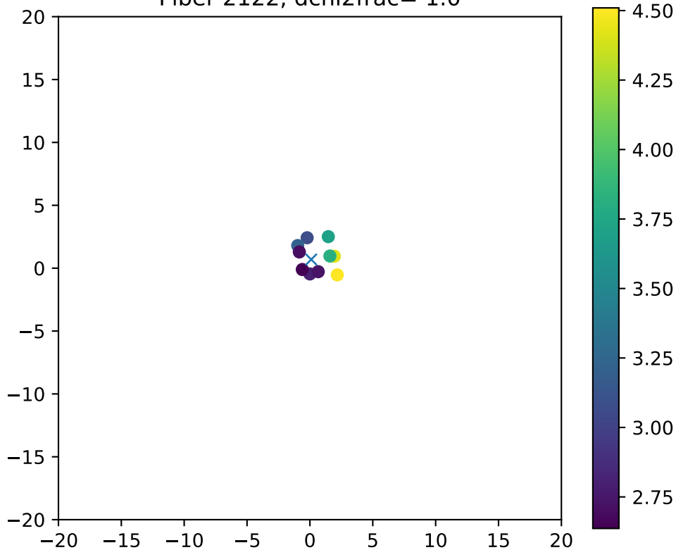
Fiber 2122, dchi2frac= 1.0
