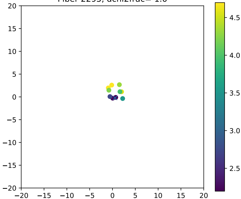
Fiber 2295, dchi2frac= 1.0
