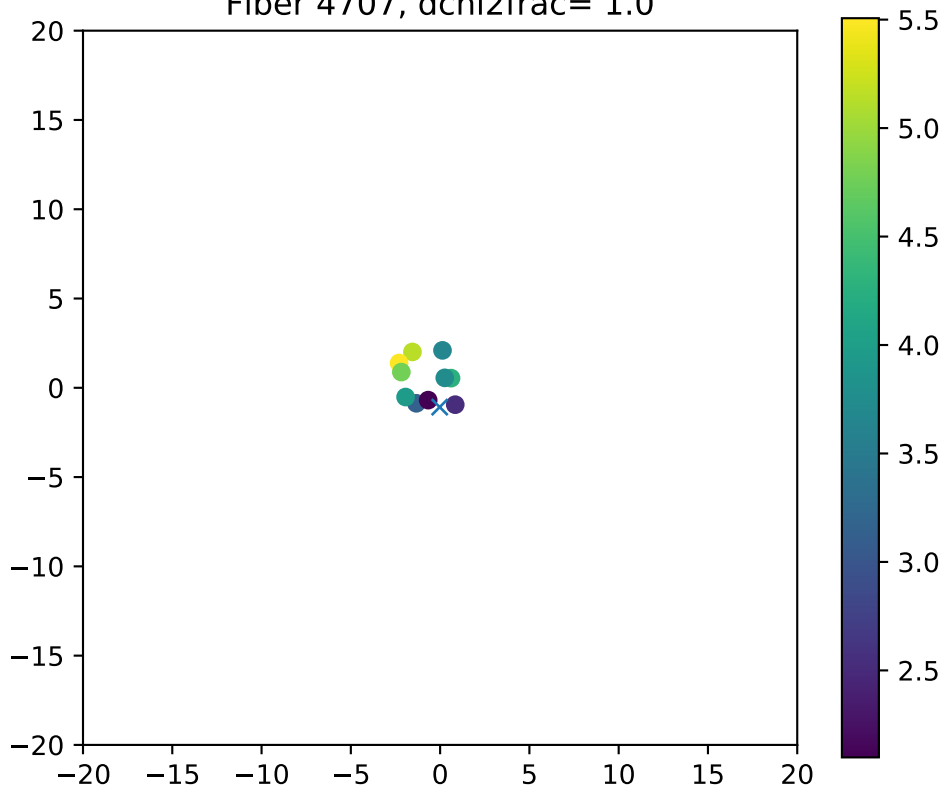
Fiber 4707, dchi2frac= 1.0
