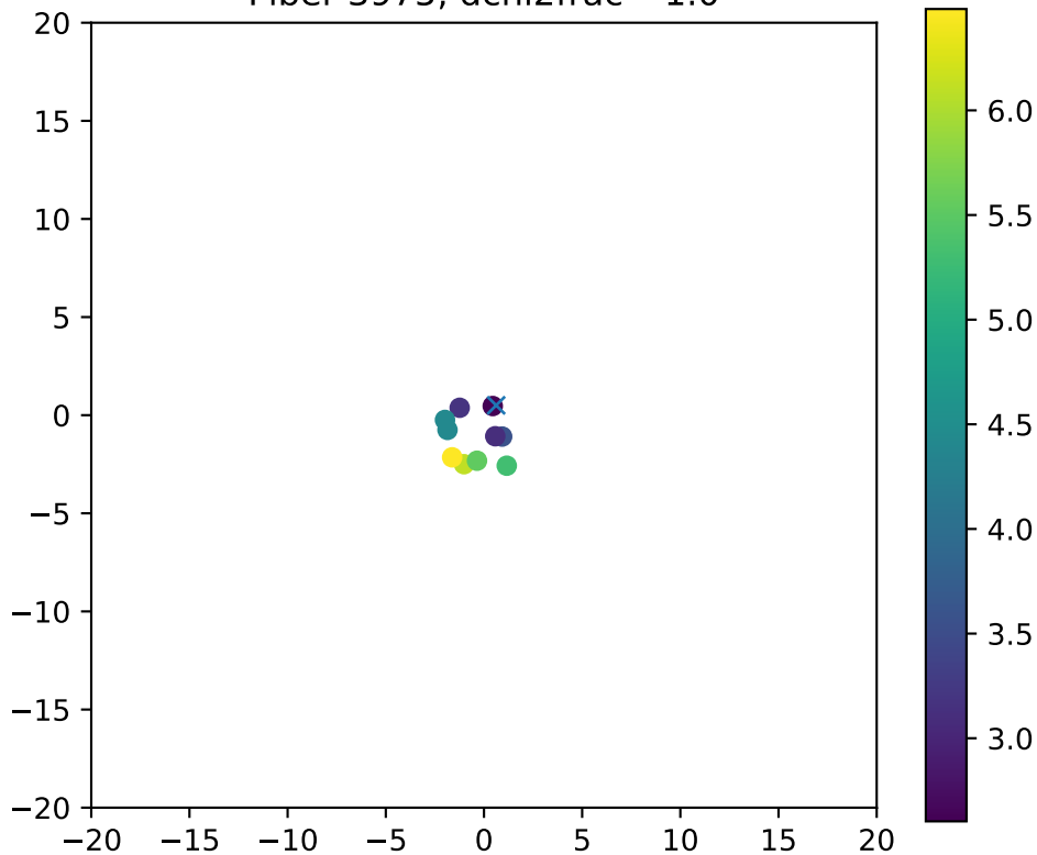
Fiber 3975, dchi2frac= 1.0
