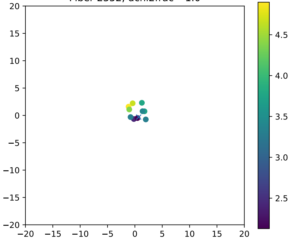
Fiber 2352, dchi2frac= 1.0
