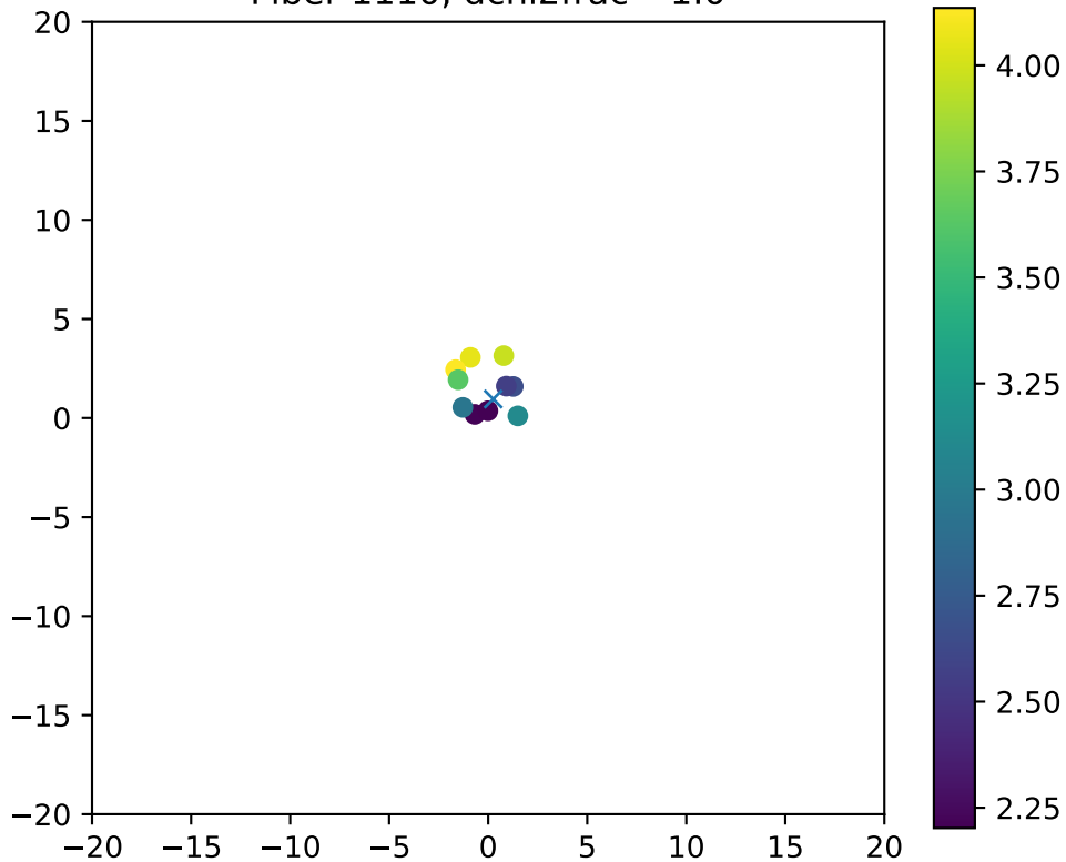
Fiber 1110, dchi2frac= 1.0
