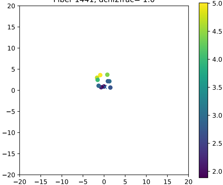
Fiber 1441, dchi2frac= 1.0
