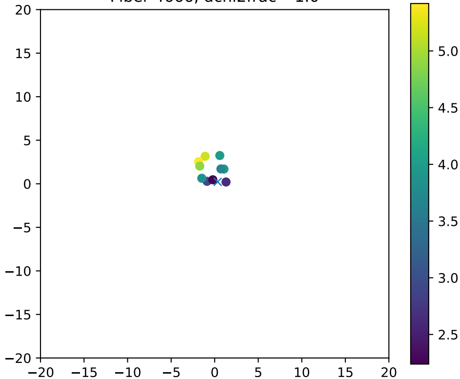
Fiber 4666, dchi2frac= 1.0
