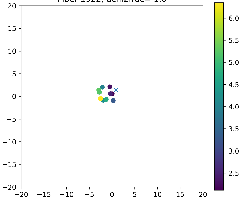
Fiber 1922, dchi2frac= 1.0
