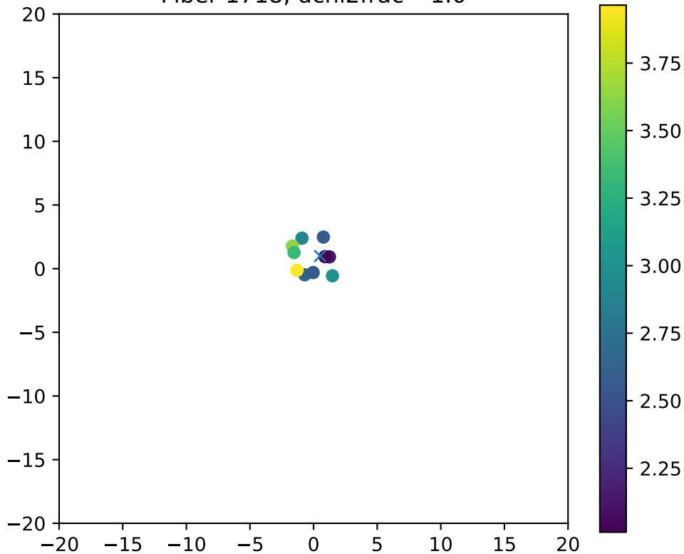
Fiber 1718, dchi2frac= 1.0
