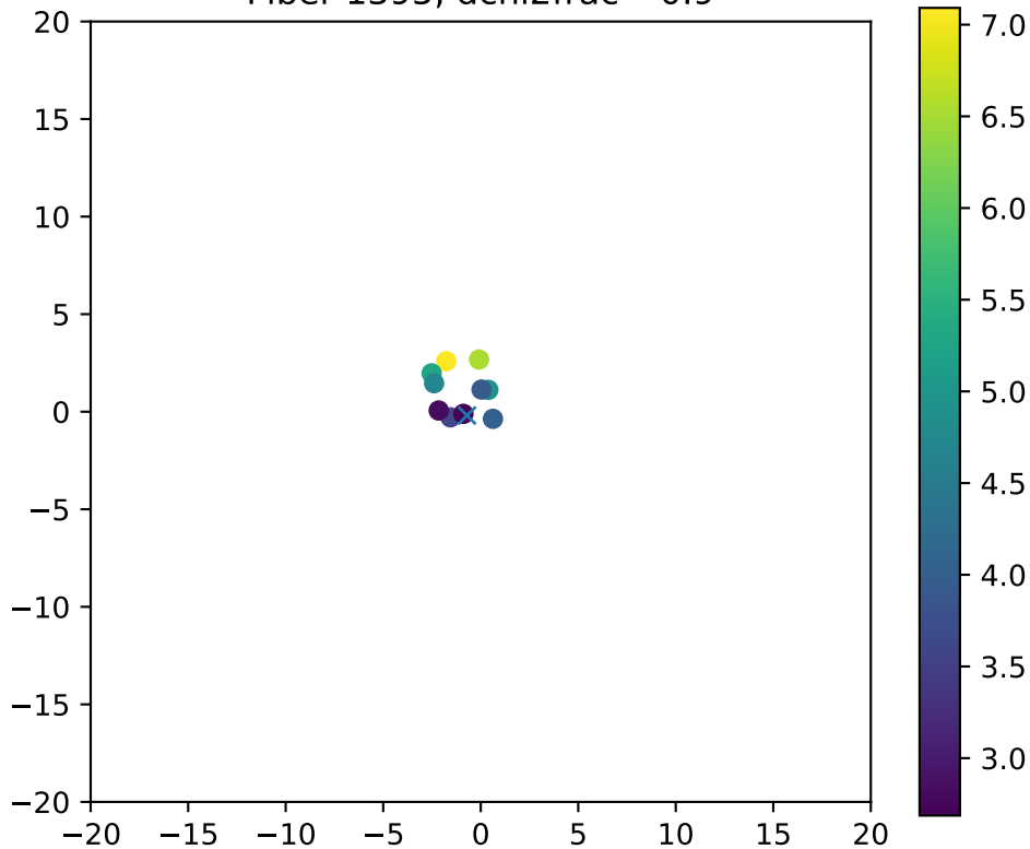
Fiber 1395, dchi2frac= 0.9
