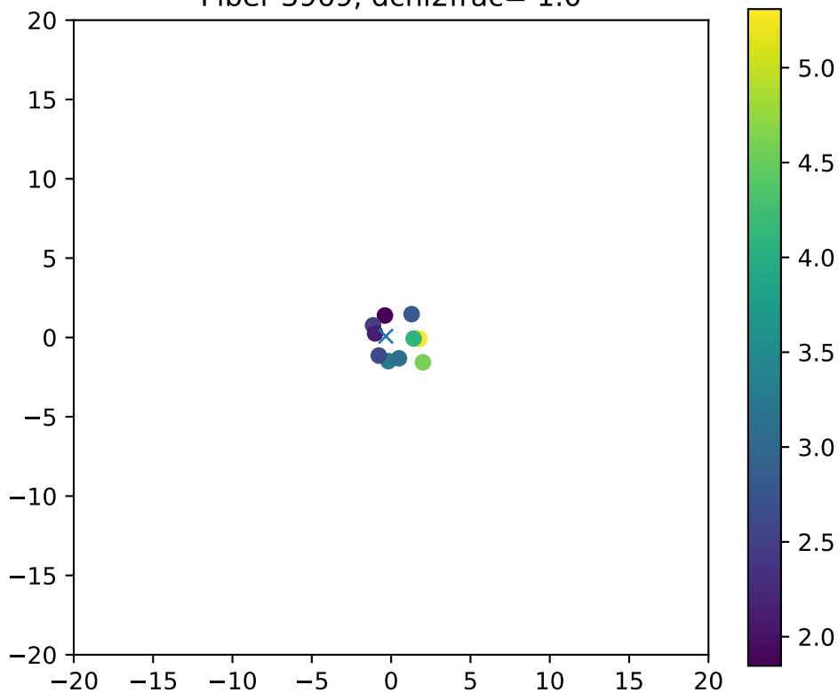
Fiber 3969, dchi2frac= 1.0
