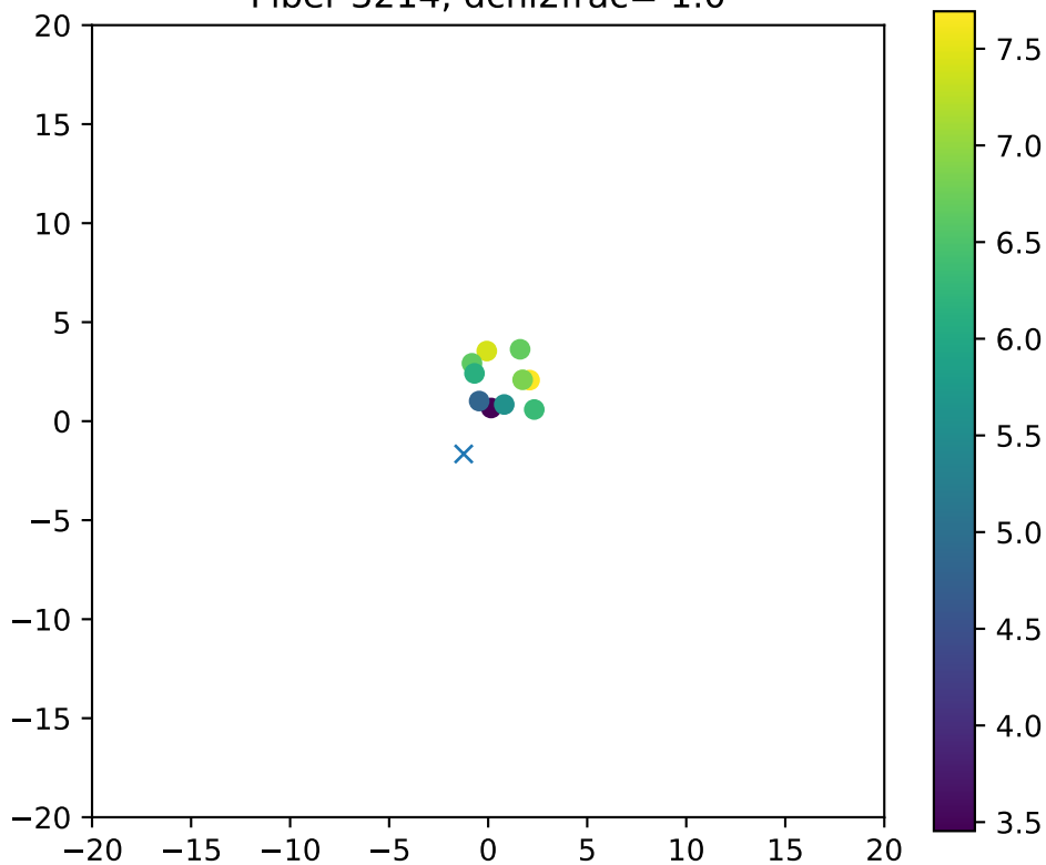
Fiber 3214, dchi2frac= 1.0
