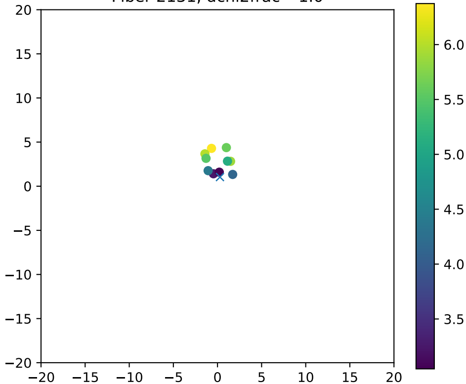
Fiber 2131, dchi2frac= 1.0
