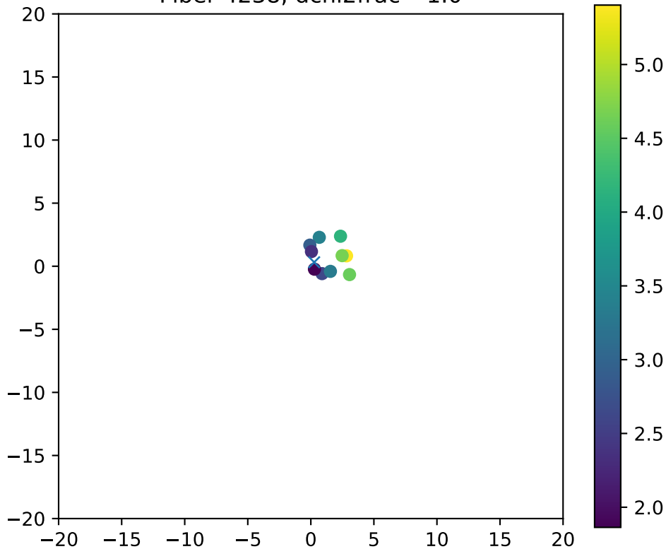
Fiber 4238, dchi2frac= 1.0
