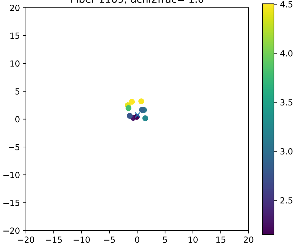
Fiber 1109, dchi2frac= 1.0
