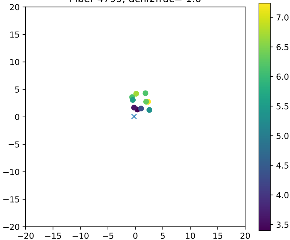
Fiber 4799, dchi2frac= 1.0
