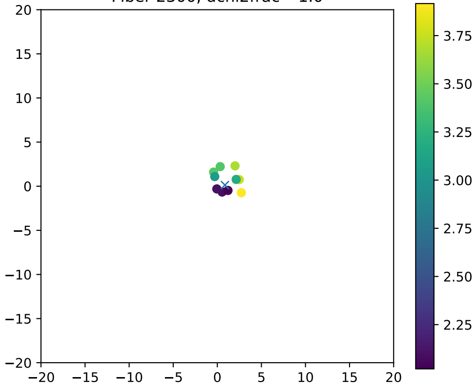
Fiber 2300, dchi2frac= 1.0
