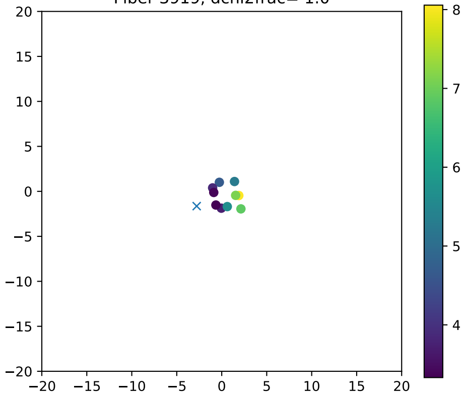
Fiber 3919, dchi2frac= 1.0
