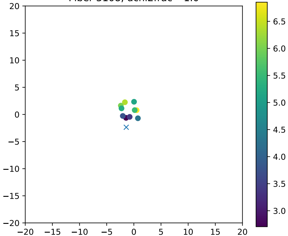
Fiber 3108, dchi2frac= 1.0
