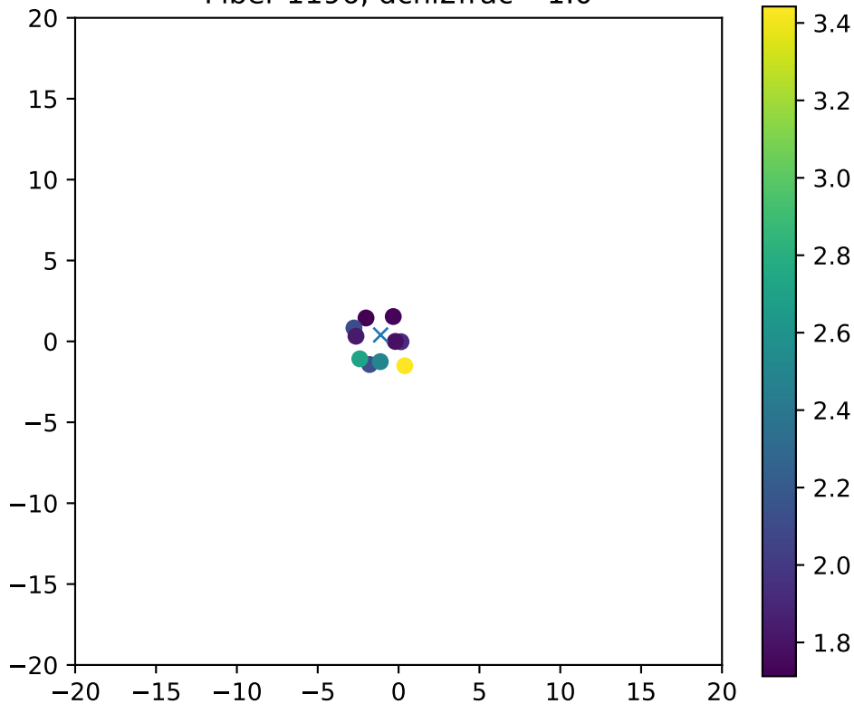
Fiber 1196, dchi2frac= 1.0
