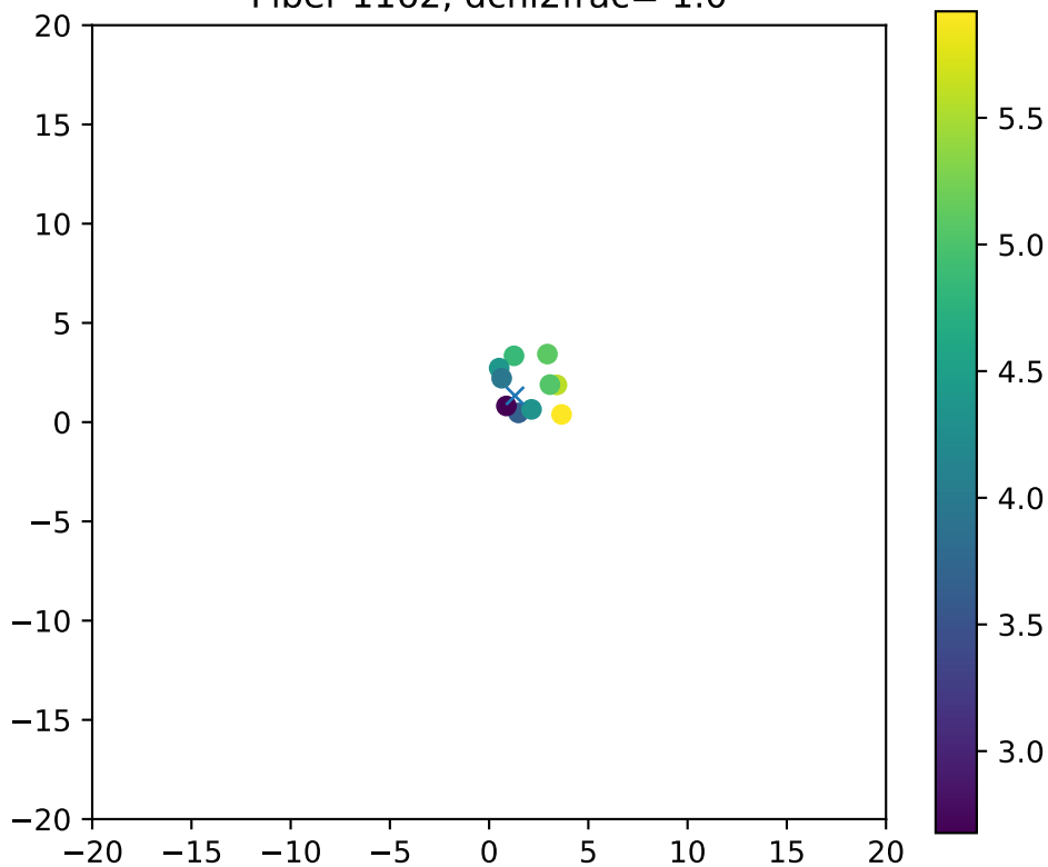
Fiber 1162, dchi2frac= 1.0
