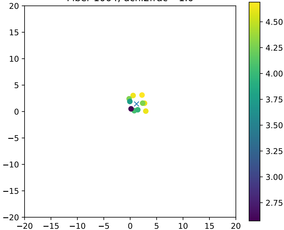
Fiber 1064, dchi2frac= 1.0
