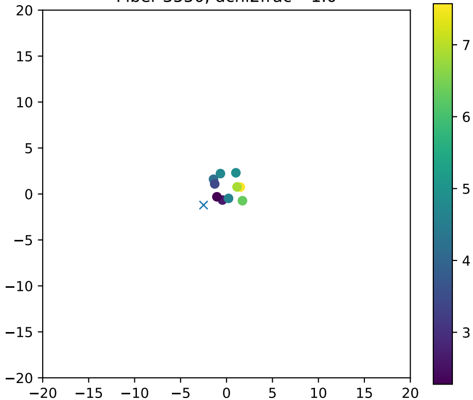
Fiber 3550, dchi2frac= 1.0
