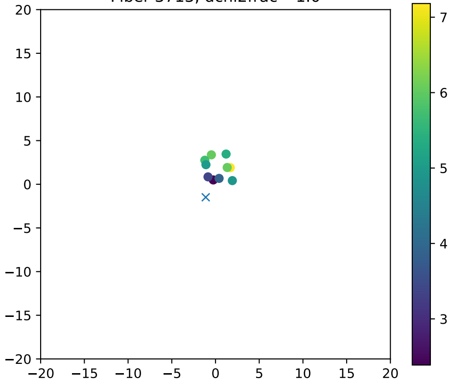
Fiber 3713, dchi2frac= 1.0
