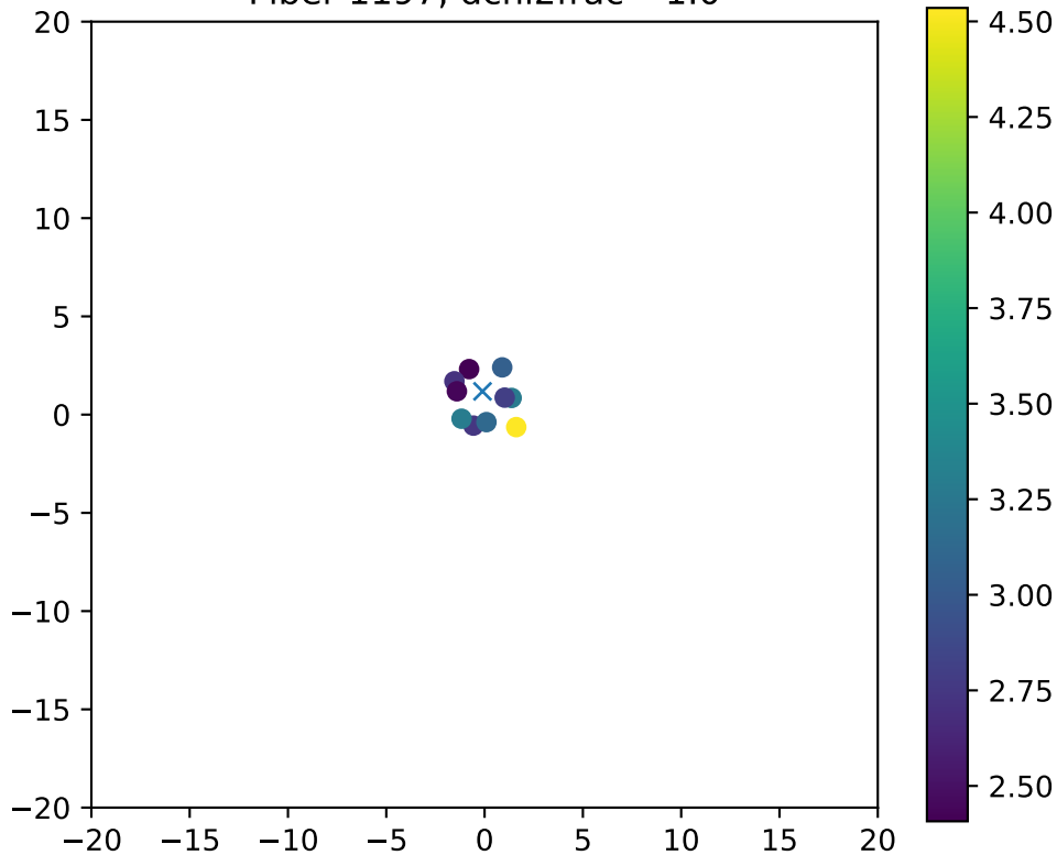
Fiber 1197, dchi2frac= 1.0
