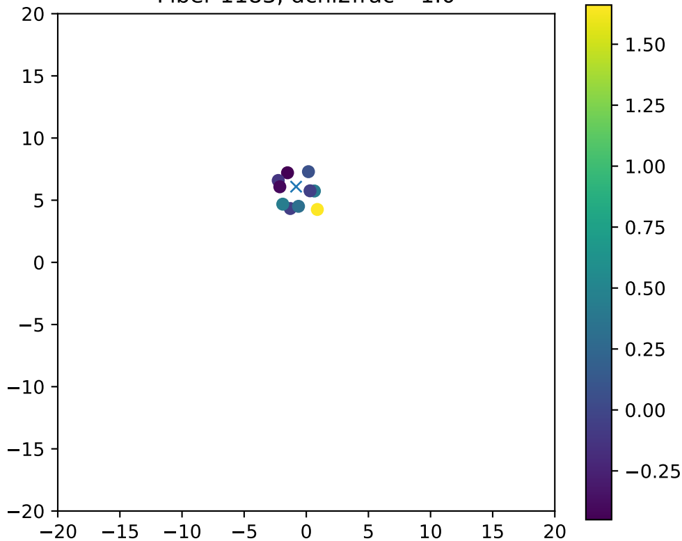
Fiber 1183, dchi2frac= 1.0
