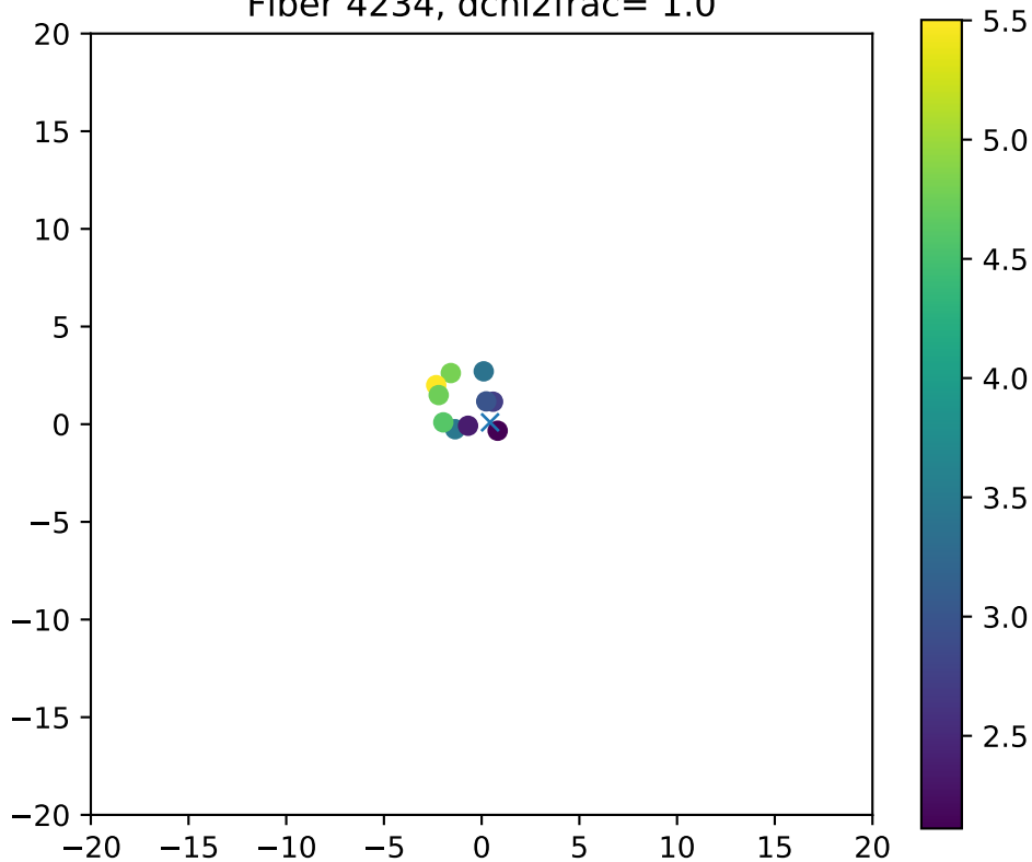
Fiber 4234, dchi2frac= 1.0
