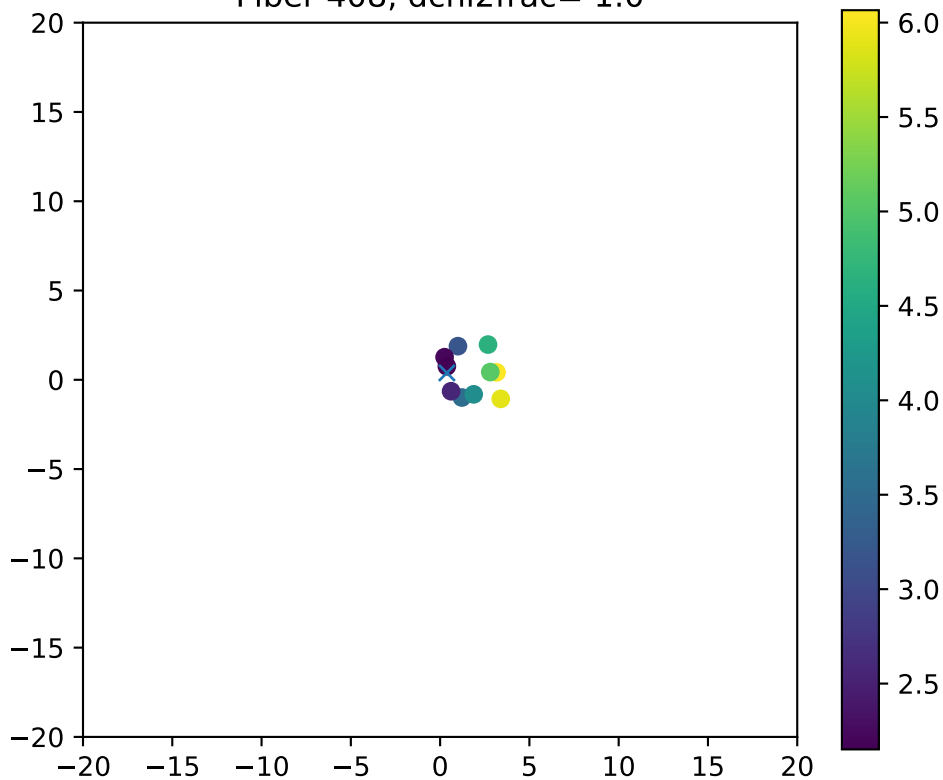
Fiber 408, dchi2frac= 1.0
