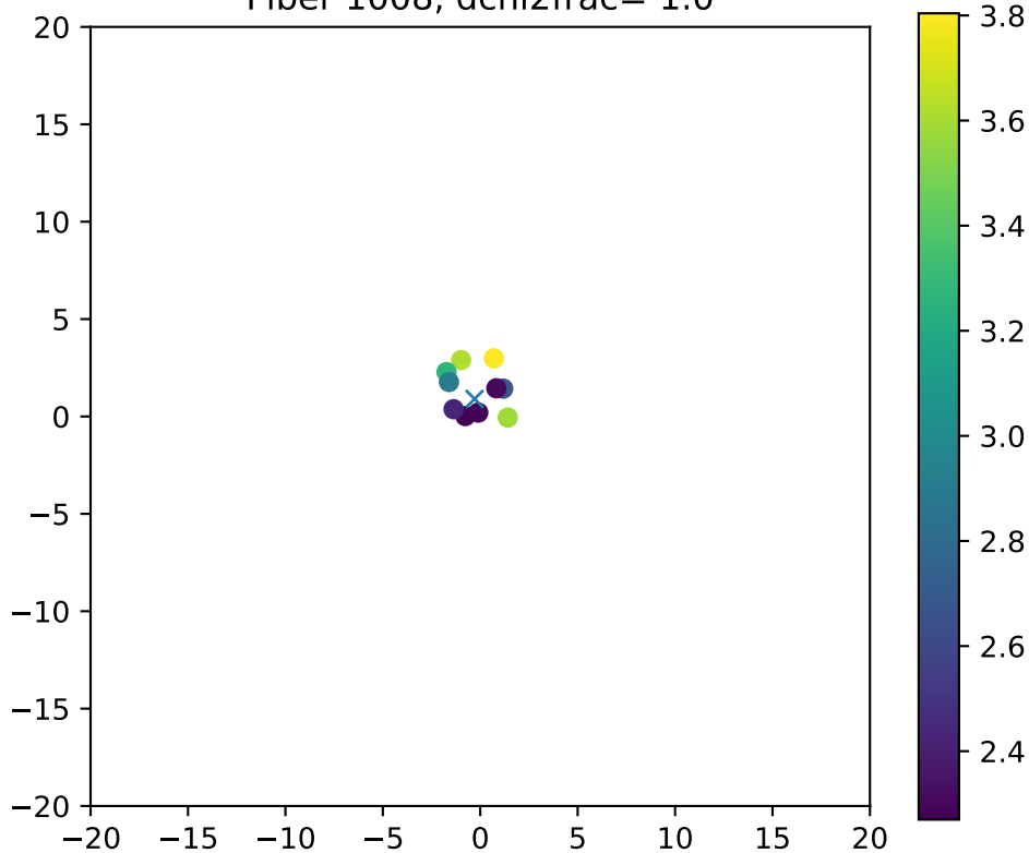
Fiber 1008, dchi2frac= 1.0
