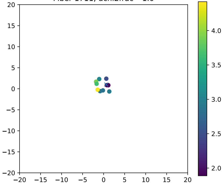
Fiber 1711, dchi2frac= 1.0
