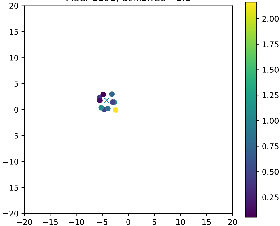
Fiber 1191, dchi2frac= 1.0
