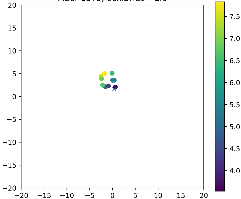
Fiber 1575, dchi2frac= 1.0
