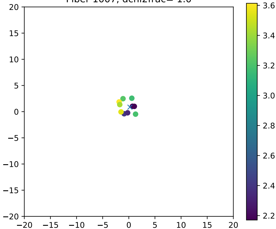
Fiber 1007, dchi2frac= 1.0
