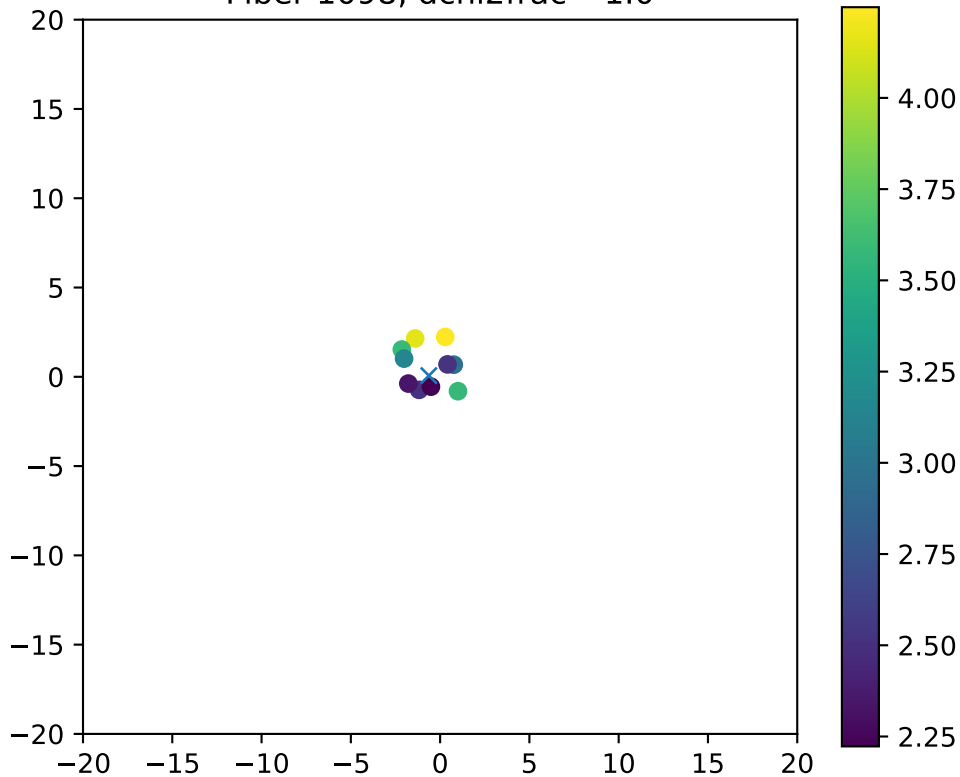
Fiber 1098, dchi2frac= 1.0
