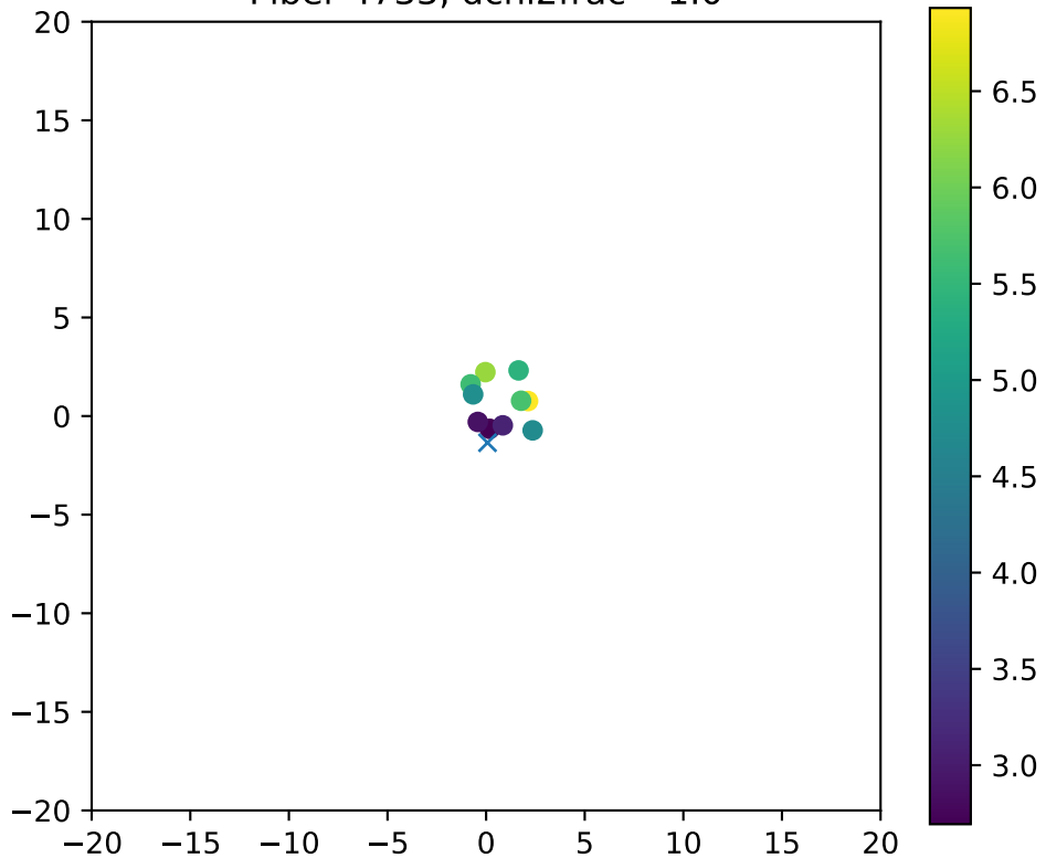
Fiber 4733, dchi2frac= 1.0
