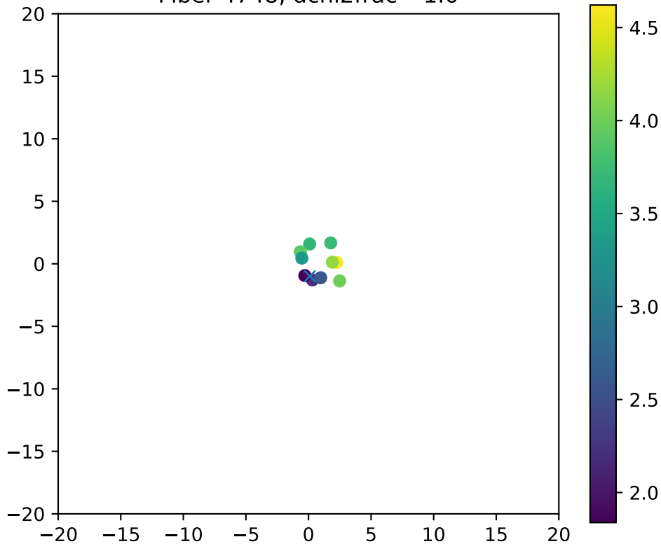
Fiber 4748, dchi2frac= 1.0
