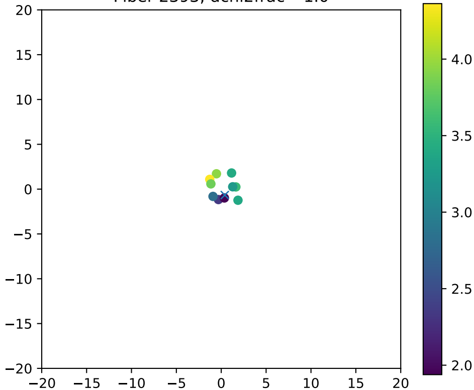
Fiber 2393, dchi2frac= 1.0
