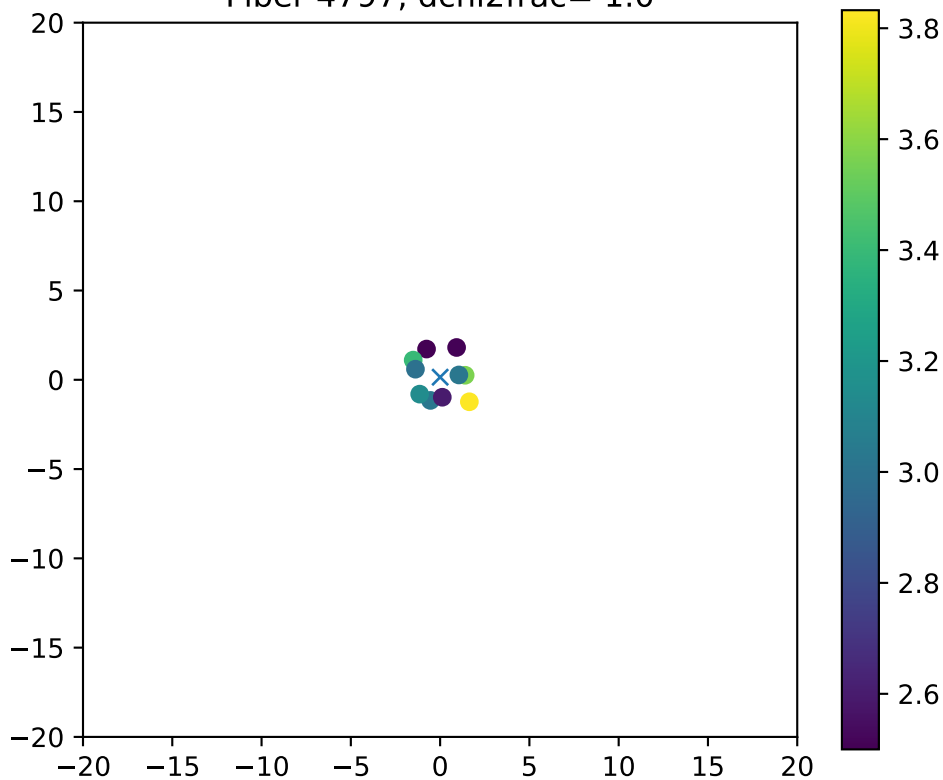
Fiber 4797, dchi2frac= 1.0
