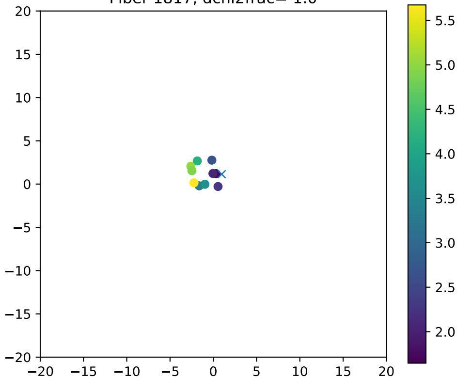
Fiber 1817, dchi2frac= 1.0
