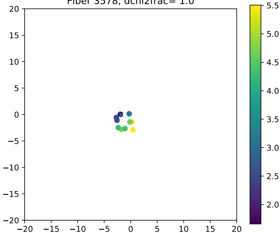
Fiber 3578, dchi2frac= 1.0
