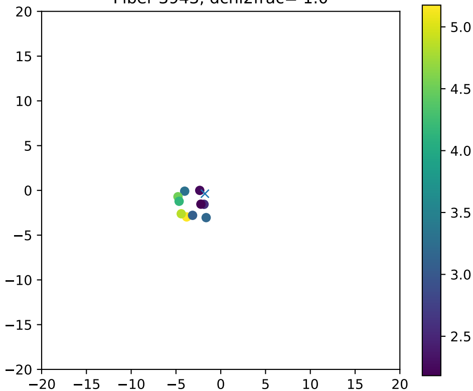
Fiber 3943, dchi2frac= 1.0
