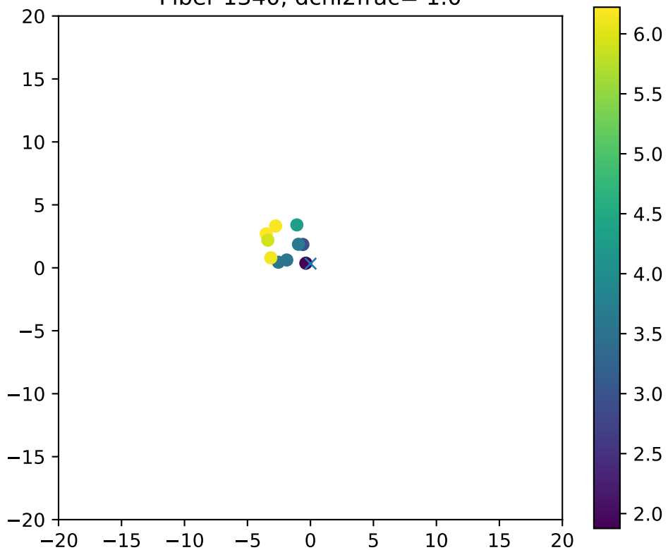
Fiber 1340, dchi2frac= 1.0
