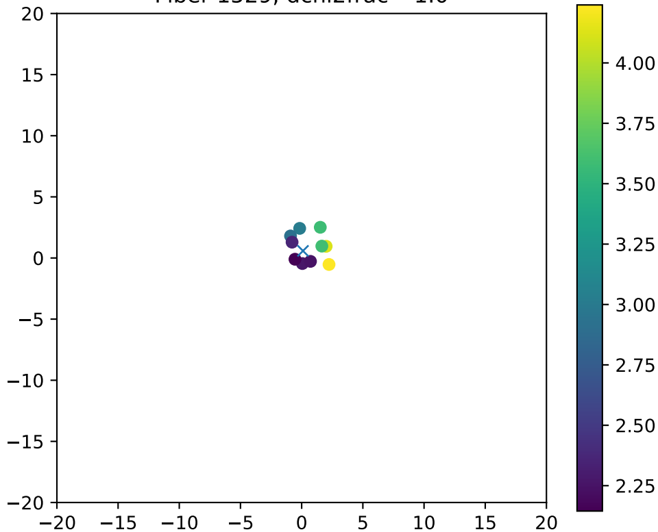
Fiber 1529, dchi2frac= 1.0
