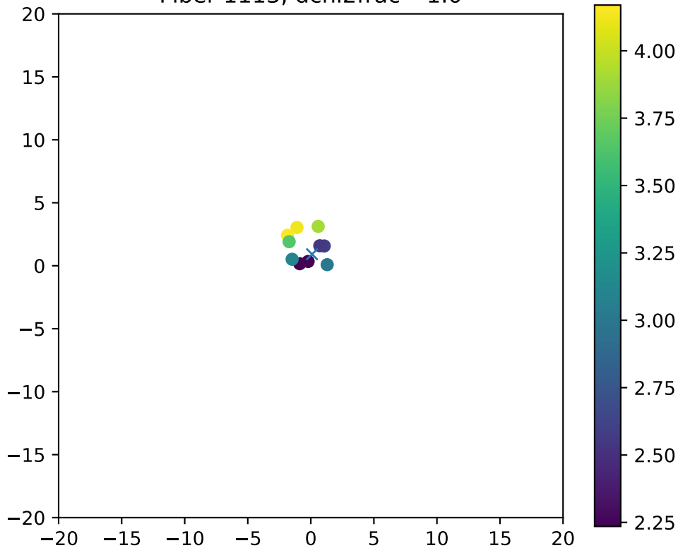
Fiber 1113, dchi2frac= 1.0
