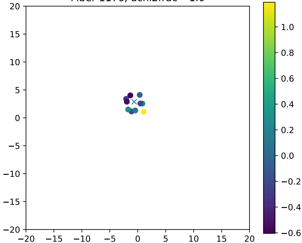
Fiber 1176, dchi2frac= 1.0
