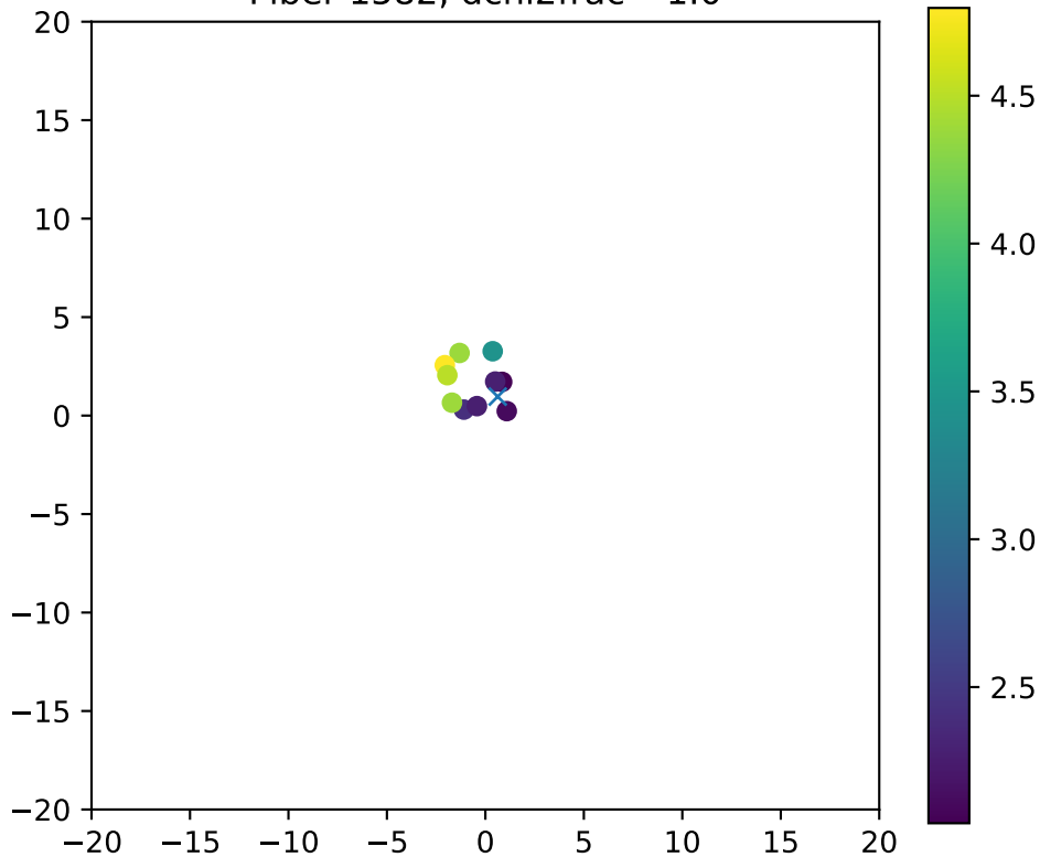
Fiber 1582, dchi2frac= 1.0
