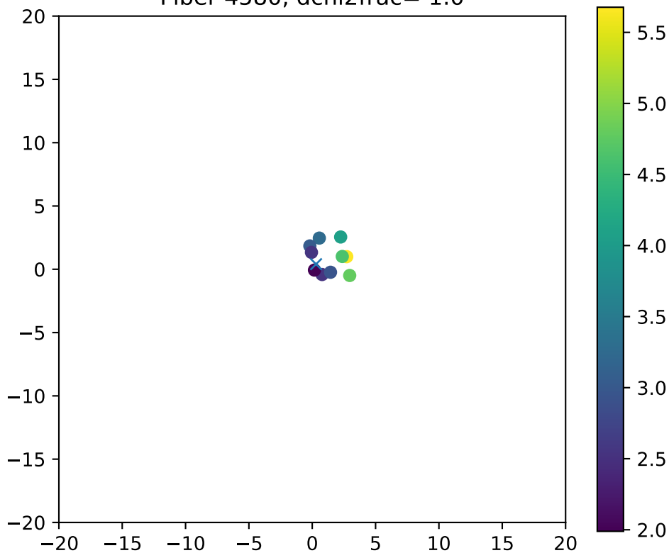
Fiber 4580, dchi2frac= 1.0
