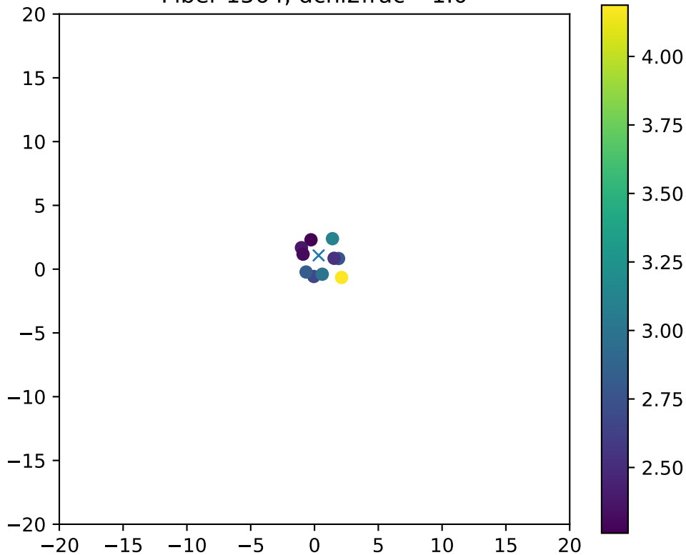
Fiber 1564, dchi2frac= 1.0
