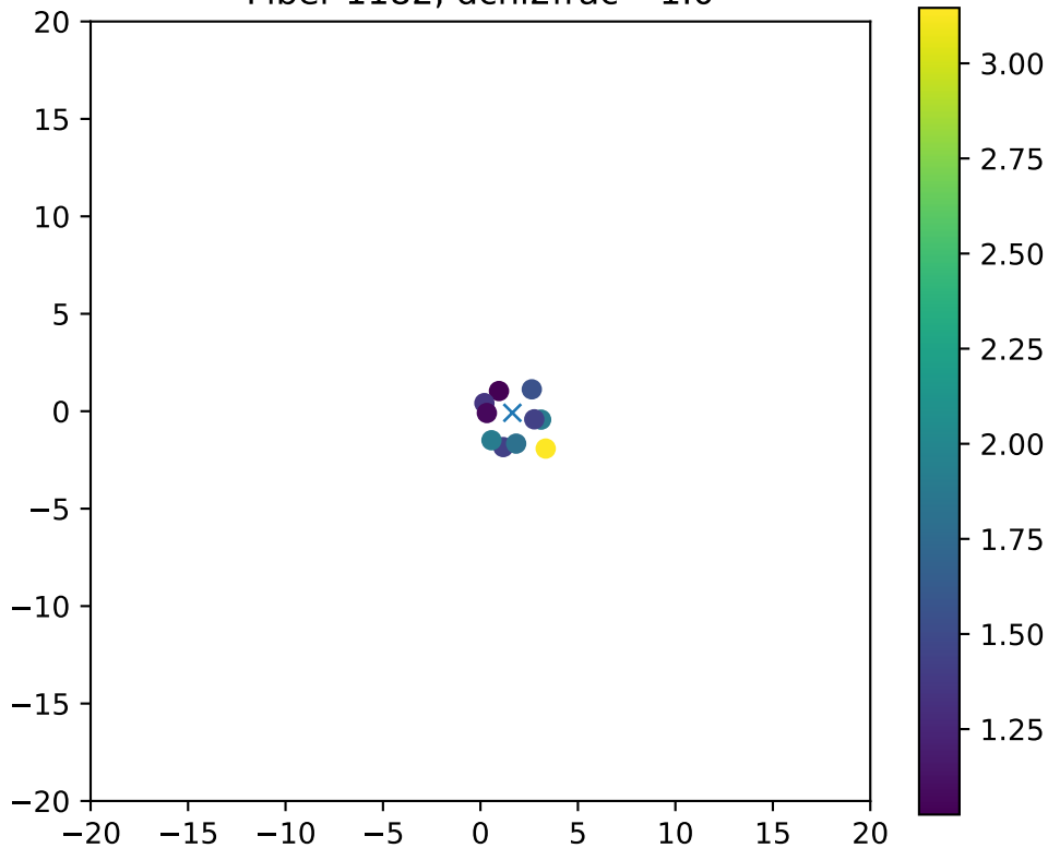
Fiber 1182, dchi2frac= 1.0
