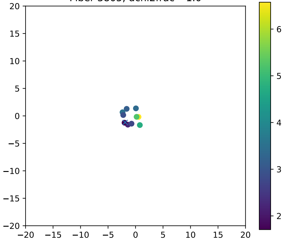
Fiber 3805, dchi2frac= 1.0
