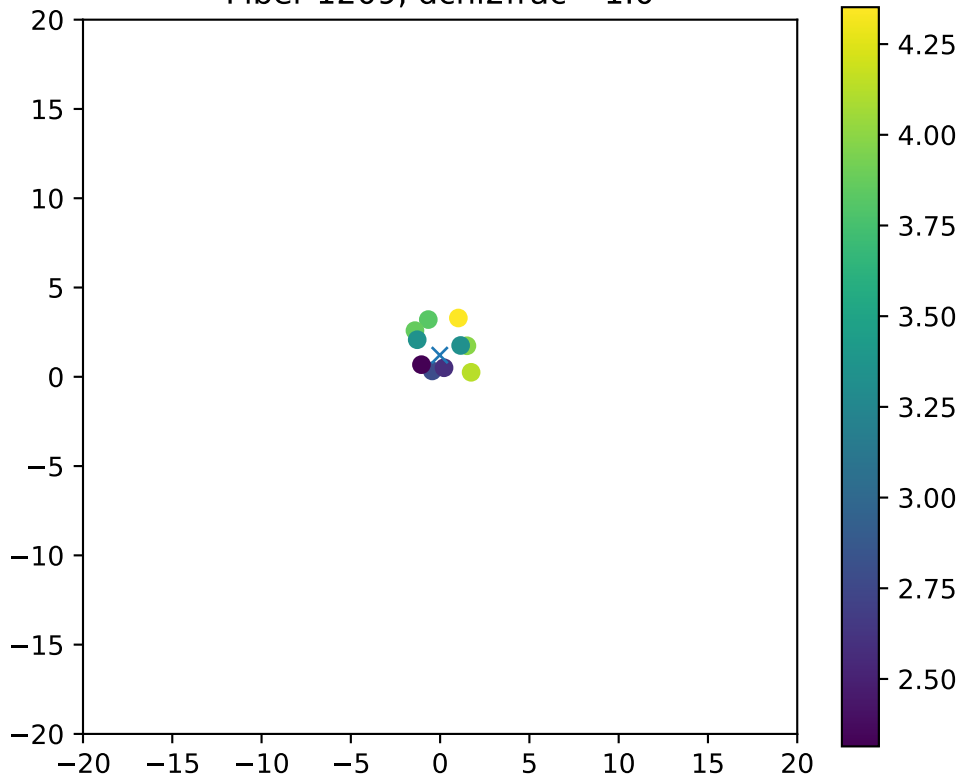
Fiber 1209, dchi2frac= 1.0
