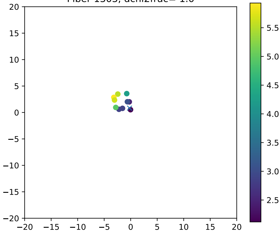
Fiber 1303, dchi2frac= 1.0
