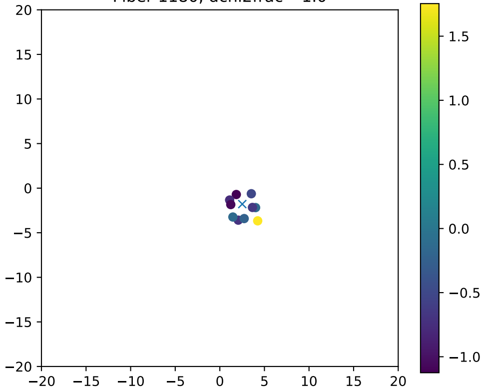
Fiber 1180, dchi2frac= 1.0
