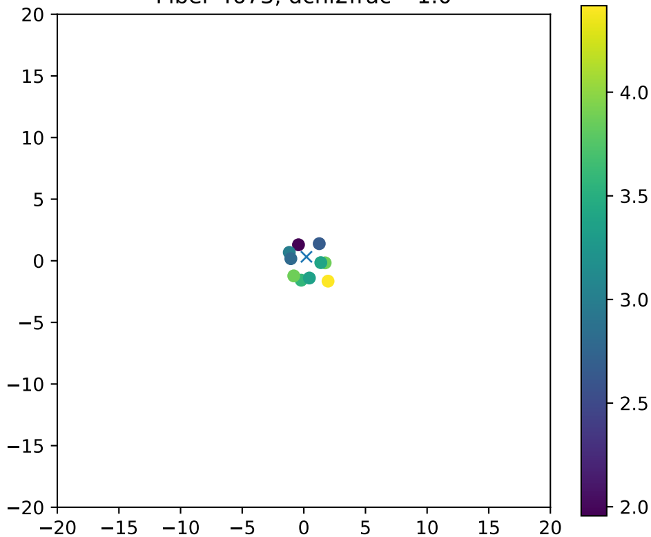
Fiber 4673, dchi2frac= 1.0
