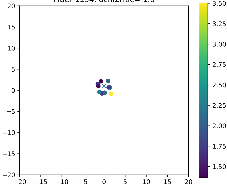
Fiber 1194, dchi2frac= 1.0
