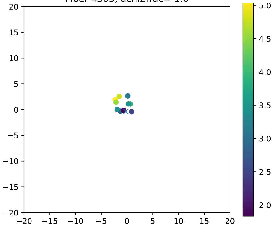
Fiber 4305, dchi2frac= 1.0
