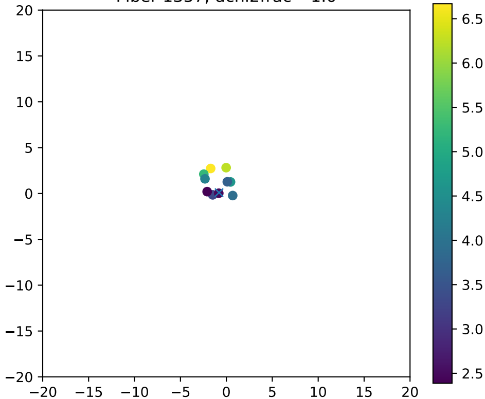
Fiber 1357, dchi2frac= 1.0
