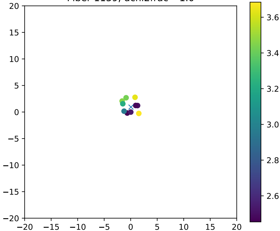
Fiber 1139, dchi2frac= 1.0
