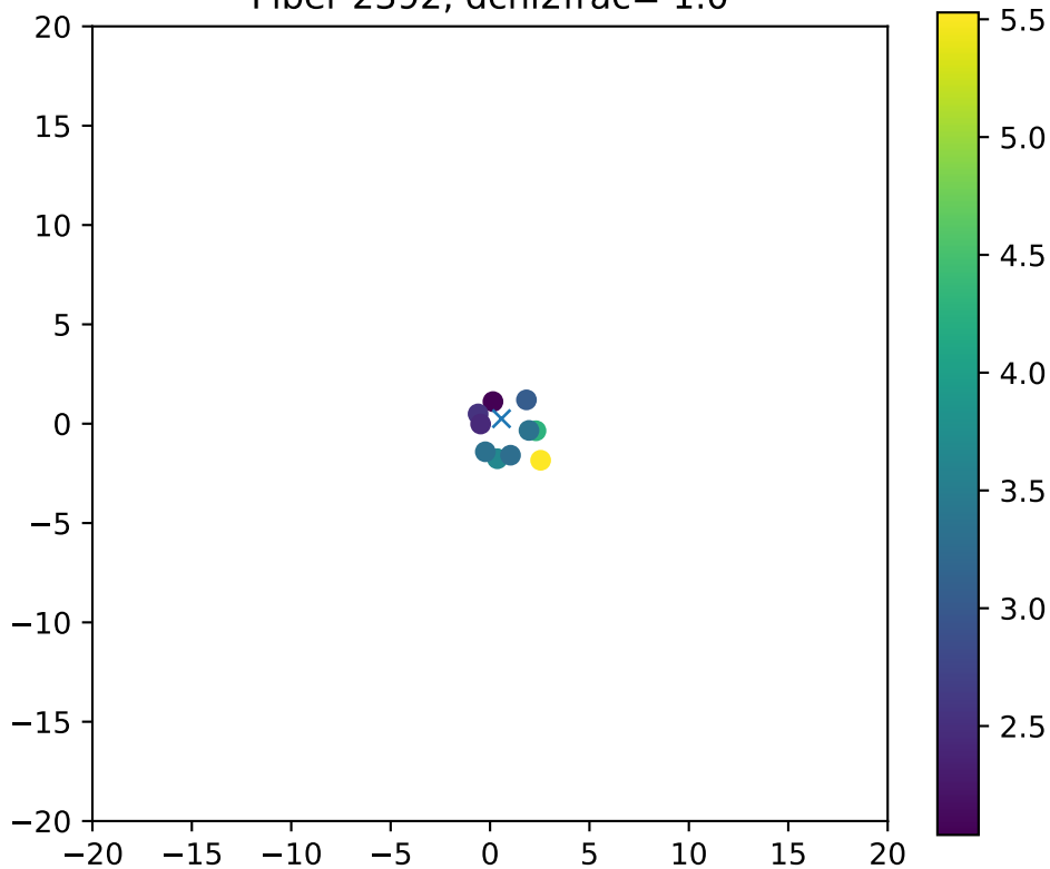
Fiber 2392, dchi2frac= 1.0
