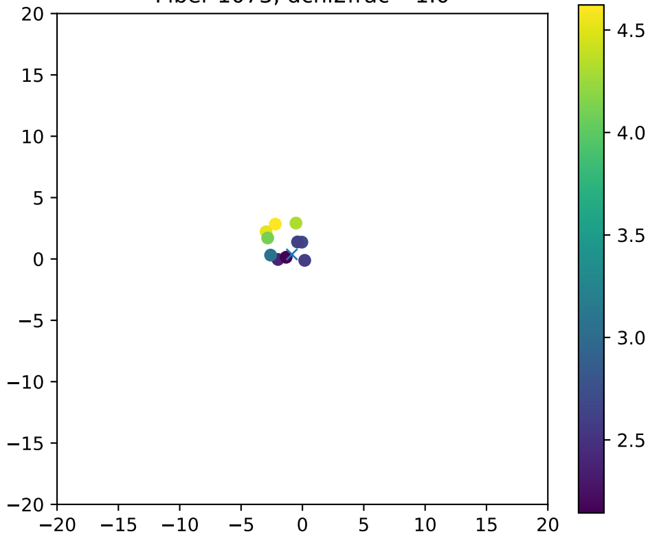
Fiber 1073, dchi2frac= 1.0
