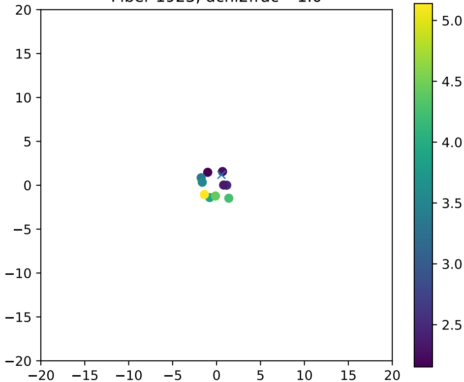
Fiber 1923, dchi2frac= 1.0
