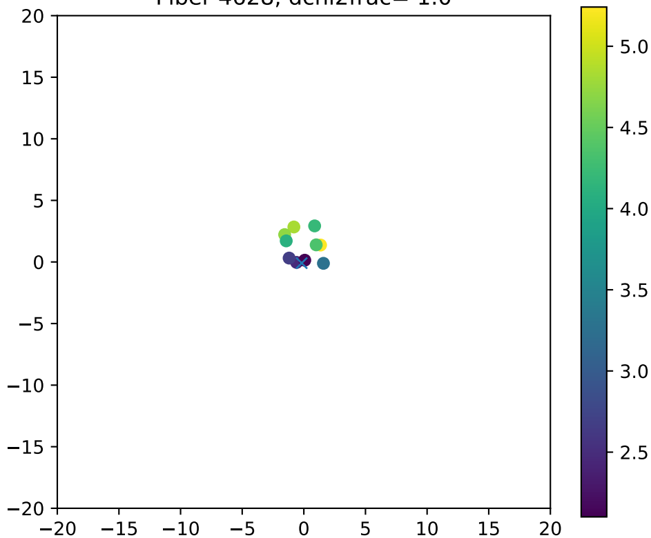
Fiber 4628, dchi2frac= 1.0
