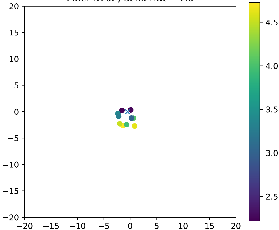
Fiber 3702, dchi2frac= 1.0
