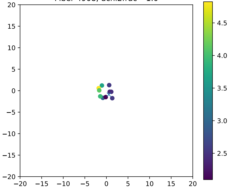
Fiber 4908, dchi2frac= 1.0
