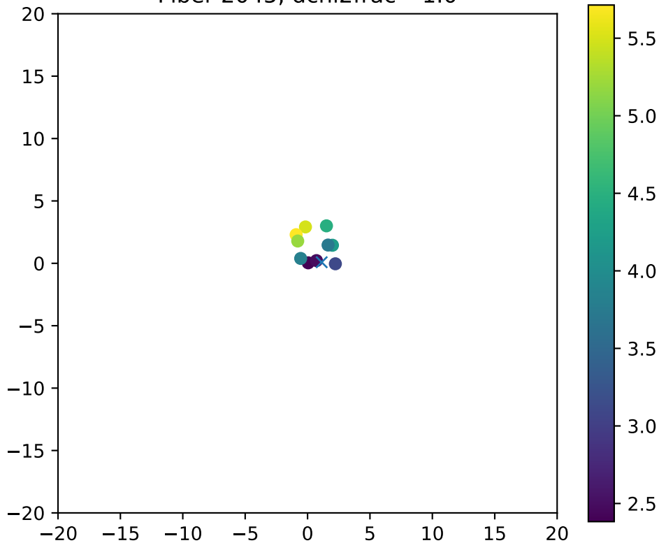
Fiber 2045, dchi2frac= 1.0
