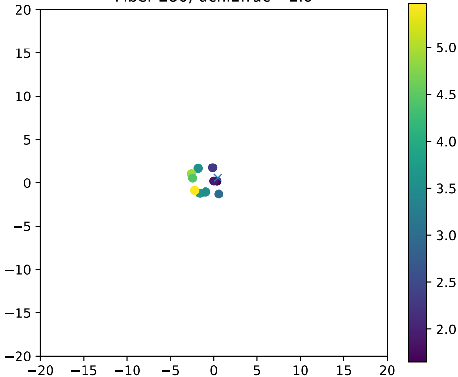
Fiber 280, dchi2frac= 1.0
