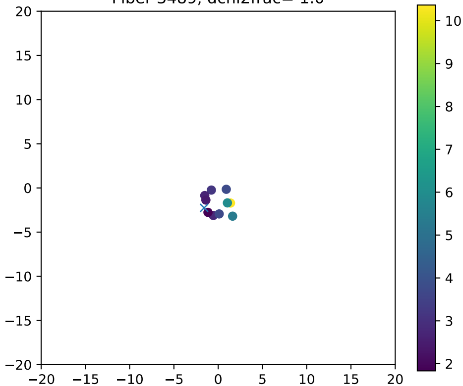
Fiber 3489, dchi2frac= 1.0
