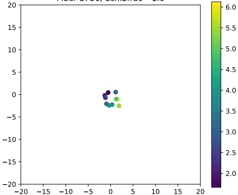
Fiber 3736, dchi2frac= 1.0
