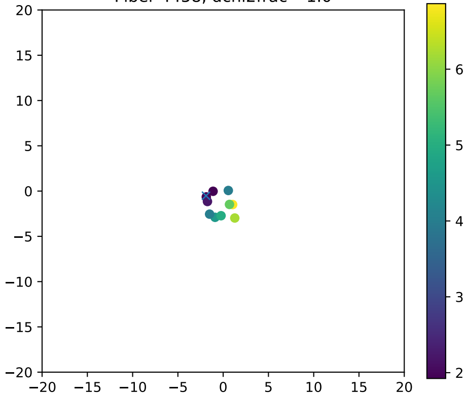
Fiber 4458, dchi2frac= 1.0
