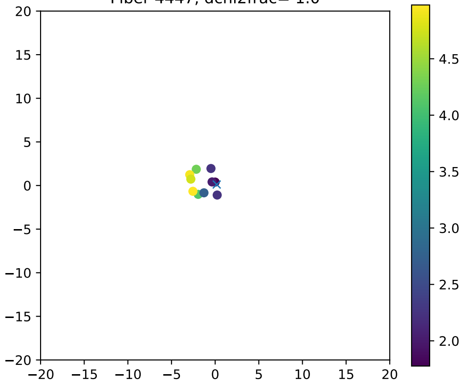
Fiber 4447, dchi2frac= 1.0
