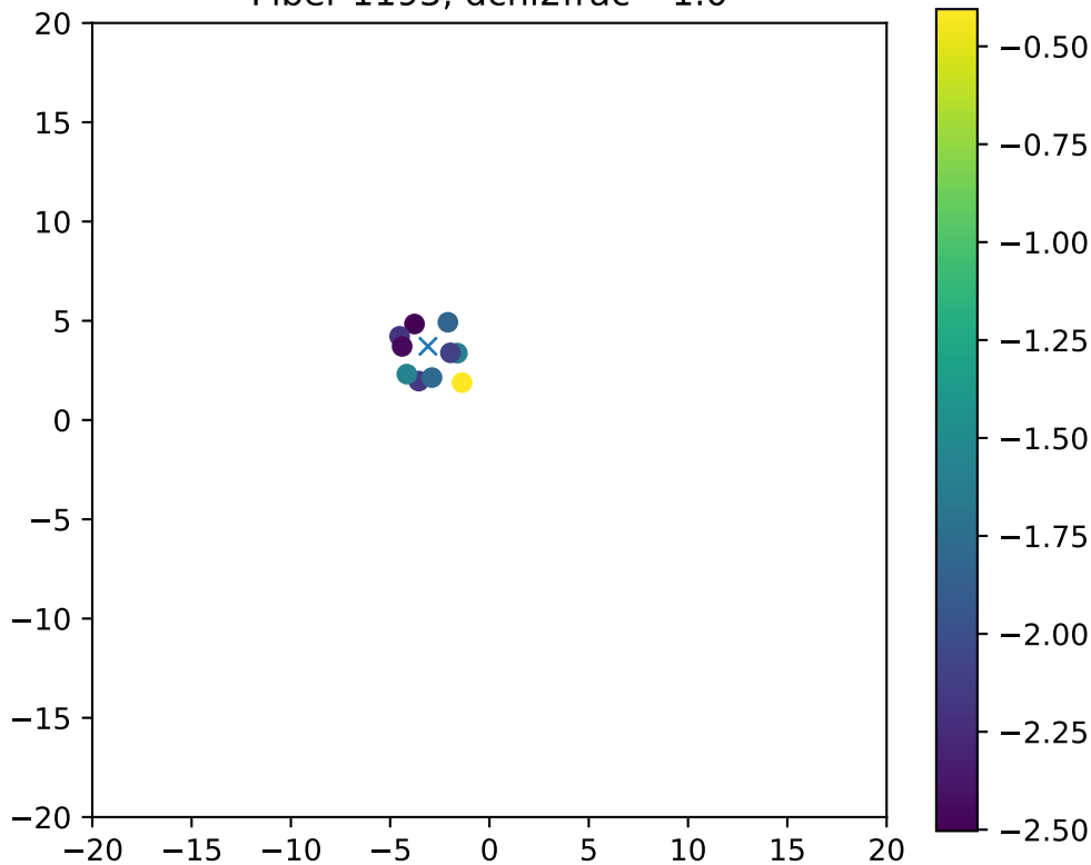
Fiber 1193, dchi2frac= 1.0
