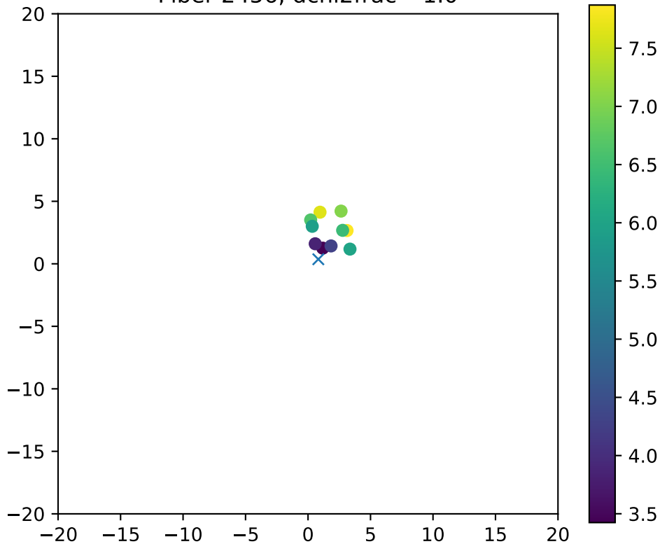
Fiber 2456, dchi2frac= 1.0
