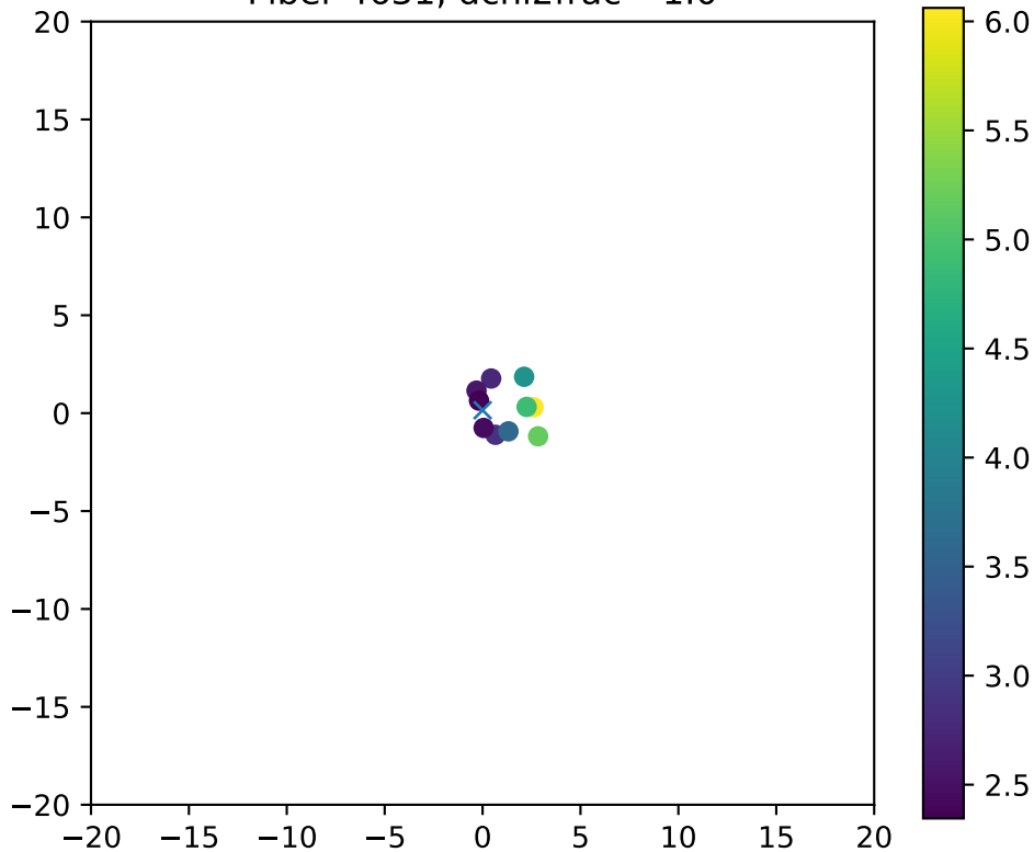
Fiber 4631, dchi2frac= 1.0
