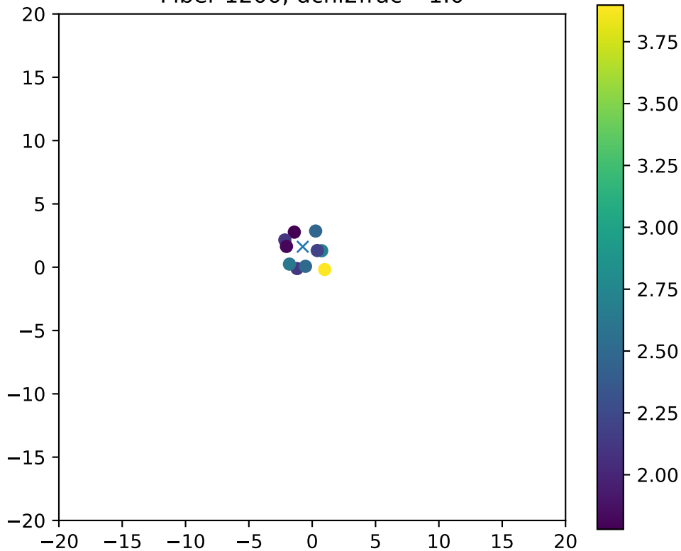
Fiber 1200, dchi2frac= 1.0
