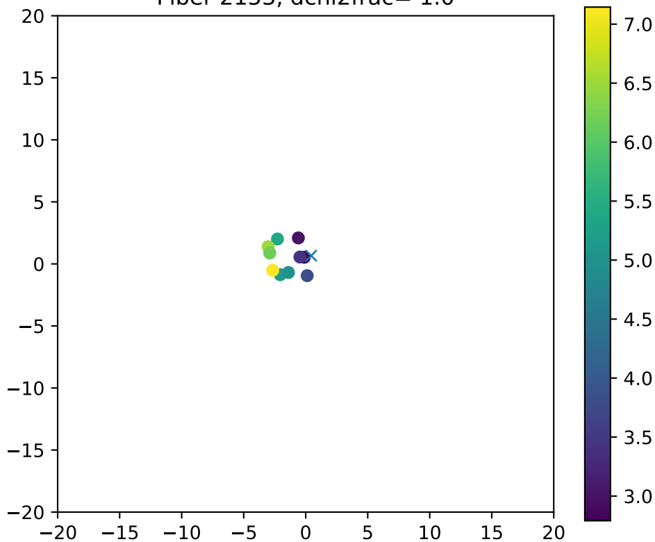
Fiber 2153, dchi2frac= 1.0
