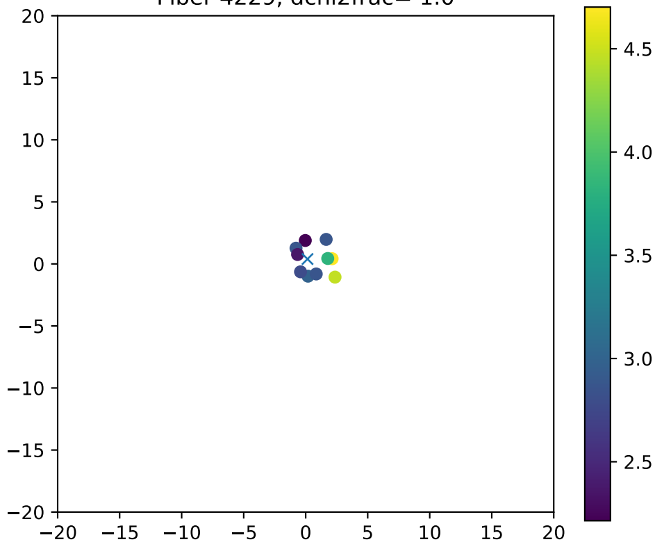
Fiber 4229, dchi2frac= 1.0
