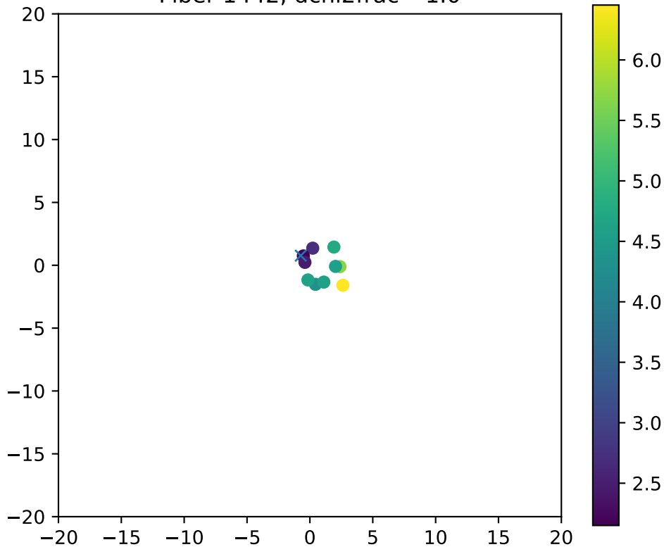
Fiber 1442, dchi2frac= 1.0
