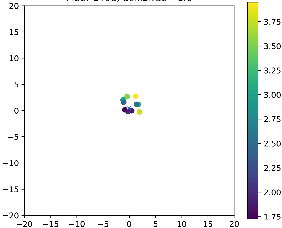
Fiber 1498, dchi2frac= 1.0
