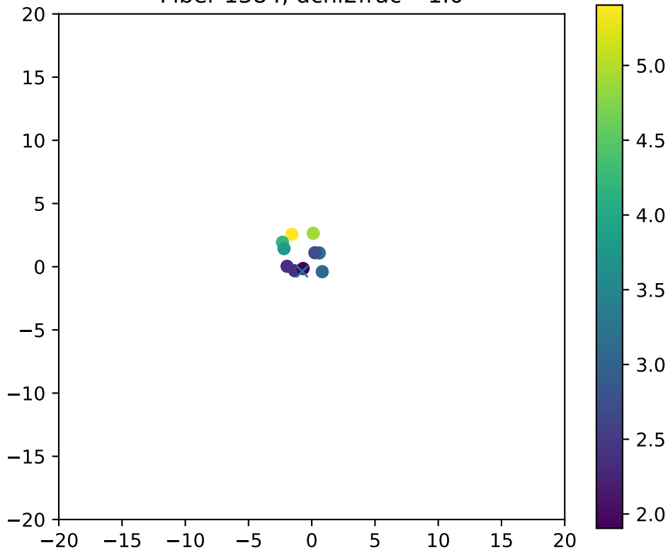
Fiber 1384, dchi2frac= 1.0
