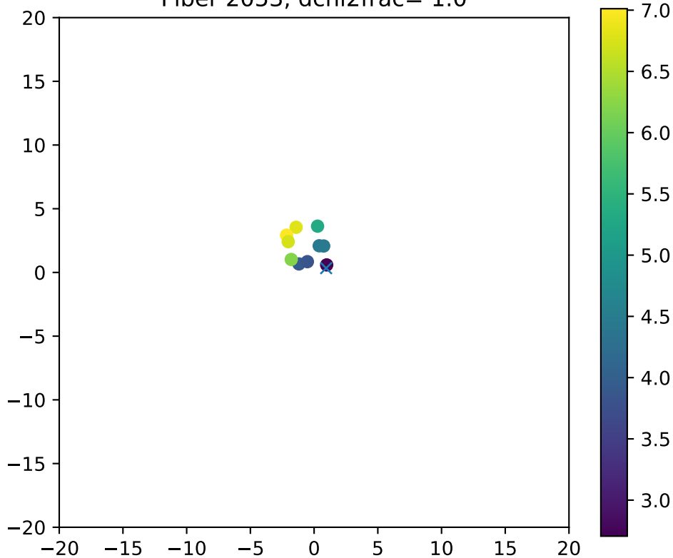
Fiber 2053, dchi2frac= 1.0
