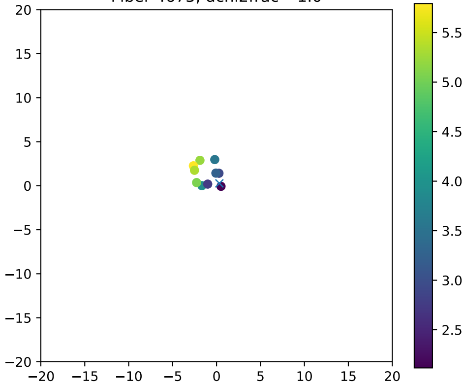
Fiber 4675, dchi2frac= 1.0
