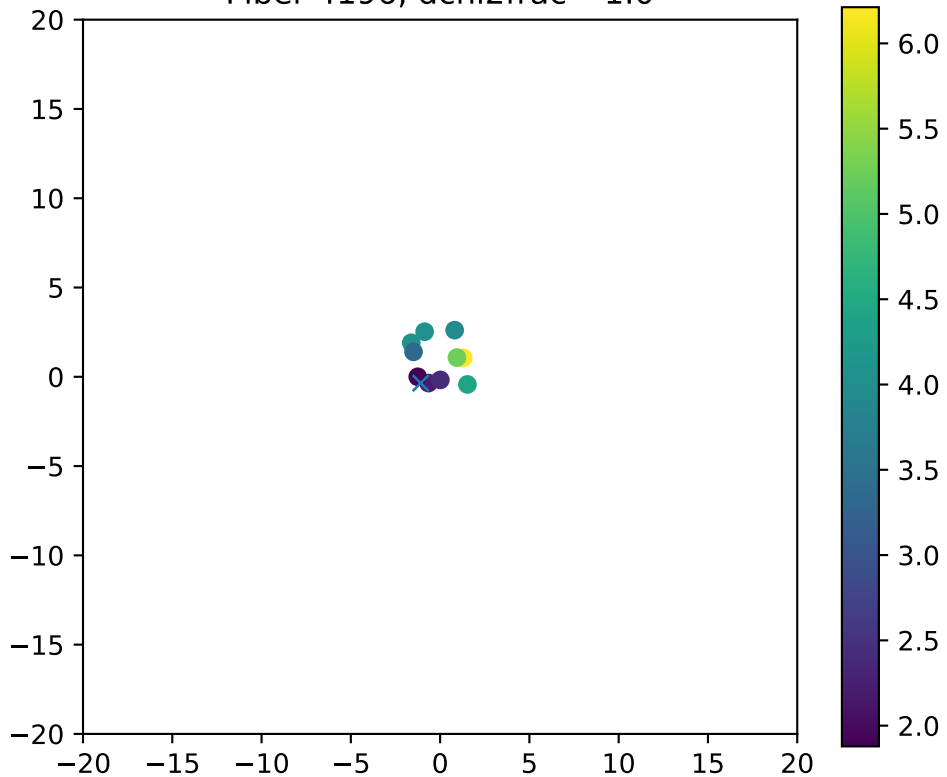
Fiber 4196, dchi2frac= 1.0
