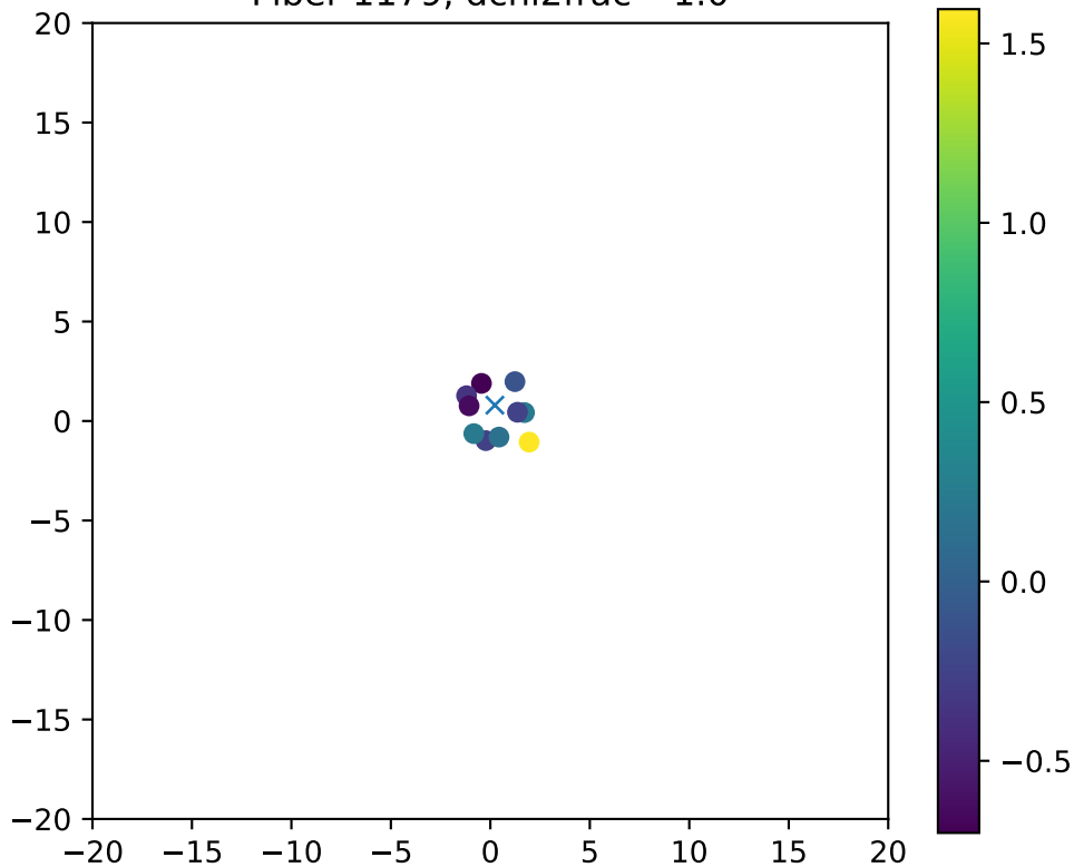
Fiber 1179, dchi2frac= 1.0
