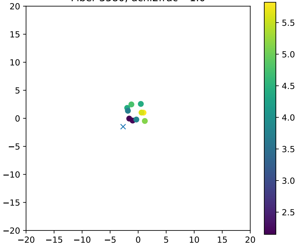
Fiber 3580, dchi2frac= 1.0
