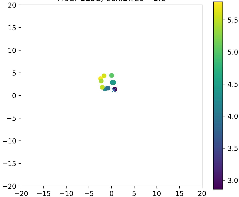
Fiber 1158, dchi2frac= 1.0
