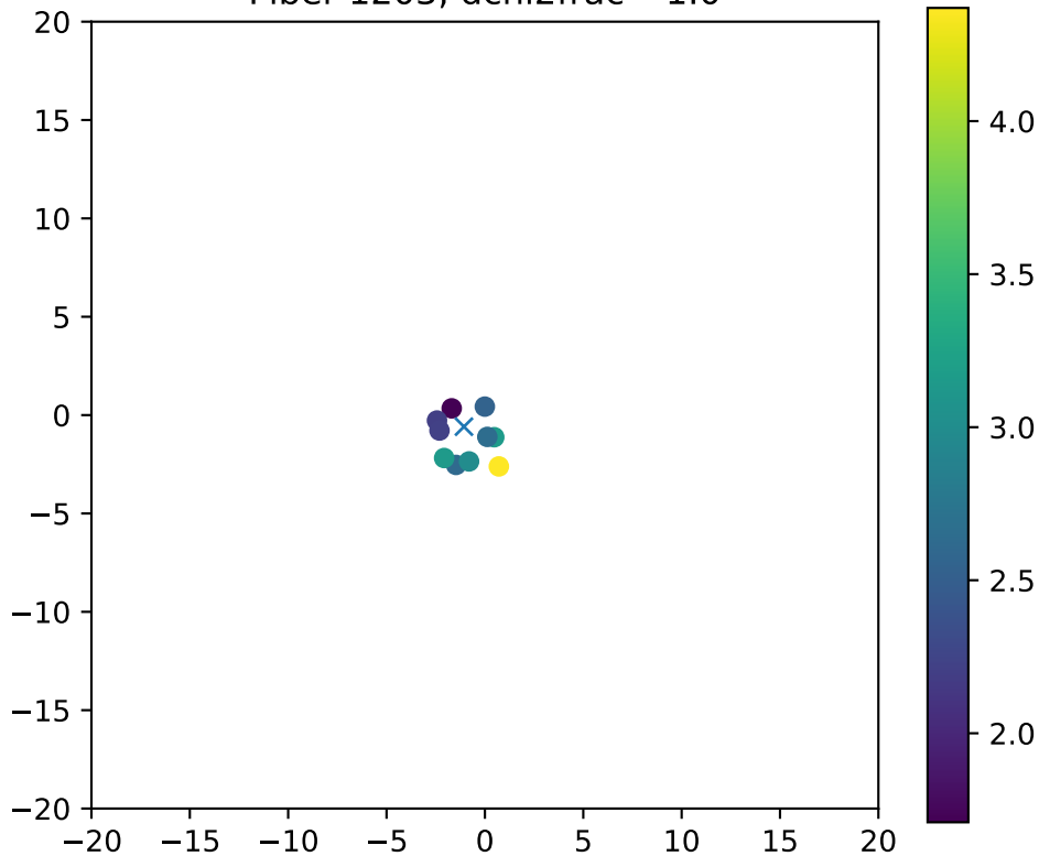
Fiber 1203, dchi2frac= 1.0
