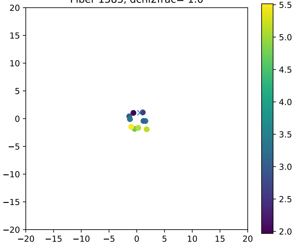
Fiber 1583, dchi2frac= 1.0
