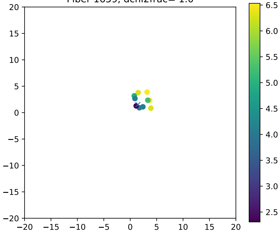
Fiber 1659, dchi2frac= 1.0
