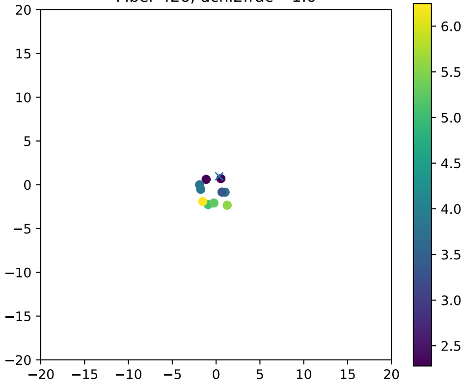
Fiber 426, dchi2frac= 1.0
