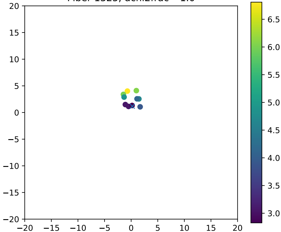
Fiber 1325, dchi2frac= 1.0
