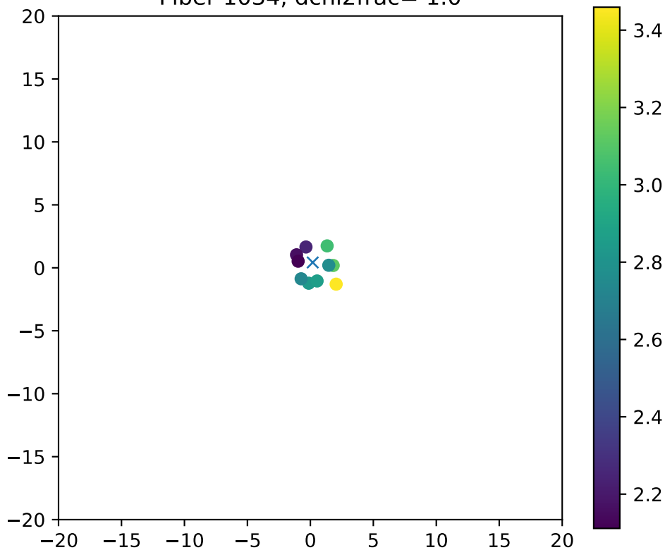
Fiber 1034, dchi2frac= 1.0
