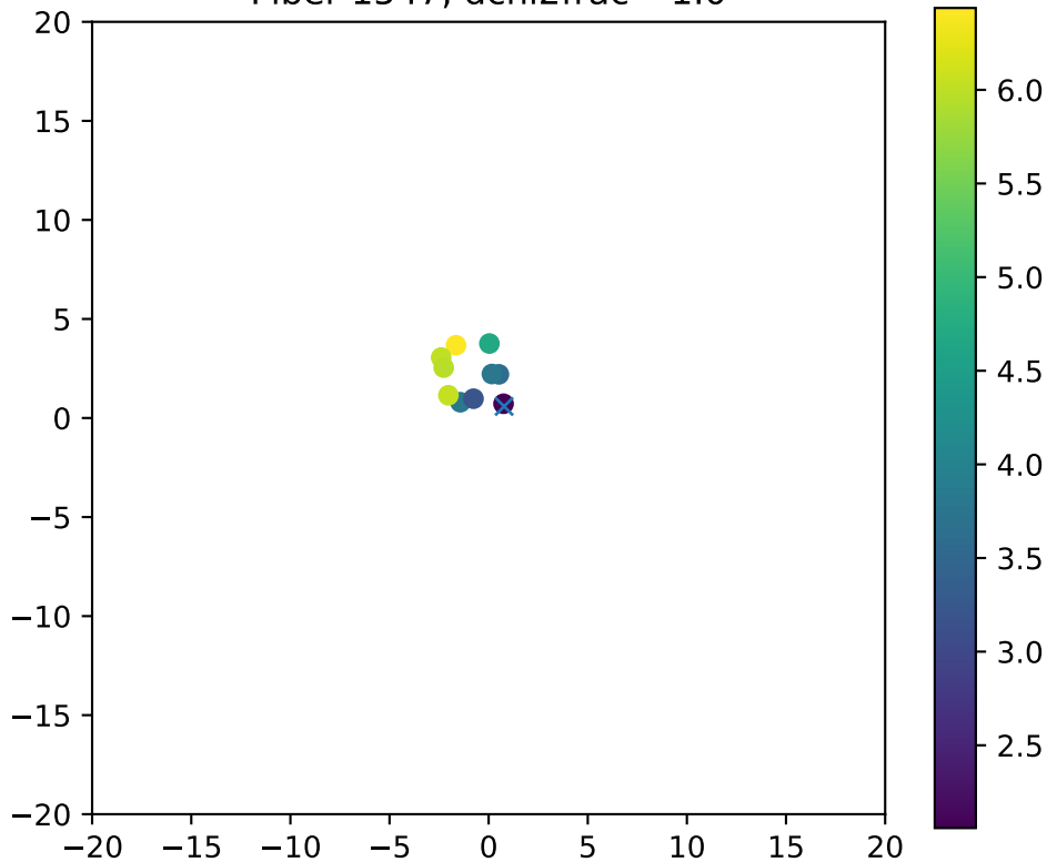
Fiber 1547, dchi2frac= 1.0
