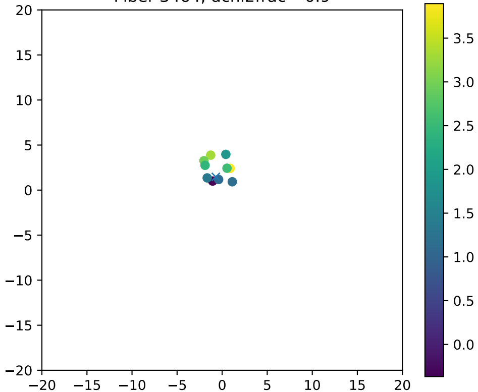
Fiber 3464, dchi2frac= 0.9
