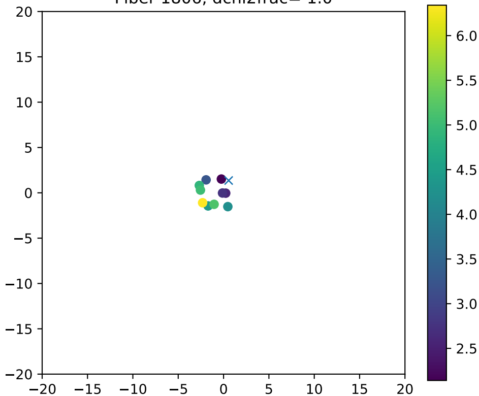
Fiber 1806, dchi2frac= 1.0
