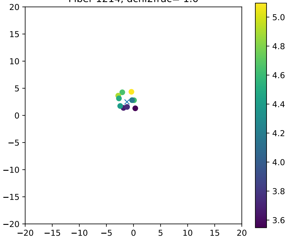
Fiber 1214, dchi2frac= 1.0
