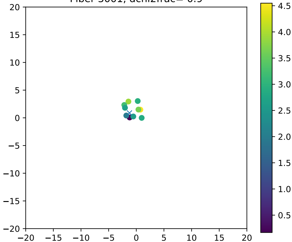
Fiber 3001, dchi2frac= 0.9
