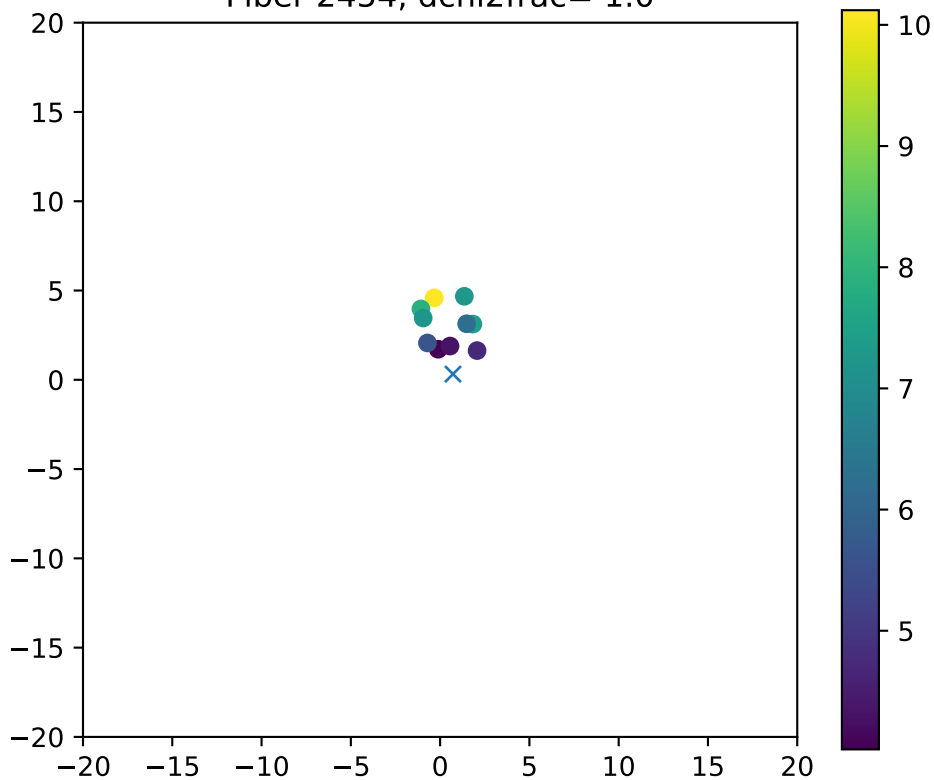
Fiber 2454, dchi2frac= 1.0
