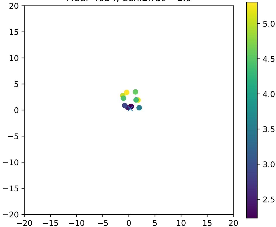
Fiber 4654, dchi2frac= 1.0
