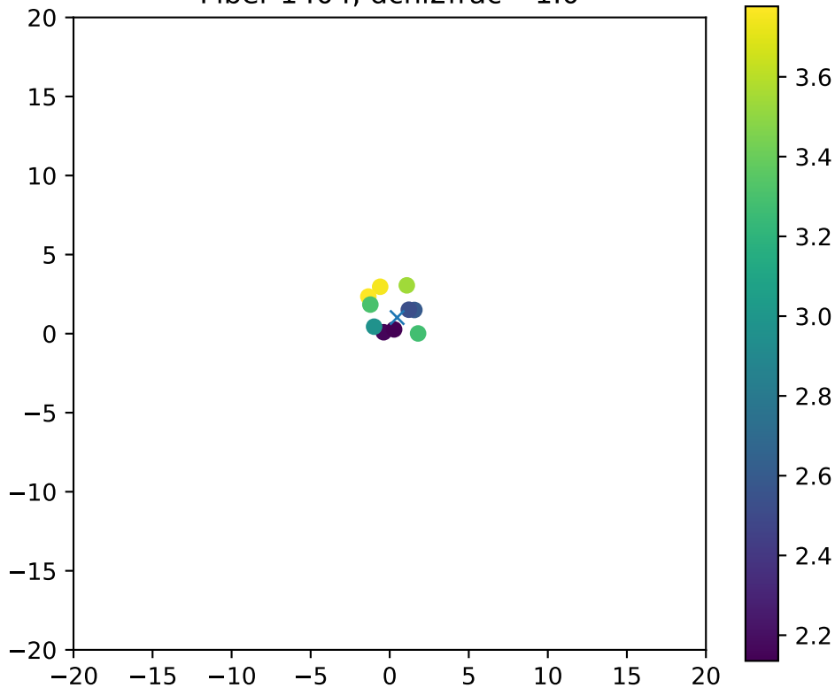
Fiber 1404, dchi2frac= 1.0
