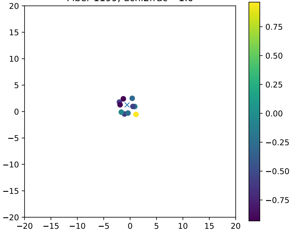
Fiber 1199, dchi2frac= 1.0
