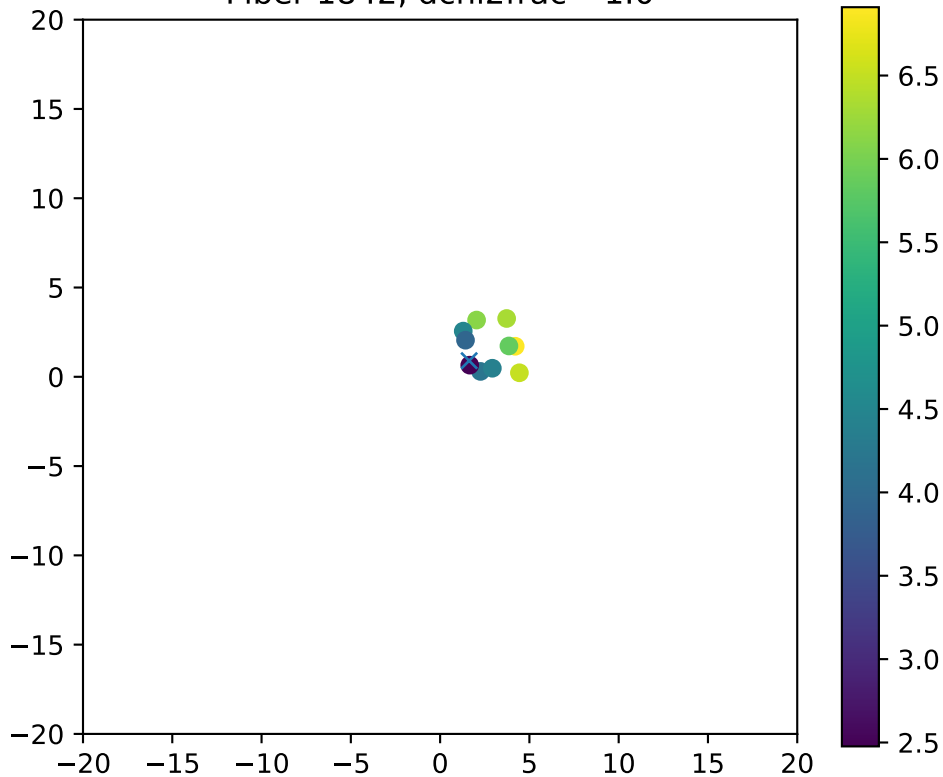
Fiber 1842, dchi2frac= 1.0
