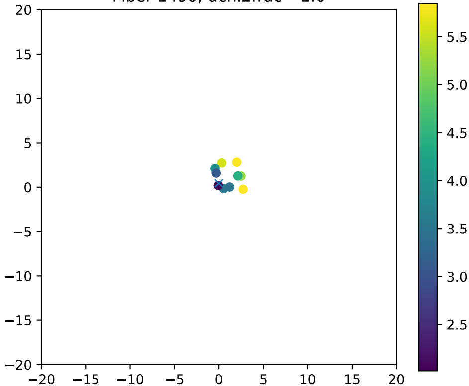
Fiber 1496, dchi2frac= 1.0
