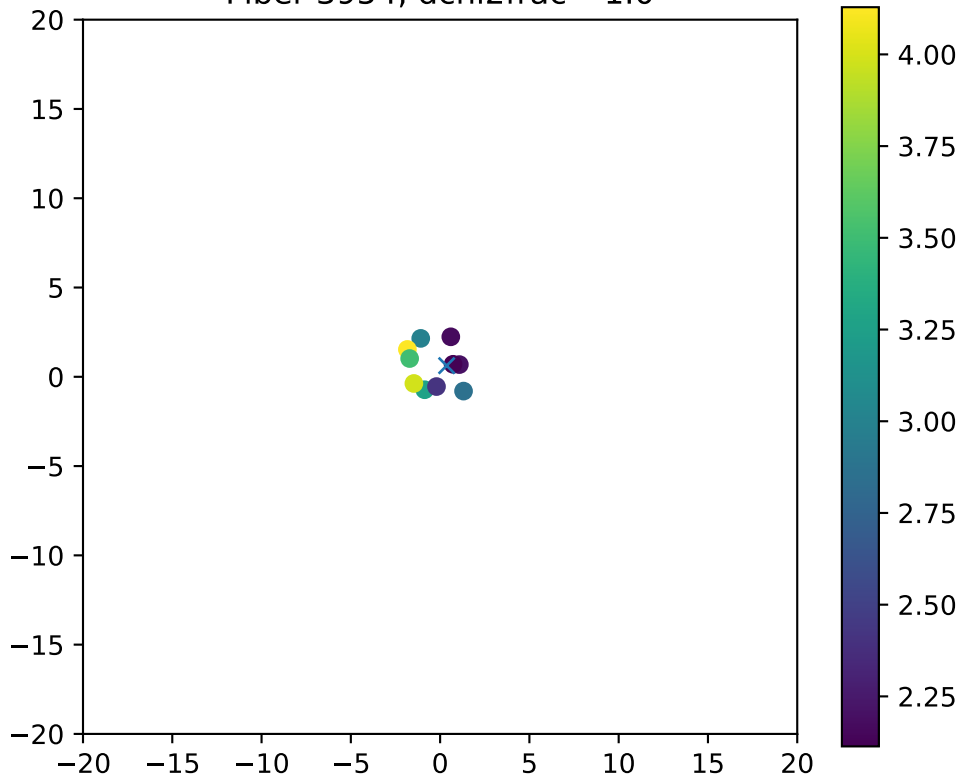
Fiber 3954, dchi2frac= 1.0
