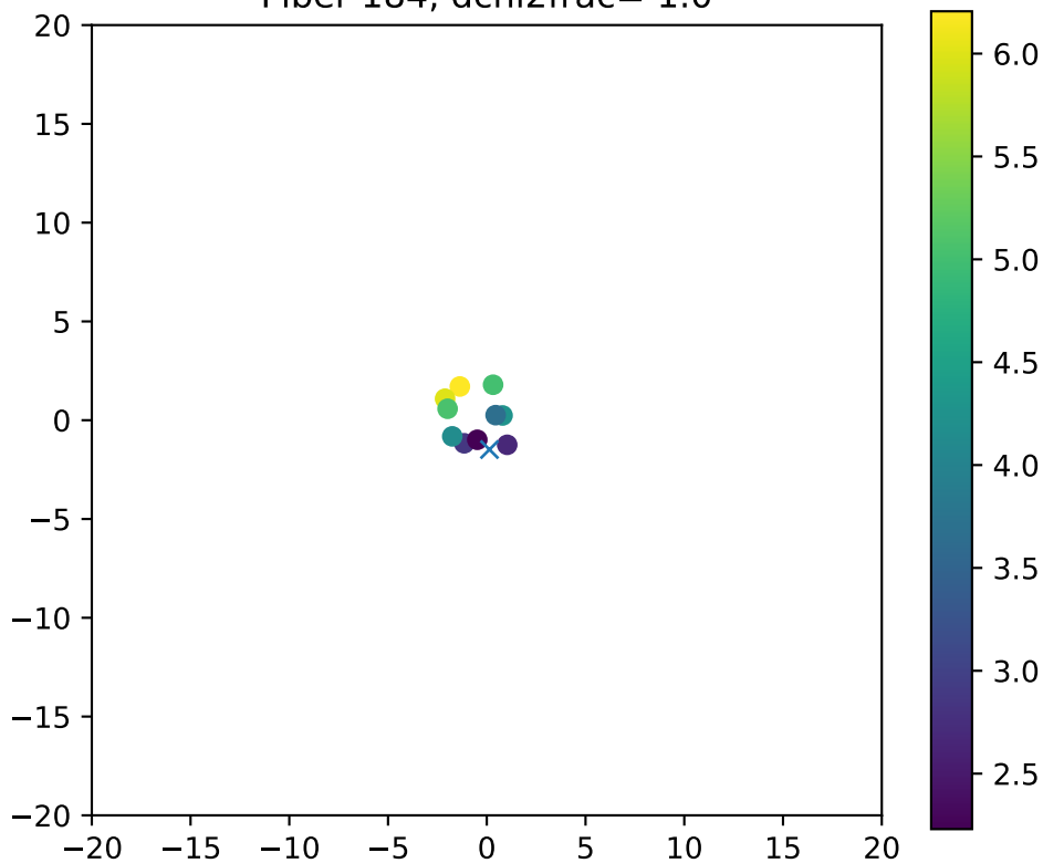
Fiber 184, dchi2frac= 1.0
