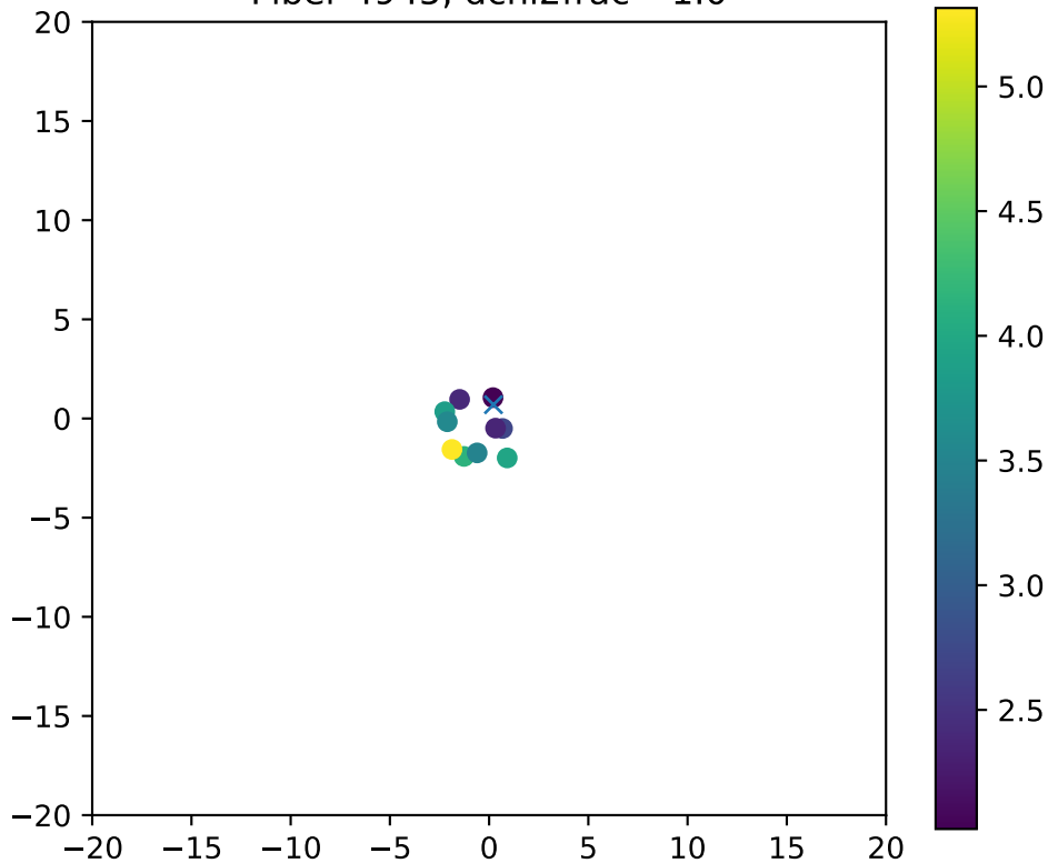
Fiber 4945, dchi2frac= 1.0
