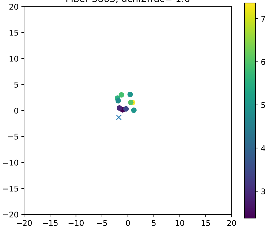
Fiber 3863, dchi2frac= 1.0
