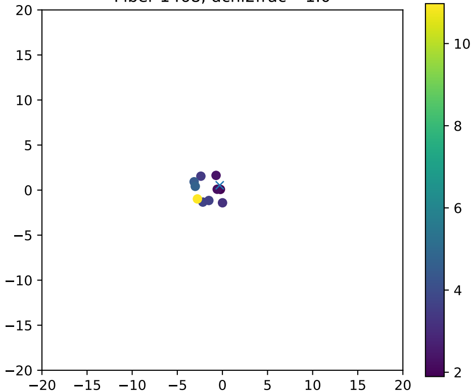
Fiber 1468, dchi2frac= 1.0
