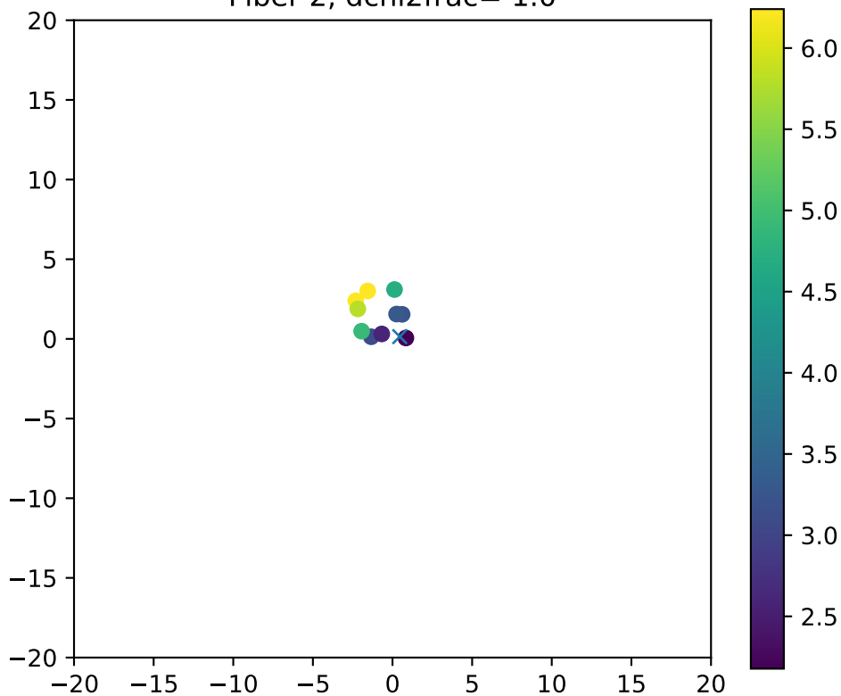
Fiber 2, dchi2frac= 1.0
