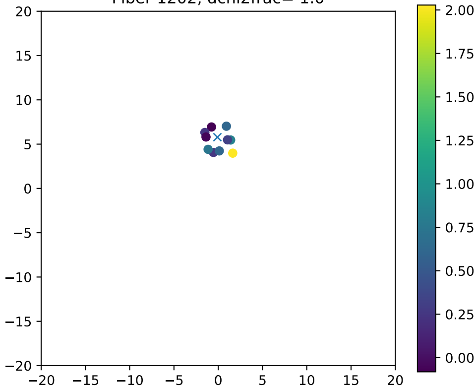
Fiber 1202, dchi2frac= 1.0
