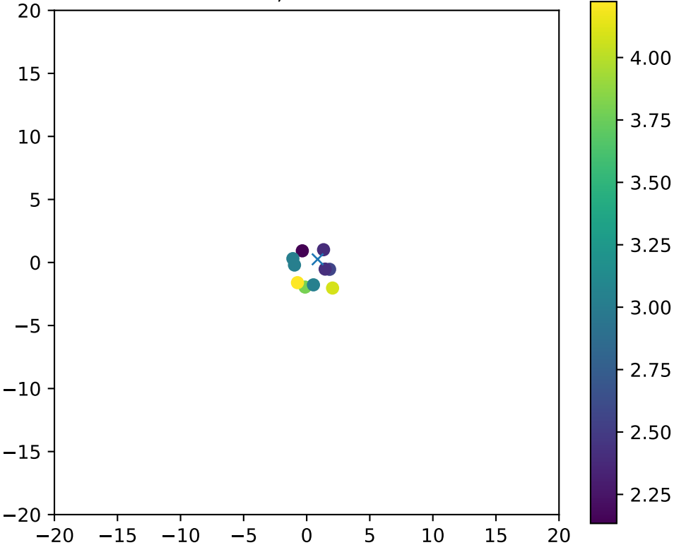
Fiber 2074, dchi2frac= 1.0
