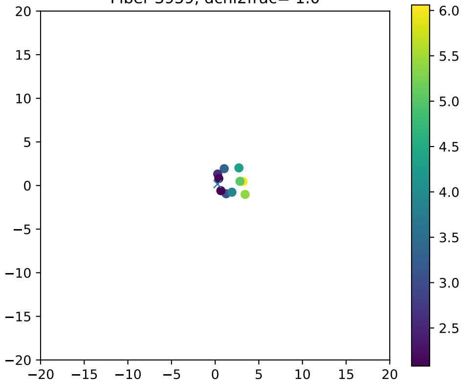
Fiber 3959, dchi2frac= 1.0
