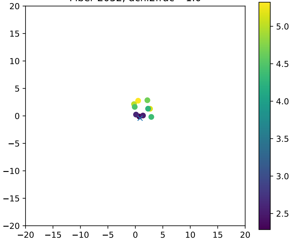
Fiber 2032, dchi2frac= 1.0
