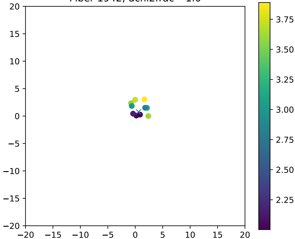
Fiber 1942, dchi2frac= 1.0
