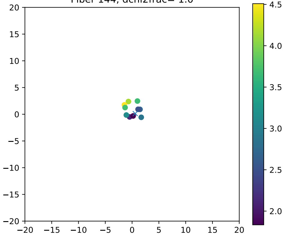
Fiber 144, dchi2frac= 1.0
