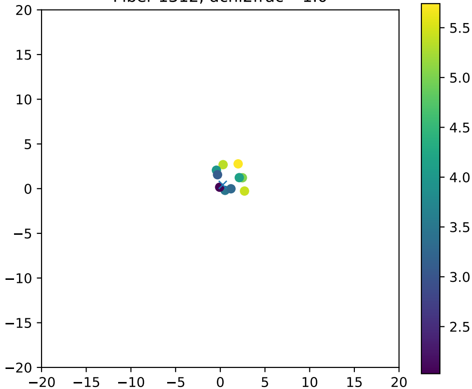
Fiber 1312, dchi2frac= 1.0
