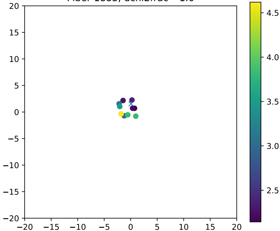
Fiber 1883, dchi2frac= 1.0
