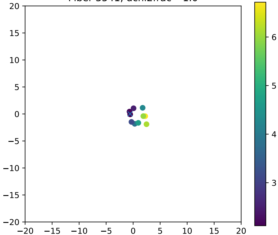
Fiber 3541, dchi2frac= 1.0
