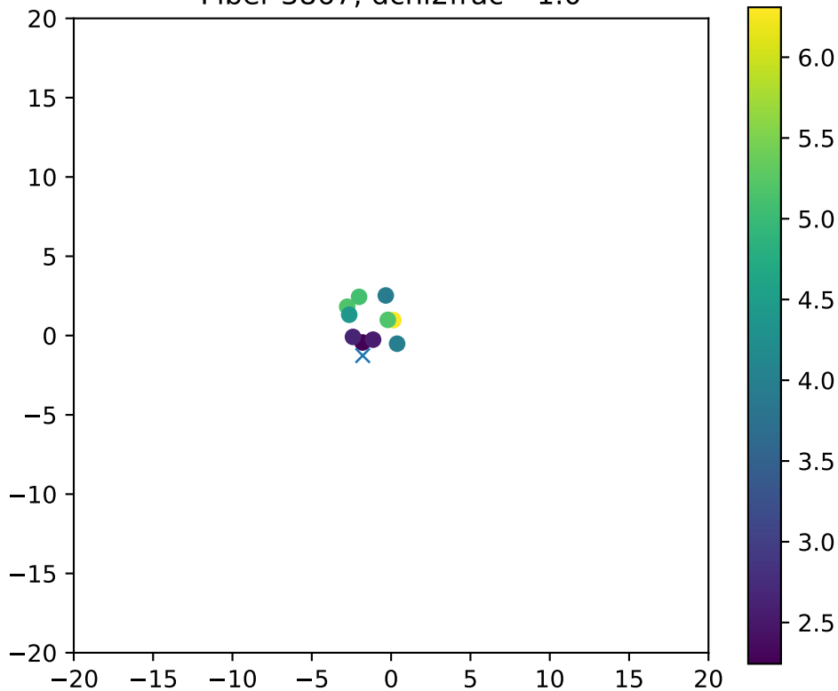
Fiber 3867, dchi2frac= 1.0
