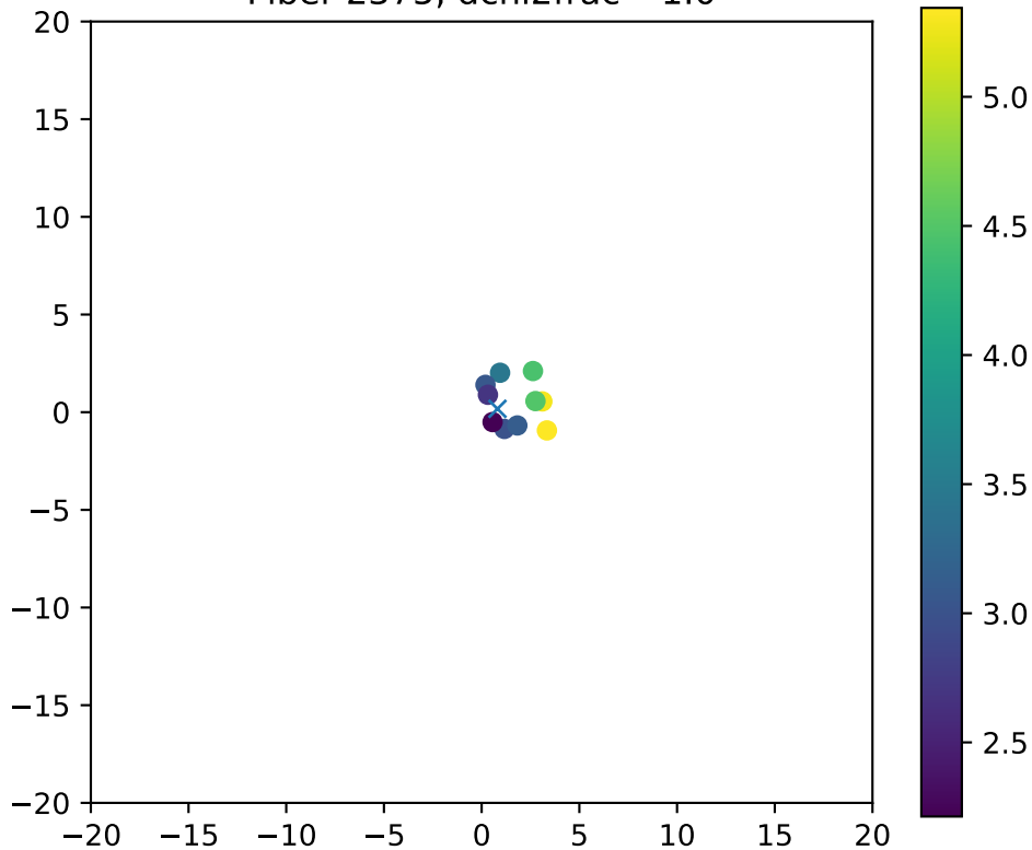
Fiber 2375, dchi2frac= 1.0
