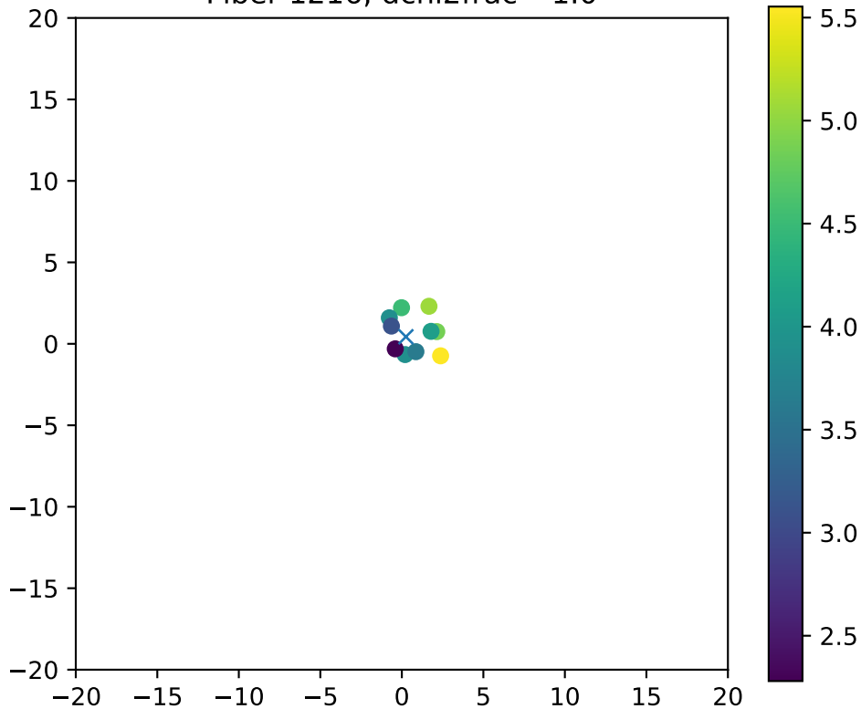
Fiber 1216, dchi2frac= 1.0
