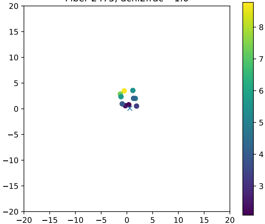
Fiber 2475, dchi2frac= 1.0
