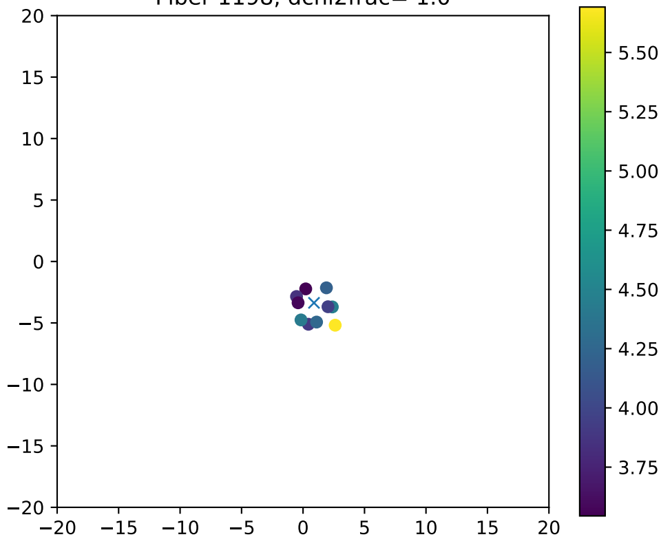
Fiber 1198, dchi2frac= 1.0
