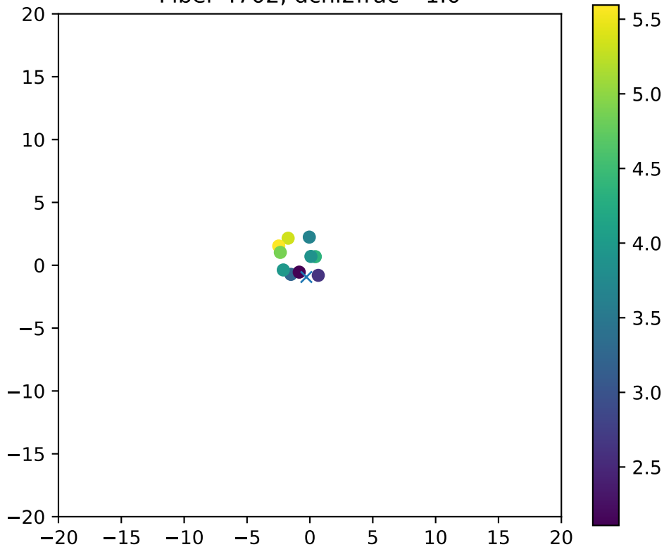
Fiber 4702, dchi2frac= 1.0
