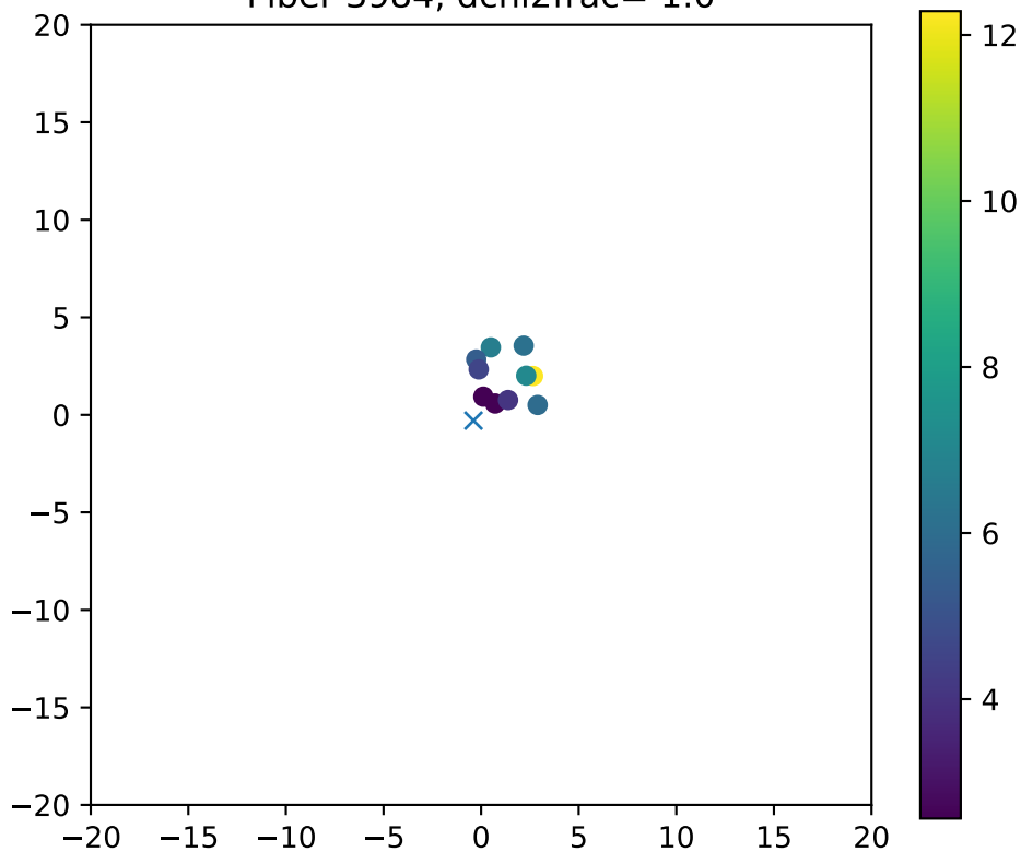
Fiber 3984, dchi2frac= 1.0
