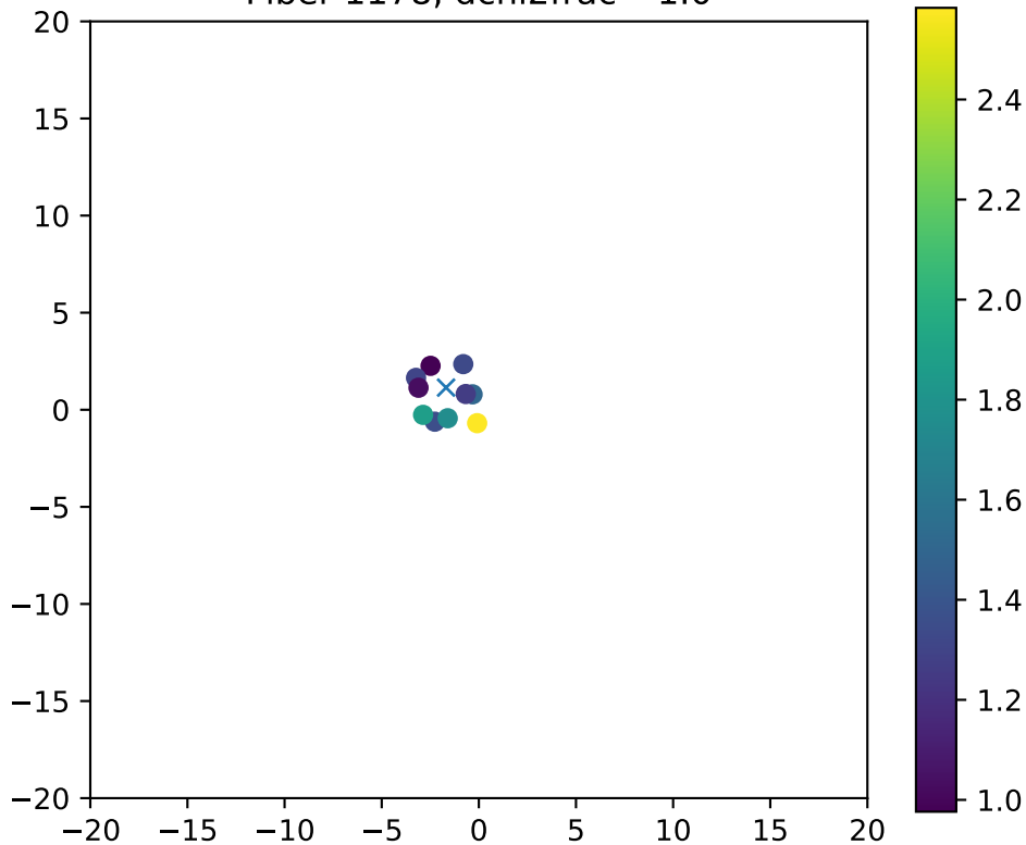
Fiber 1178, dchi2frac= 1.0
