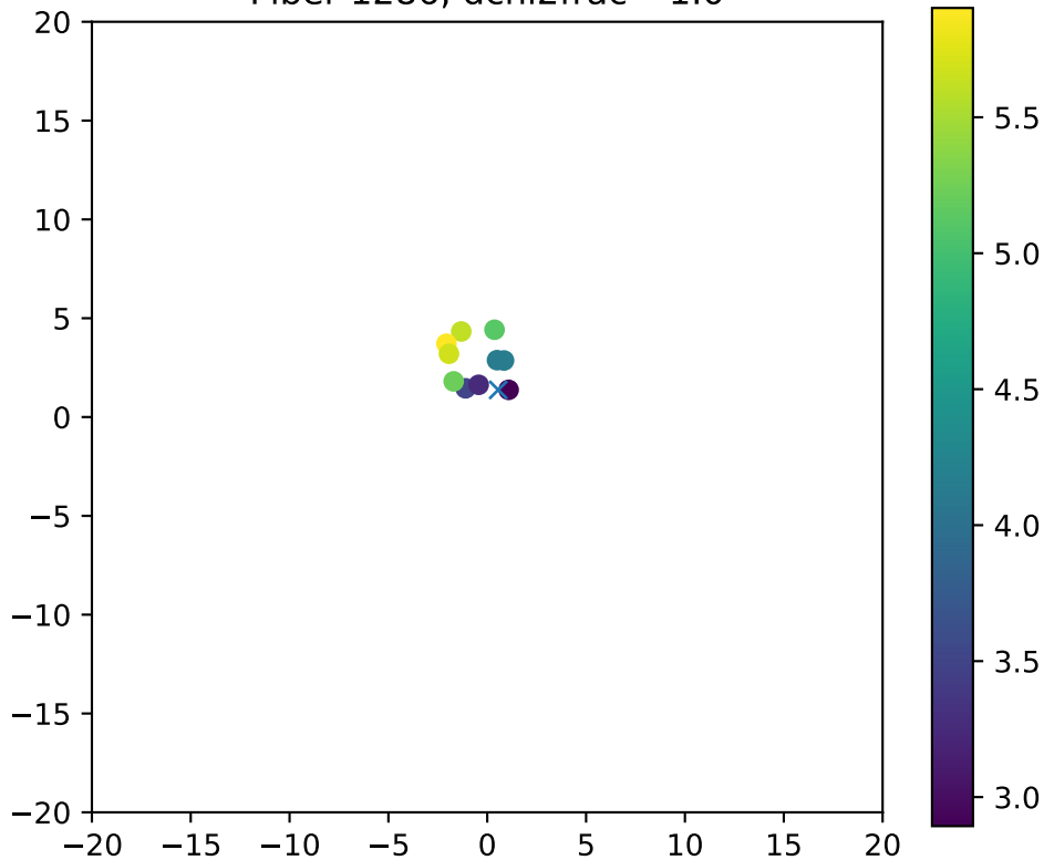
Fiber 1286, dchi2frac= 1.0
