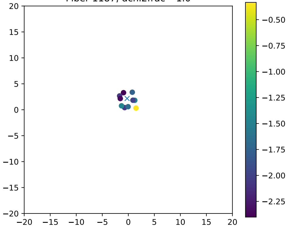
Fiber 1187, dchi2frac= 1.0
