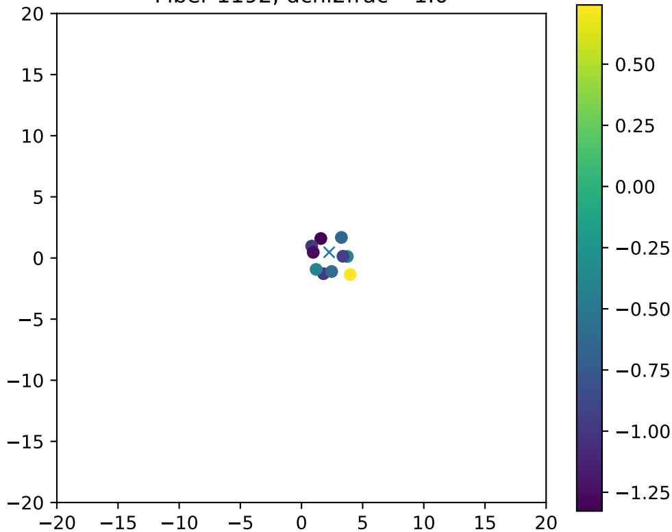
Fiber 1192, dchi2frac= 1.0
