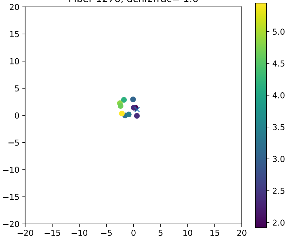
Fiber 1276, dchi2frac= 1.0
