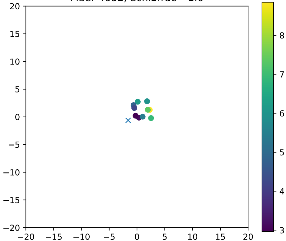
Fiber 4052, dchi2frac= 1.0
