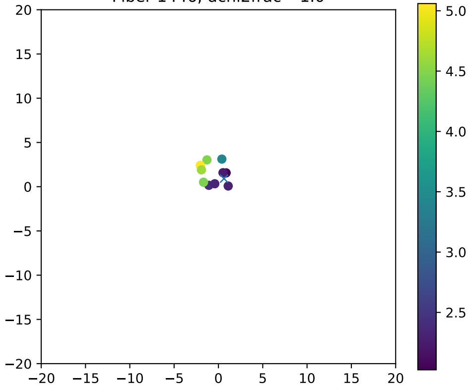
Fiber 1446, dchi2frac= 1.0
