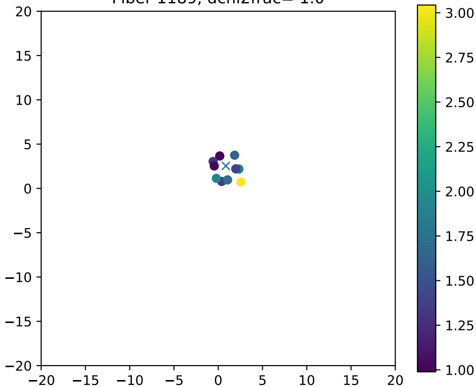
Fiber 1189, dchi2frac= 1.0
