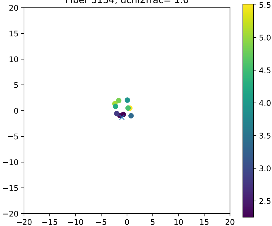
Fiber 3134, dchi2frac= 1.0
