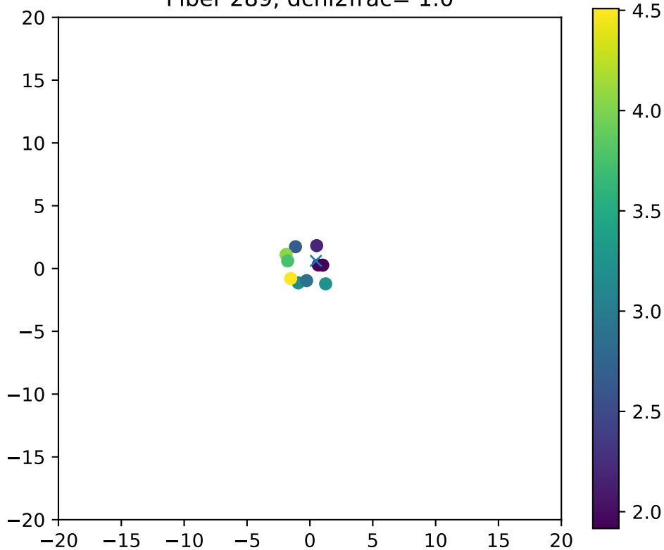
Fiber 289, dchi2frac= 1.0
