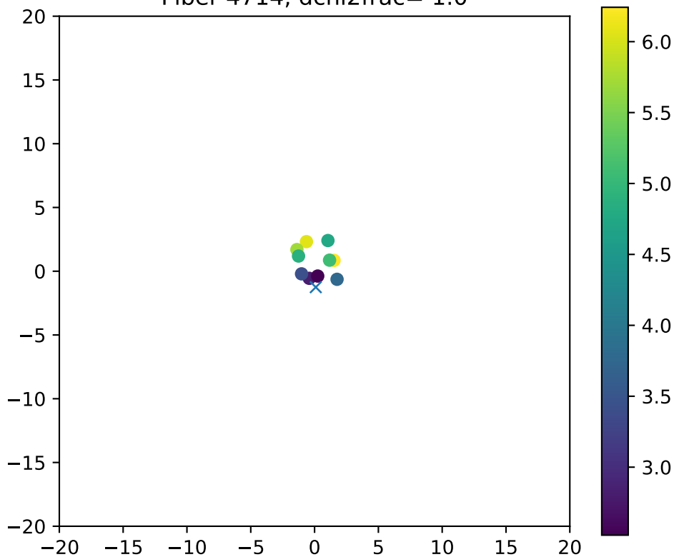
Fiber 4714, dchi2frac= 1.0
