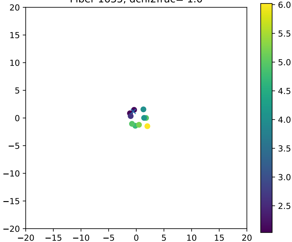
Fiber 1635, dchi2frac= 1.0
