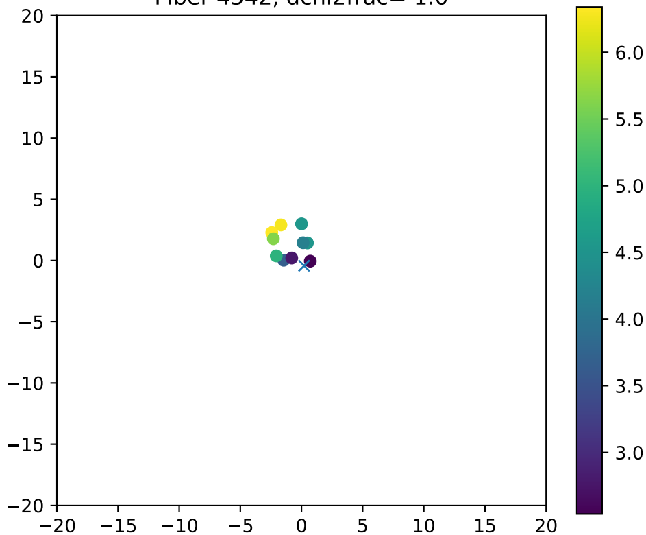
Fiber 4542, dchi2frac= 1.0
