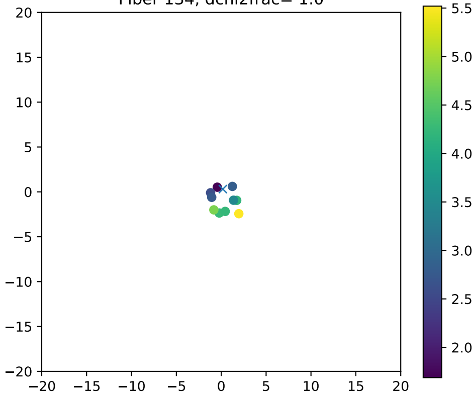
Fiber 134, dchi2frac= 1.0
