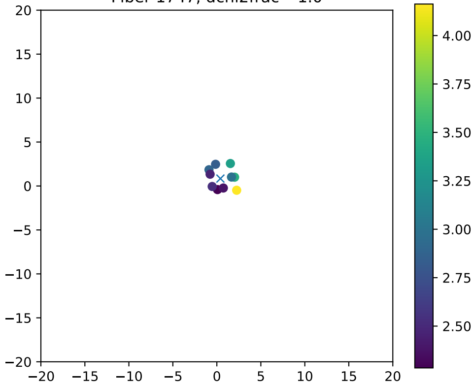
Fiber 1747, dchi2frac= 1.0
