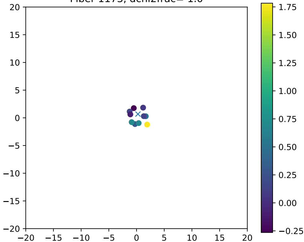
Fiber 1173, dchi2frac= 1.0
