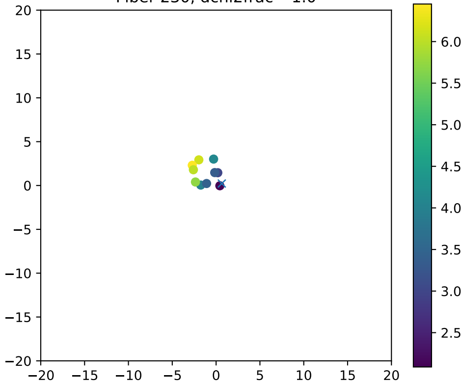
Fiber 230, dchi2frac= 1.0
