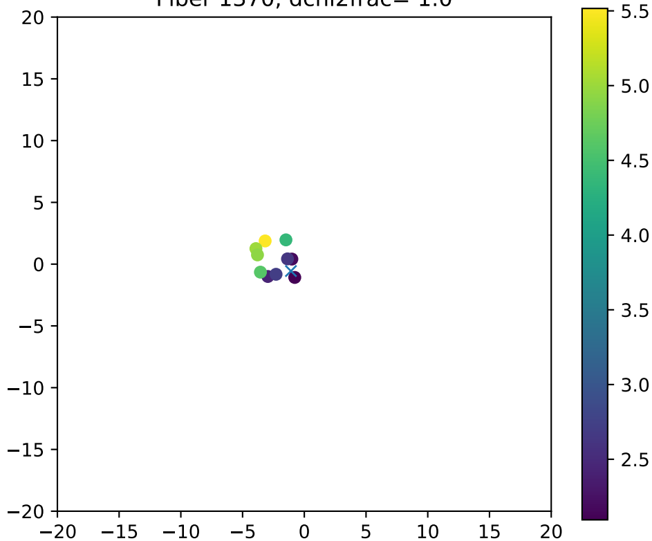
Fiber 1370, dchi2frac= 1.0
