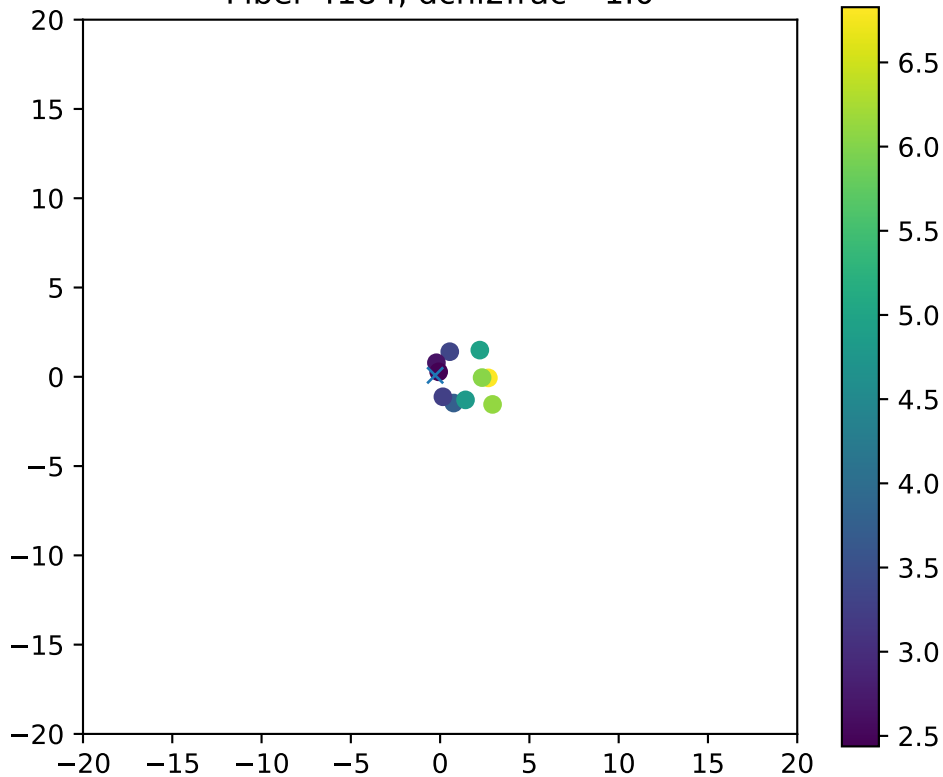
Fiber 4184, dchi2frac= 1.0
