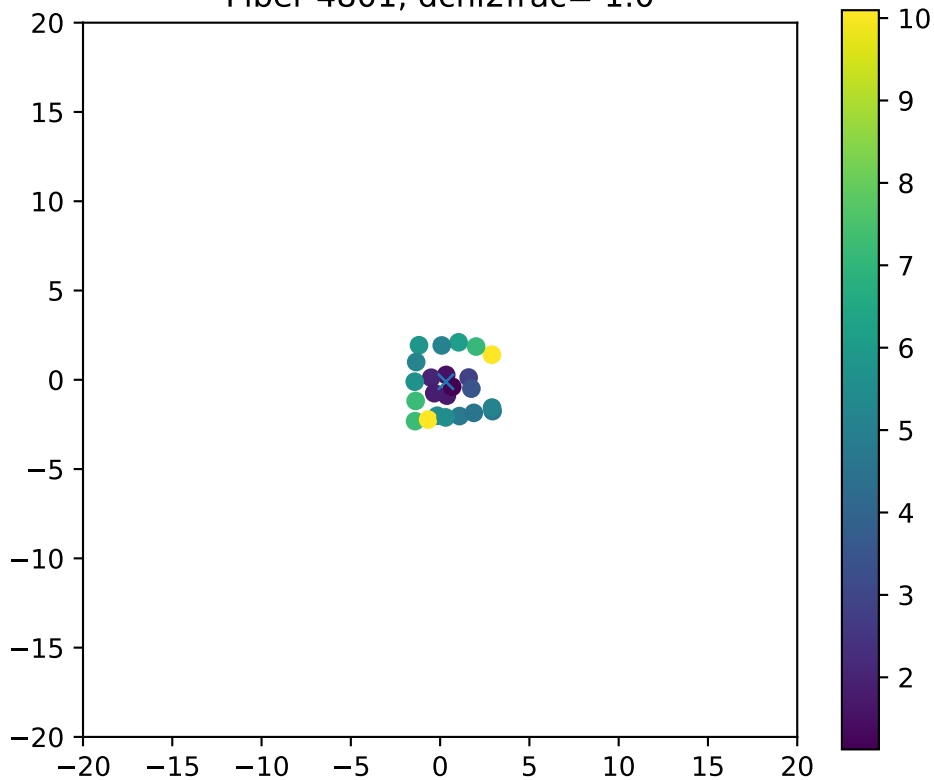
Fiber 4801, dchi2frac= 1.0
