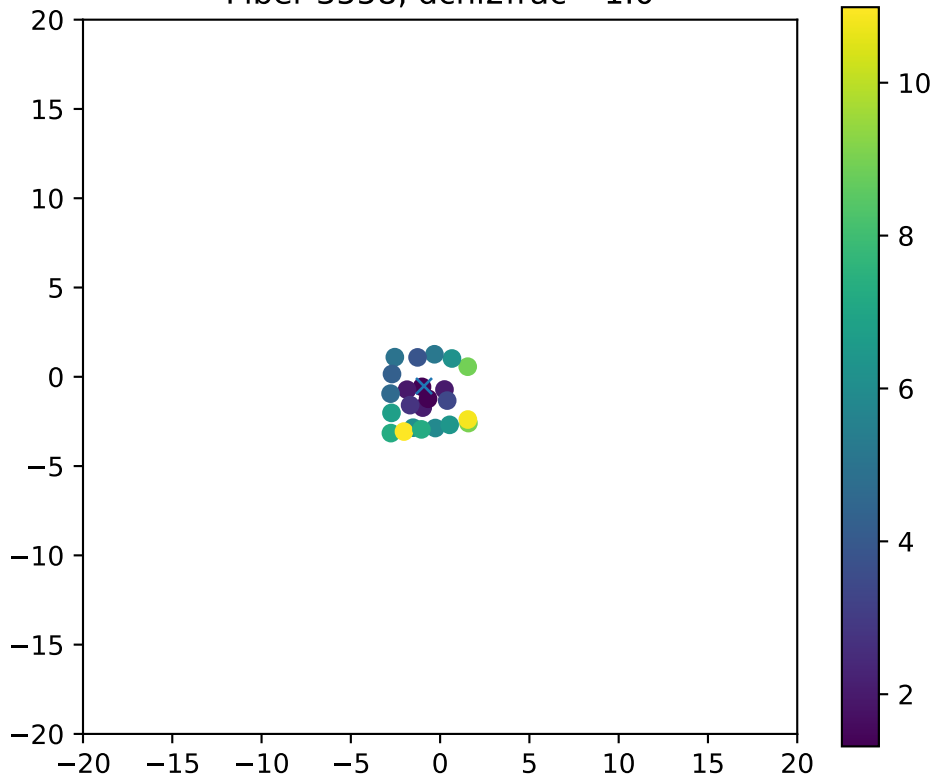
Fiber 3558, dchi2frac= 1.0
