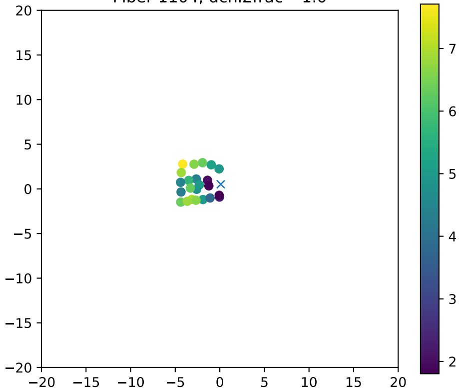
Fiber 1104, dchi2frac= 1.0
