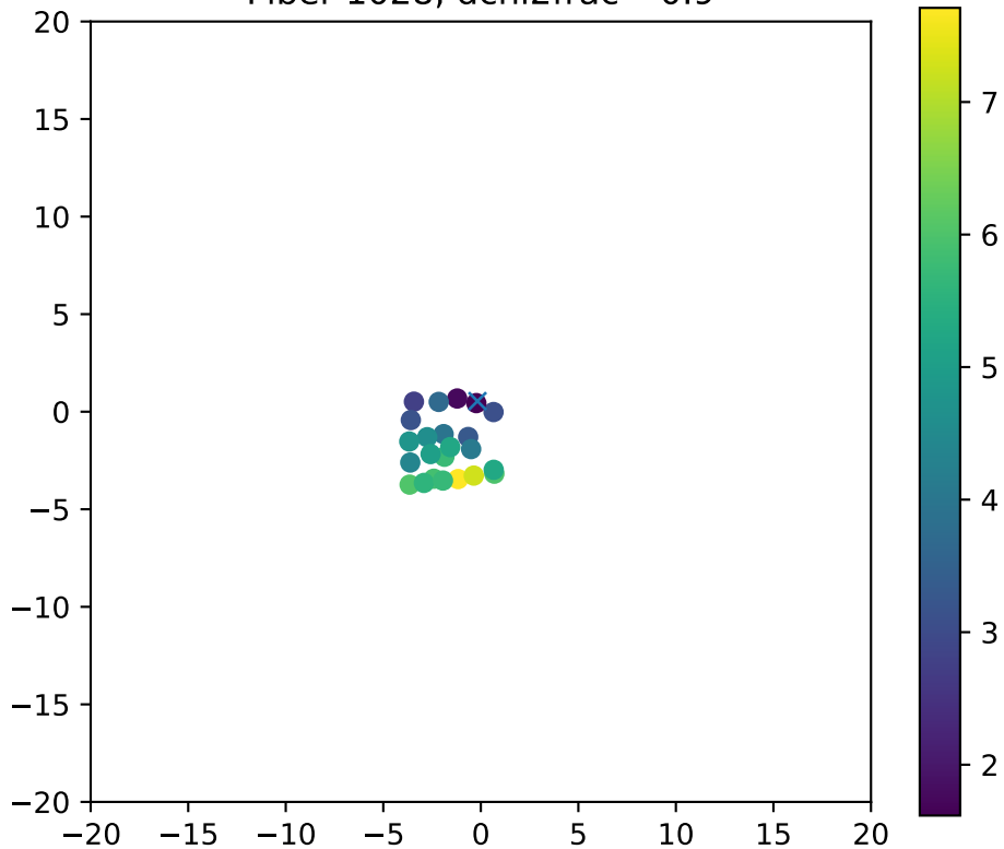
Fiber 1028, dchi2frac= 0.9
