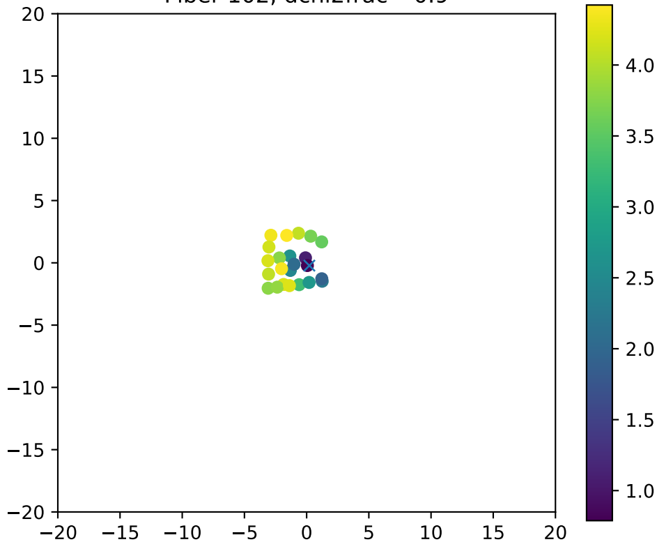
Fiber 102, dchi2frac= 0.9
