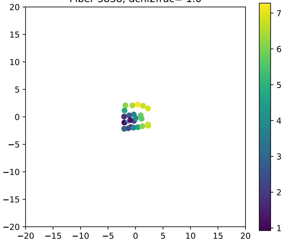
Fiber 3838, dchi2frac= 1.0
