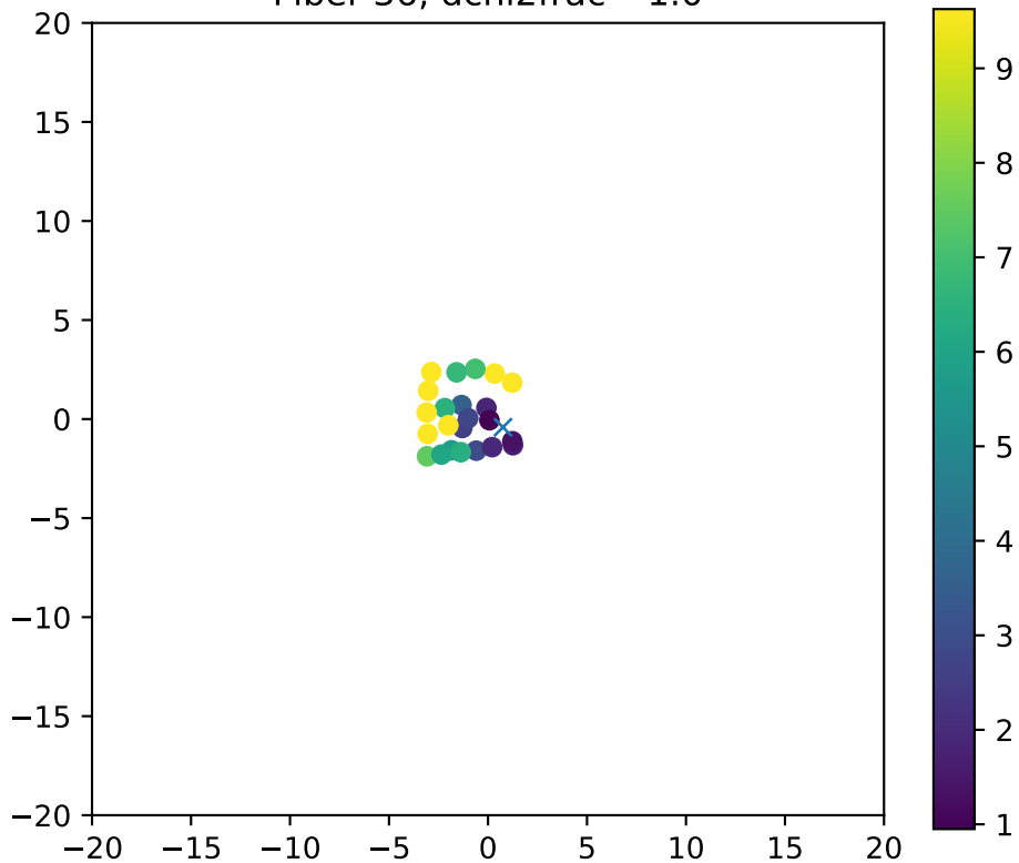
Fiber 36, dchi2frac= 1.0
