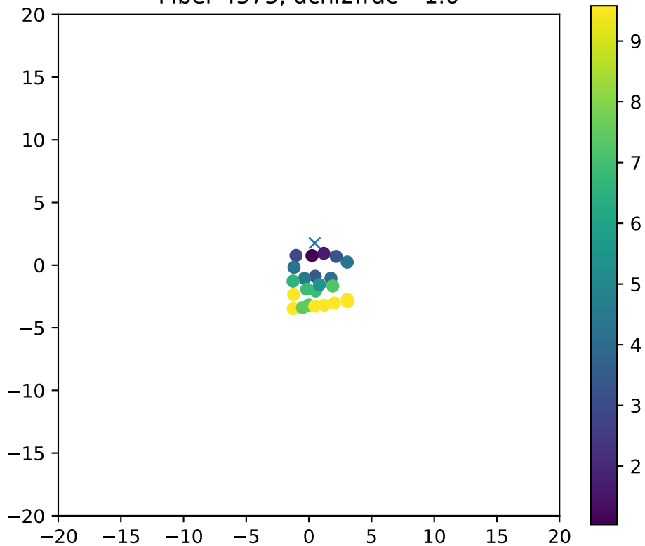
Fiber 4575, dchi2frac= 1.0
