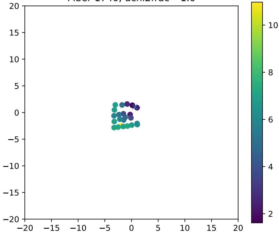
Fiber 1740, dchi2frac= 1.0
