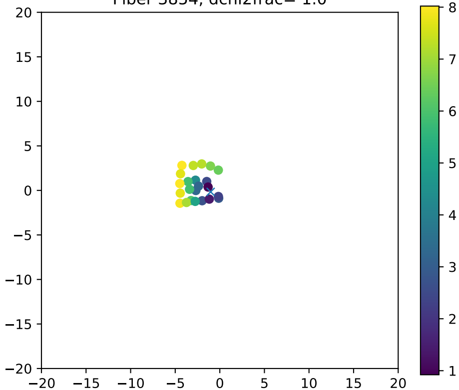
Fiber 3854, dchi2frac= 1.0
