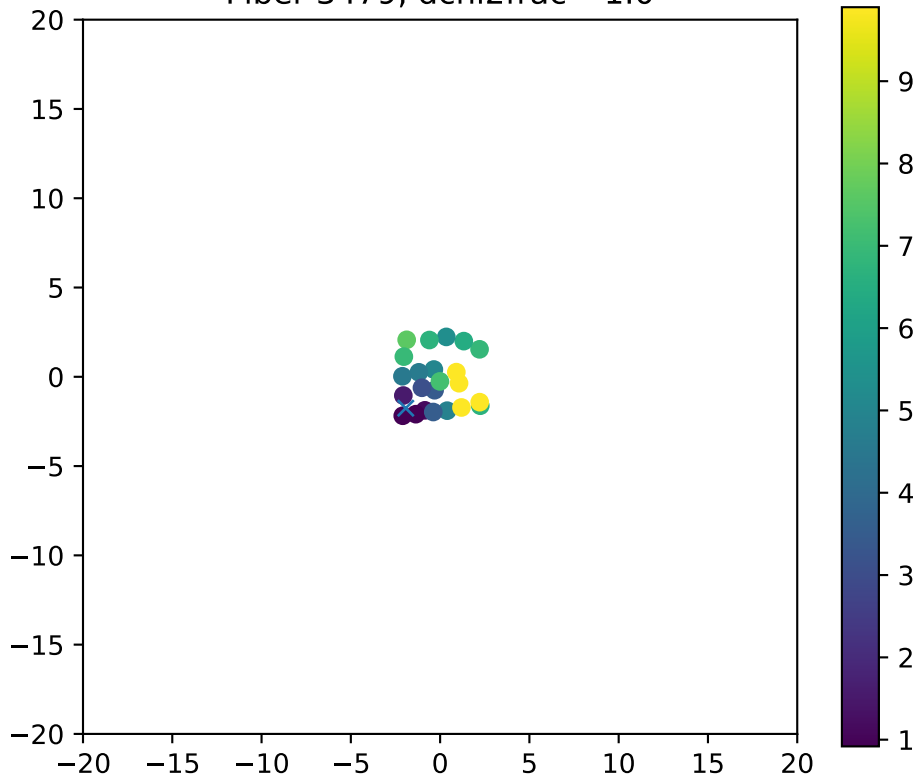
Fiber 3479, dchi2frac= 1.0
