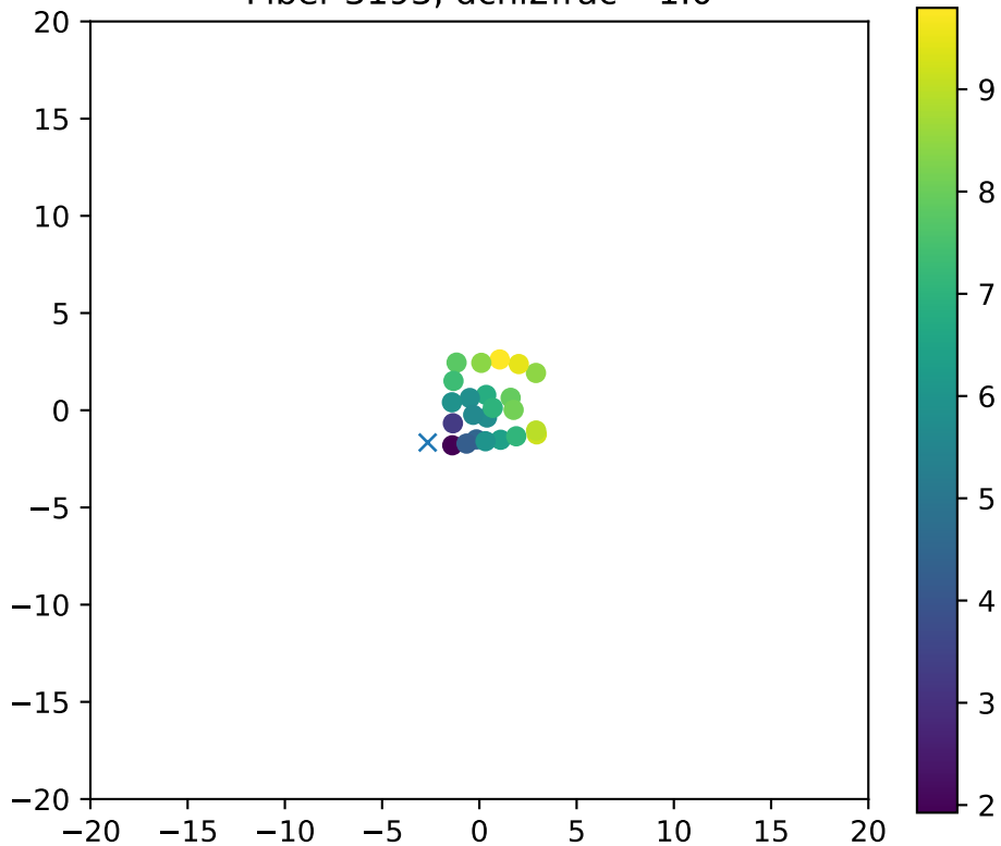
Fiber 3193, dchi2frac= 1.0
