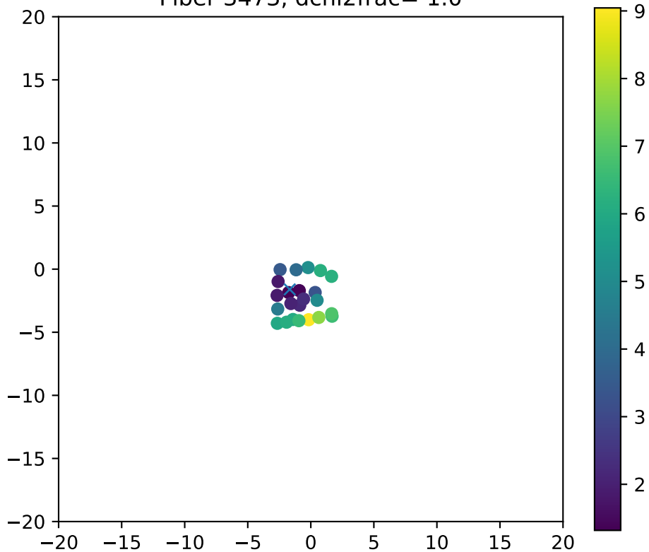
Fiber 3473, dchi2frac= 1.0
