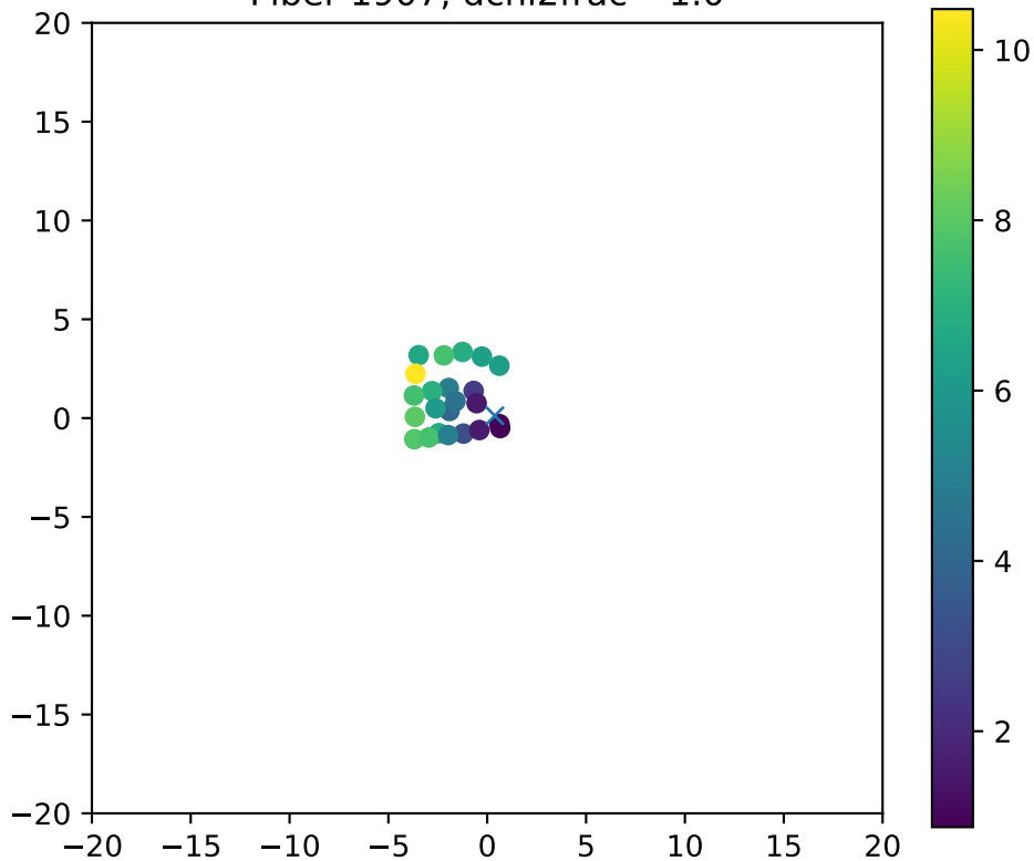
Fiber 1907, dchi2frac= 1.0
