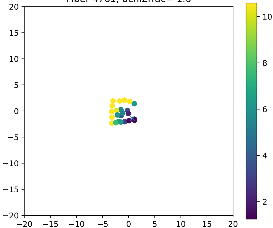
Fiber 4761, dchi2frac= 1.0
