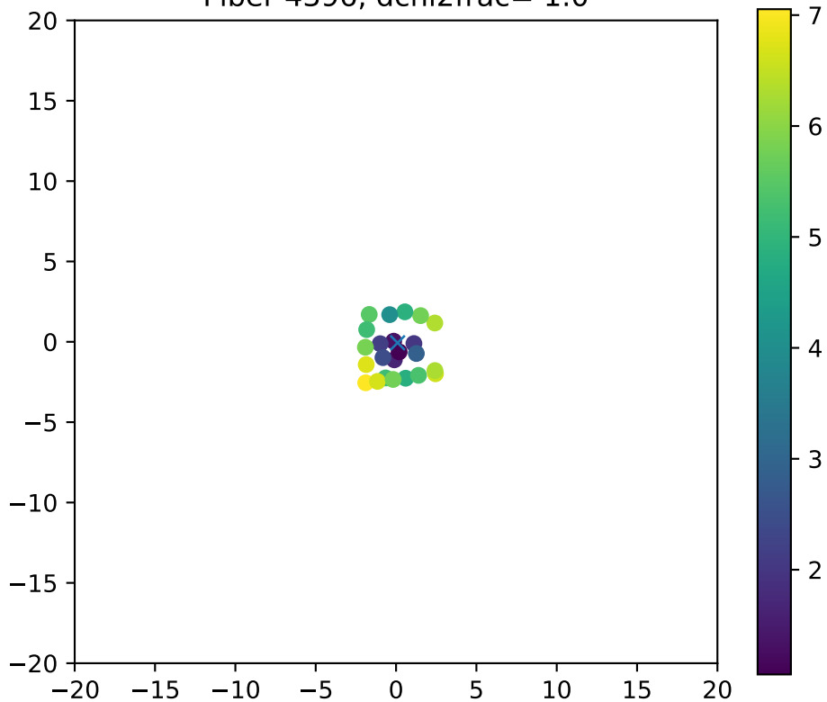
Fiber 4396, dchi2frac= 1.0
