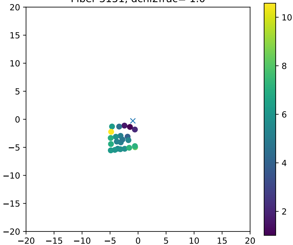
Fiber 3151, dchi2frac= 1.0
