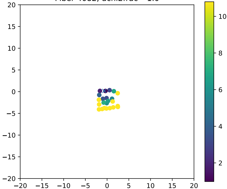
Fiber 4082, dchi2frac= 1.0
