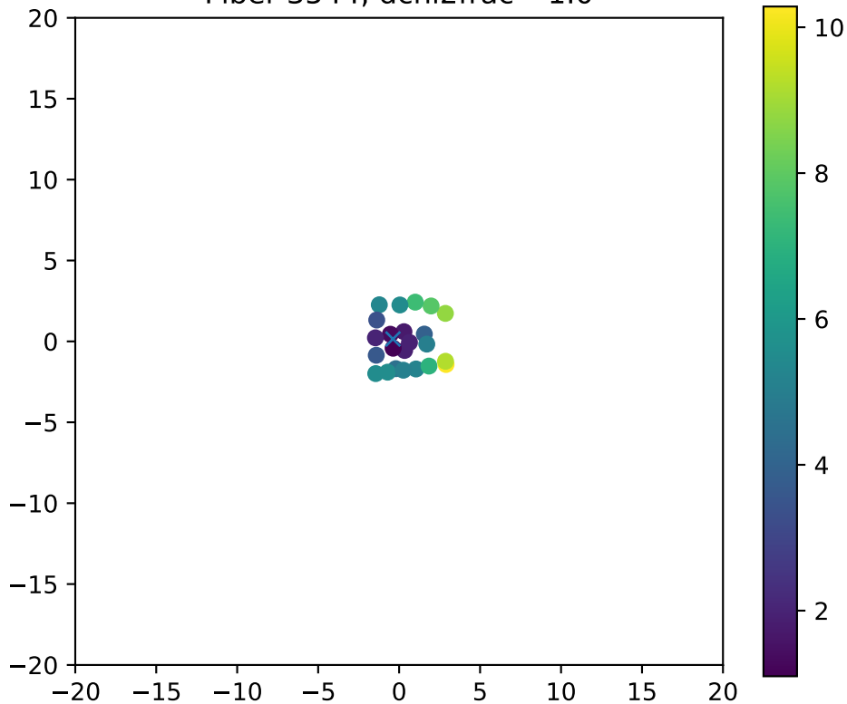
Fiber 3544, dchi2frac= 1.0
