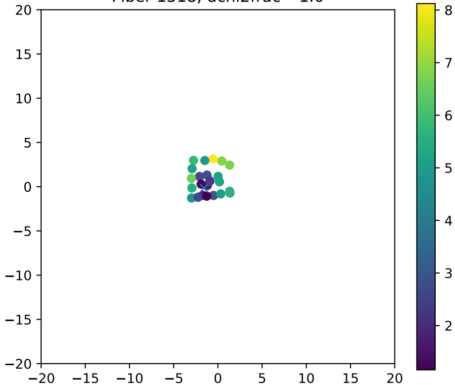
Fiber 1318, dchi2frac= 1.0
