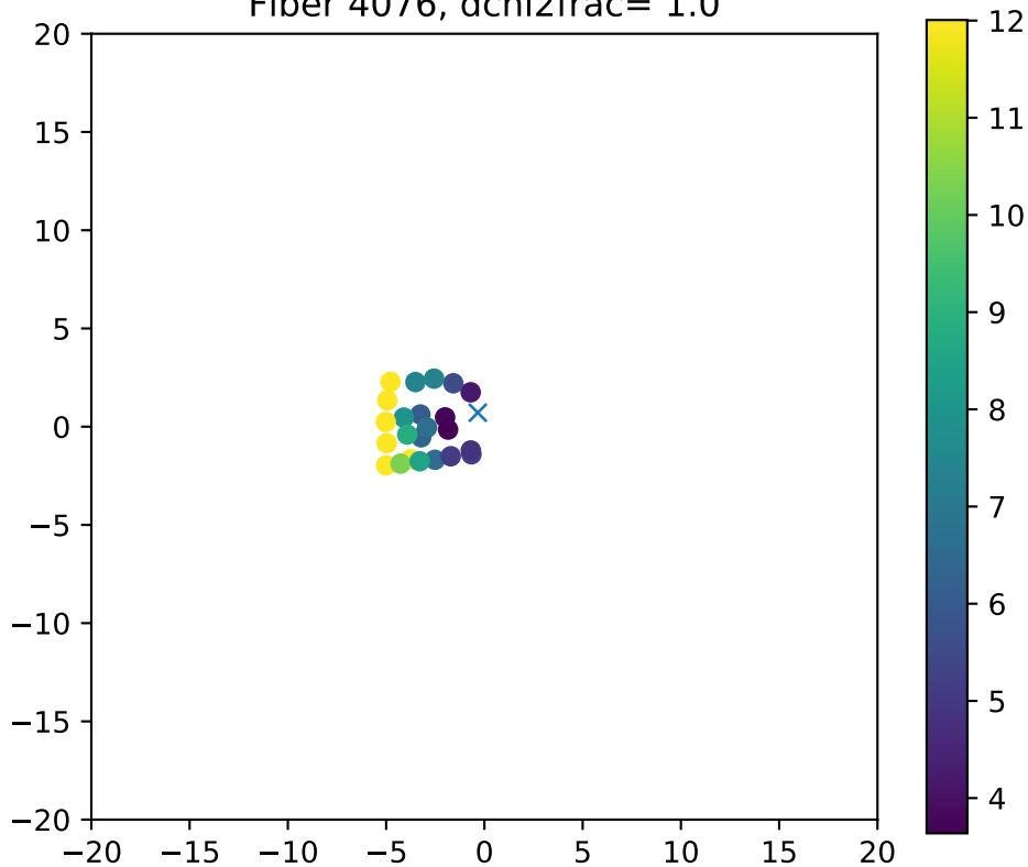
Fiber 4076, dchi2frac= 1.0
