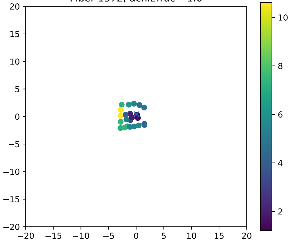
Fiber 1572, dchi2frac= 1.0
