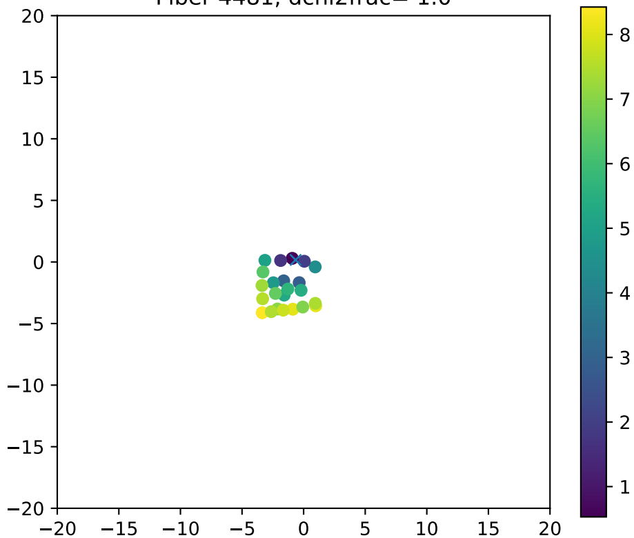
Fiber 4481, dchi2frac= 1.0
