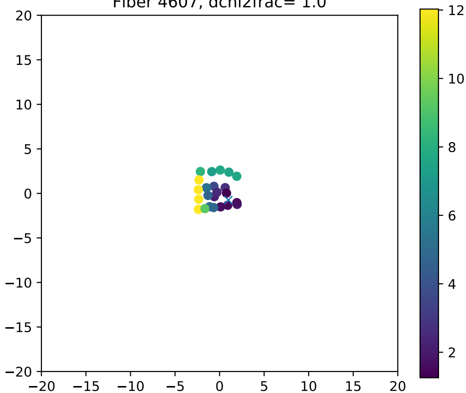
Fiber 4607, dchi2frac= 1.0
