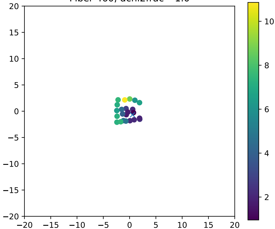
Fiber 460, dchi2frac= 1.0
