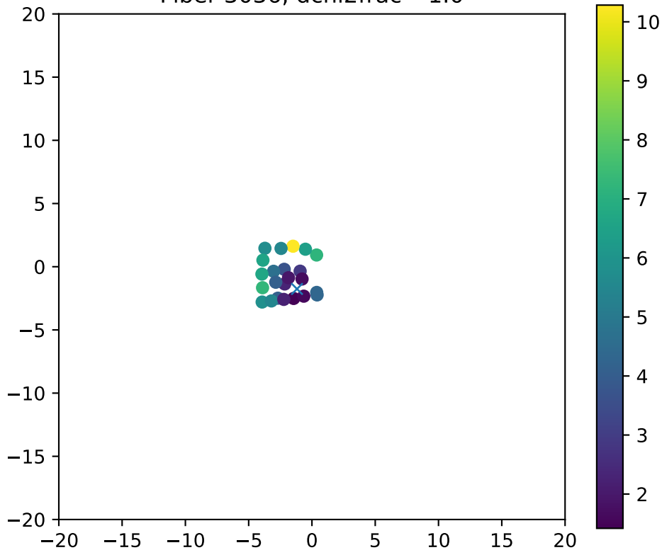
Fiber 3036, dchi2frac= 1.0
