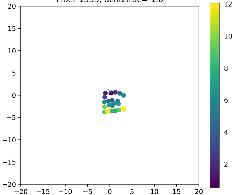
Fiber 1533, dchi2frac= 1.0
