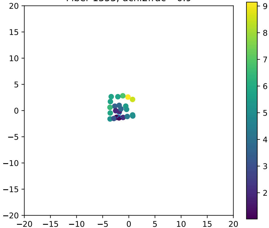
Fiber 1353, dchi2frac= 0.9
