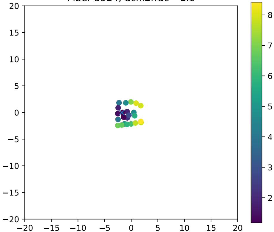
Fiber 3924, dchi2frac= 1.0
