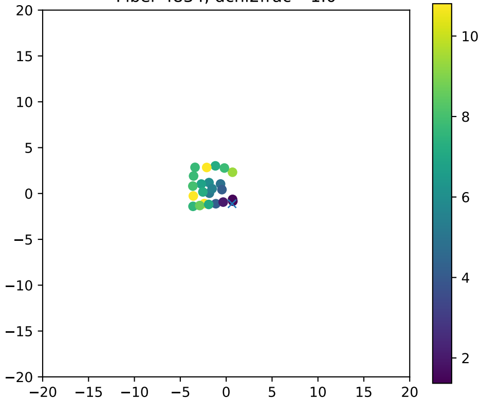
Fiber 4834, dchi2frac= 1.0
