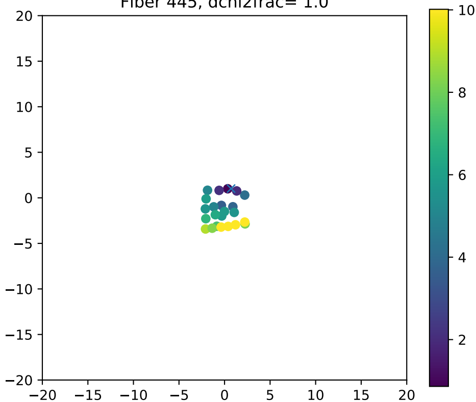
Fiber 445, dchi2frac= 1.0
