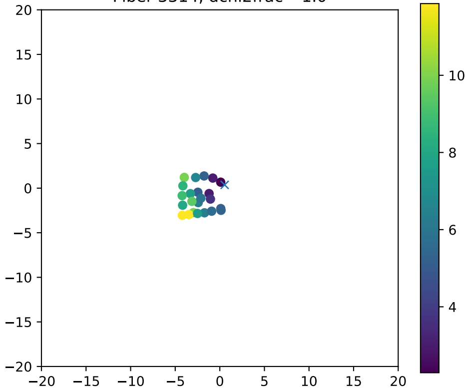
Fiber 3314, dchi2frac= 1.0
