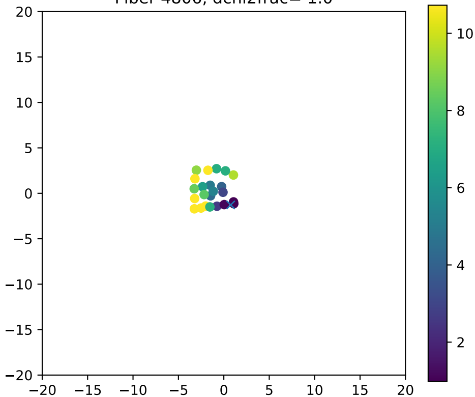
Fiber 4806, dchi2frac= 1.0
