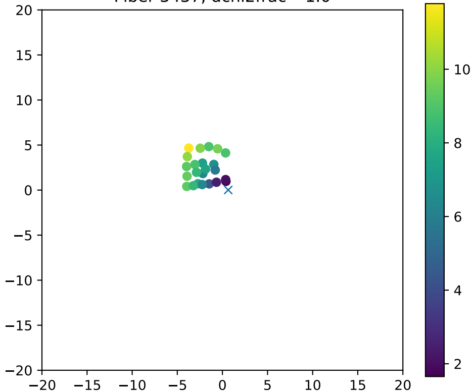
Fiber 3437, dchi2frac= 1.0
