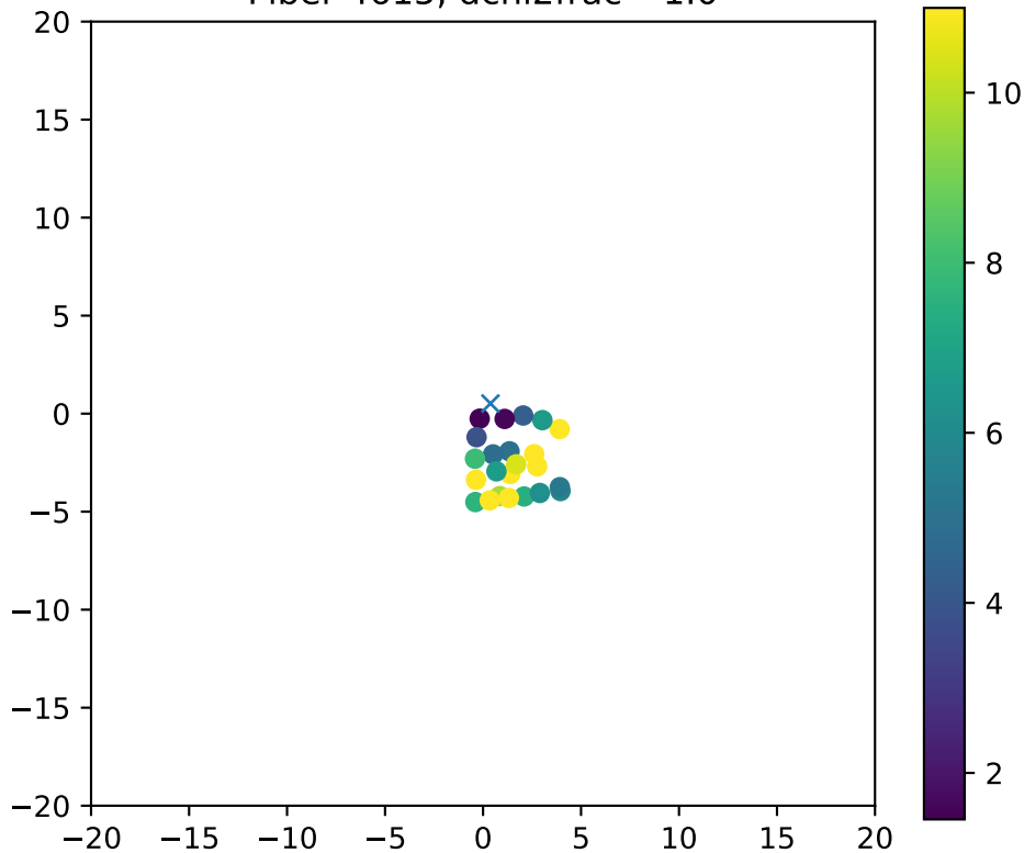
Fiber 4615, dchi2frac= 1.0
