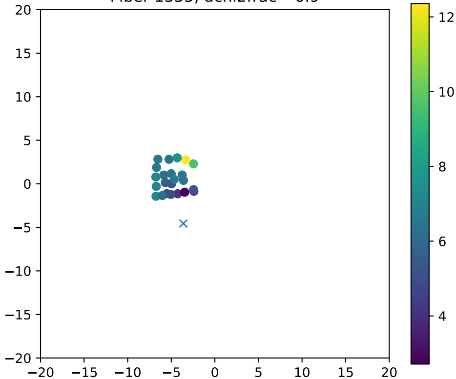
Fiber 1355, dchi2frac= 0.9
