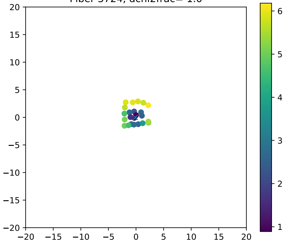
Fiber 3724, dchi2frac= 1.0
