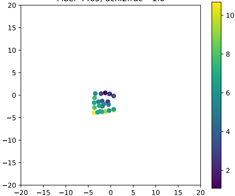
Fiber 4465, dchi2frac= 1.0
