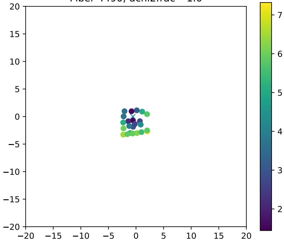
Fiber 4490, dchi2frac= 1.0
