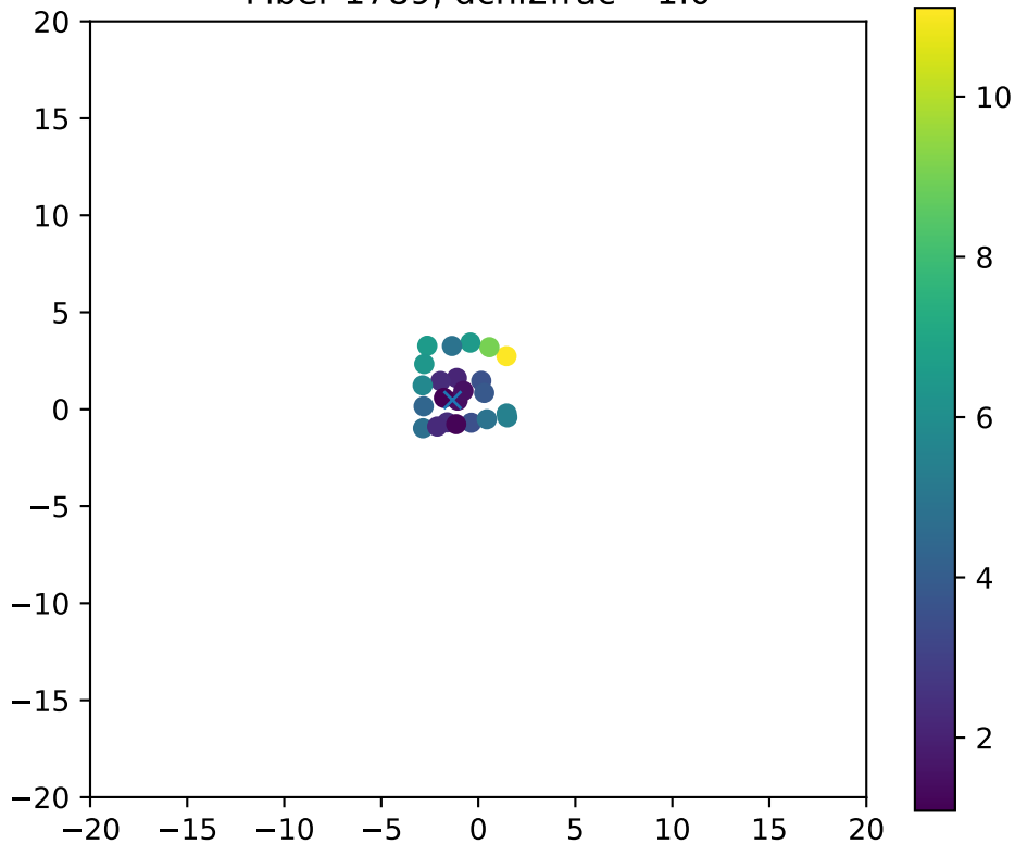
Fiber 1789, dchi2frac= 1.0
