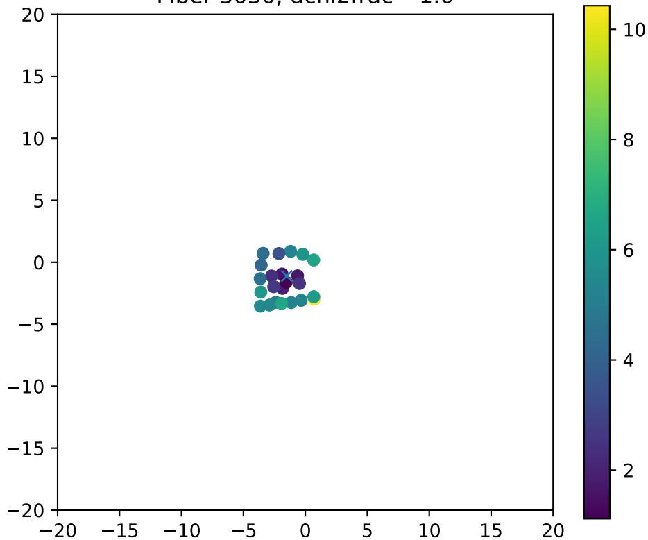
Fiber 3030, dchi2frac= 1.0
