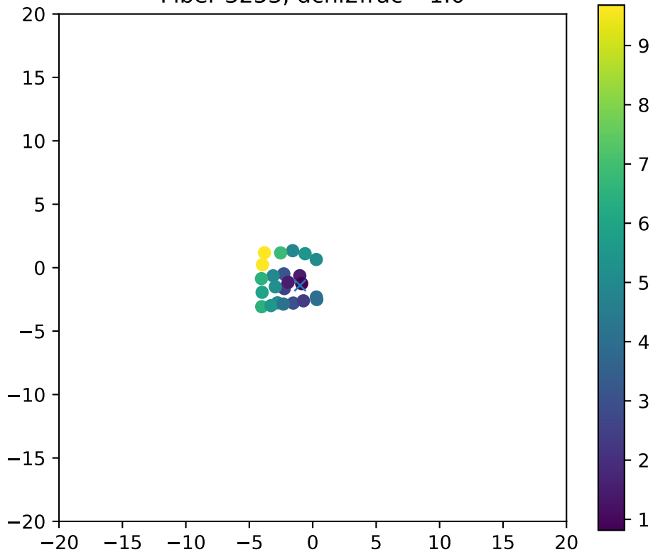
Fiber 3253, dchi2frac= 1.0
