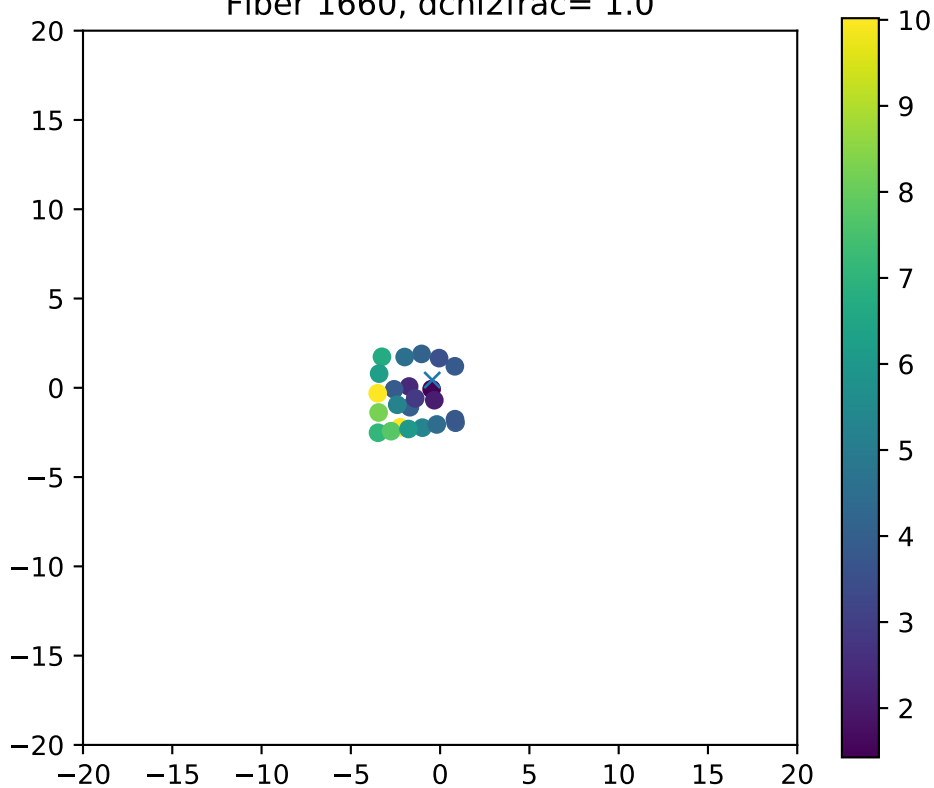
Fiber 1660, dchi2frac= 1.0
