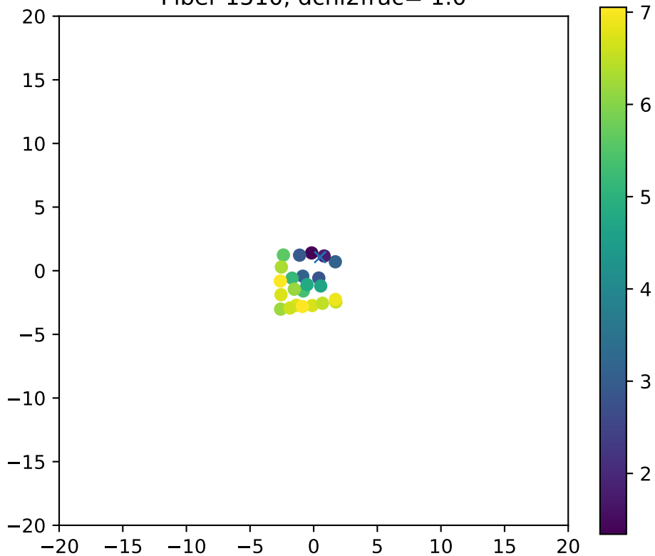
Fiber 1510, dchi2frac= 1.0
