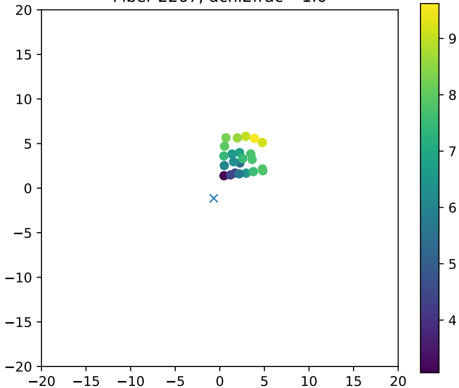
Fiber 2267, dchi2frac= 1.0
