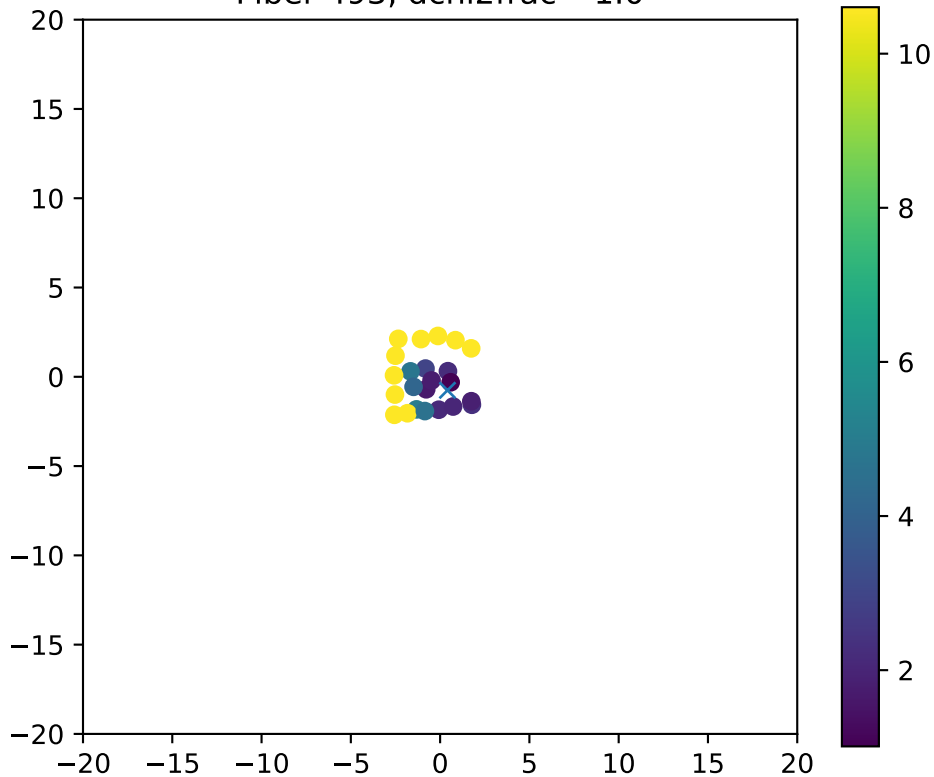
Fiber 493, dchi2frac= 1.0
