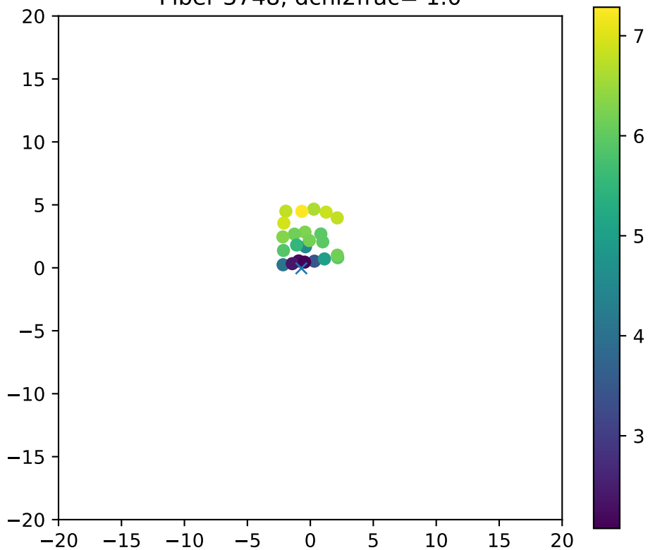
Fiber 3748, dchi2frac= 1.0
