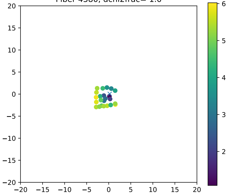
Fiber 4380, dchi2frac= 1.0
