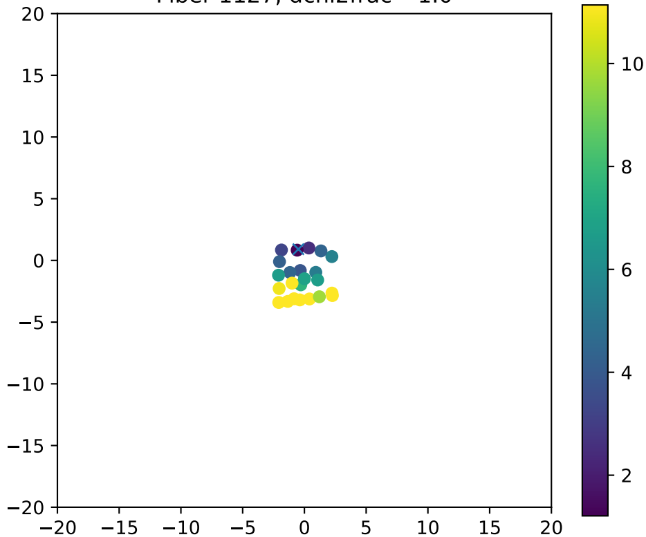
Fiber 1127, dchi2frac= 1.0
