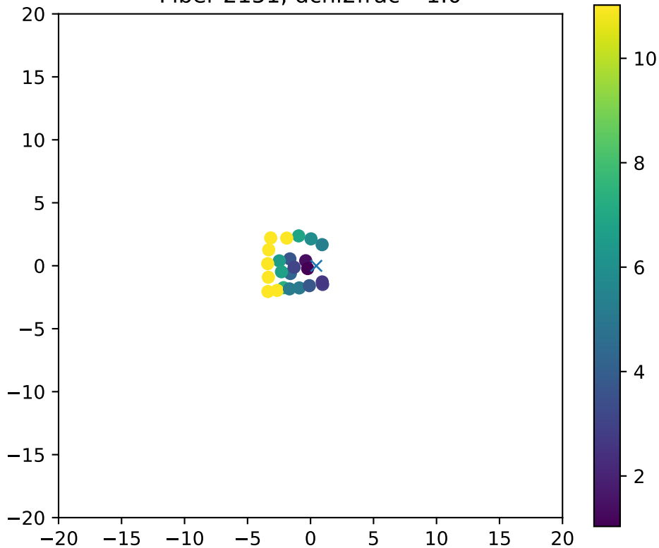
Fiber 2151, dchi2frac= 1.0
