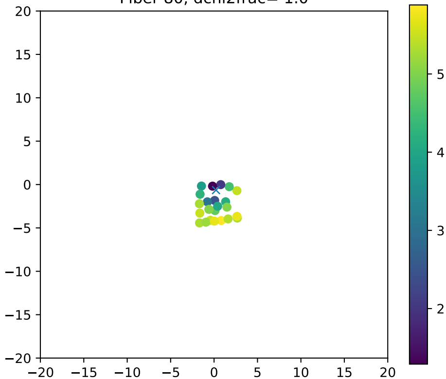
Fiber 80, dchi2frac= 1.0
