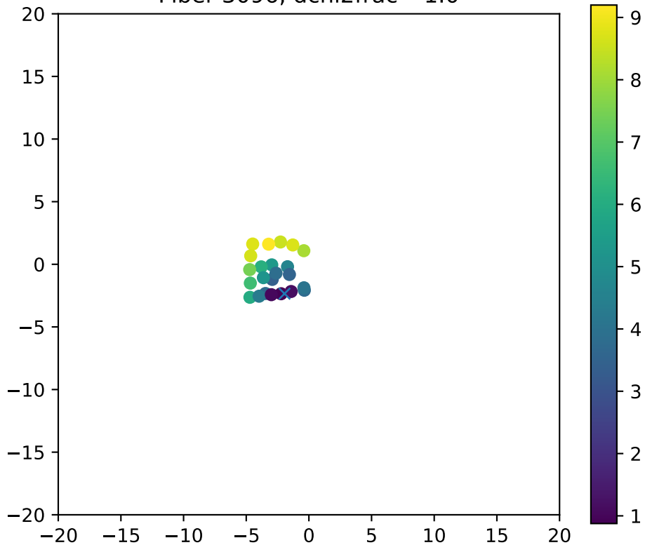
Fiber 3096, dchi2frac= 1.0
