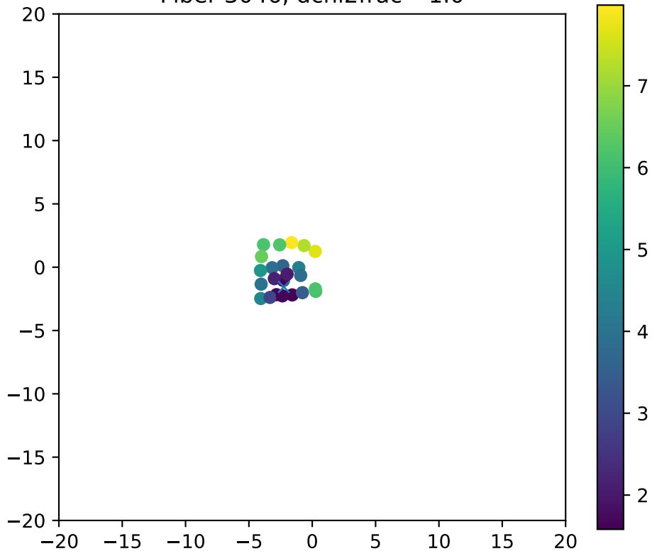
Fiber 3046, dchi2frac= 1.0
