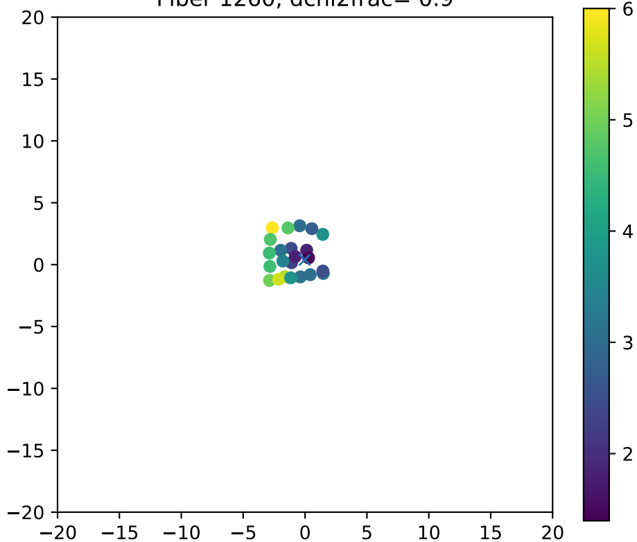
Fiber 1260, dchi2frac= 0.9
