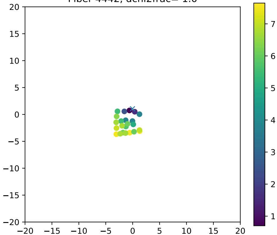
Fiber 4442, dchi2frac= 1.0
