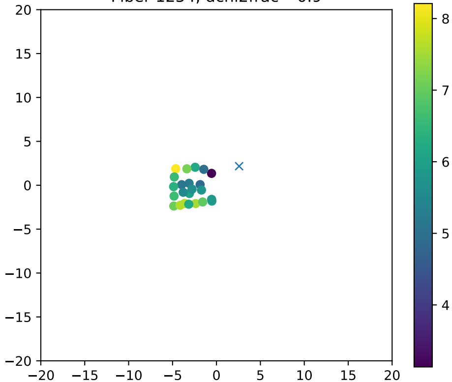
Fiber 1254, dchi2frac= 0.9
