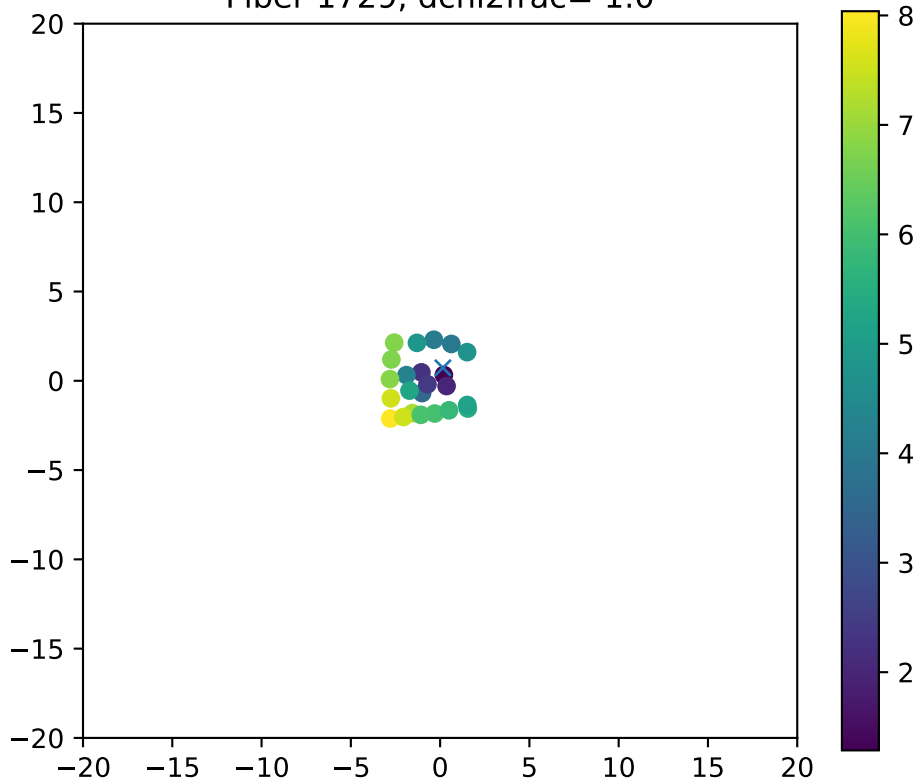
Fiber 1729, dchi2frac= 1.0
