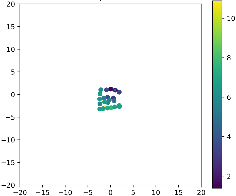
Fiber 4861, dchi2frac= 1.0
