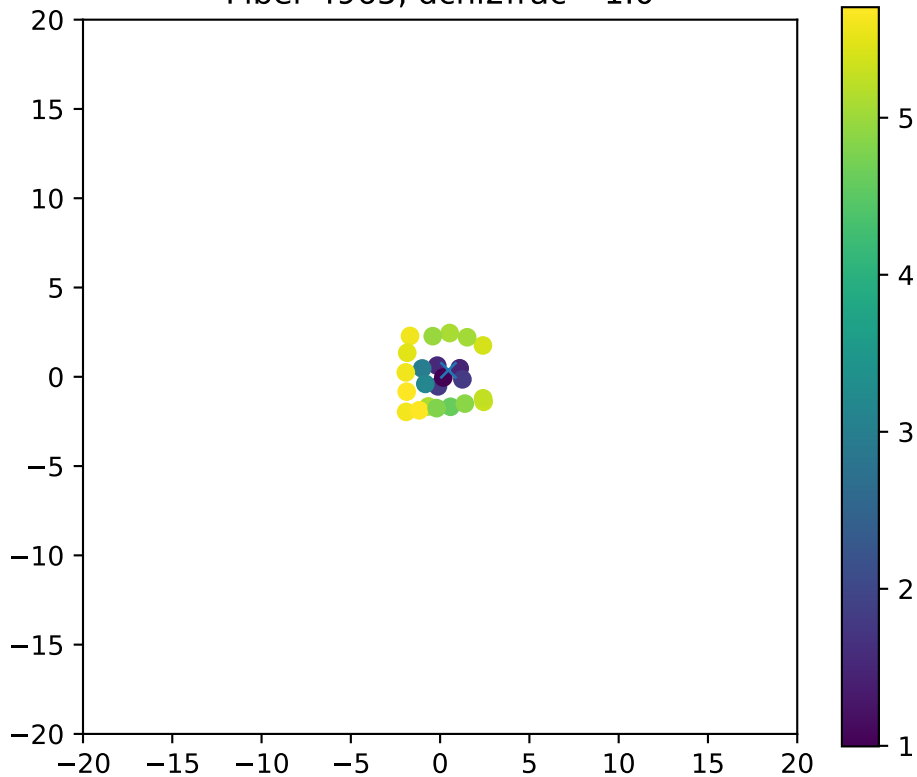
Fiber 4965, dchi2frac= 1.0
