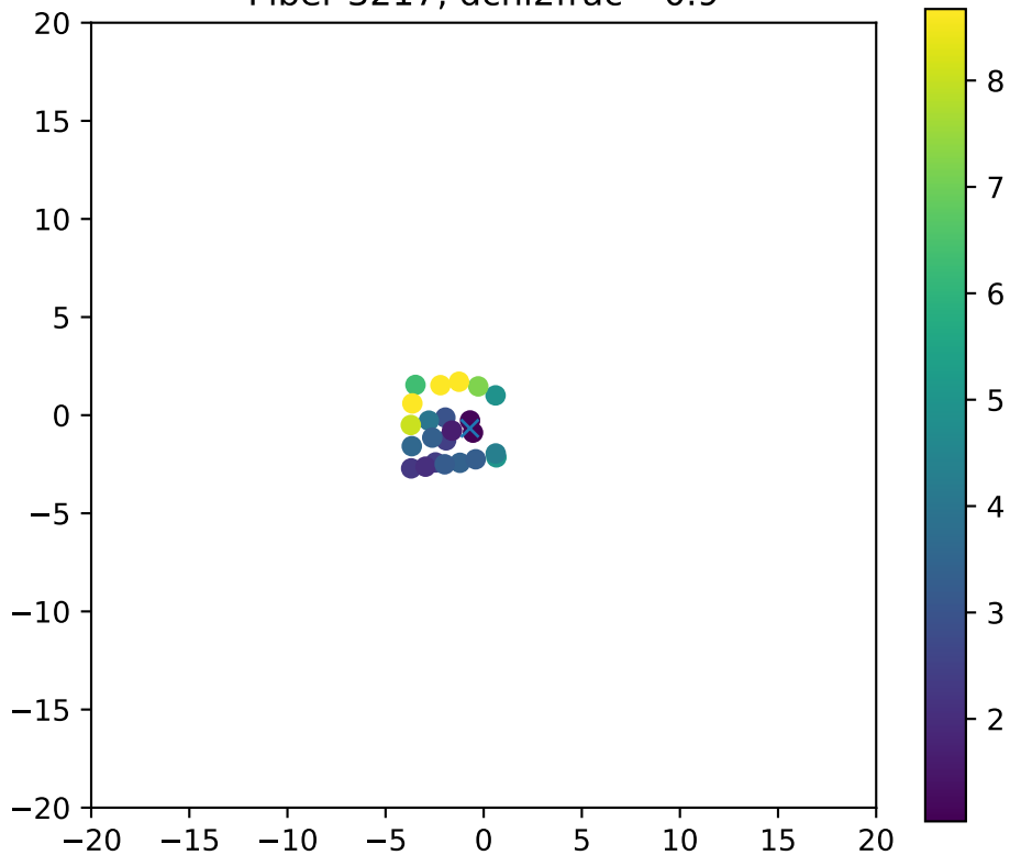
Fiber 3217, dchi2frac= 0.9
