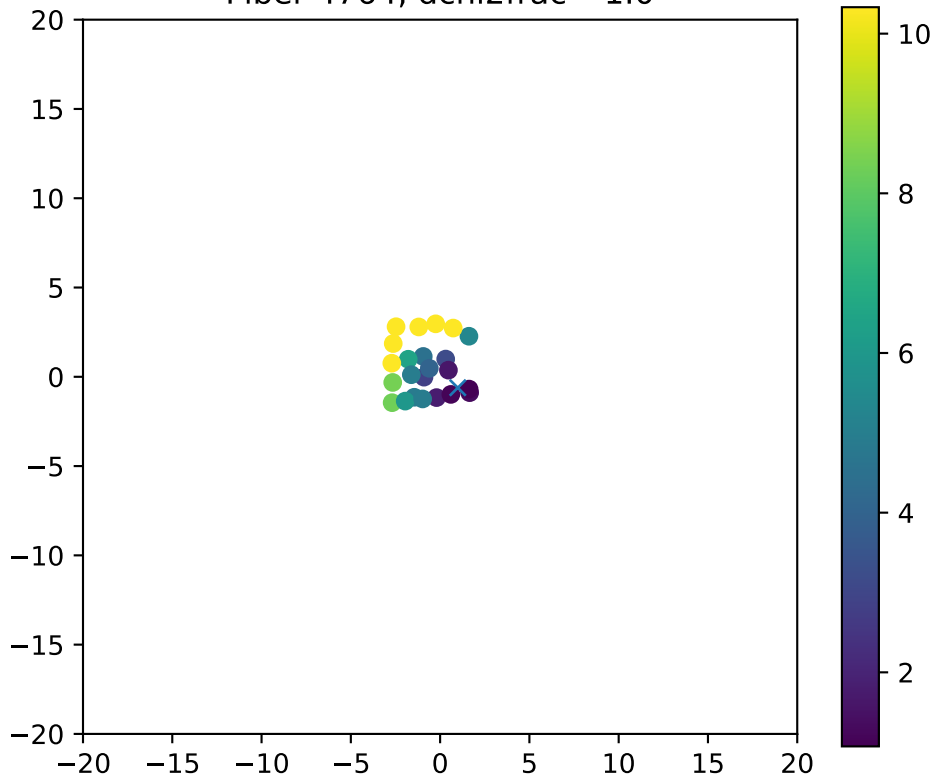
Fiber 4764, dchi2frac= 1.0
