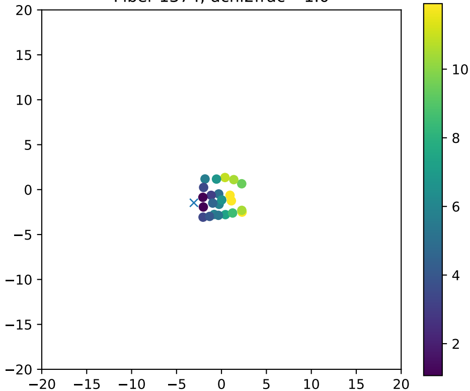
Fiber 1374, dchi2frac= 1.0
