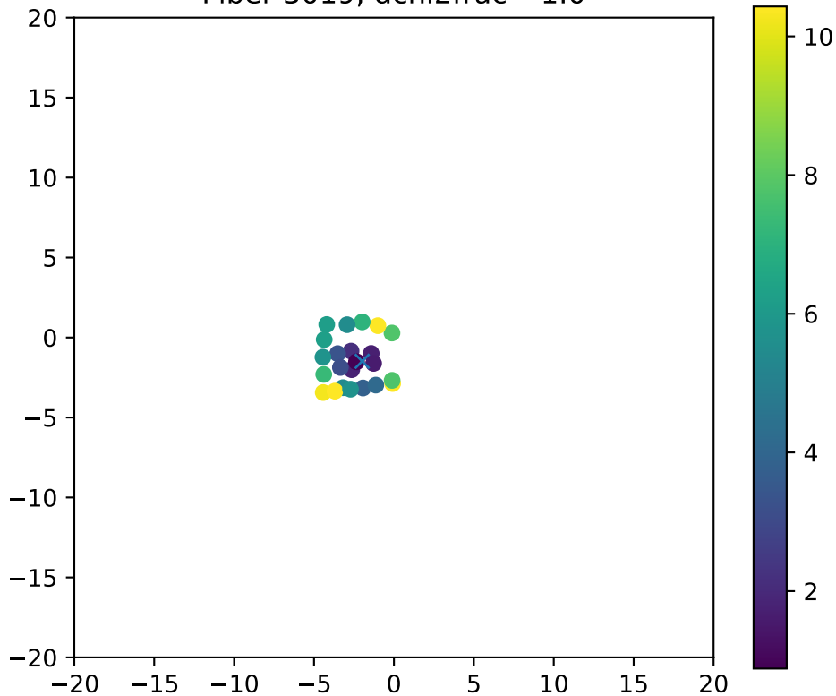
Fiber 3019, dchi2frac= 1.0
