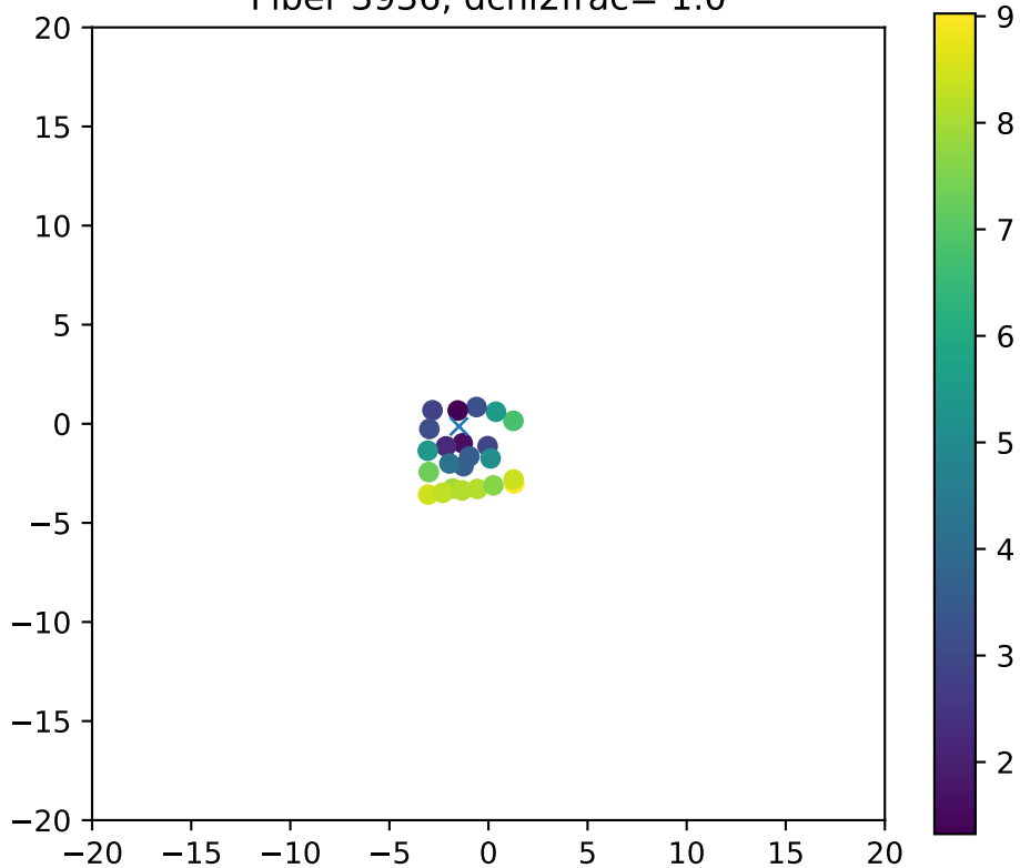
Fiber 3936, dchi2frac= 1.0
