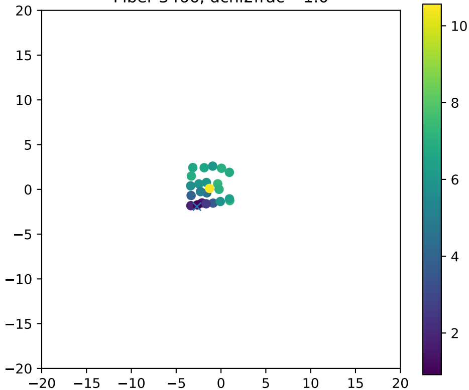
Fiber 3466, dchi2frac= 1.0
