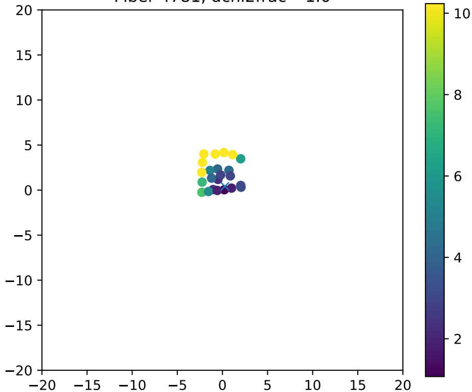
Fiber 4781, dchi2frac= 1.0
