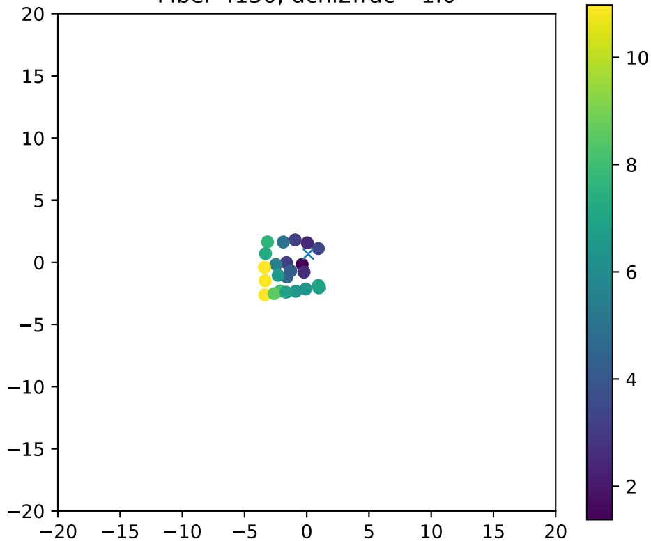
Fiber 4150, dchi2frac= 1.0
