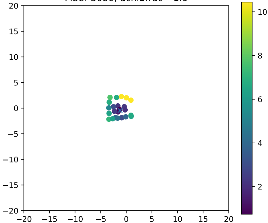
Fiber 3680, dchi2frac= 1.0
