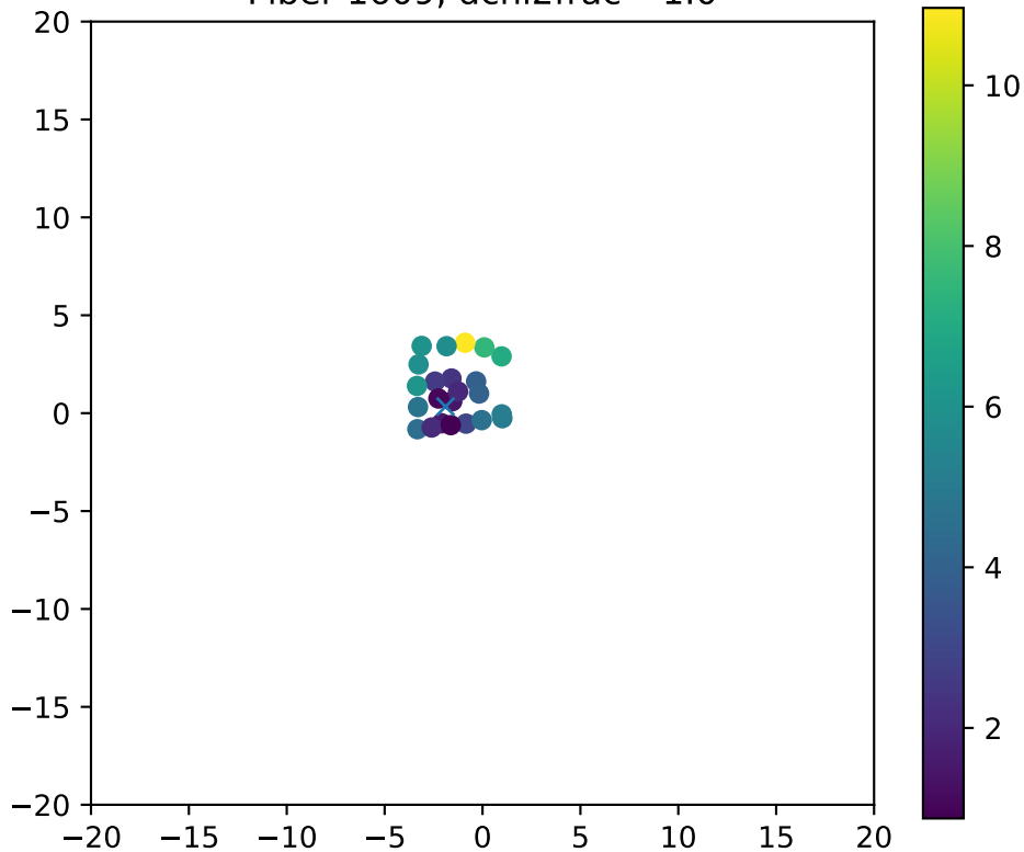
Fiber 1609, dchi2frac= 1.0
