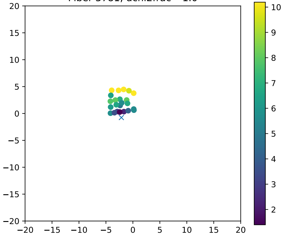
Fiber 3781, dchi2frac= 1.0
