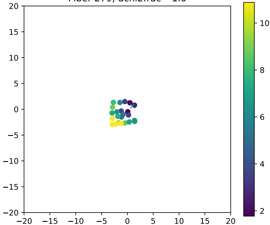
Fiber 279, dchi2frac= 1.0
