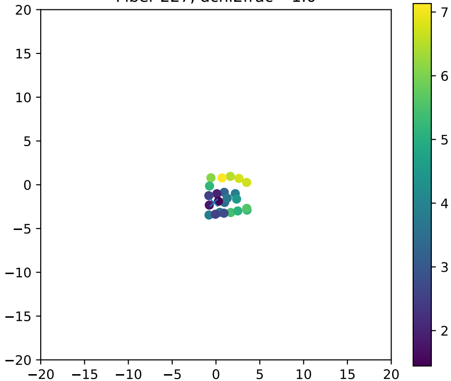
Fiber 227, dchi2frac= 1.0
