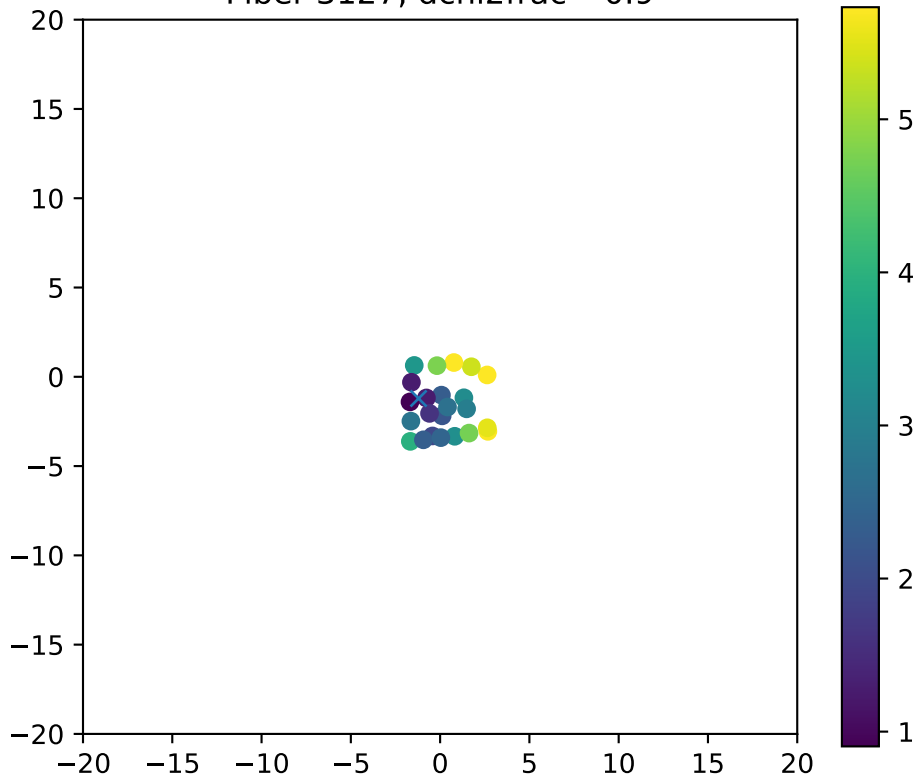
Fiber 3127, dchi2frac= 0.9
