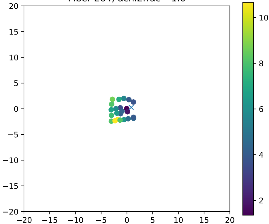
Fiber 264, dchi2frac= 1.0
