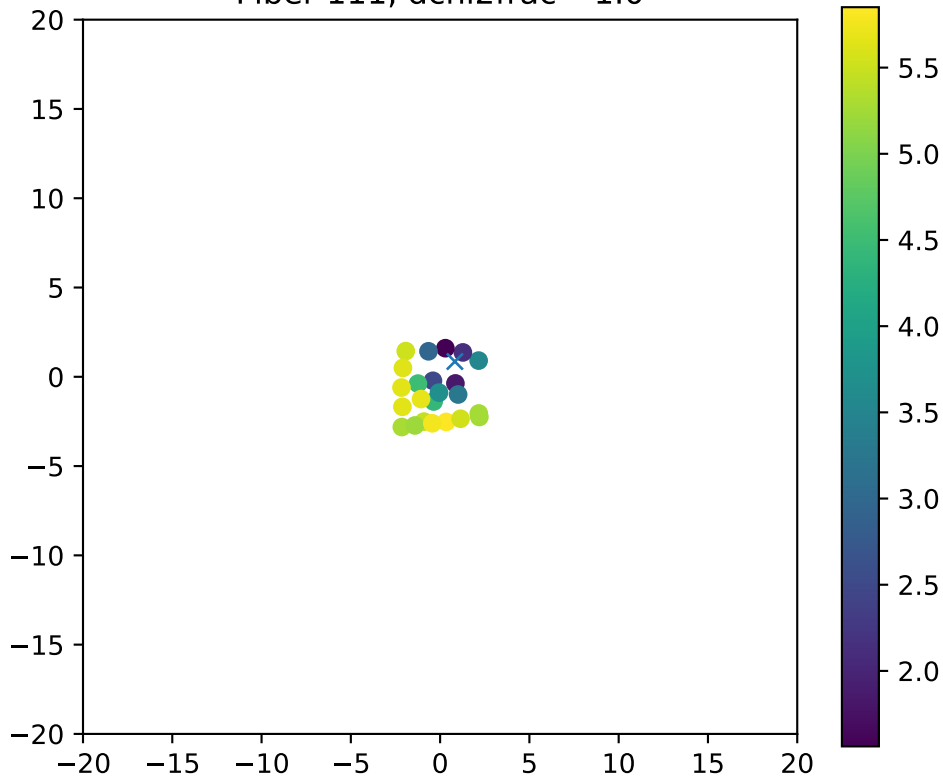
Fiber 111, dchi2frac= 1.0
