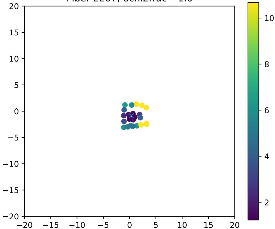
Fiber 2207, dchi2frac= 1.0
