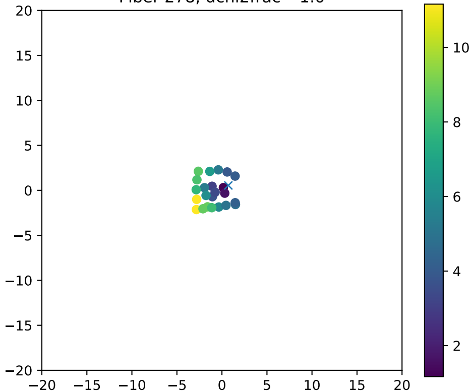
Fiber 278, dchi2frac= 1.0
