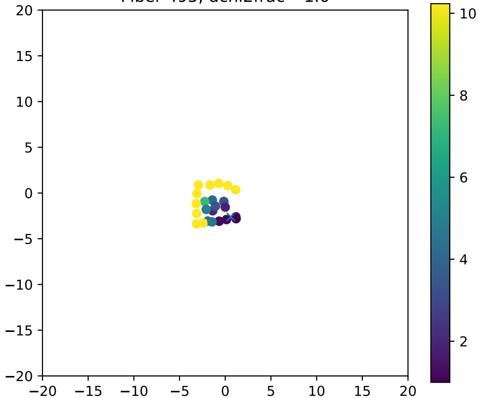
Fiber 495, dchi2frac= 1.0
