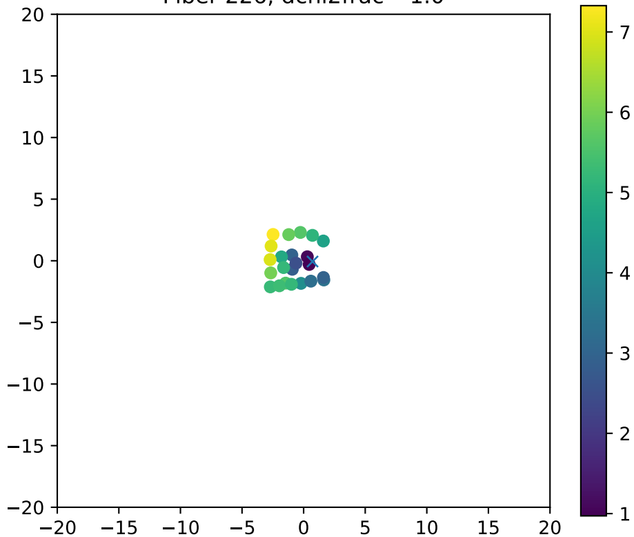
Fiber 226, dchi2frac= 1.0
