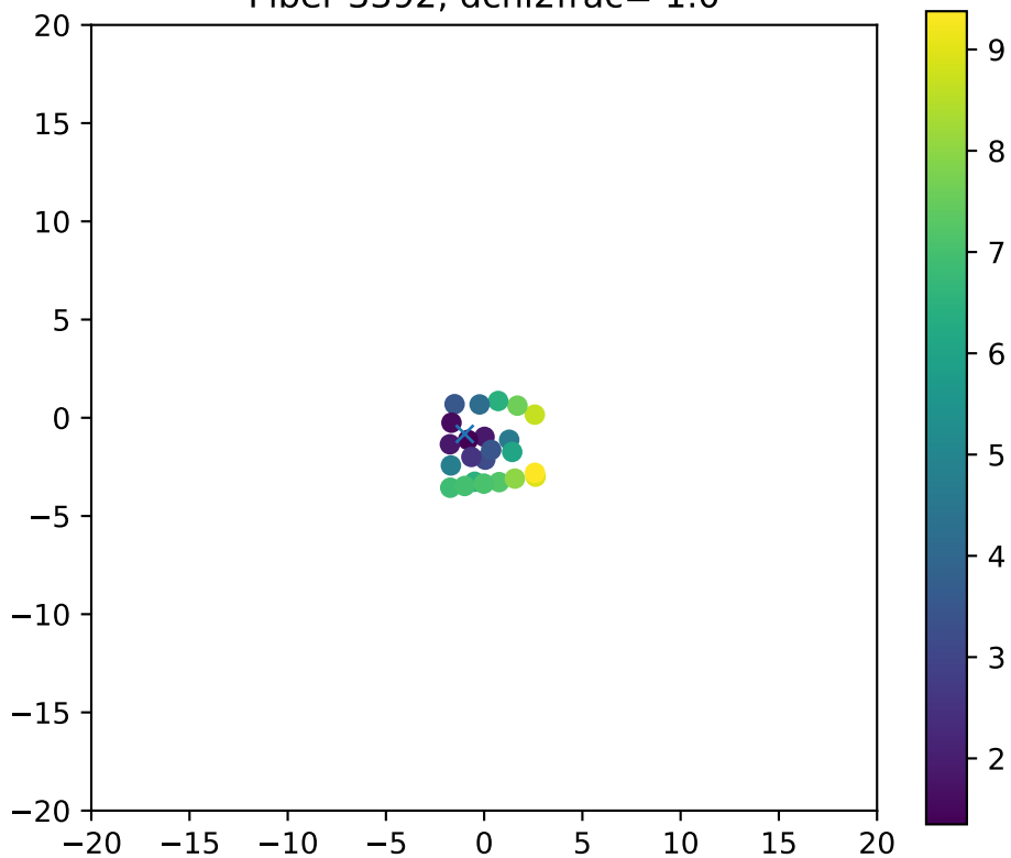
Fiber 3392, dchi2frac= 1.0
