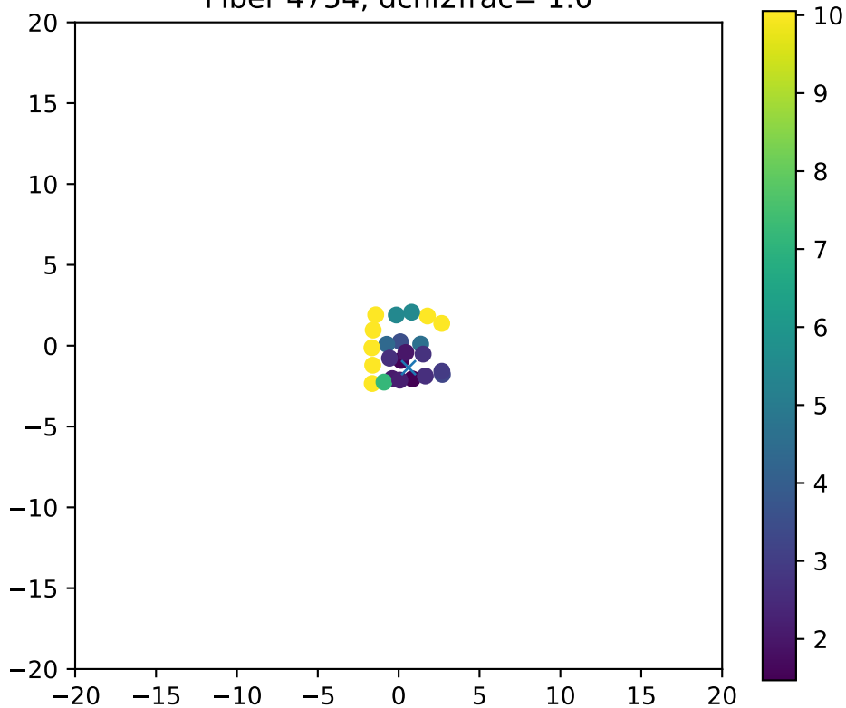
Fiber 4754, dchi2frac= 1.0
