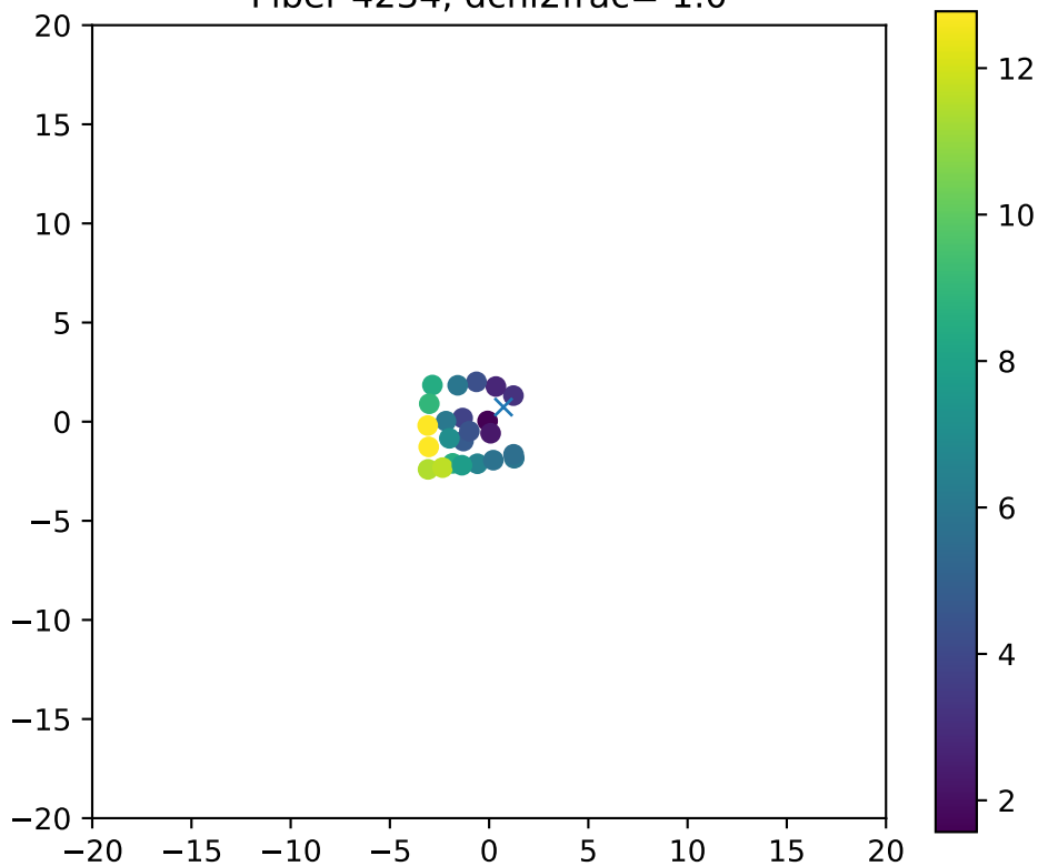
Fiber 4234, dchi2frac= 1.0
