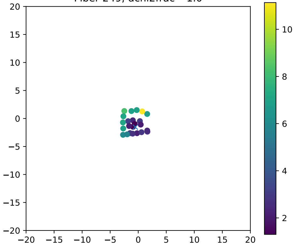
Fiber 249, dchi2frac= 1.0
