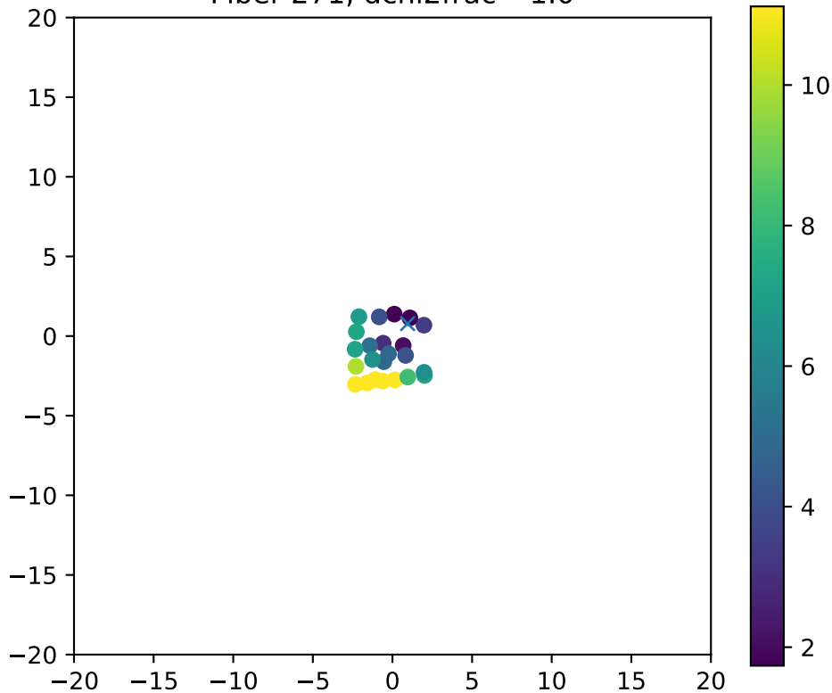
Fiber 271, dchi2frac= 1.0
