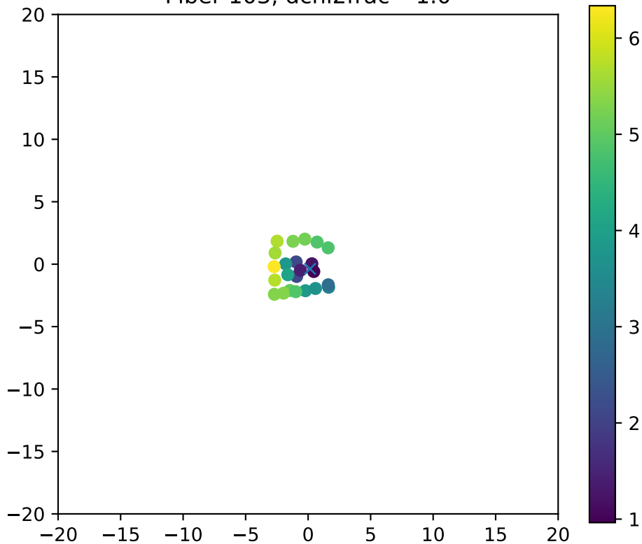
Fiber 103, dchi2frac= 1.0
