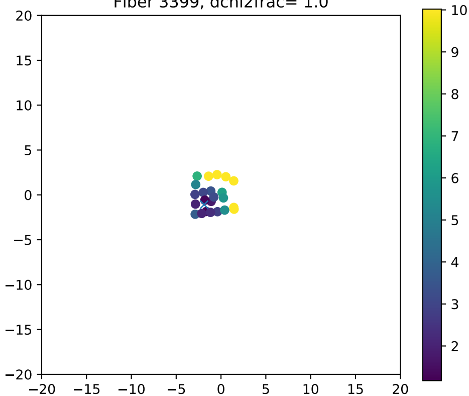
Fiber 3399, dchi2frac= 1.0
