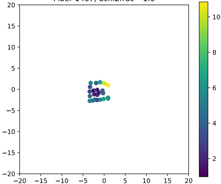
Fiber 1467, dchi2frac= 1.0
