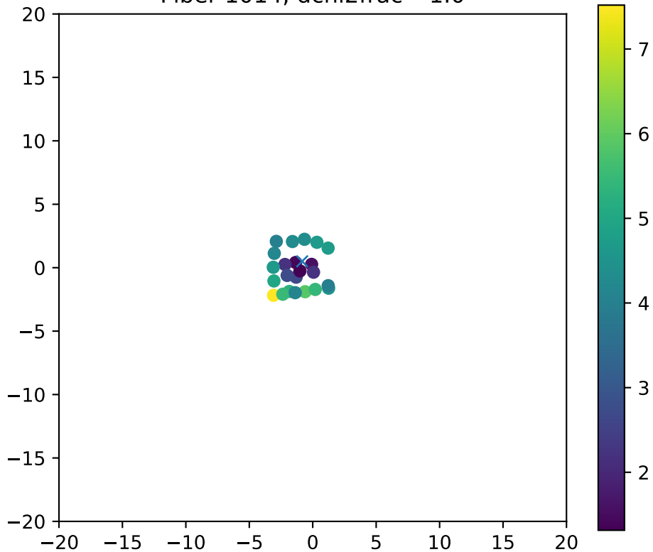
Fiber 1014, dchi2frac= 1.0
