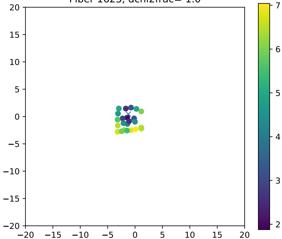
Fiber 1623, dchi2frac= 1.0
