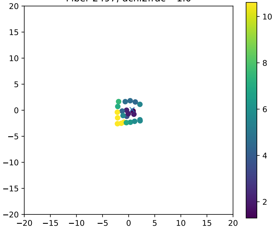
Fiber 2497, dchi2frac= 1.0
