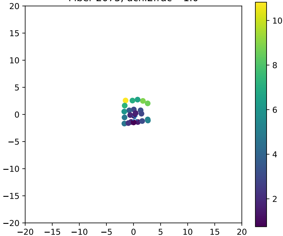
Fiber 2073, dchi2frac= 1.0
