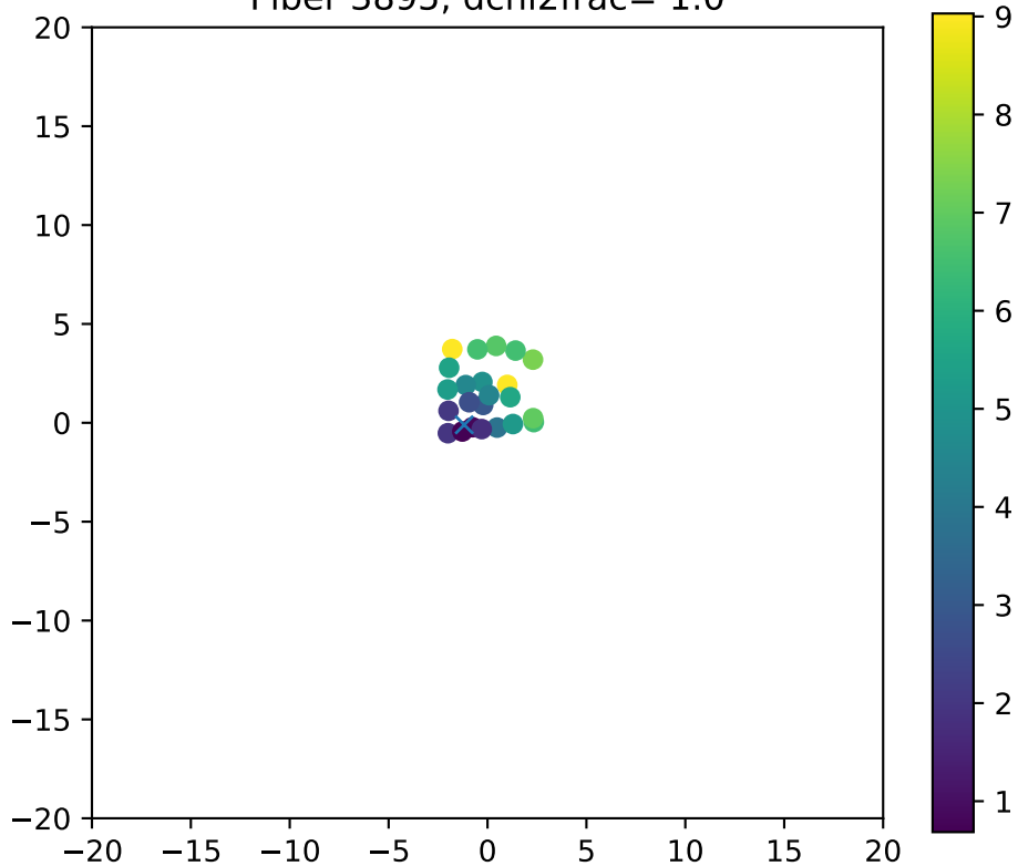
Fiber 3895, dchi2frac= 1.0
