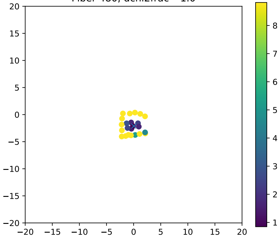
Fiber 480, dchi2frac= 1.0
