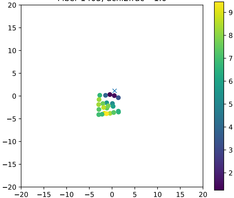
Fiber 1403, dchi2frac= 1.0
