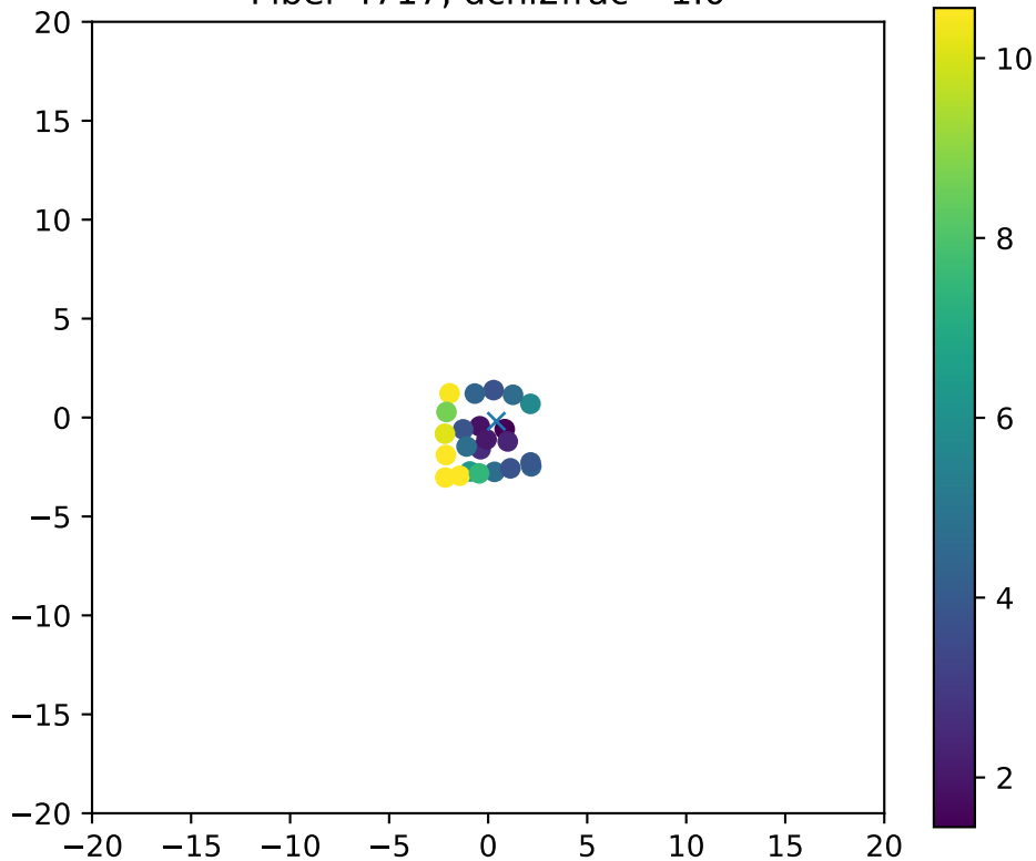
Fiber 4717, dchi2frac= 1.0
