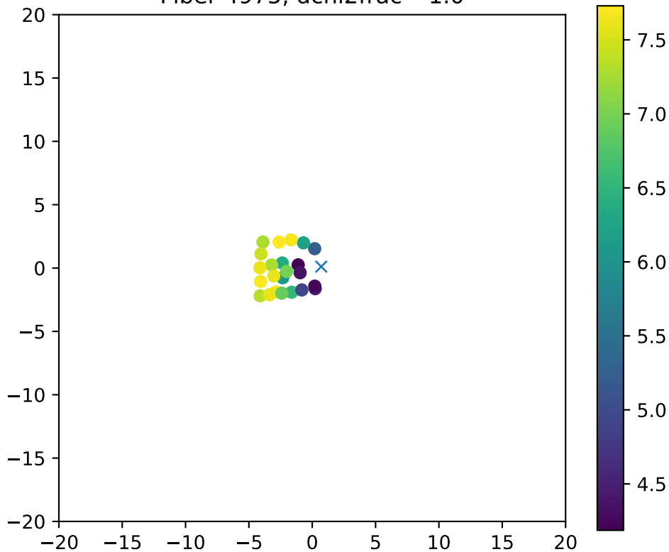
Fiber 4975, dchi2frac= 1.0
