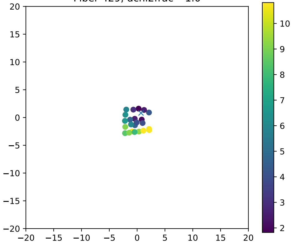
Fiber 429, dchi2frac= 1.0
