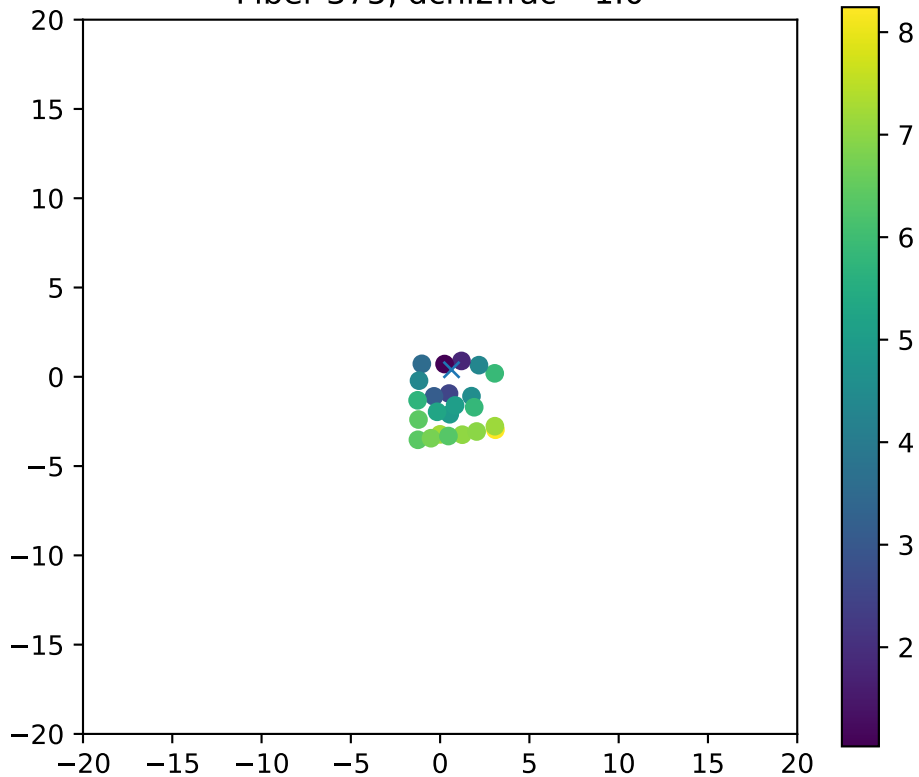
Fiber 375, dchi2frac= 1.0
