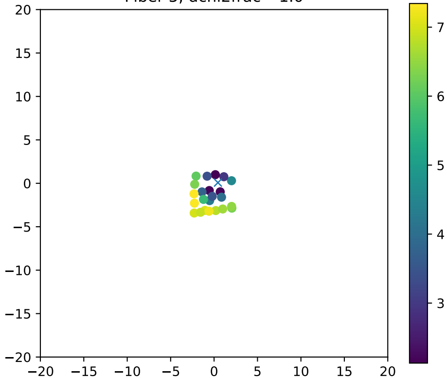
Fiber 5, dchi2frac= 1.0
