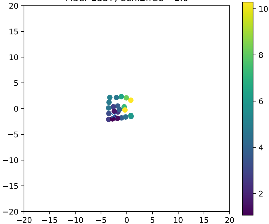
Fiber 1357, dchi2frac= 1.0
