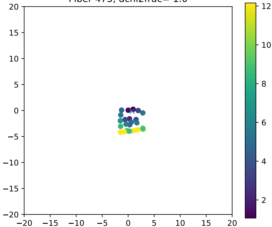
Fiber 475, dchi2frac= 1.0
