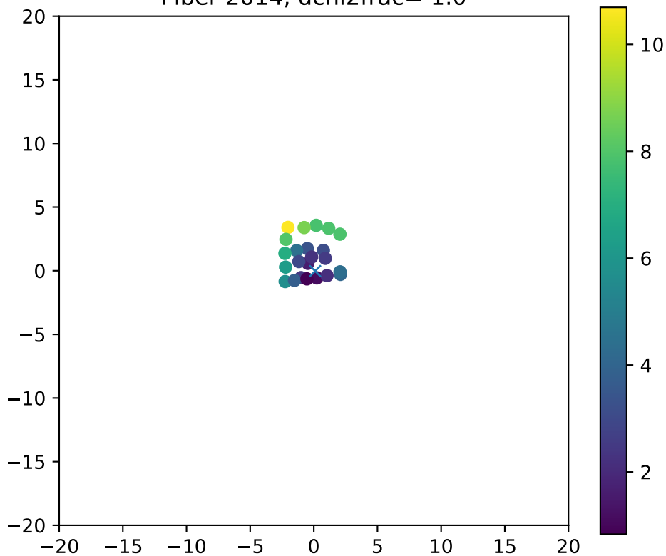
Fiber 2014, dchi2frac= 1.0
