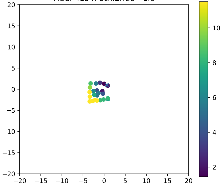
Fiber 4134, dchi2frac= 1.0
