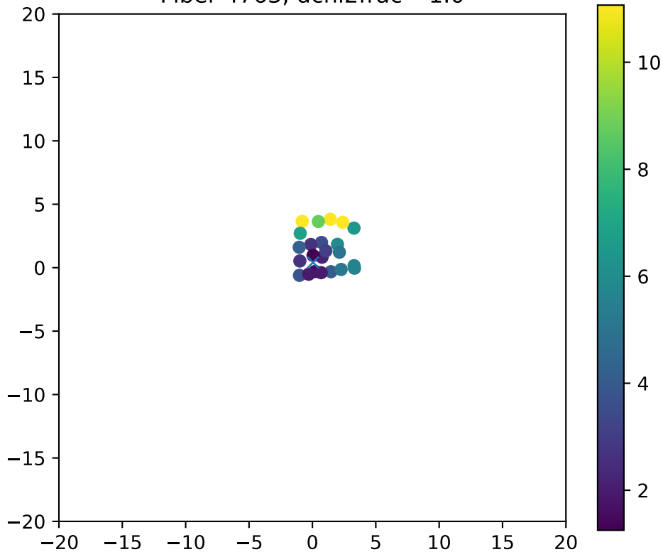
Fiber 4763, dchi2frac= 1.0
