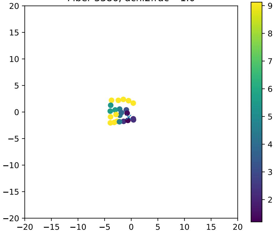
Fiber 3386, dchi2frac= 1.0
