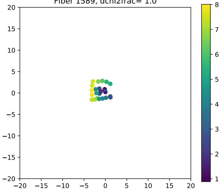
Fiber 1589, dchi2frac= 1.0
