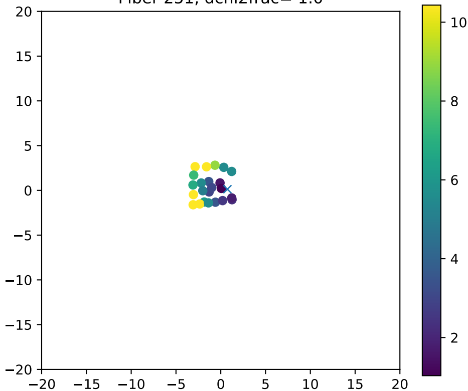
Fiber 251, dchi2frac= 1.0
