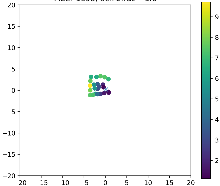
Fiber 1658, dchi2frac= 1.0
