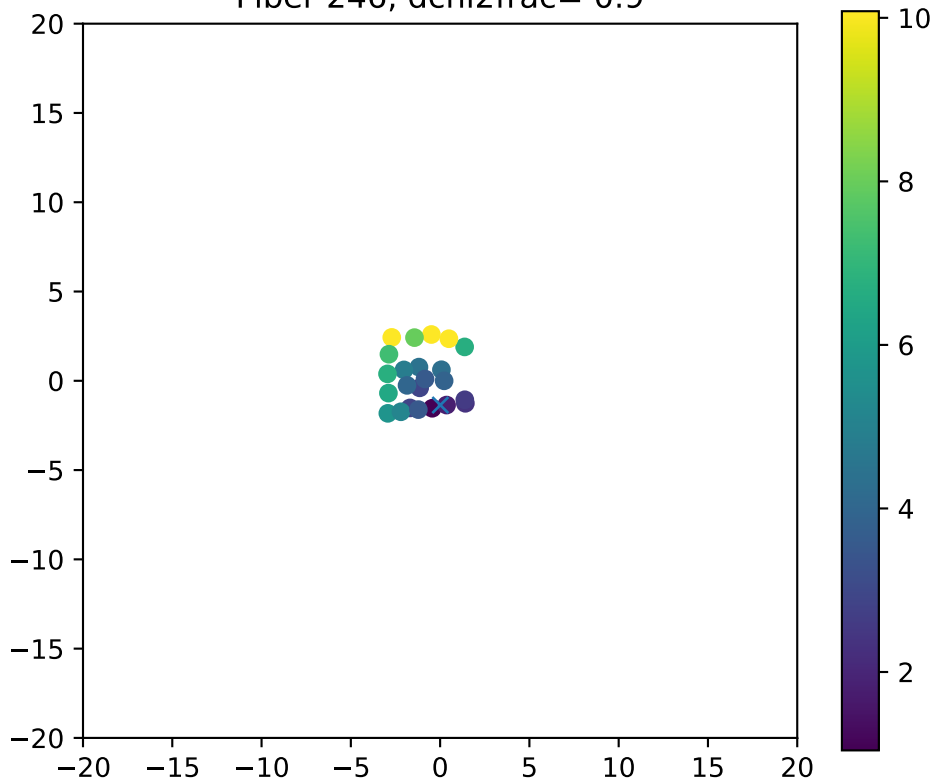
Fiber 246, dchi2frac= 0.9
