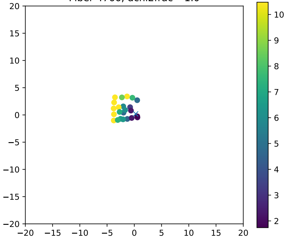
Fiber 4766, dchi2frac= 1.0
