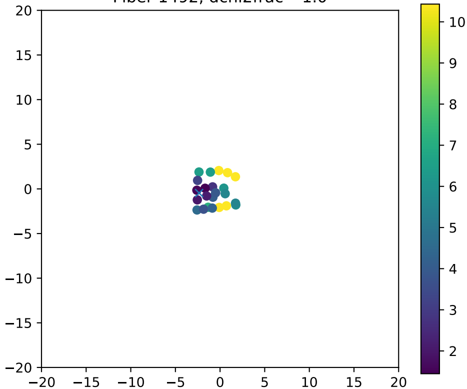
Fiber 1492, dchi2frac= 1.0
