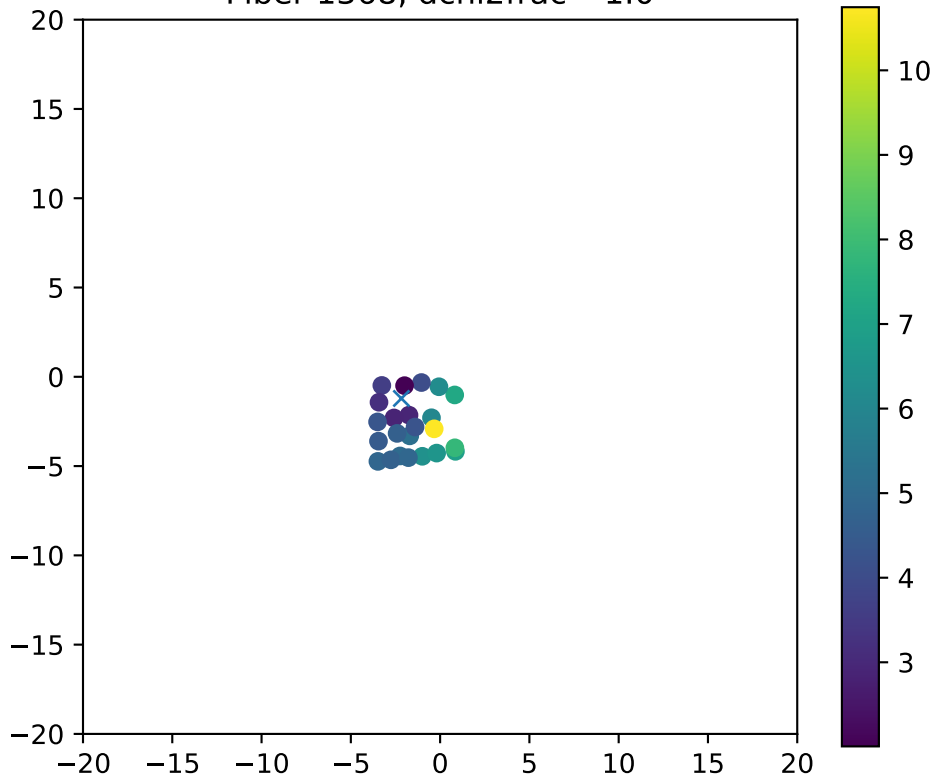
Fiber 1368, dchi2frac= 1.0
