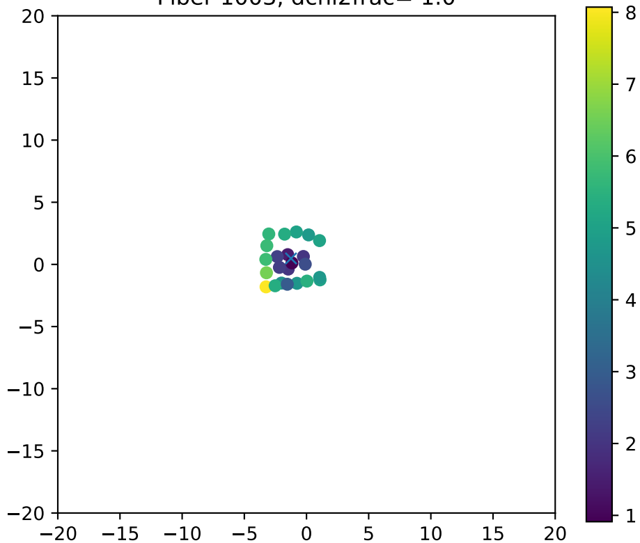
Fiber 1003, dchi2frac= 1.0
