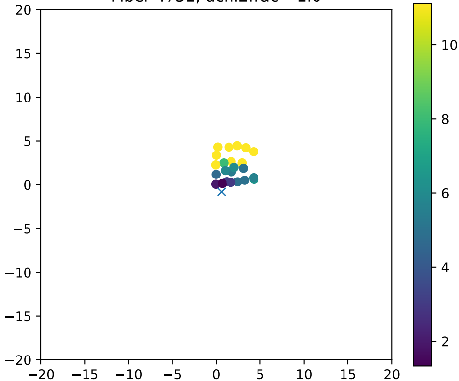
Fiber 4731, dchi2frac= 1.0
