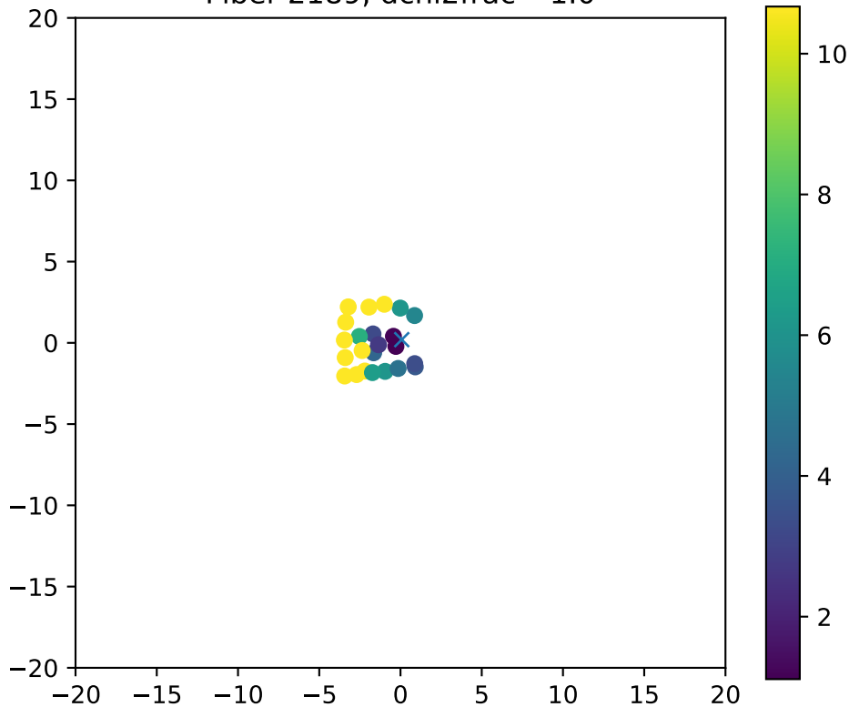
Fiber 2189, dchi2frac= 1.0
