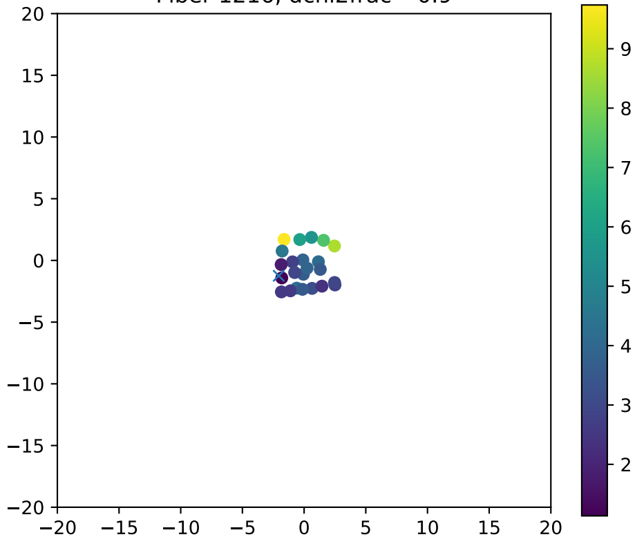
Fiber 1216, dchi2frac= 0.9
