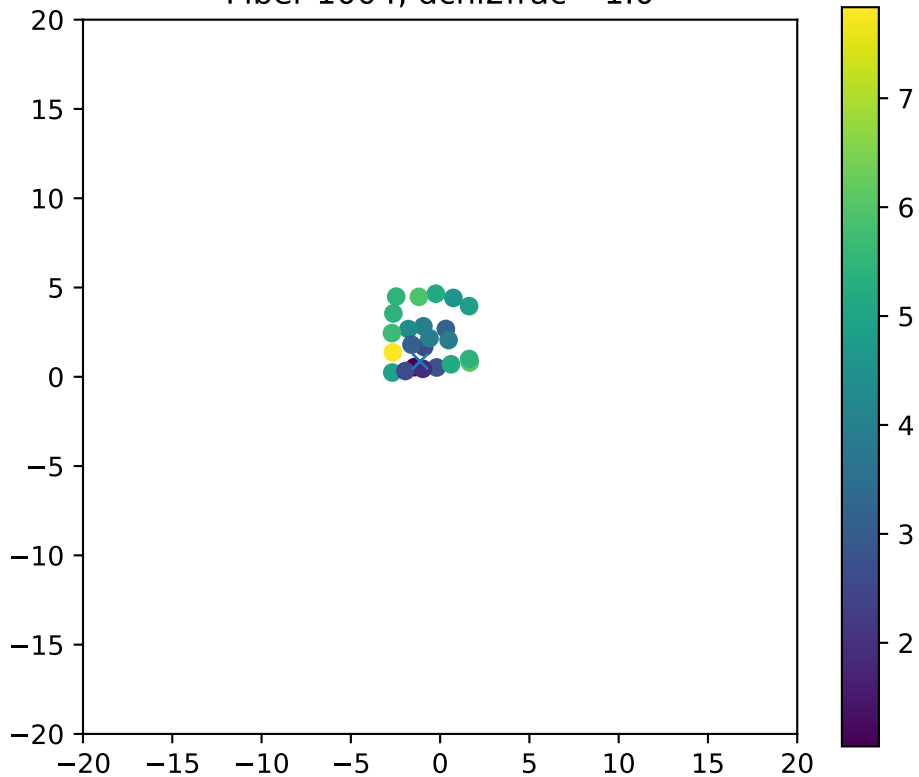
Fiber 1004, dchi2frac= 1.0
