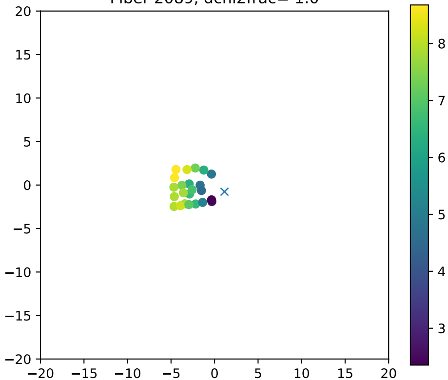
Fiber 2089, dchi2frac= 1.0
