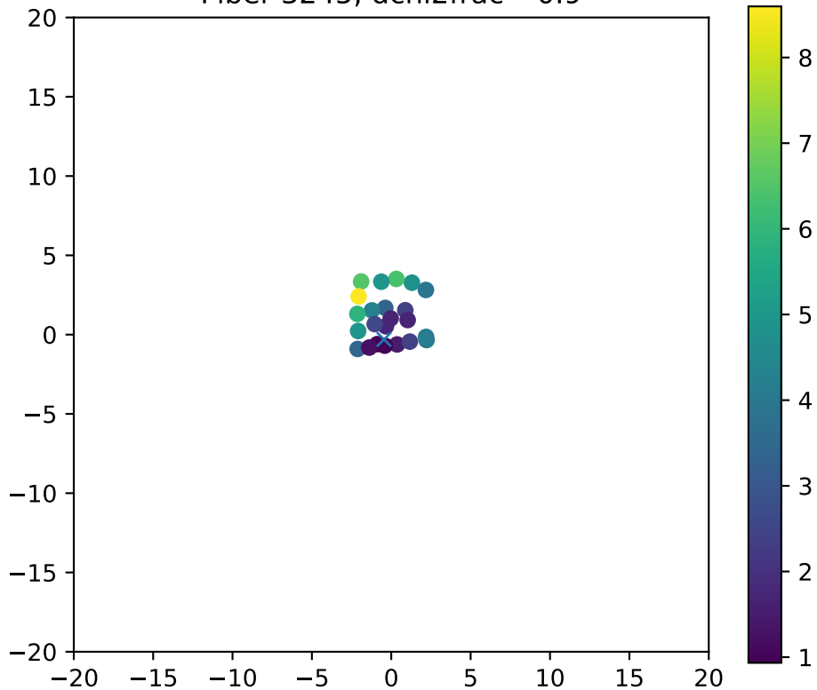
Fiber 3245, dchi2frac= 0.9
