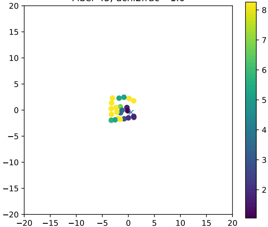
Fiber 45, dchi2frac= 1.0
