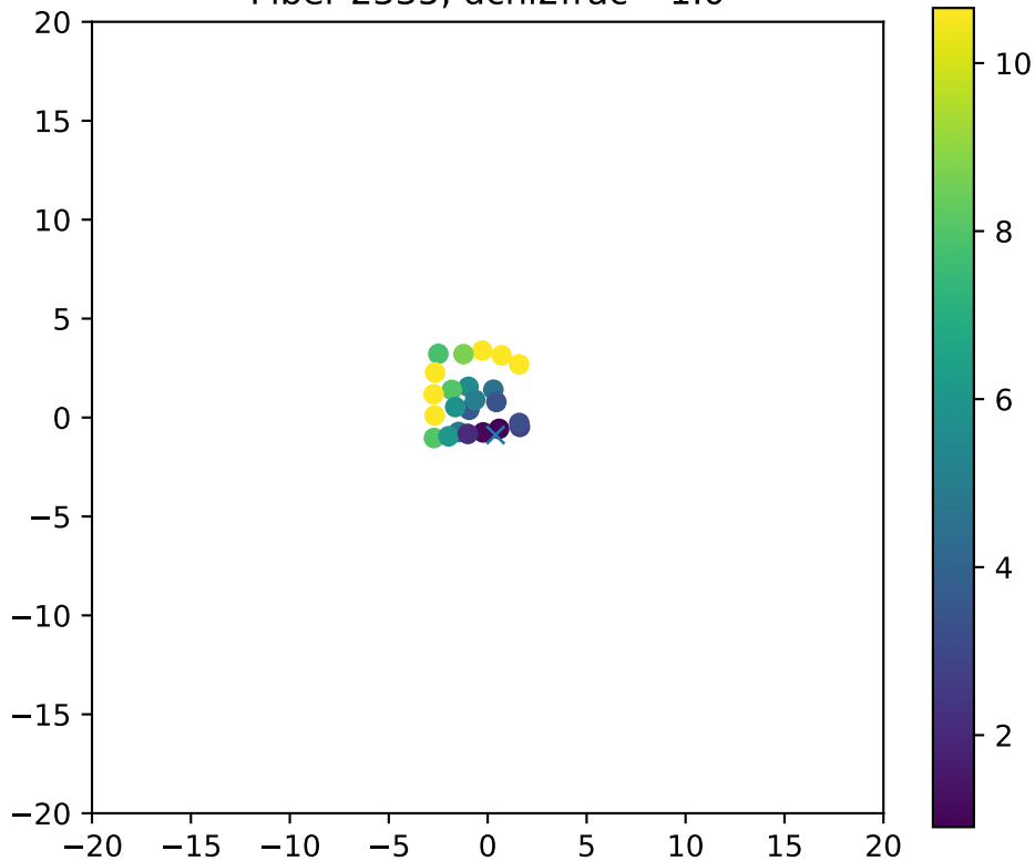
Fiber 2335, dchi2frac= 1.0
