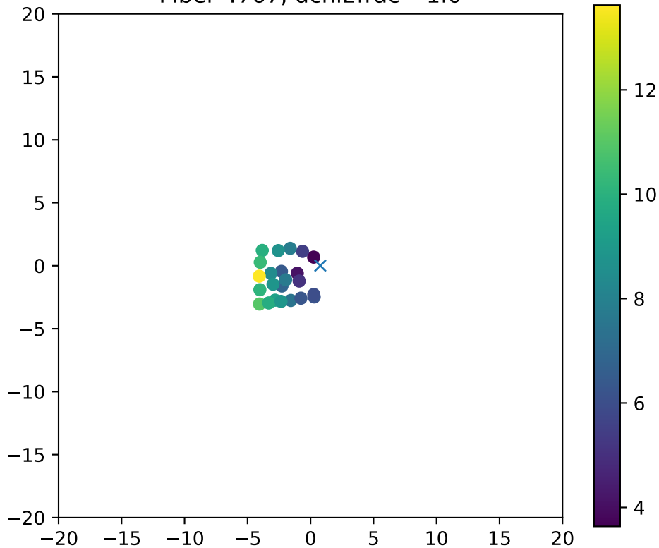
Fiber 4767, dchi2frac= 1.0
