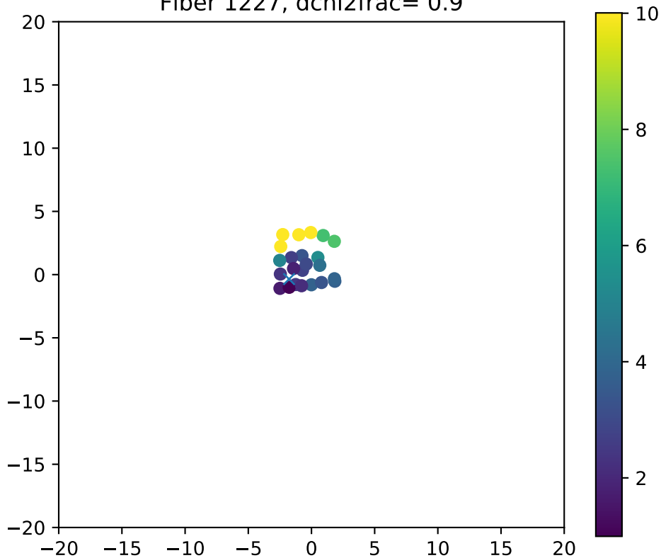
Fiber 1227, dchi2frac= 0.9
