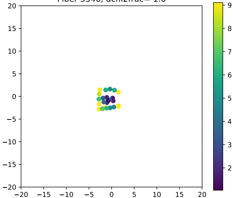
Fiber 3346, dchi2frac= 1.0
