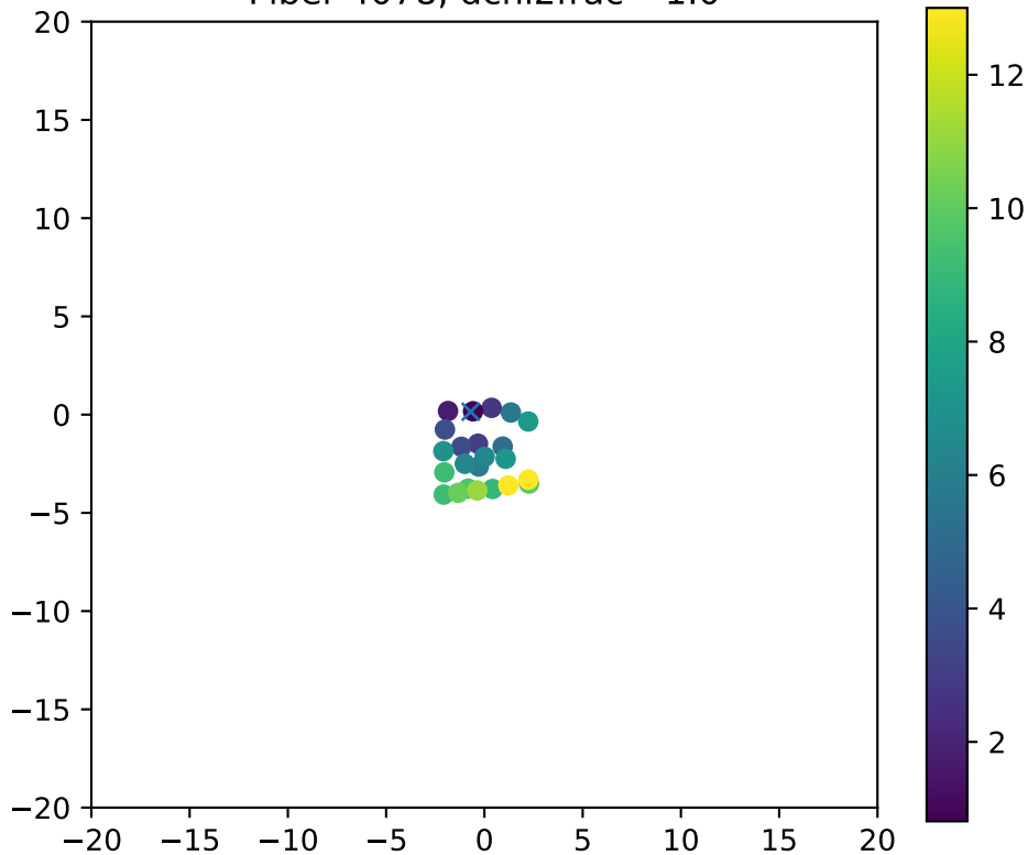
Fiber 4078, dchi2frac= 1.0
