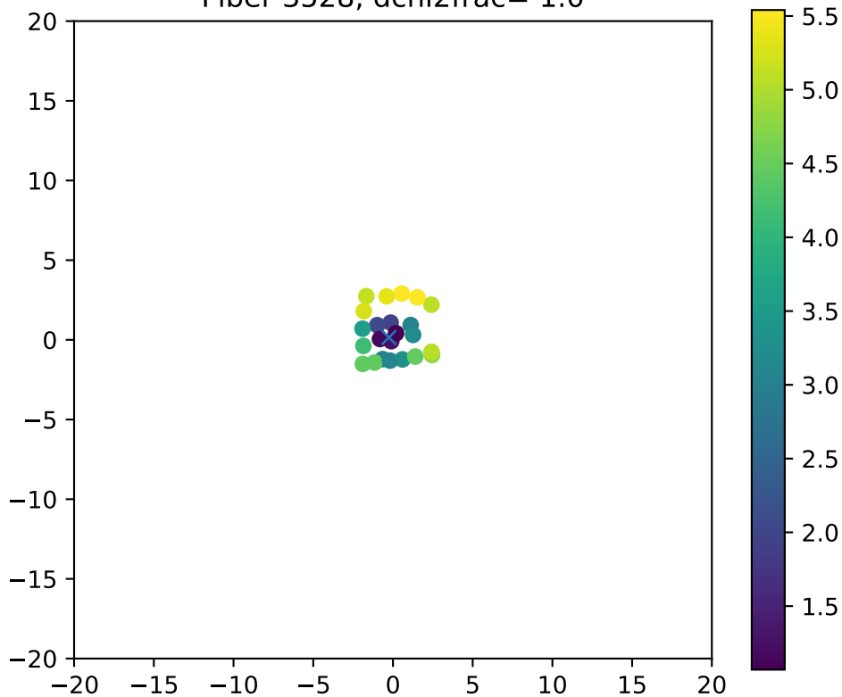
Fiber 3528, dchi2frac= 1.0
