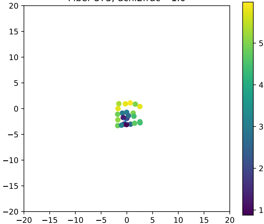
Fiber 373, dchi2frac= 1.0
