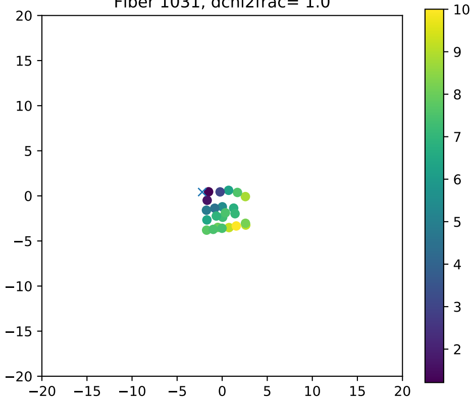
Fiber 1031, dchi2frac= 1.0
