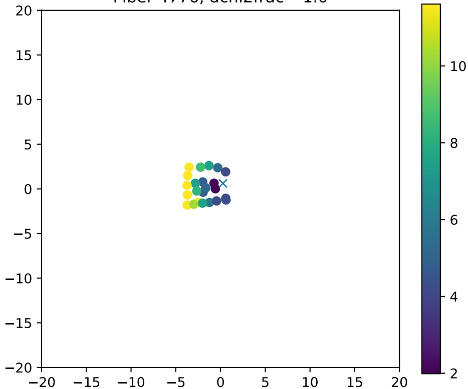
Fiber 4776, dchi2frac= 1.0
