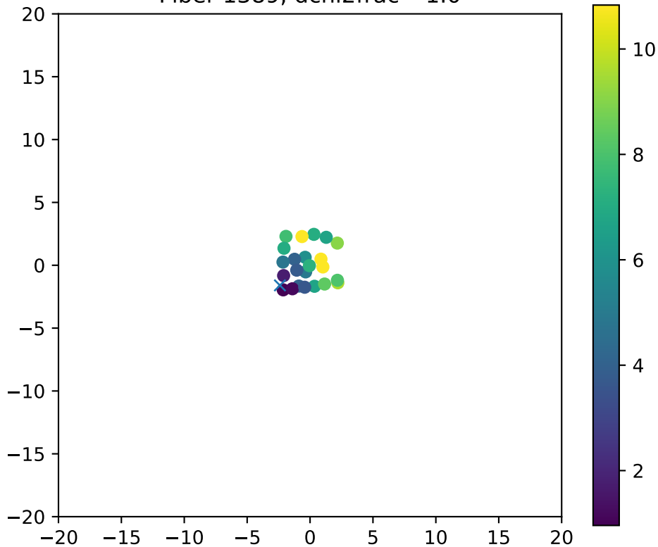
Fiber 1389, dchi2frac= 1.0
