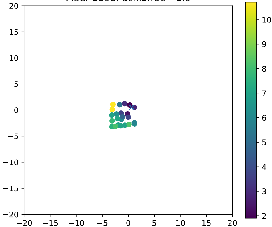
Fiber 2006, dchi2frac= 1.0
