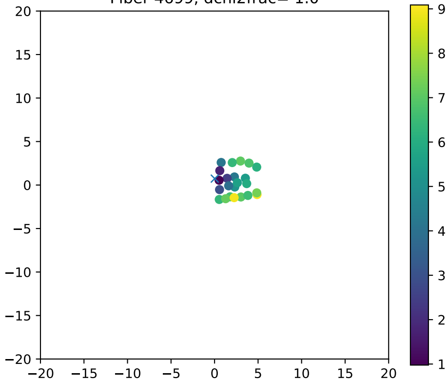
Fiber 4699, dchi2frac= 1.0
