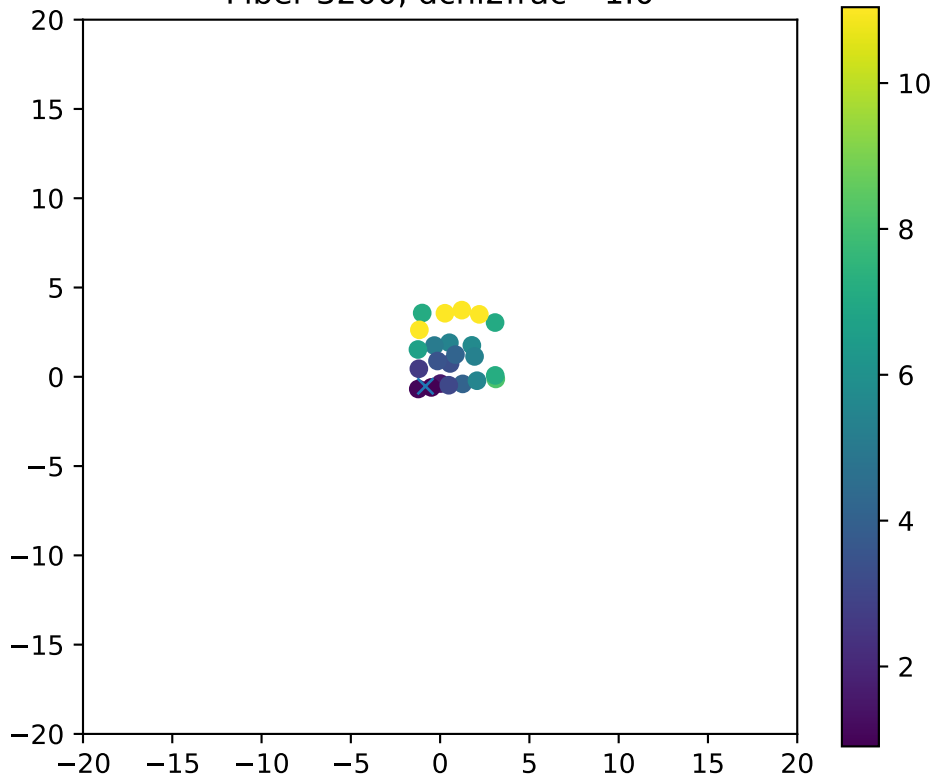
Fiber 3200, dchi2frac= 1.0
