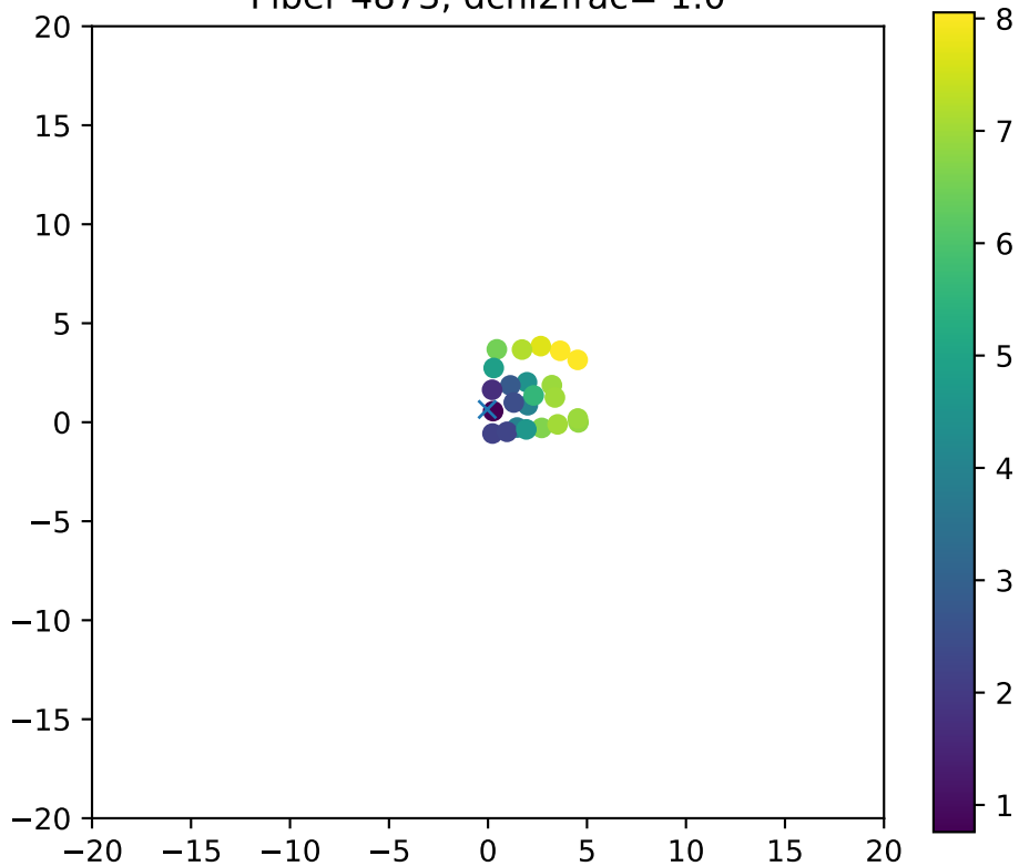
Fiber 4873, dchi2frac= 1.0
