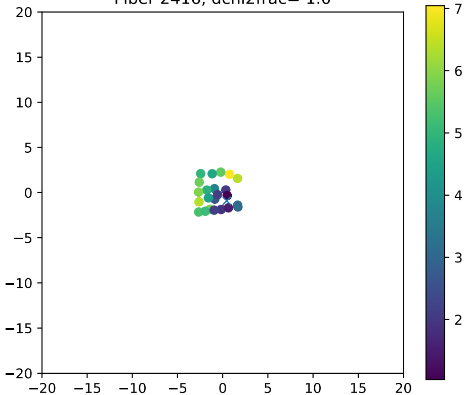
Fiber 2416, dchi2frac= 1.0
