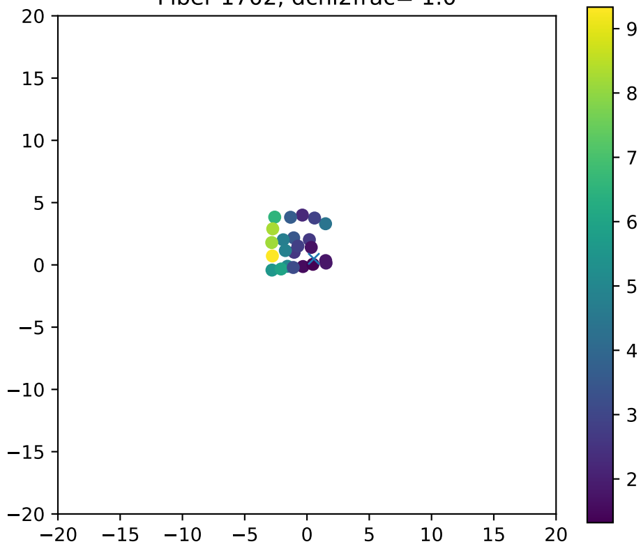
Fiber 1702, dchi2frac= 1.0
