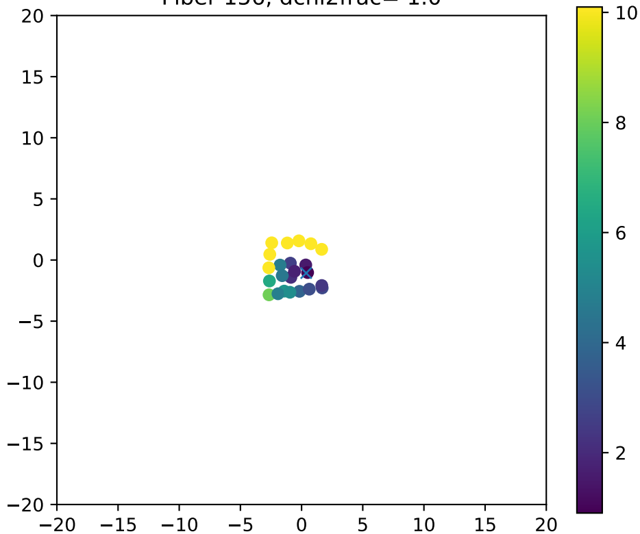
Fiber 156, dchi2frac= 1.0
