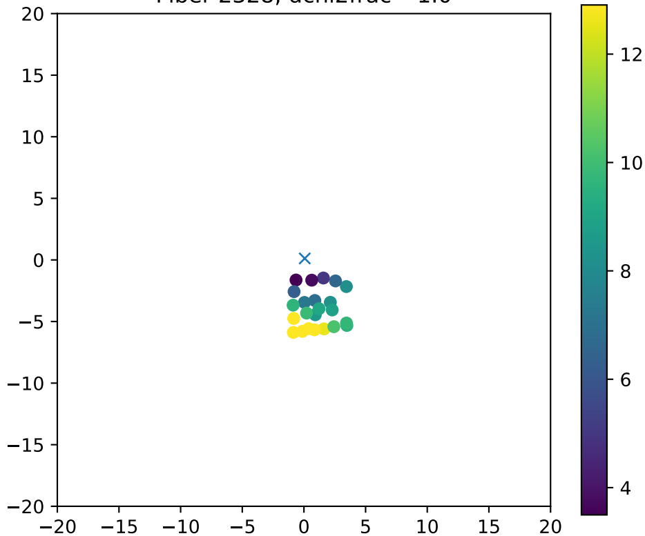
Fiber 2328, dchi2frac= 1.0
