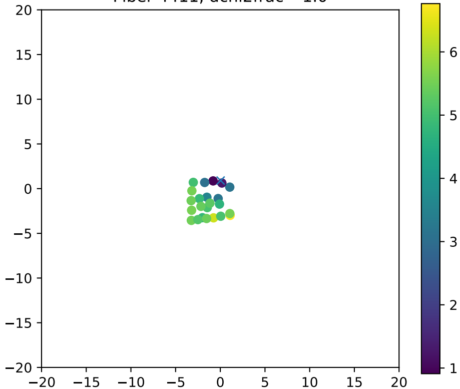
Fiber 4411, dchi2frac= 1.0
