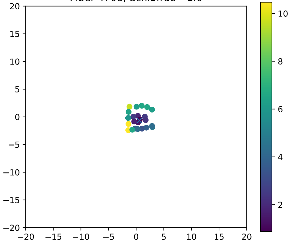
Fiber 4706, dchi2frac= 1.0
