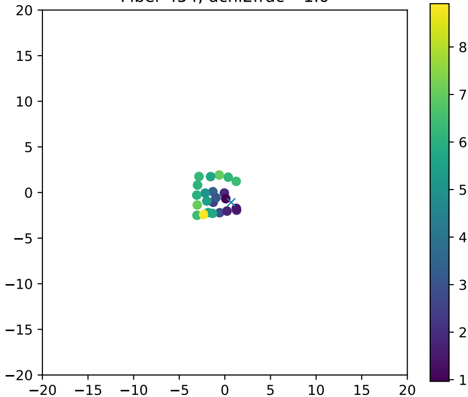
Fiber 454, dchi2frac= 1.0
