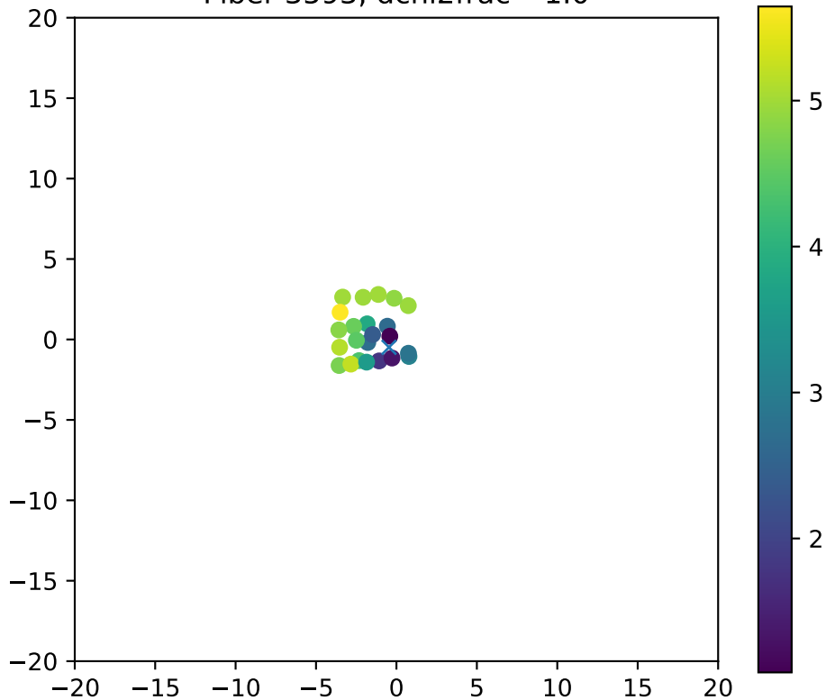
Fiber 3593, dchi2frac= 1.0
