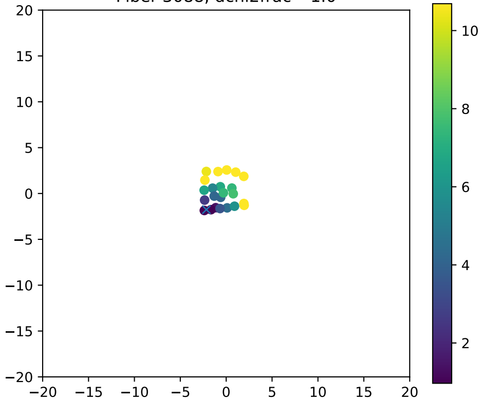
Fiber 3088, dchi2frac= 1.0
