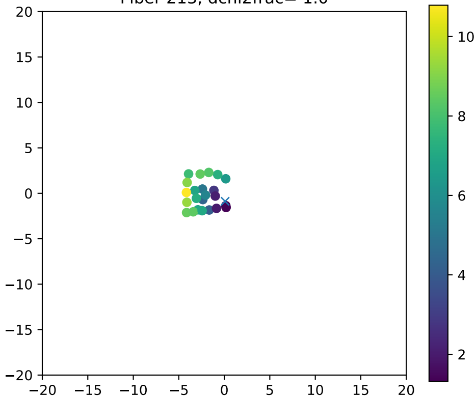
Fiber 213, dchi2frac= 1.0
