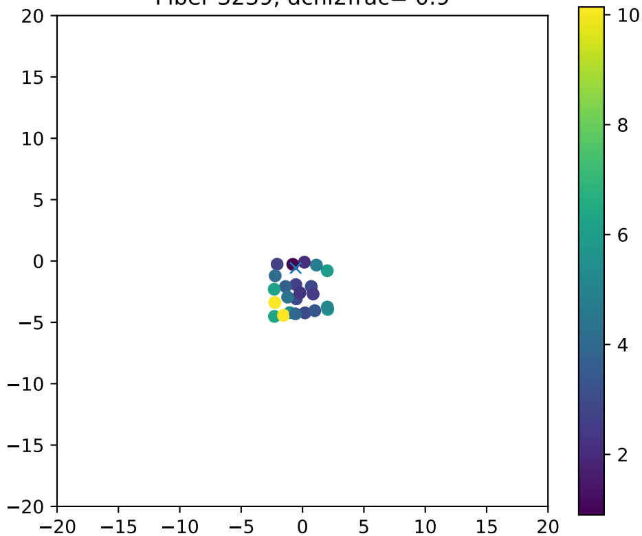
Fiber 3239, dchi2frac= 0.9
