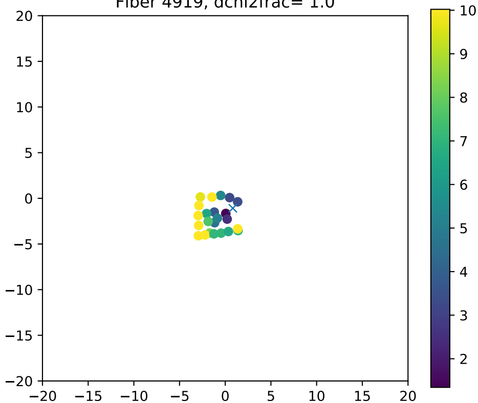
Fiber 4919, dchi2frac= 1.0
