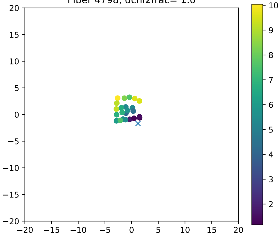
Fiber 4798, dchi2frac= 1.0
