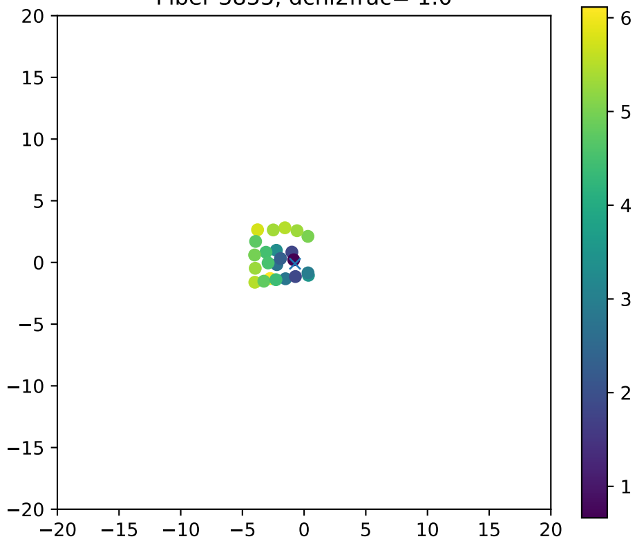
Fiber 3855, dchi2frac= 1.0
