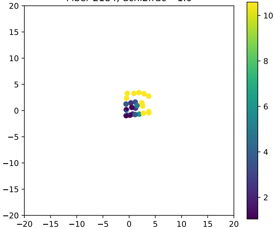
Fiber 2184, dchi2frac= 1.0
