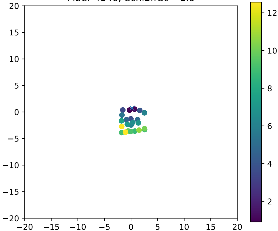
Fiber 4140, dchi2frac= 1.0
