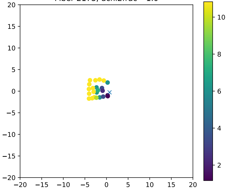
Fiber 2173, dchi2frac= 1.0
