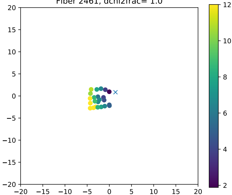
Fiber 2461, dchi2frac= 1.0
