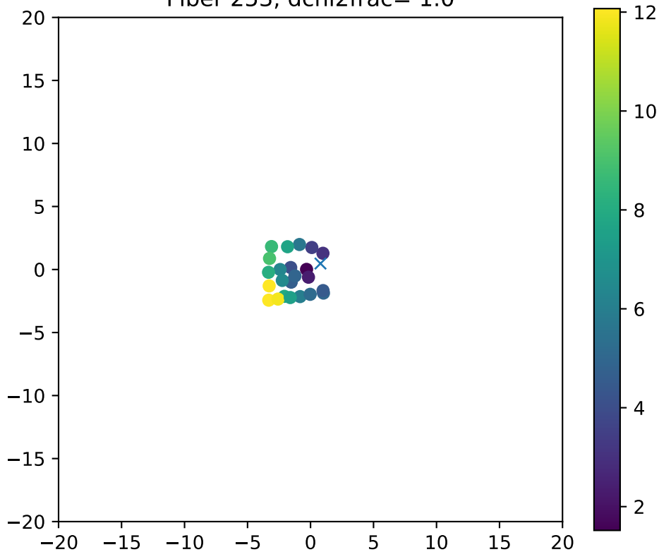
Fiber 253, dchi2frac= 1.0
