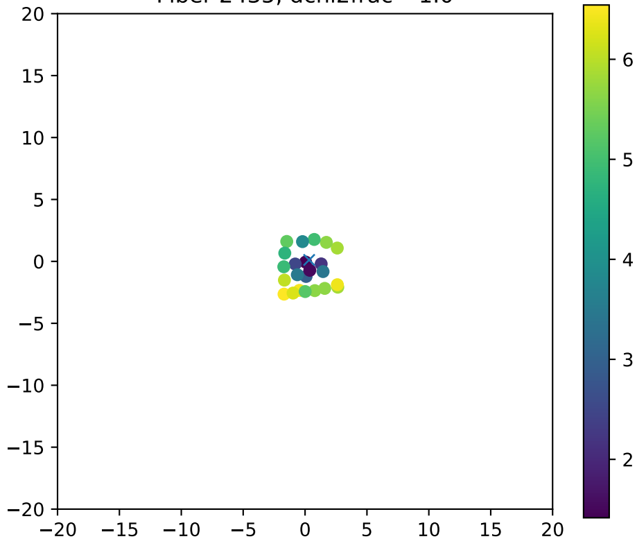
Fiber 2435, dchi2frac= 1.0
