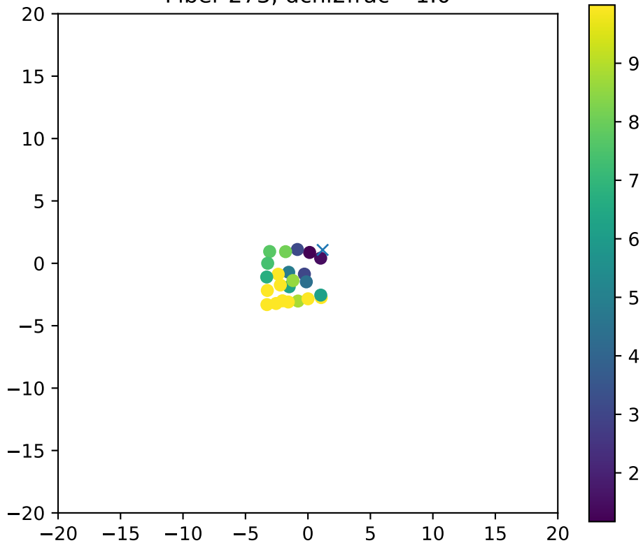
Fiber 273, dchi2frac= 1.0
