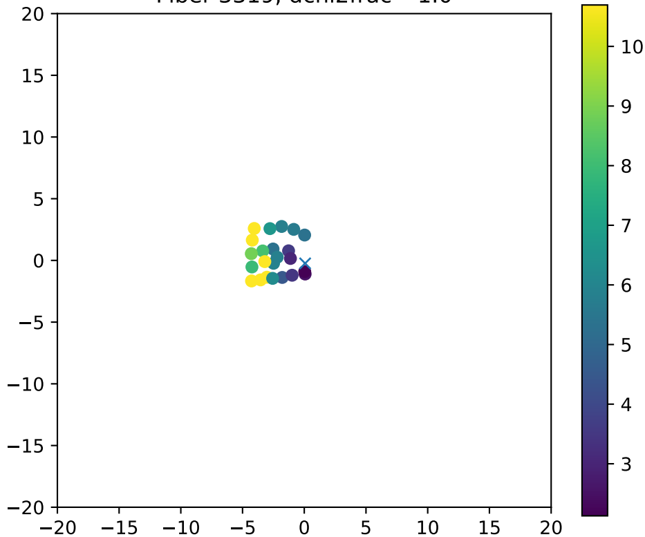
Fiber 3319, dchi2frac= 1.0
