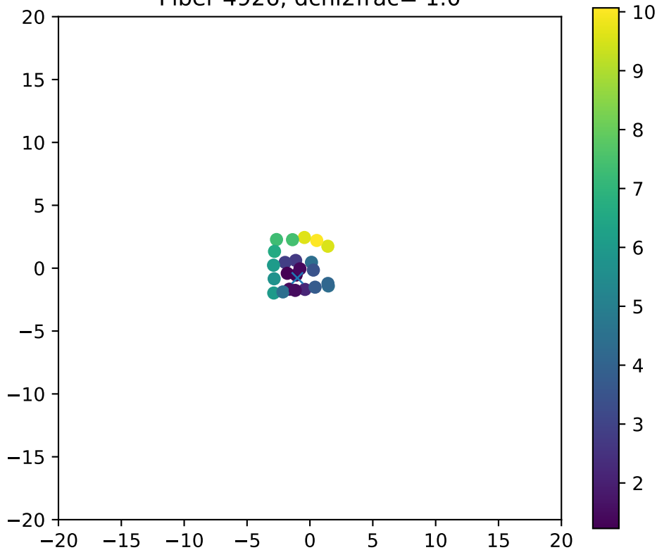
Fiber 4926, dchi2frac= 1.0
