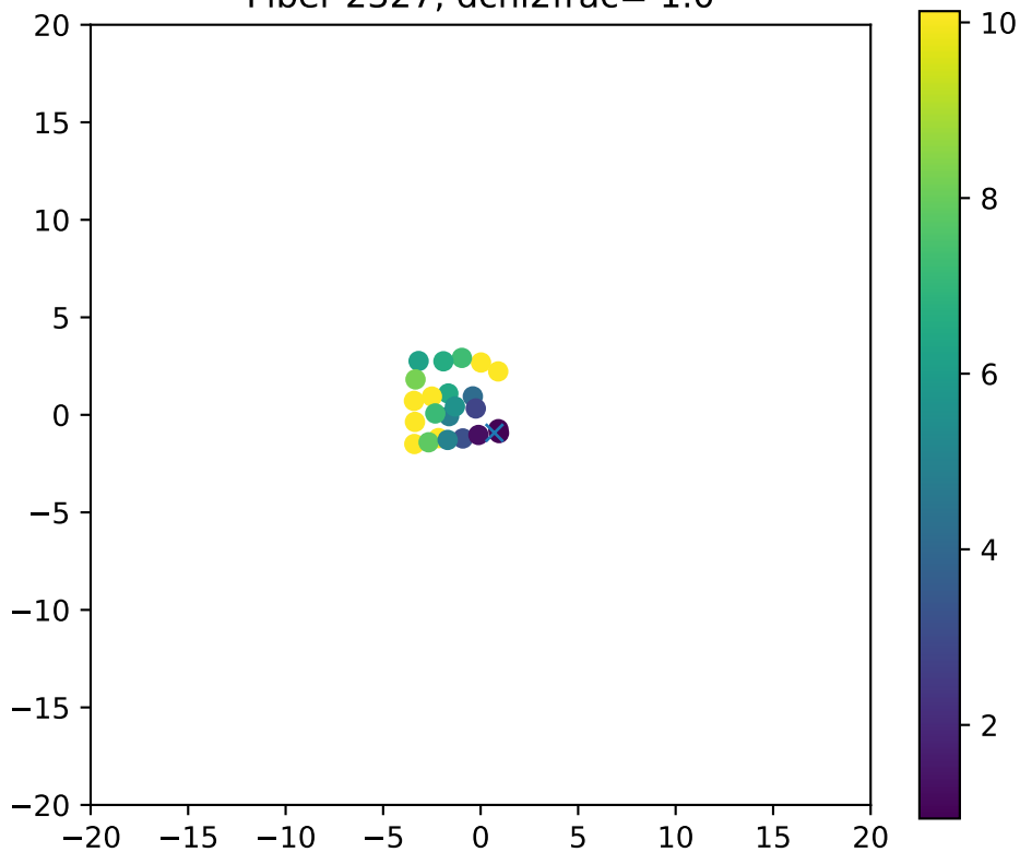
Fiber 2327, dchi2frac= 1.0
