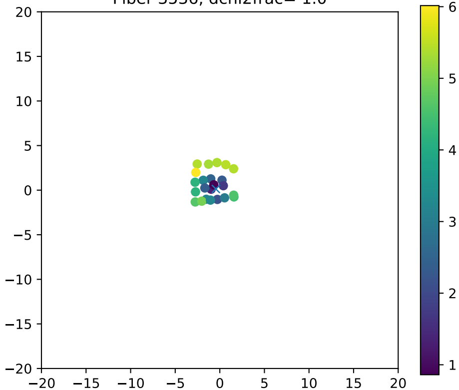
Fiber 3536, dchi2frac= 1.0
