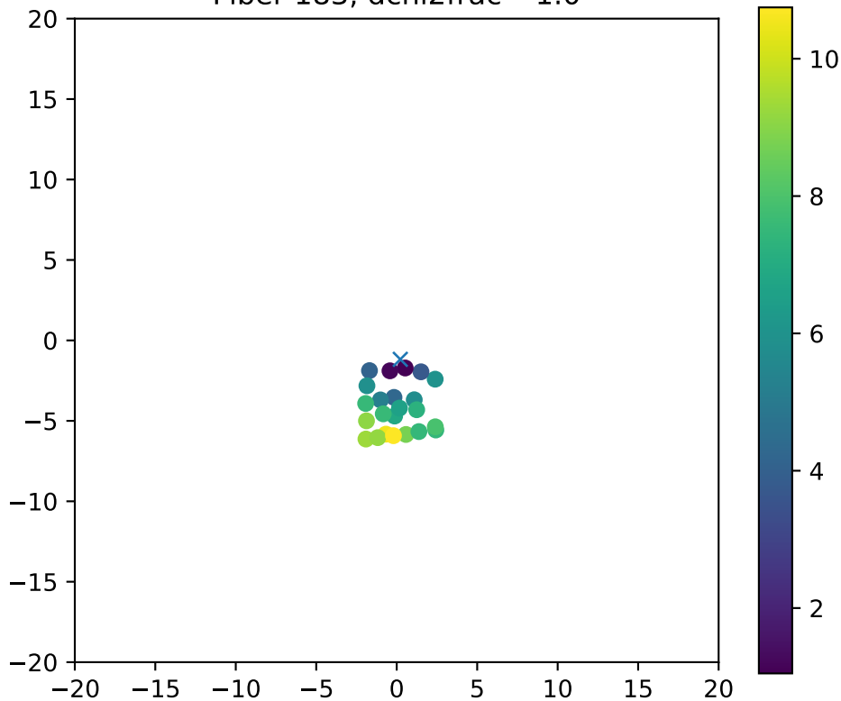
Fiber 183, dchi2frac= 1.0
