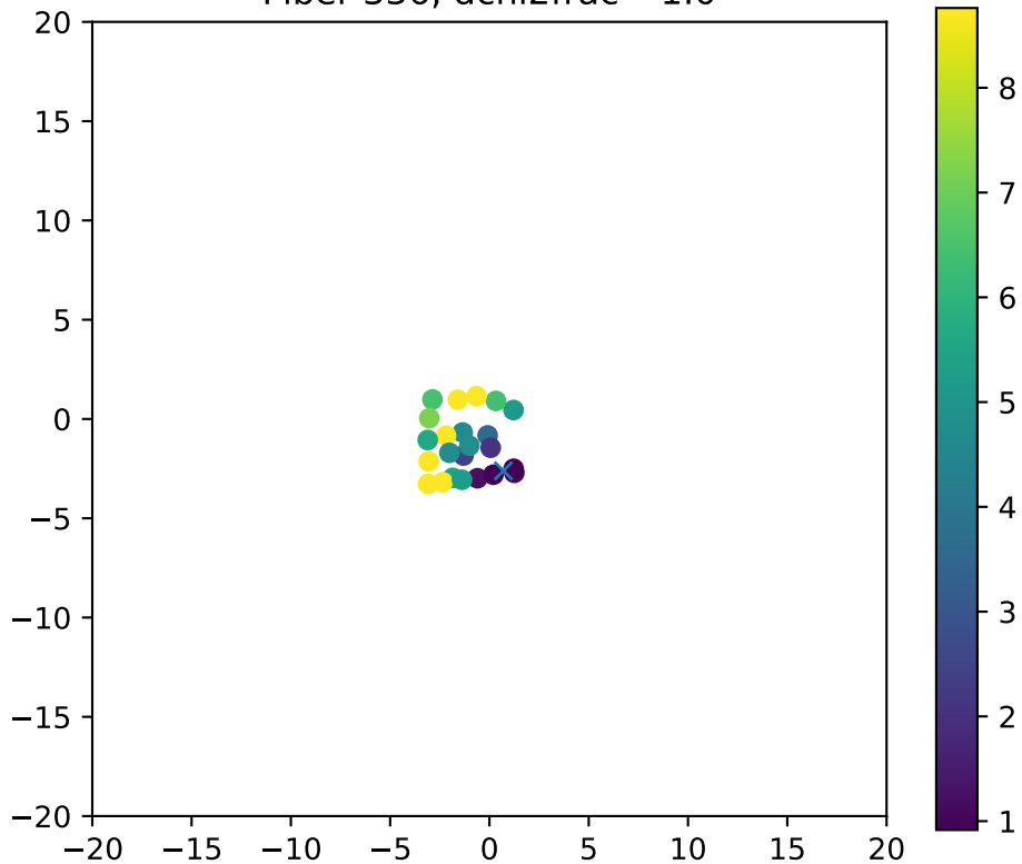
Fiber 336, dchi2frac= 1.0
