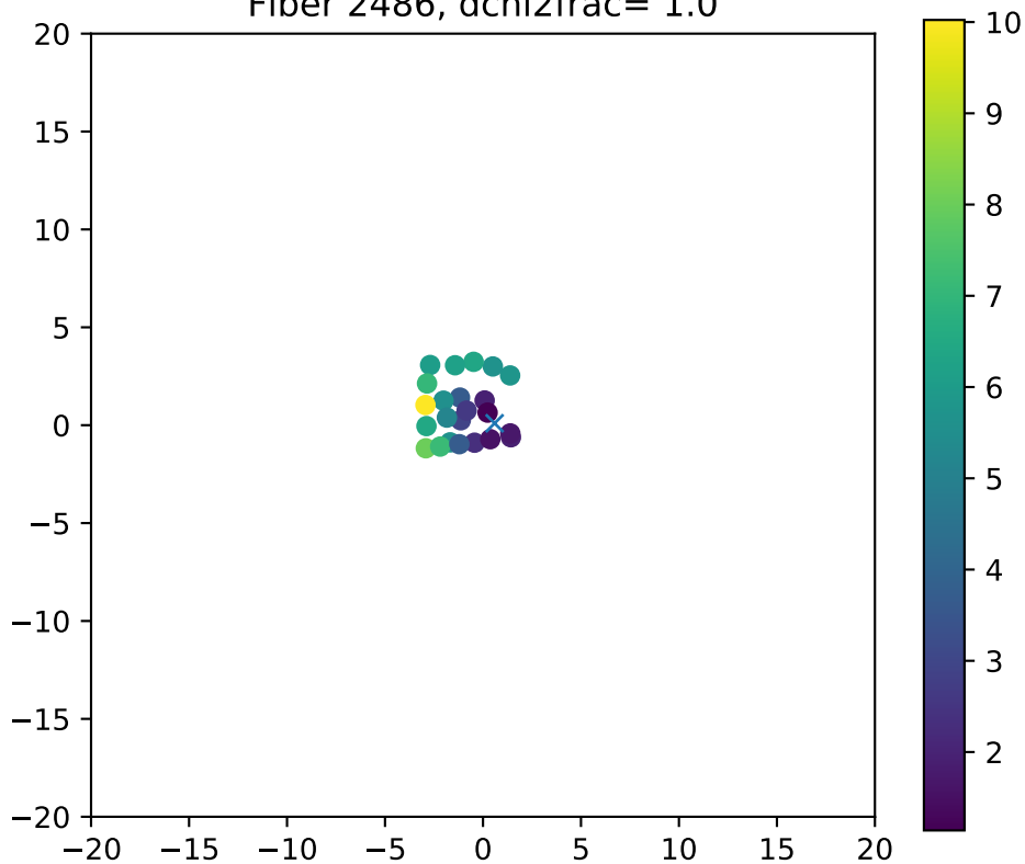
Fiber 2486, dchi2frac= 1.0
