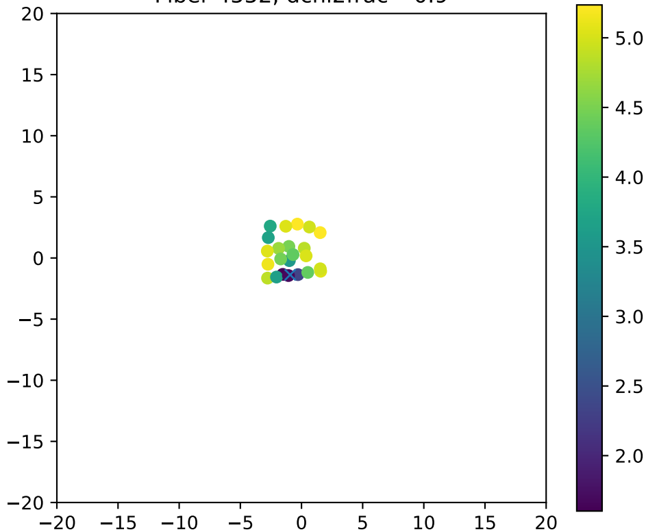
Fiber 4552, dchi2frac= 0.9
