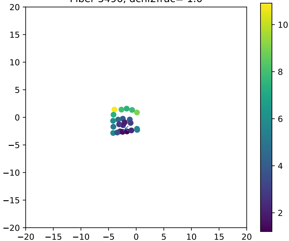
Fiber 3496, dchi2frac= 1.0
