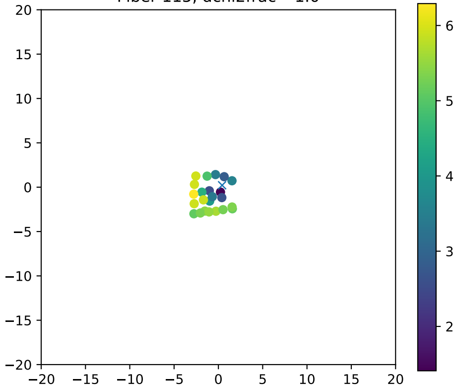
Fiber 115, dchi2frac= 1.0
