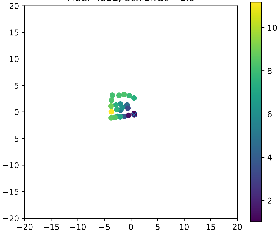
Fiber 4621, dchi2frac= 1.0
