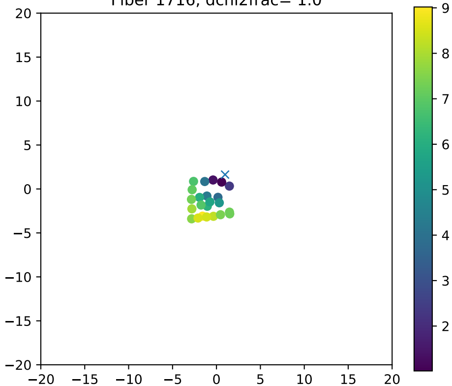
Fiber 1716, dchi2frac= 1.0
