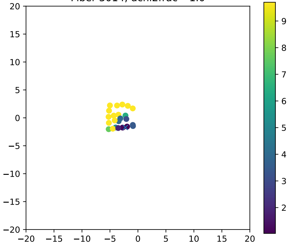
Fiber 3014, dchi2frac= 1.0
