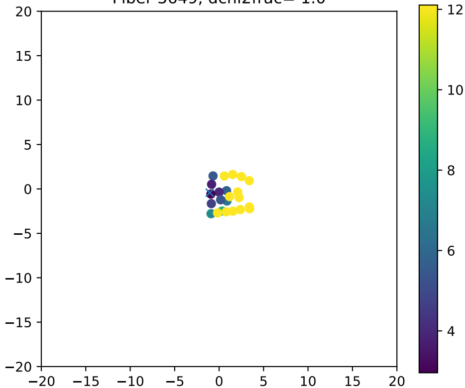
Fiber 3649, dchi2frac= 1.0
