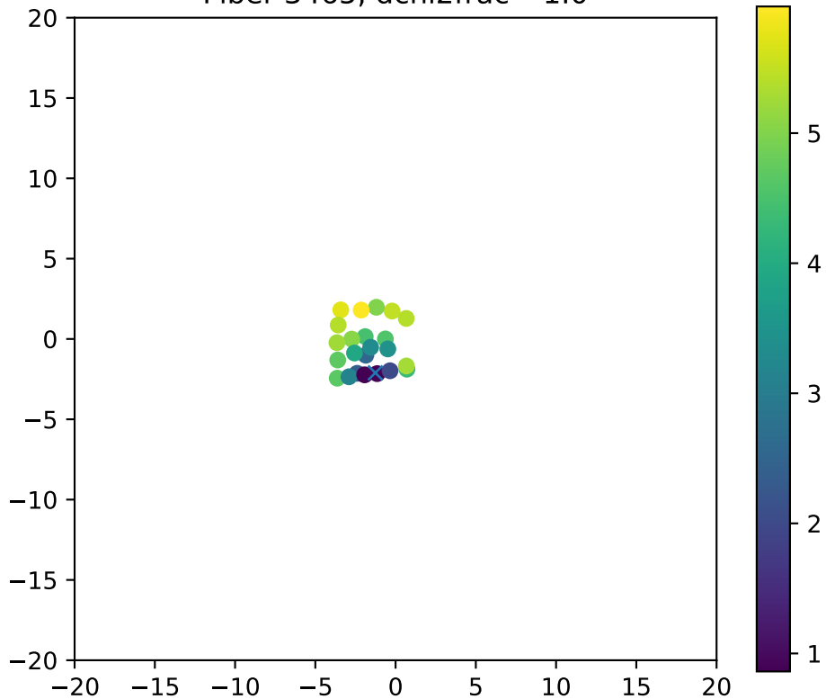
Fiber 3465, dchi2frac= 1.0
