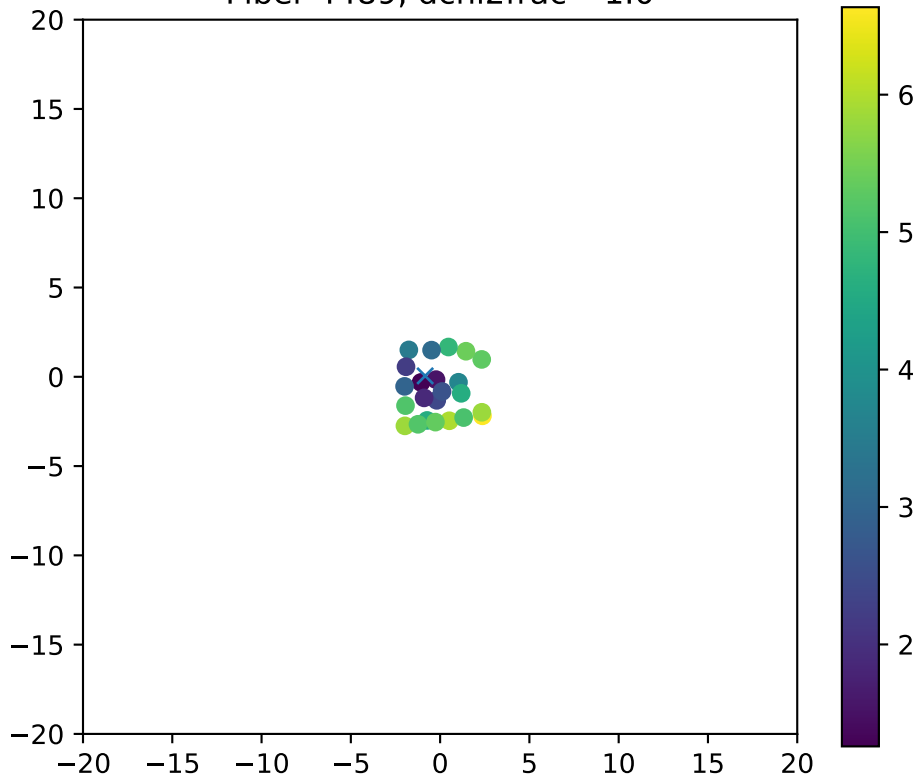
Fiber 4489, dchi2frac= 1.0
