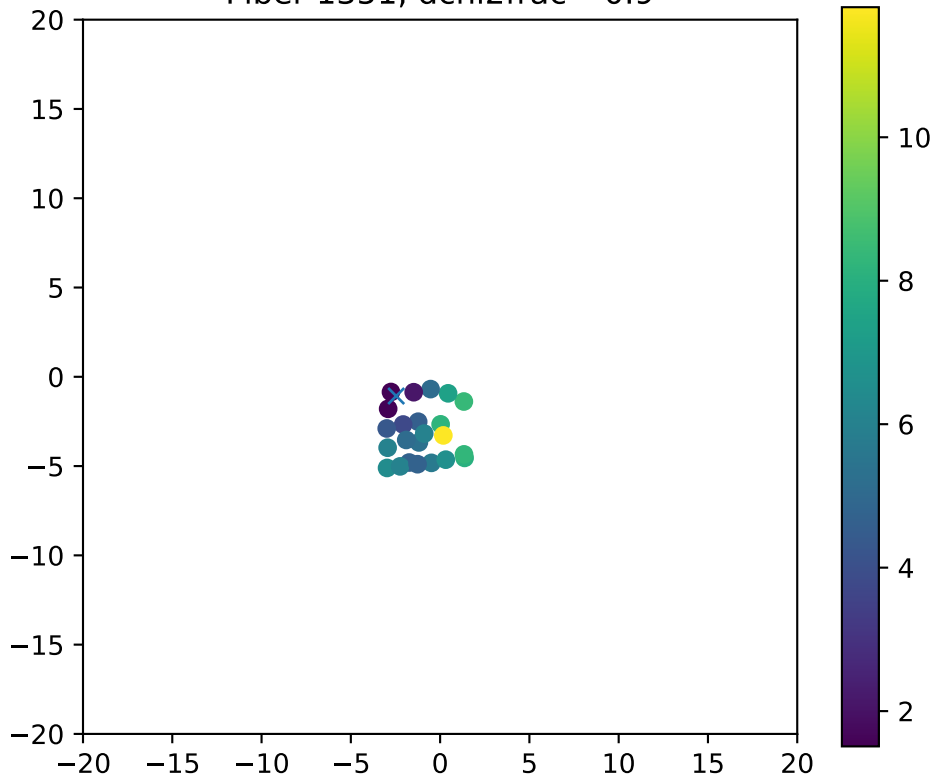
Fiber 1351, dchi2frac= 0.9
