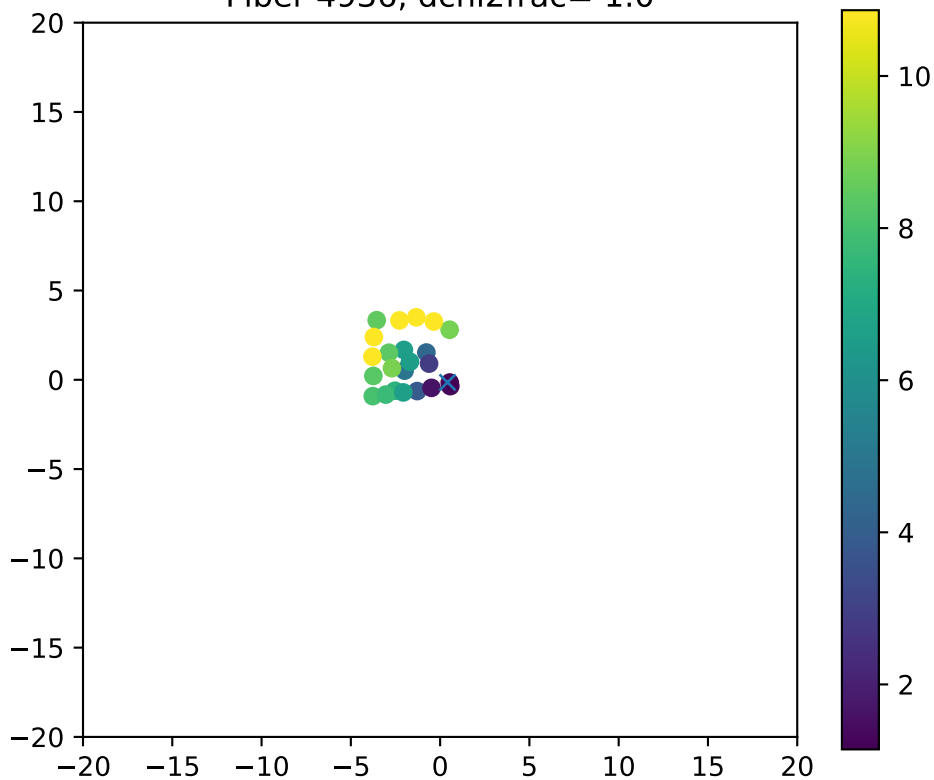
Fiber 4936, dchi2frac= 1.0
