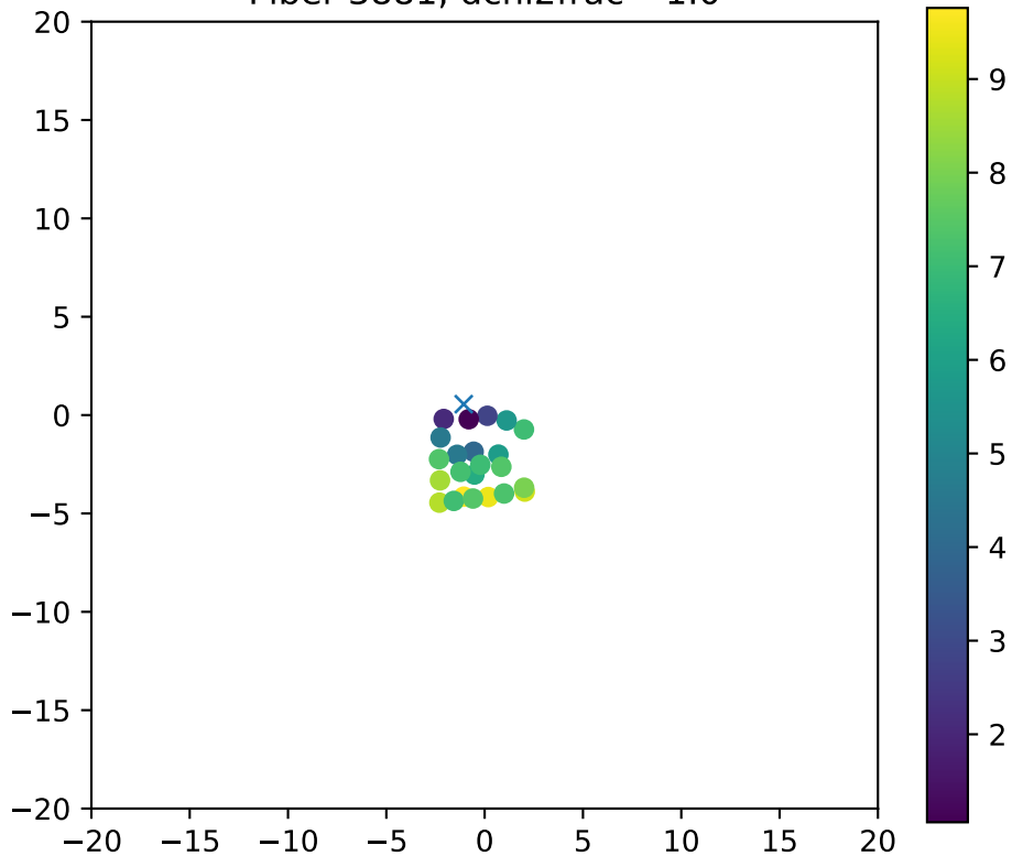
Fiber 3881, dchi2frac= 1.0
