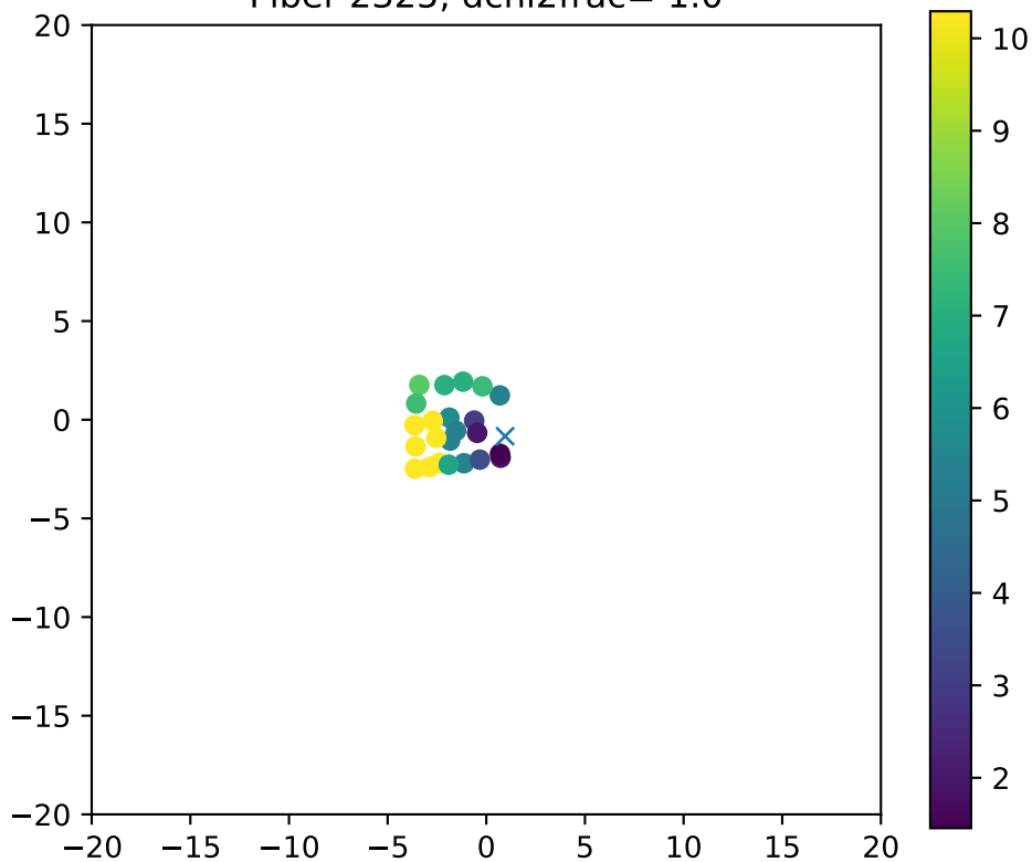
Fiber 2325, dchi2frac= 1.0
