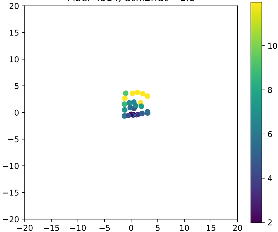
Fiber 4914, dchi2frac= 1.0
