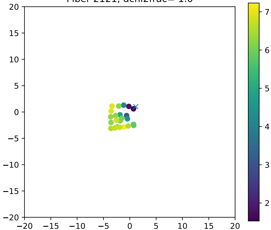
Fiber 2121, dchi2frac= 1.0
