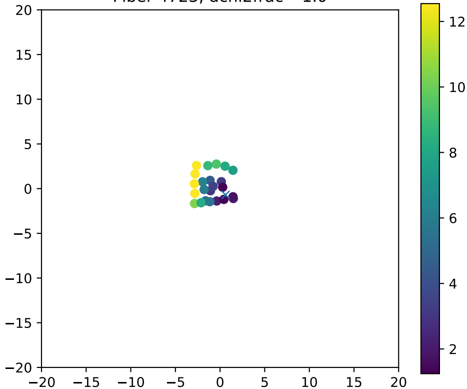
Fiber 4723, dchi2frac= 1.0
