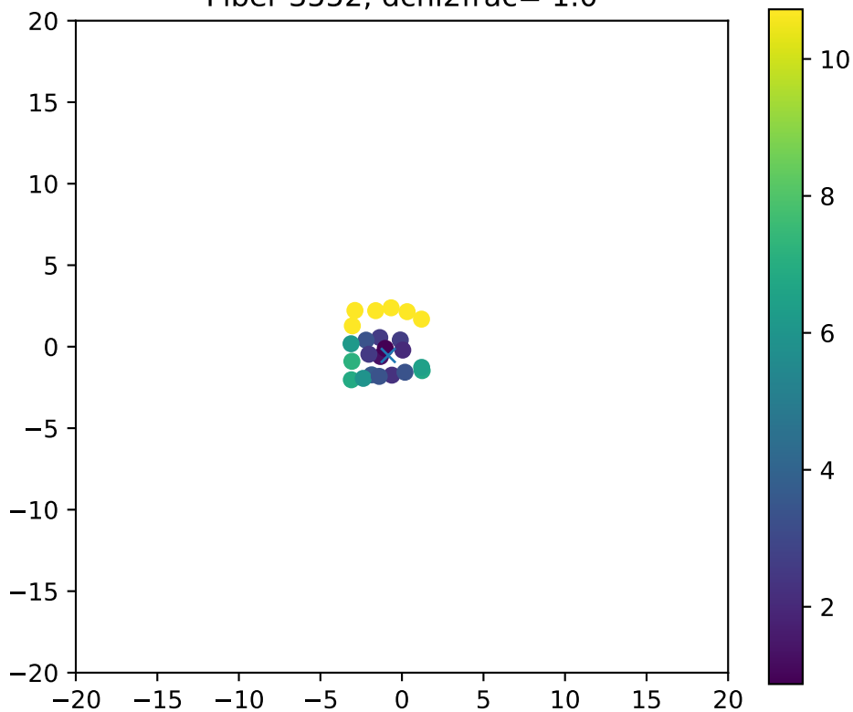
Fiber 3552, dchi2frac= 1.0
