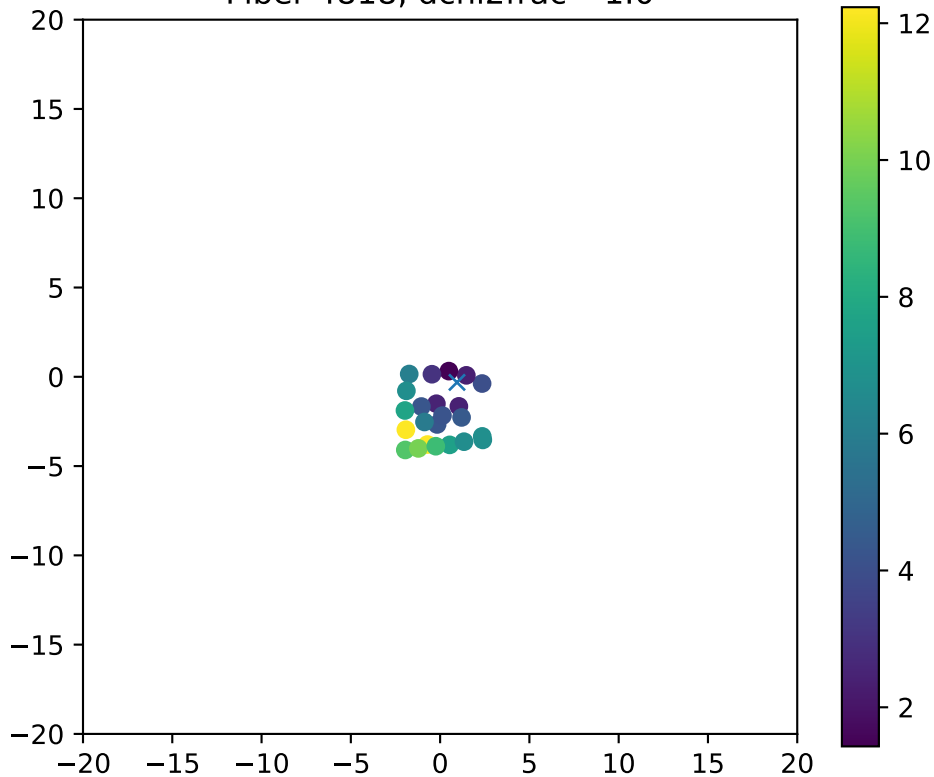
Fiber 4818, dchi2frac= 1.0
