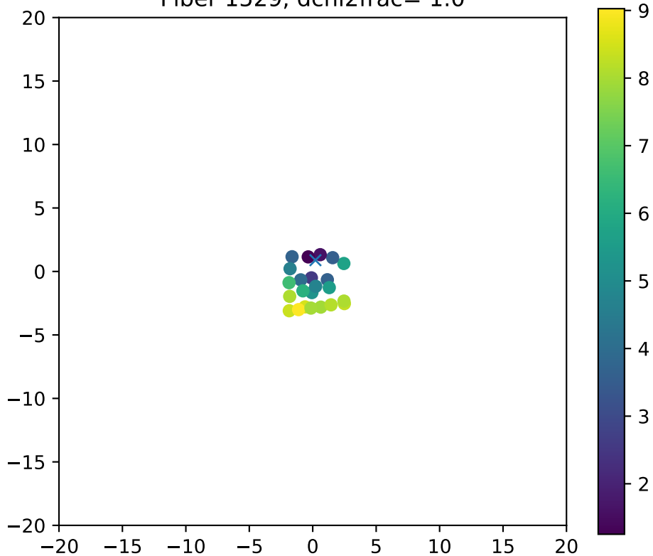
Fiber 1529, dchi2frac= 1.0
