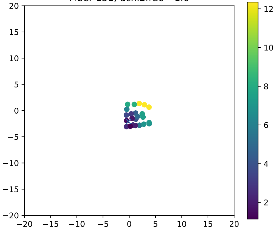
Fiber 151, dchi2frac= 1.0
