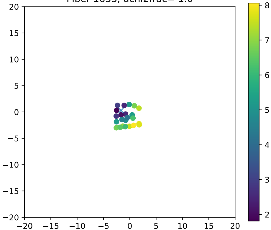
Fiber 1633, dchi2frac= 1.0
