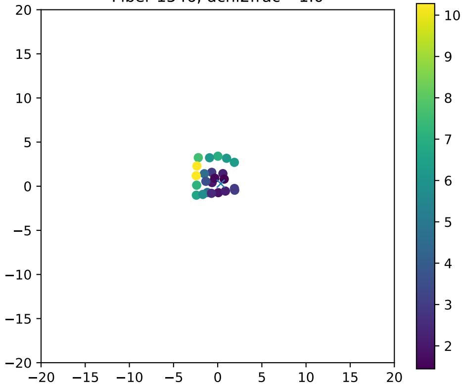
Fiber 1546, dchi2frac= 1.0
