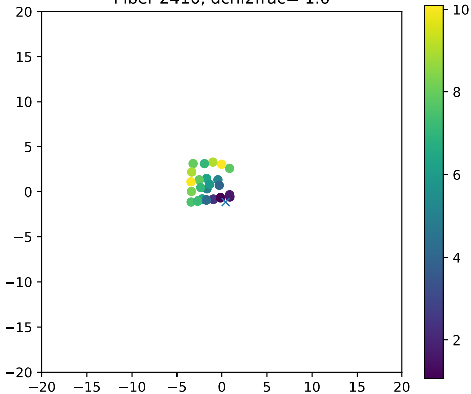
Fiber 2410, dchi2frac= 1.0
