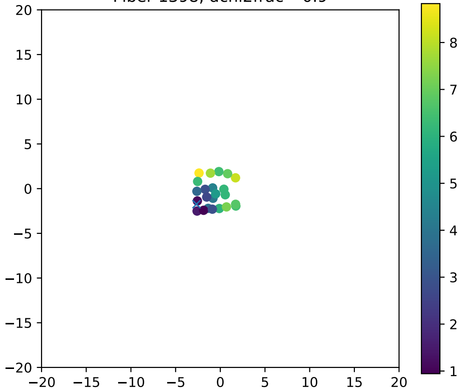
Fiber 1398, dchi2frac= 0.9
