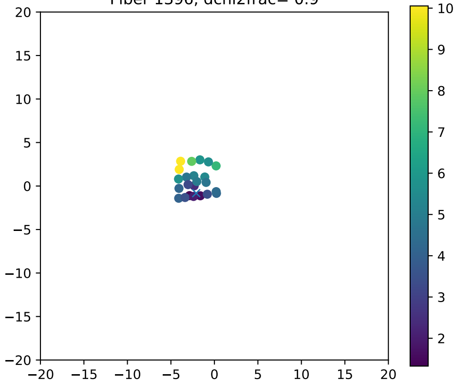
Fiber 1396, dchi2frac= 0.9
