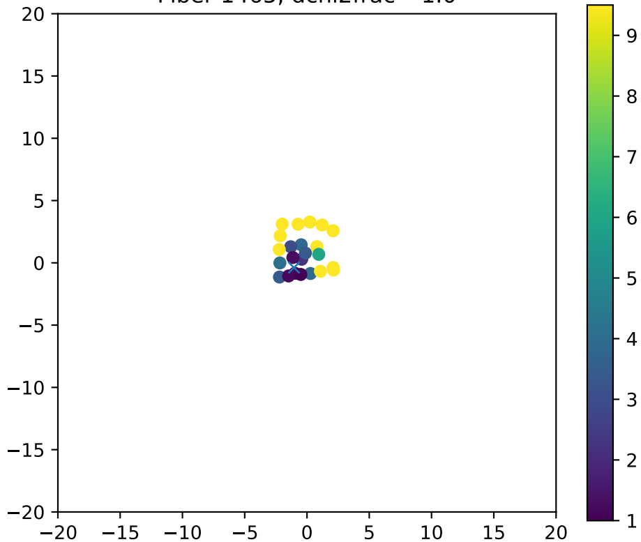
Fiber 1465, dchi2frac= 1.0
