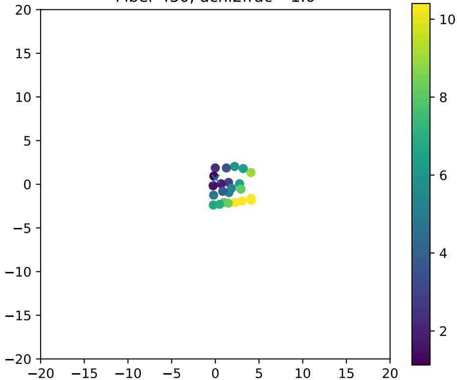
Fiber 430, dchi2frac= 1.0
