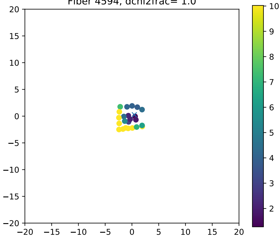
Fiber 4594, dchi2frac= 1.0
