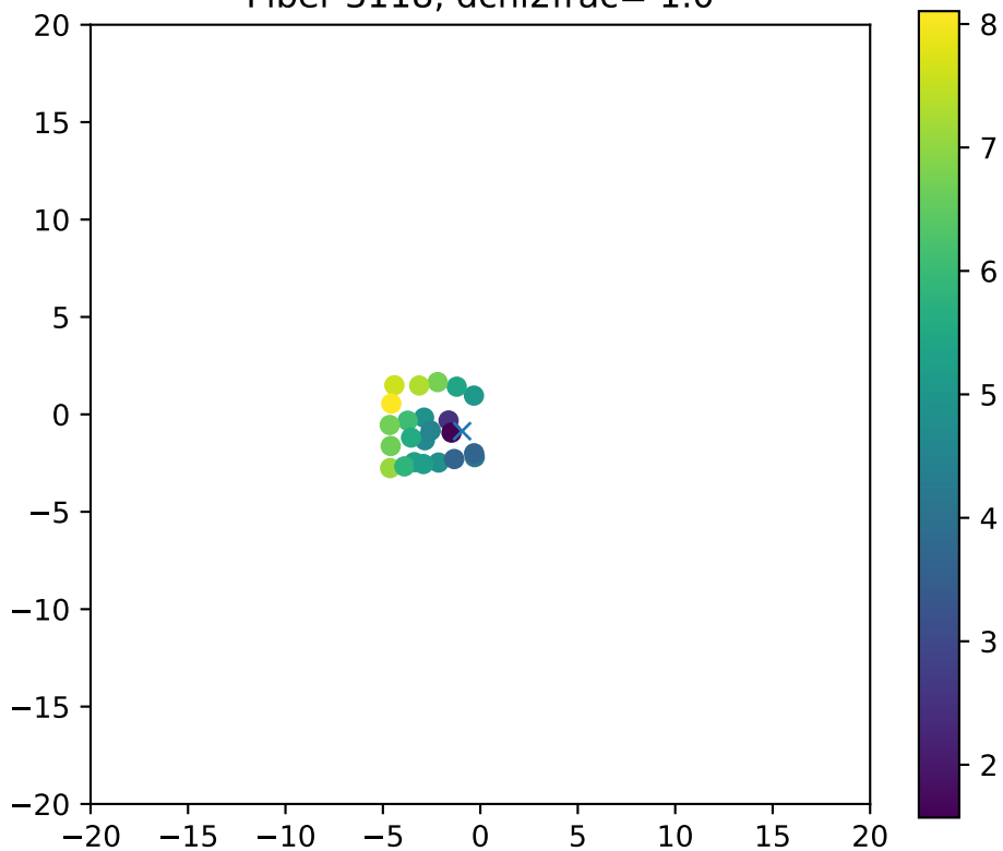
Fiber 3118, dchi2frac= 1.0
