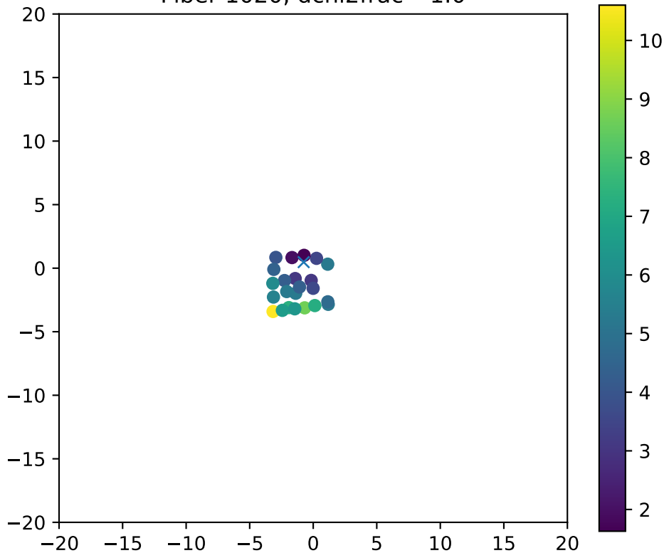
Fiber 1020, dchi2frac= 1.0
