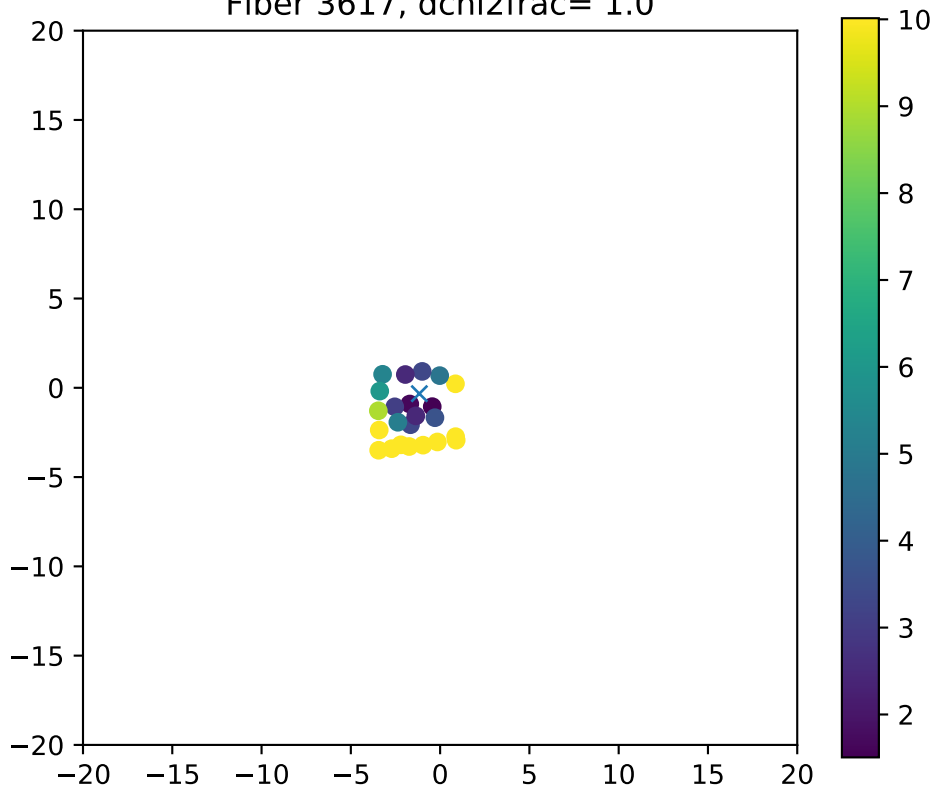
Fiber 3617, dchi2frac= 1.0
