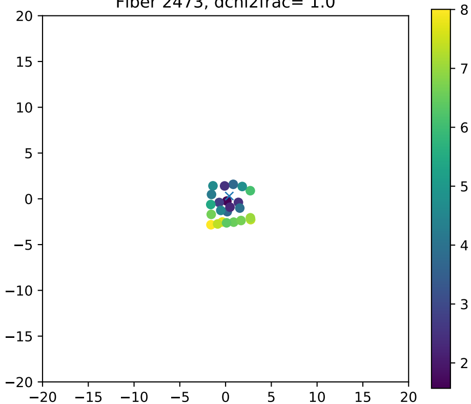
Fiber 2473, dchi2frac= 1.0
