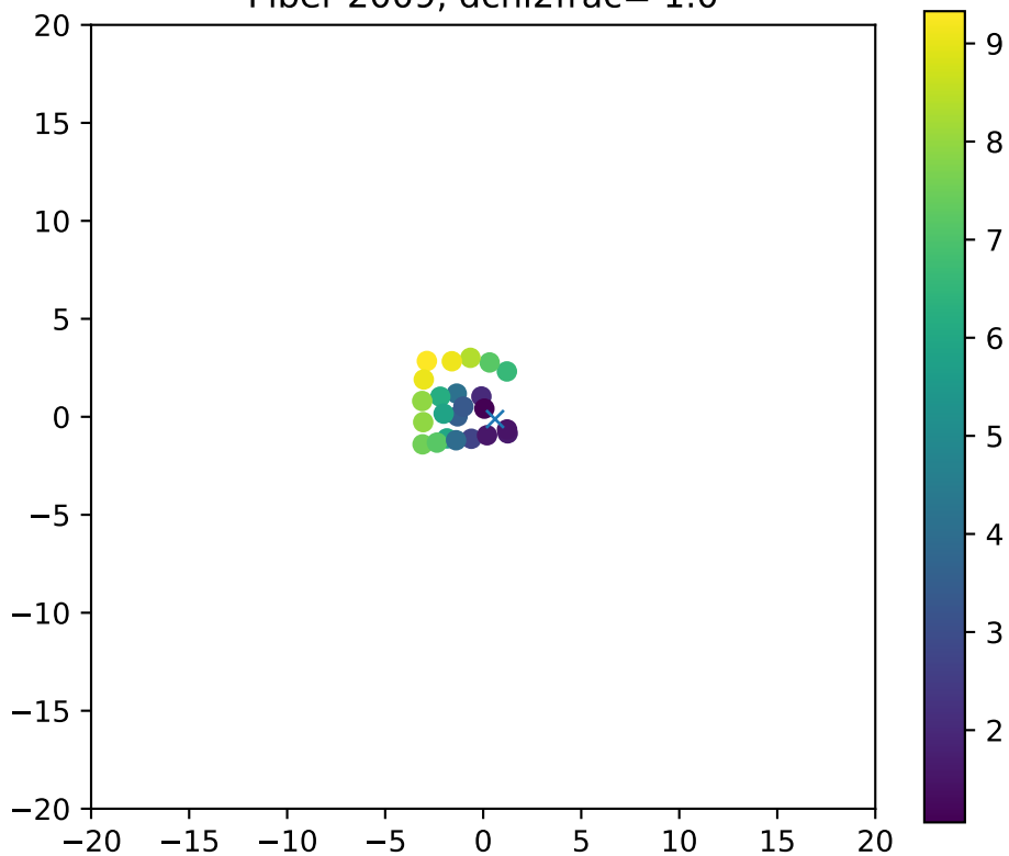
Fiber 2009, dchi2frac= 1.0
