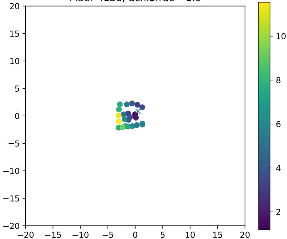
Fiber 4138, dchi2frac= 1.0
