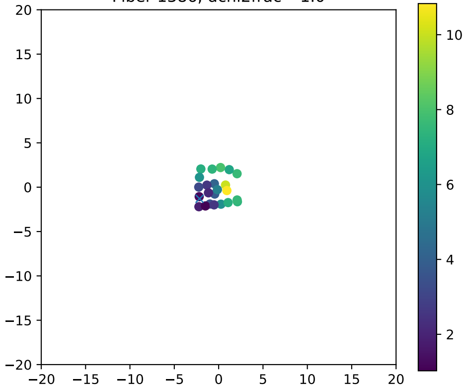
Fiber 1386, dchi2frac= 1.0
