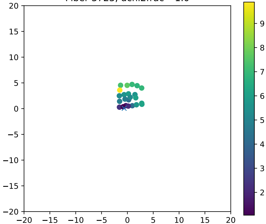
Fiber 3723, dchi2frac= 1.0
