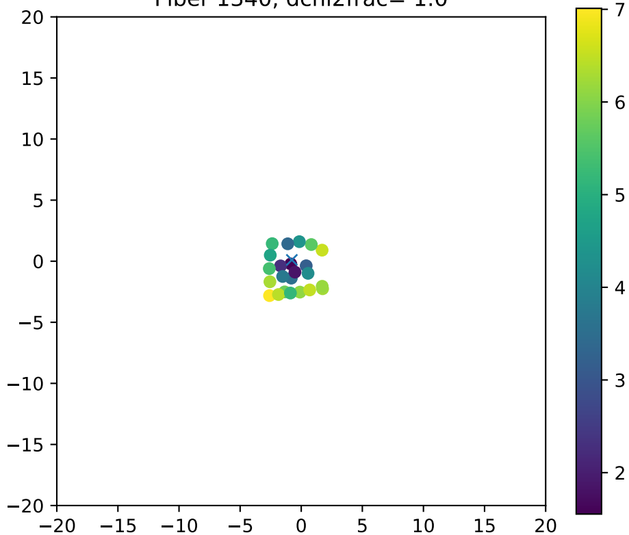
Fiber 1340, dchi2frac= 1.0
