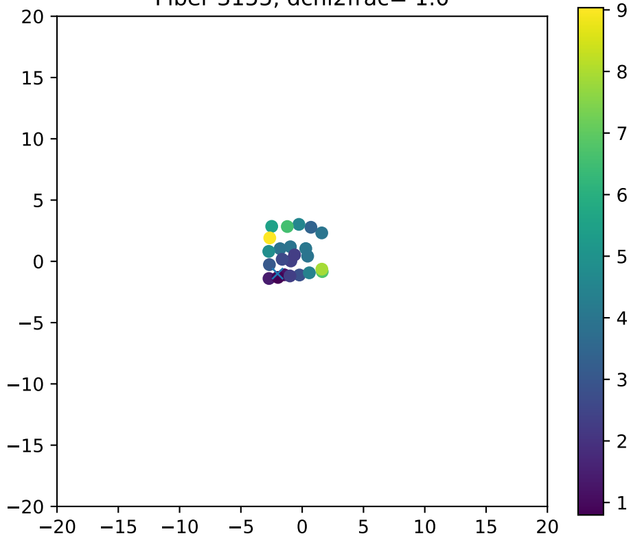
Fiber 3155, dchi2frac= 1.0
