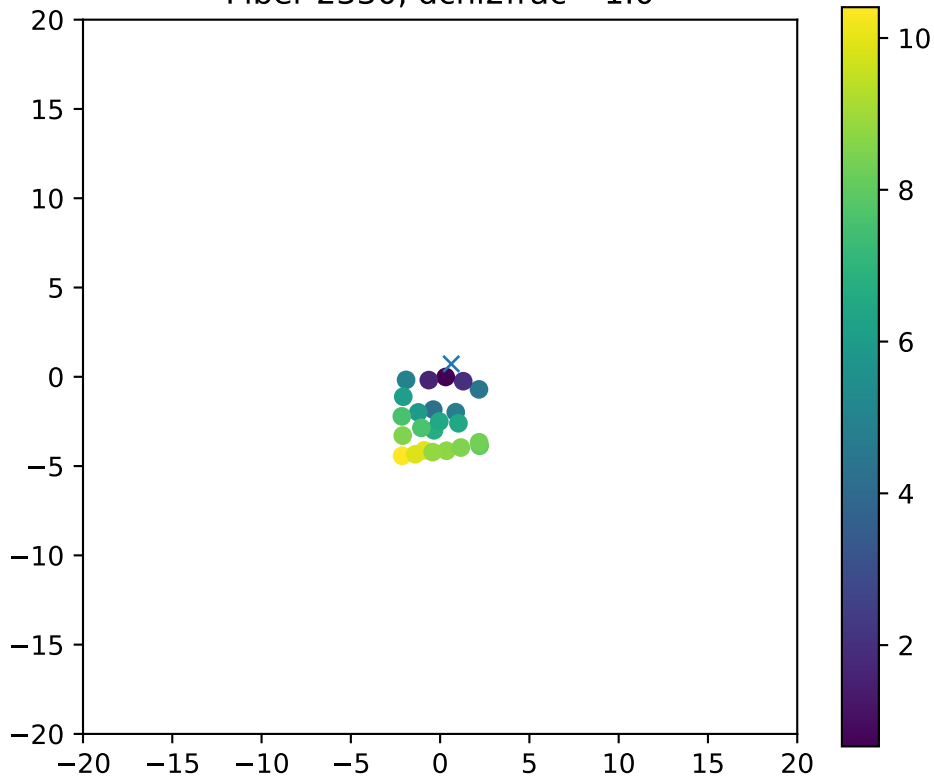
Fiber 2330, dchi2frac= 1.0
