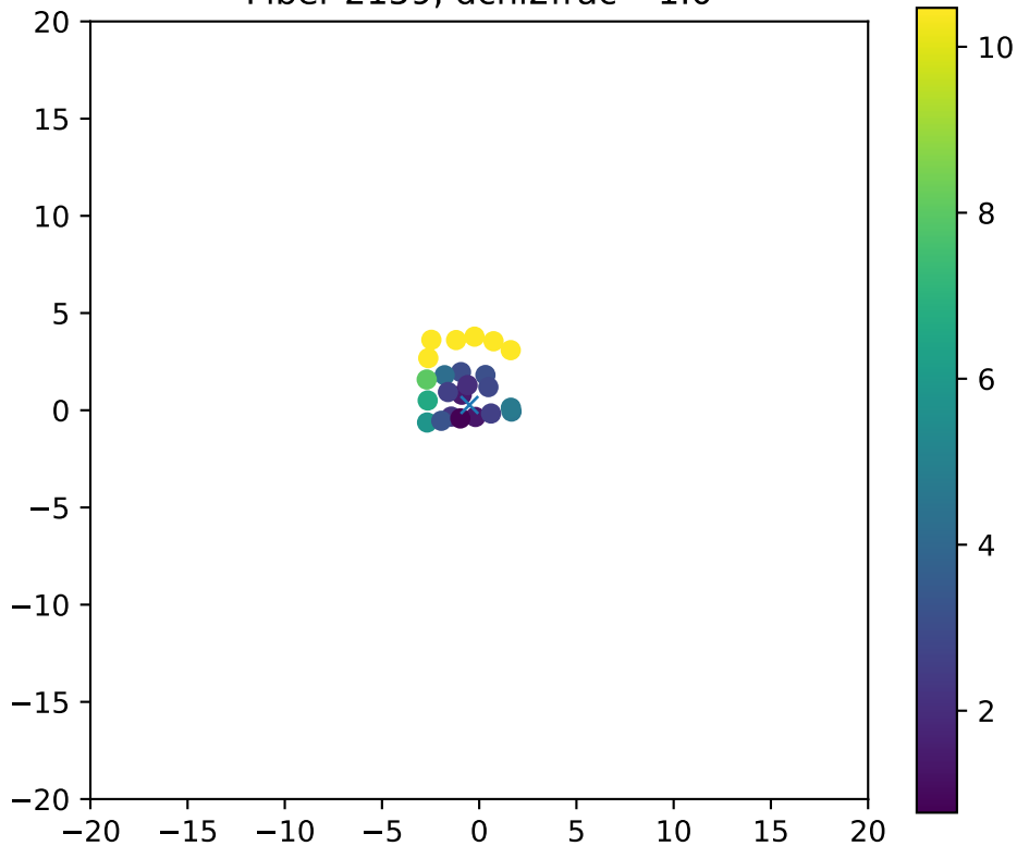
Fiber 2159, dchi2frac= 1.0
