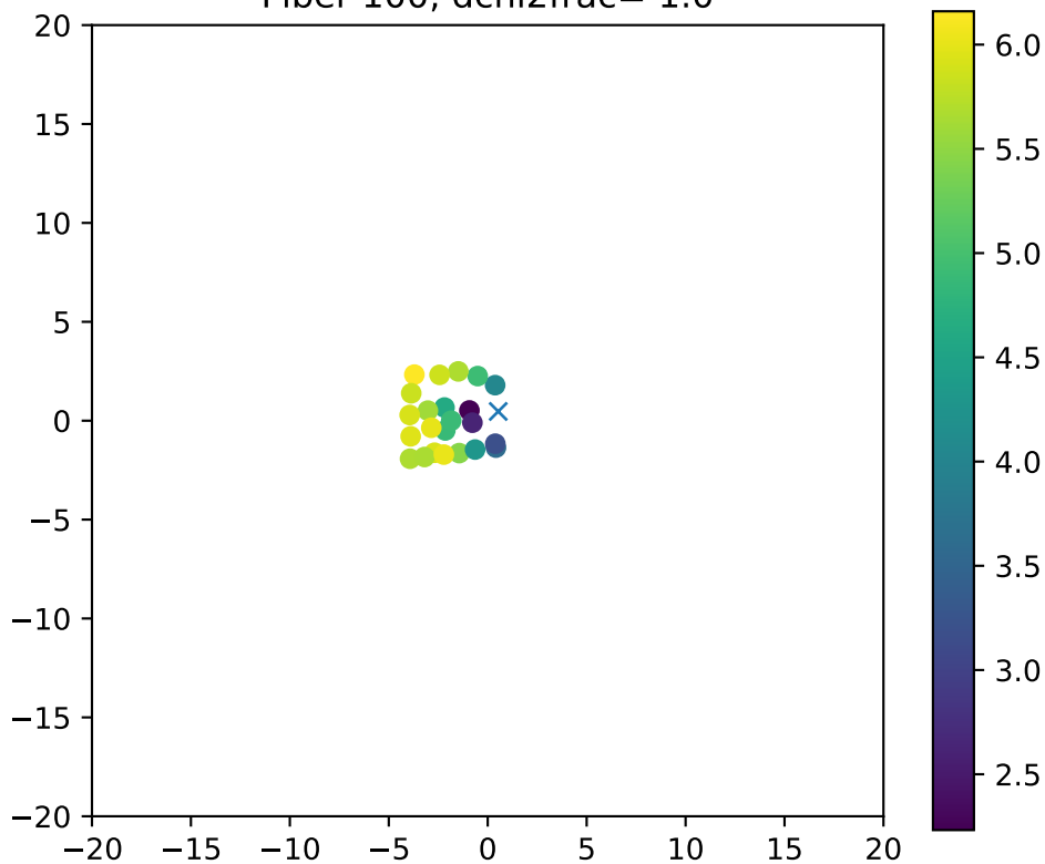
Fiber 100, dchi2frac= 1.0
