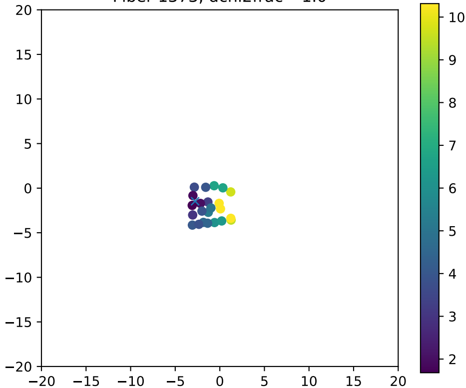
Fiber 1373, dchi2frac= 1.0
