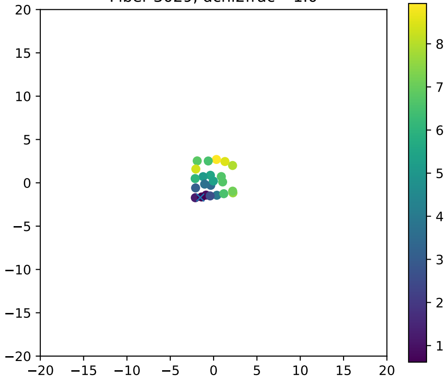
Fiber 3029, dchi2frac= 1.0
