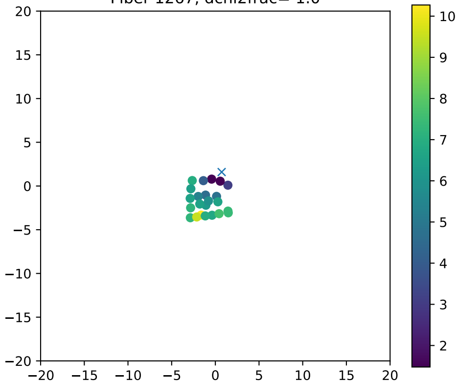
Fiber 1267, dchi2frac= 1.0
