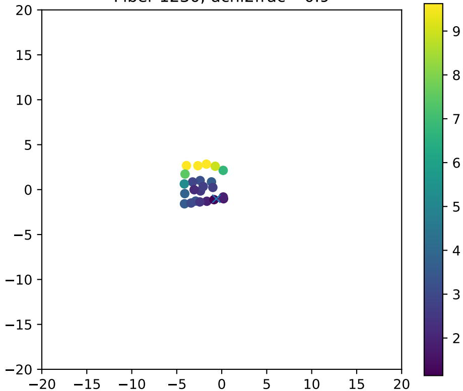
Fiber 1230, dchi2frac= 0.9
