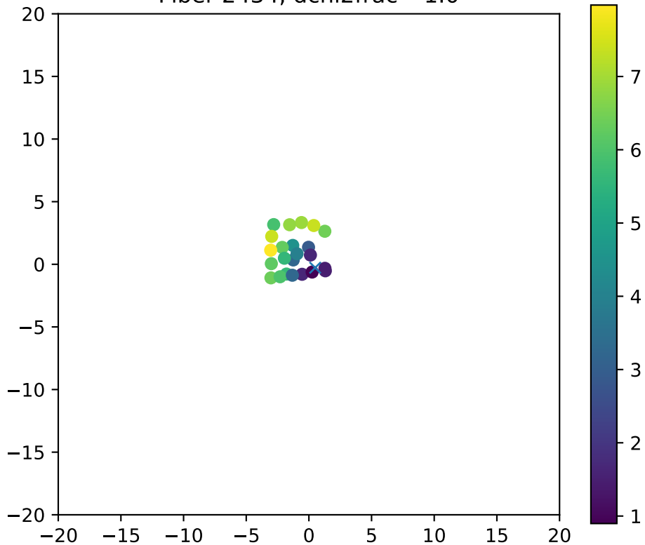
Fiber 2434, dchi2frac= 1.0
