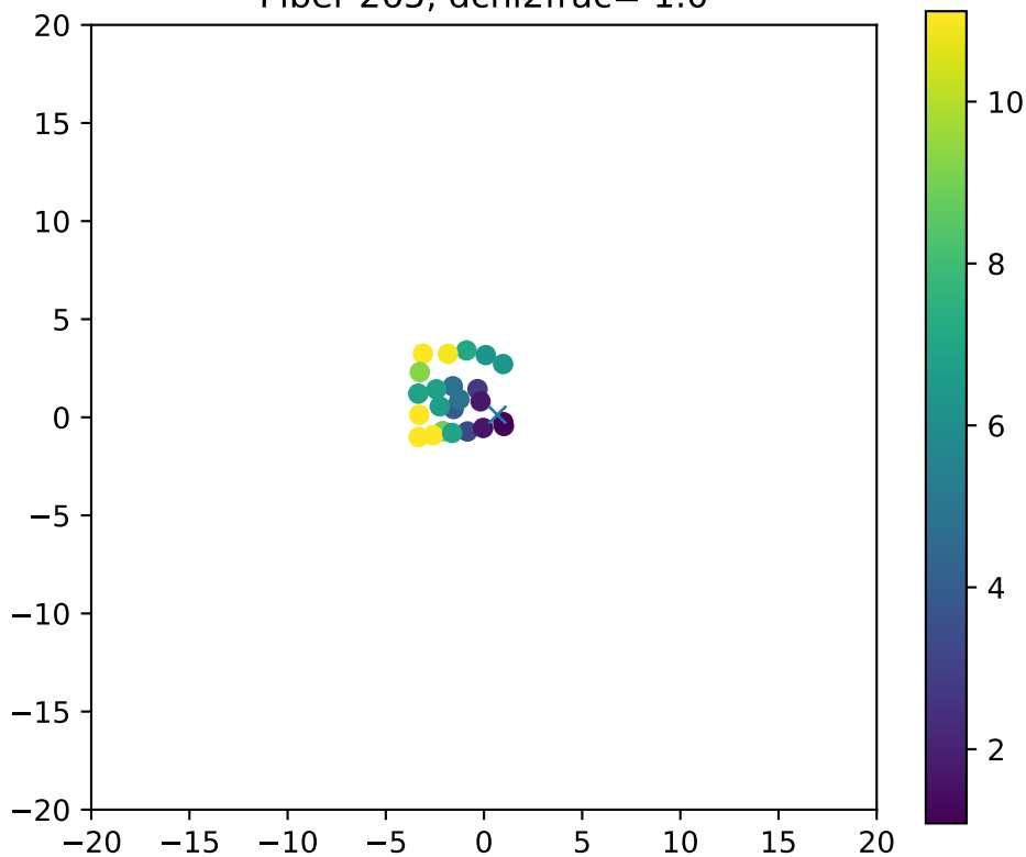
Fiber 265, dchi2frac= 1.0
