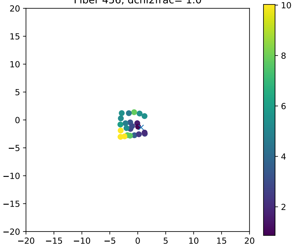
Fiber 456, dchi2frac= 1.0
