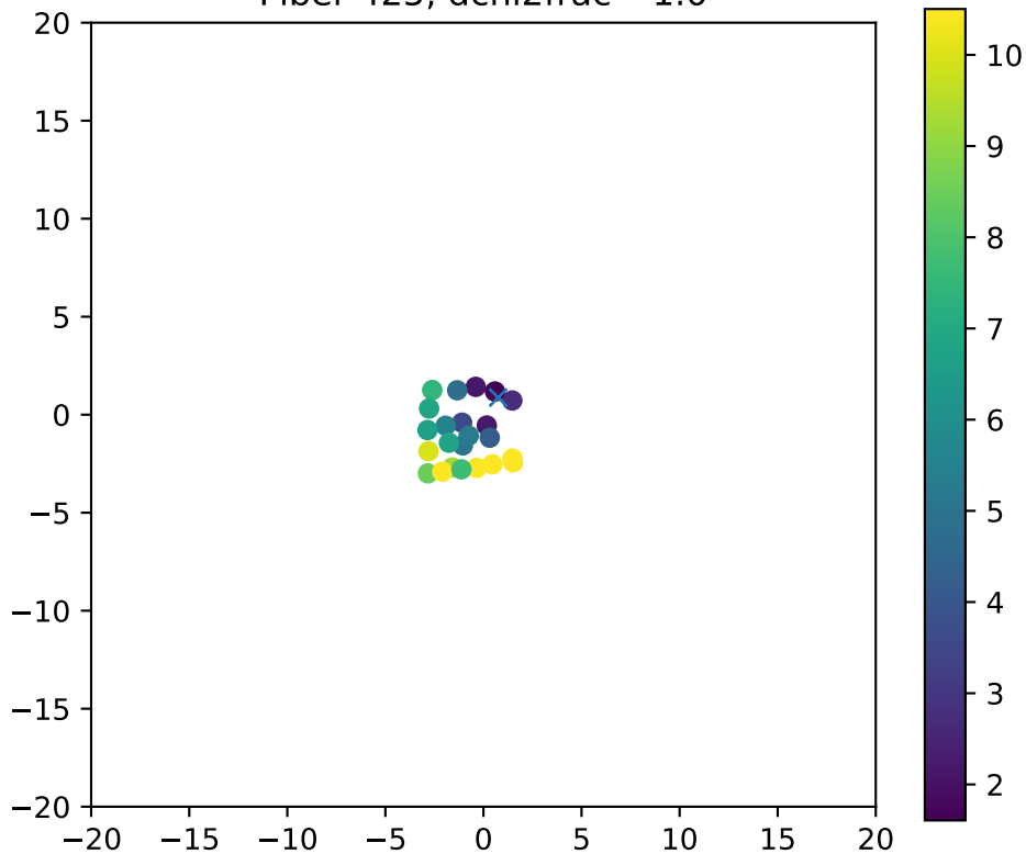
Fiber 425, dchi2frac= 1.0
