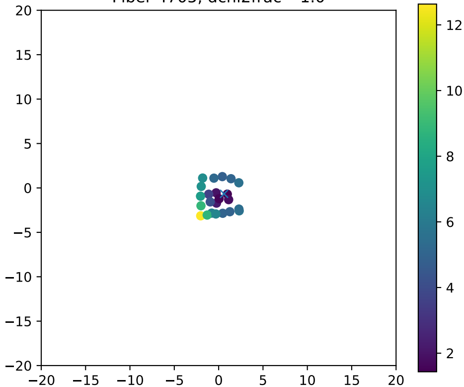
Fiber 4705, dchi2frac= 1.0
