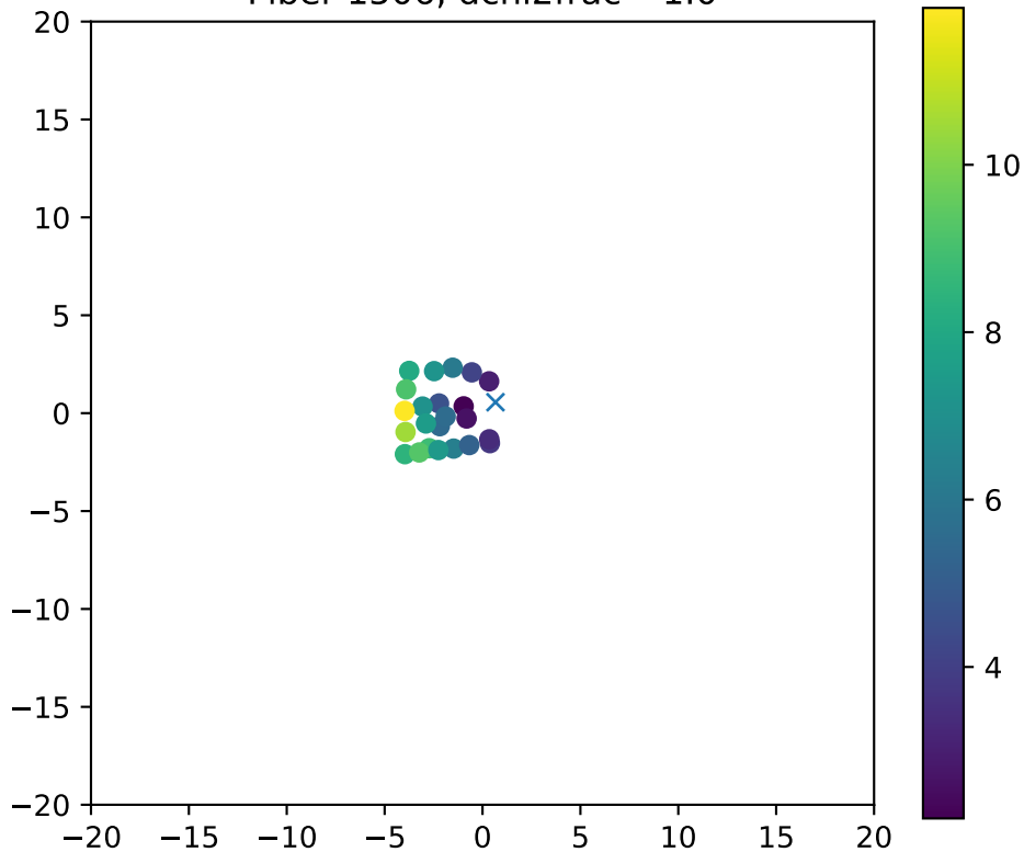
Fiber 1506, dchi2frac= 1.0
