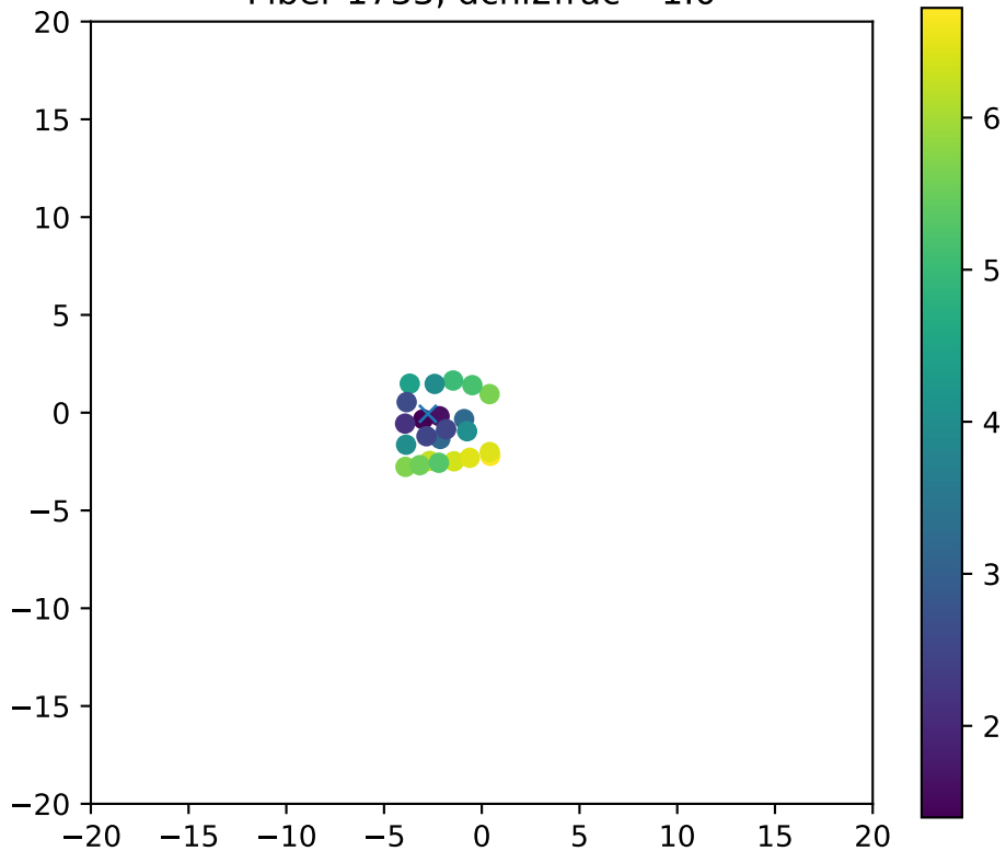
Fiber 1733, dchi2frac= 1.0
