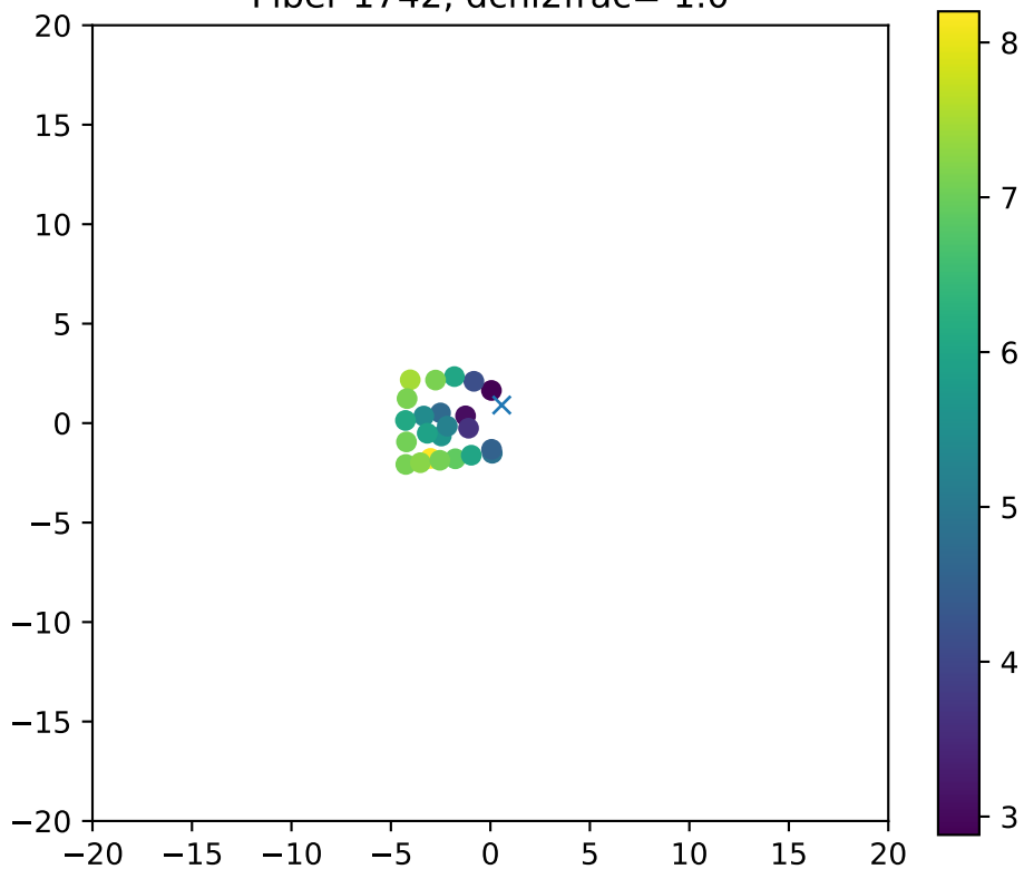
Fiber 1742, dchi2frac= 1.0
