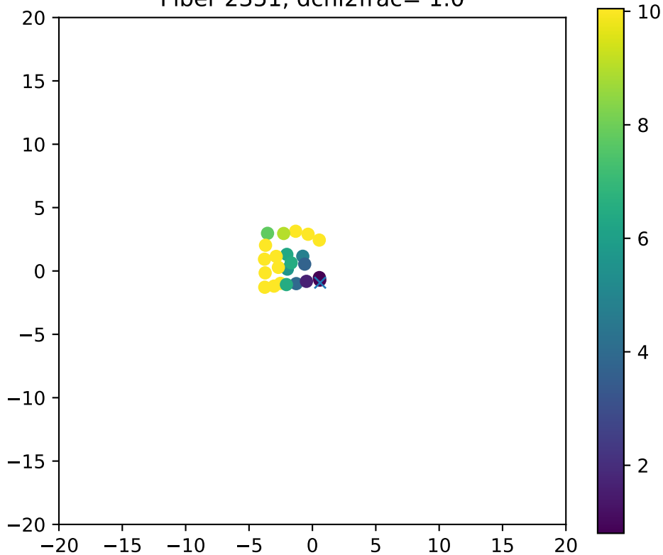
Fiber 2351, dchi2frac= 1.0
