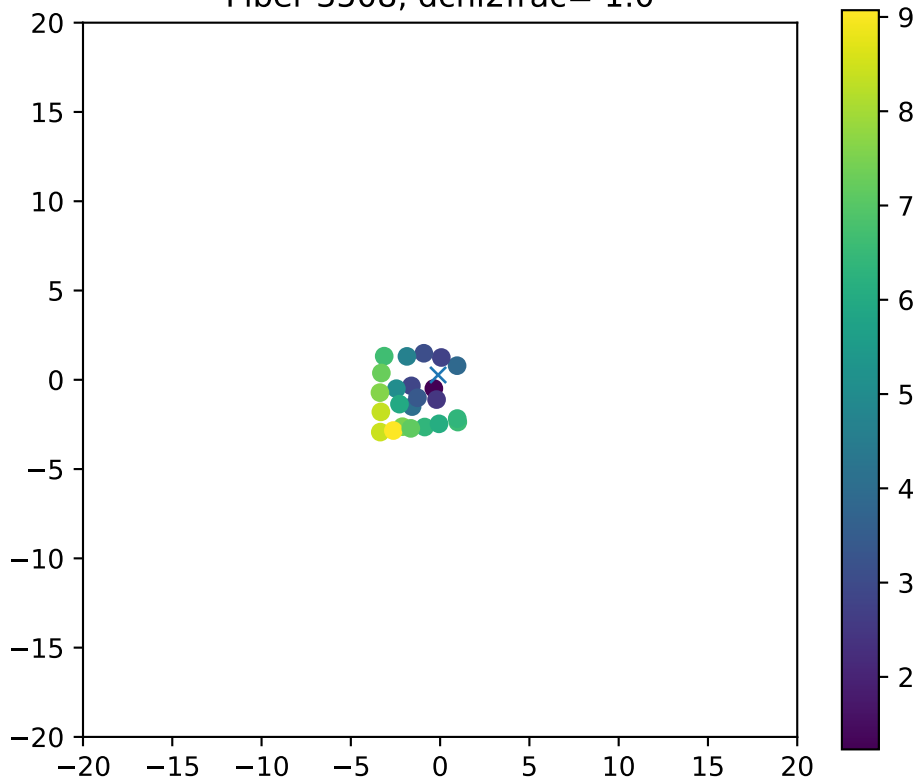
Fiber 3508, dchi2frac= 1.0
