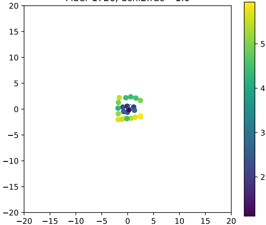
Fiber 1726, dchi2frac= 1.0
