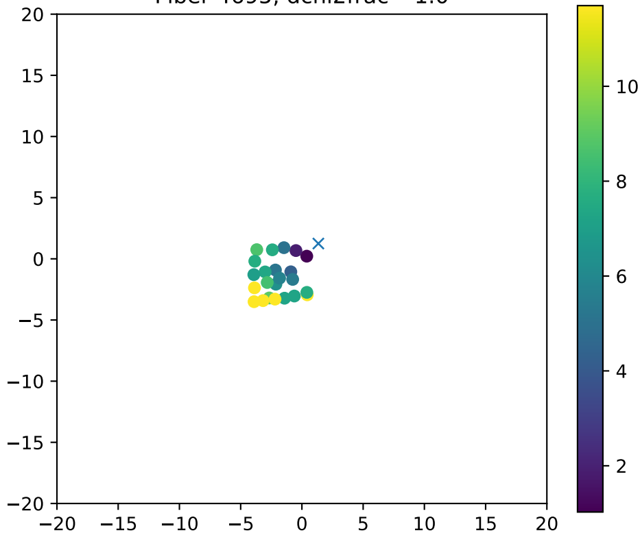
Fiber 4695, dchi2frac= 1.0
