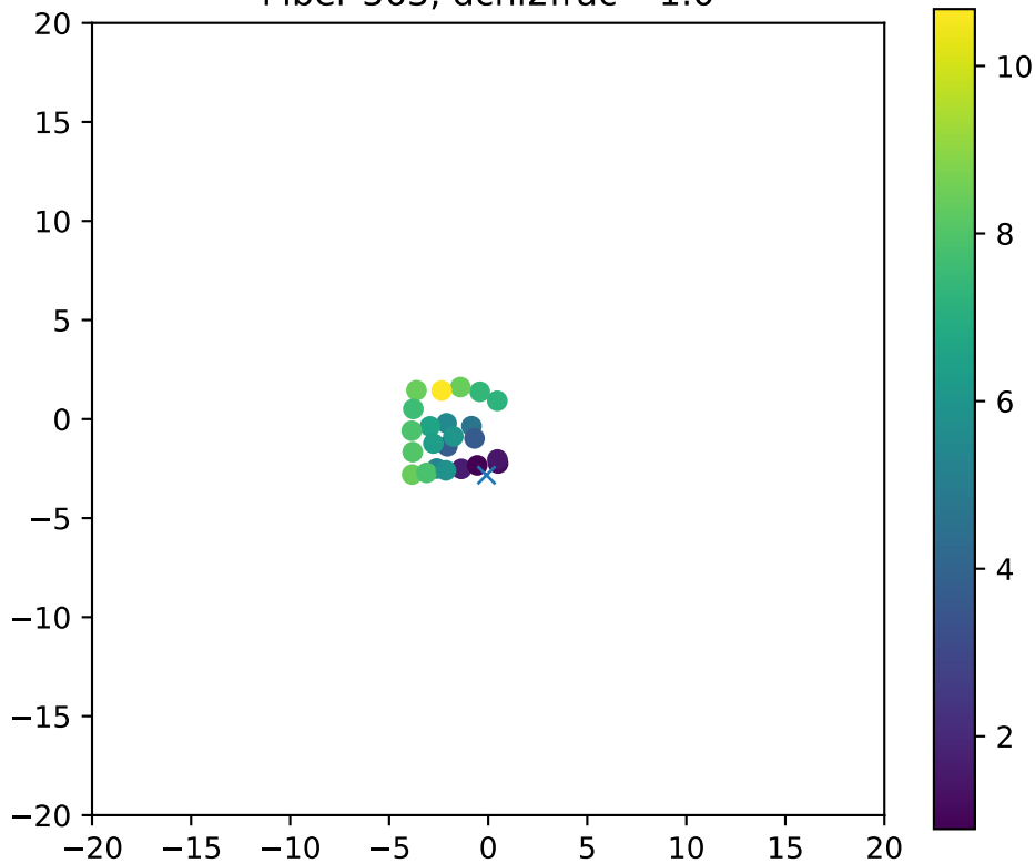
Fiber 363, dchi2frac= 1.0
