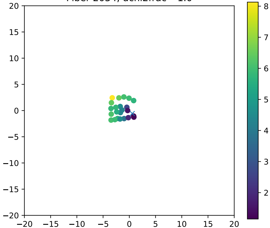
Fiber 2034, dchi2frac= 1.0
