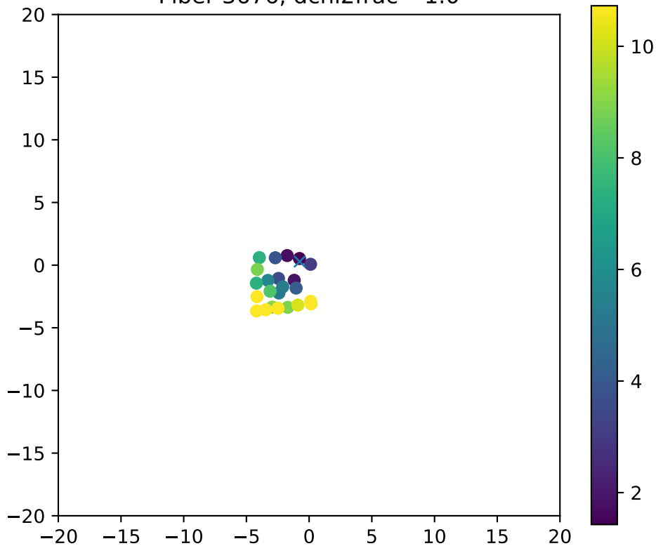
Fiber 3676, dchi2frac= 1.0
