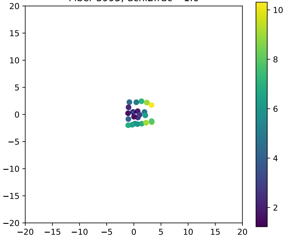
Fiber 3995, dchi2frac= 1.0
