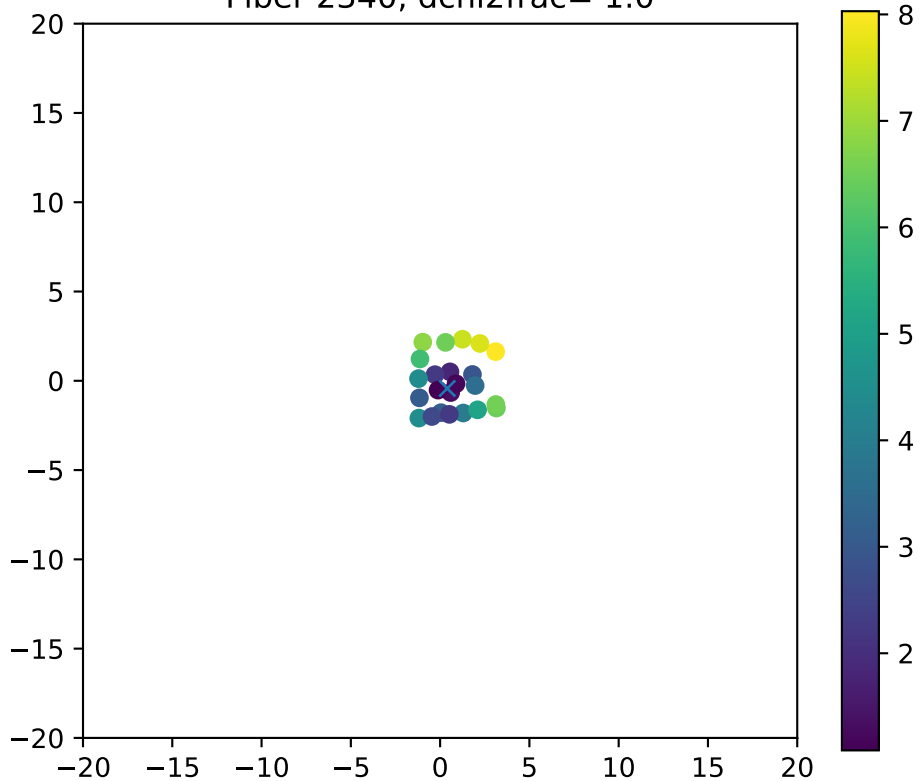
Fiber 2340, dchi2frac= 1.0
