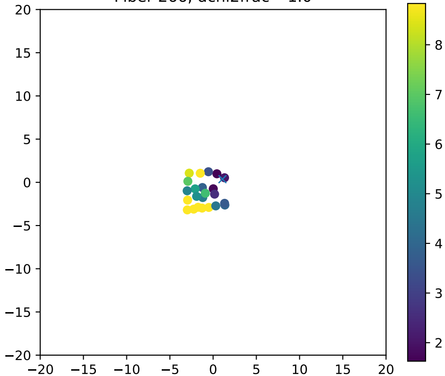
Fiber 266, dchi2frac= 1.0
