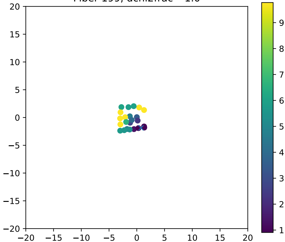
Fiber 199, dchi2frac= 1.0
