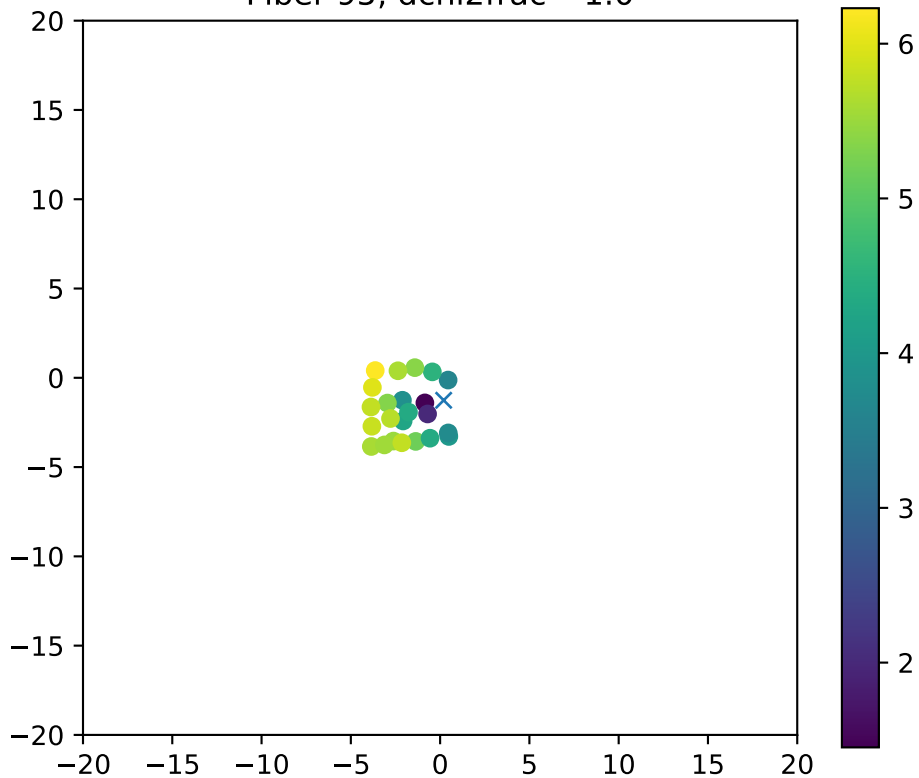
Fiber 95, dchi2frac= 1.0
