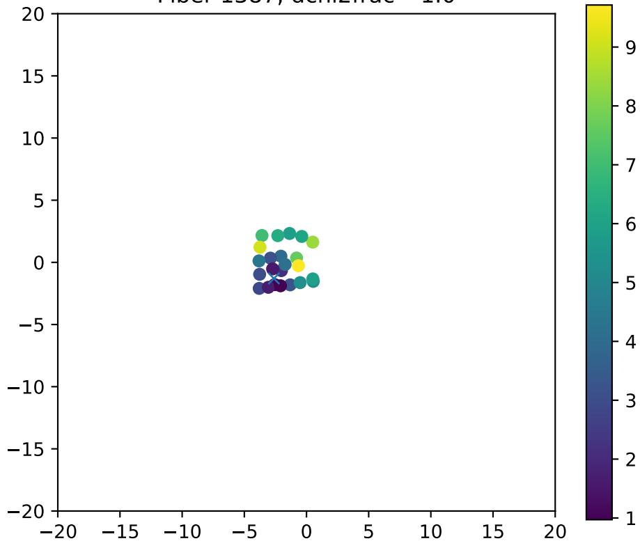
Fiber 1387, dchi2frac= 1.0
