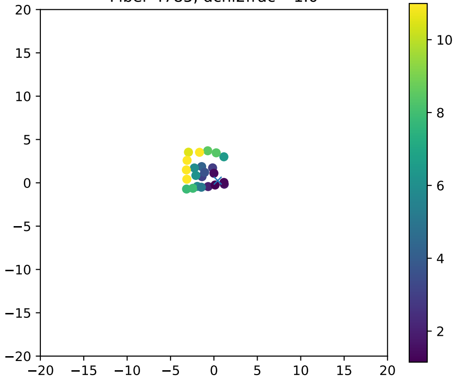
Fiber 4785, dchi2frac= 1.0
