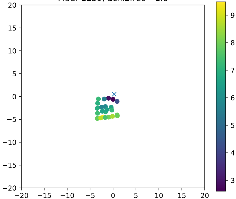
Fiber 1259, dchi2frac= 1.0
