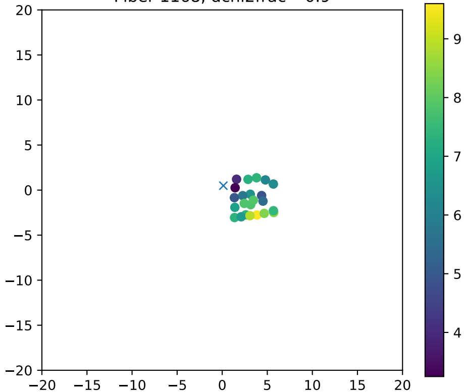
Fiber 1168, dchi2frac= 0.9
