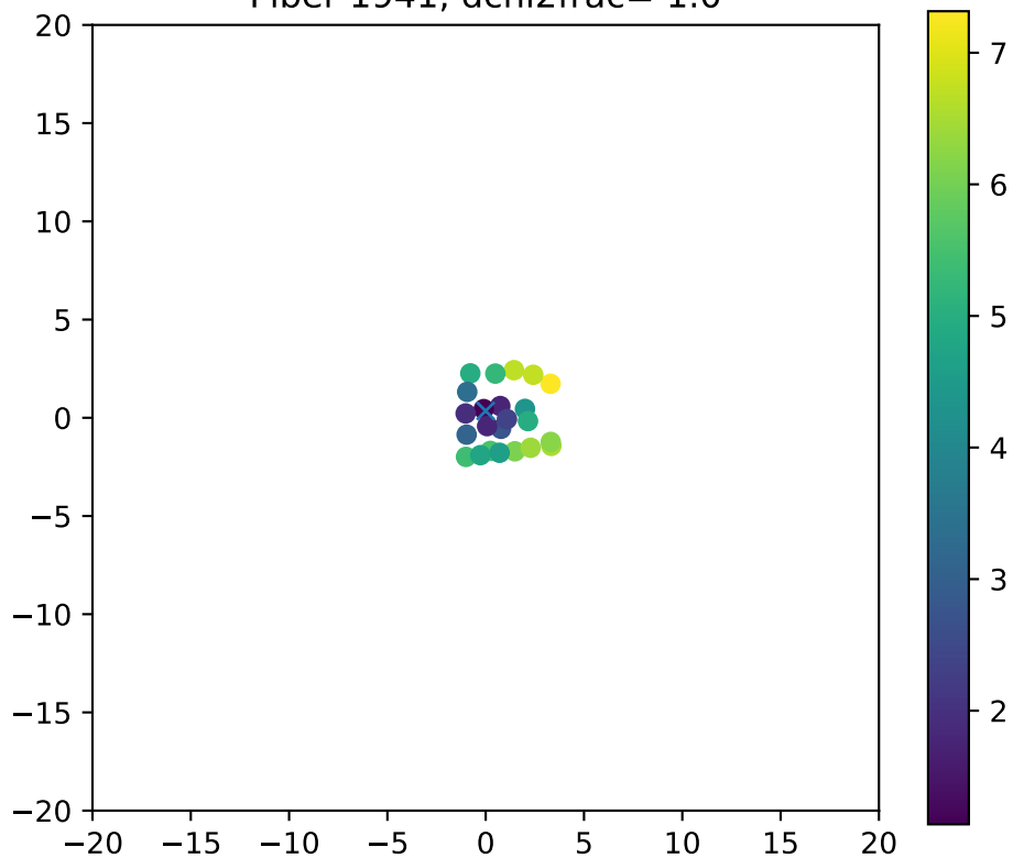
Fiber 1941, dchi2frac= 1.0
