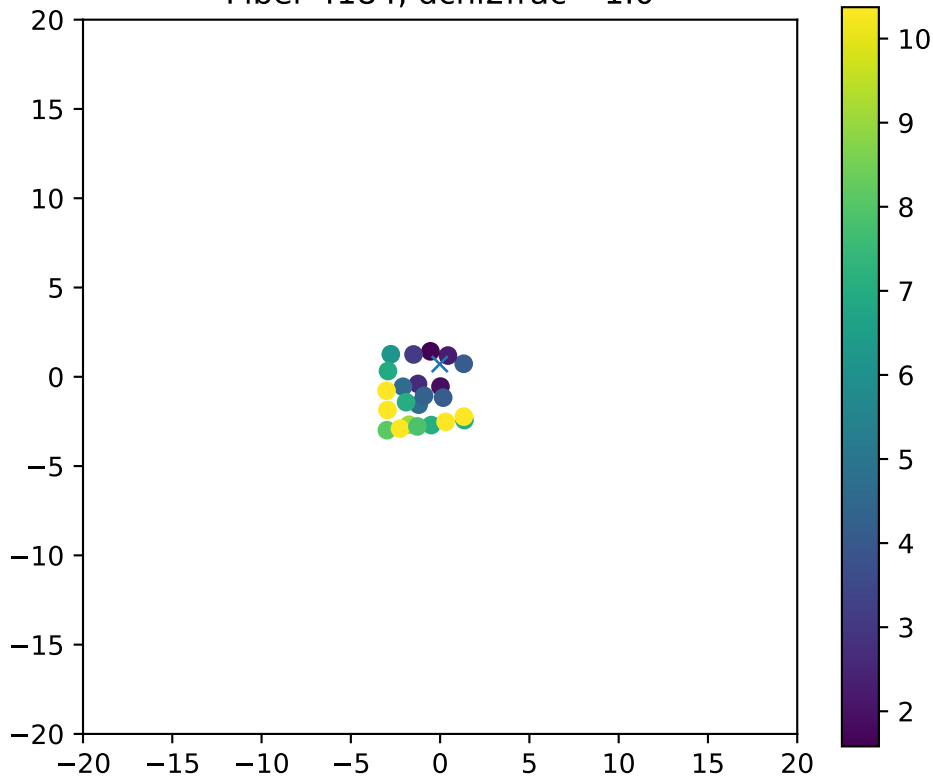
Fiber 4184, dchi2frac= 1.0
