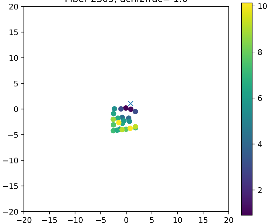
Fiber 2305, dchi2frac= 1.0
