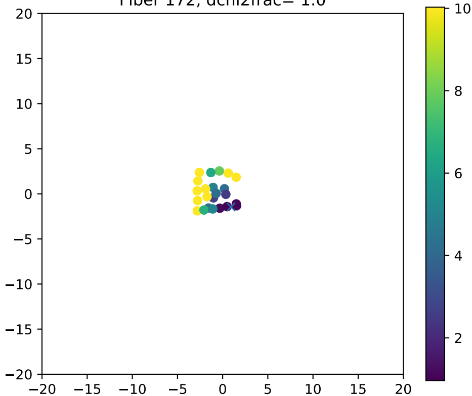
Fiber 172, dchi2frac= 1.0
