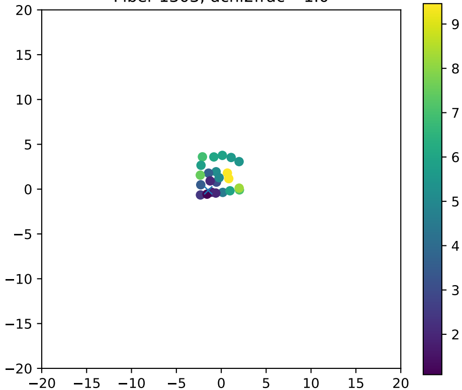
Fiber 1303, dchi2frac= 1.0
