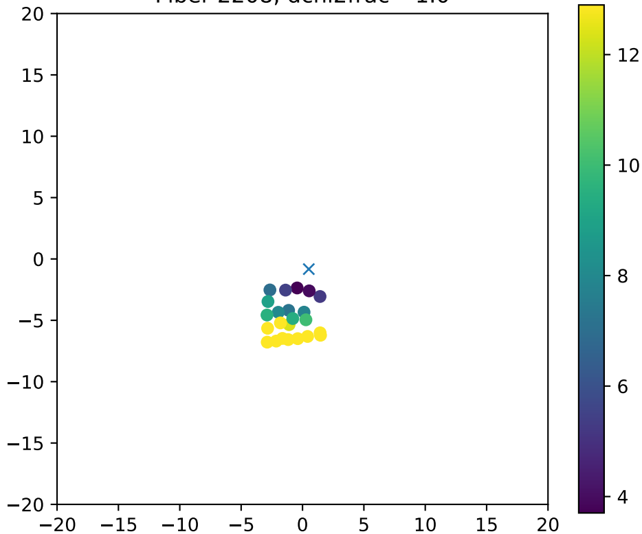
Fiber 2208, dchi2frac= 1.0
