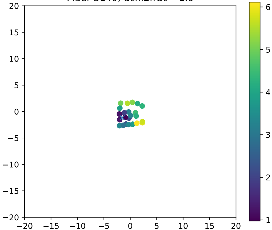
Fiber 3140, dchi2frac= 1.0
