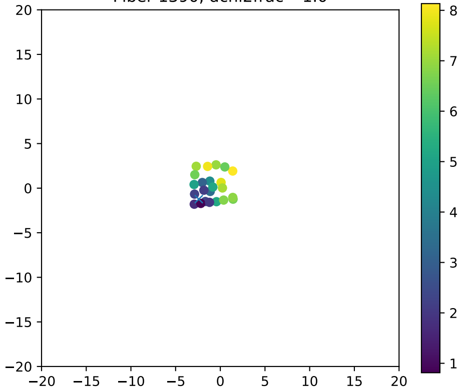
Fiber 1390, dchi2frac= 1.0
