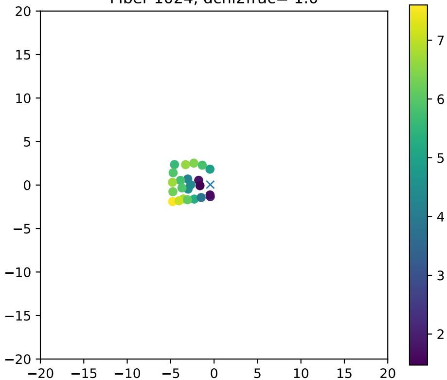
Fiber 1024, dchi2frac= 1.0
