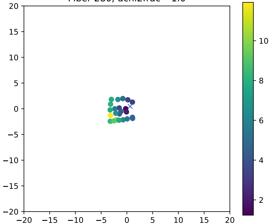
Fiber 280, dchi2frac= 1.0
