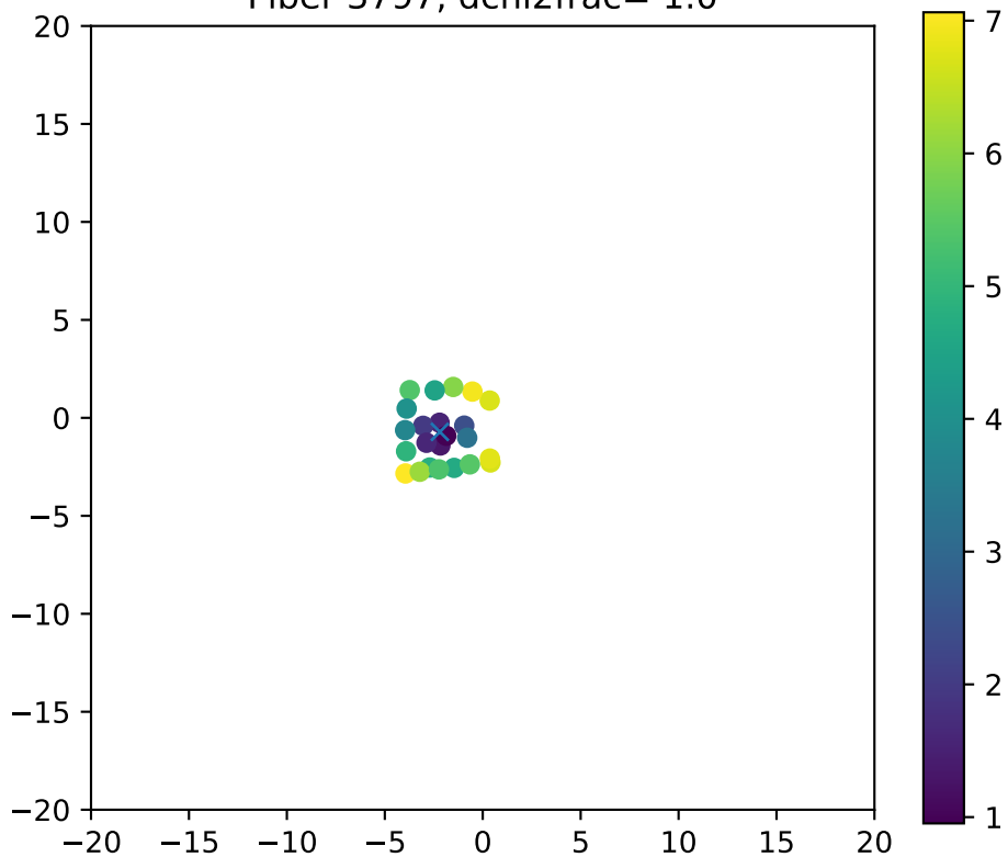
Fiber 3797, dchi2frac= 1.0
