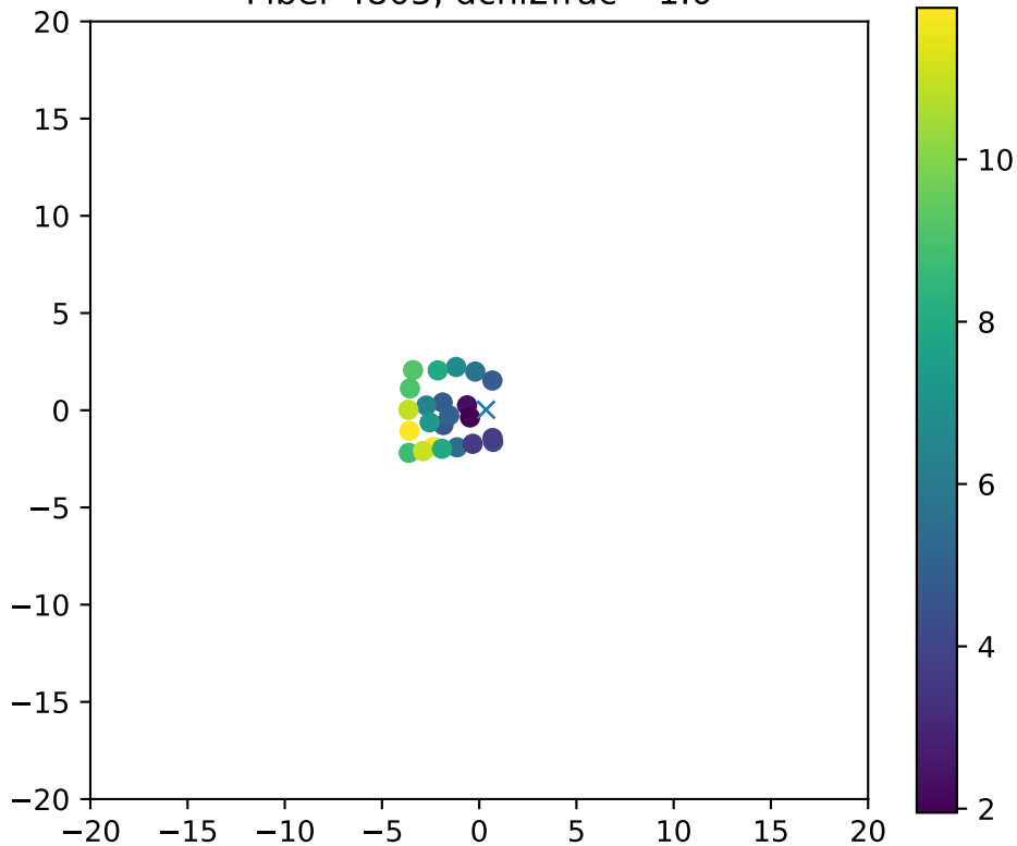
Fiber 4805, dchi2frac= 1.0
