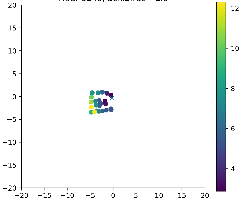
Fiber 3248, dchi2frac= 1.0
