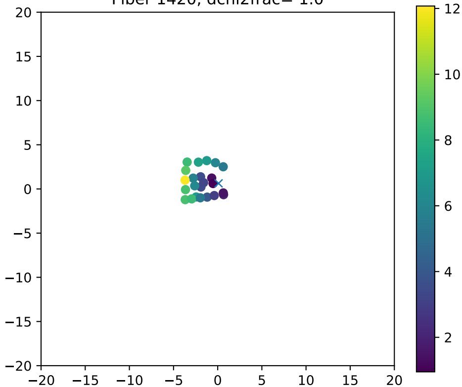
Fiber 1420, dchi2frac= 1.0
