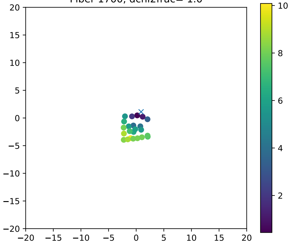
Fiber 1700, dchi2frac= 1.0
