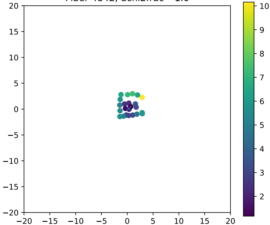
Fiber 4842, dchi2frac= 1.0
