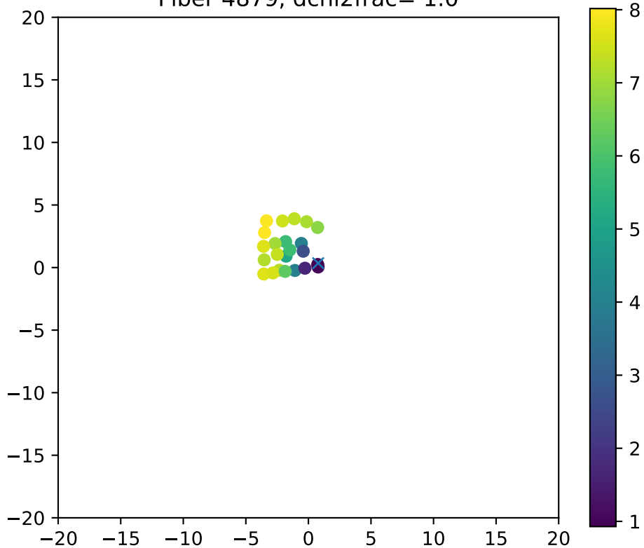
Fiber 4879, dchi2frac= 1.0
