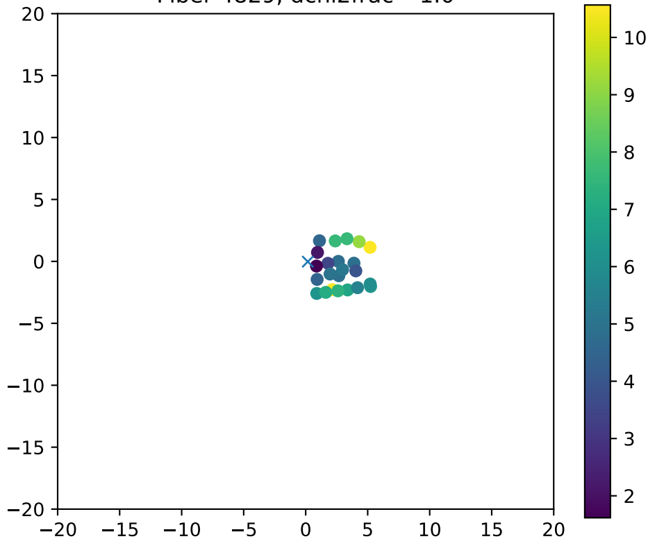
Fiber 4829, dchi2frac= 1.0
