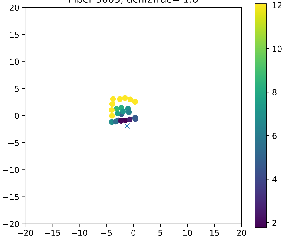
Fiber 3003, dchi2frac= 1.0
