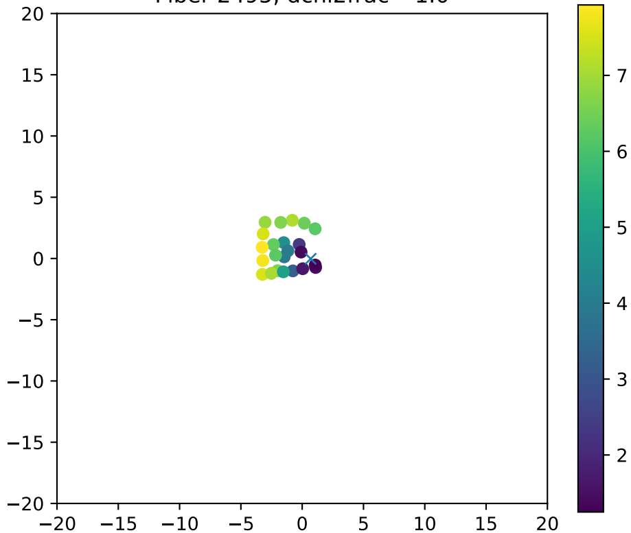
Fiber 2495, dchi2frac= 1.0
