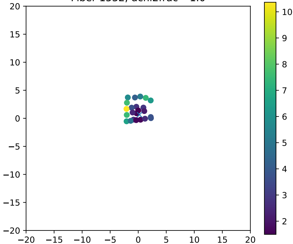
Fiber 1532, dchi2frac= 1.0
