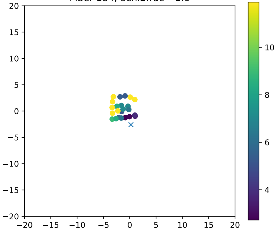
Fiber 184, dchi2frac= 1.0
