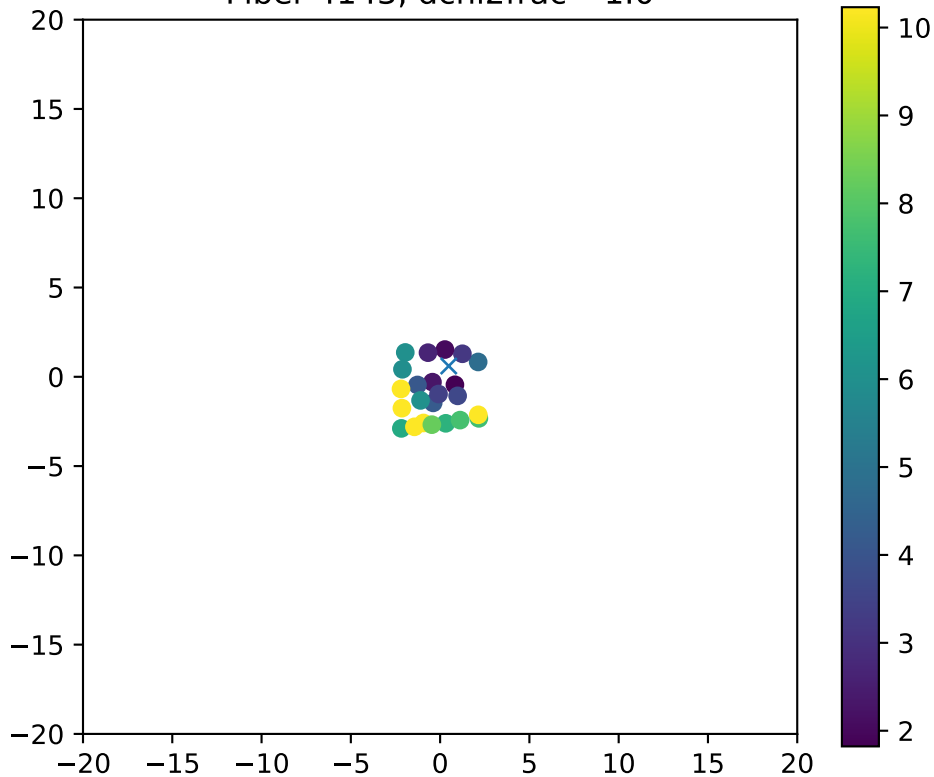
Fiber 4143, dchi2frac= 1.0
