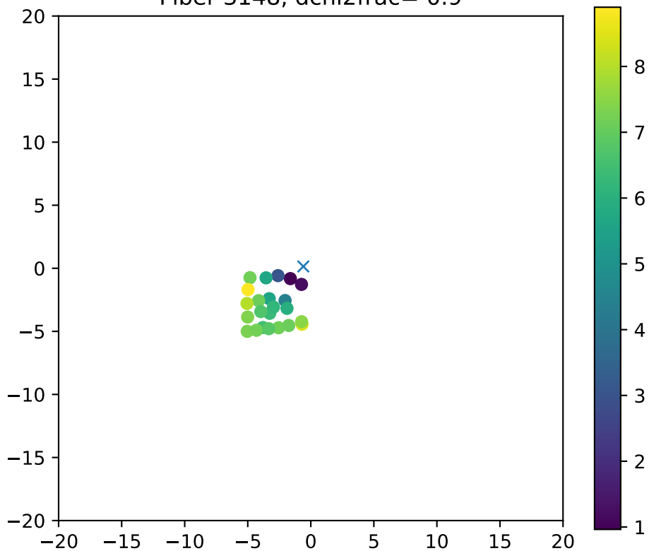
Fiber 3148, dchi2frac= 0.9
