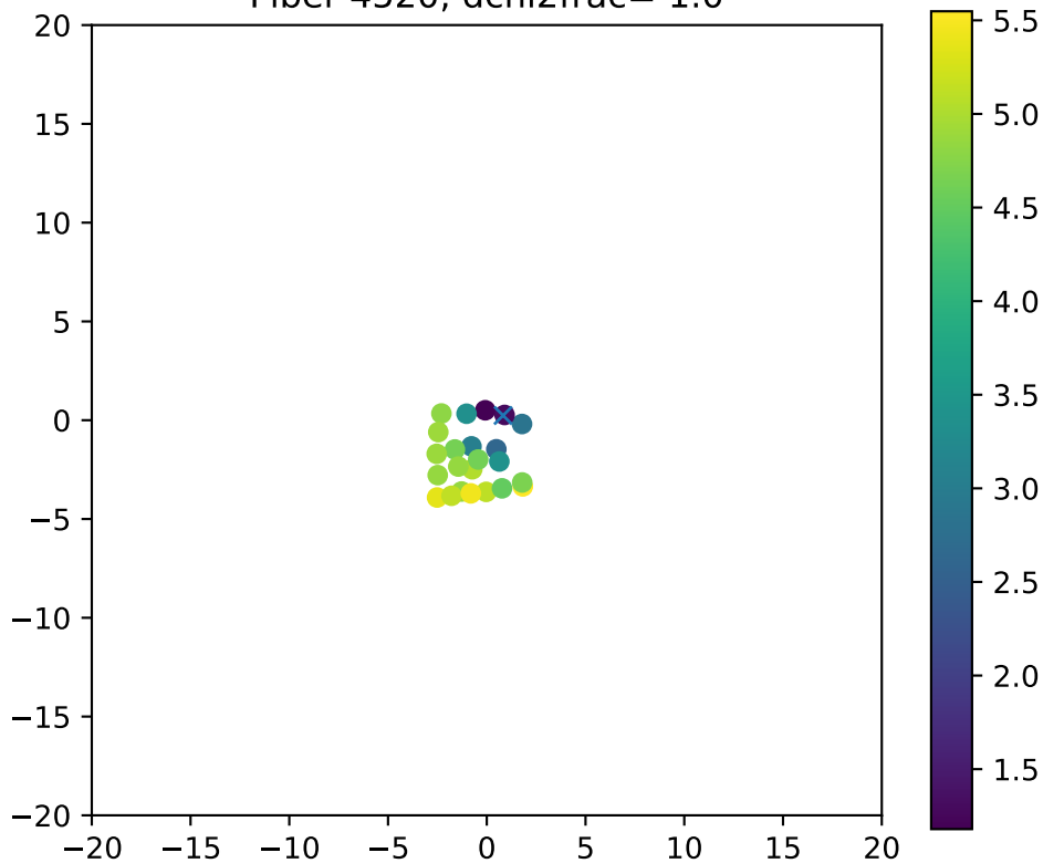
Fiber 4520, dchi2frac= 1.0
