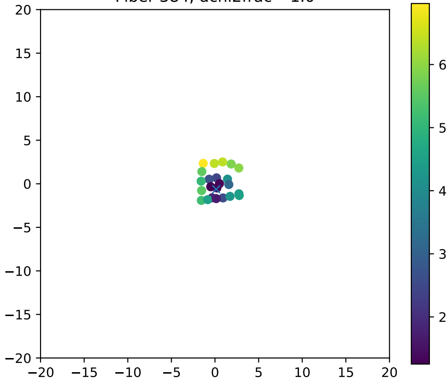
Fiber 384, dchi2frac= 1.0
