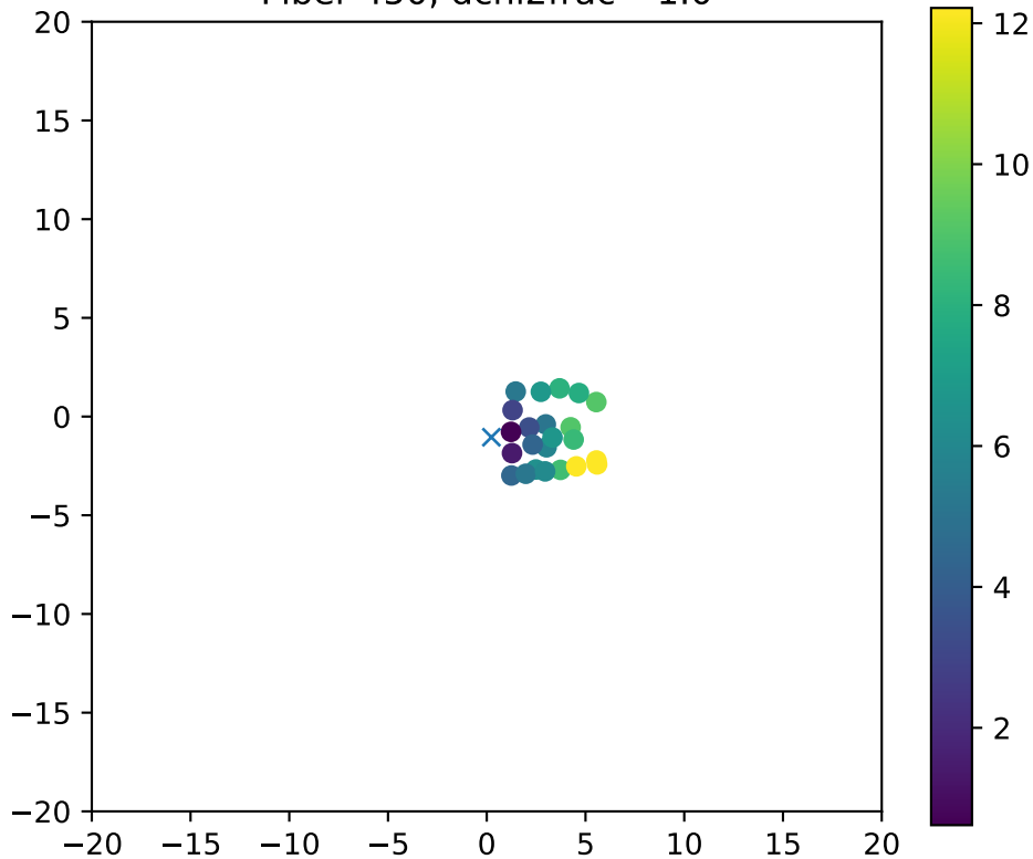
Fiber 450, dchi2frac= 1.0
