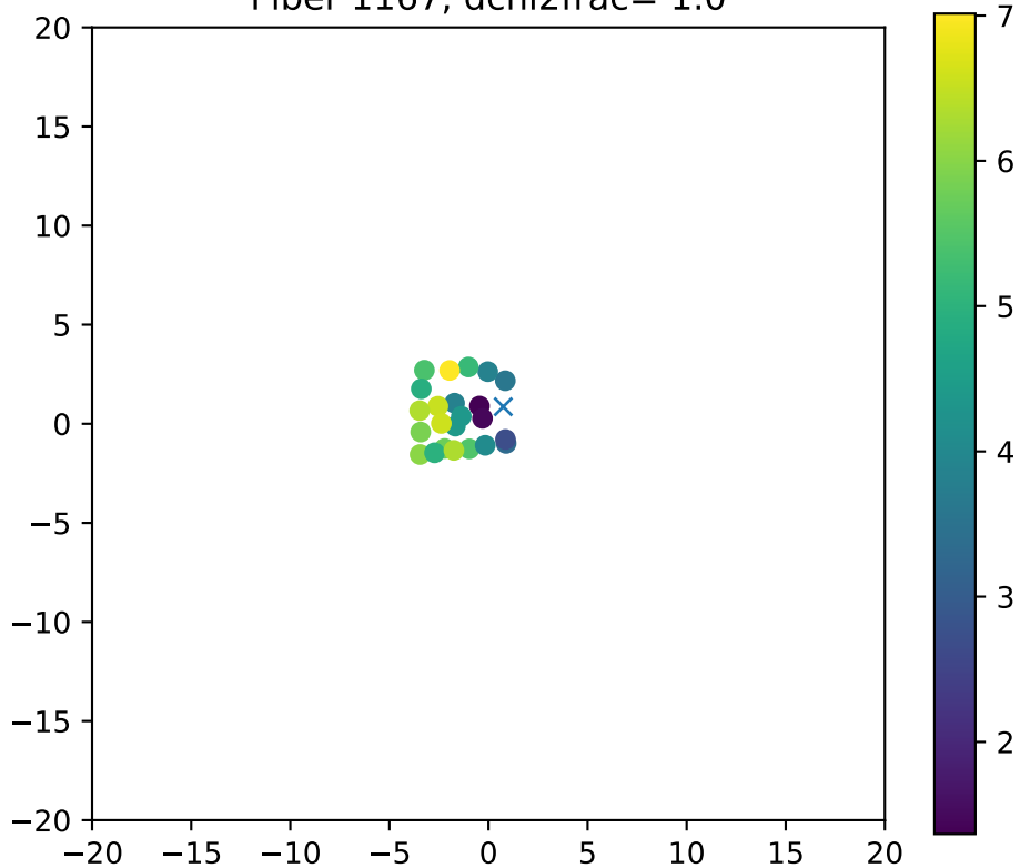
Fiber 1167, dchi2frac= 1.0
