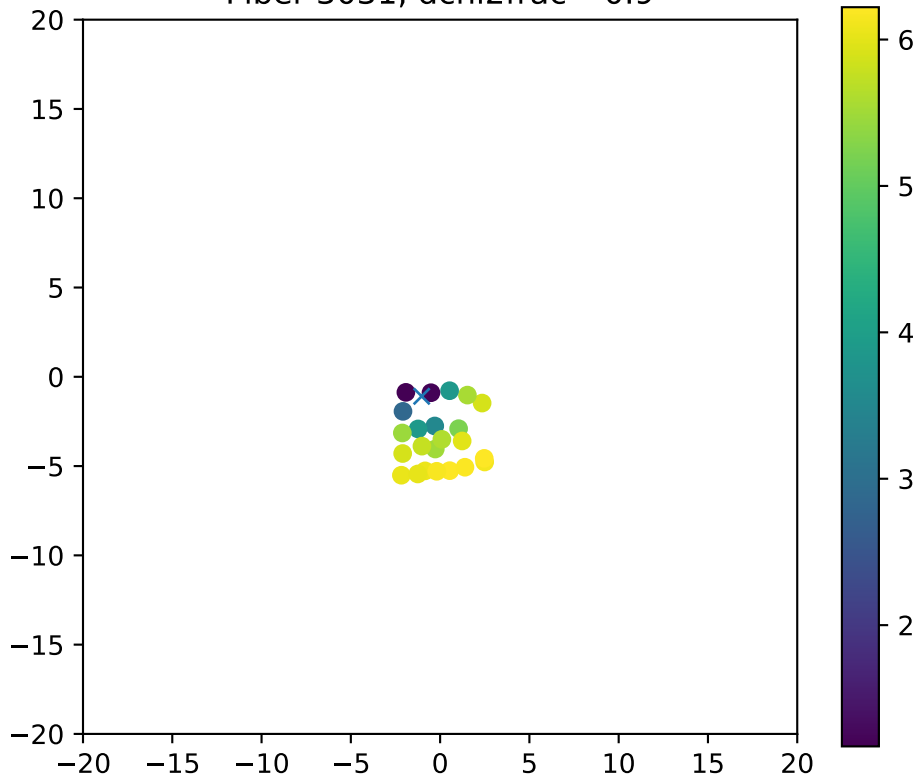
Fiber 3031, dchi2frac= 0.9
