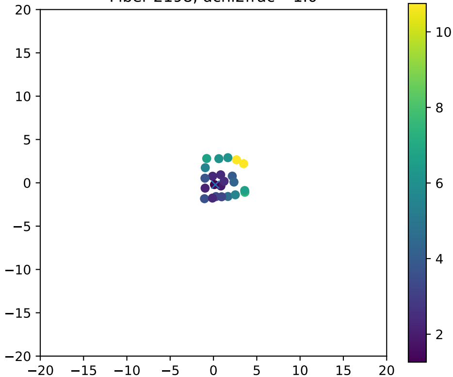
Fiber 2198, dchi2frac= 1.0
