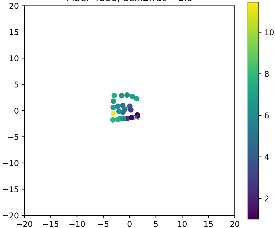
Fiber 4806, dchi2frac= 1.0
