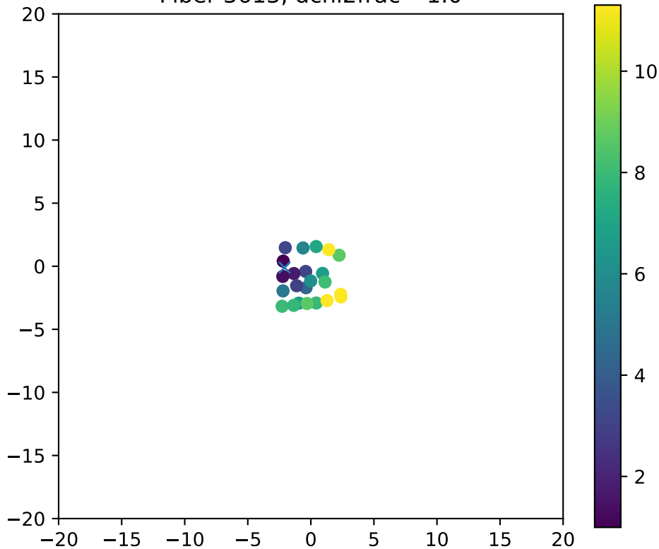
Fiber 3613, dchi2frac= 1.0
