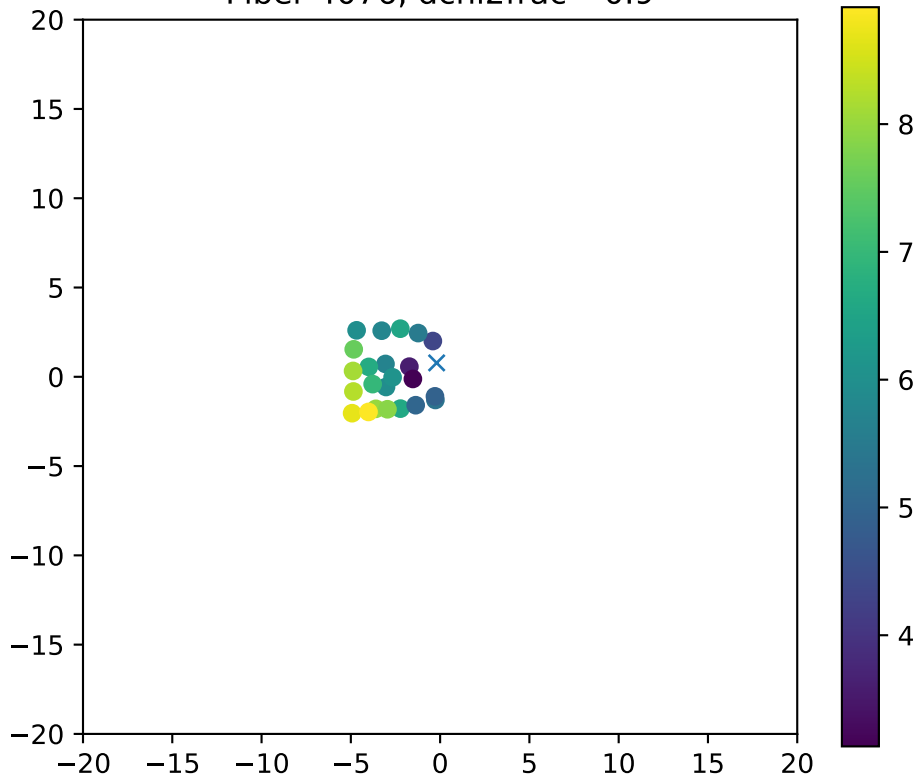
Fiber 4076, dchi2frac= 0.9
