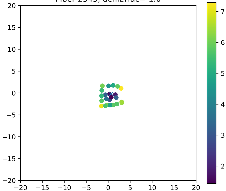
Fiber 2343, dchi2frac= 1.0
