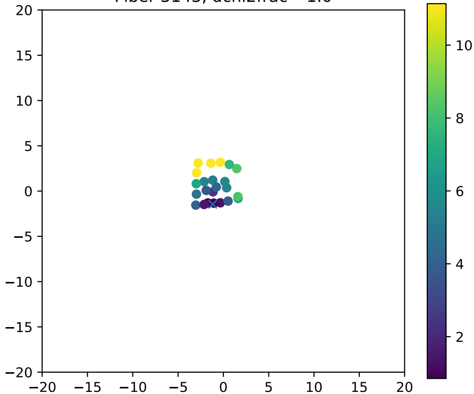
Fiber 3143, dchi2frac= 1.0
