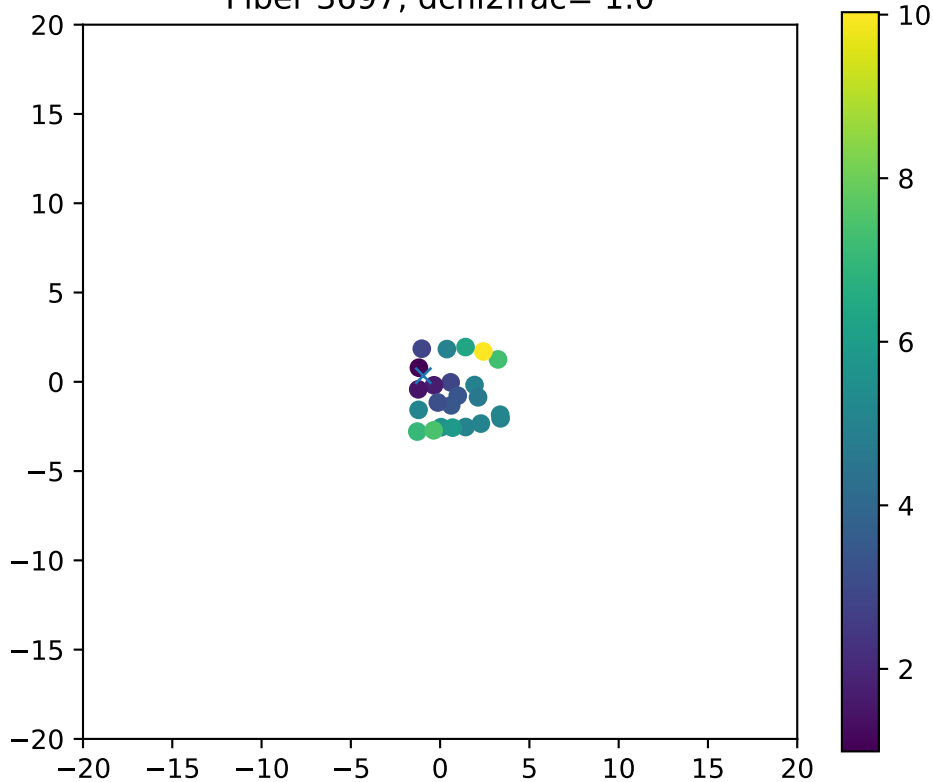
Fiber 3697, dchi2frac= 1.0
