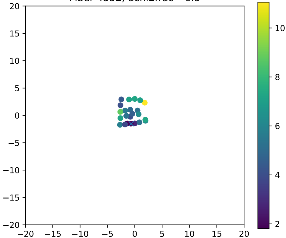
Fiber 4552, dchi2frac= 0.9
