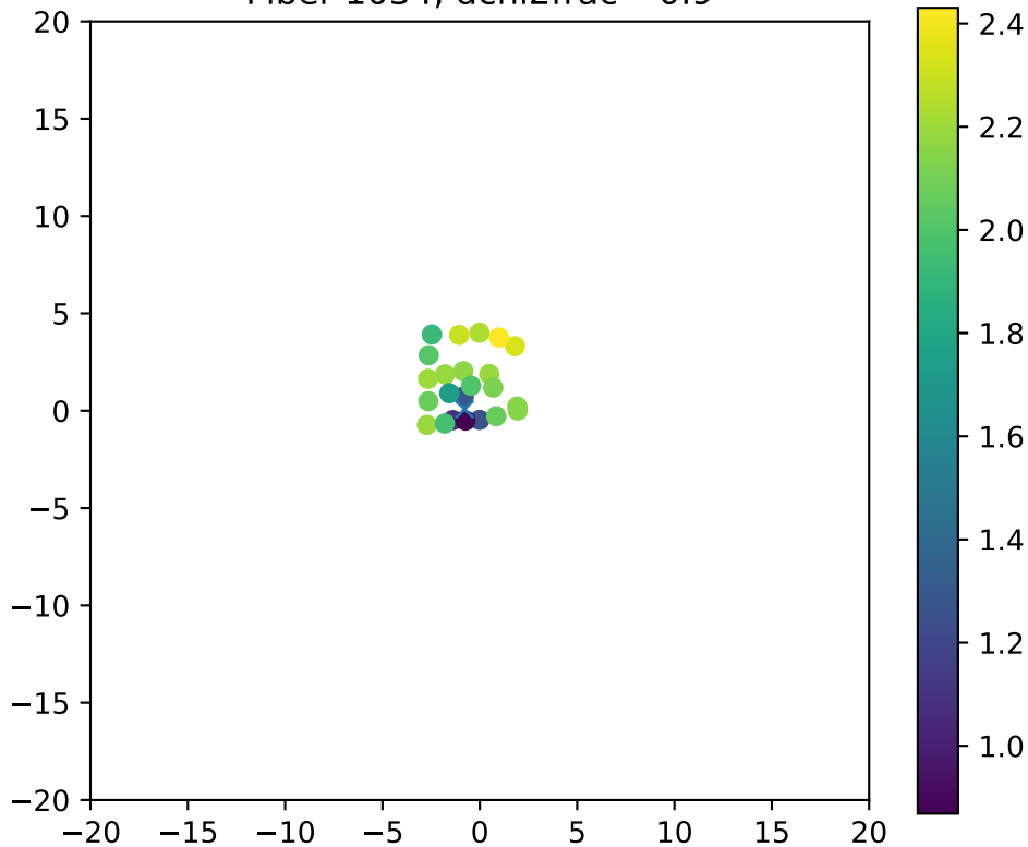
Fiber 1034, dchi2frac= 0.9
