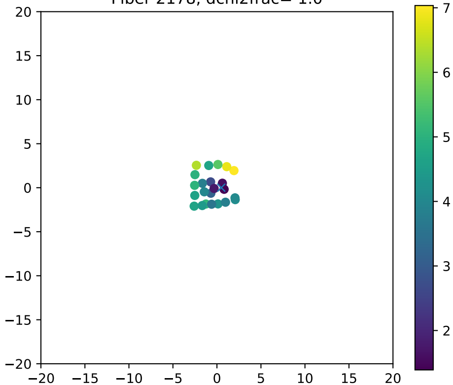
Fiber 2178, dchi2frac= 1.0
