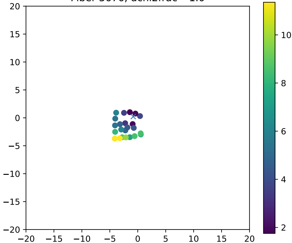
Fiber 3676, dchi2frac= 1.0
