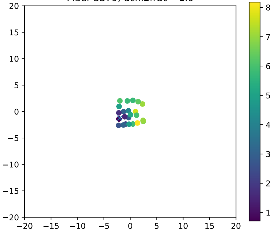
Fiber 3379, dchi2frac= 1.0
