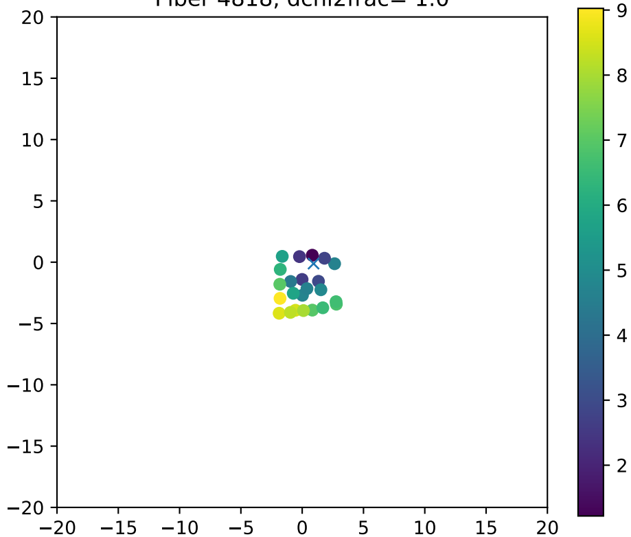
Fiber 4818, dchi2frac= 1.0
