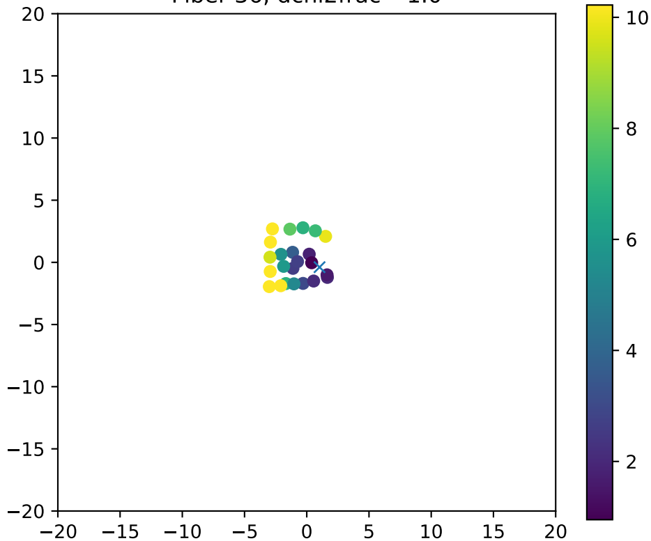
Fiber 36, dchi2frac= 1.0
