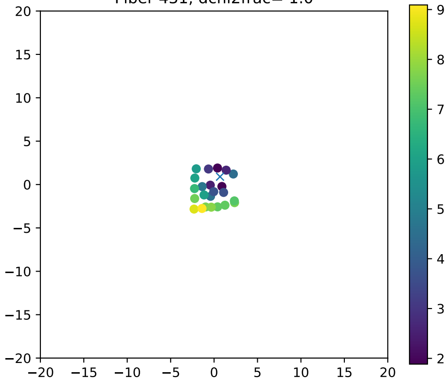
Fiber 431, dchi2frac= 1.0
