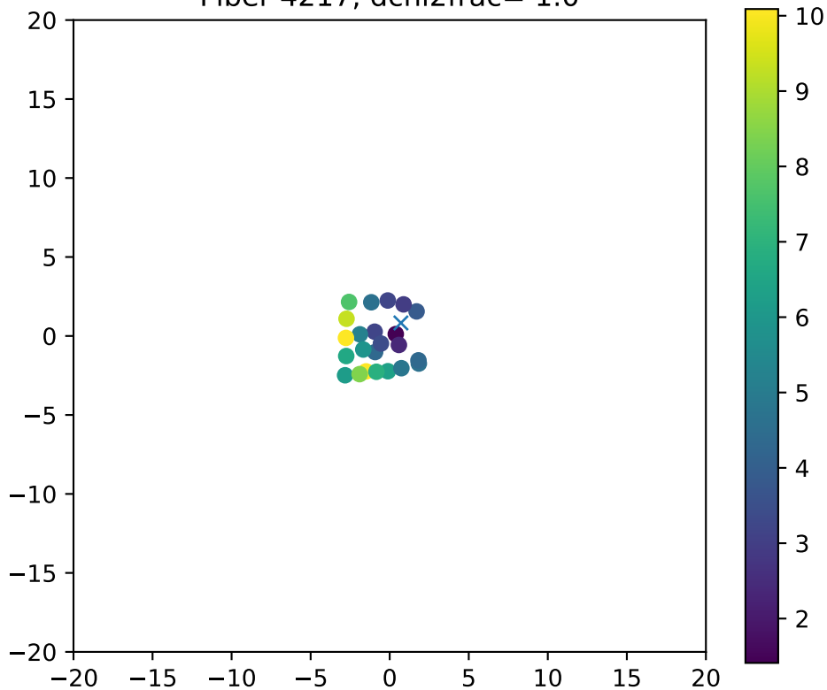
Fiber 4217, dchi2frac= 1.0
