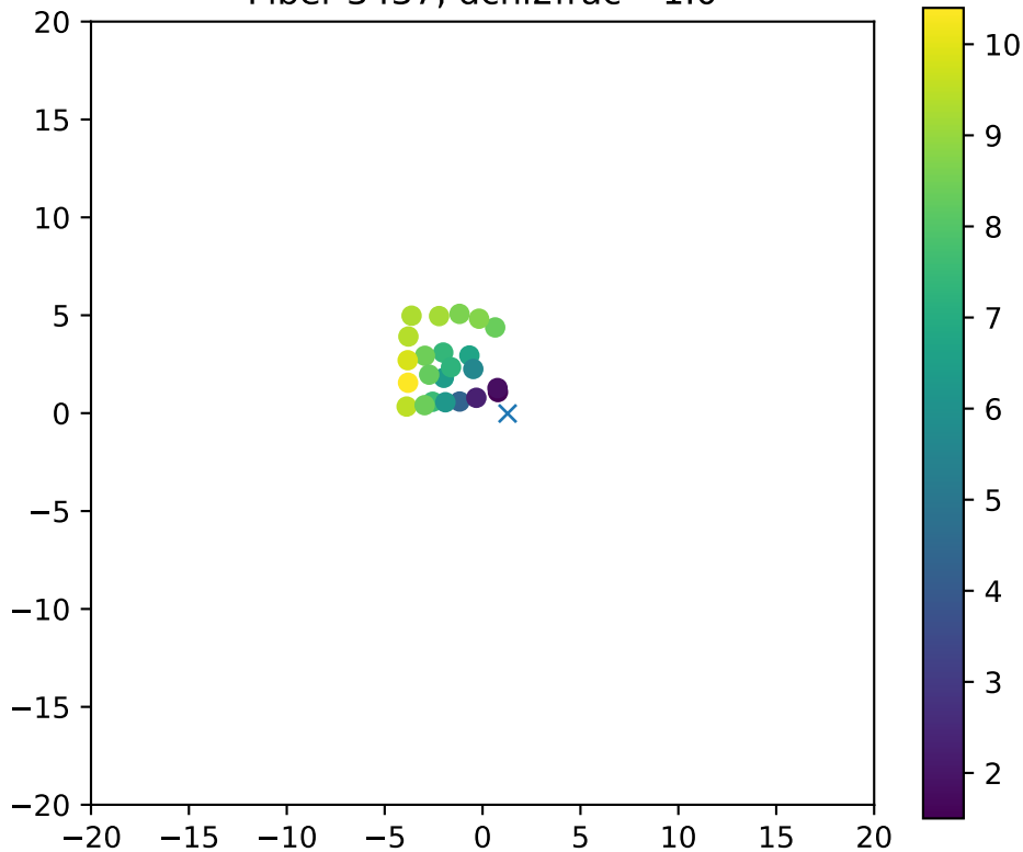
Fiber 3437, dchi2frac= 1.0
