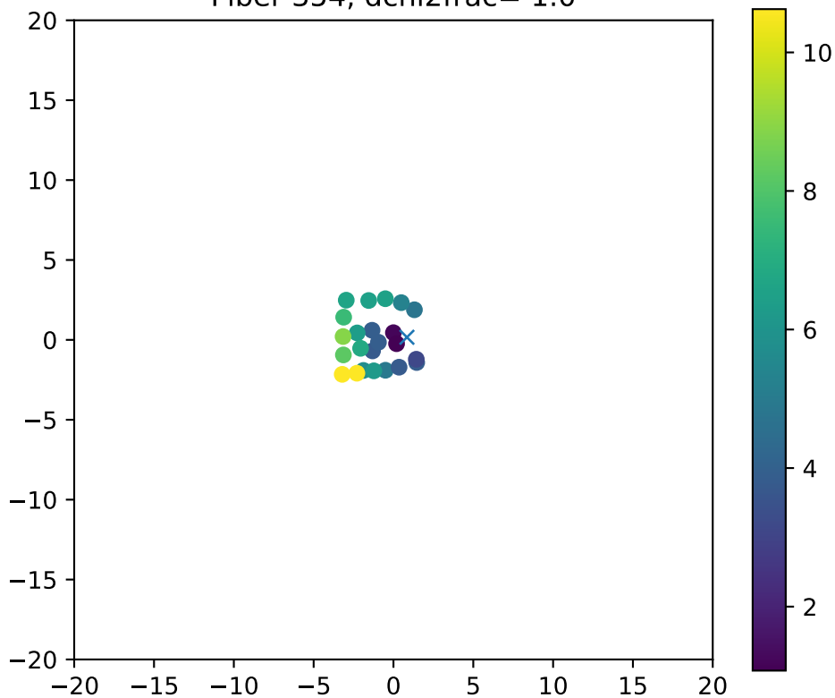
Fiber 354, dchi2frac= 1.0
