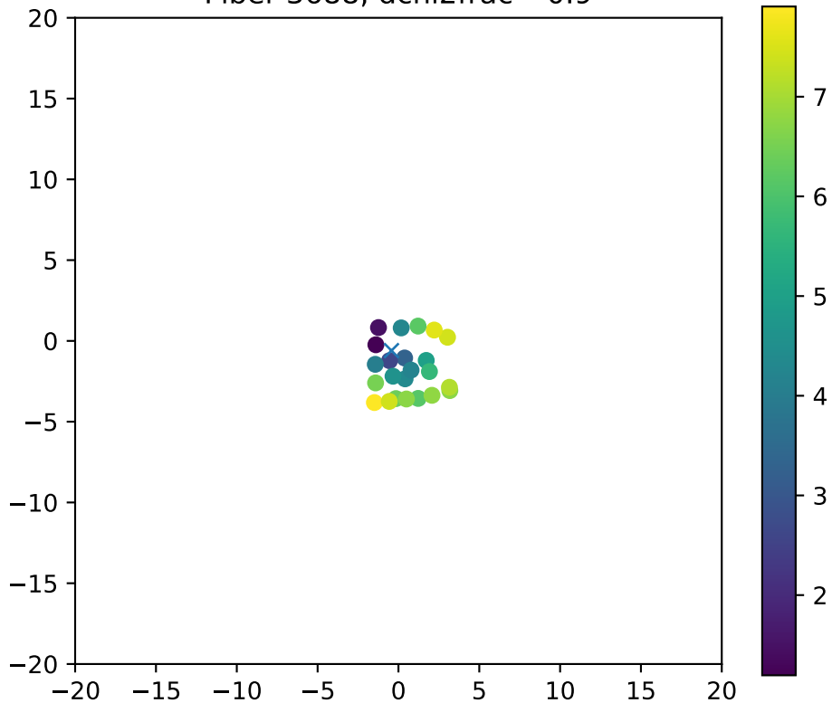
Fiber 3688, dchi2frac= 0.9
