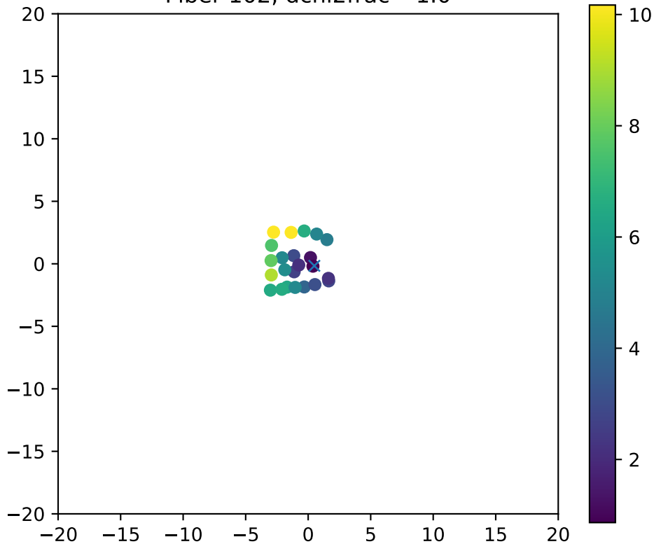
Fiber 102, dchi2frac= 1.0
