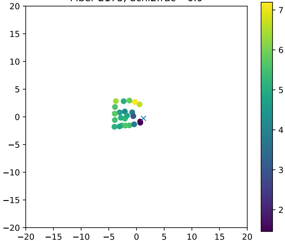
Fiber 2173, dchi2frac= 0.9
