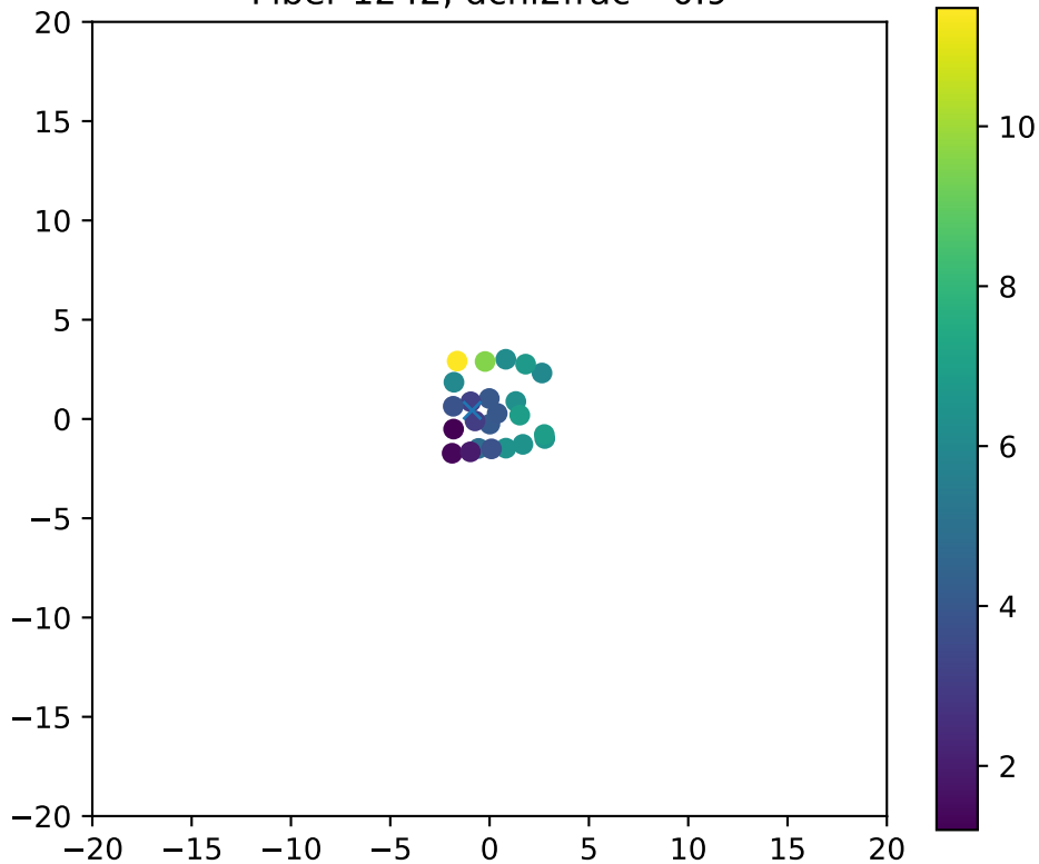
Fiber 1242, dchi2frac= 0.9
