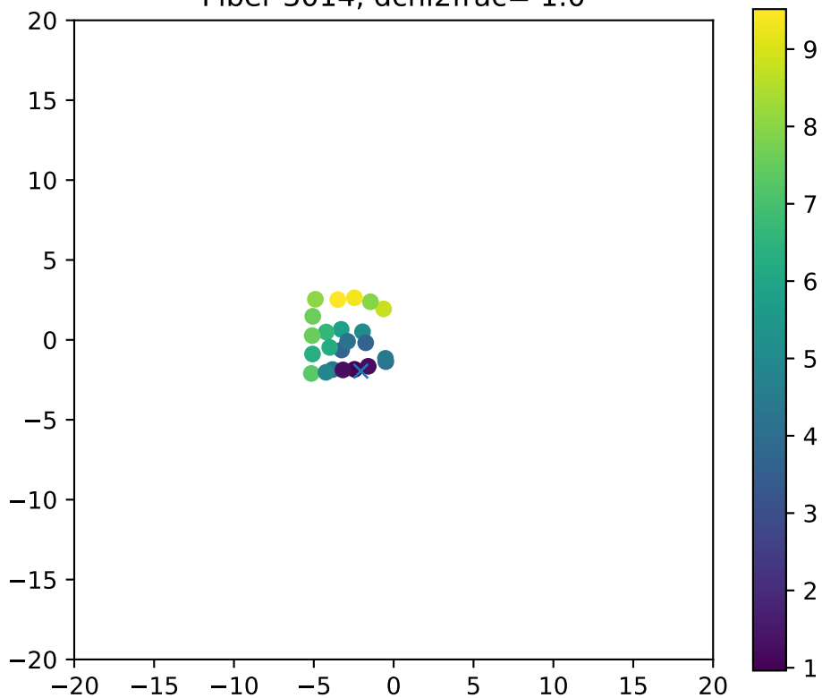
Fiber 3014, dchi2frac= 1.0
