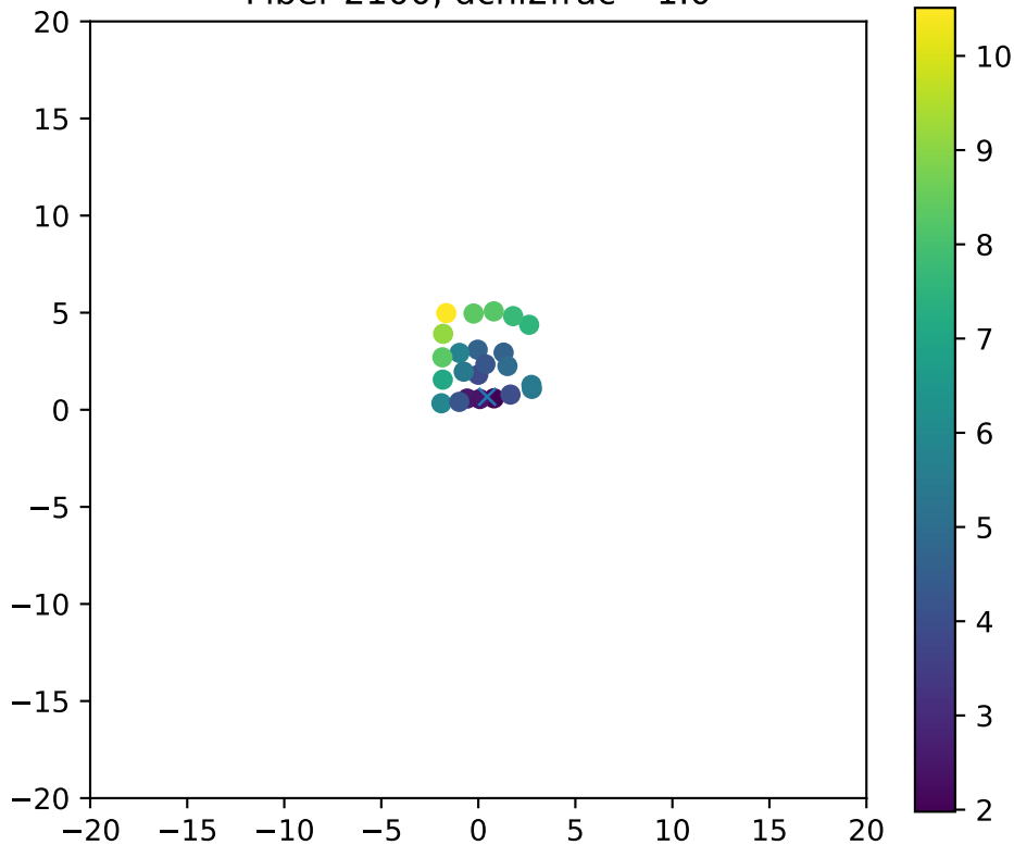
Fiber 2100, dchi2frac= 1.0
