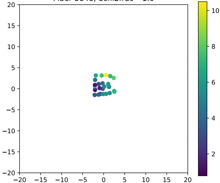
Fiber 3848, dchi2frac= 1.0
