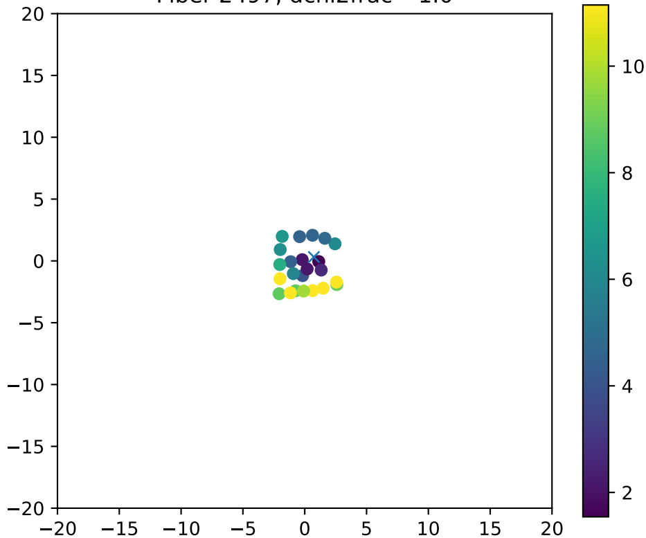
Fiber 2497, dchi2frac= 1.0
