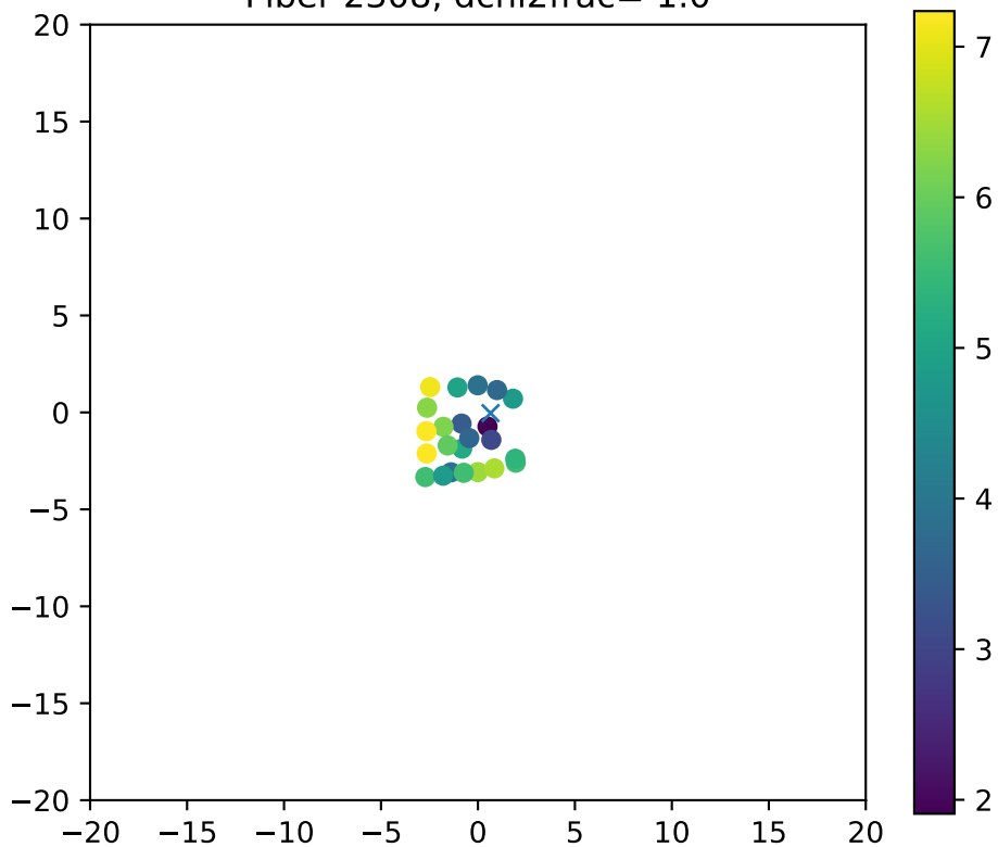
Fiber 2308, dchi2frac= 1.0
