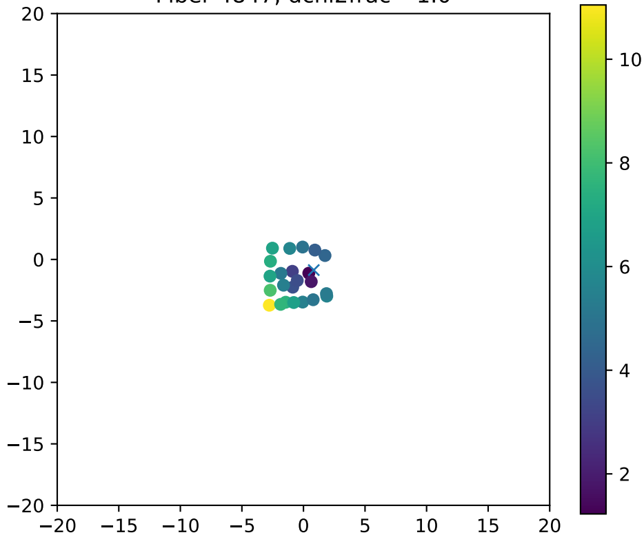
Fiber 4847, dchi2frac= 1.0
