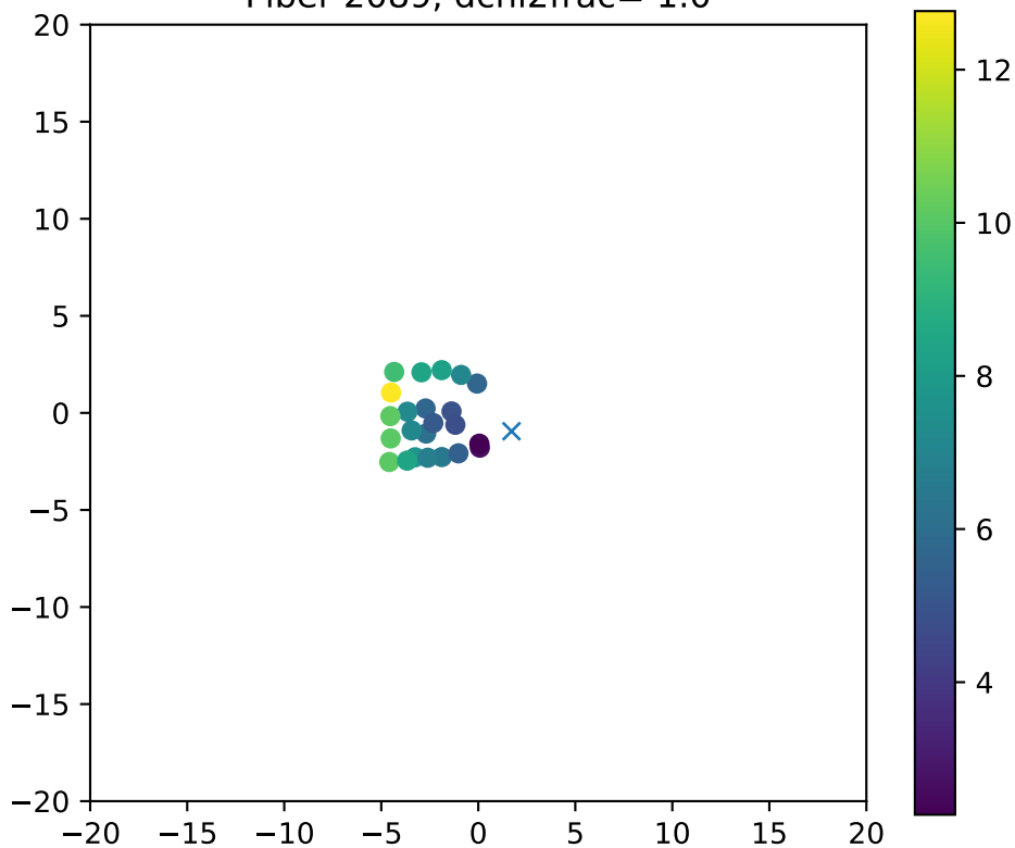
Fiber 2089, dchi2frac= 1.0
