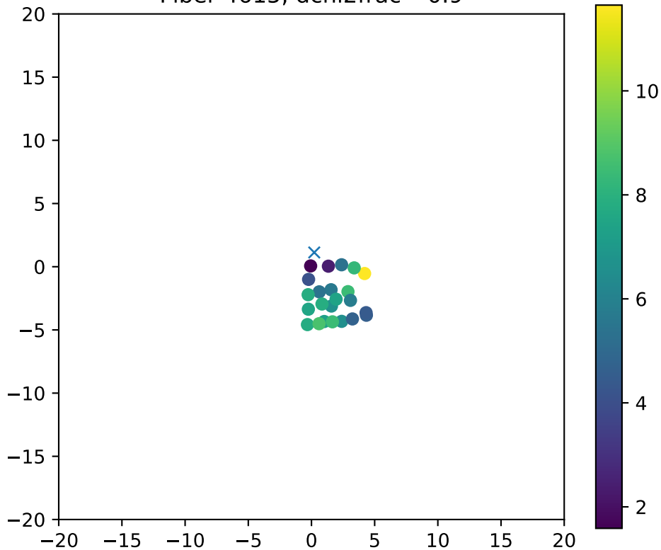
Fiber 4615, dchi2frac= 0.9
