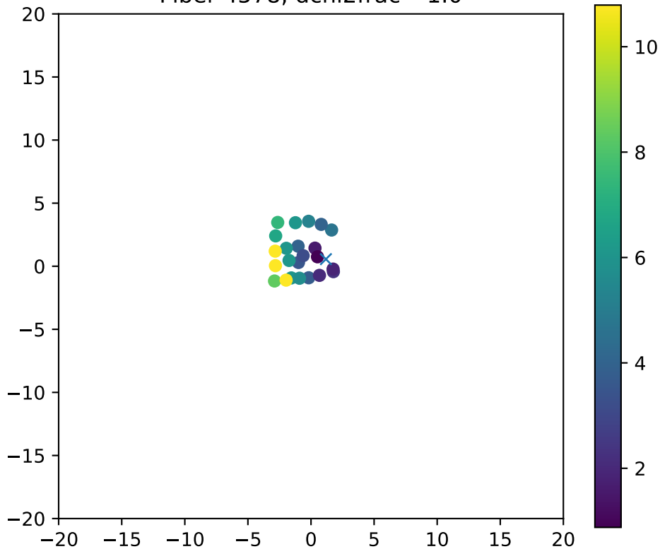
Fiber 4578, dchi2frac= 1.0
