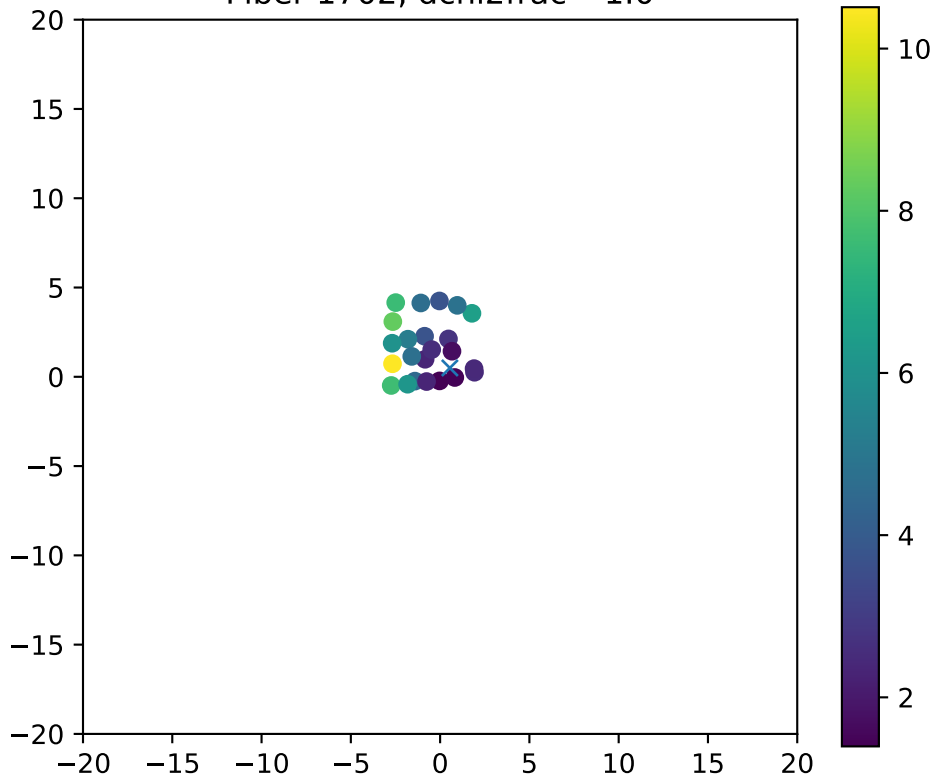
Fiber 1702, dchi2frac= 1.0
