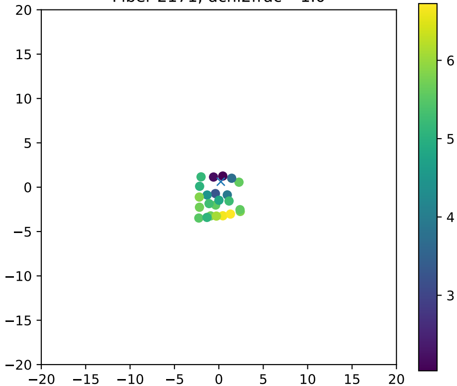
Fiber 2171, dchi2frac= 1.0
