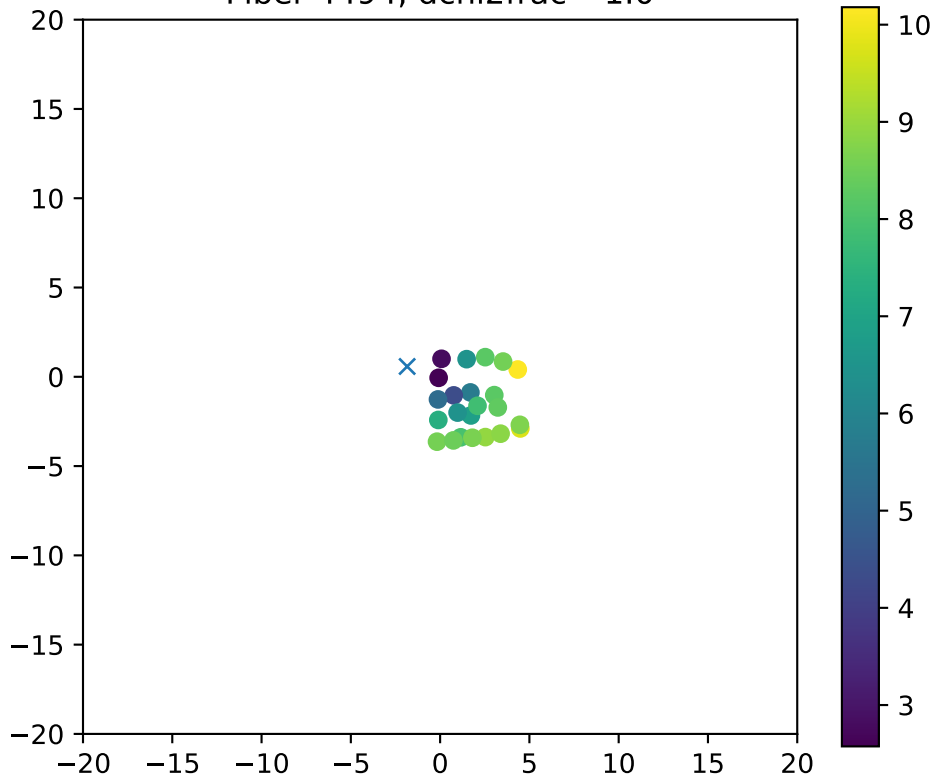
Fiber 4494, dchi2frac= 1.0
