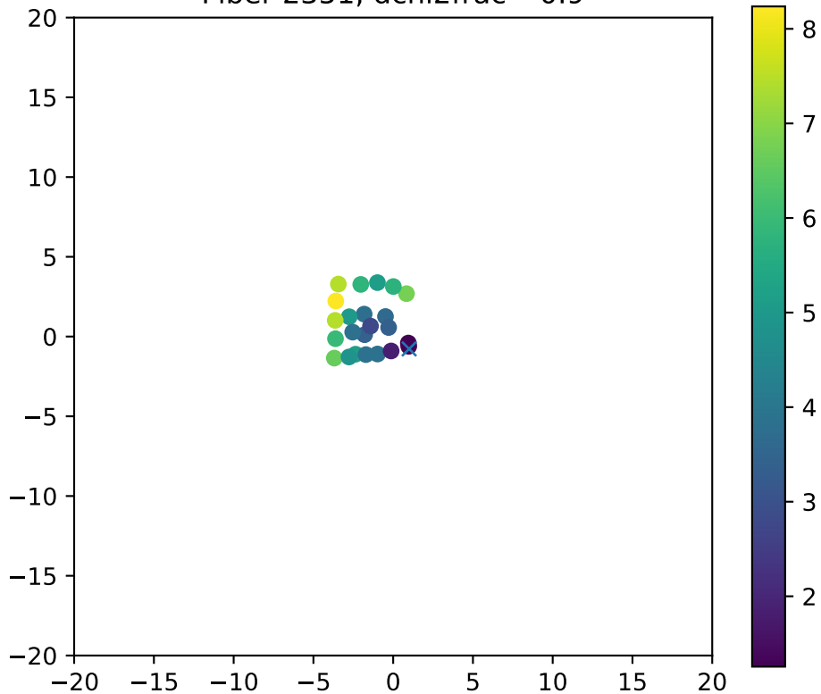
Fiber 2351, dchi2frac= 0.9
