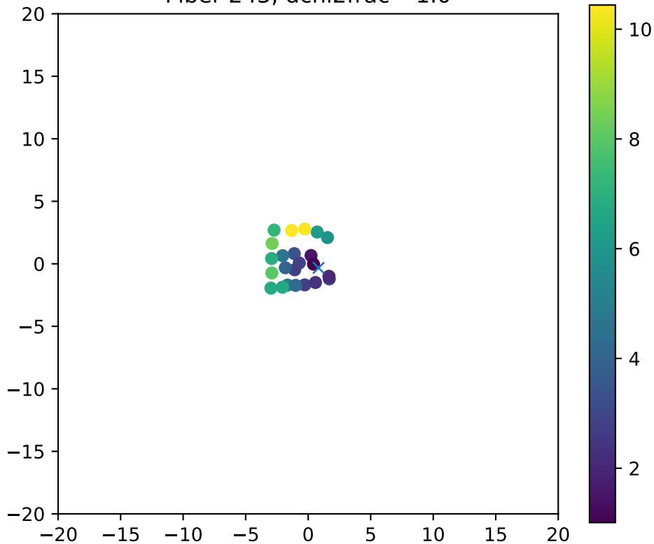
Fiber 243, dchi2frac= 1.0
