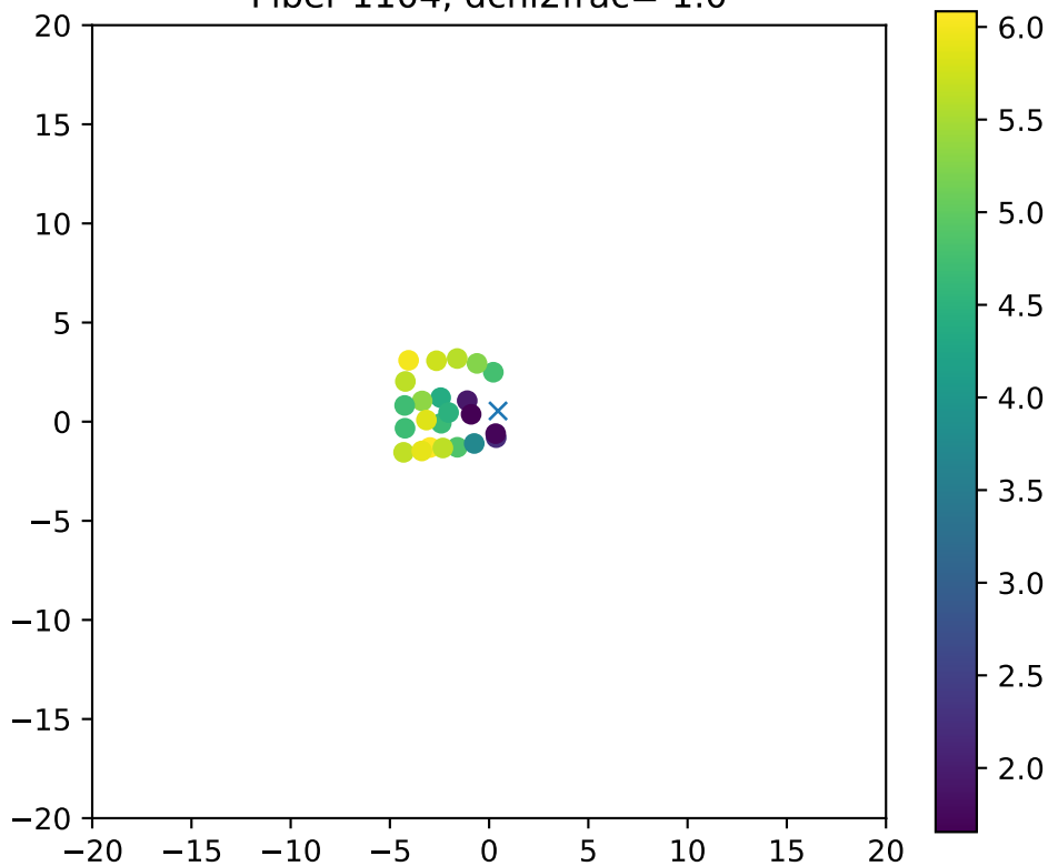
Fiber 1104, dchi2frac= 1.0
