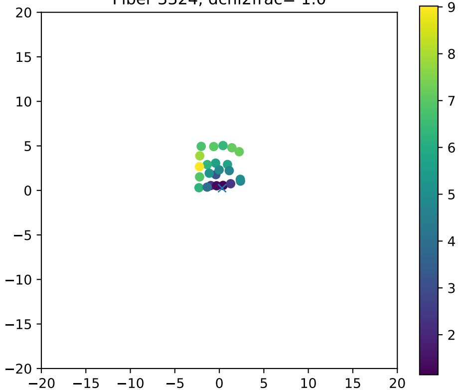
Fiber 3324, dchi2frac= 1.0
