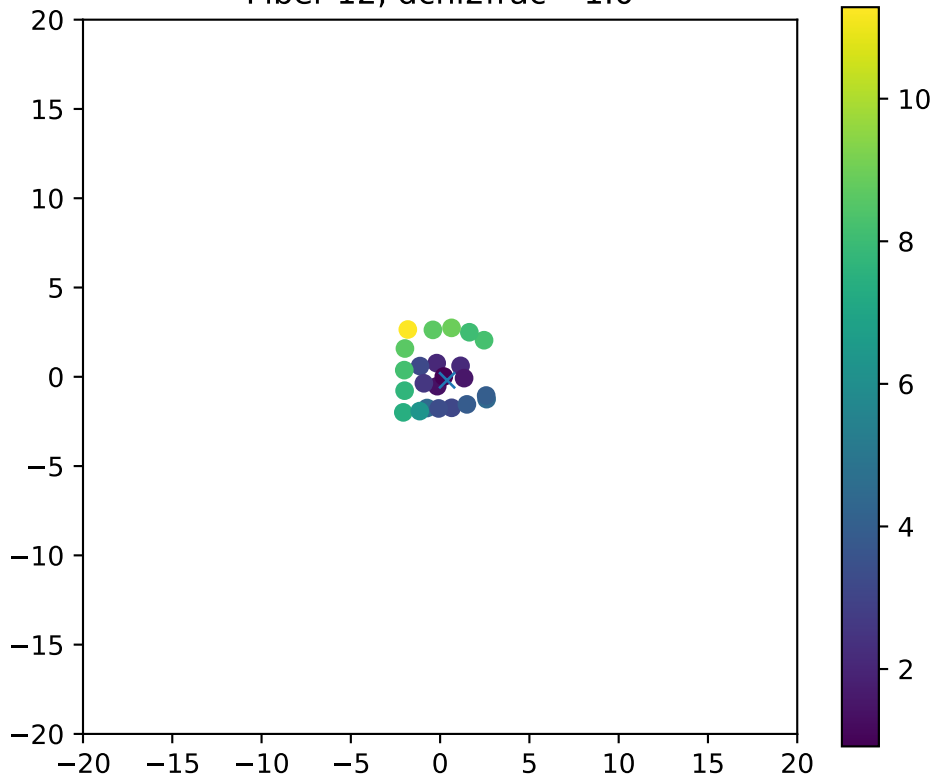
Fiber 12, dchi2frac= 1.0
