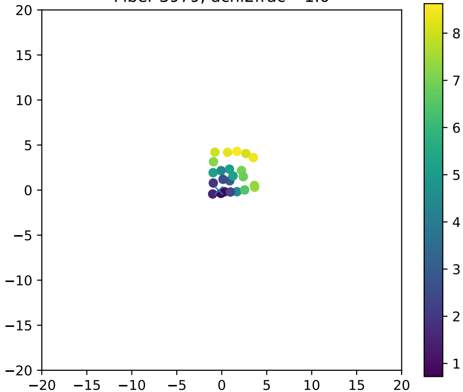
Fiber 3979, dchi2frac= 1.0
