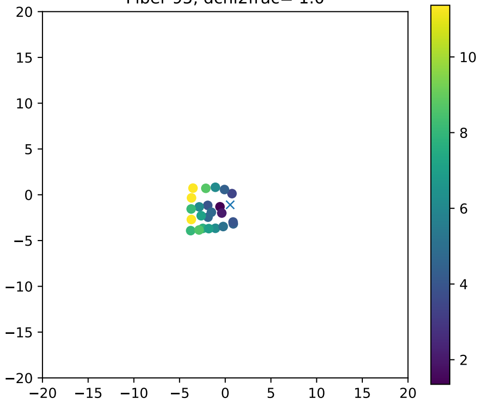
Fiber 95, dchi2frac= 1.0
