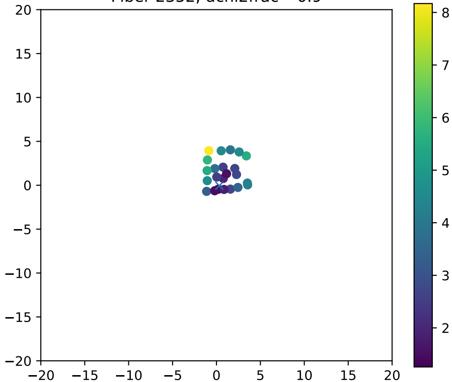
Fiber 2352, dchi2frac= 0.9
