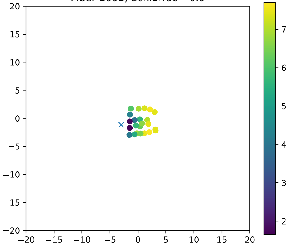
Fiber 1092, dchi2frac= 0.9
