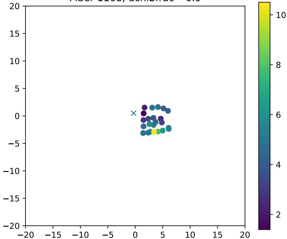
Fiber 1168, dchi2frac= 0.9
