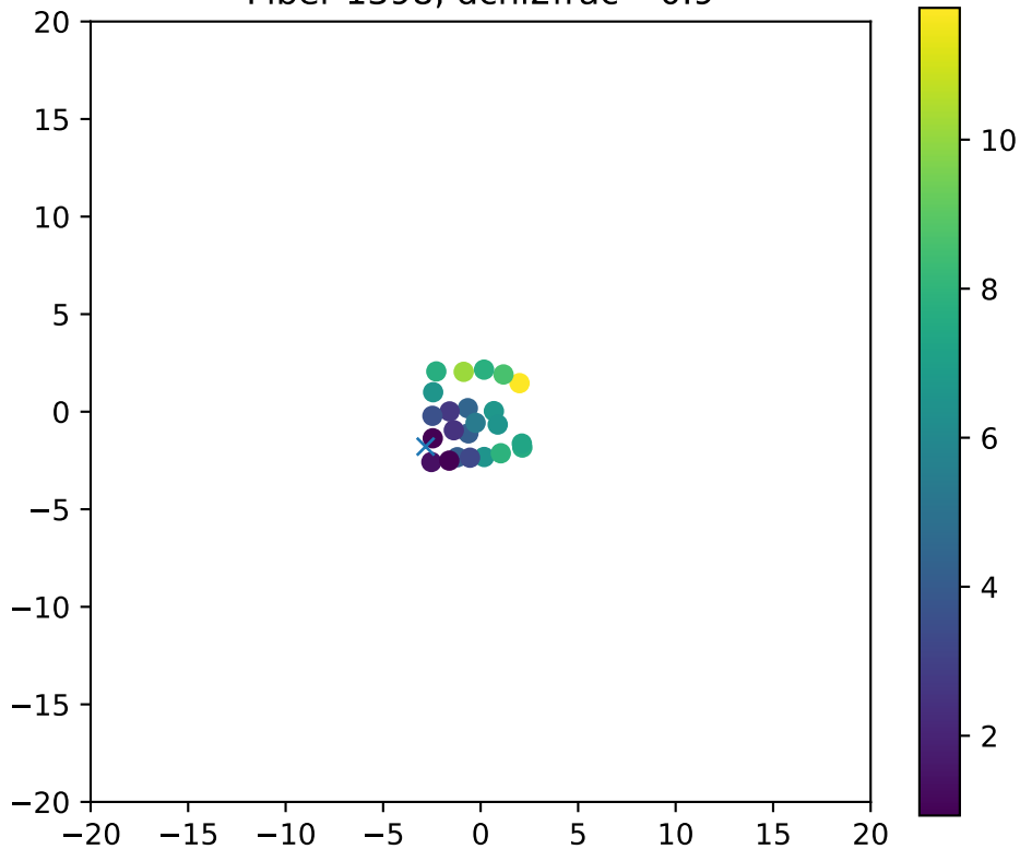
Fiber 1398, dchi2frac= 0.9
