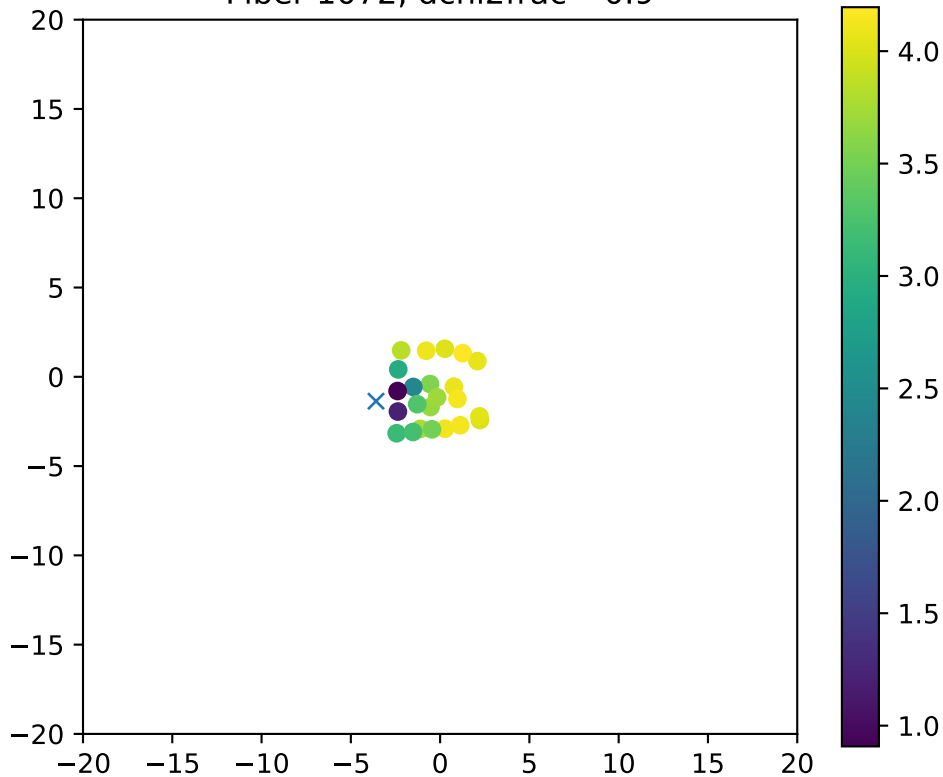
Fiber 1072, dchi2frac= 0.9
