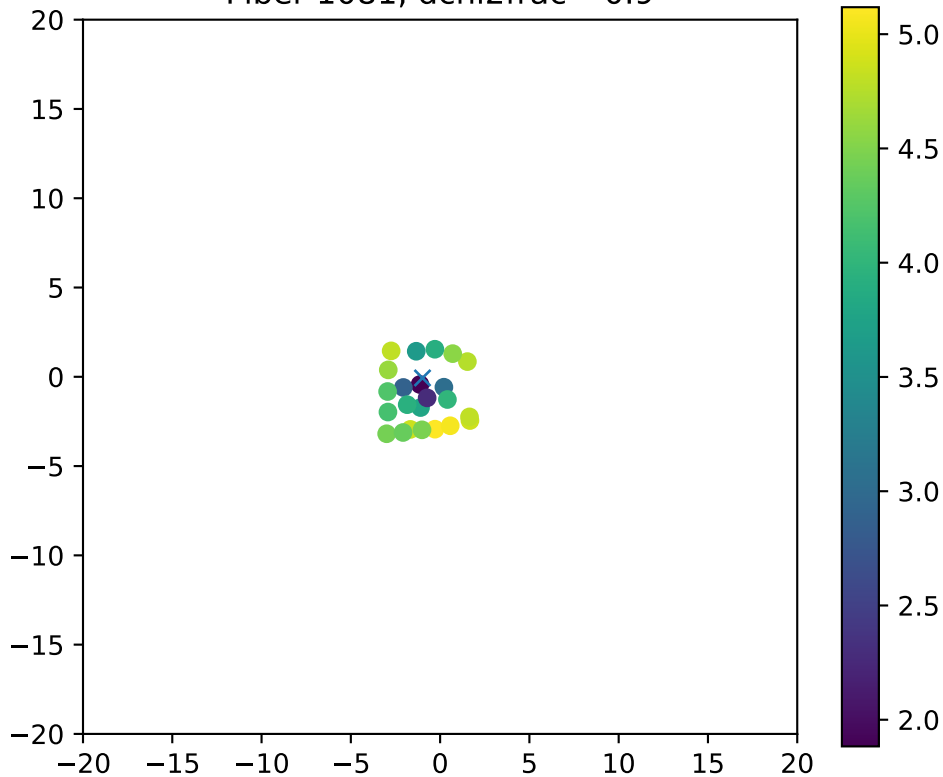
Fiber 1081, dchi2frac= 0.9
