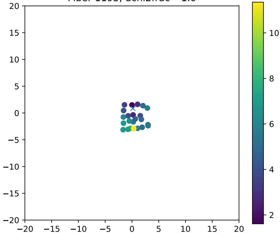
Fiber 1195, dchi2frac= 1.0
