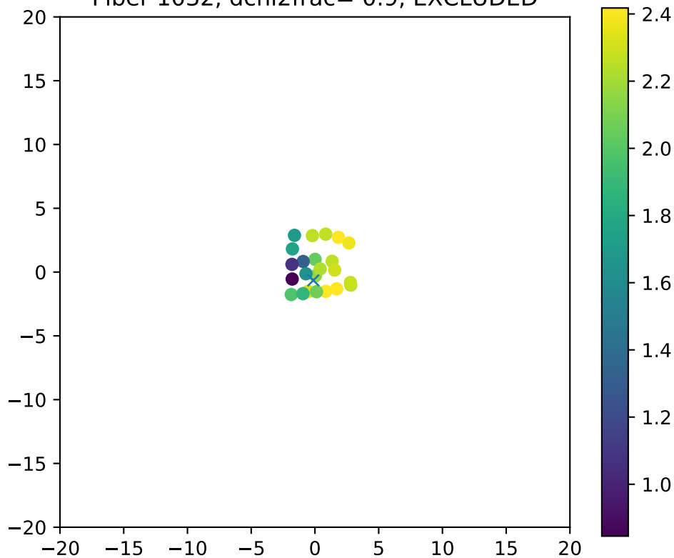
Fiber 1032, dchi2frac= 0.9, EXCLUDED
