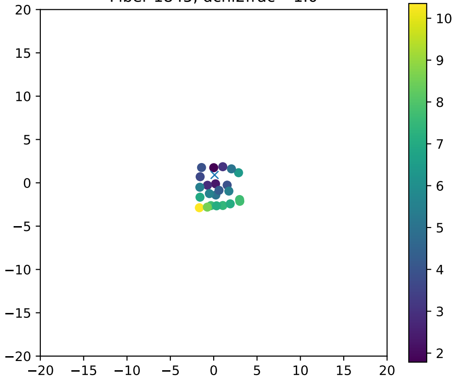
Fiber 1845, dchi2frac= 1.0
