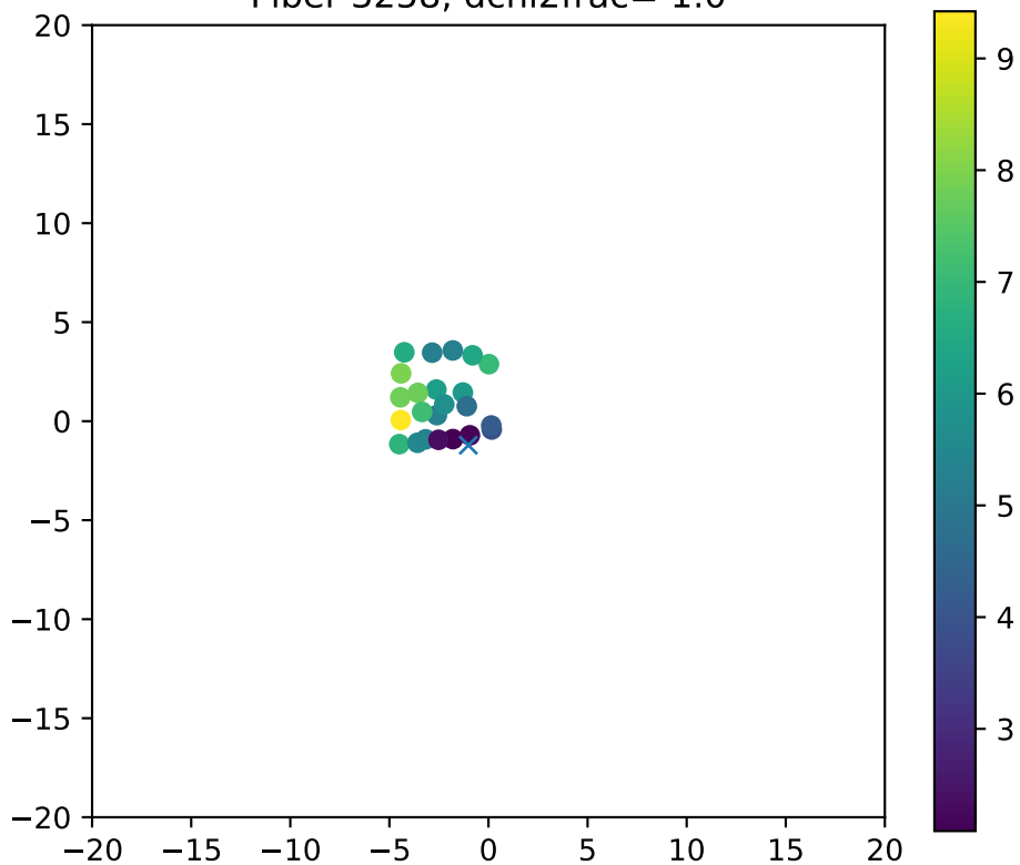
Fiber 3258, dchi2frac= 1.0
