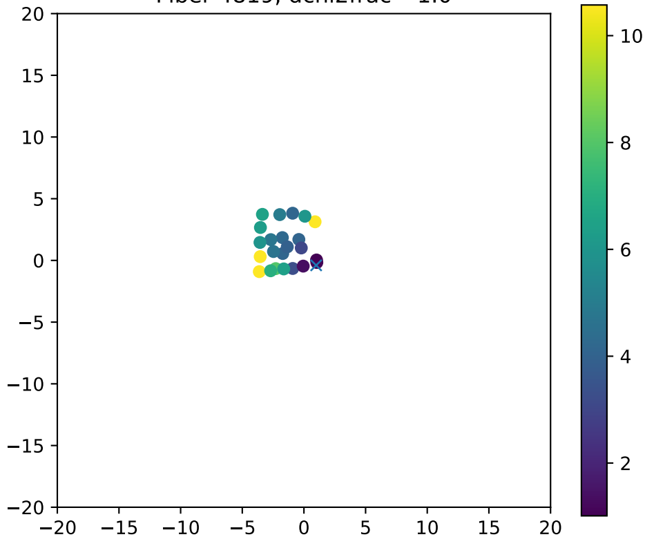
Fiber 4819, dchi2frac= 1.0
