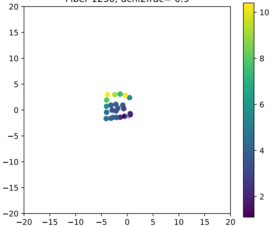
Fiber 1230, dchi2frac= 0.9
