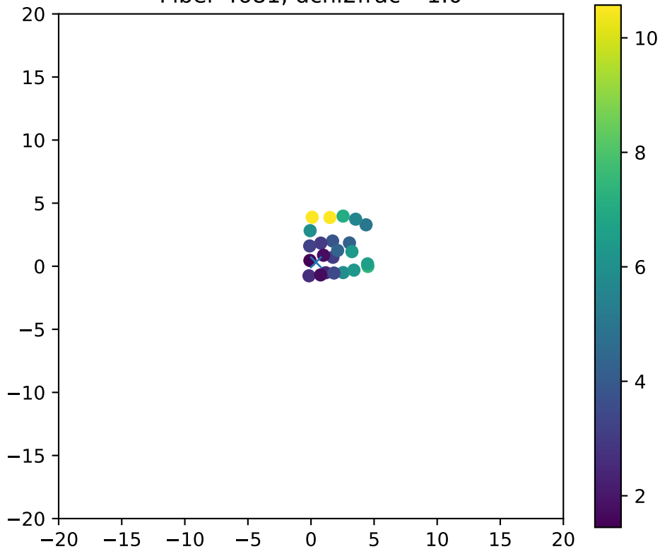
Fiber 4681, dchi2frac= 1.0
