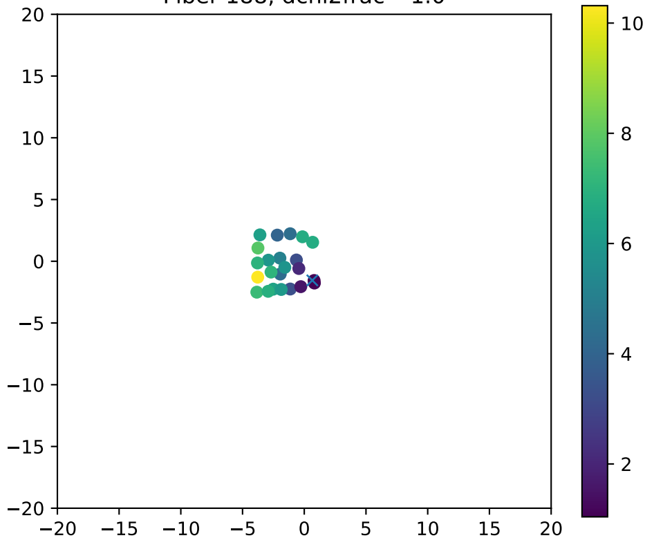
Fiber 188, dchi2frac= 1.0
