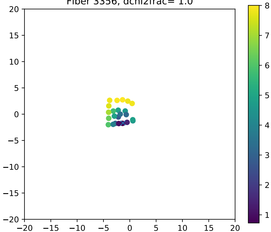
Fiber 3356, dchi2frac= 1.0
