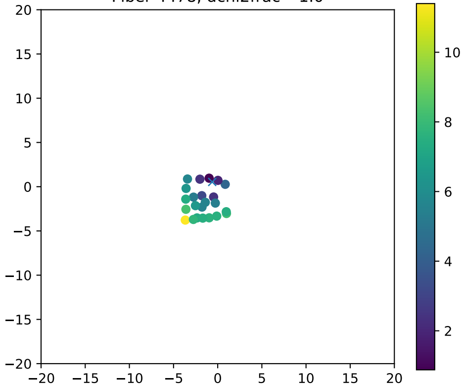
Fiber 4478, dchi2frac= 1.0
