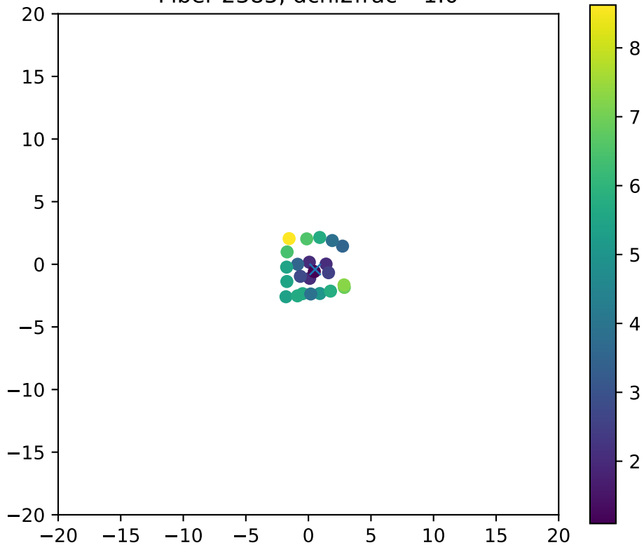
Fiber 2385, dchi2frac= 1.0
