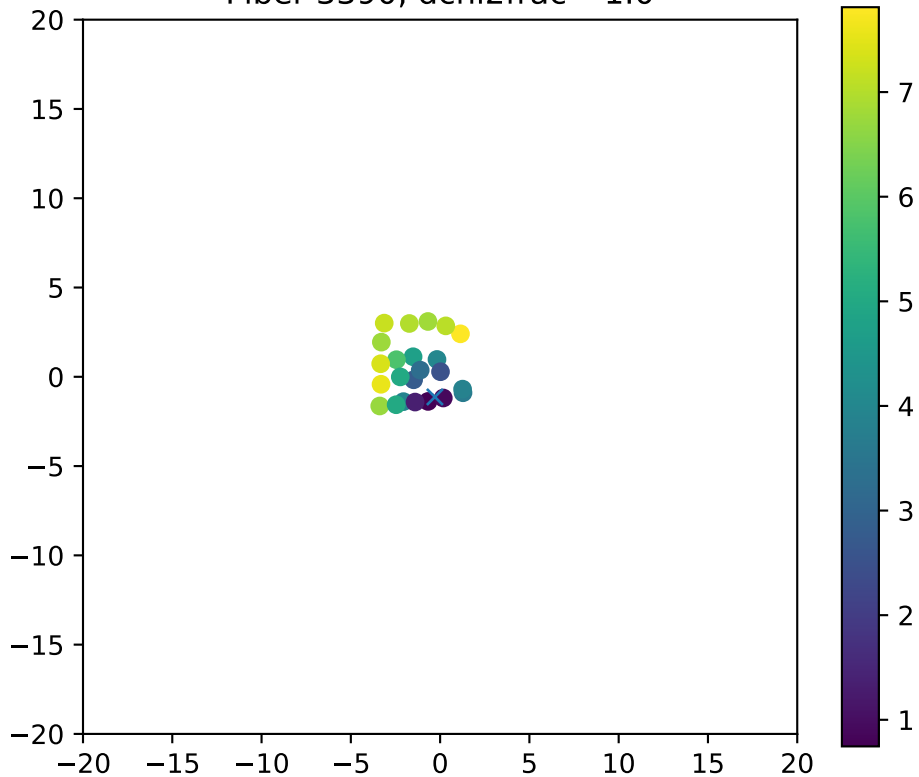
Fiber 3390, dchi2frac= 1.0
