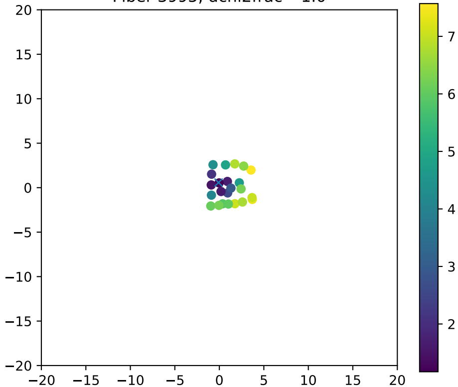
Fiber 3995, dchi2frac= 1.0
