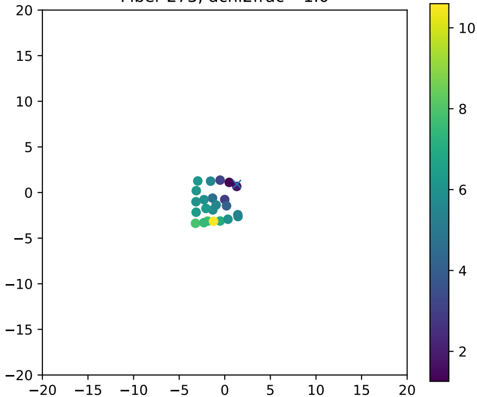
Fiber 273, dchi2frac= 1.0
