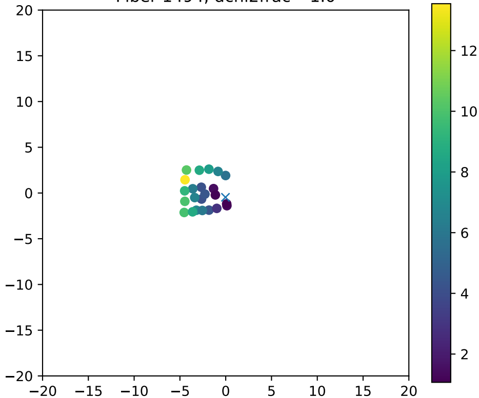
Fiber 1494, dchi2frac= 1.0
