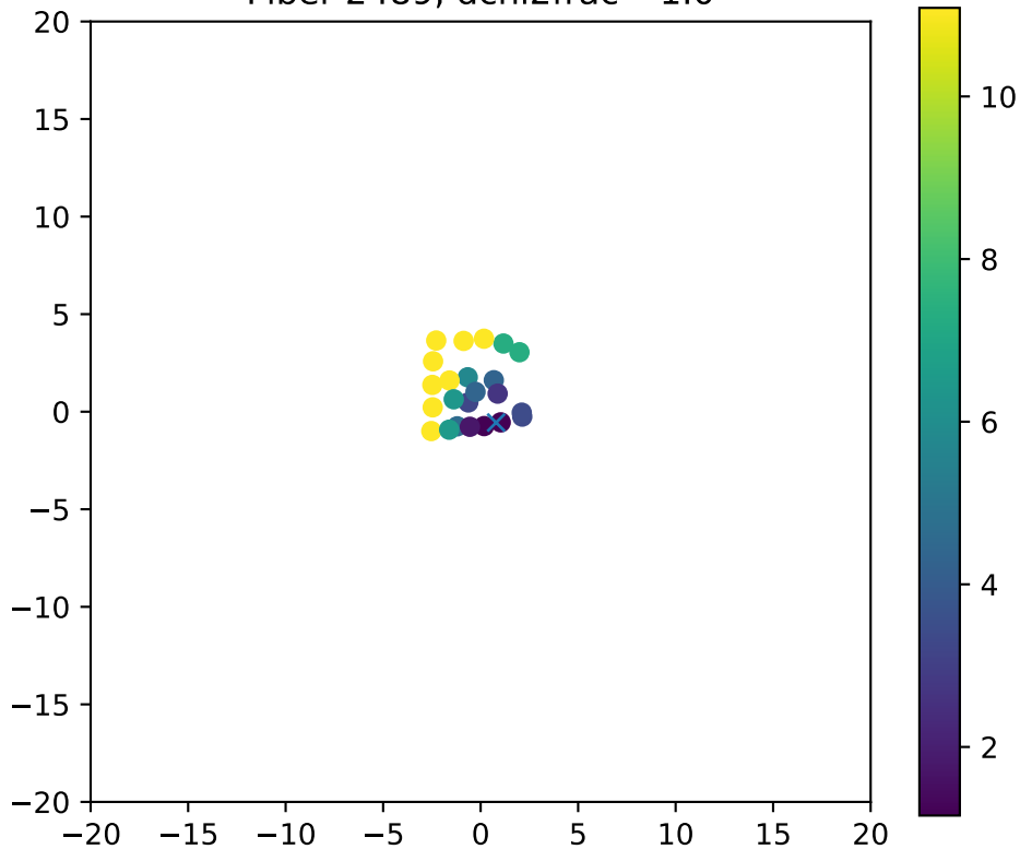
Fiber 2489, dchi2frac= 1.0
