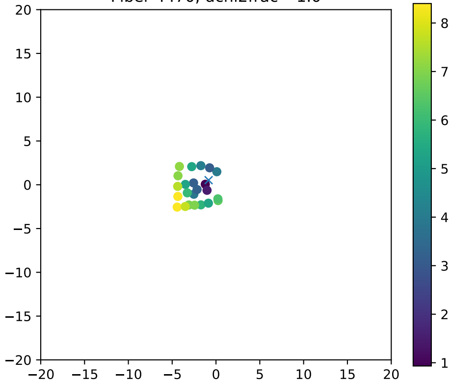
Fiber 4470, dchi2frac= 1.0
