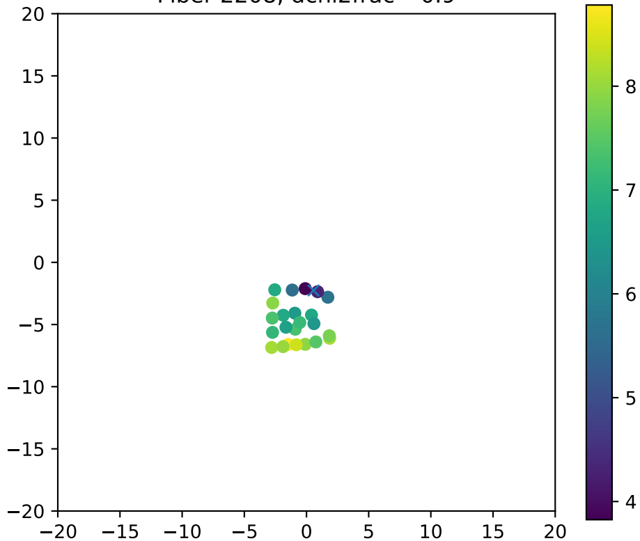
Fiber 2208, dchi2frac= 0.9
