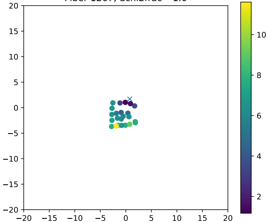
Fiber 1267, dchi2frac= 1.0
