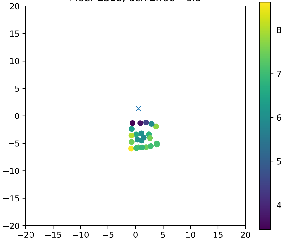
Fiber 2328, dchi2frac= 0.9
