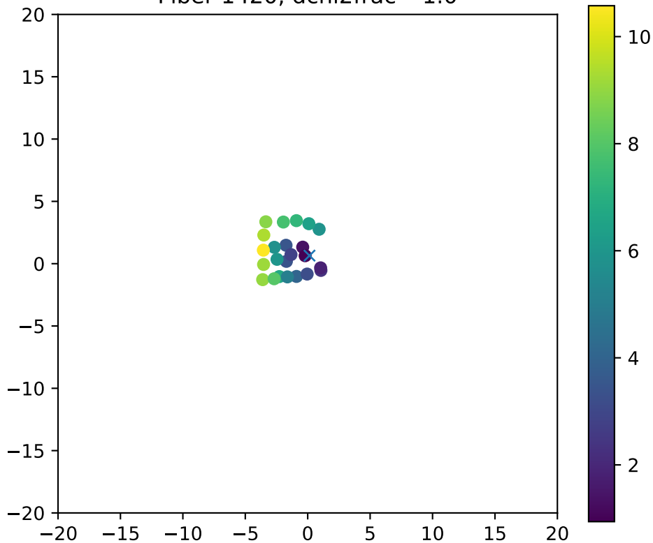
Fiber 1420, dchi2frac= 1.0
