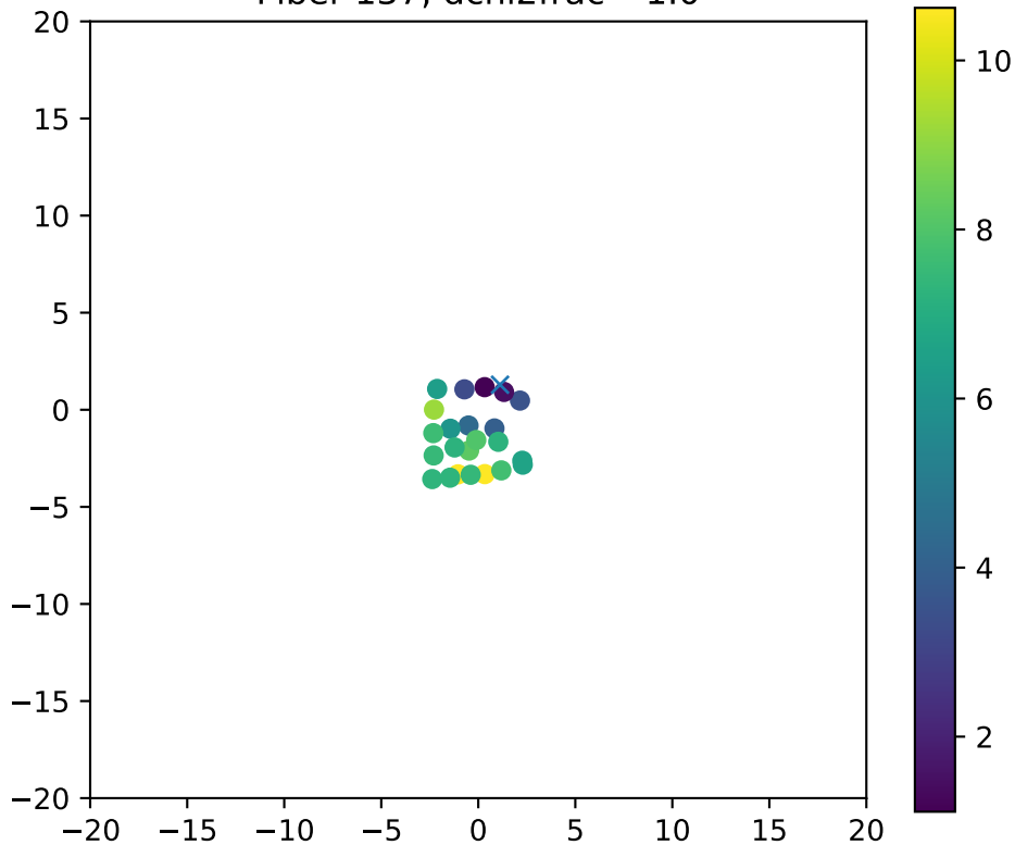
Fiber 137, dchi2frac= 1.0
