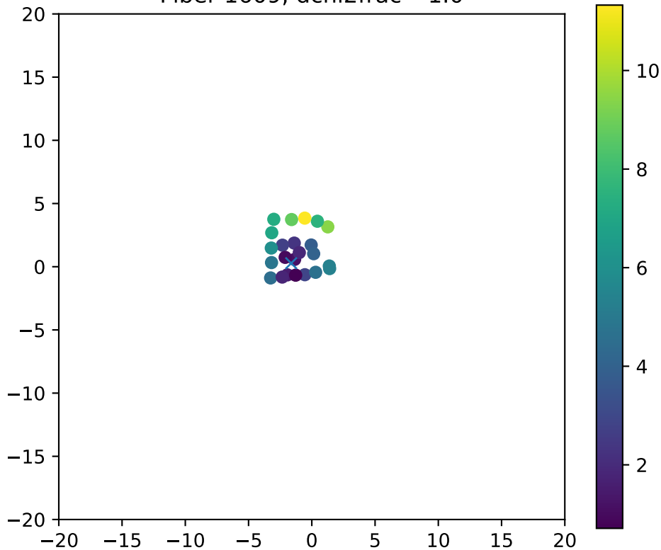
Fiber 1609, dchi2frac= 1.0
