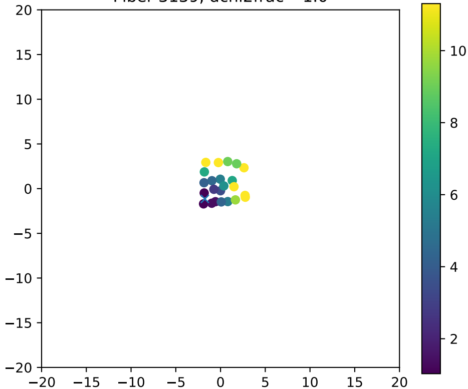
Fiber 3139, dchi2frac= 1.0
