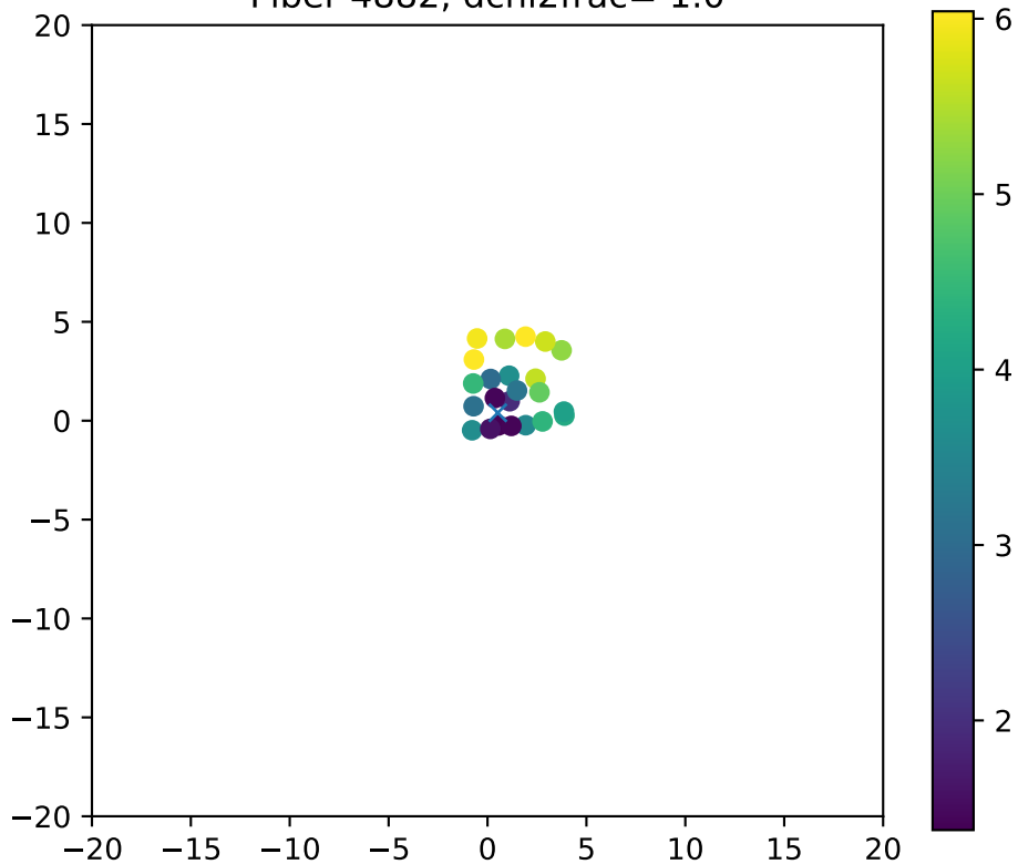
Fiber 4882, dchi2frac= 1.0
