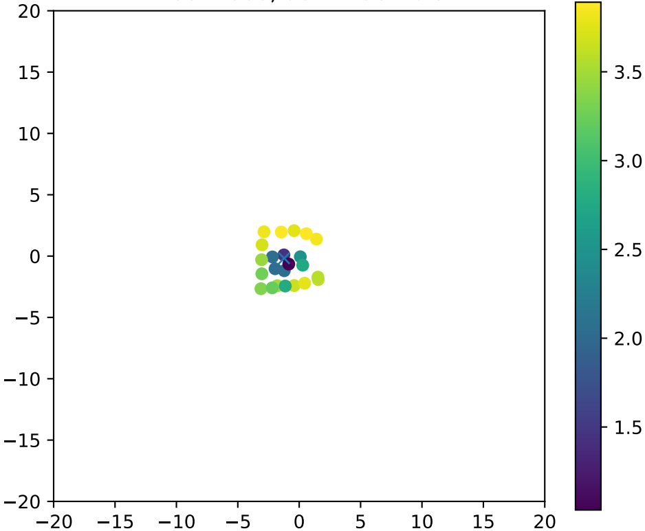
Fiber 1068, dchi2frac= 0.9
