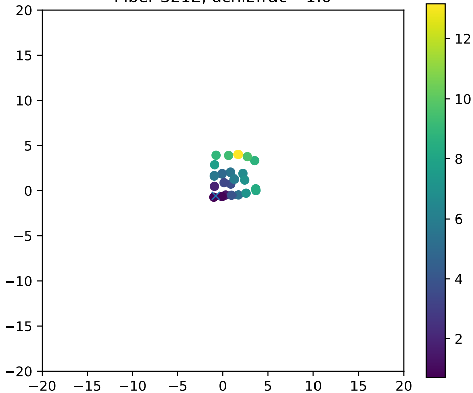
Fiber 3212, dchi2frac= 1.0
