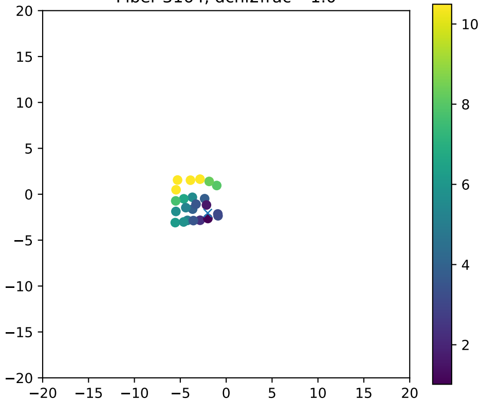
Fiber 3164, dchi2frac= 1.0
