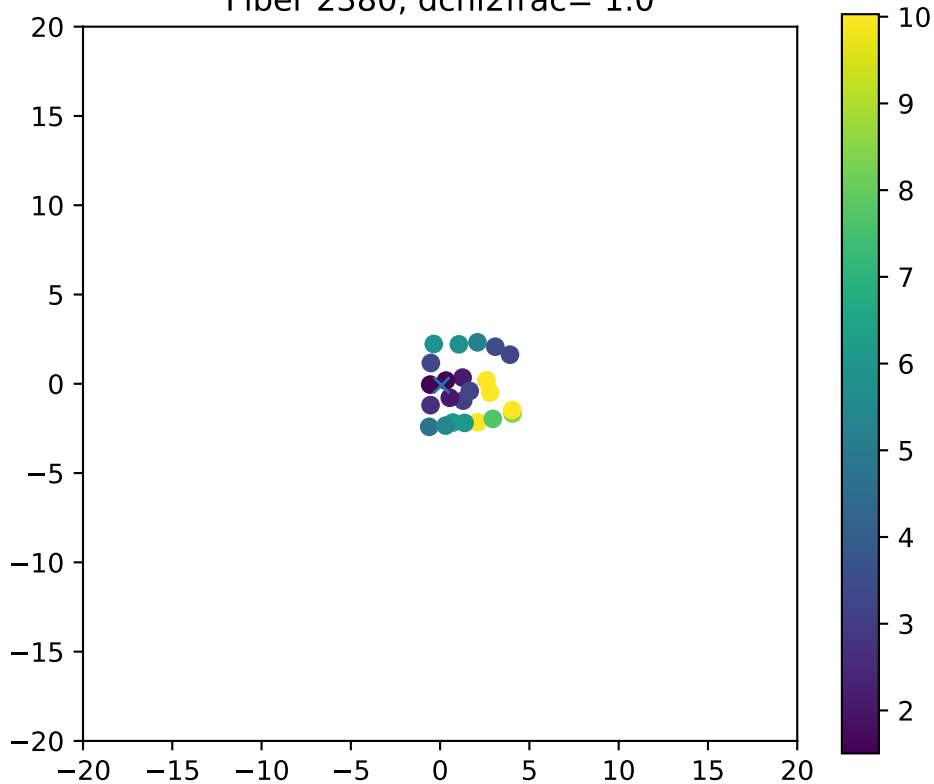
Fiber 2380, dchi2frac= 1.0
