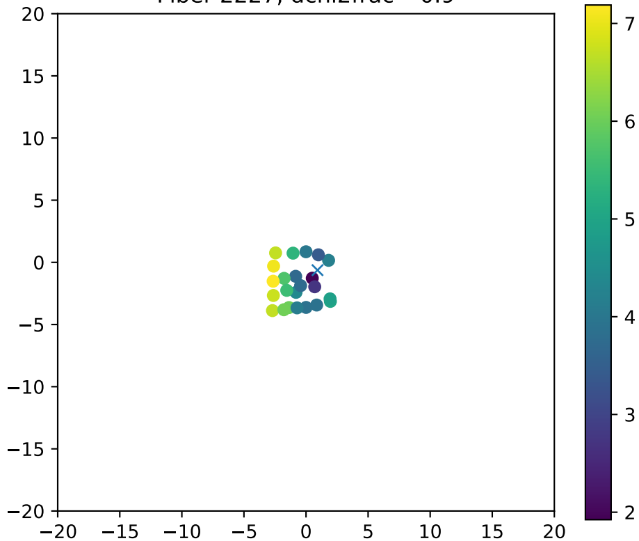
Fiber 2227, dchi2frac= 0.9
