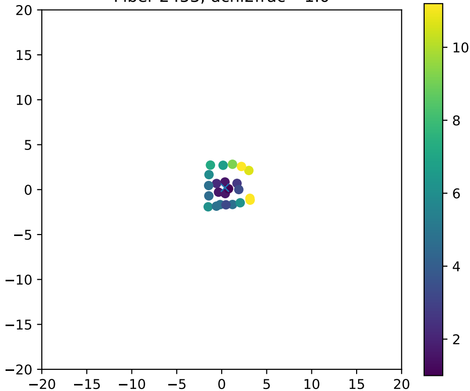
Fiber 2453, dchi2frac= 1.0
