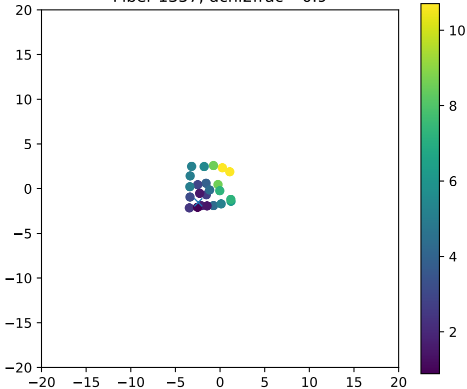
Fiber 1357, dchi2frac= 0.9
