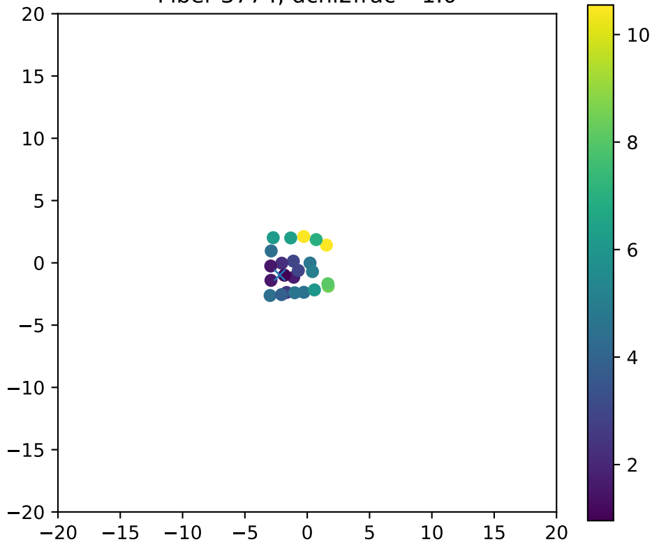
Fiber 3774, dchi2frac= 1.0
