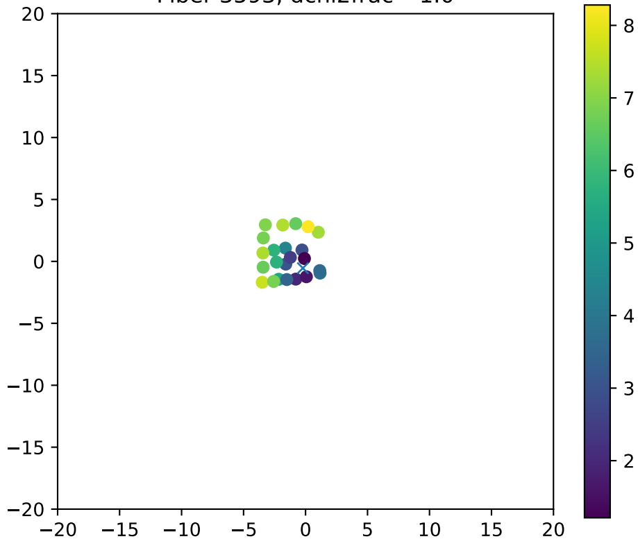
Fiber 3593, dchi2frac= 1.0
