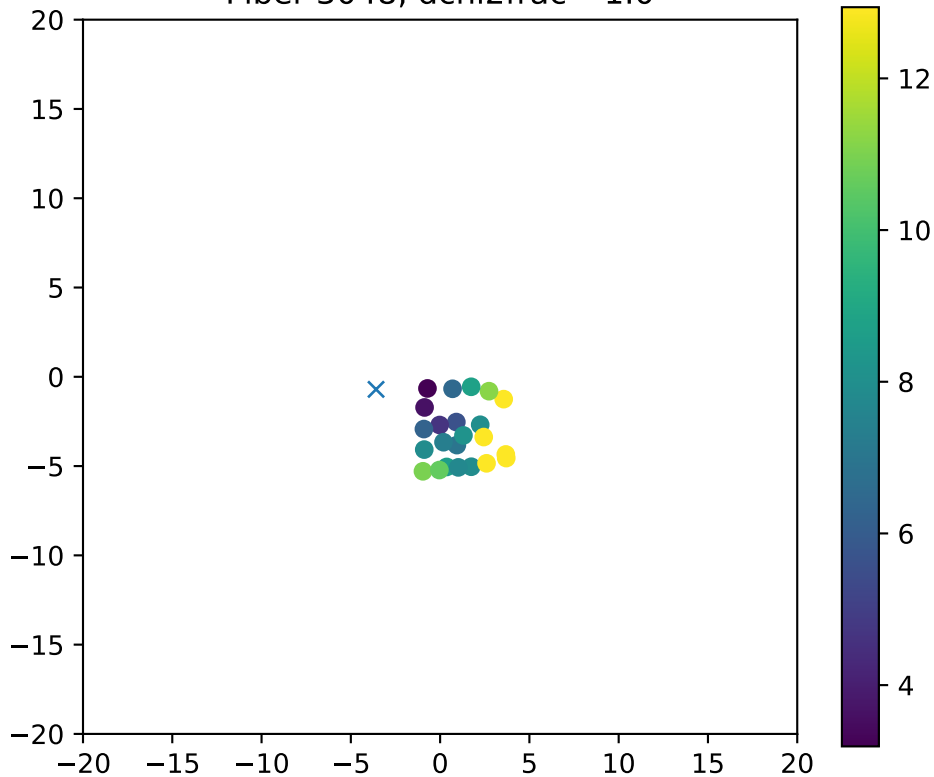
Fiber 3048, dchi2frac= 1.0
