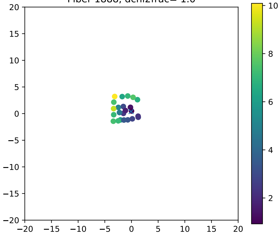
Fiber 1888, dchi2frac= 1.0
