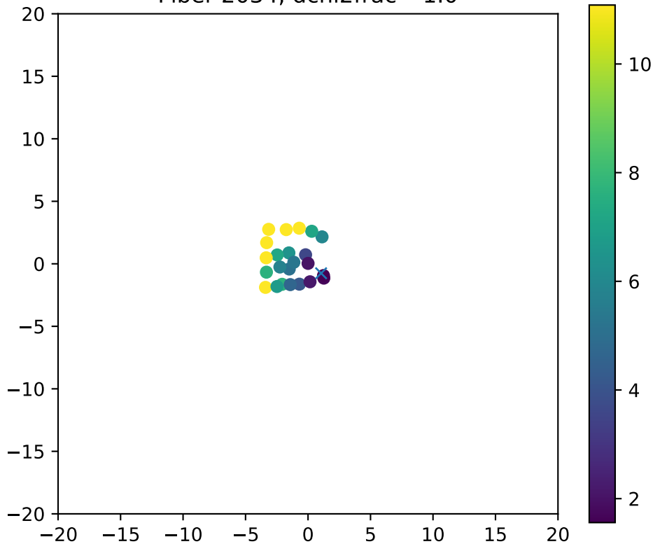
Fiber 2034, dchi2frac= 1.0
