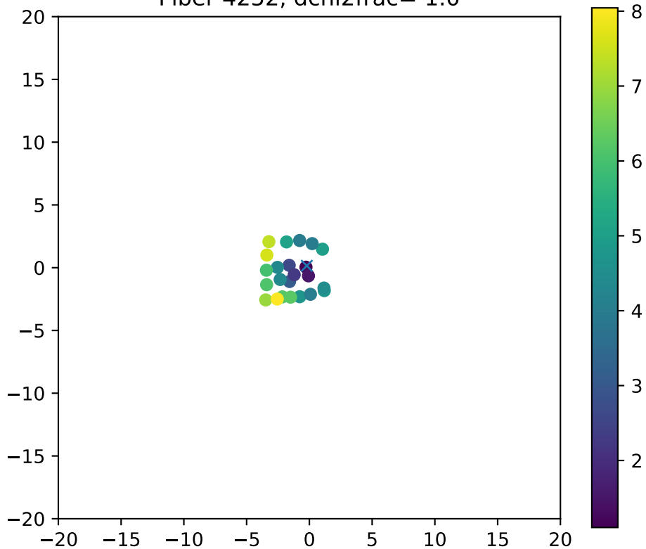
Fiber 4252, dchi2frac= 1.0
