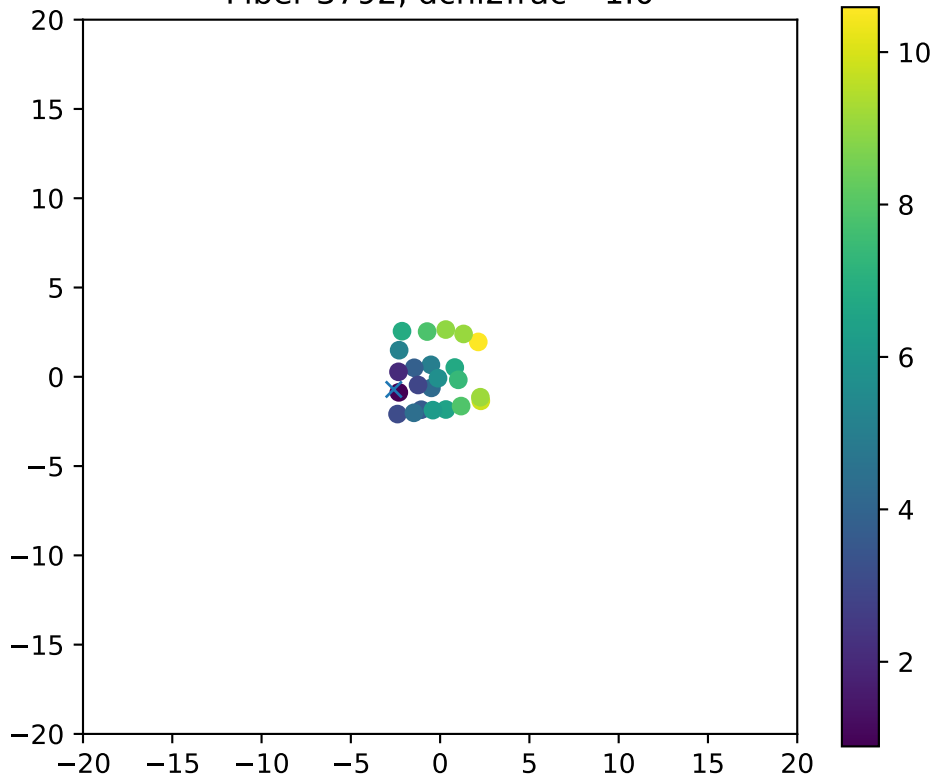
Fiber 3792, dchi2frac= 1.0
