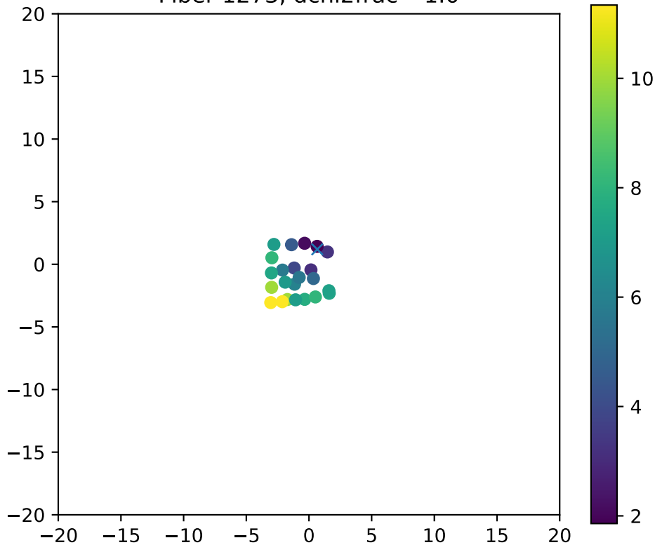
Fiber 1273, dchi2frac= 1.0
