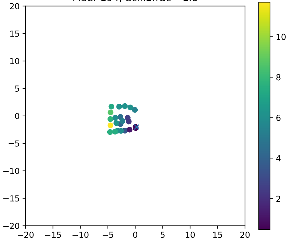
Fiber 194, dchi2frac= 1.0
