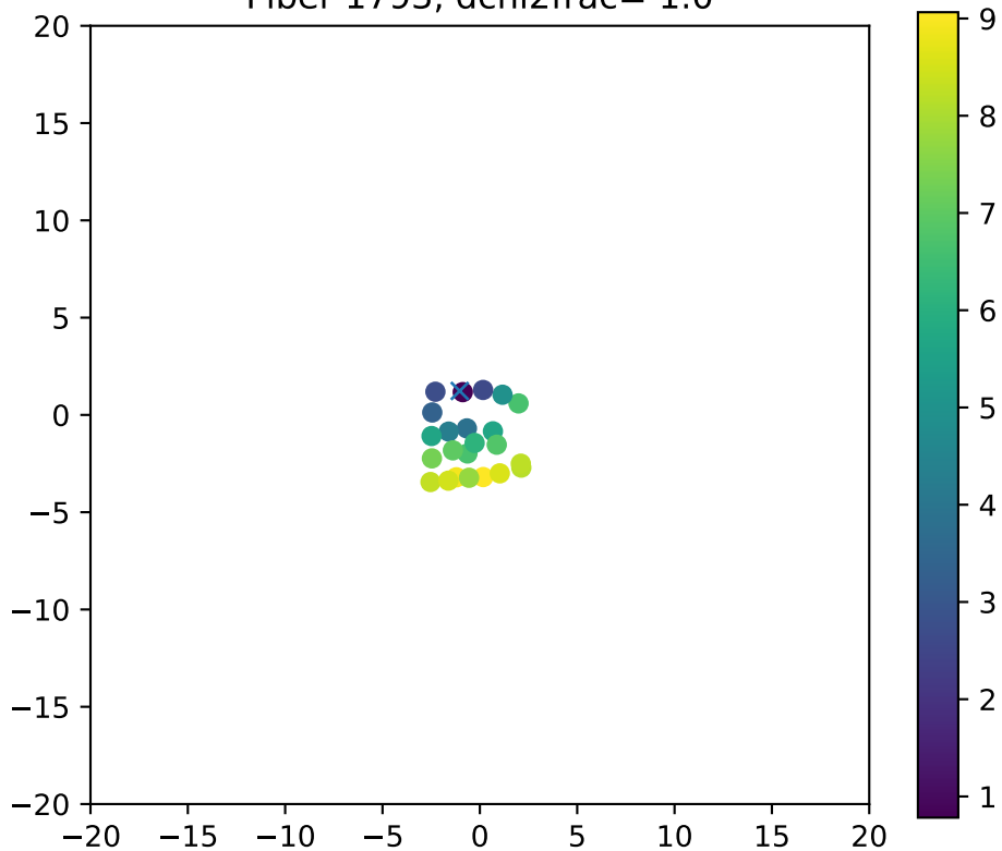
Fiber 1793, dchi2frac= 1.0
