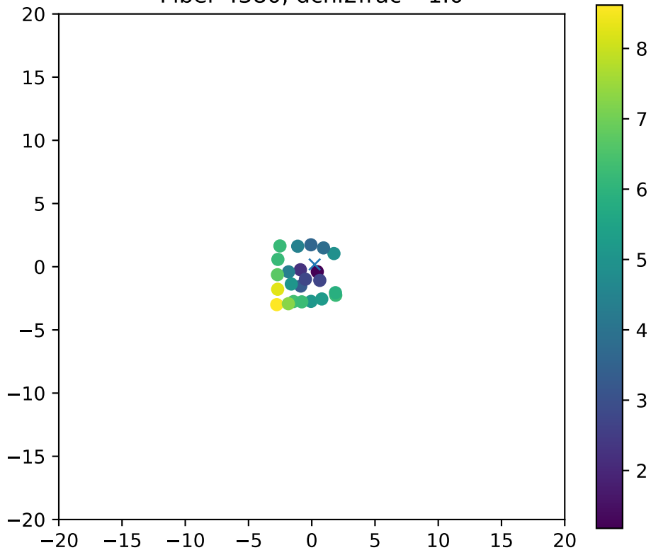
Fiber 4380, dchi2frac= 1.0
