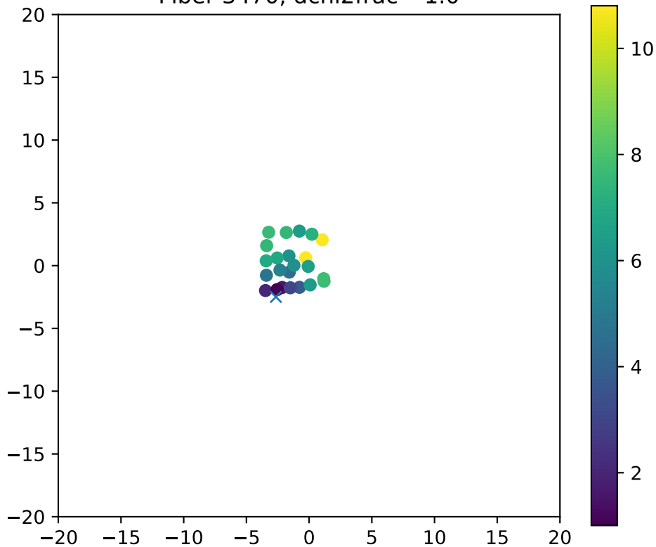
Fiber 3470, dchi2frac= 1.0
