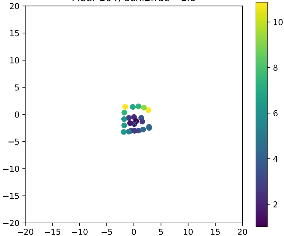
Fiber 164, dchi2frac= 1.0
