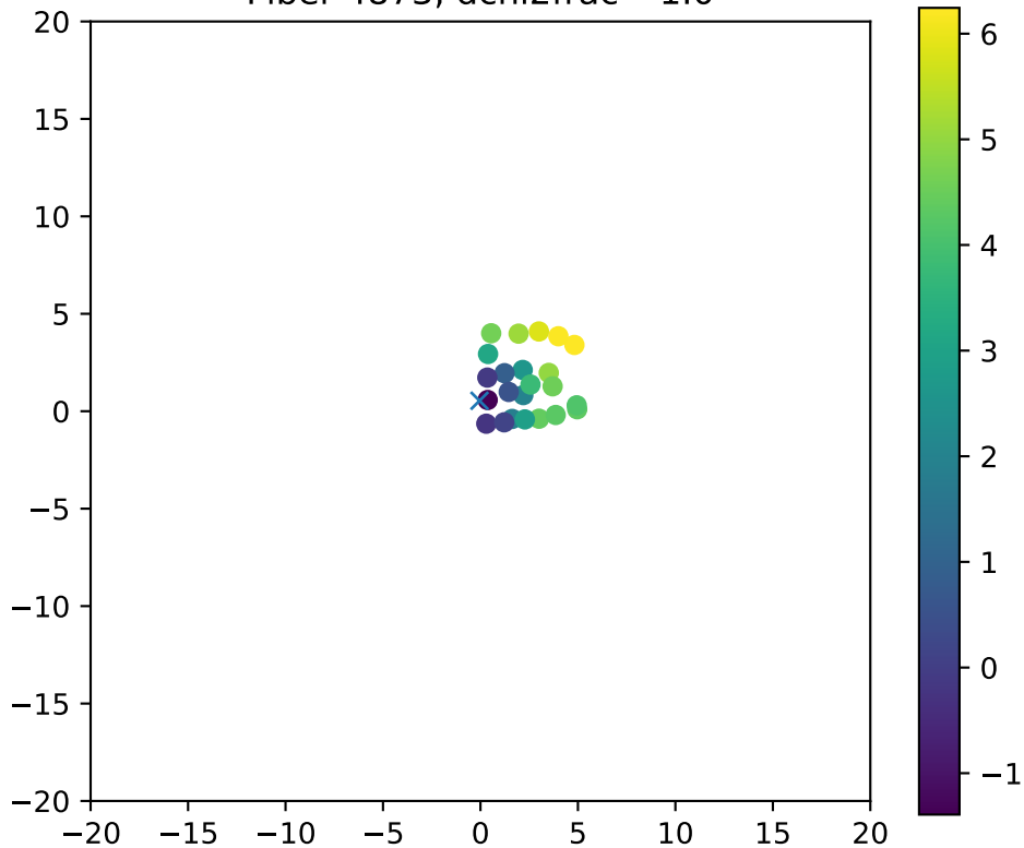
Fiber 4873, dchi2frac= 1.0
