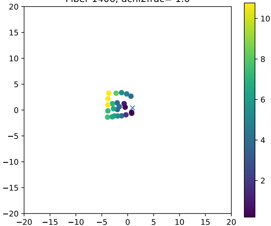
Fiber 1406, dchi2frac= 1.0
