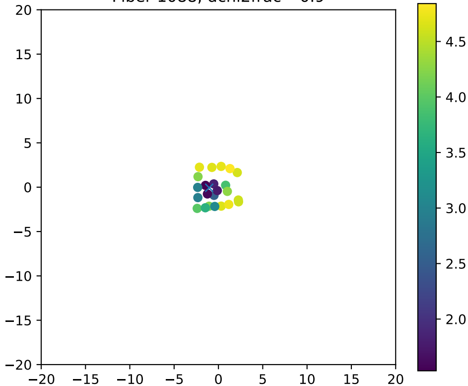
Fiber 1088, dchi2frac= 0.9
