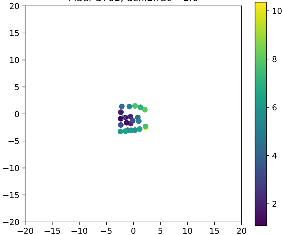
Fiber 3762, dchi2frac= 1.0
