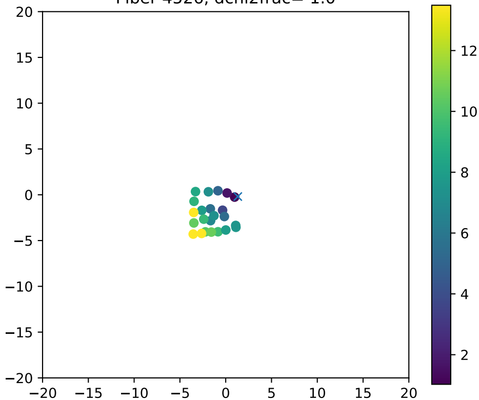
Fiber 4526, dchi2frac= 1.0
