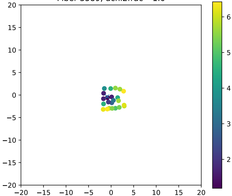
Fiber 3589, dchi2frac= 1.0
