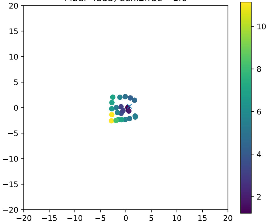
Fiber 4833, dchi2frac= 1.0
