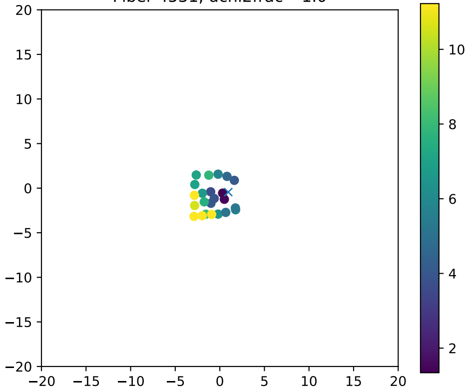
Fiber 4531, dchi2frac= 1.0
