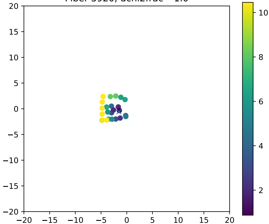
Fiber 3920, dchi2frac= 1.0
