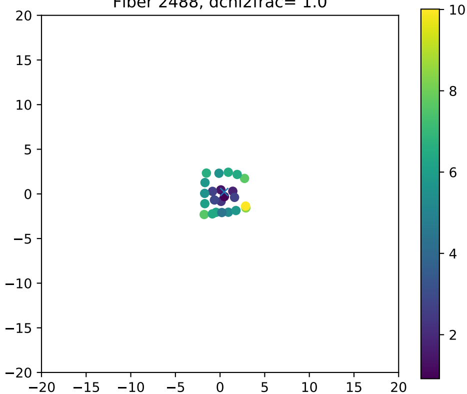
Fiber 2488, dchi2frac= 1.0
