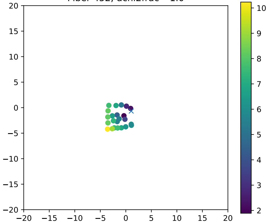
Fiber 452, dchi2frac= 1.0
