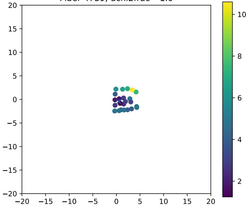
Fiber 4739, dchi2frac= 1.0
