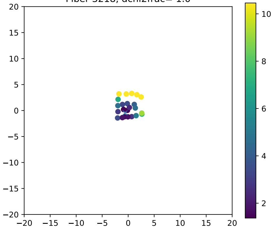
Fiber 3218, dchi2frac= 1.0
