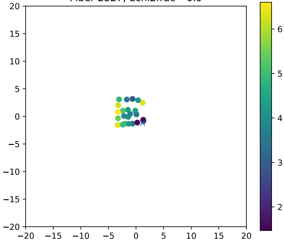
Fiber 2327, dchi2frac= 0.9
