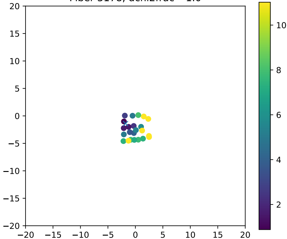
Fiber 3178, dchi2frac= 1.0
