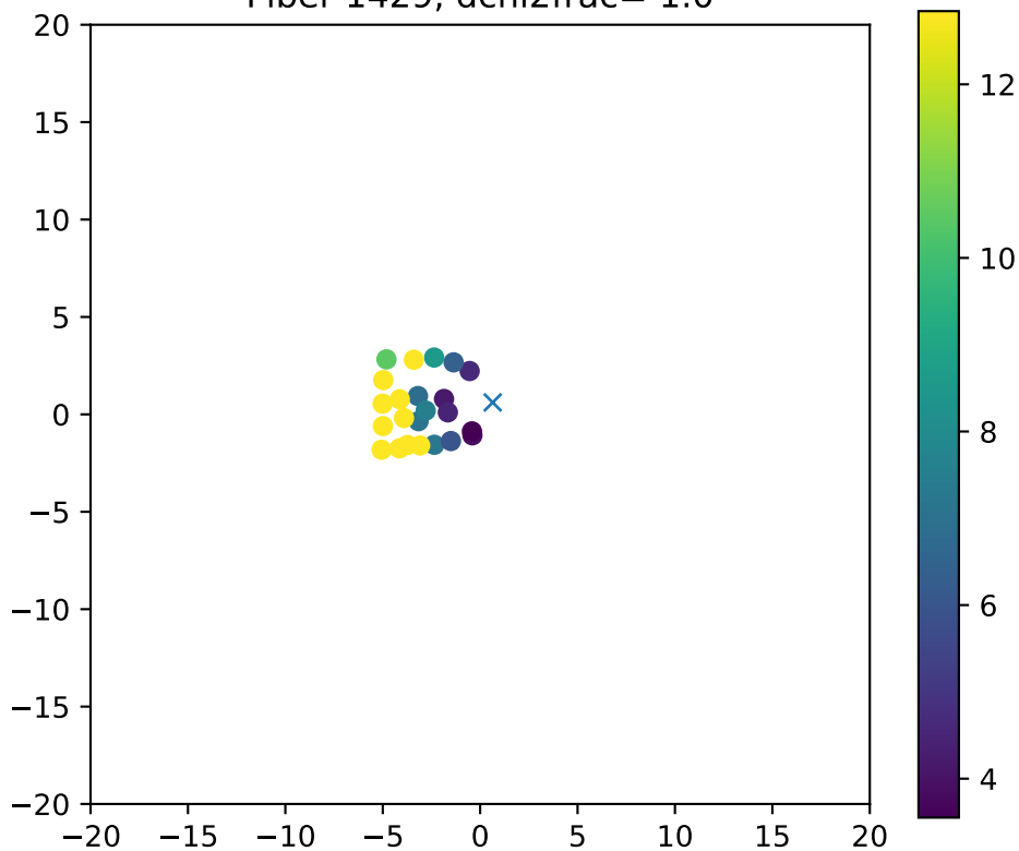
Fiber 1429, dchi2frac= 1.0
