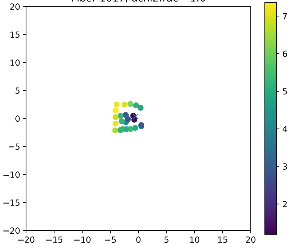
Fiber 1617, dchi2frac= 1.0
