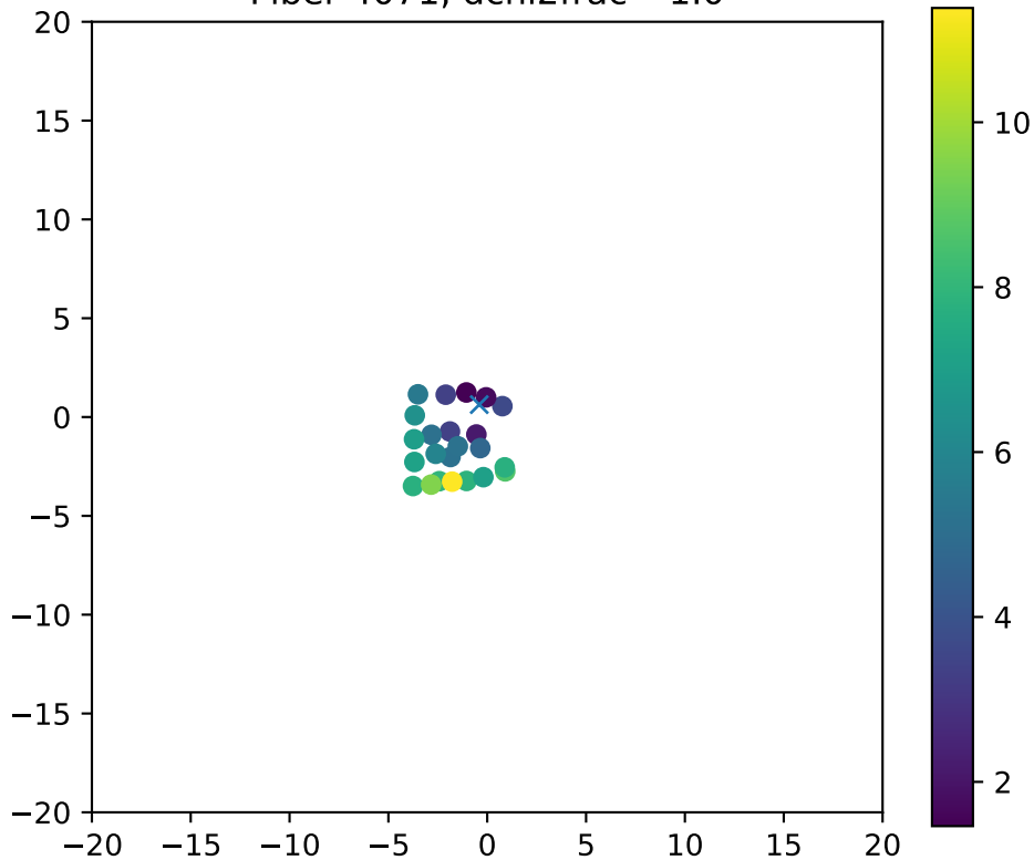
Fiber 4071, dchi2frac= 1.0
