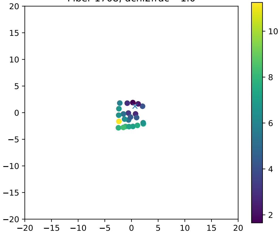
Fiber 1708, dchi2frac= 1.0
