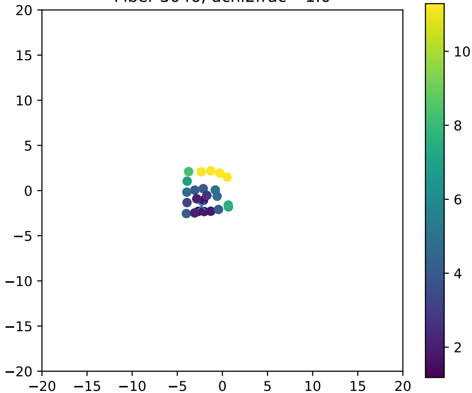
Fiber 3046, dchi2frac= 1.0
