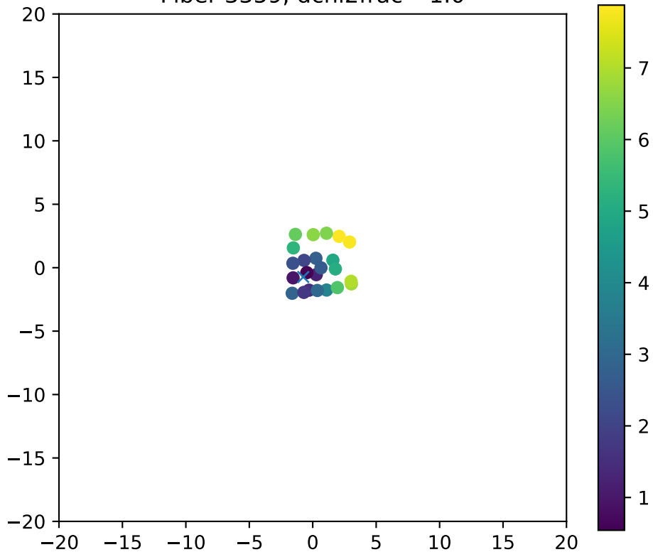
Fiber 3359, dchi2frac= 1.0
