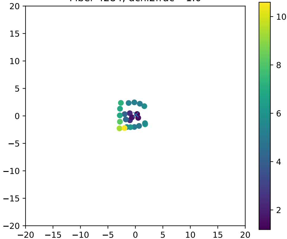
Fiber 4284, dchi2frac= 1.0
