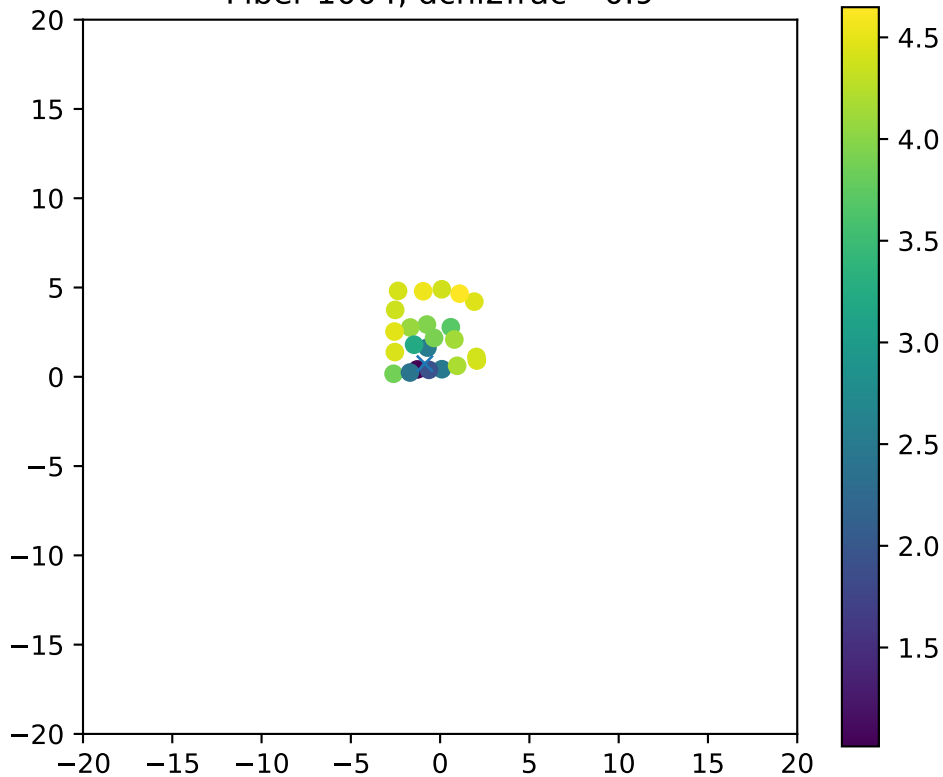
Fiber 1004, dchi2frac= 0.9
