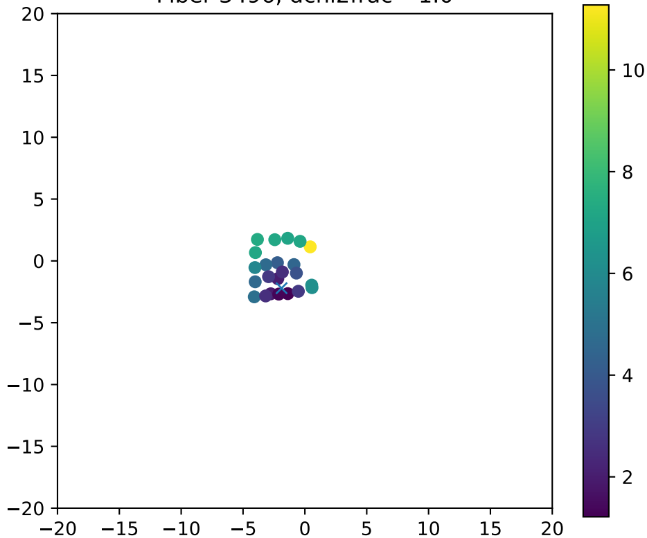
Fiber 3496, dchi2frac= 1.0
