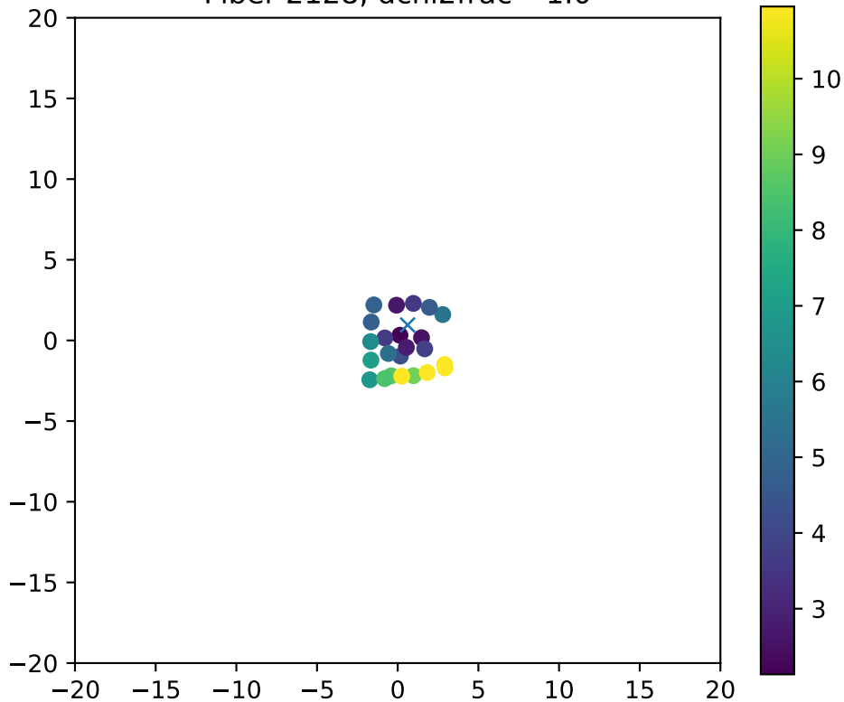
Fiber 2128, dchi2frac= 1.0
