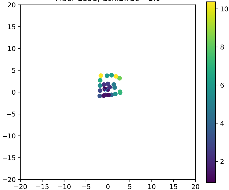
Fiber 1898, dchi2frac= 1.0
