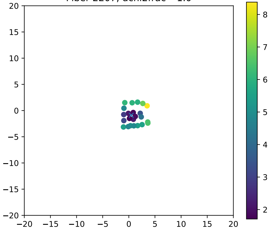
Fiber 2207, dchi2frac= 1.0
