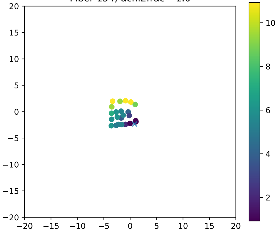
Fiber 154, dchi2frac= 1.0
