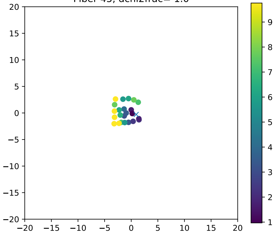
Fiber 45, dchi2frac= 1.0
