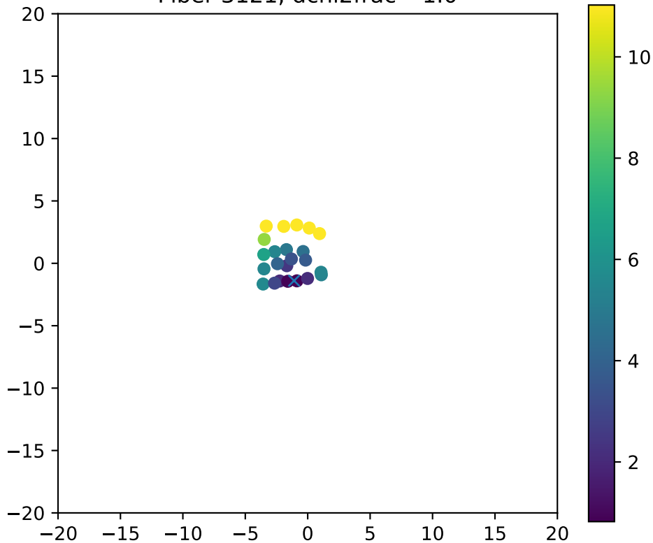
Fiber 3121, dchi2frac= 1.0
