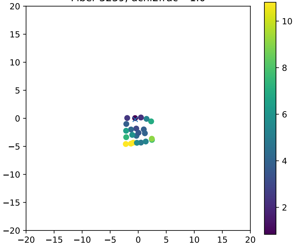
Fiber 3239, dchi2frac= 1.0
