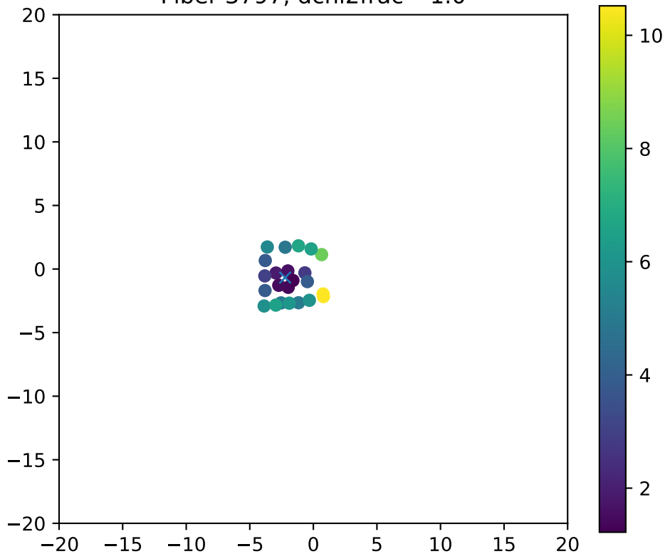
Fiber 3797, dchi2frac= 1.0
