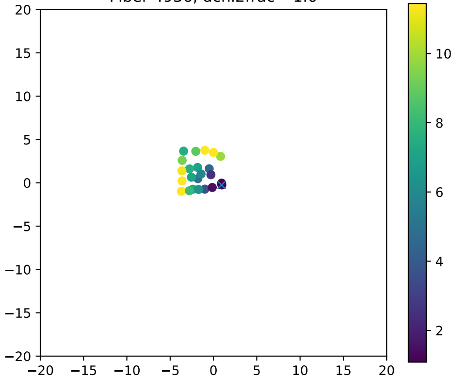
Fiber 4936, dchi2frac= 1.0
