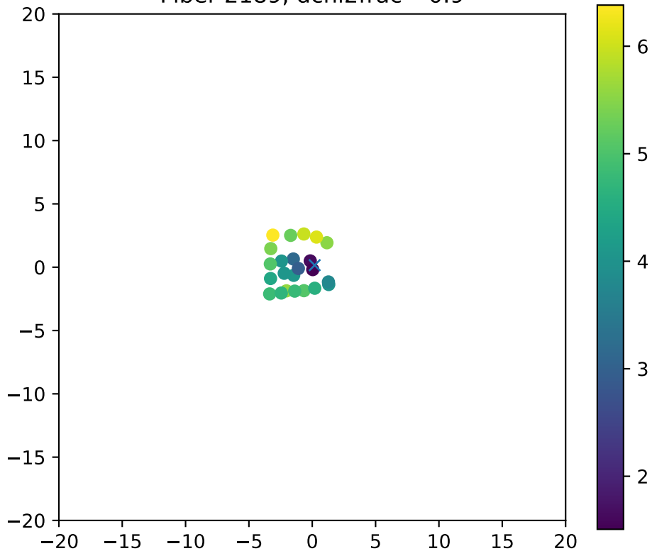
Fiber 2189, dchi2frac= 0.9
