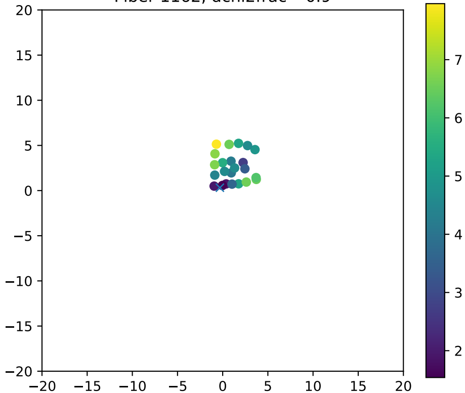
Fiber 1162, dchi2frac= 0.9
