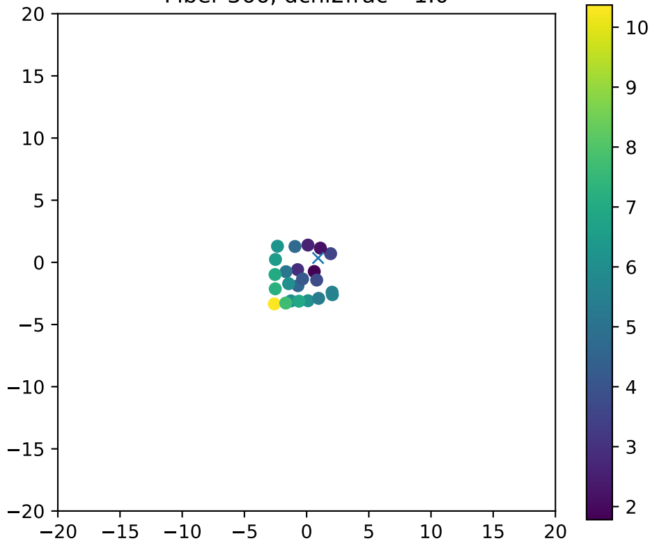
Fiber 366, dchi2frac= 1.0
