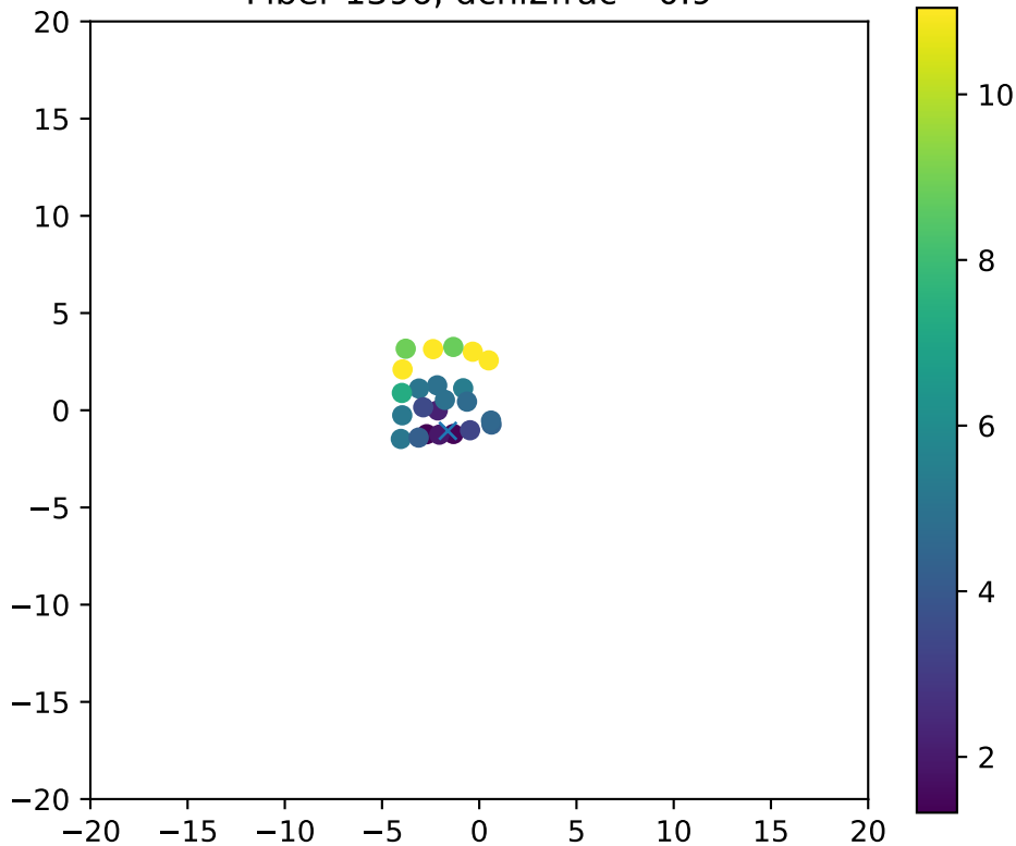
Fiber 1396, dchi2frac= 0.9
