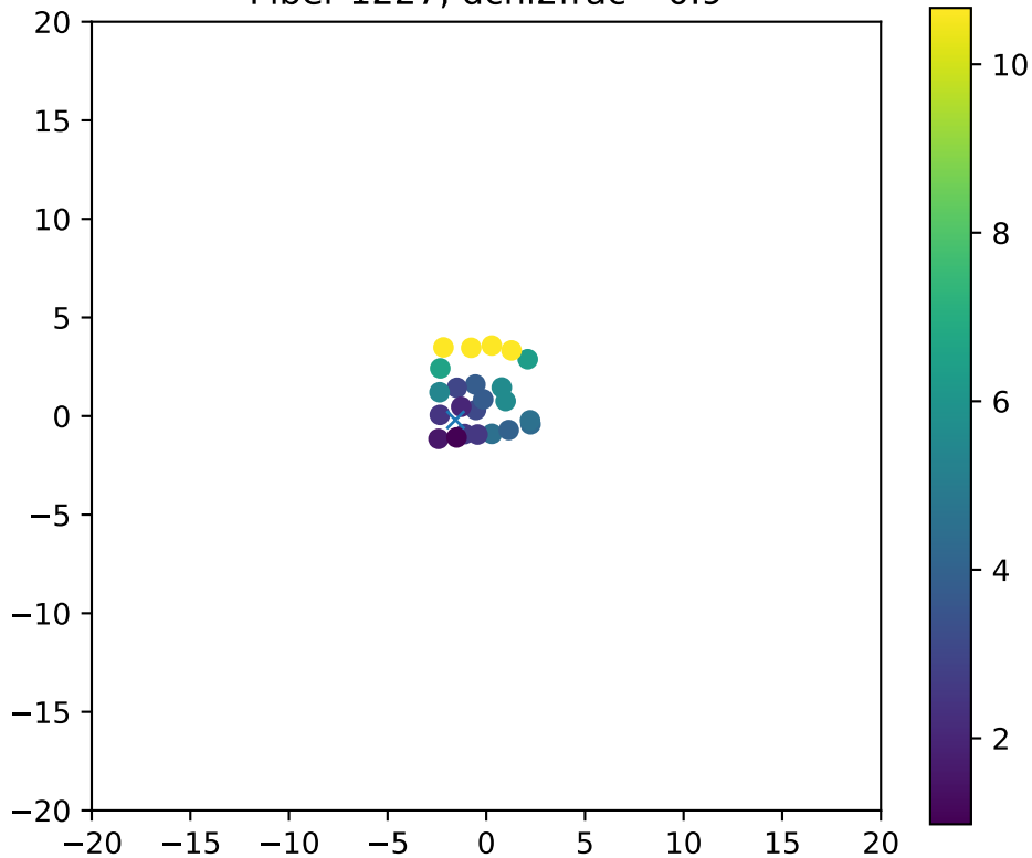
Fiber 1227, dchi2frac= 0.9
