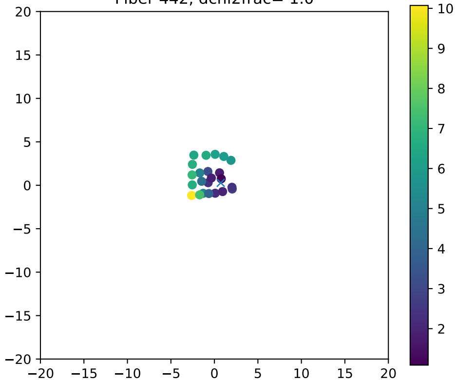
Fiber 442, dchi2frac= 1.0
