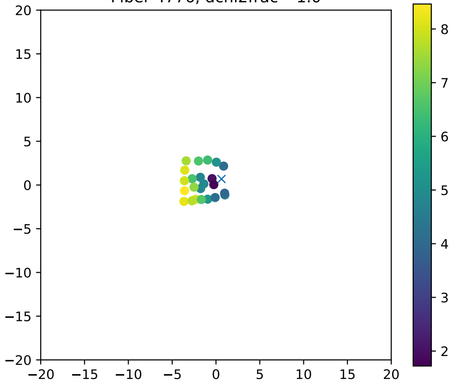
Fiber 4776, dchi2frac= 1.0
