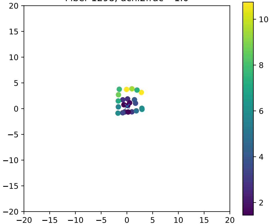
Fiber 1298, dchi2frac= 1.0
