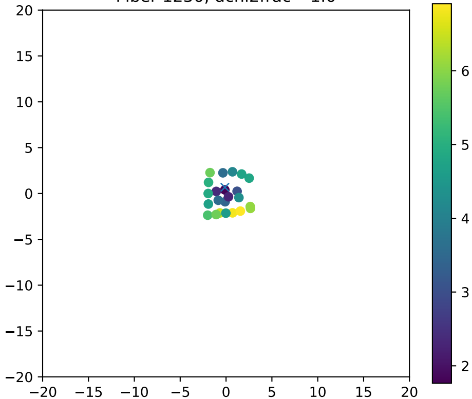
Fiber 1250, dchi2frac= 1.0
