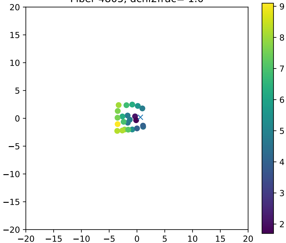
Fiber 4805, dchi2frac= 1.0
