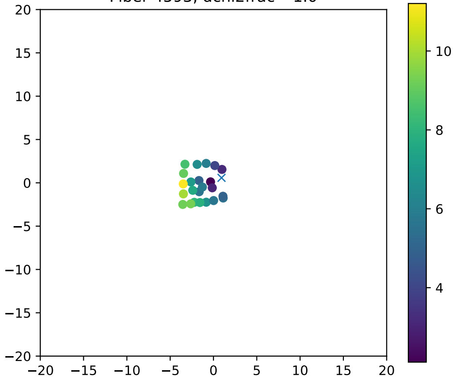
Fiber 4593, dchi2frac= 1.0
