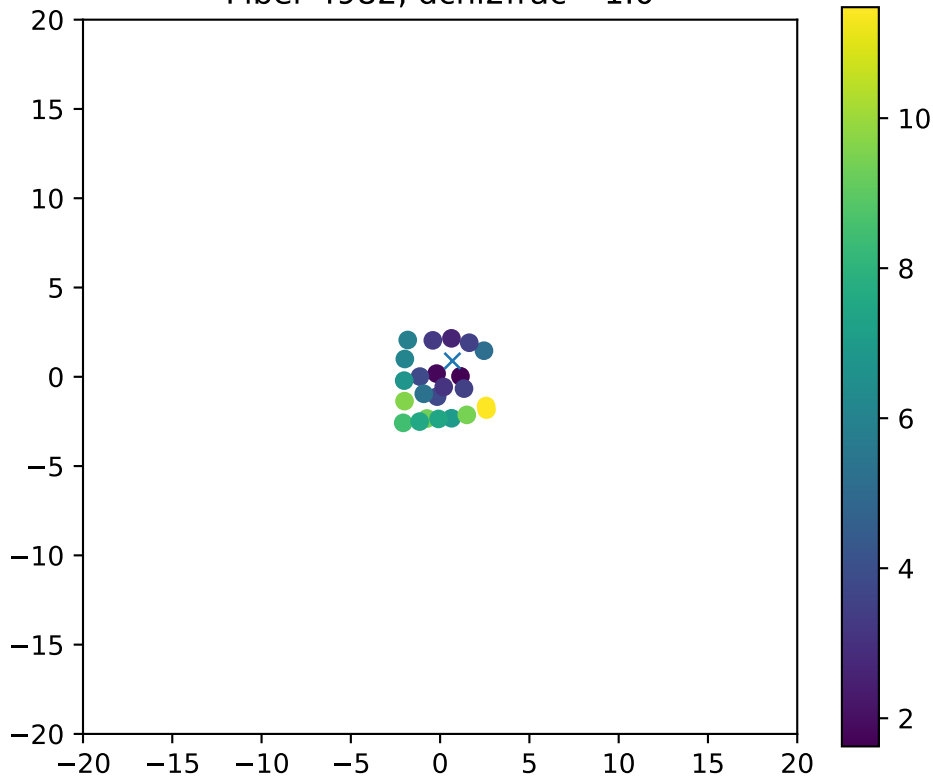
Fiber 4982, dchi2frac= 1.0
