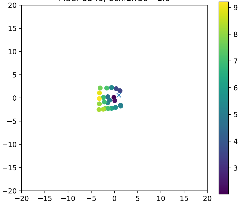
Fiber 3546, dchi2frac= 1.0
