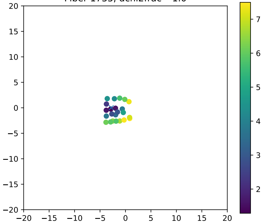
Fiber 1733, dchi2frac= 1.0
