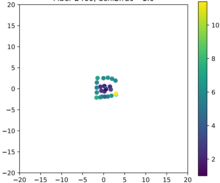
Fiber 2460, dchi2frac= 1.0
