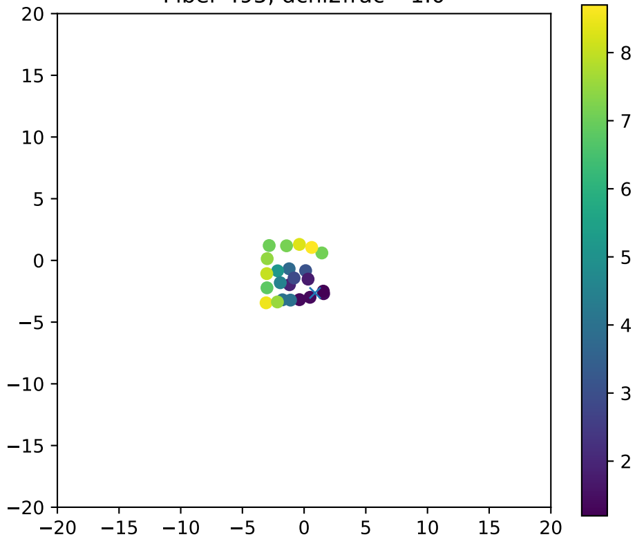
Fiber 495, dchi2frac= 1.0
