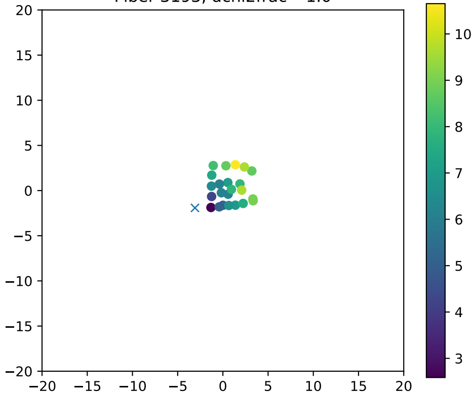
Fiber 3193, dchi2frac= 1.0
