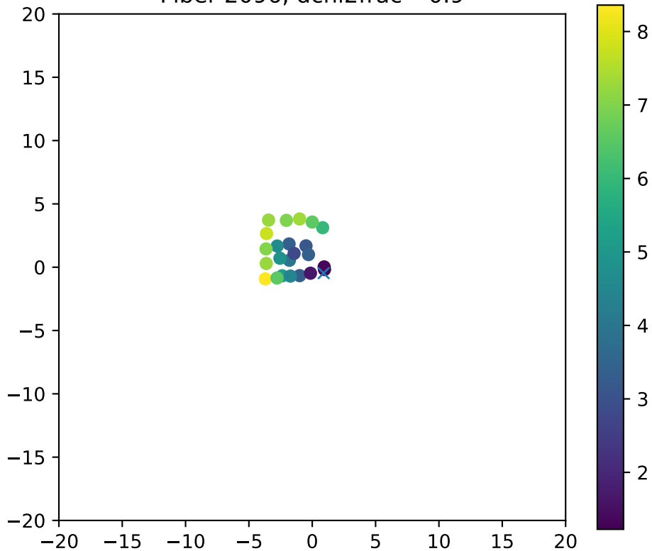
Fiber 2096, dchi2frac= 0.9
