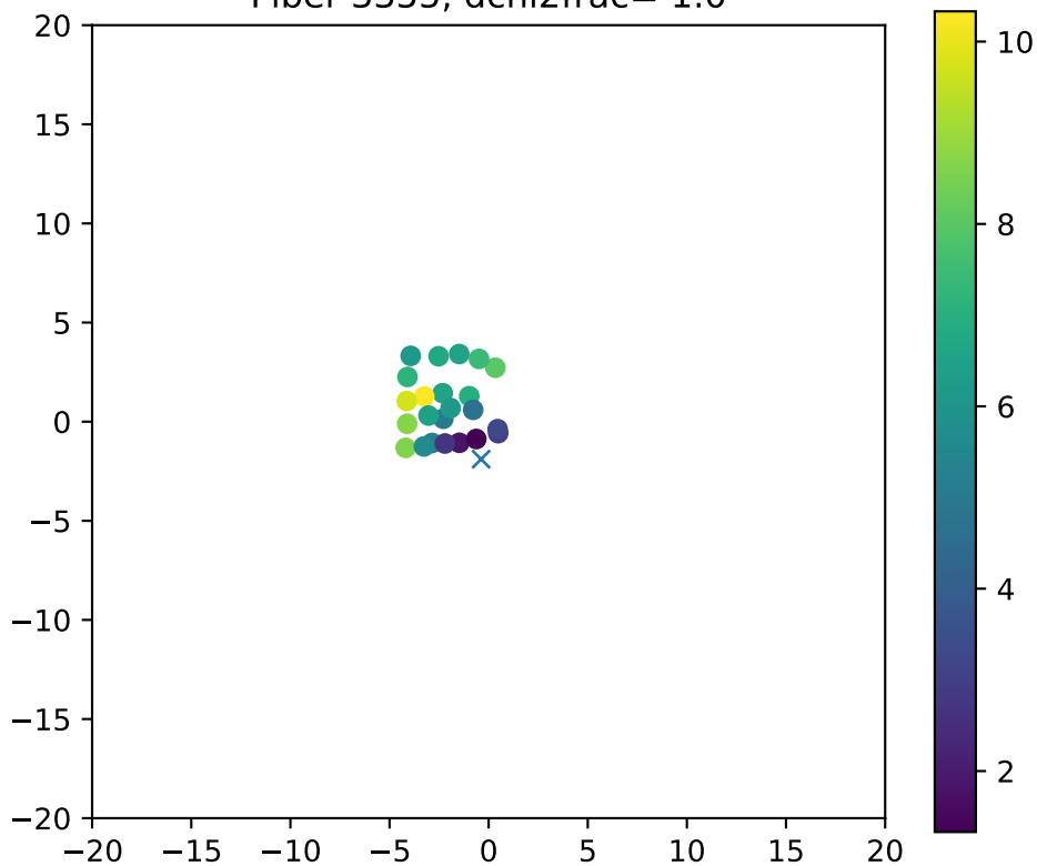
Fiber 3355, dchi2frac= 1.0
