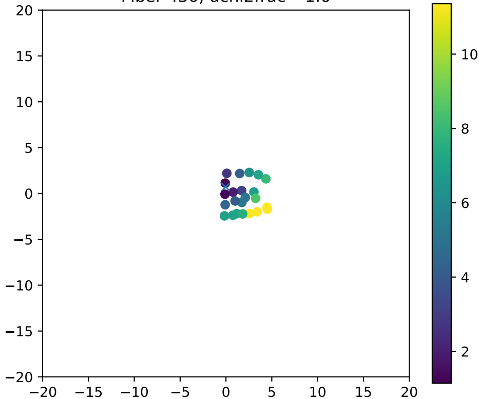
Fiber 430, dchi2frac= 1.0
