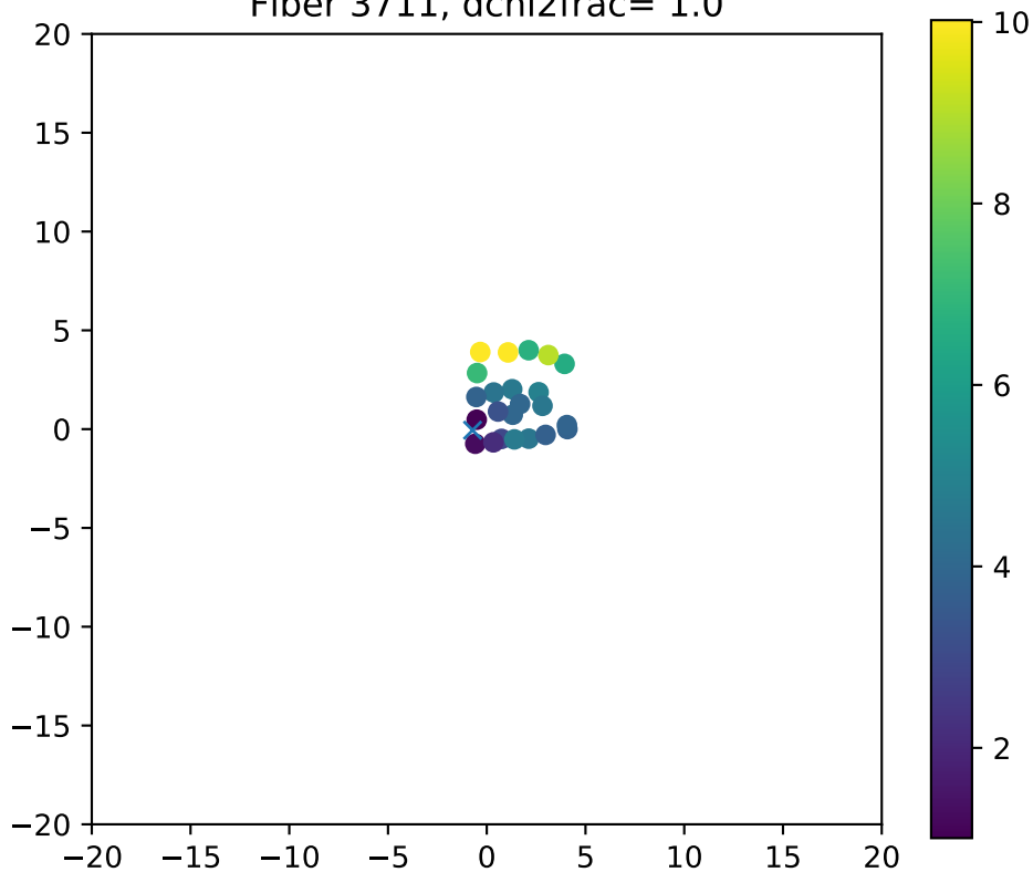
Fiber 3711, dchi2frac= 1.0
