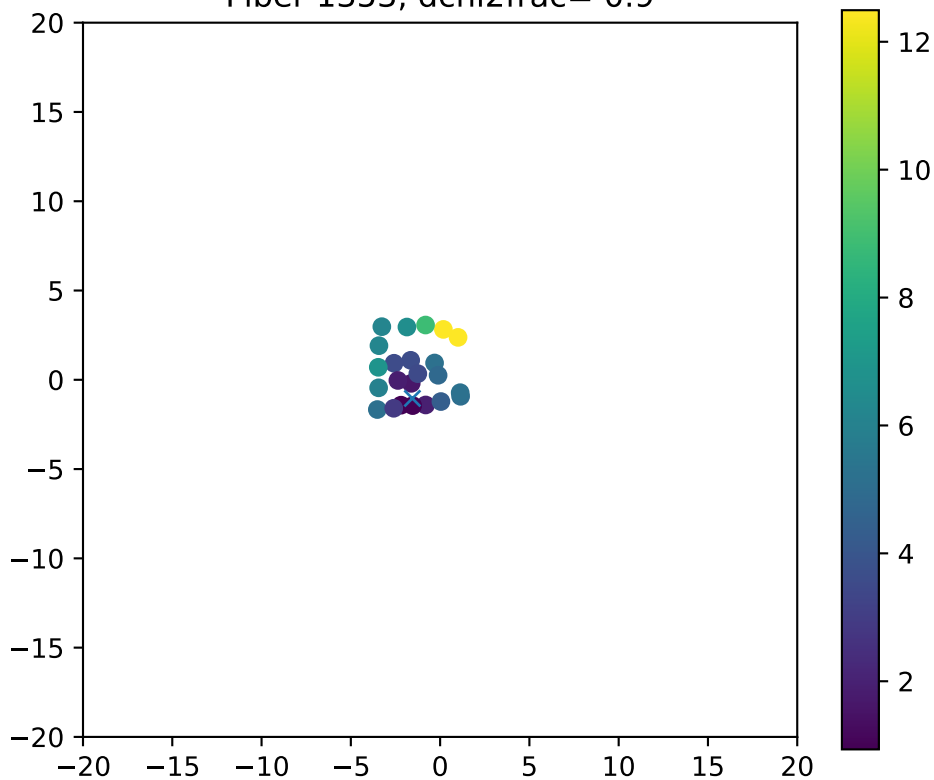
Fiber 1353, dchi2frac= 0.9
