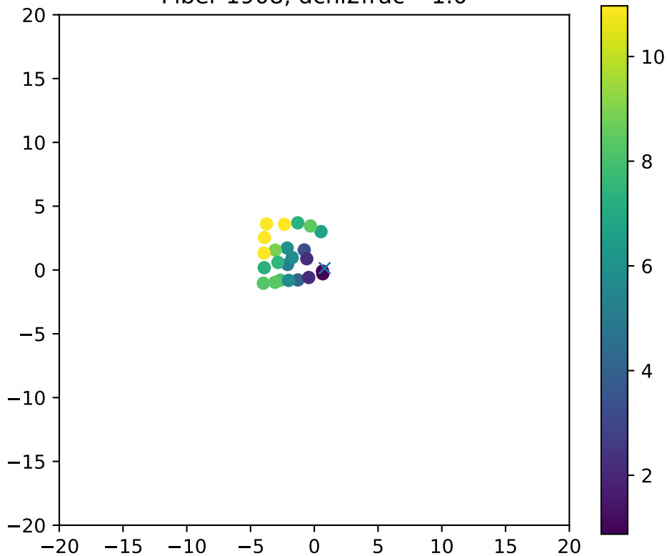
Fiber 1908, dchi2frac= 1.0
