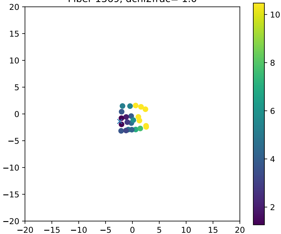
Fiber 1369, dchi2frac= 1.0
