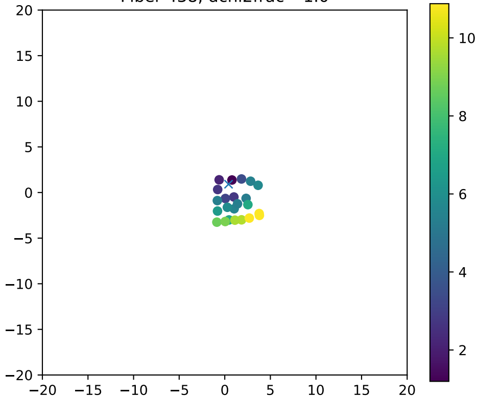
Fiber 438, dchi2frac= 1.0
