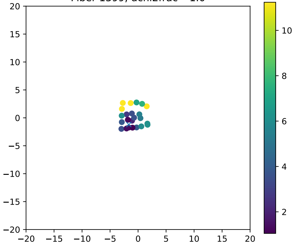
Fiber 1399, dchi2frac= 1.0
