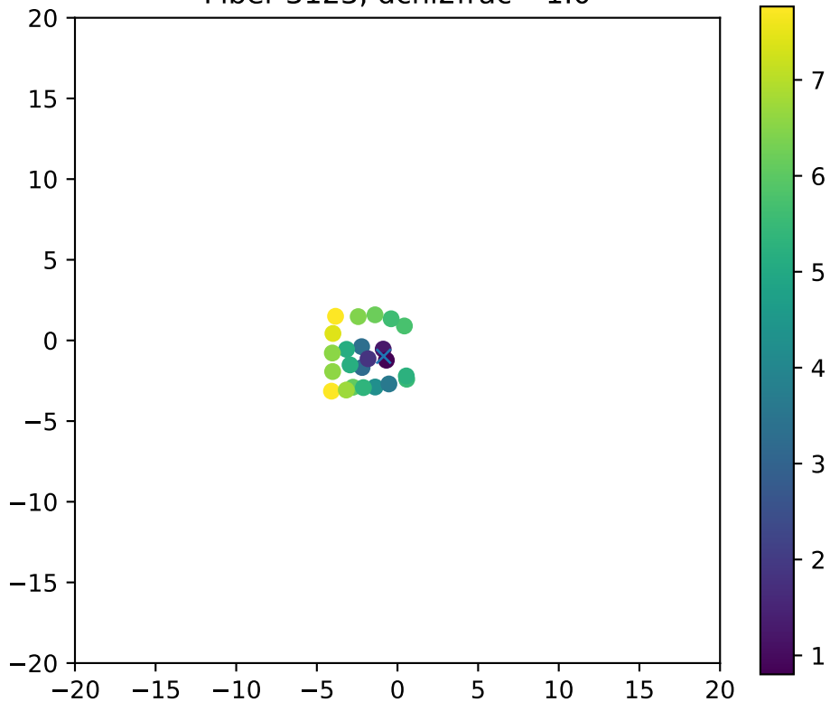
Fiber 3123, dchi2frac= 1.0
