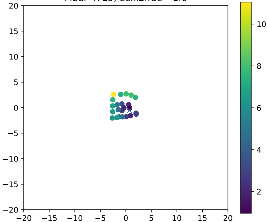
Fiber 4715, dchi2frac= 1.0
