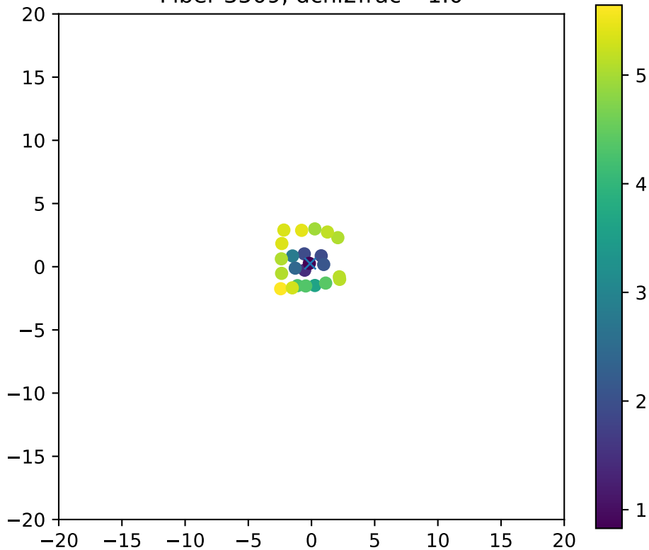
Fiber 3509, dchi2frac= 1.0
