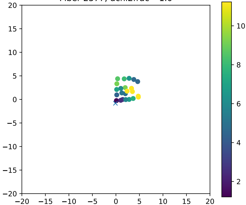
Fiber 2377, dchi2frac= 1.0
