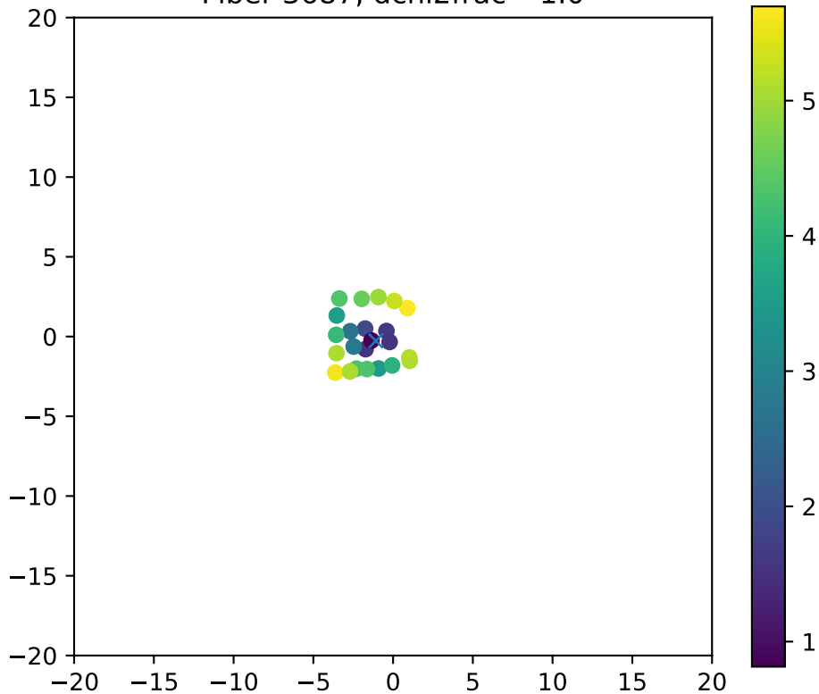
Fiber 3687, dchi2frac= 1.0
