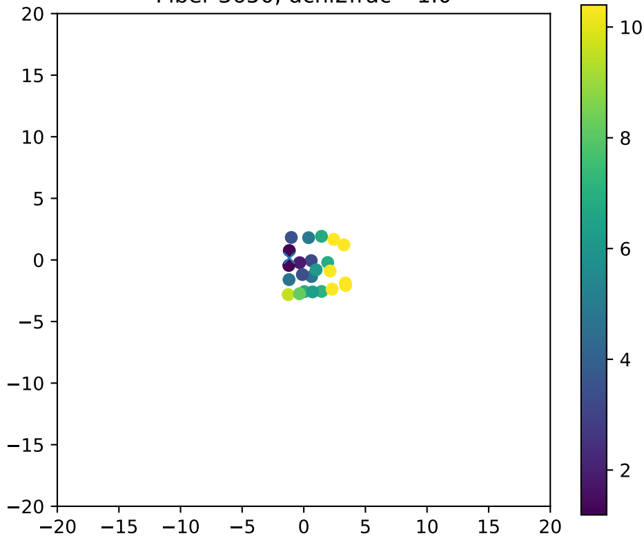
Fiber 3650, dchi2frac= 1.0
