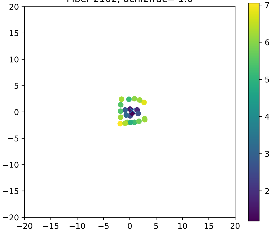
Fiber 2102, dchi2frac= 1.0
