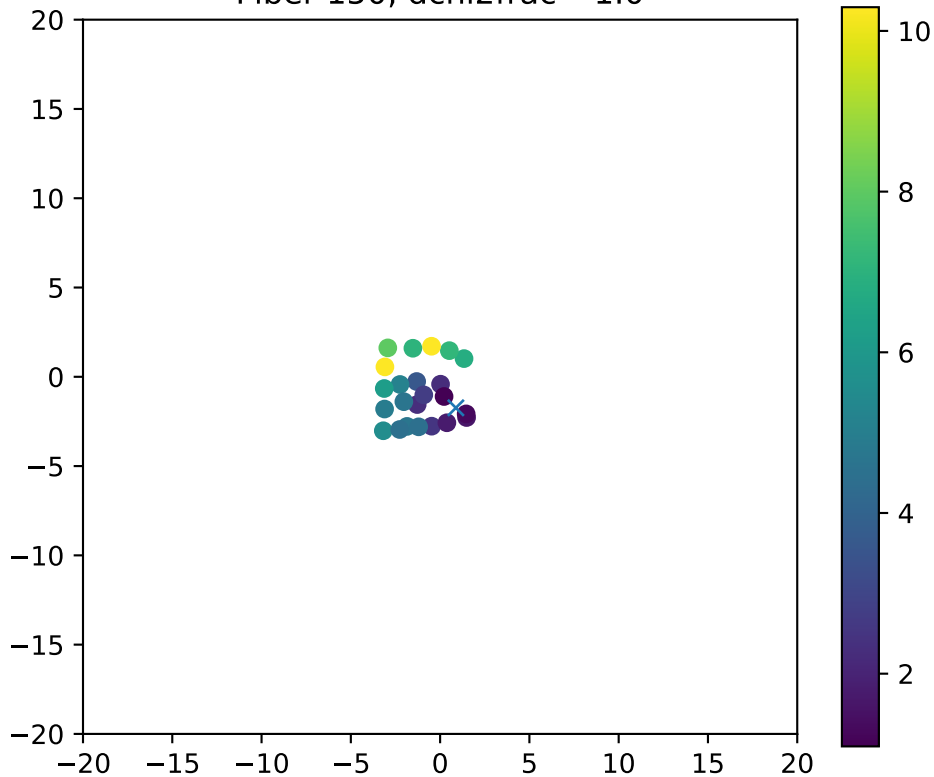
Fiber 150, dchi2frac= 1.0
