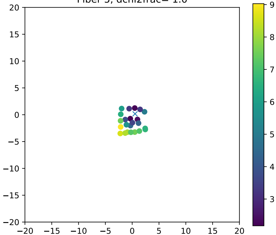
Fiber 5, dchi2frac= 1.0
