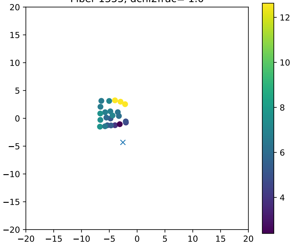
Fiber 1355, dchi2frac= 1.0
