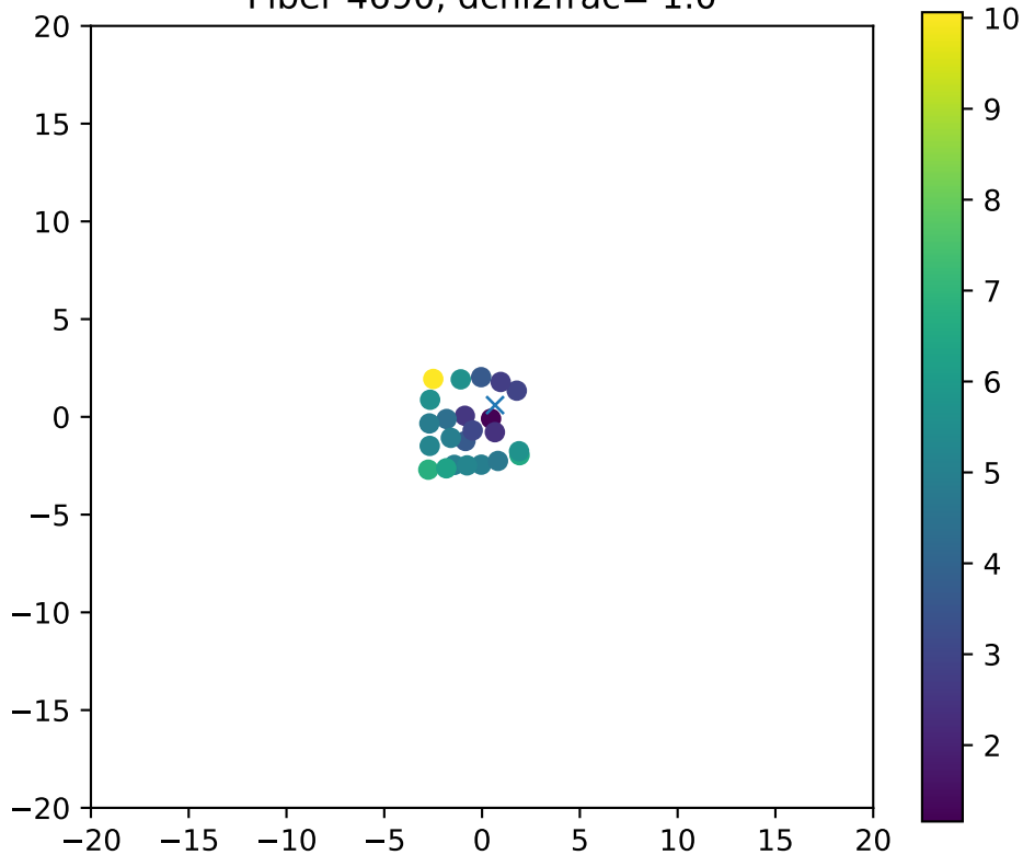
Fiber 4690, dchi2frac= 1.0
