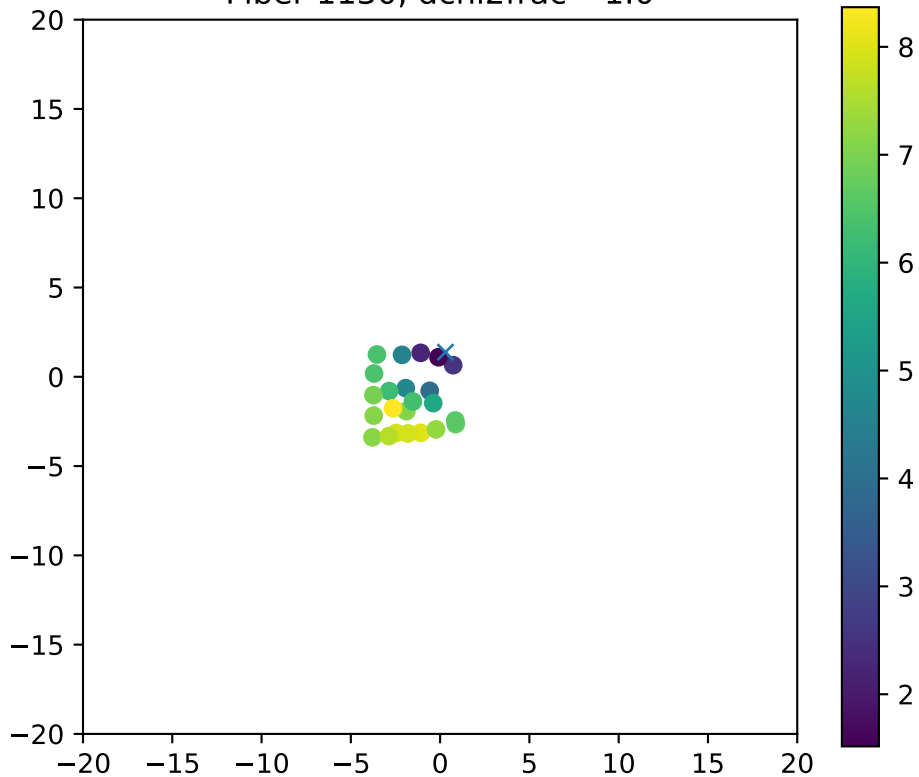
Fiber 1130, dchi2frac= 1.0
