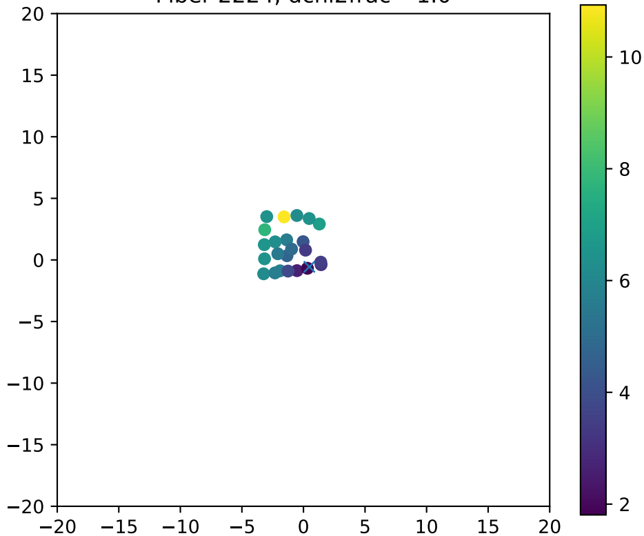
Fiber 2224, dchi2frac= 1.0
