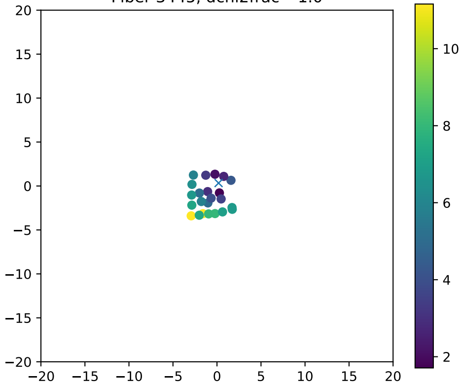
Fiber 3445, dchi2frac= 1.0
