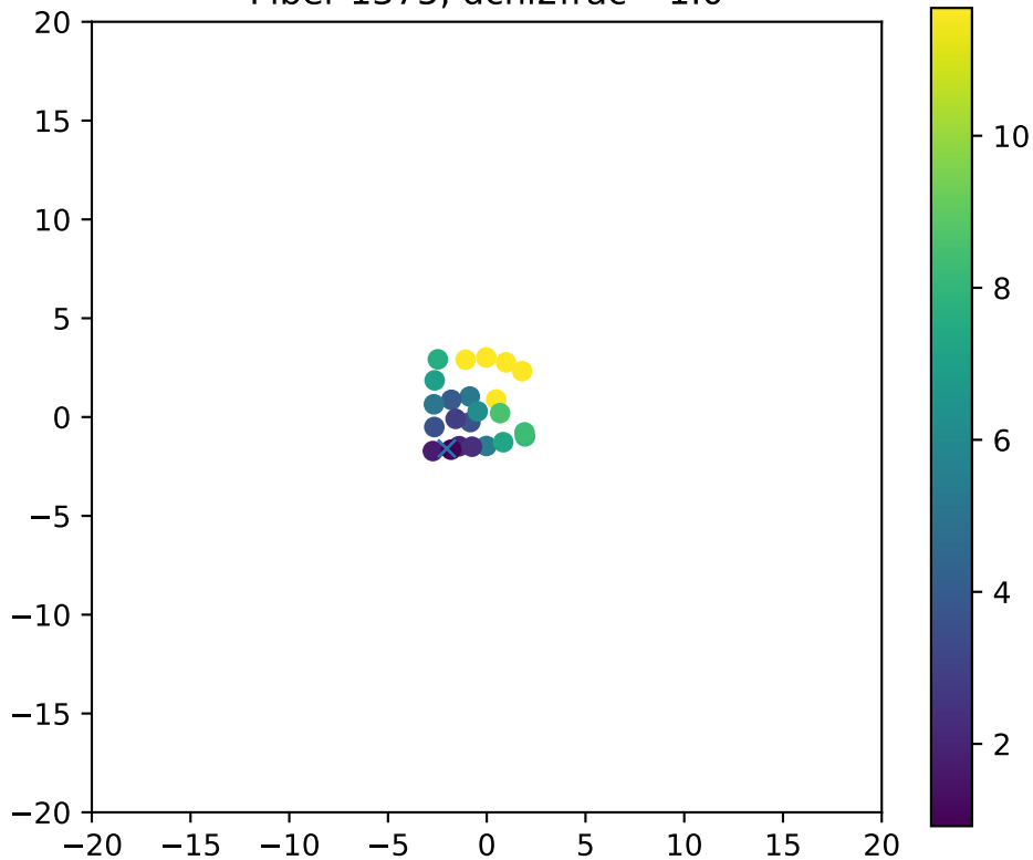
Fiber 1375, dchi2frac= 1.0
