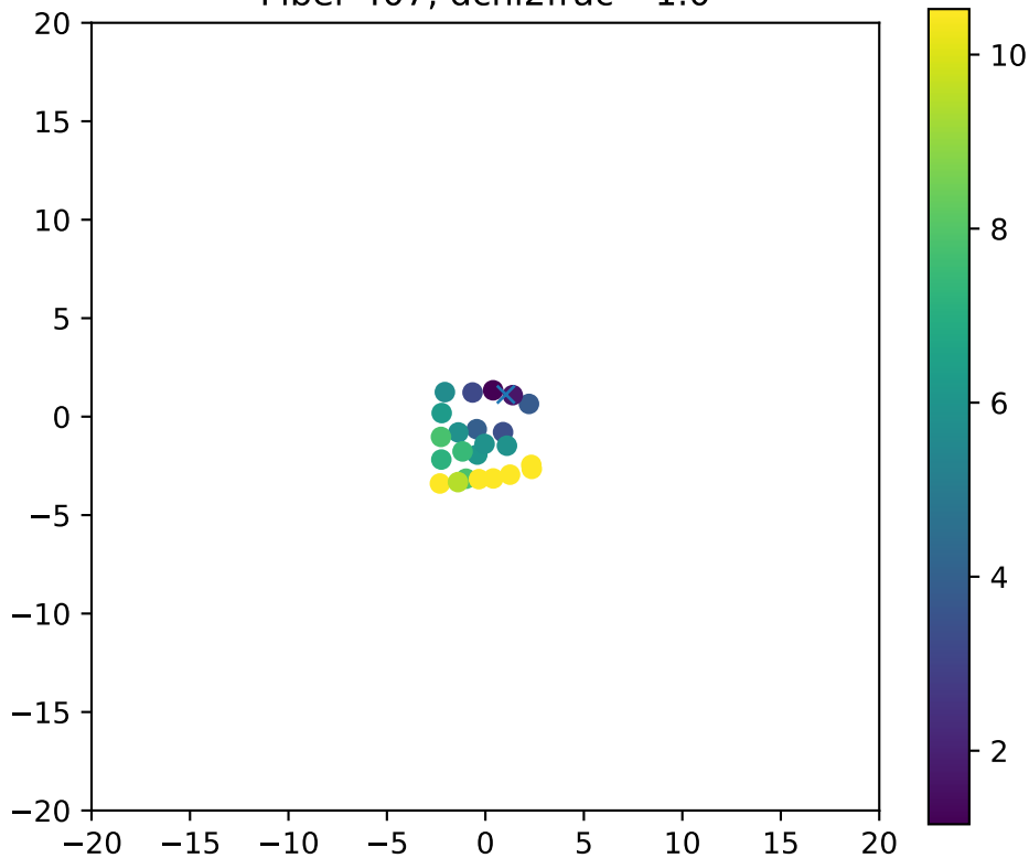
Fiber 407, dchi2frac= 1.0
