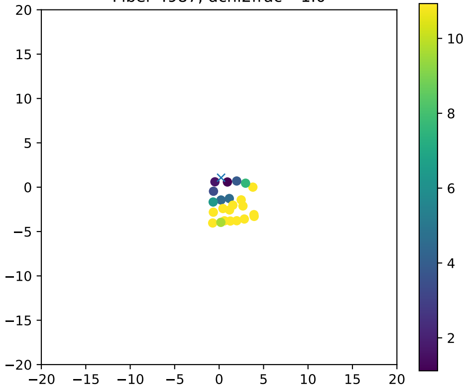
Fiber 4987, dchi2frac= 1.0
