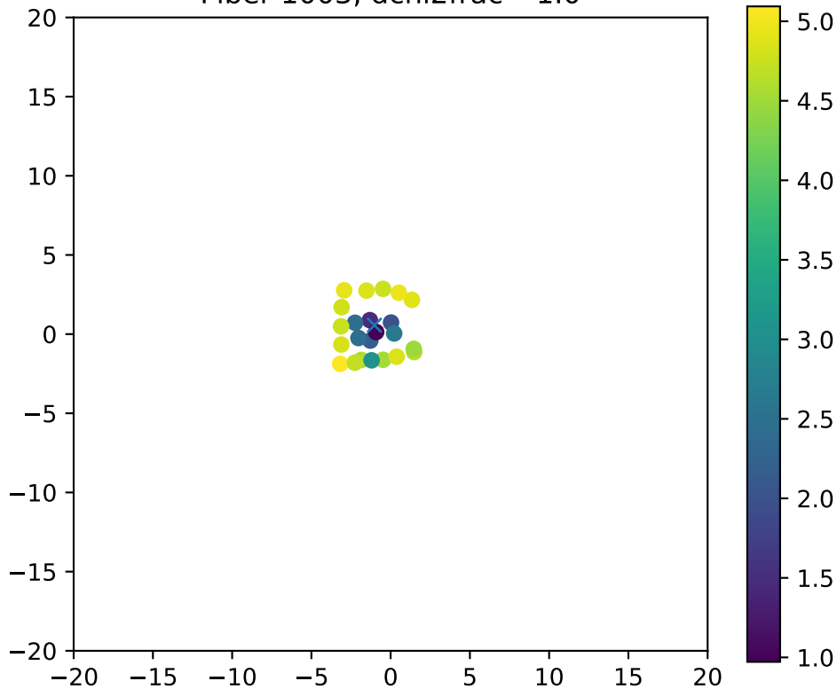
Fiber 1003, dchi2frac= 1.0
