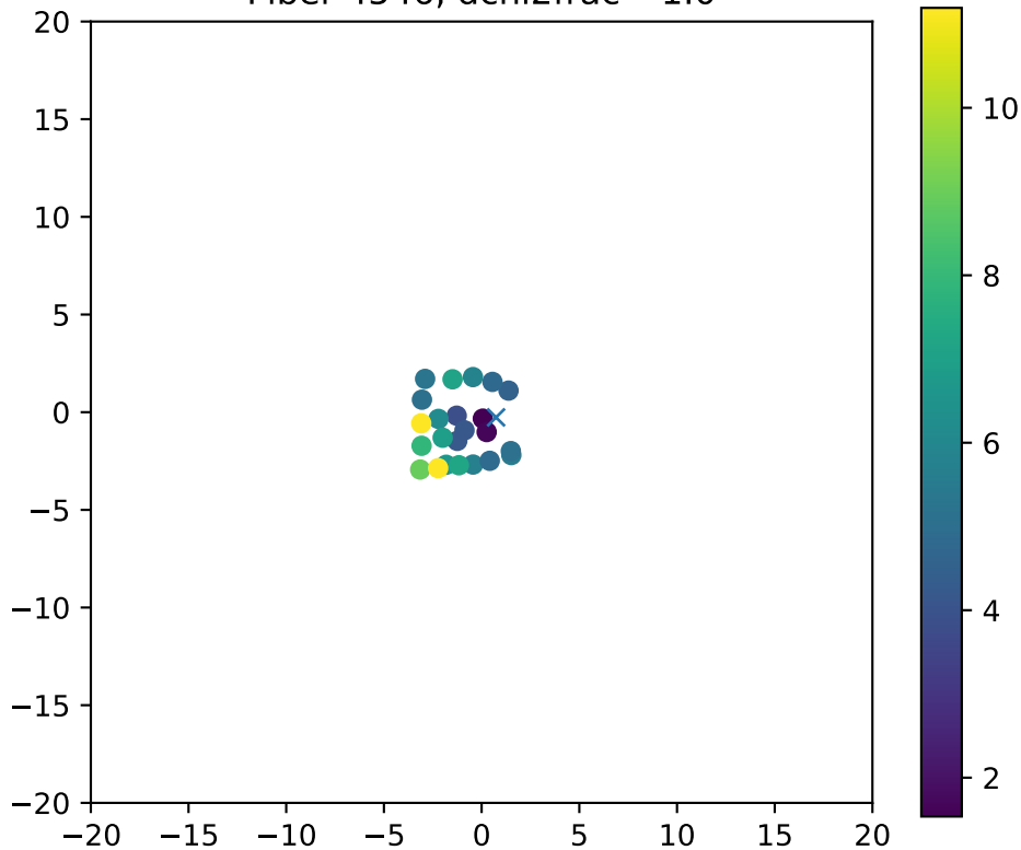
Fiber 4546, dchi2frac= 1.0
