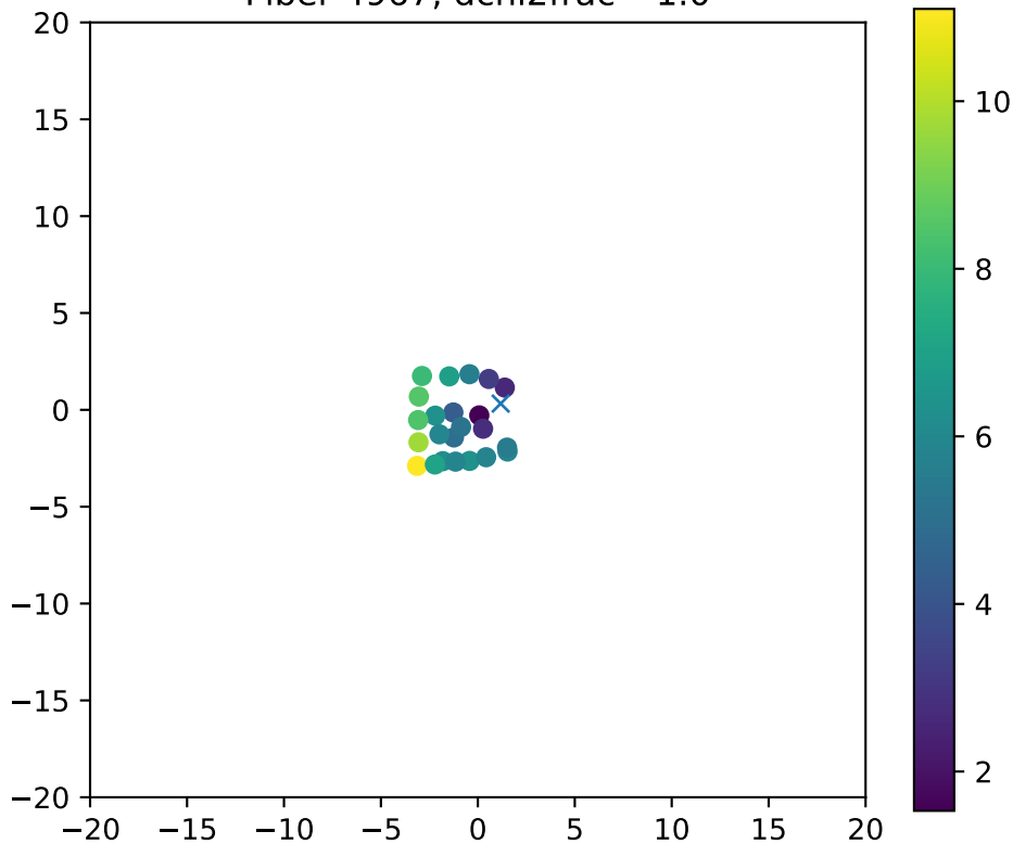
Fiber 4967, dchi2frac= 1.0
