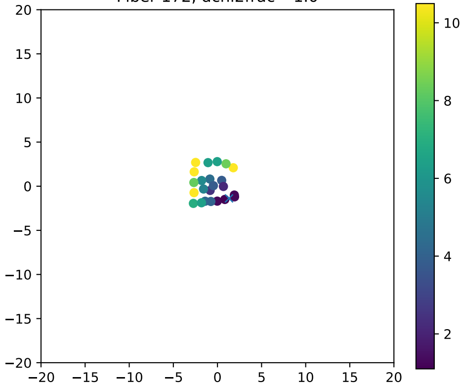
Fiber 172, dchi2frac= 1.0
