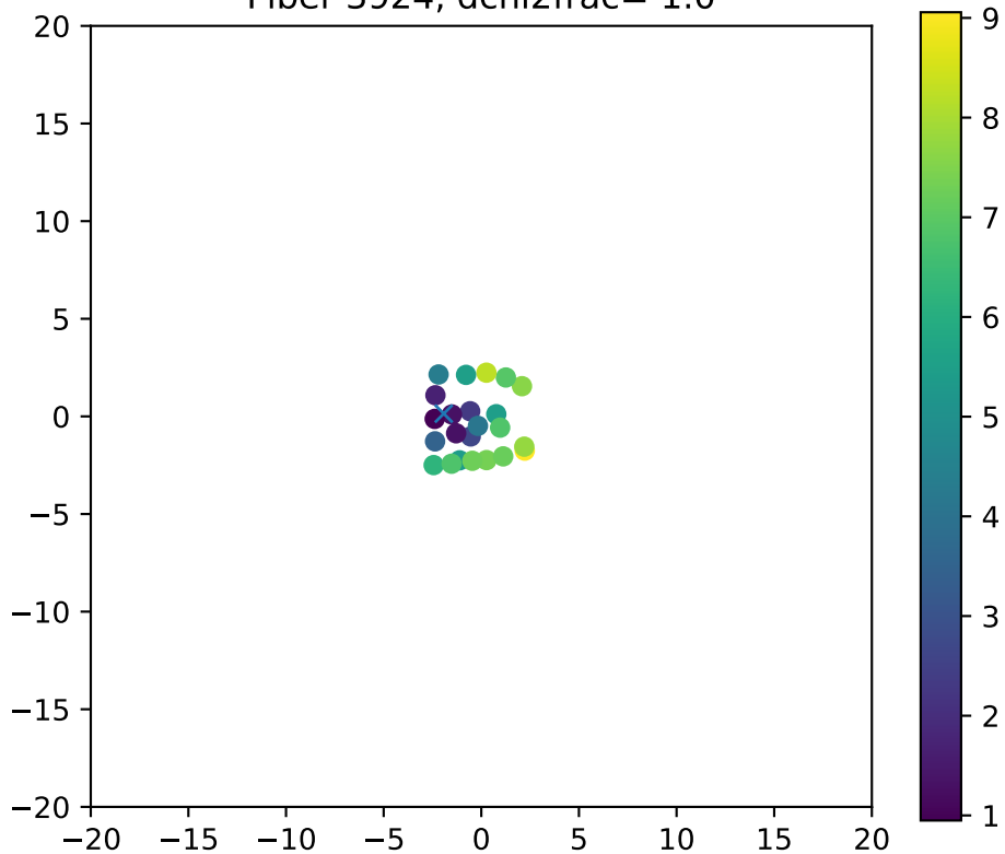
Fiber 3924, dchi2frac= 1.0
