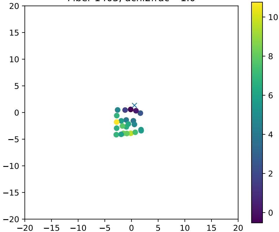
Fiber 1403, dchi2frac= 1.0
