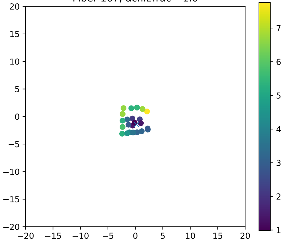
Fiber 167, dchi2frac= 1.0
