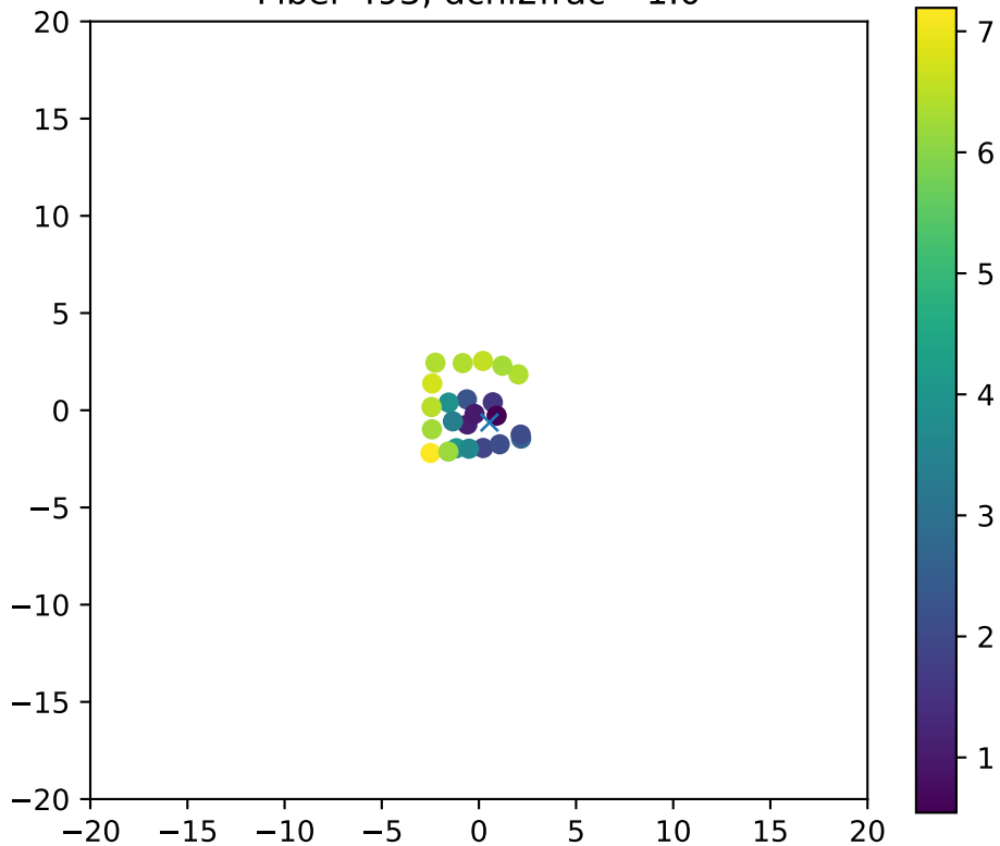
Fiber 493, dchi2frac= 1.0
