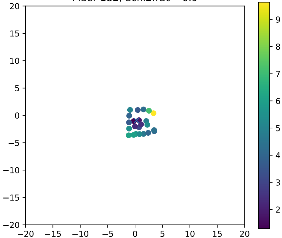
Fiber 182, dchi2frac= 0.9
