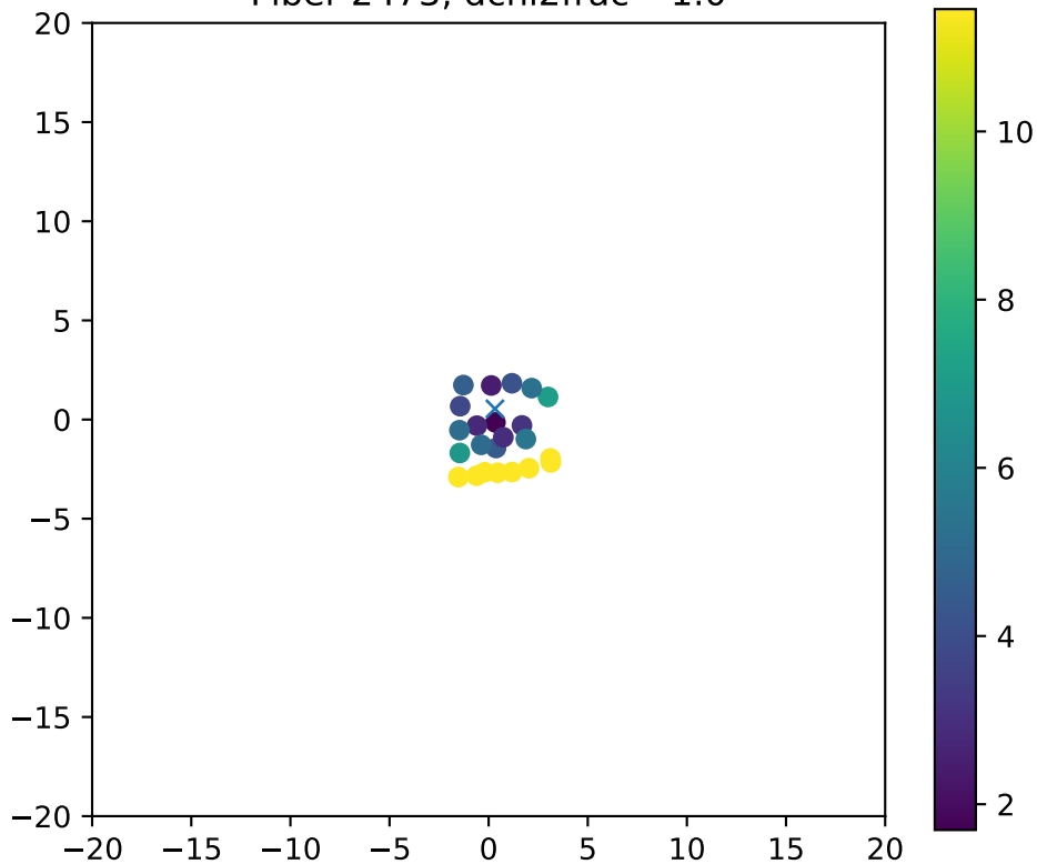
Fiber 2473, dchi2frac= 1.0
