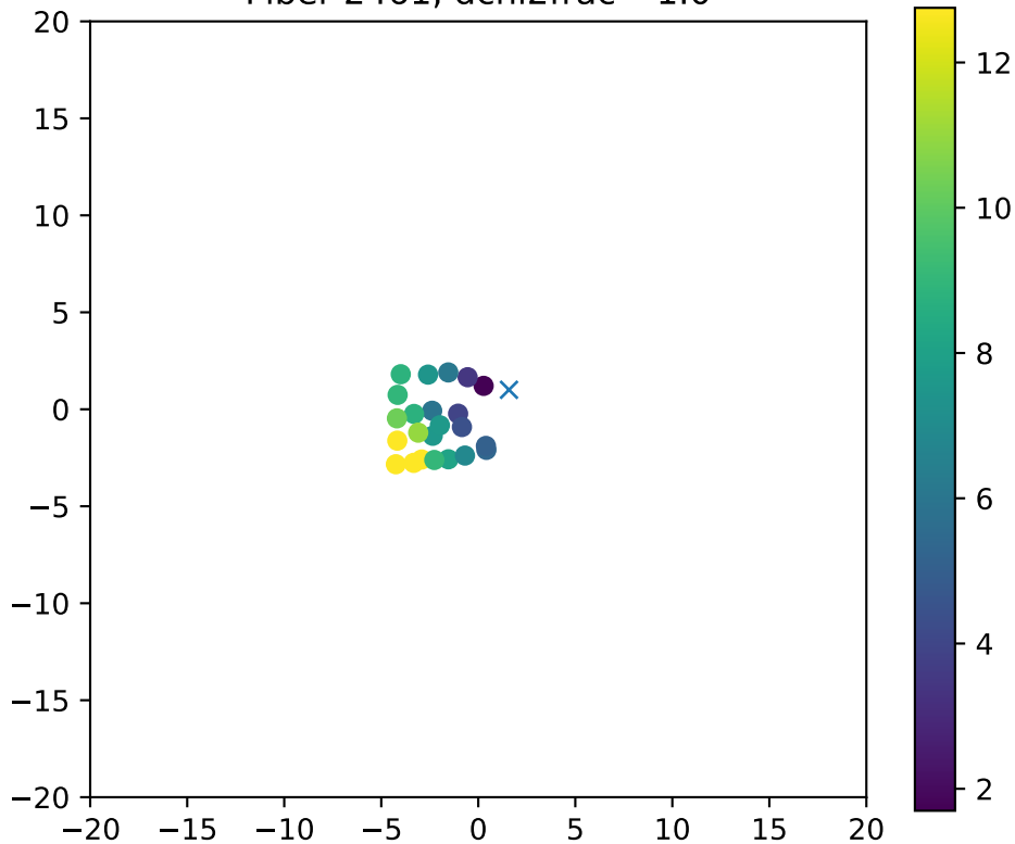
Fiber 2461, dchi2frac= 1.0
