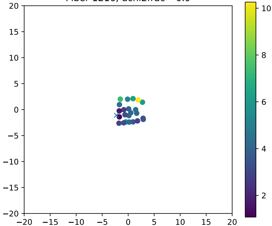
Fiber 1216, dchi2frac= 0.9
