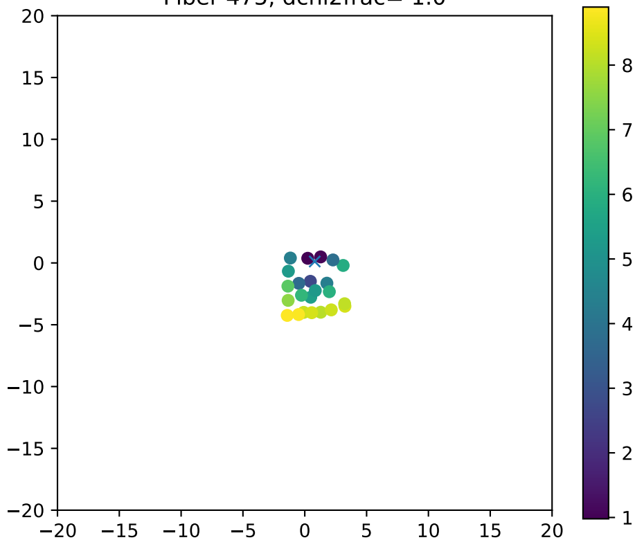
Fiber 475, dchi2frac= 1.0
