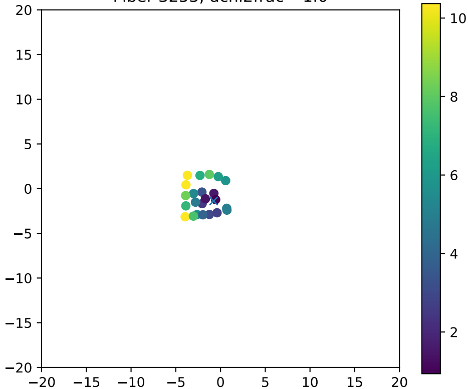
Fiber 3253, dchi2frac= 1.0
