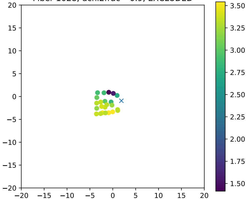
Fiber 1028, dchi2frac= 0.9, EXCLUDED
