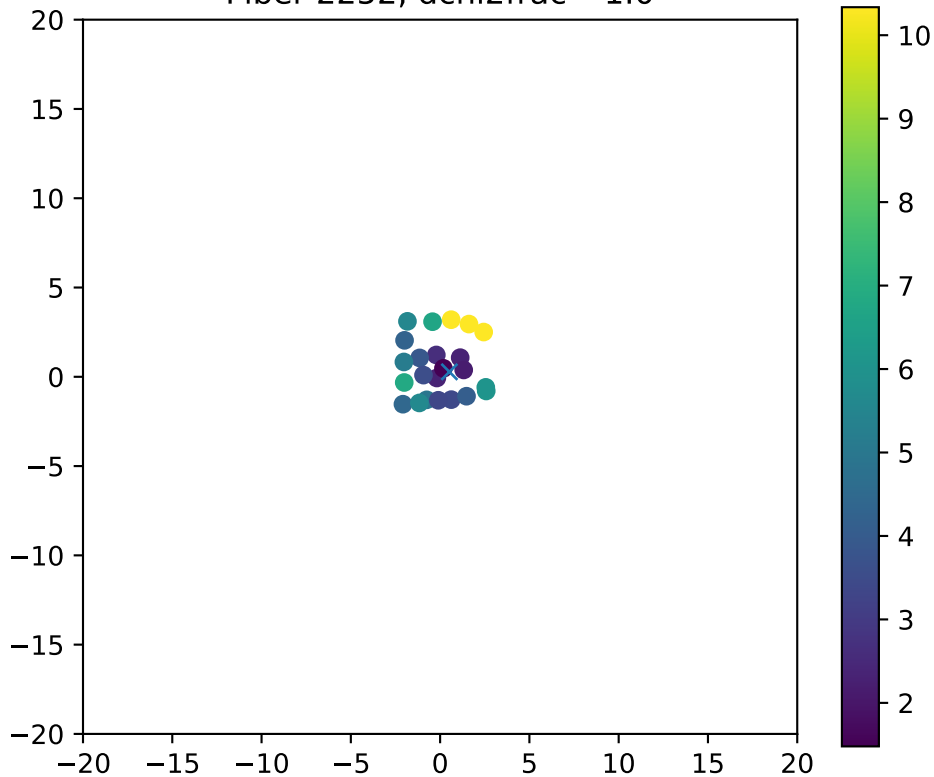
Fiber 2252, dchi2frac= 1.0
