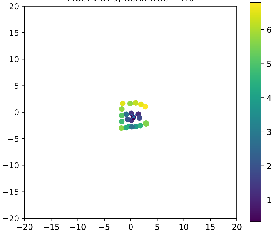
Fiber 2075, dchi2frac= 1.0
