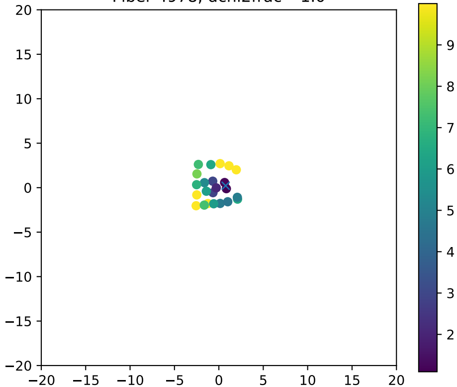
Fiber 4978, dchi2frac= 1.0
