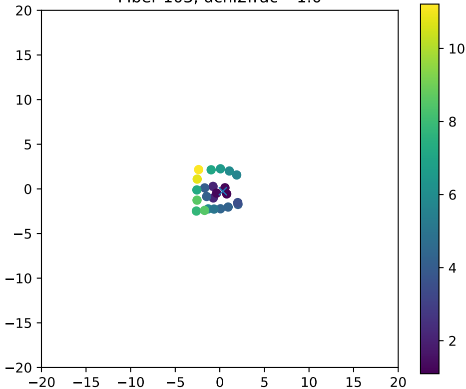
Fiber 103, dchi2frac= 1.0
