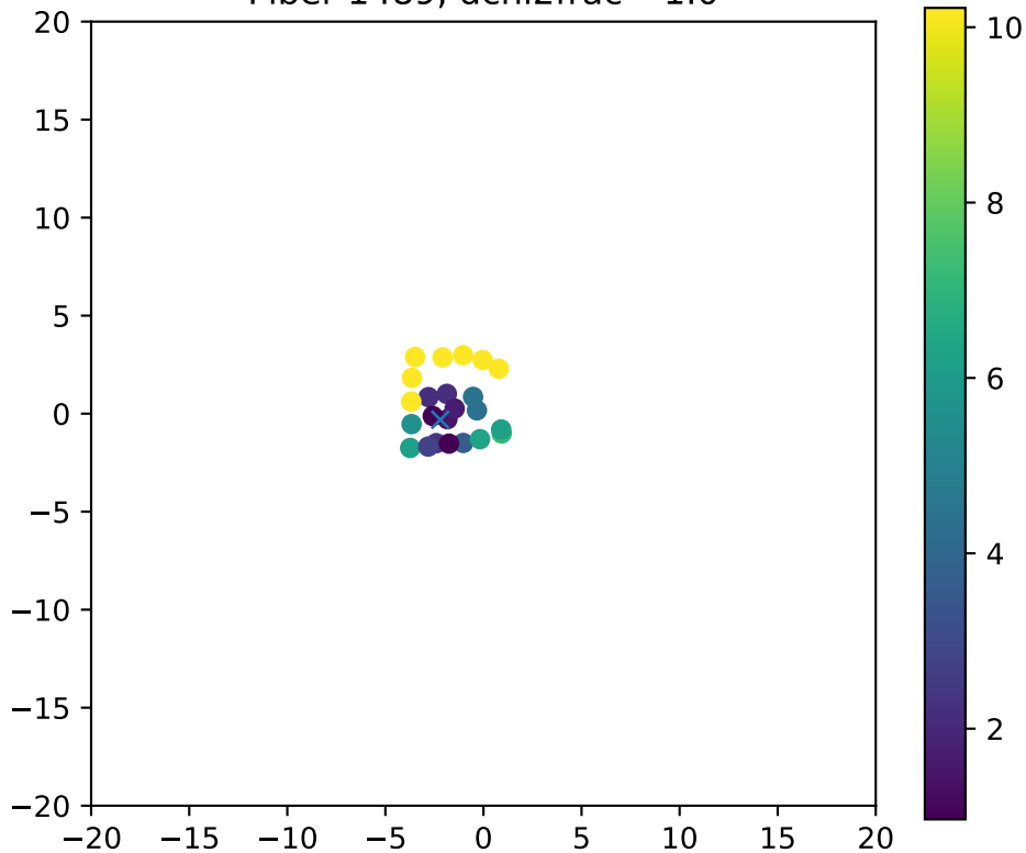
Fiber 1489, dchi2frac= 1.0
