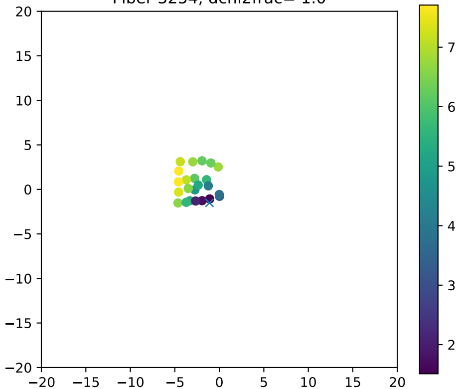
Fiber 3254, dchi2frac= 1.0
