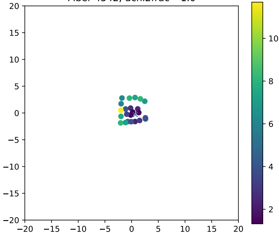
Fiber 4542, dchi2frac= 1.0
