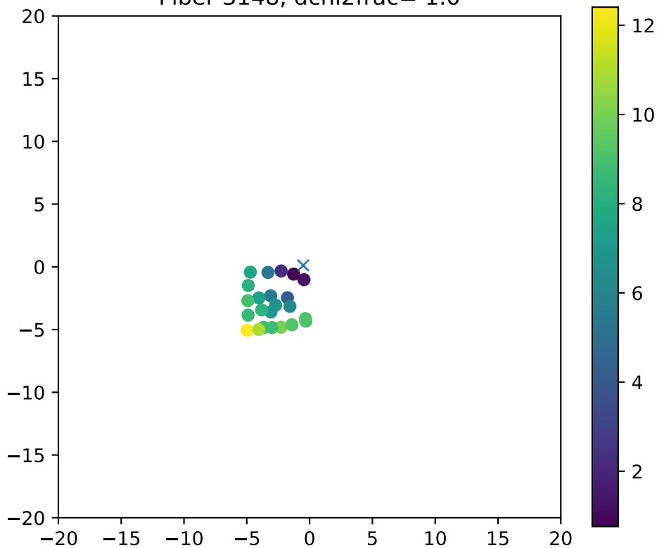
Fiber 3148, dchi2frac= 1.0
