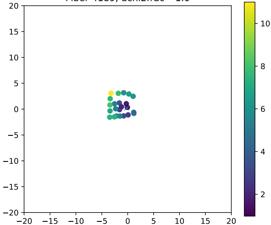
Fiber 4189, dchi2frac= 1.0
