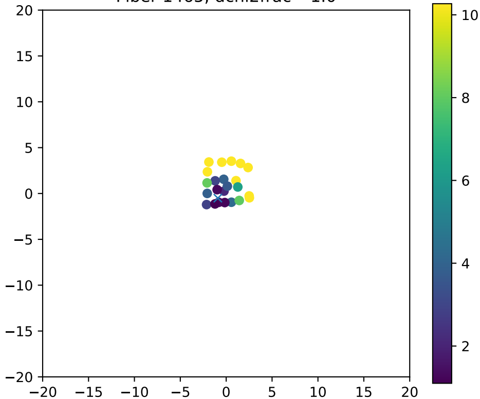
Fiber 1465, dchi2frac= 1.0
