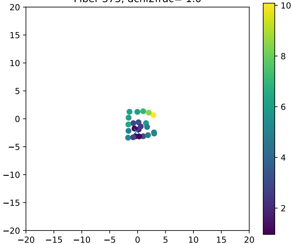
Fiber 373, dchi2frac= 1.0
