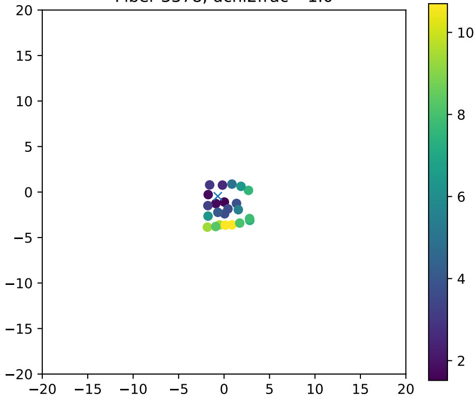
Fiber 3378, dchi2frac= 1.0
