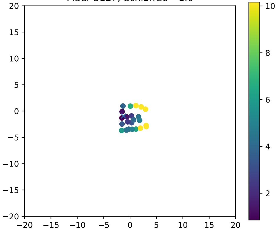
Fiber 3127, dchi2frac= 1.0
