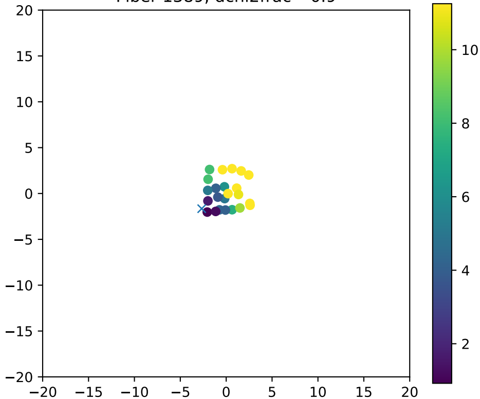
Fiber 1389, dchi2frac= 0.9
