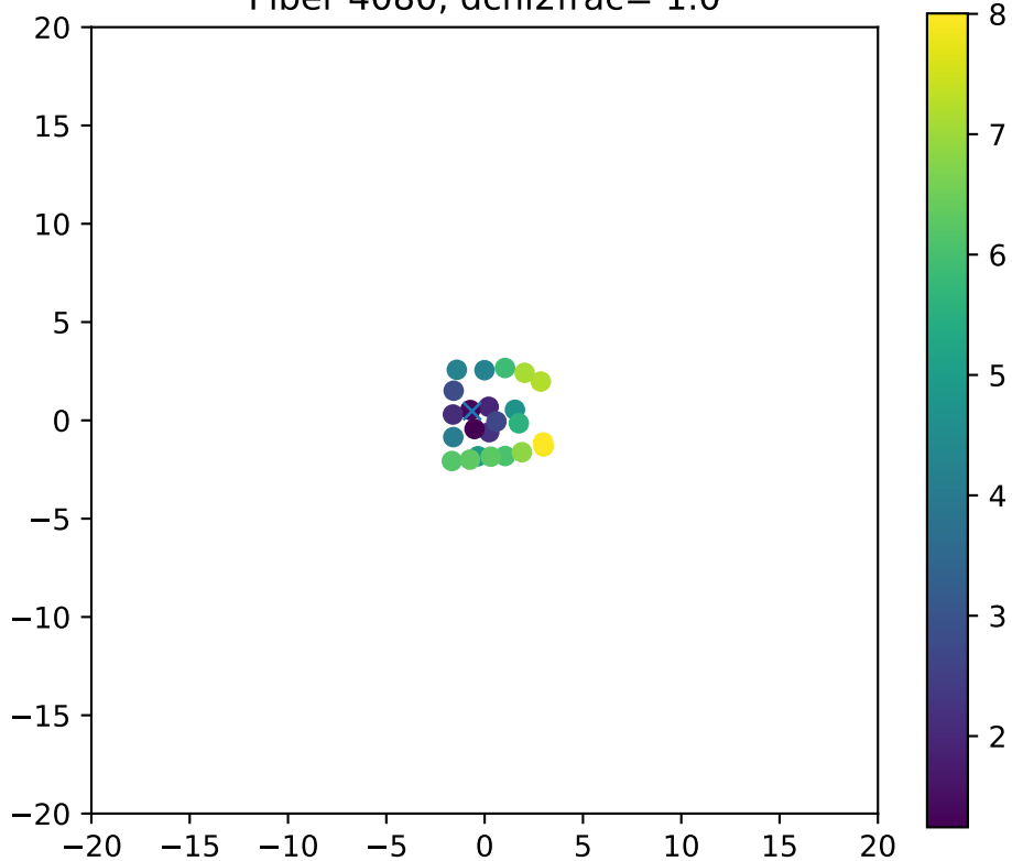
Fiber 4080, dchi2frac= 1.0
