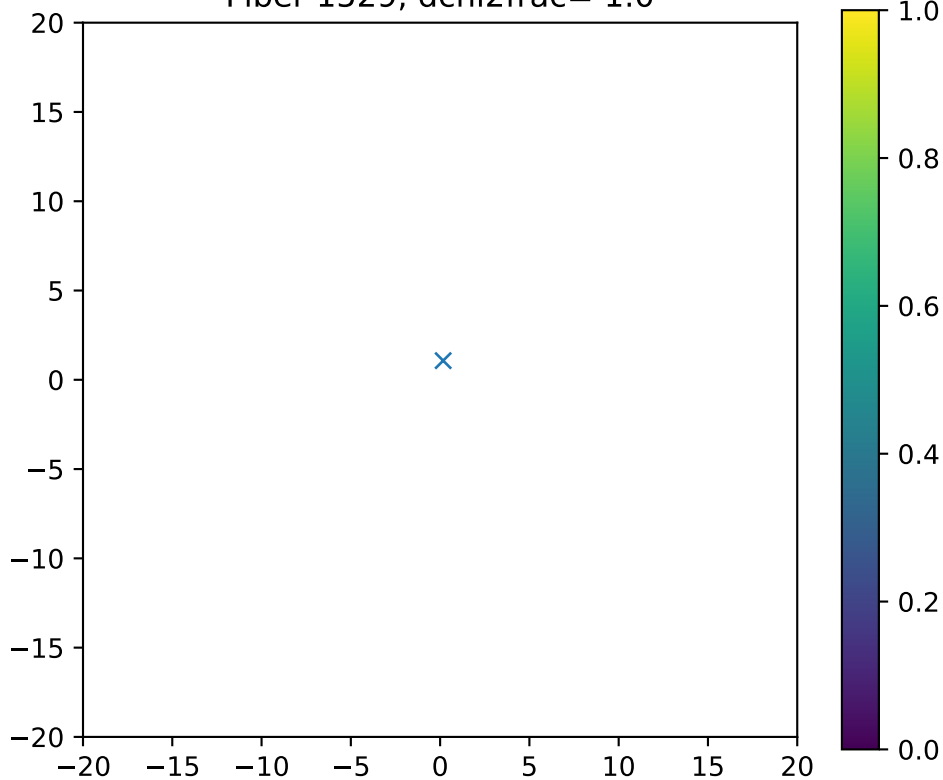
Fiber 1529, dchi2frac= 1.0
