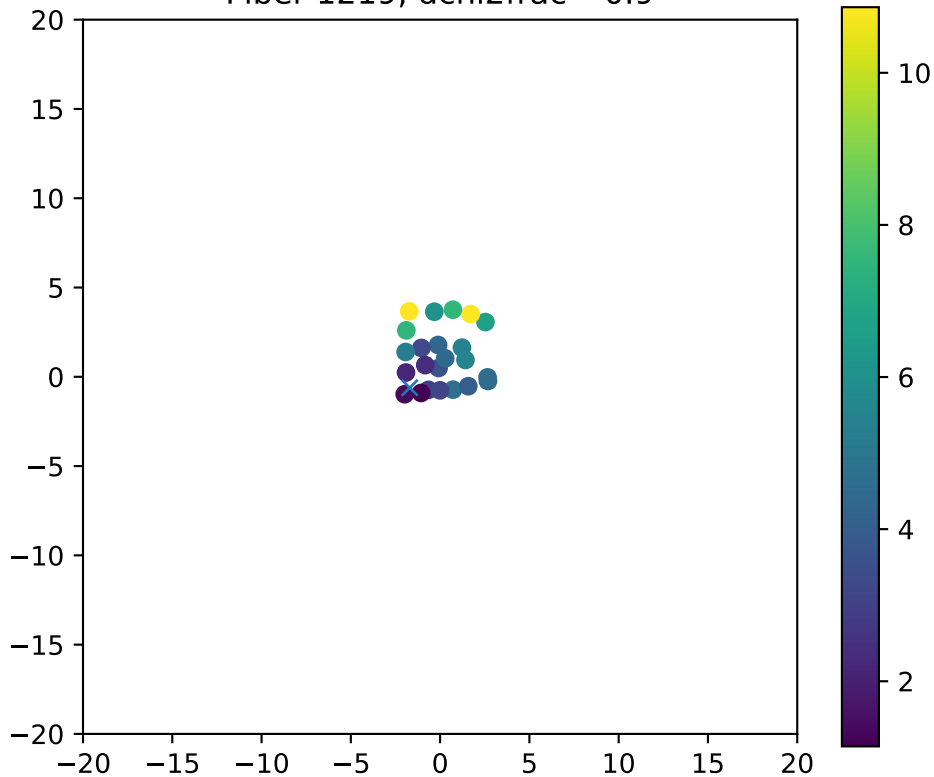
Fiber 1219, dchi2frac= 0.9
