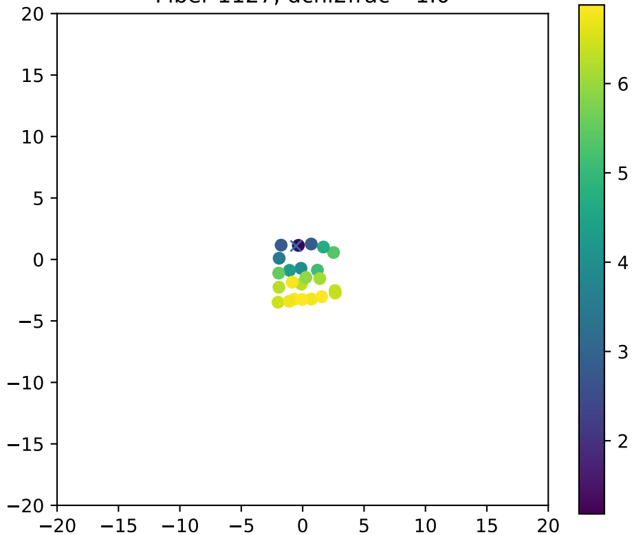
Fiber 1127, dchi2frac= 1.0
