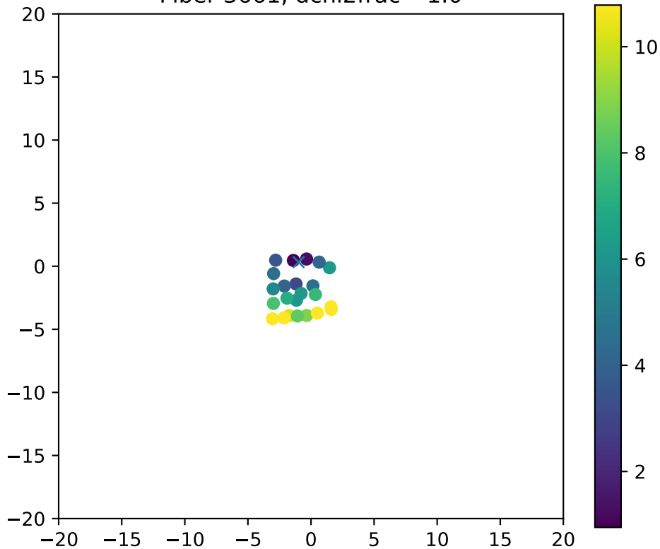
Fiber 3661, dchi2frac= 1.0
