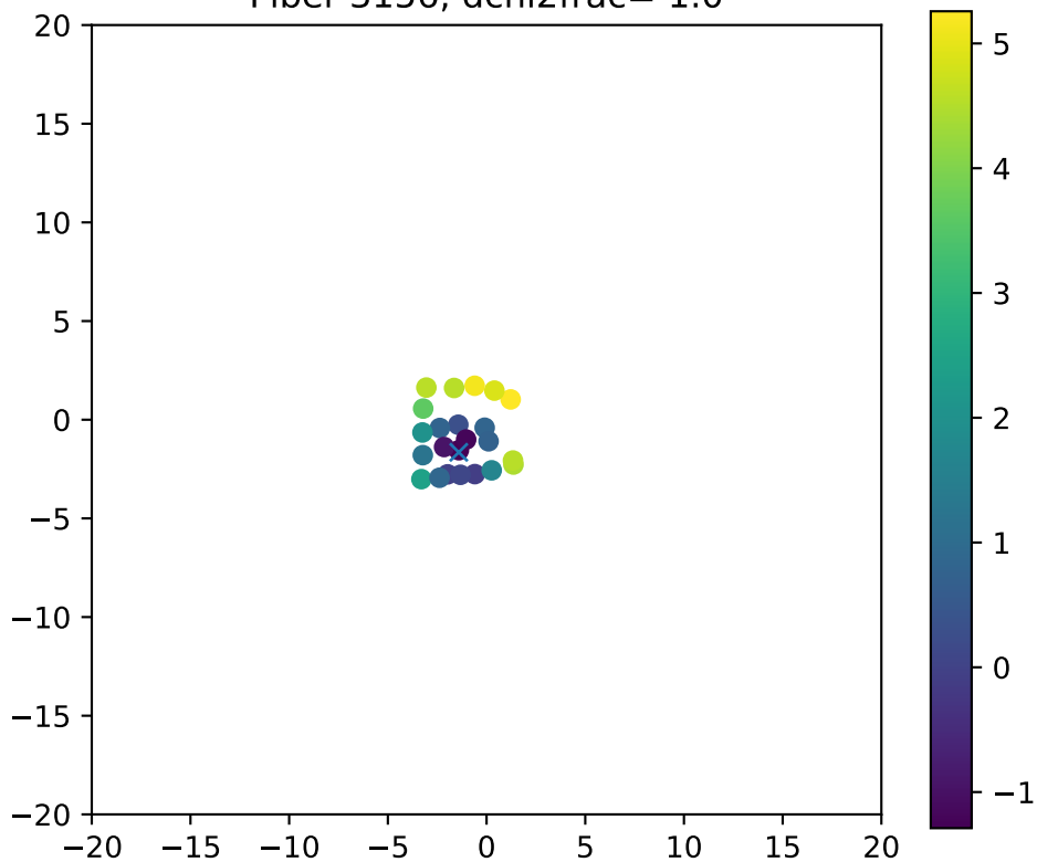
Fiber 3156, dchi2frac= 1.0
