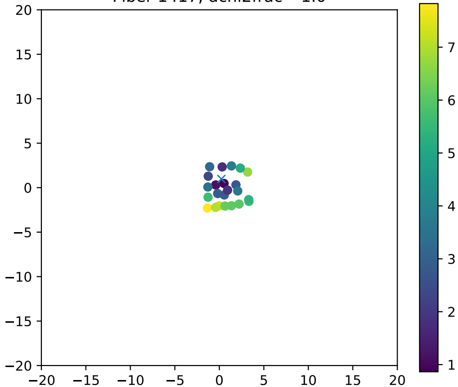
Fiber 1417, dchi2frac= 1.0
