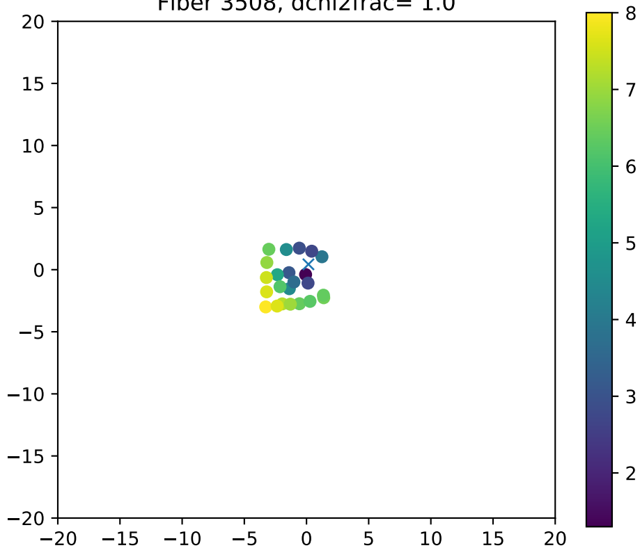
Fiber 3508, dchi2frac= 1.0
