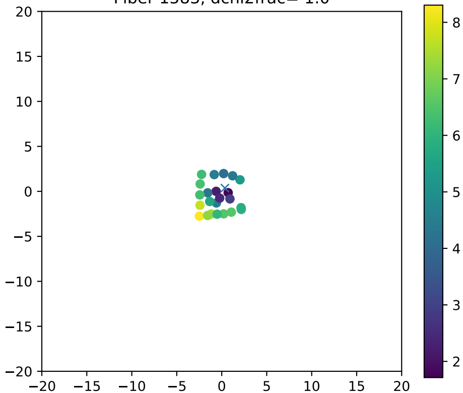
Fiber 1583, dchi2frac= 1.0
