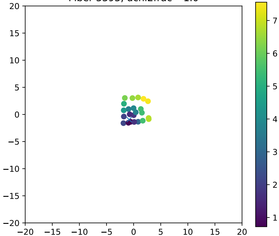
Fiber 3393, dchi2frac= 1.0
