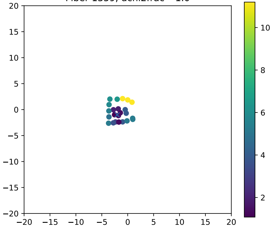
Fiber 1359, dchi2frac= 1.0
