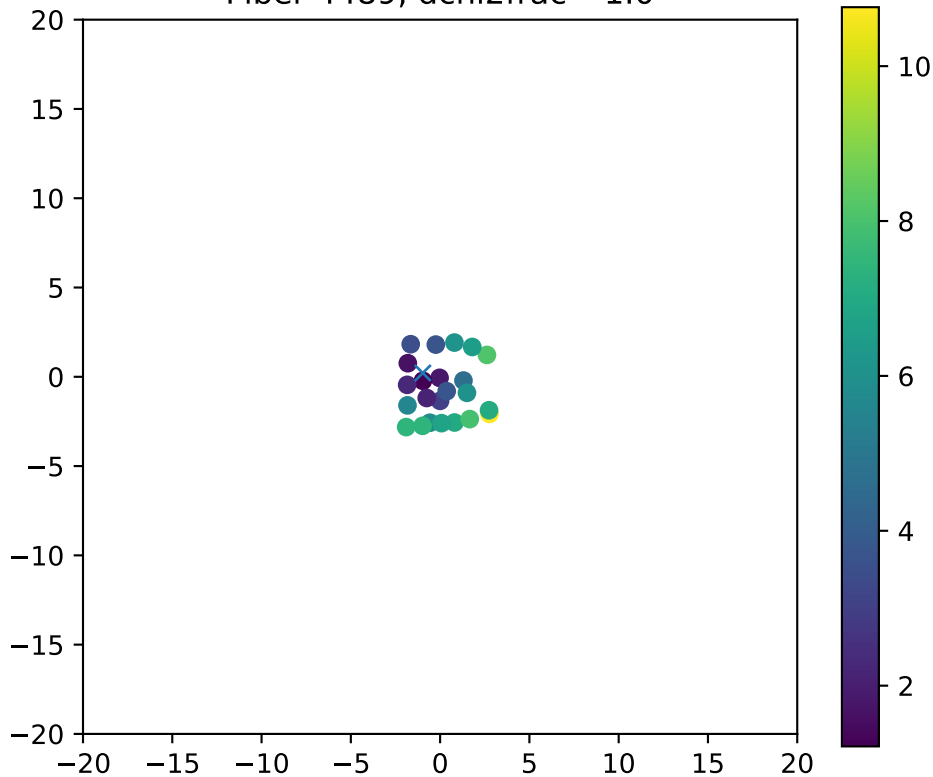
Fiber 4489, dchi2frac= 1.0
