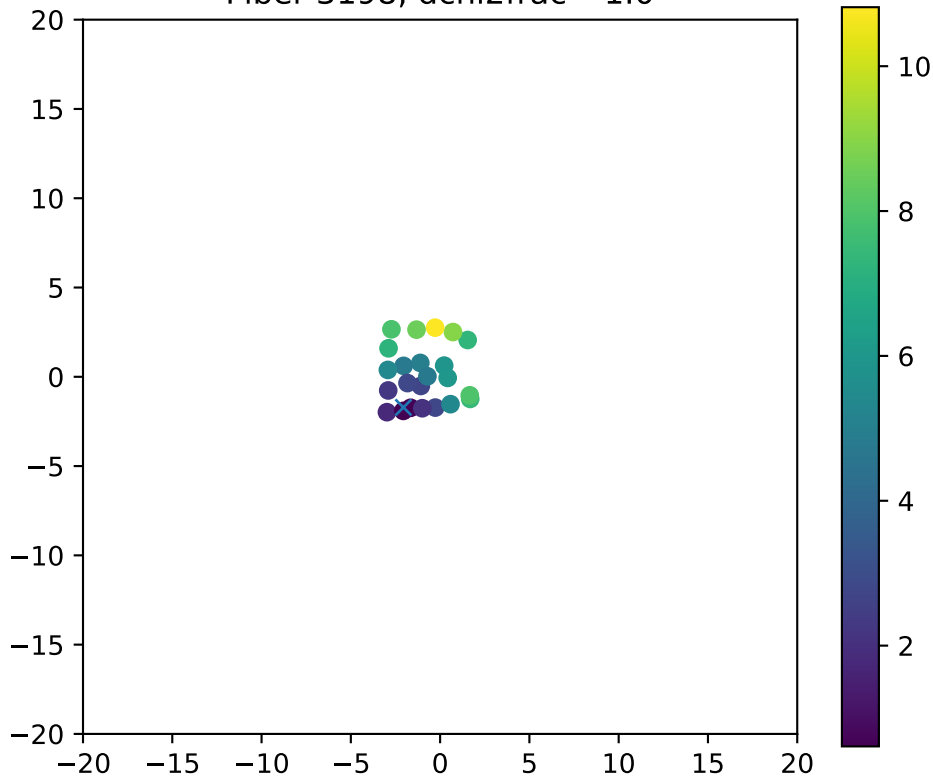
Fiber 3198, dchi2frac= 1.0
