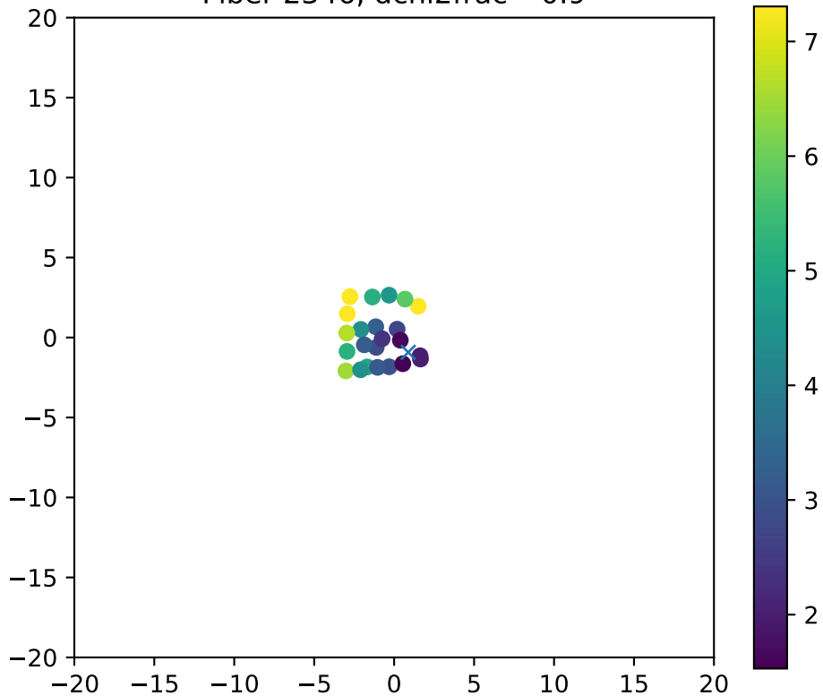
Fiber 2346, dchi2frac= 0.9
