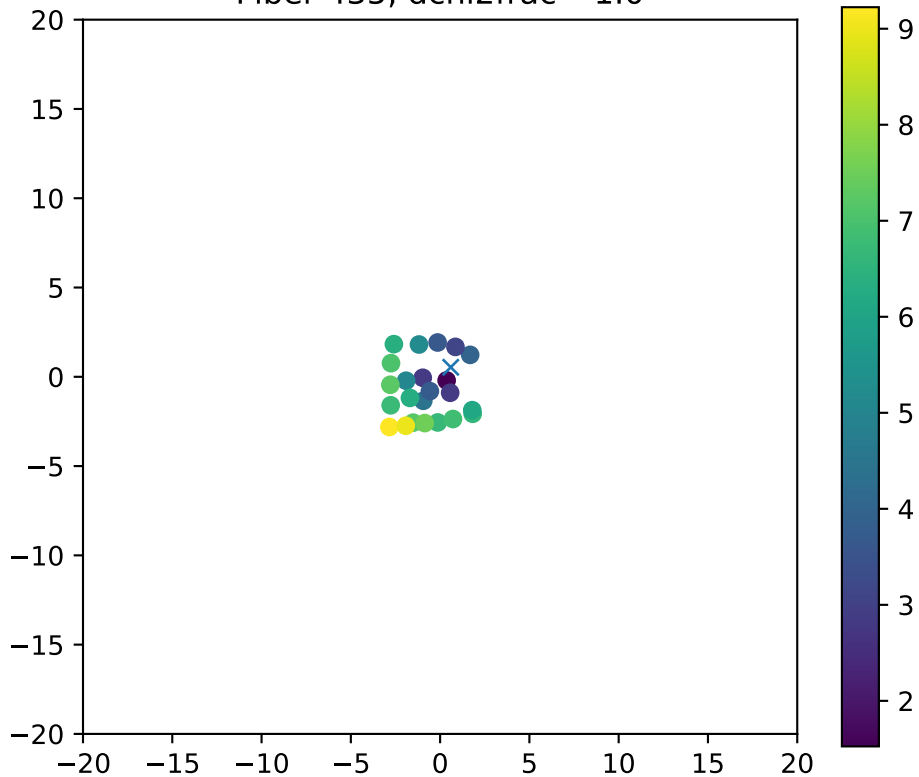
Fiber 435, dchi2frac= 1.0
