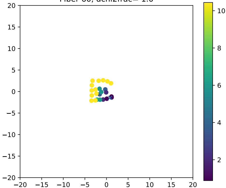
Fiber 60, dchi2frac= 1.0
