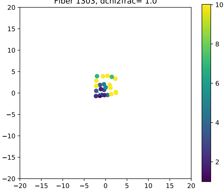
Fiber 1303, dchi2frac= 1.0
