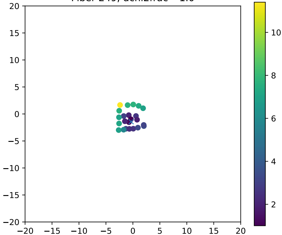
Fiber 249, dchi2frac= 1.0
