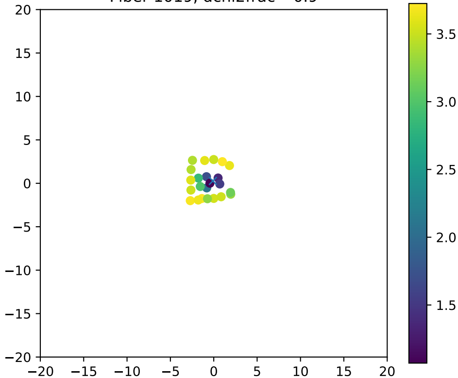
Fiber 1019, dchi2frac= 0.9
