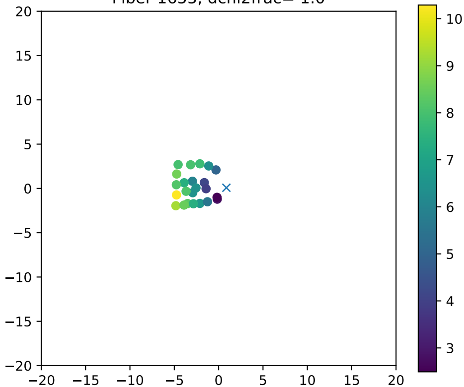
Fiber 1655, dchi2frac= 1.0
