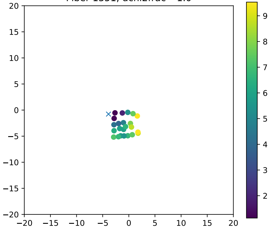
Fiber 1351, dchi2frac= 1.0
