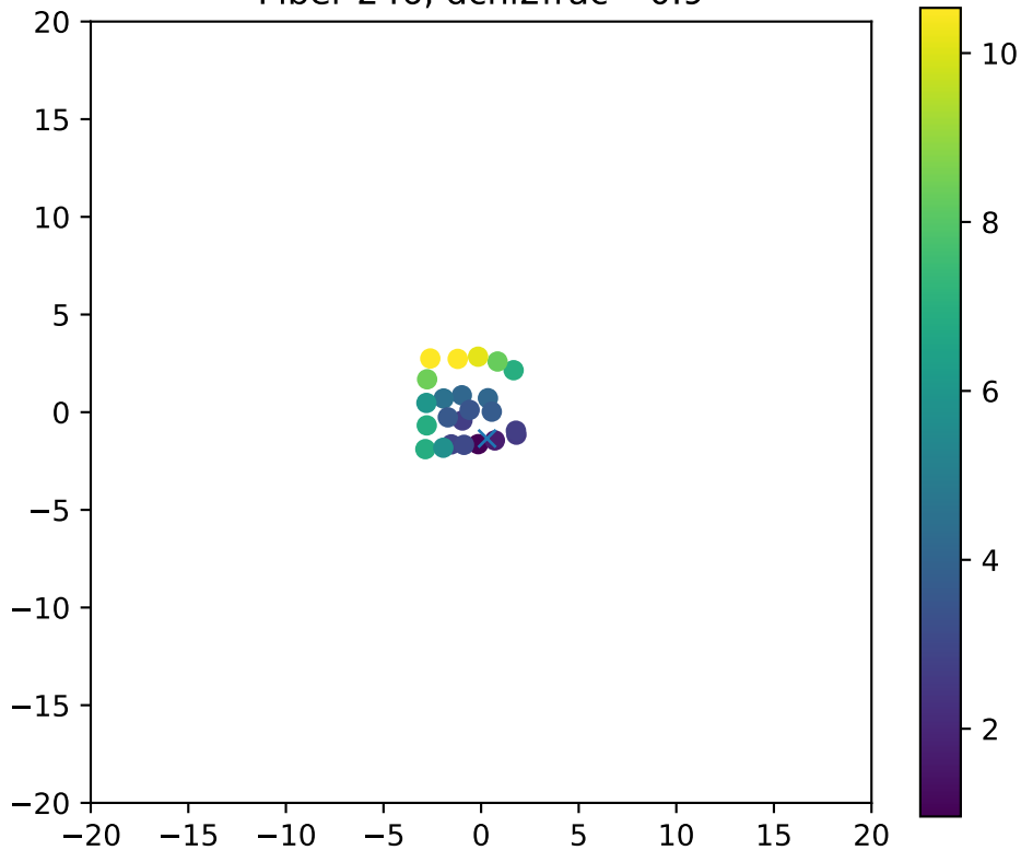
Fiber 246, dchi2frac= 0.9
