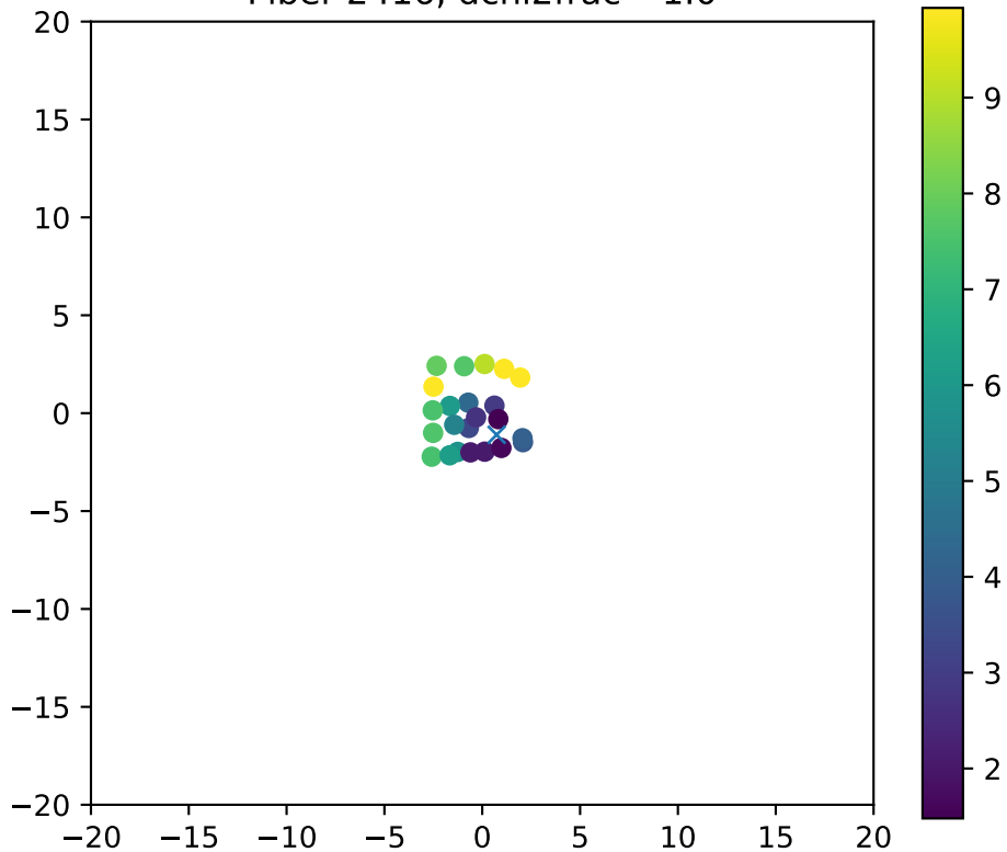
Fiber 2416, dchi2frac= 1.0
