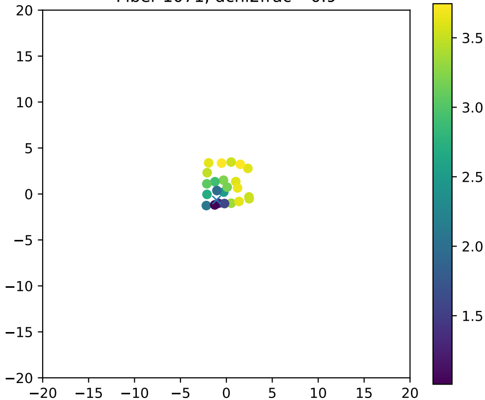
Fiber 1071, dchi2frac= 0.9
