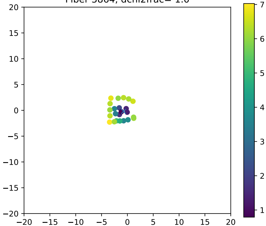
Fiber 3864, dchi2frac= 1.0
