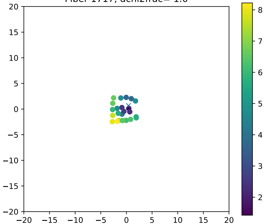
Fiber 1717, dchi2frac= 1.0
