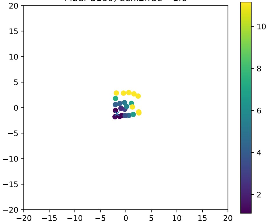
Fiber 3100, dchi2frac= 1.0
