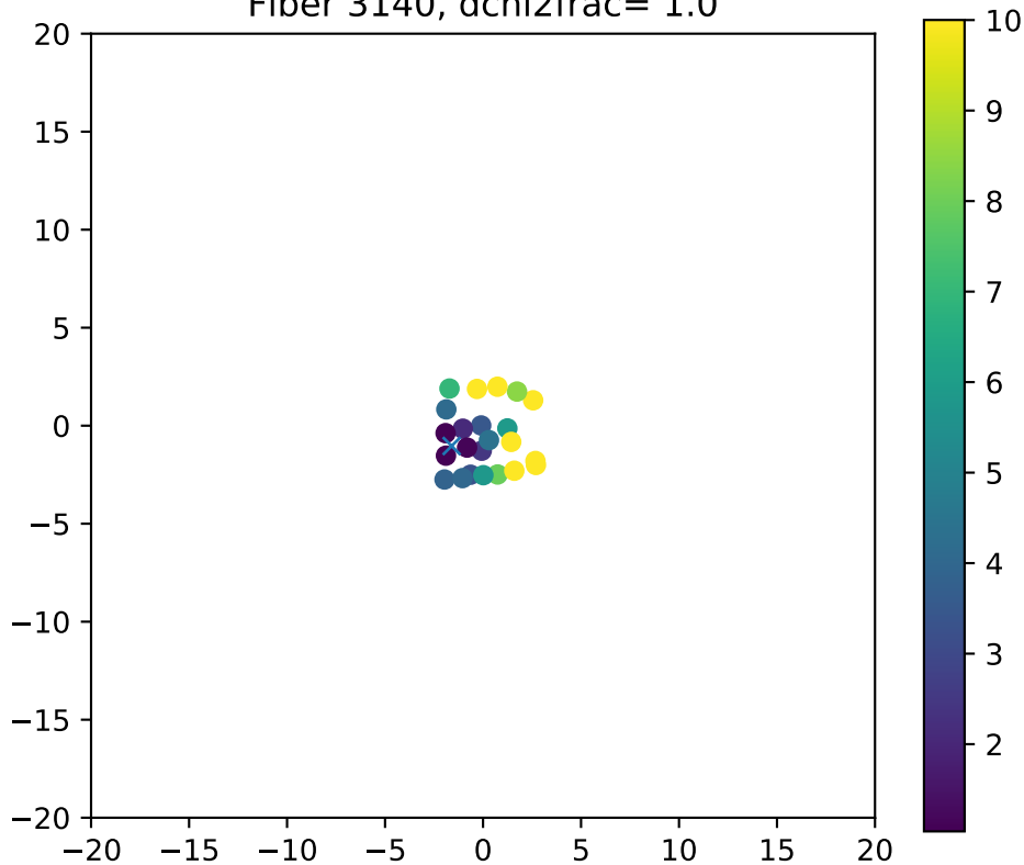
Fiber 3140, dchi2frac= 1.0
