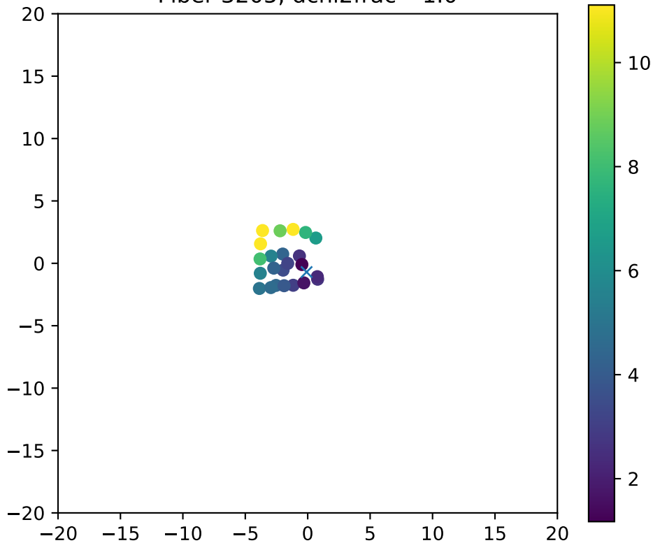
Fiber 3205, dchi2frac= 1.0
