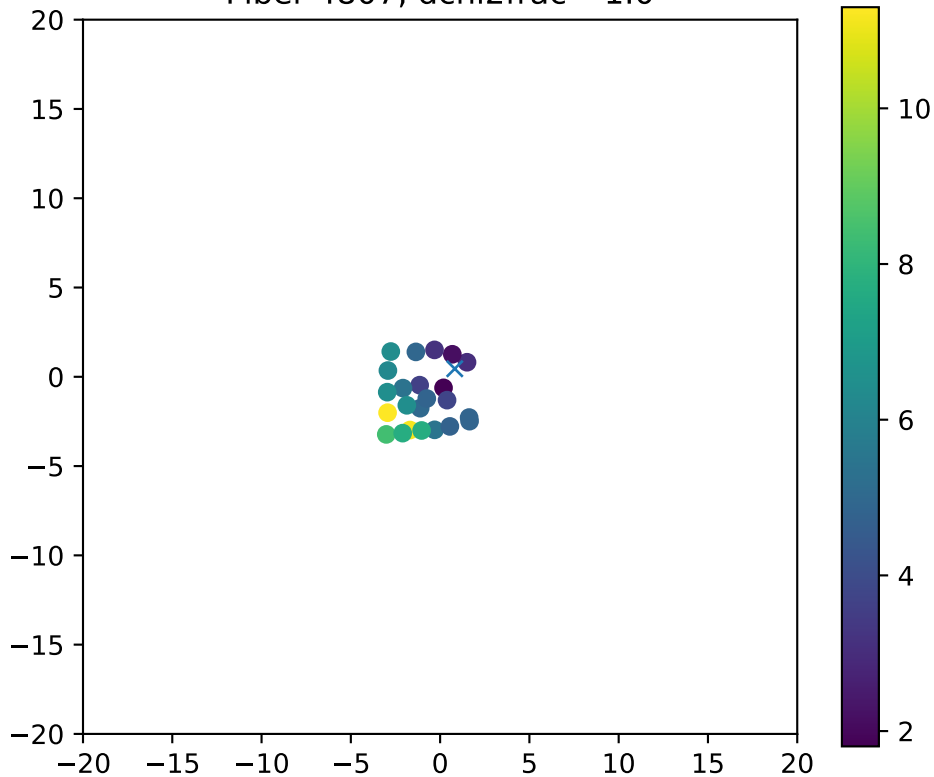
Fiber 4807, dchi2frac= 1.0
