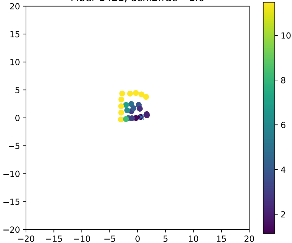
Fiber 1421, dchi2frac= 1.0
