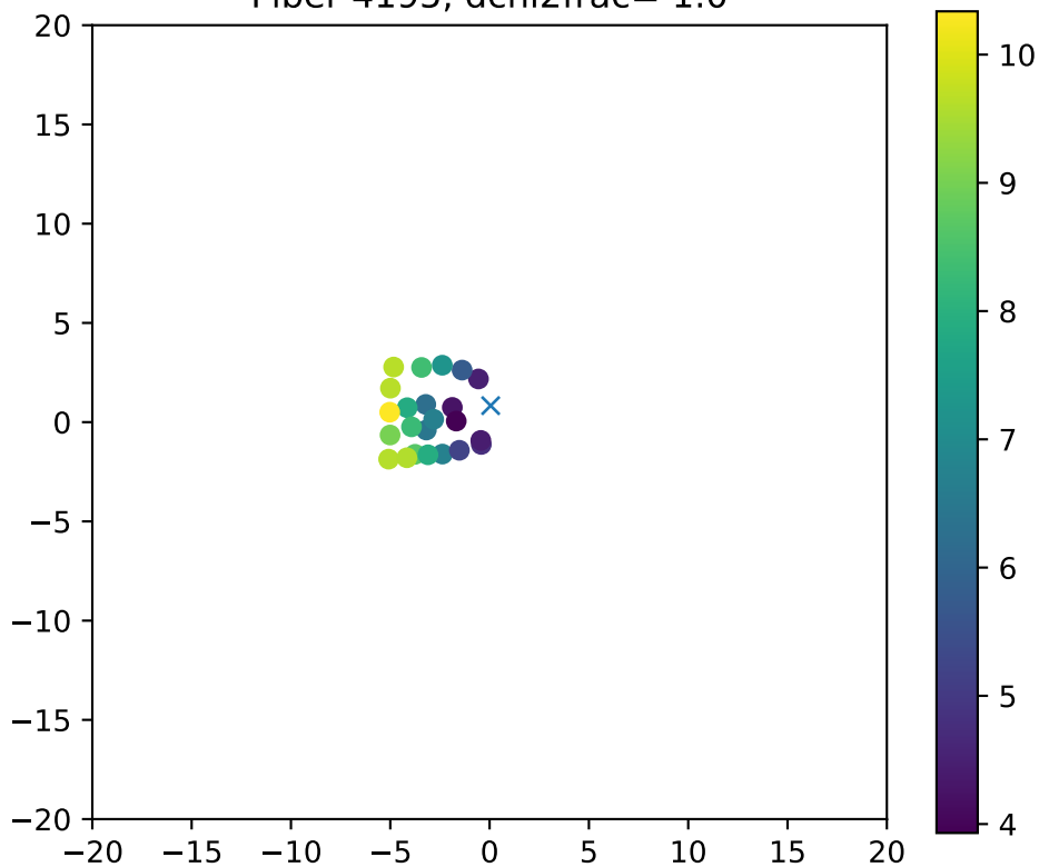
Fiber 4195, dchi2frac= 1.0
