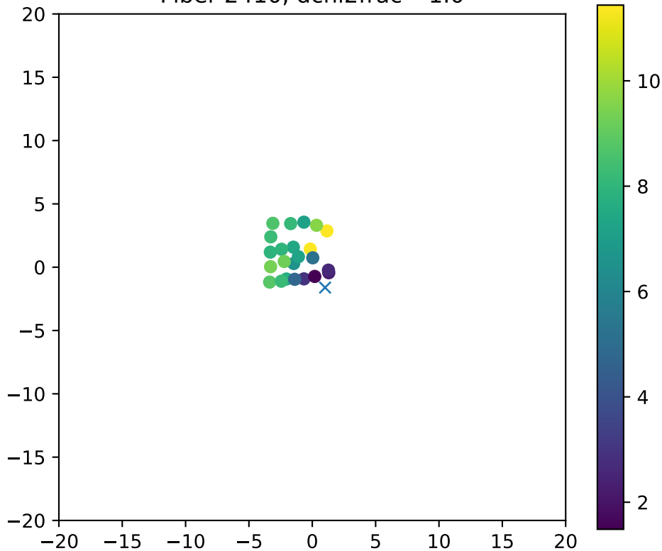
Fiber 2410, dchi2frac= 1.0
