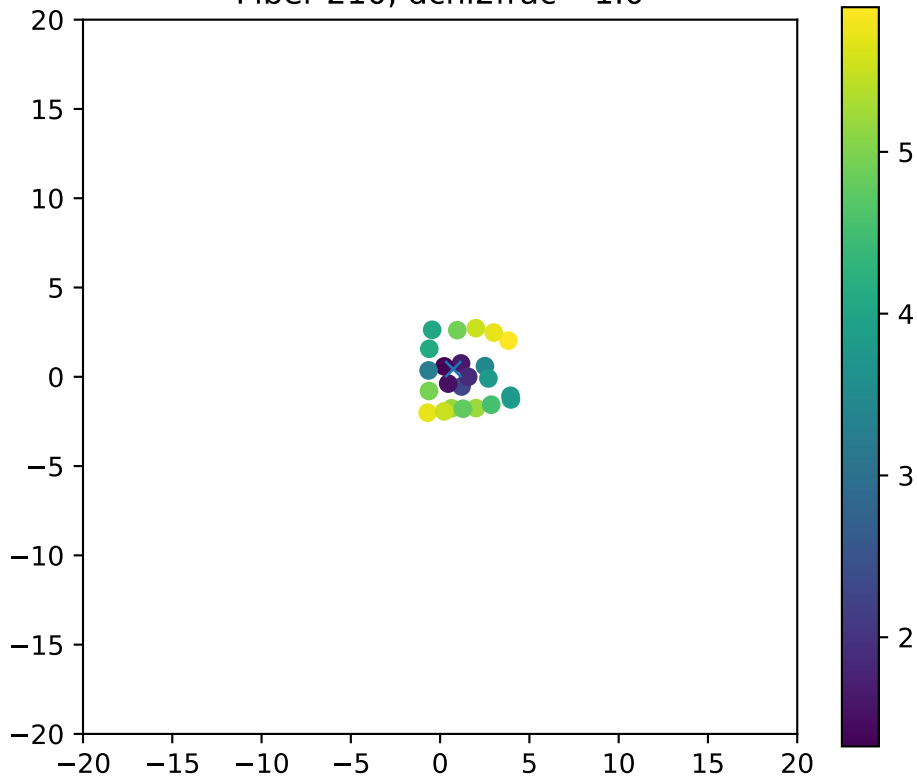
Fiber 210, dchi2frac= 1.0
