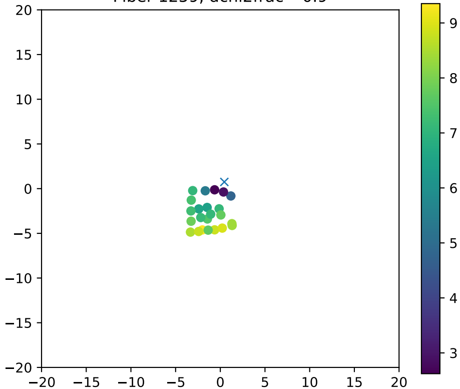
Fiber 1259, dchi2frac= 0.9
