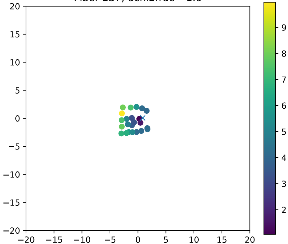
Fiber 237, dchi2frac= 1.0
