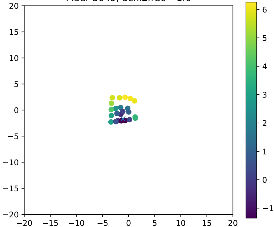
Fiber 3049, dchi2frac= 1.0
