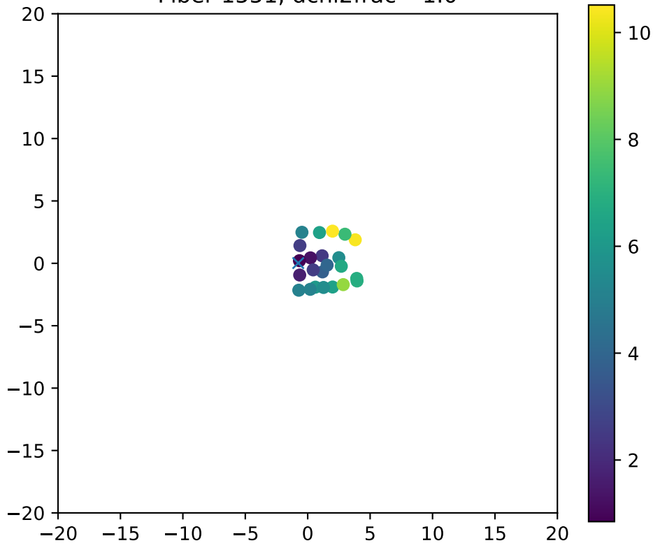
Fiber 1551, dchi2frac= 1.0
