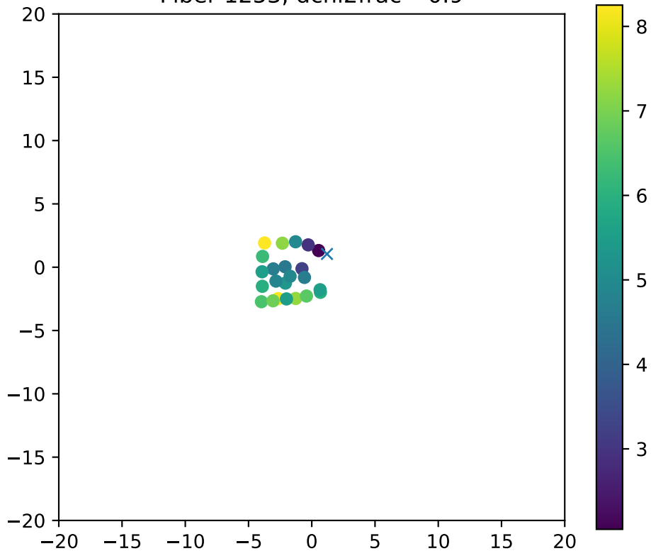
Fiber 1253, dchi2frac= 0.9
