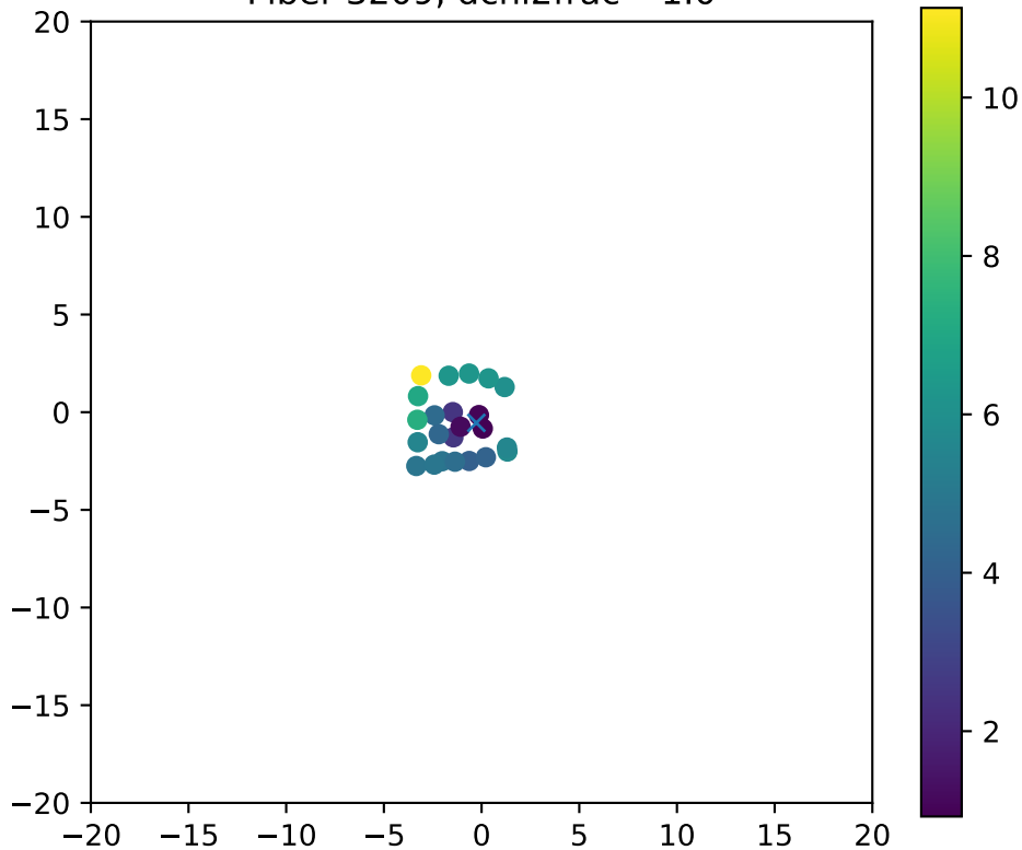
Fiber 3209, dchi2frac= 1.0
