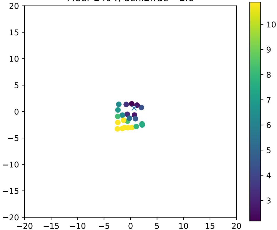
Fiber 2494, dchi2frac= 1.0
