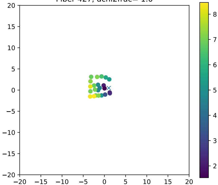
Fiber 427, dchi2frac= 1.0
