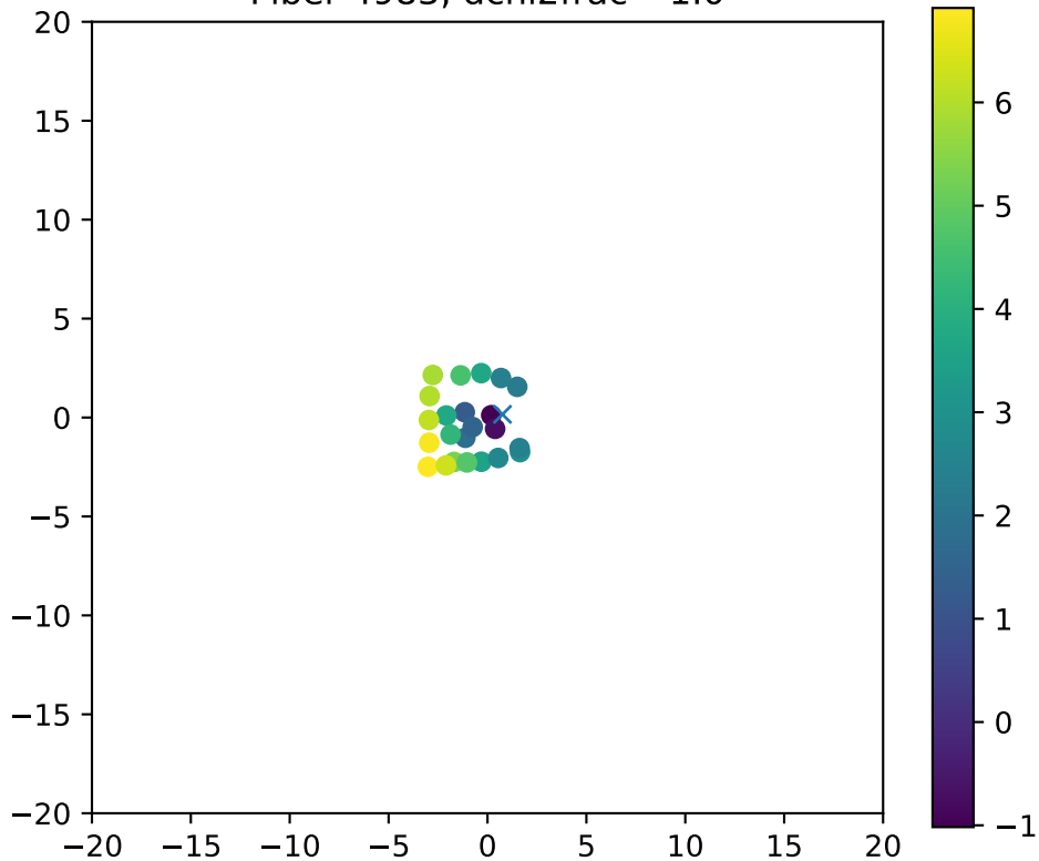
Fiber 4983, dchi2frac= 1.0
