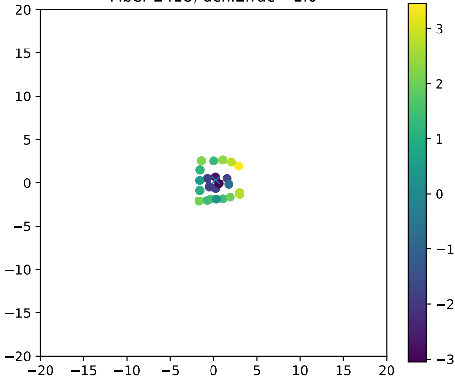
Fiber 2418, dchi2frac= 1.0
