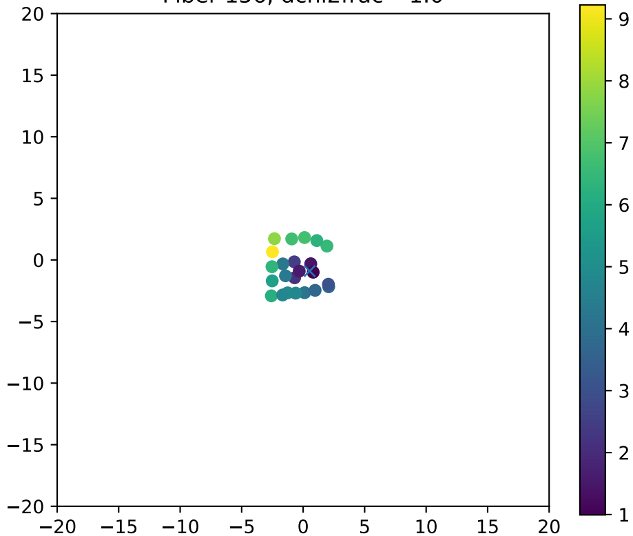
Fiber 156, dchi2frac= 1.0
