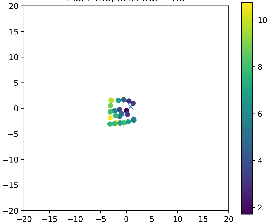
Fiber 130, dchi2frac= 1.0
