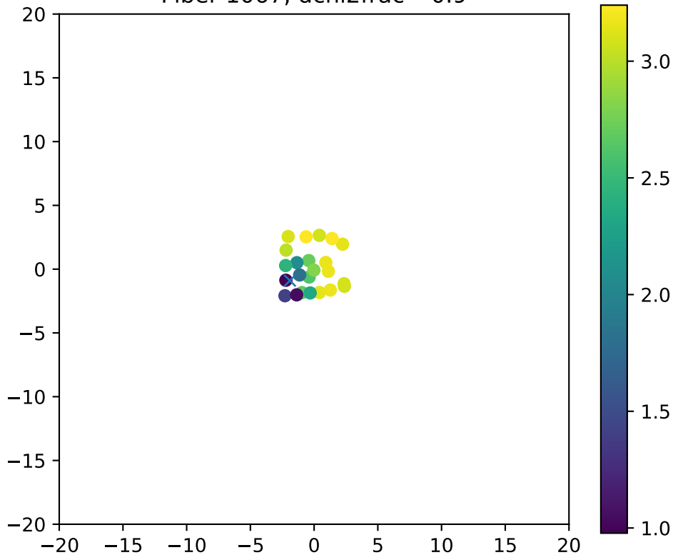
Fiber 1067, dchi2frac= 0.9
