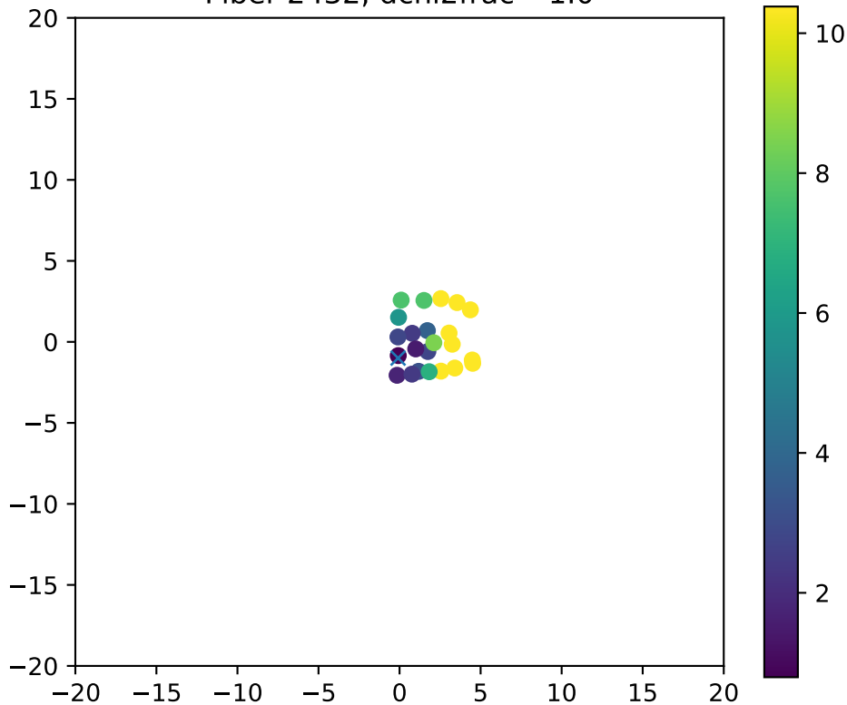
Fiber 2432, dchi2frac= 1.0
