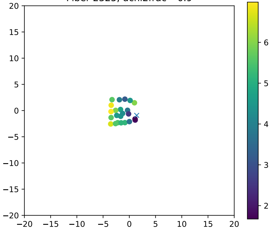
Fiber 2325, dchi2frac= 0.9
