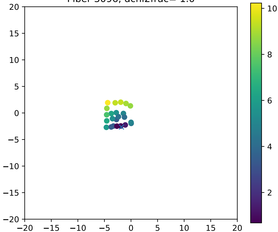
Fiber 3096, dchi2frac= 1.0
