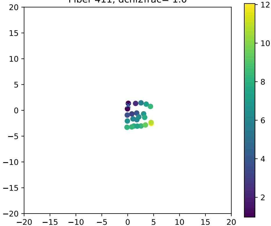
Fiber 411, dchi2frac= 1.0
