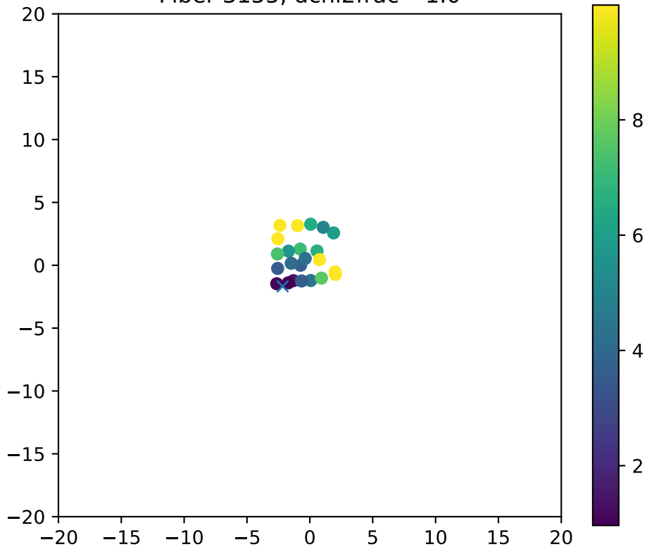
Fiber 3155, dchi2frac= 1.0
