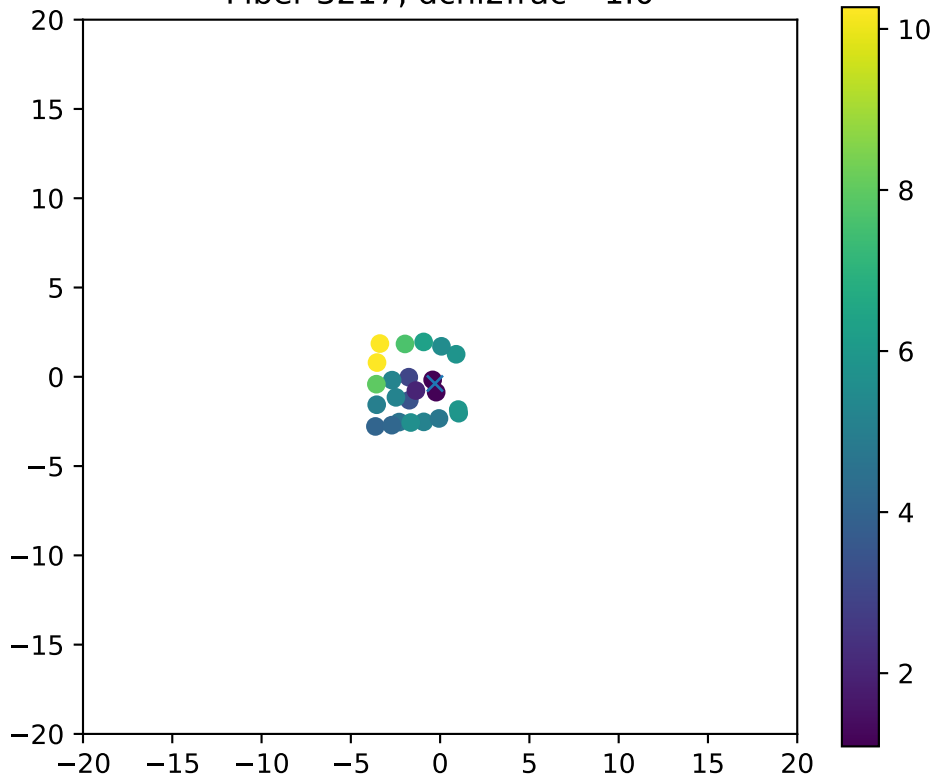
Fiber 3217, dchi2frac= 1.0
