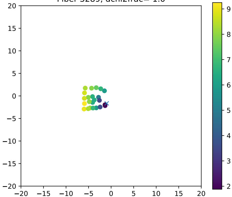
Fiber 3289, dchi2frac= 1.0
