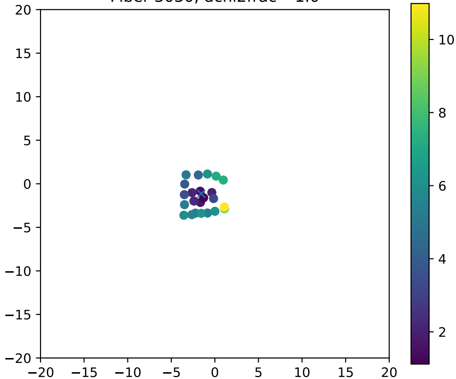
Fiber 3030, dchi2frac= 1.0
