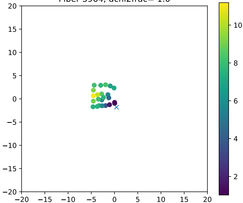
Fiber 3964, dchi2frac= 1.0
