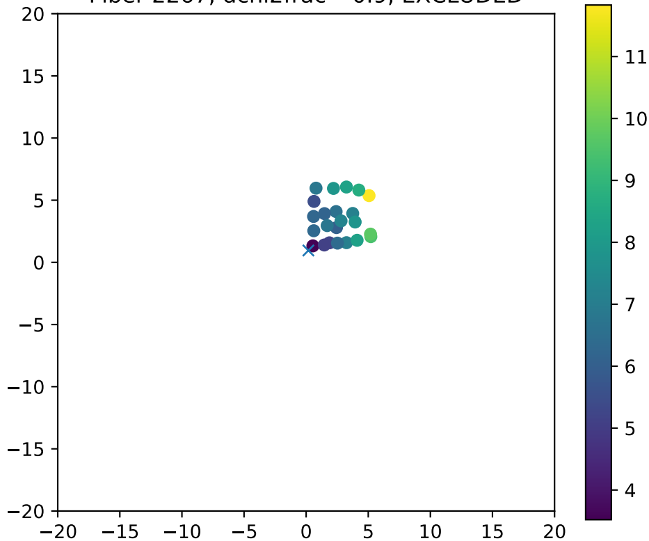
Fiber 2267, dchi2frac= 0.9, EXCLUDED
