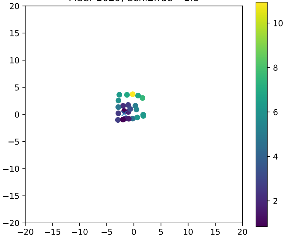
Fiber 1629, dchi2frac= 1.0
