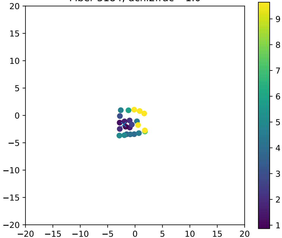
Fiber 3184, dchi2frac= 1.0
