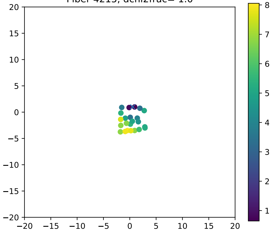
Fiber 4215, dchi2frac= 1.0
