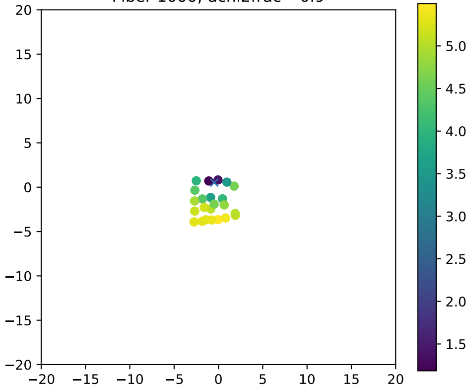
Fiber 1000, dchi2frac= 0.9
