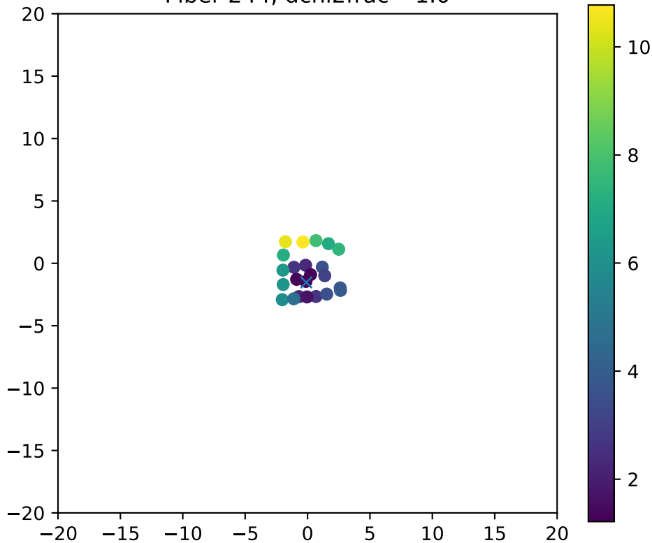
Fiber 244, dchi2frac= 1.0
