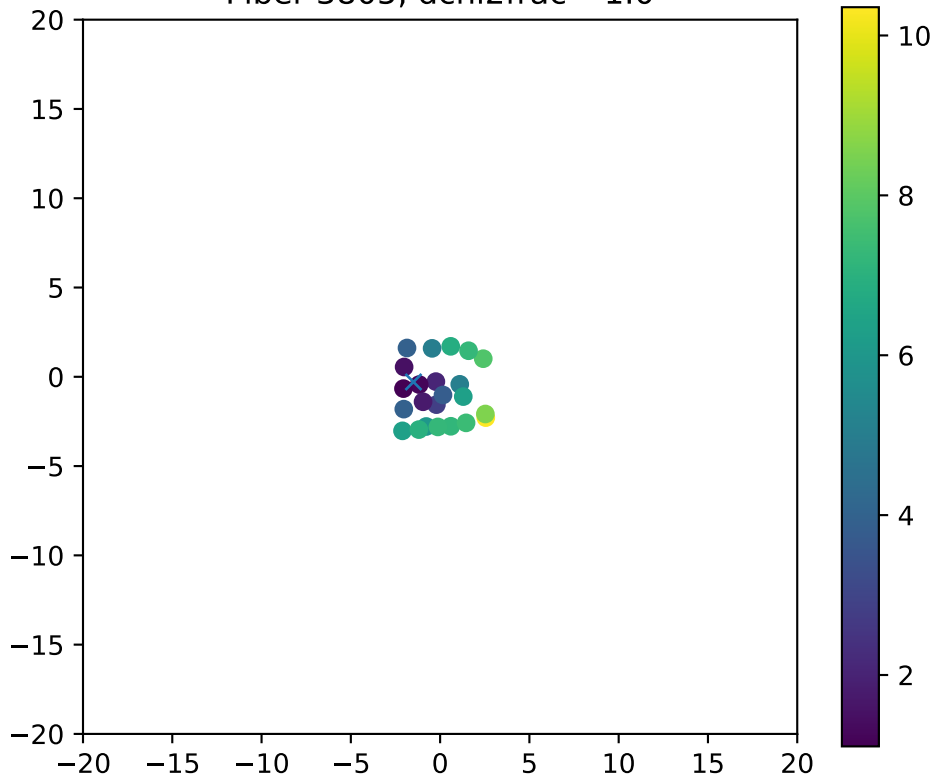
Fiber 3805, dchi2frac= 1.0
