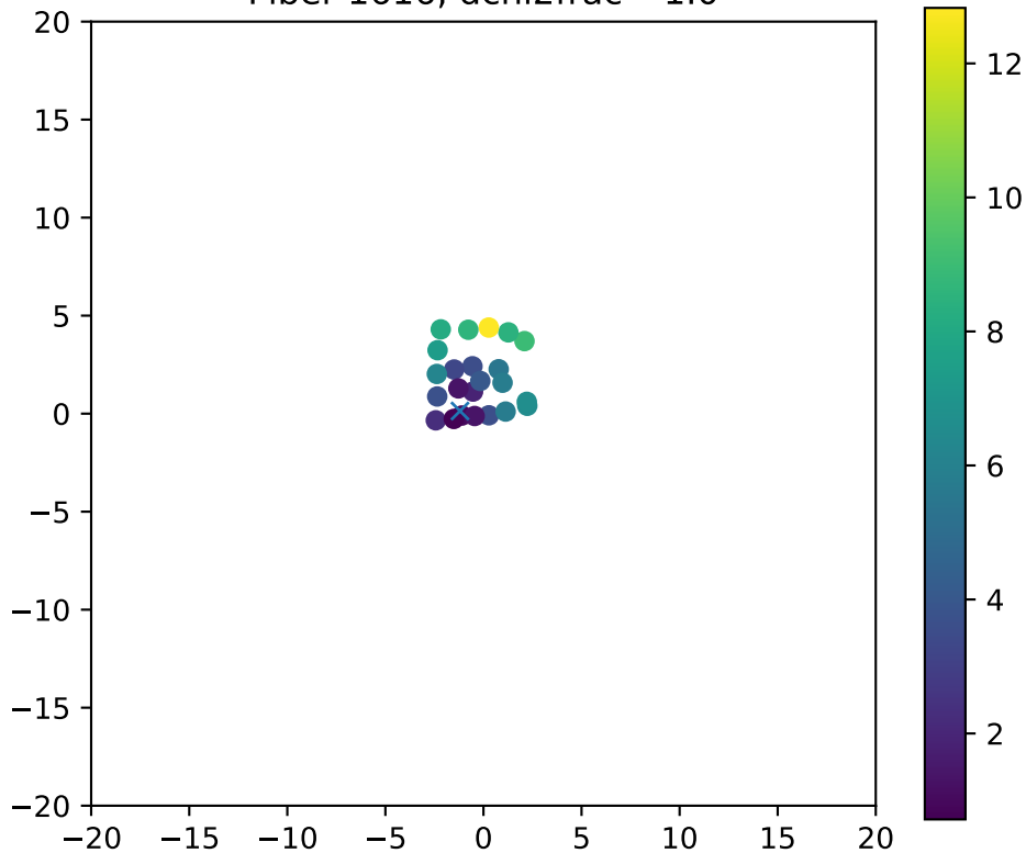
Fiber 1616, dchi2frac= 1.0
