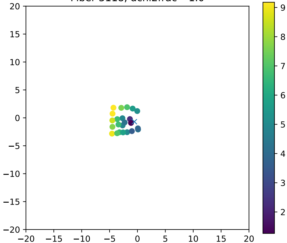
Fiber 3118, dchi2frac= 1.0
