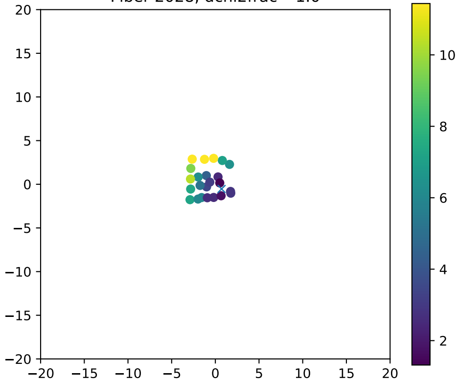
Fiber 2028, dchi2frac= 1.0
