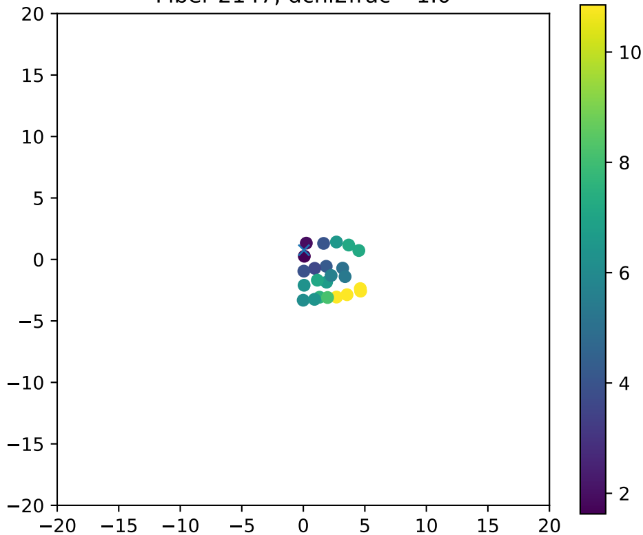
Fiber 2147, dchi2frac= 1.0
