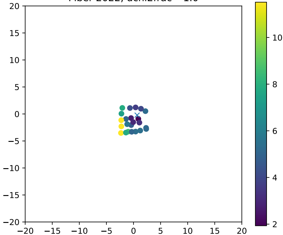
Fiber 2022, dchi2frac= 1.0
