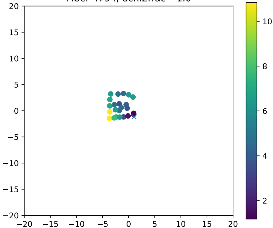
Fiber 4794, dchi2frac= 1.0
