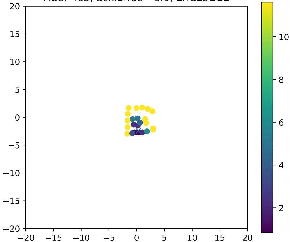
Fiber 465, dchi2frac= 0.9, EXCLUDED
