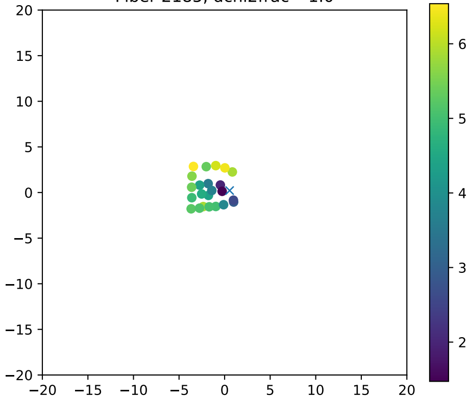
Fiber 2185, dchi2frac= 1.0
