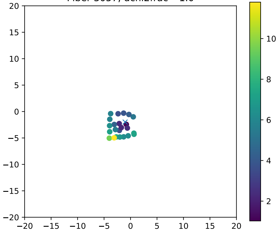
Fiber 3057, dchi2frac= 1.0
