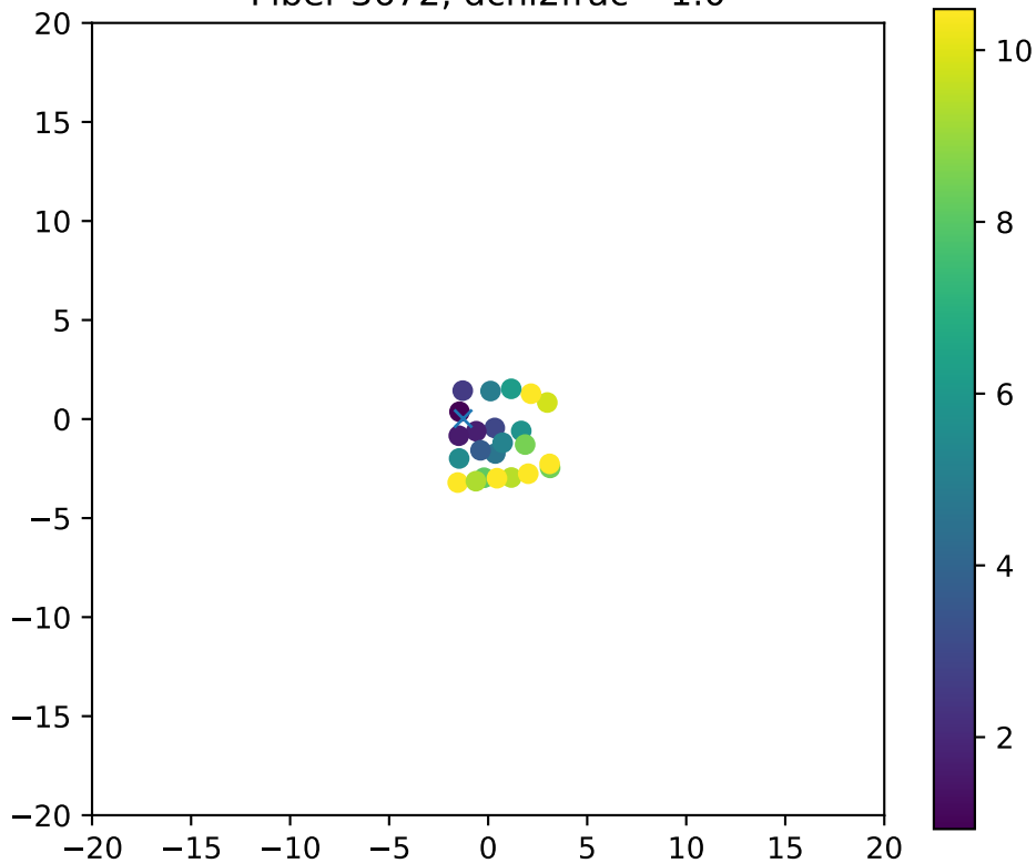
Fiber 3672, dchi2frac= 1.0
