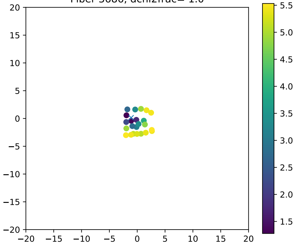
Fiber 3686, dchi2frac= 1.0
