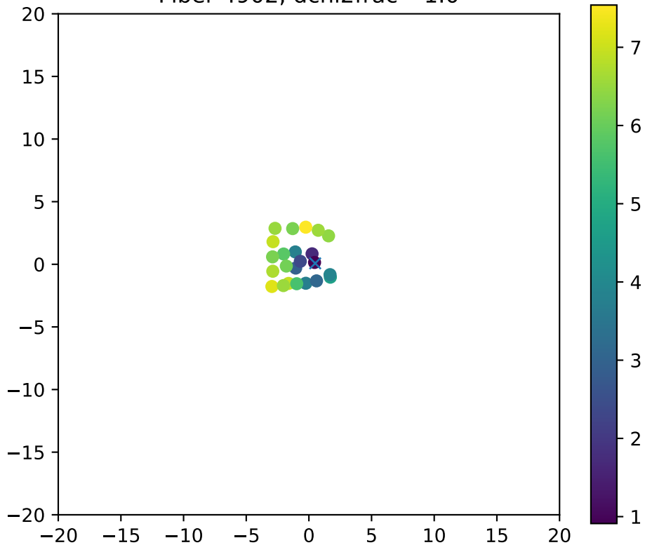
Fiber 4902, dchi2frac= 1.0
