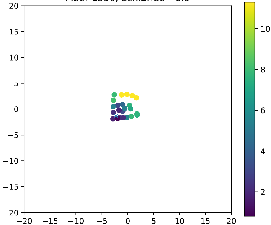
Fiber 1390, dchi2frac= 0.9
