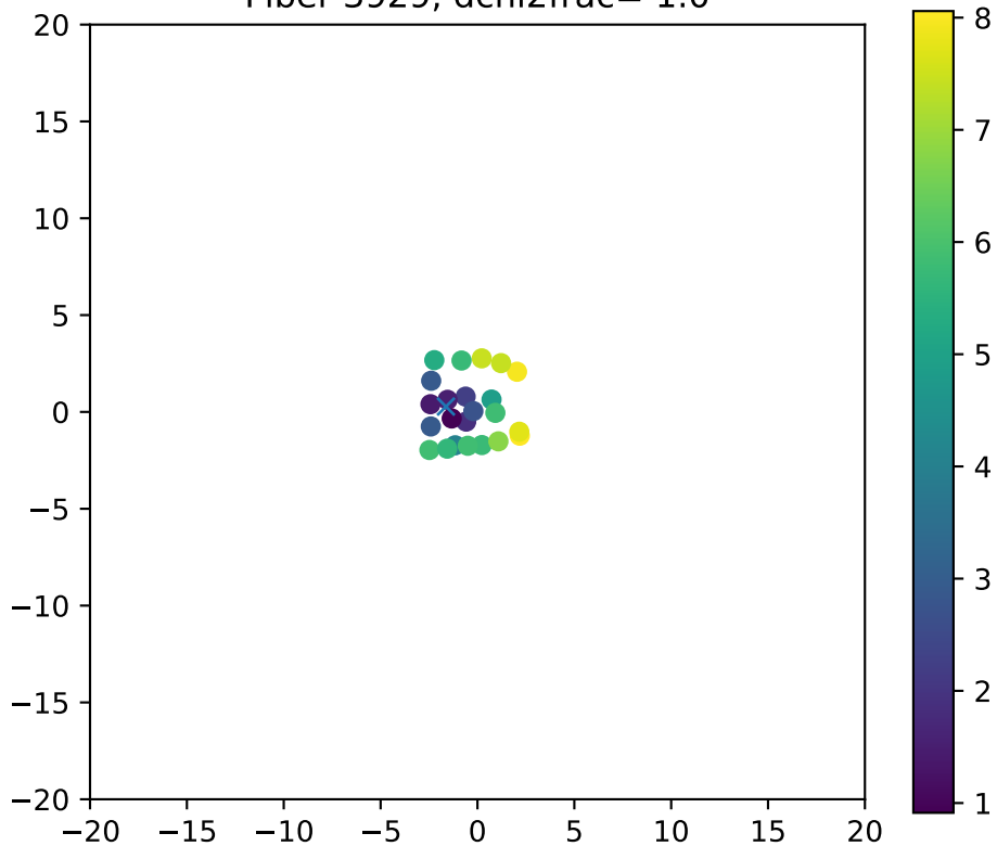
Fiber 3929, dchi2frac= 1.0
