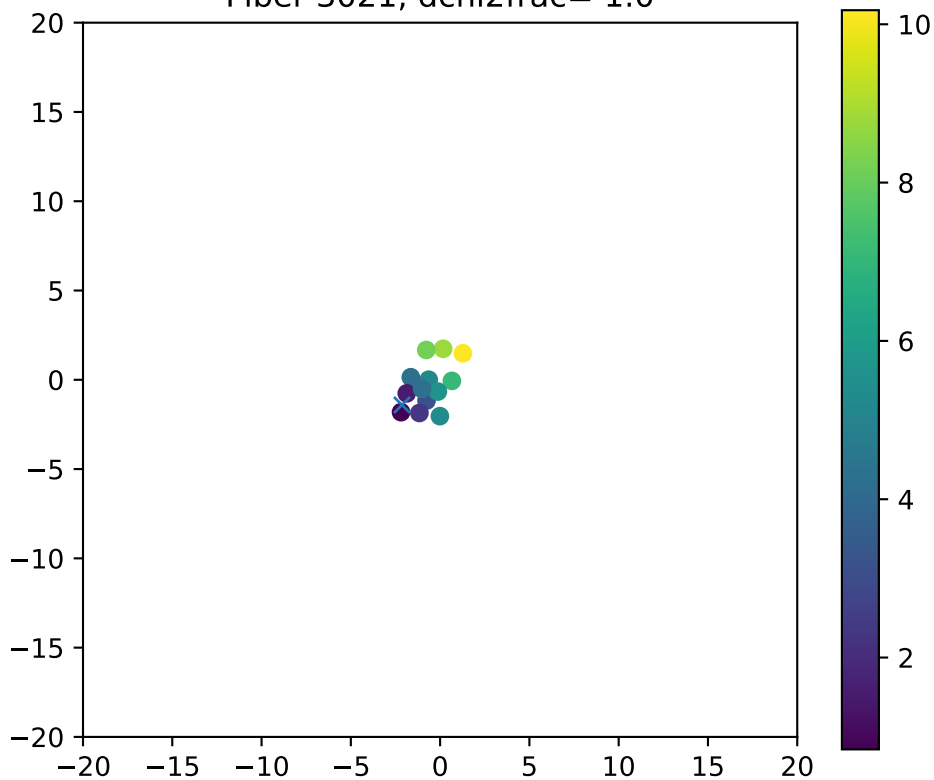
Fiber 3021, dchi2frac= 1.0
