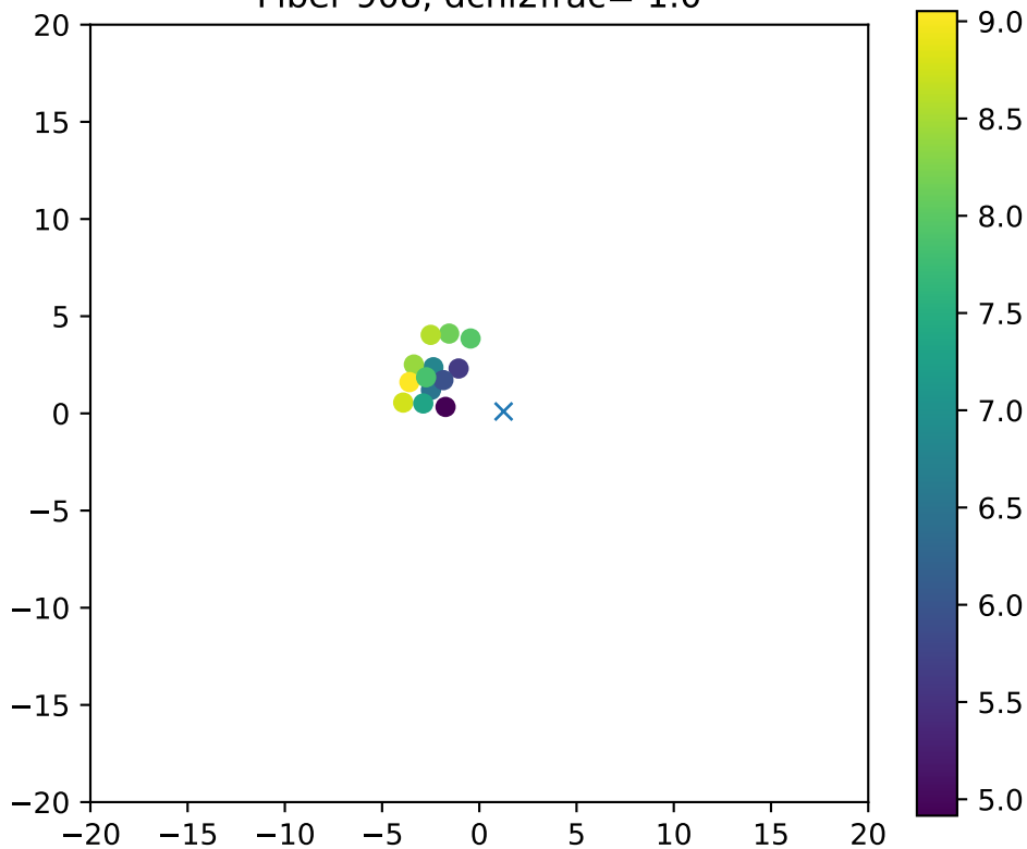
Fiber 908, dchi2frac= 1.0
