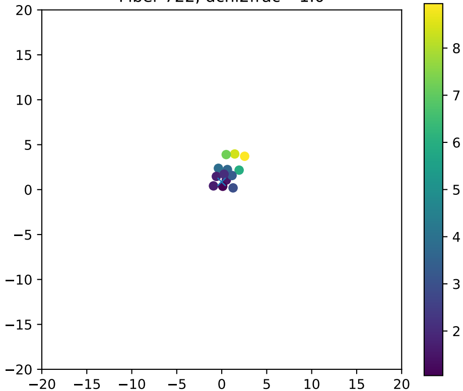
Fiber 722, dchi2frac= 1.0
