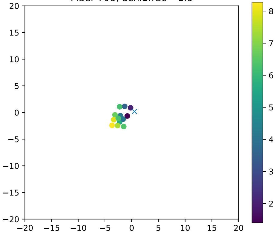
Fiber 790, dchi2frac= 1.0
