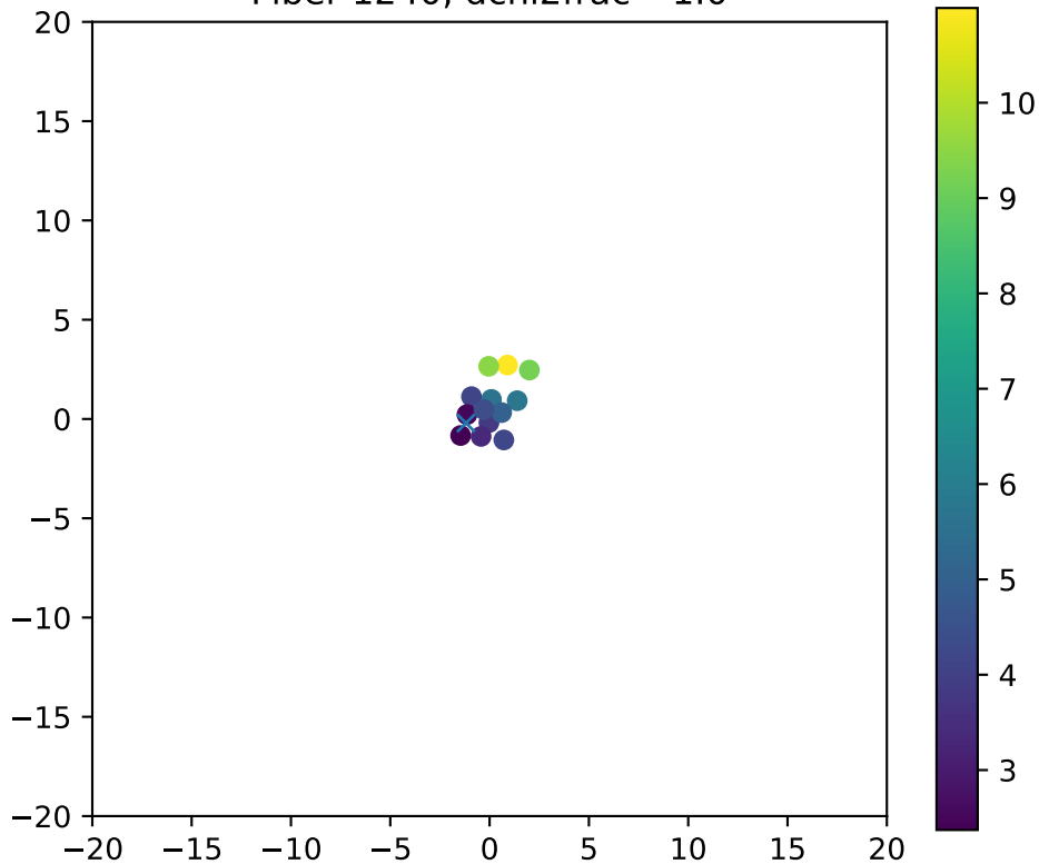
Fiber 1240, dchi2frac= 1.0
