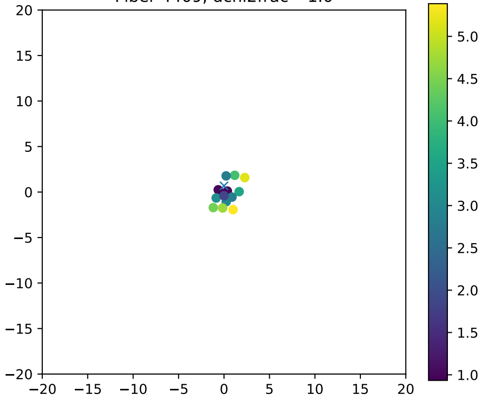
Fiber 4409, dchi2frac= 1.0
