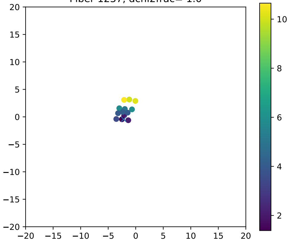
Fiber 1237, dchi2frac= 1.0
