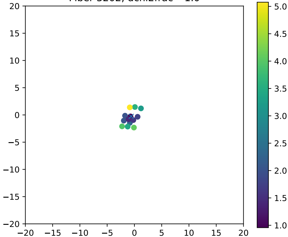
Fiber 3202, dchi2frac= 1.0
