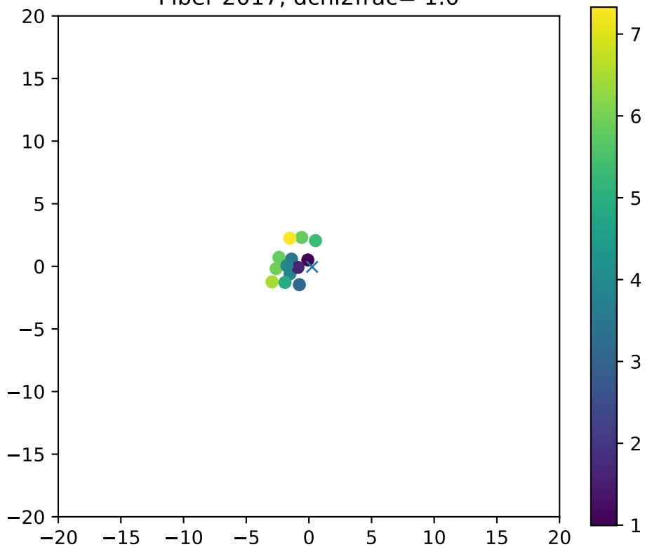
Fiber 2017, dchi2frac= 1.0
