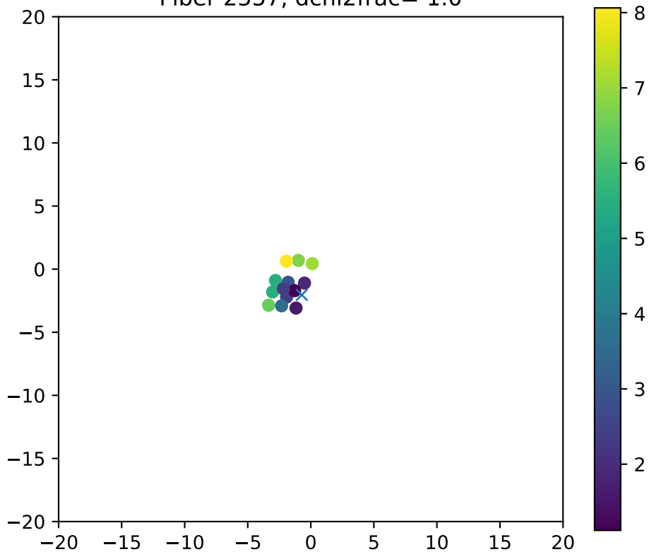
Fiber 2557, dchi2frac= 1.0
