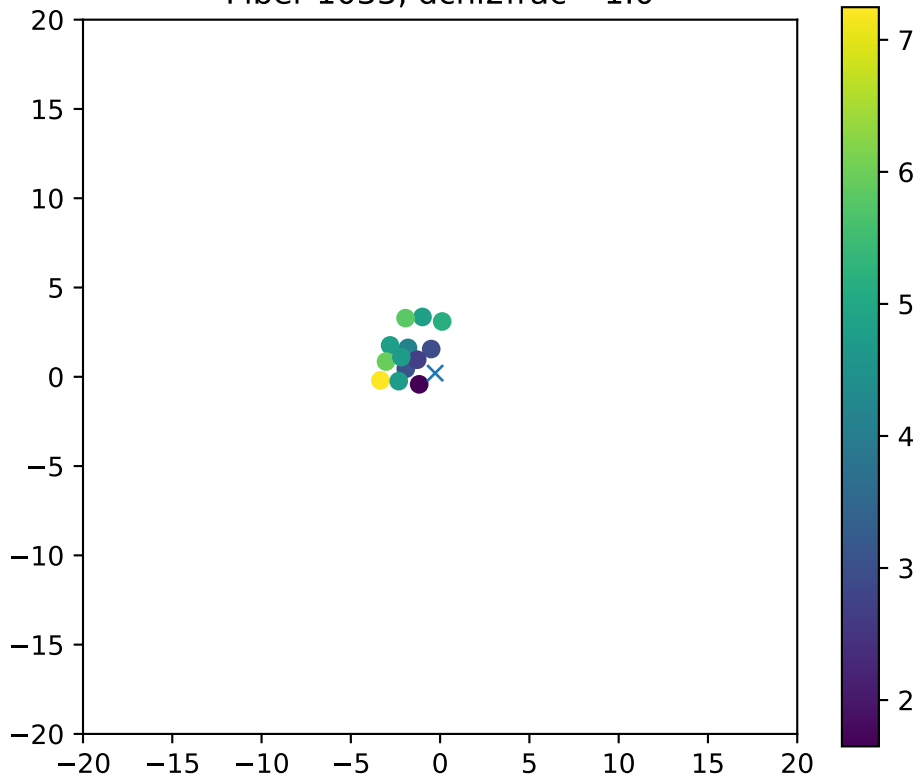
Fiber 1033, dchi2frac= 1.0
