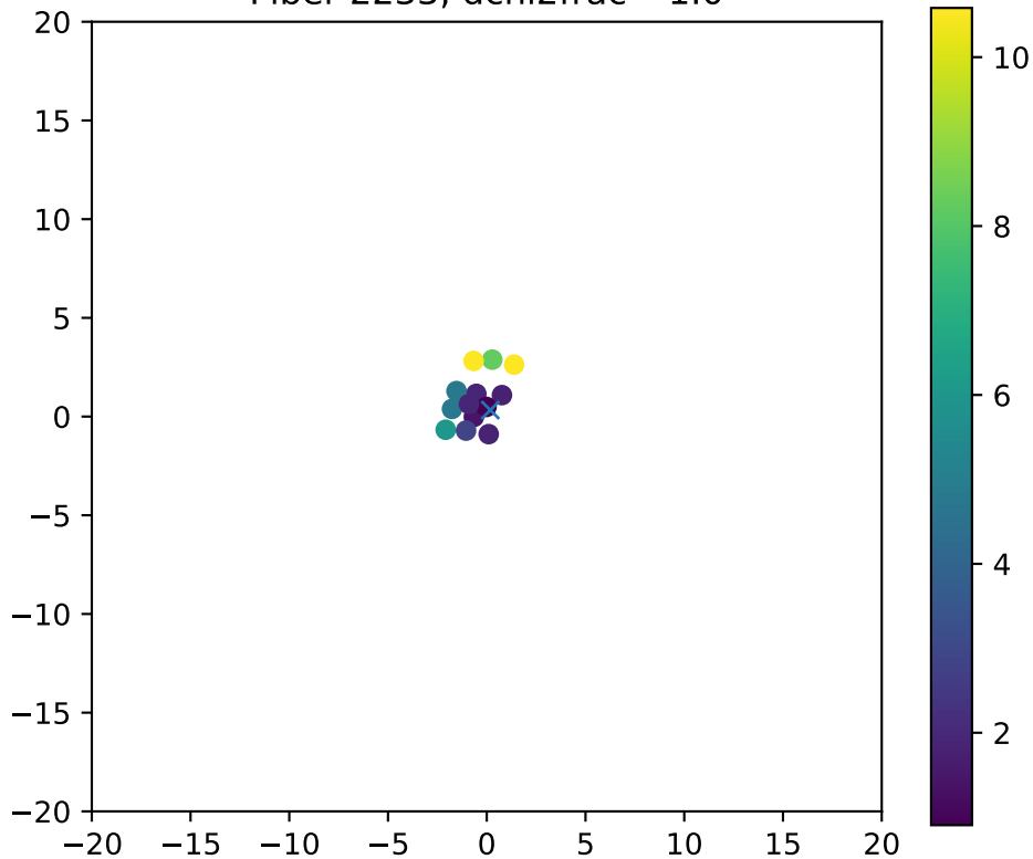
Fiber 2233, dchi2frac= 1.0
