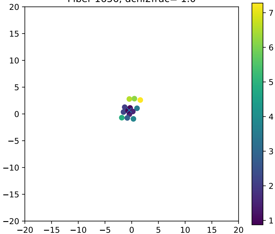
Fiber 1656, dchi2frac= 1.0
