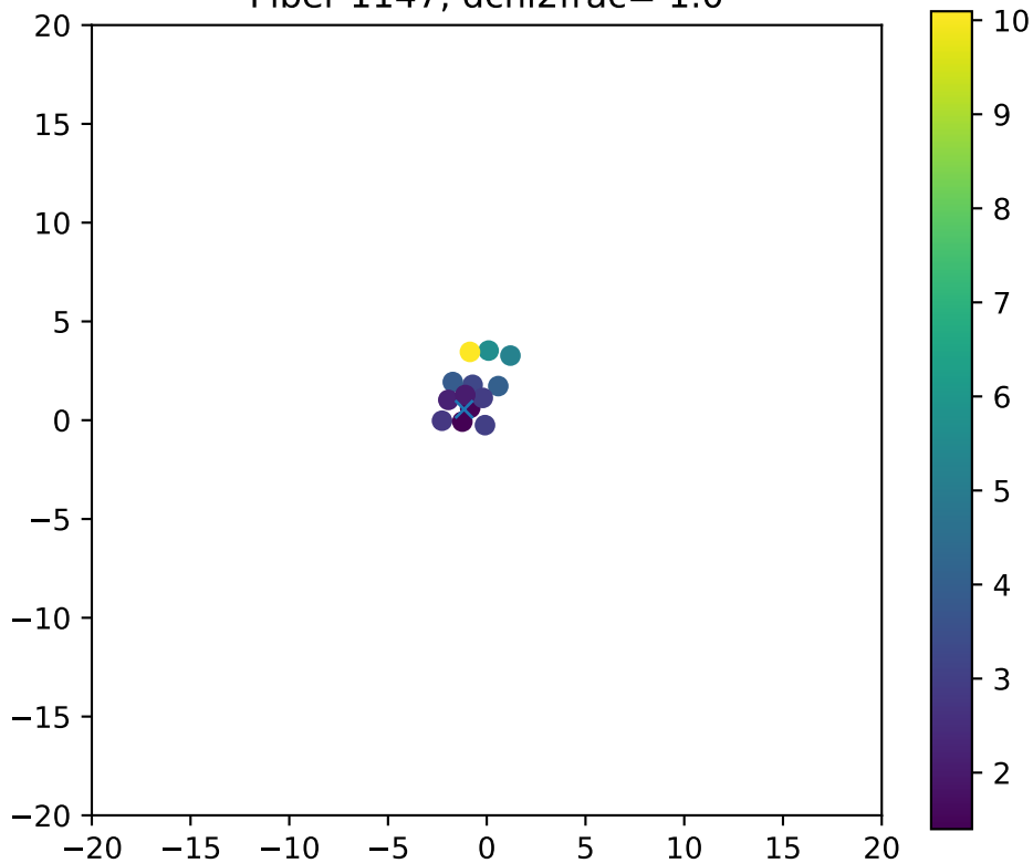
Fiber 1147, dchi2frac= 1.0
