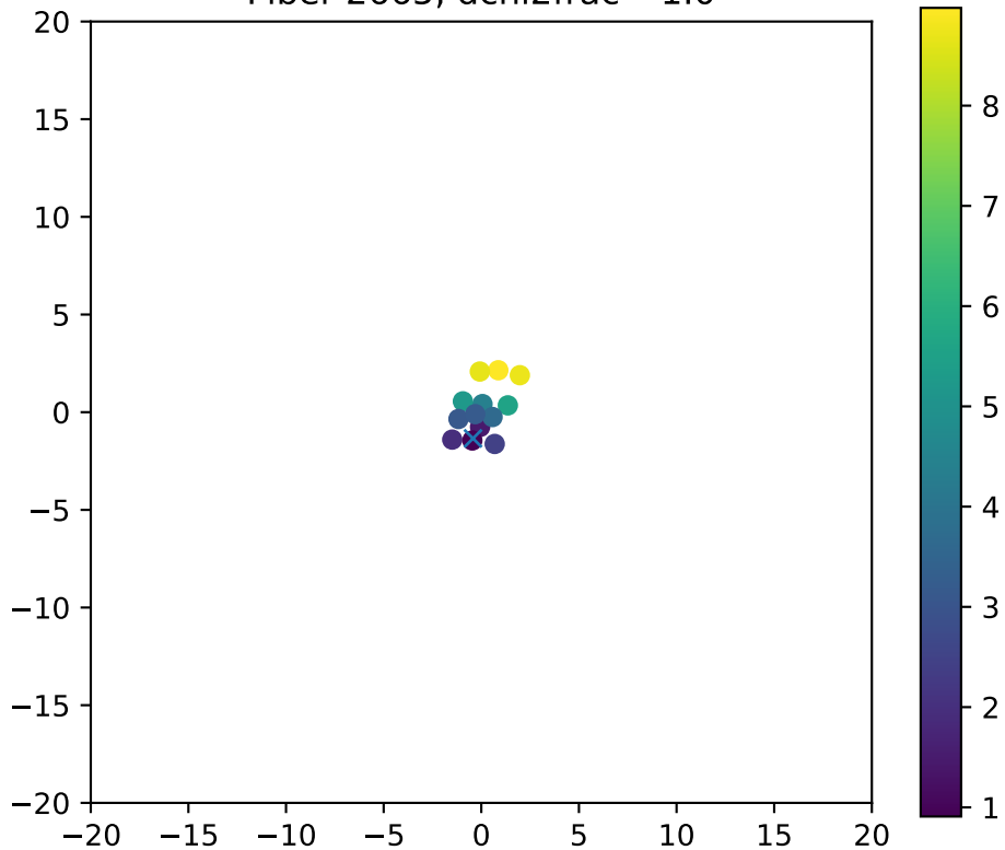
Fiber 2665, dchi2frac= 1.0
