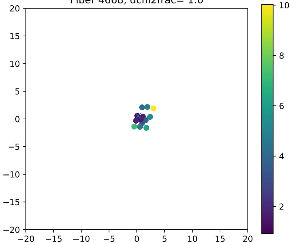
Fiber 4668, dchi2frac= 1.0
