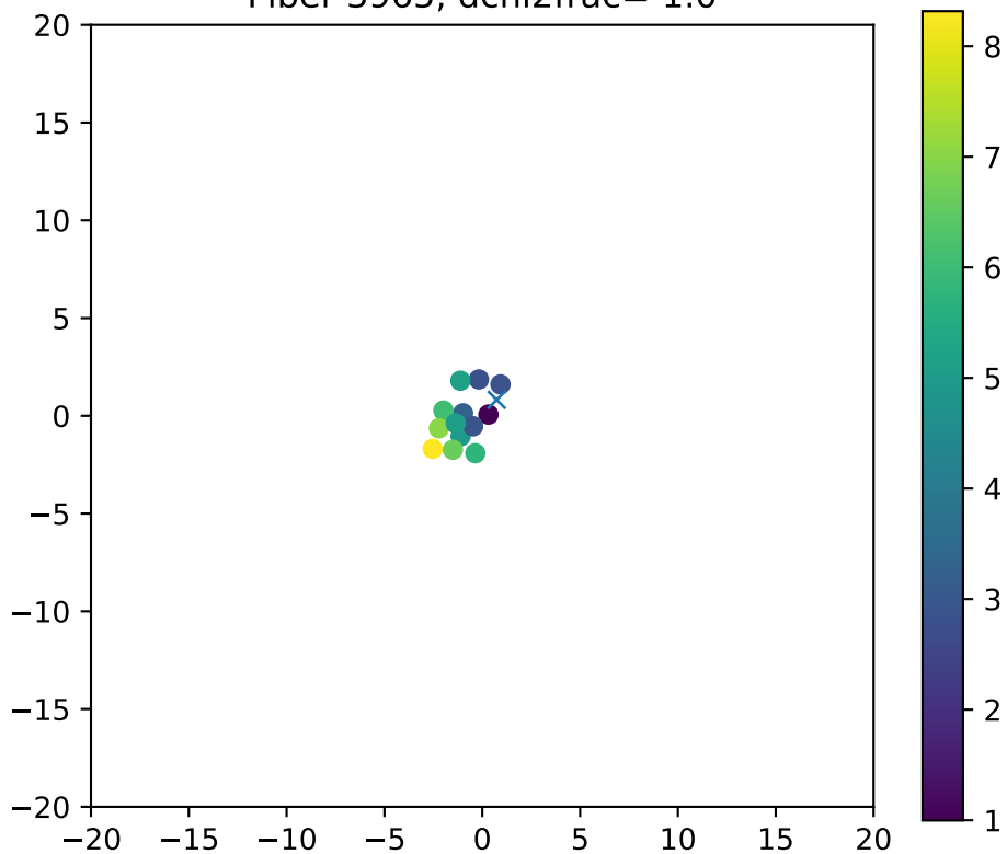
Fiber 3965, dchi2frac= 1.0
