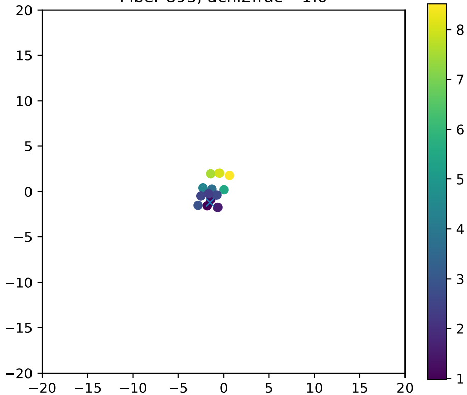
Fiber 893, dchi2frac= 1.0
