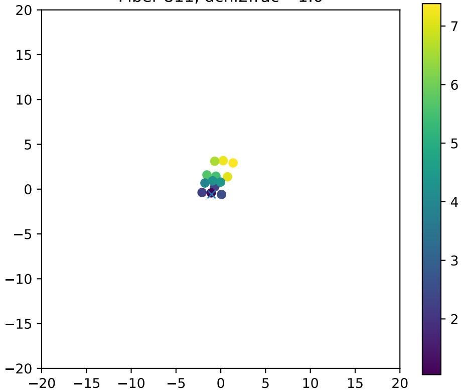
Fiber 811, dchi2frac= 1.0
