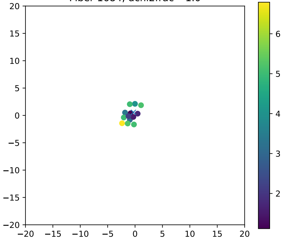
Fiber 1684, dchi2frac= 1.0
