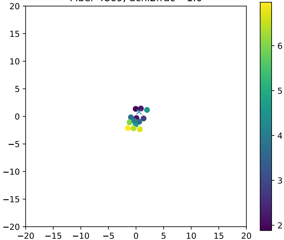
Fiber 4869, dchi2frac= 1.0
