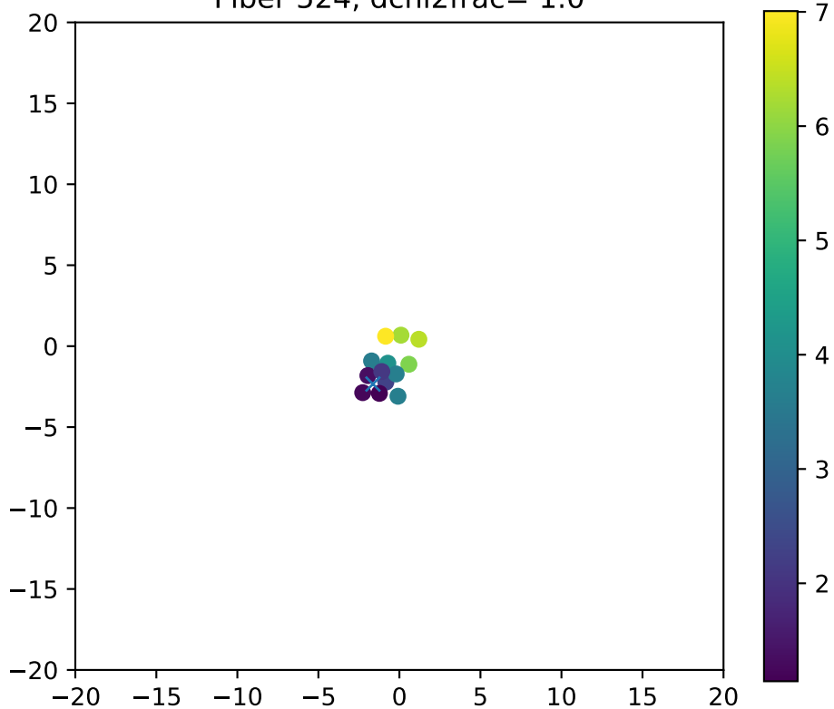
Fiber 524, dchi2frac= 1.0
