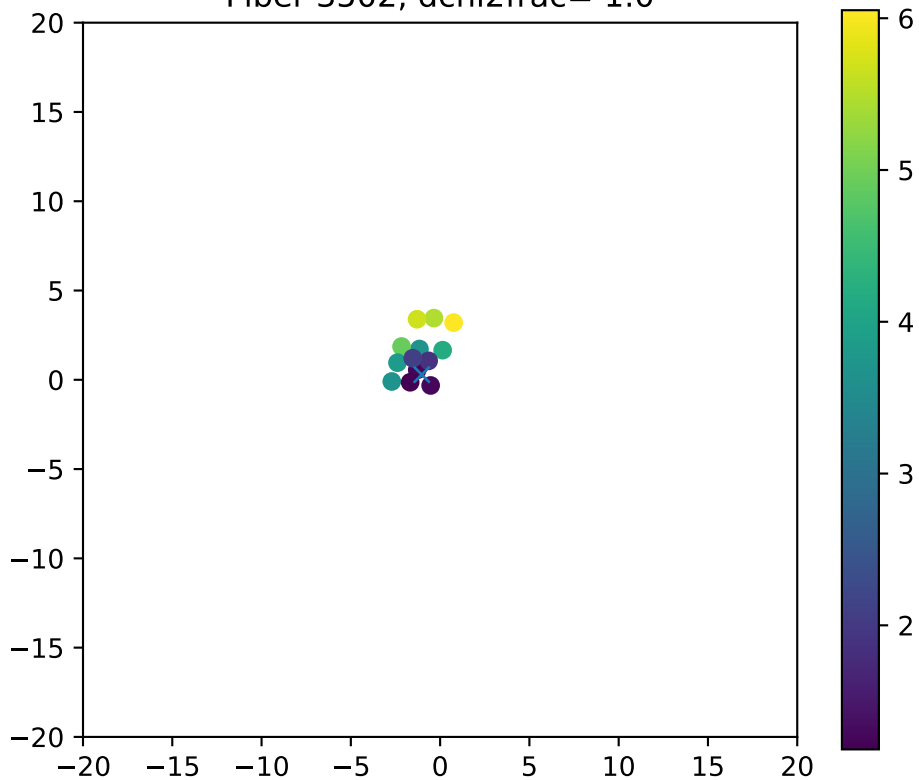
Fiber 3502, dchi2frac= 1.0
