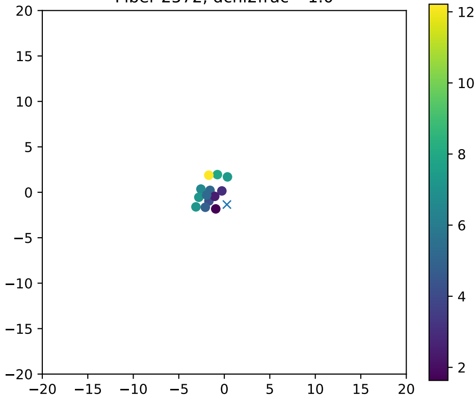
Fiber 2572, dchi2frac= 1.0
