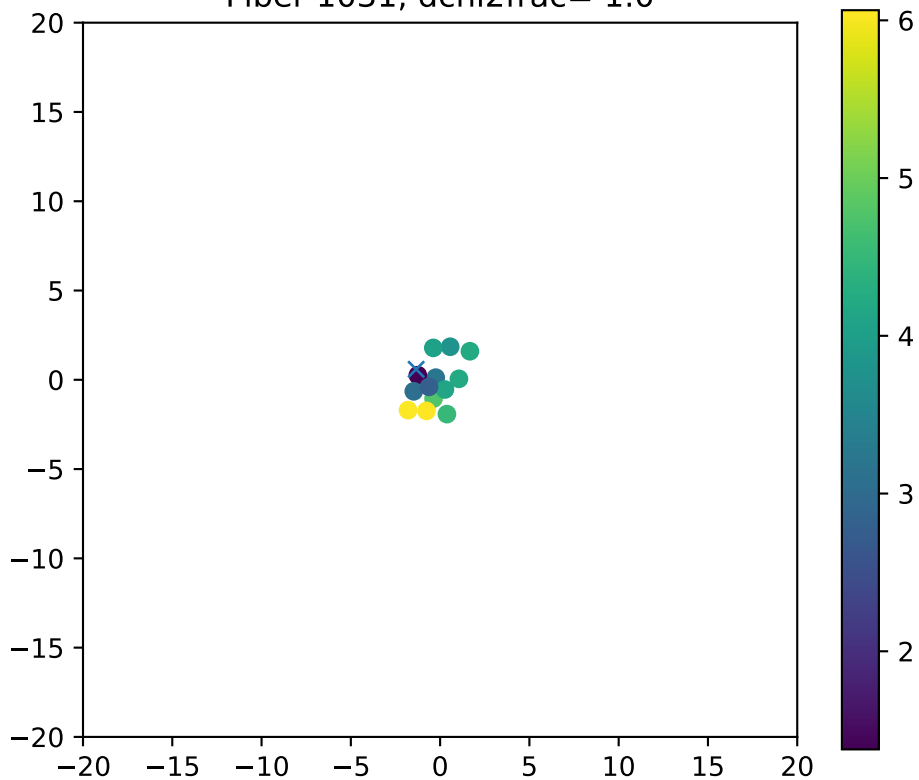
Fiber 1031, dchi2frac= 1.0
