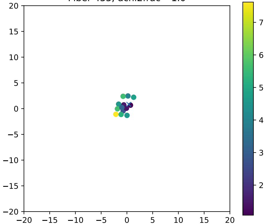
Fiber 433, dchi2frac= 1.0
