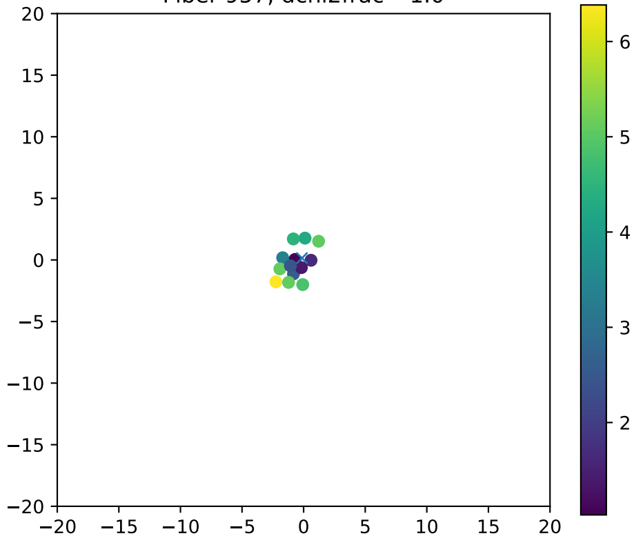
Fiber 957, dchi2frac= 1.0
