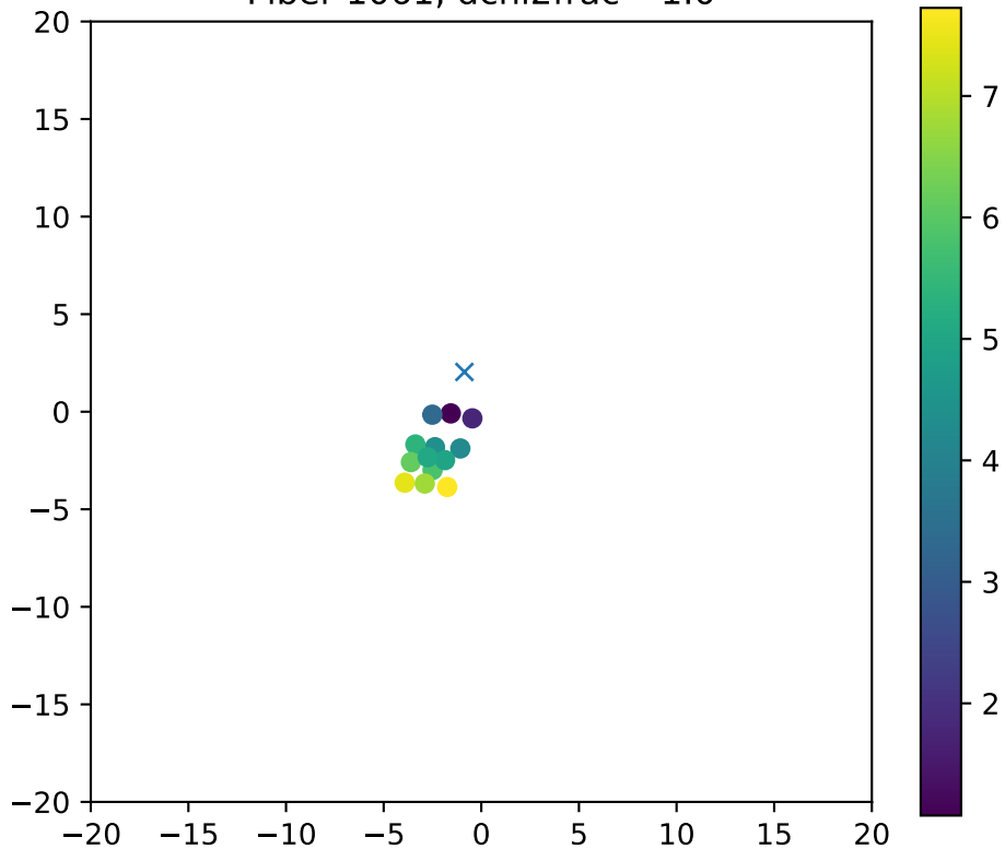
Fiber 1061, dchi2frac= 1.0
