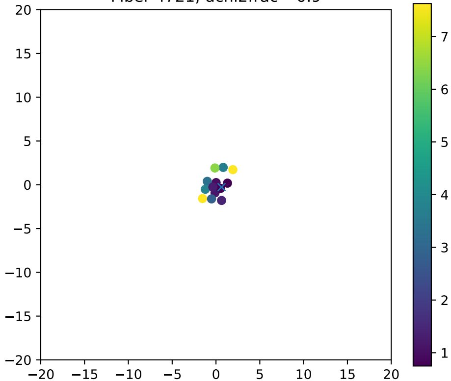
Fiber 4721, dchi2frac= 0.9
