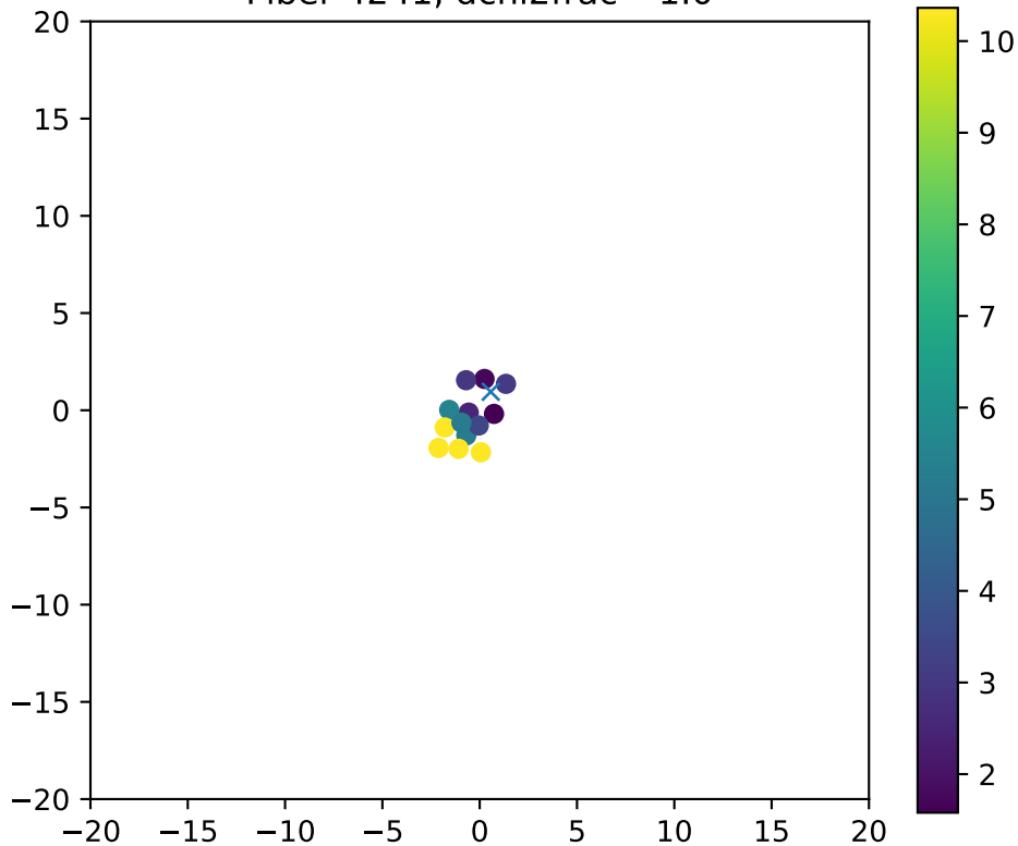
Fiber 4241, dchi2frac= 1.0
