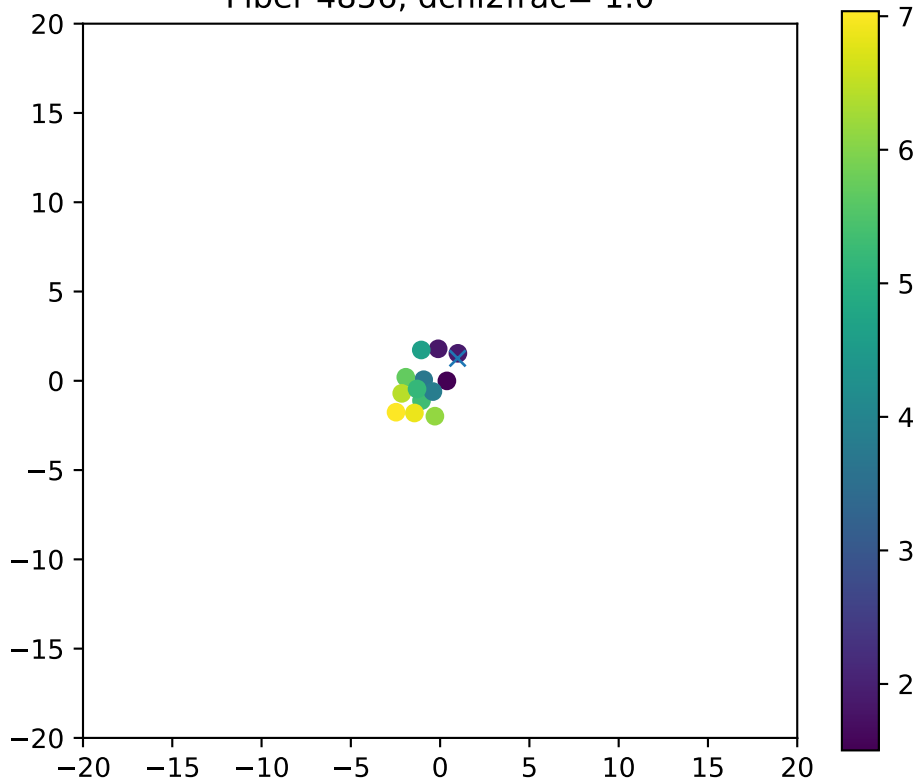
Fiber 4856, dchi2frac= 1.0
