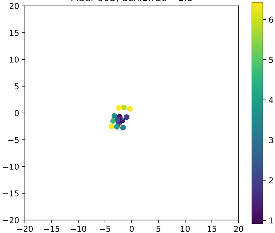
Fiber 995, dchi2frac= 1.0
