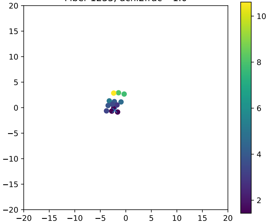
Fiber 1233, dchi2frac= 1.0
