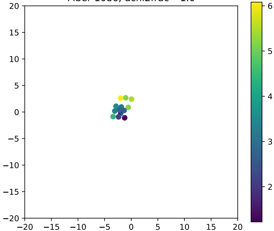
Fiber 1086, dchi2frac= 1.0
