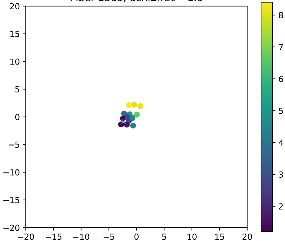
Fiber 1389, dchi2frac= 1.0
