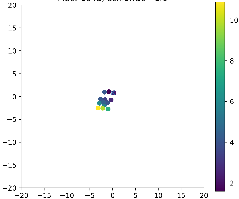
Fiber 1043, dchi2frac= 1.0
