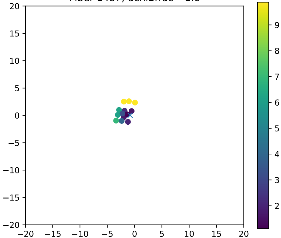
Fiber 1487, dchi2frac= 1.0
