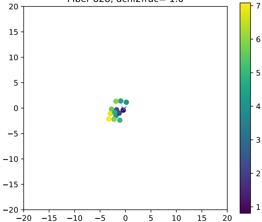
Fiber 828, dchi2frac= 1.0
