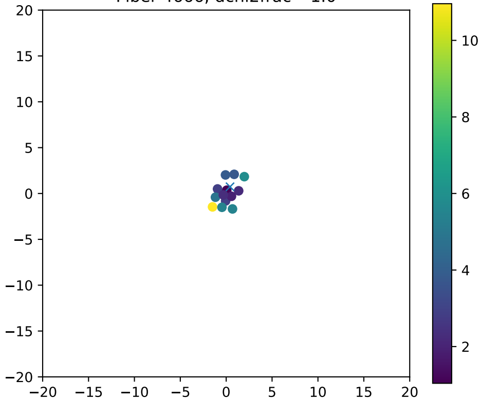
Fiber 4666, dchi2frac= 1.0
