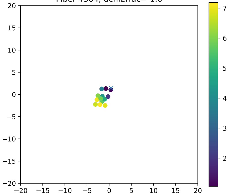
Fiber 4304, dchi2frac= 1.0
