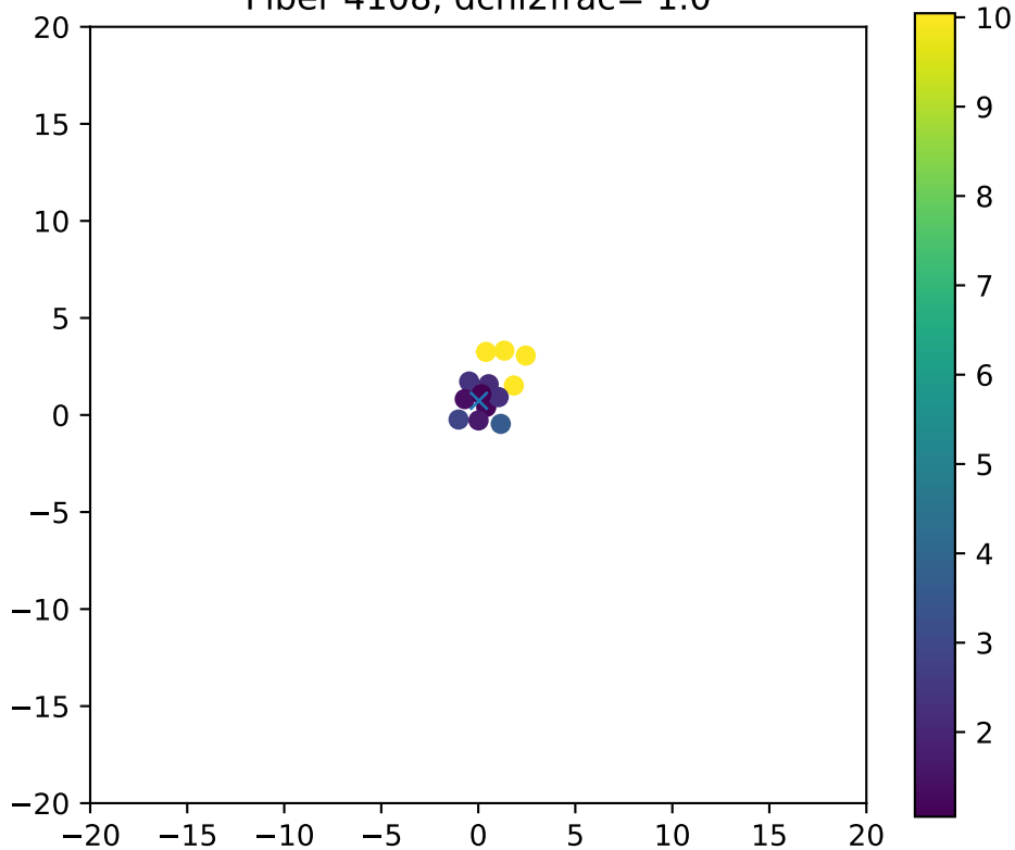
Fiber 4108, dchi2frac= 1.0
