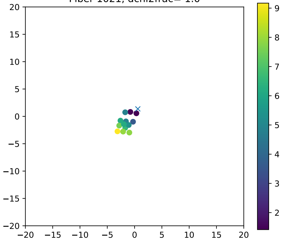
Fiber 1021, dchi2frac= 1.0
