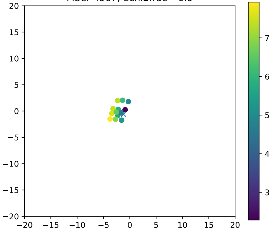
Fiber 4967, dchi2frac= 0.9
