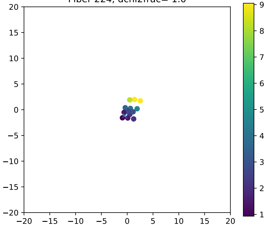
Fiber 224, dchi2frac= 1.0
