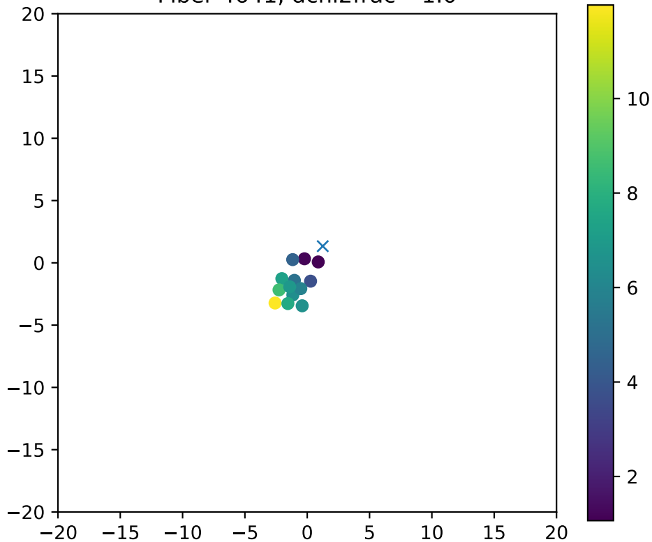
Fiber 4641, dchi2frac= 1.0
