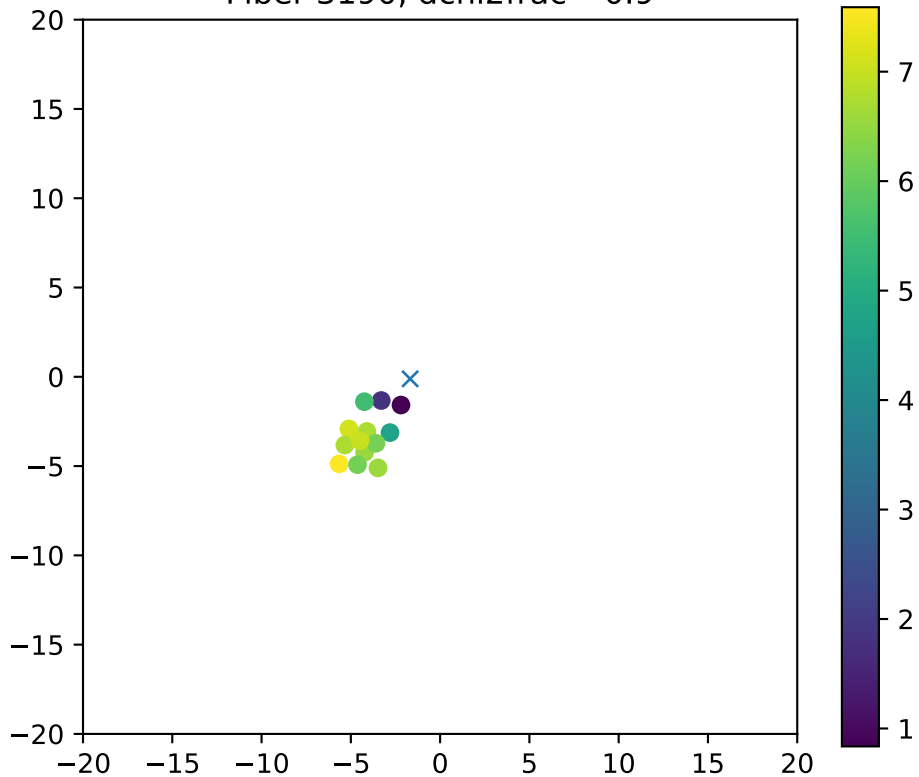
Fiber 3190, dchi2frac= 0.9
