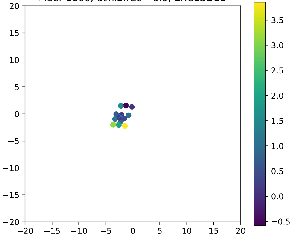
Fiber 1060, dchi2frac= 0.9, EXCLUDED
