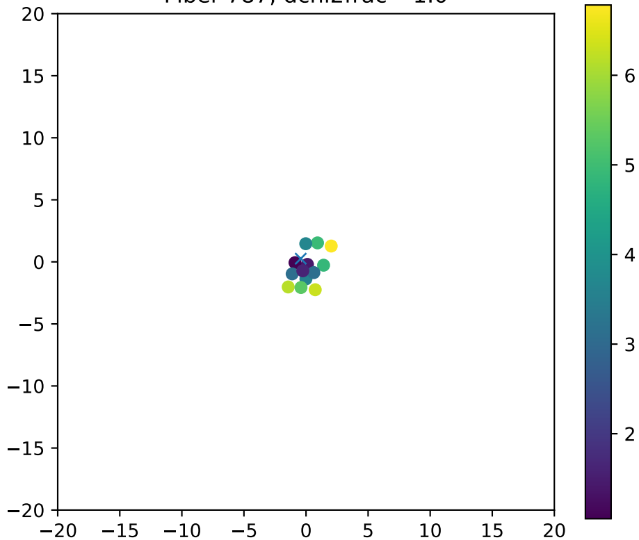
Fiber 787, dchi2frac= 1.0
