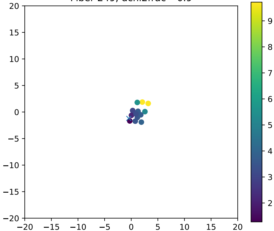
Fiber 249, dchi2frac= 0.9
