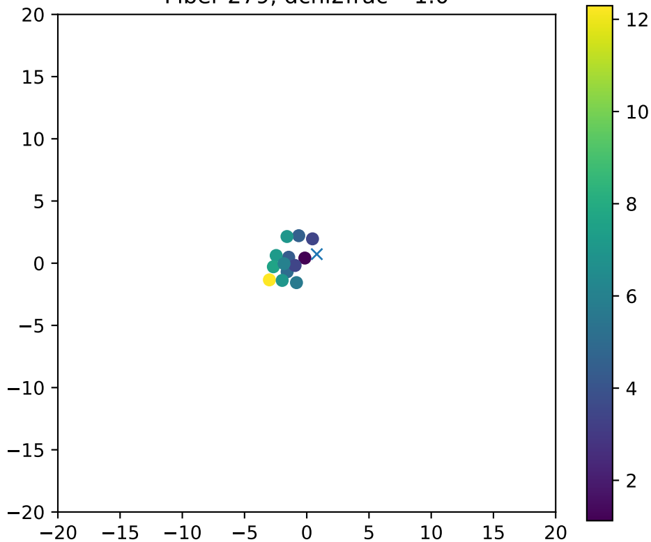
Fiber 279, dchi2frac= 1.0
