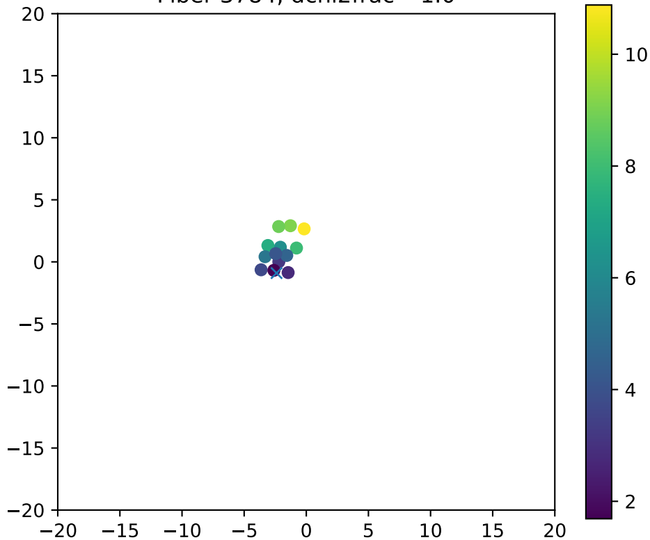
Fiber 3784, dchi2frac= 1.0
