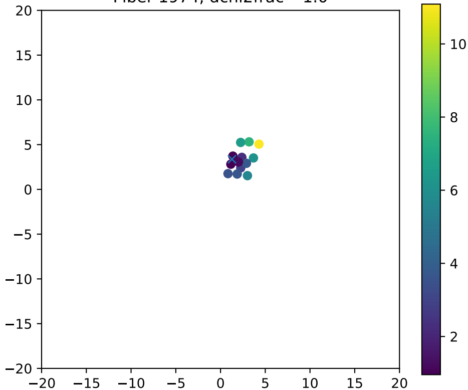
Fiber 1974, dchi2frac= 1.0
