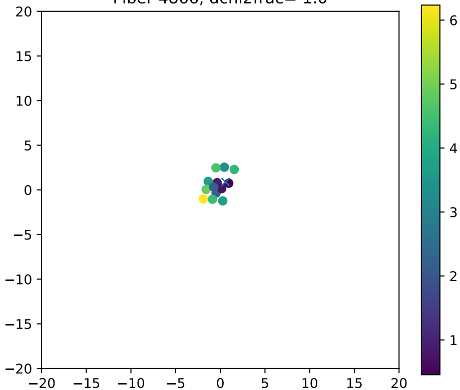
Fiber 4866, dchi2frac= 1.0
