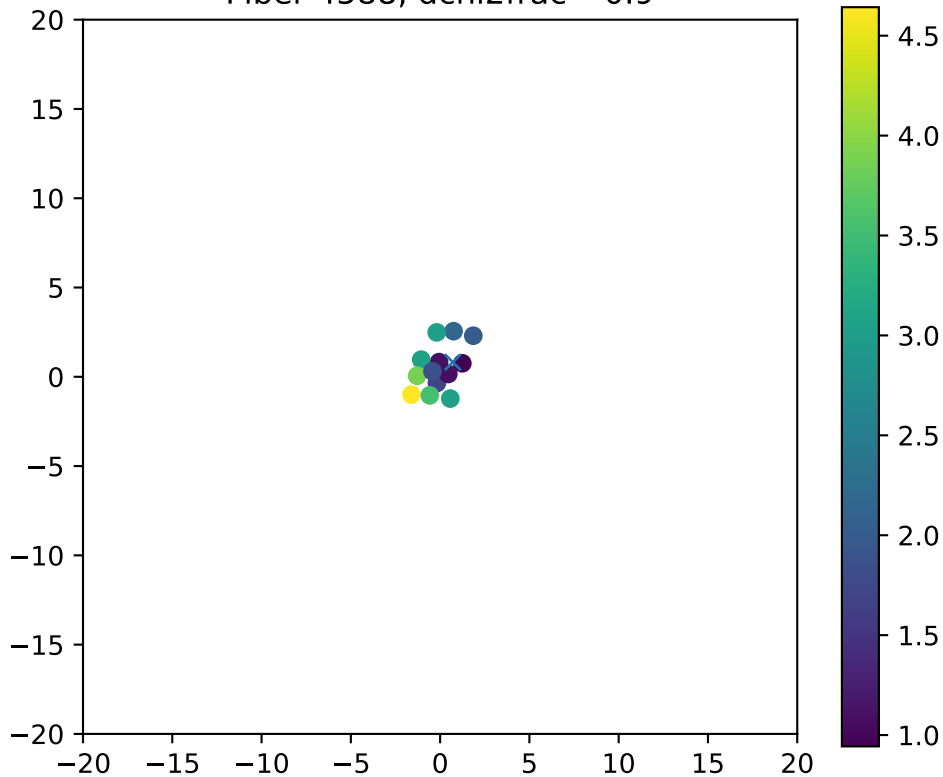
Fiber 4588, dchi2frac= 0.9
