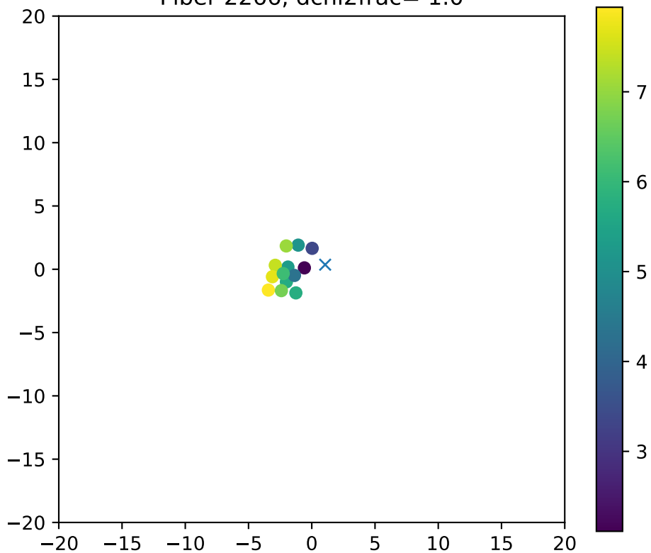
Fiber 2266, dchi2frac= 1.0
