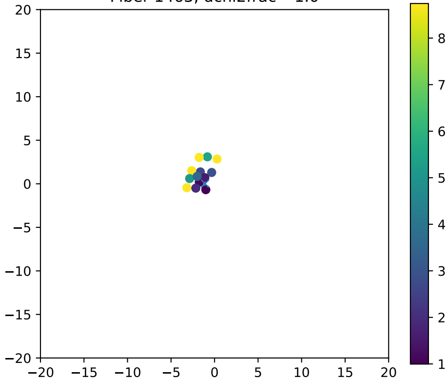
Fiber 1463, dchi2frac= 1.0
