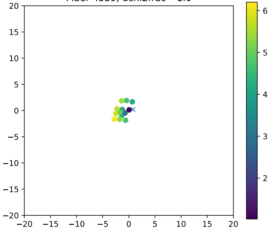
Fiber 4539, dchi2frac= 1.0
