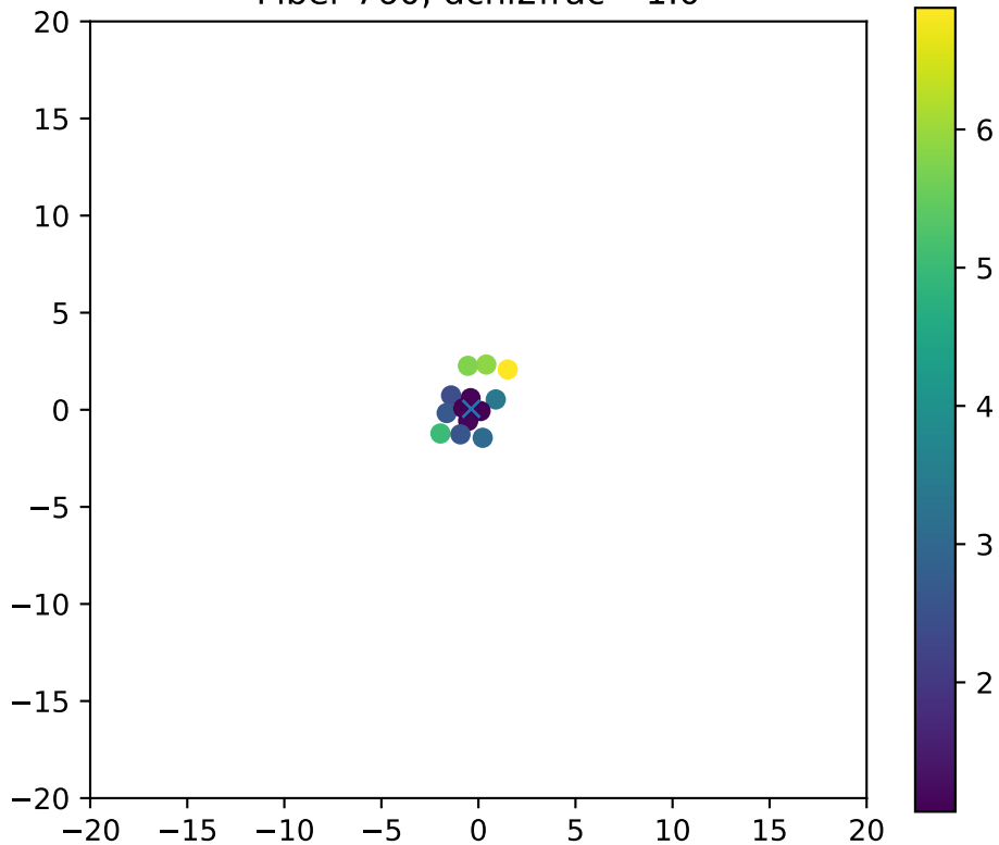
Fiber 760, dchi2frac= 1.0
