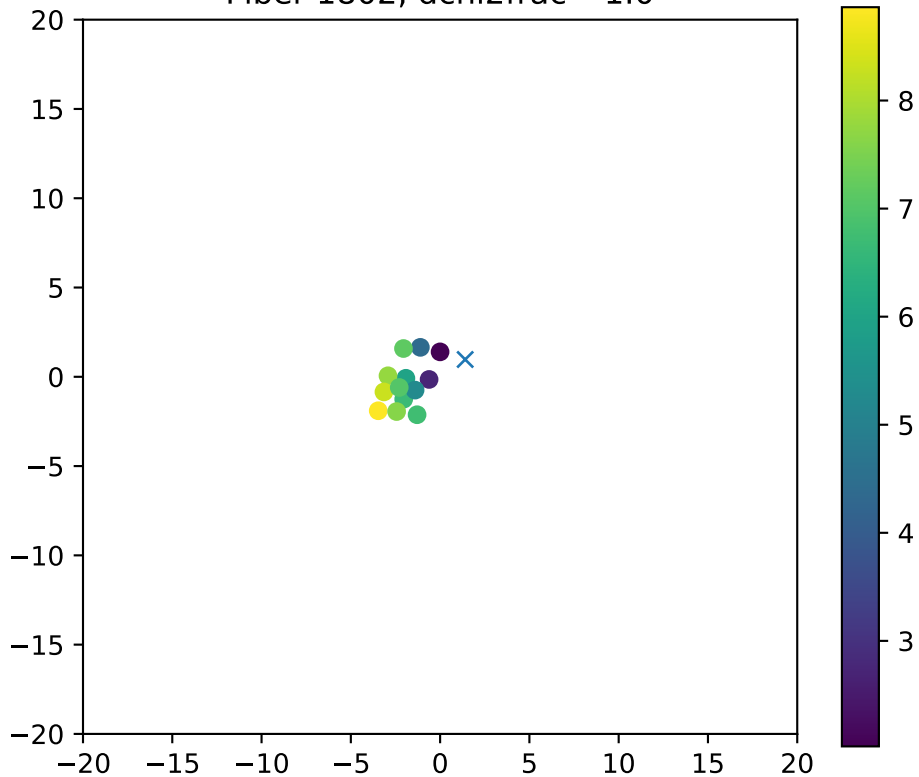
Fiber 1802, dchi2frac= 1.0
