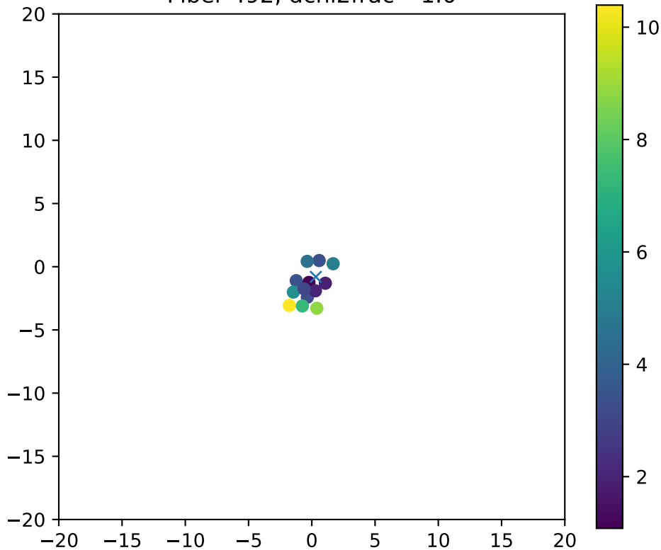
Fiber 492, dchi2frac= 1.0
