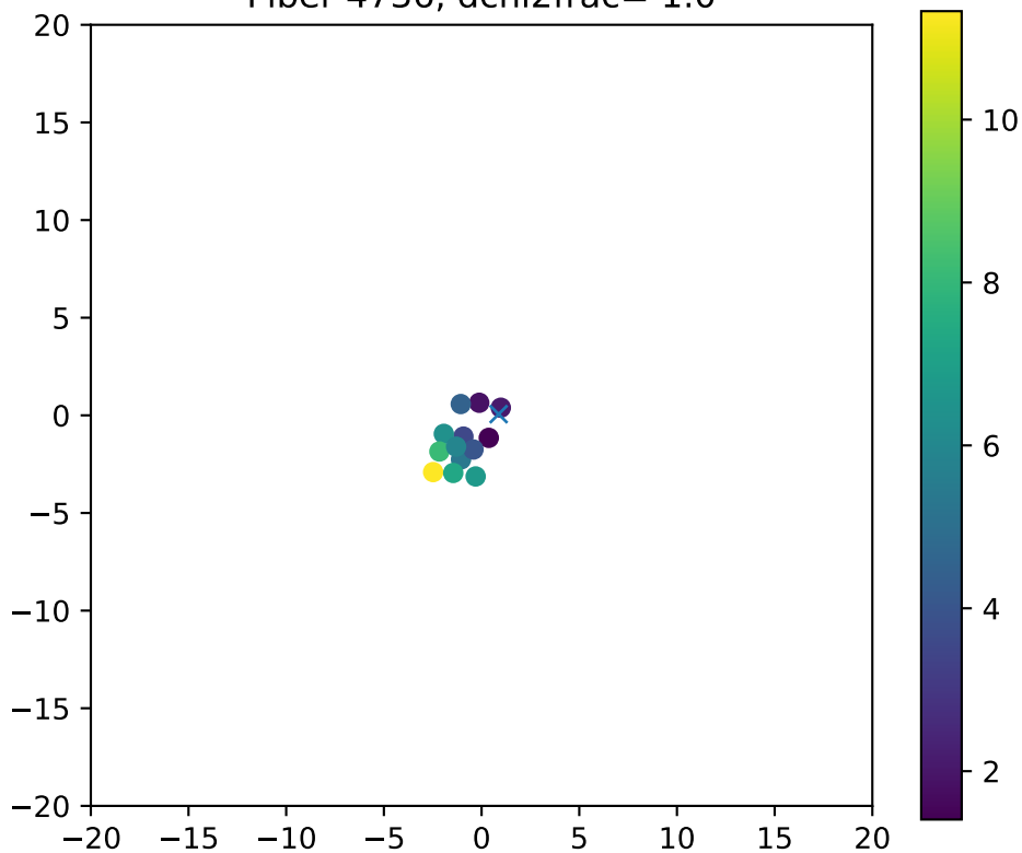
Fiber 4736, dchi2frac= 1.0
