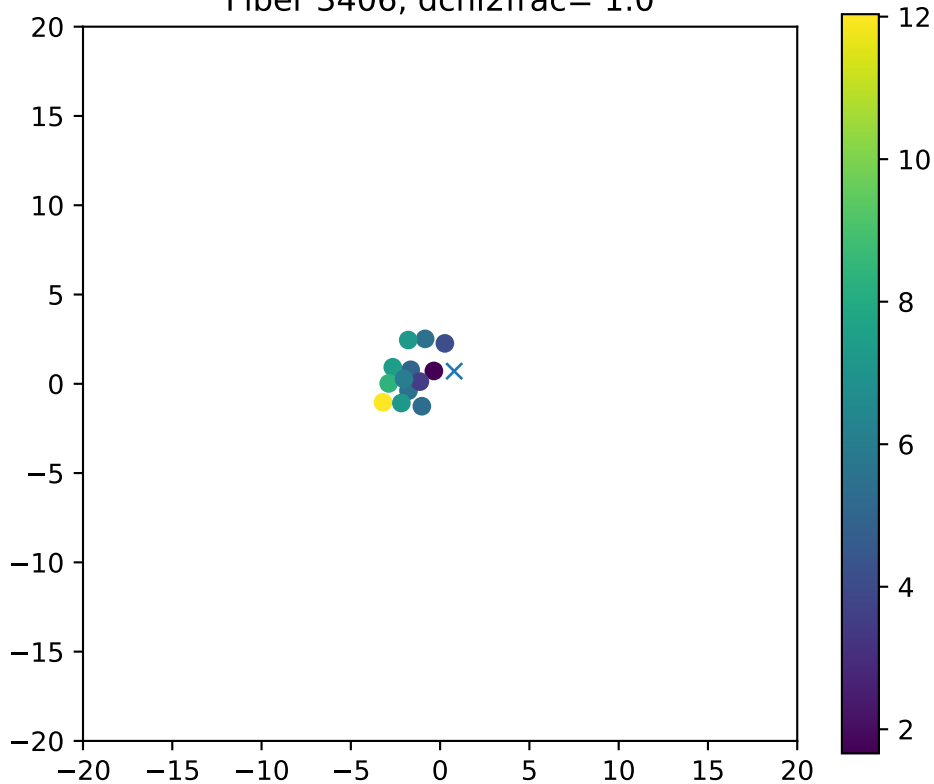
Fiber 3406, dchi2frac= 1.0
