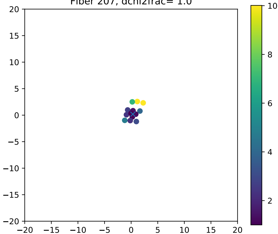
Fiber 207, dchi2frac= 1.0
