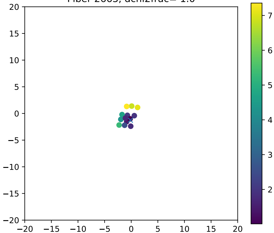
Fiber 2663, dchi2frac= 1.0
