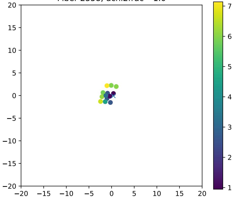
Fiber 2358, dchi2frac= 1.0
