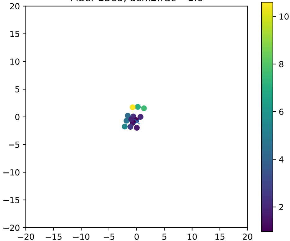
Fiber 2565, dchi2frac= 1.0
