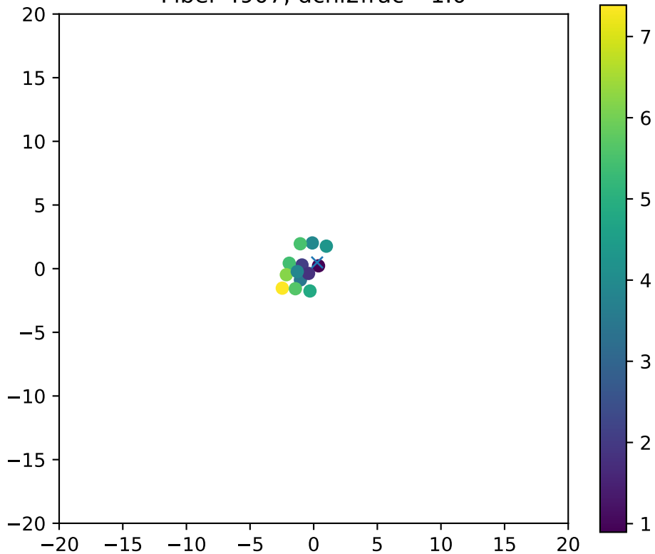
Fiber 4907, dchi2frac= 1.0
