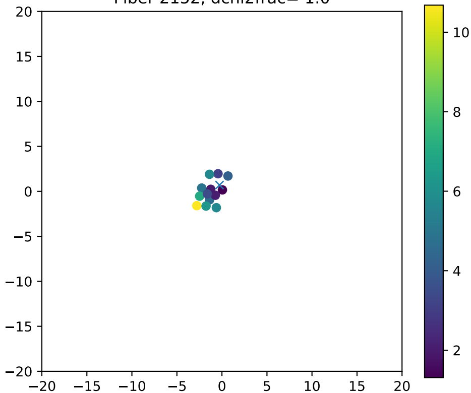
Fiber 2152, dchi2frac= 1.0
