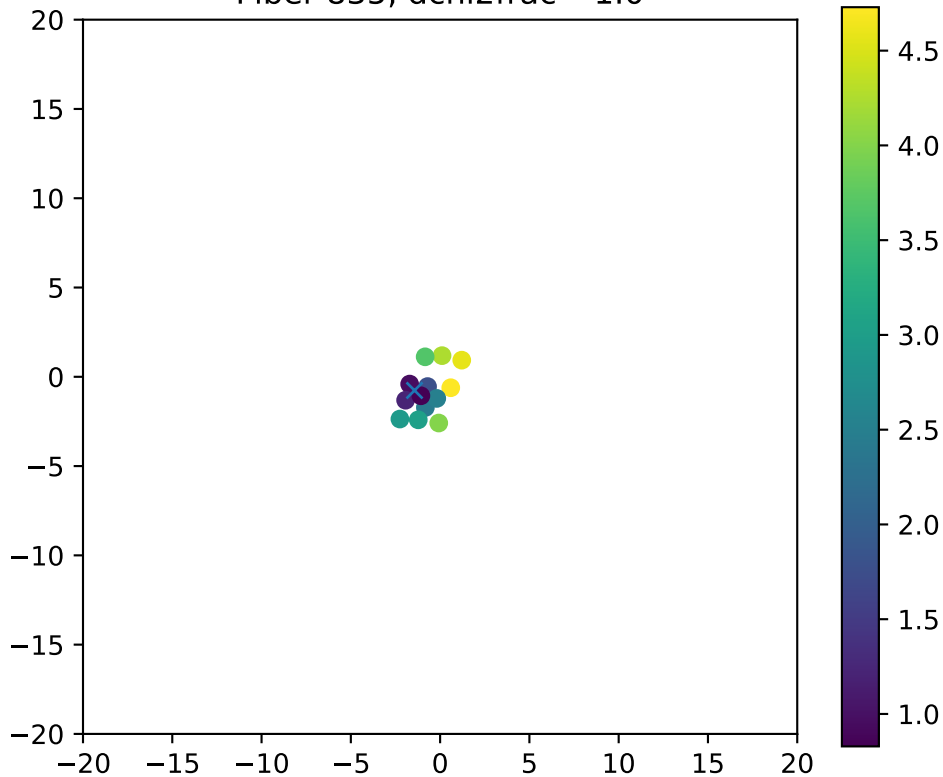
Fiber 835, dchi2frac= 1.0
