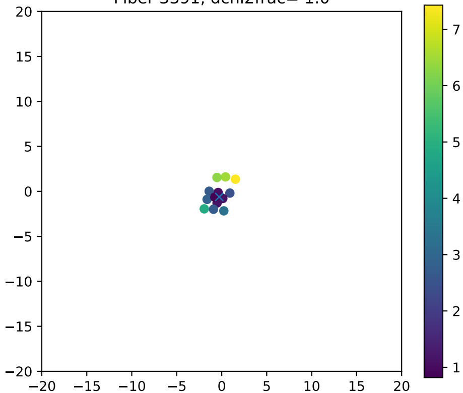
Fiber 3391, dchi2frac= 1.0
