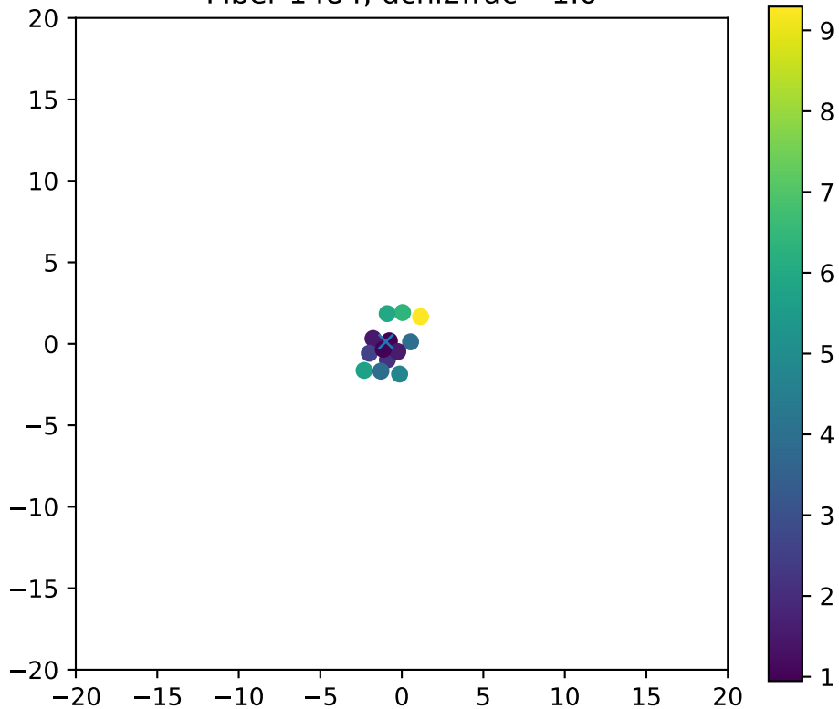
Fiber 1484, dchi2frac= 1.0
