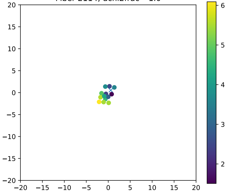
Fiber 2114, dchi2frac= 1.0
