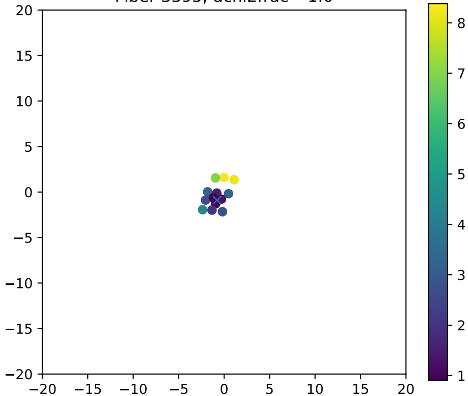
Fiber 3395, dchi2frac= 1.0
