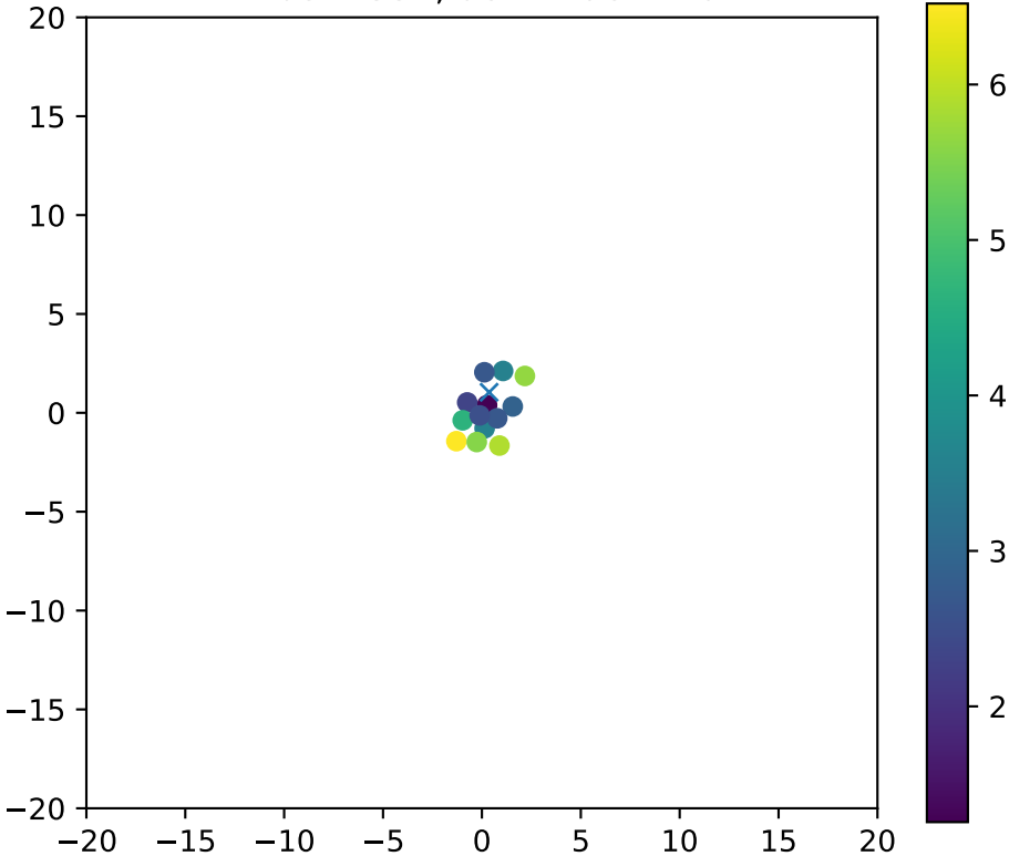
Fiber 4551, dchi2frac= 1.0
