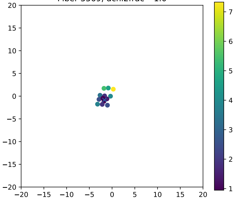
Fiber 3369, dchi2frac= 1.0
