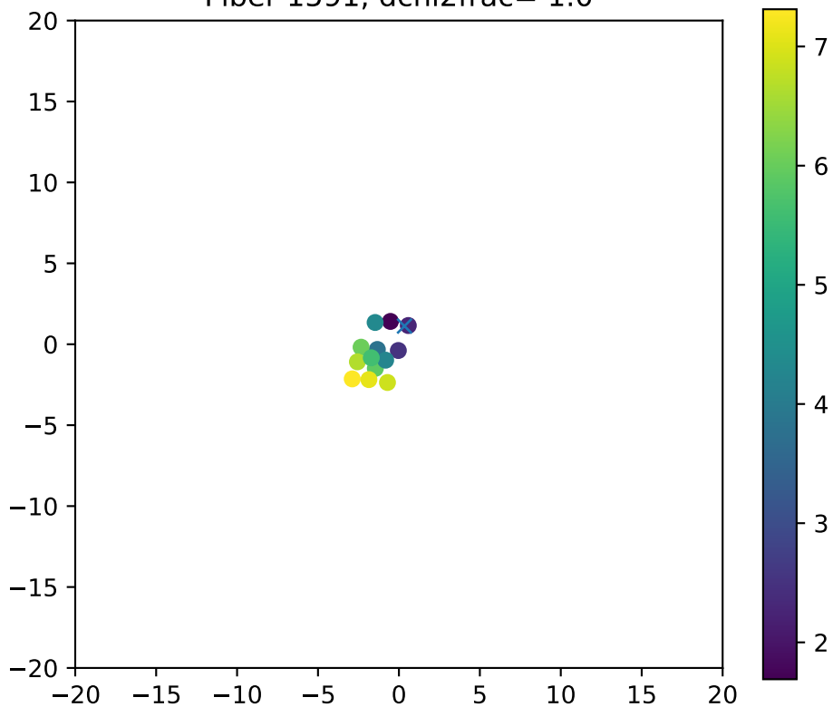
Fiber 1591, dchi2frac= 1.0
