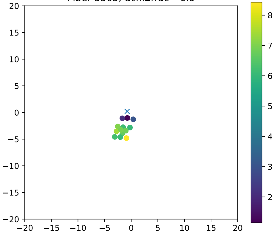
Fiber 3365, dchi2frac= 0.9
