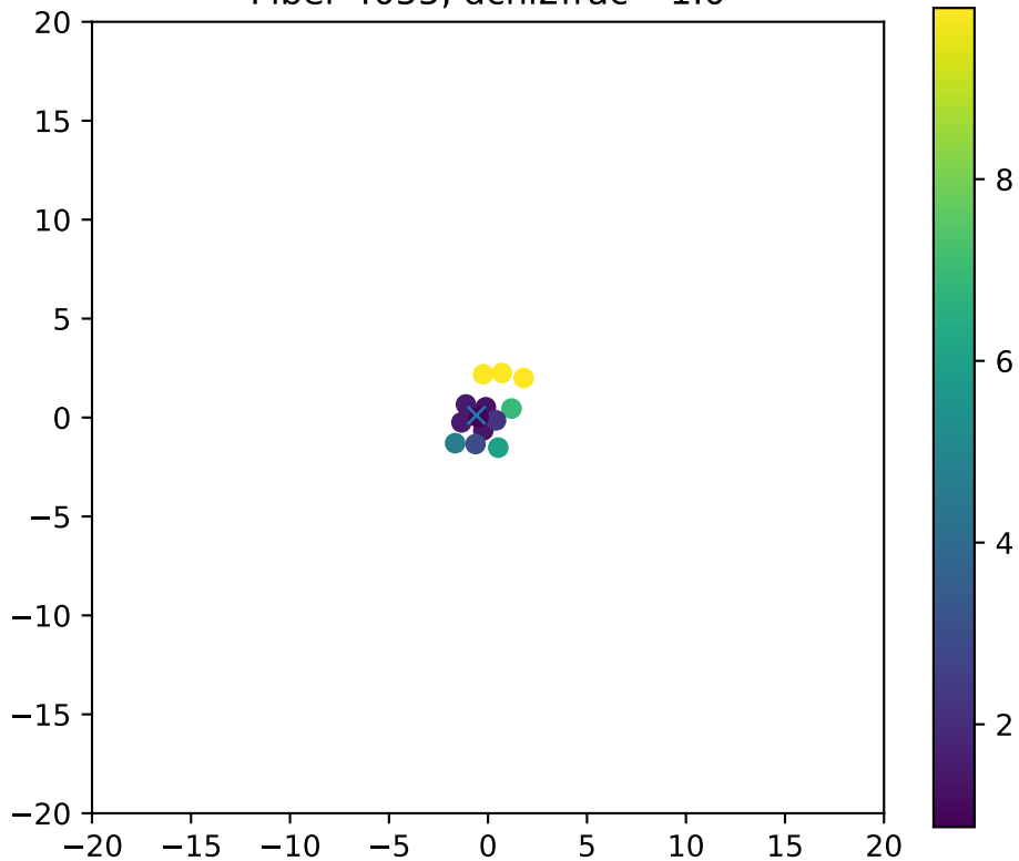
Fiber 4055, dchi2frac= 1.0
