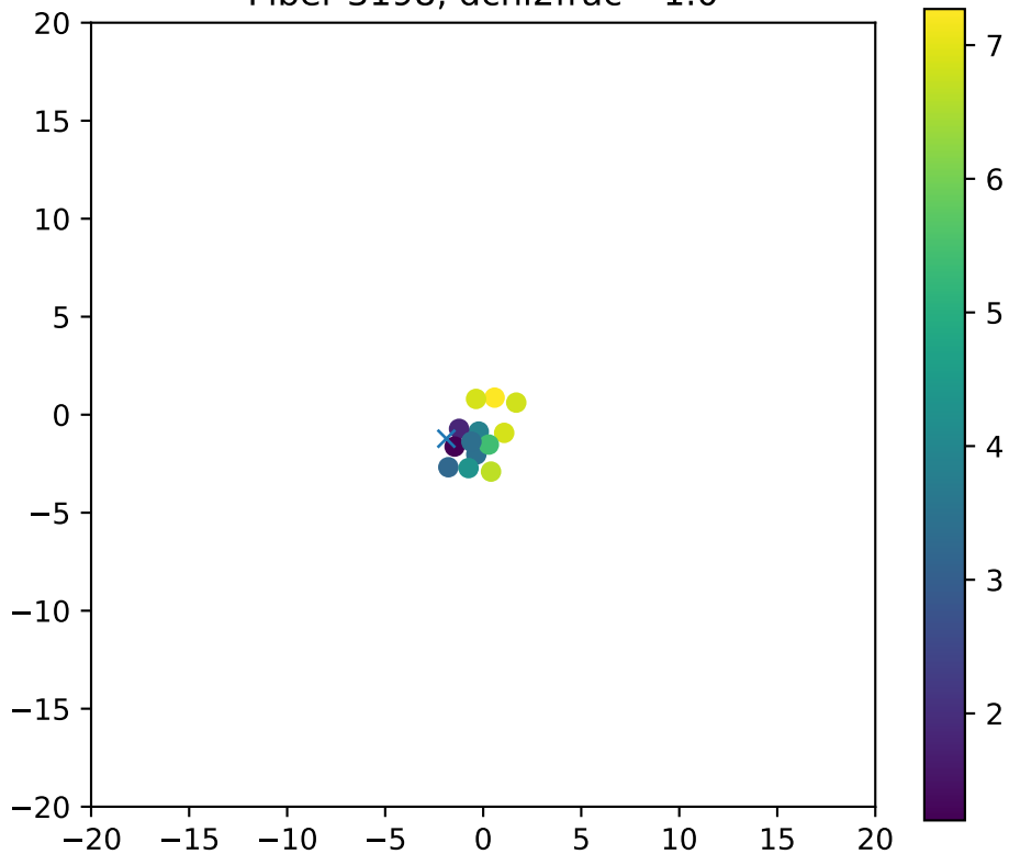
Fiber 3198, dchi2frac= 1.0
