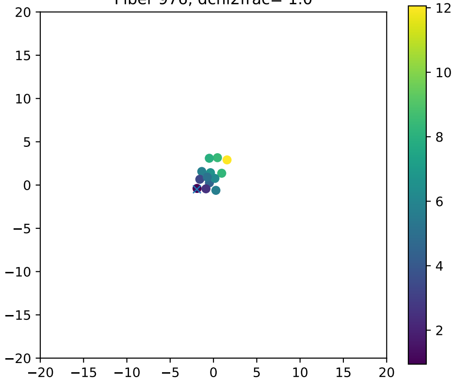
Fiber 976, dchi2frac= 1.0
