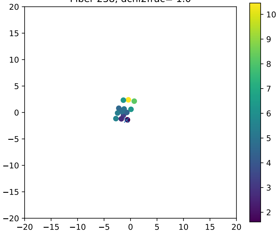
Fiber 238, dchi2frac= 1.0
