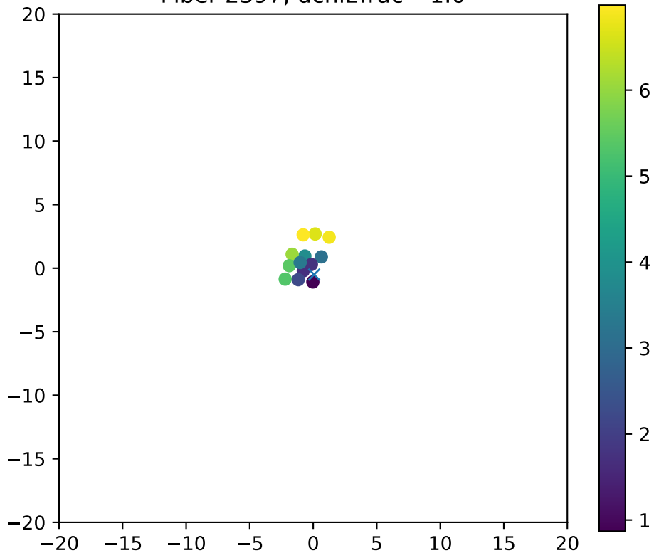
Fiber 2397, dchi2frac= 1.0
