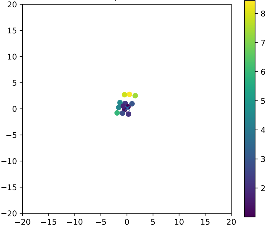
Fiber 4801, dchi2frac= 1.0
