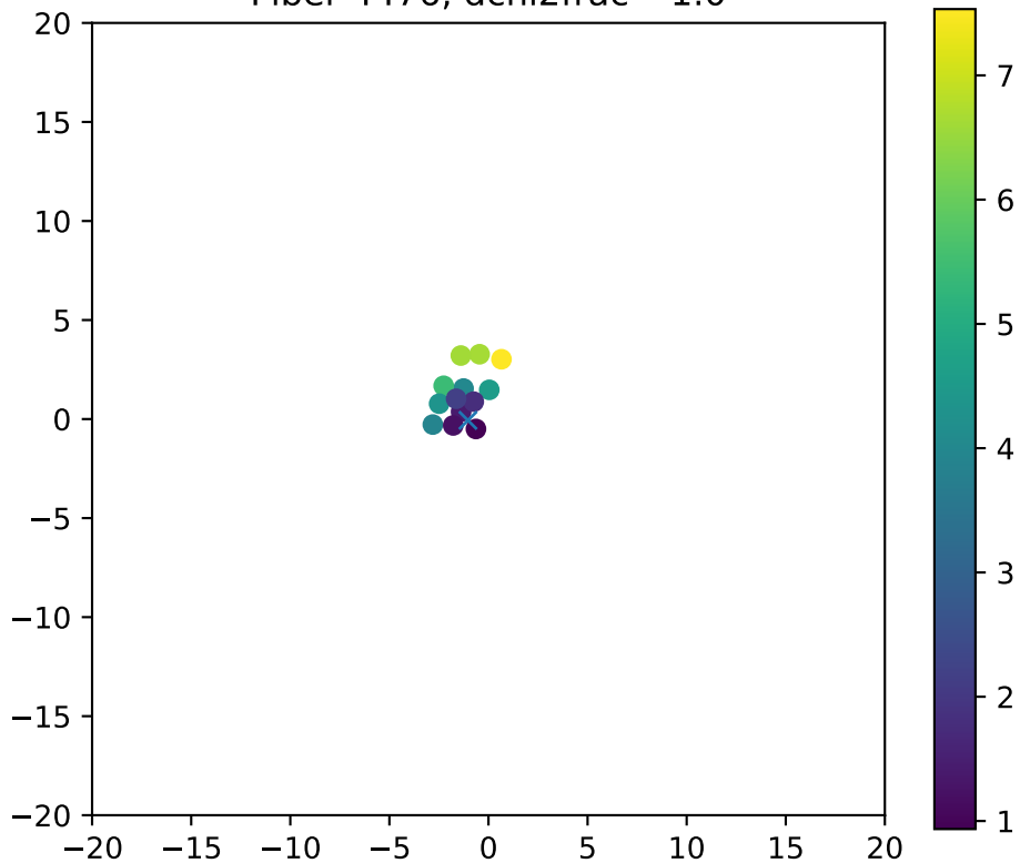
Fiber 4476, dchi2frac= 1.0
