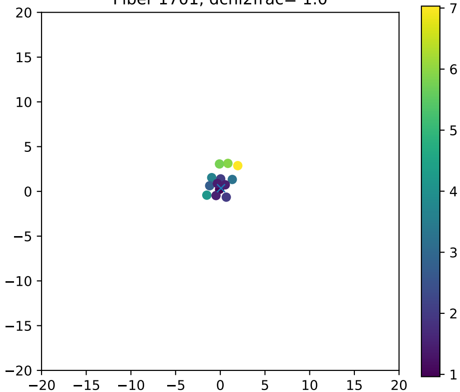
Fiber 1701, dchi2frac= 1.0
