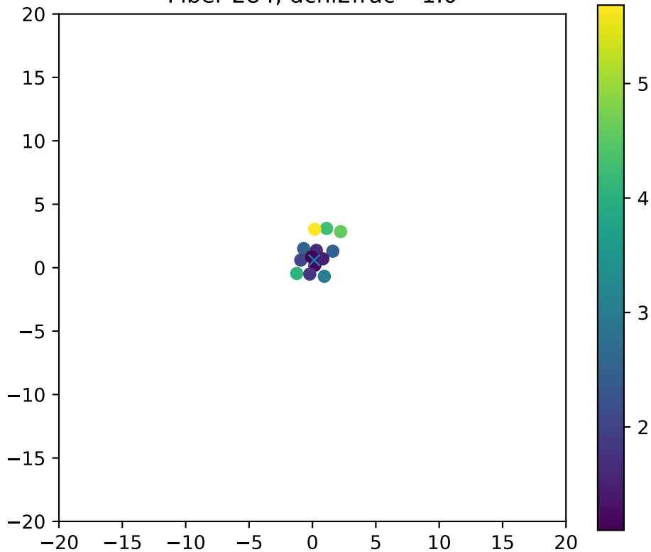
Fiber 284, dchi2frac= 1.0
