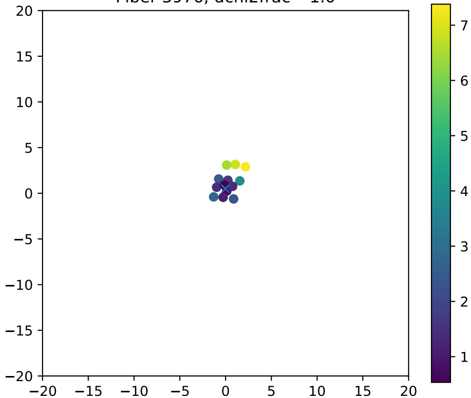
Fiber 3976, dchi2frac= 1.0
