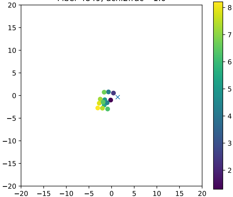
Fiber 4849, dchi2frac= 1.0
