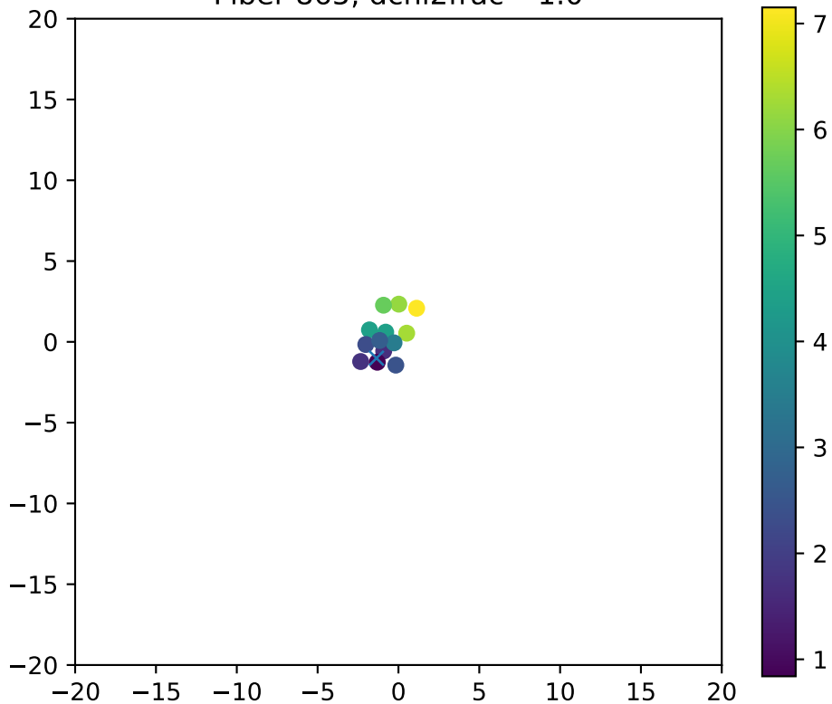
Fiber 865, dchi2frac= 1.0
