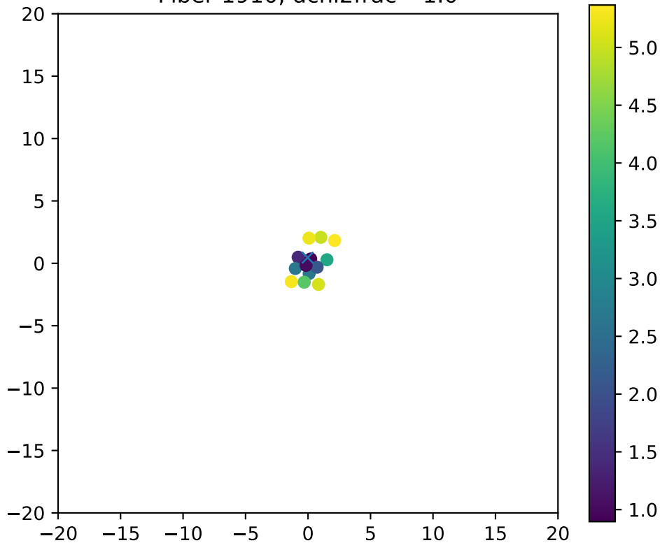
Fiber 1910, dchi2frac= 1.0
