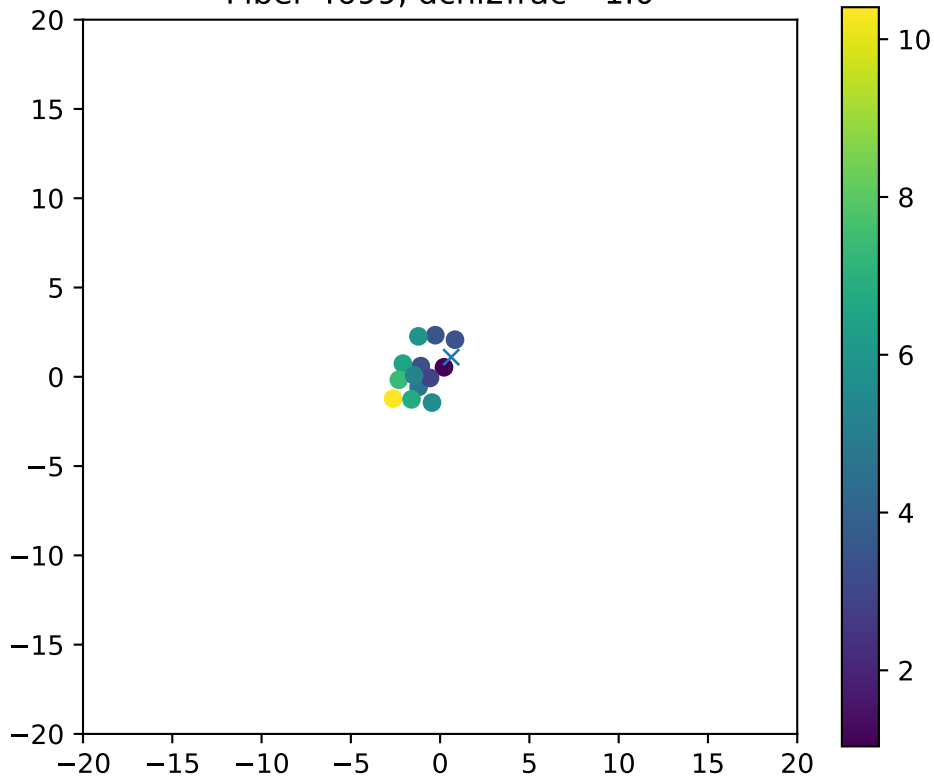
Fiber 4699, dchi2frac= 1.0
