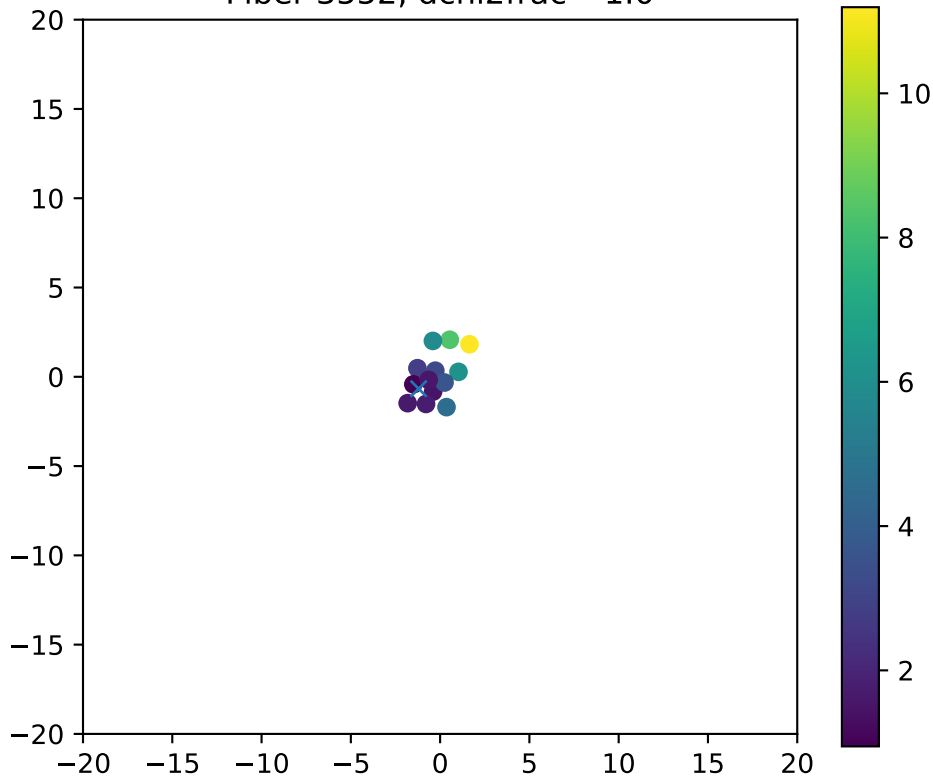
Fiber 3552, dchi2frac= 1.0
