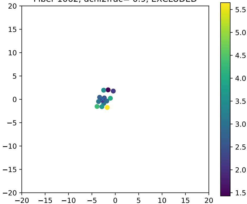
Fiber 1062, dchi2frac= 0.9, EXCLUDED
