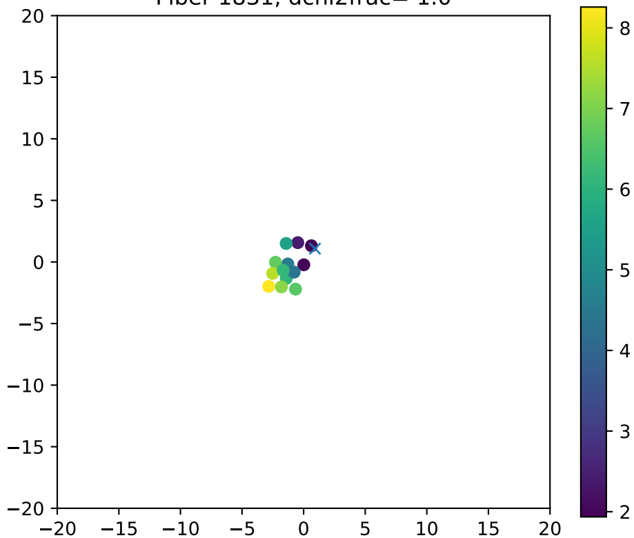
Fiber 1831, dchi2frac= 1.0
