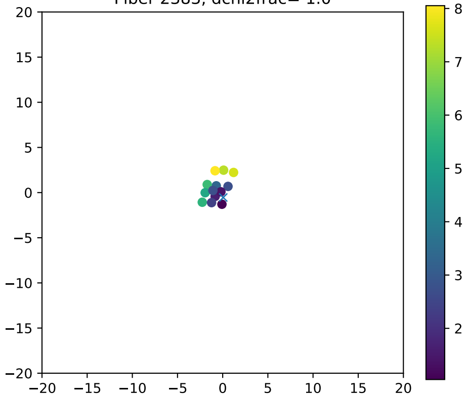
Fiber 2383, dchi2frac= 1.0
