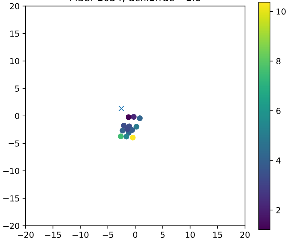
Fiber 1054, dchi2frac= 1.0
