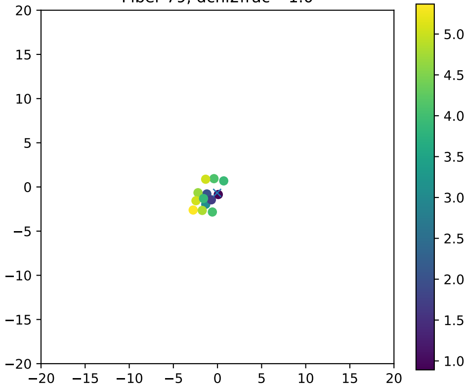
Fiber 79, dchi2frac= 1.0
