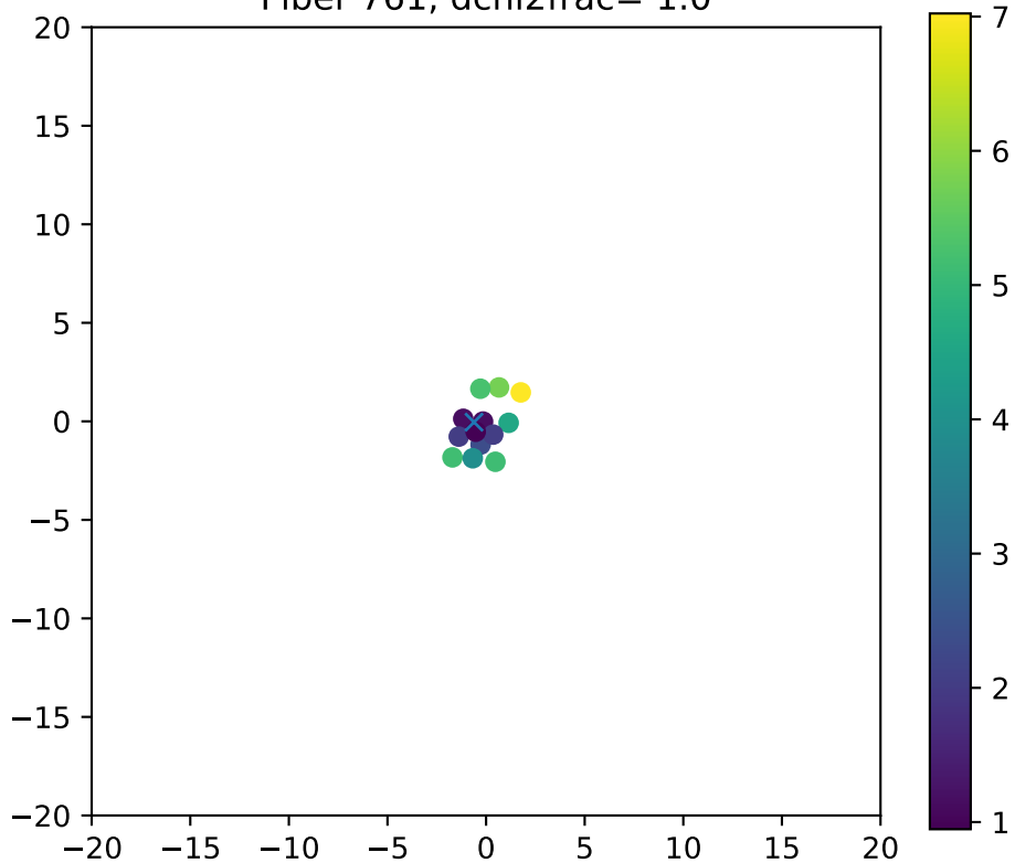
Fiber 761, dchi2frac= 1.0
