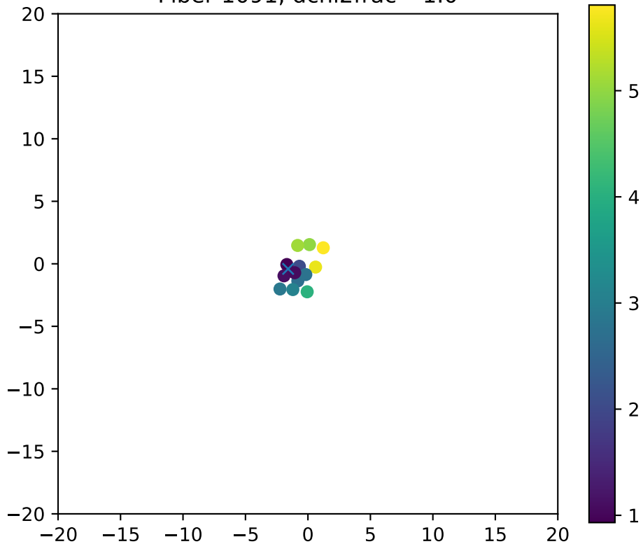
Fiber 1091, dchi2frac= 1.0
