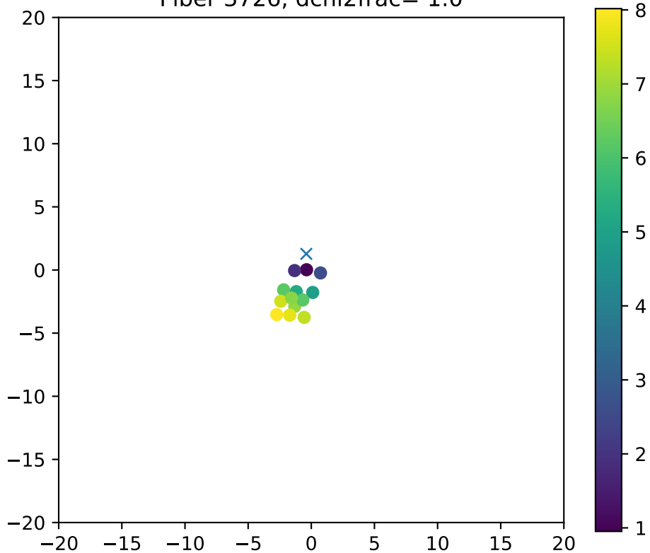
Fiber 3726, dchi2frac= 1.0
