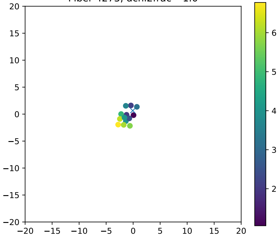
Fiber 4273, dchi2frac= 1.0
