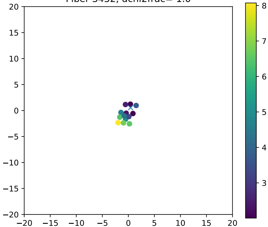
Fiber 3432, dchi2frac= 1.0
