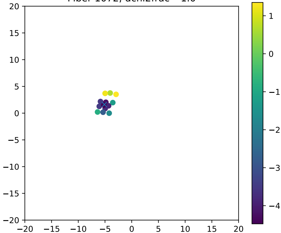
Fiber 1072, dchi2frac= 1.0
