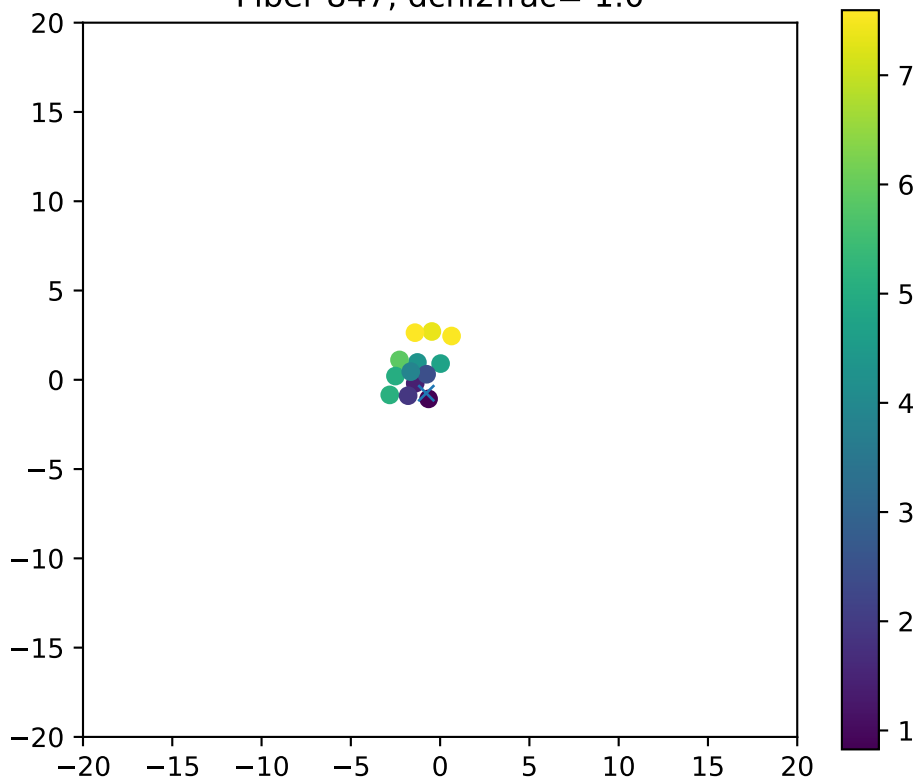
Fiber 847, dchi2frac= 1.0
