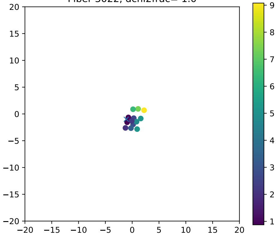
Fiber 3022, dchi2frac= 1.0
