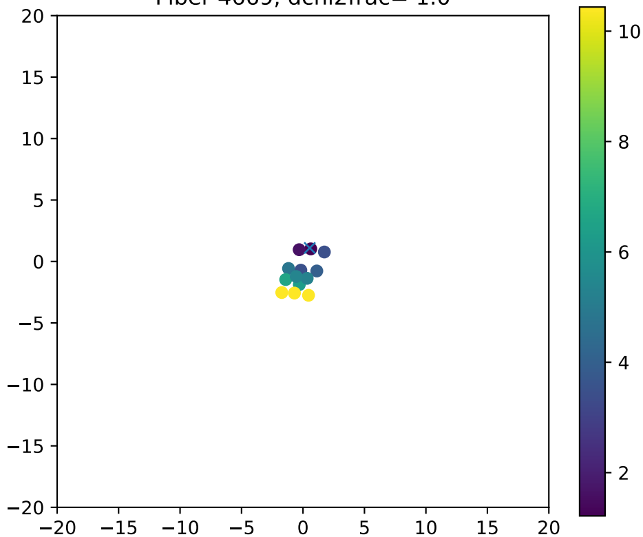
Fiber 4669, dchi2frac= 1.0
