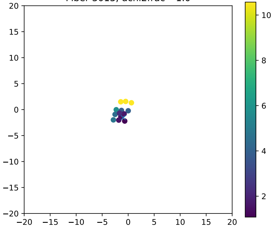
Fiber 3013, dchi2frac= 1.0
