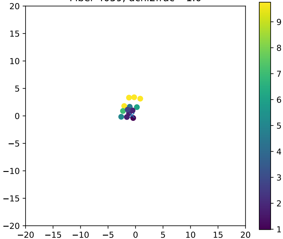
Fiber 4059, dchi2frac= 1.0
