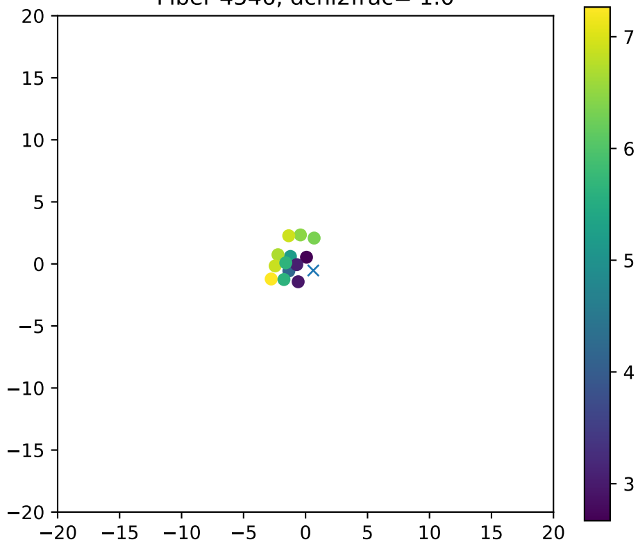
Fiber 4546, dchi2frac= 1.0
