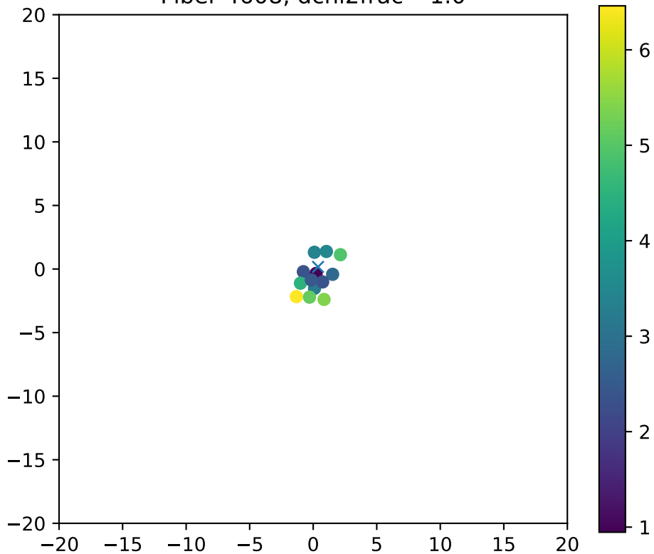
Fiber 4608, dchi2frac= 1.0
