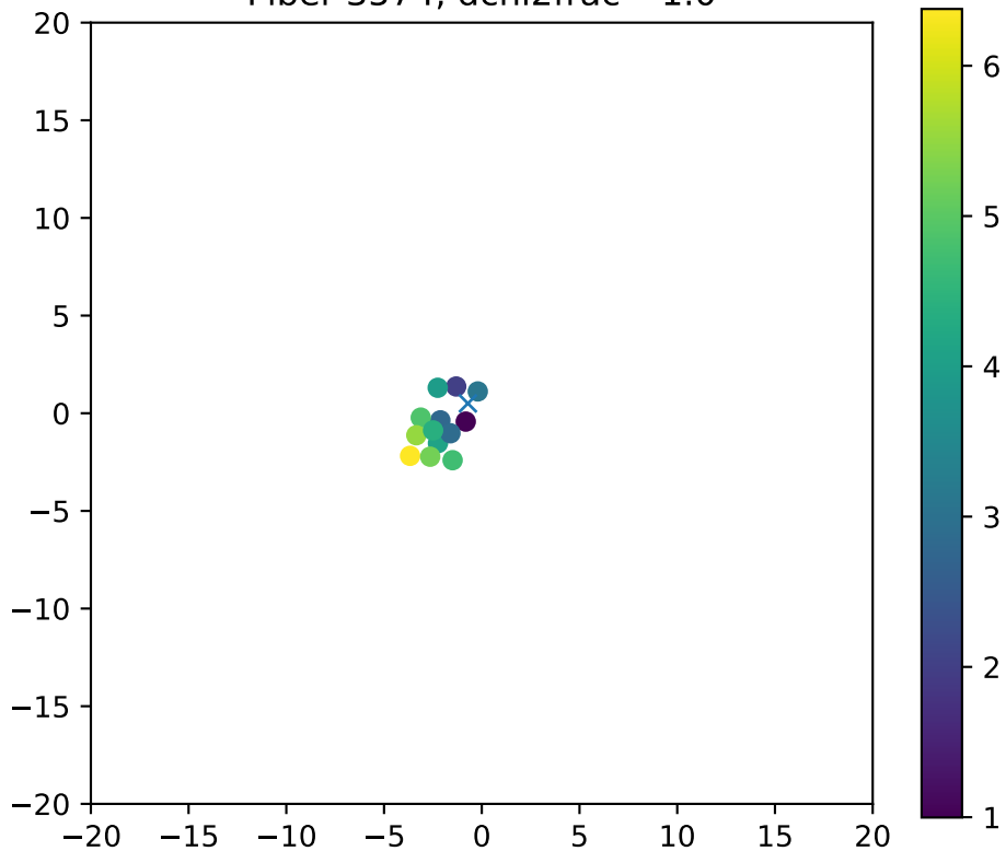
Fiber 3574, dchi2frac= 1.0
