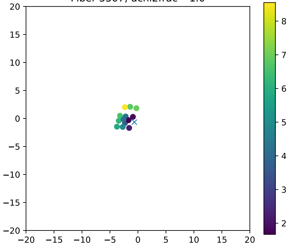
Fiber 3307, dchi2frac= 1.0
