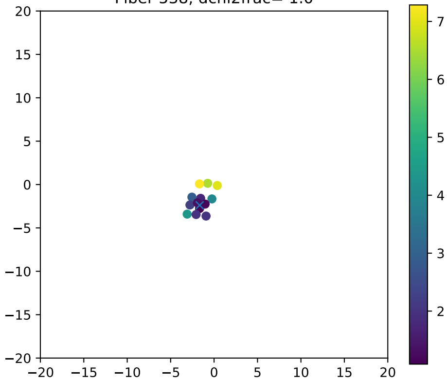
Fiber 538, dchi2frac= 1.0
