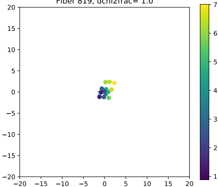
Fiber 819, dchi2frac= 1.0
