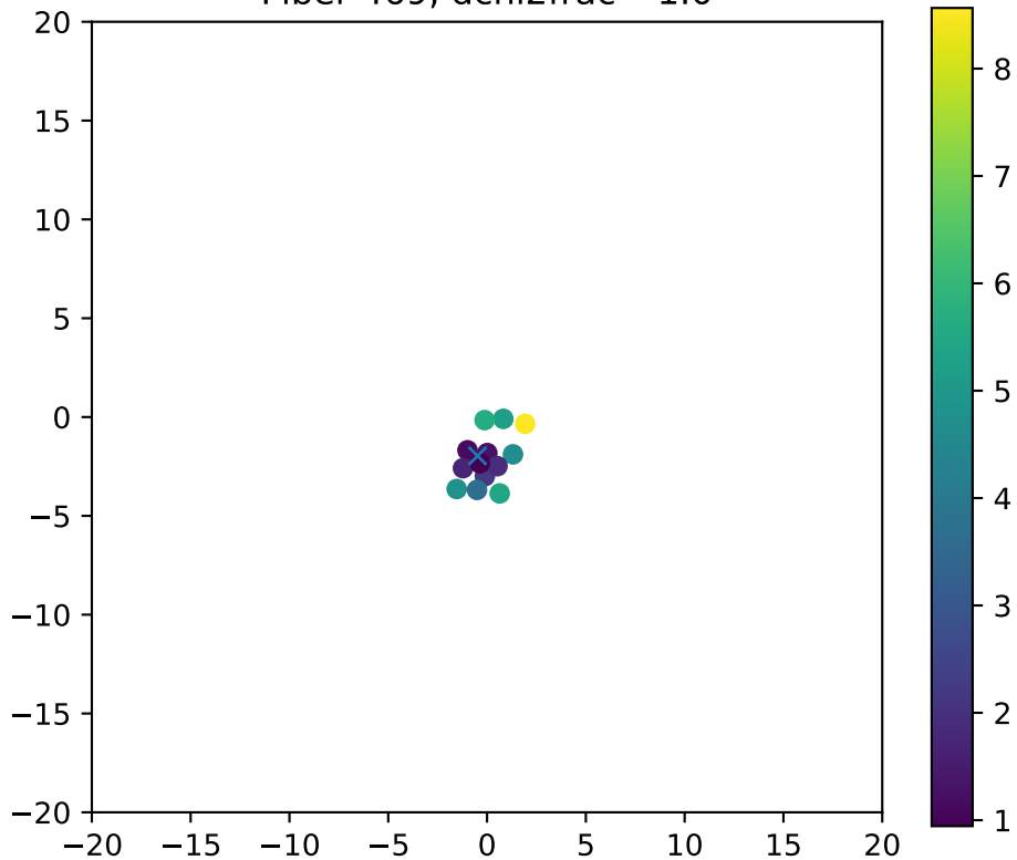
Fiber 469, dchi2frac= 1.0
