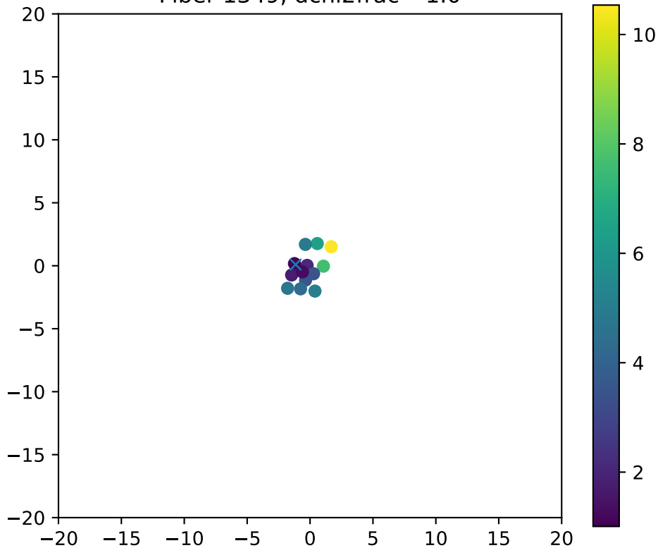
Fiber 1349, dchi2frac= 1.0
