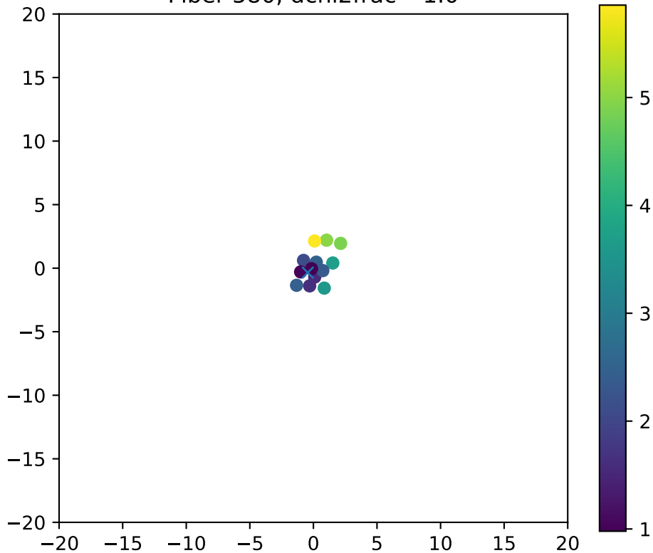
Fiber 580, dchi2frac= 1.0
