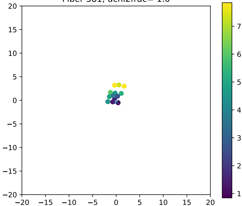
Fiber 381, dchi2frac= 1.0
