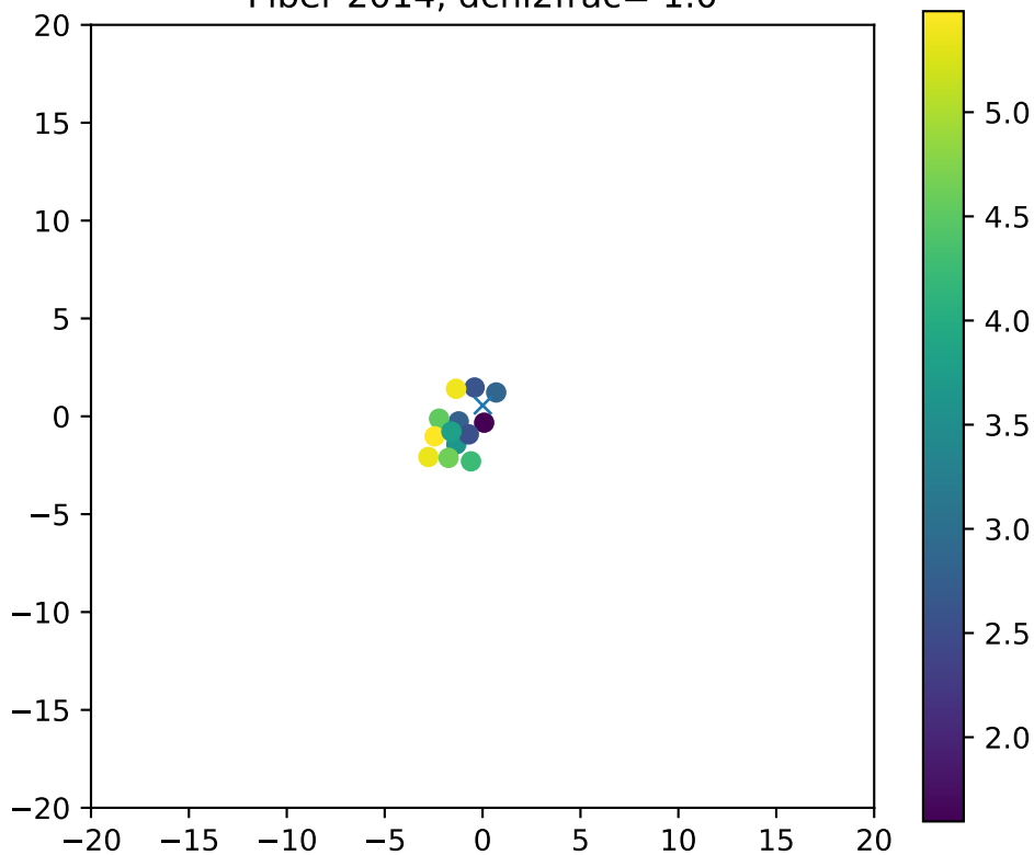
Fiber 2014, dchi2frac= 1.0
