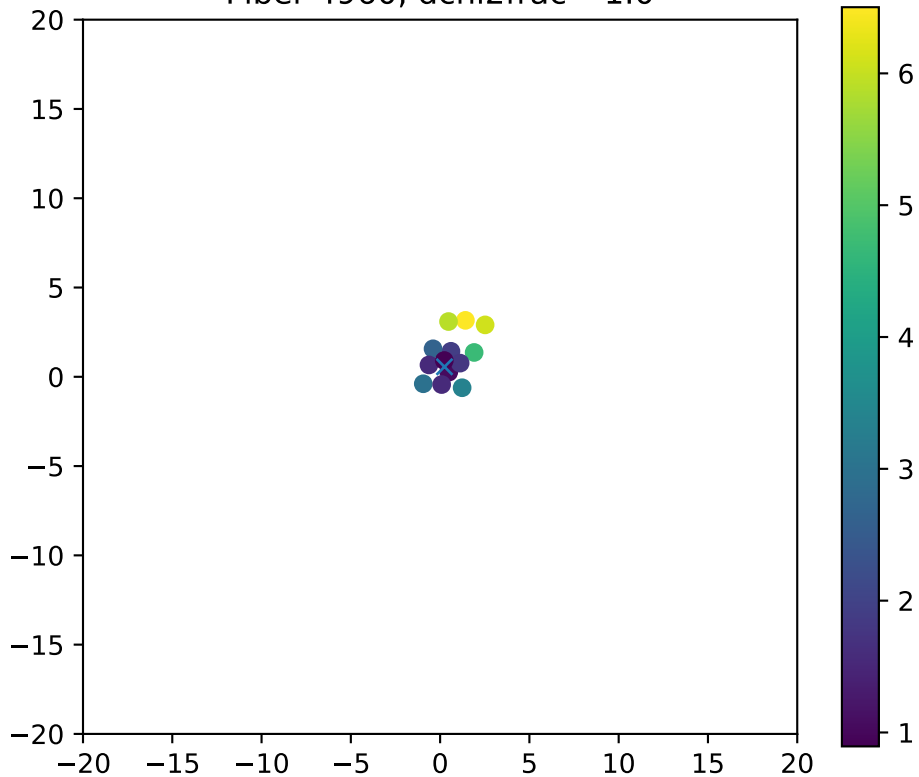
Fiber 4960, dchi2frac= 1.0
