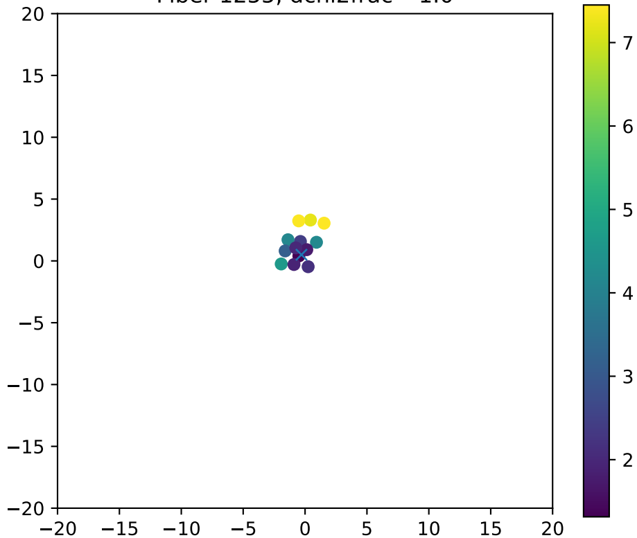
Fiber 1255, dchi2frac= 1.0
