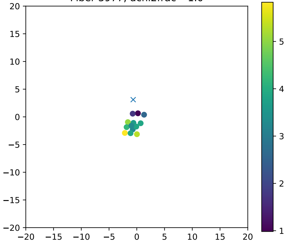
Fiber 3977, dchi2frac= 1.0
