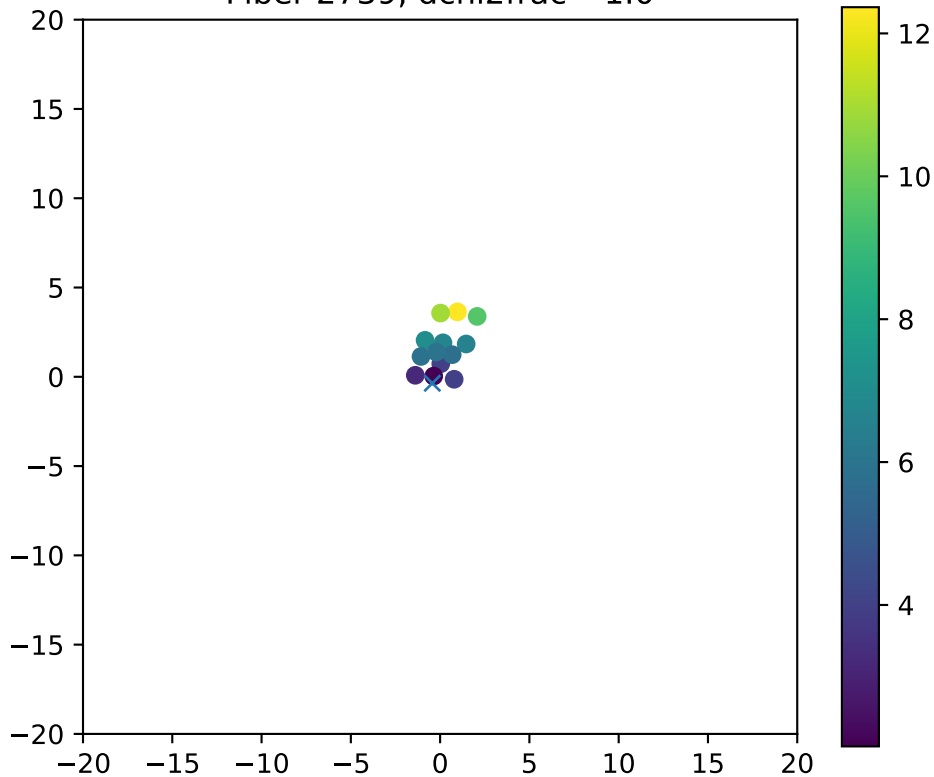
Fiber 2739, dchi2frac= 1.0
