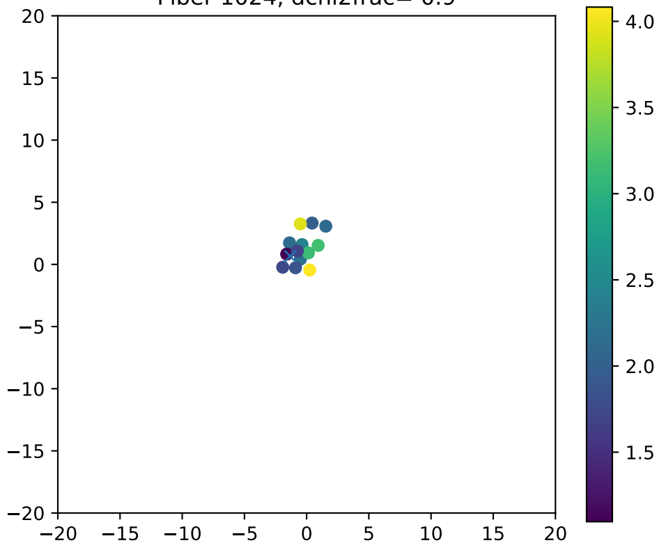
Fiber 1024, dchi2frac= 0.9
