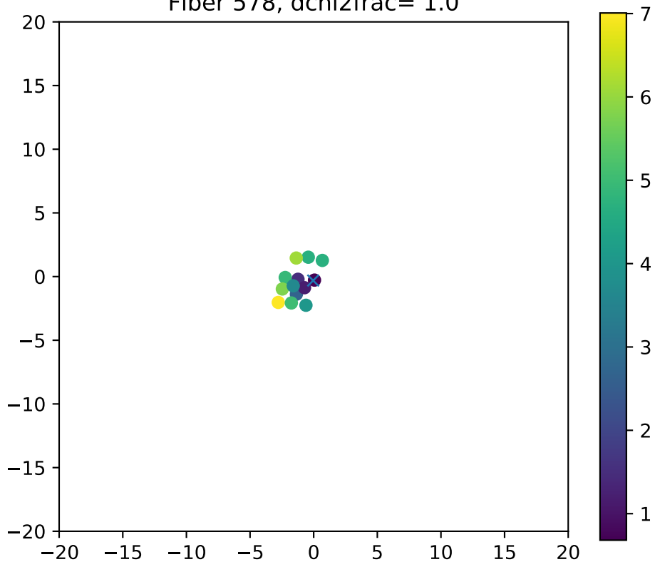
Fiber 578, dchi2frac= 1.0
