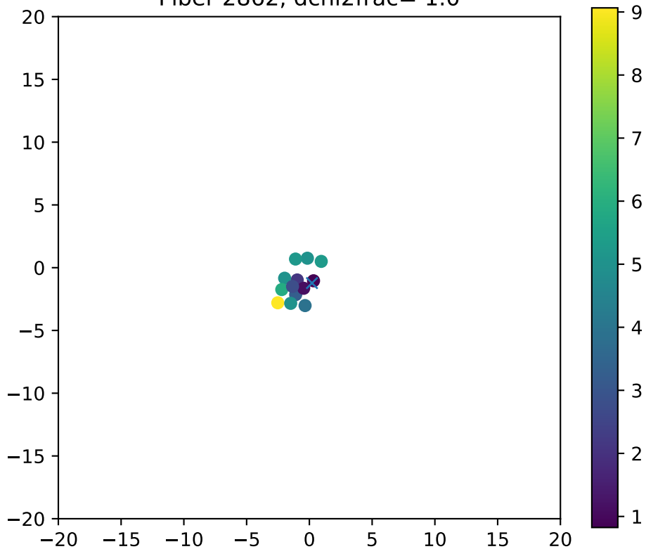
Fiber 2862, dchi2frac= 1.0
