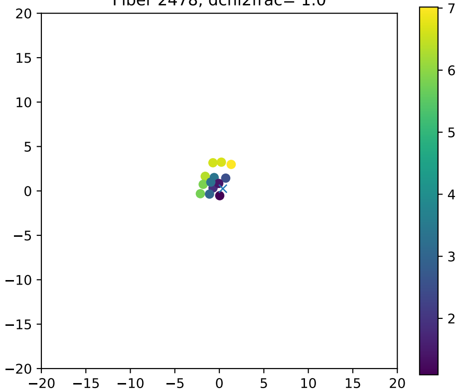
Fiber 2478, dchi2frac= 1.0
