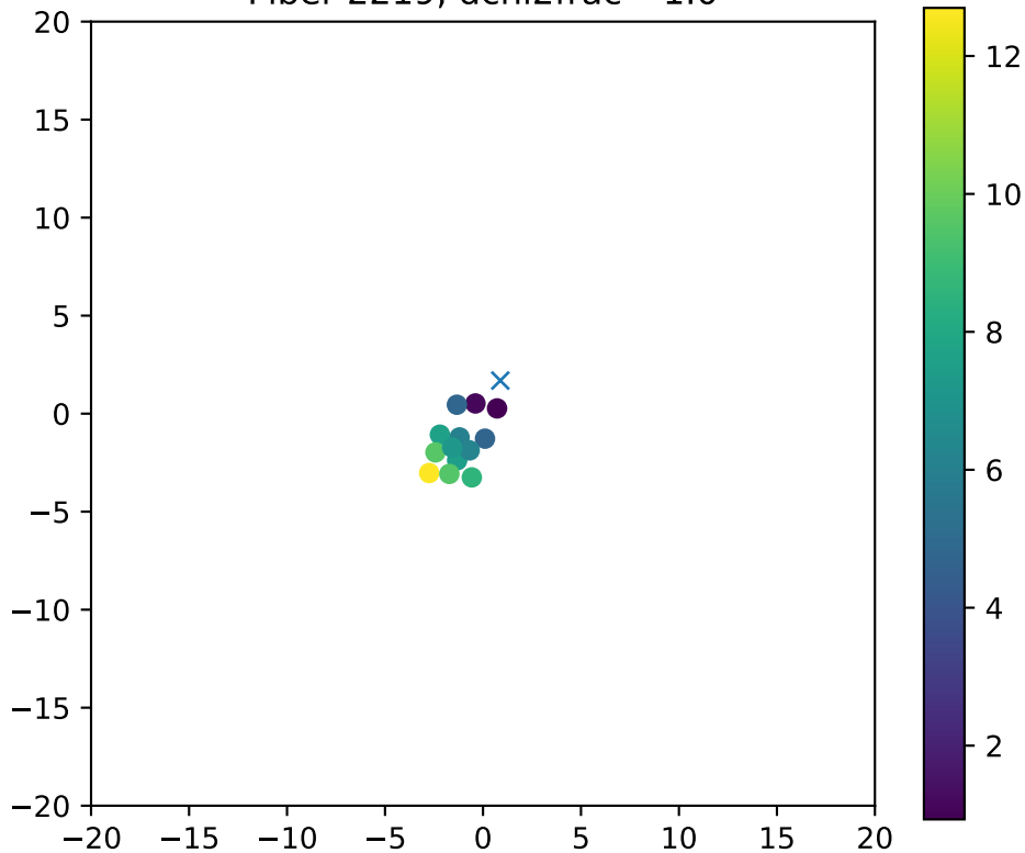
Fiber 2219, dchi2frac= 1.0
