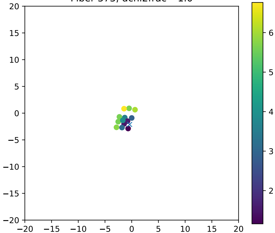
Fiber 373, dchi2frac= 1.0
