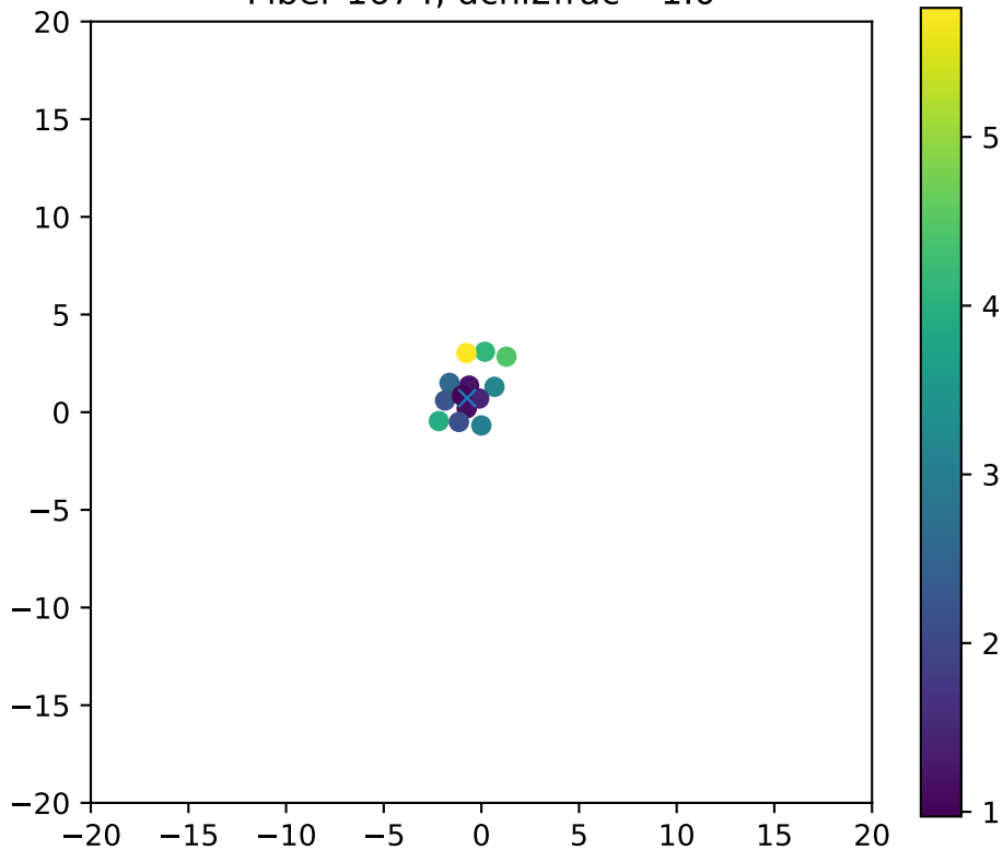
Fiber 1674, dchi2frac= 1.0
