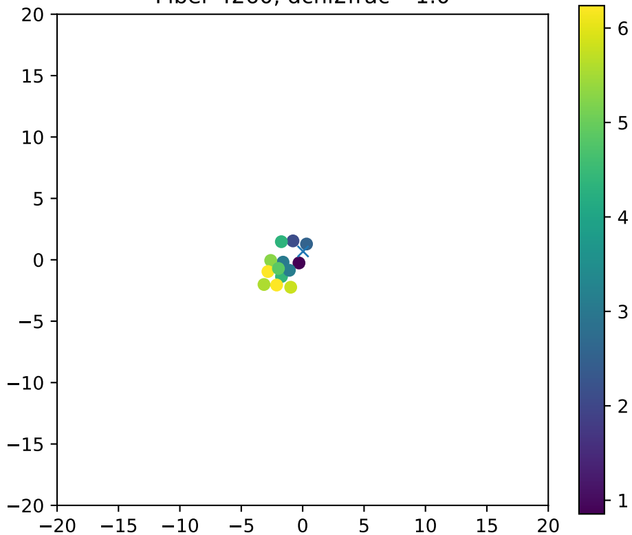
Fiber 4260, dchi2frac= 1.0
