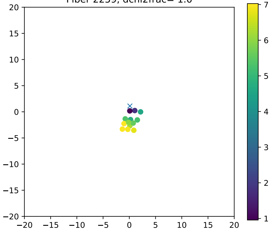
Fiber 2259, dchi2frac= 1.0
