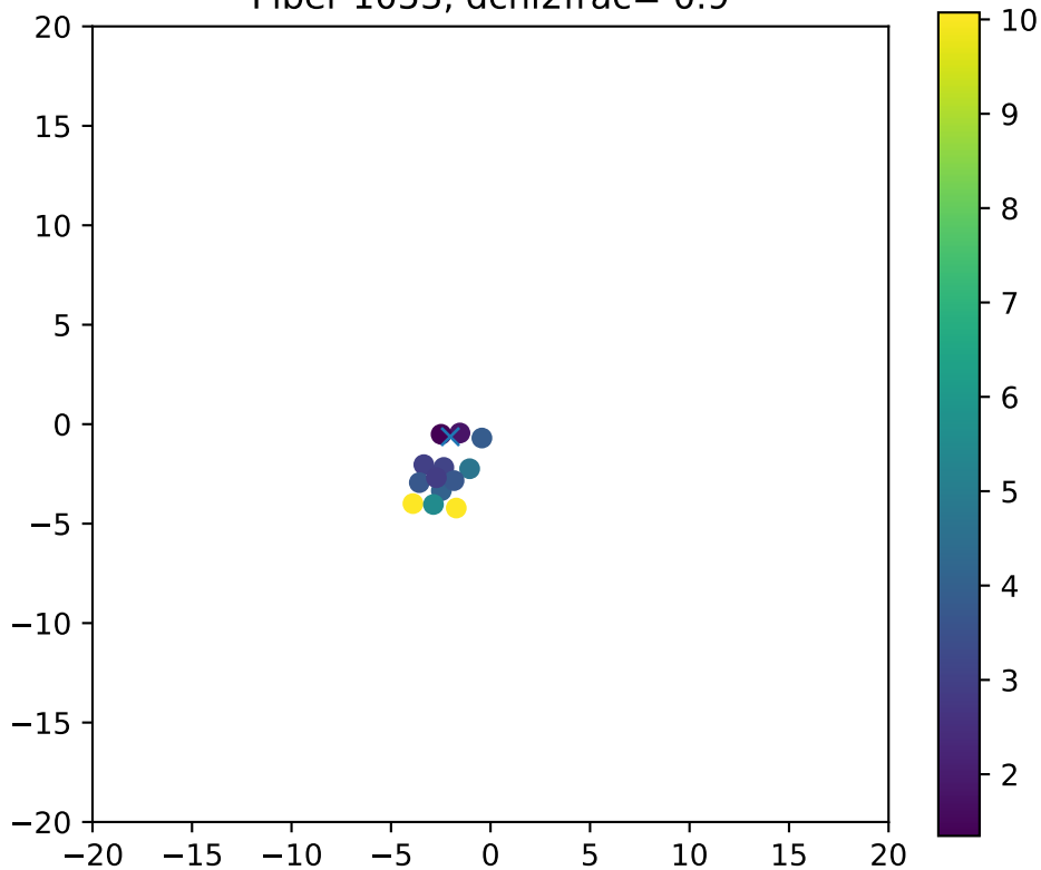
Fiber 1053, dchi2frac= 0.9
