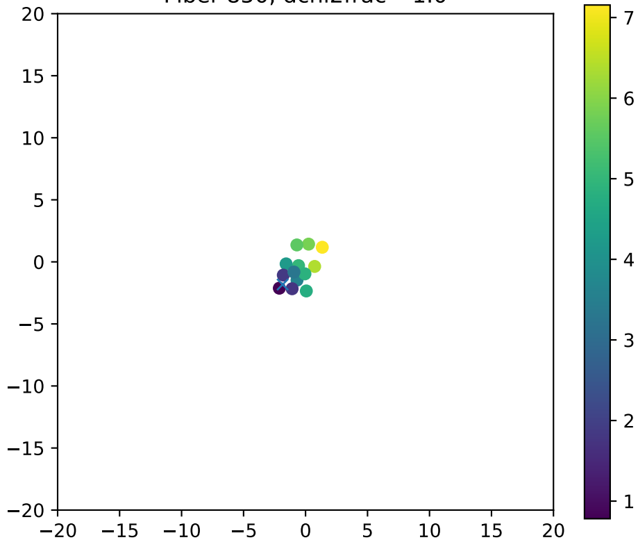
Fiber 850, dchi2frac= 1.0
