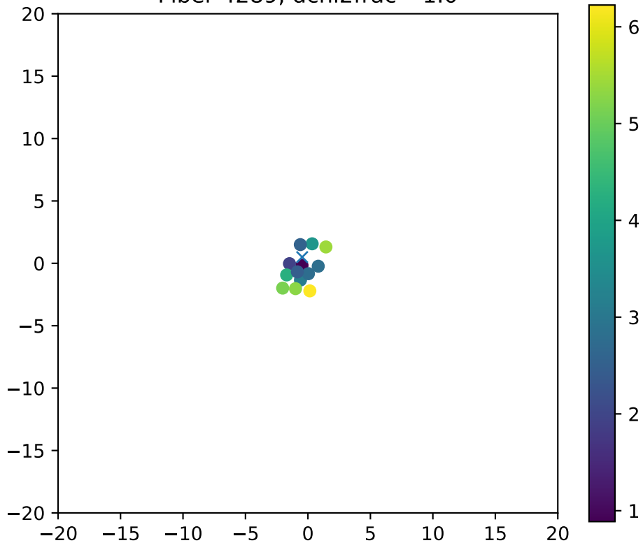
Fiber 4289, dchi2frac= 1.0
