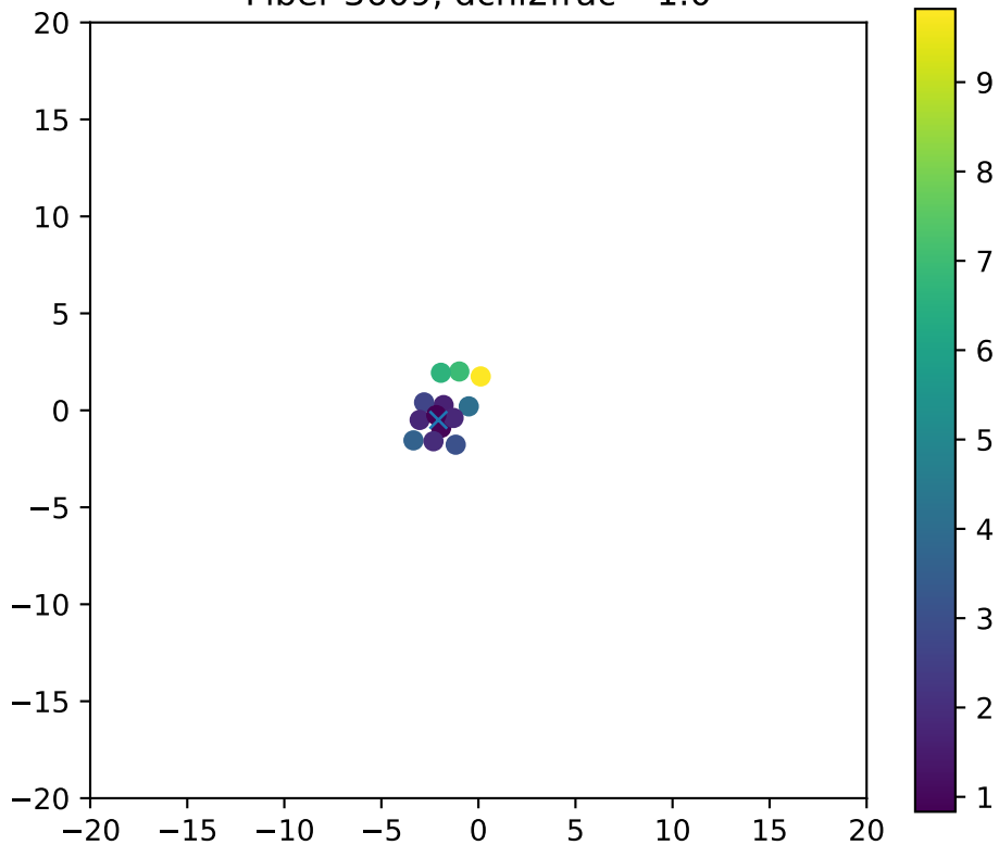
Fiber 3609, dchi2frac= 1.0
