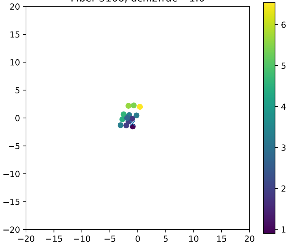
Fiber 3106, dchi2frac= 1.0
