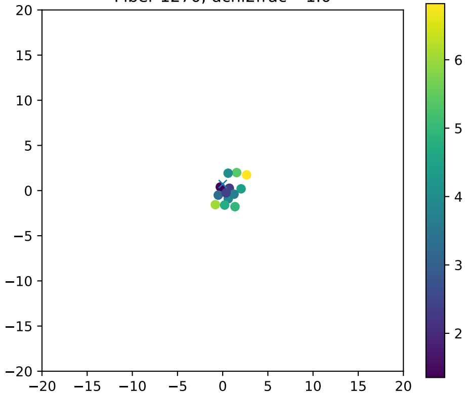
Fiber 1270, dchi2frac= 1.0
