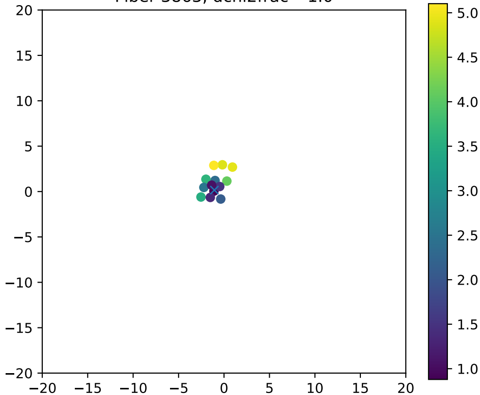
Fiber 3863, dchi2frac= 1.0
