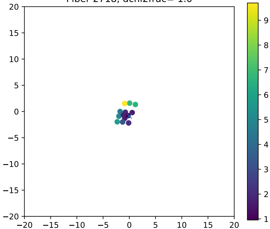
Fiber 2718, dchi2frac= 1.0
