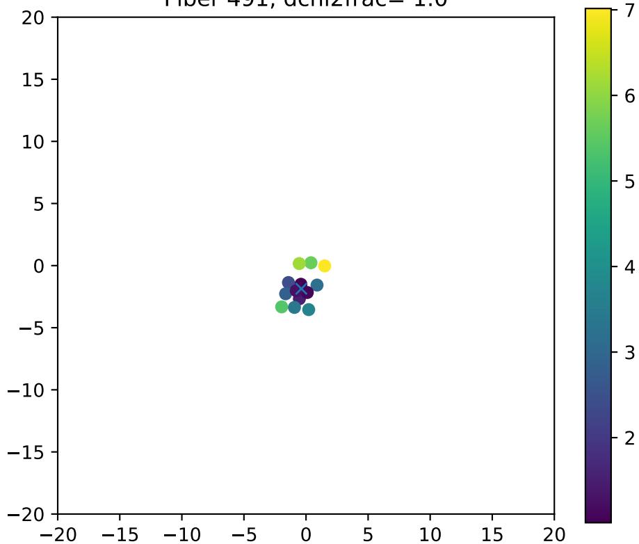
Fiber 491, dchi2frac= 1.0
