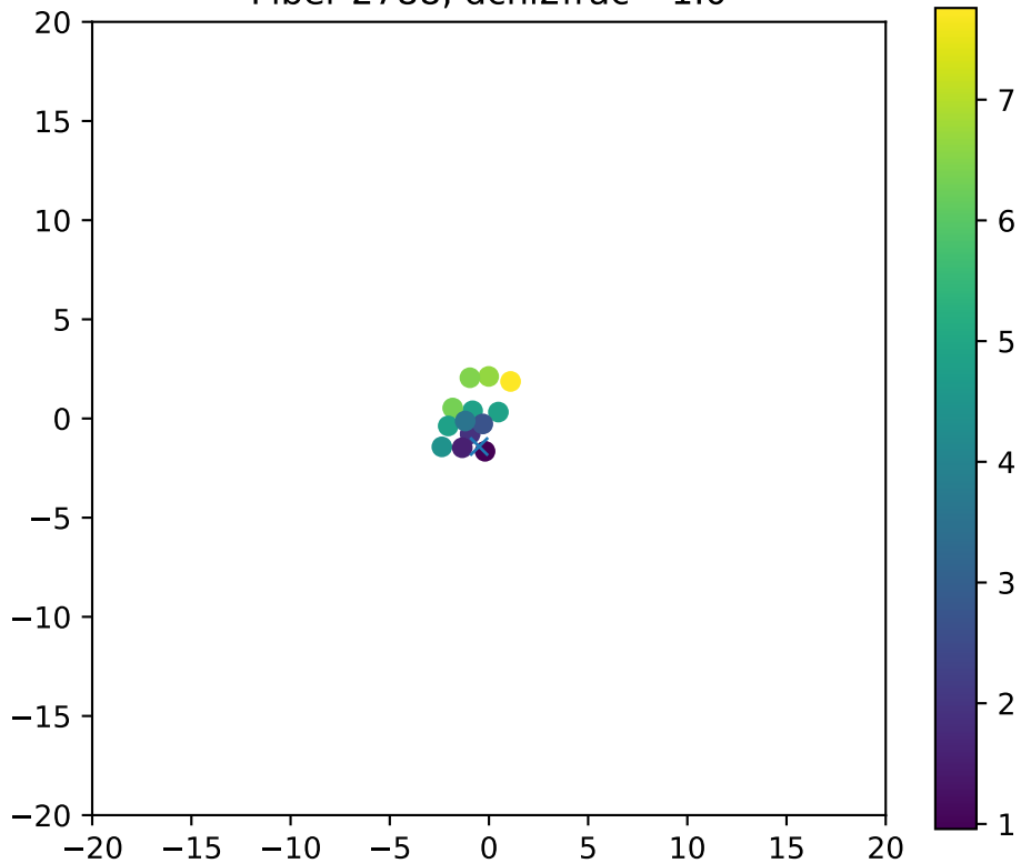
Fiber 2788, dchi2frac= 1.0
