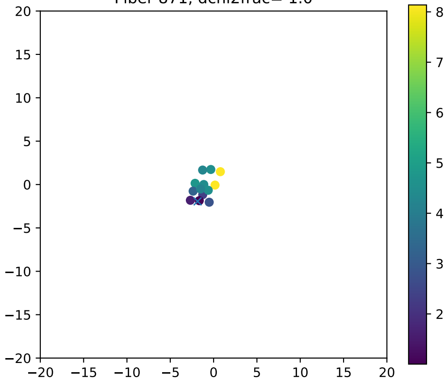
Fiber 871, dchi2frac= 1.0
