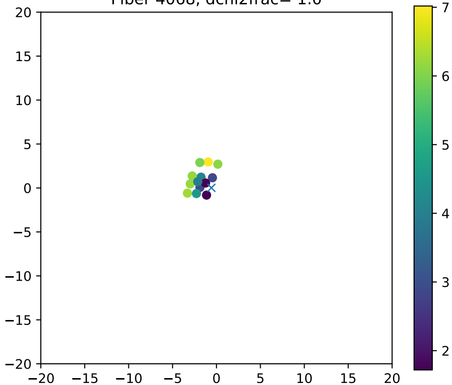
Fiber 4068, dchi2frac= 1.0
