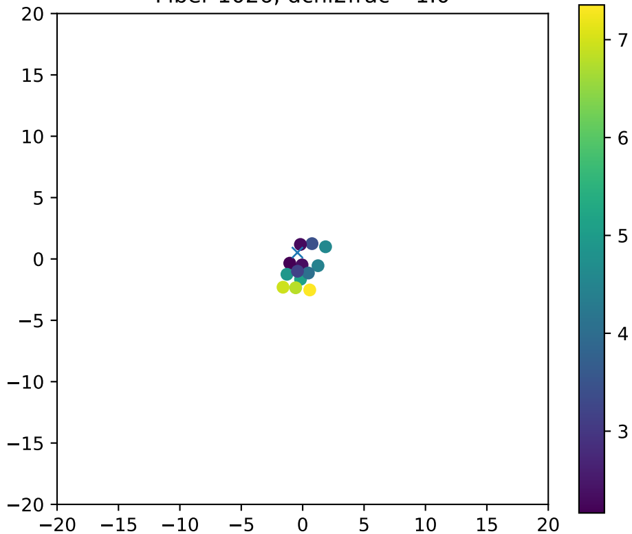
Fiber 1026, dchi2frac= 1.0
