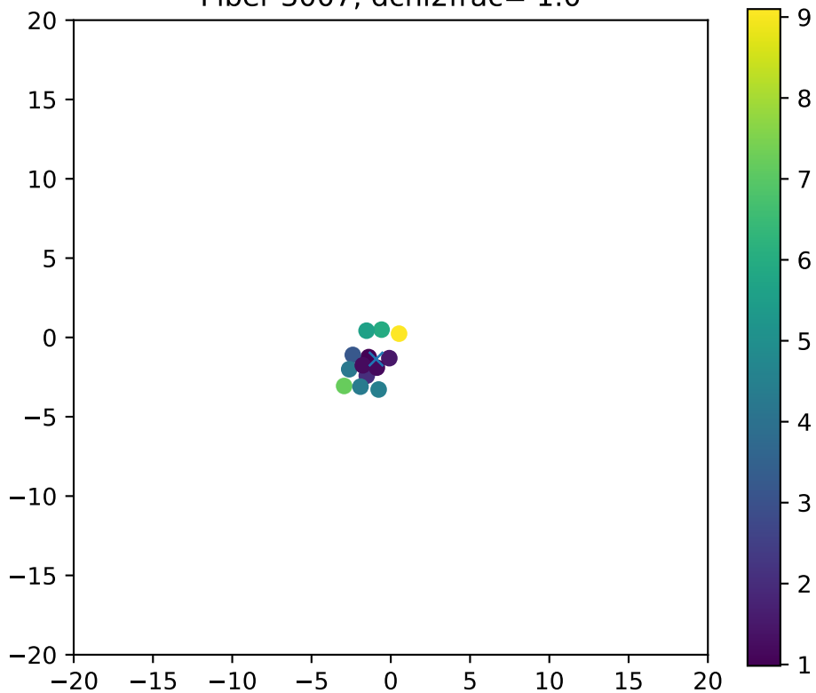
Fiber 3007, dchi2frac= 1.0
