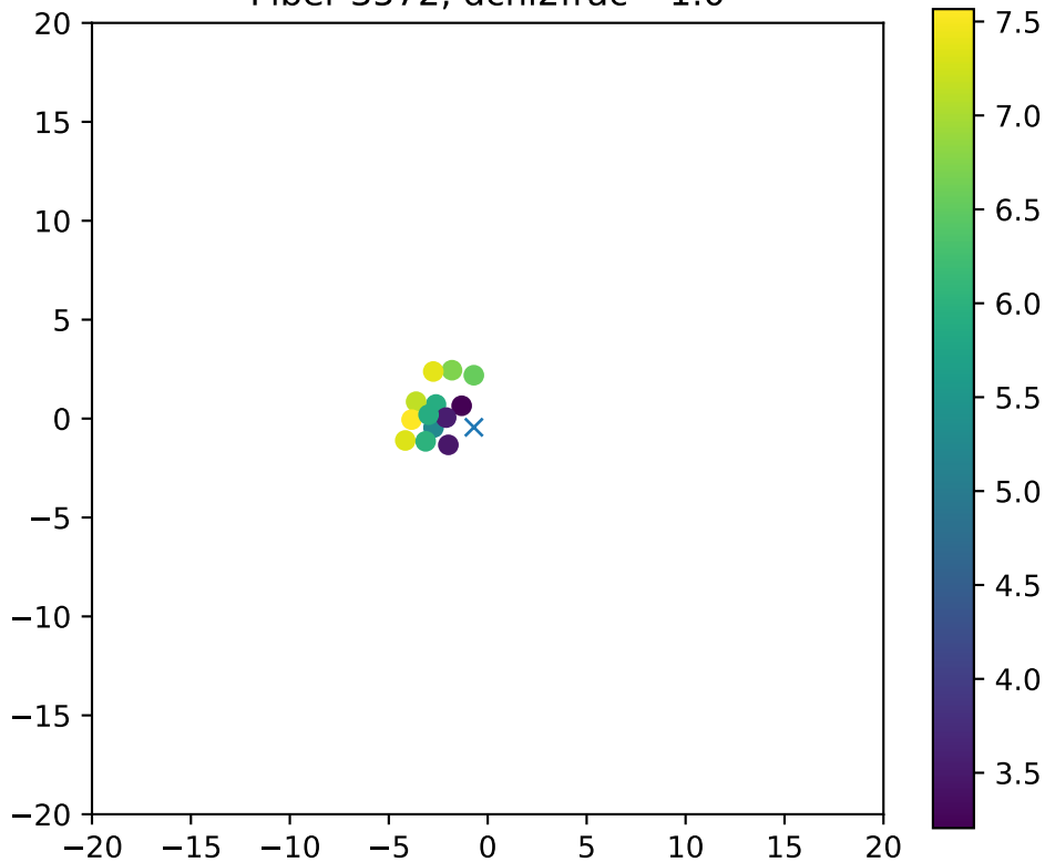
Fiber 3572, dchi2frac= 1.0
