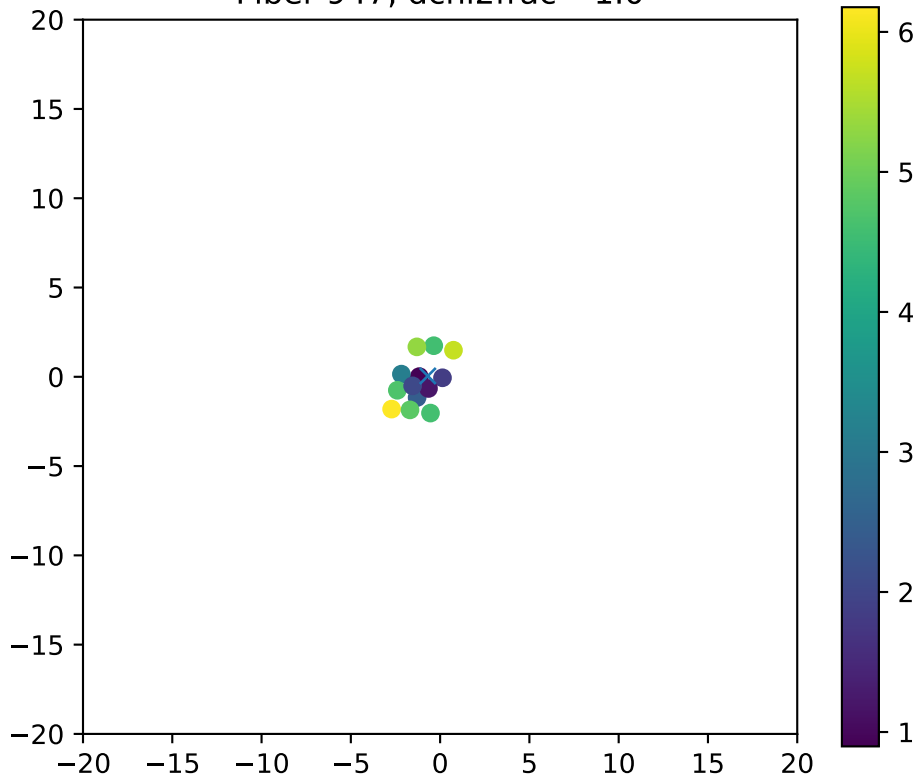
Fiber 947, dchi2frac= 1.0
