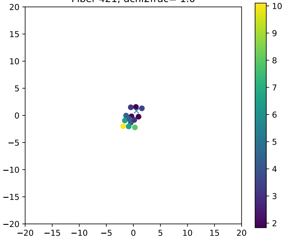
Fiber 421, dchi2frac= 1.0
