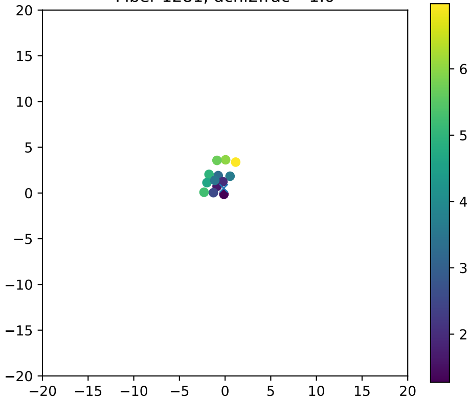
Fiber 1281, dchi2frac= 1.0
