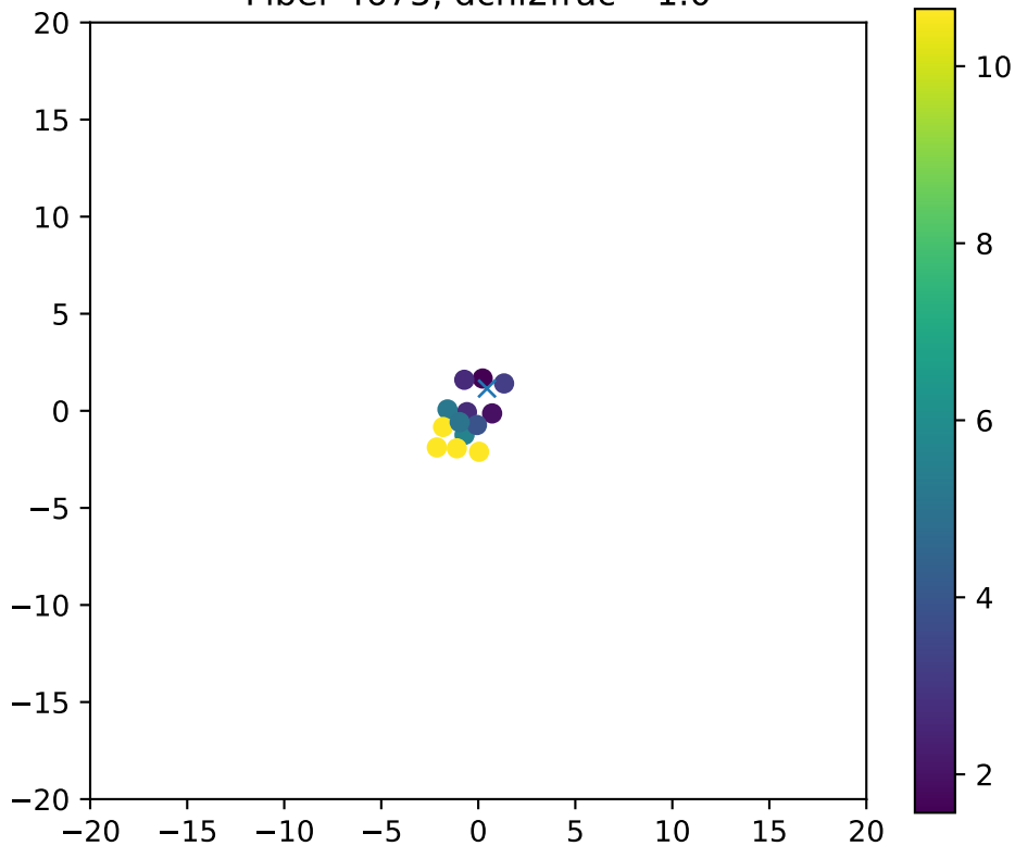
Fiber 4675, dchi2frac= 1.0
