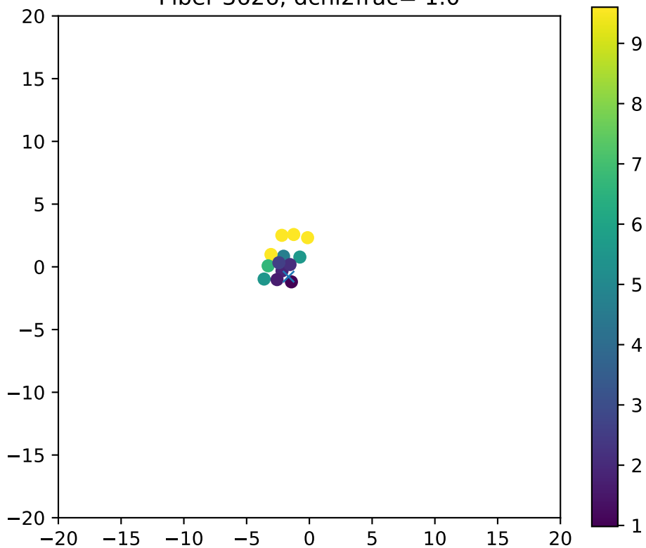
Fiber 3626, dchi2frac= 1.0
