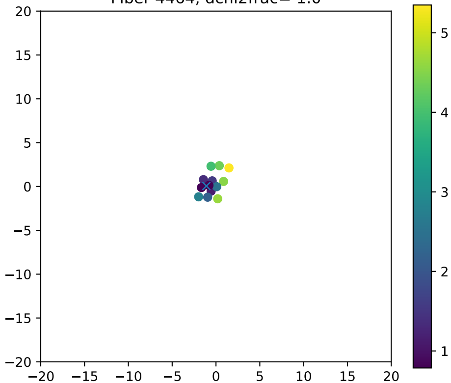
Fiber 4464, dchi2frac= 1.0
