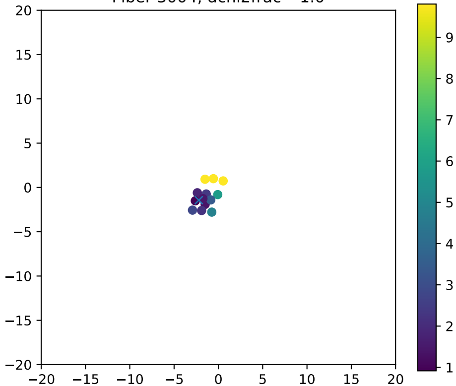
Fiber 3004, dchi2frac= 1.0
