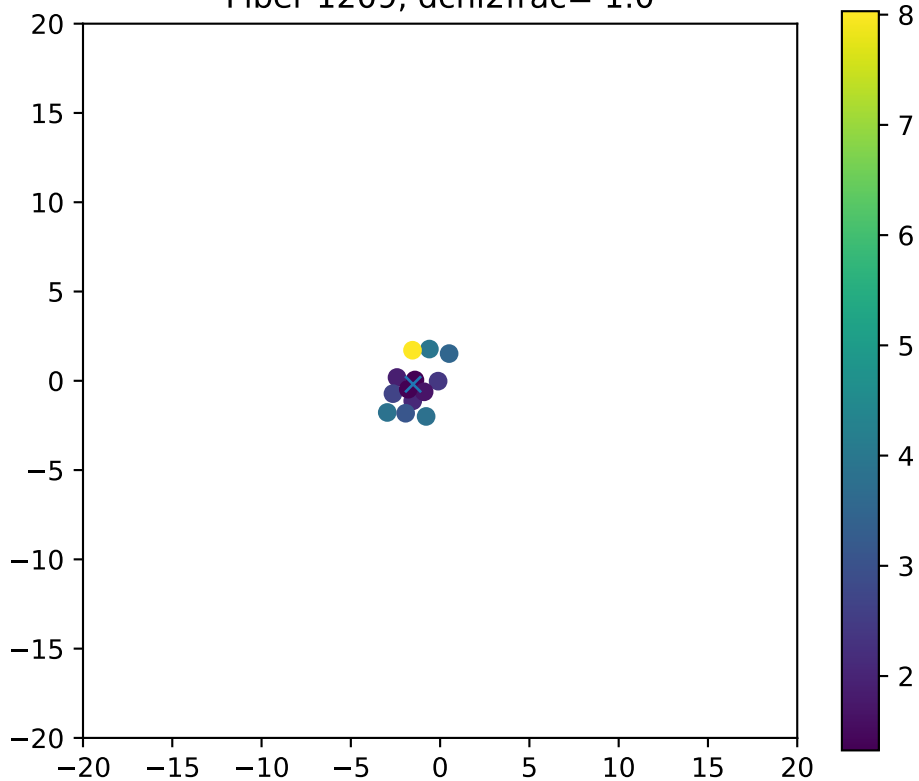
Fiber 1209, dchi2frac= 1.0
