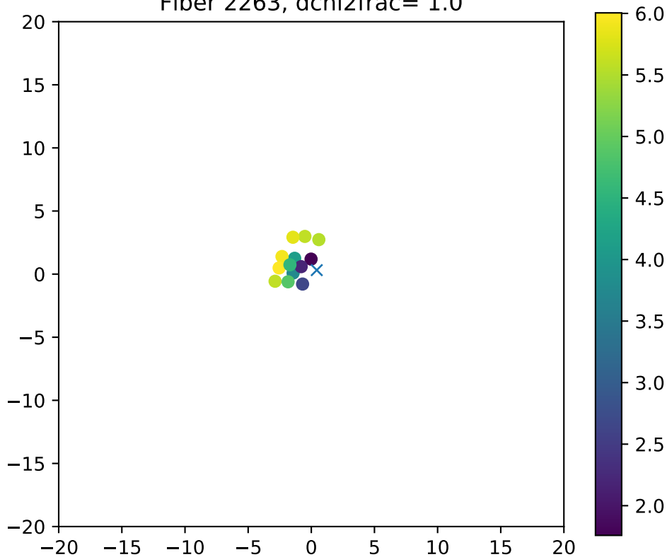
Fiber 2263, dchi2frac= 1.0
