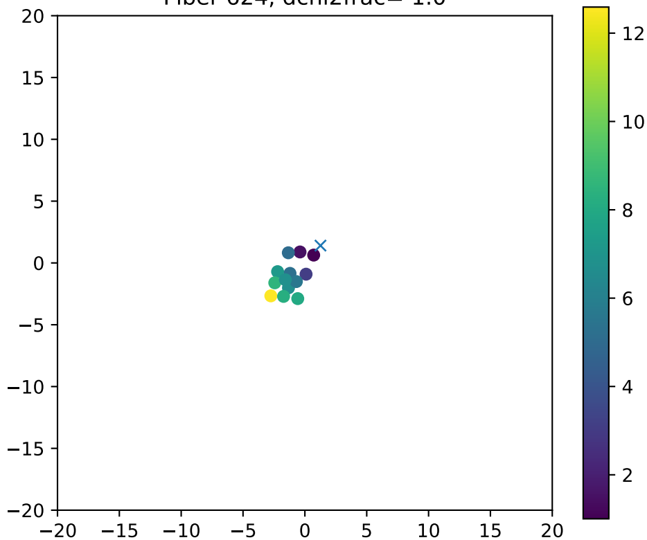
Fiber 624, dchi2frac= 1.0
