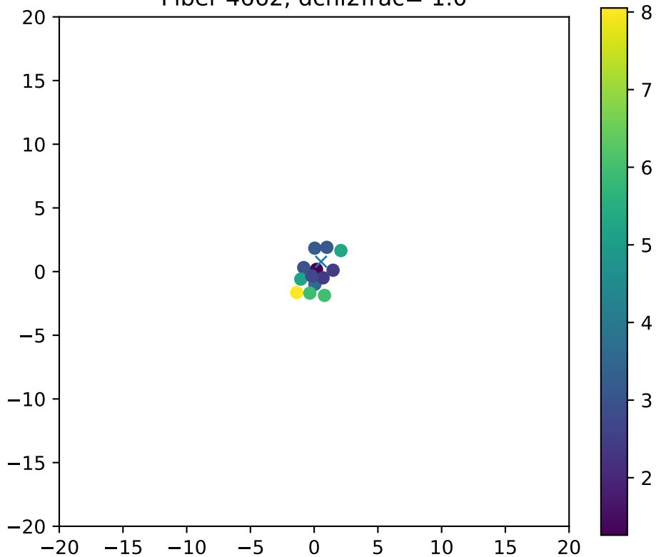
Fiber 4662, dchi2frac= 1.0
