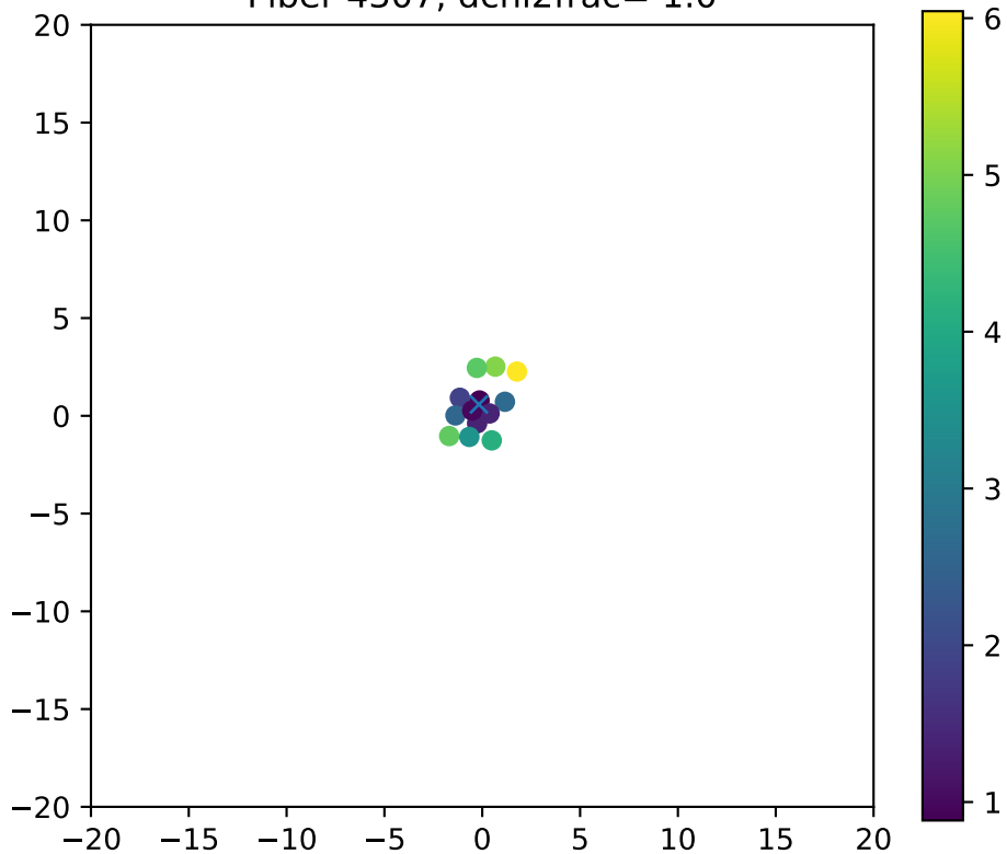
Fiber 4307, dchi2frac= 1.0
