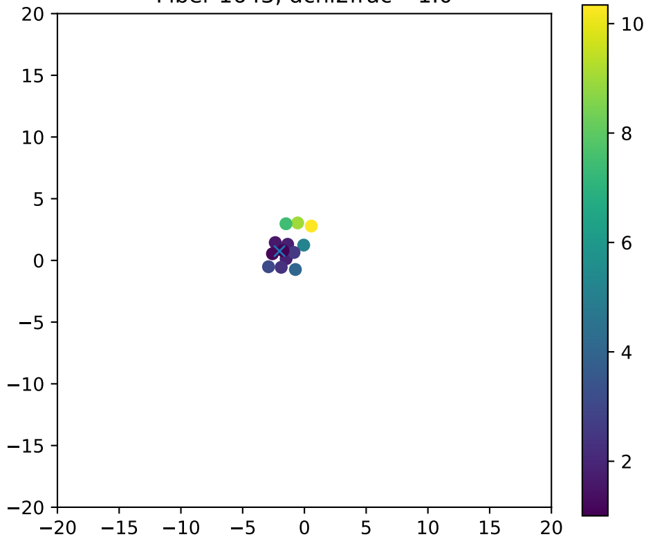
Fiber 1643, dchi2frac= 1.0
