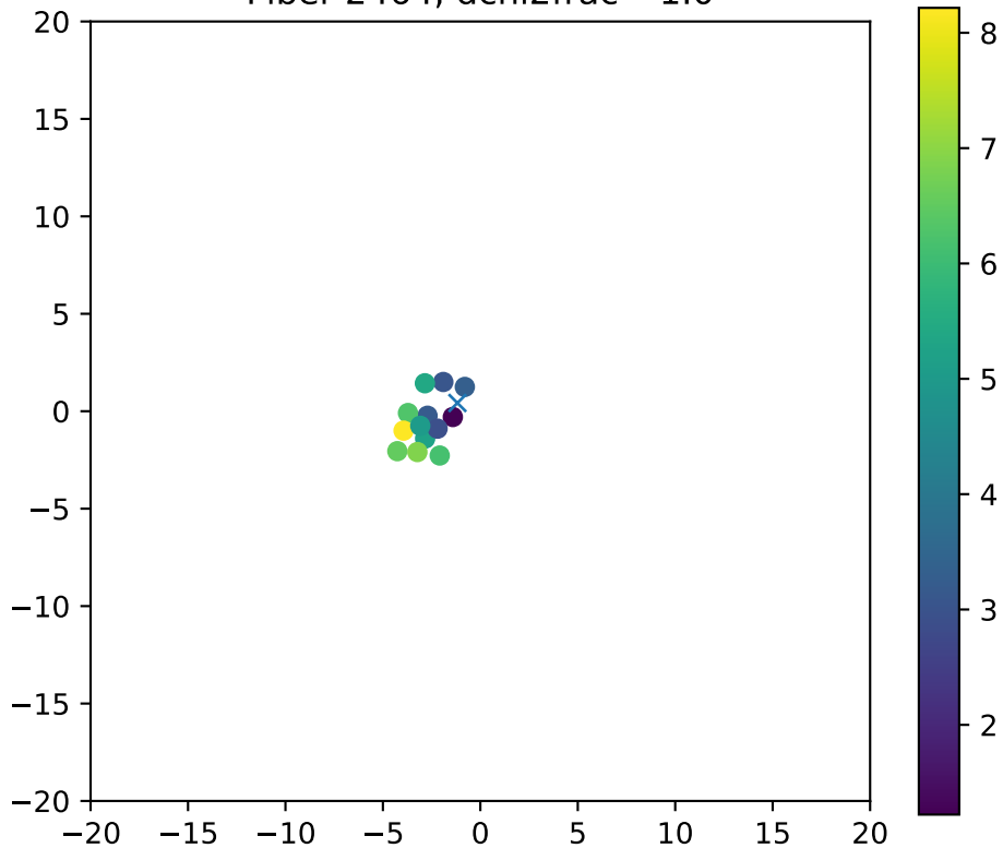
Fiber 2464, dchi2frac= 1.0
