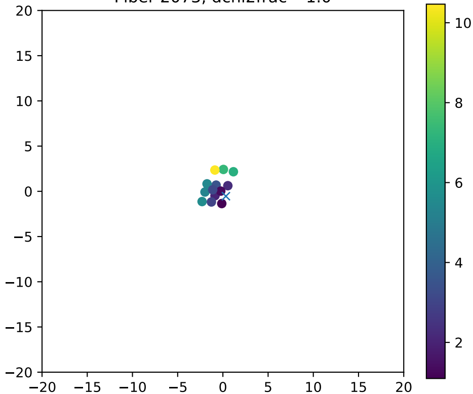
Fiber 2073, dchi2frac= 1.0
