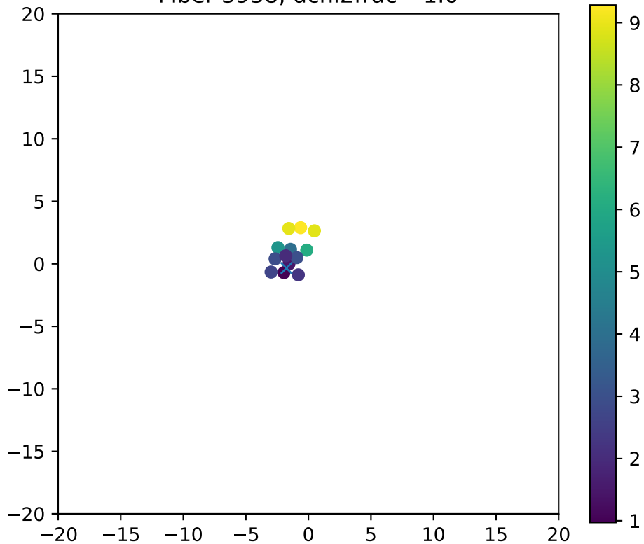
Fiber 3938, dchi2frac= 1.0
