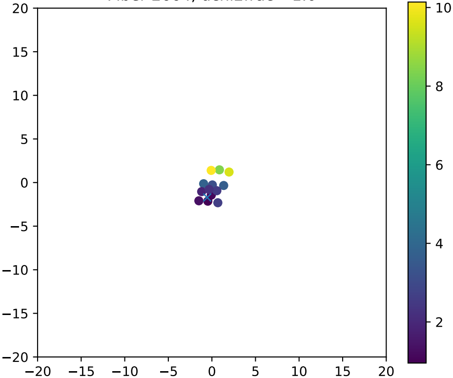
Fiber 2664, dchi2frac= 1.0
