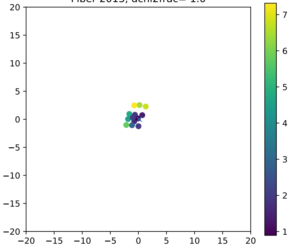
Fiber 2013, dchi2frac= 1.0
