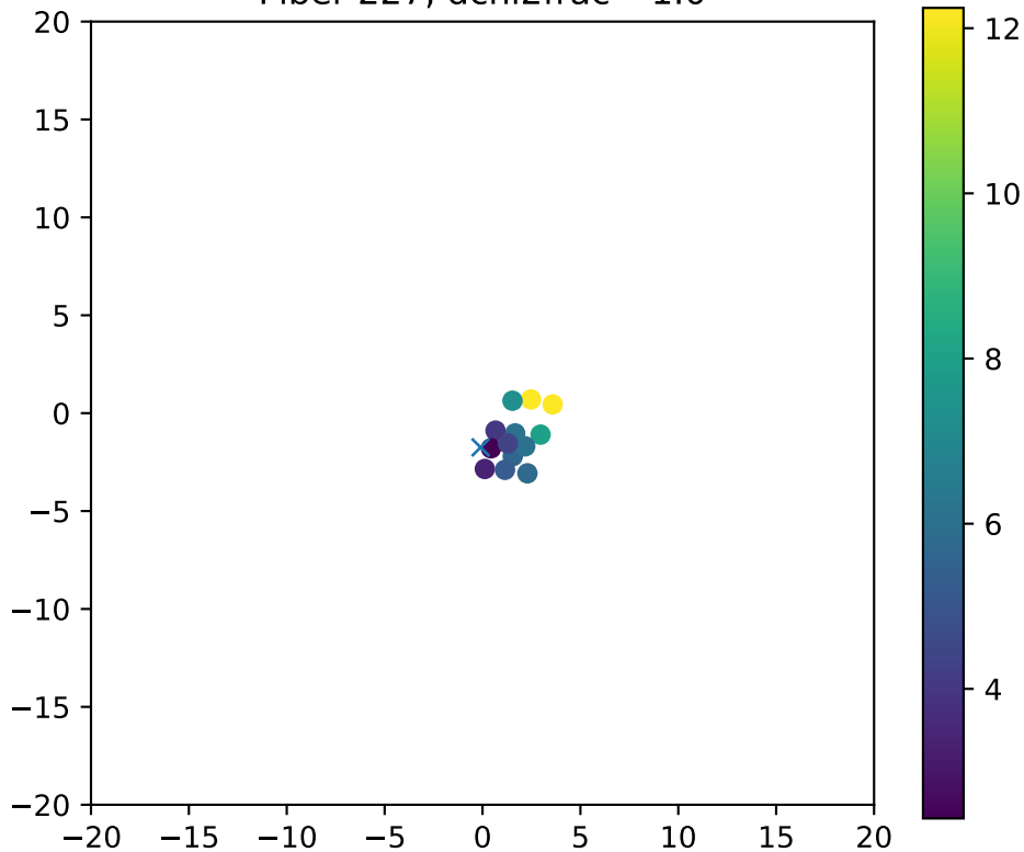
Fiber 227, dchi2frac= 1.0
