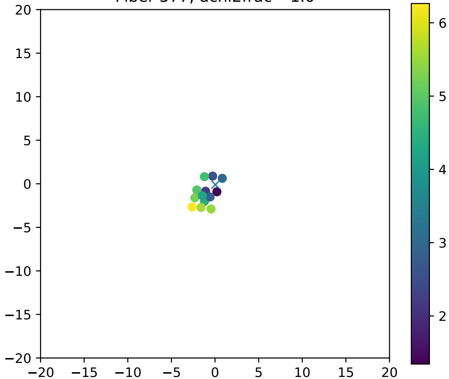
Fiber 577, dchi2frac= 1.0
