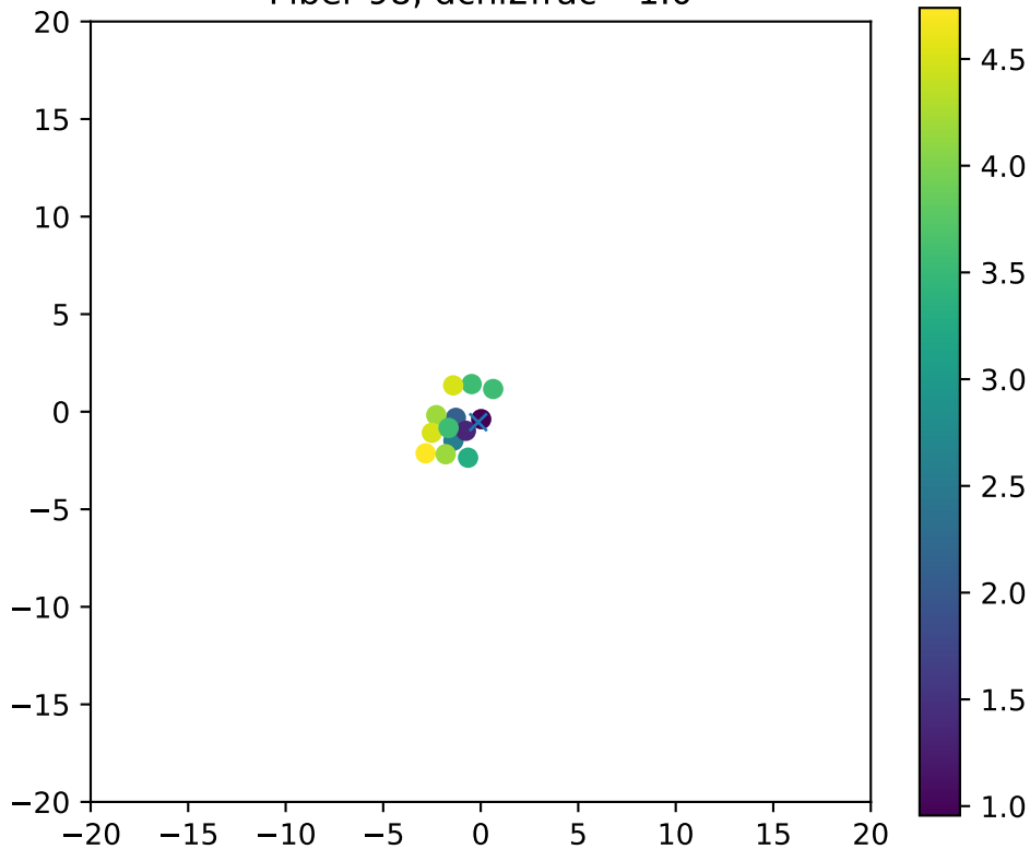
Fiber 98, dchi2frac= 1.0
