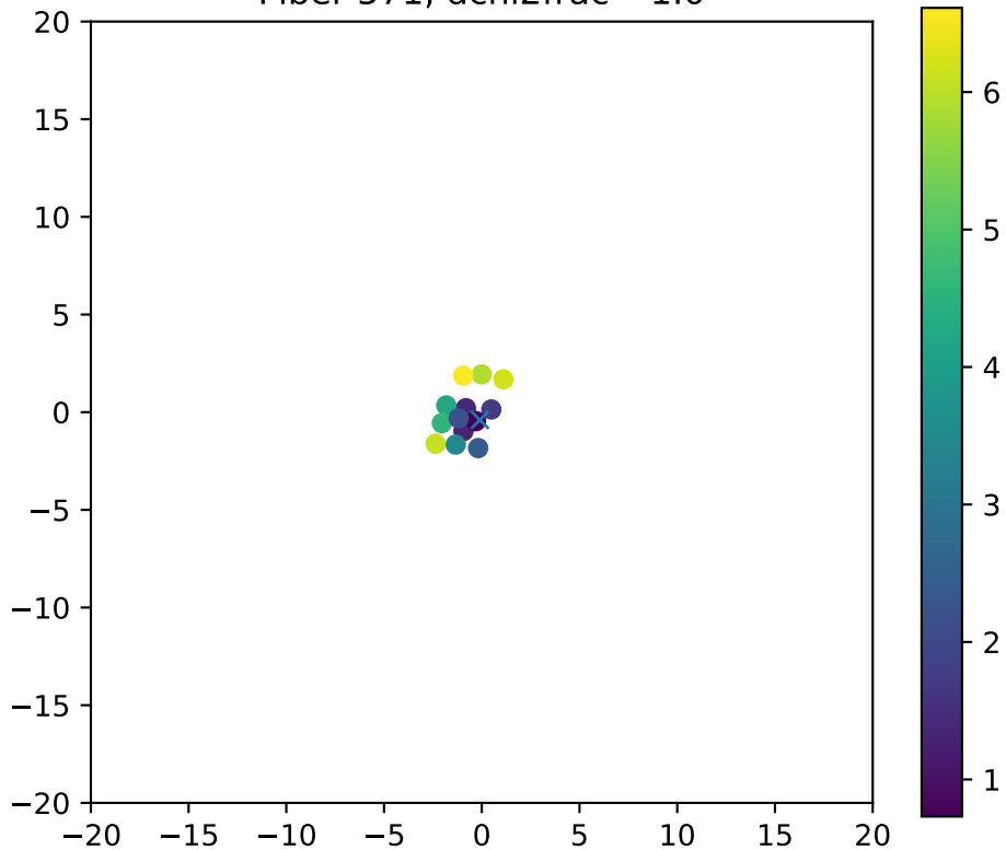
Fiber 571, dchi2frac= 1.0
