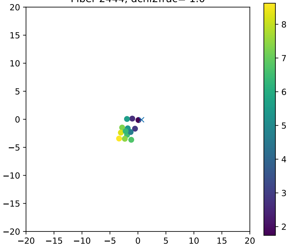
Fiber 2444, dchi2frac= 1.0
