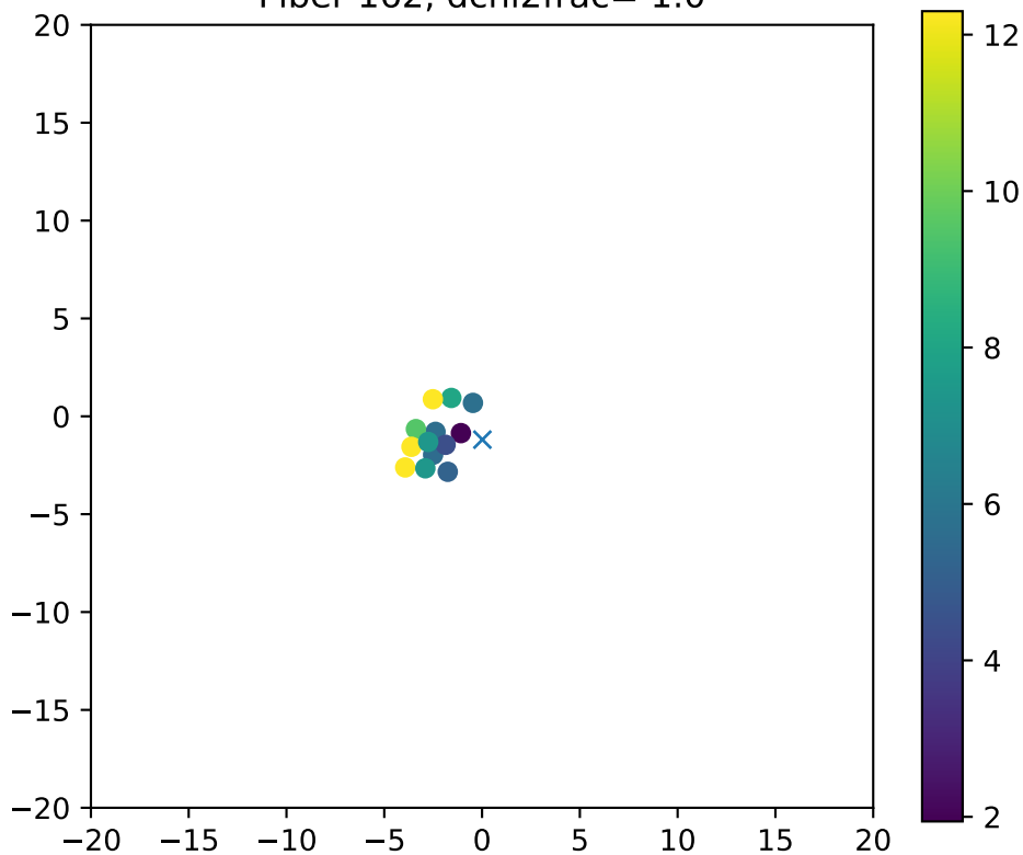
Fiber 162, dchi2frac= 1.0
