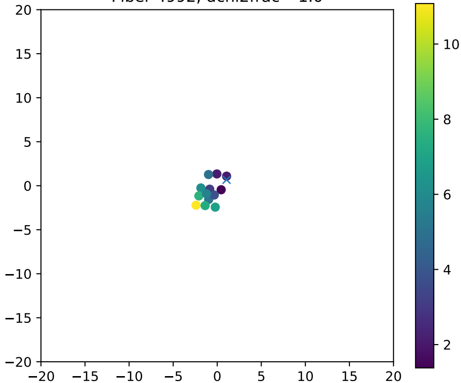
Fiber 4992, dchi2frac= 1.0
