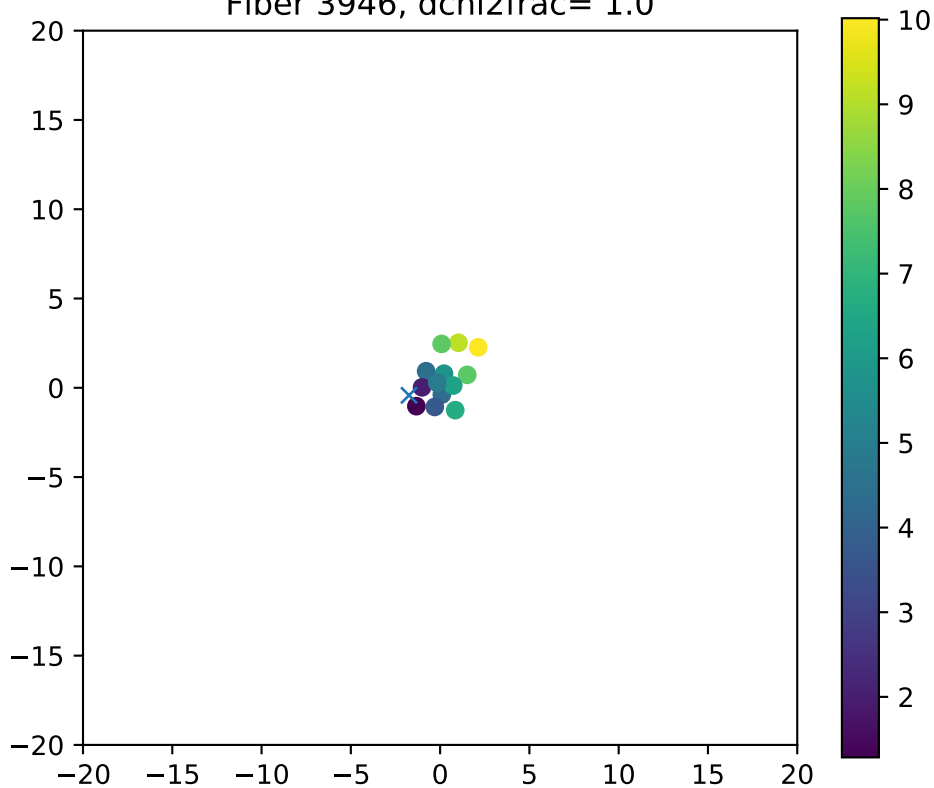
Fiber 3946, dchi2frac= 1.0
