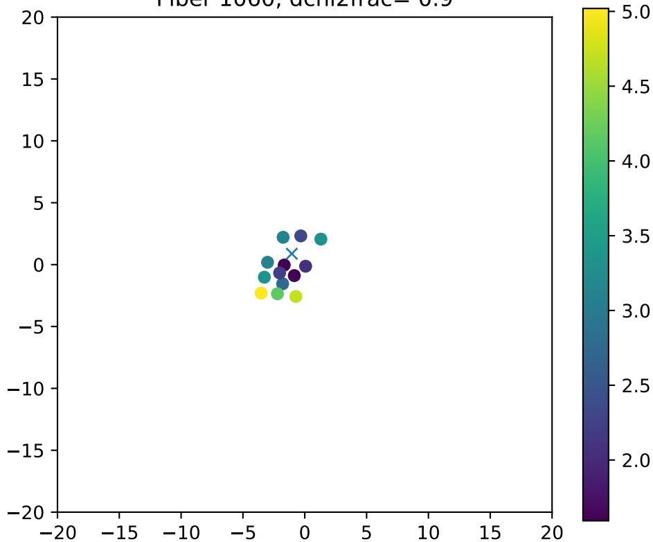
Fiber 1060, dchi2frac= 0.9
