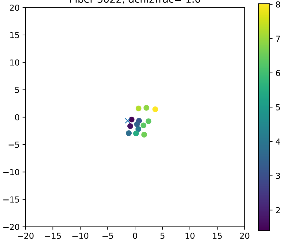
Fiber 3022, dchi2frac= 1.0
