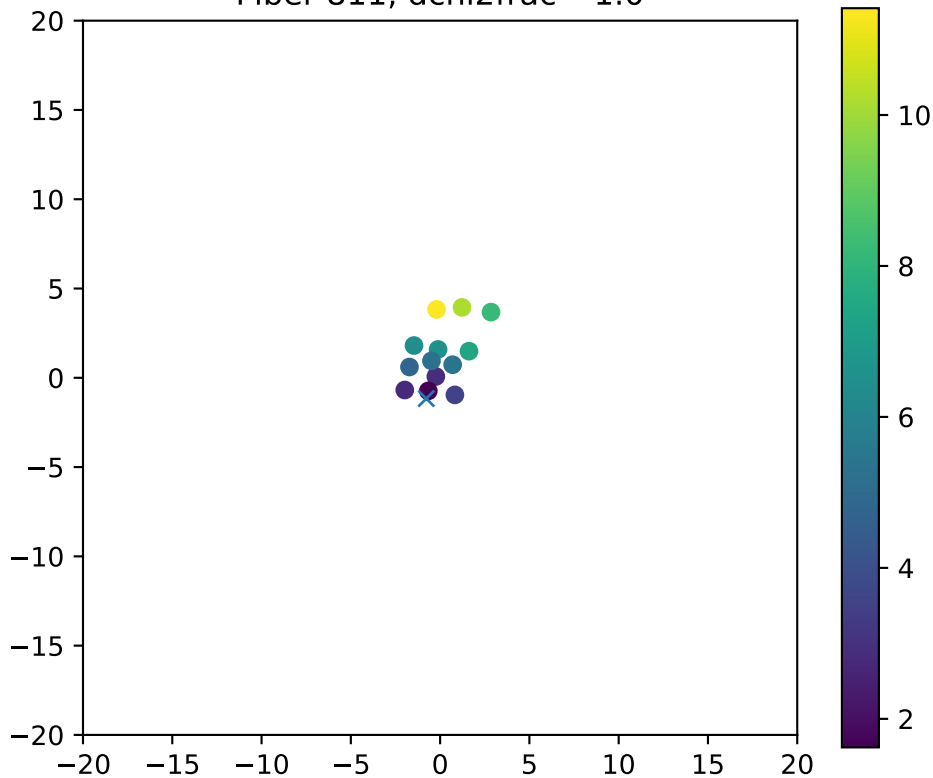
Fiber 811, dchi2frac= 1.0
