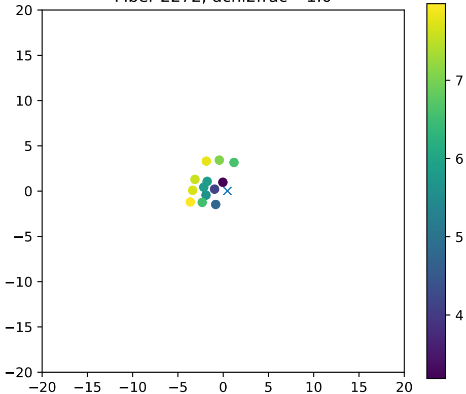
Fiber 2272, dchi2frac= 1.0
