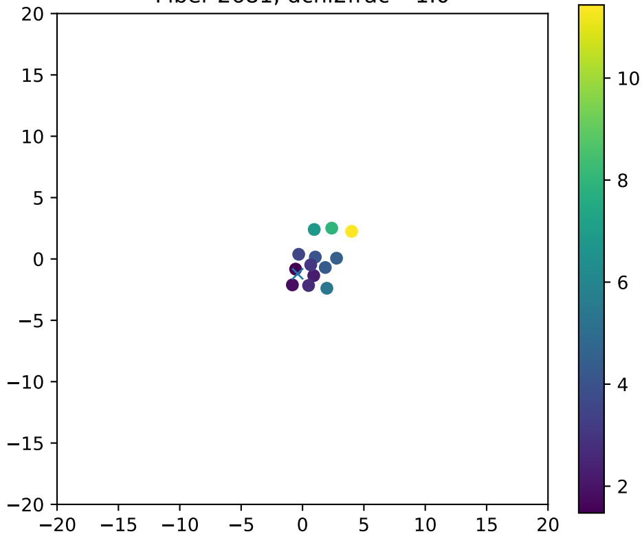
Fiber 2681, dchi2frac= 1.0
