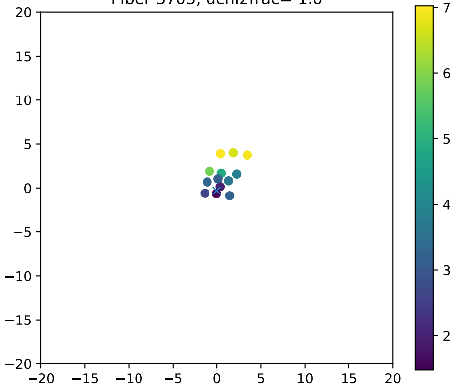
Fiber 3705, dchi2frac= 1.0
