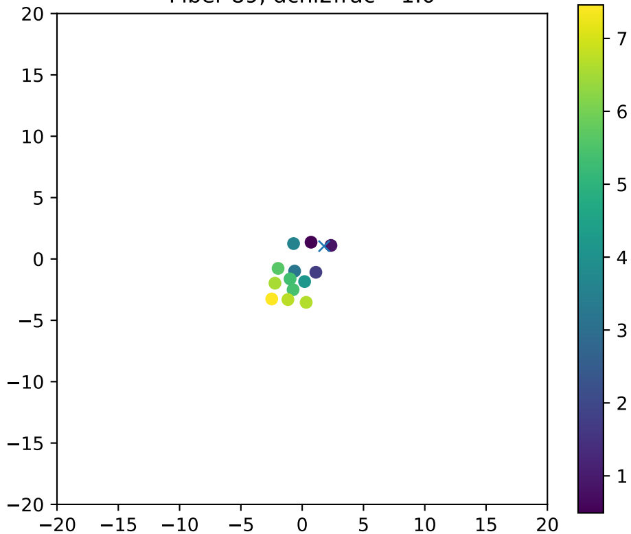
Fiber 89, dchi2frac= 1.0
