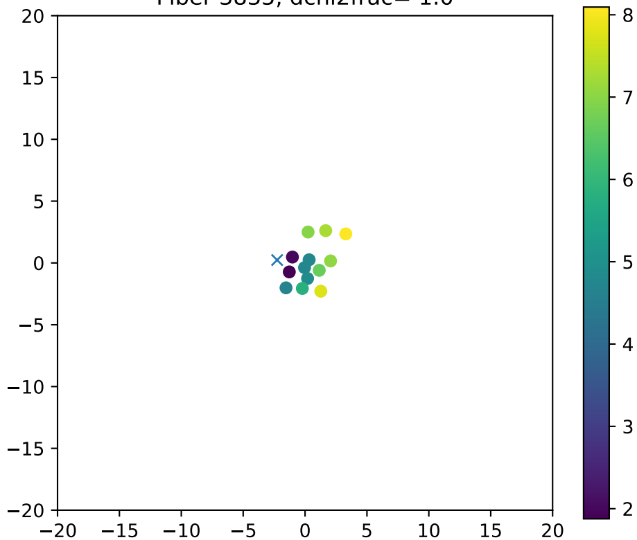
Fiber 3835, dchi2frac= 1.0
