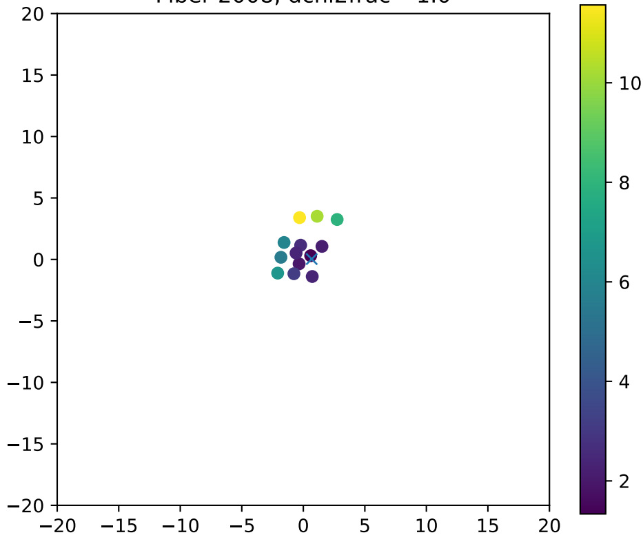
Fiber 2008, dchi2frac= 1.0
