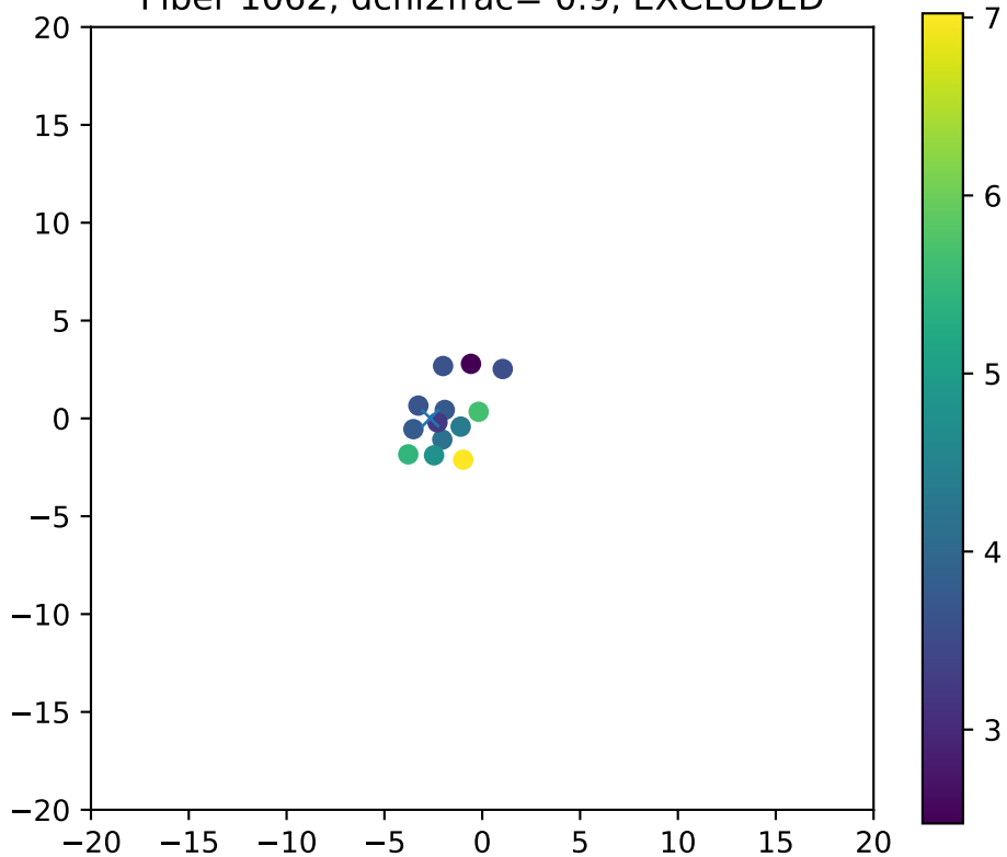
Fiber 1062, dchi2frac= 0.9, EXCLUDED
