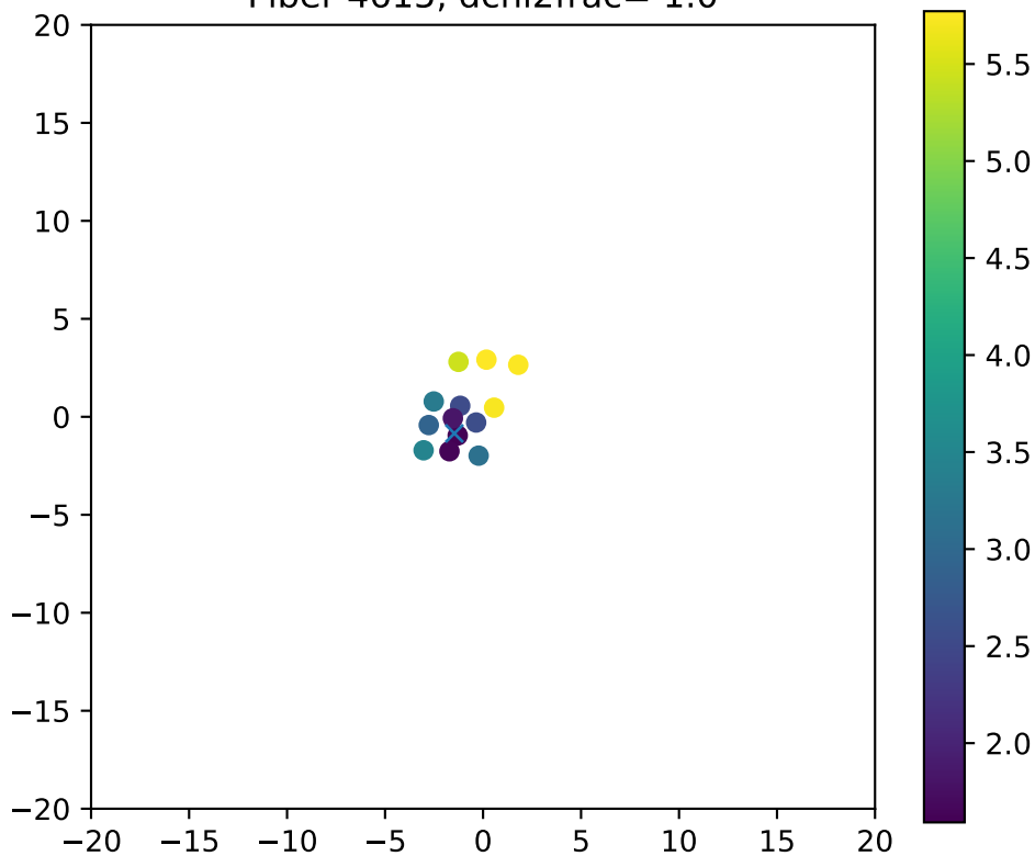
Fiber 4615, dchi2frac= 1.0
