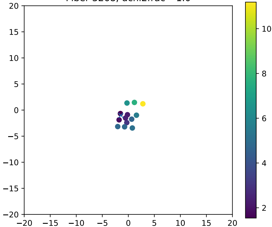
Fiber 3268, dchi2frac= 1.0
