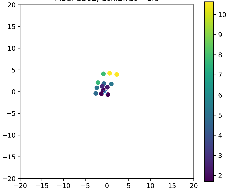
Fiber 3502, dchi2frac= 1.0
