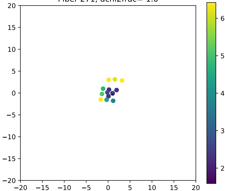
Fiber 271, dchi2frac= 1.0
