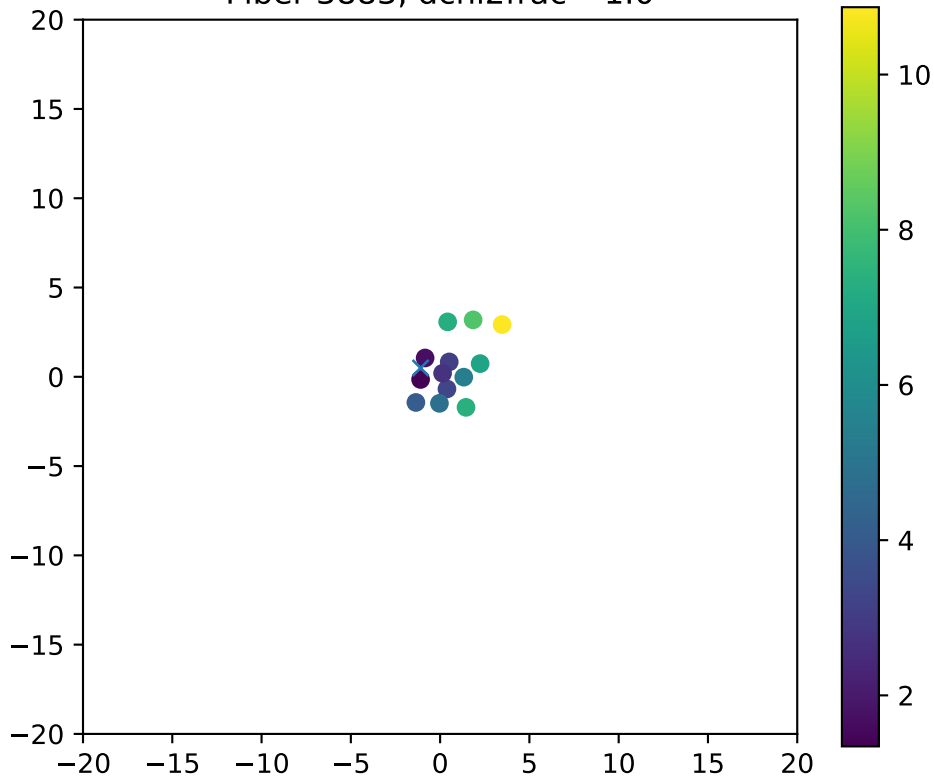
Fiber 3883, dchi2frac= 1.0
