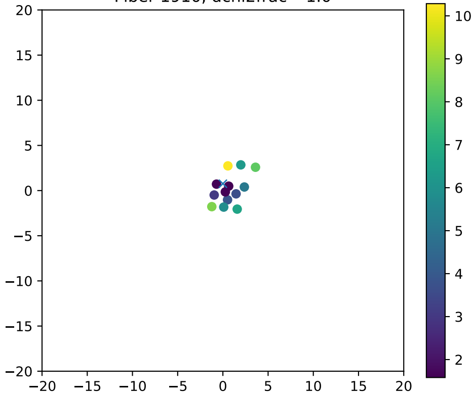
Fiber 1910, dchi2frac= 1.0
