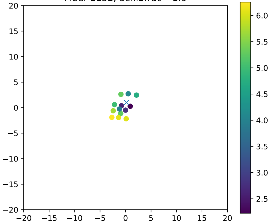
Fiber 2152, dchi2frac= 1.0
