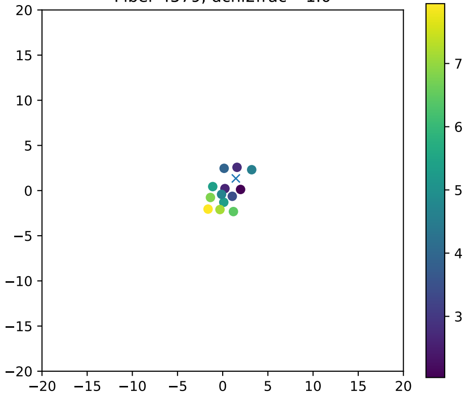
Fiber 4579, dchi2frac= 1.0
