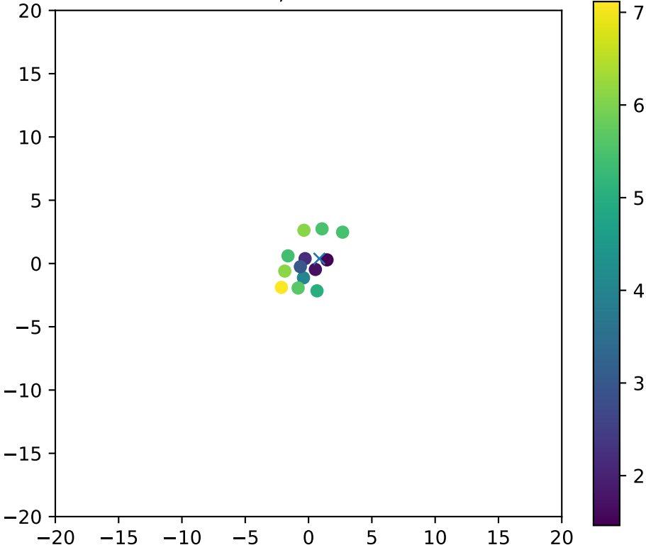
Fiber 2095, dchi2frac= 1.0
