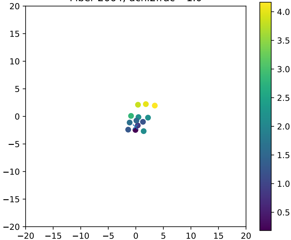
Fiber 2664, dchi2frac= 1.0
