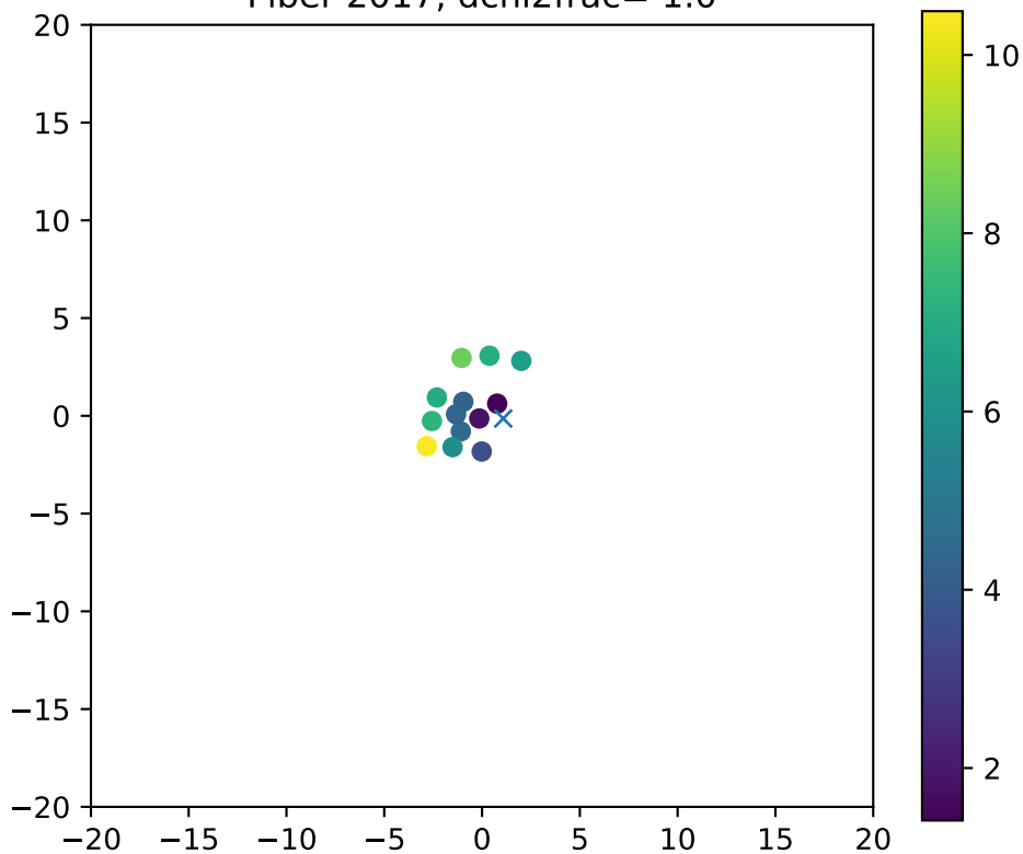
Fiber 2017, dchi2frac= 1.0
