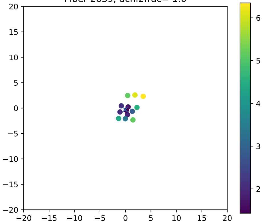
Fiber 2639, dchi2frac= 1.0
