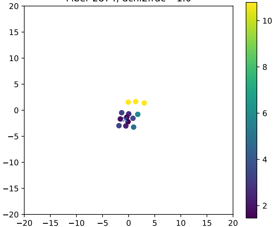
Fiber 2874, dchi2frac= 1.0
