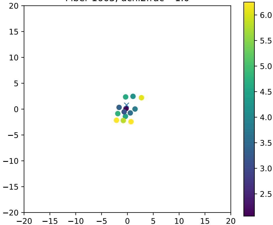
Fiber 1663, dchi2frac= 1.0
