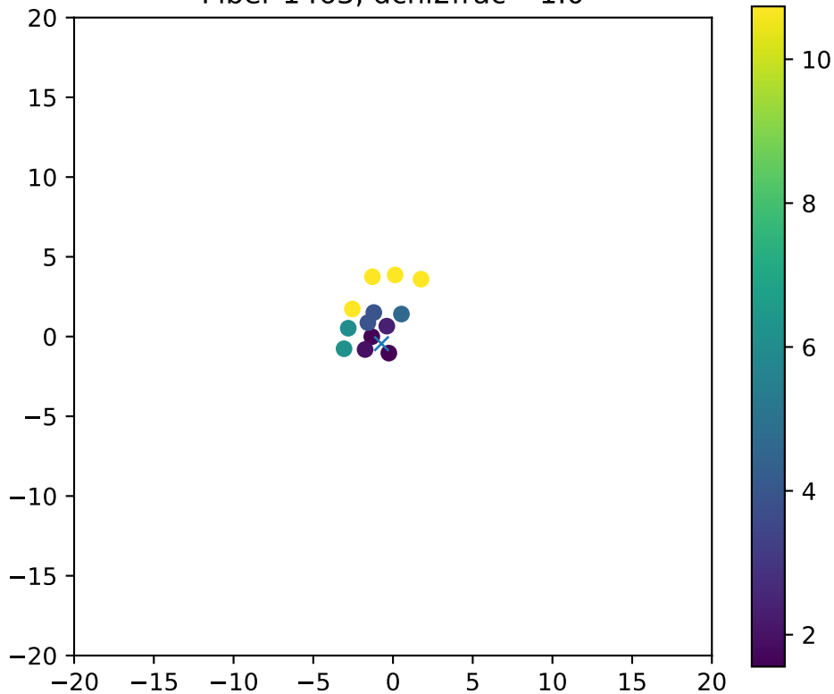
Fiber 1463, dchi2frac= 1.0
