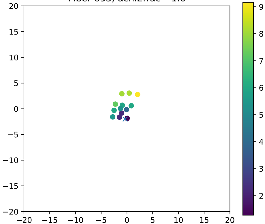
Fiber 653, dchi2frac= 1.0
