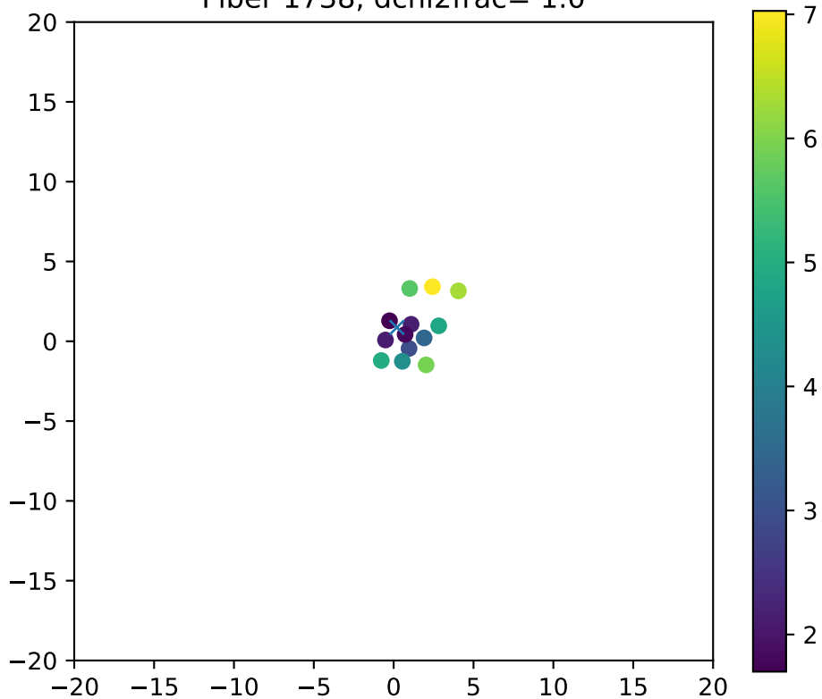
Fiber 1738, dchi2frac= 1.0
