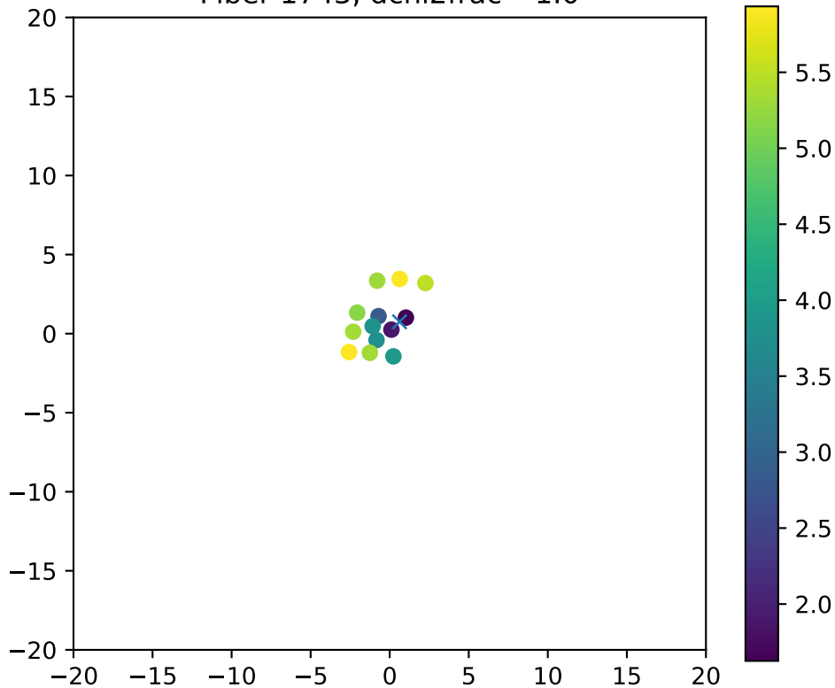
Fiber 1743, dchi2frac= 1.0
