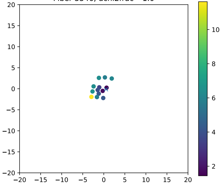
Fiber 3346, dchi2frac= 1.0
