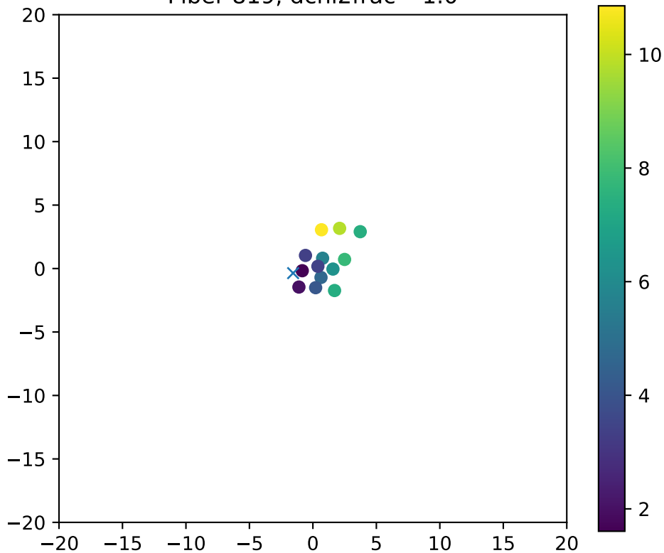
Fiber 819, dchi2frac= 1.0
