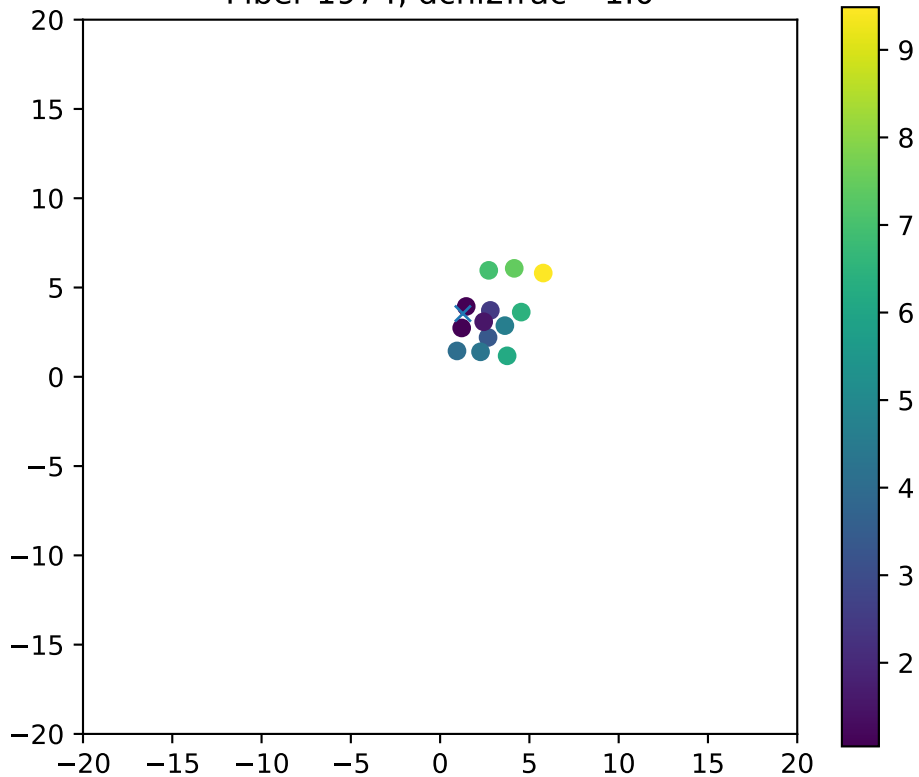
Fiber 1974, dchi2frac= 1.0
