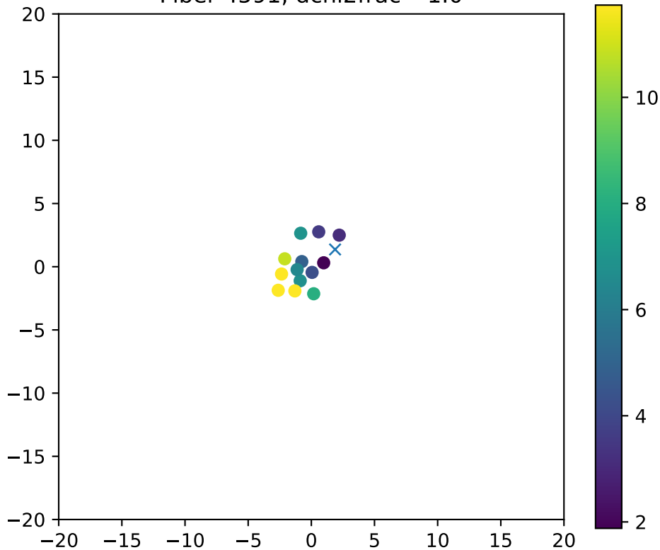
Fiber 4591, dchi2frac= 1.0
