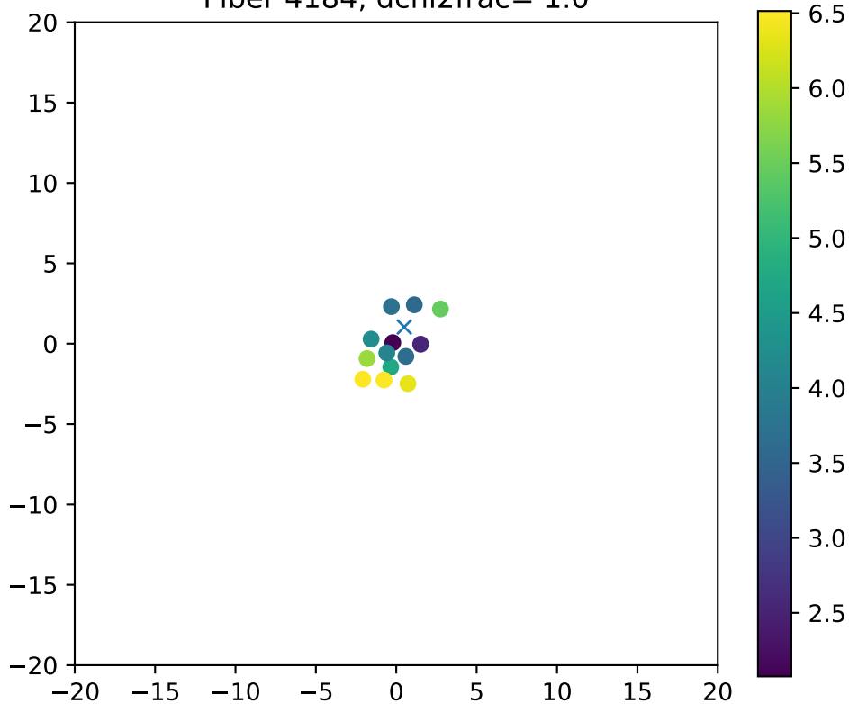
Fiber 4184, dchi2frac= 1.0
