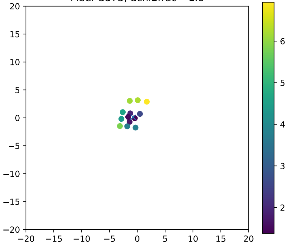
Fiber 3575, dchi2frac= 1.0
