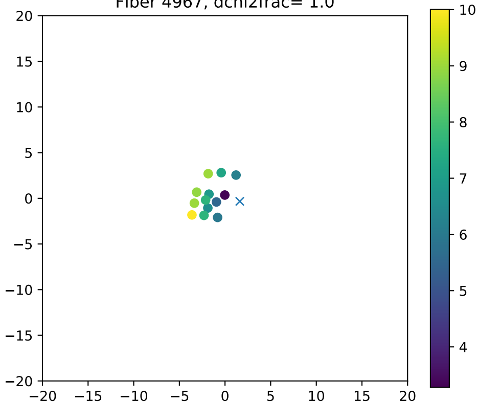
Fiber 4967, dchi2frac= 1.0
