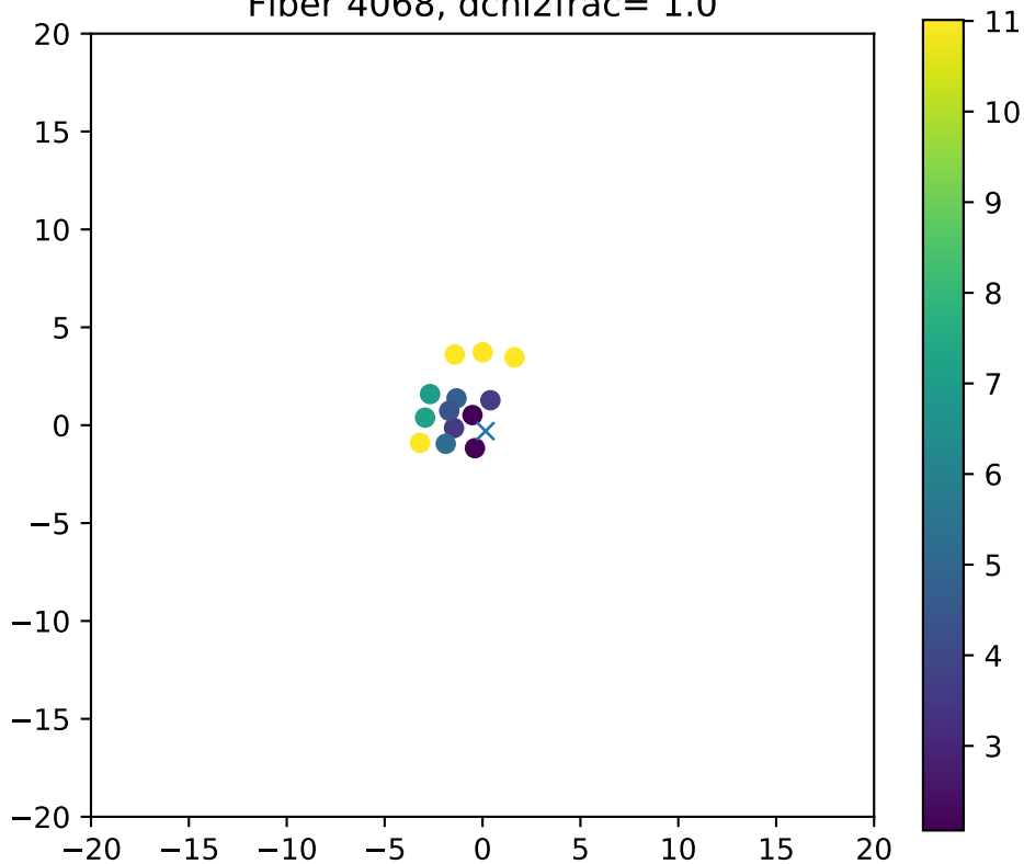
Fiber 4068, dchi2frac= 1.0
