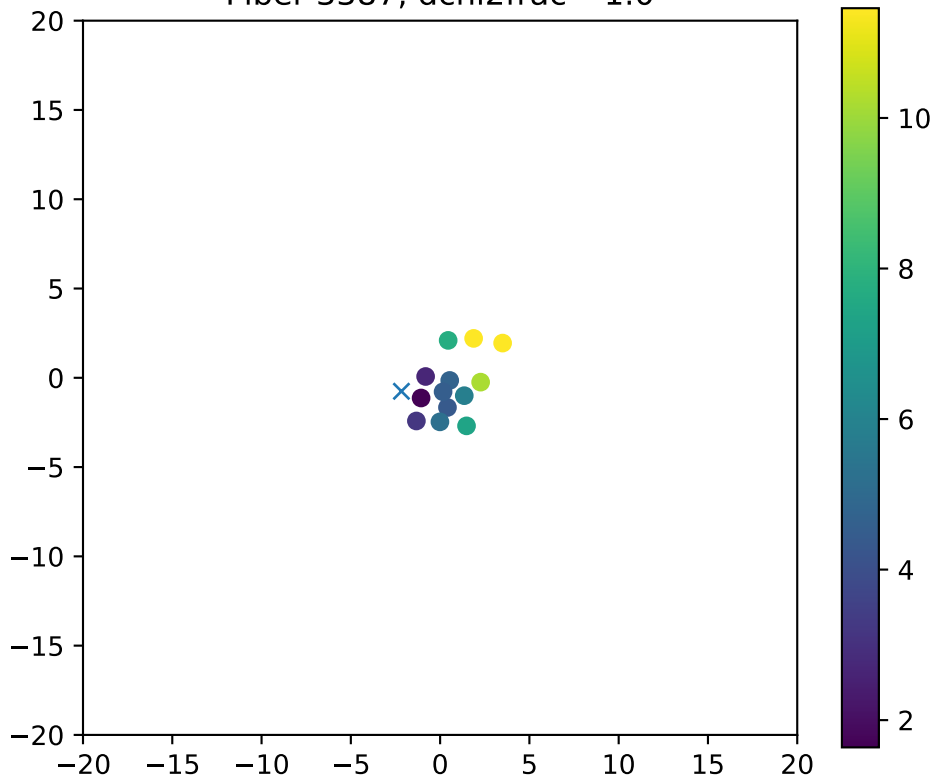
Fiber 3387, dchi2frac= 1.0
