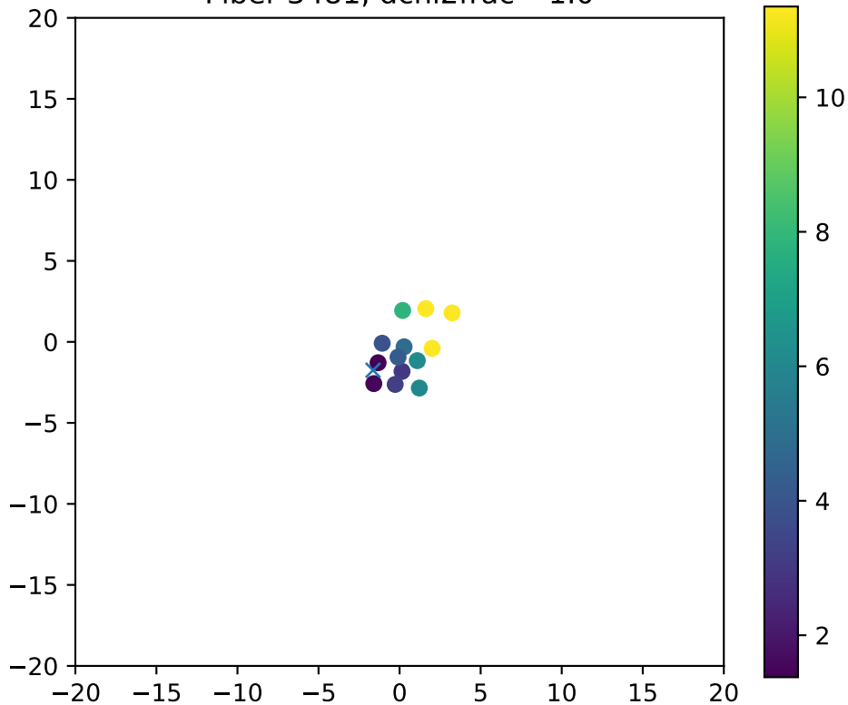
Fiber 3481, dchi2frac= 1.0
