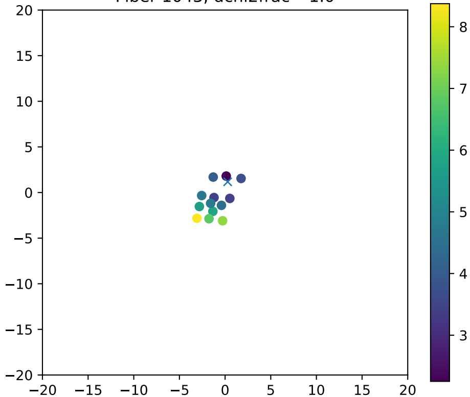
Fiber 1043, dchi2frac= 1.0
