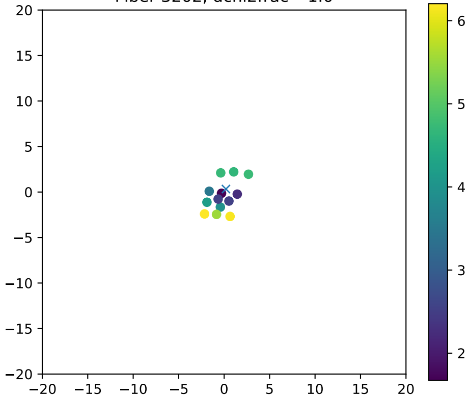
Fiber 3202, dchi2frac= 1.0
