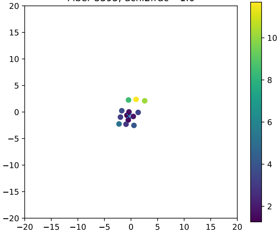
Fiber 3395, dchi2frac= 1.0
