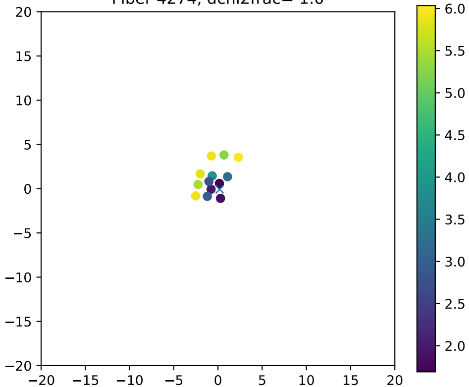
Fiber 4274, dchi2frac= 1.0
