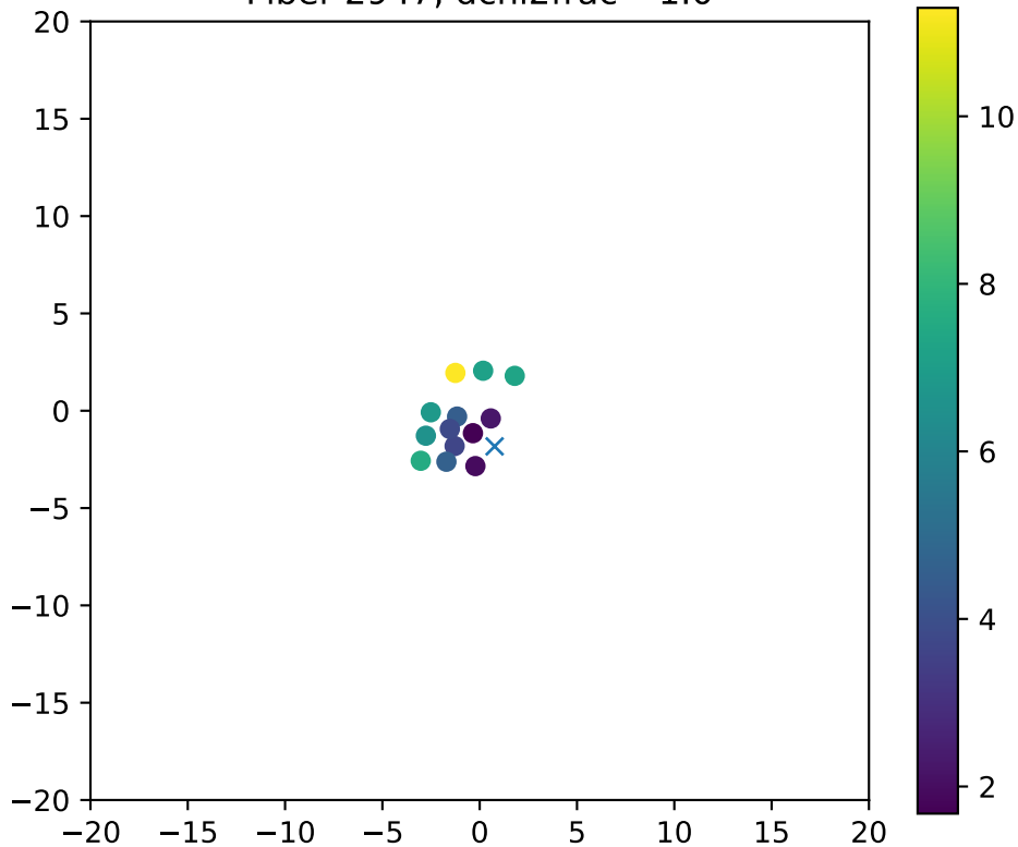
Fiber 2947, dchi2frac= 1.0
