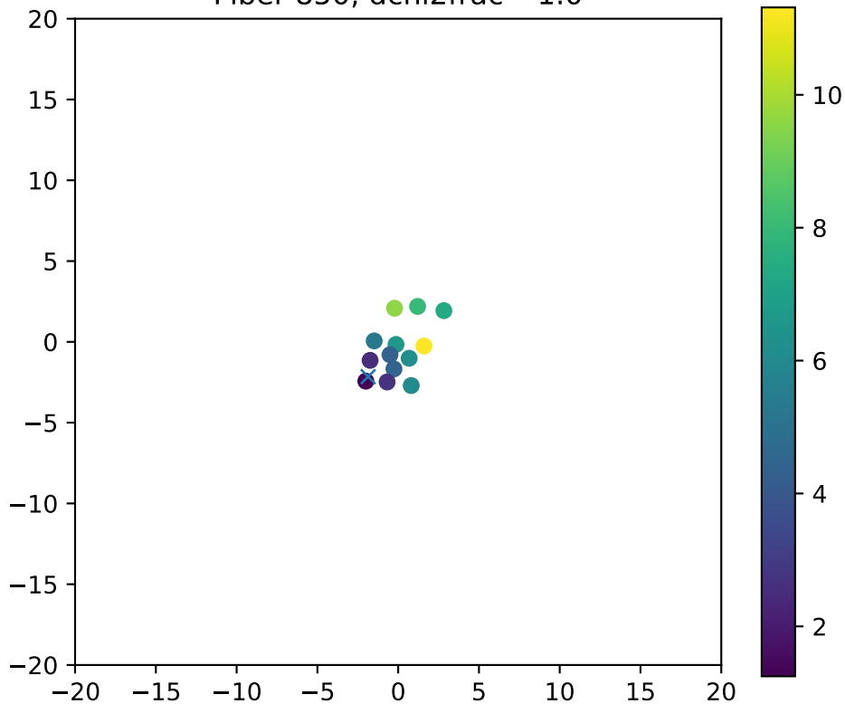
Fiber 850, dchi2frac= 1.0
