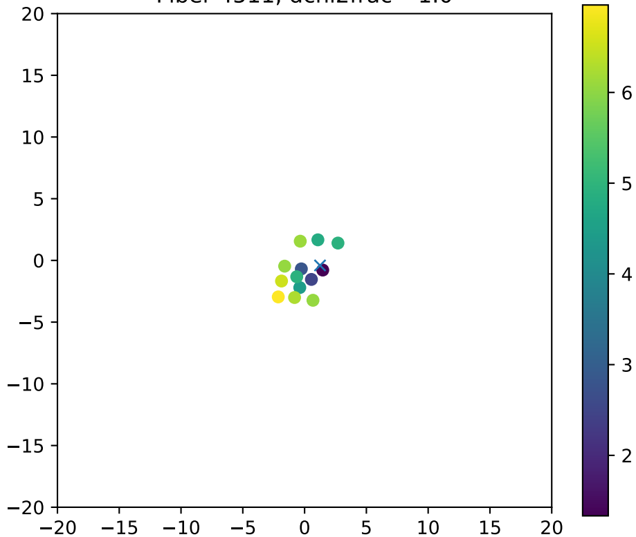
Fiber 4511, dchi2frac= 1.0
