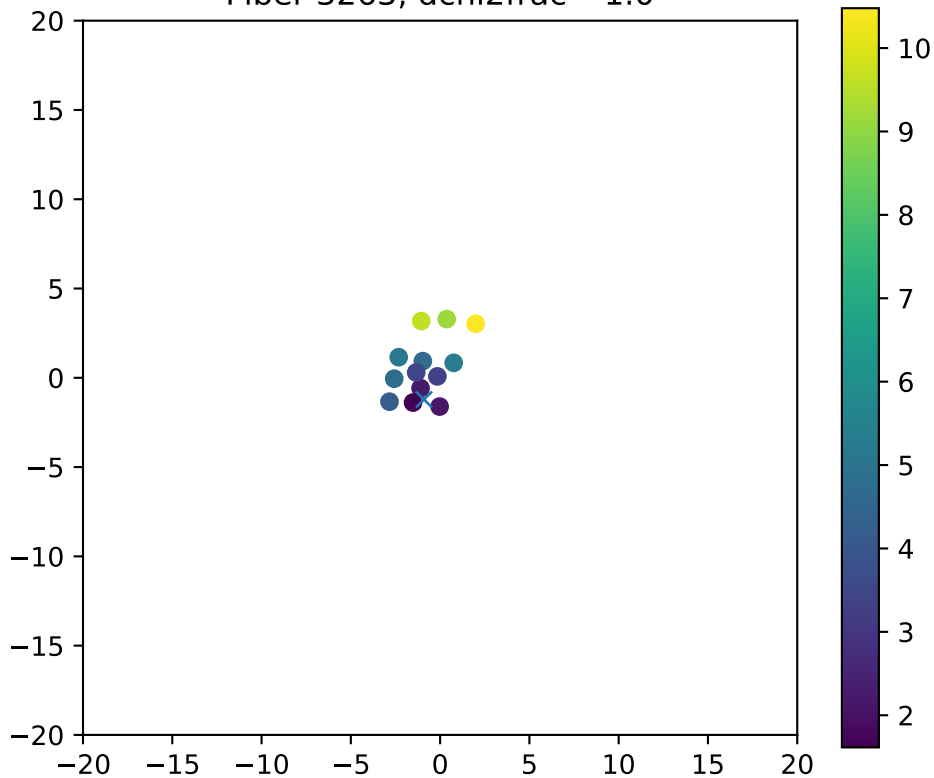
Fiber 3263, dchi2frac= 1.0
