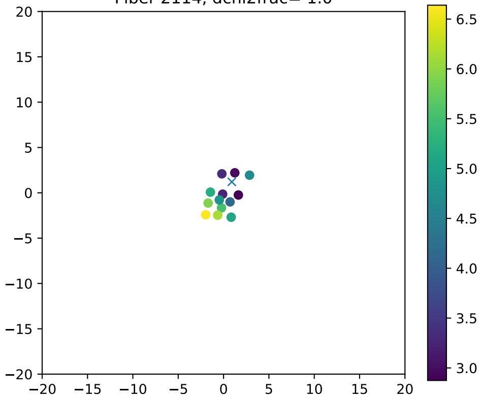
Fiber 2114, dchi2frac= 1.0
