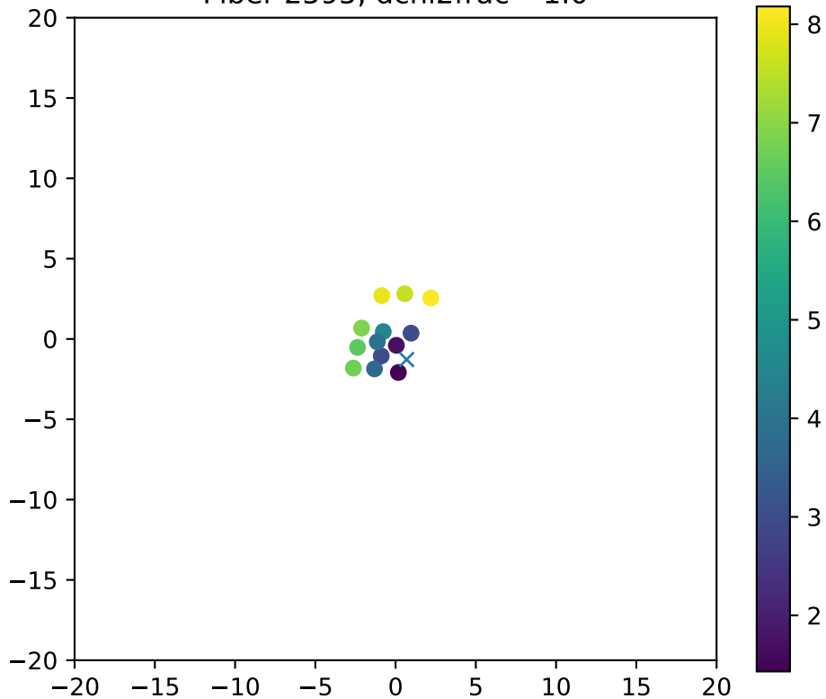
Fiber 2595, dchi2frac= 1.0
