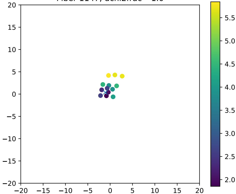
Fiber 1147, dchi2frac= 1.0
