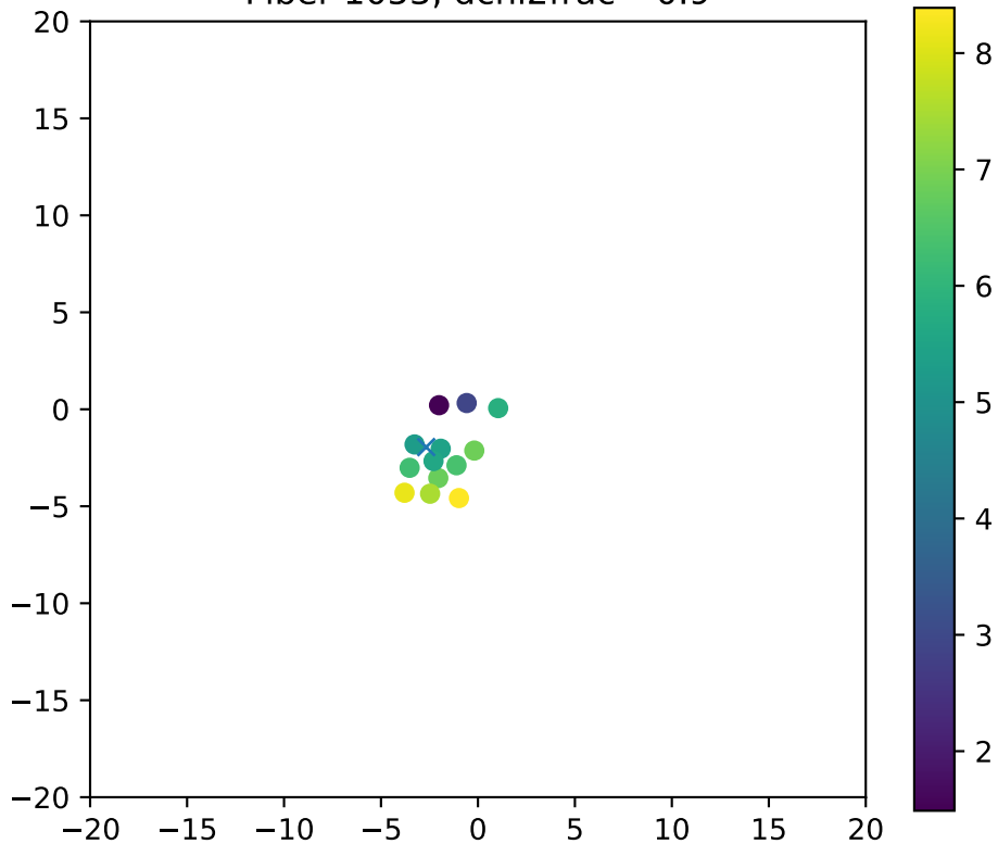
Fiber 1053, dchi2frac= 0.9
