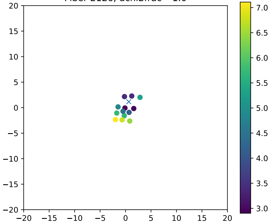
Fiber 2126, dchi2frac= 1.0
