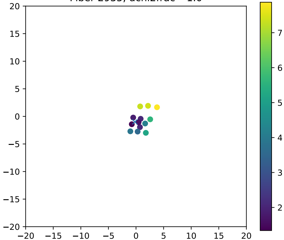
Fiber 2935, dchi2frac= 1.0
