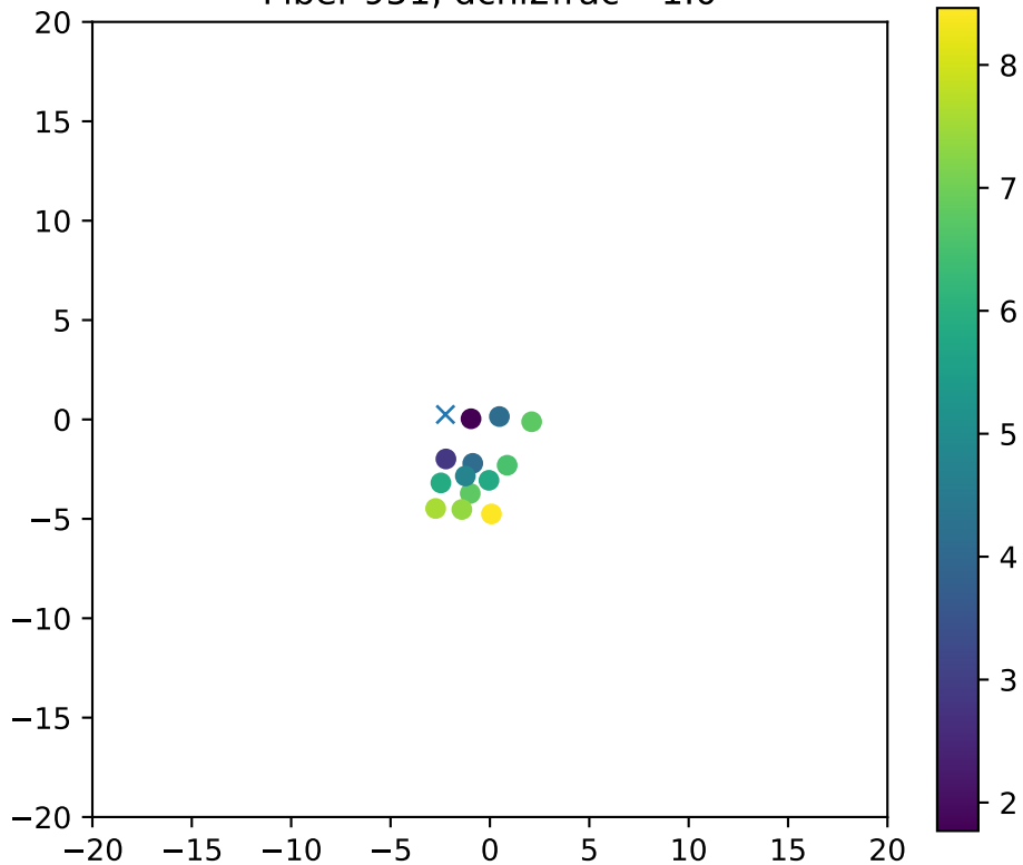
Fiber 951, dchi2frac= 1.0
