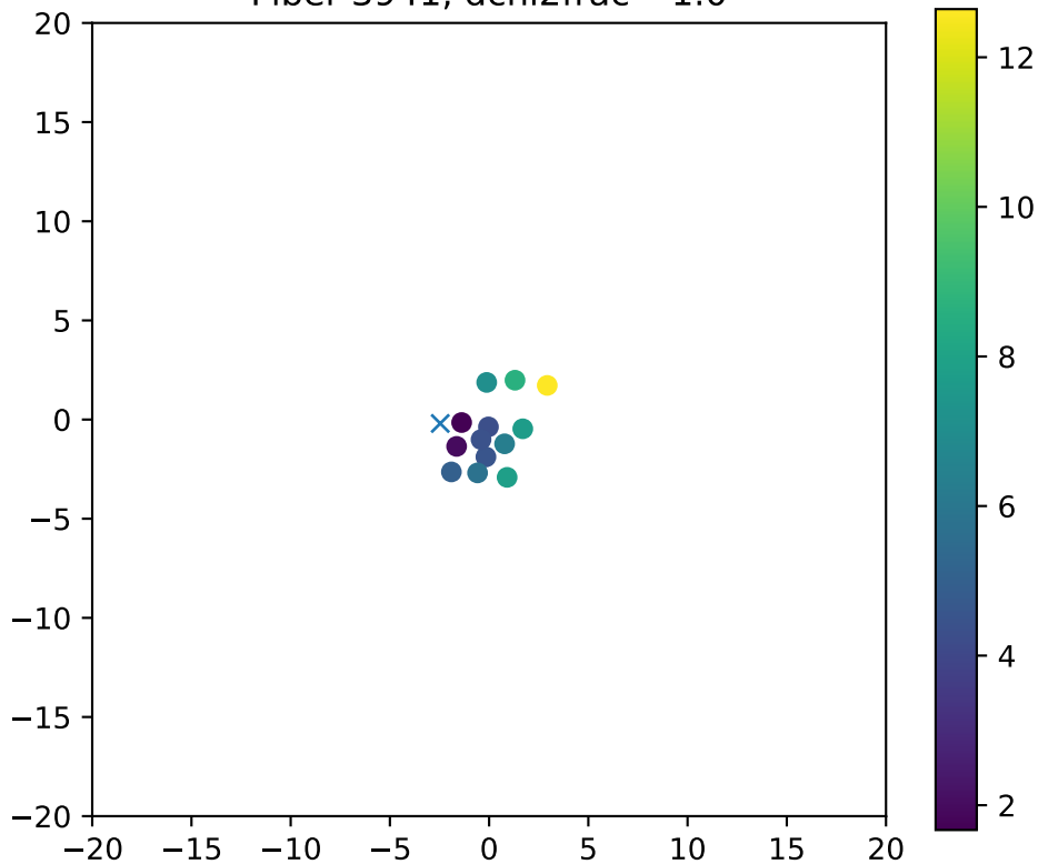
Fiber 3941, dchi2frac= 1.0
