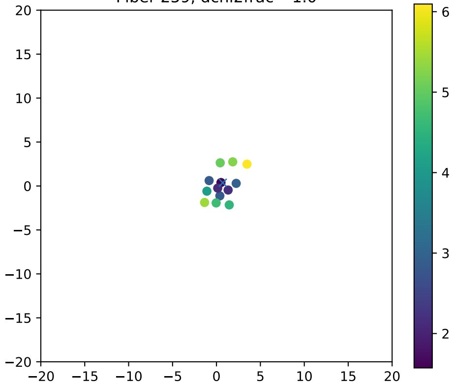
Fiber 259, dchi2frac= 1.0
