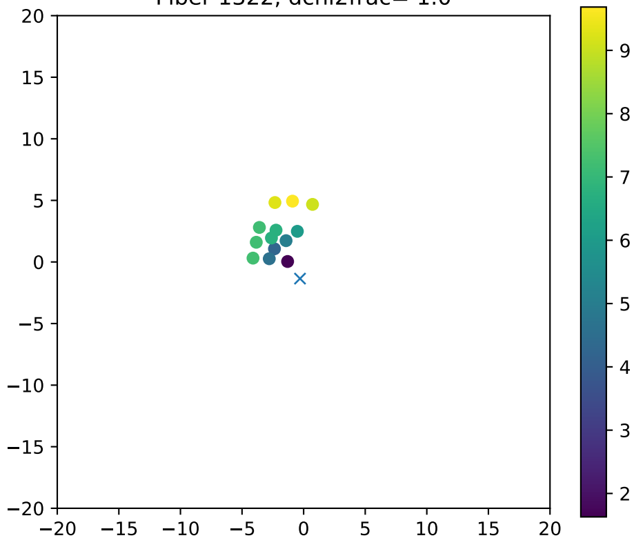
Fiber 1322, dchi2frac= 1.0
