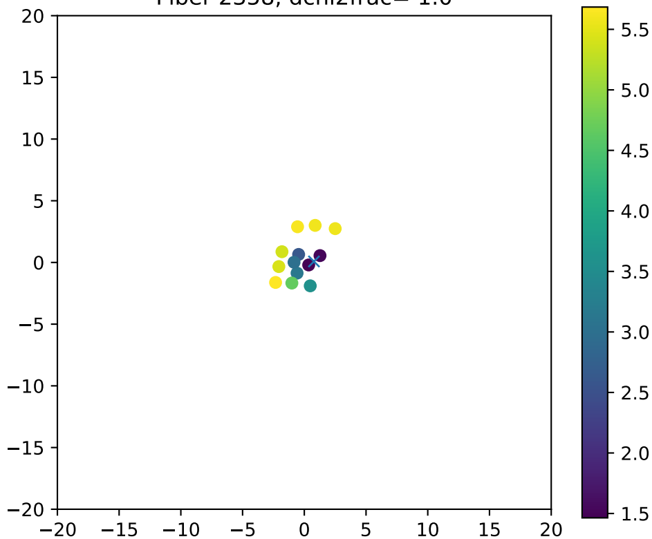
Fiber 2358, dchi2frac= 1.0
