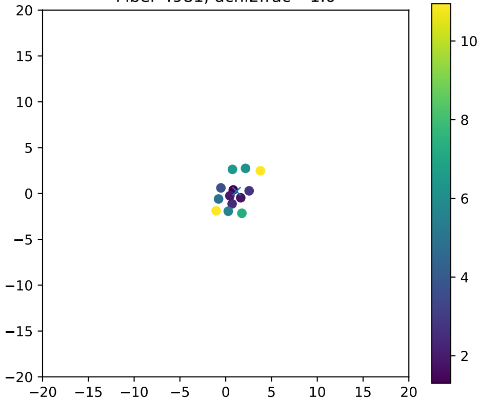
Fiber 4981, dchi2frac= 1.0
