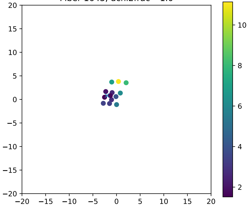
Fiber 1643, dchi2frac= 1.0
