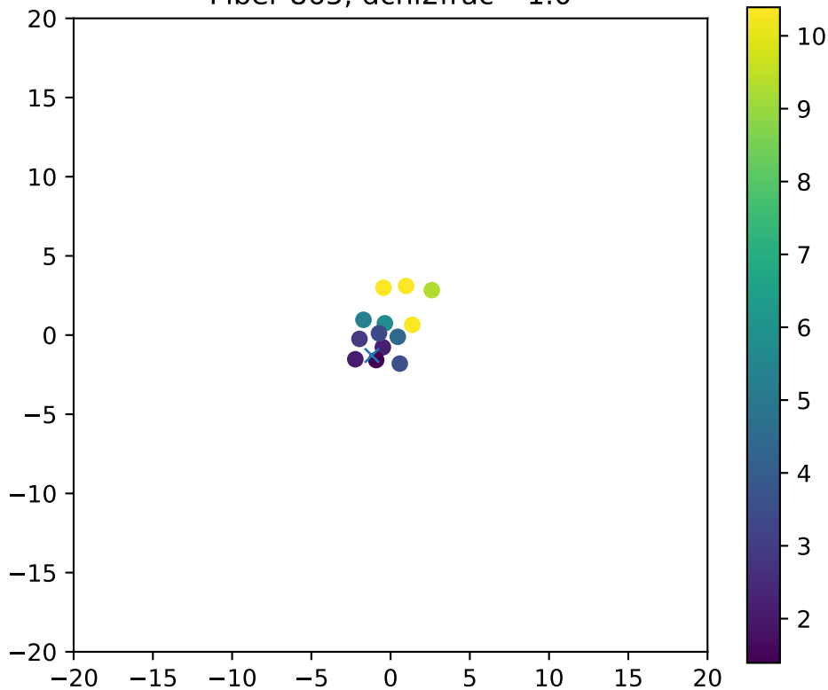
Fiber 865, dchi2frac= 1.0
