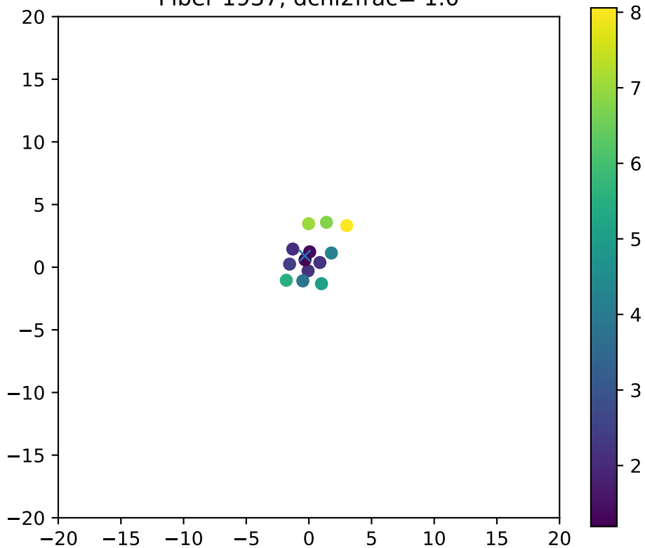
Fiber 1937, dchi2frac= 1.0
