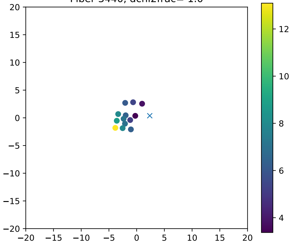
Fiber 3440, dchi2frac= 1.0
