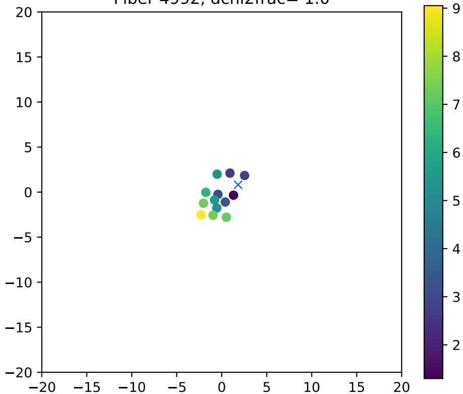
Fiber 4992, dchi2frac= 1.0
