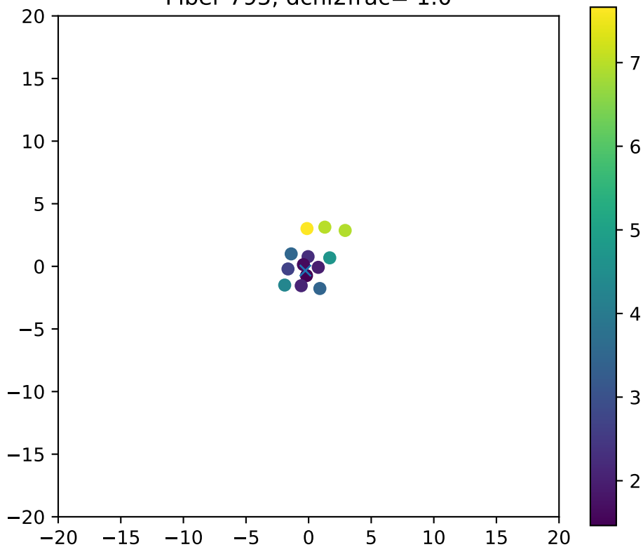
Fiber 795, dchi2frac= 1.0
