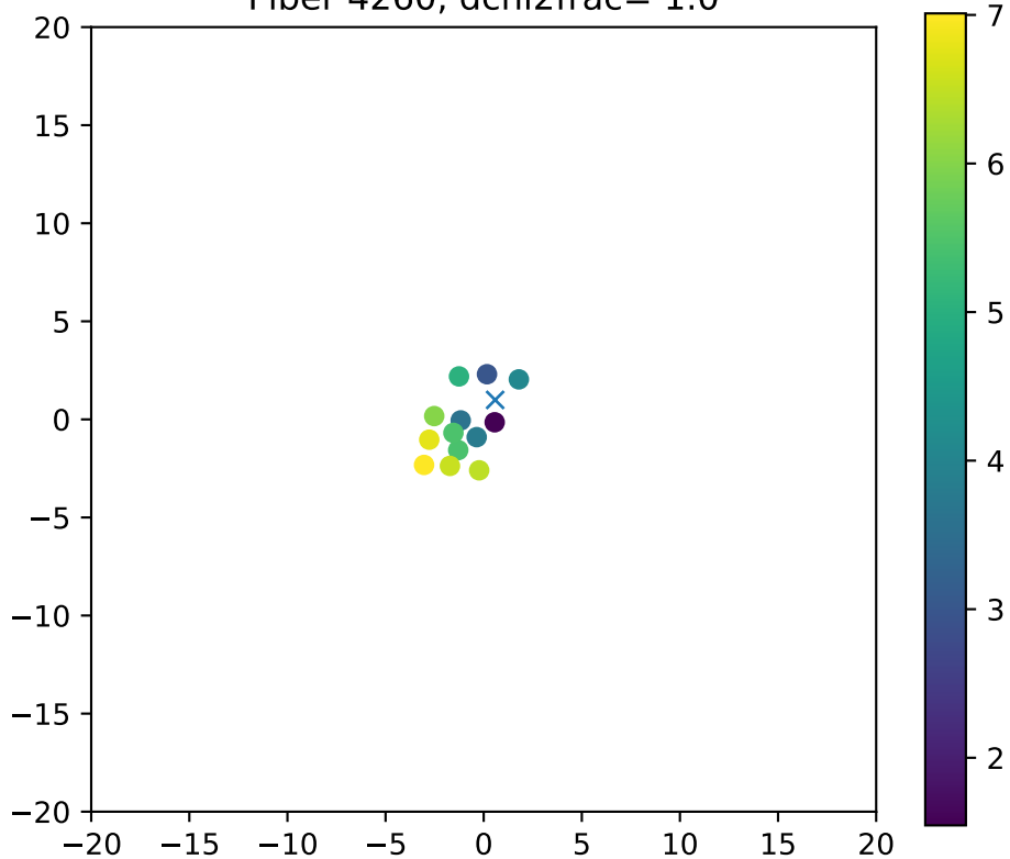
Fiber 4260, dchi2frac= 1.0
