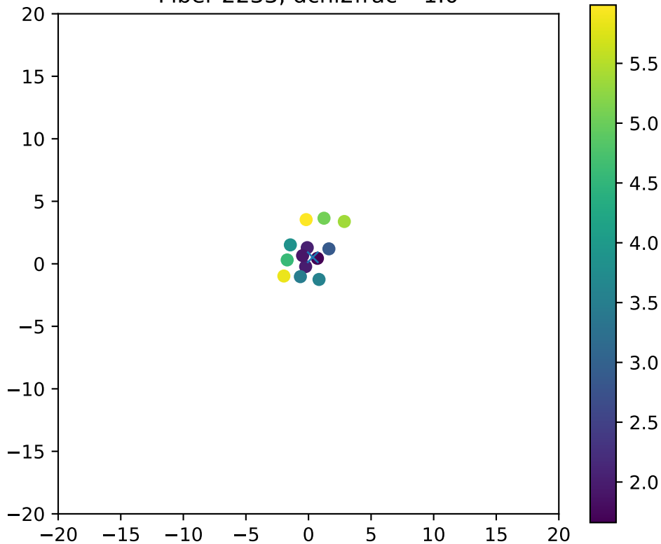
Fiber 2233, dchi2frac= 1.0
