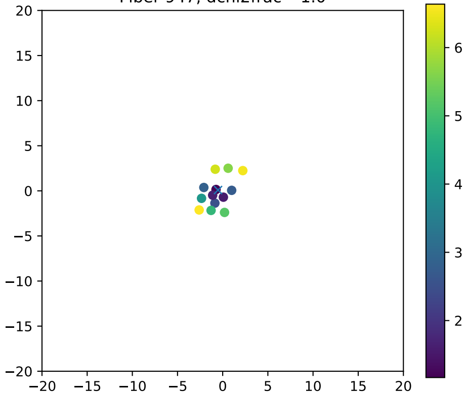
Fiber 947, dchi2frac= 1.0
