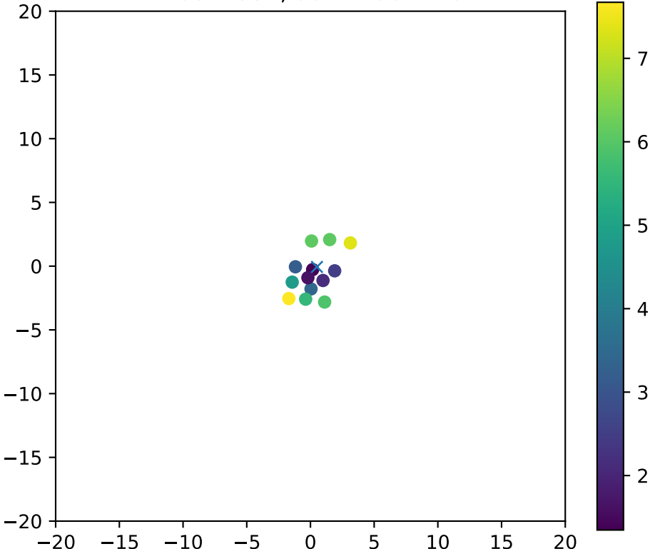
Fiber 2951, dchi2frac= 1.0
