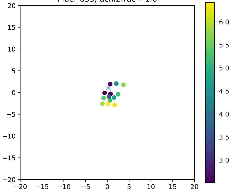
Fiber 633, dchi2frac= 1.0
