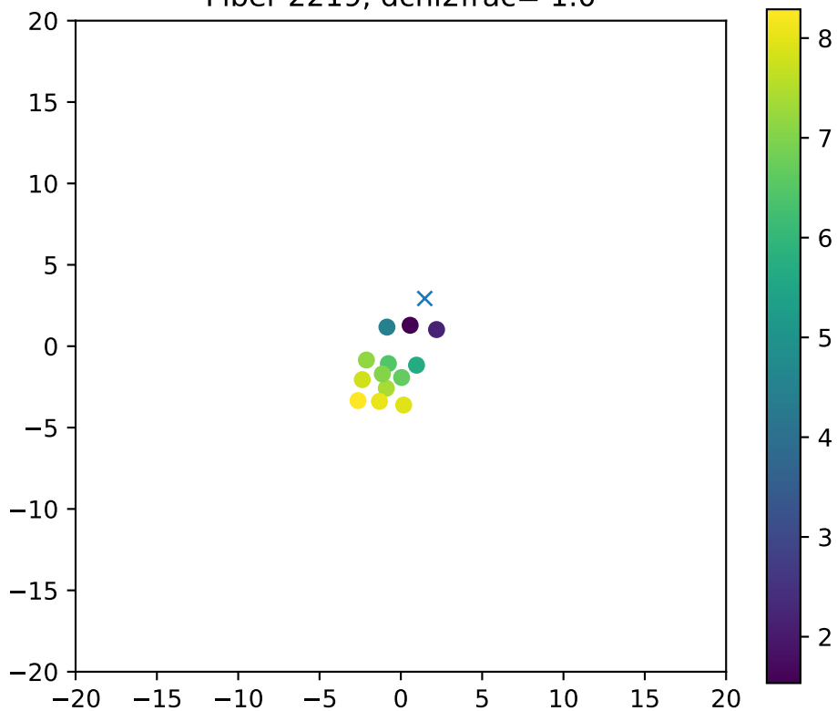
Fiber 2219, dchi2frac= 1.0
