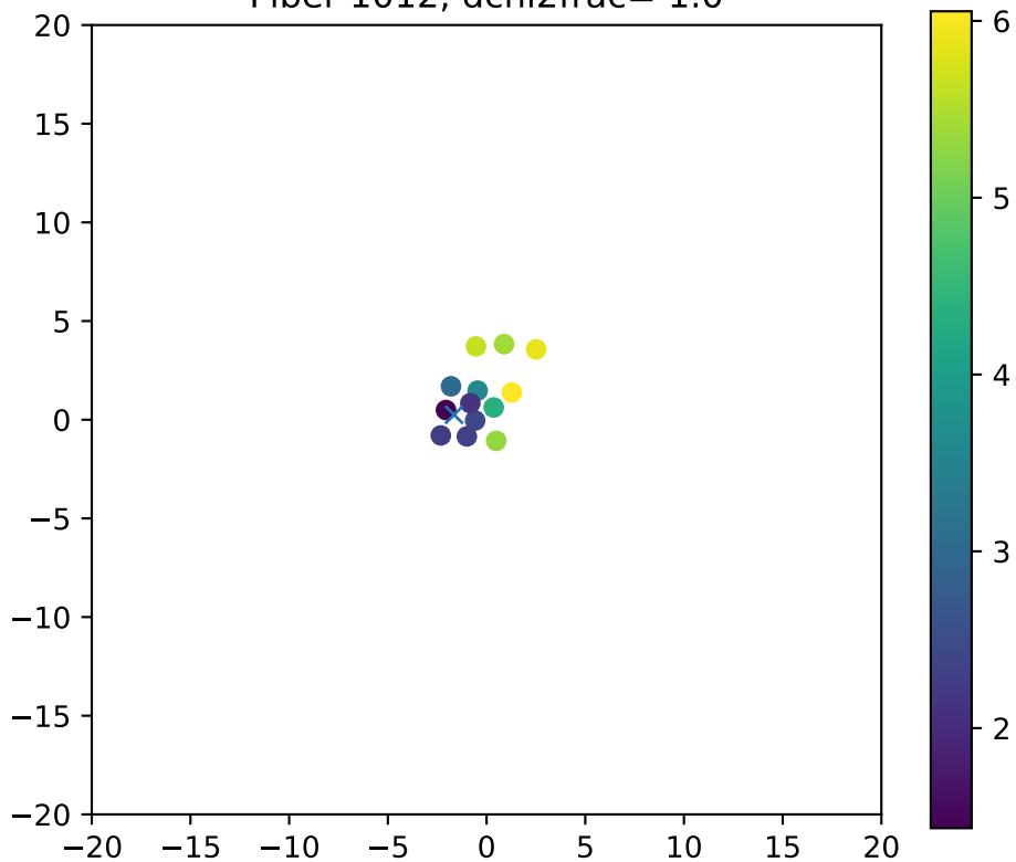
Fiber 1012, dchi2frac= 1.0
