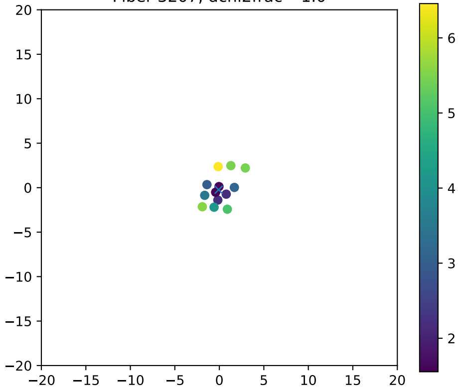
Fiber 3207, dchi2frac= 1.0
