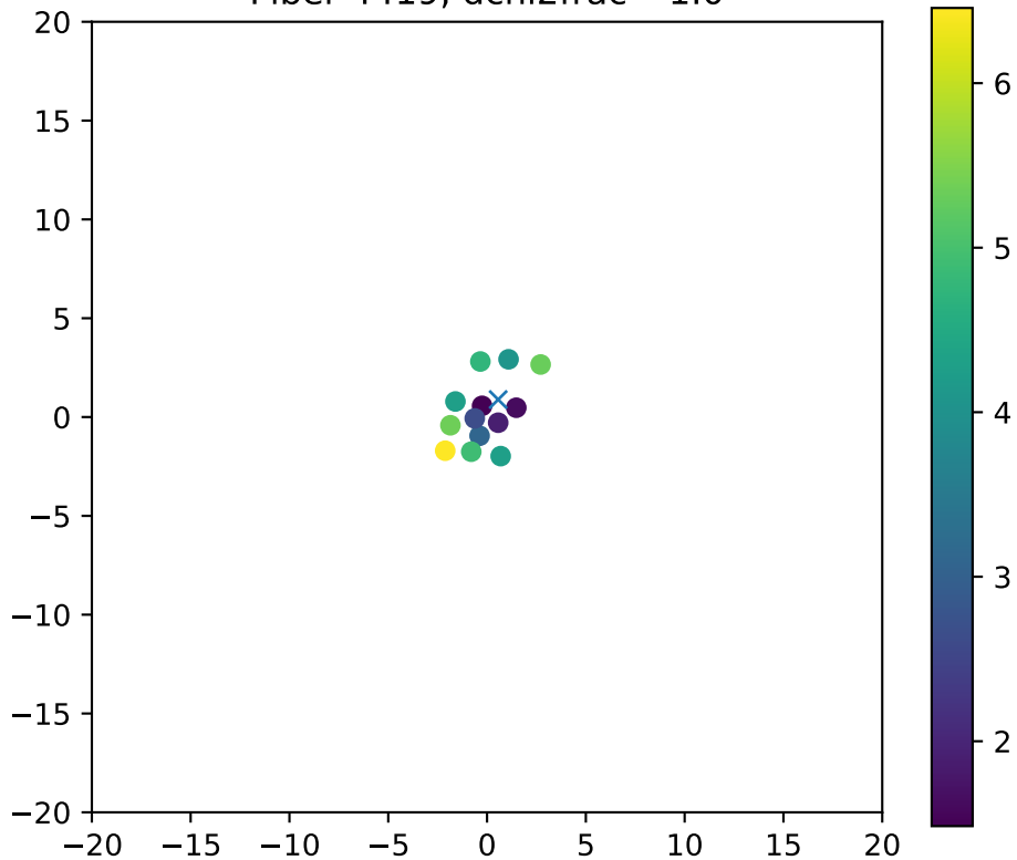
Fiber 4419, dchi2frac= 1.0
