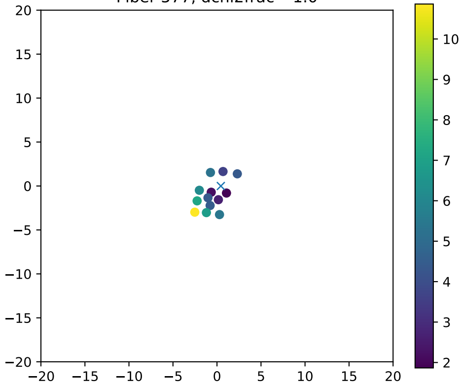
Fiber 577, dchi2frac= 1.0
