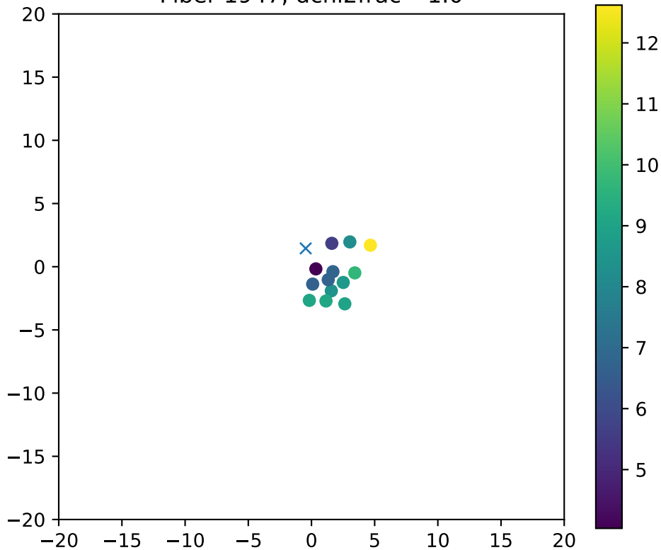
Fiber 1947, dchi2frac= 1.0
