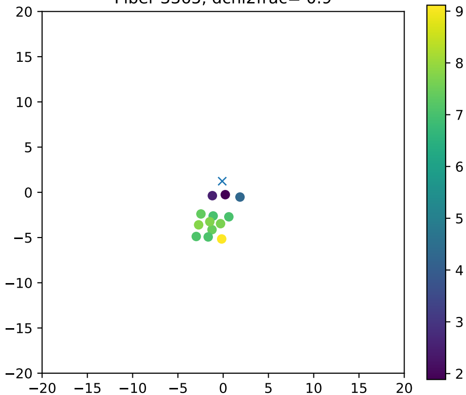
Fiber 3365, dchi2frac= 0.9
