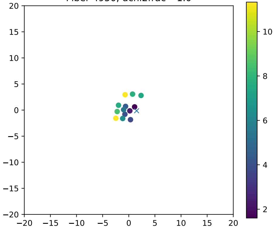
Fiber 4950, dchi2frac= 1.0
