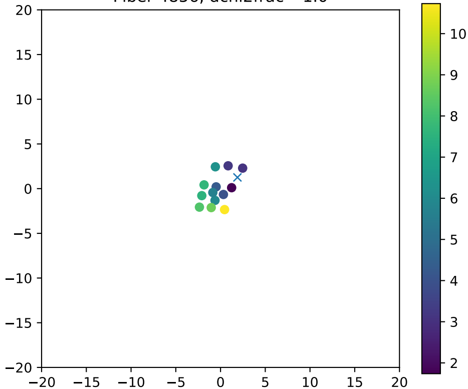
Fiber 4856, dchi2frac= 1.0
