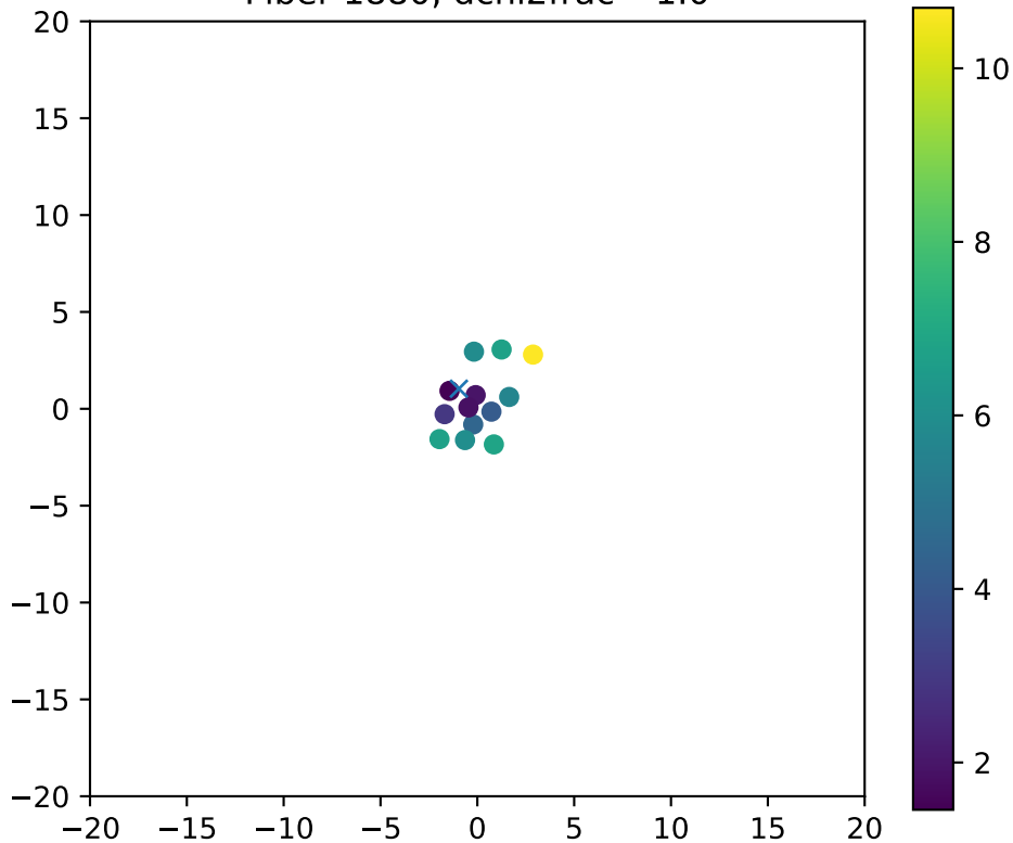
Fiber 1880, dchi2frac= 1.0
