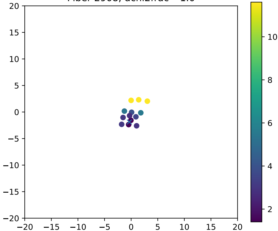
Fiber 2908, dchi2frac= 1.0
