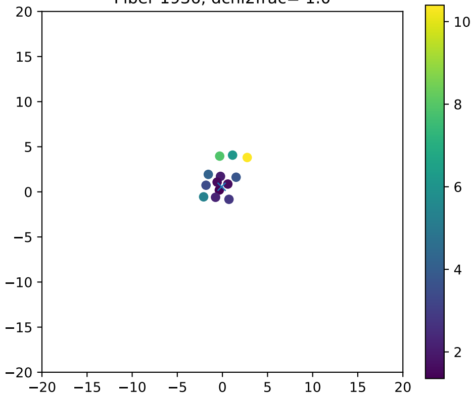
Fiber 1936, dchi2frac= 1.0
