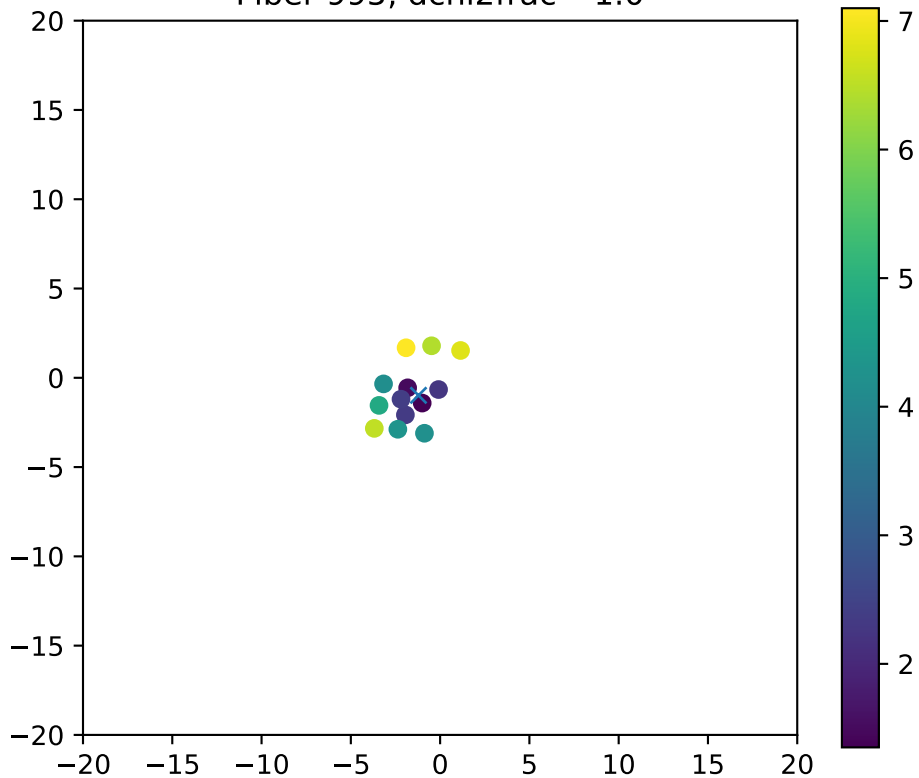
Fiber 995, dchi2frac= 1.0
