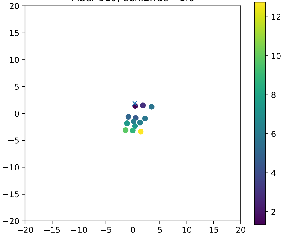
Fiber 919, dchi2frac= 1.0
