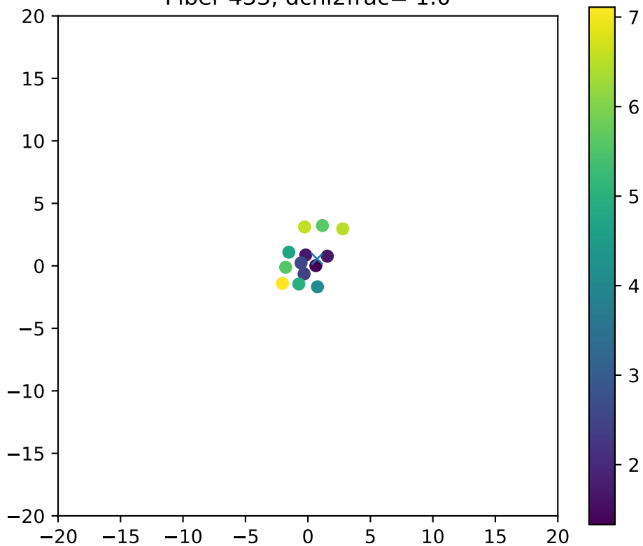
Fiber 433, dchi2frac= 1.0
