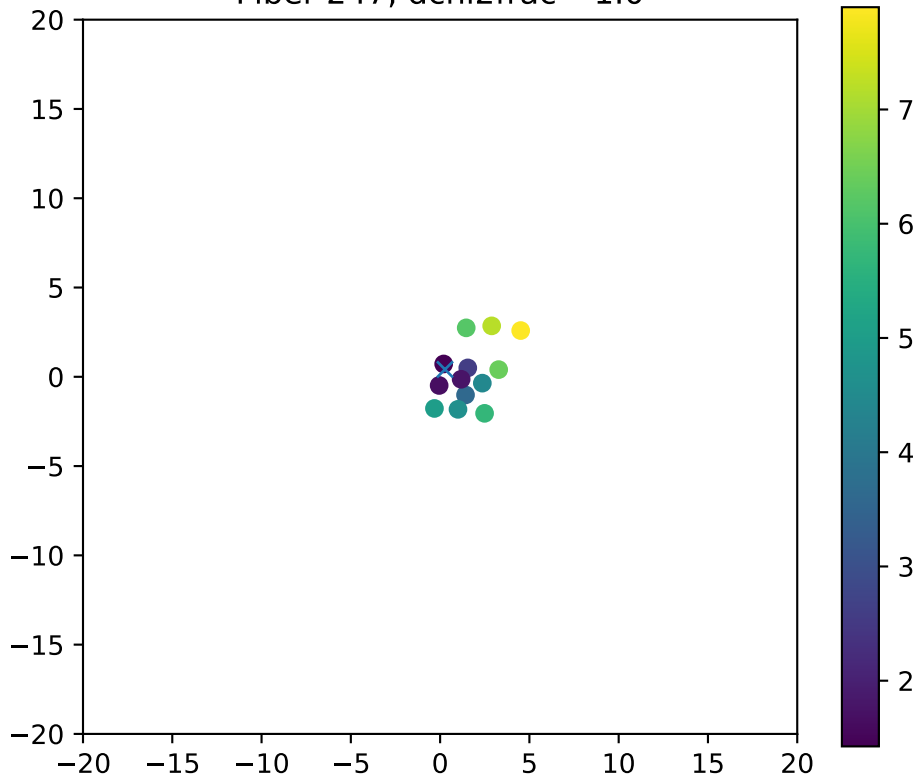
Fiber 247, dchi2frac= 1.0
