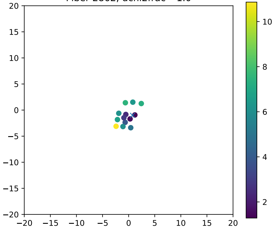
Fiber 2862, dchi2frac= 1.0
