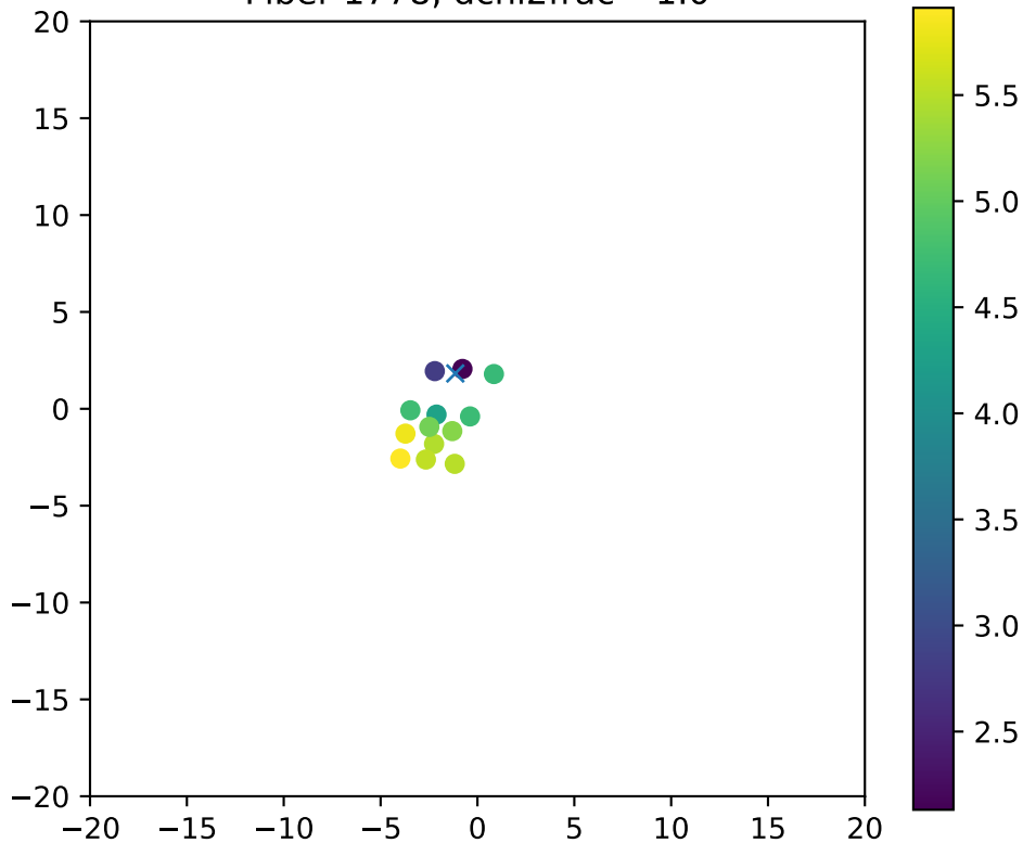
Fiber 1778, dchi2frac= 1.0
