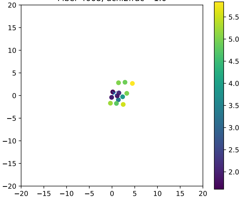
Fiber 4668, dchi2frac= 1.0
