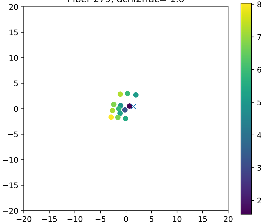
Fiber 279, dchi2frac= 1.0
