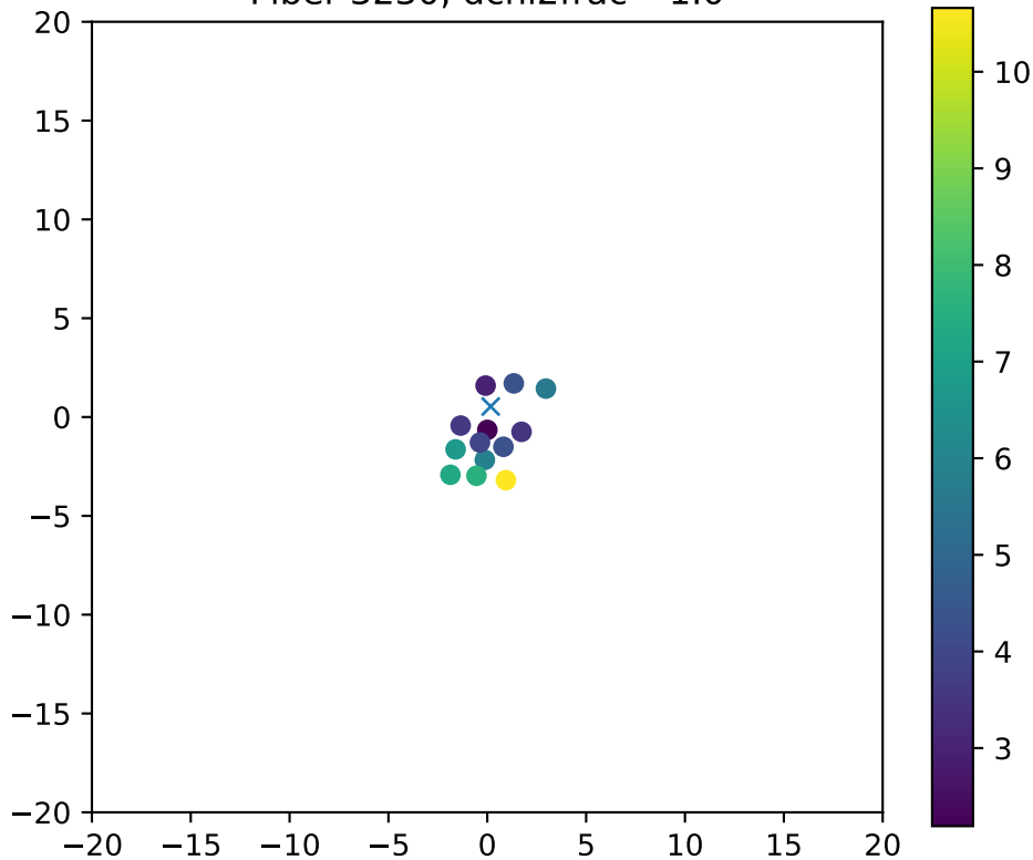
Fiber 3230, dchi2frac= 1.0
