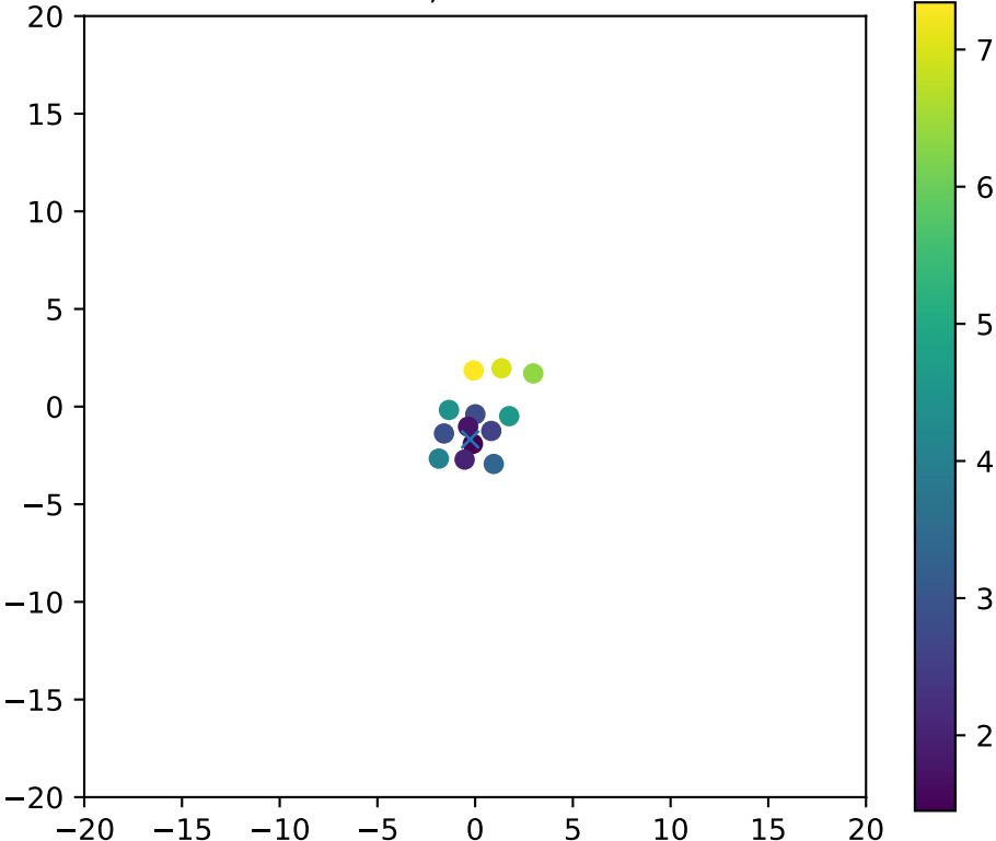
Fiber 2758, dchi2frac= 1.0
