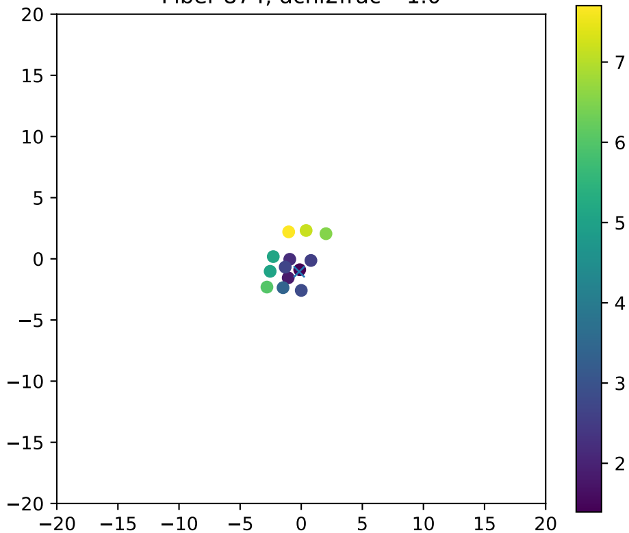
Fiber 874, dchi2frac= 1.0
