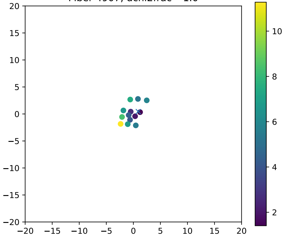
Fiber 4907, dchi2frac= 1.0
