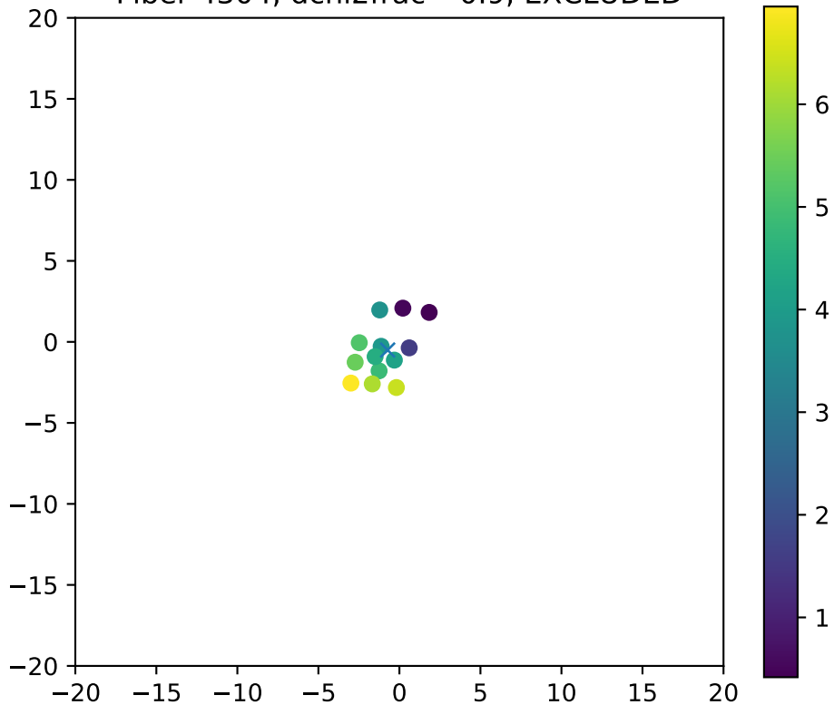
Fiber 4304, dchi2frac= 0.9, EXCLUDED
