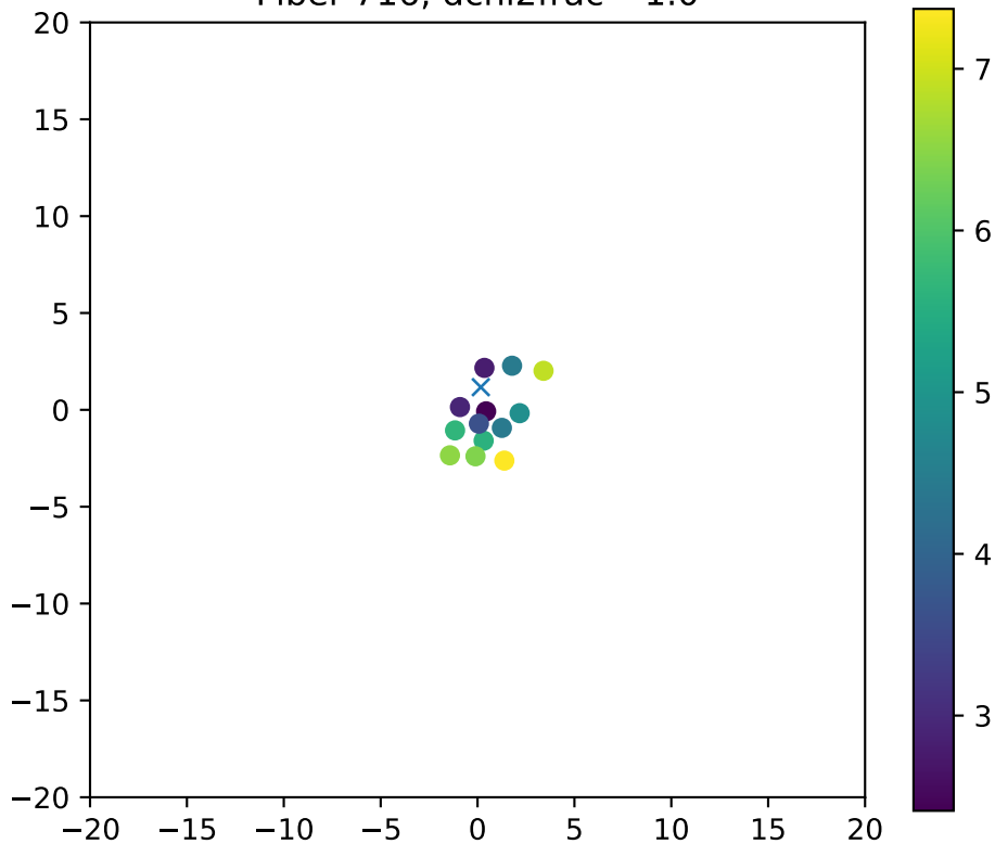
Fiber 716, dchi2frac= 1.0
