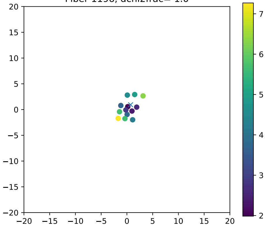
Fiber 1196, dchi2frac= 1.0
