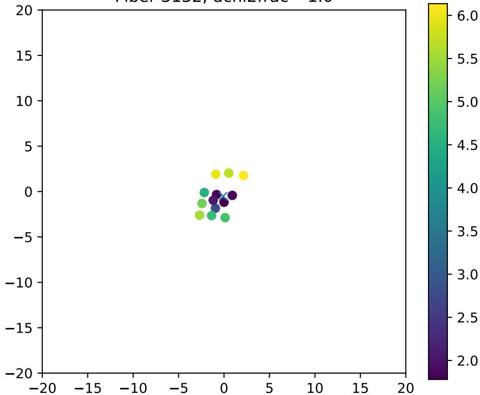
Fiber 3132, dchi2frac= 1.0
