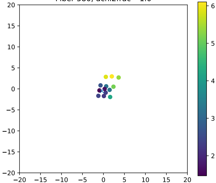
Fiber 580, dchi2frac= 1.0
