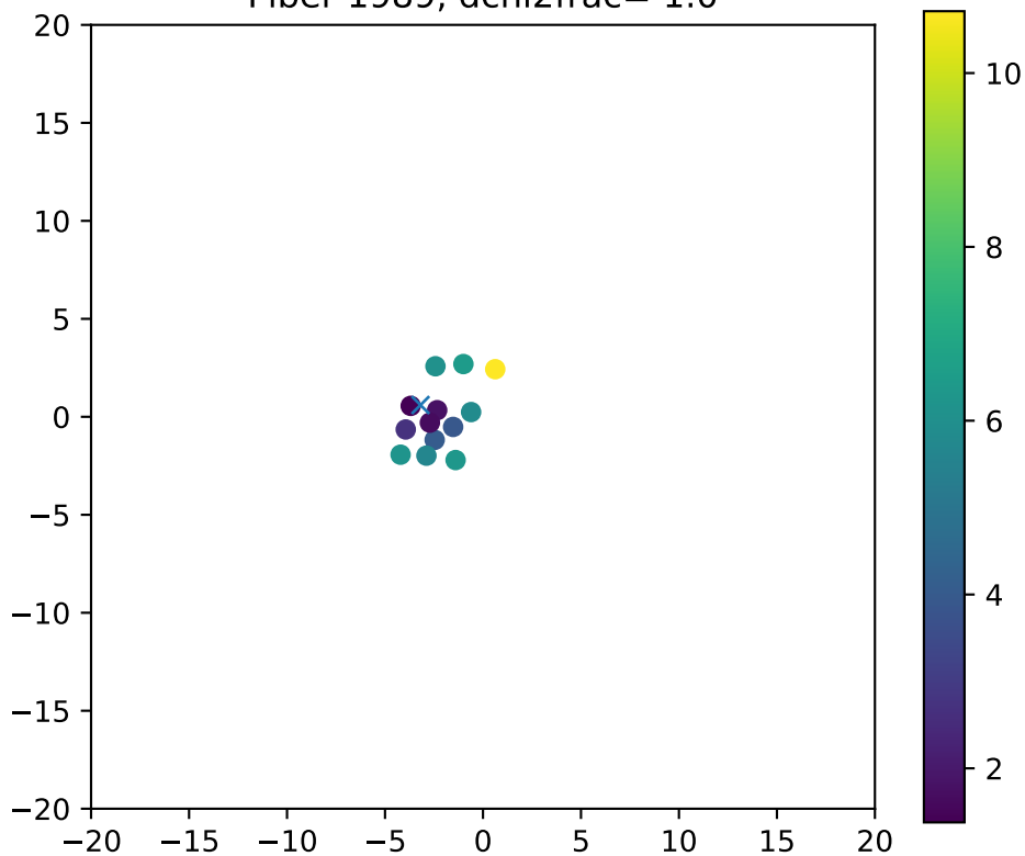
Fiber 1989, dchi2frac= 1.0
