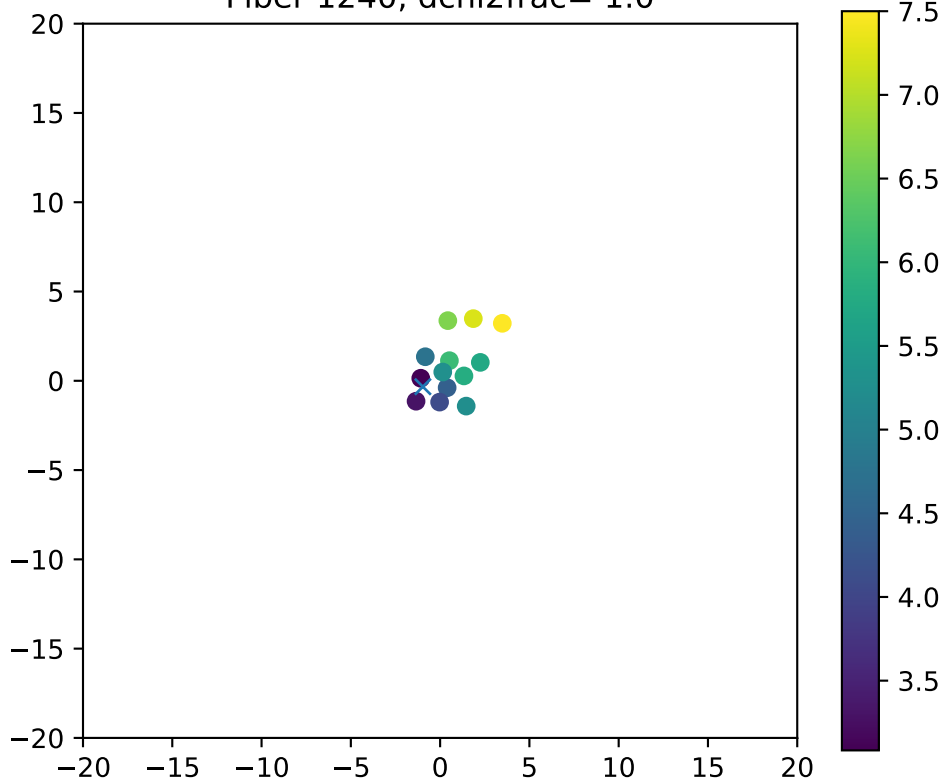
Fiber 1240, dchi2frac= 1.0
