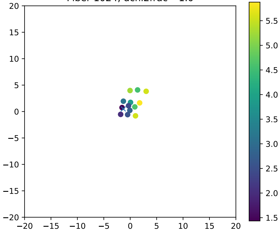
Fiber 1024, dchi2frac= 1.0
