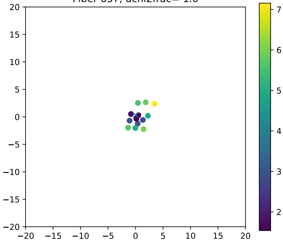
Fiber 637, dchi2frac= 1.0
