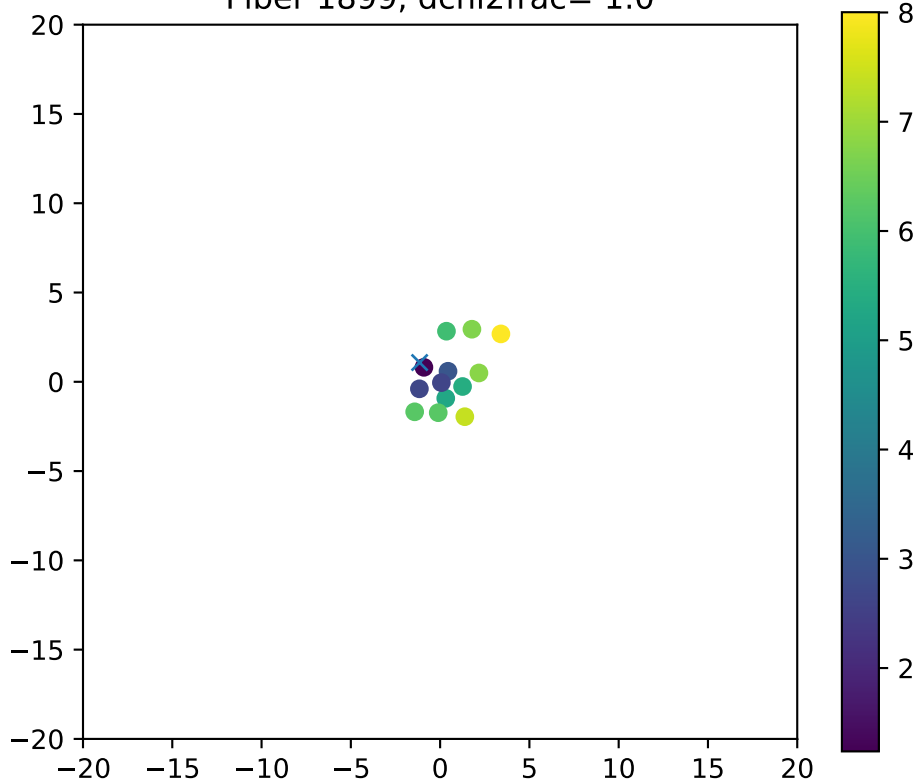
Fiber 1899, dchi2frac= 1.0
