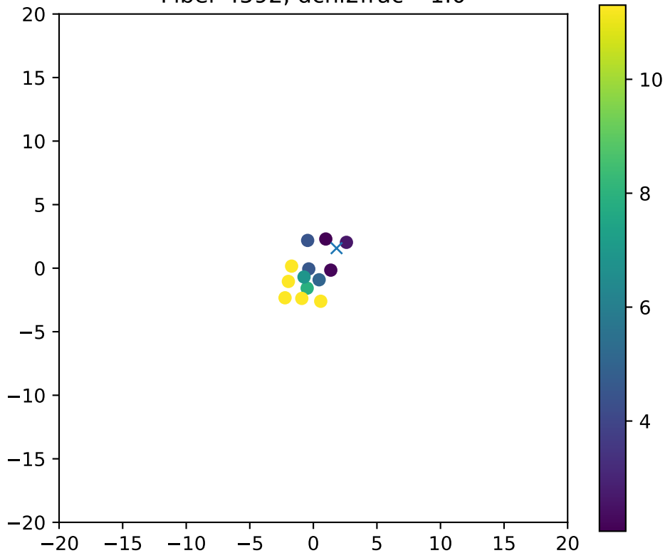
Fiber 4592, dchi2frac= 1.0
