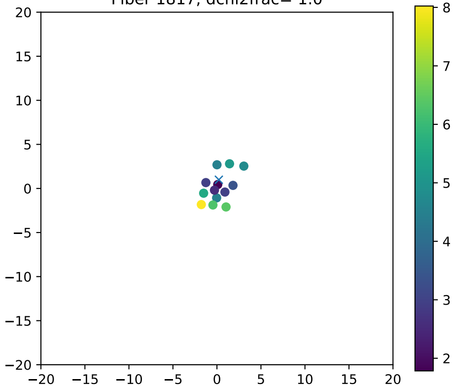
Fiber 1817, dchi2frac= 1.0
