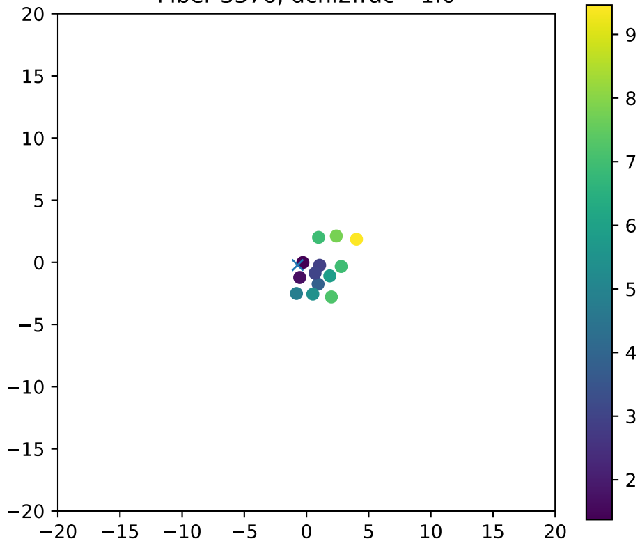
Fiber 3376, dchi2frac= 1.0
