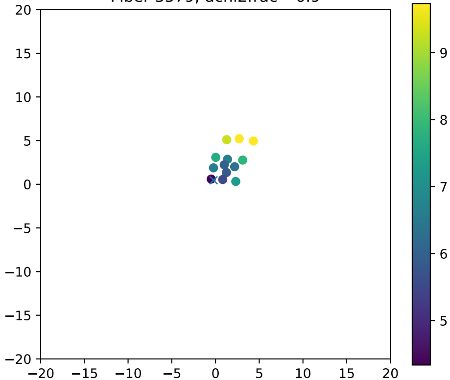
Fiber 3579, dchi2frac= 0.9
