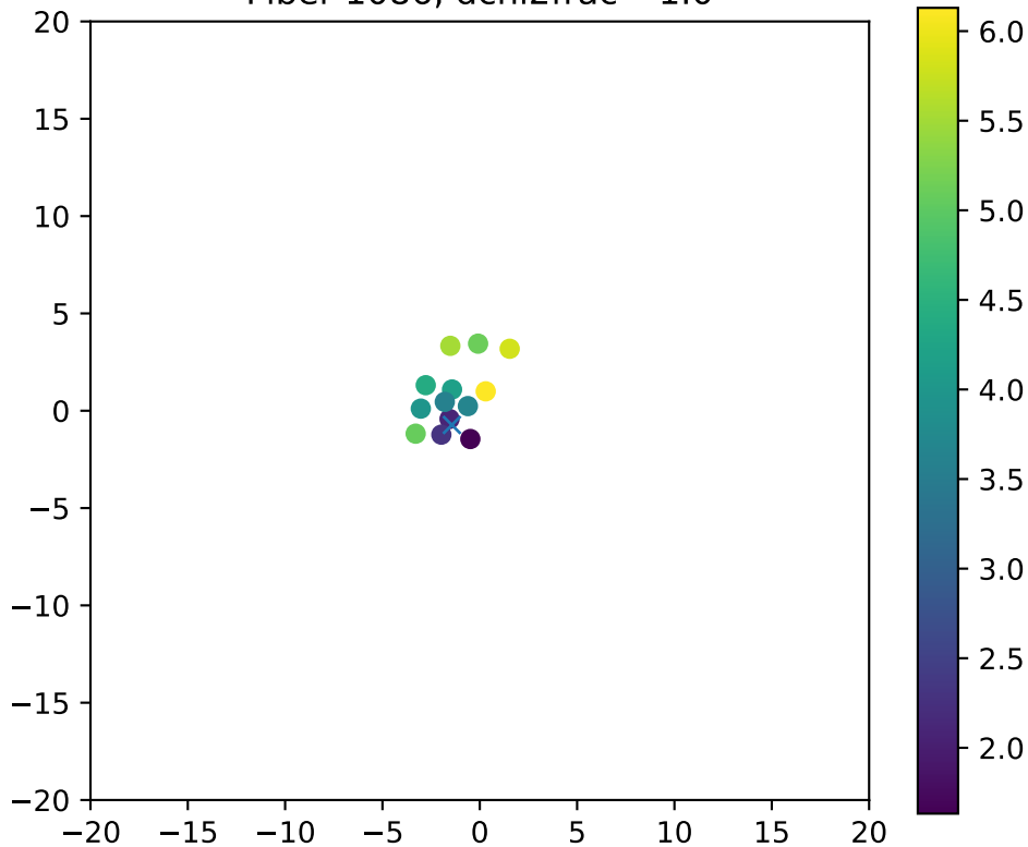
Fiber 1086, dchi2frac= 1.0
