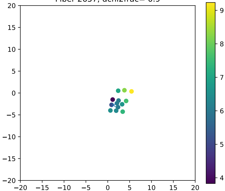
Fiber 2657, dchi2frac= 0.9
