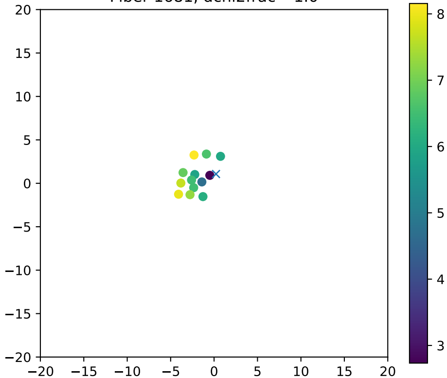
Fiber 1681, dchi2frac= 1.0
