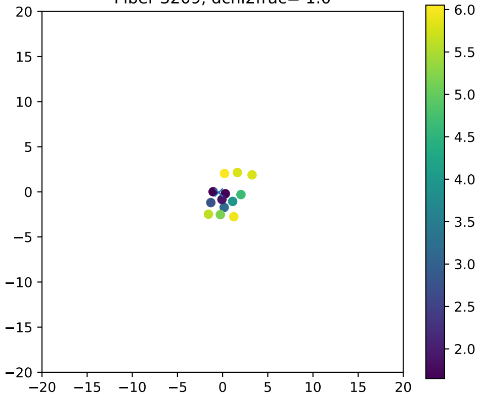
Fiber 3209, dchi2frac= 1.0
