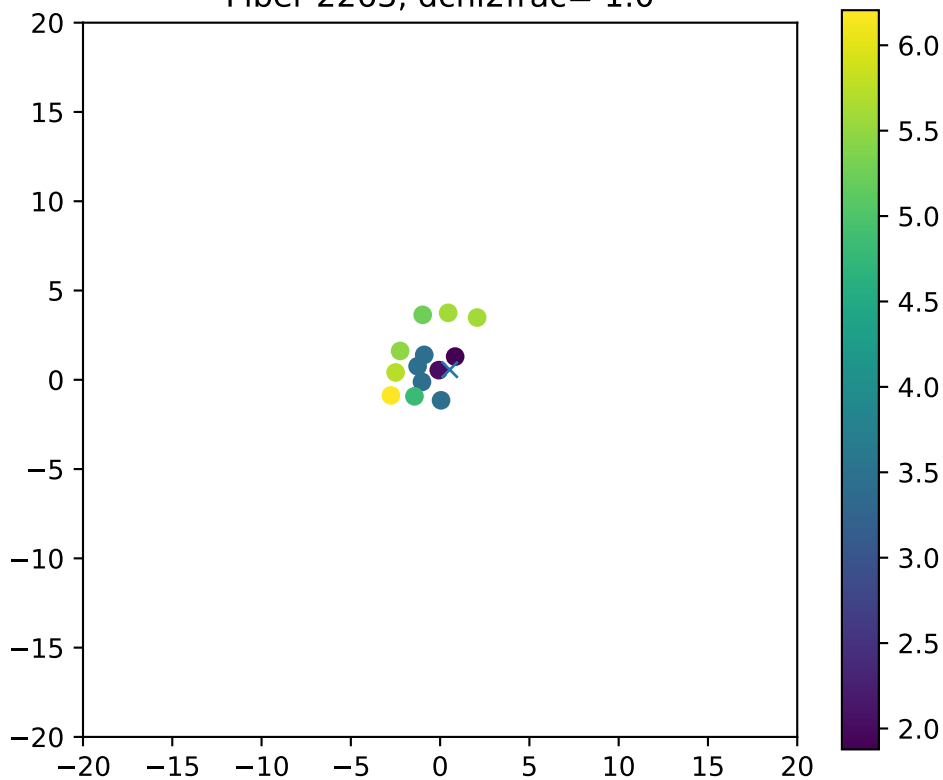
Fiber 2263, dchi2frac= 1.0
