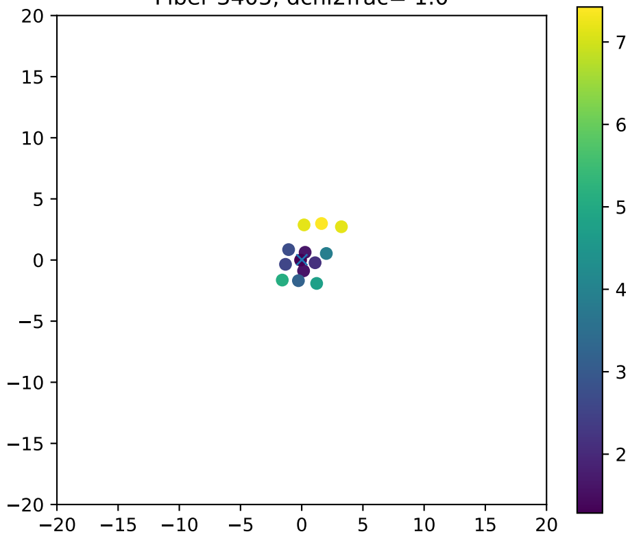
Fiber 3405, dchi2frac= 1.0
