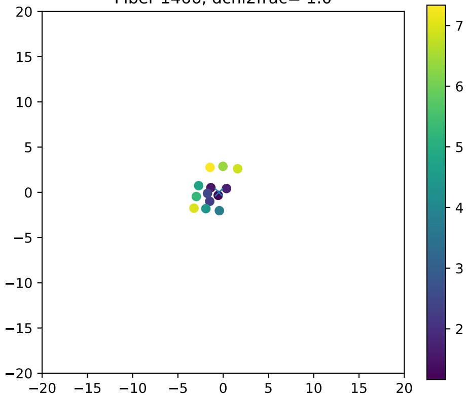
Fiber 1466, dchi2frac= 1.0
