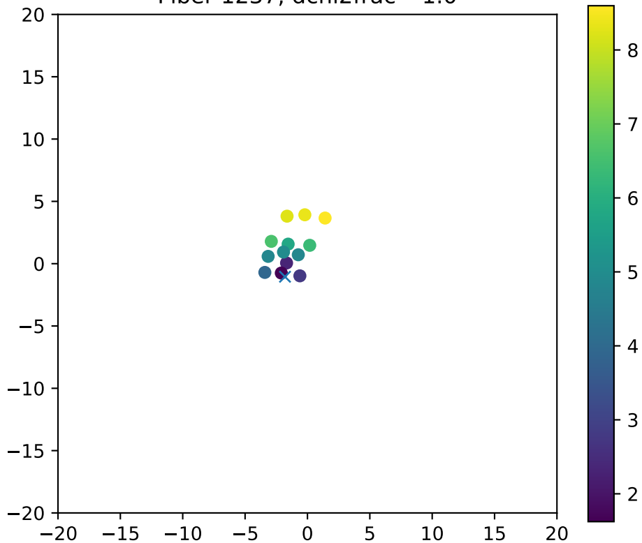
Fiber 1237, dchi2frac= 1.0
