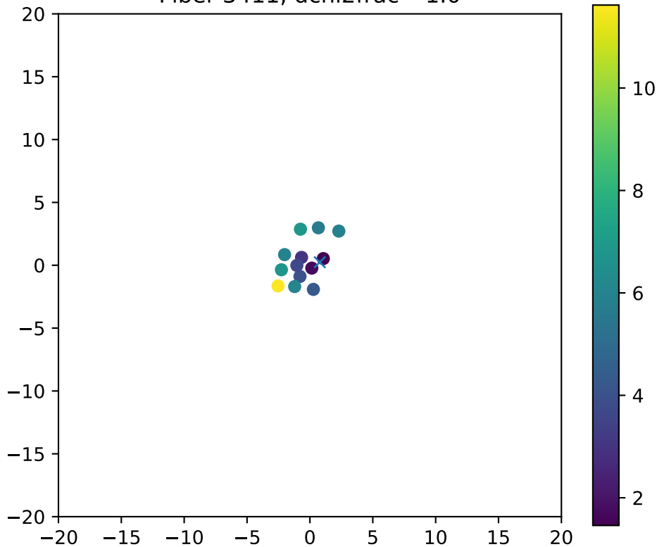
Fiber 3411, dchi2frac= 1.0
