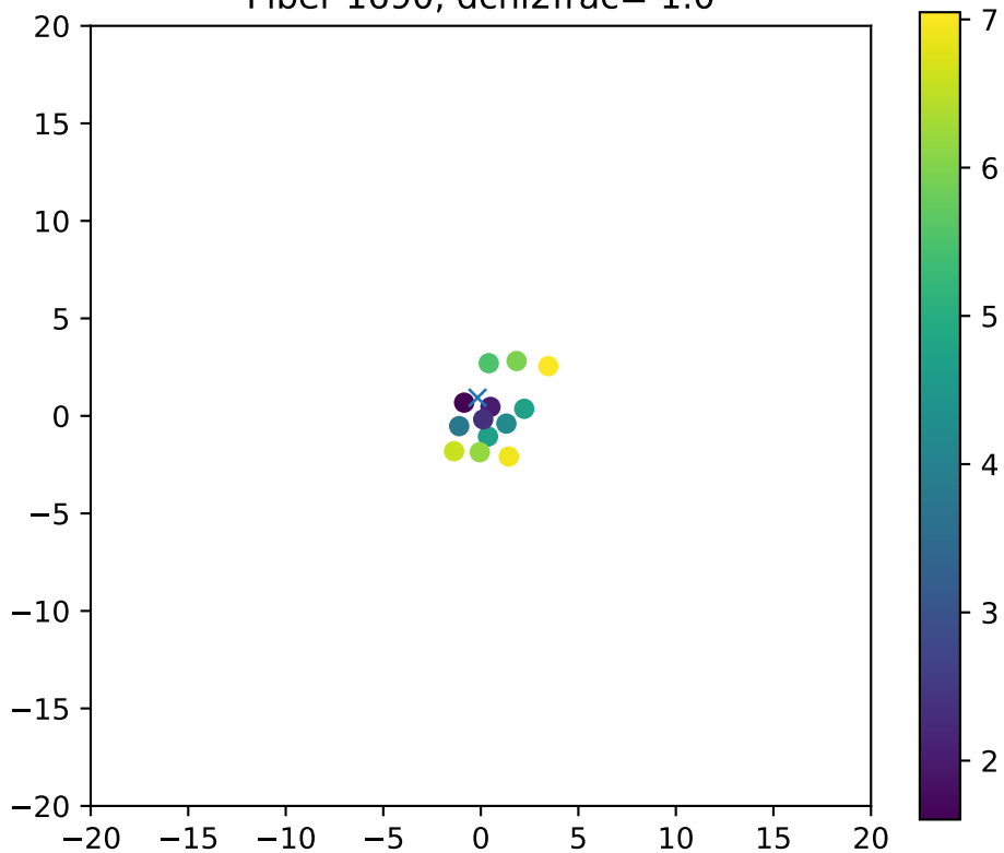
Fiber 1690, dchi2frac= 1.0
