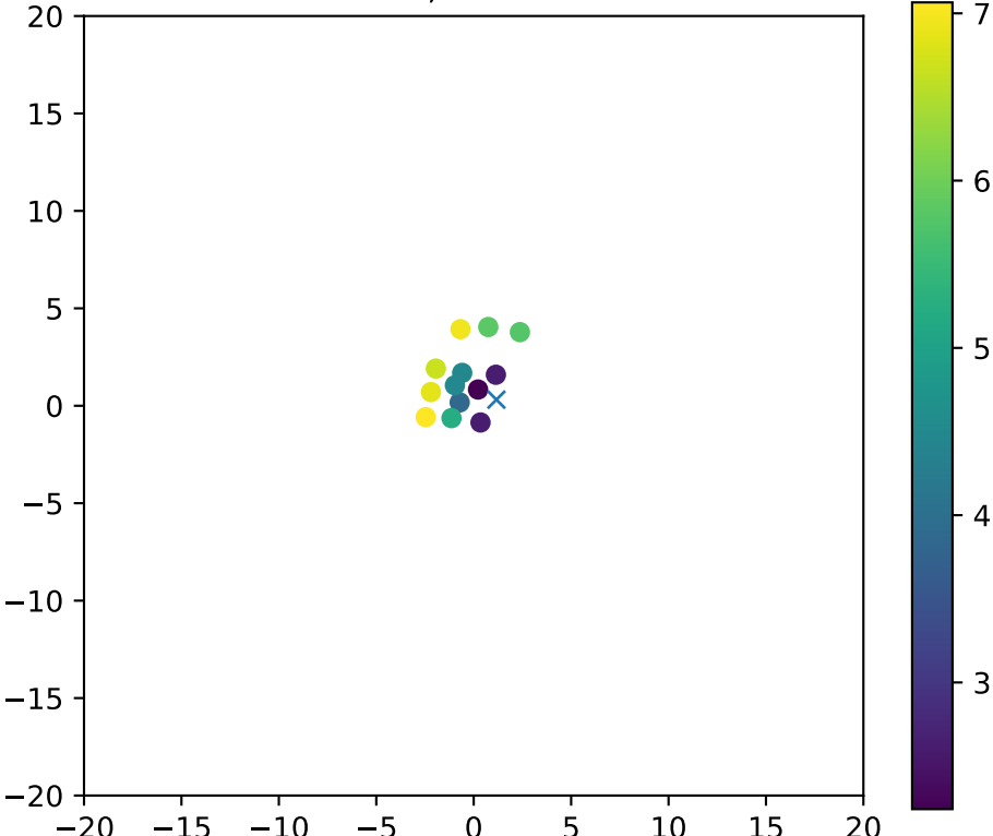
Fiber 4575, dchi2frac= 1.0
