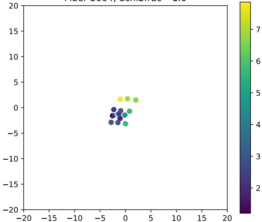
Fiber 3004, dchi2frac= 1.0
