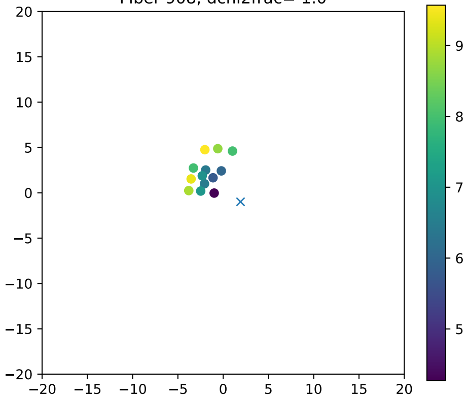
Fiber 908, dchi2frac= 1.0
