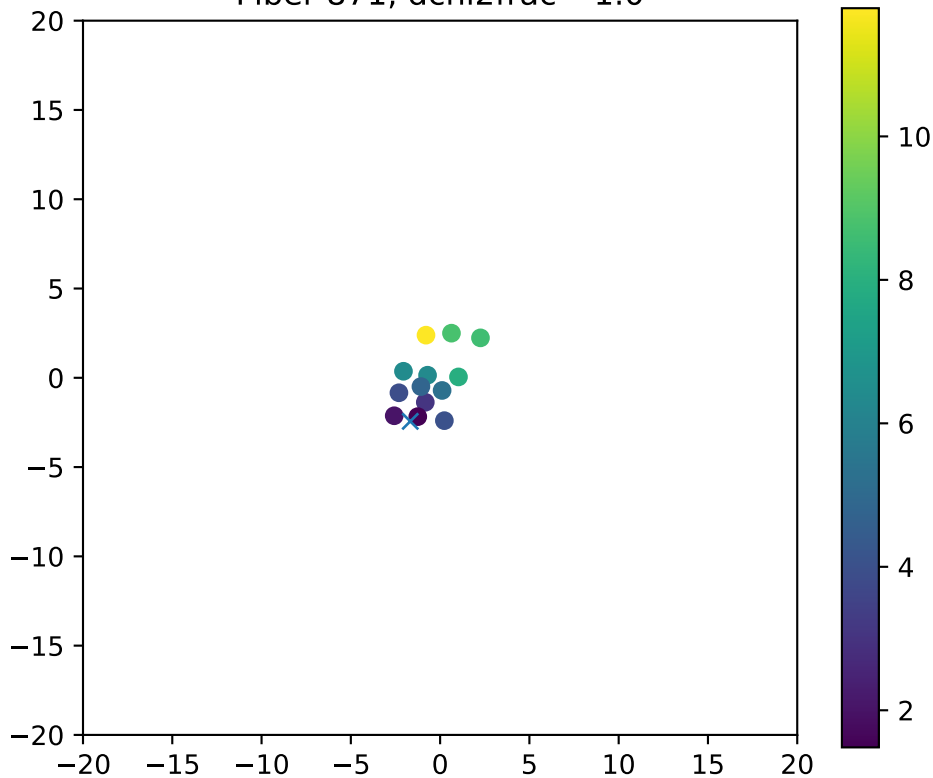
Fiber 871, dchi2frac= 1.0
