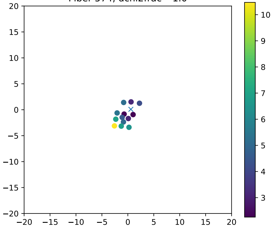
Fiber 574, dchi2frac= 1.0
