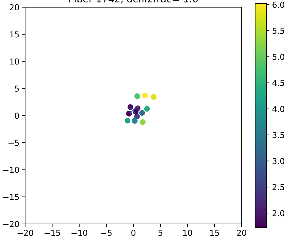
Fiber 1742, dchi2frac= 1.0
