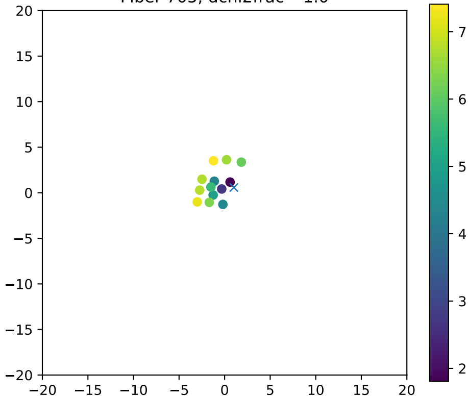
Fiber 705, dchi2frac= 1.0
