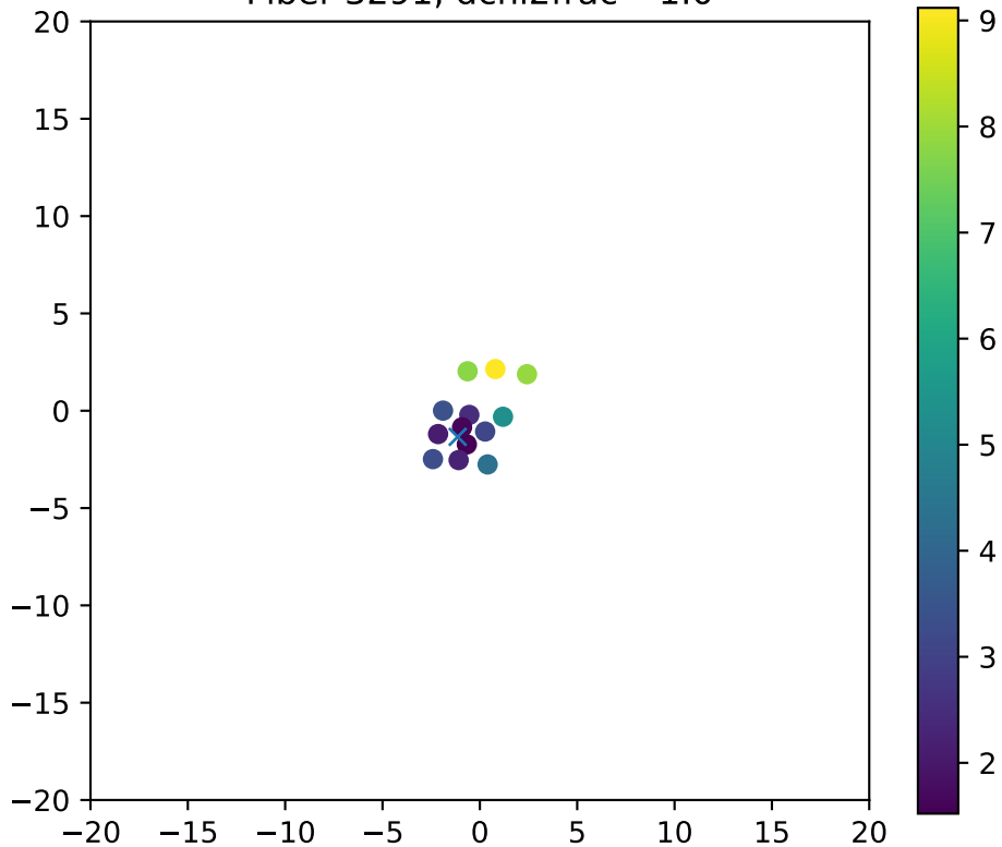
Fiber 3291, dchi2frac= 1.0
