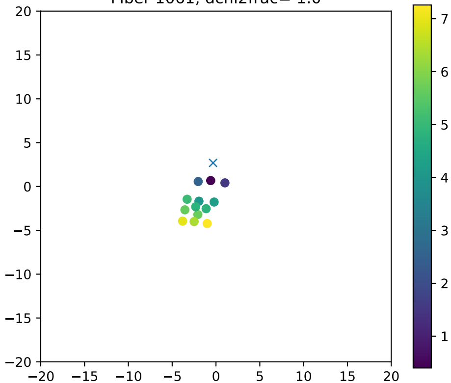
Fiber 1061, dchi2frac= 1.0
