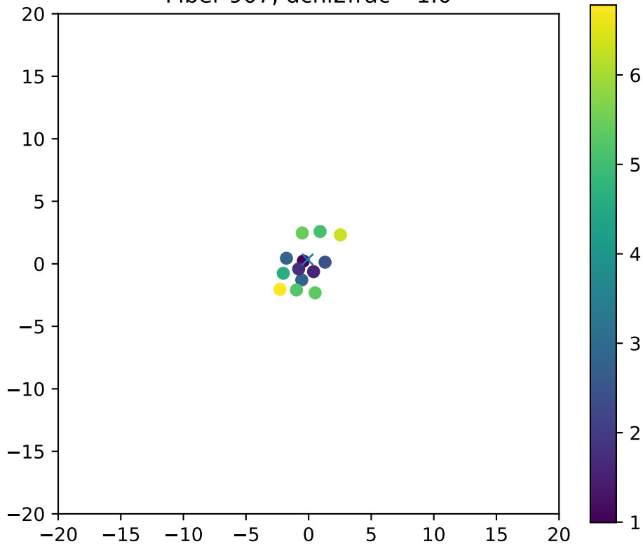
Fiber 907, dchi2frac= 1.0
