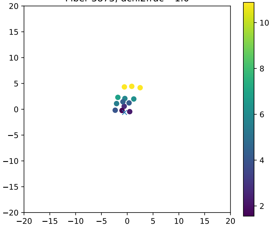
Fiber 3873, dchi2frac= 1.0
