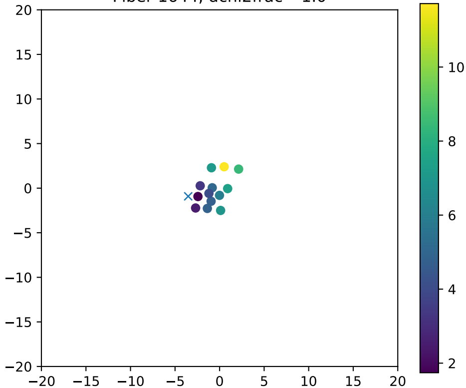
Fiber 1644, dchi2frac= 1.0
