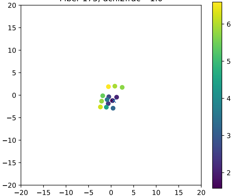
Fiber 173, dchi2frac= 1.0
