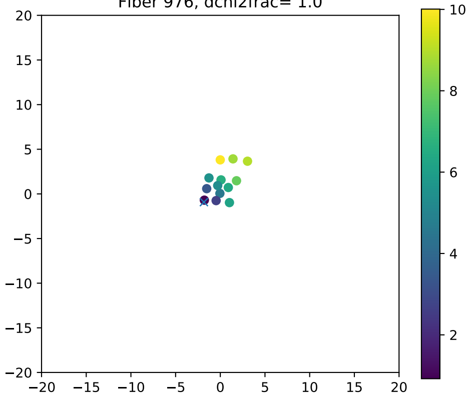
Fiber 976, dchi2frac= 1.0
