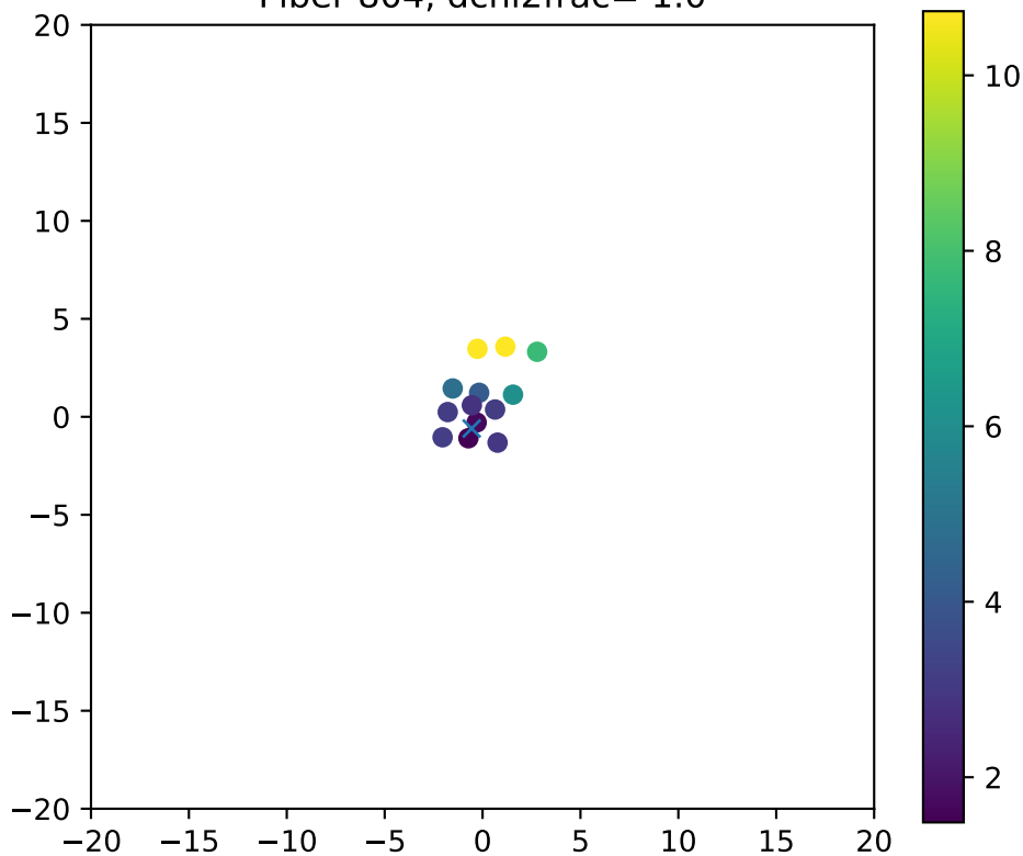
Fiber 804, dchi2frac= 1.0
