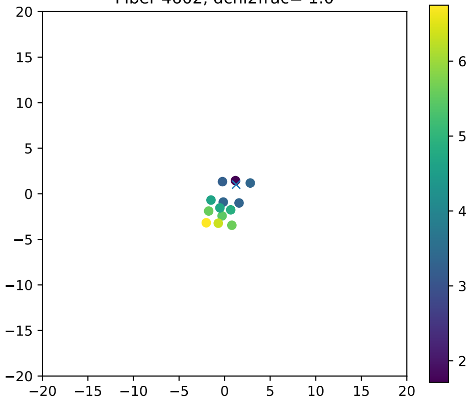
Fiber 4602, dchi2frac= 1.0
