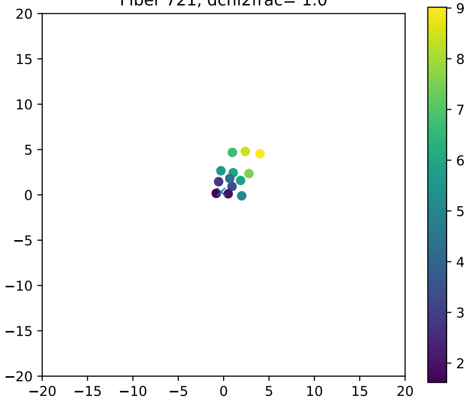
Fiber 721, dchi2frac= 1.0
