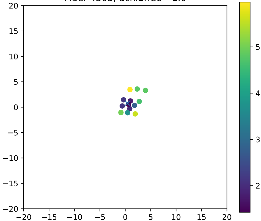
Fiber 4303, dchi2frac= 1.0
