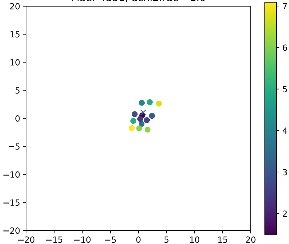
Fiber 4551, dchi2frac= 1.0
