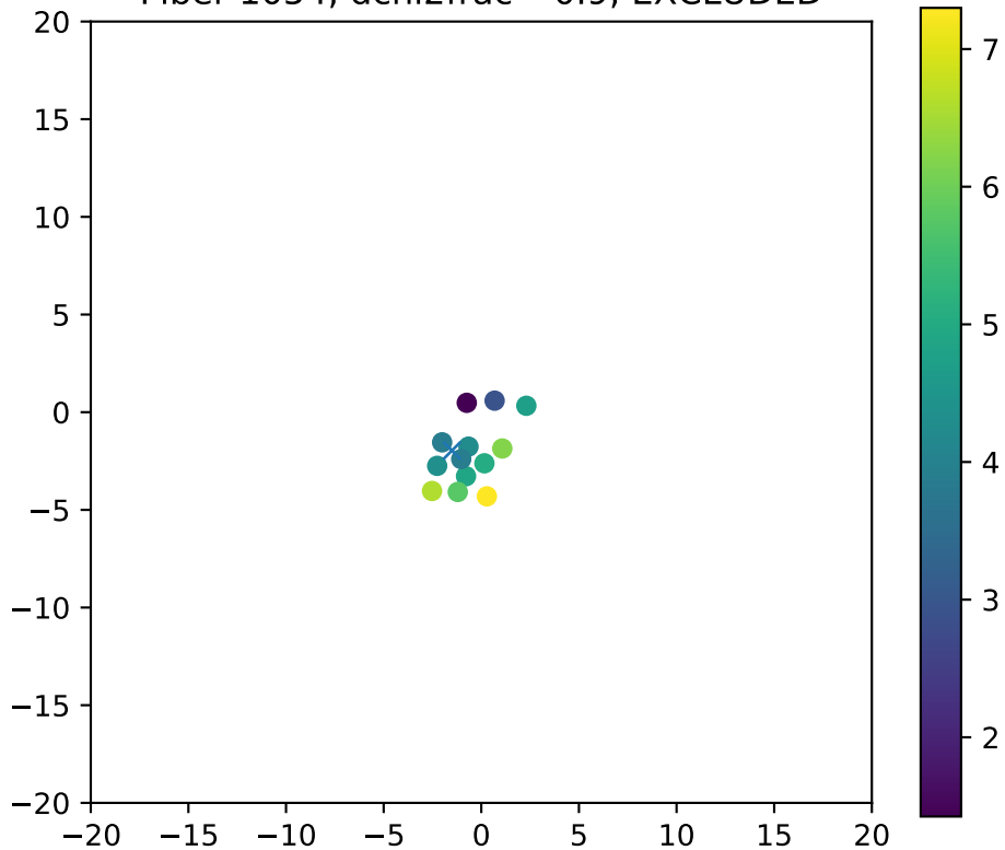
Fiber 1054, dchi2frac= 0.9, EXCLUDED
