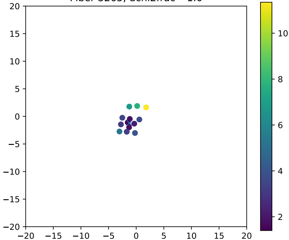
Fiber 3265, dchi2frac= 1.0
