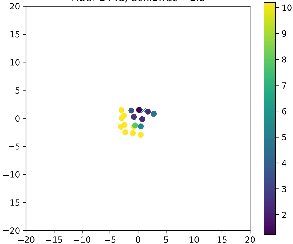
Fiber 1448, dchi2frac= 1.0
