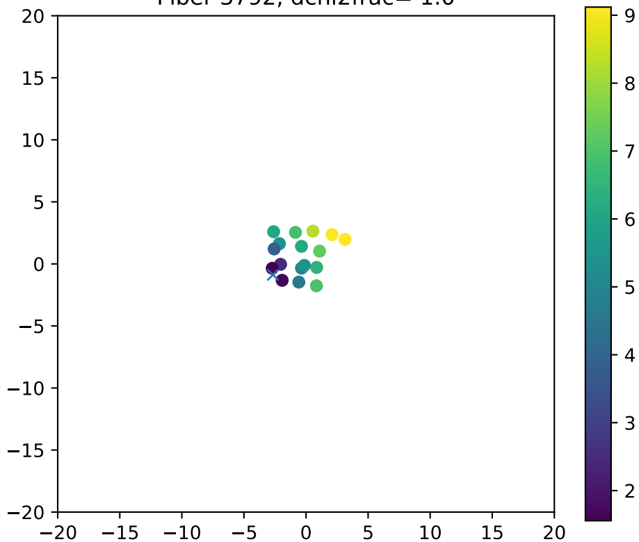
Fiber 3792, dchi2frac= 1.0
