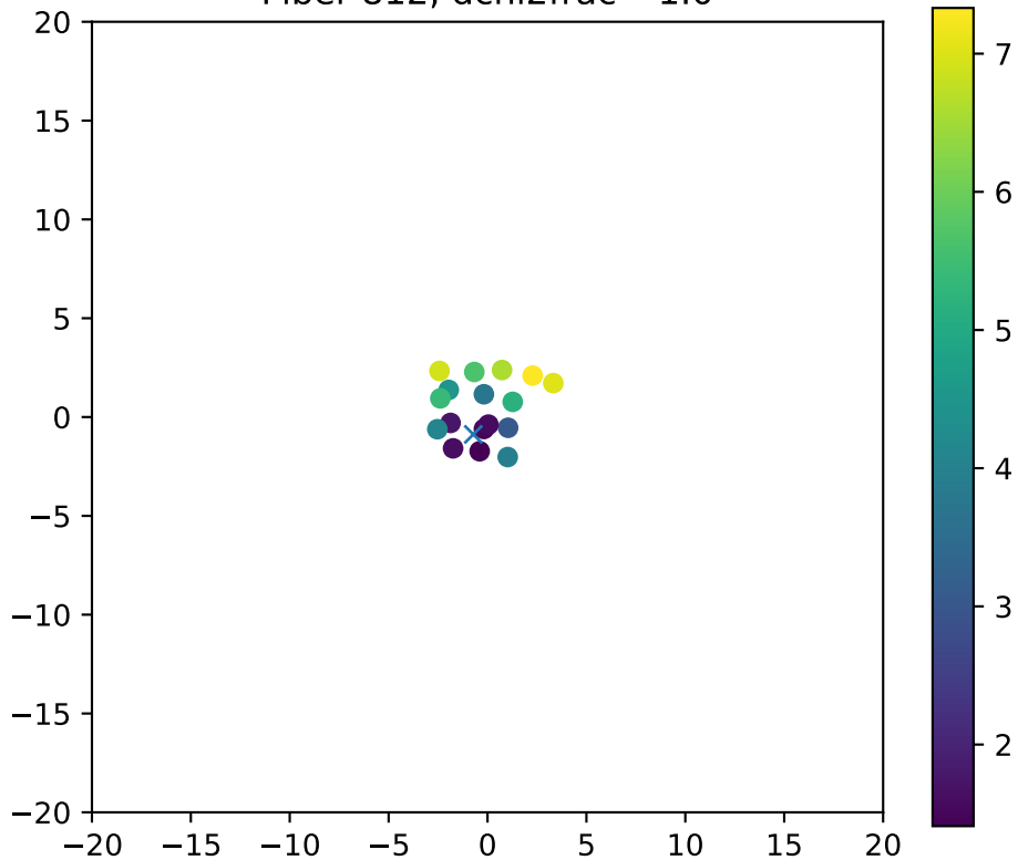
Fiber 812, dchi2frac= 1.0
