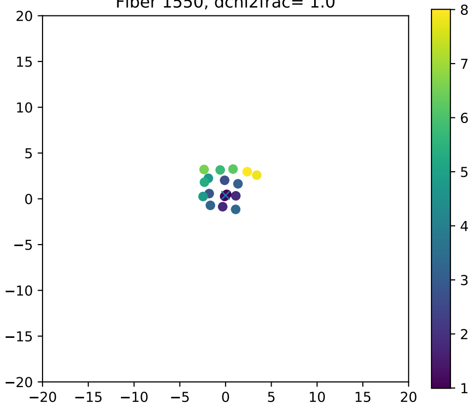
Fiber 1550, dchi2frac= 1.0
