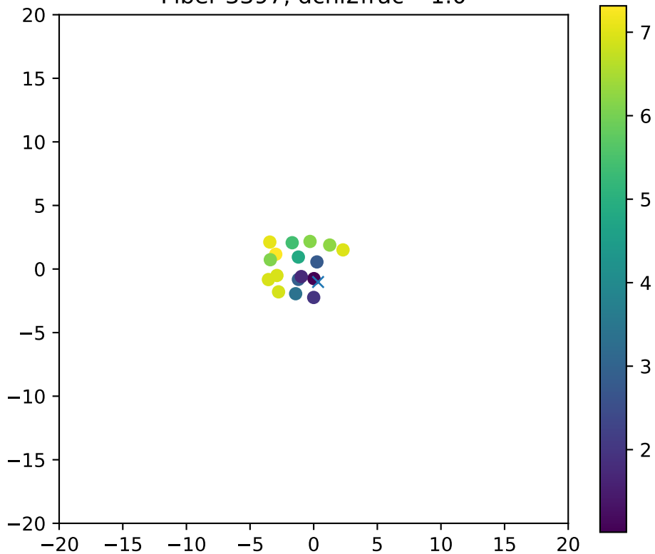
Fiber 3397, dchi2frac= 1.0
