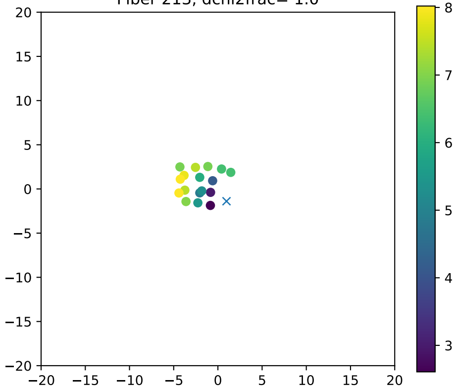
Fiber 213, dchi2frac= 1.0
