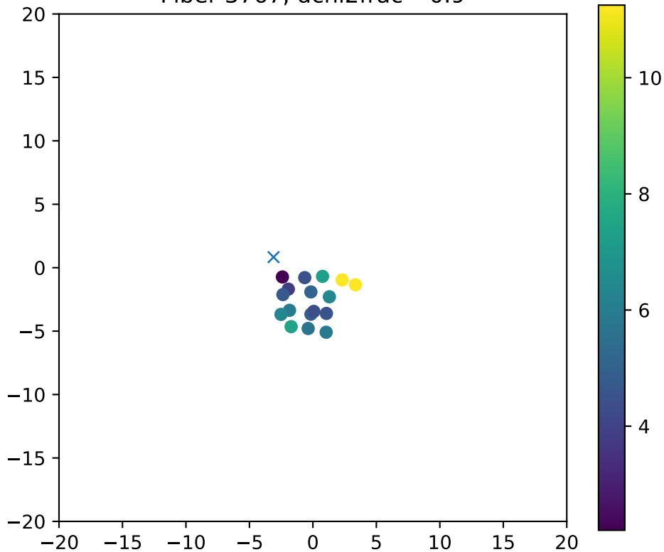
Fiber 3767, dchi2frac= 0.9
