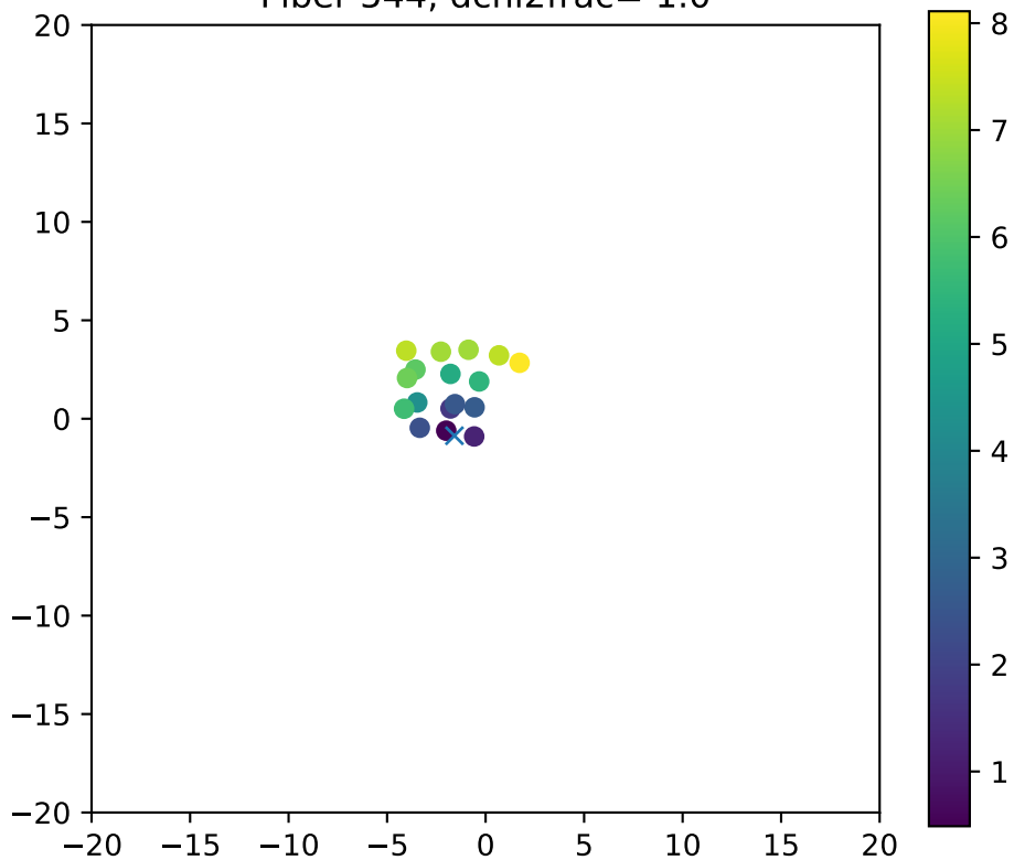
Fiber 544, dchi2frac= 1.0
