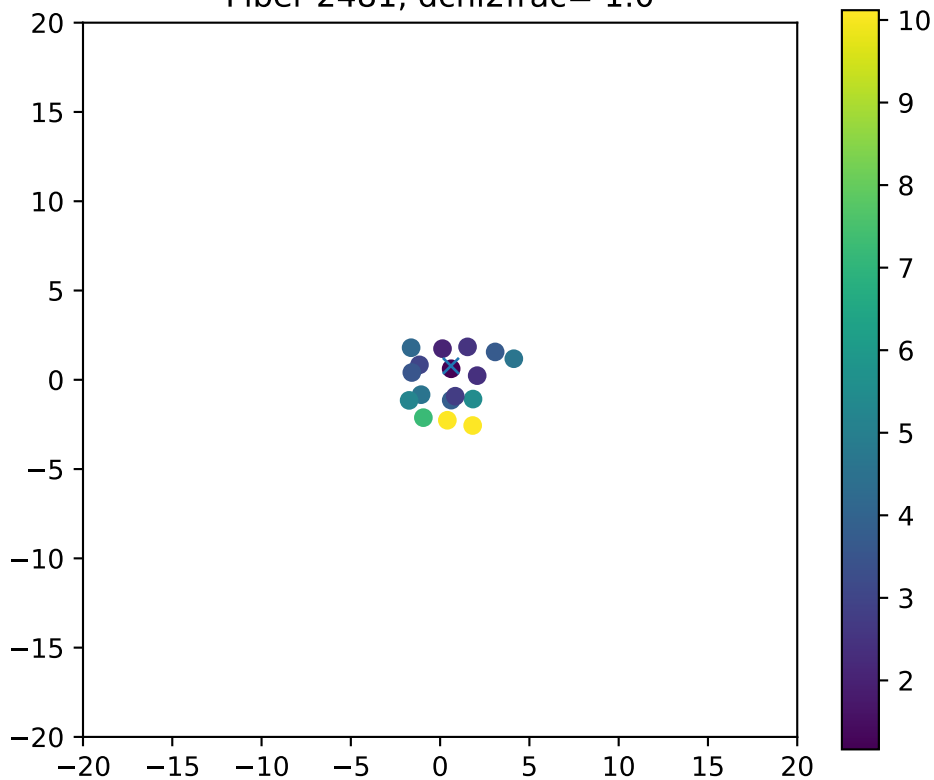
Fiber 2481, dchi2frac= 1.0
