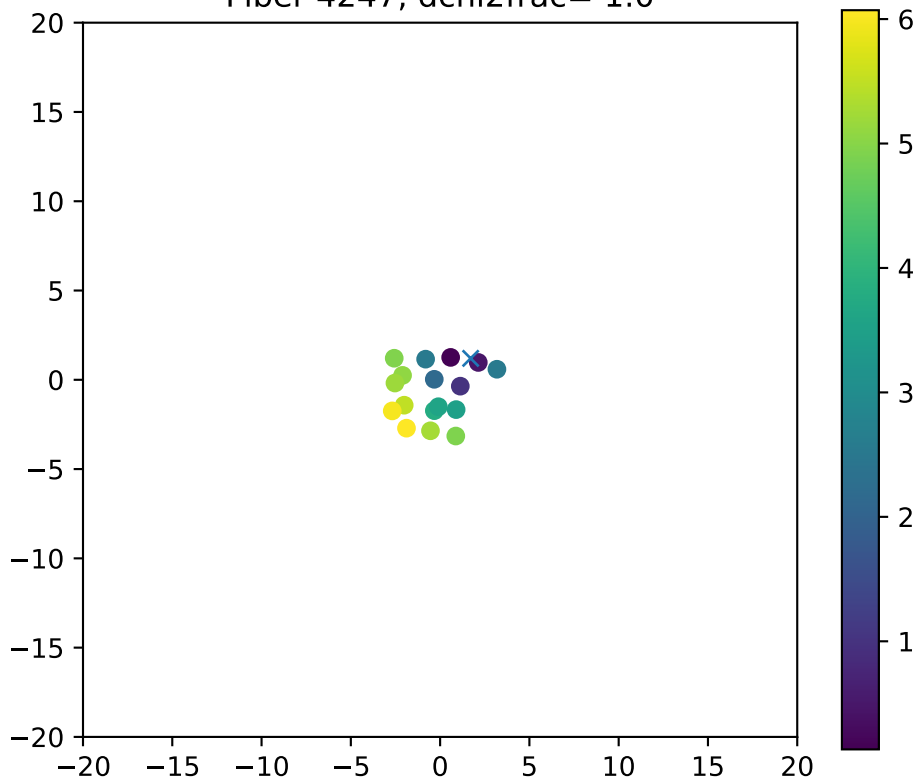
Fiber 4247, dchi2frac= 1.0
