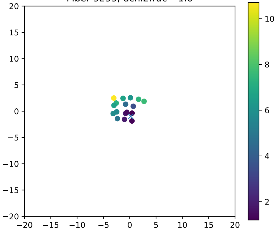
Fiber 3233, dchi2frac= 1.0
