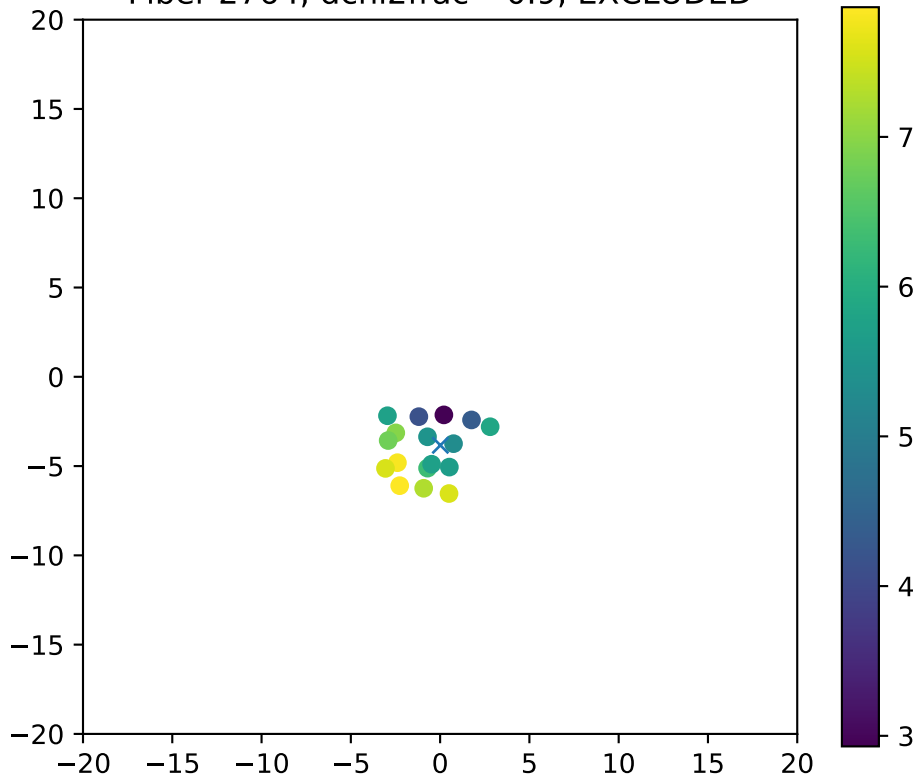
Fiber 2764, dchi2frac= 0.9, EXCLUDED
