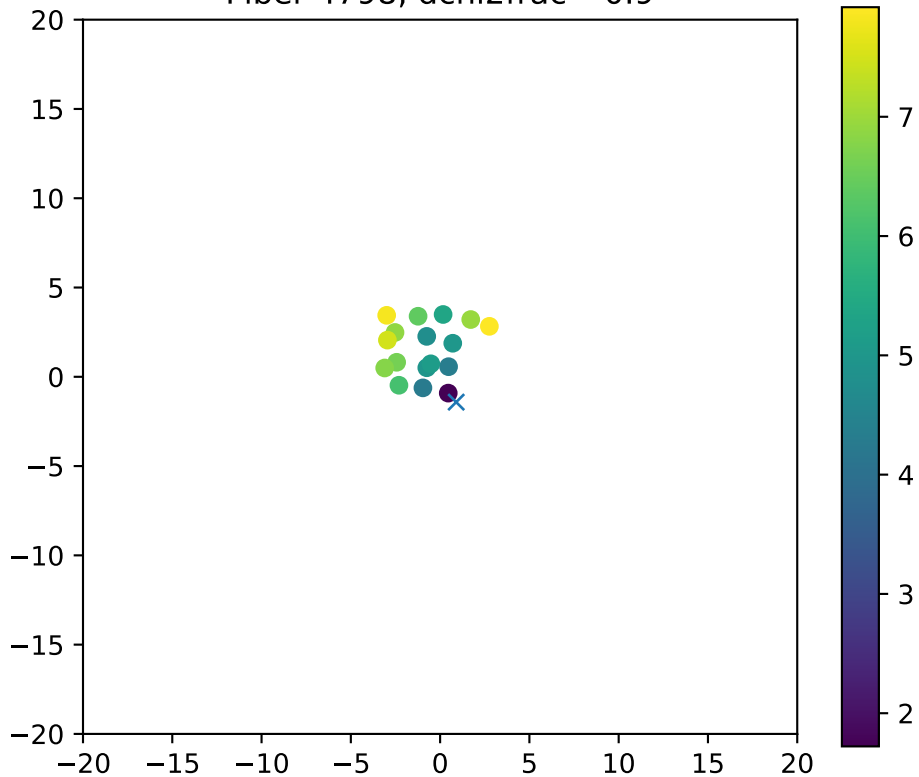
Fiber 4798, dchi2frac= 0.9
