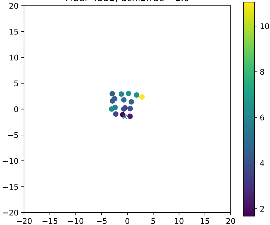
Fiber 4552, dchi2frac= 1.0
