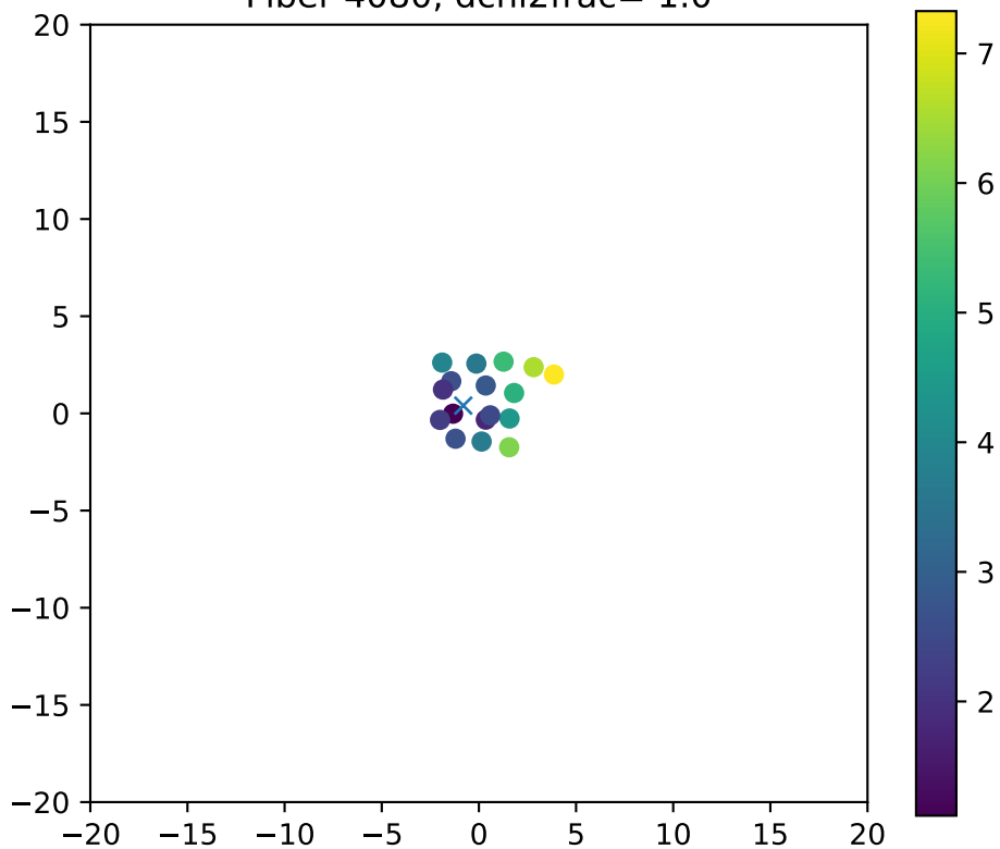
Fiber 4080, dchi2frac= 1.0
