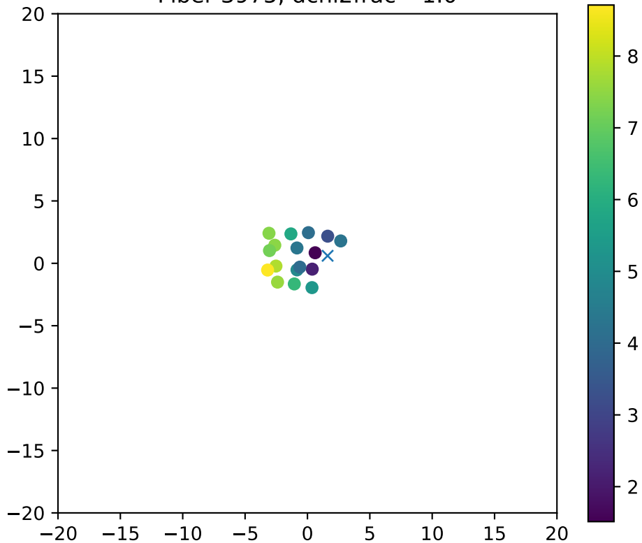
Fiber 3975, dchi2frac= 1.0
