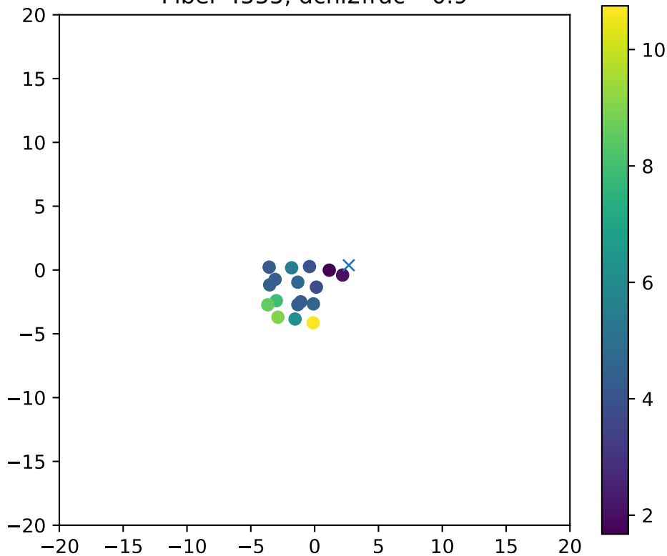
Fiber 4555, dchi2frac= 0.9
