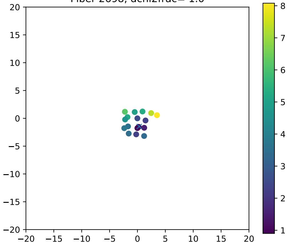
Fiber 2698, dchi2frac= 1.0
