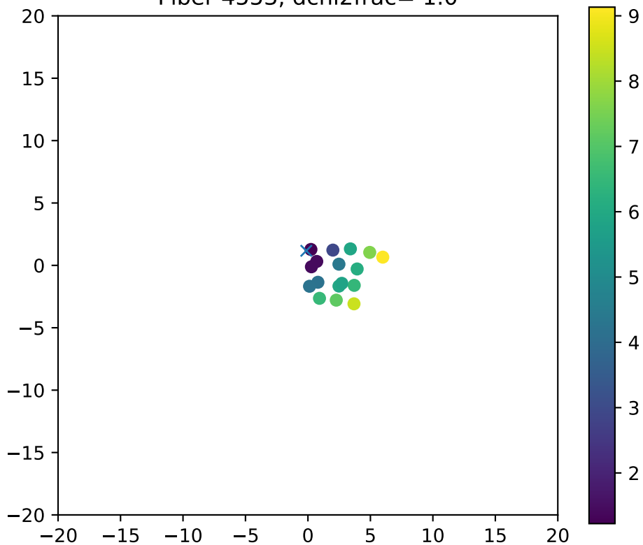
Fiber 4553, dchi2frac= 1.0
