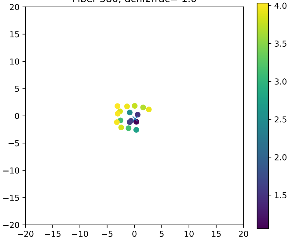
Fiber 580, dchi2frac= 1.0
