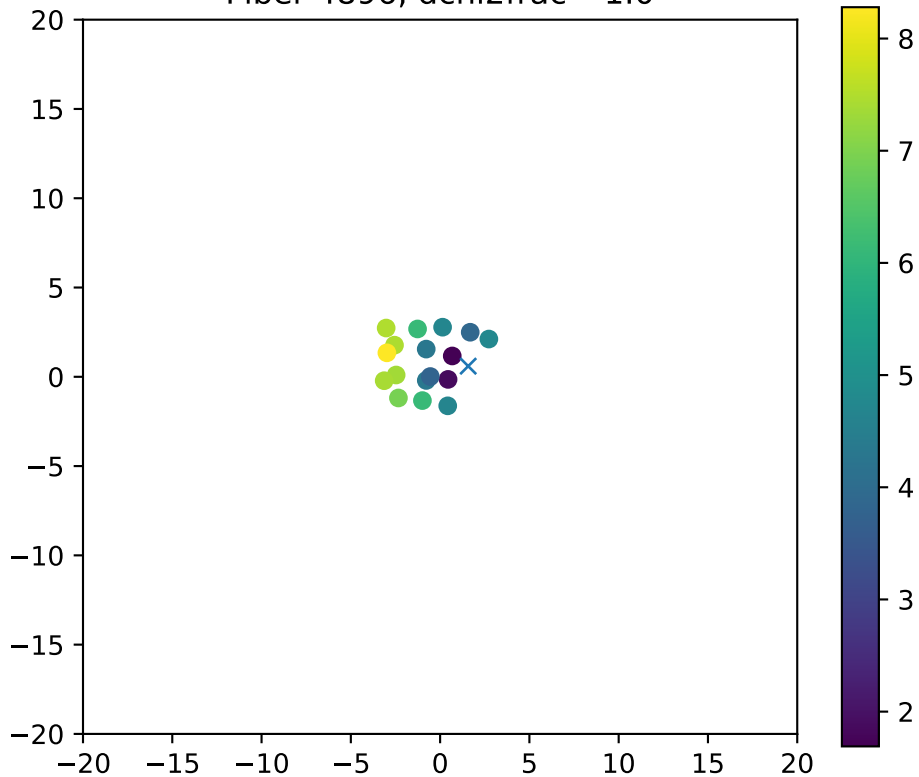
Fiber 4896, dchi2frac= 1.0
