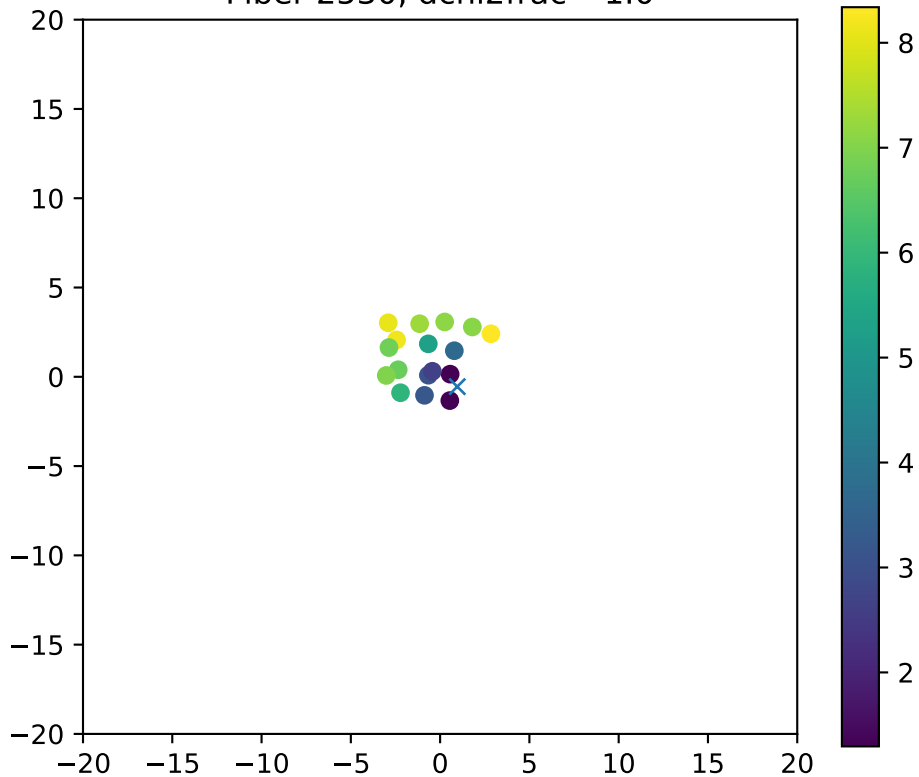
Fiber 2530, dchi2frac= 1.0
