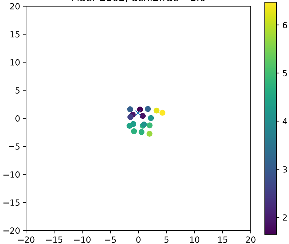
Fiber 2162, dchi2frac= 1.0
