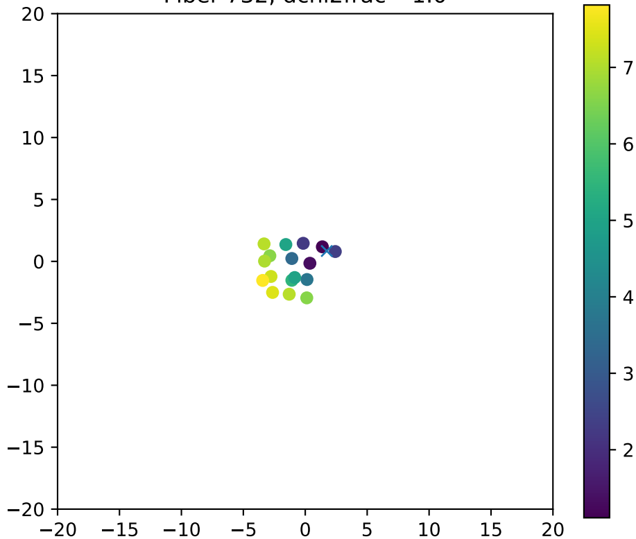
Fiber 732, dchi2frac= 1.0
