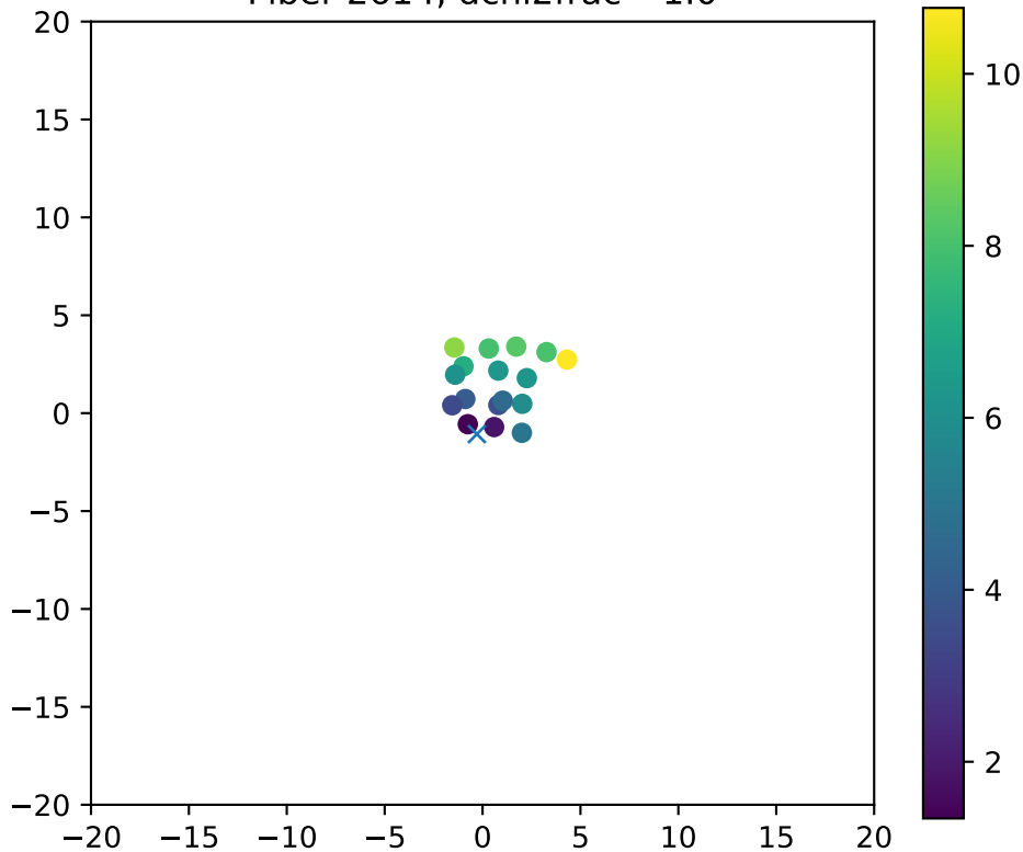
Fiber 2614, dchi2frac= 1.0
