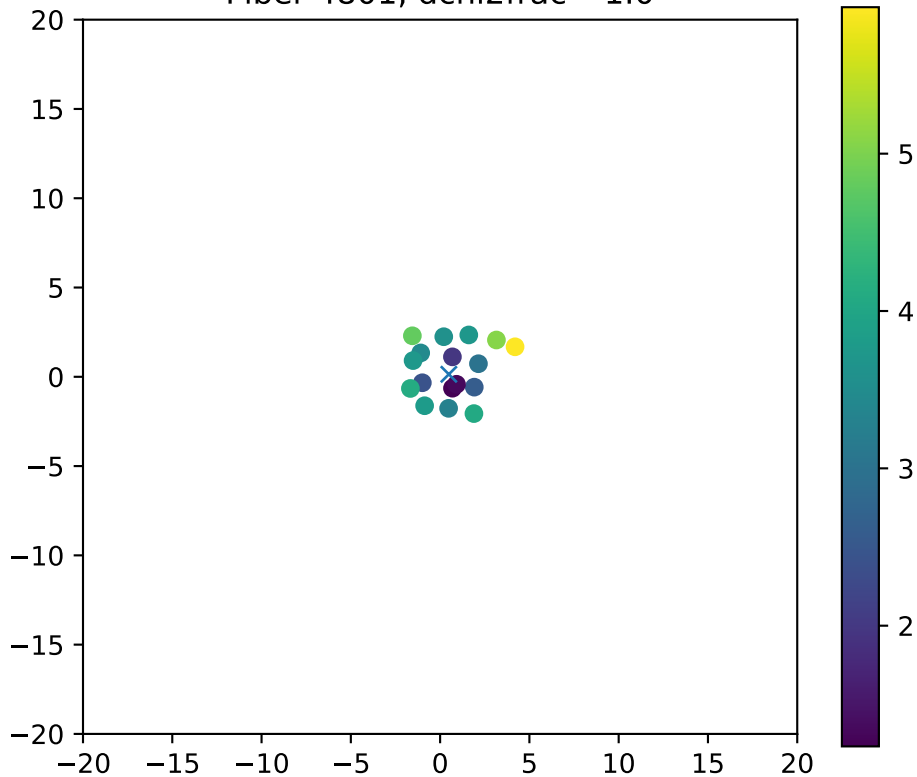
Fiber 4801, dchi2frac= 1.0
