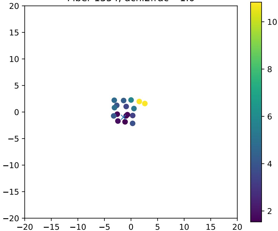
Fiber 1354, dchi2frac= 1.0
