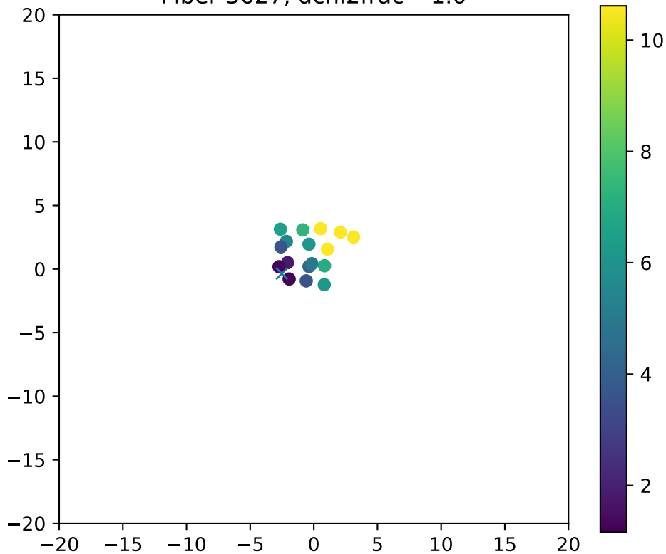
Fiber 3627, dchi2frac= 1.0
