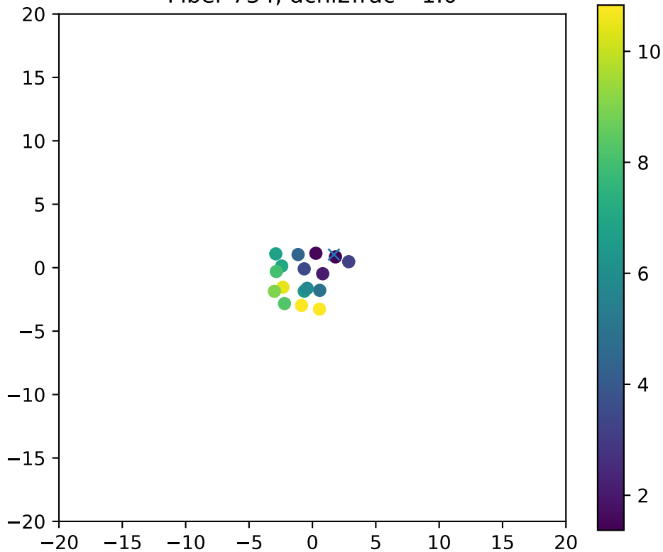
Fiber 734, dchi2frac= 1.0
