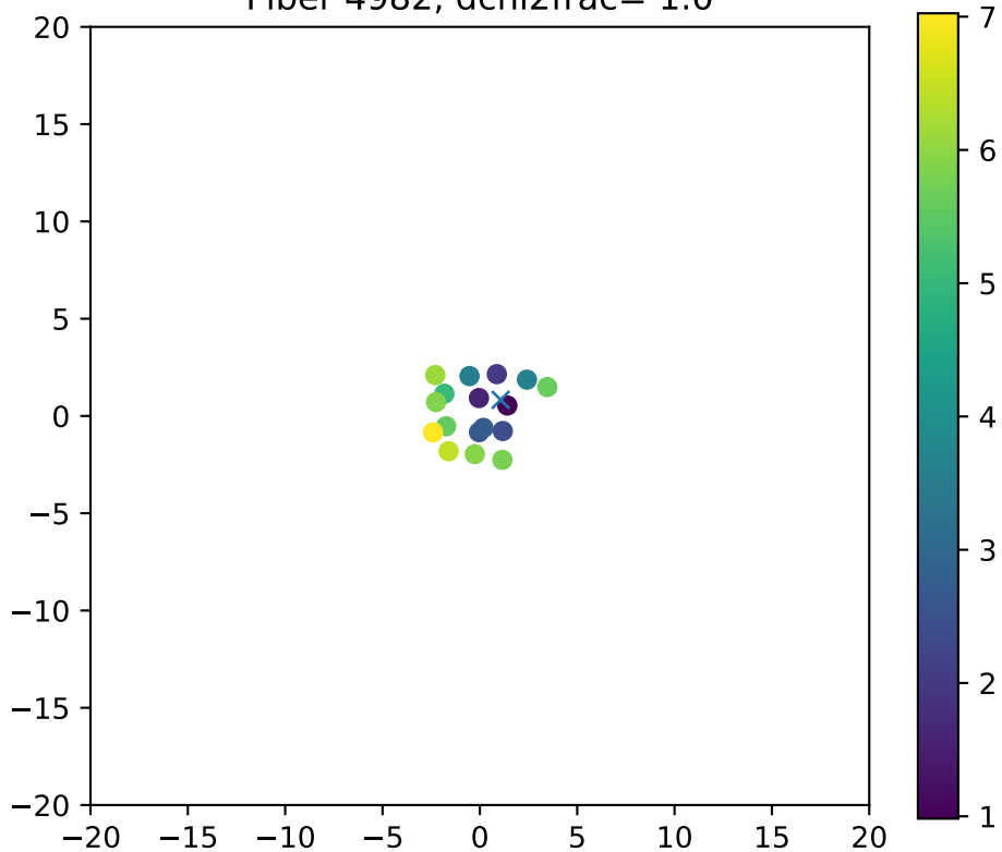
Fiber 4982, dchi2frac= 1.0
