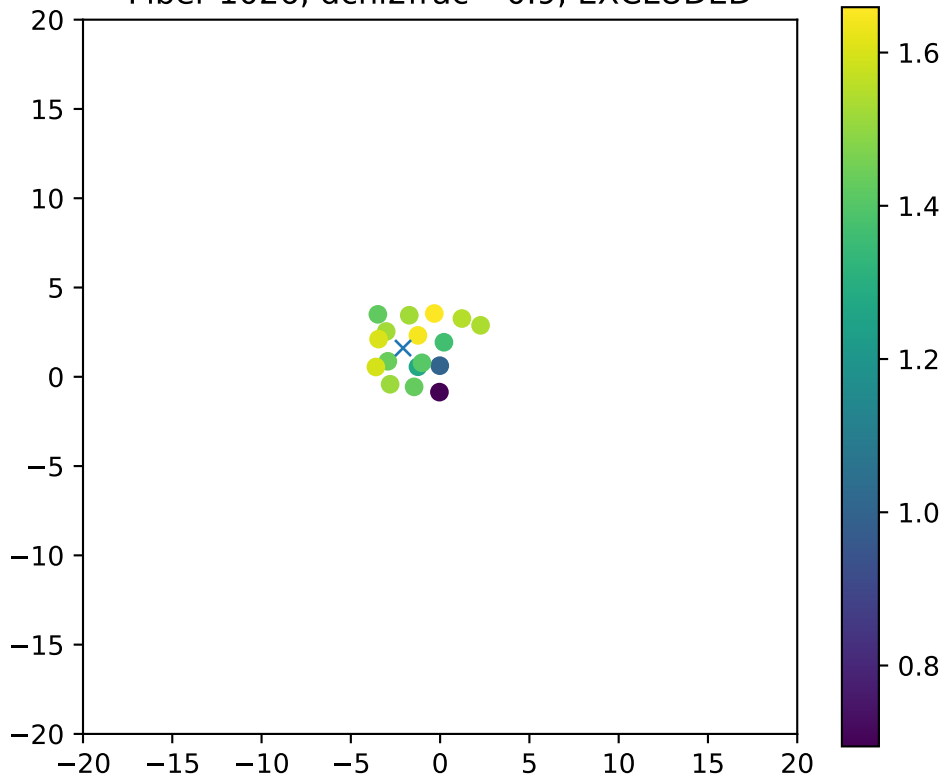
Fiber 1026, dchi2frac= 0.9, EXCLUDED
