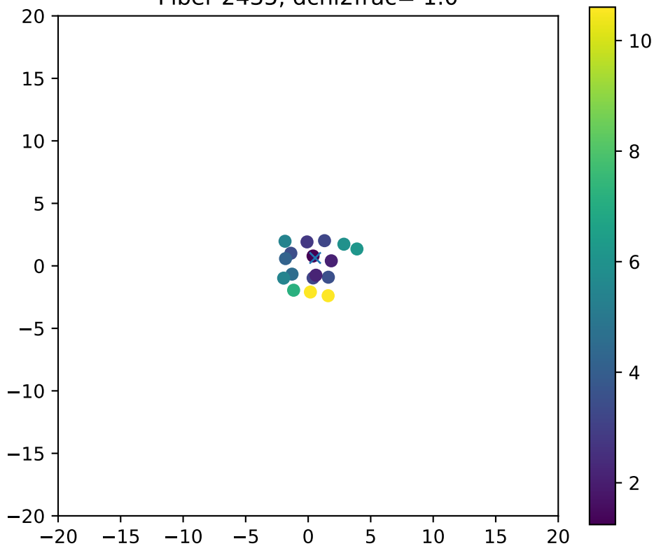
Fiber 2435, dchi2frac= 1.0
