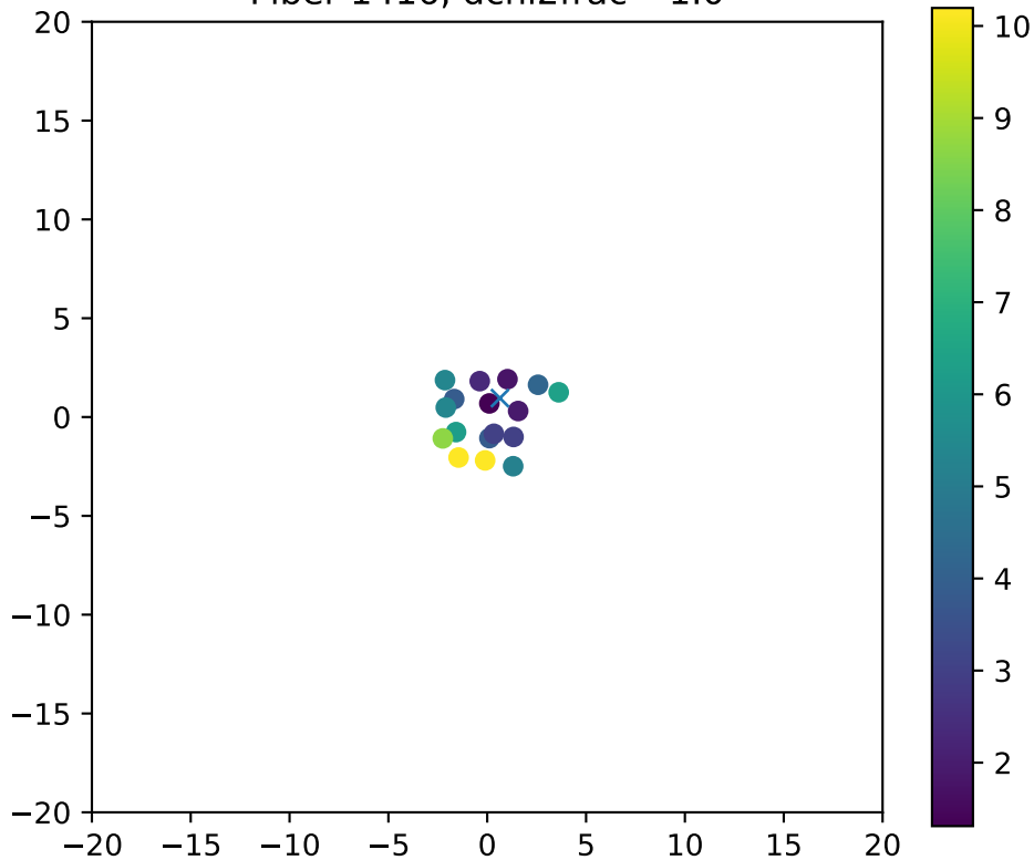
Fiber 1416, dchi2frac= 1.0
