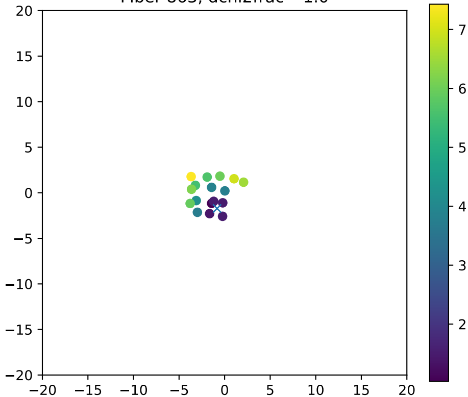
Fiber 863, dchi2frac= 1.0
