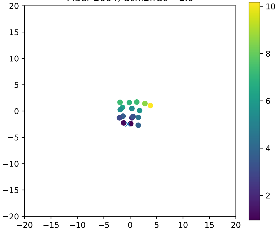
Fiber 2664, dchi2frac= 1.0
