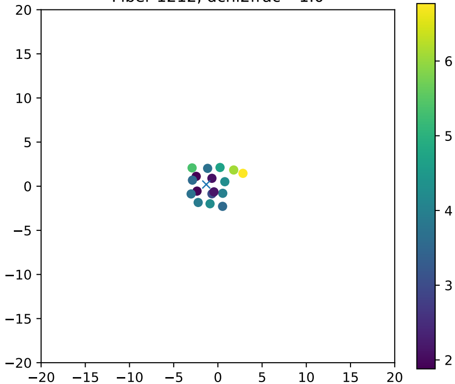
Fiber 1212, dchi2frac= 1.0
