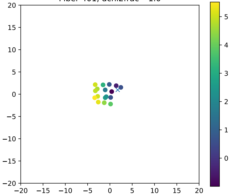
Fiber 401, dchi2frac= 1.0
