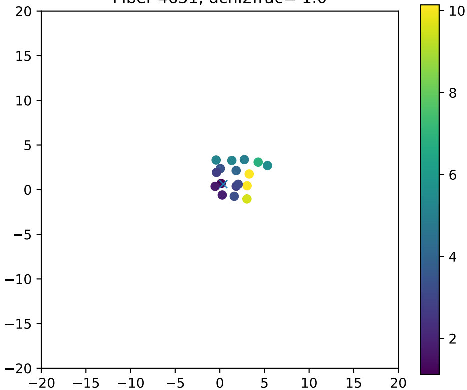
Fiber 4651, dchi2frac= 1.0
