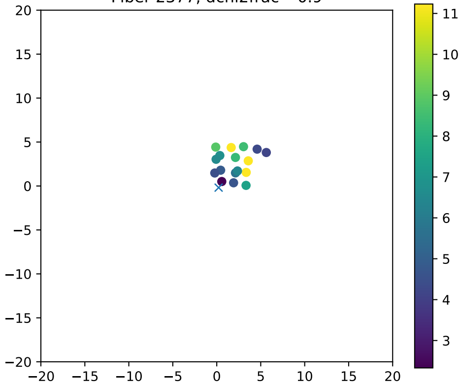
Fiber 2377, dchi2frac= 0.9
