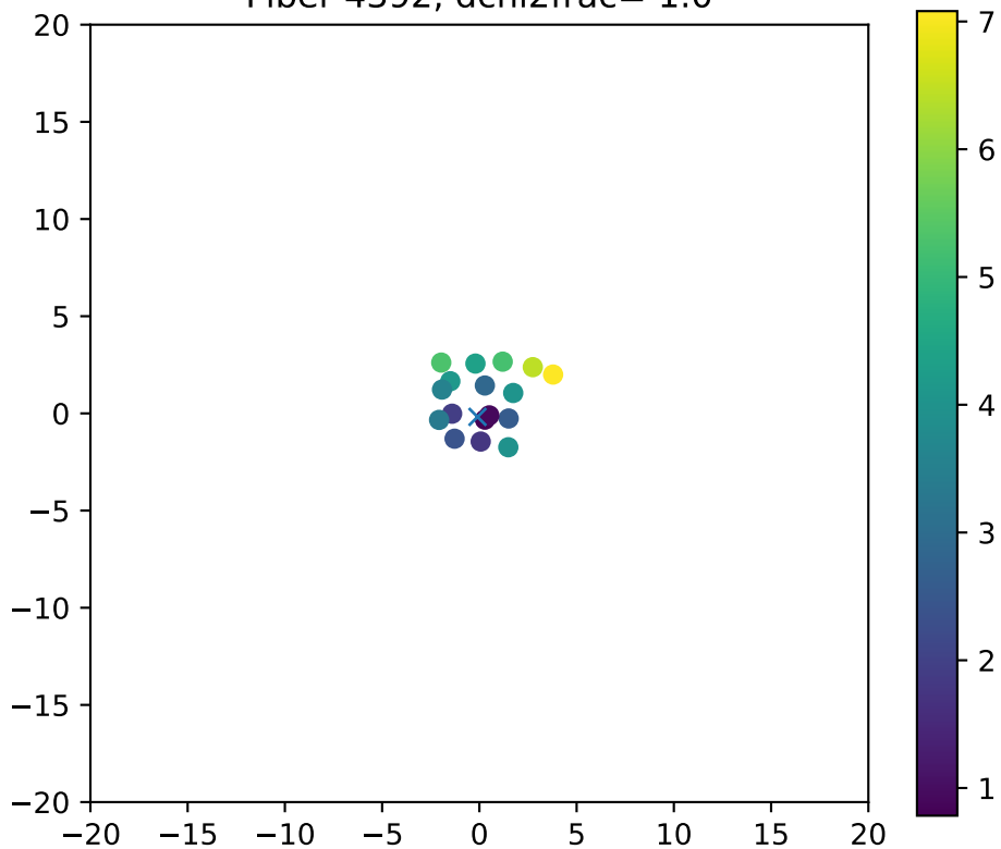
Fiber 4392, dchi2frac= 1.0
