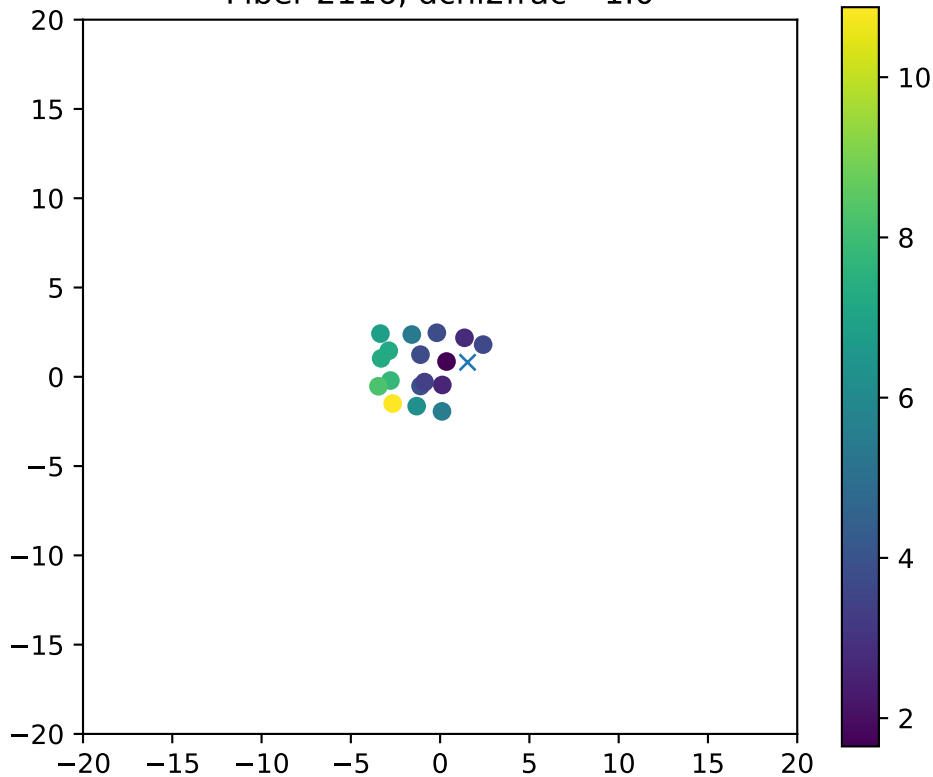
Fiber 2116, dchi2frac= 1.0
