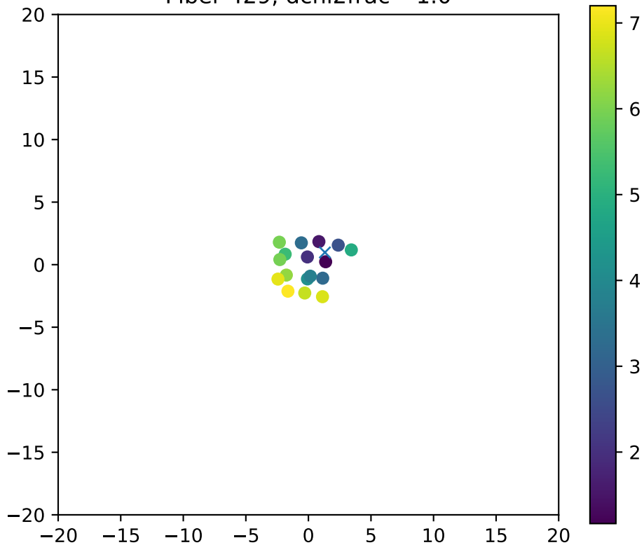
Fiber 429, dchi2frac= 1.0
