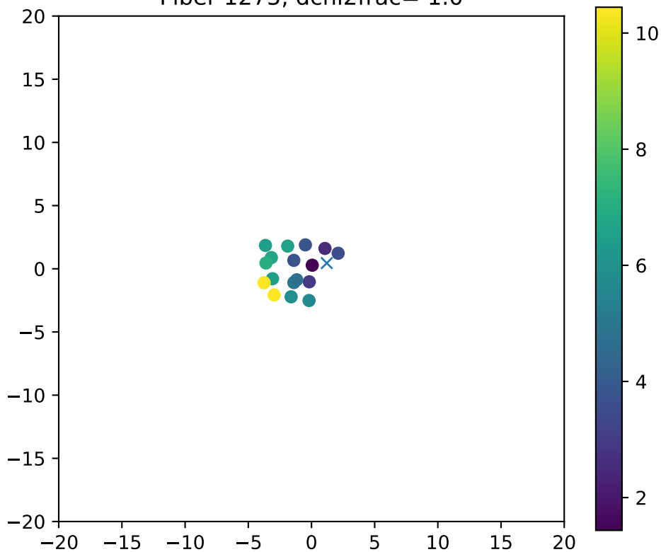
Fiber 1275, dchi2frac= 1.0
