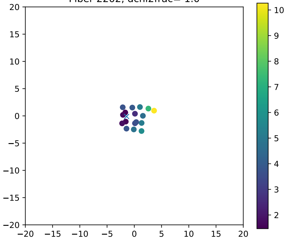
Fiber 2202, dchi2frac= 1.0
