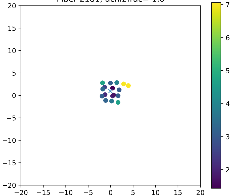
Fiber 2181, dchi2frac= 1.0
