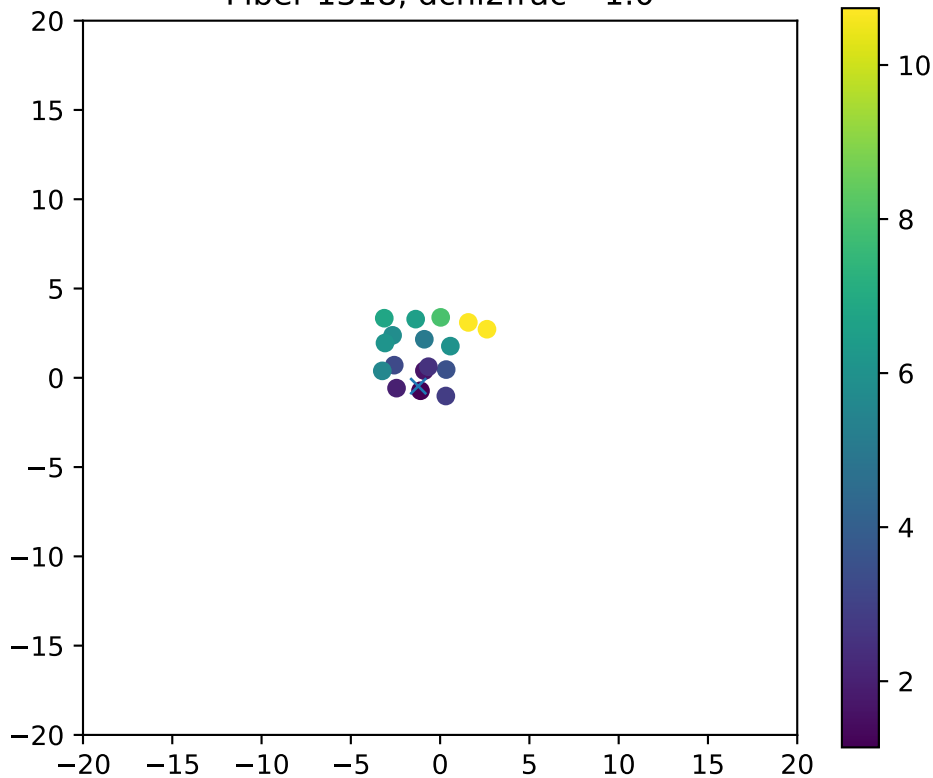
Fiber 1318, dchi2frac= 1.0
