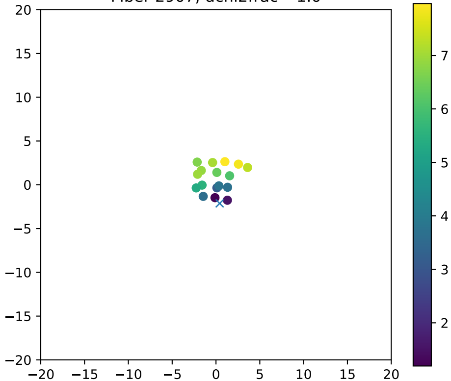
Fiber 2907, dchi2frac= 1.0
