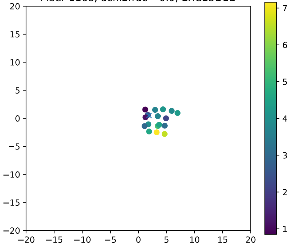
Fiber 1168, dchi2frac= 0.9, EXCLUDED
