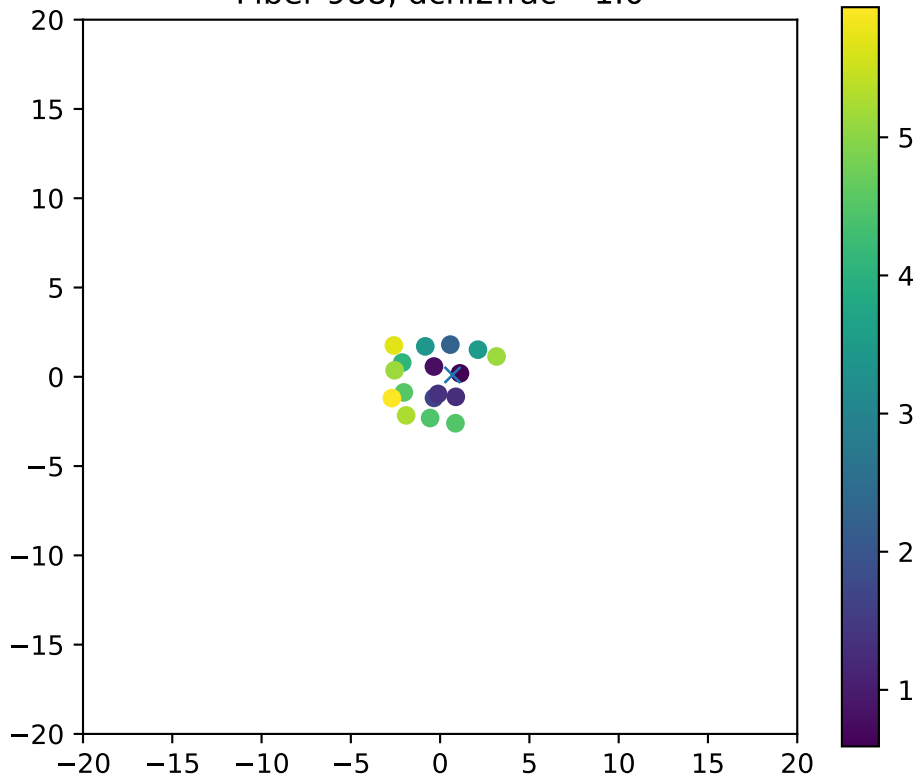
Fiber 988, dchi2frac= 1.0
