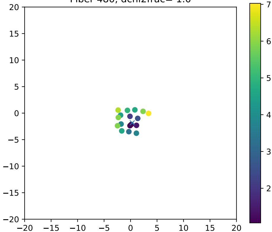
Fiber 480, dchi2frac= 1.0
