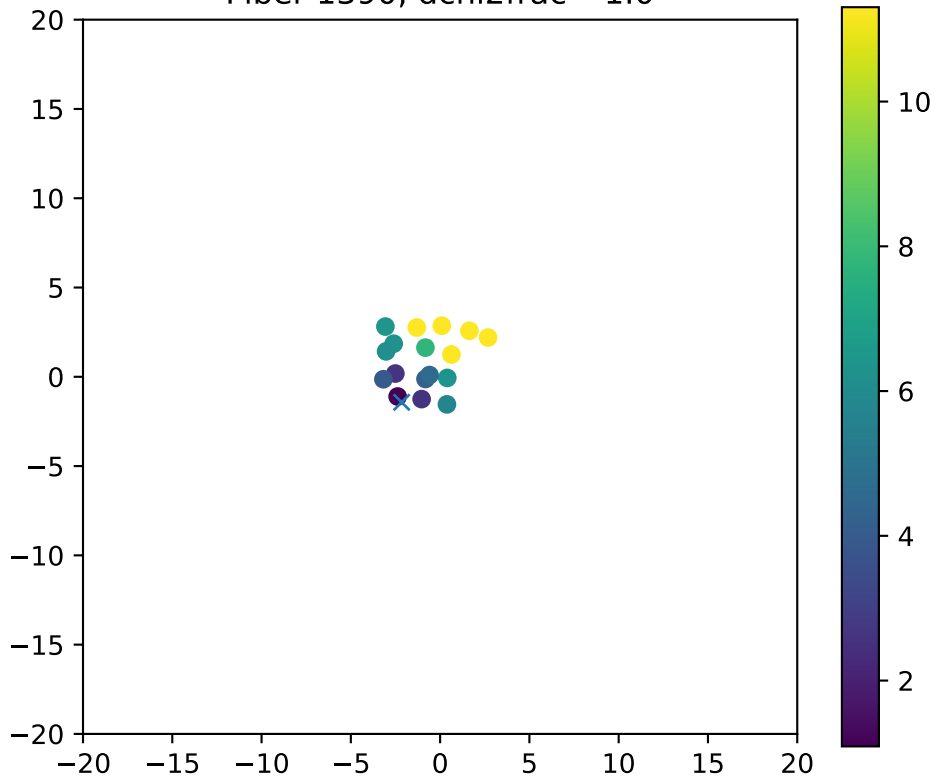
Fiber 1390, dchi2frac= 1.0
