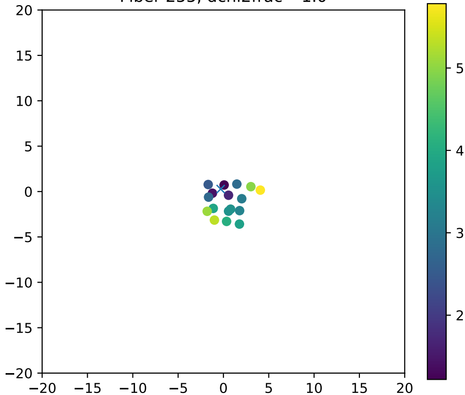
Fiber 255, dchi2frac= 1.0
