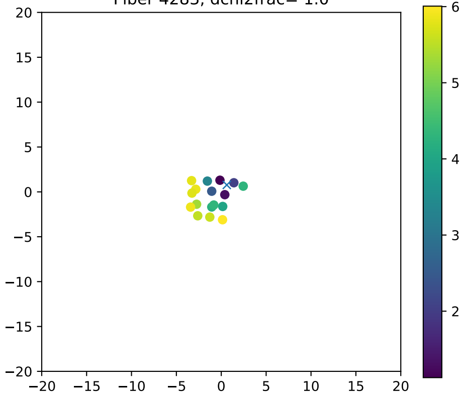
Fiber 4283, dchi2frac= 1.0
