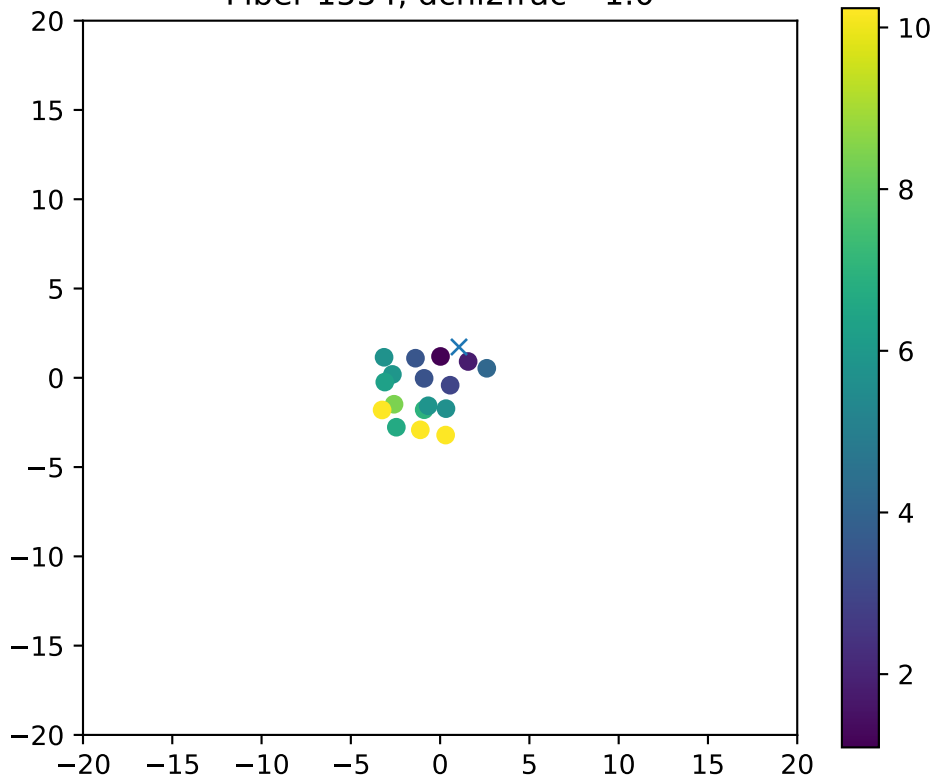
Fiber 1554, dchi2frac= 1.0
