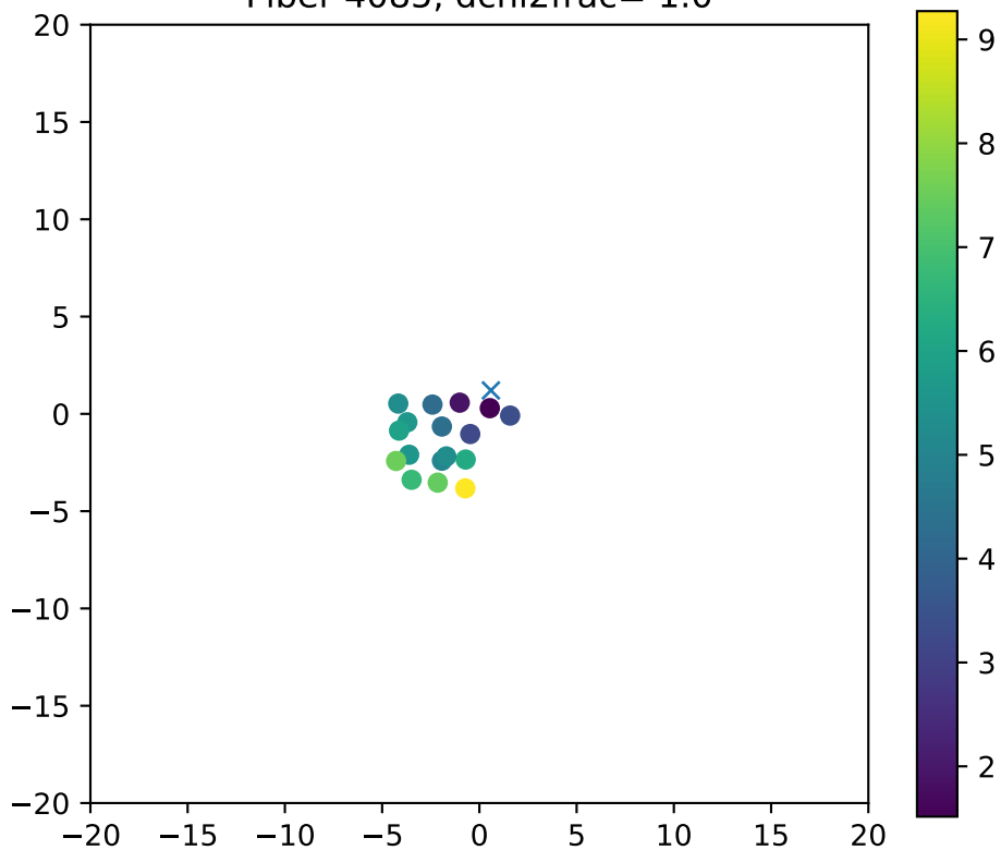
Fiber 4085, dchi2frac= 1.0
