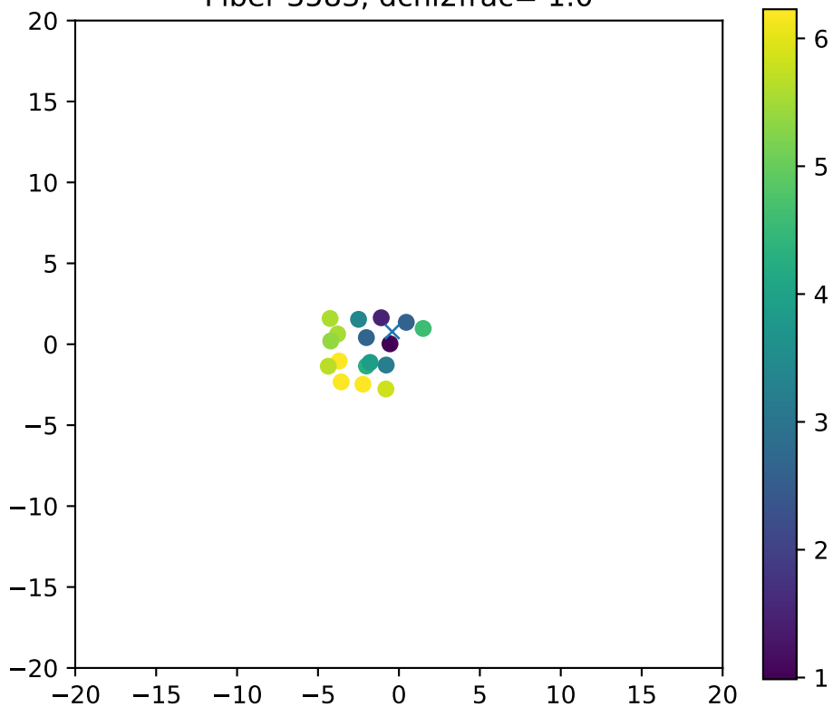
Fiber 3583, dchi2frac= 1.0
