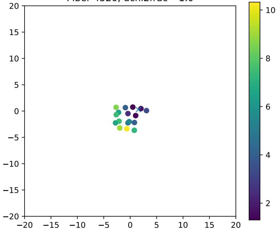
Fiber 4520, dchi2frac= 1.0
