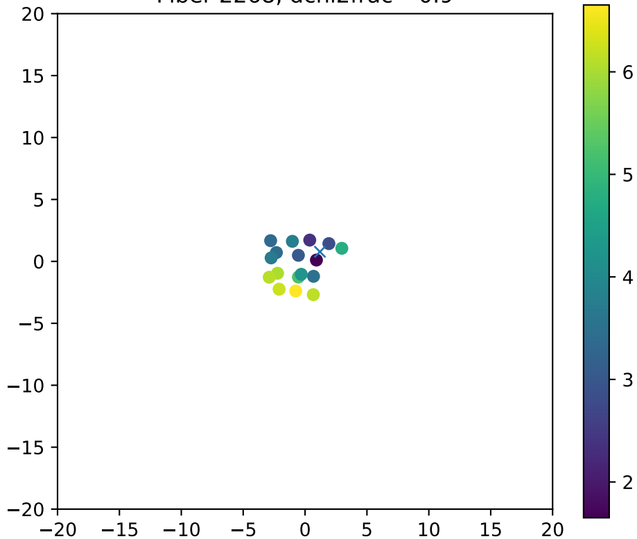
Fiber 2268, dchi2frac= 0.9
