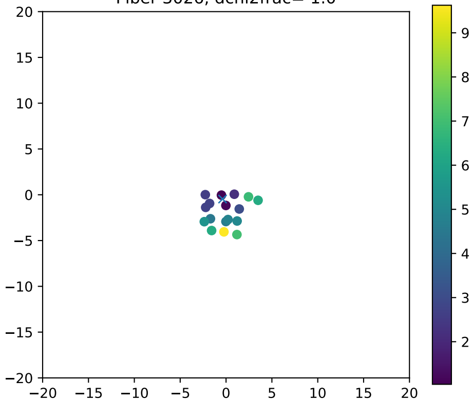
Fiber 3026, dchi2frac= 1.0
