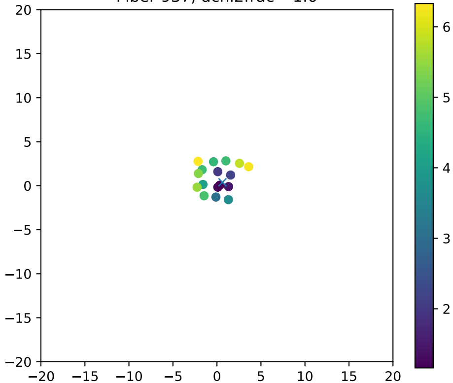
Fiber 937, dchi2frac= 1.0
