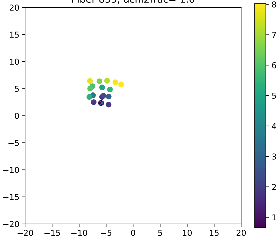
Fiber 859, dchi2frac= 1.0
