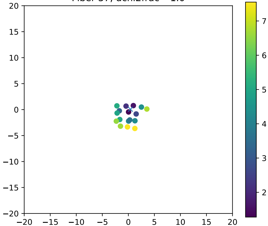
Fiber 37, dchi2frac= 1.0
