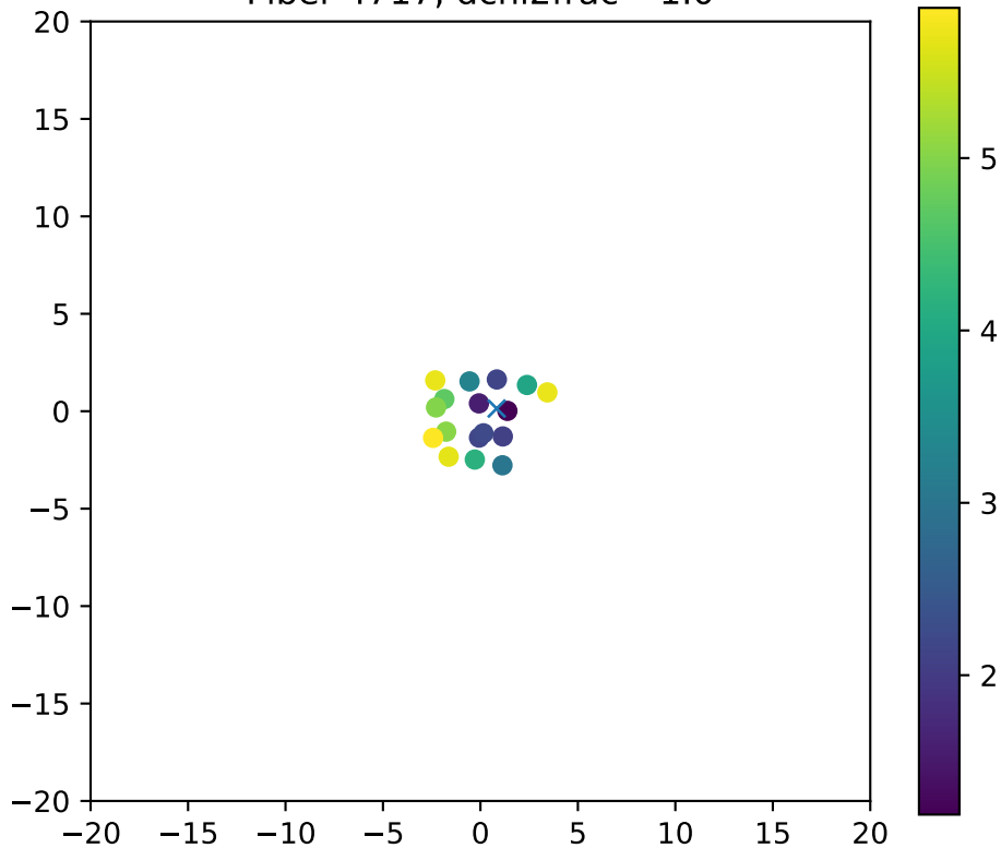
Fiber 4717, dchi2frac= 1.0
