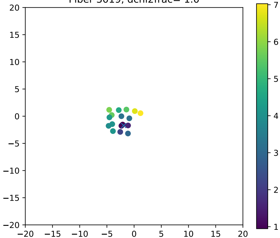
Fiber 3019, dchi2frac= 1.0
