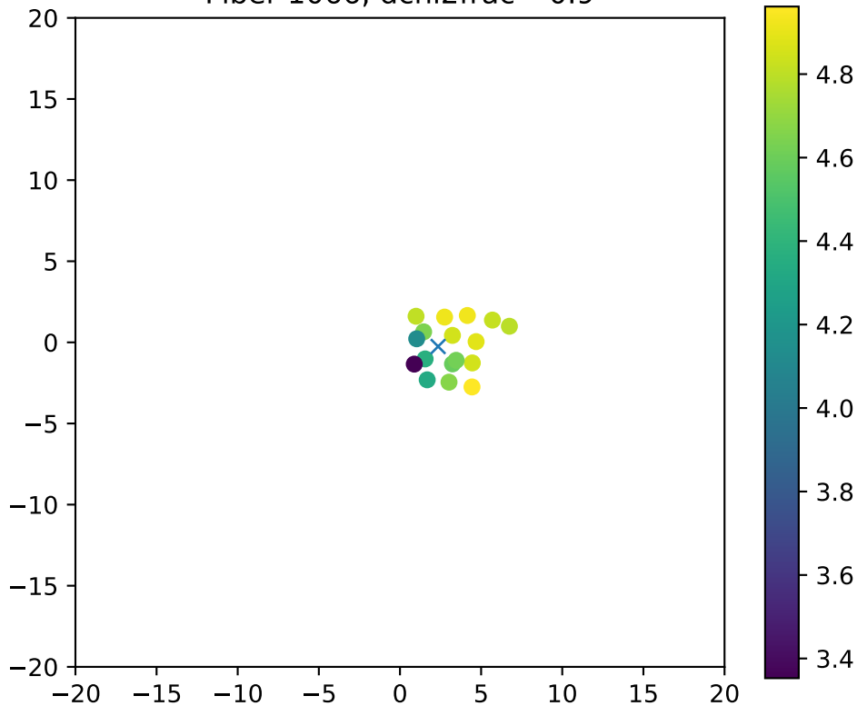
Fiber 1066, dchi2frac= 0.9
