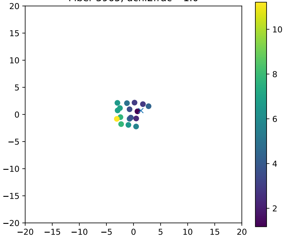
Fiber 3965, dchi2frac= 1.0
