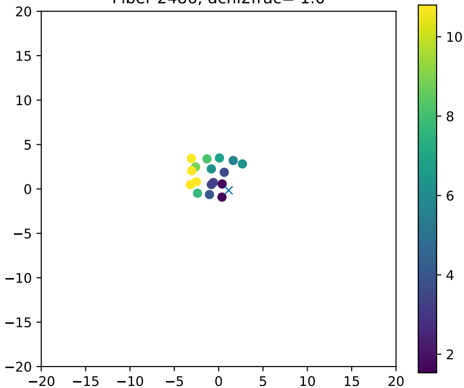
Fiber 2486, dchi2frac= 1.0
