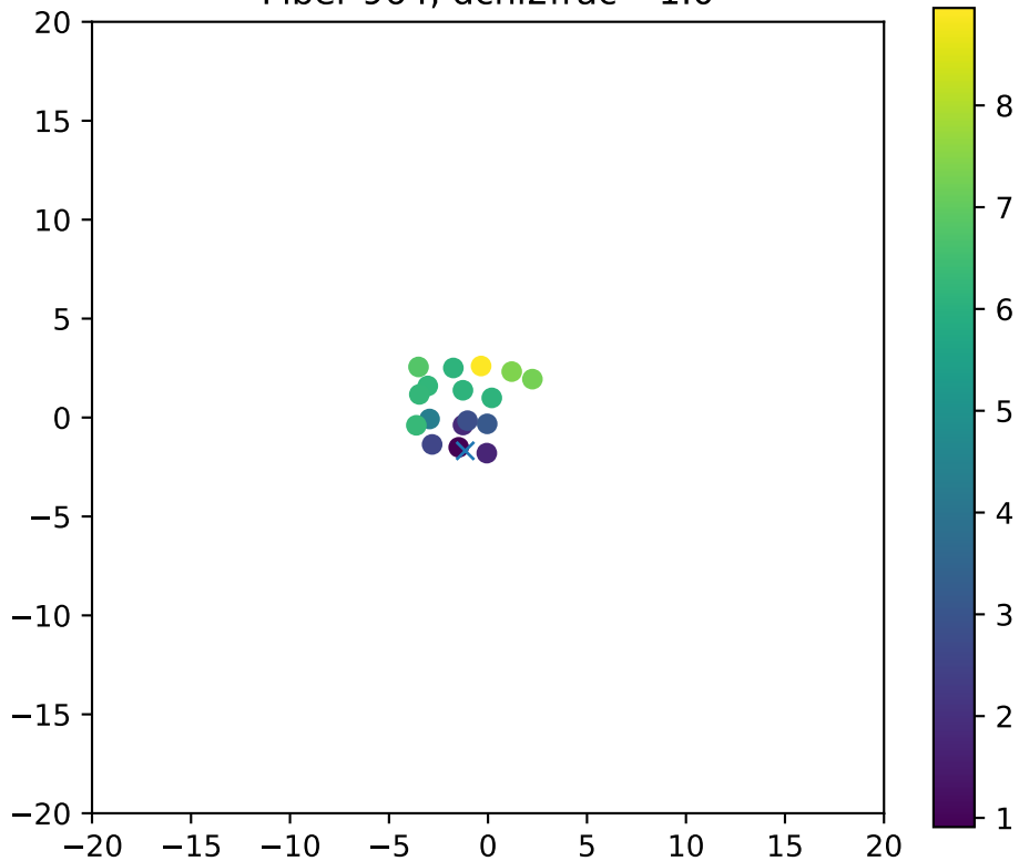
Fiber 964, dchi2frac= 1.0
