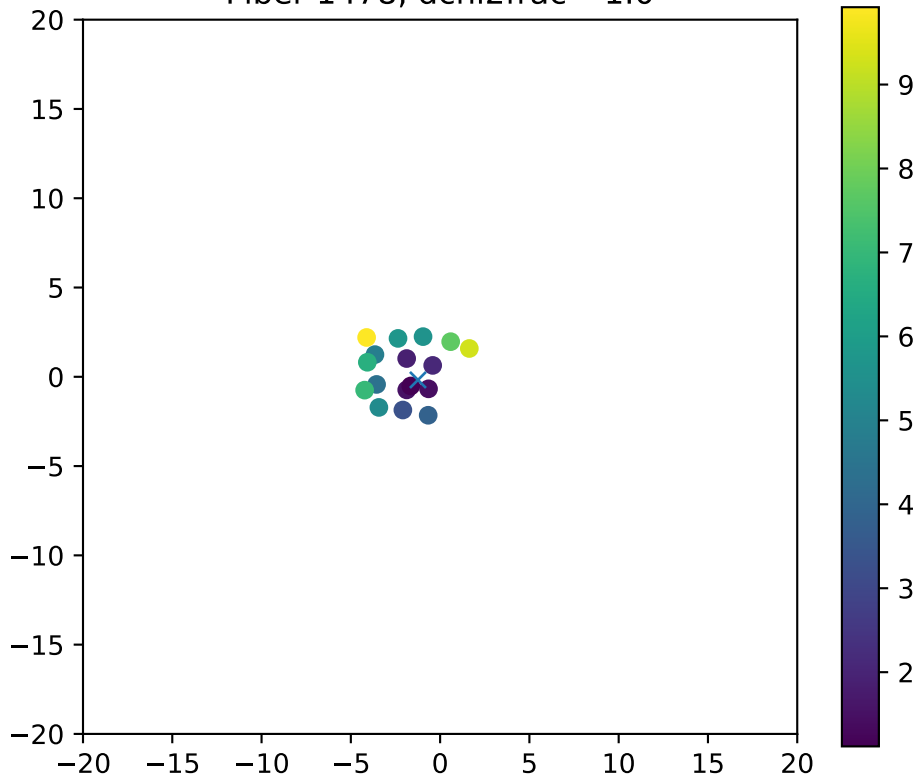
Fiber 1478, dchi2frac= 1.0
