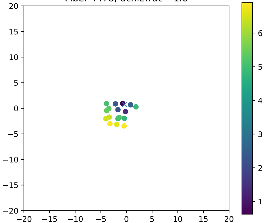
Fiber 4478, dchi2frac= 1.0
