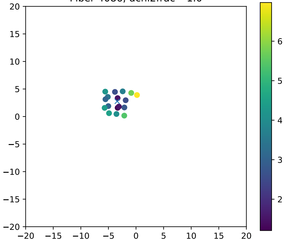
Fiber 4086, dchi2frac= 1.0
