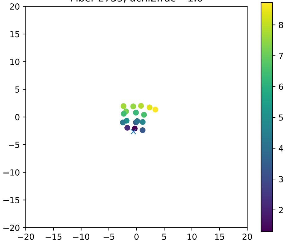
Fiber 2755, dchi2frac= 1.0
