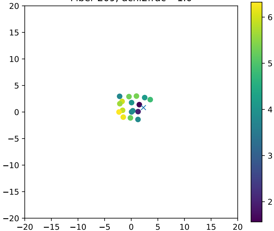
Fiber 209, dchi2frac= 1.0
