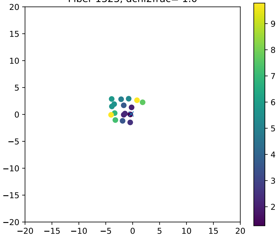
Fiber 1323, dchi2frac= 1.0
