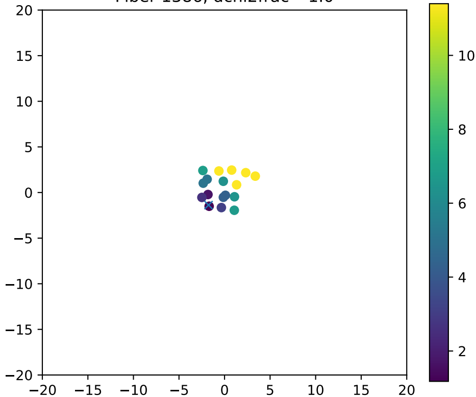
Fiber 1386, dchi2frac= 1.0
