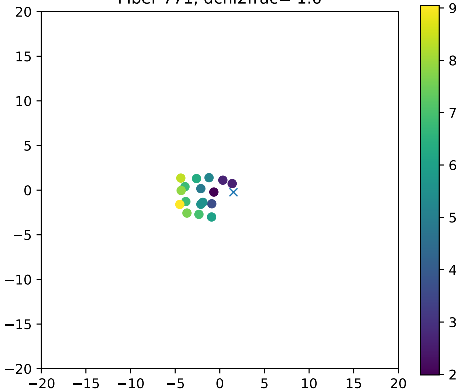
Fiber 771, dchi2frac= 1.0
