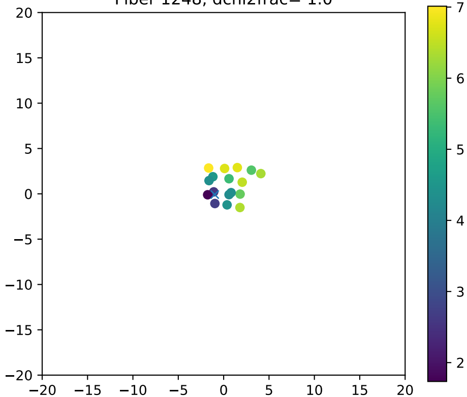
Fiber 1248, dchi2frac= 1.0
