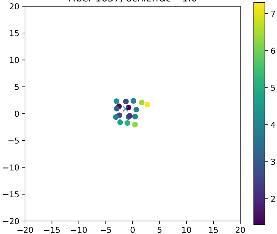
Fiber 1637, dchi2frac= 1.0
