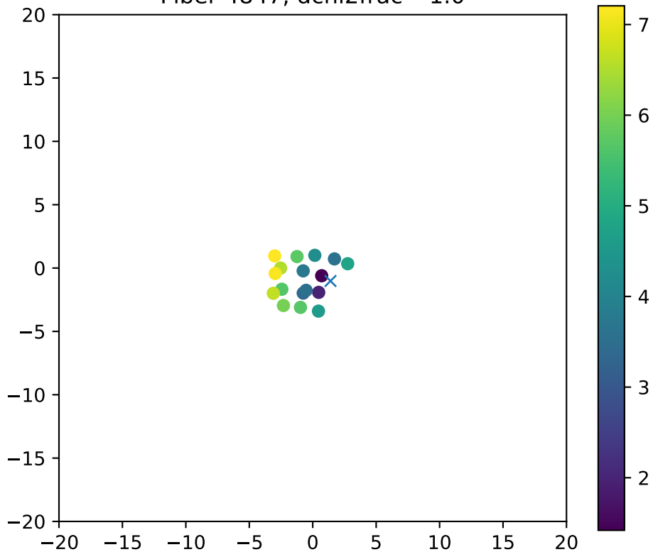
Fiber 4847, dchi2frac= 1.0
