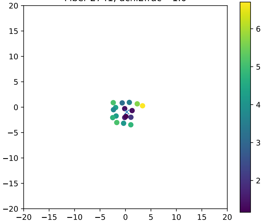
Fiber 2741, dchi2frac= 1.0
