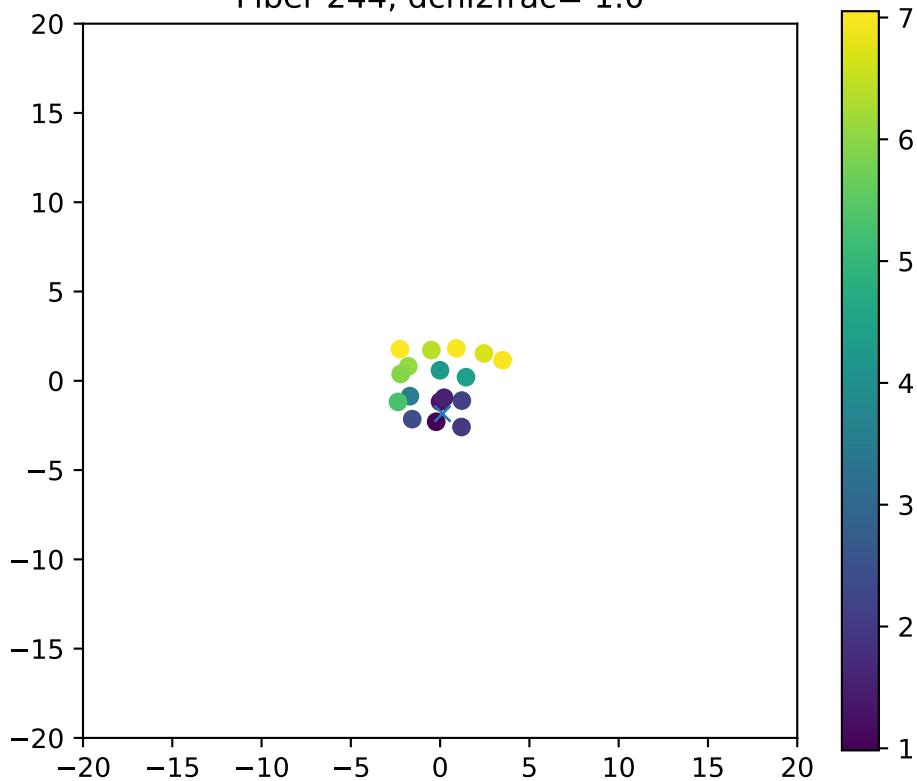
Fiber 244, dchi2frac= 1.0
