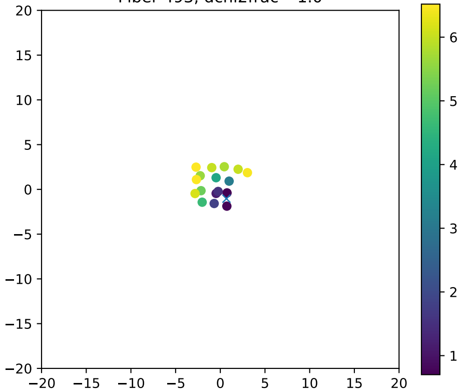
Fiber 493, dchi2frac= 1.0
