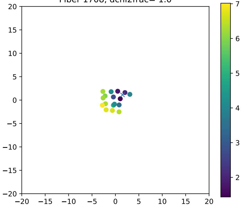
Fiber 1708, dchi2frac= 1.0
