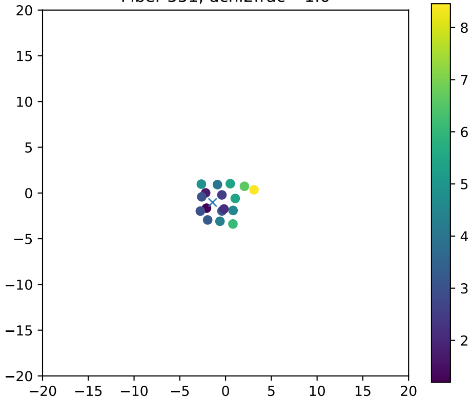
Fiber 551, dchi2frac= 1.0
