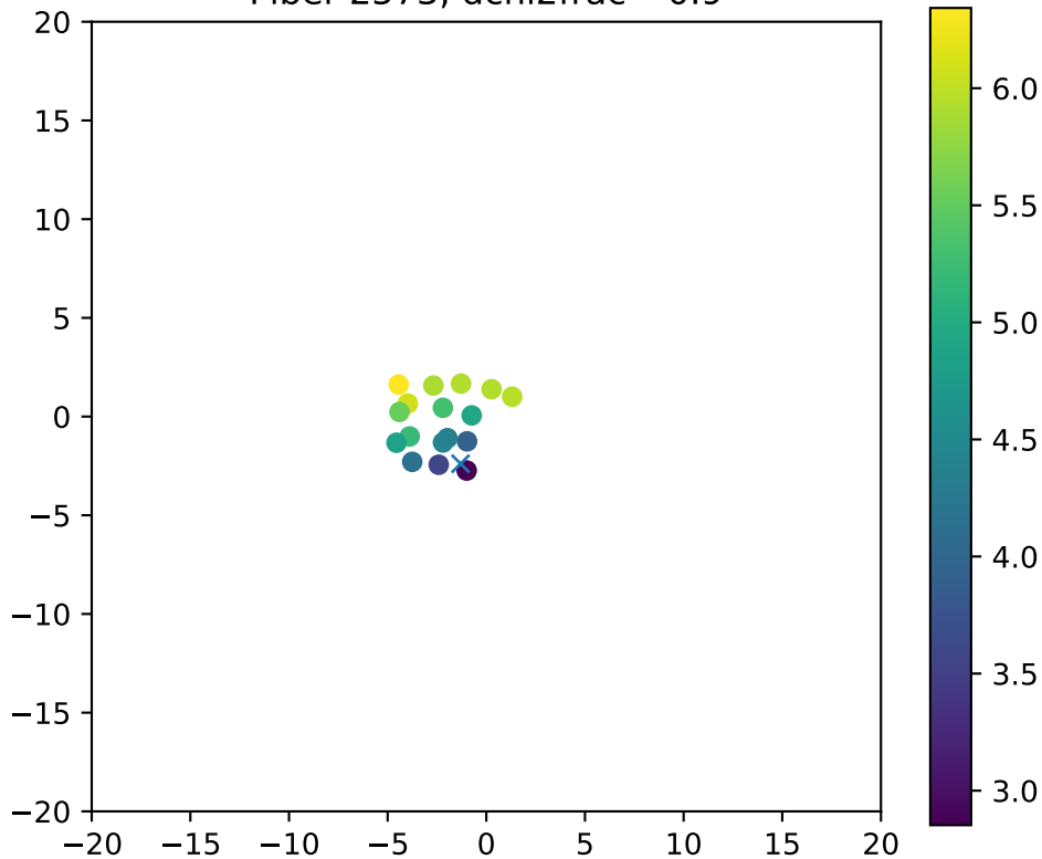
Fiber 2573, dchi2frac= 0.9
