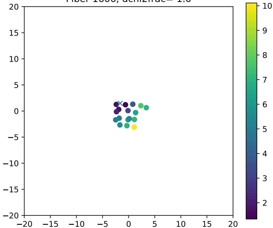
Fiber 1606, dchi2frac= 1.0
