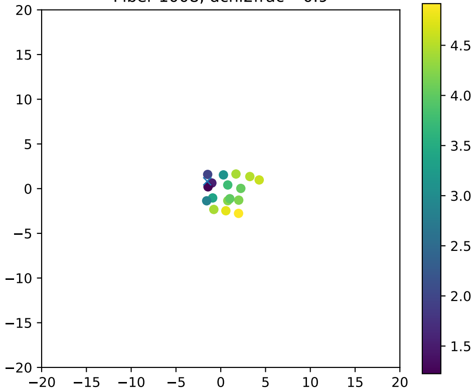
Fiber 1008, dchi2frac= 0.9
