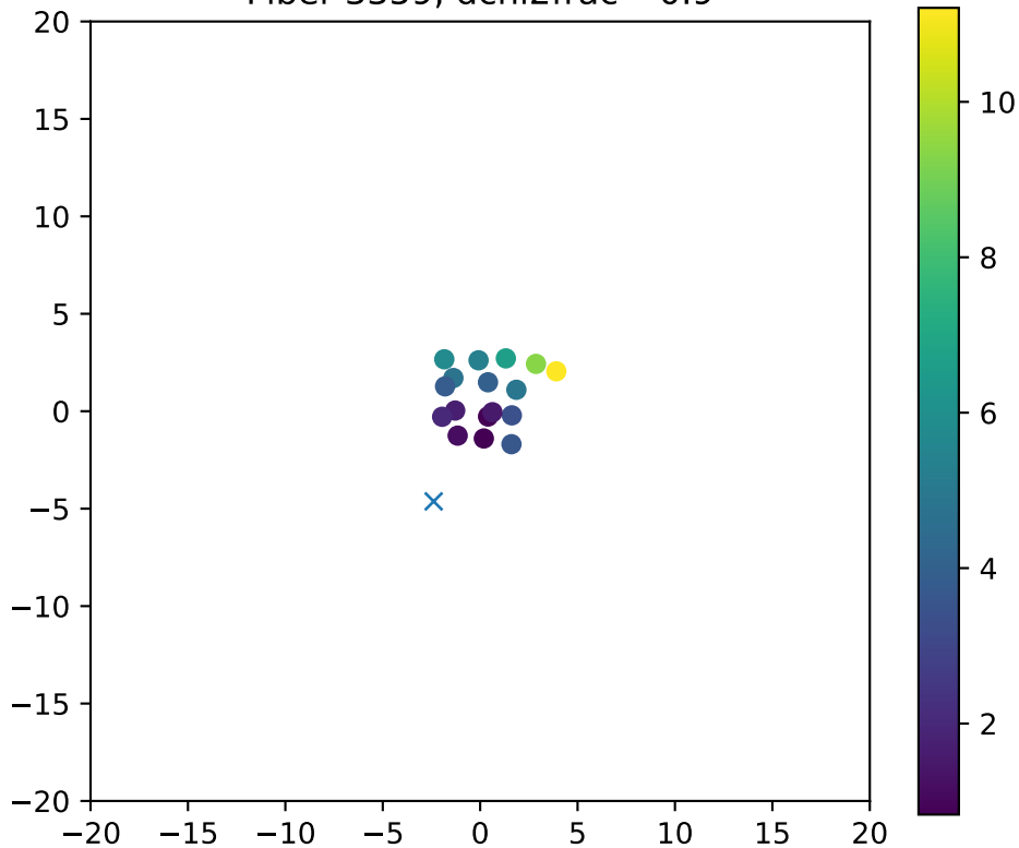
Fiber 3359, dchi2frac= 0.9
