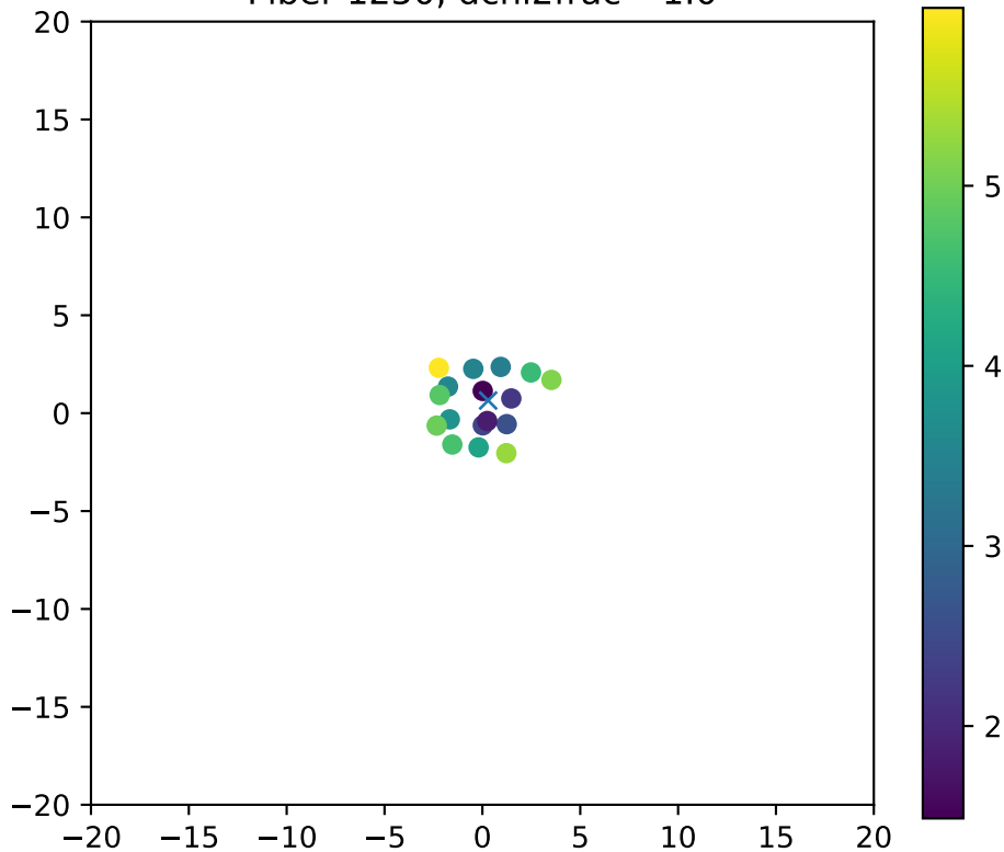
Fiber 1250, dchi2frac= 1.0
