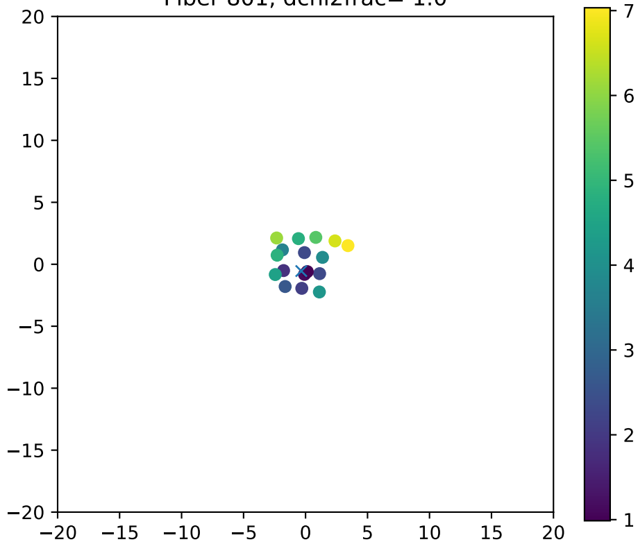
Fiber 801, dchi2frac= 1.0
