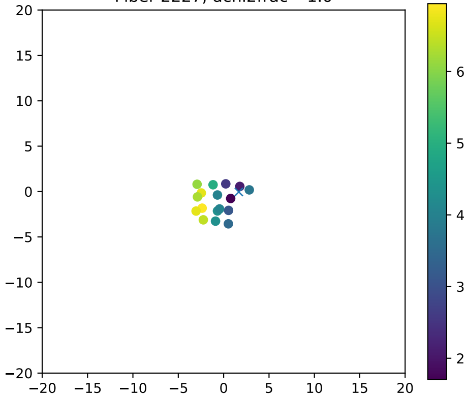
Fiber 2227, dchi2frac= 1.0
