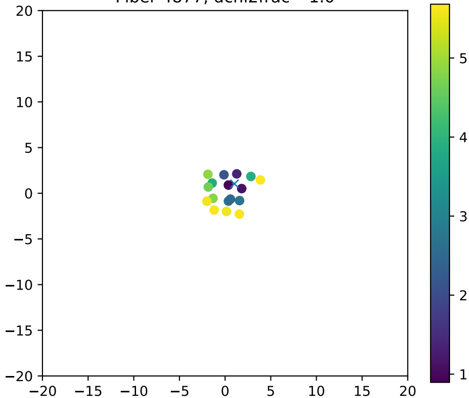
Fiber 4877, dchi2frac= 1.0
