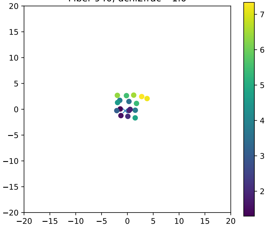
Fiber 940, dchi2frac= 1.0
