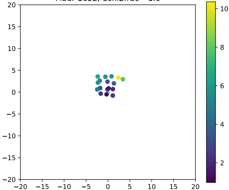
Fiber 1652, dchi2frac= 1.0
