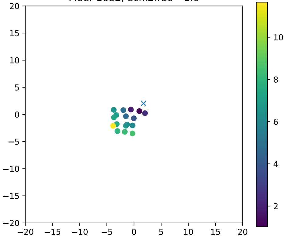
Fiber 1682, dchi2frac= 1.0
