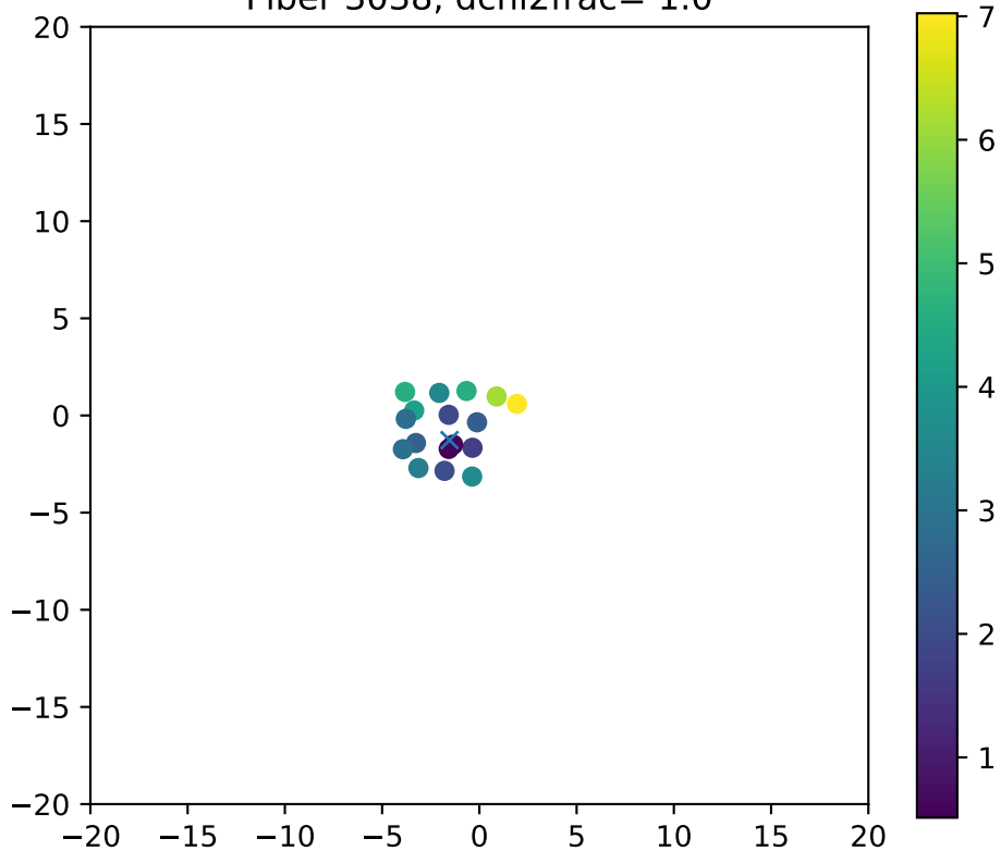
Fiber 3038, dchi2frac= 1.0
