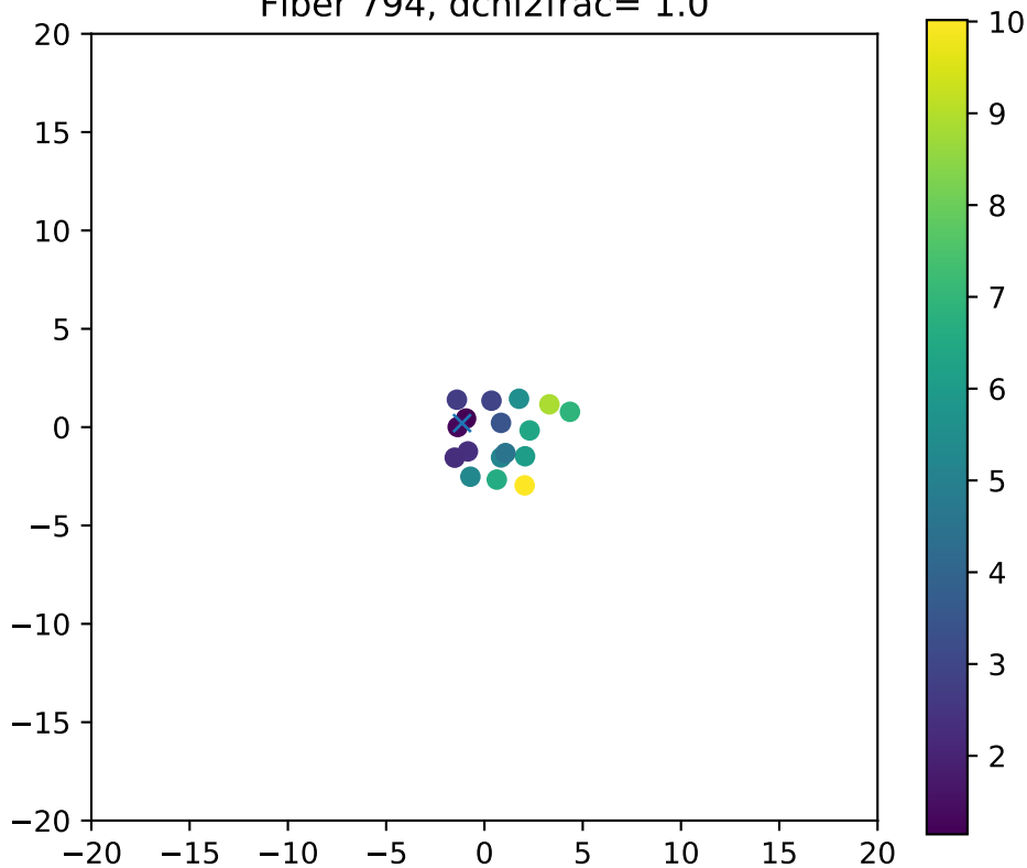
Fiber 794, dchi2frac= 1.0
