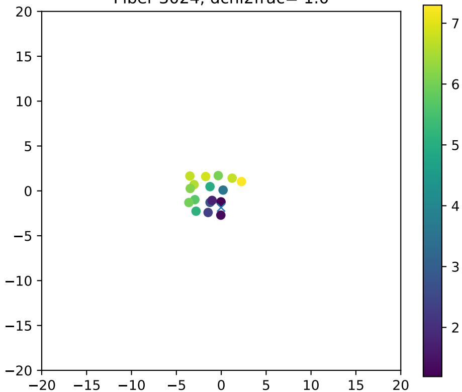
Fiber 3024, dchi2frac= 1.0
