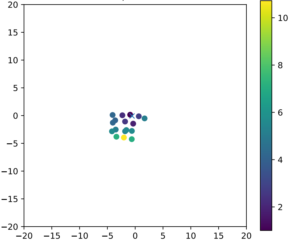
Fiber 3606, dchi2frac= 1.0
