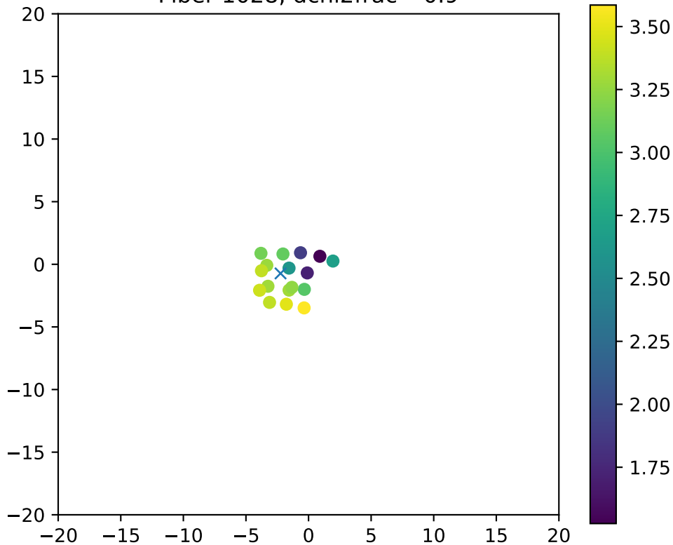
Fiber 1028, dchi2frac= 0.9
