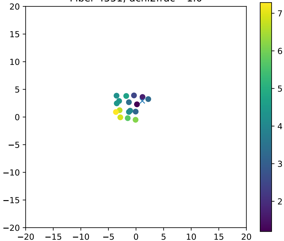
Fiber 4551, dchi2frac= 1.0
