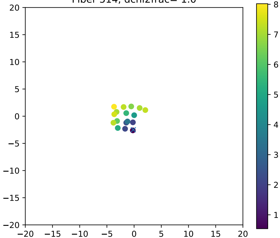
Fiber 514, dchi2frac= 1.0
