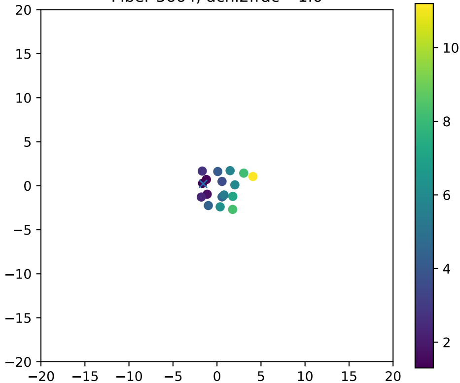
Fiber 3664, dchi2frac= 1.0
