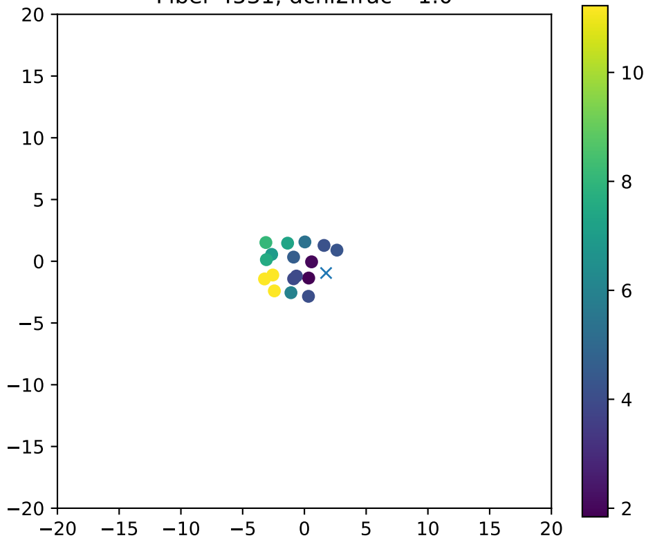
Fiber 4531, dchi2frac= 1.0
