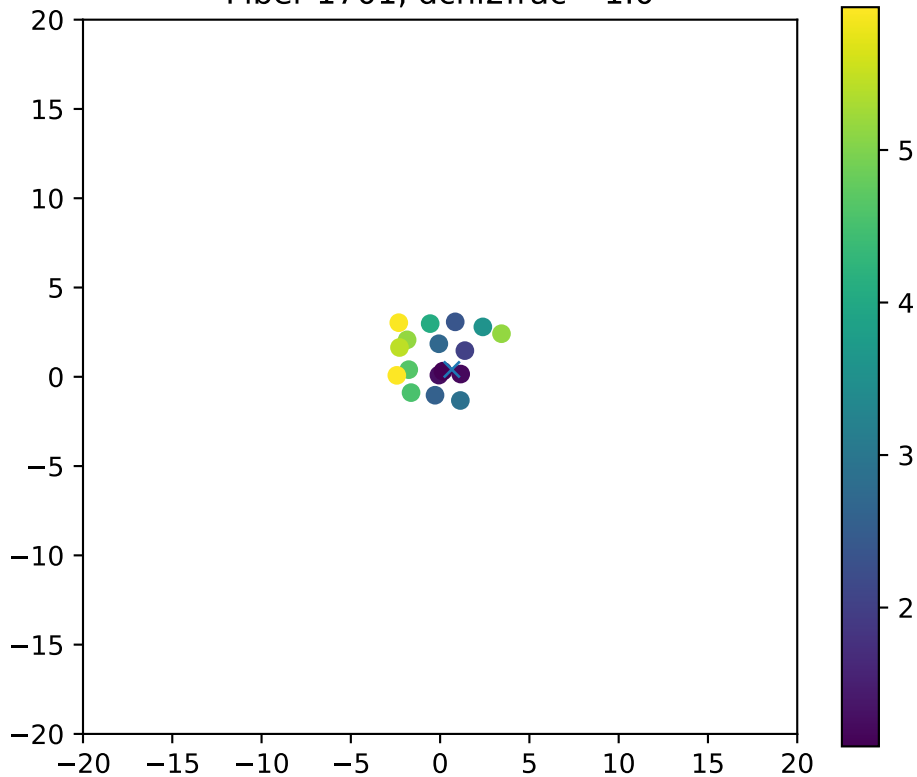
Fiber 1701, dchi2frac= 1.0
