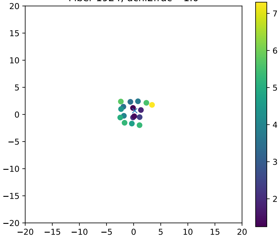
Fiber 1924, dchi2frac= 1.0
