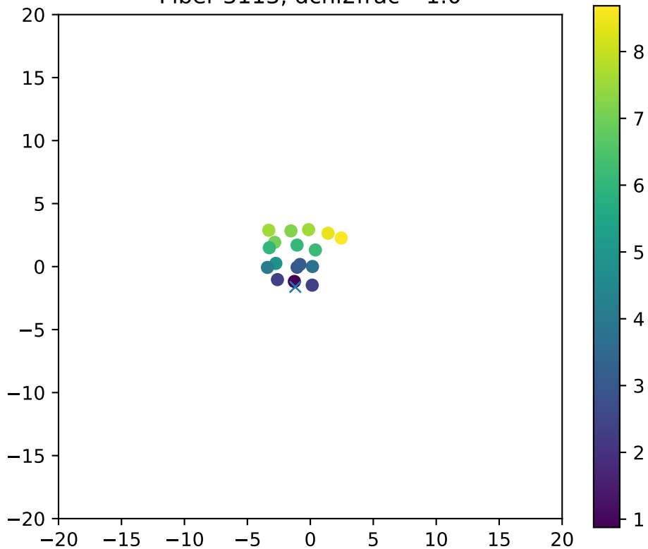
Fiber 3113, dchi2frac= 1.0
