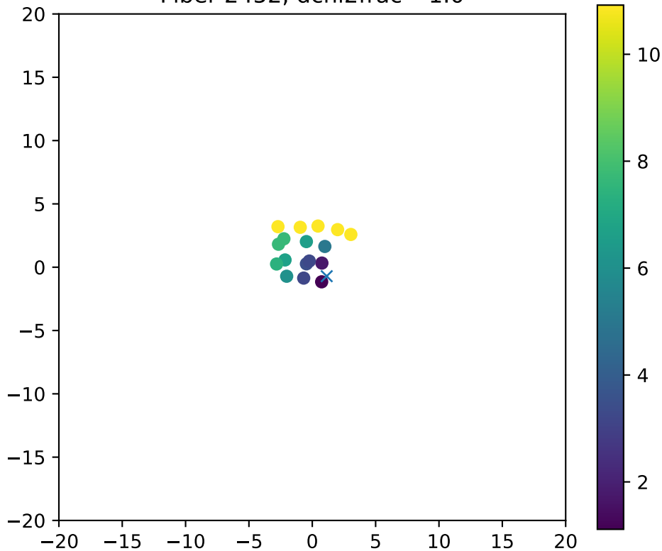
Fiber 2452, dchi2frac= 1.0
