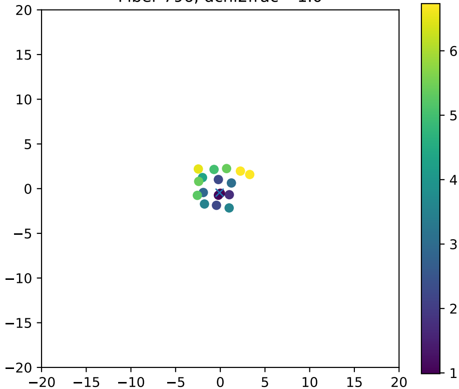
Fiber 796, dchi2frac= 1.0
