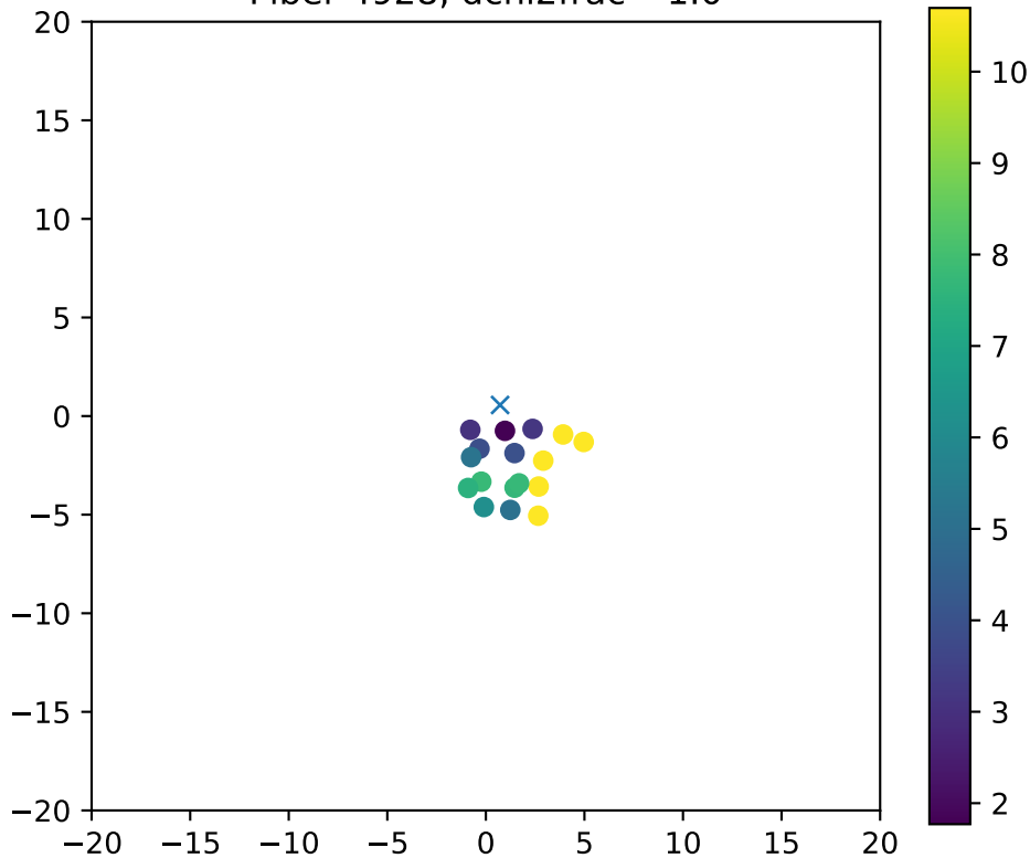
Fiber 4928, dchi2frac= 1.0
