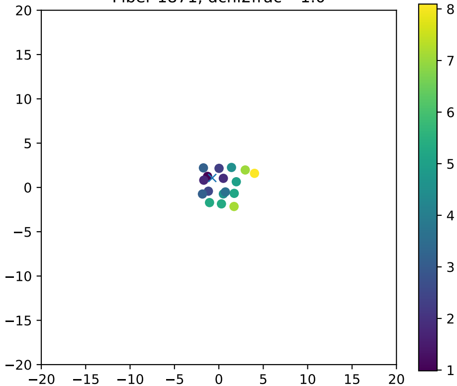
Fiber 1871, dchi2frac= 1.0
