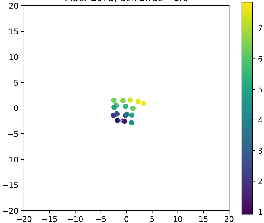
Fiber 2973, dchi2frac= 1.0
