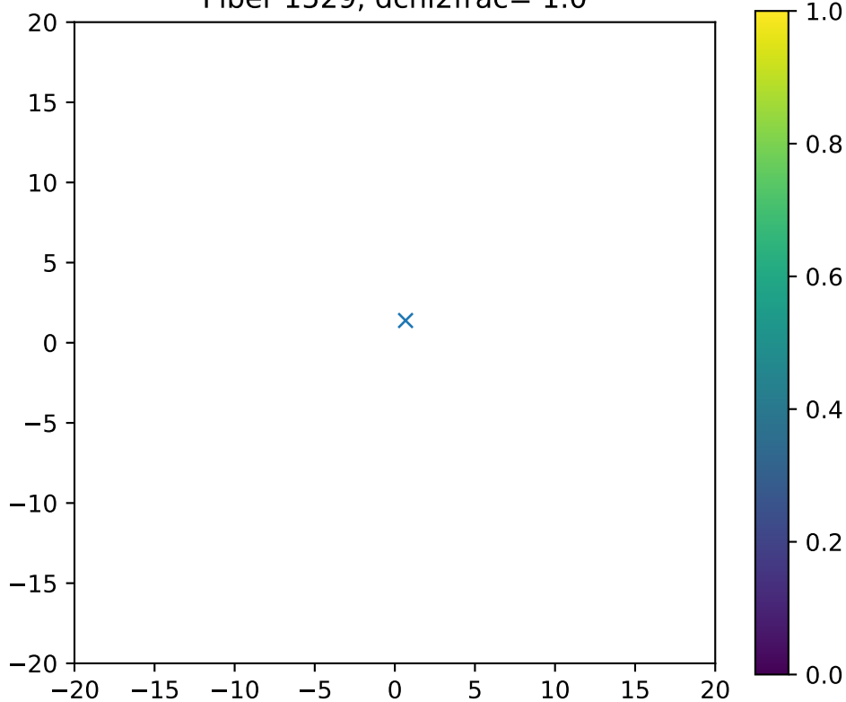
Fiber 1529, dchi2frac= 1.0
