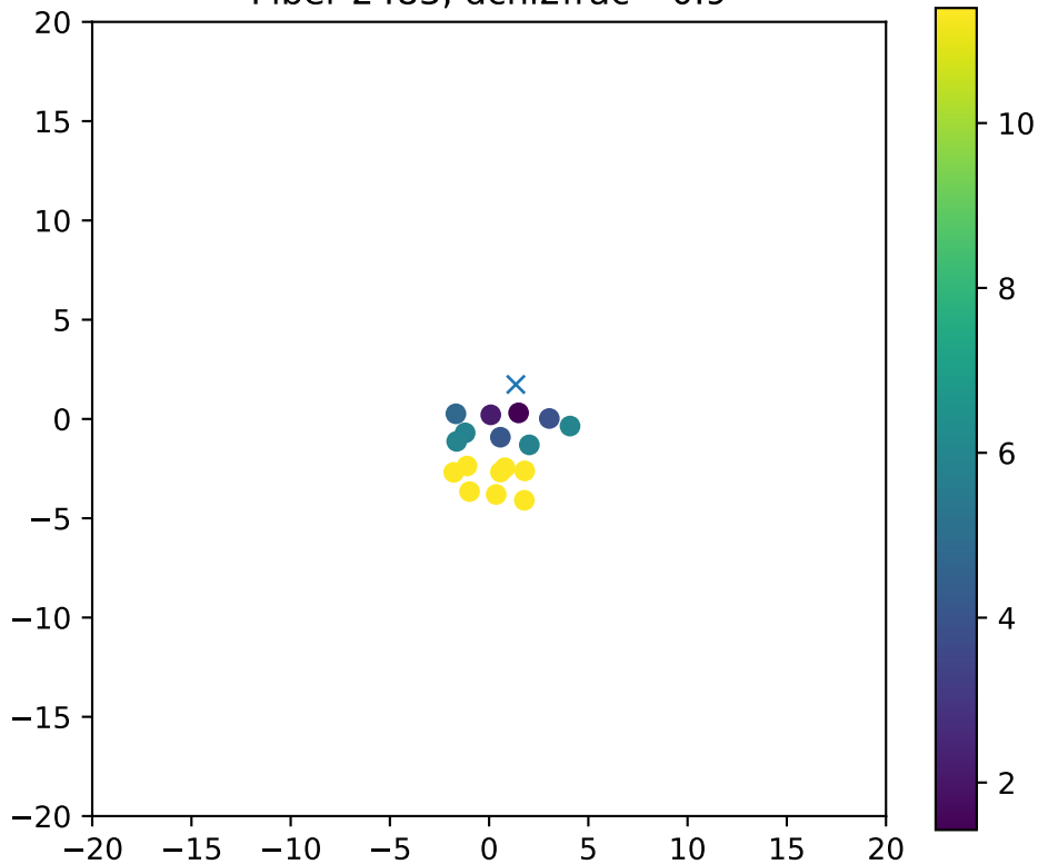
Fiber 2483, dchi2frac= 0.9
