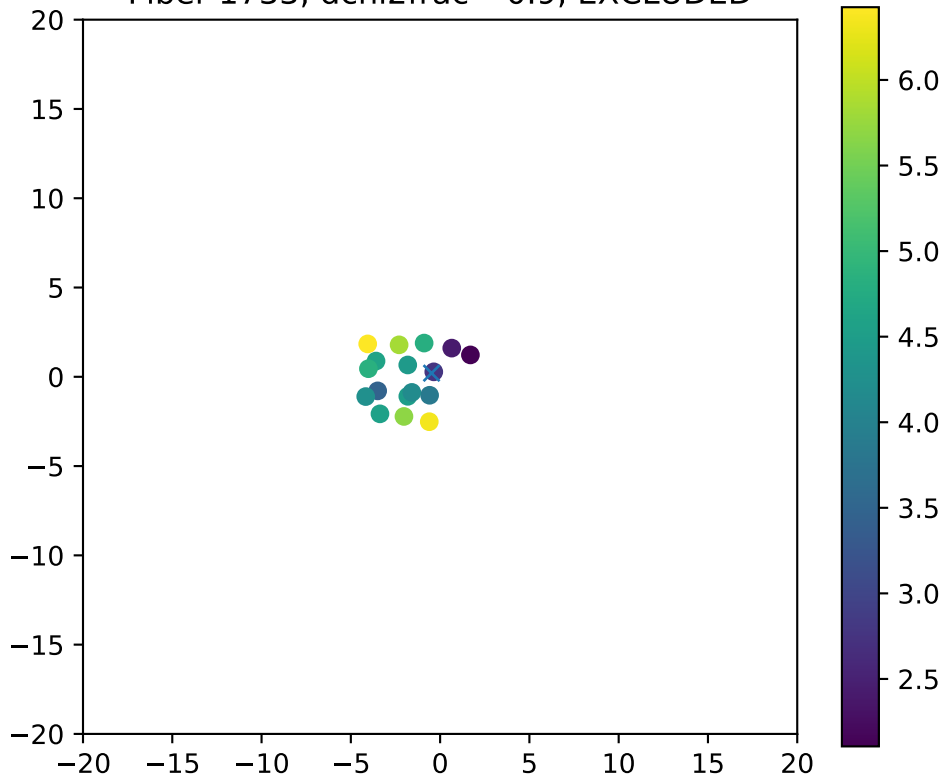
Fiber 1733, dchi2frac= 0.9, EXCLUDED
