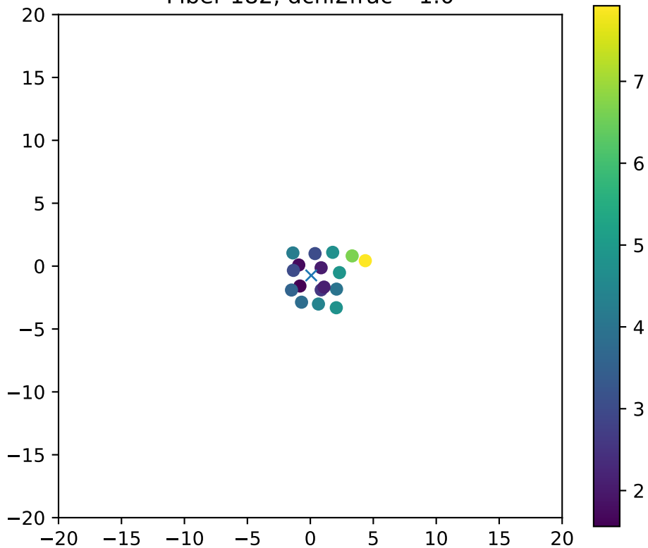
Fiber 182, dchi2frac= 1.0
