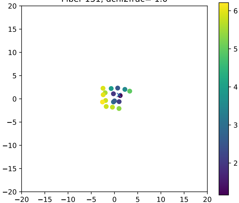
Fiber 131, dchi2frac= 1.0
