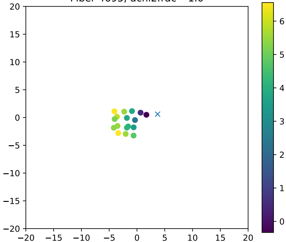
Fiber 4695, dchi2frac= 1.0
