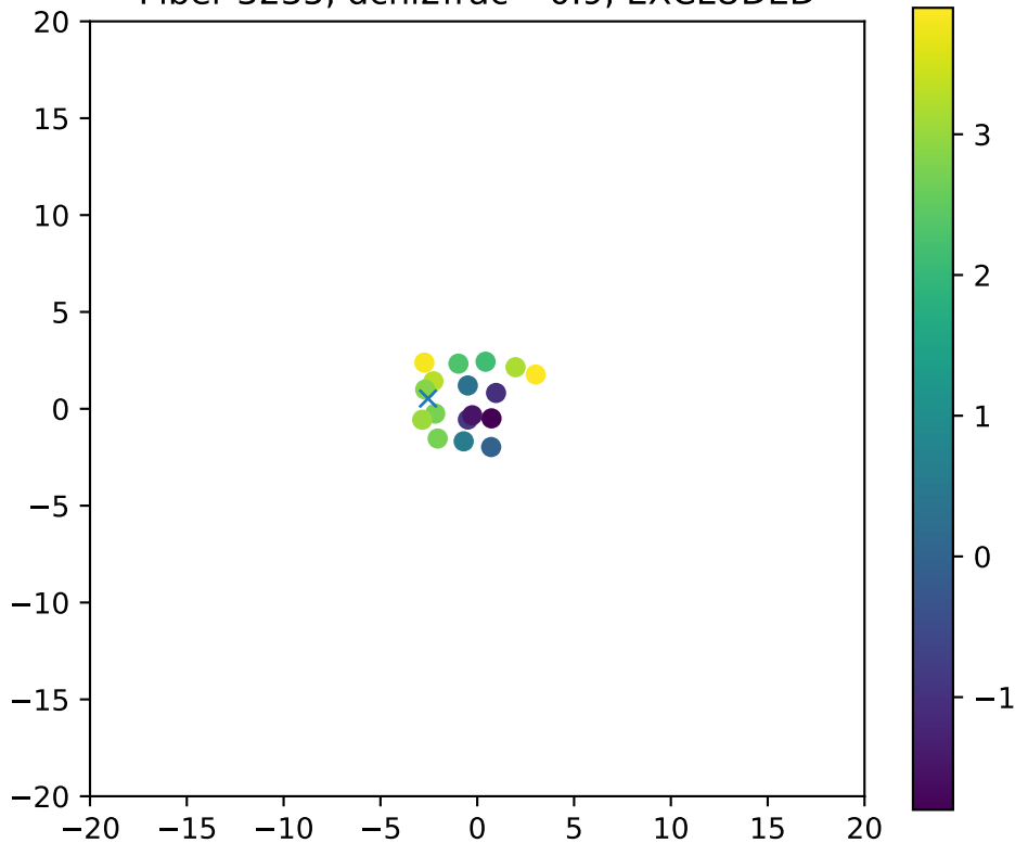
Fiber 3235, dchi2frac= 0.9, EXCLUDED
