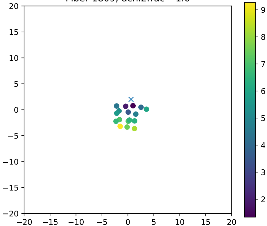
Fiber 1809, dchi2frac= 1.0
