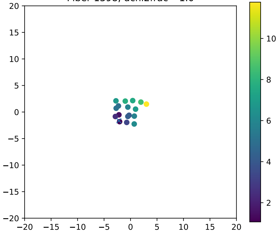
Fiber 1398, dchi2frac= 1.0
