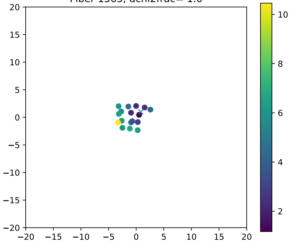
Fiber 1563, dchi2frac= 1.0
