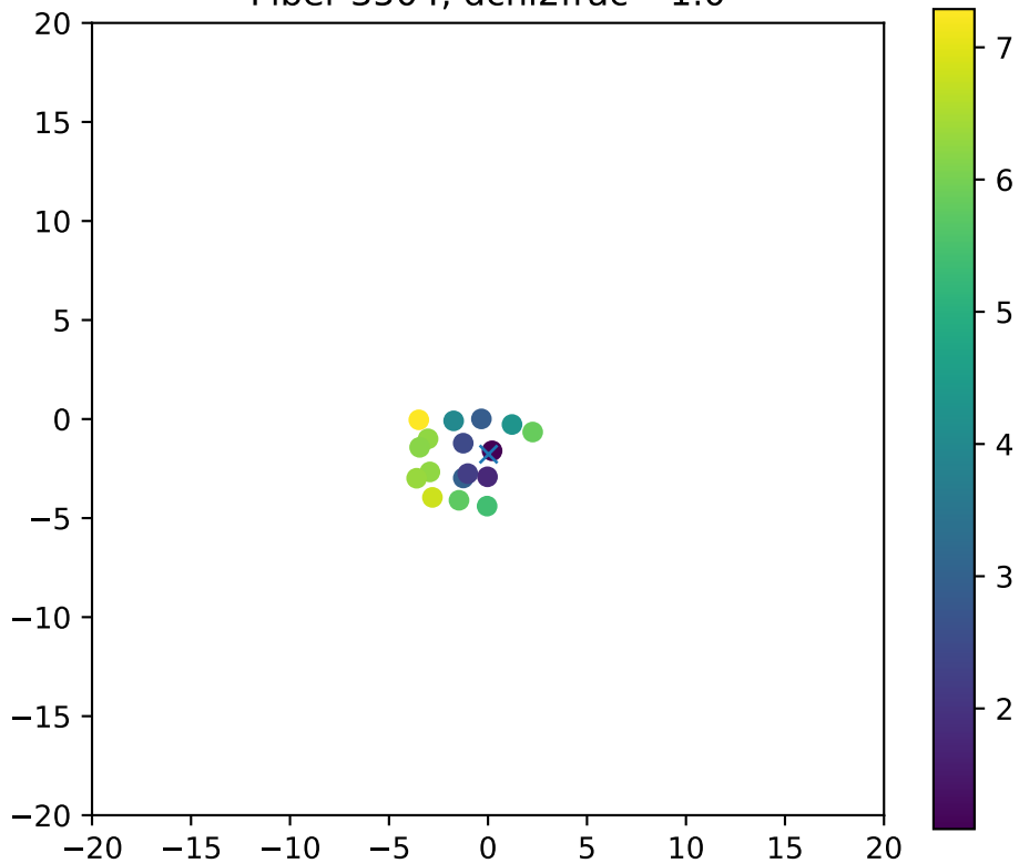
Fiber 3504, dchi2frac= 1.0
