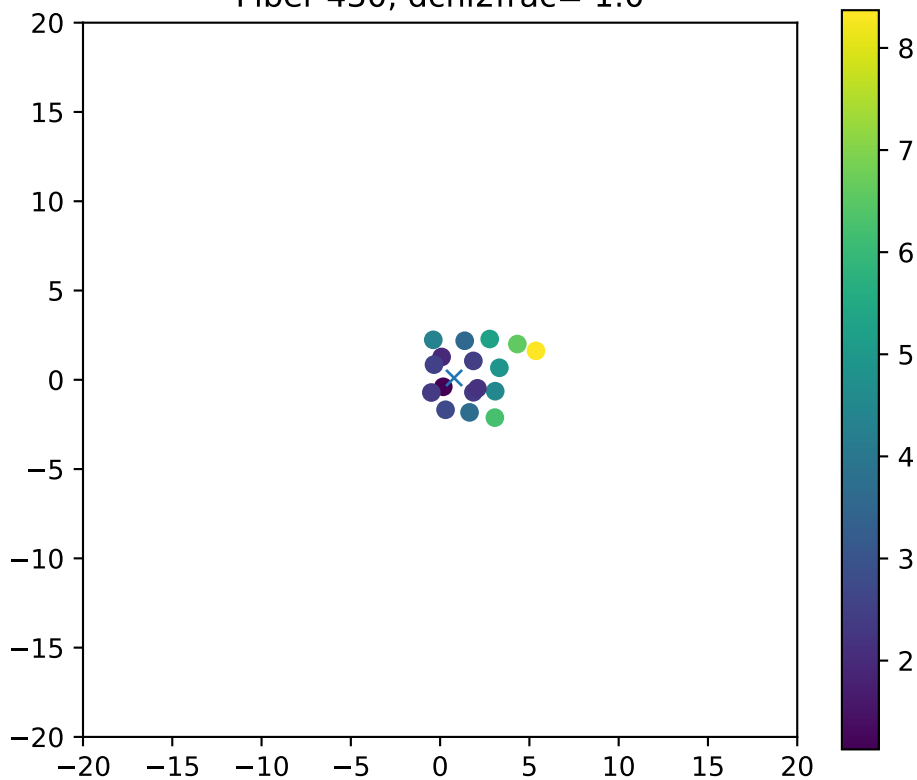
Fiber 430, dchi2frac= 1.0
