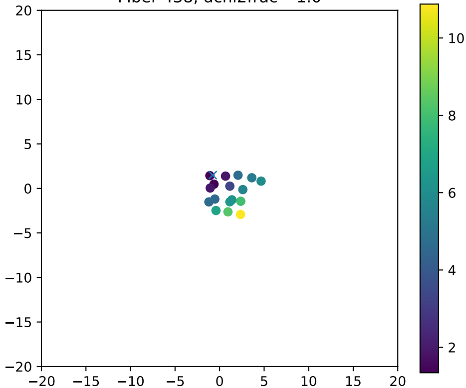
Fiber 438, dchi2frac= 1.0
