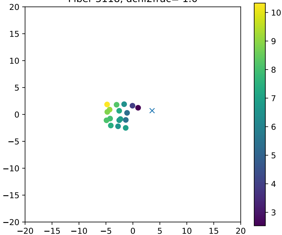
Fiber 3118, dchi2frac= 1.0
