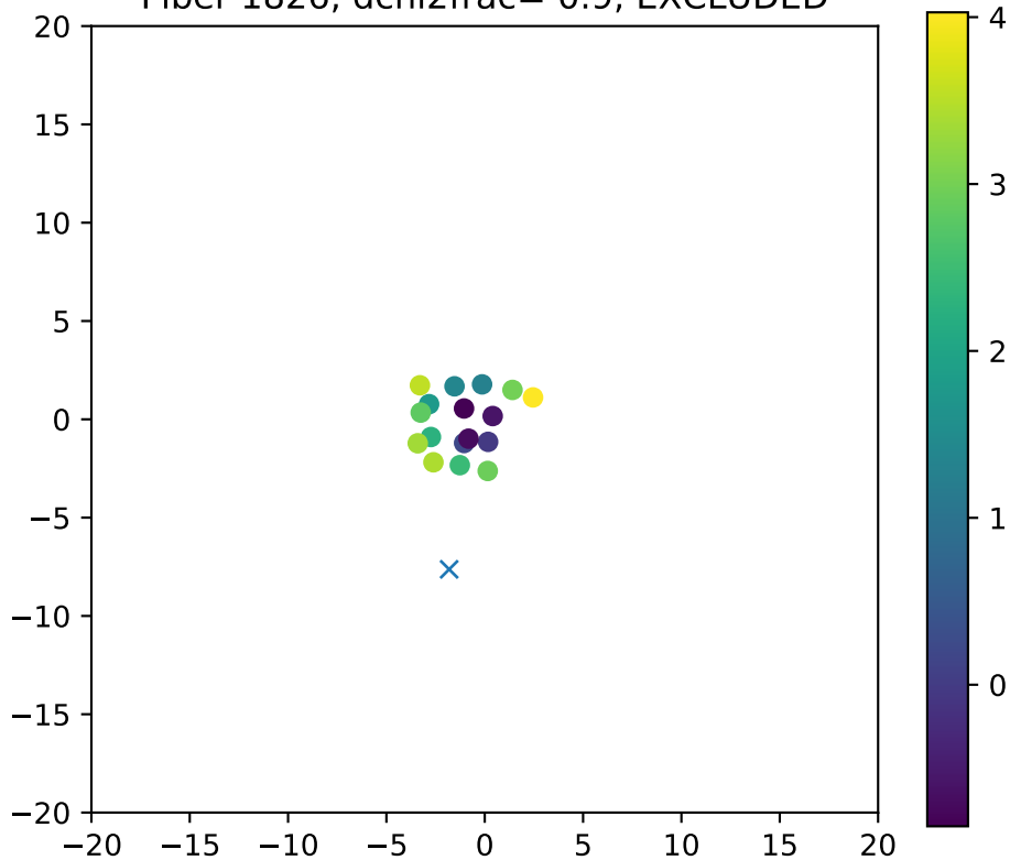
Fiber 1826, dchi2frac= 0.9, EXCLUDED
