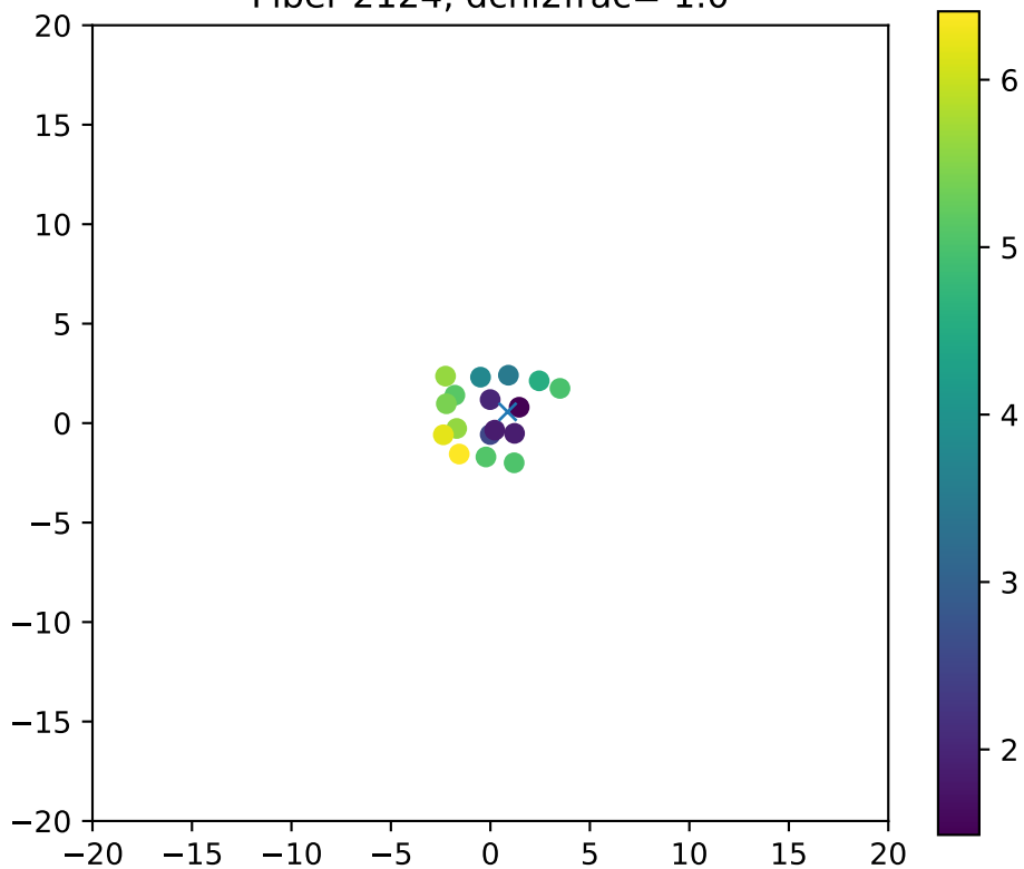
Fiber 2124, dchi2frac= 1.0
