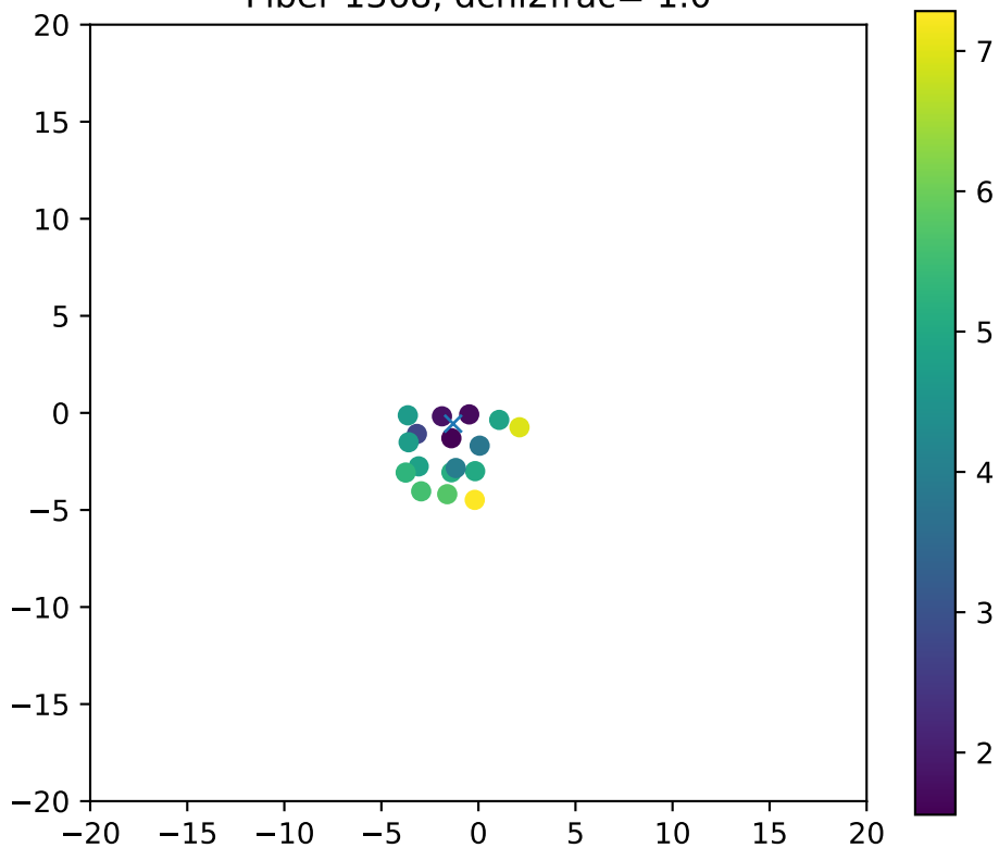
Fiber 1368, dchi2frac= 1.0
