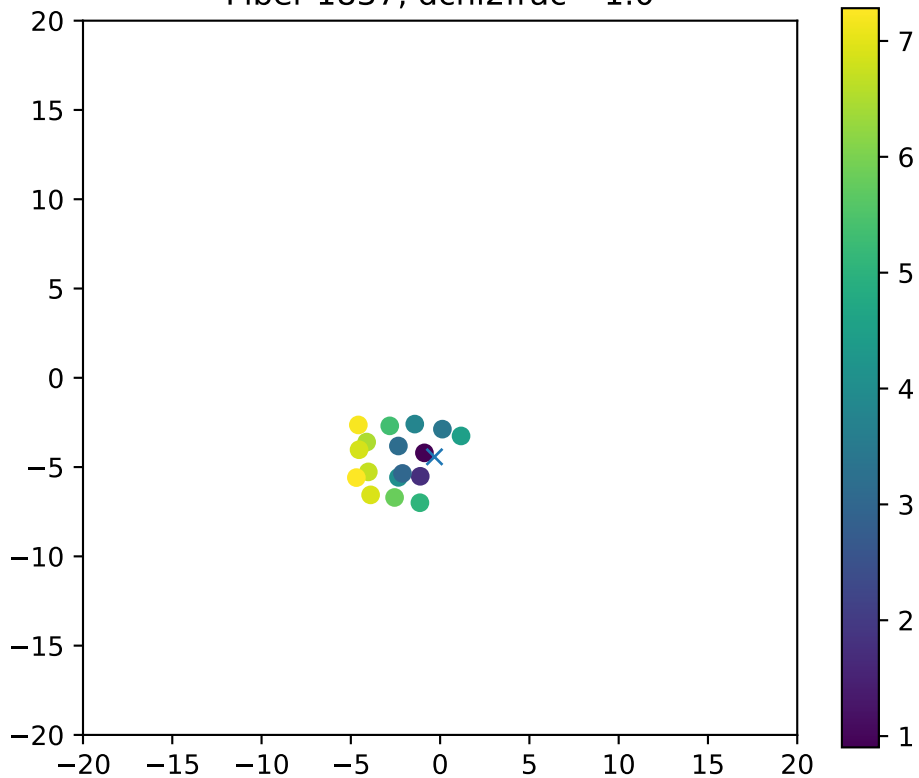
Fiber 1837, dchi2frac= 1.0
