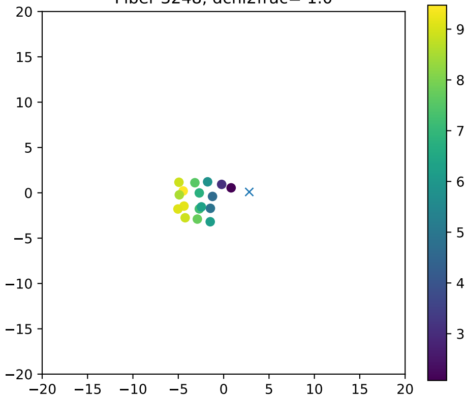
Fiber 3248, dchi2frac= 1.0
