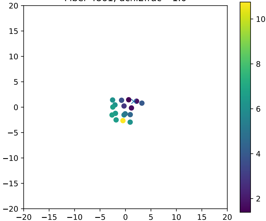
Fiber 4861, dchi2frac= 1.0
