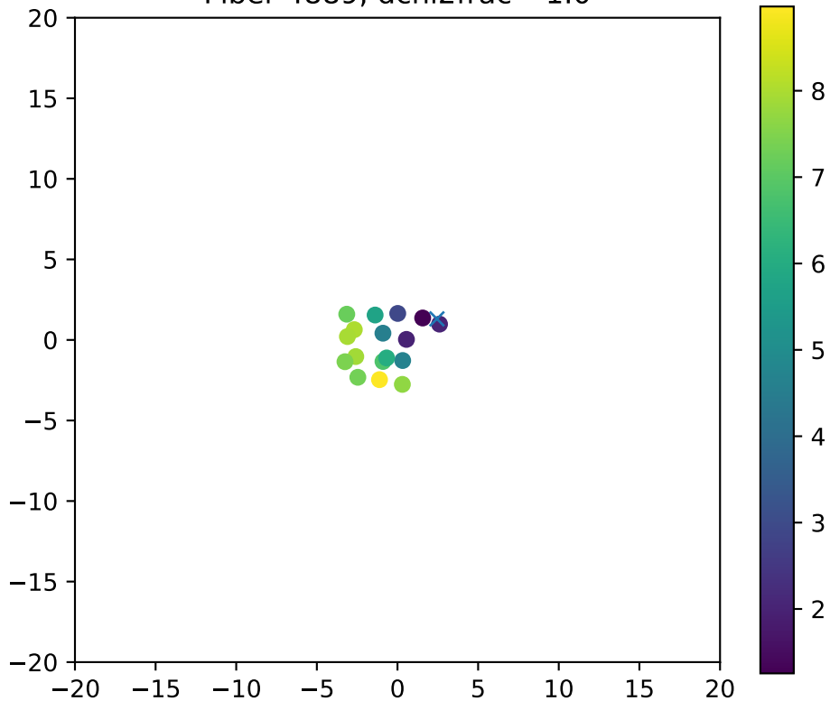
Fiber 4889, dchi2frac= 1.0
