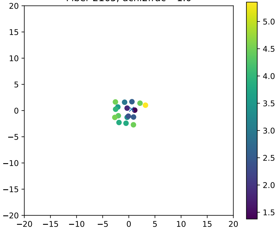
Fiber 2165, dchi2frac= 1.0
