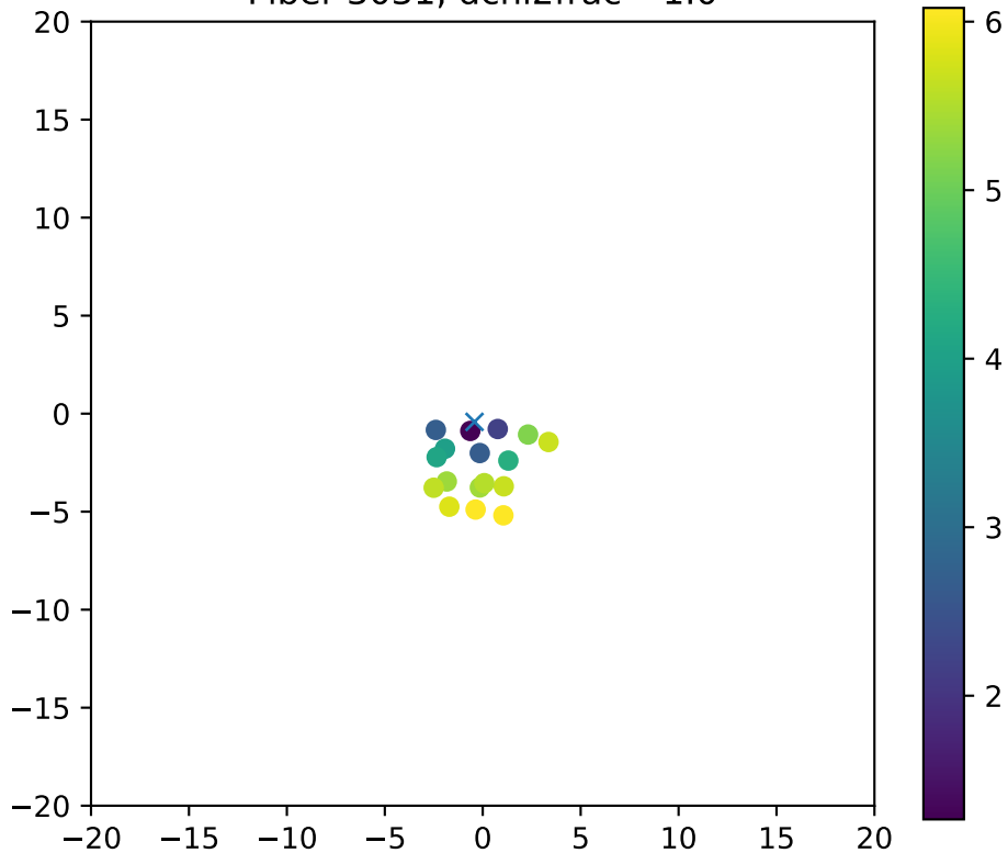
Fiber 3031, dchi2frac= 1.0
