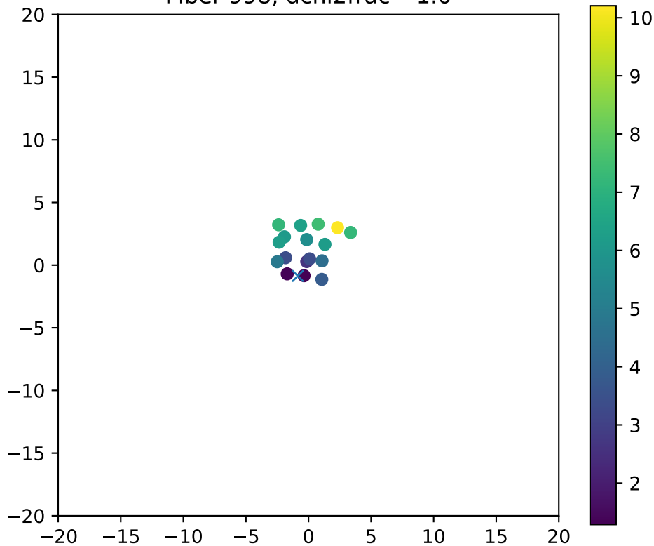
Fiber 998, dchi2frac= 1.0
