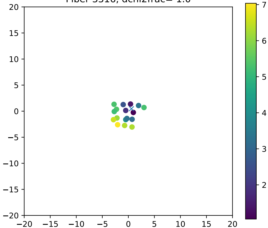
Fiber 3316, dchi2frac= 1.0
