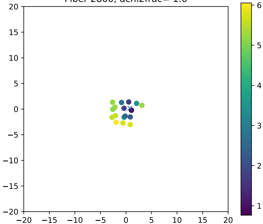
Fiber 2800, dchi2frac= 1.0
