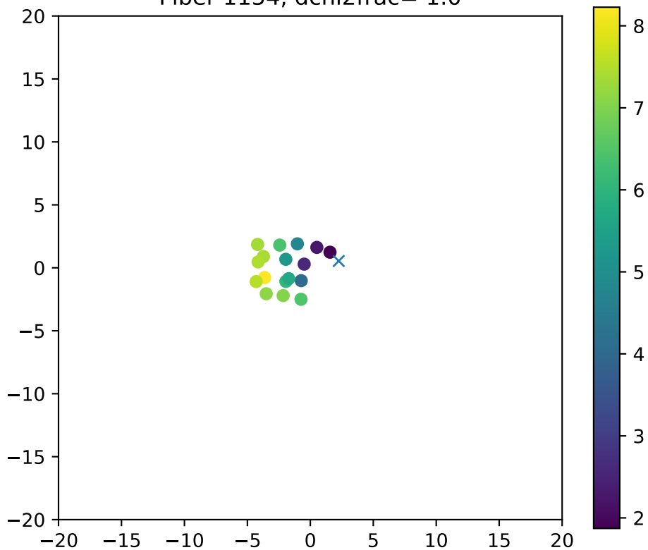
Fiber 1154, dchi2frac= 1.0
