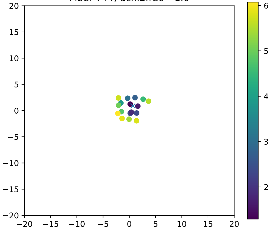
Fiber 744, dchi2frac= 1.0
