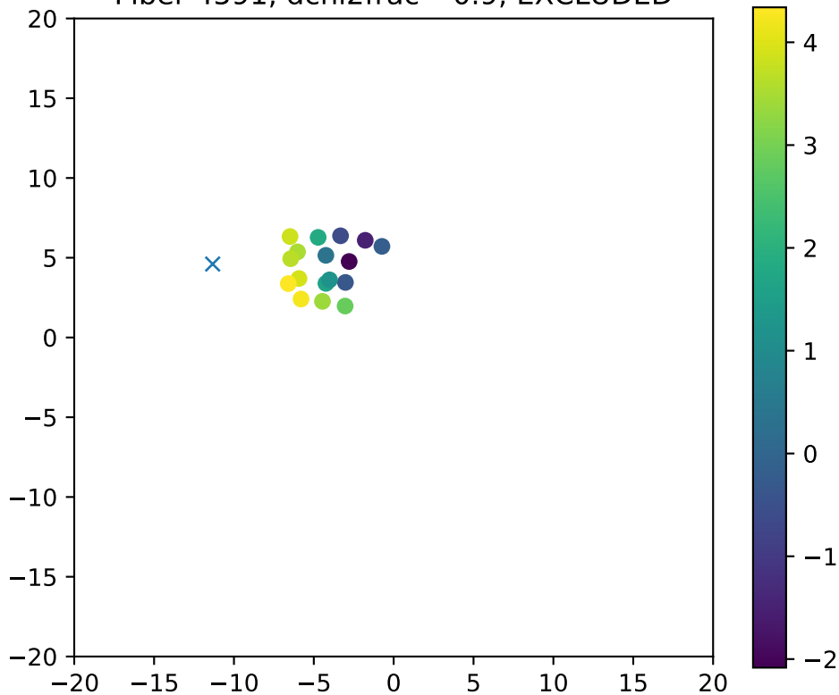
Fiber 4591, dchi2frac= 0.9, EXCLUDED
