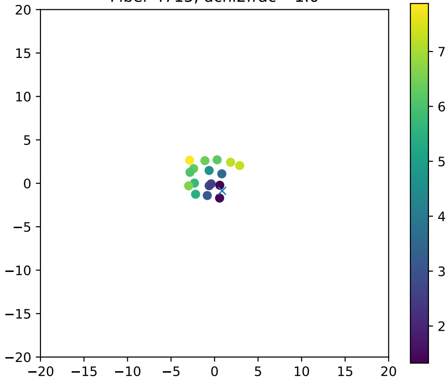
Fiber 4715, dchi2frac= 1.0
