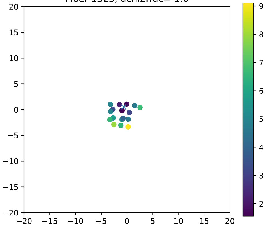
Fiber 1325, dchi2frac= 1.0
