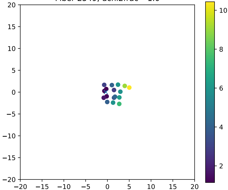
Fiber 2549, dchi2frac= 1.0
