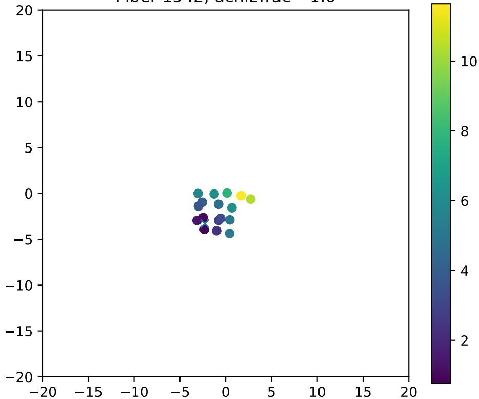
Fiber 1542, dchi2frac= 1.0
