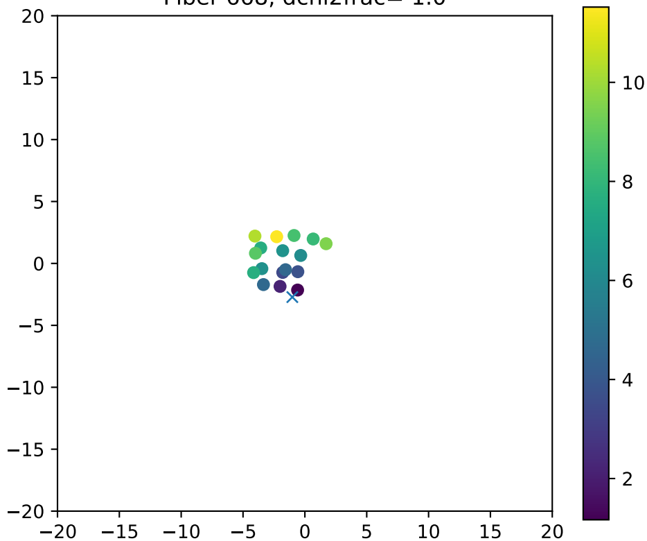
Fiber 668, dchi2frac= 1.0
