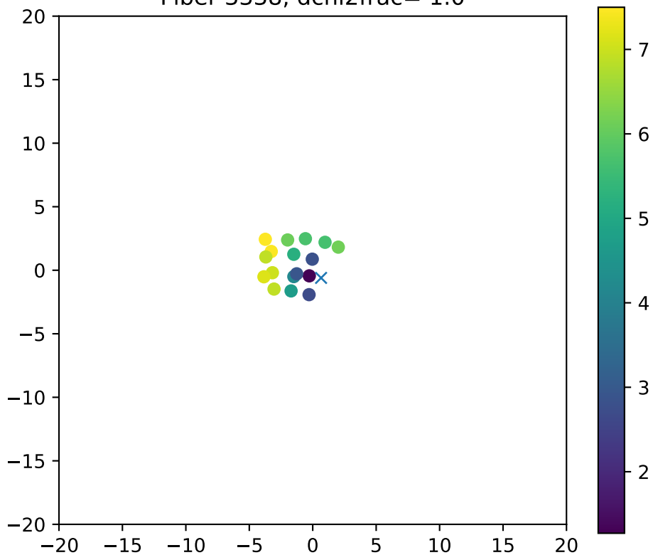
Fiber 3338, dchi2frac= 1.0
