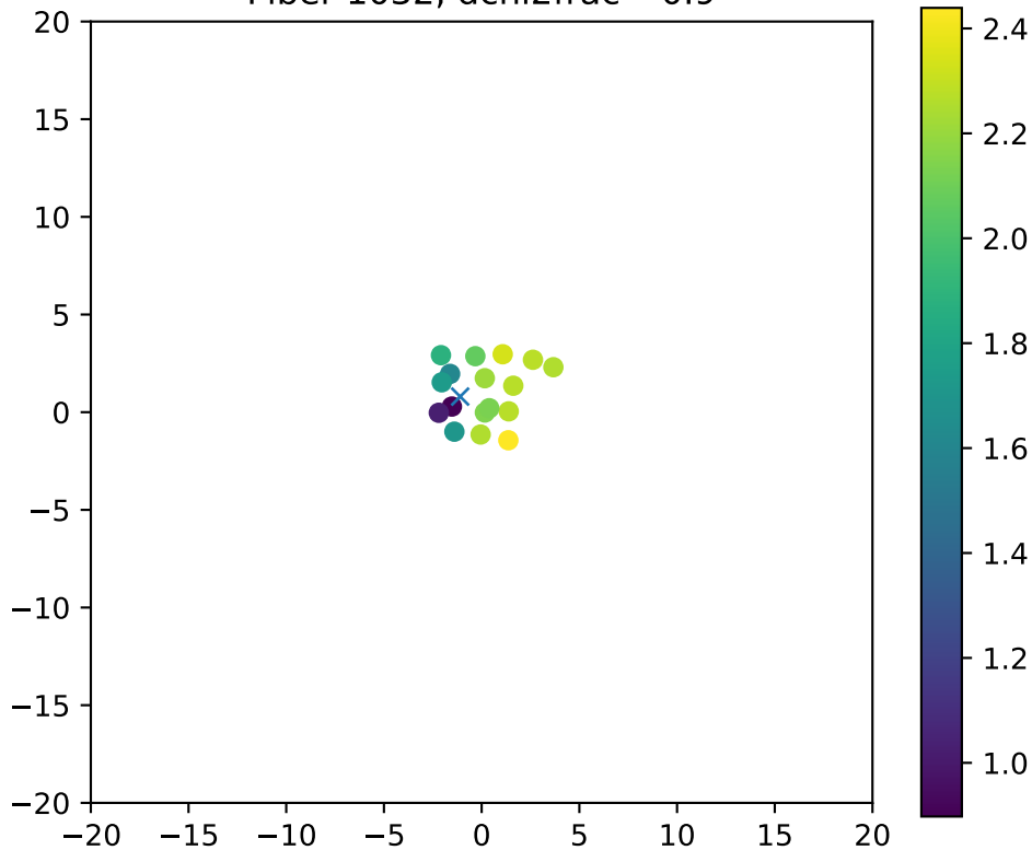
Fiber 1032, dchi2frac= 0.9
