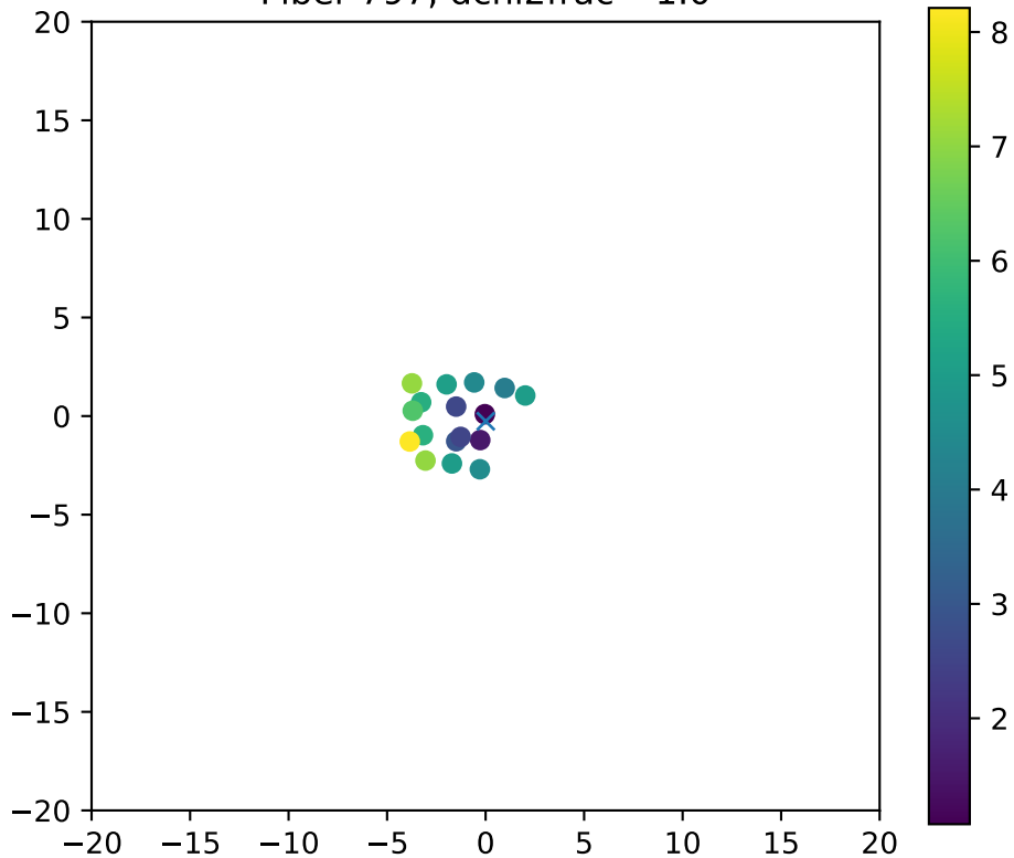
Fiber 797, dchi2frac= 1.0
