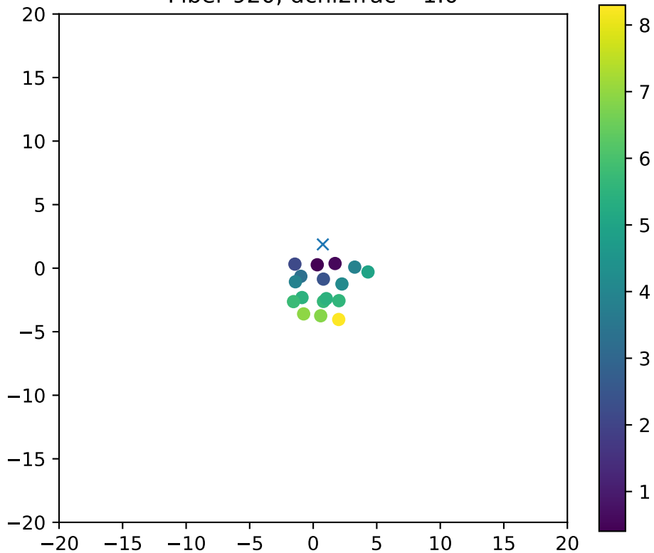
Fiber 920, dchi2frac= 1.0
