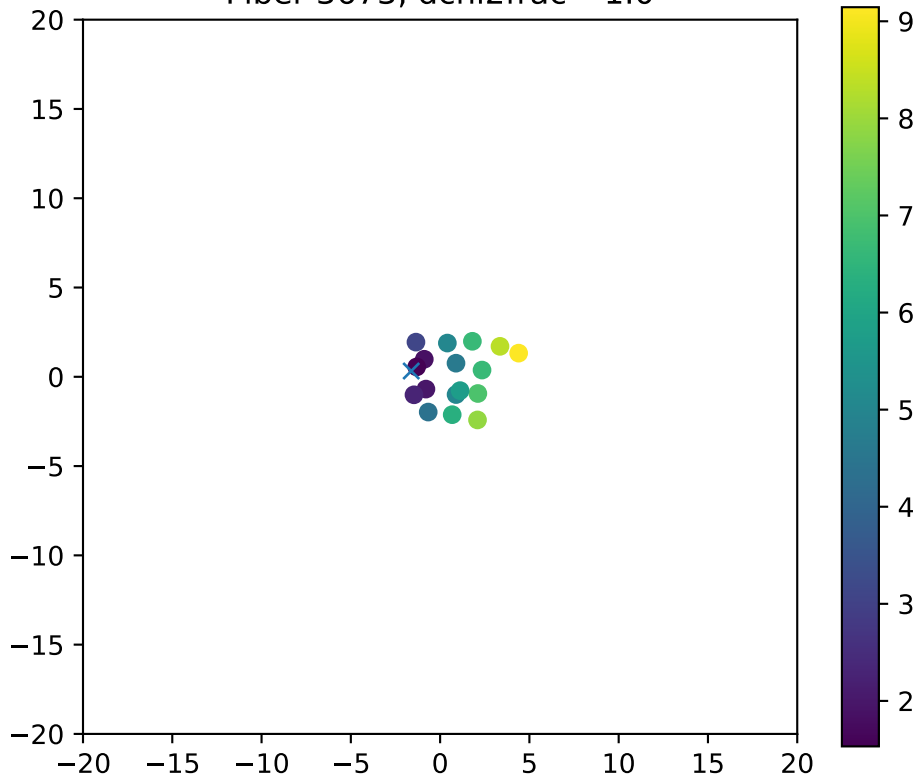
Fiber 3673, dchi2frac= 1.0
