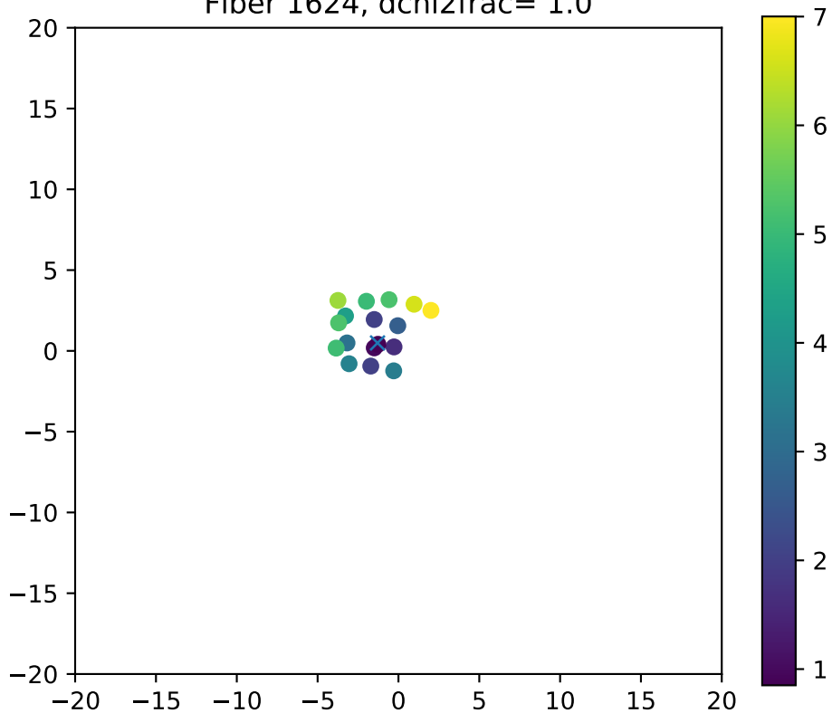
Fiber 1624, dchi2frac= 1.0
