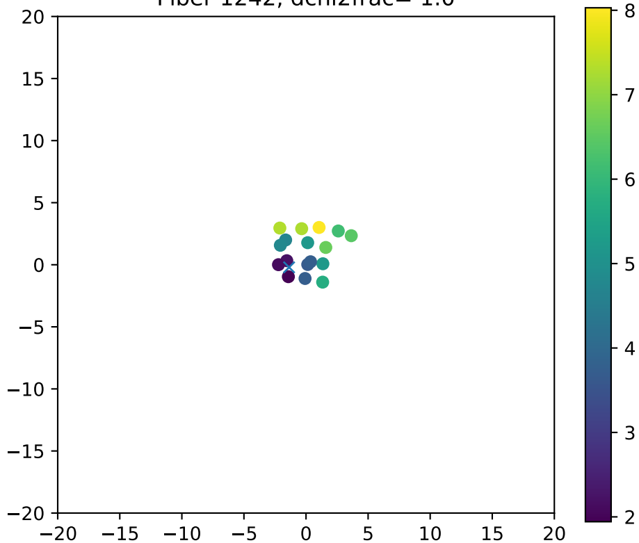
Fiber 1242, dchi2frac= 1.0
