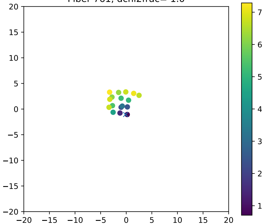
Fiber 761, dchi2frac= 1.0
