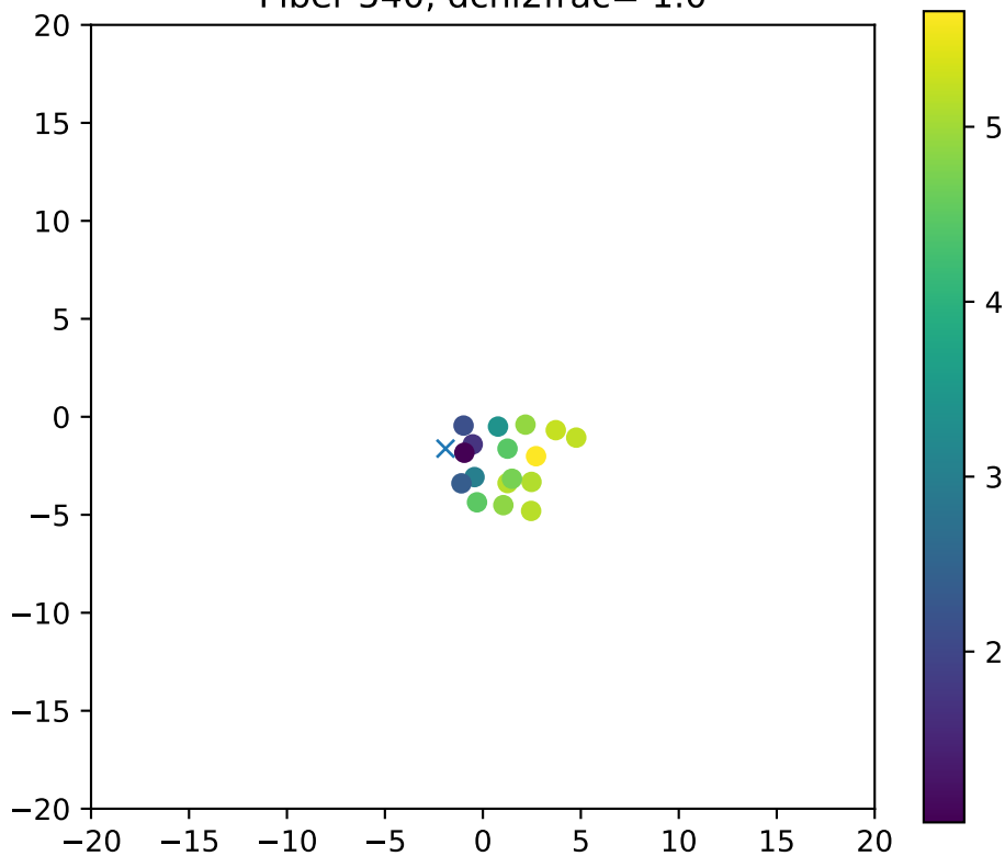
Fiber 540, dchi2frac= 1.0
