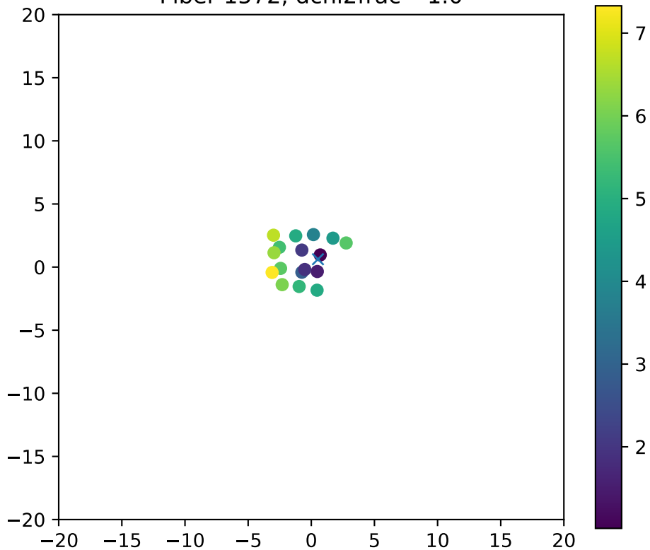
Fiber 1572, dchi2frac= 1.0
