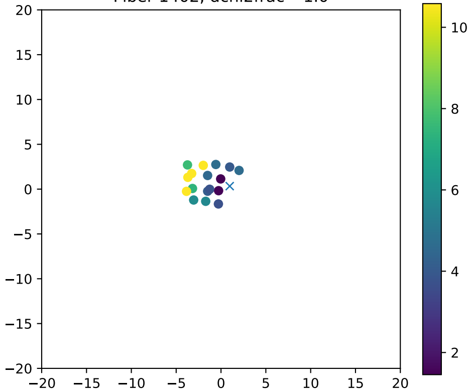
Fiber 1402, dchi2frac= 1.0
