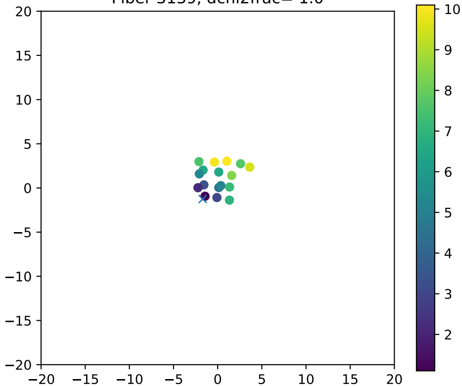
Fiber 3139, dchi2frac= 1.0
