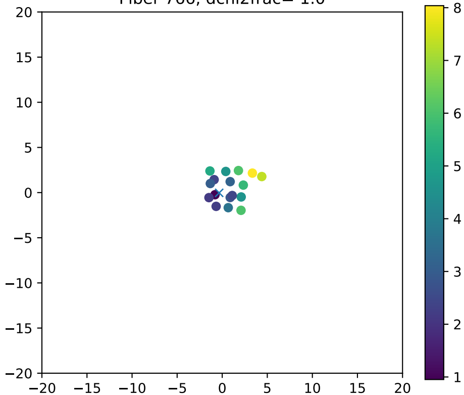
Fiber 766, dchi2frac= 1.0
