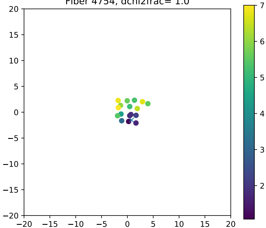
Fiber 4754, dchi2frac= 1.0
