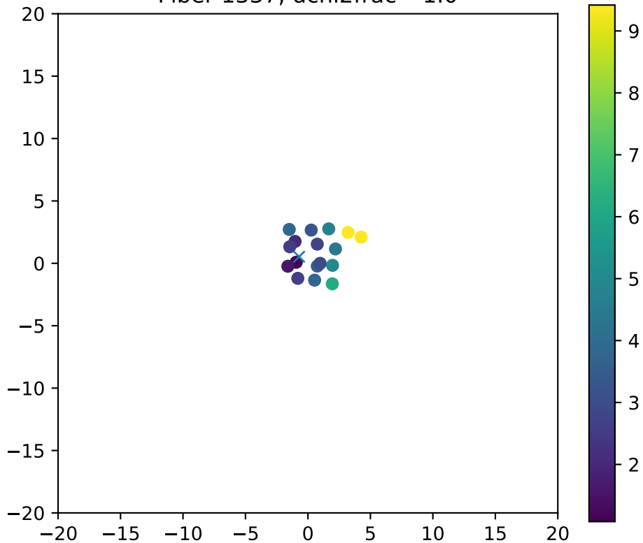
Fiber 1337, dchi2frac= 1.0
