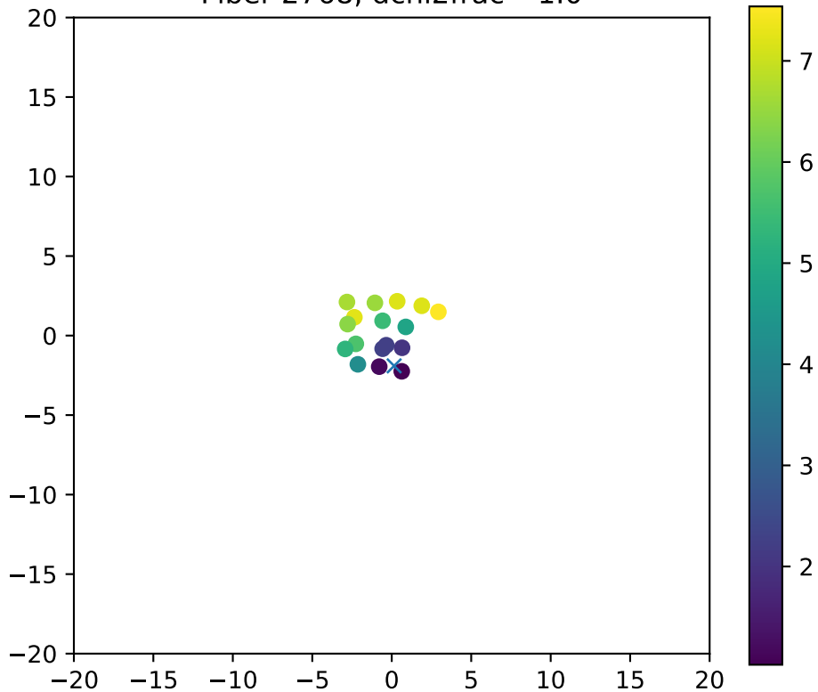
Fiber 2768, dchi2frac= 1.0
