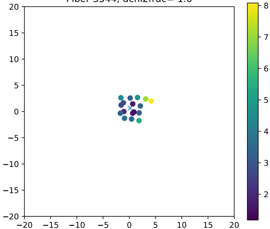
Fiber 3544, dchi2frac= 1.0
