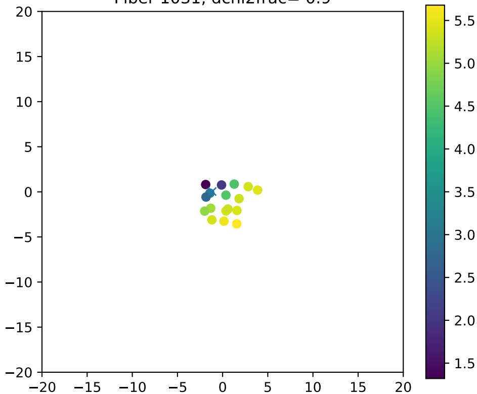
Fiber 1031, dchi2frac= 0.9
