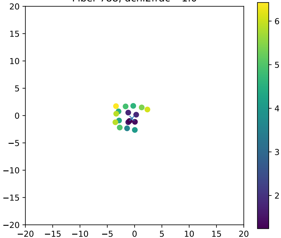
Fiber 788, dchi2frac= 1.0
