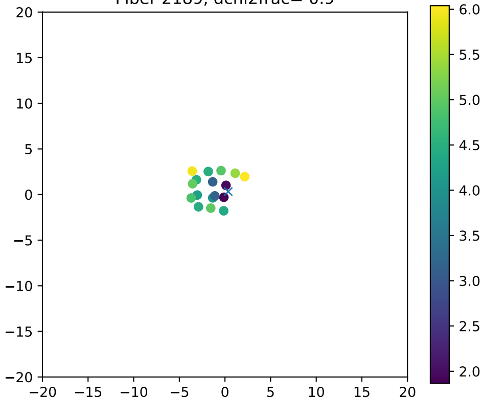
Fiber 2189, dchi2frac= 0.9
