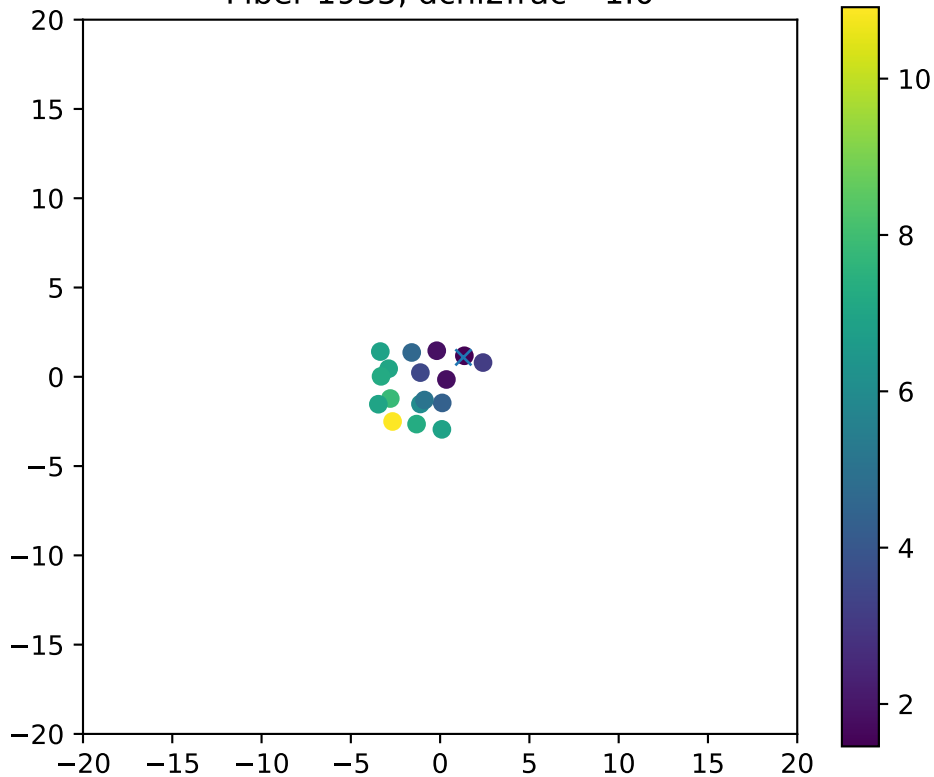
Fiber 1935, dchi2frac= 1.0
