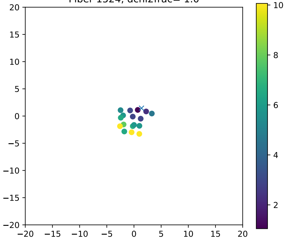
Fiber 1524, dchi2frac= 1.0
