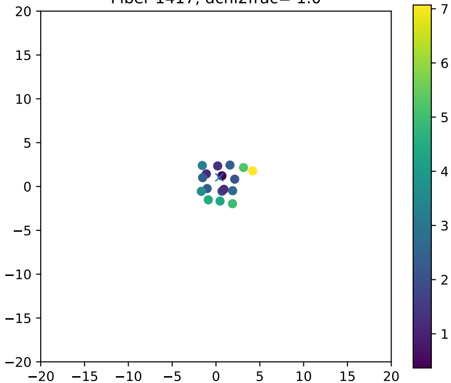
Fiber 1417, dchi2frac= 1.0
