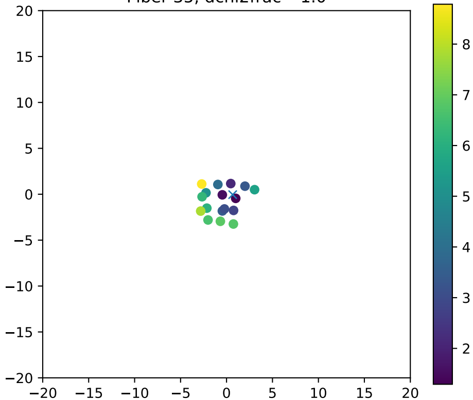
Fiber 35, dchi2frac= 1.0
