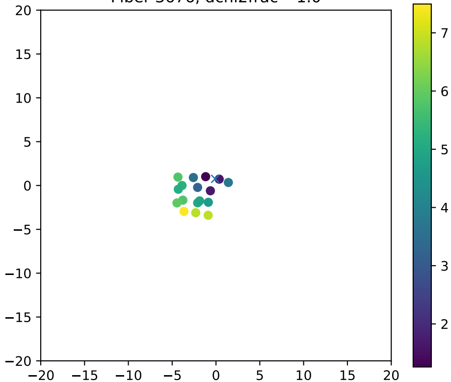
Fiber 3676, dchi2frac= 1.0
