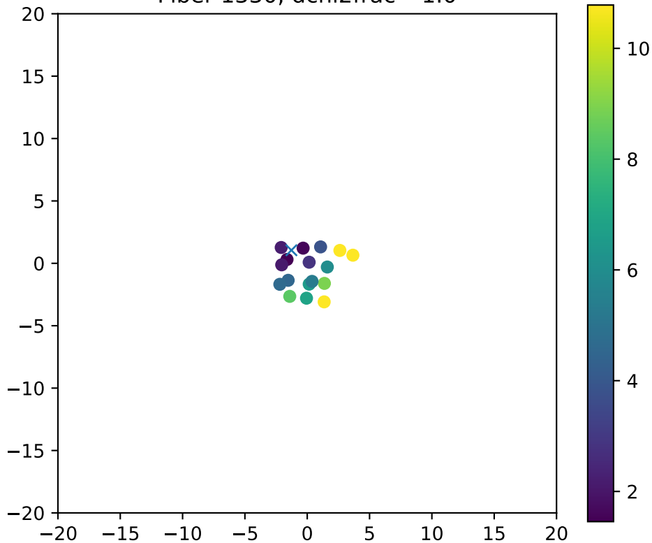
Fiber 1330, dchi2frac= 1.0
