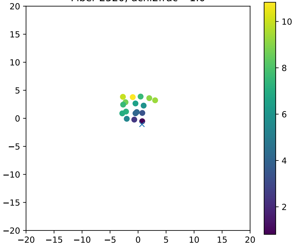
Fiber 2520, dchi2frac= 1.0
