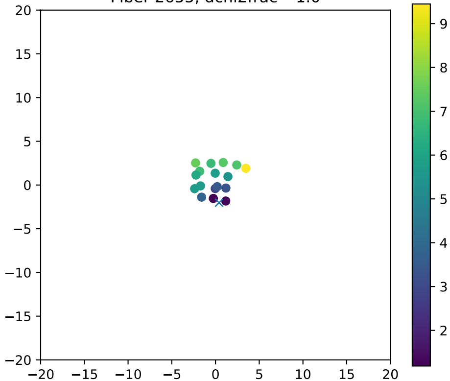
Fiber 2655, dchi2frac= 1.0
