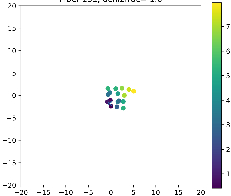
Fiber 151, dchi2frac= 1.0
