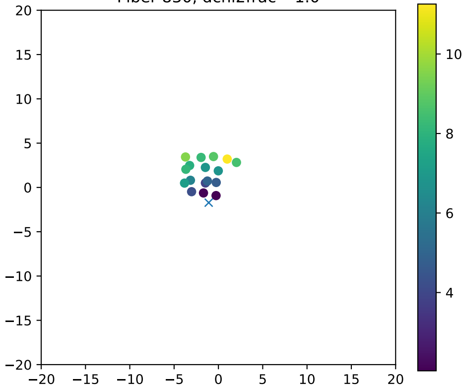
Fiber 830, dchi2frac= 1.0
