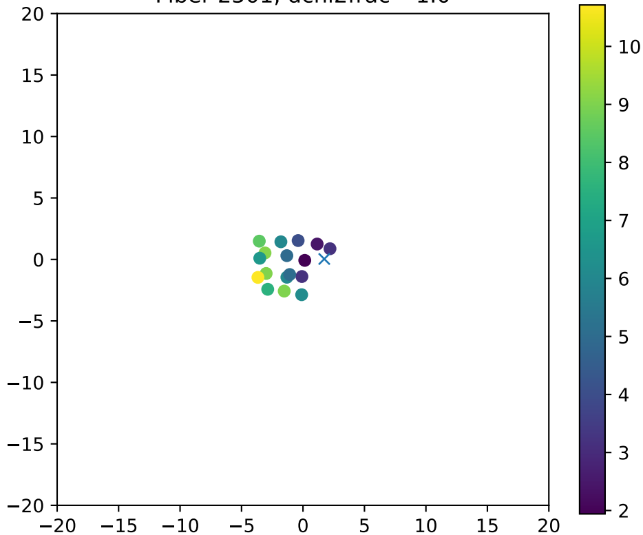
Fiber 2501, dchi2frac= 1.0
