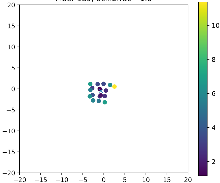
Fiber 989, dchi2frac= 1.0
