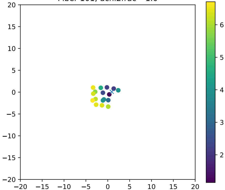
Fiber 101, dchi2frac= 1.0
