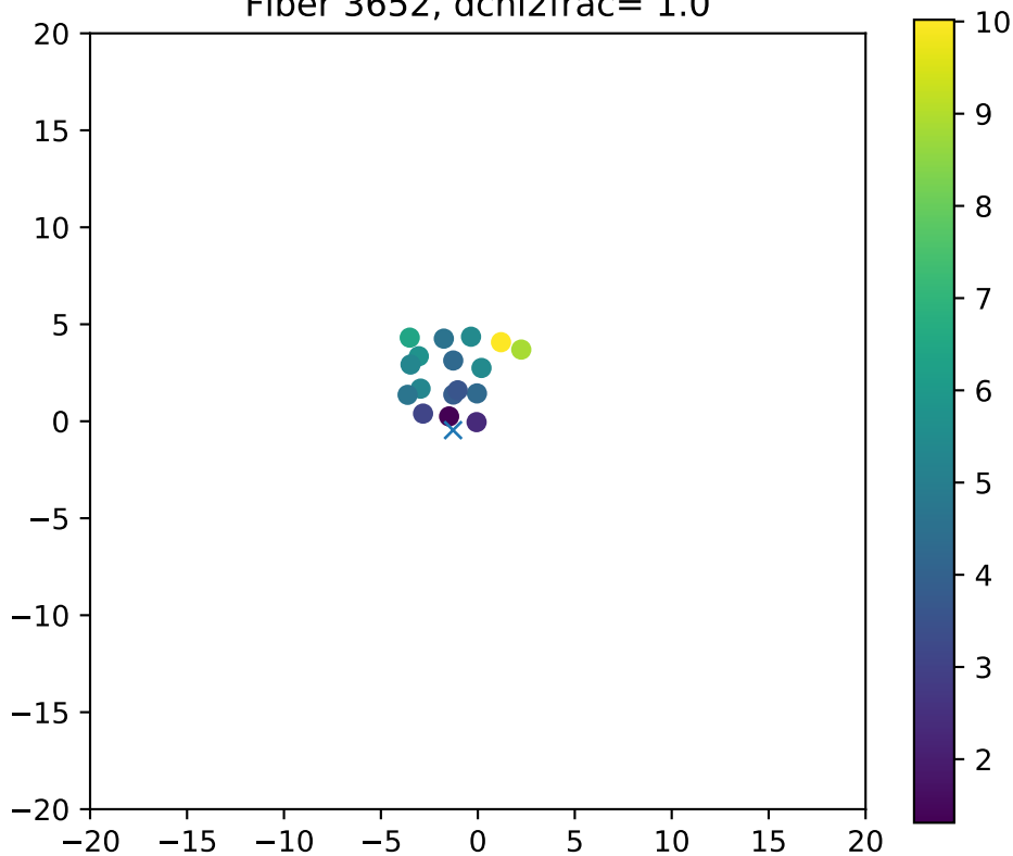
Fiber 3652, dchi2frac= 1.0
