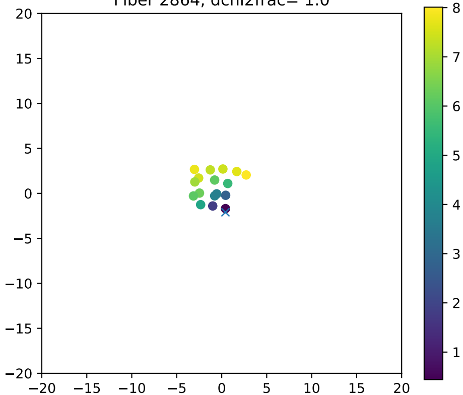
Fiber 2864, dchi2frac= 1.0
