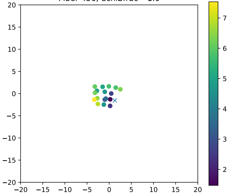
Fiber 456, dchi2frac= 1.0
