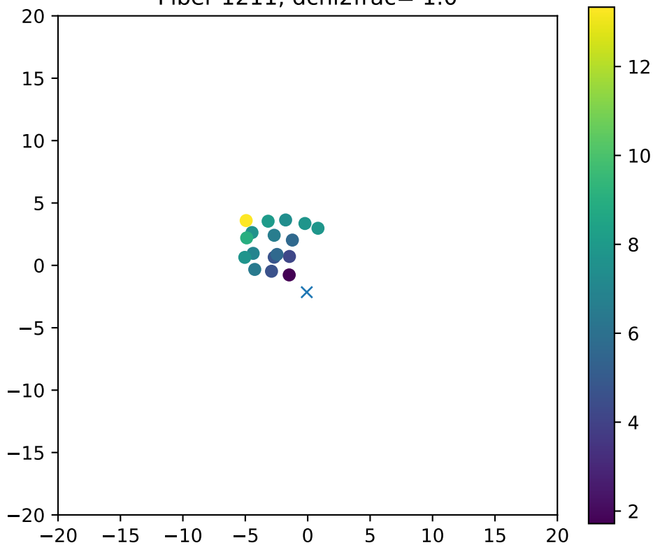
Fiber 1211, dchi2frac= 1.0
