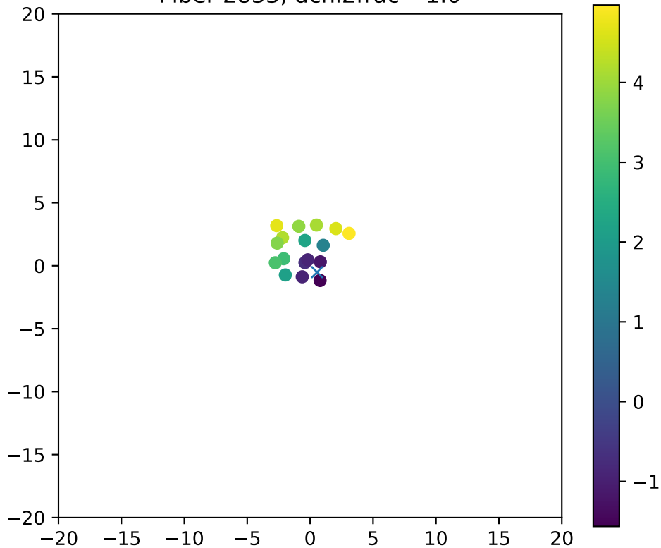
Fiber 2833, dchi2frac= 1.0
