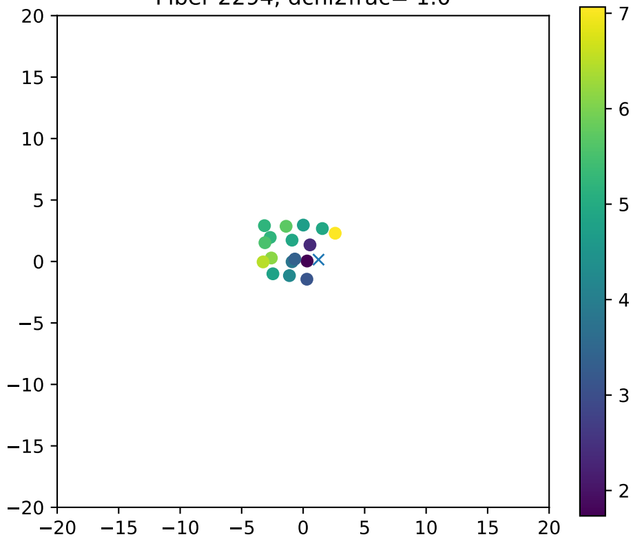
Fiber 2294, dchi2frac= 1.0
