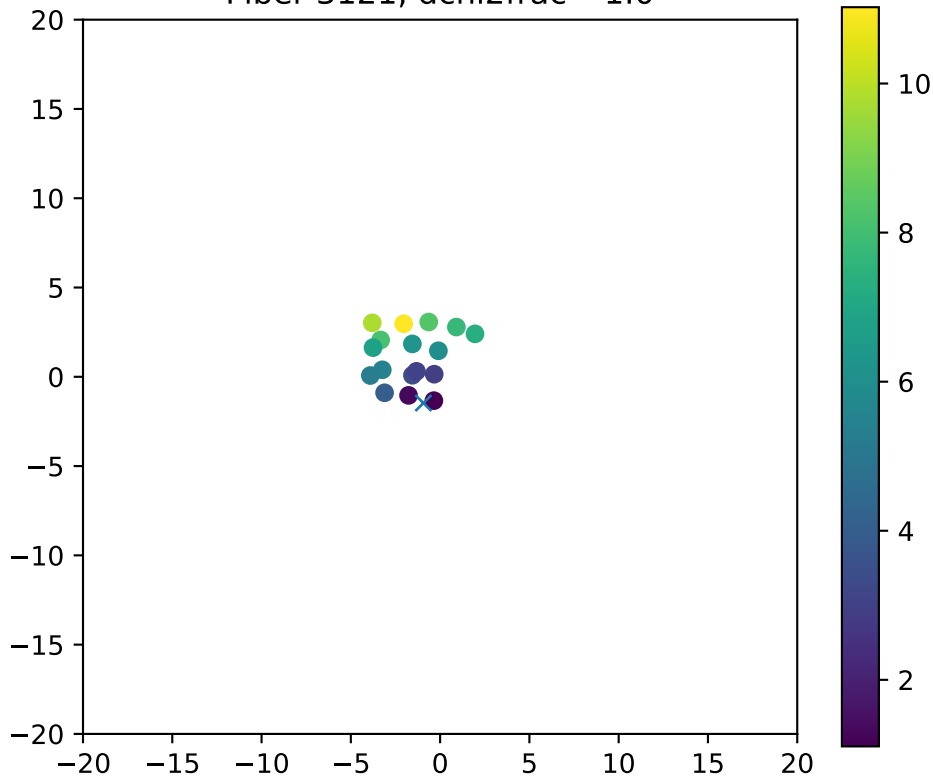
Fiber 3121, dchi2frac= 1.0
