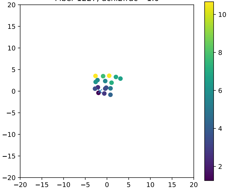
Fiber 1227, dchi2frac= 1.0
