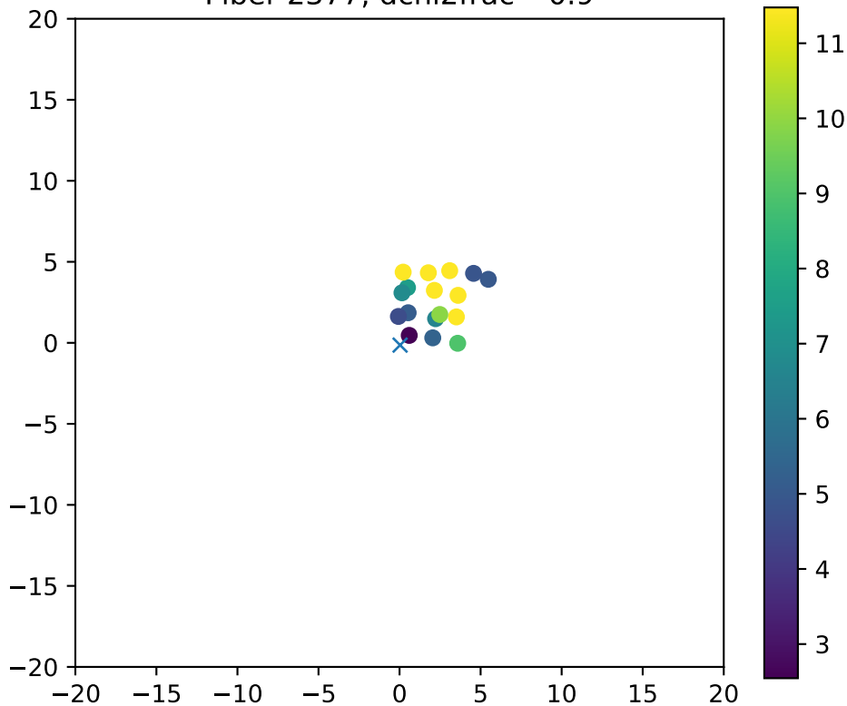
Fiber 2377, dchi2frac= 0.9
