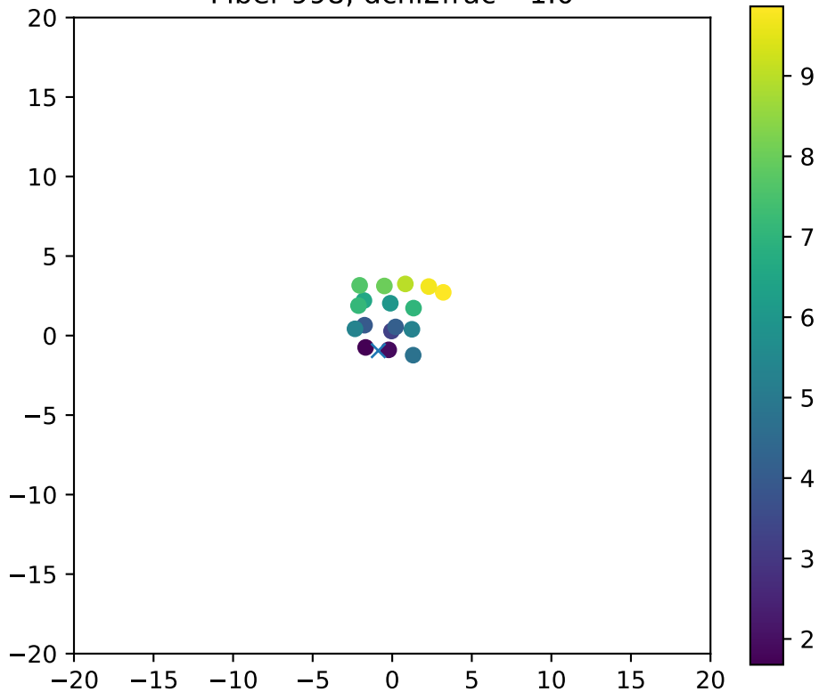
Fiber 998, dchi2frac= 1.0
