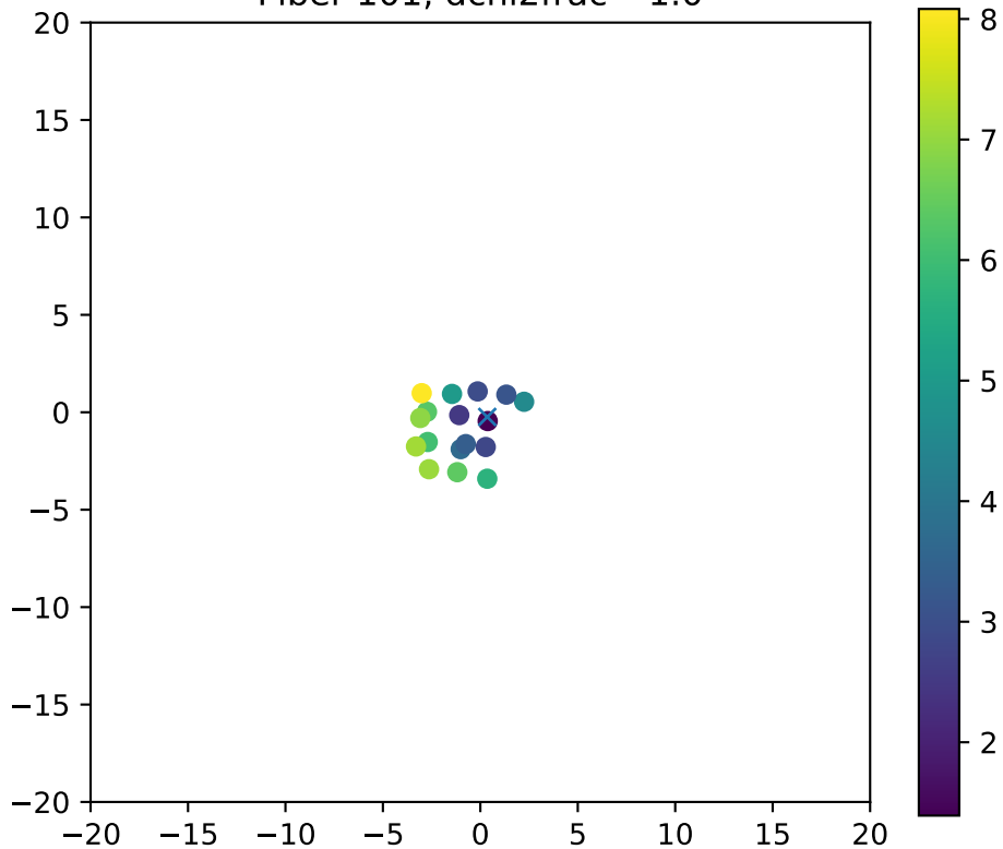
Fiber 101, dchi2frac= 1.0
