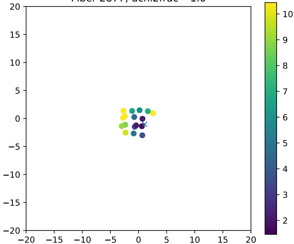
Fiber 2877, dchi2frac= 1.0
