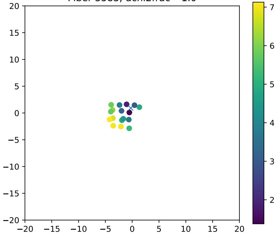
Fiber 3583, dchi2frac= 1.0
