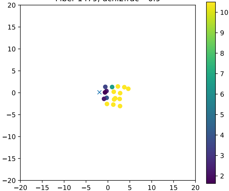
Fiber 1479, dchi2frac= 0.9
