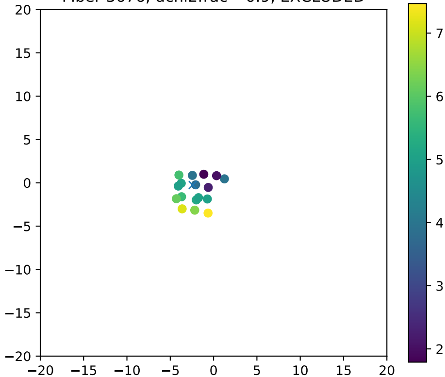
Fiber 3676, dchi2frac= 0.9, EXCLUDED
