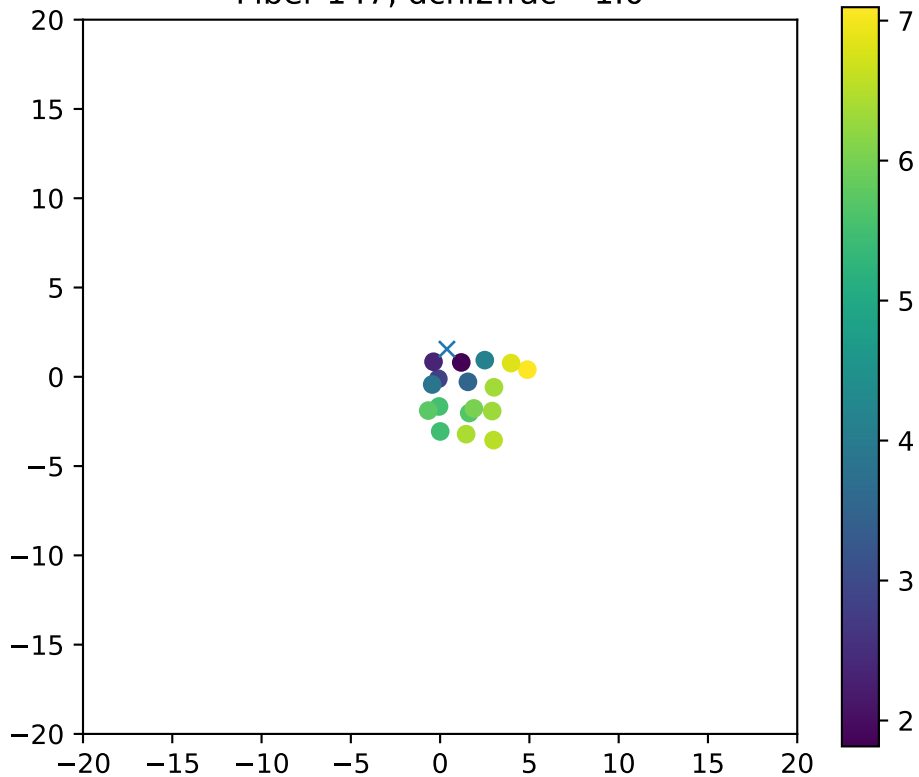
Fiber 147, dchi2frac= 1.0
