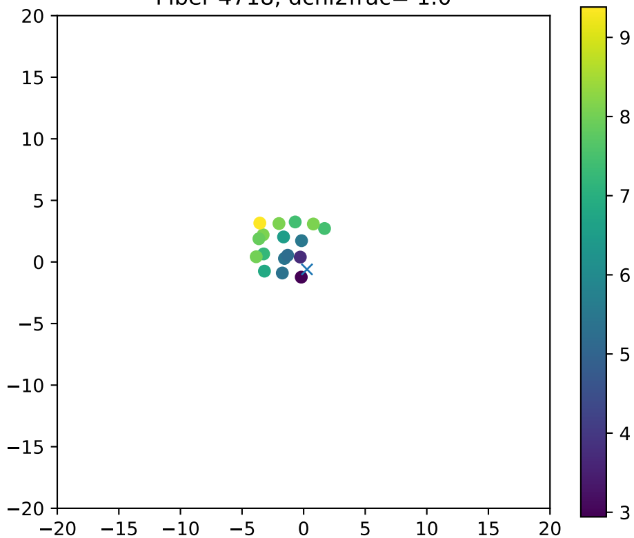
Fiber 4718, dchi2frac= 1.0
