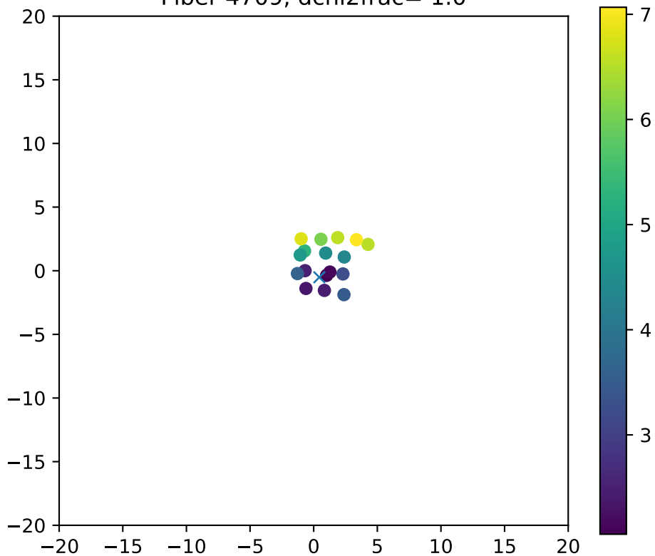
Fiber 4709, dchi2frac= 1.0
