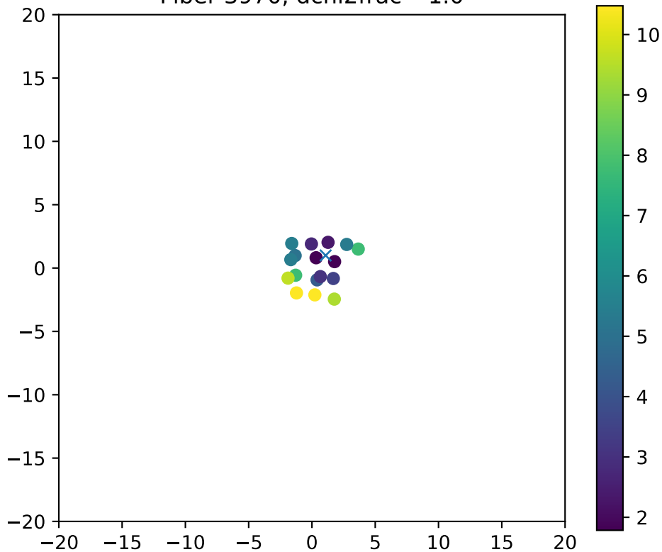
Fiber 3970, dchi2frac= 1.0
