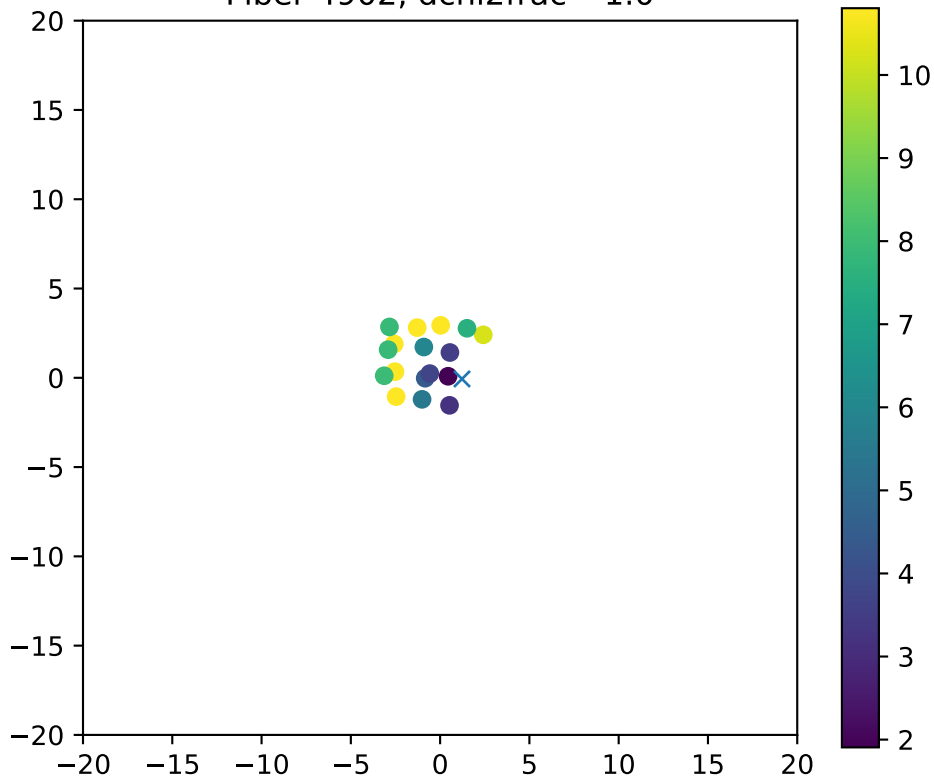
Fiber 4902, dchi2frac= 1.0
