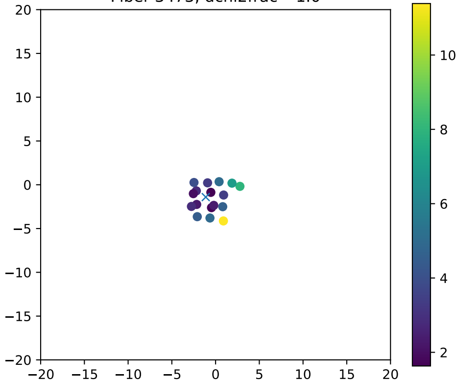
Fiber 3473, dchi2frac= 1.0
