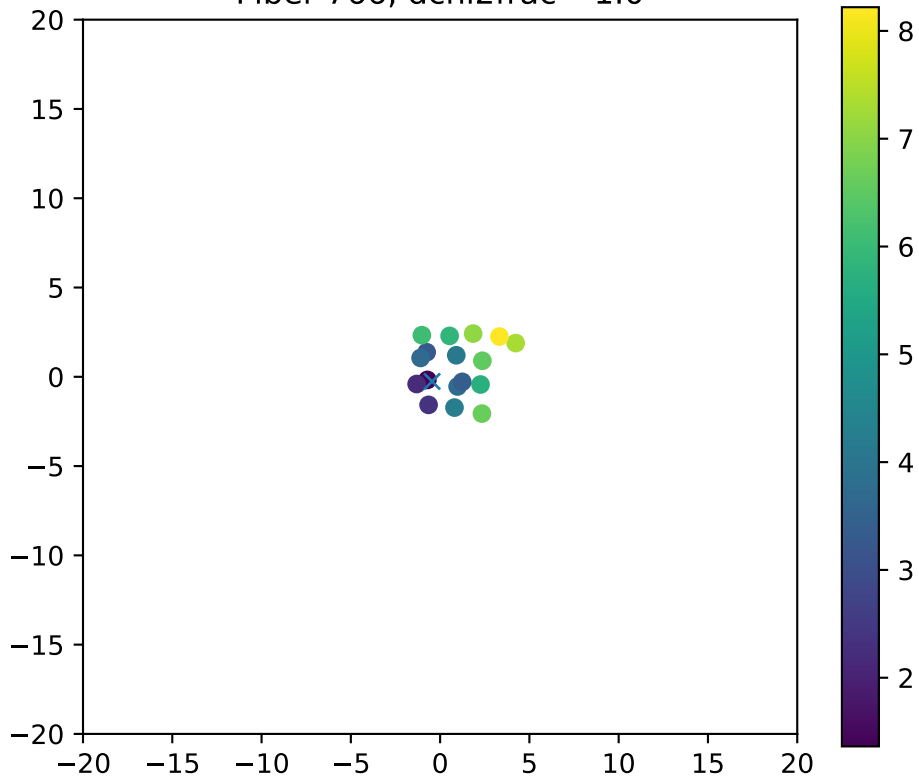
Fiber 766, dchi2frac= 1.0
