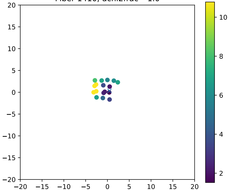
Fiber 1410, dchi2frac= 1.0
