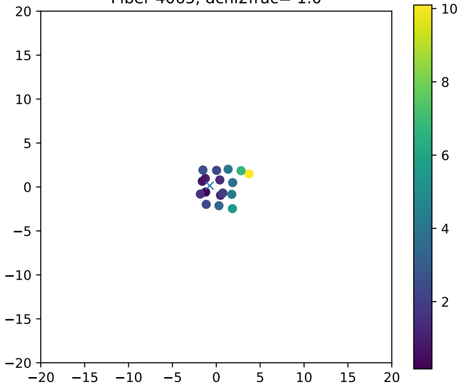
Fiber 4065, dchi2frac= 1.0
