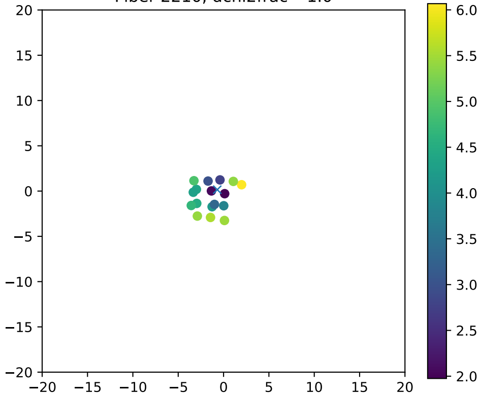
Fiber 2210, dchi2frac= 1.0
