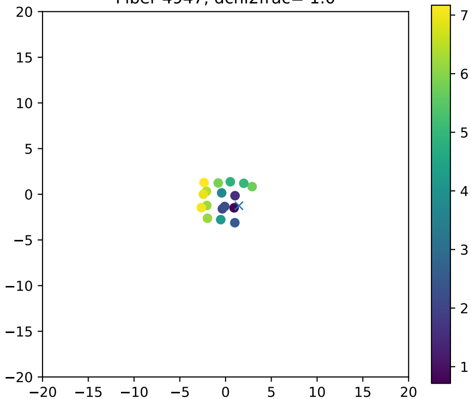
Fiber 4947, dchi2frac= 1.0
