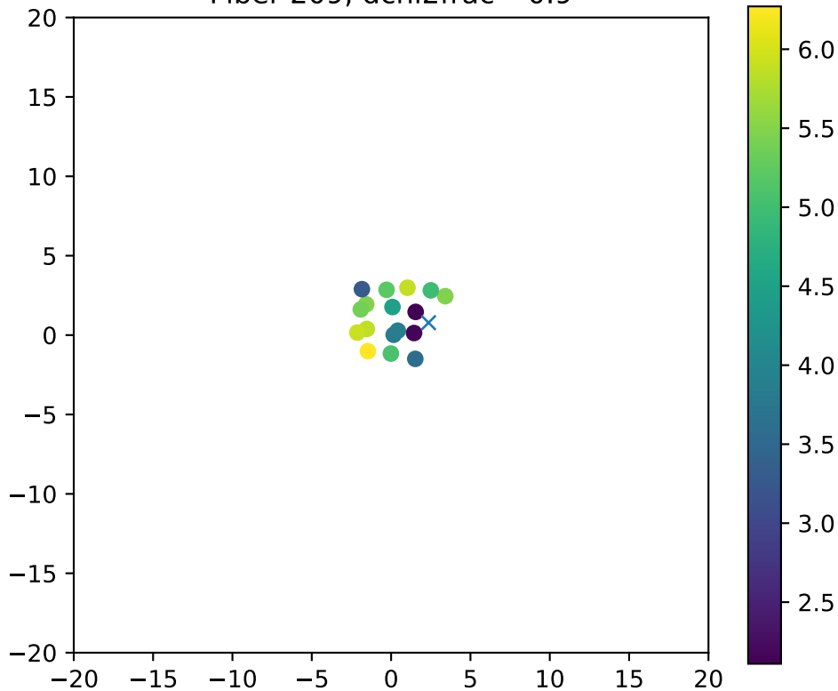
Fiber 209, dchi2frac= 0.9
