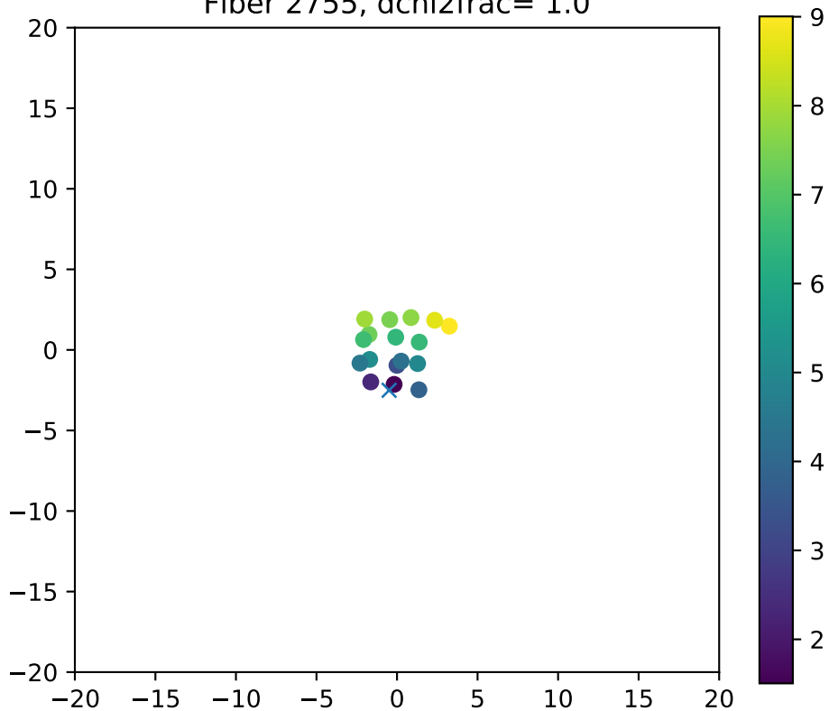
Fiber 2755, dchi2frac= 1.0
