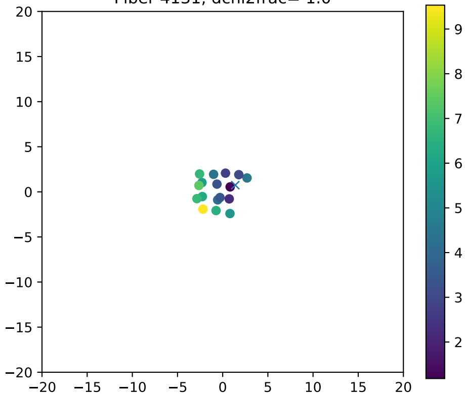
Fiber 4131, dchi2frac= 1.0
