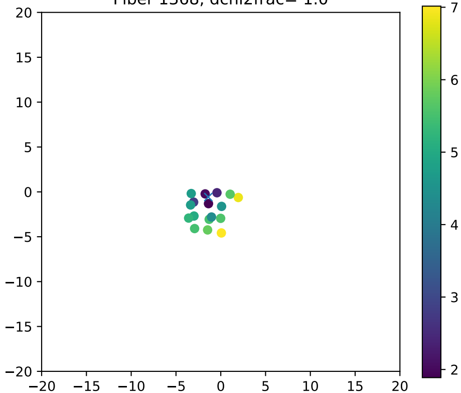
Fiber 1368, dchi2frac= 1.0
