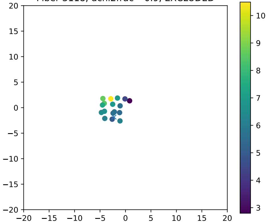
Fiber 3118, dchi2frac= 0.9, EXCLUDED
