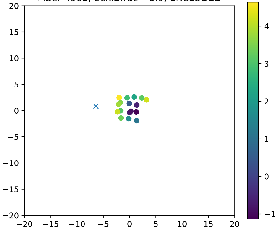
Fiber 4962, dchi2frac= 0.9, EXCLUDED
