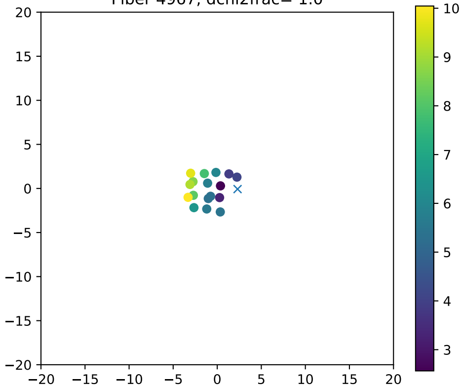
Fiber 4967, dchi2frac= 1.0
