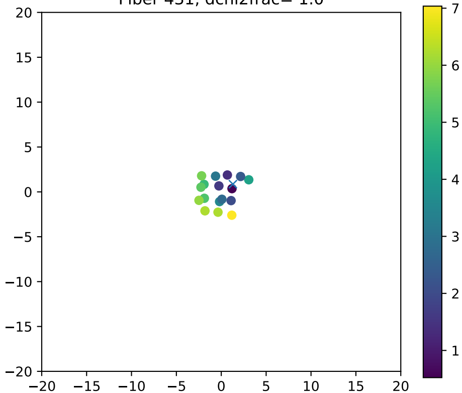
Fiber 431, dchi2frac= 1.0
