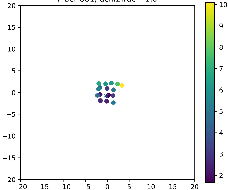
Fiber 801, dchi2frac= 1.0
