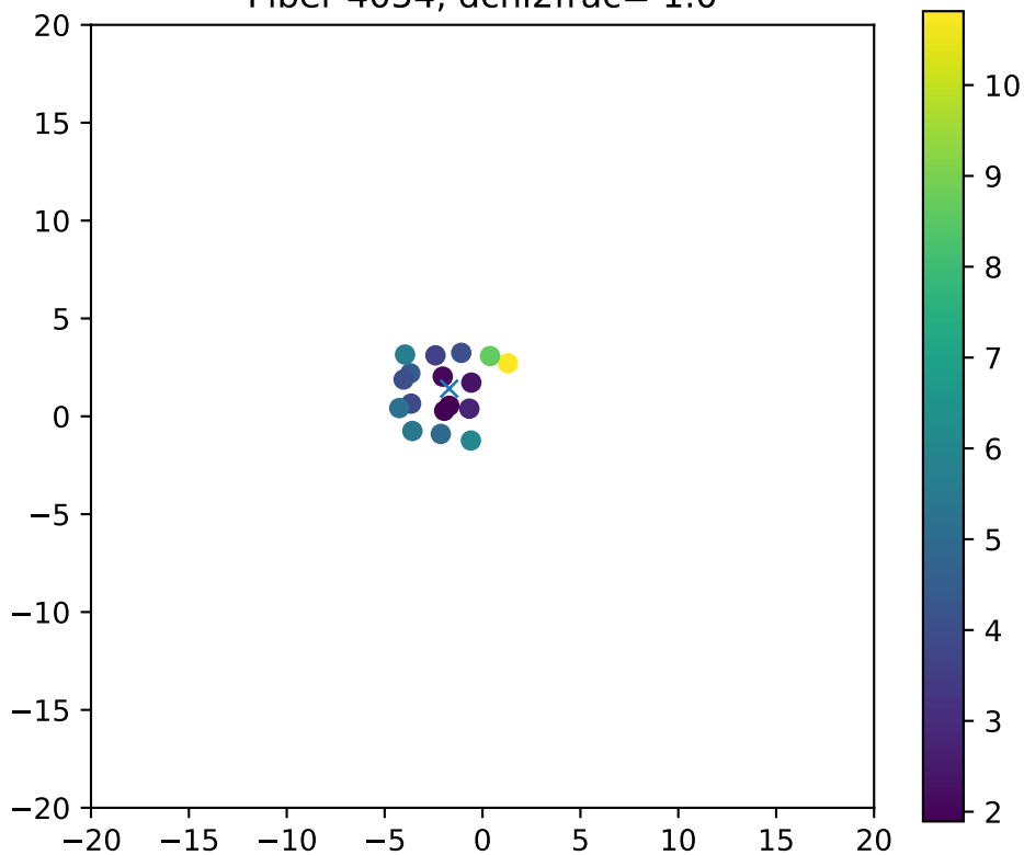
Fiber 4054, dchi2frac= 1.0
