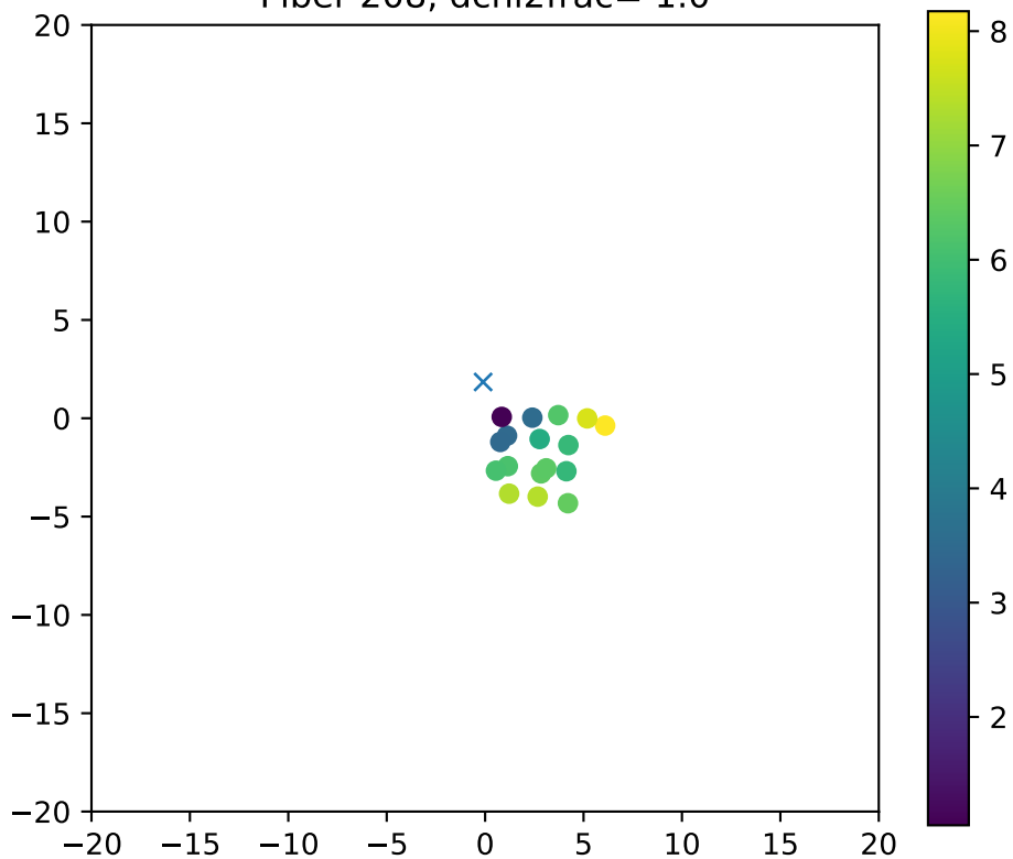
Fiber 208, dchi2frac= 1.0
