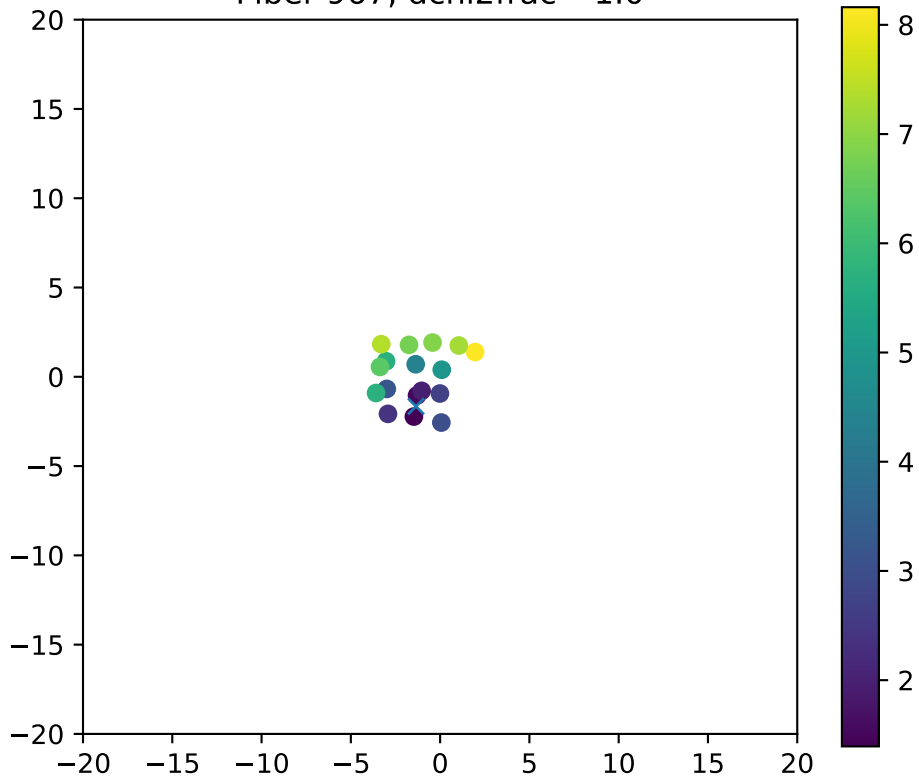
Fiber 967, dchi2frac= 1.0
