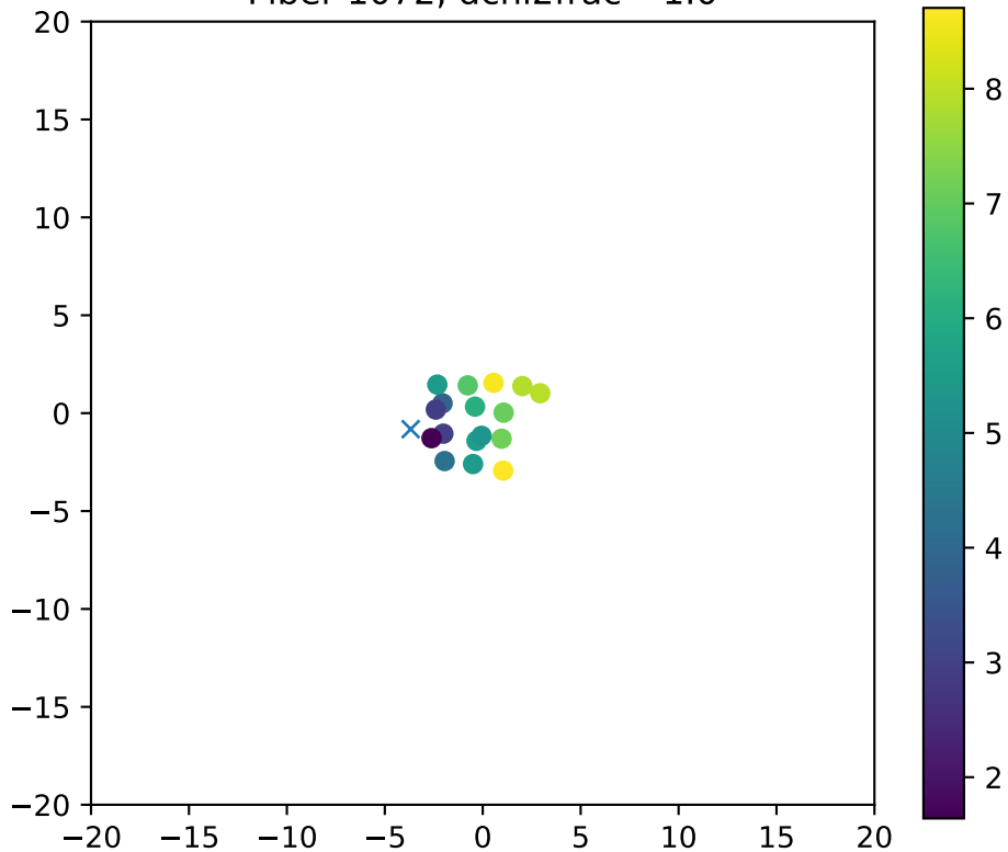
Fiber 1072, dchi2frac= 1.0
