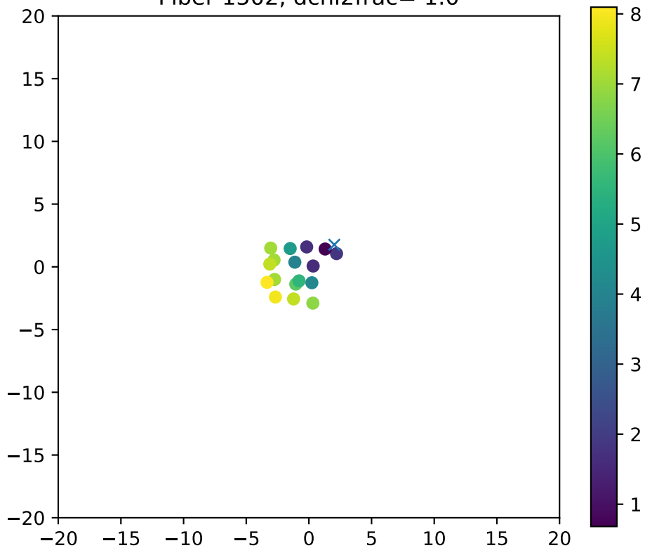
Fiber 1502, dchi2frac= 1.0
