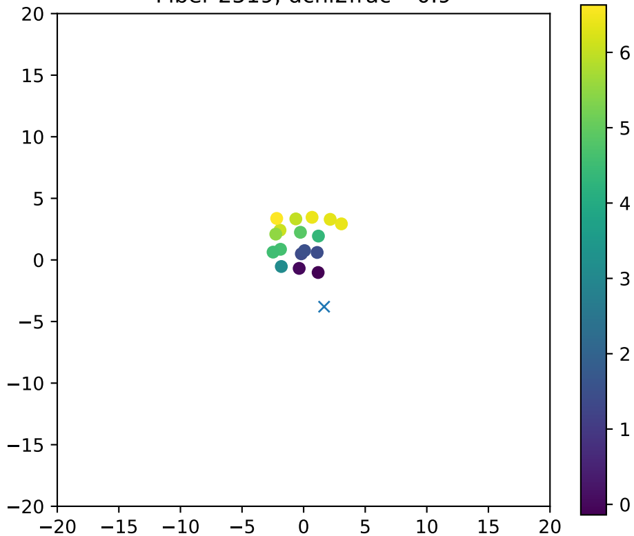
Fiber 2519, dchi2frac= 0.9
