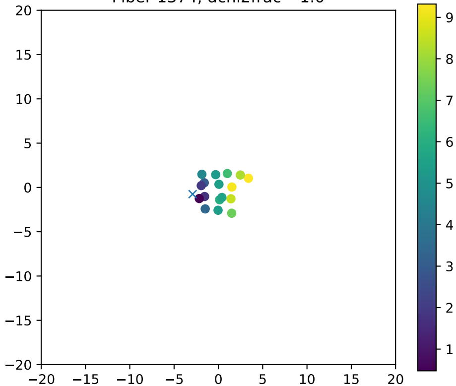
Fiber 1374, dchi2frac= 1.0
