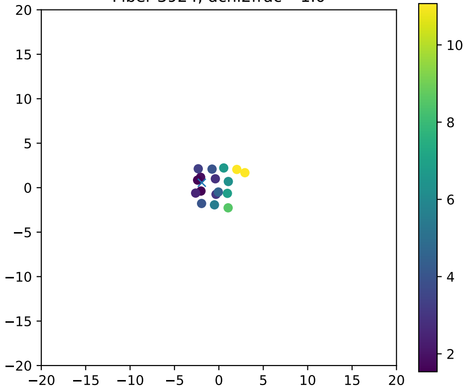
Fiber 3924, dchi2frac= 1.0
