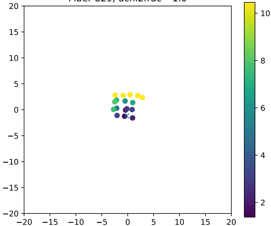
Fiber 829, dchi2frac= 1.0
