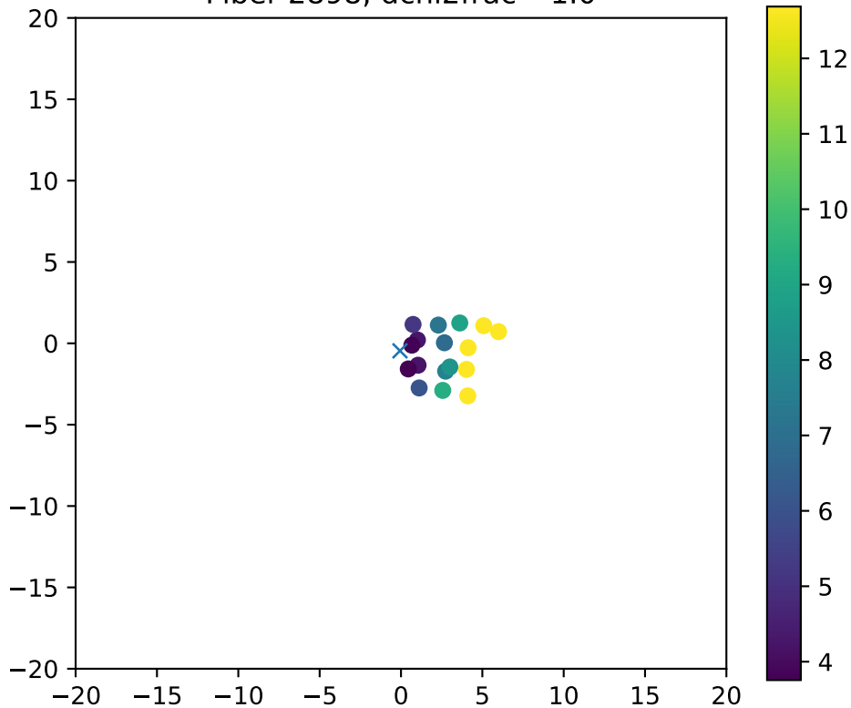
Fiber 2898, dchi2frac= 1.0
