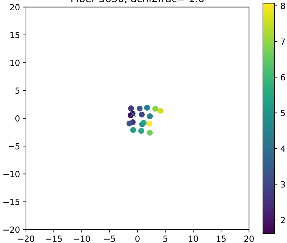
Fiber 3650, dchi2frac= 1.0
