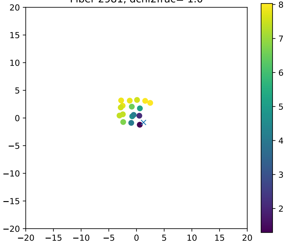
Fiber 2981, dchi2frac= 1.0
