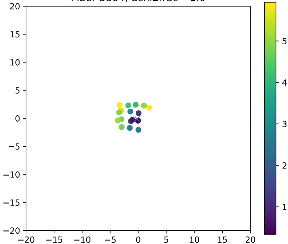
Fiber 3864, dchi2frac= 1.0
