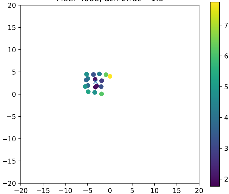
Fiber 4086, dchi2frac= 1.0
