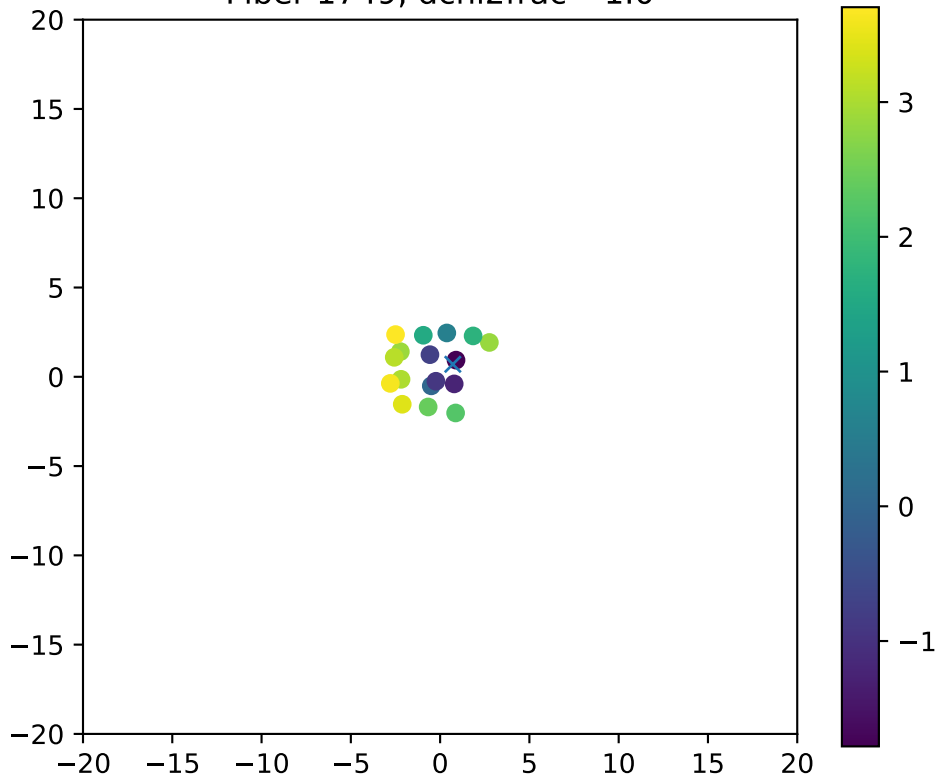
Fiber 1749, dchi2frac= 1.0
