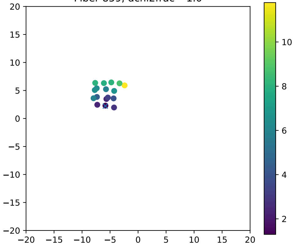
Fiber 859, dchi2frac= 1.0
