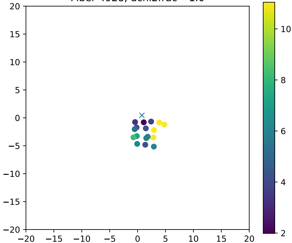
Fiber 4928, dchi2frac= 1.0
