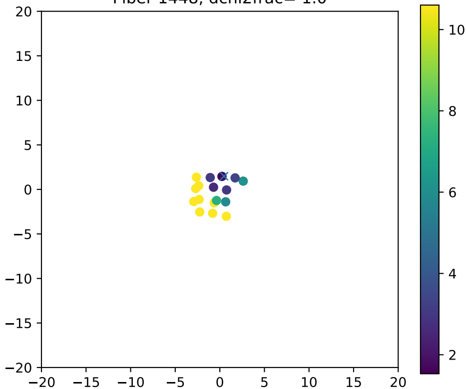
Fiber 1448, dchi2frac= 1.0
