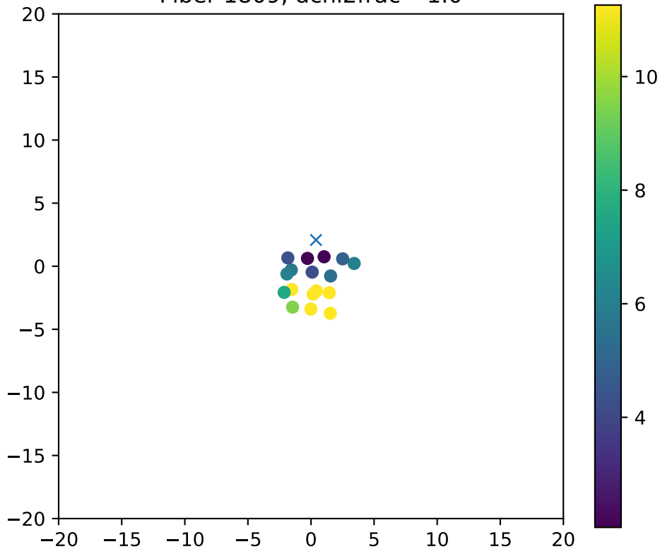
Fiber 1809, dchi2frac= 1.0
