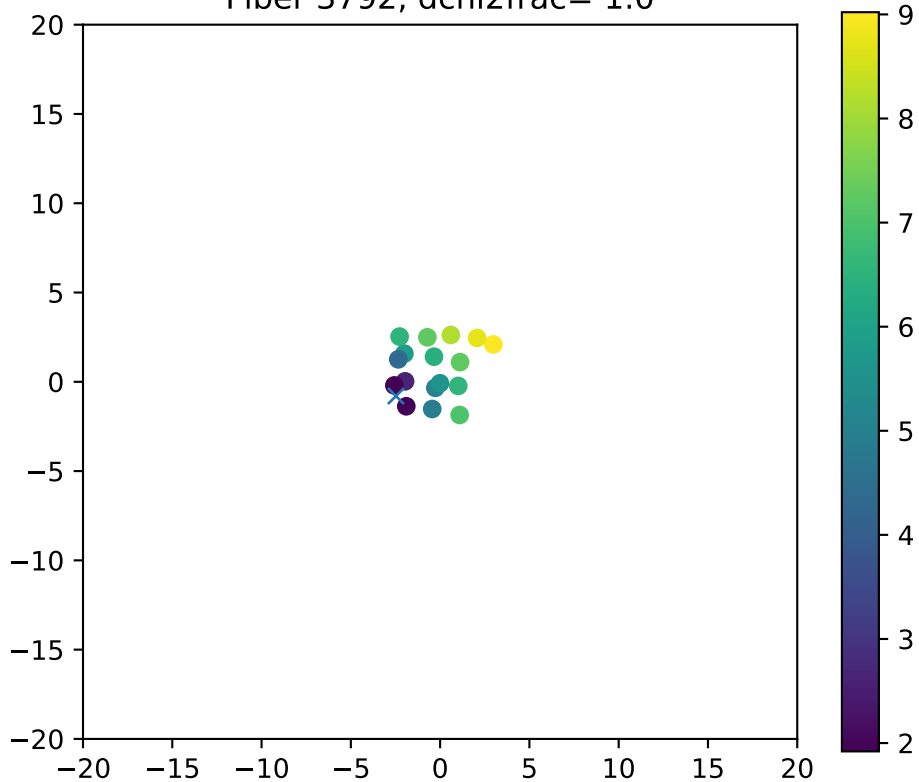
Fiber 3792, dchi2frac= 1.0
