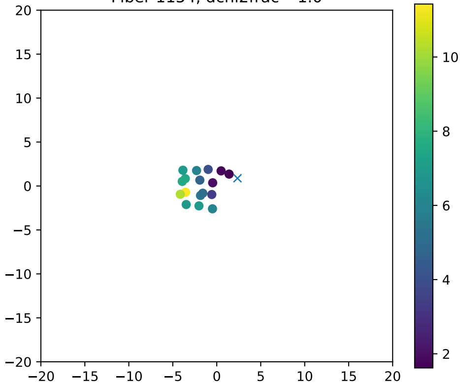
Fiber 1154, dchi2frac= 1.0
