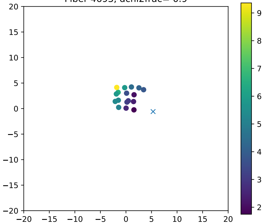
Fiber 4693, dchi2frac= 0.9
