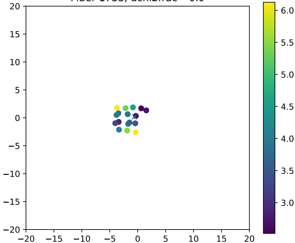
Fiber 1733, dchi2frac= 0.9
