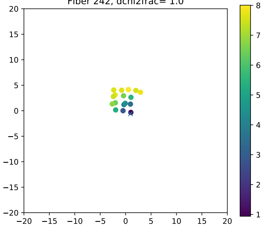
Fiber 242, dchi2frac= 1.0
