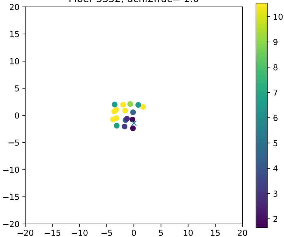
Fiber 3352, dchi2frac= 1.0
