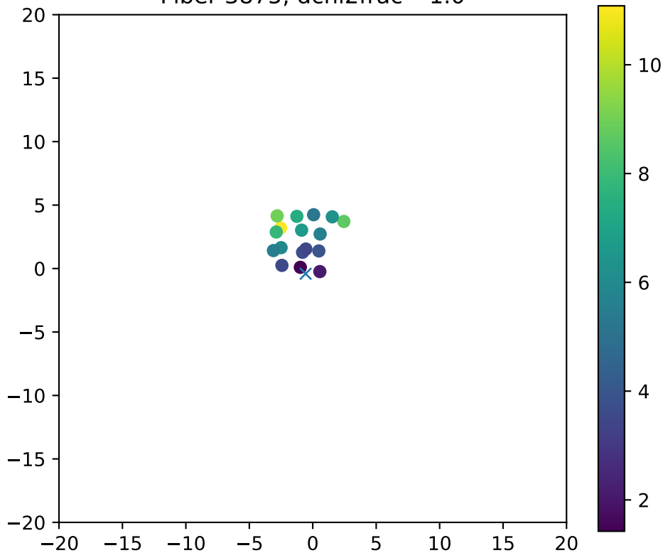
Fiber 3875, dchi2frac= 1.0
