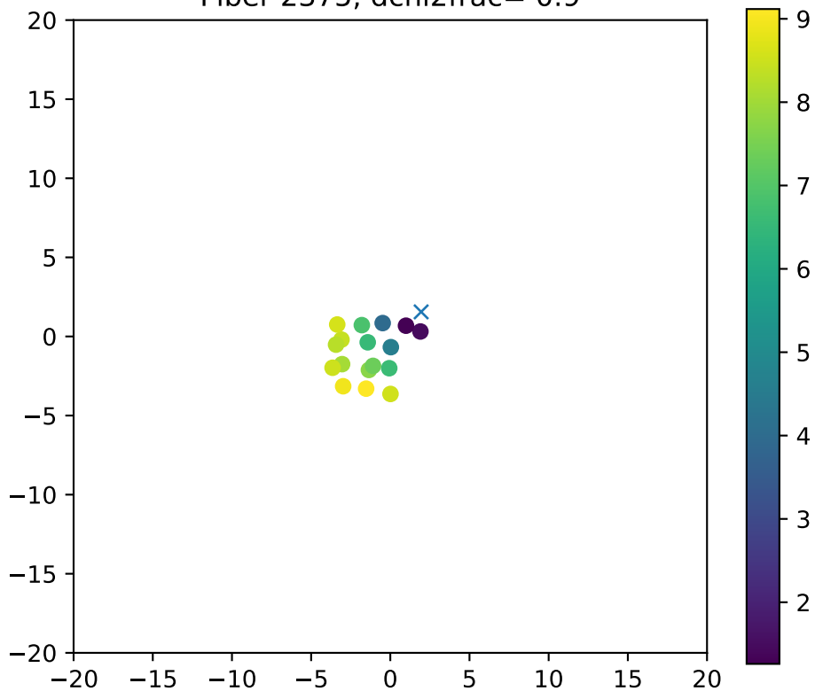
Fiber 2375, dchi2frac= 0.9
