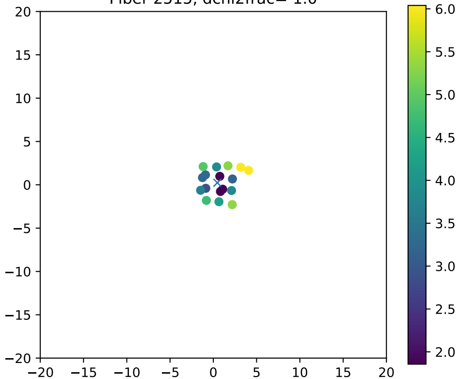
Fiber 2515, dchi2frac= 1.0
