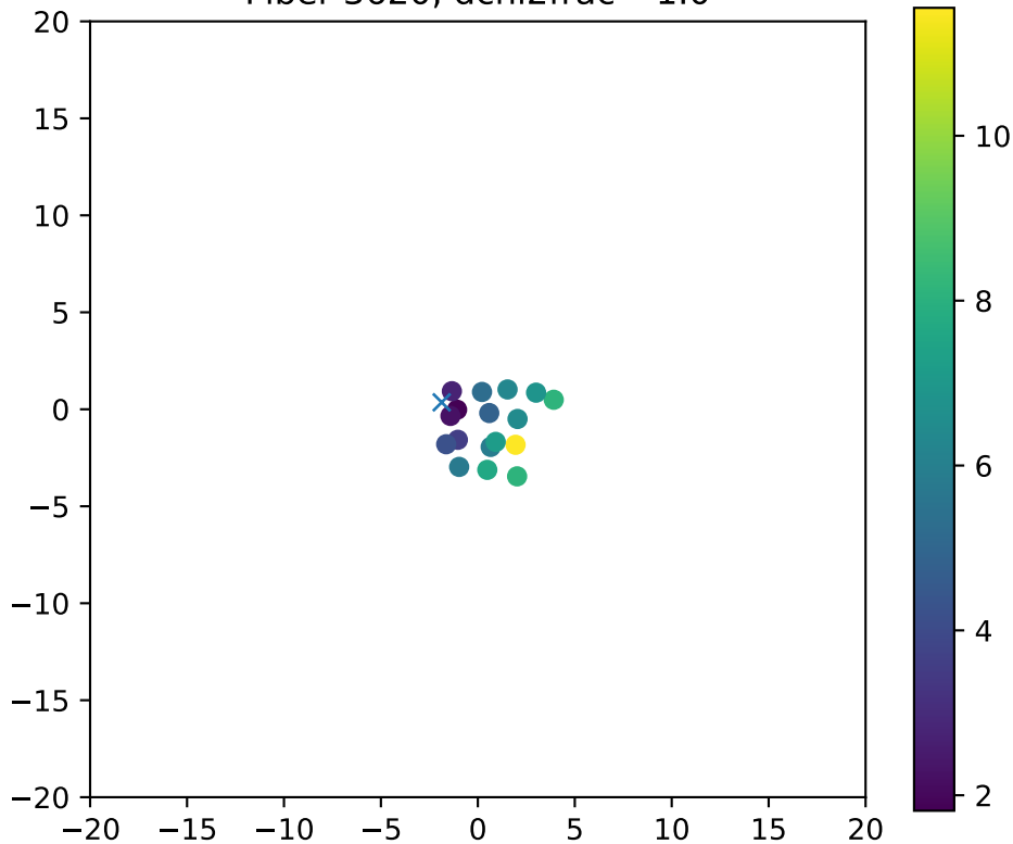
Fiber 3620, dchi2frac= 1.0
