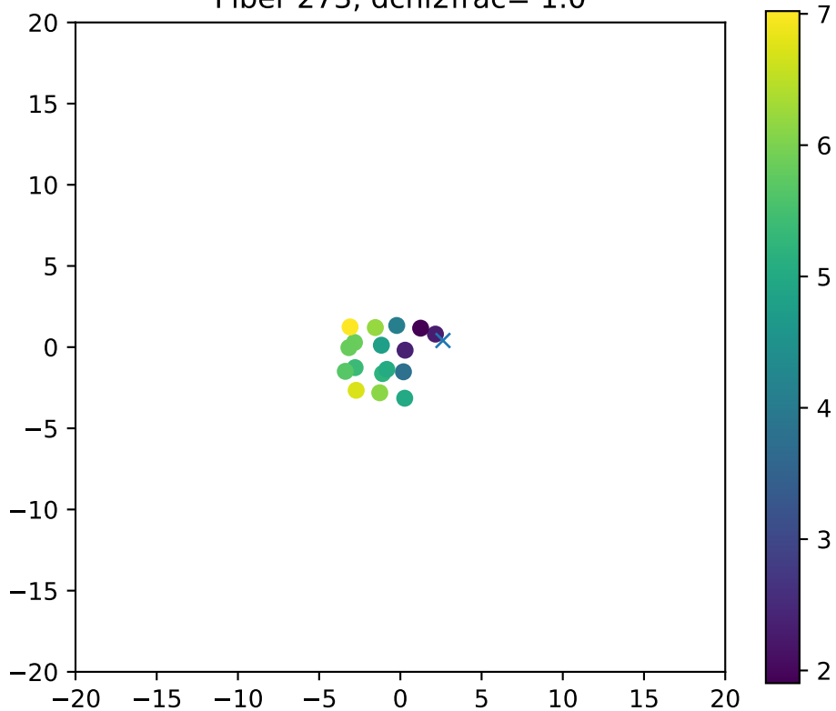
Fiber 273, dchi2frac= 1.0
