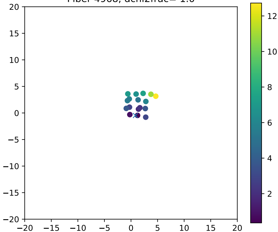
Fiber 4968, dchi2frac= 1.0
