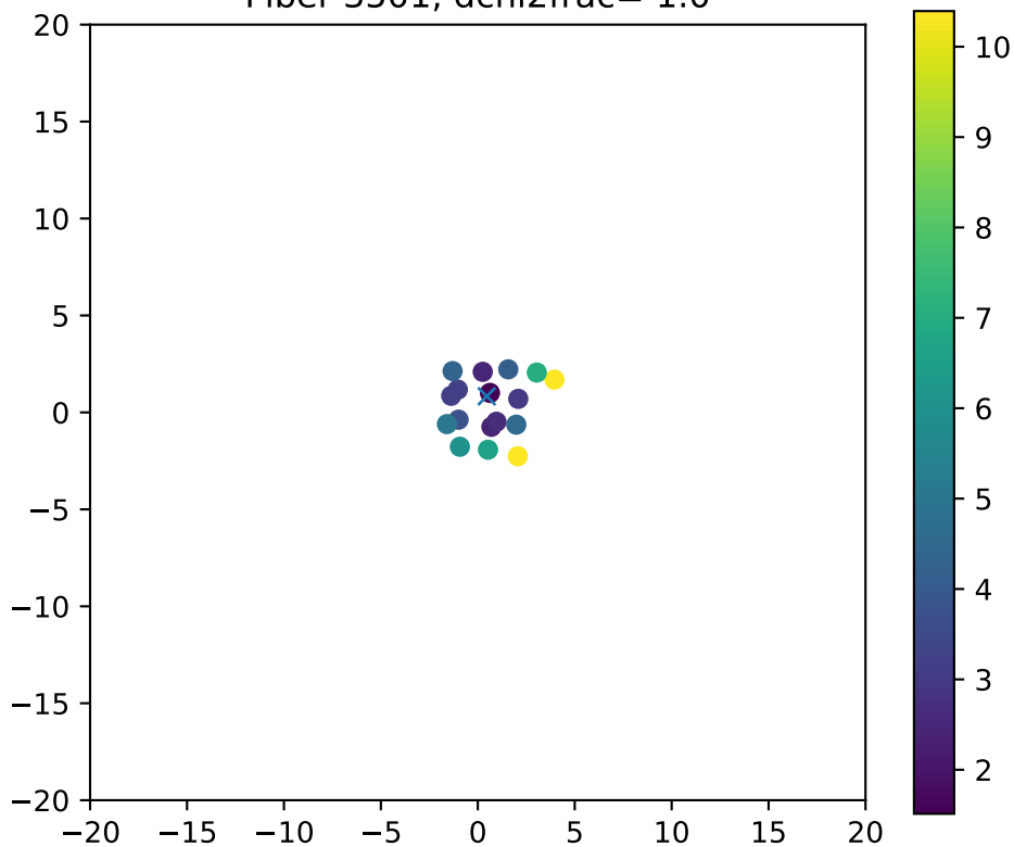
Fiber 3501, dchi2frac= 1.0
