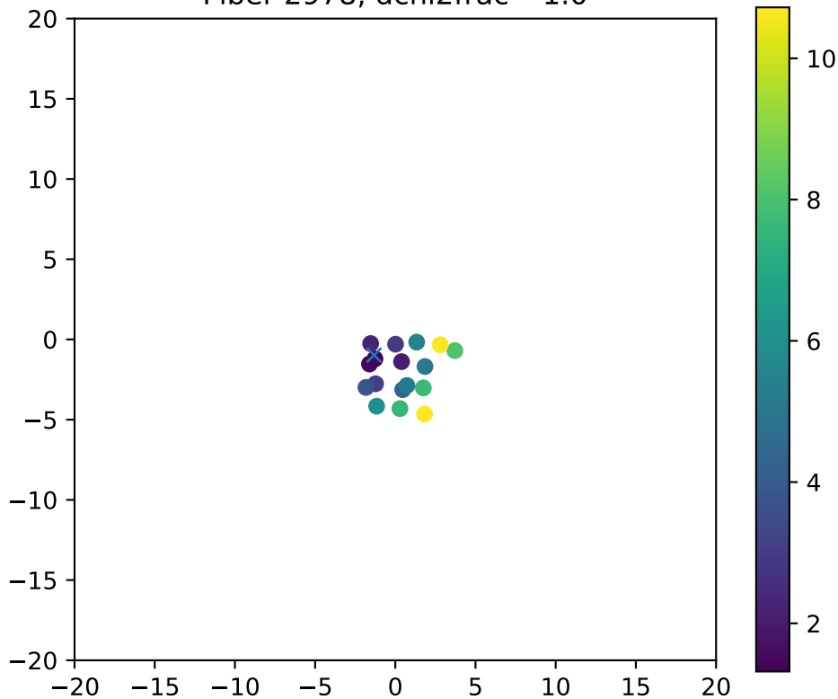
Fiber 2978, dchi2frac= 1.0
