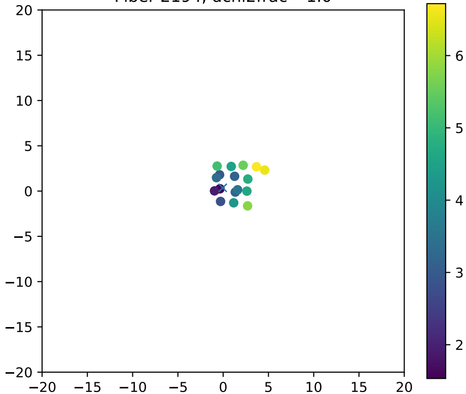
Fiber 2194, dchi2frac= 1.0
