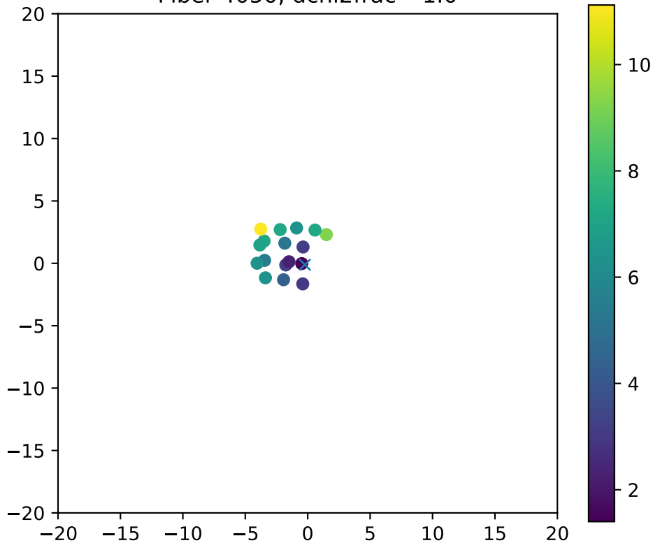
Fiber 4050, dchi2frac= 1.0
