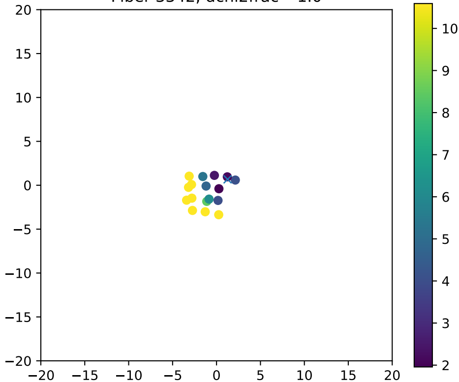
Fiber 3342, dchi2frac= 1.0
