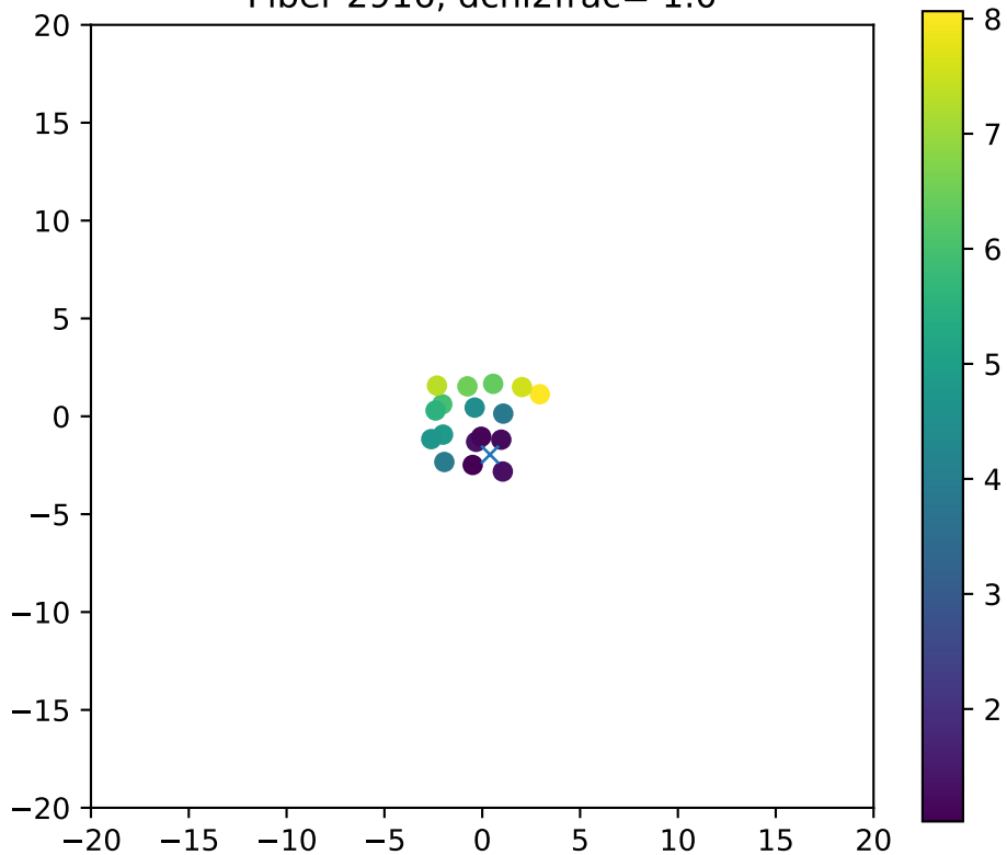
Fiber 2916, dchi2frac= 1.0
