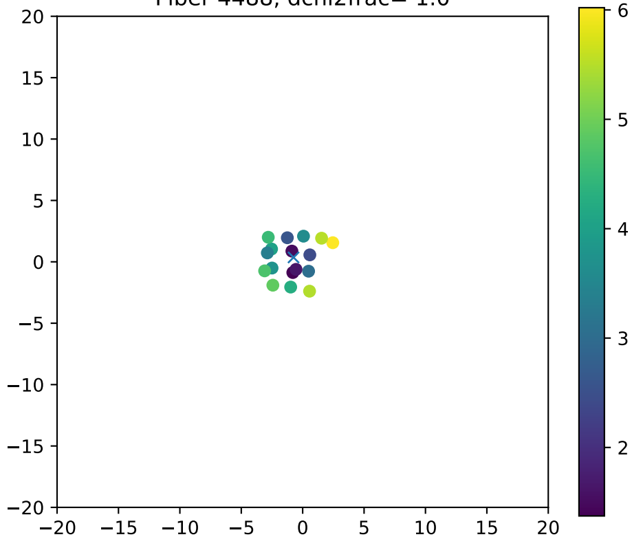
Fiber 4488, dchi2frac= 1.0
