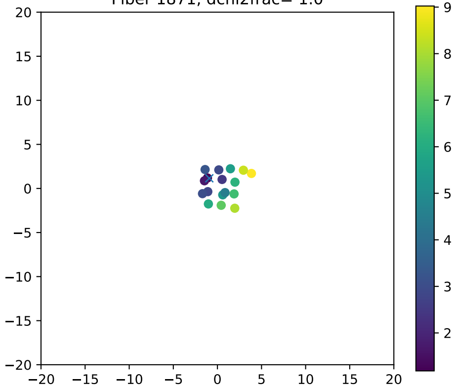
Fiber 1871, dchi2frac= 1.0
