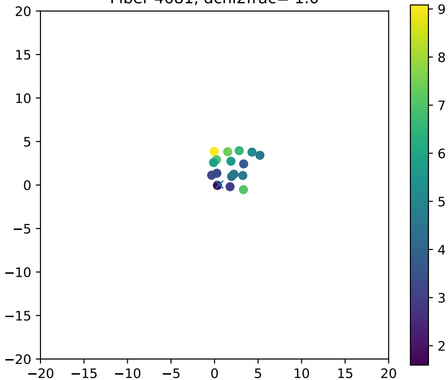
Fiber 4681, dchi2frac= 1.0
