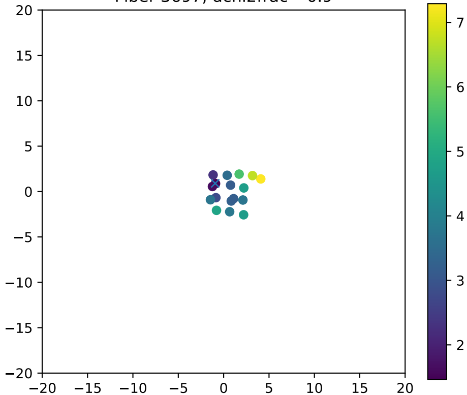
Fiber 3697, dchi2frac= 0.9
