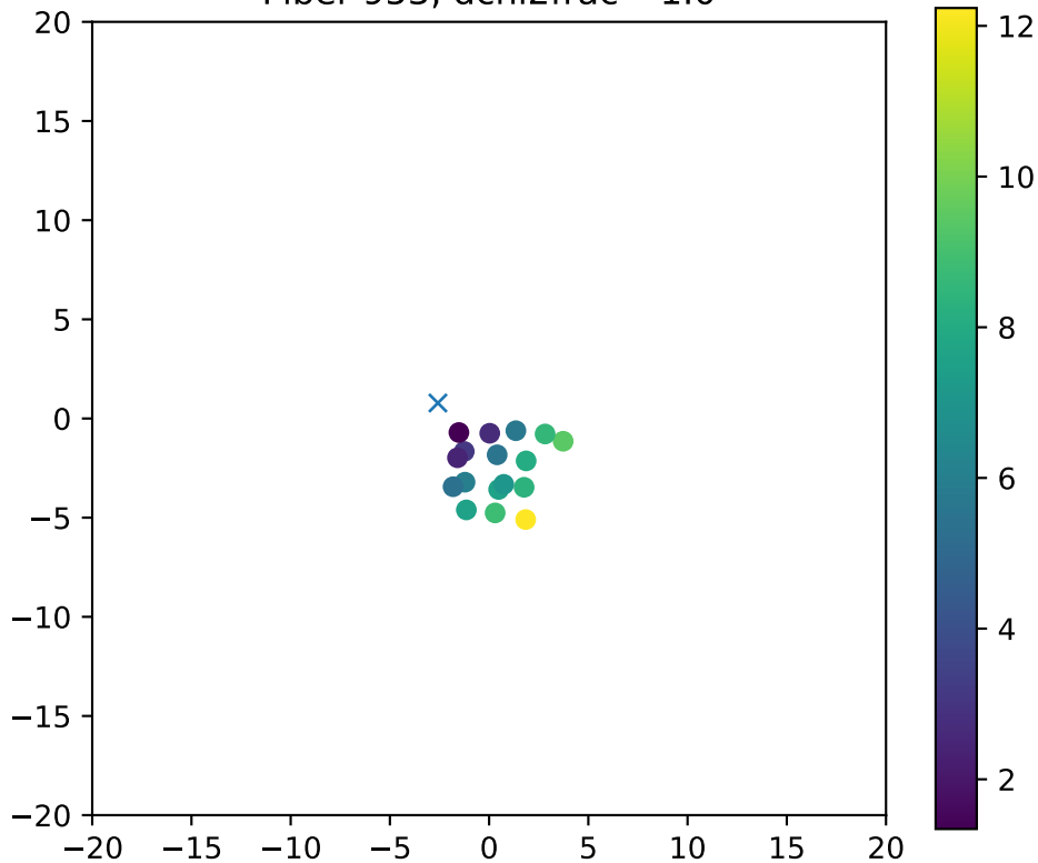
Fiber 953, dchi2frac= 1.0
