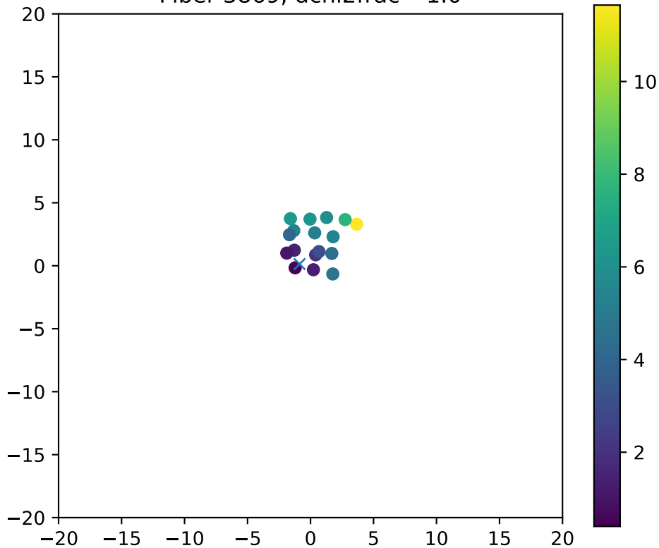
Fiber 3869, dchi2frac= 1.0
