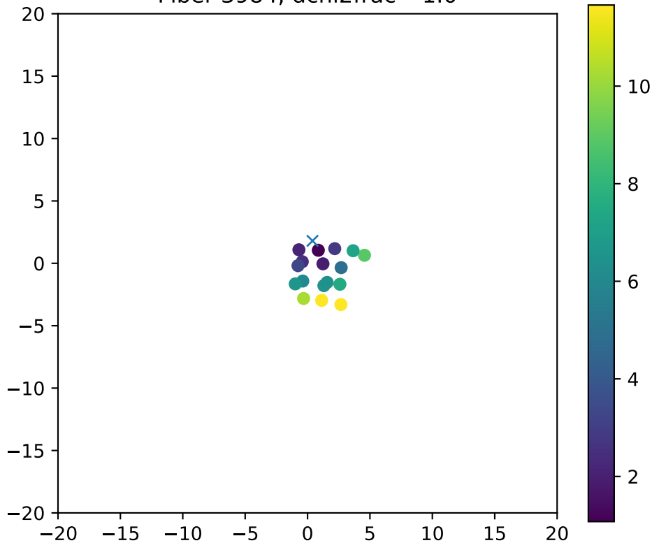
Fiber 3984, dchi2frac= 1.0
