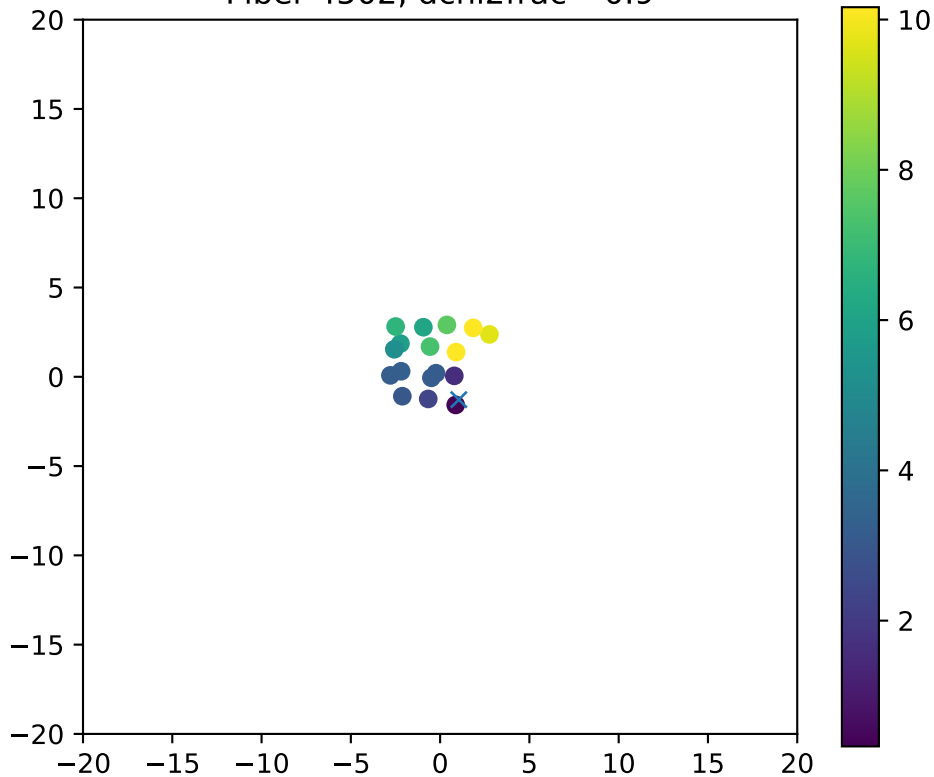
Fiber 4502, dchi2frac= 0.9
