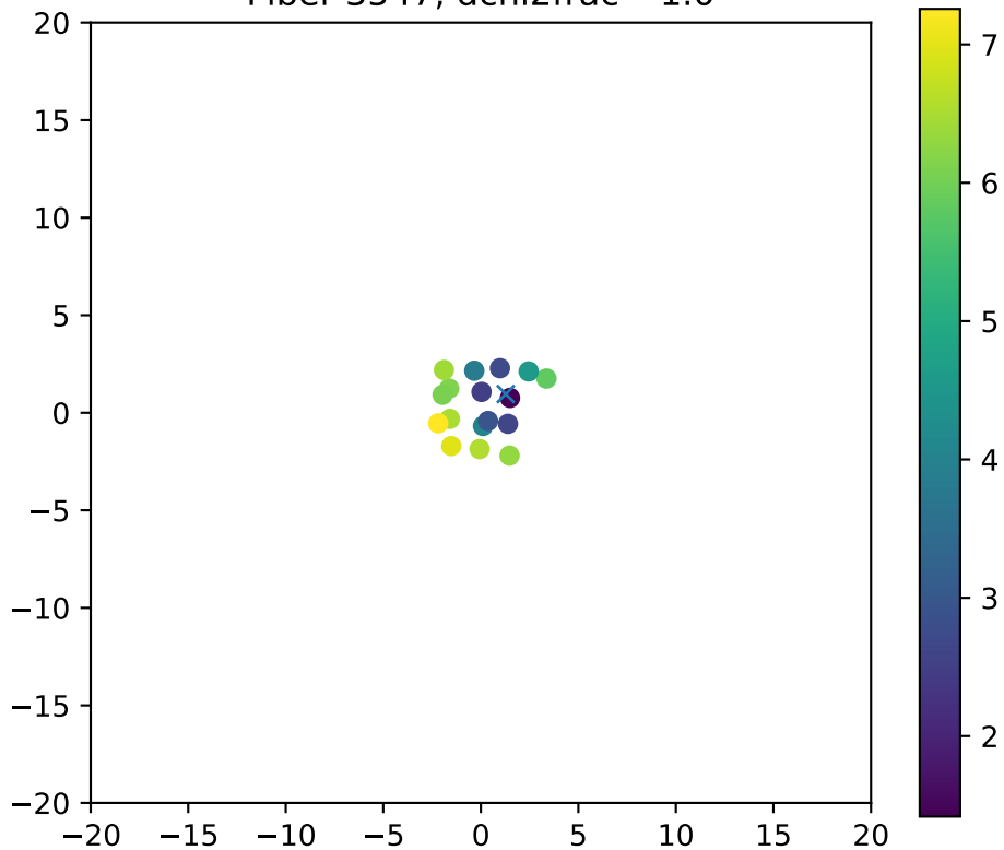
Fiber 3547, dchi2frac= 1.0
