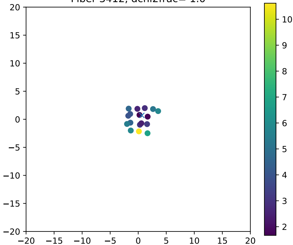
Fiber 3412, dchi2frac= 1.0
