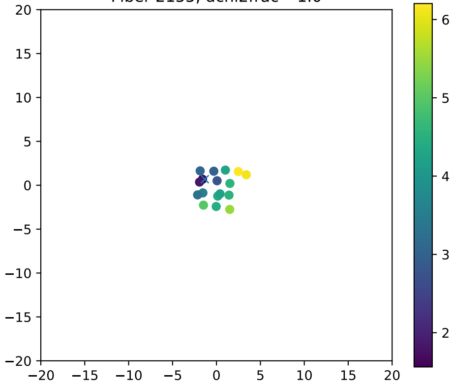
Fiber 2155, dchi2frac= 1.0
