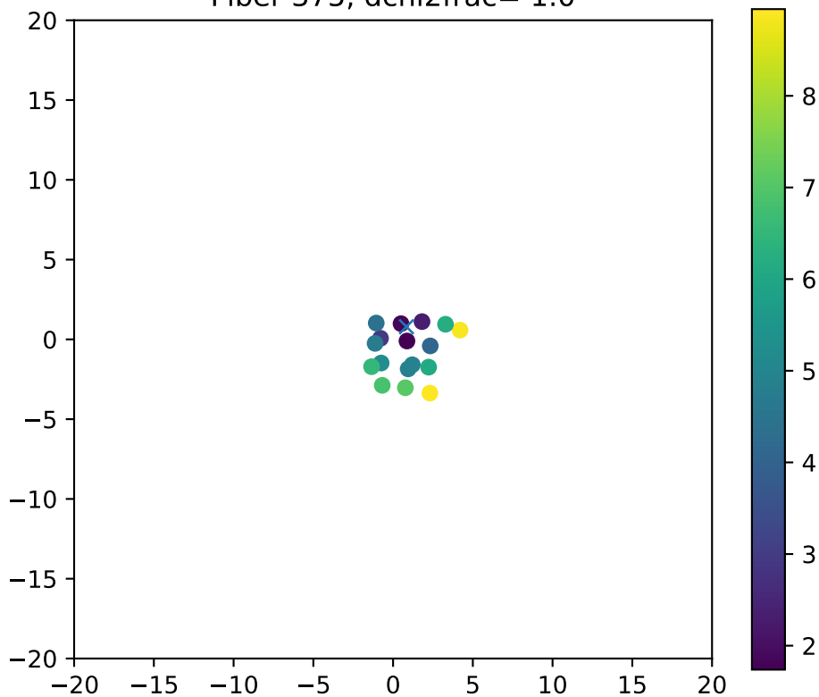
Fiber 375, dchi2frac= 1.0
