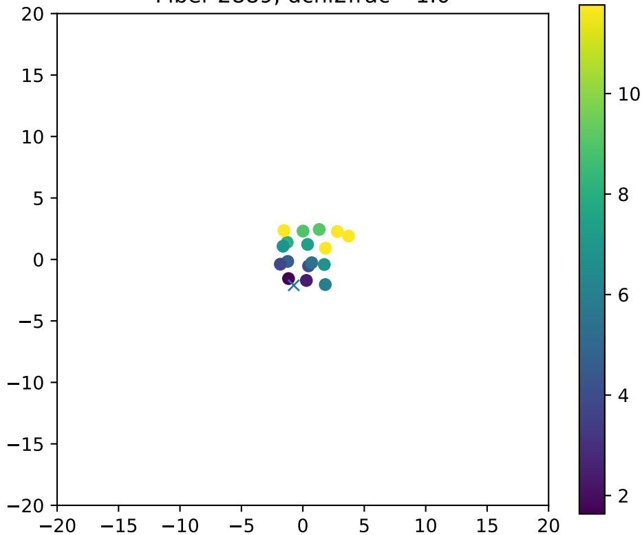
Fiber 2889, dchi2frac= 1.0
