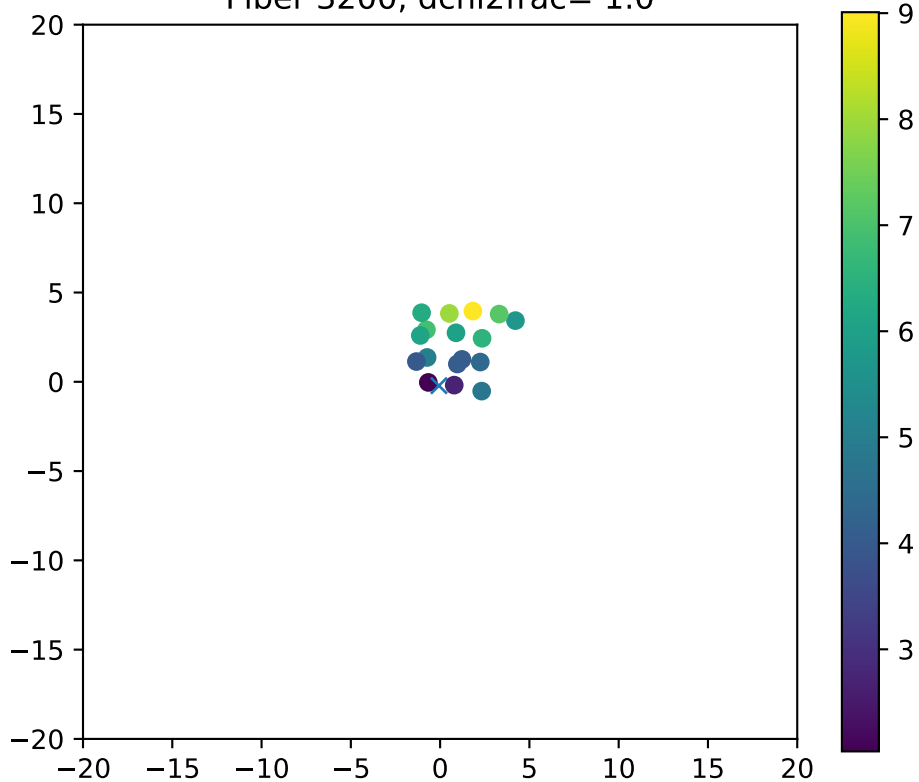
Fiber 3200, dchi2frac= 1.0
