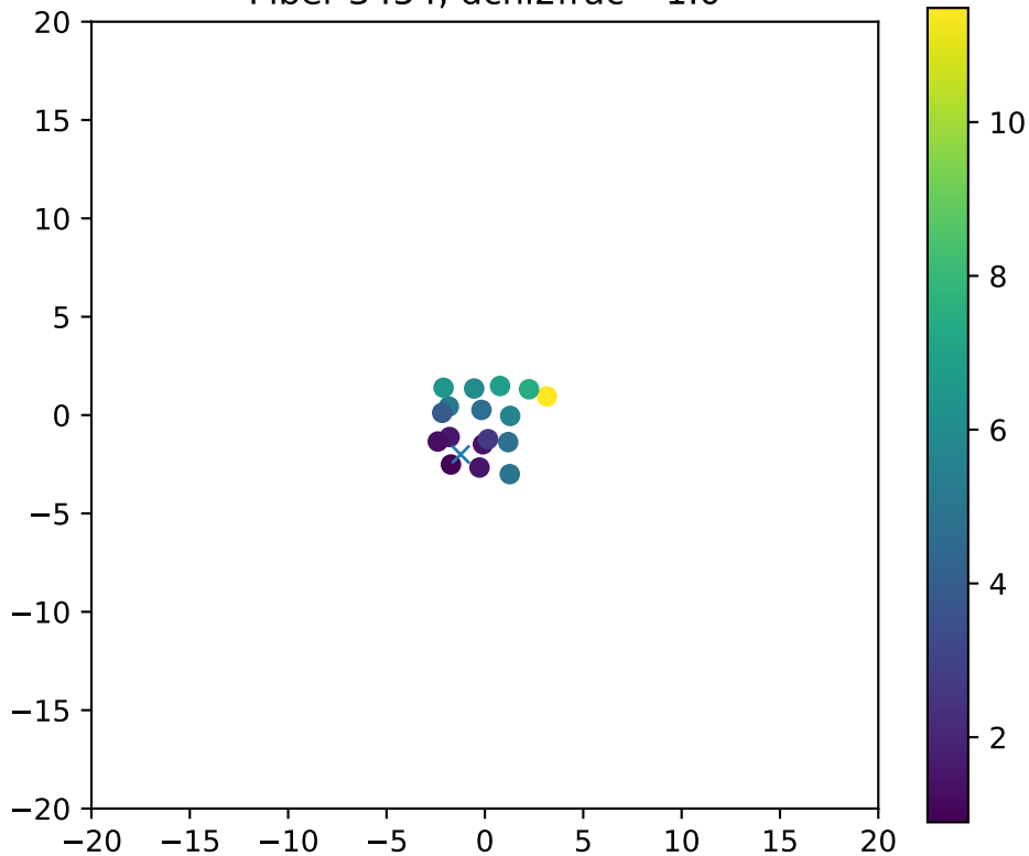
Fiber 3454, dchi2frac= 1.0
