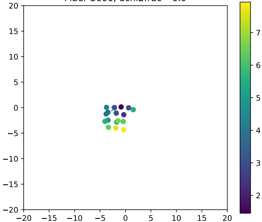
Fiber 3606, dchi2frac= 0.9
