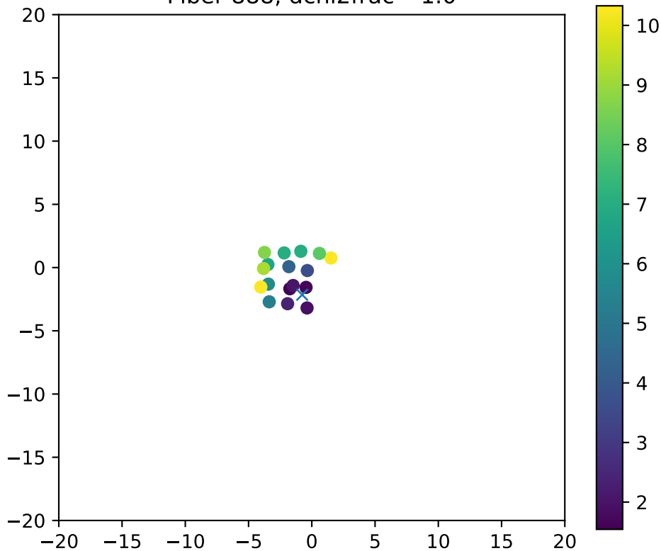
Fiber 888, dchi2frac= 1.0
