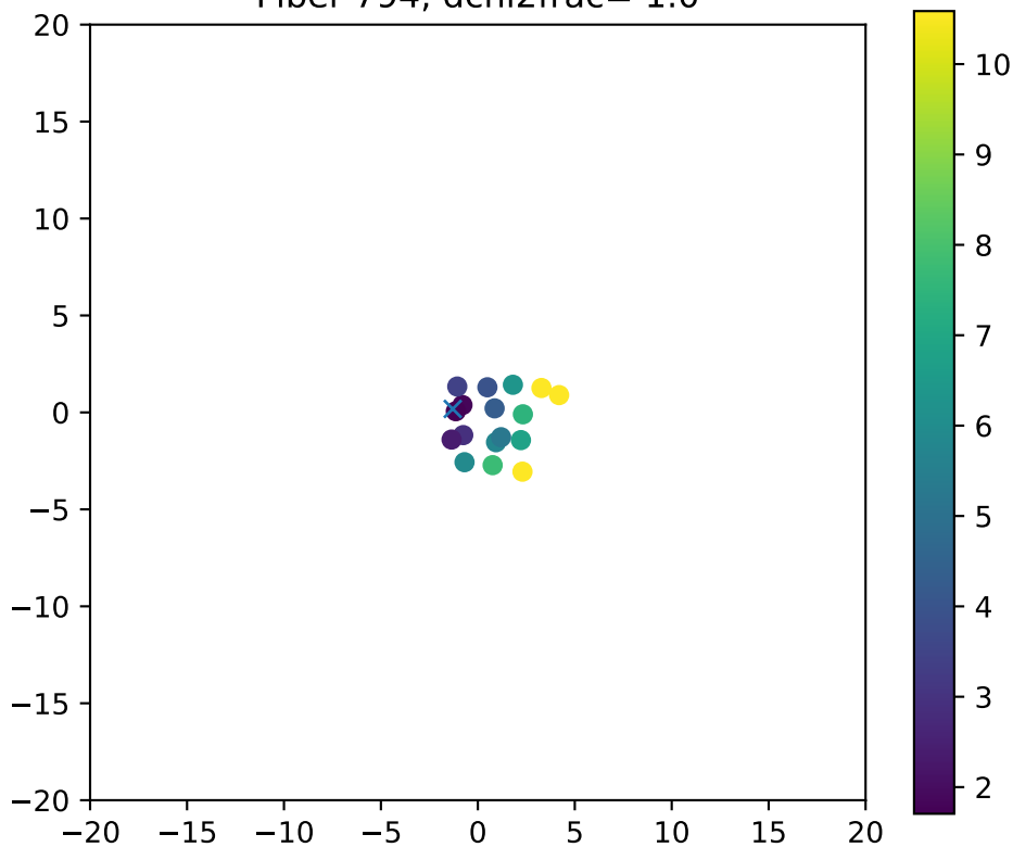
Fiber 794, dchi2frac= 1.0
