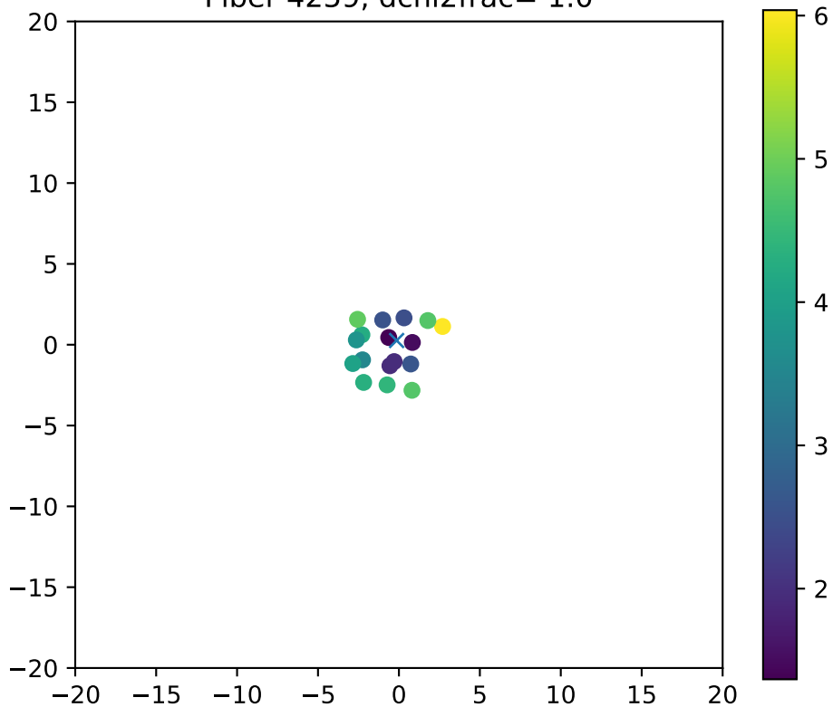
Fiber 4259, dchi2frac= 1.0
