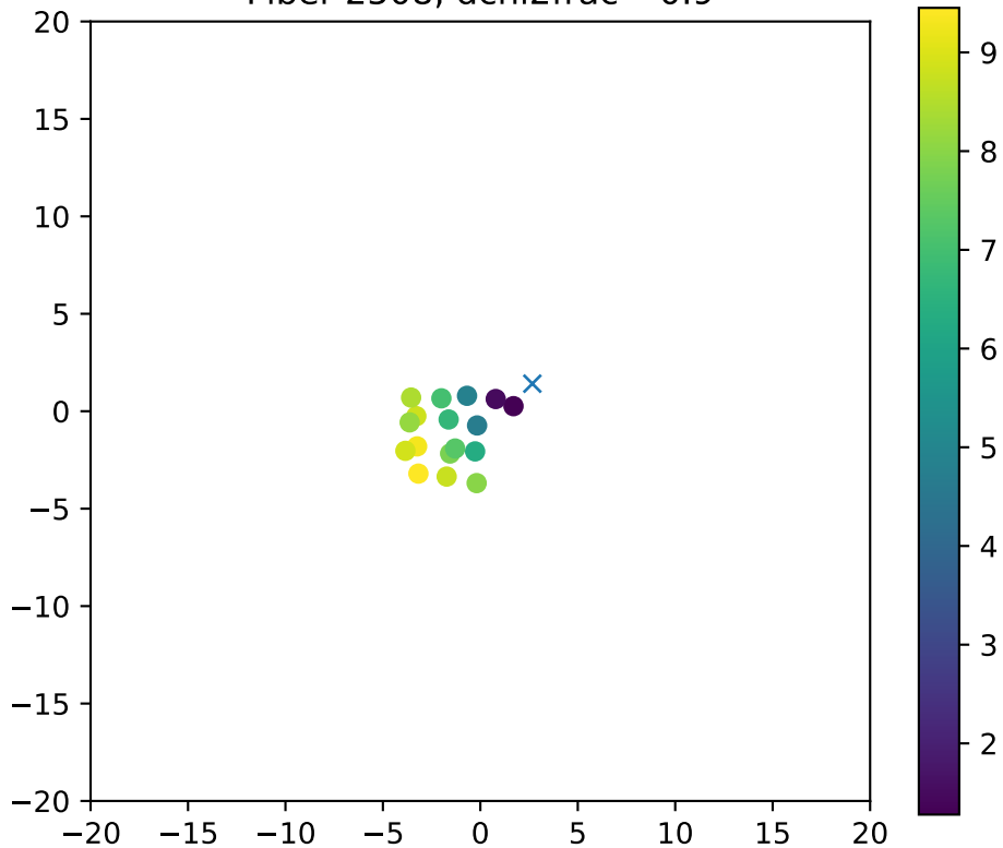
Fiber 2508, dchi2frac= 0.9
