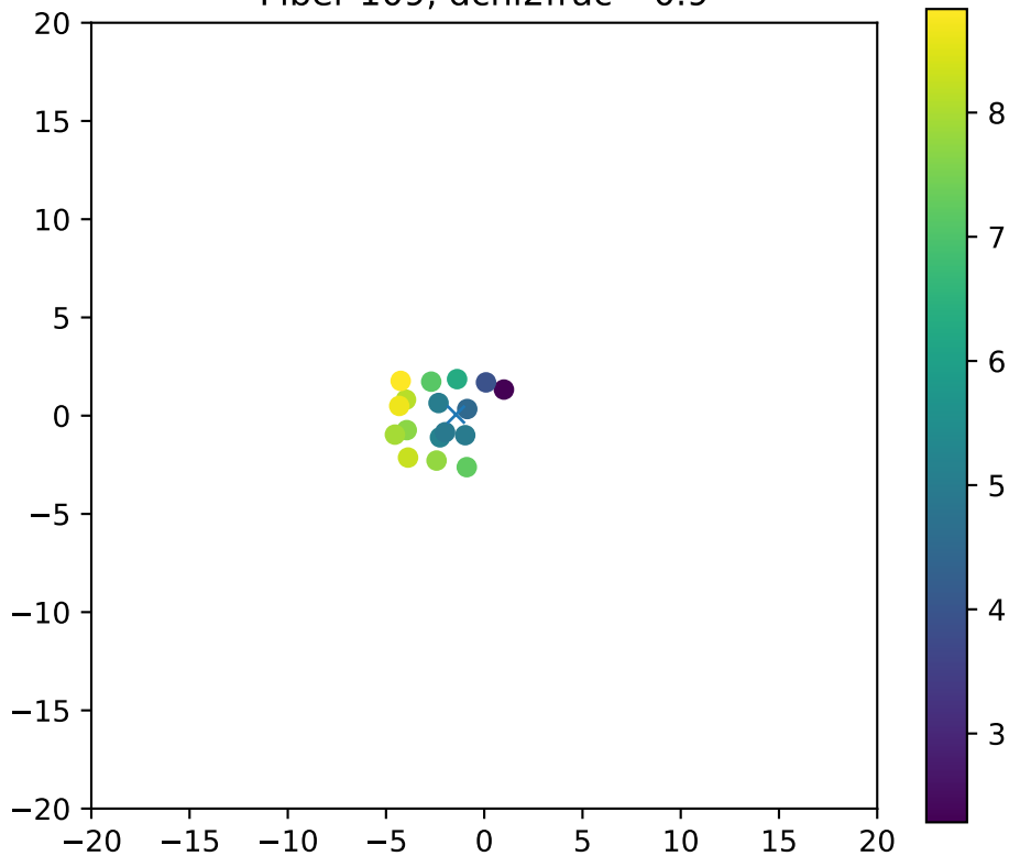
Fiber 109, dchi2frac= 0.9
