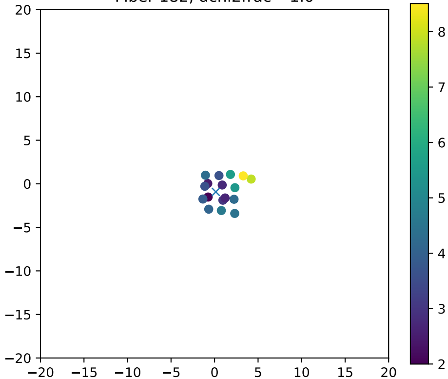
Fiber 182, dchi2frac= 1.0
