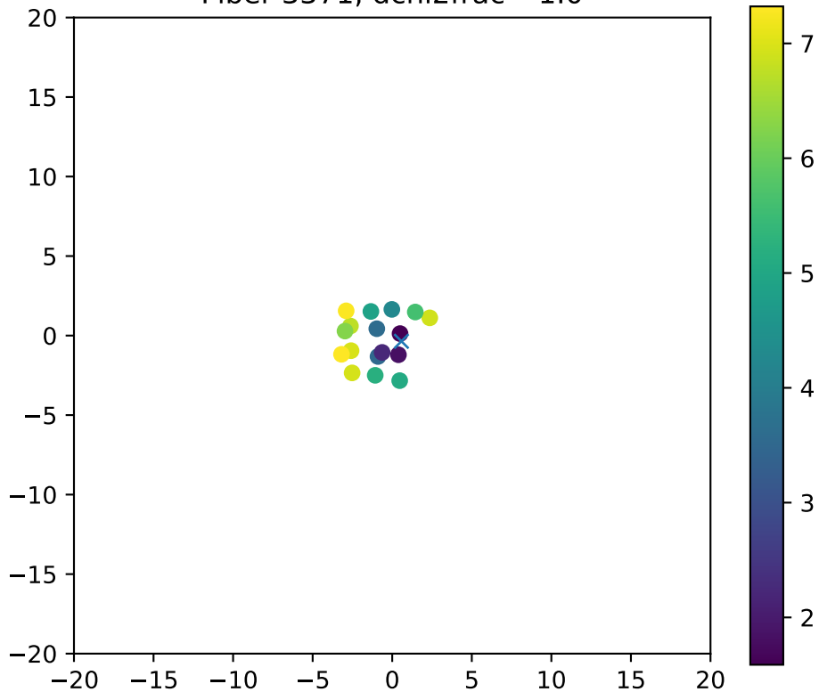
Fiber 3371, dchi2frac= 1.0
