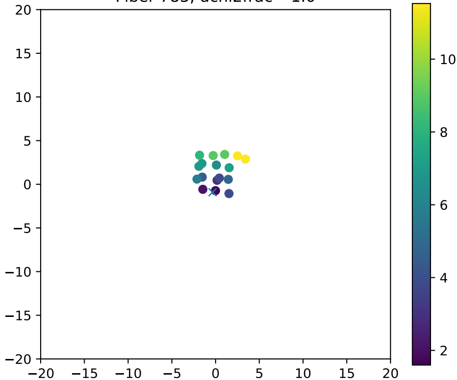
Fiber 783, dchi2frac= 1.0
