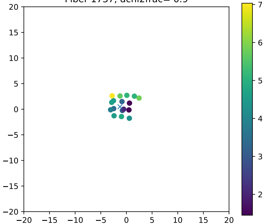
Fiber 1737, dchi2frac= 0.9
