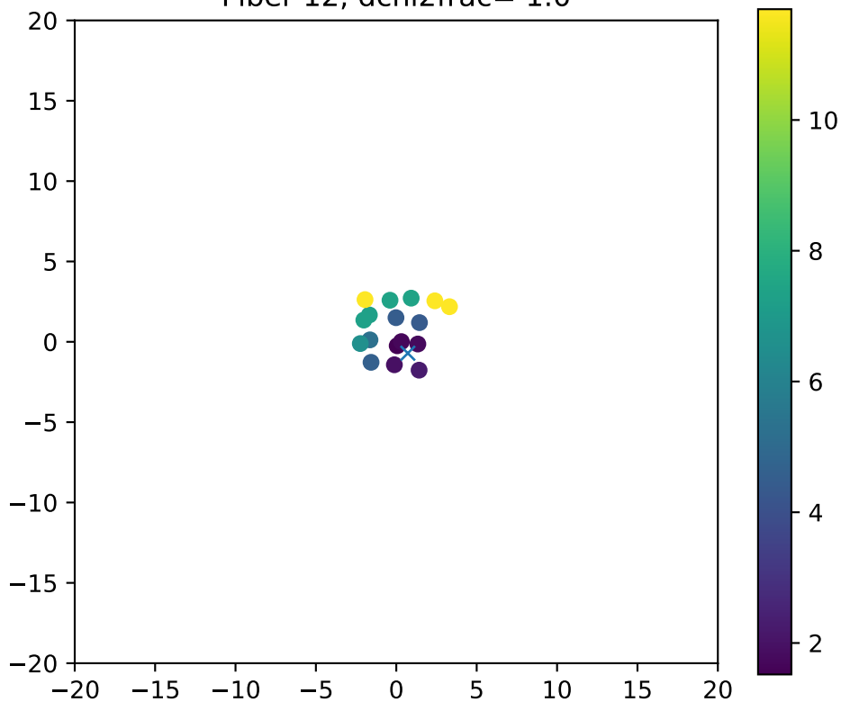
Fiber 12, dchi2frac= 1.0
