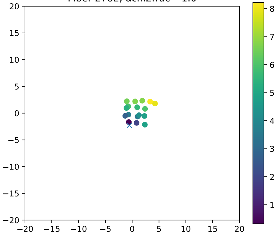
Fiber 2782, dchi2frac= 1.0
