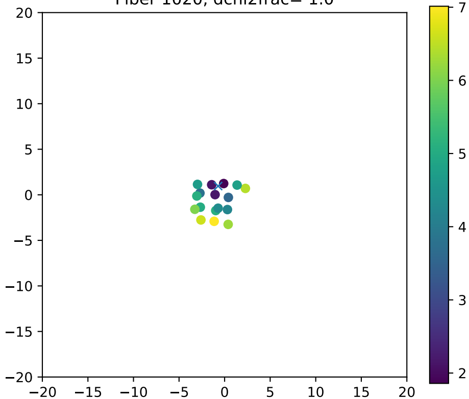
Fiber 1020, dchi2frac= 1.0
