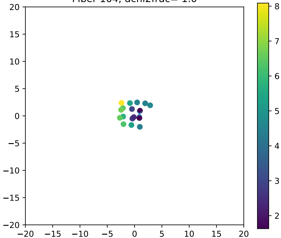
Fiber 104, dchi2frac= 1.0
