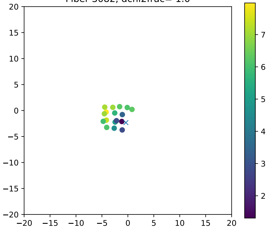
Fiber 3082, dchi2frac= 1.0
