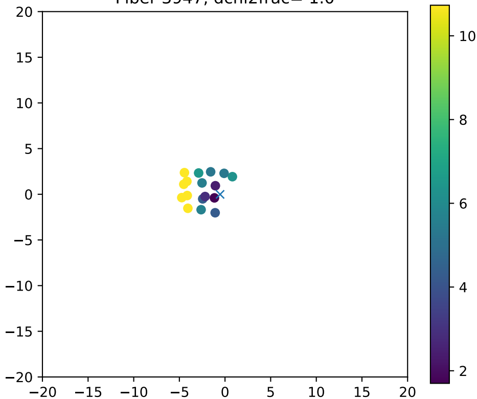
Fiber 3947, dchi2frac= 1.0
