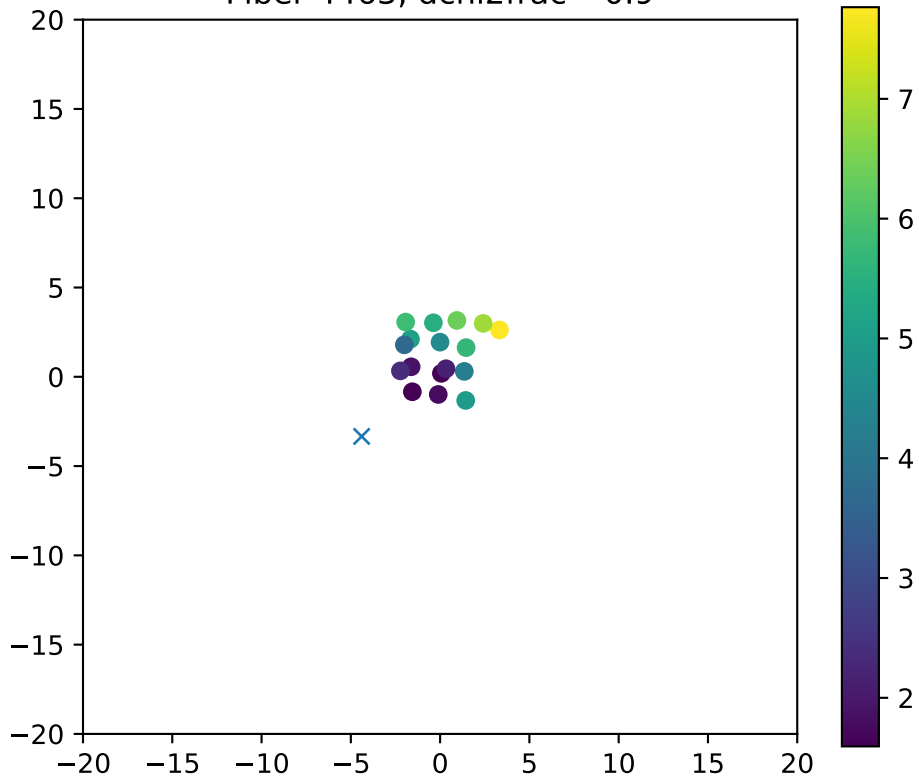
Fiber 4463, dchi2frac= 0.9
