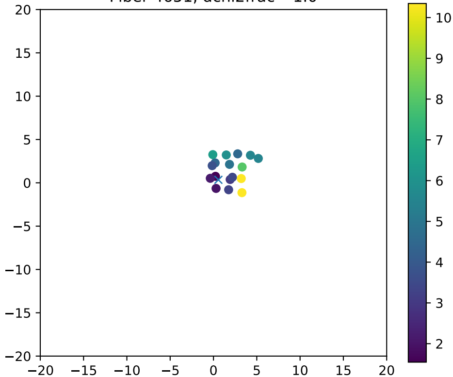
Fiber 4651, dchi2frac= 1.0
