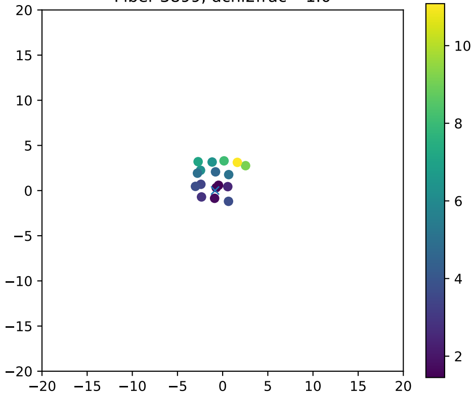
Fiber 3899, dchi2frac= 1.0
