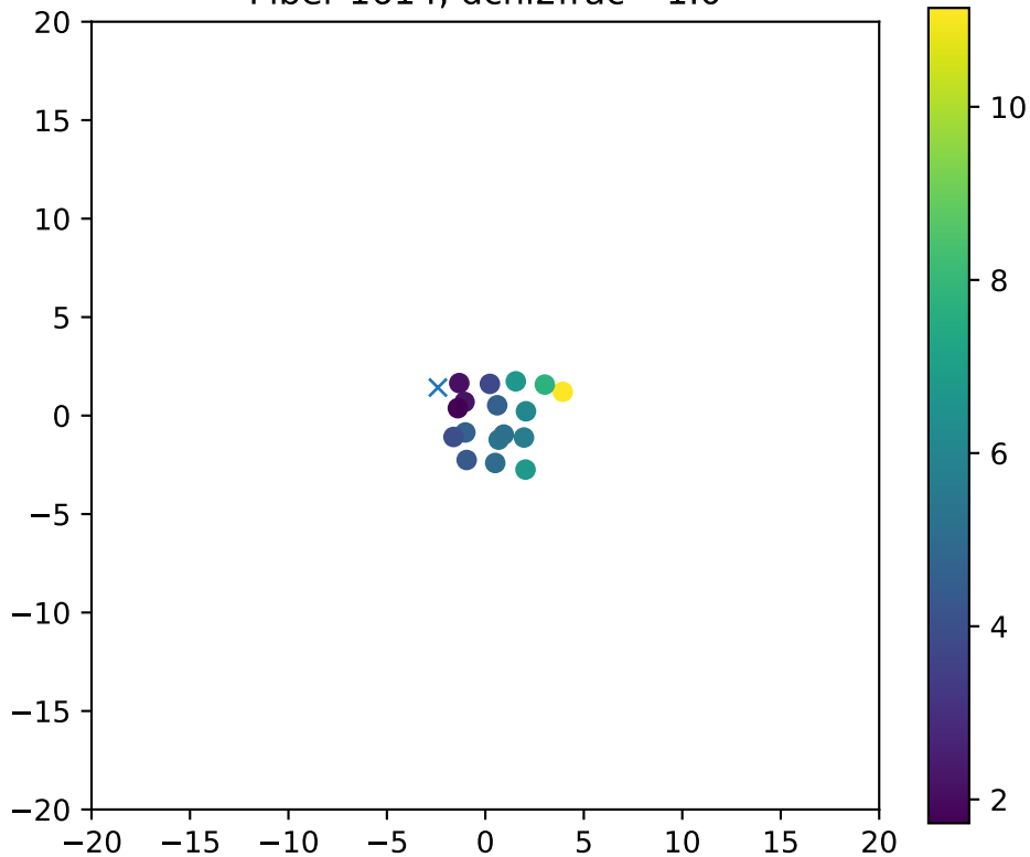
Fiber 1614, dchi2frac= 1.0
