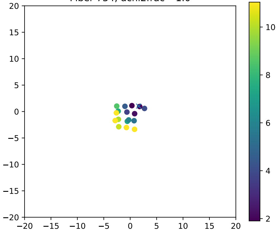
Fiber 734, dchi2frac= 1.0
