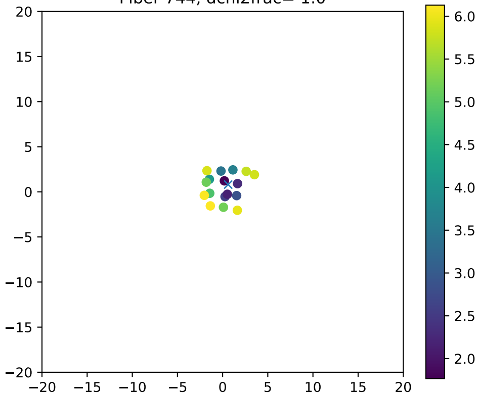
Fiber 744, dchi2frac= 1.0
