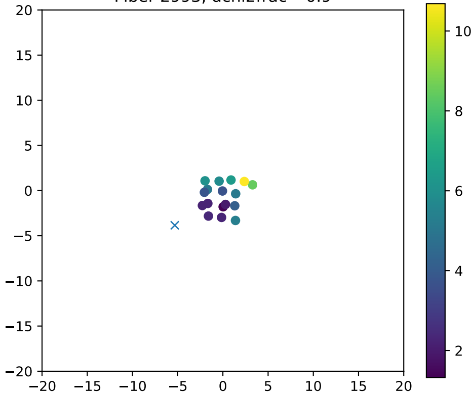
Fiber 2993, dchi2frac= 0.9
