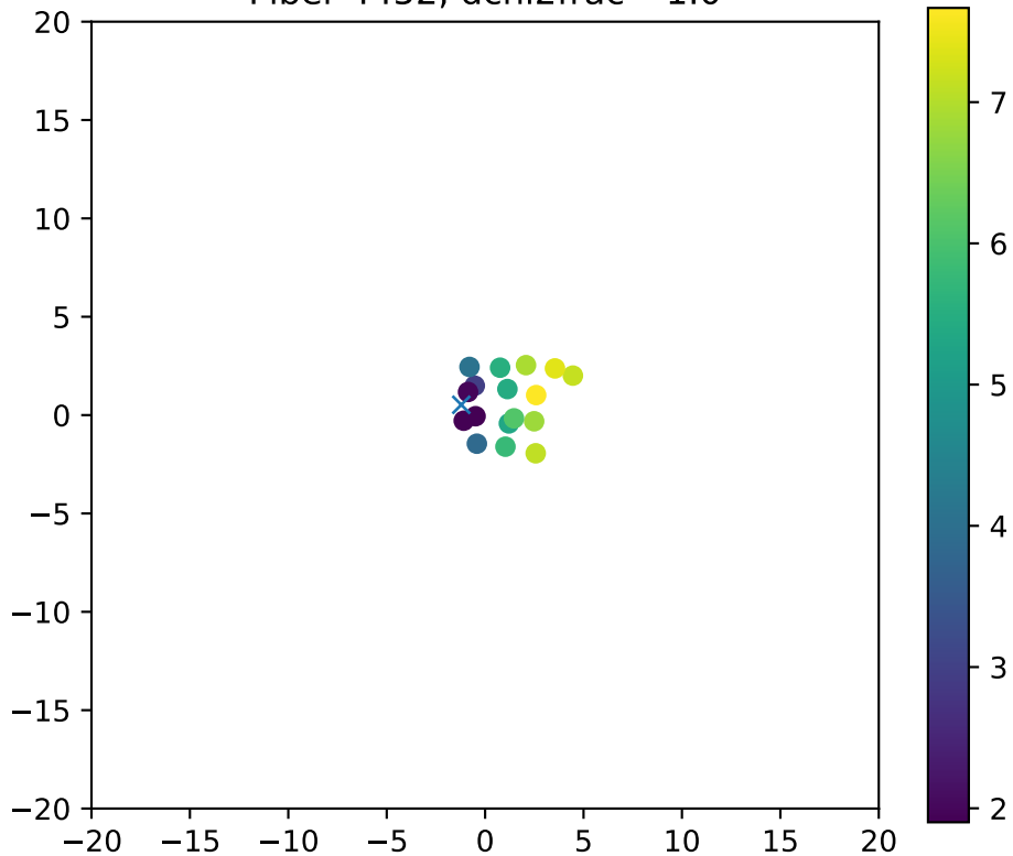
Fiber 4452, dchi2frac= 1.0
