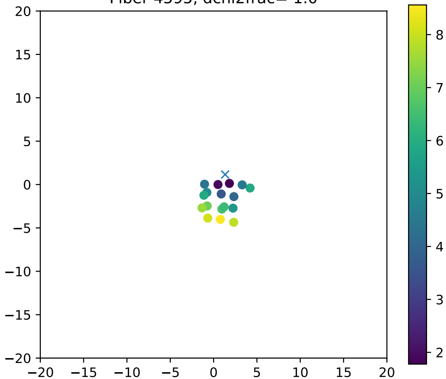
Fiber 4595, dchi2frac= 1.0
