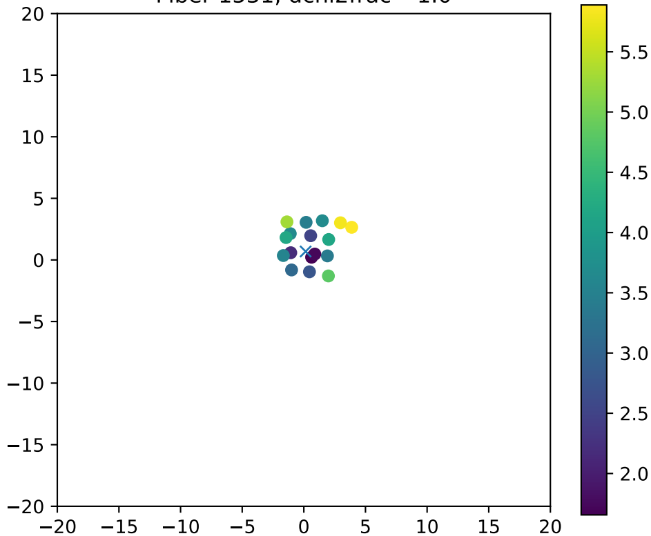
Fiber 1531, dchi2frac= 1.0
