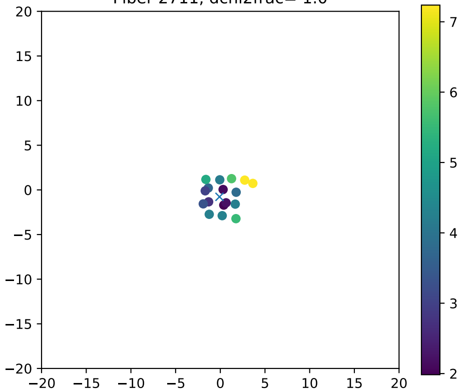
Fiber 2711, dchi2frac= 1.0
