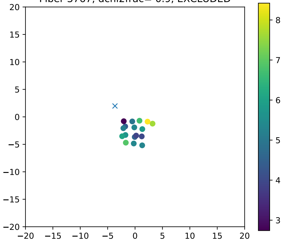
Fiber 3767, dchi2frac= 0.9, EXCLUDED
