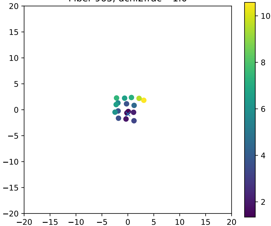
Fiber 963, dchi2frac= 1.0
