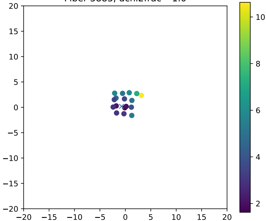
Fiber 3883, dchi2frac= 1.0
