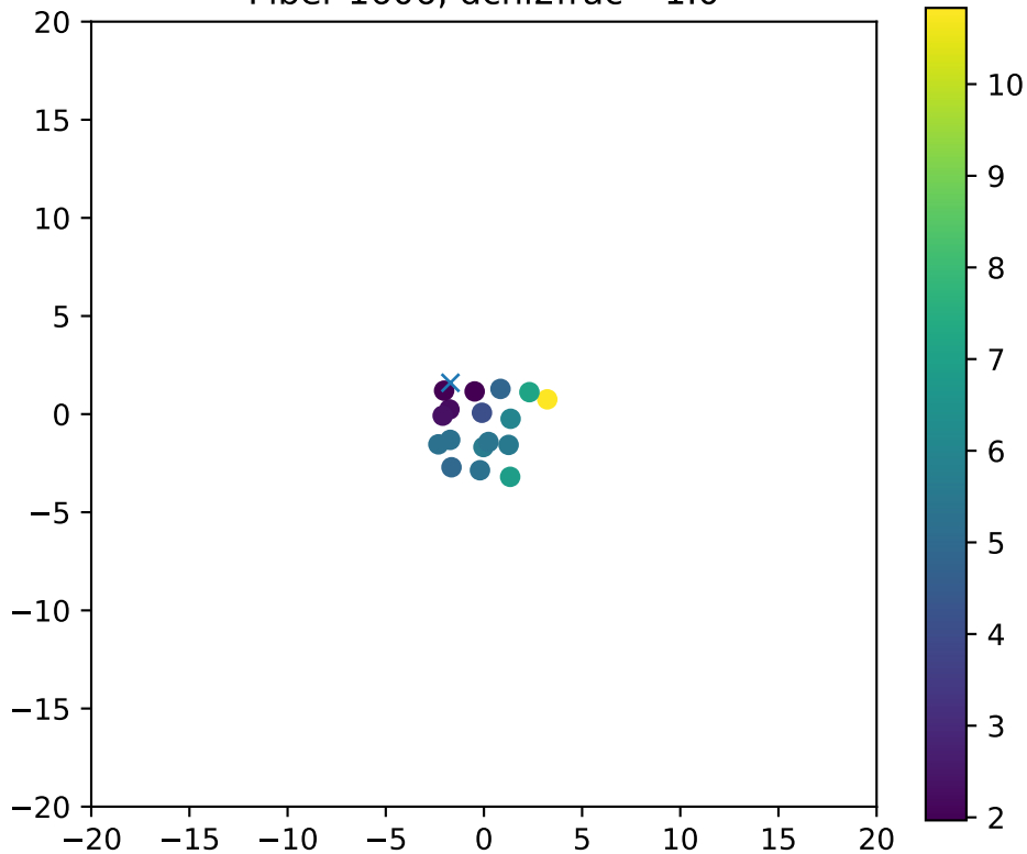
Fiber 1606, dchi2frac= 1.0
