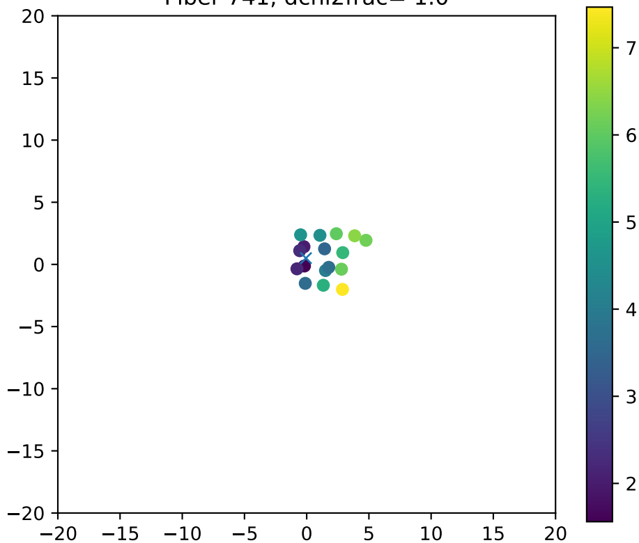
Fiber 741, dchi2frac= 1.0
