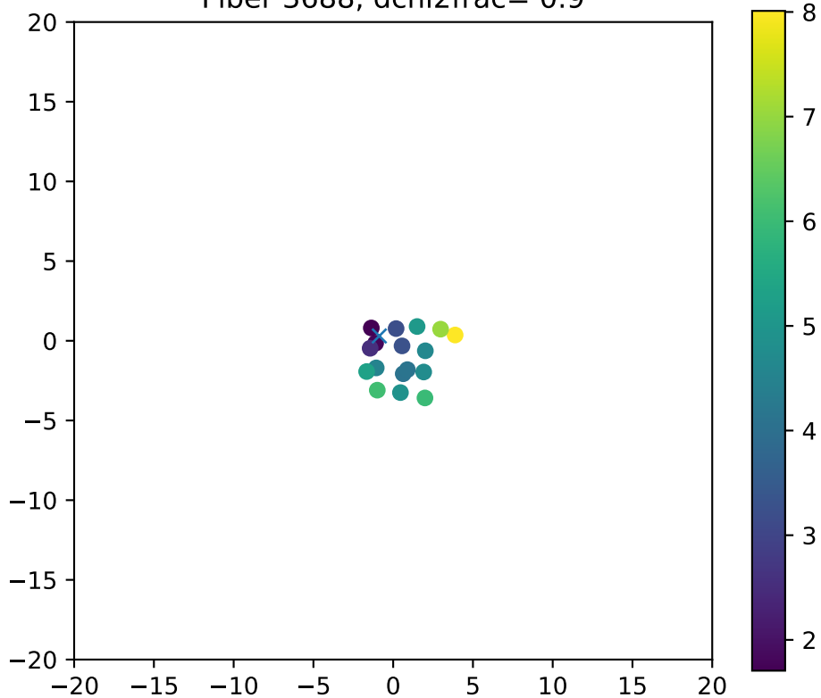
Fiber 3688, dchi2frac= 0.9
