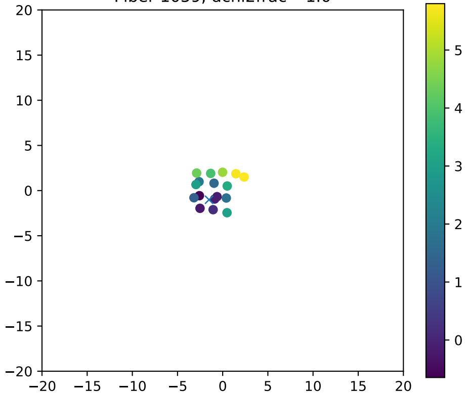
Fiber 1059, dchi2frac= 1.0
