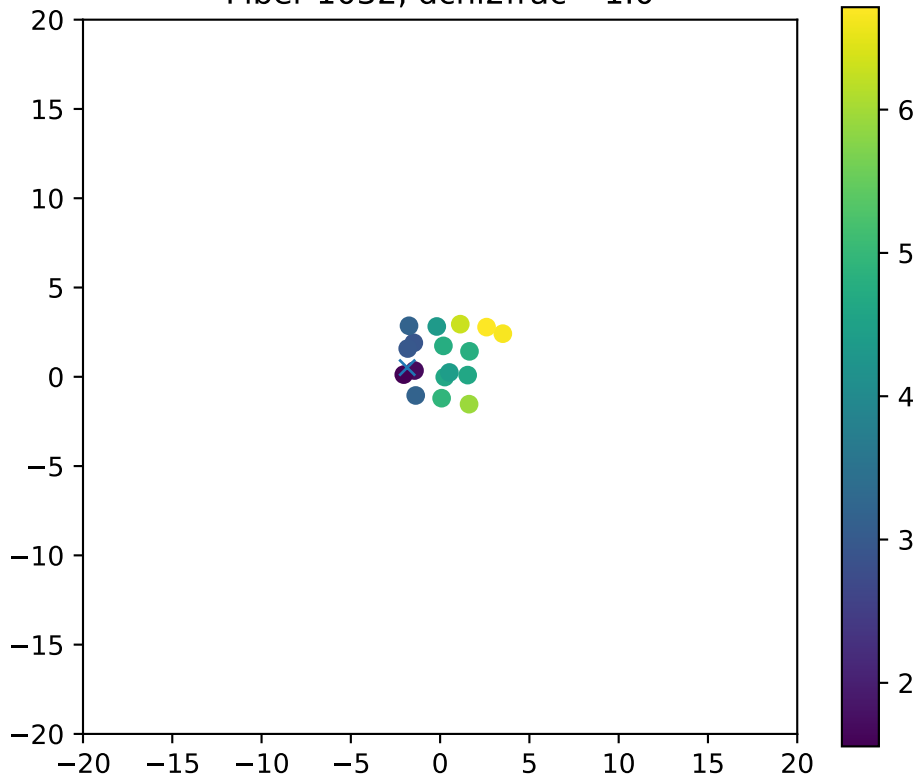
Fiber 1032, dchi2frac= 1.0
