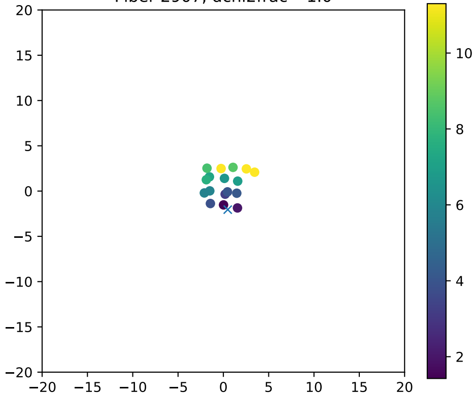
Fiber 2907, dchi2frac= 1.0
