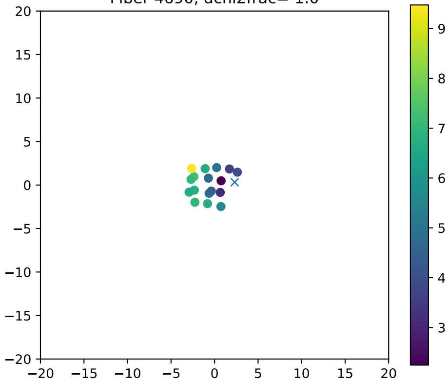
Fiber 4690, dchi2frac= 1.0
