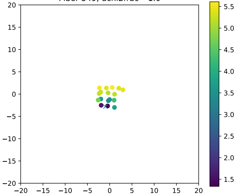
Fiber 549, dchi2frac= 1.0
