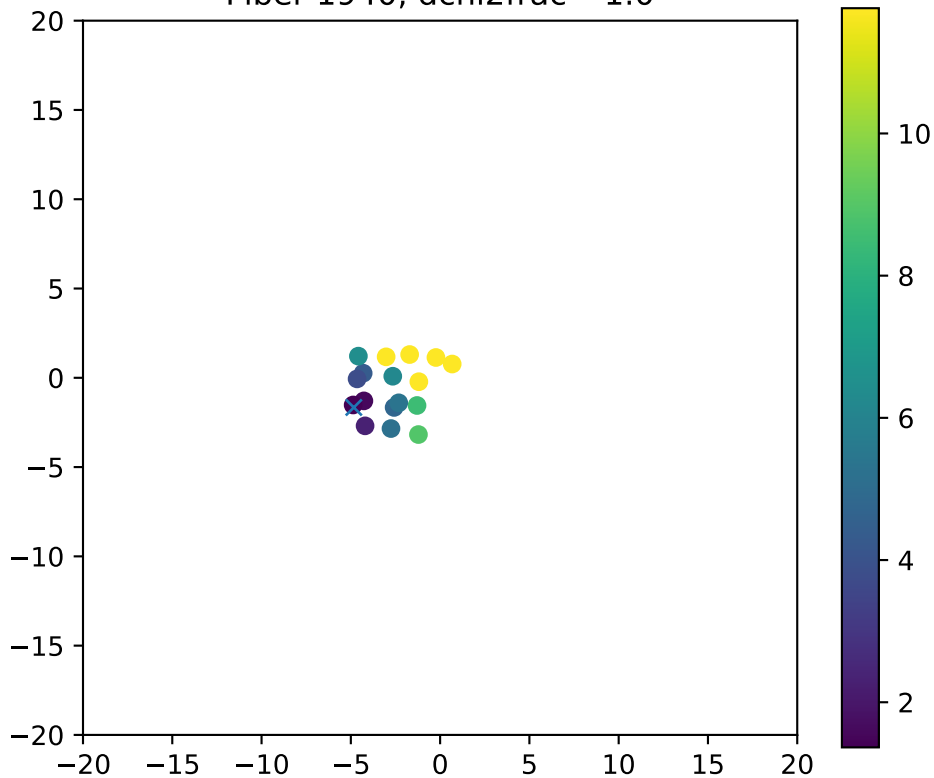
Fiber 1940, dchi2frac= 1.0
