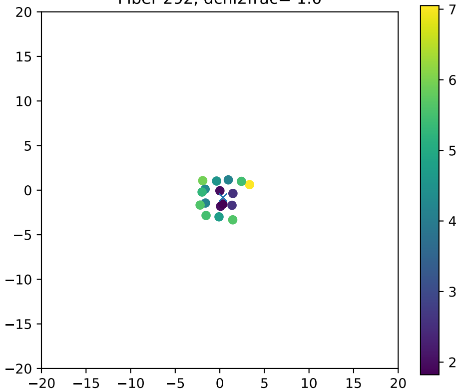
Fiber 292, dchi2frac= 1.0
