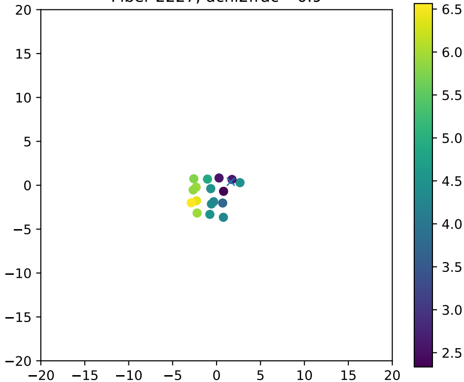
Fiber 2227, dchi2frac= 0.9
