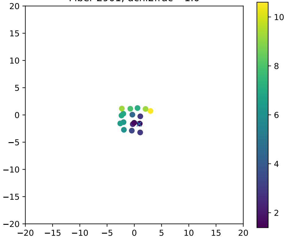
Fiber 2901, dchi2frac= 1.0
