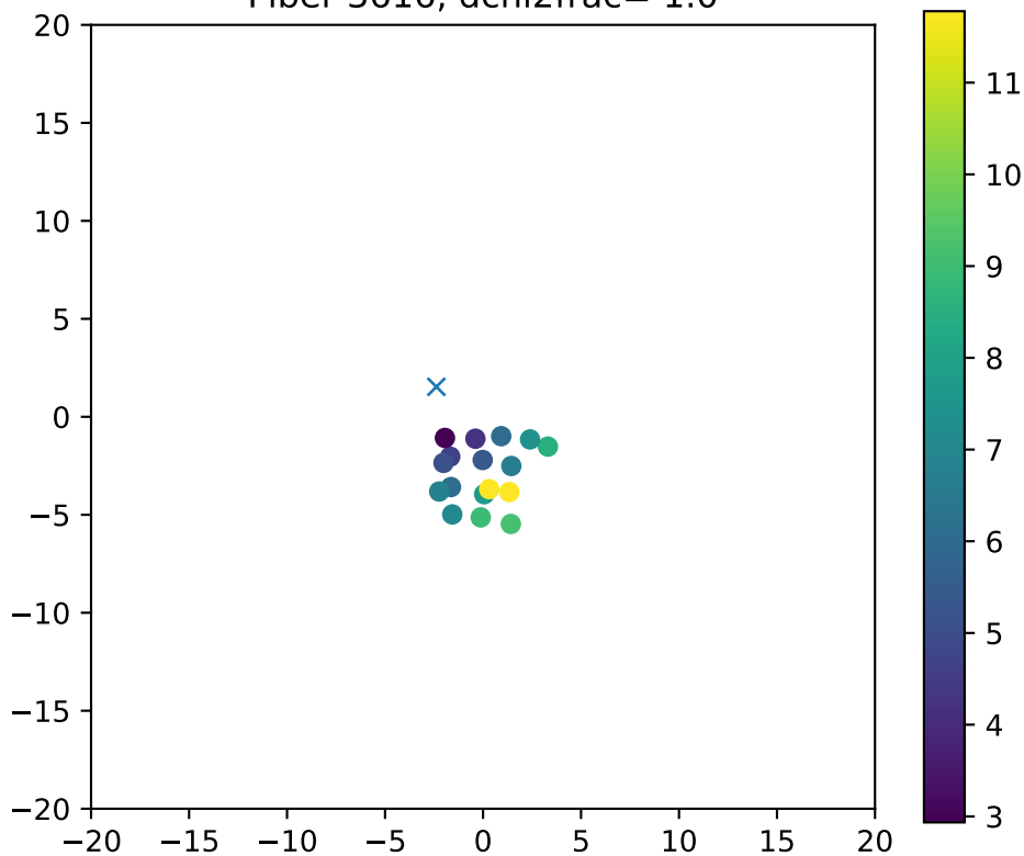
Fiber 3616, dchi2frac= 1.0
