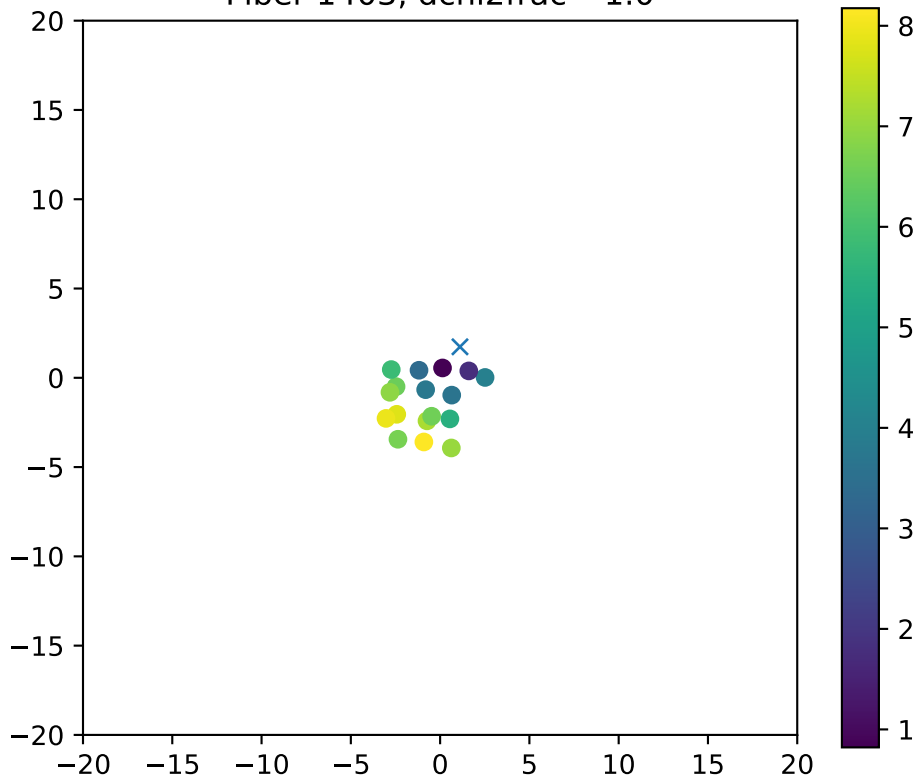
Fiber 1403, dchi2frac= 1.0
