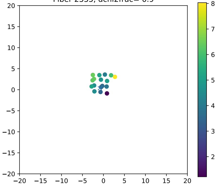
Fiber 2335, dchi2frac= 0.9
