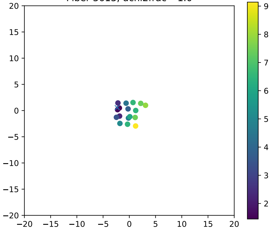
Fiber 3613, dchi2frac= 1.0
