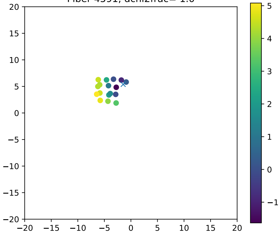
Fiber 4591, dchi2frac= 1.0
