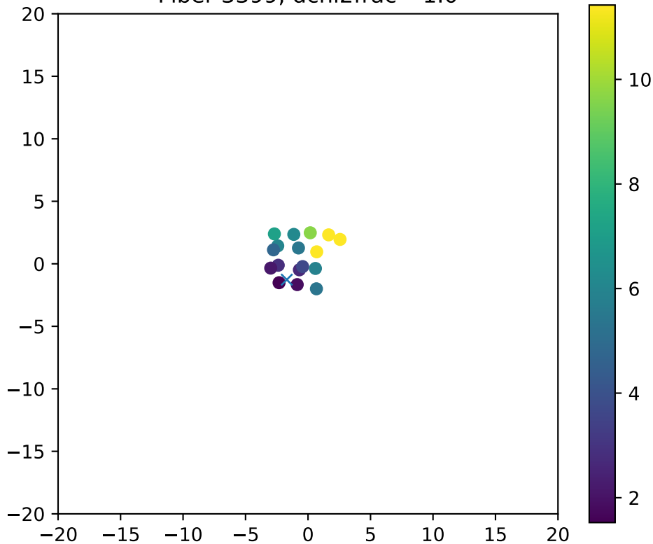
Fiber 3399, dchi2frac= 1.0
