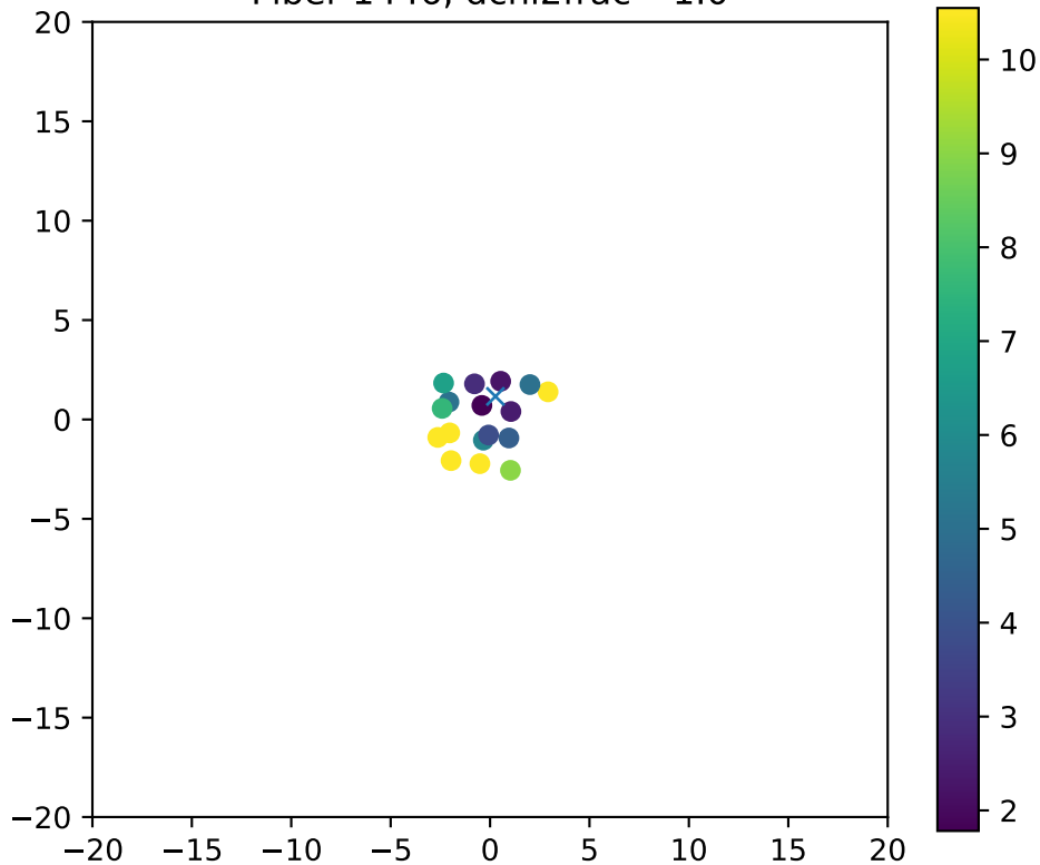
Fiber 1446, dchi2frac= 1.0
