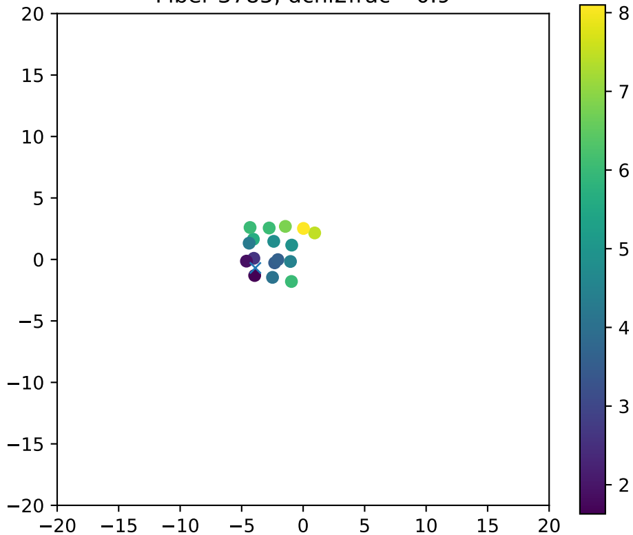
Fiber 3785, dchi2frac= 0.9
