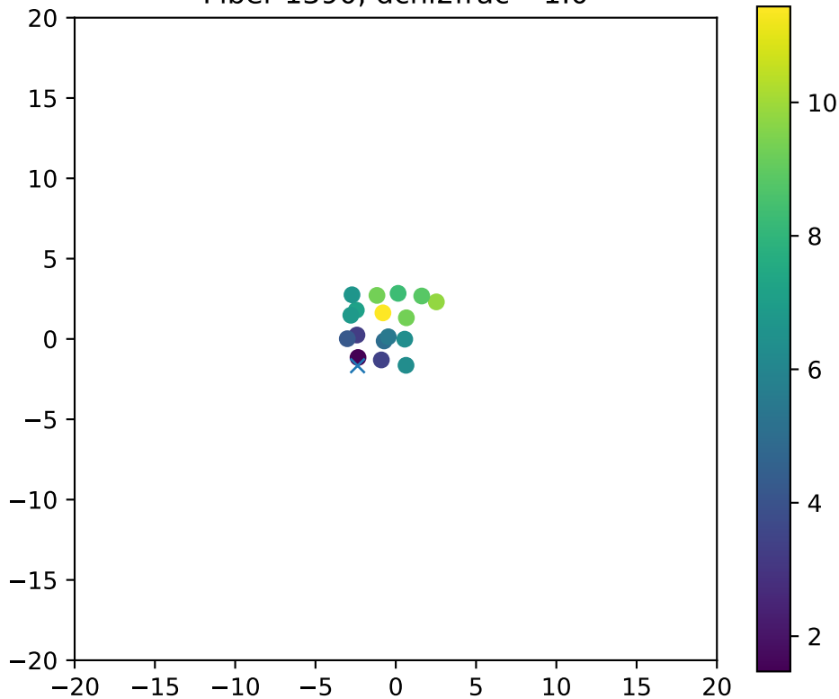
Fiber 1390, dchi2frac= 1.0
