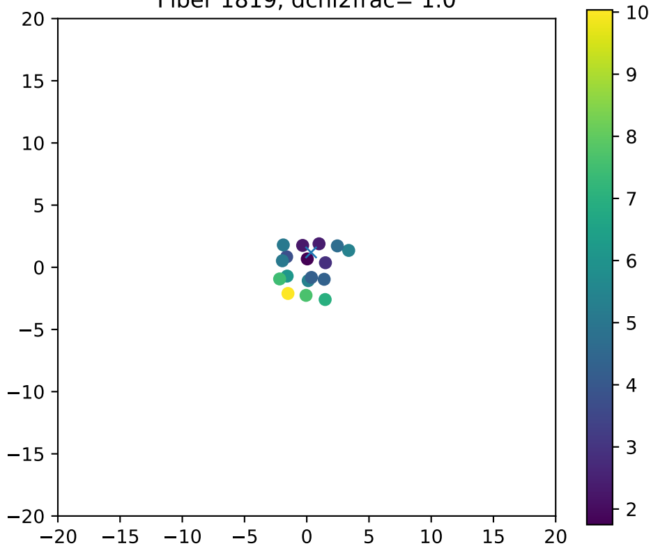
Fiber 1819, dchi2frac= 1.0
