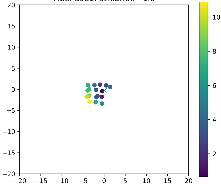
Fiber 3981, dchi2frac= 1.0
