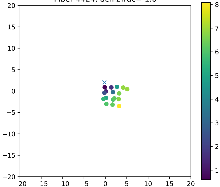
Fiber 4424, dchi2frac= 1.0
