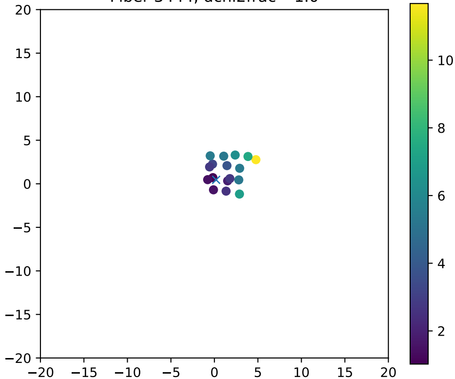
Fiber 3444, dchi2frac= 1.0
