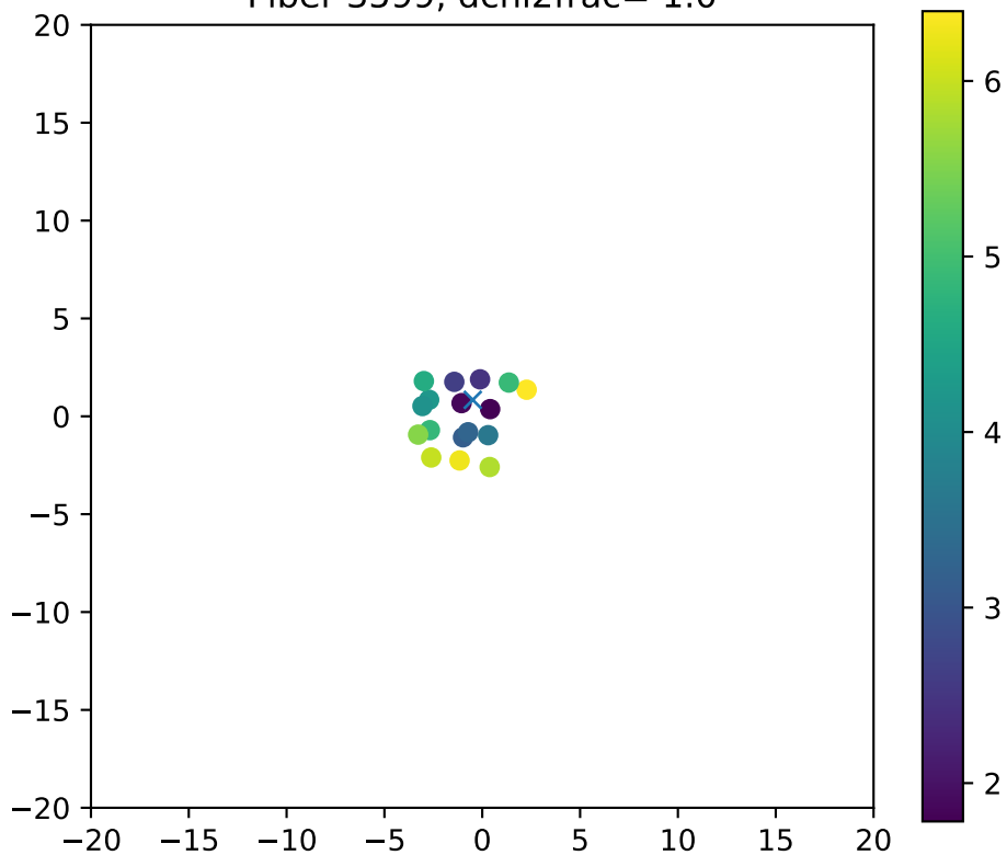
Fiber 3599, dchi2frac= 1.0
