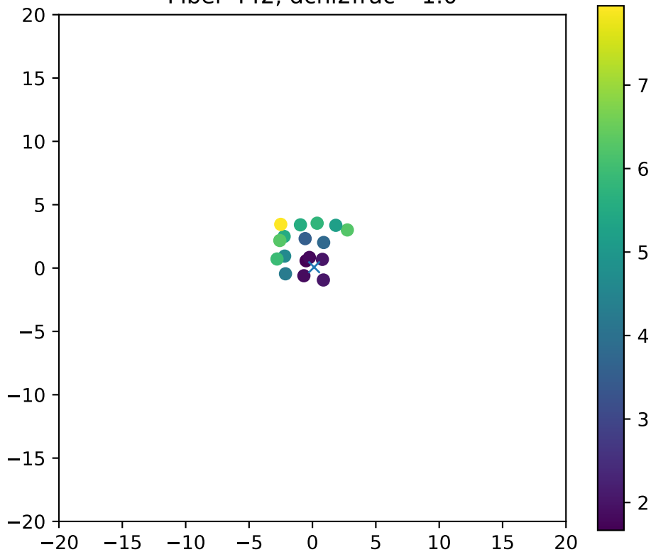
Fiber 442, dchi2frac= 1.0
