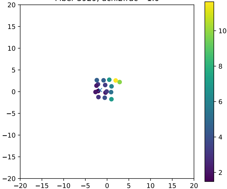
Fiber 3929, dchi2frac= 1.0
