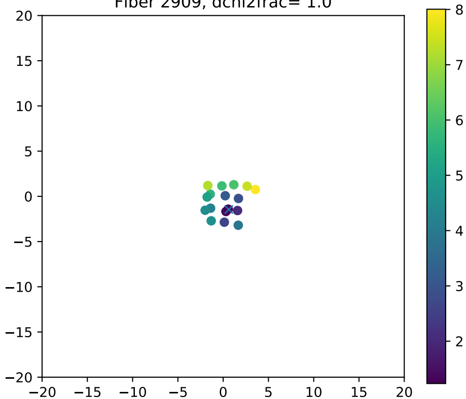
Fiber 2909, dchi2frac= 1.0
