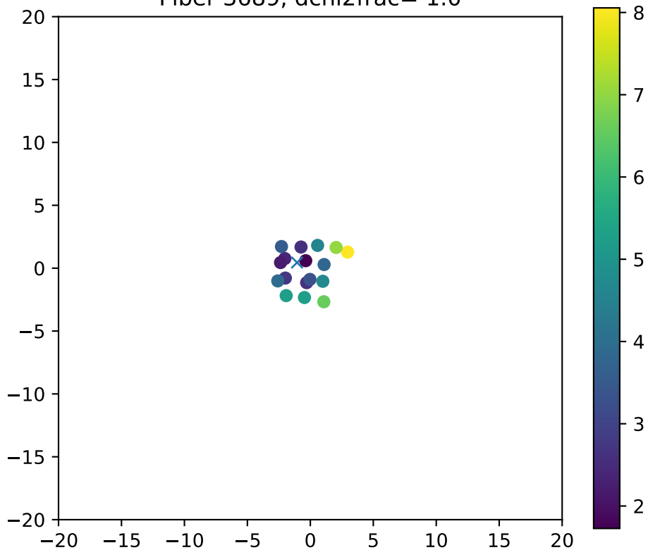
Fiber 3689, dchi2frac= 1.0
