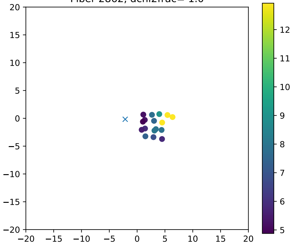
Fiber 2862, dchi2frac= 1.0
