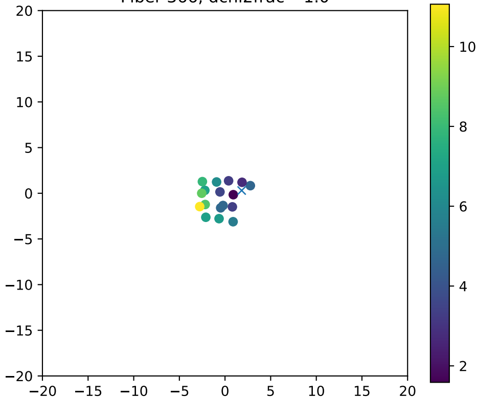
Fiber 366, dchi2frac= 1.0
