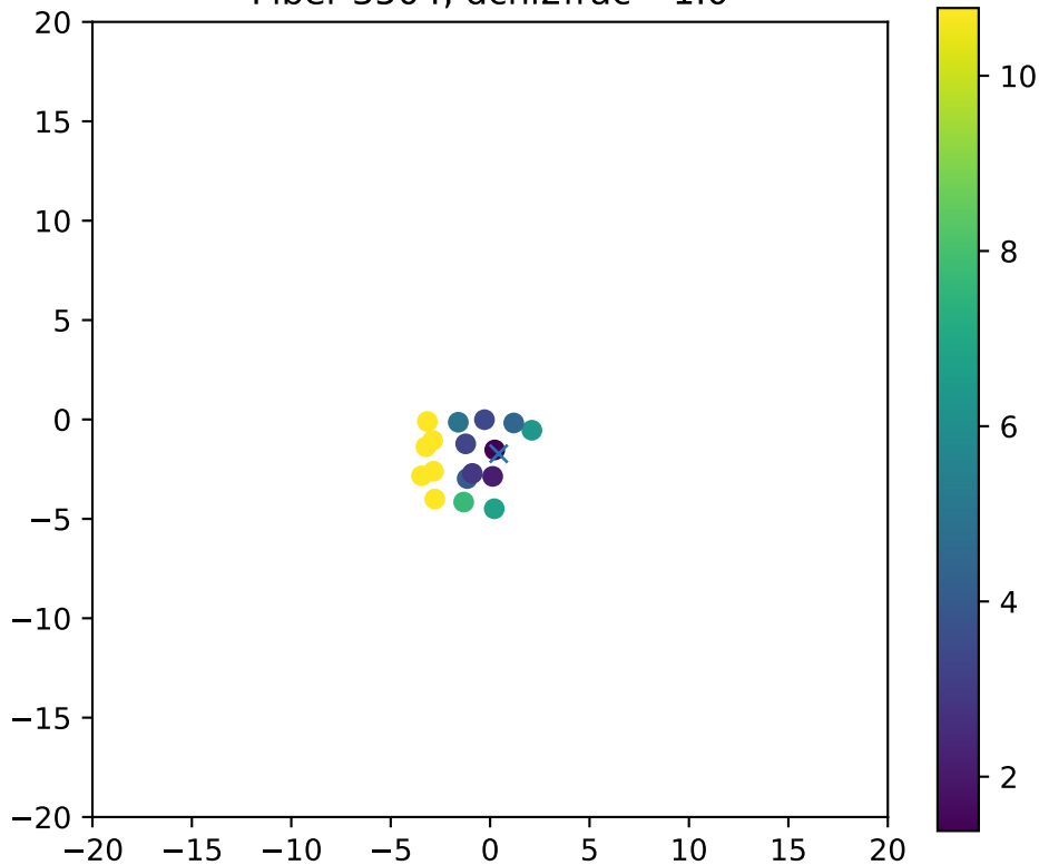
Fiber 3504, dchi2frac= 1.0
