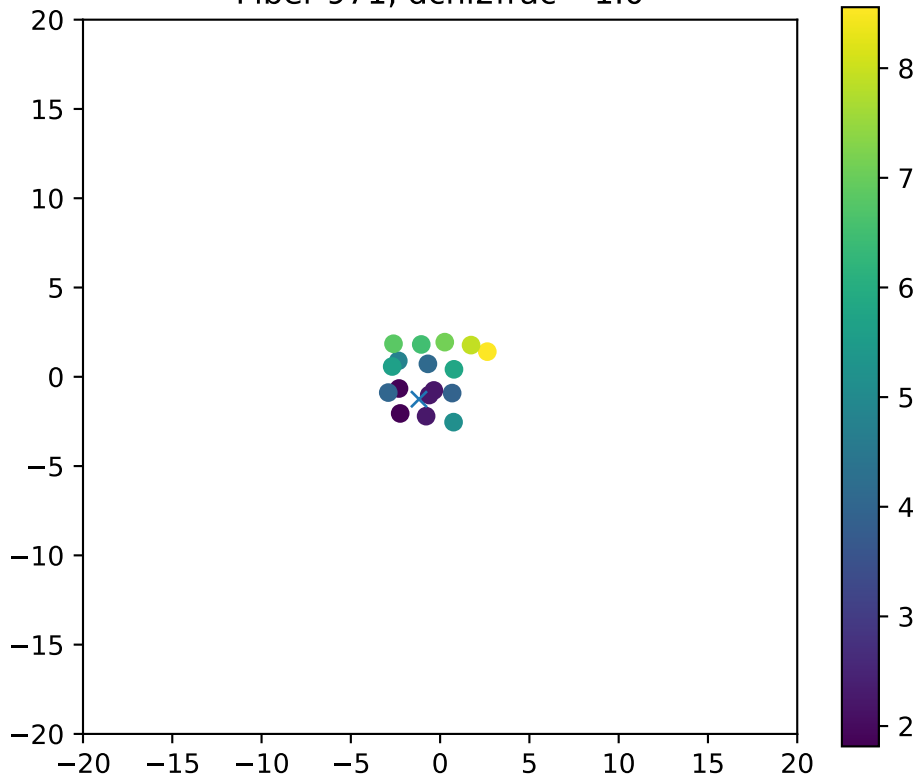
Fiber 971, dchi2frac= 1.0
