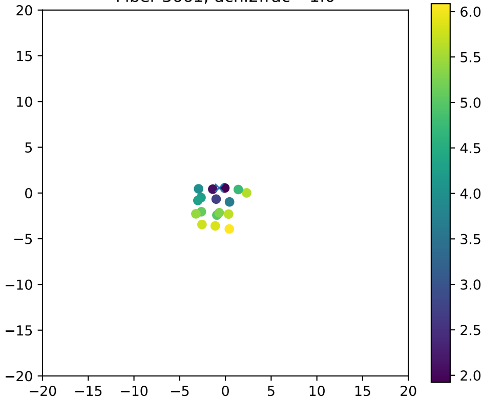
Fiber 3661, dchi2frac= 1.0
