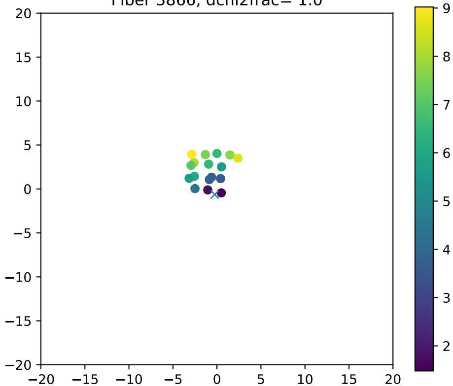
Fiber 3866, dchi2frac= 1.0
