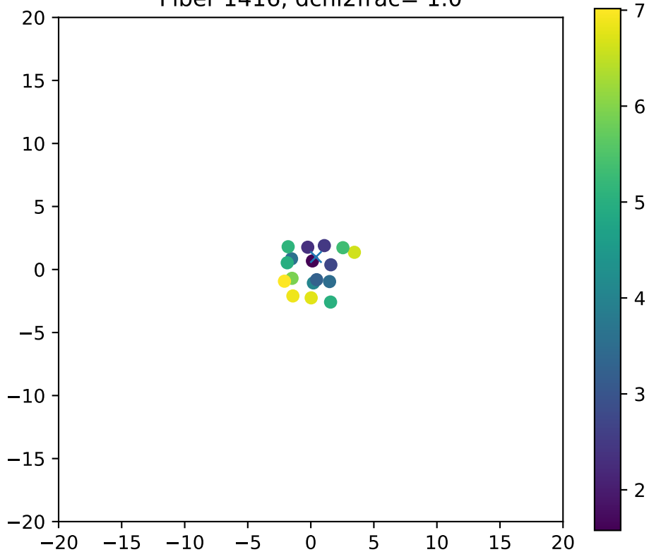
Fiber 1416, dchi2frac= 1.0
