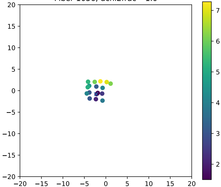
Fiber 1056, dchi2frac= 1.0
