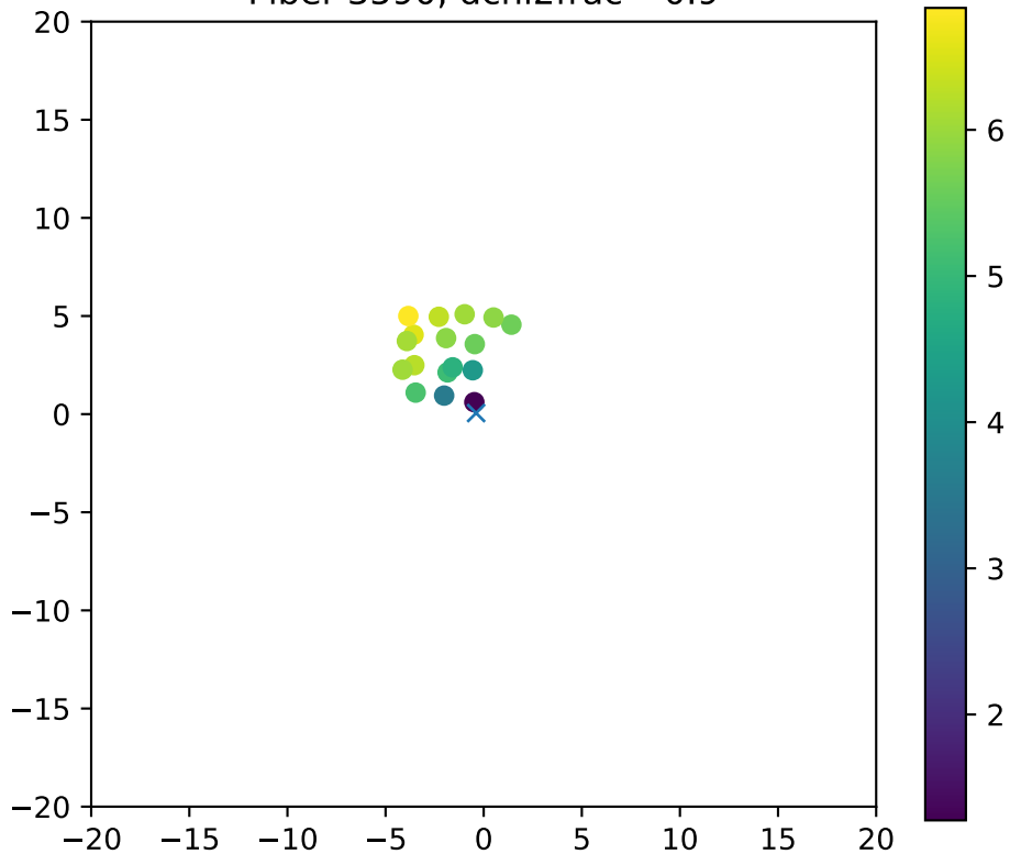
Fiber 3590, dchi2frac= 0.9
