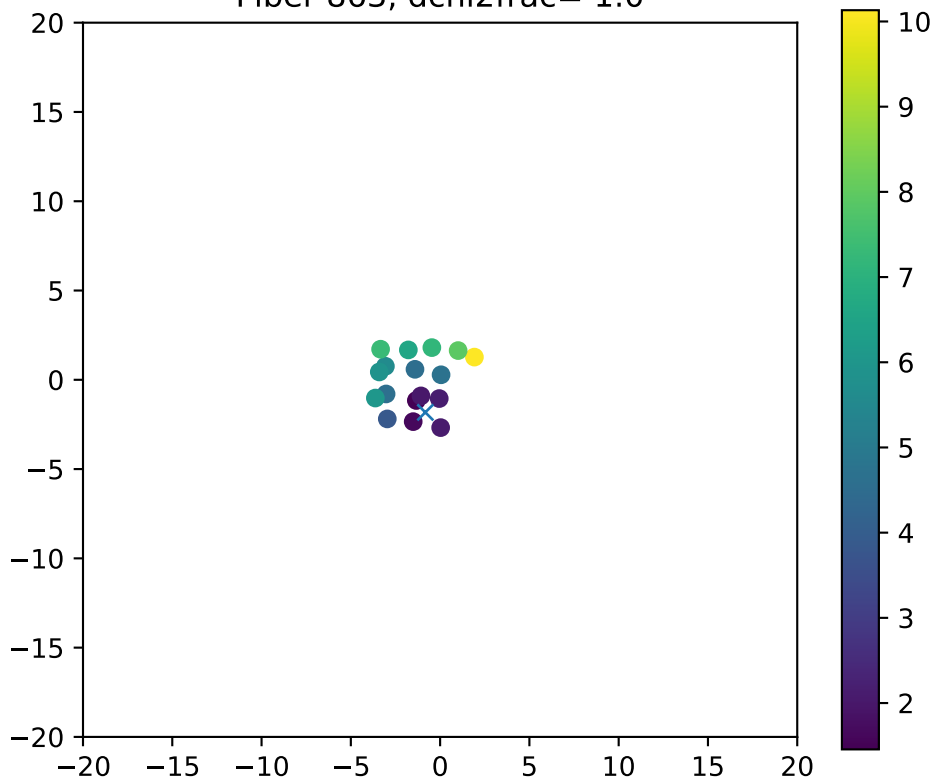
Fiber 863, dchi2frac= 1.0
