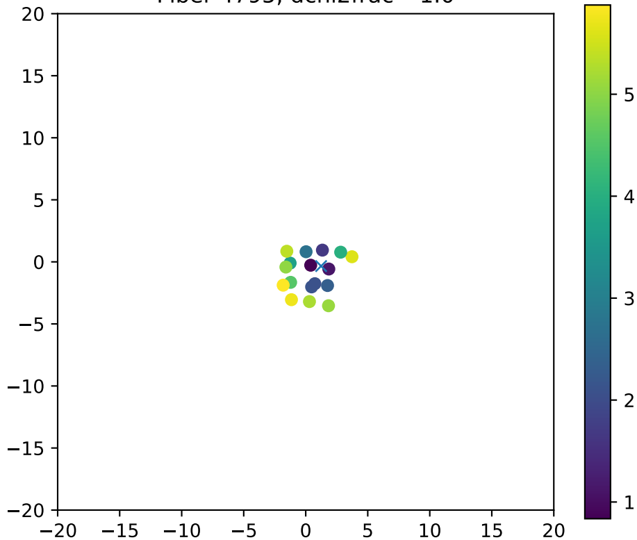
Fiber 4795, dchi2frac= 1.0
