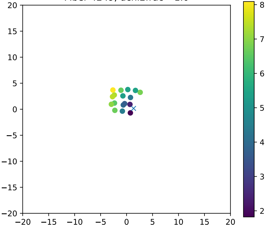
Fiber 4249, dchi2frac= 1.0
