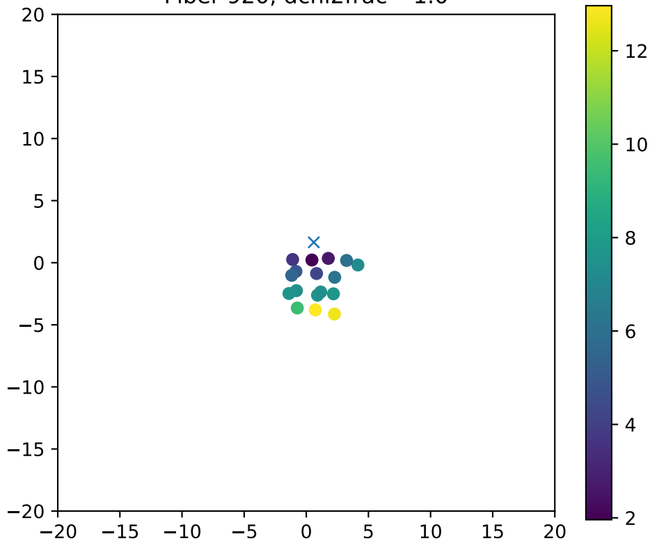
Fiber 920, dchi2frac= 1.0
