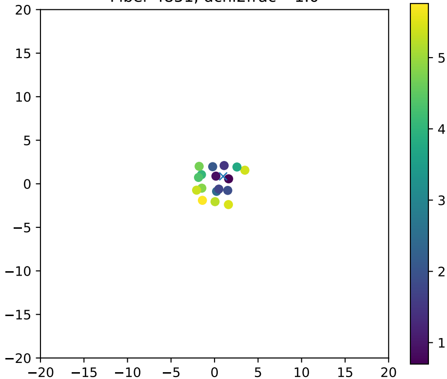
Fiber 4851, dchi2frac= 1.0
