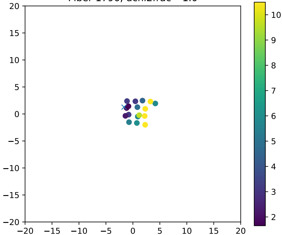
Fiber 1796, dchi2frac= 1.0
