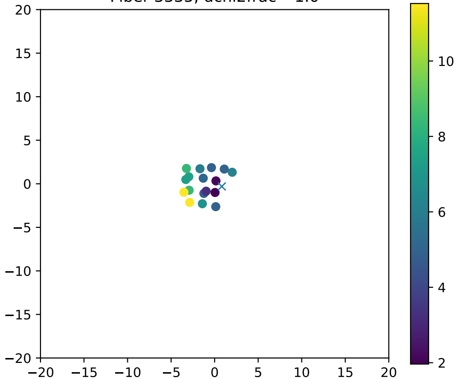
Fiber 3335, dchi2frac= 1.0
