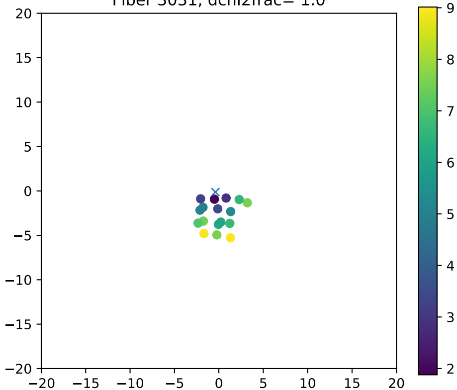
Fiber 3031, dchi2frac= 1.0
