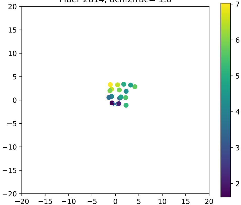
Fiber 2614, dchi2frac= 1.0
