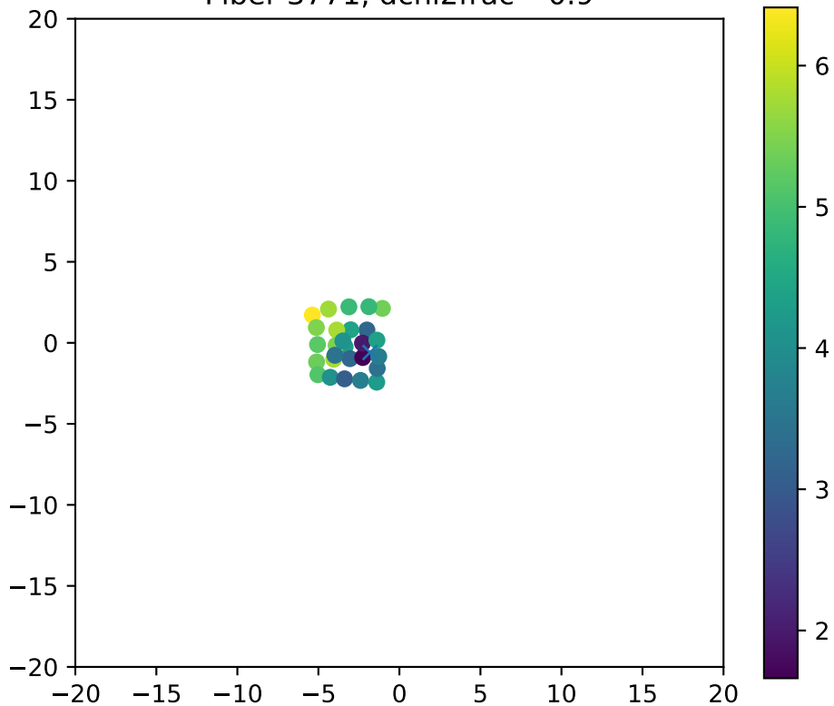
Fiber 3771, dchi2frac= 0.9
