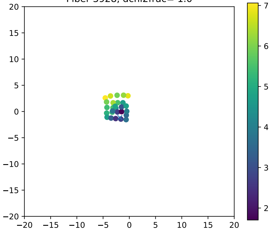
Fiber 3928, dchi2frac= 1.0
