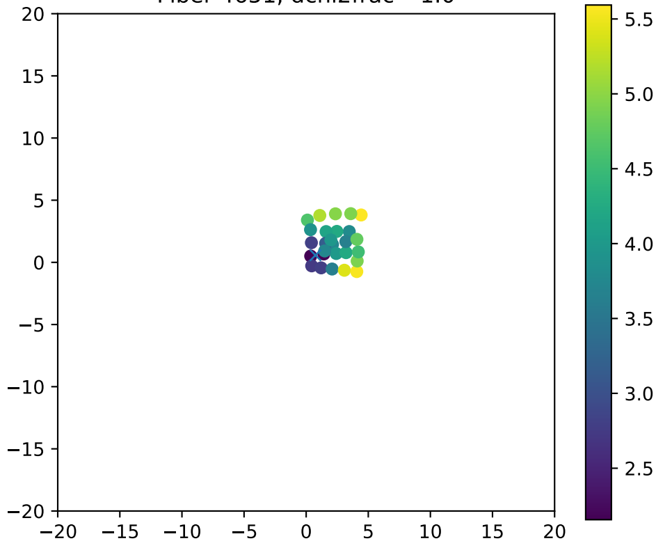
Fiber 4651, dchi2frac= 1.0
