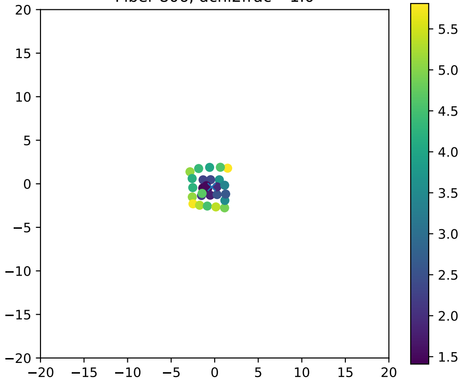
Fiber 806, dchi2frac= 1.0
