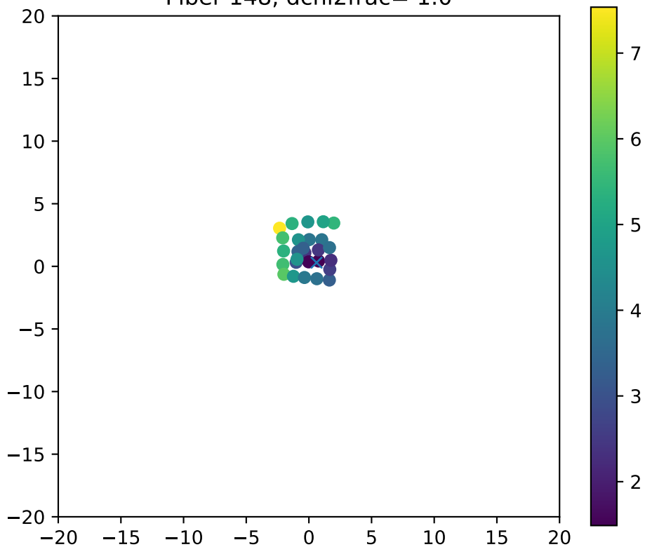
Fiber 148, dchi2frac= 1.0
