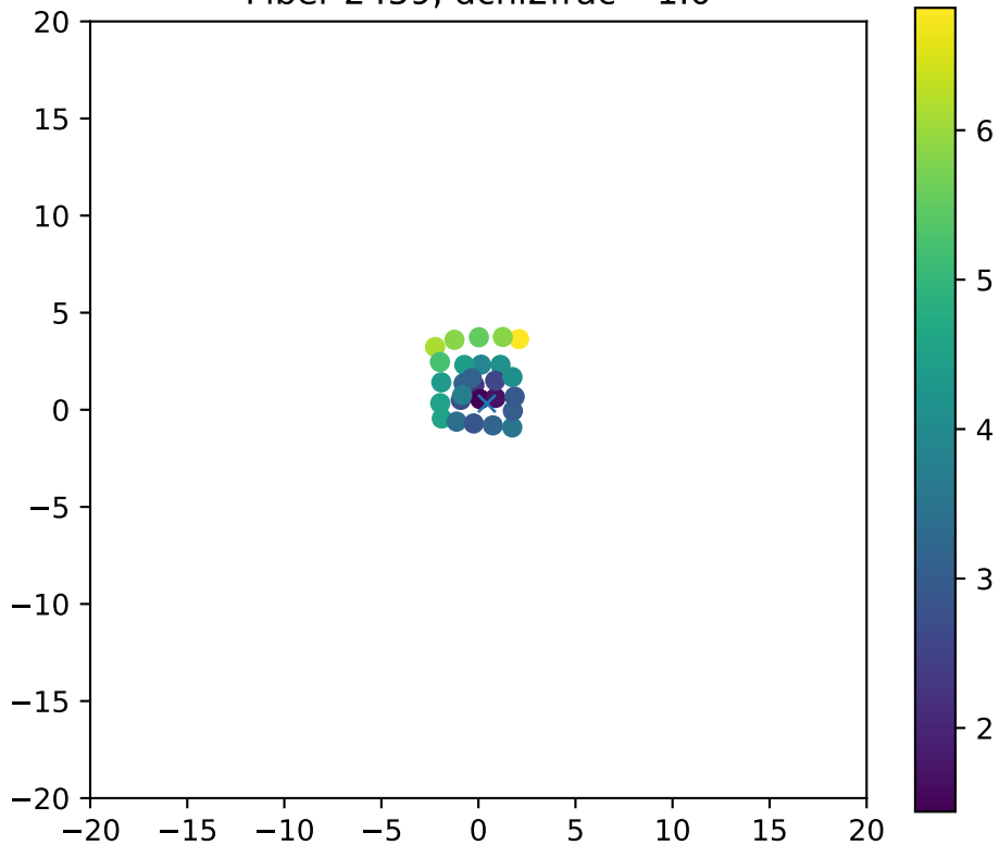
Fiber 2459, dchi2frac= 1.0
