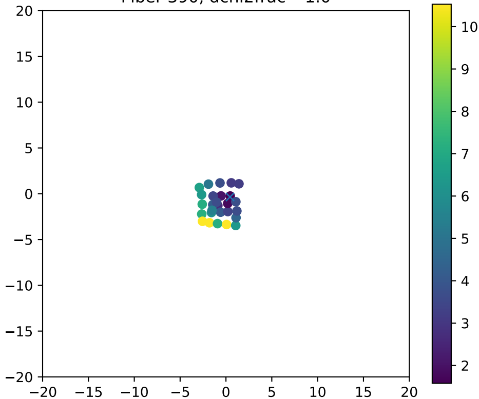
Fiber 390, dchi2frac= 1.0
