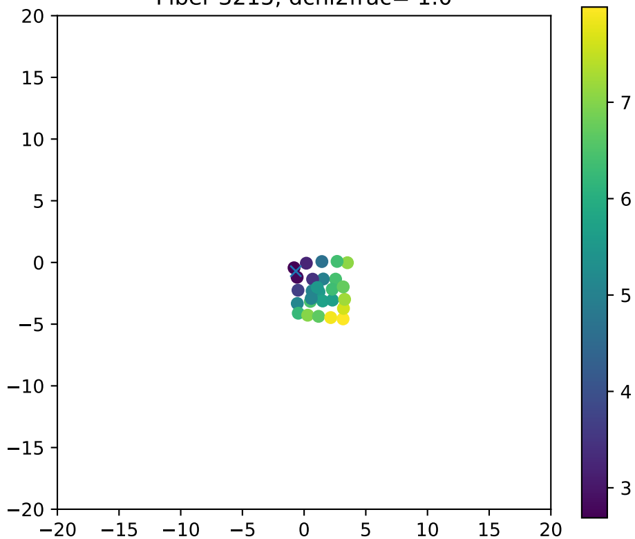
Fiber 3215, dchi2frac= 1.0
