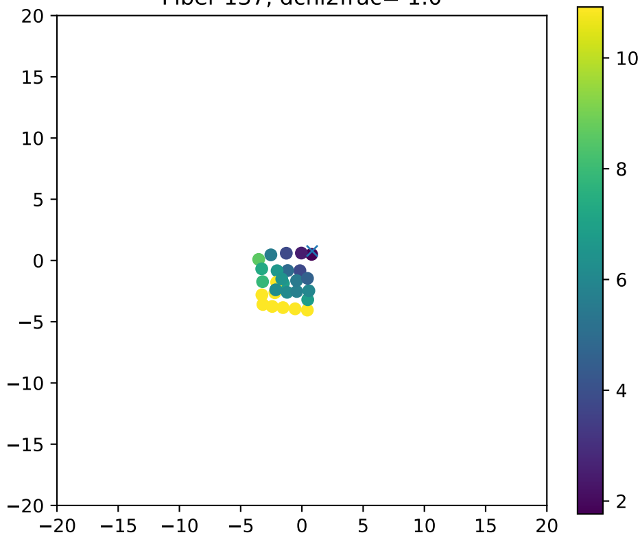
Fiber 137, dchi2frac= 1.0
