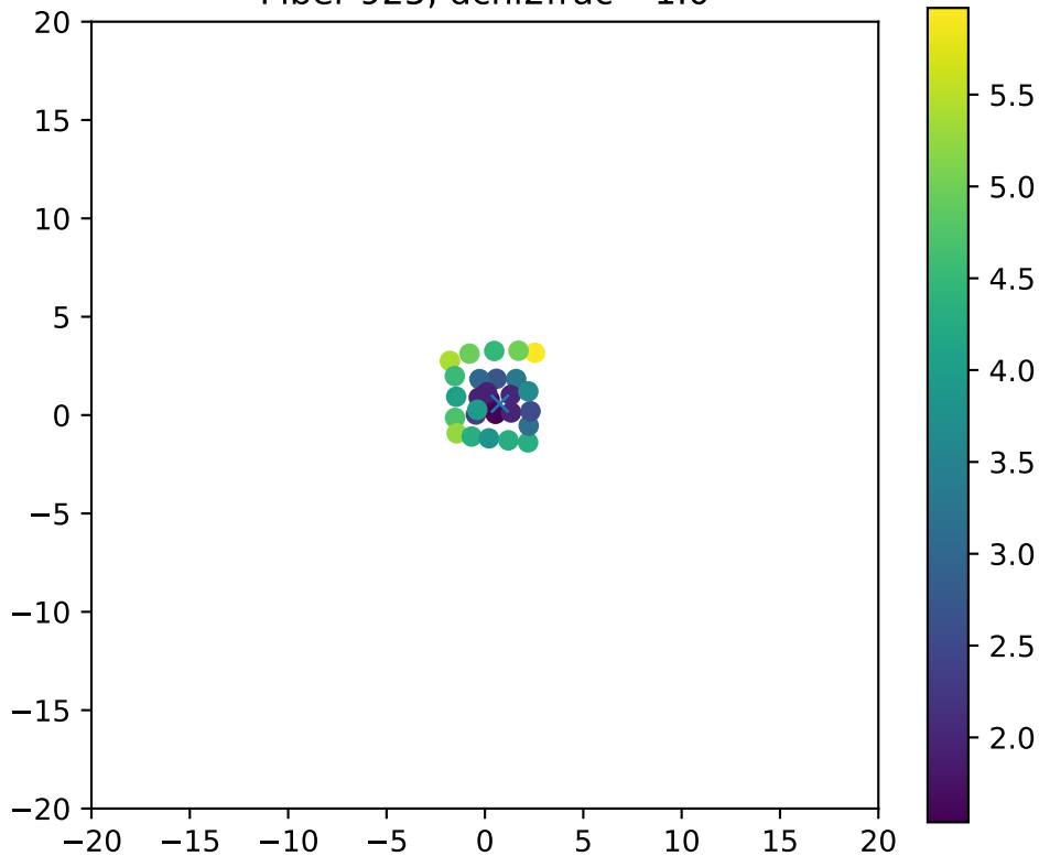
Fiber 925, dchi2frac= 1.0
