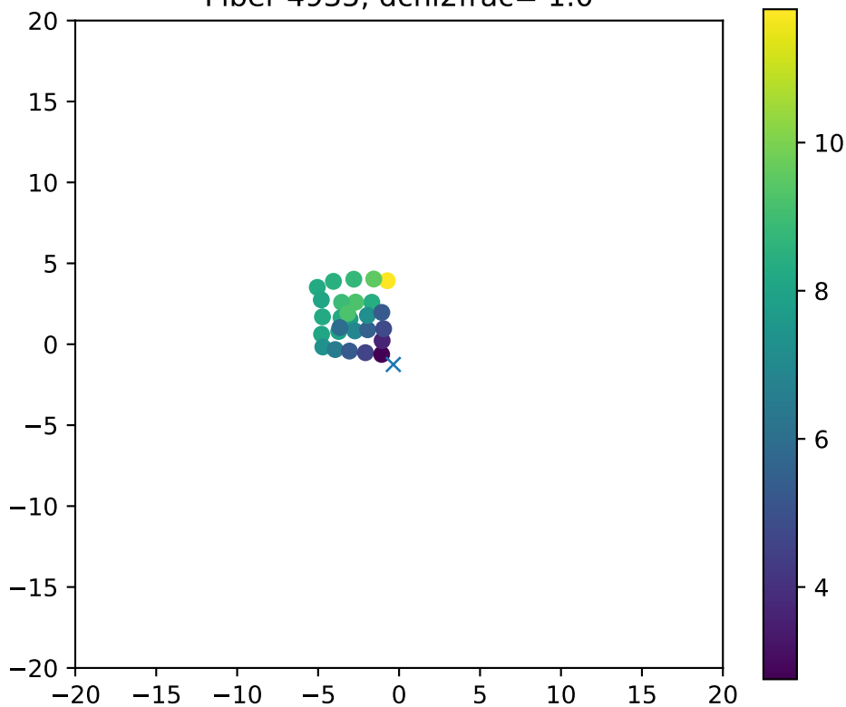
Fiber 4935, dchi2frac= 1.0
