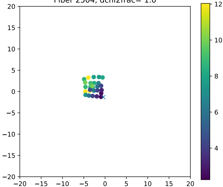
Fiber 2504, dchi2frac= 1.0
