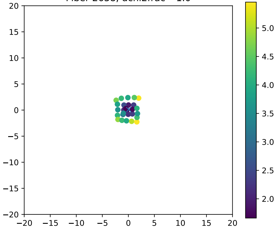
Fiber 2638, dchi2frac= 1.0
