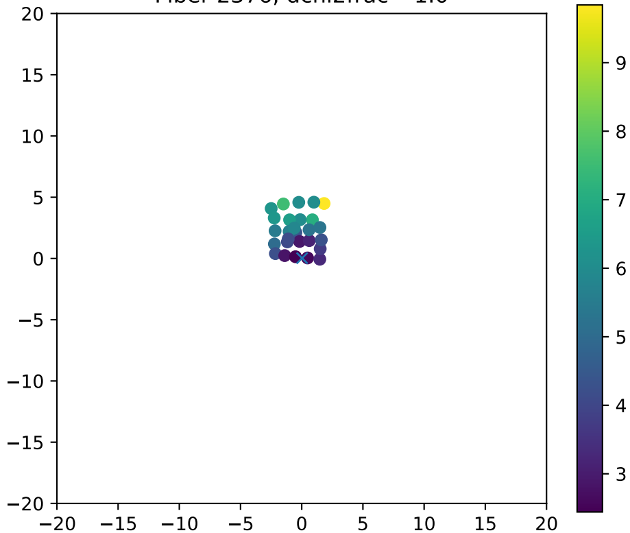
Fiber 2376, dchi2frac= 1.0
