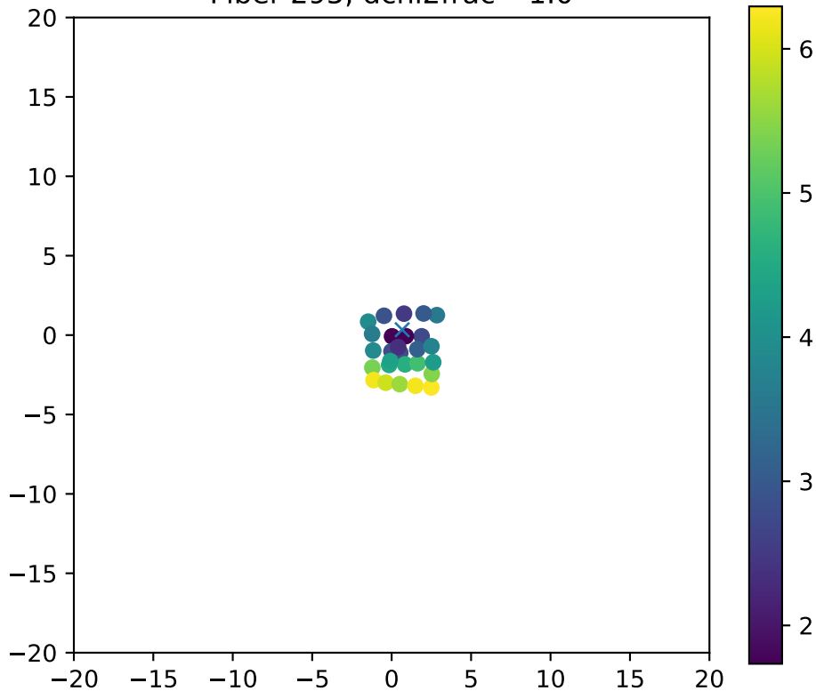
Fiber 295, dchi2frac= 1.0
