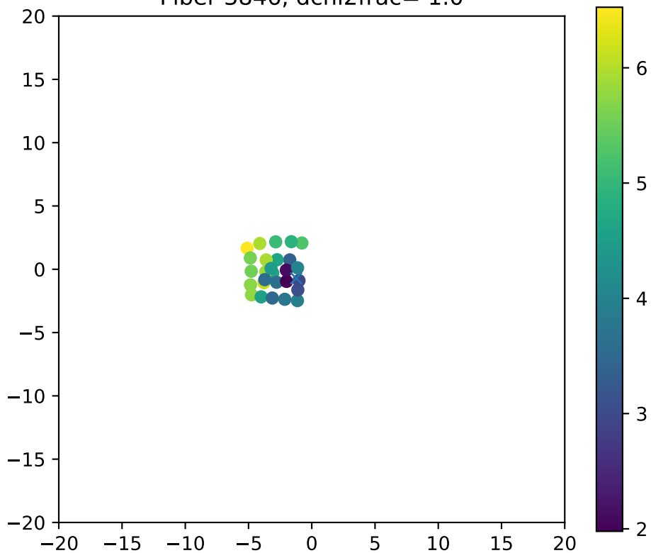
Fiber 3846, dchi2frac= 1.0
