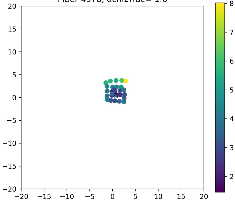
Fiber 4978, dchi2frac= 1.0
