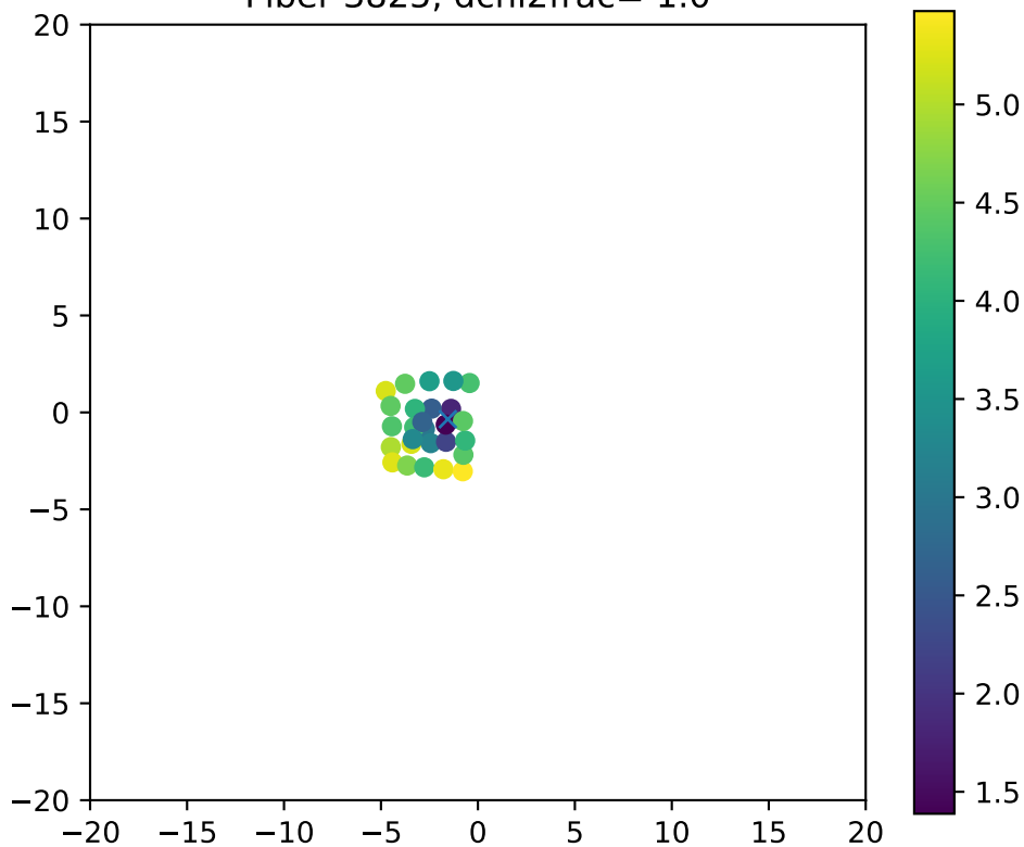
Fiber 3825, dchi2frac= 1.0
