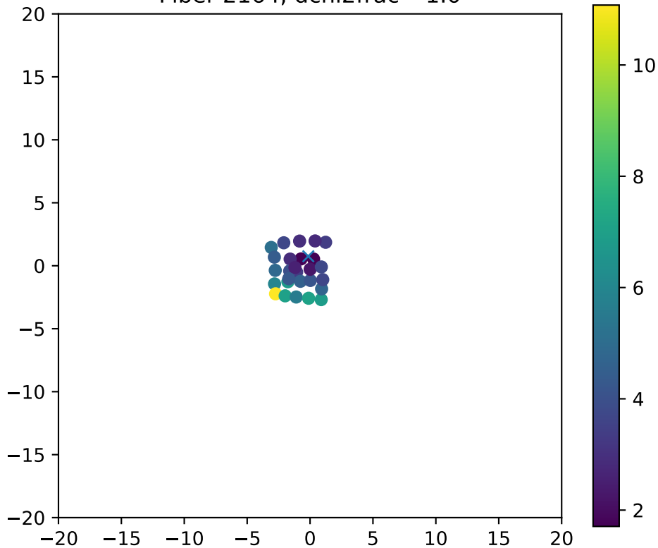
Fiber 2164, dchi2frac= 1.0
