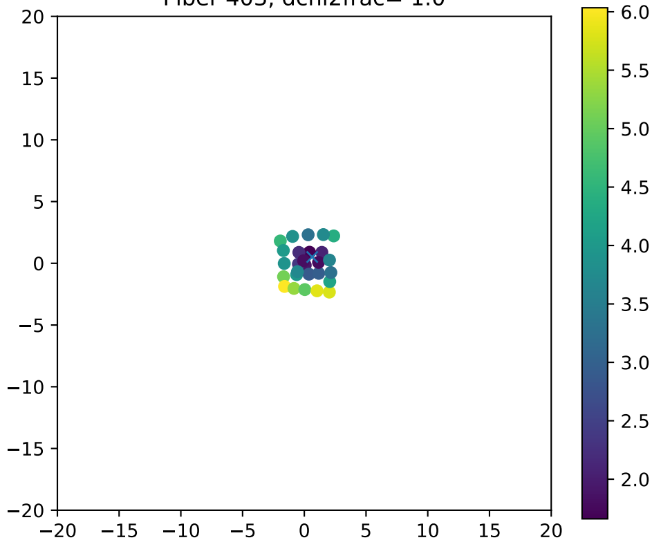
Fiber 403, dchi2frac= 1.0
