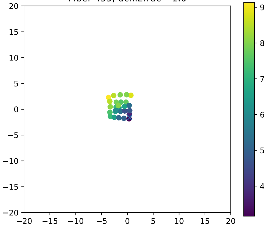
Fiber 459, dchi2frac= 1.0
