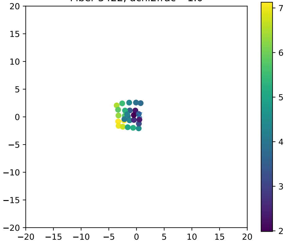
Fiber 3422, dchi2frac= 1.0
