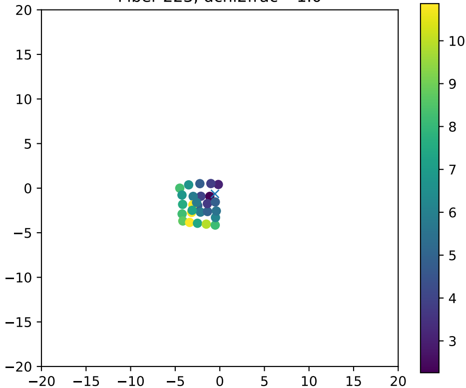
Fiber 223, dchi2frac= 1.0
