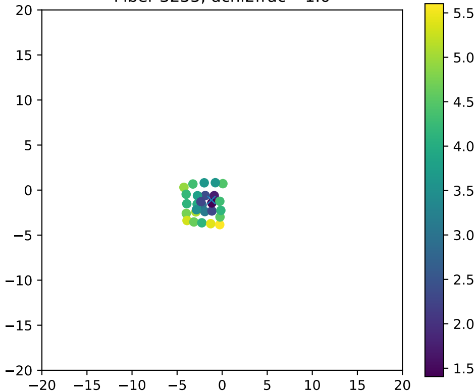
Fiber 3255, dchi2frac= 1.0
