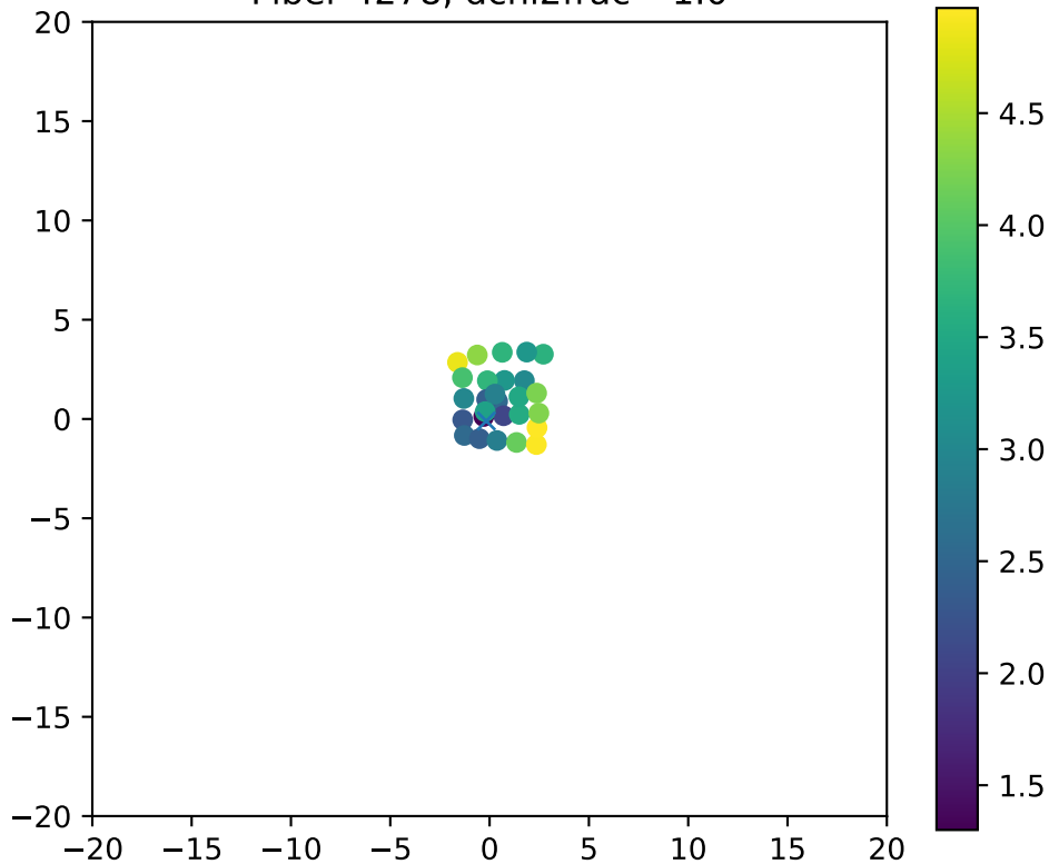
Fiber 4278, dchi2frac= 1.0
