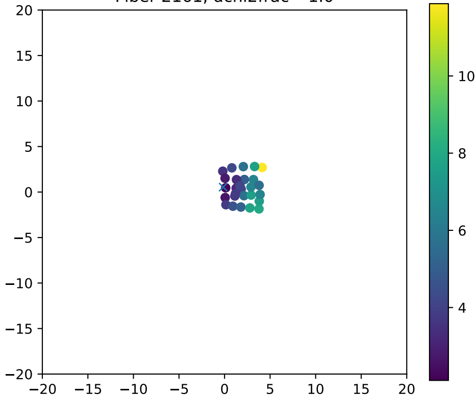
Fiber 2161, dchi2frac= 1.0
