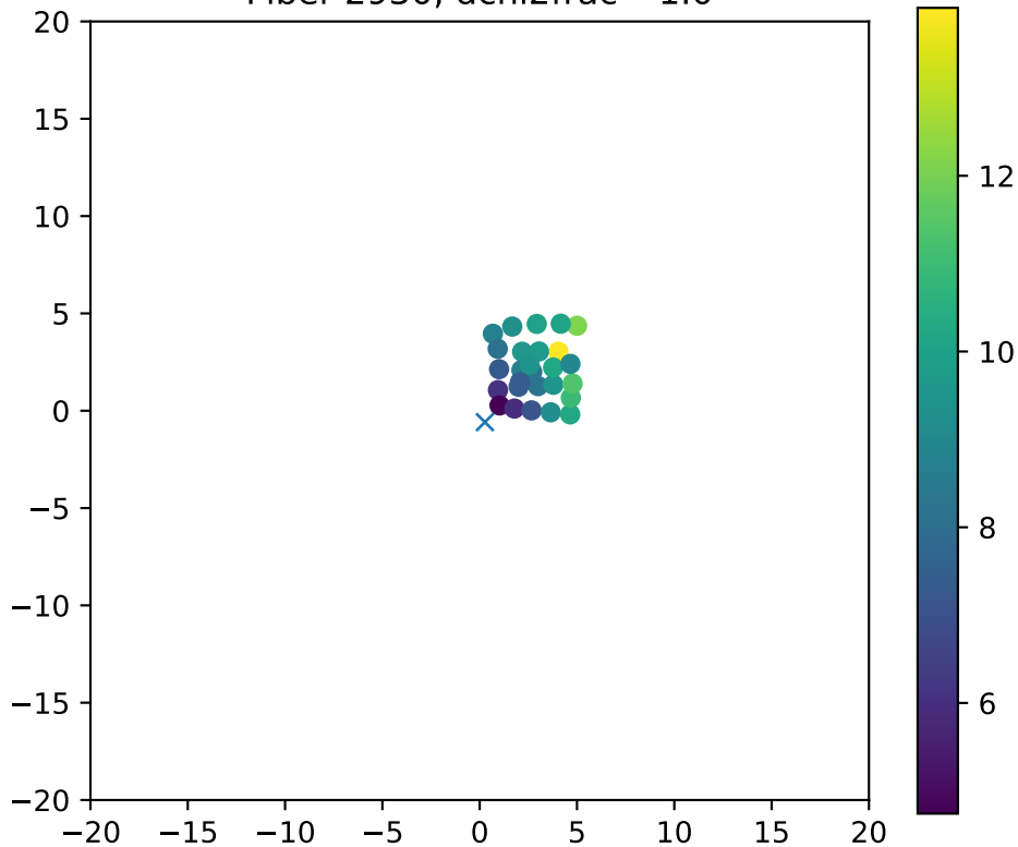
Fiber 2930, dchi2frac= 1.0
