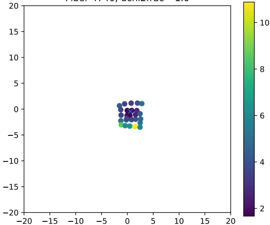
Fiber 4740, dchi2frac= 1.0
