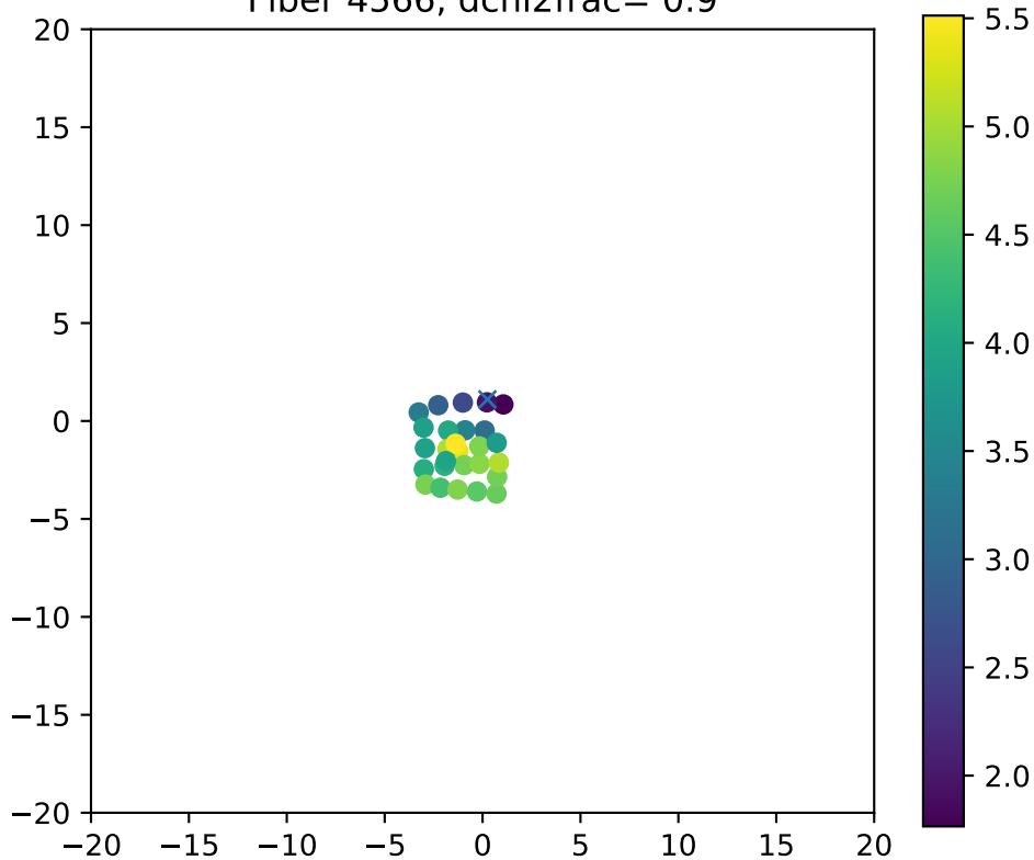
Fiber 4566, dchi2frac= 0.9
