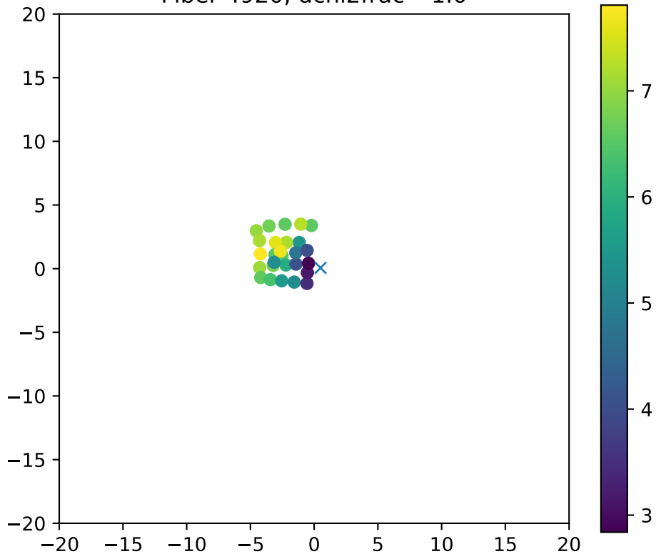
Fiber 4920, dchi2frac= 1.0
