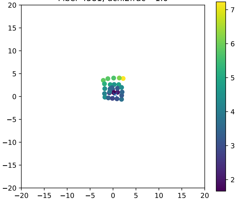
Fiber 4581, dchi2frac= 1.0
