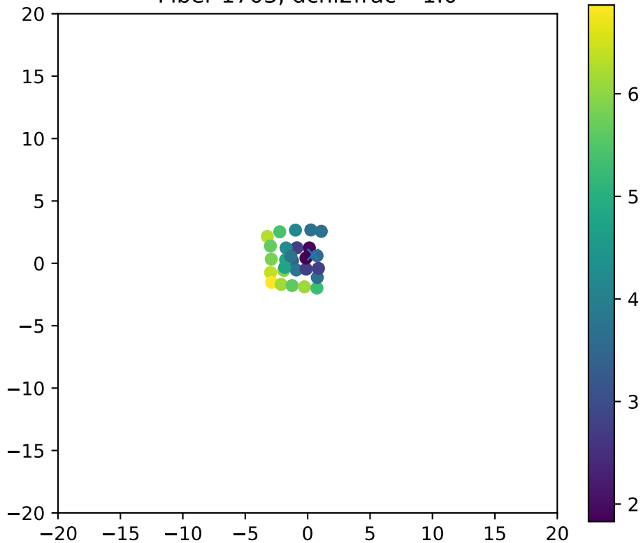
Fiber 1703, dchi2frac= 1.0
