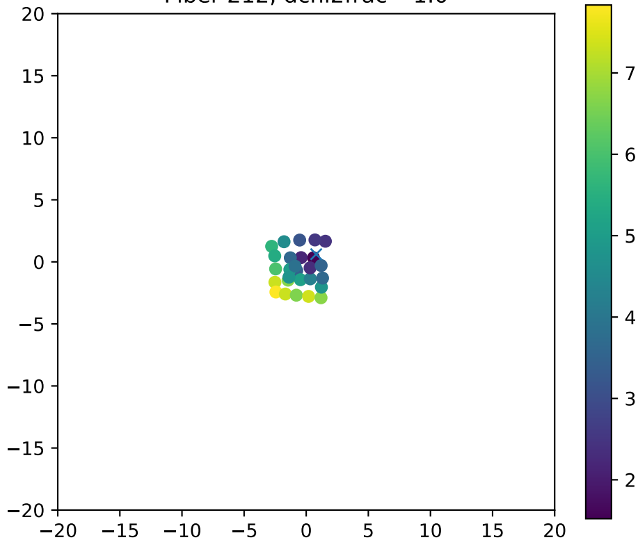
Fiber 212, dchi2frac= 1.0
