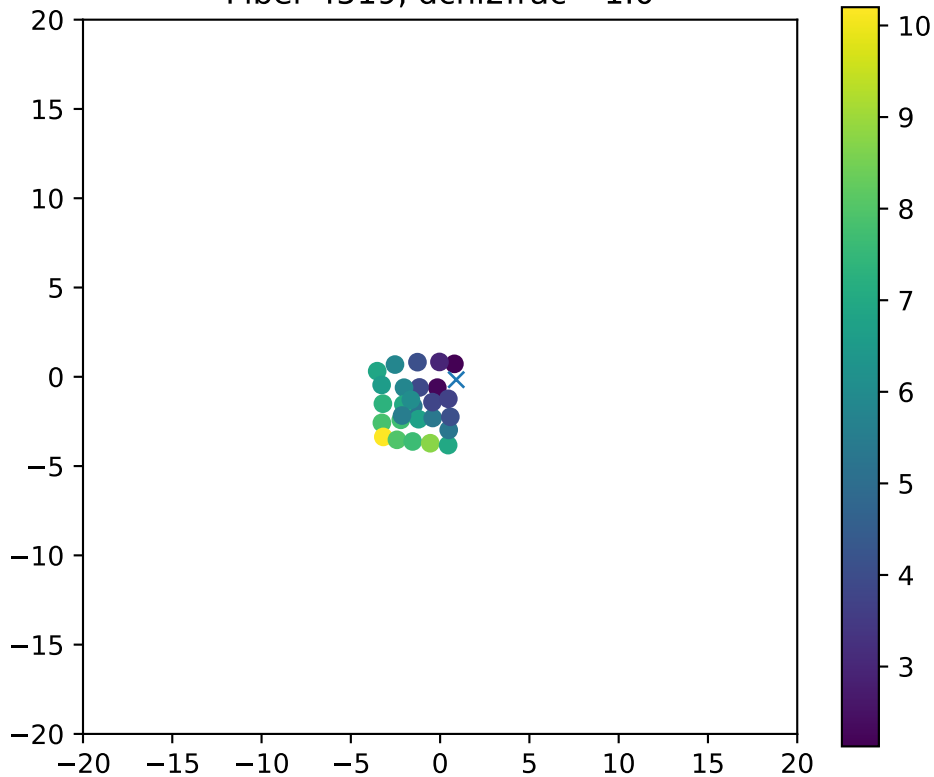
Fiber 4519, dchi2frac= 1.0
