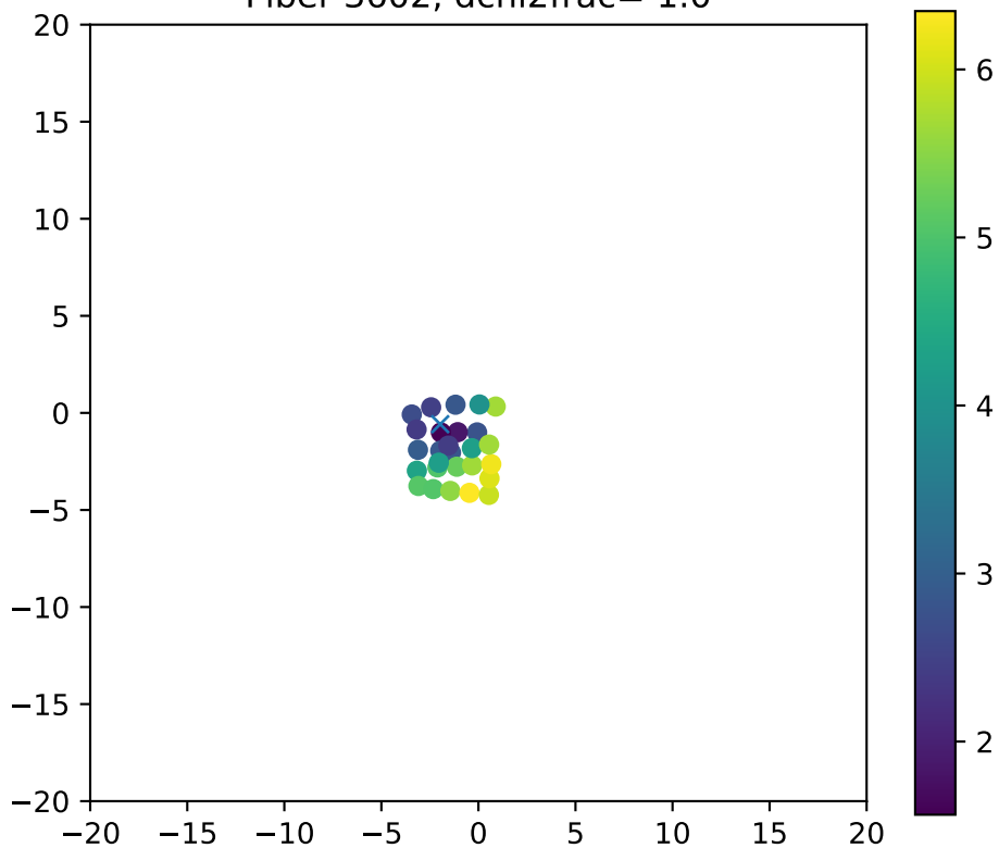
Fiber 3602, dchi2frac= 1.0
