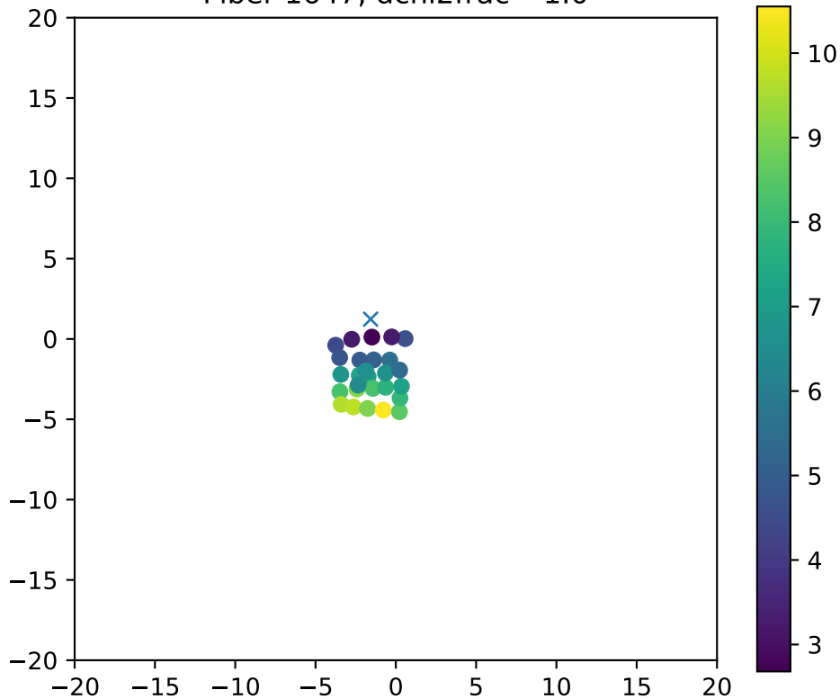
Fiber 1647, dchi2frac= 1.0
