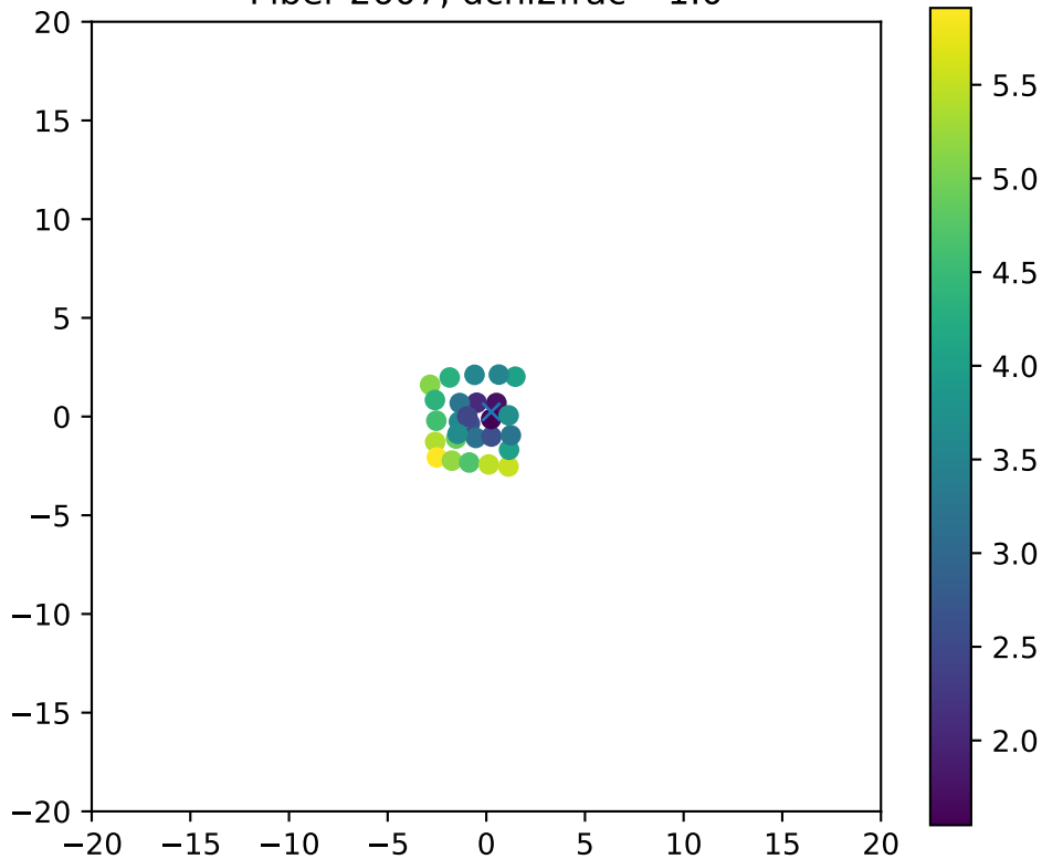
Fiber 2607, dchi2frac= 1.0
