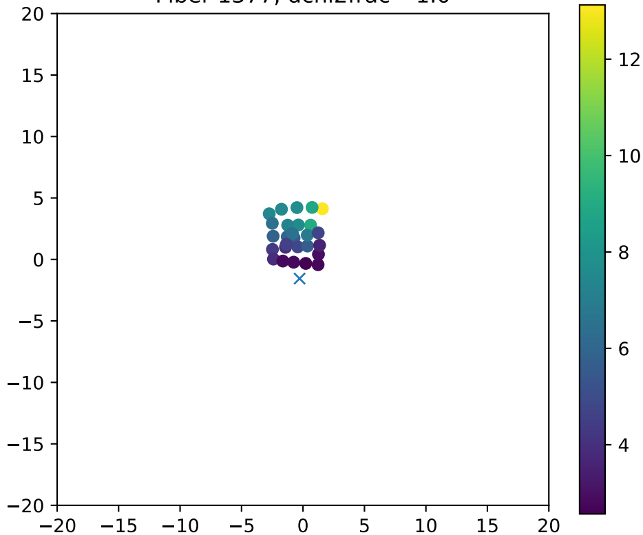
Fiber 1377, dchi2frac= 1.0
