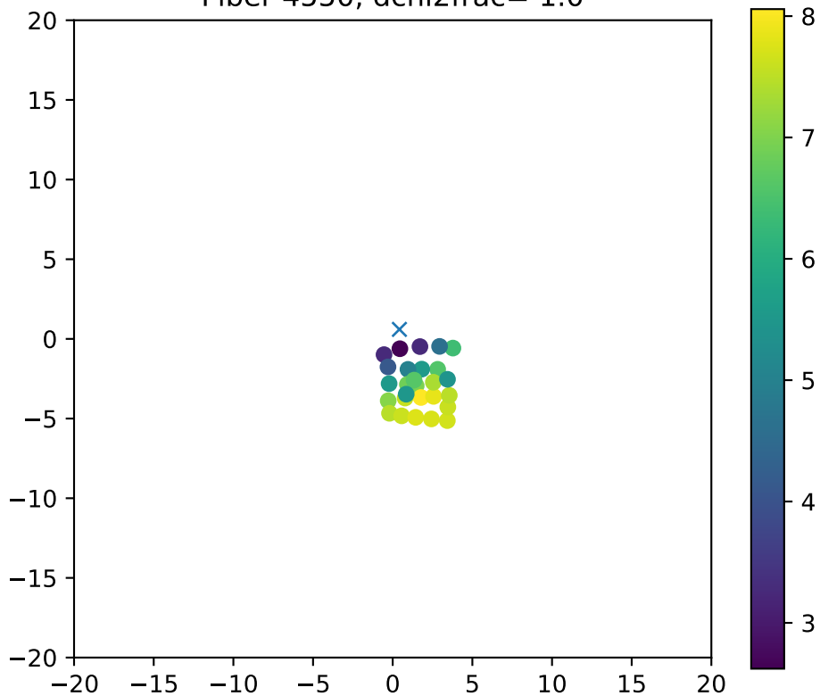
Fiber 4550, dchi2frac= 1.0
