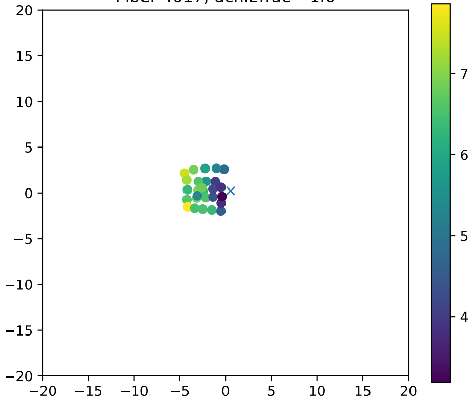
Fiber 4617, dchi2frac= 1.0
