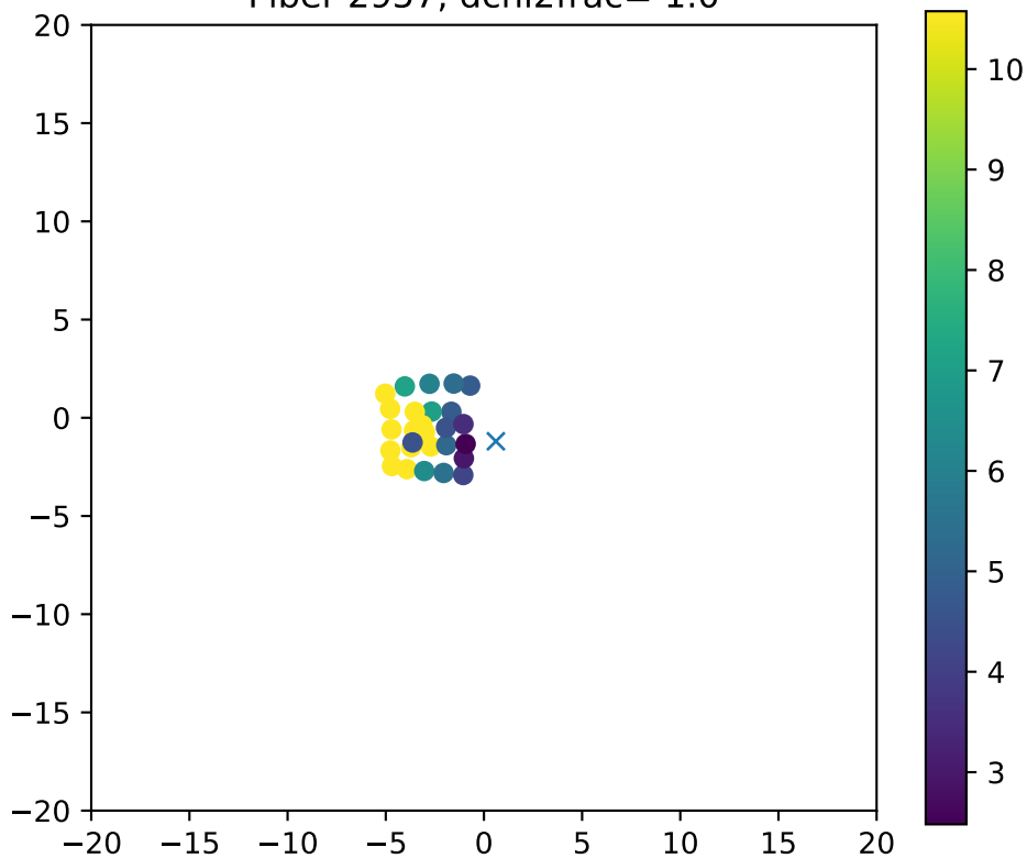
Fiber 2957, dchi2frac= 1.0
