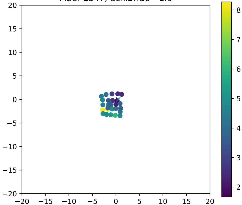
Fiber 2547, dchi2frac= 1.0
