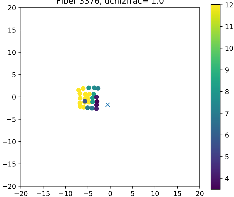
Fiber 3376, dchi2frac= 1.0
