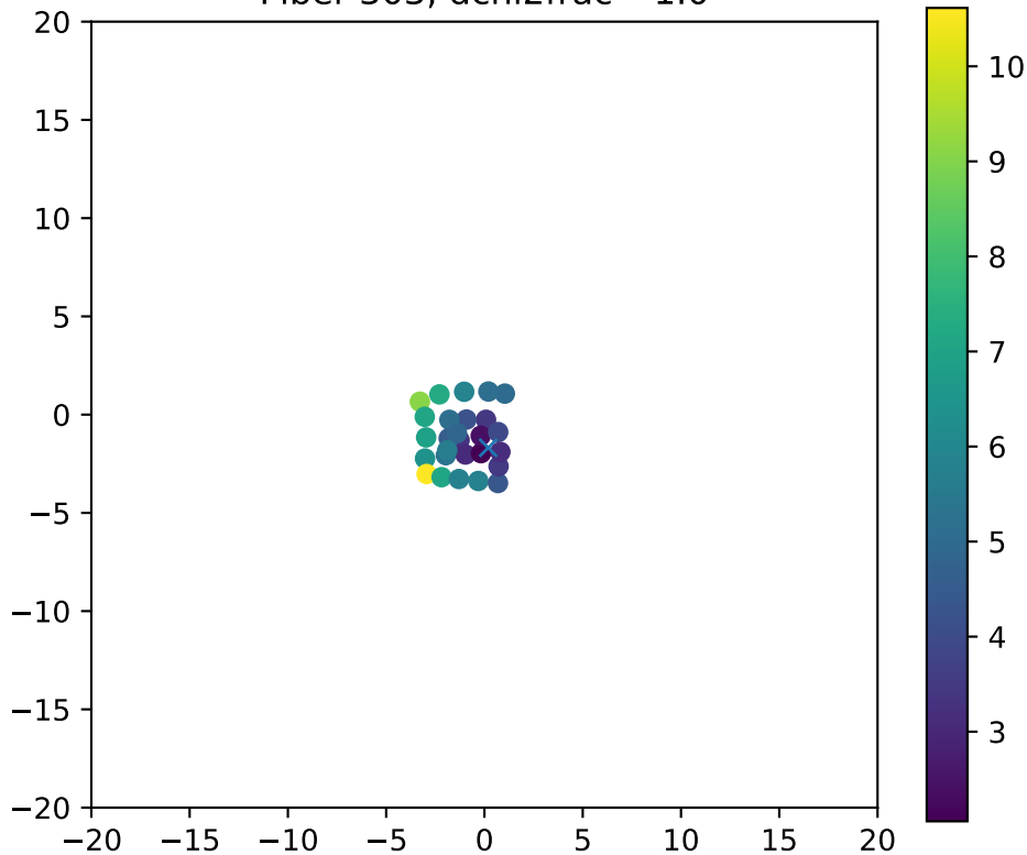
Fiber 303, dchi2frac= 1.0
