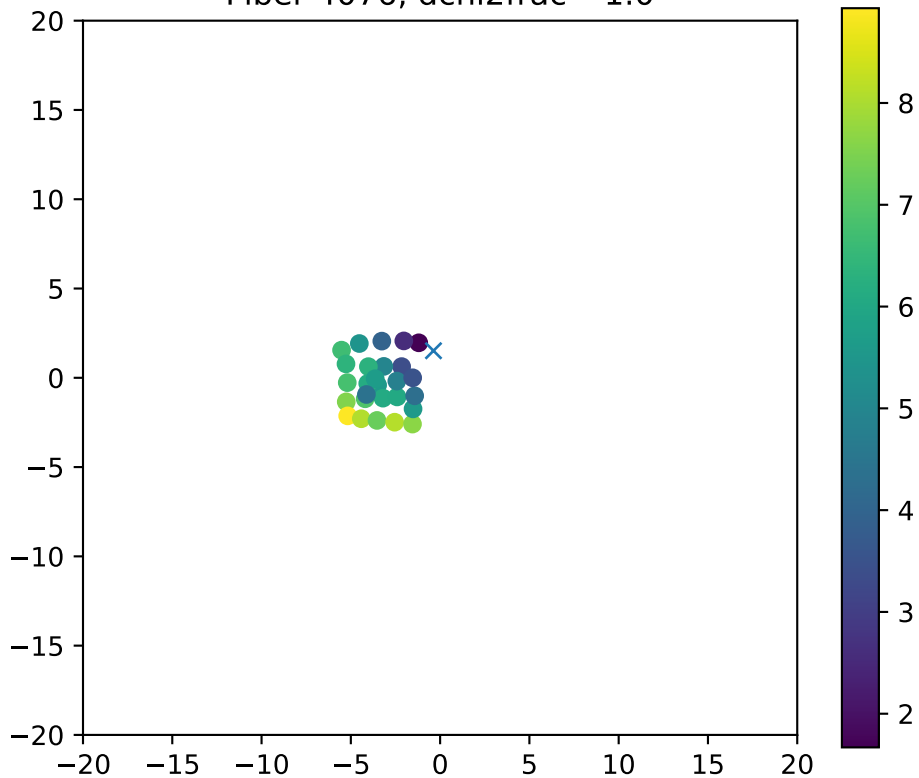
Fiber 4076, dchi2frac= 1.0
