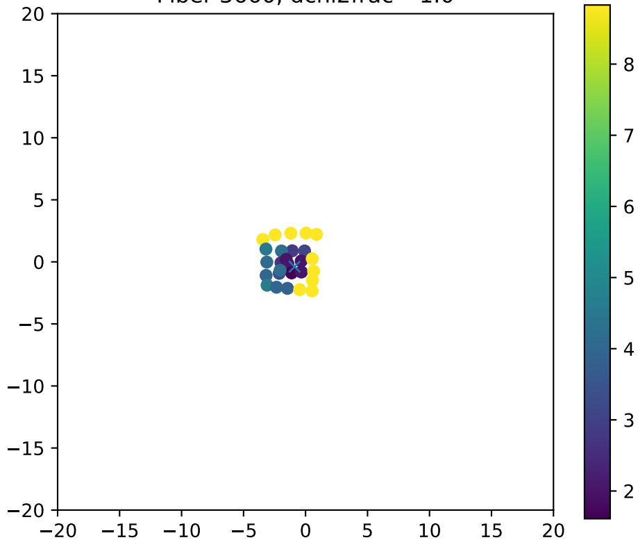
Fiber 3660, dchi2frac= 1.0
