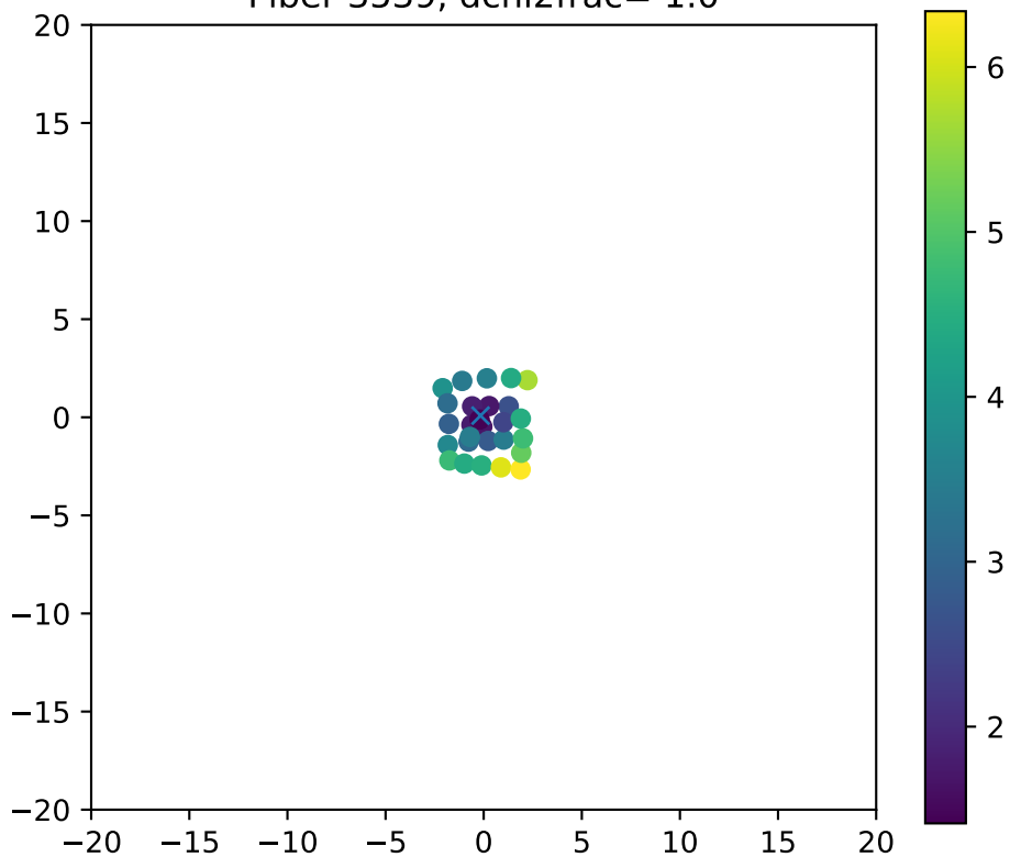
Fiber 3539, dchi2frac= 1.0
