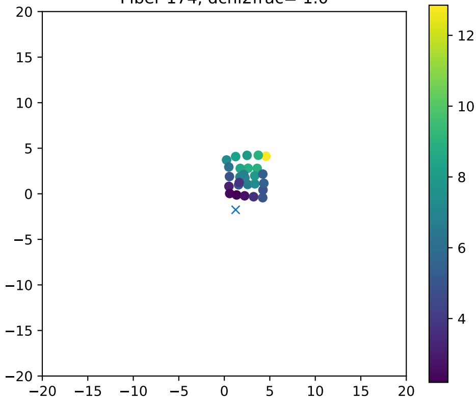
Fiber 174, dchi2frac= 1.0
