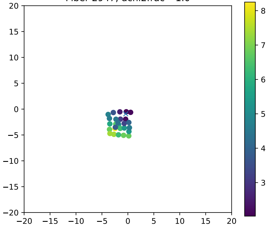
Fiber 2947, dchi2frac= 1.0
