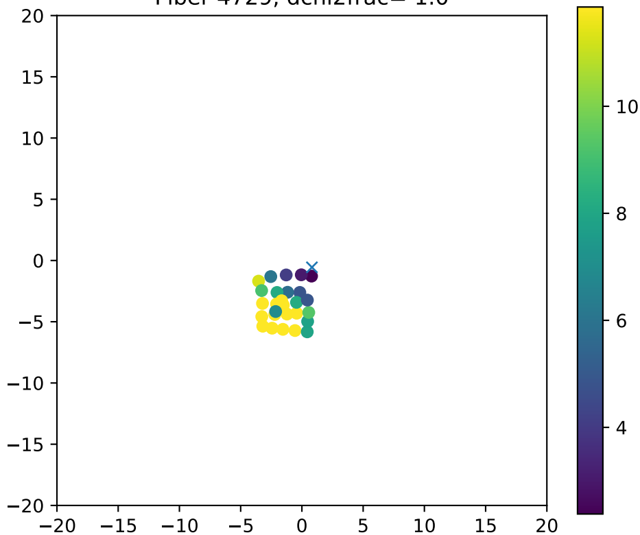
Fiber 4729, dchi2frac= 1.0
