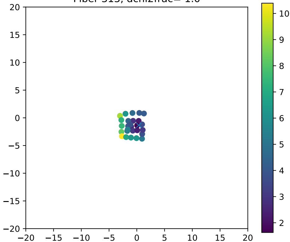
Fiber 313, dchi2frac= 1.0
