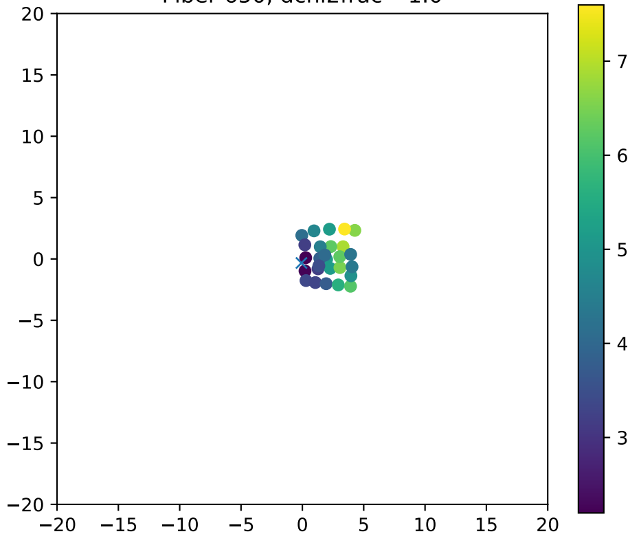
Fiber 650, dchi2frac= 1.0
