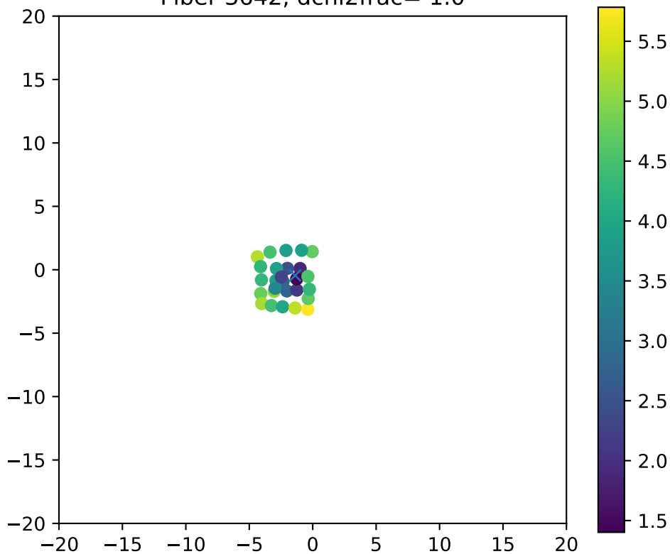
Fiber 3642, dchi2frac= 1.0
