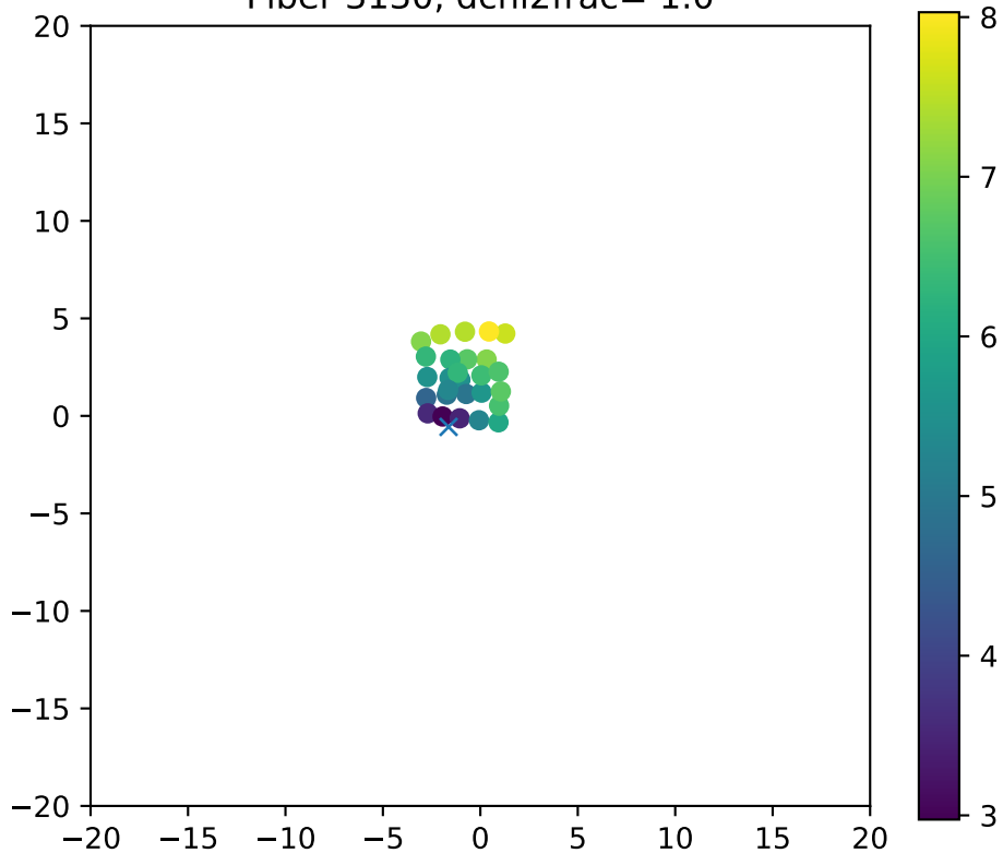
Fiber 3130, dchi2frac= 1.0
