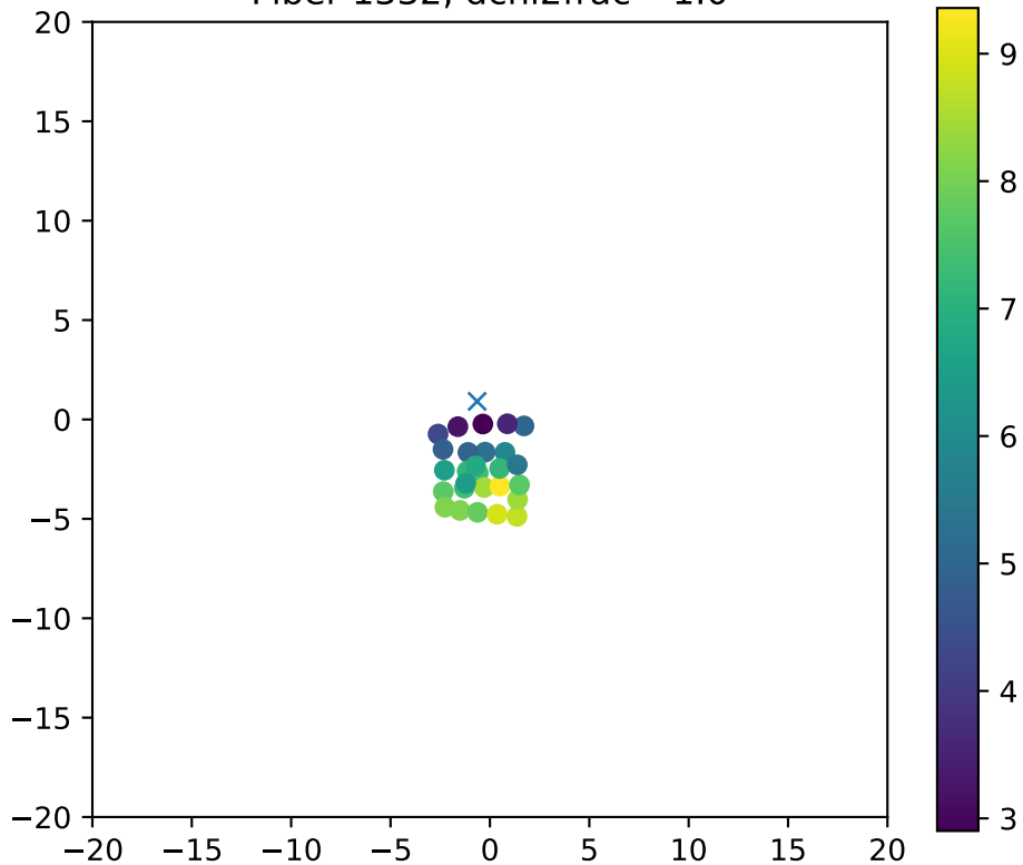
Fiber 1332, dchi2frac= 1.0
