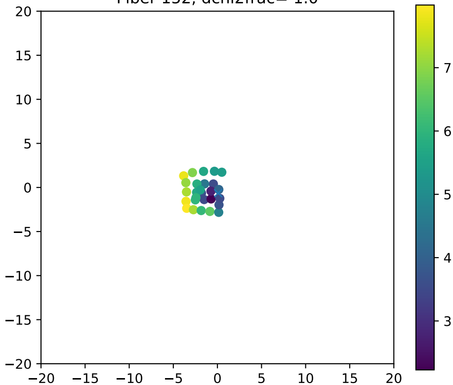
Fiber 152, dchi2frac= 1.0
