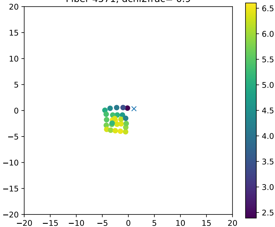
Fiber 4571, dchi2frac= 0.9
