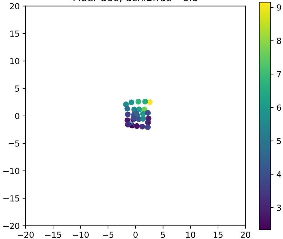
Fiber 866, dchi2frac= 0.9
