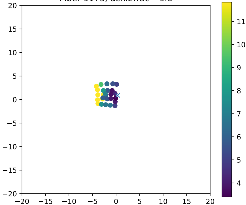
Fiber 1173, dchi2frac= 1.0
