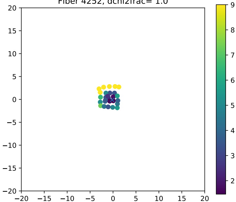
Fiber 4252, dchi2frac= 1.0
