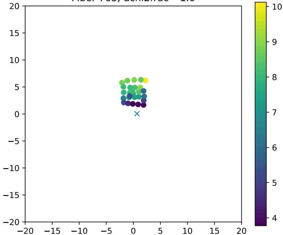
Fiber 765, dchi2frac= 1.0
