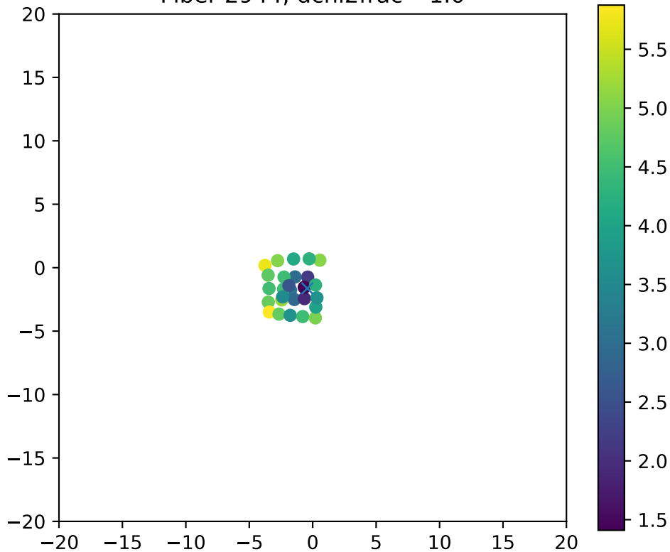
Fiber 2944, dchi2frac= 1.0
