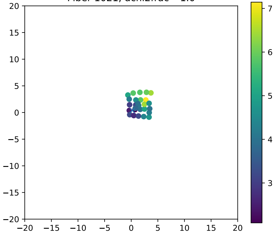
Fiber 1021, dchi2frac= 1.0
