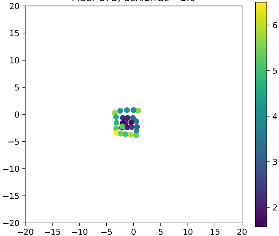
Fiber 873, dchi2frac= 1.0
