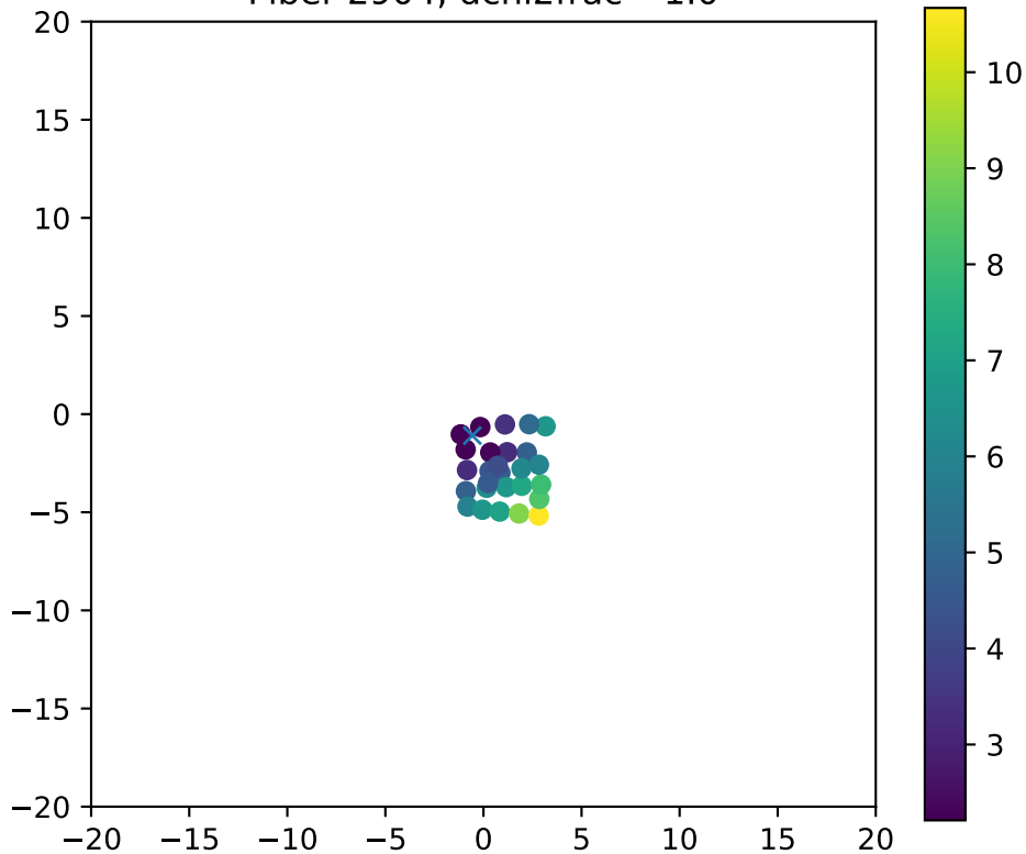
Fiber 2904, dchi2frac= 1.0
