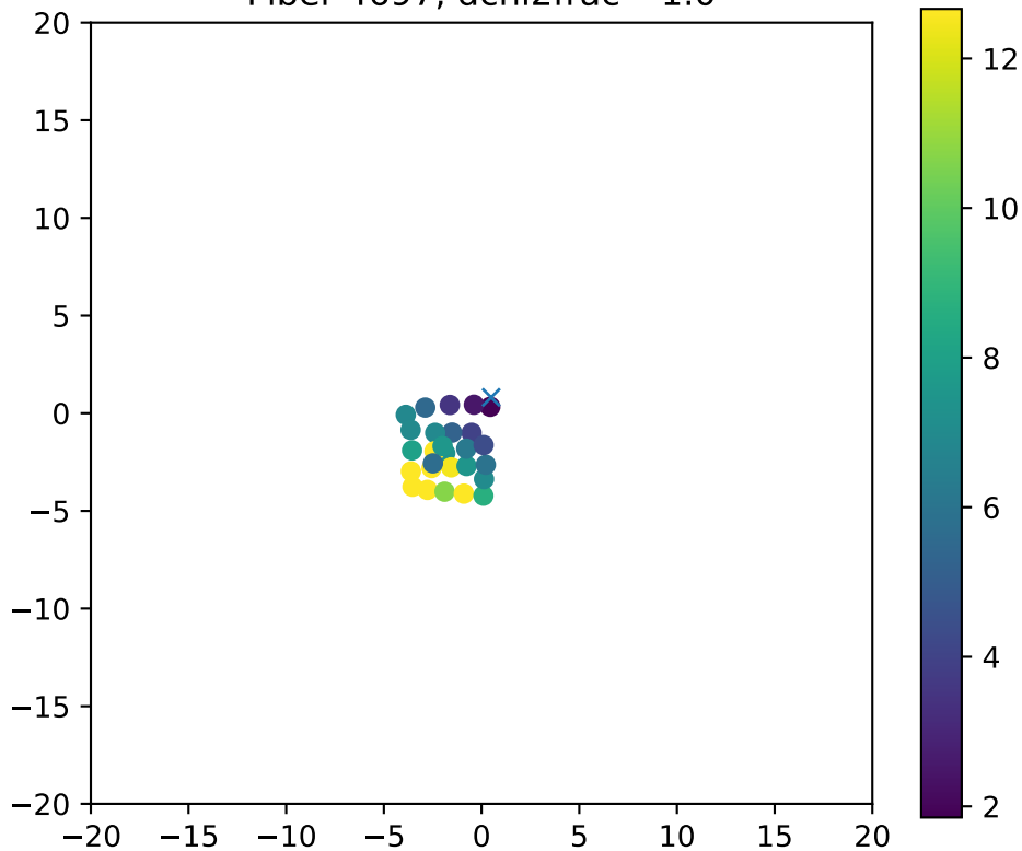
Fiber 4697, dchi2frac= 1.0
