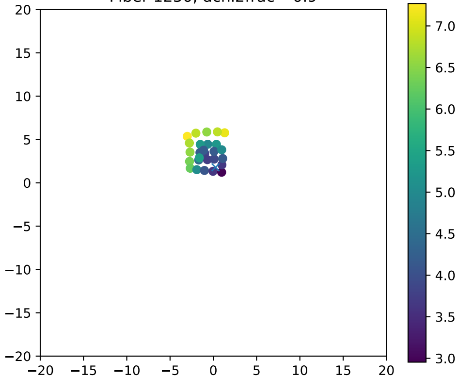
Fiber 1250, dchi2frac= 0.9
