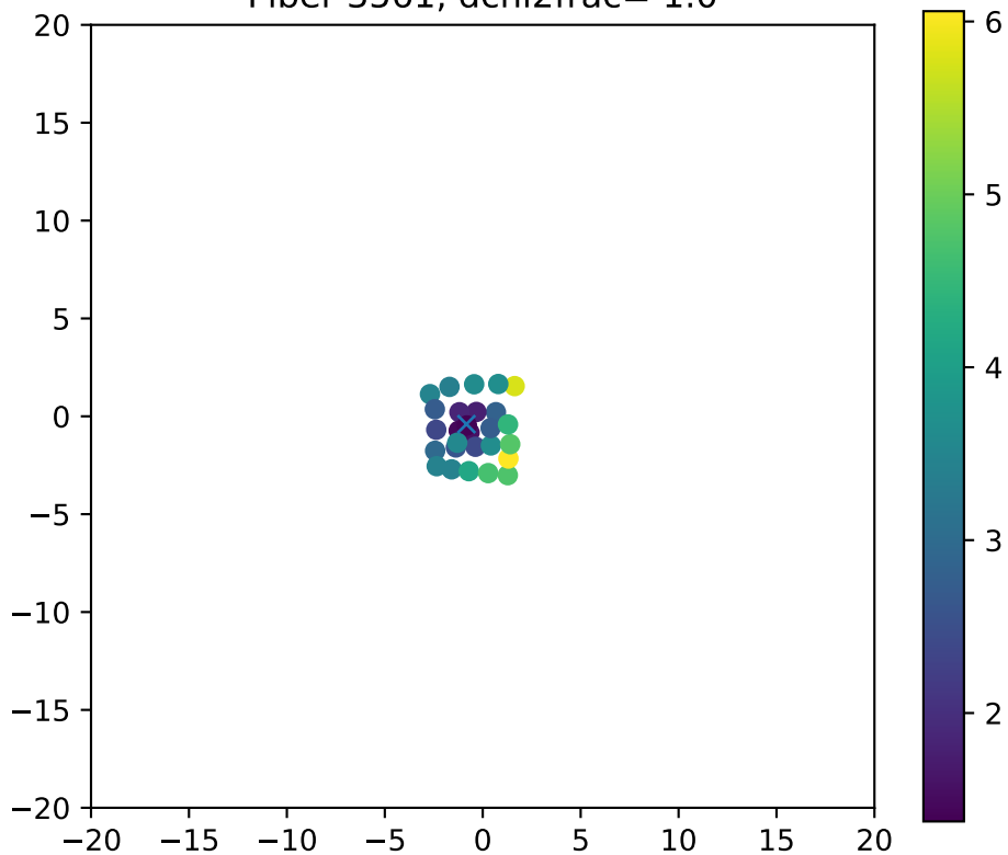
Fiber 3561, dchi2frac= 1.0
