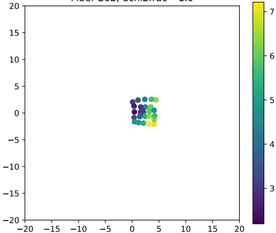
Fiber 262, dchi2frac= 1.0
