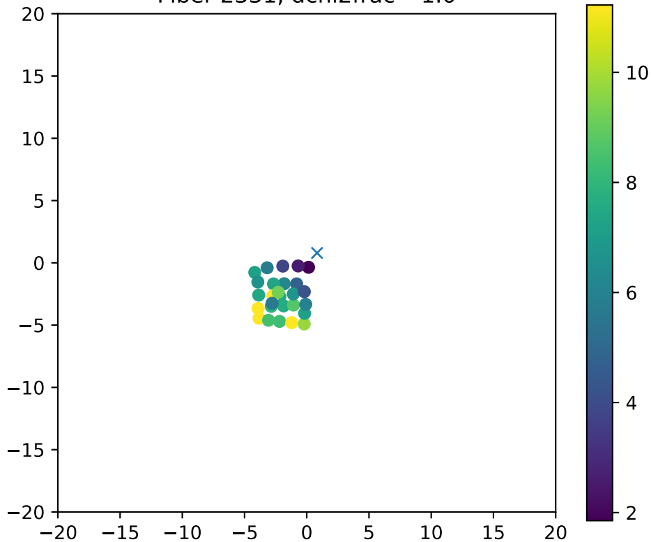
Fiber 2331, dchi2frac= 1.0
