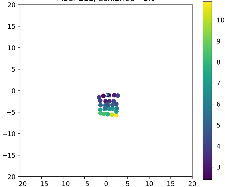
Fiber 211, dchi2frac= 1.0
