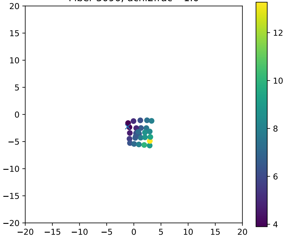
Fiber 3096, dchi2frac= 1.0
