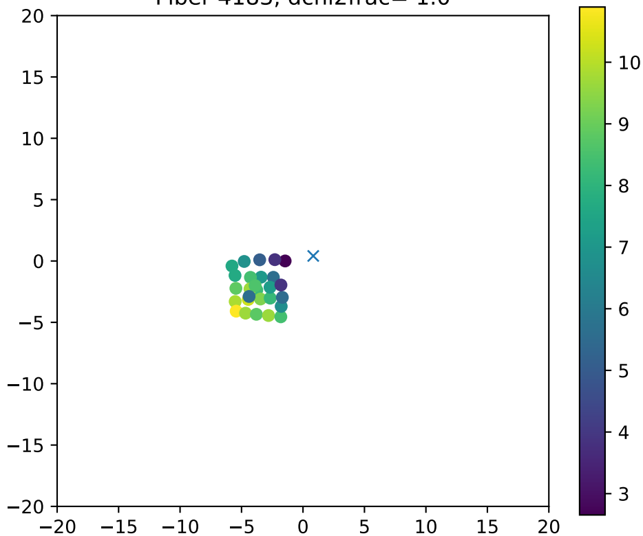
Fiber 4183, dchi2frac= 1.0
