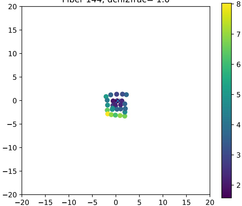
Fiber 144, dchi2frac= 1.0
