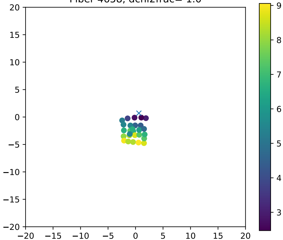
Fiber 4658, dchi2frac= 1.0
