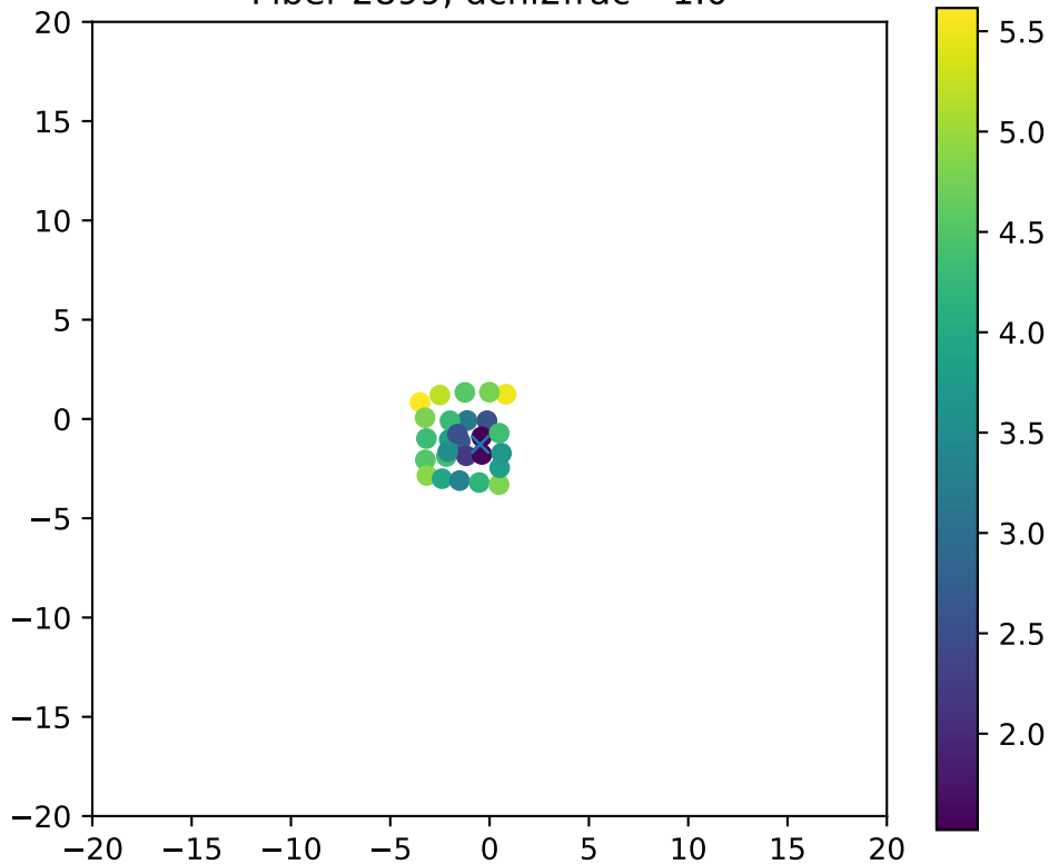
Fiber 2899, dchi2frac= 1.0
