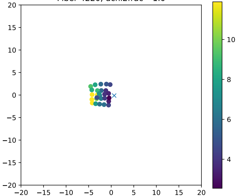
Fiber 4220, dchi2frac= 1.0
