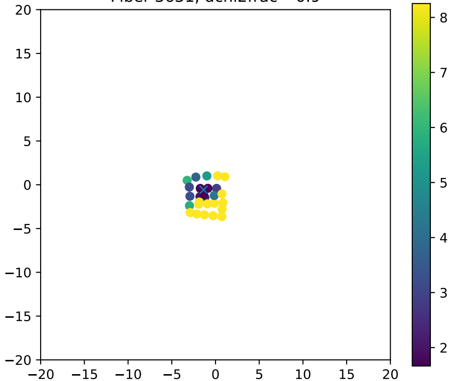
Fiber 3631, dchi2frac= 0.9
