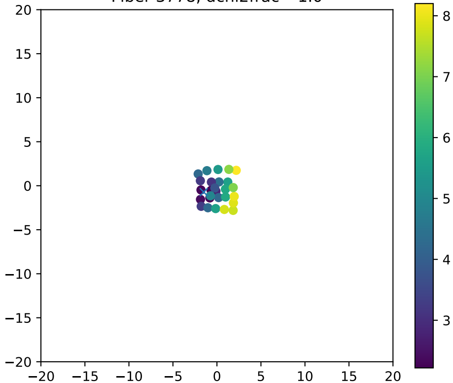
Fiber 3778, dchi2frac= 1.0
