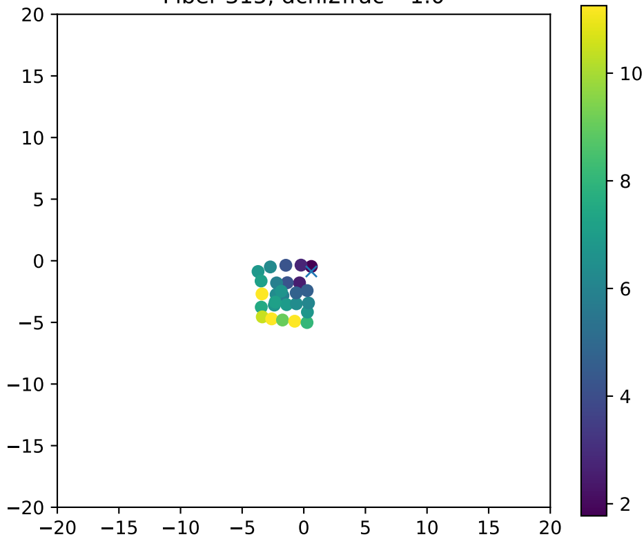
Fiber 315, dchi2frac= 1.0
