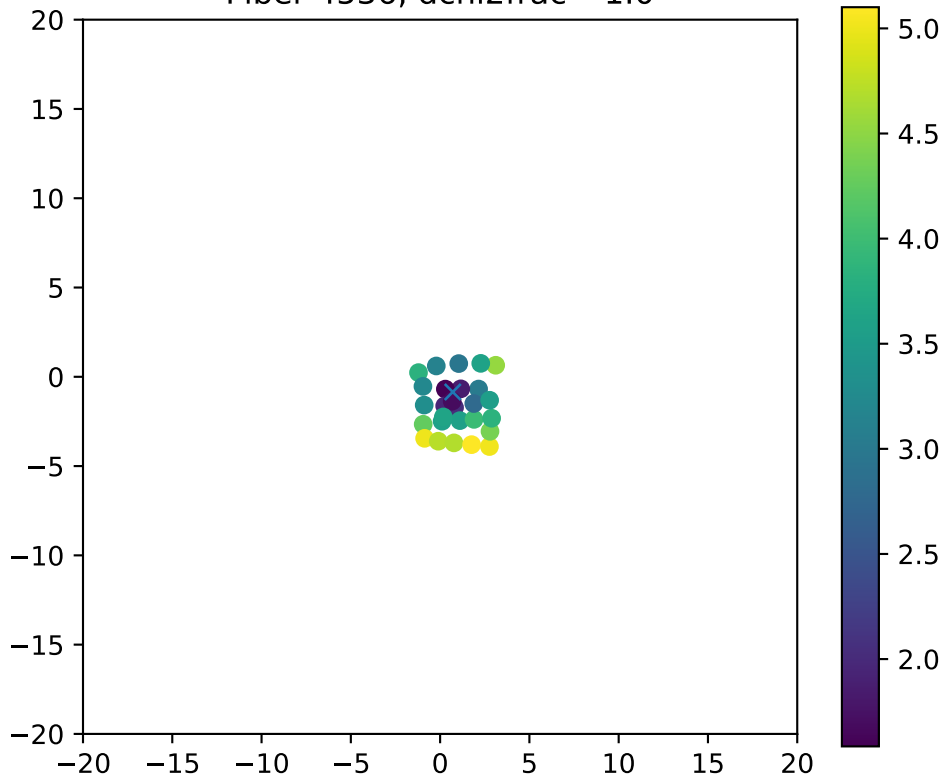
Fiber 4536, dchi2frac= 1.0
