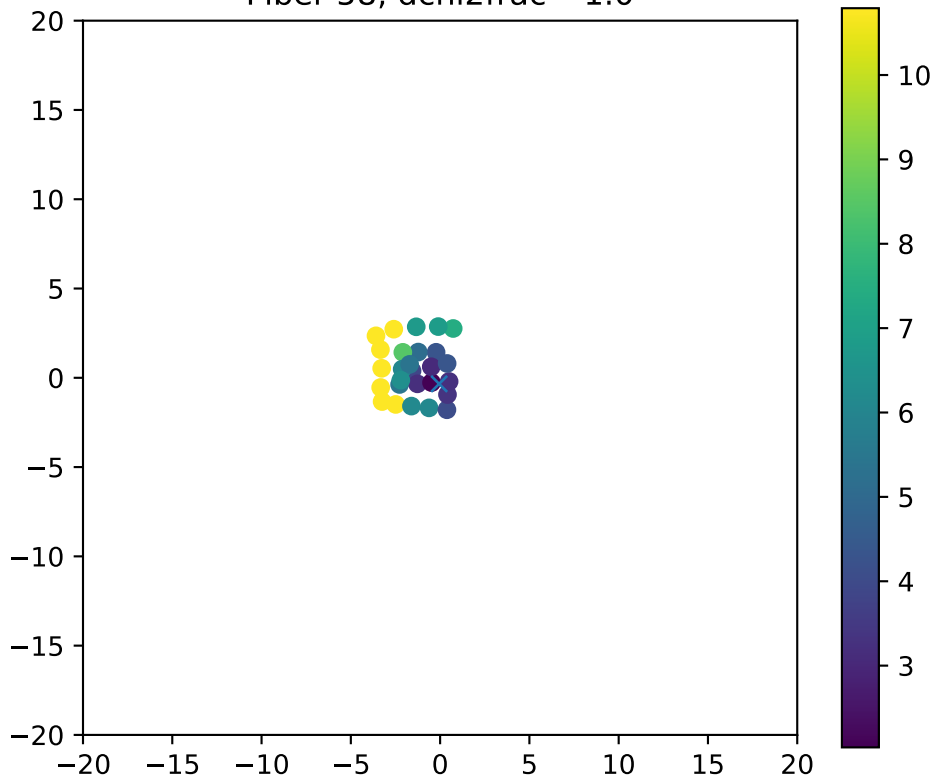
Fiber 58, dchi2frac= 1.0
