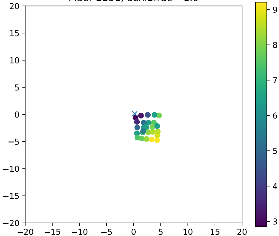
Fiber 2291, dchi2frac= 1.0
