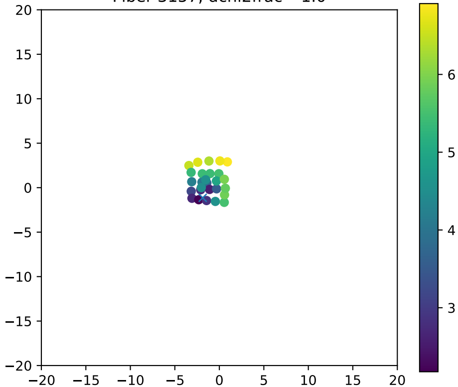
Fiber 3157, dchi2frac= 1.0
