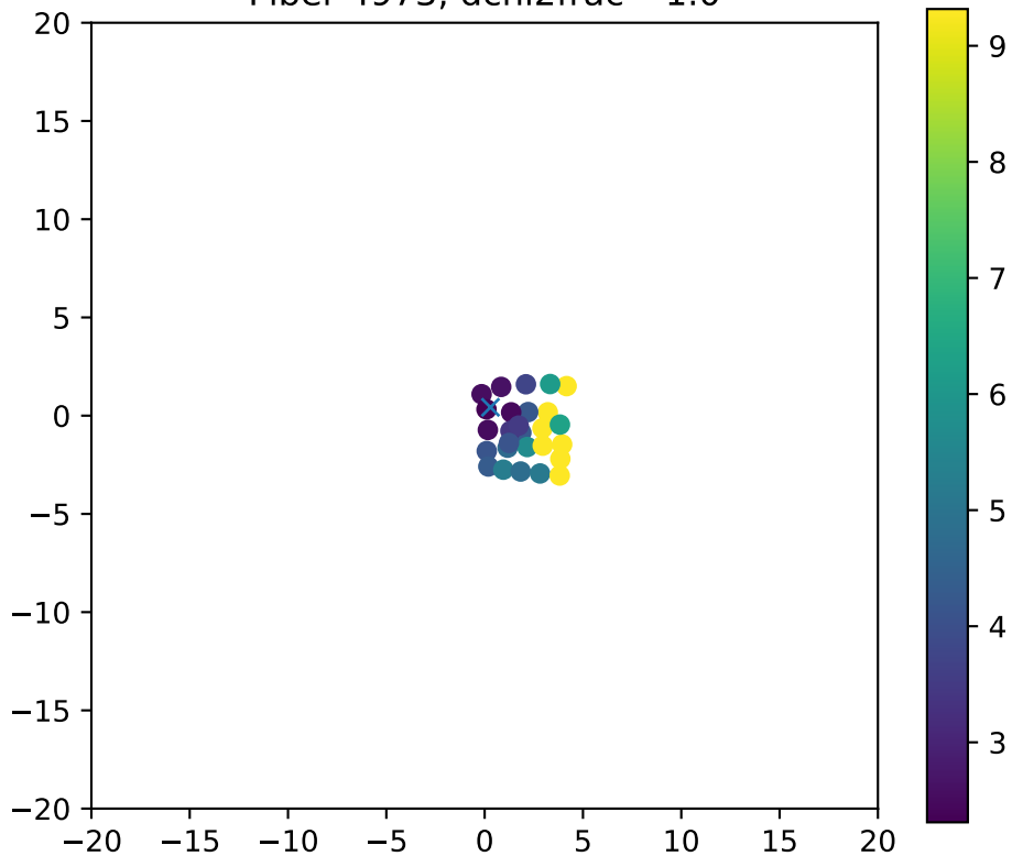
Fiber 4973, dchi2frac= 1.0
