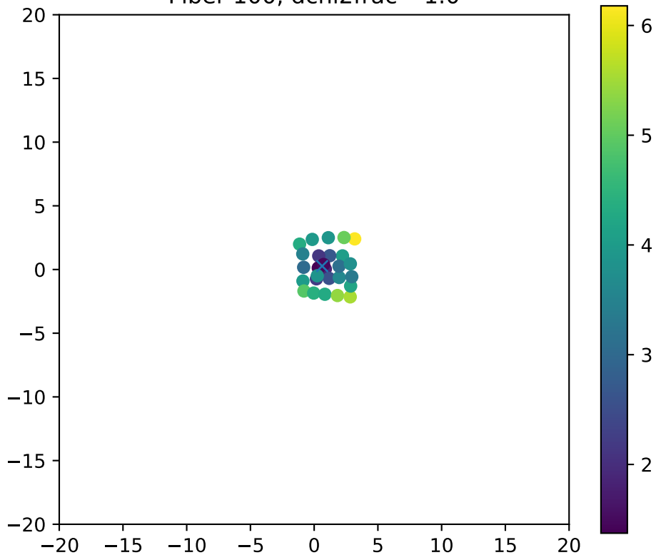
Fiber 100, dchi2frac= 1.0
