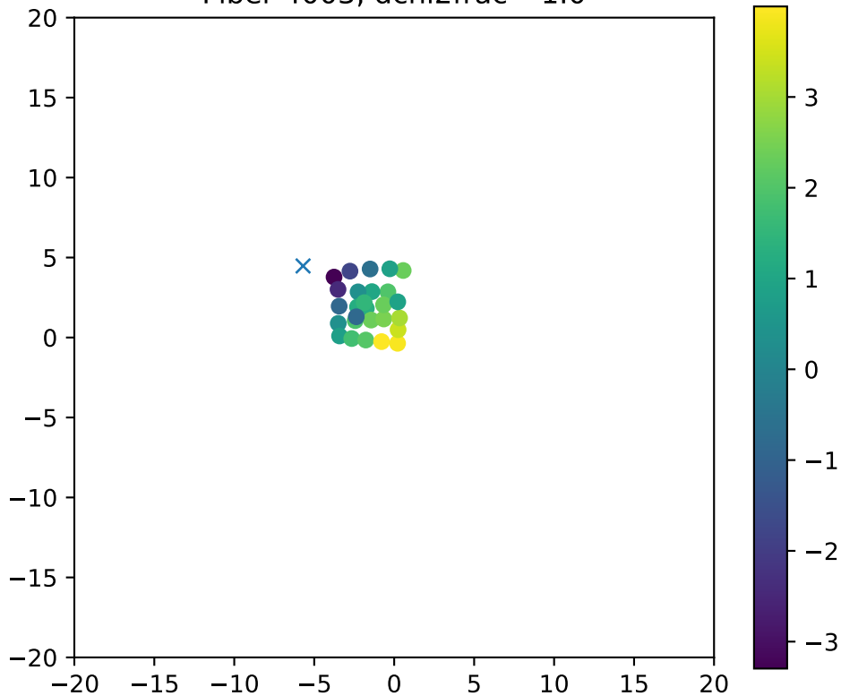
Fiber 4003, dchi2frac= 1.0
