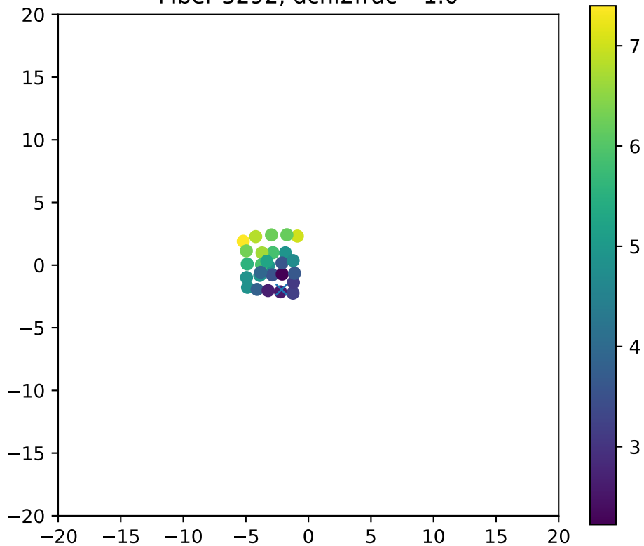
Fiber 3292, dchi2frac= 1.0
