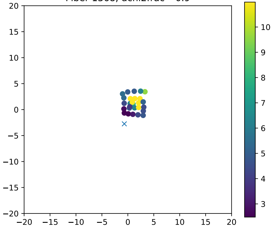
Fiber 1368, dchi2frac= 0.9
