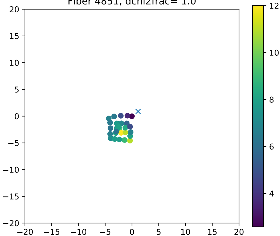
Fiber 4851, dchi2frac= 1.0
