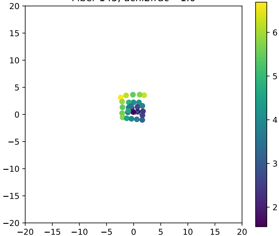
Fiber 145, dchi2frac= 1.0
