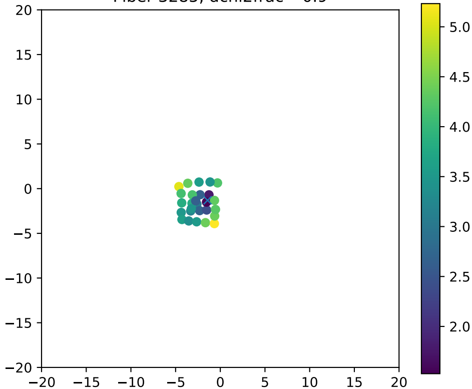
Fiber 3285, dchi2frac= 0.9
