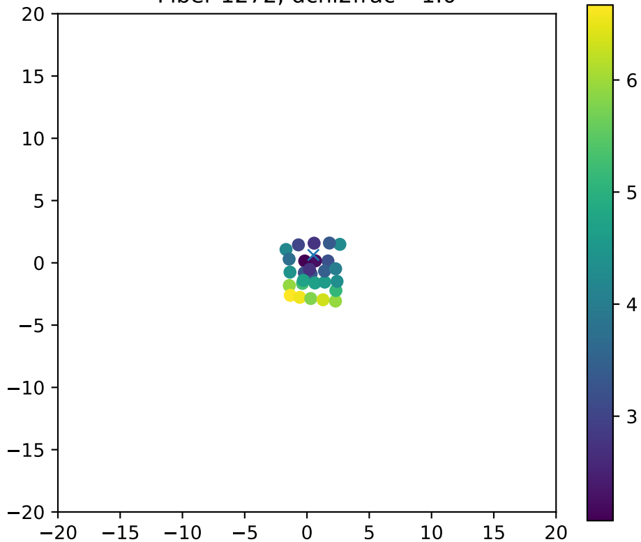
Fiber 1272, dchi2frac= 1.0
