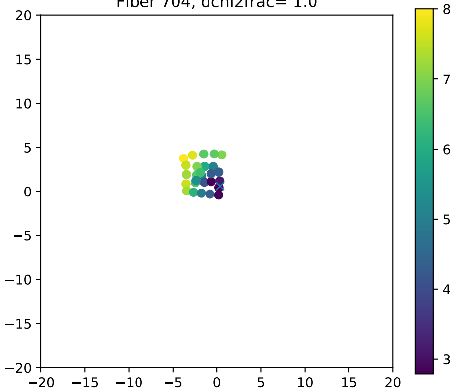
Fiber 704, dchi2frac= 1.0
