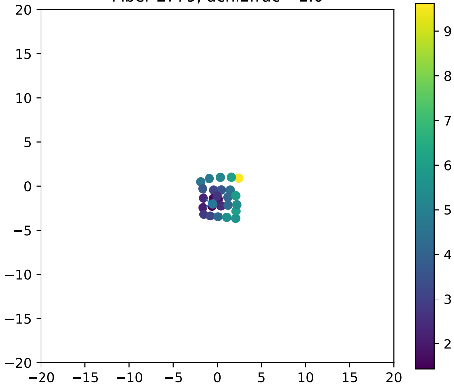
Fiber 2779, dchi2frac= 1.0
