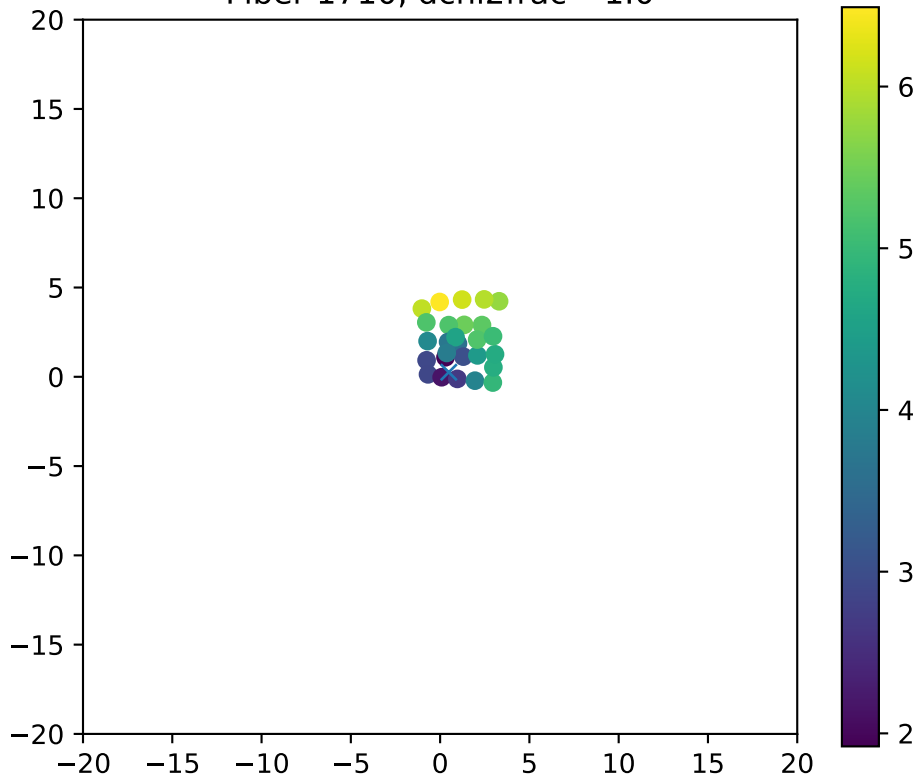
Fiber 1710, dchi2frac= 1.0
