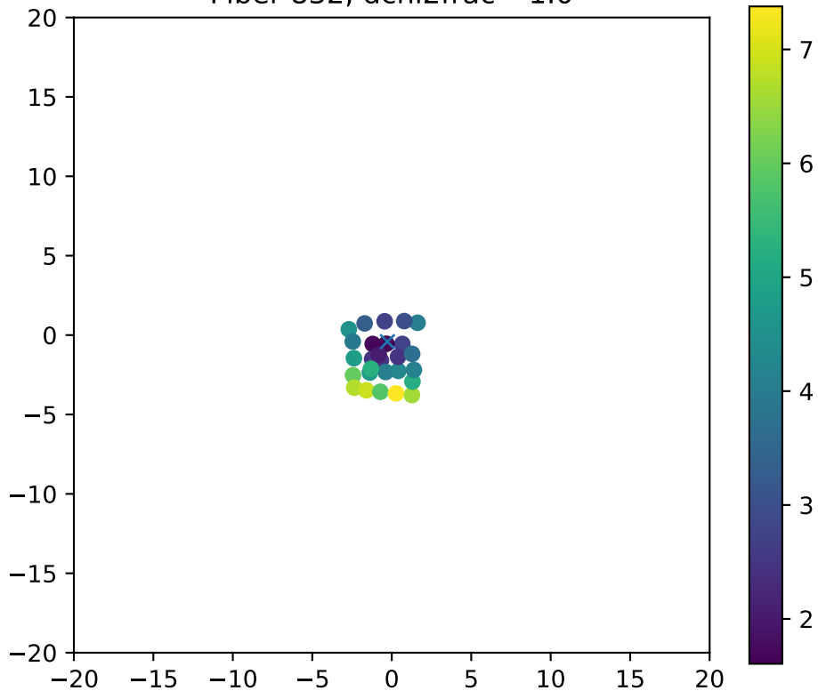
Fiber 832, dchi2frac= 1.0
