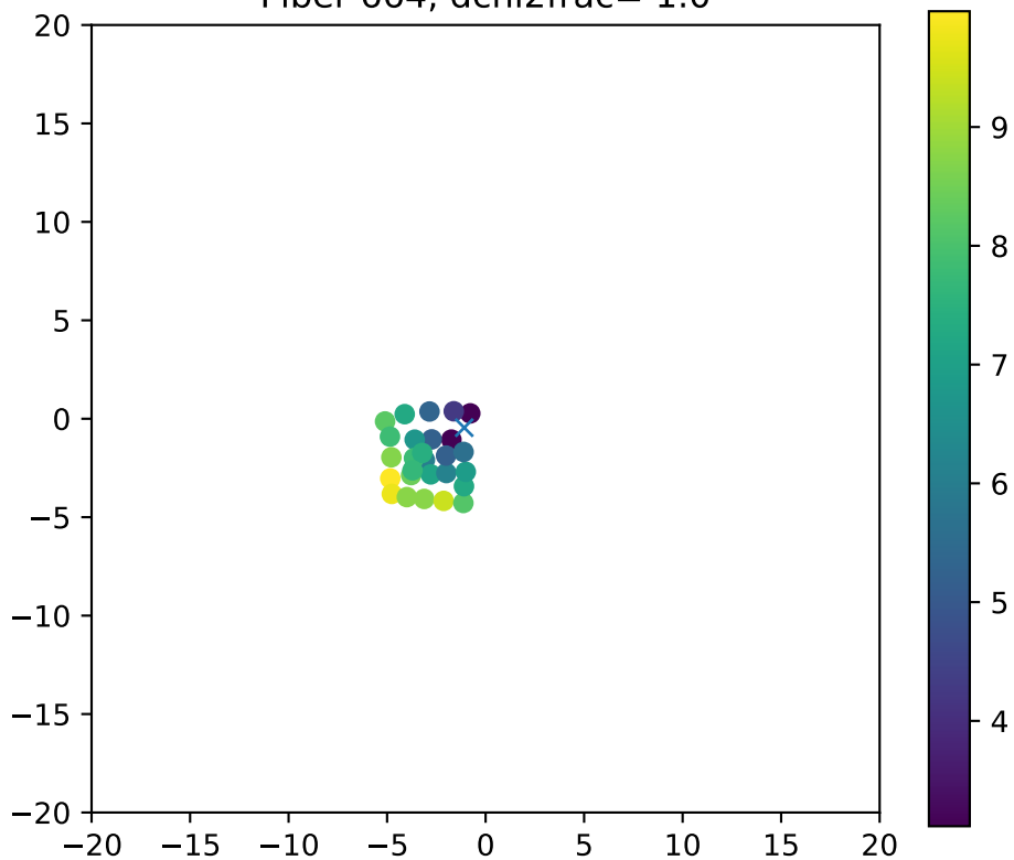
Fiber 664, dchi2frac= 1.0
