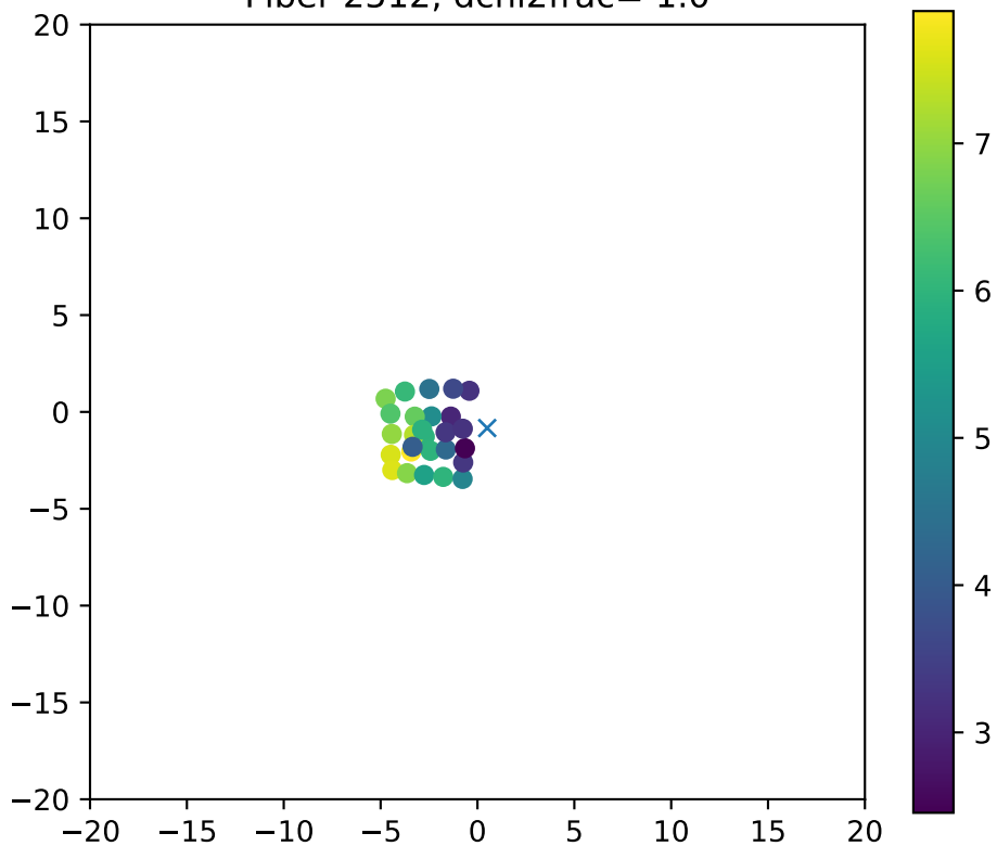
Fiber 2512, dchi2frac= 1.0
