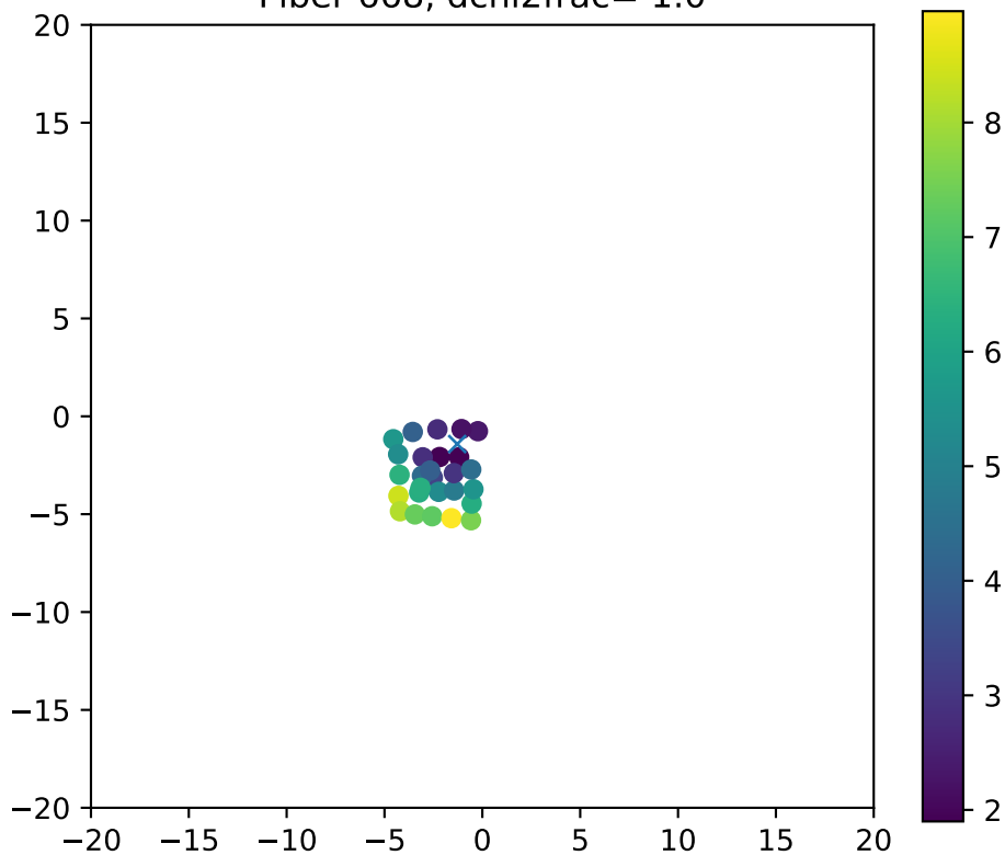
Fiber 668, dchi2frac= 1.0
