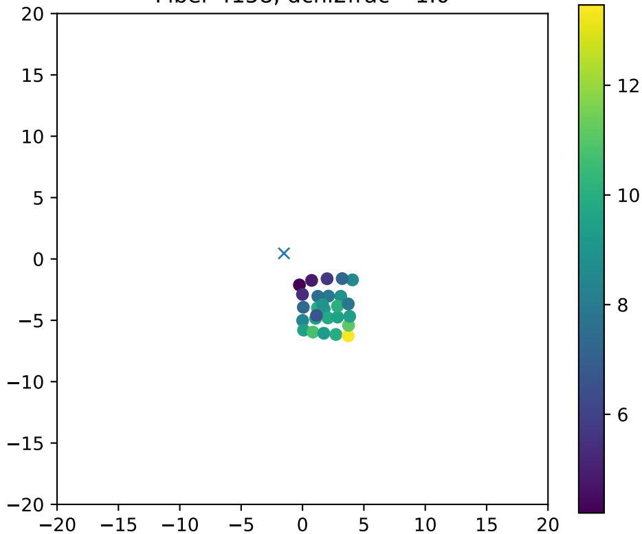
Fiber 4158, dchi2frac= 1.0
