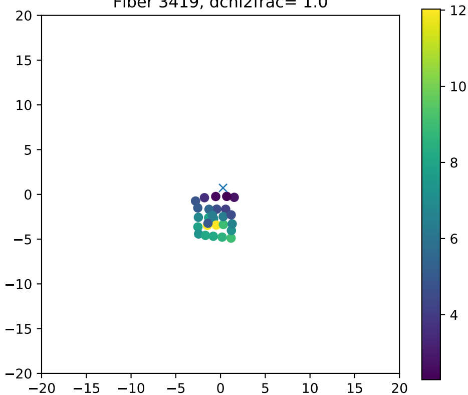
Fiber 3419, dchi2frac= 1.0
