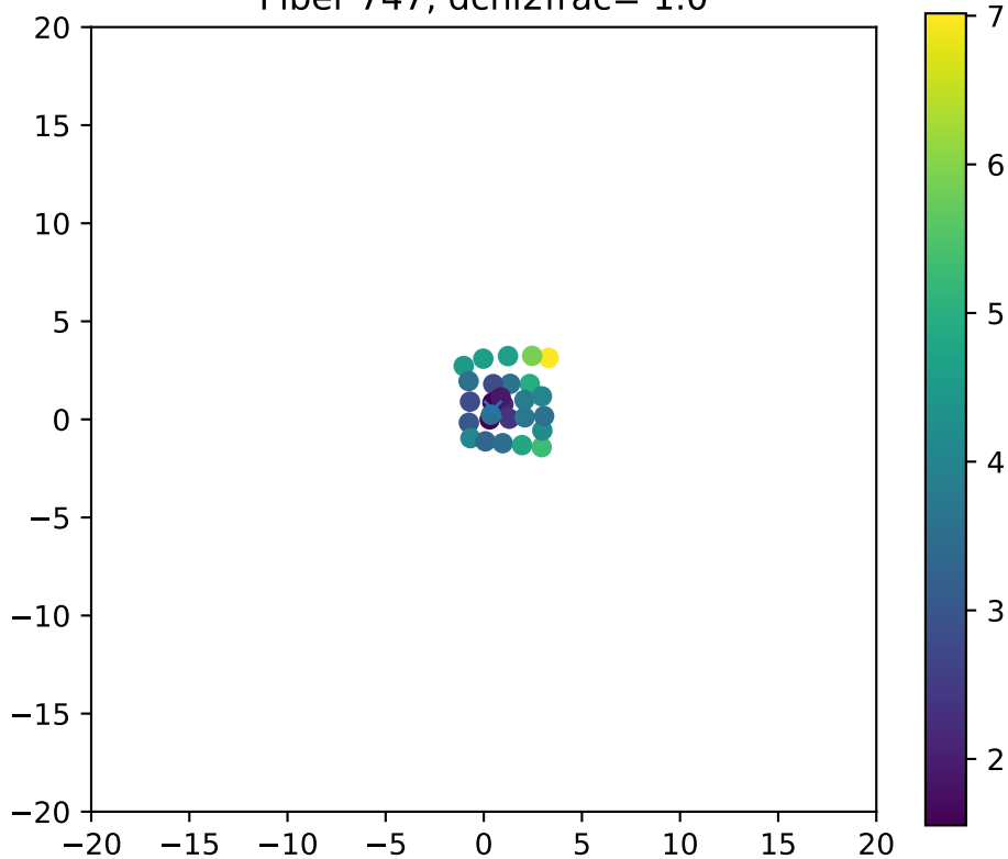
Fiber 747, dchi2frac= 1.0
