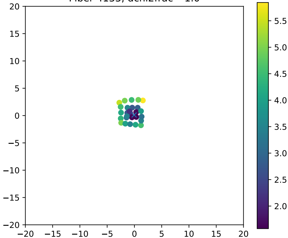
Fiber 4133, dchi2frac= 1.0
