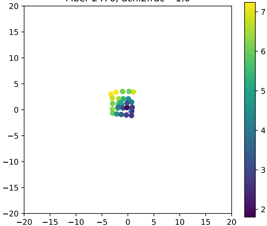
Fiber 2476, dchi2frac= 1.0
