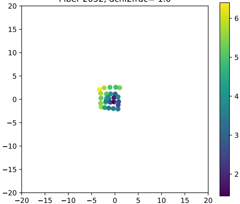
Fiber 2052, dchi2frac= 1.0
