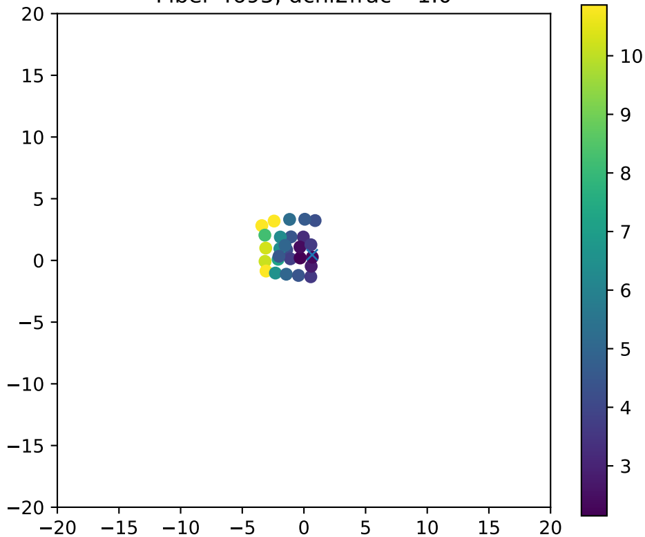
Fiber 4695, dchi2frac= 1.0
