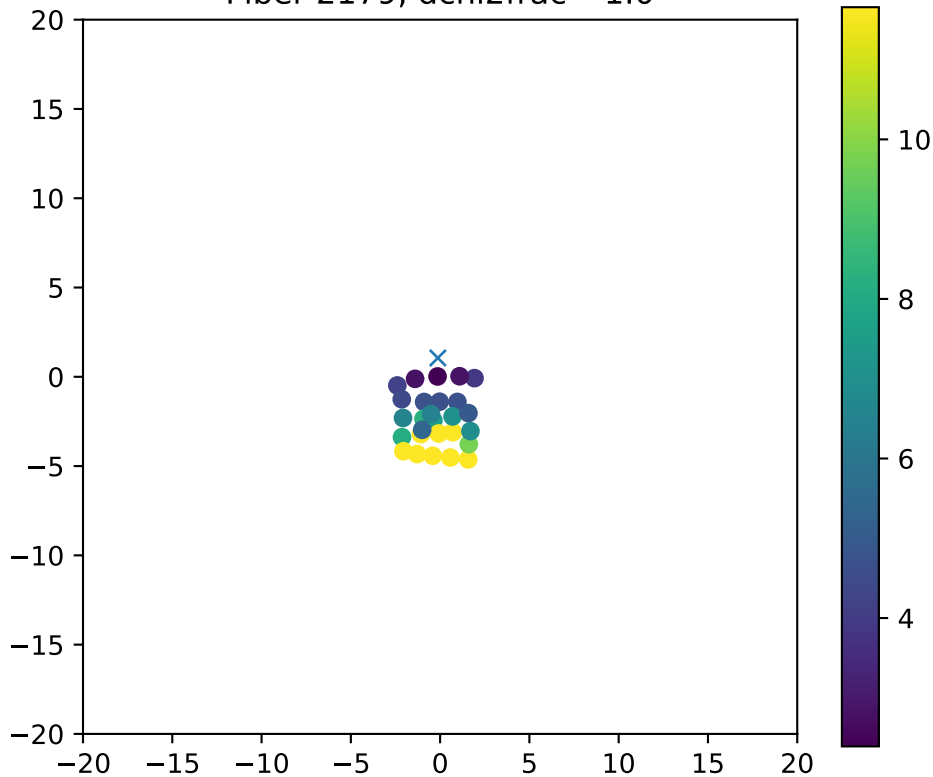
Fiber 2179, dchi2frac= 1.0
