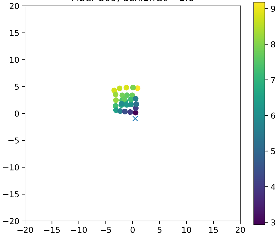
Fiber 809, dchi2frac= 1.0
