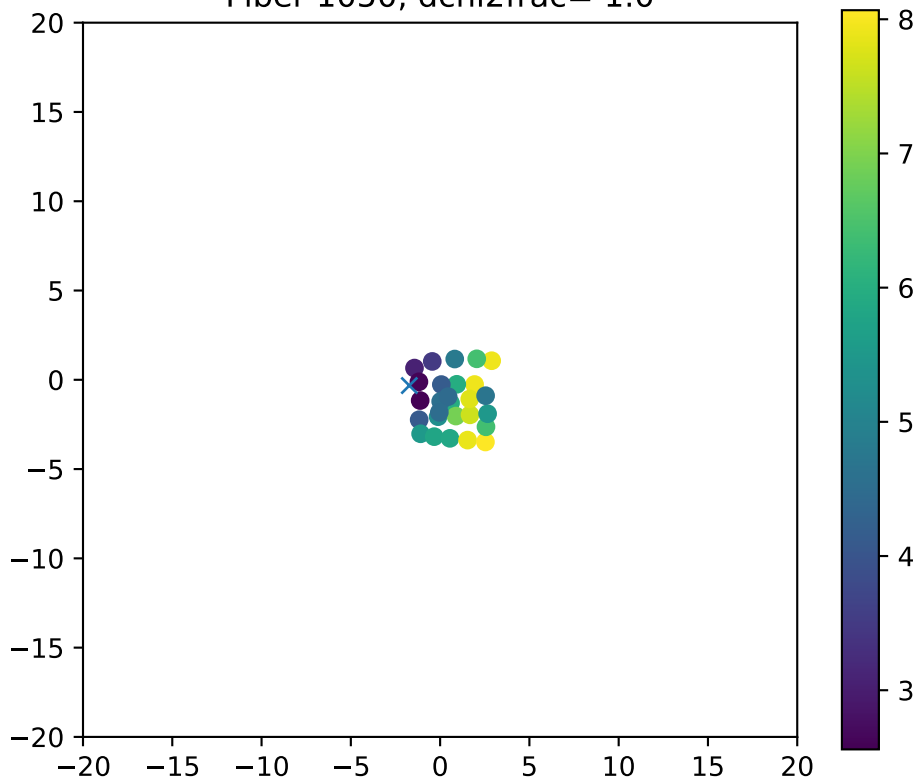
Fiber 1050, dchi2frac= 1.0
