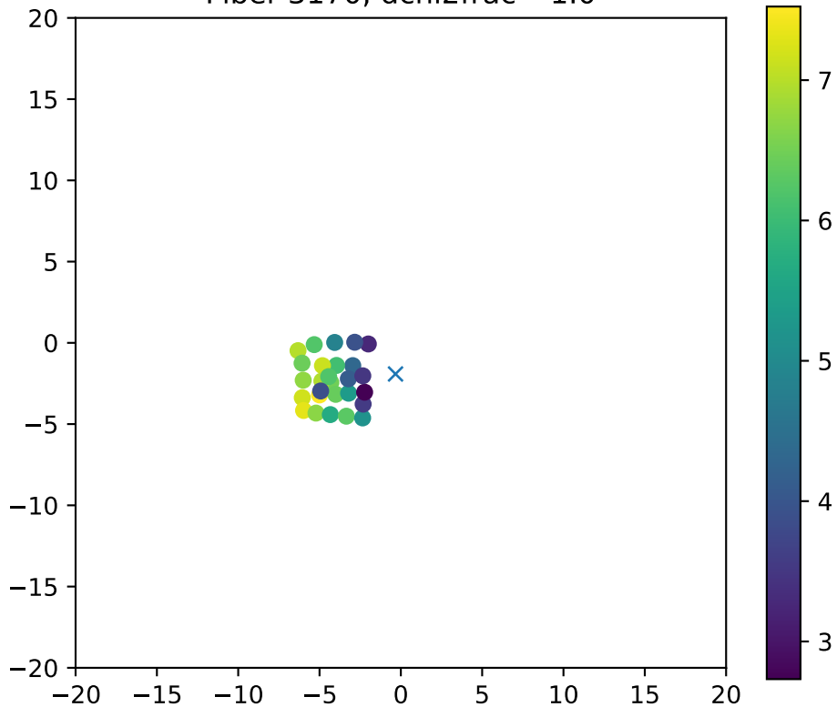
Fiber 3170, dchi2frac= 1.0
