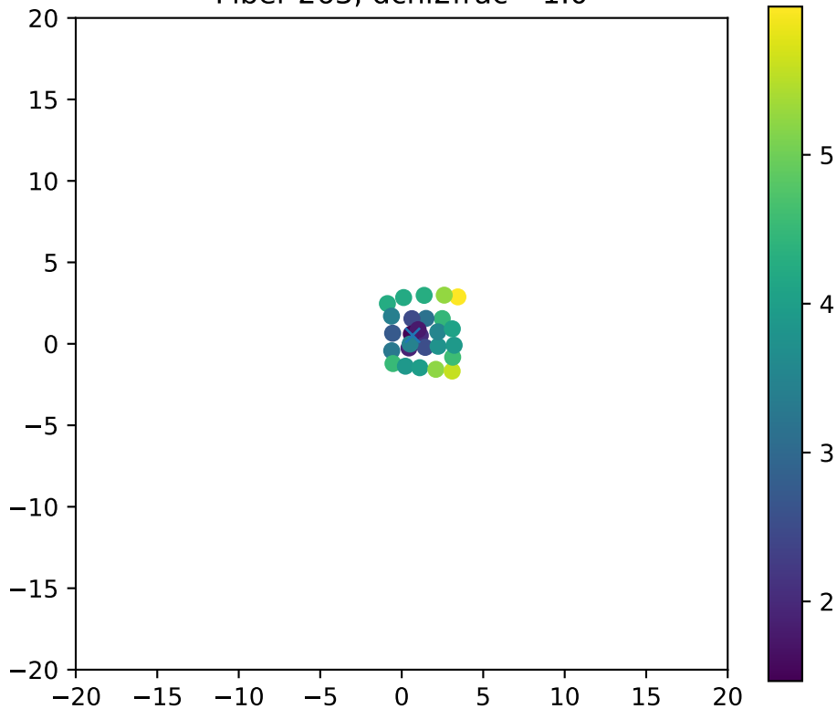
Fiber 263, dchi2frac= 1.0
