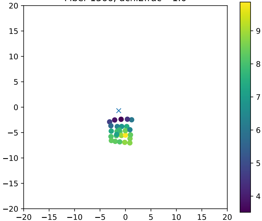
Fiber 1366, dchi2frac= 1.0
