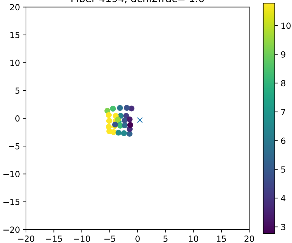
Fiber 4194, dchi2frac= 1.0
