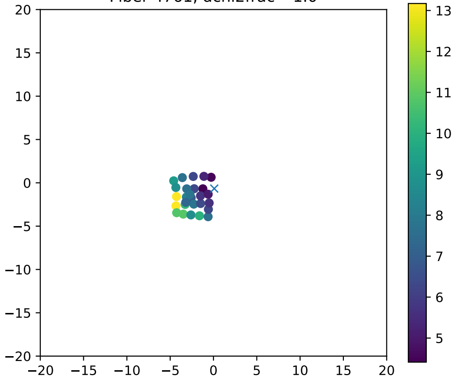
Fiber 4761, dchi2frac= 1.0
