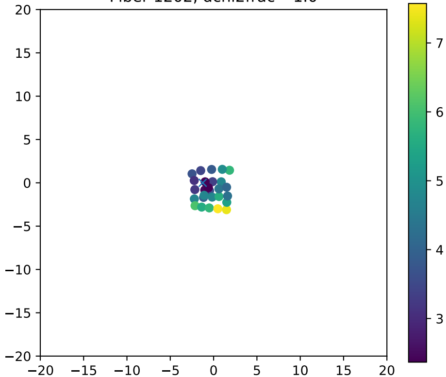
Fiber 1202, dchi2frac= 1.0
