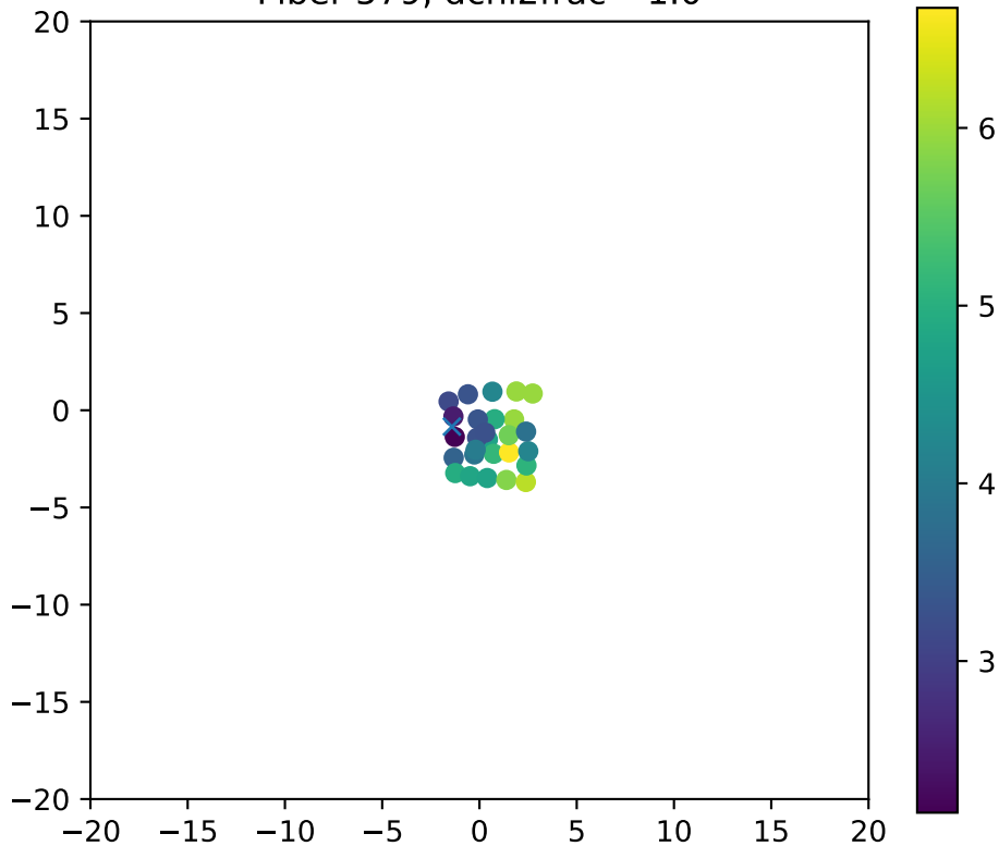
Fiber 579, dchi2frac= 1.0
