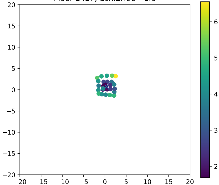
Fiber 1427, dchi2frac= 1.0
