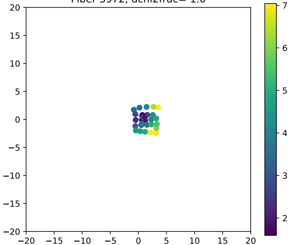
Fiber 3972, dchi2frac= 1.0
