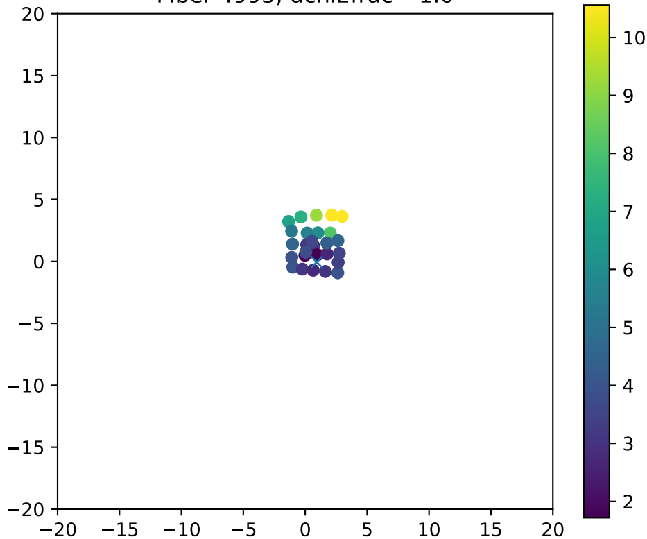
Fiber 4993, dchi2frac= 1.0
