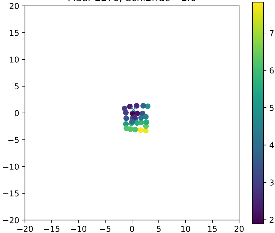
Fiber 2270, dchi2frac= 1.0
