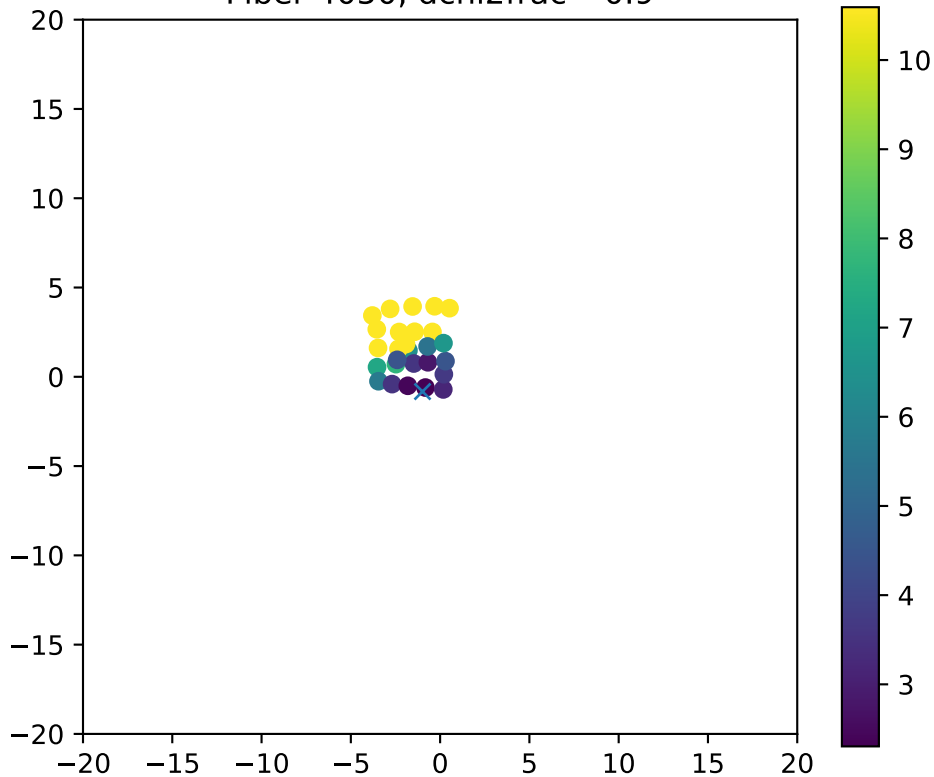
Fiber 4050, dchi2frac= 0.9
