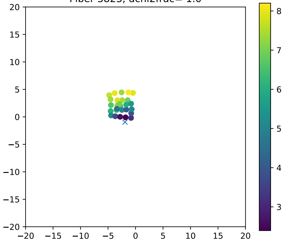
Fiber 3823, dchi2frac= 1.0
