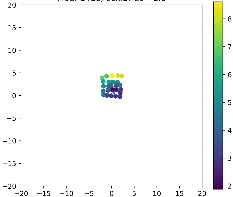
Fiber 1418, dchi2frac= 1.0
