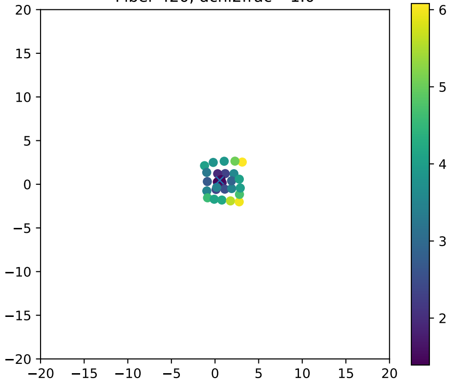
Fiber 420, dchi2frac= 1.0
