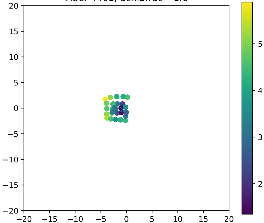
Fiber 4461, dchi2frac= 1.0
