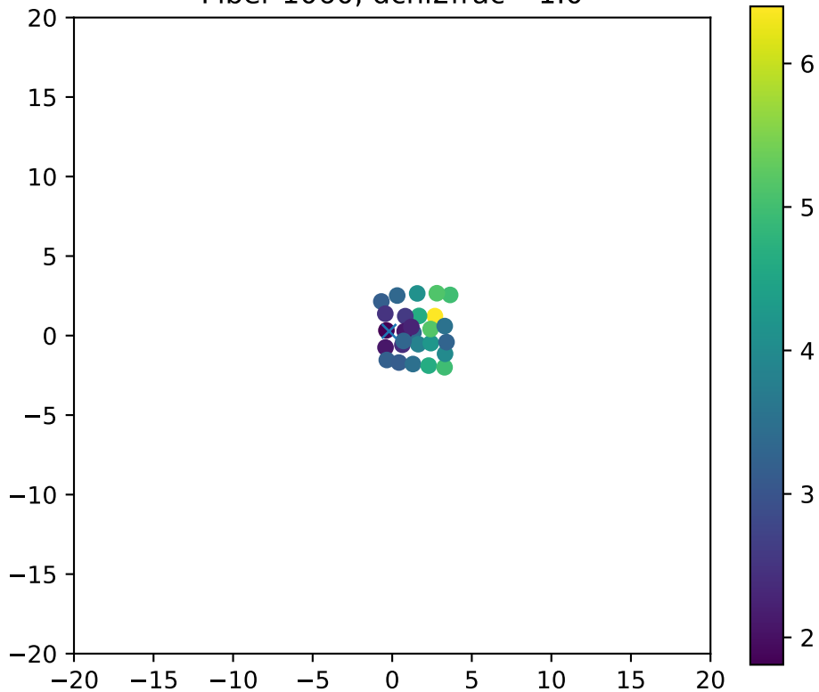
Fiber 1060, dchi2frac= 1.0
