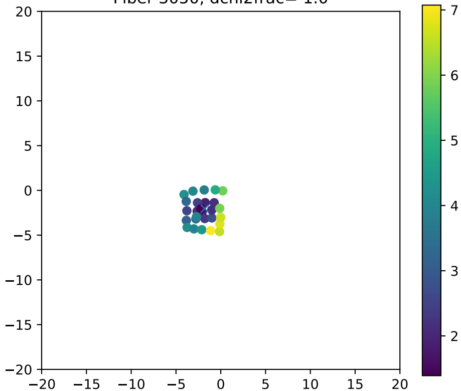
Fiber 3050, dchi2frac= 1.0
