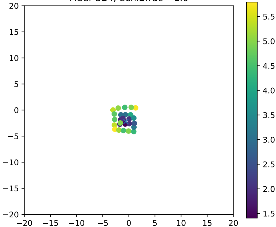
Fiber 524, dchi2frac= 1.0
