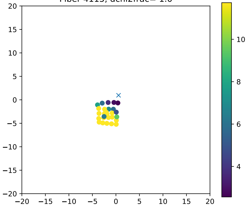
Fiber 4115, dchi2frac= 1.0
