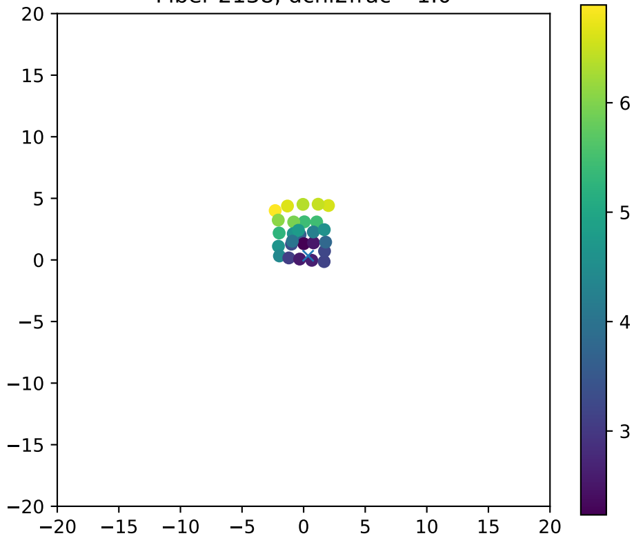
Fiber 2138, dchi2frac= 1.0
