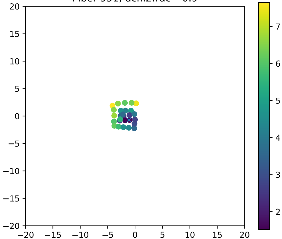
Fiber 951, dchi2frac= 0.9
