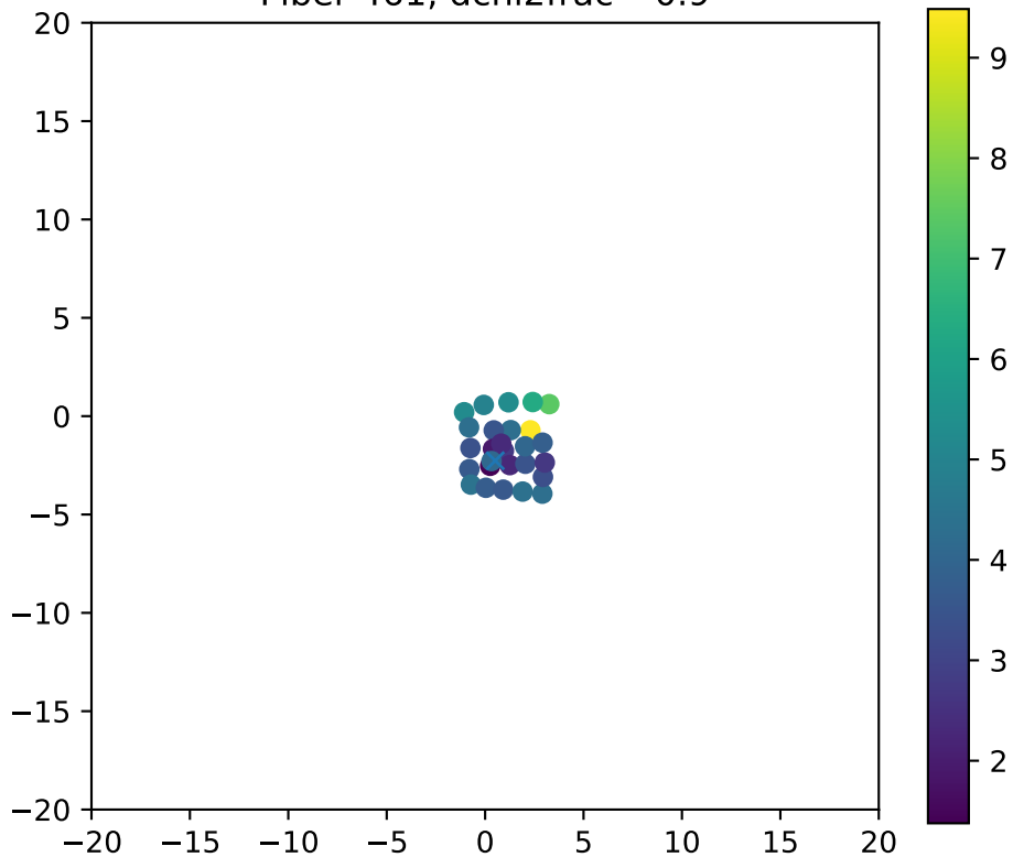
Fiber 461, dchi2frac= 0.9
