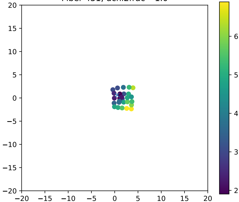
Fiber 431, dchi2frac= 1.0
