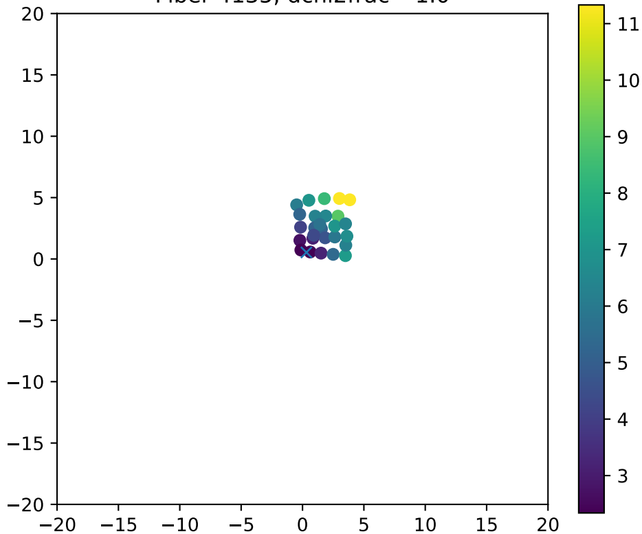
Fiber 4135, dchi2frac= 1.0
