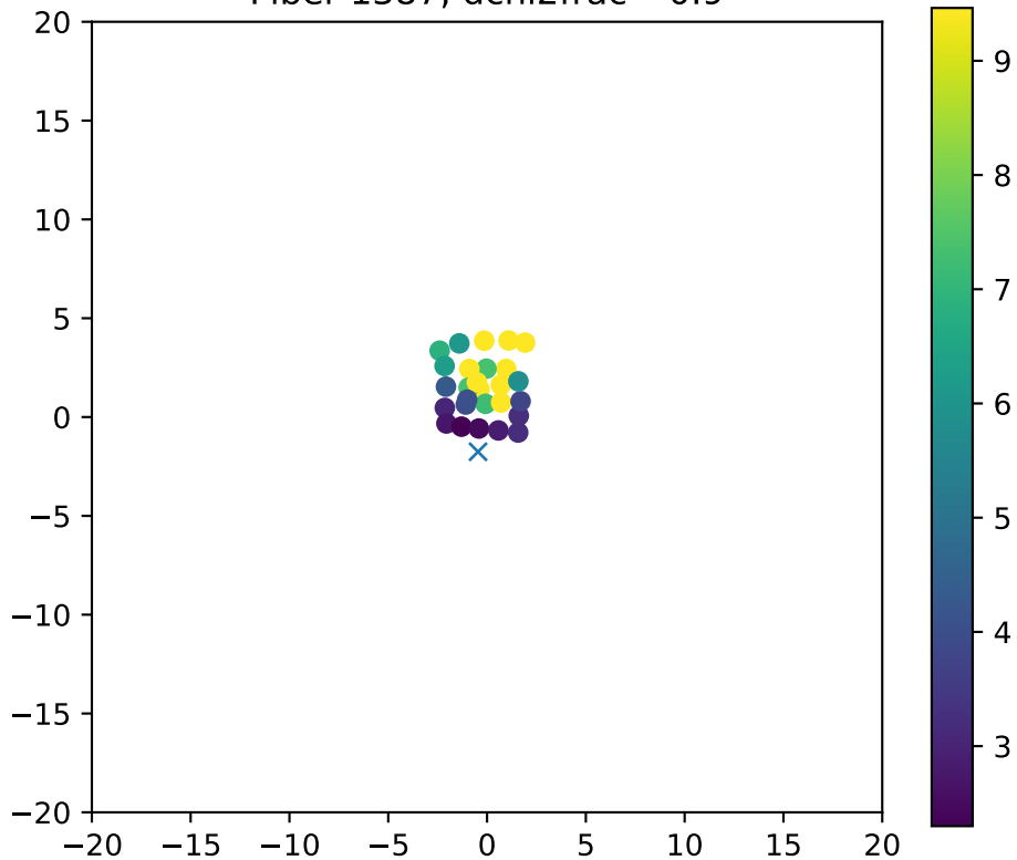
Fiber 1387, dchi2frac= 0.9
