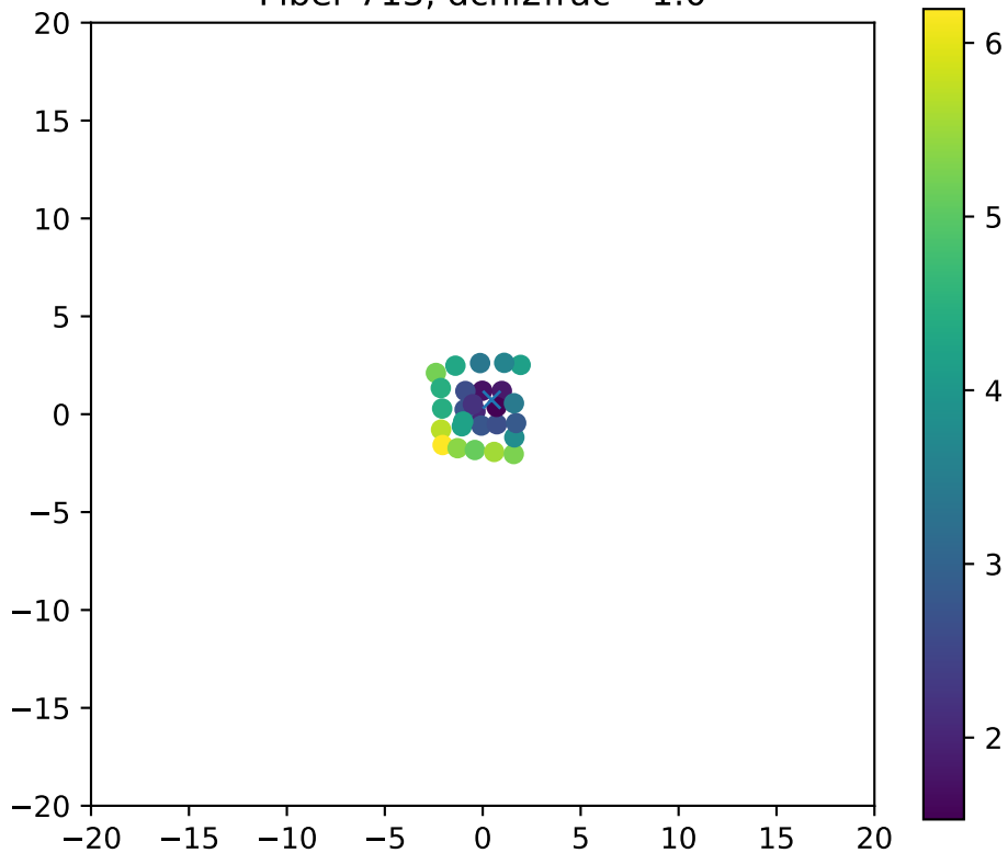
Fiber 713, dchi2frac= 1.0
