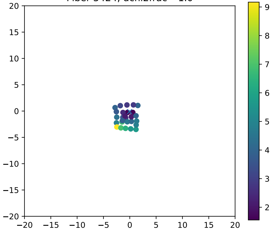
Fiber 3424, dchi2frac= 1.0
