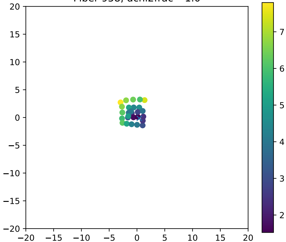
Fiber 958, dchi2frac= 1.0
