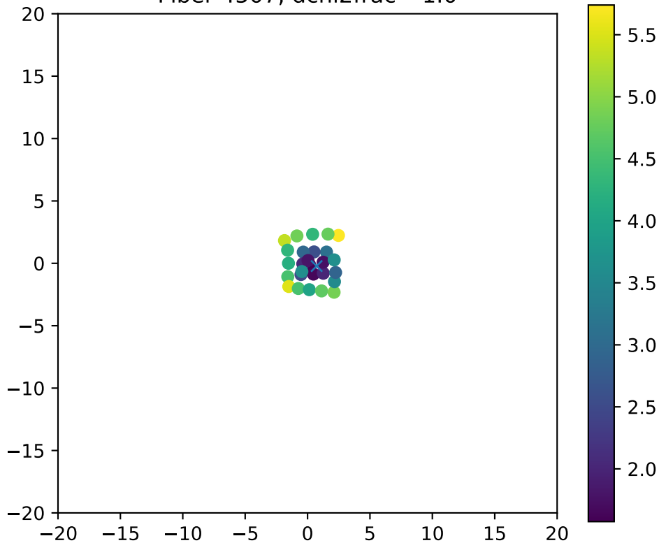
Fiber 4507, dchi2frac= 1.0
