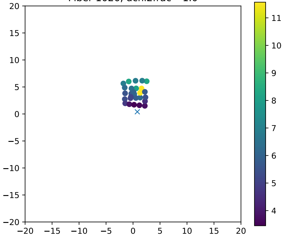
Fiber 1026, dchi2frac= 1.0
