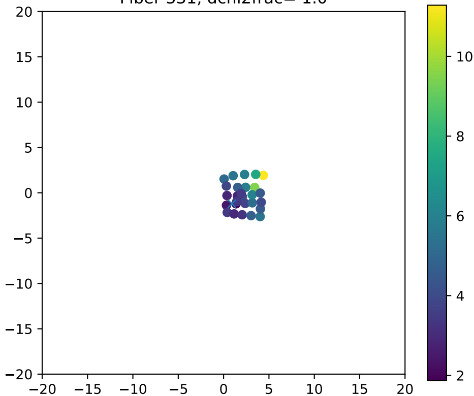
Fiber 331, dchi2frac= 1.0
