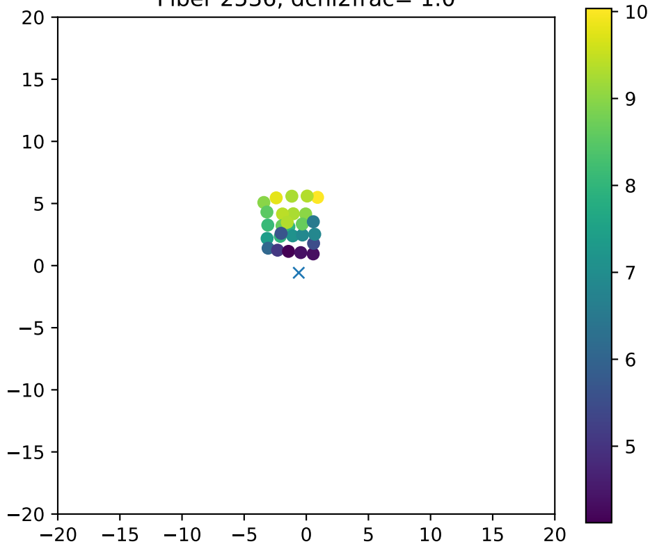
Fiber 2536, dchi2frac= 1.0
