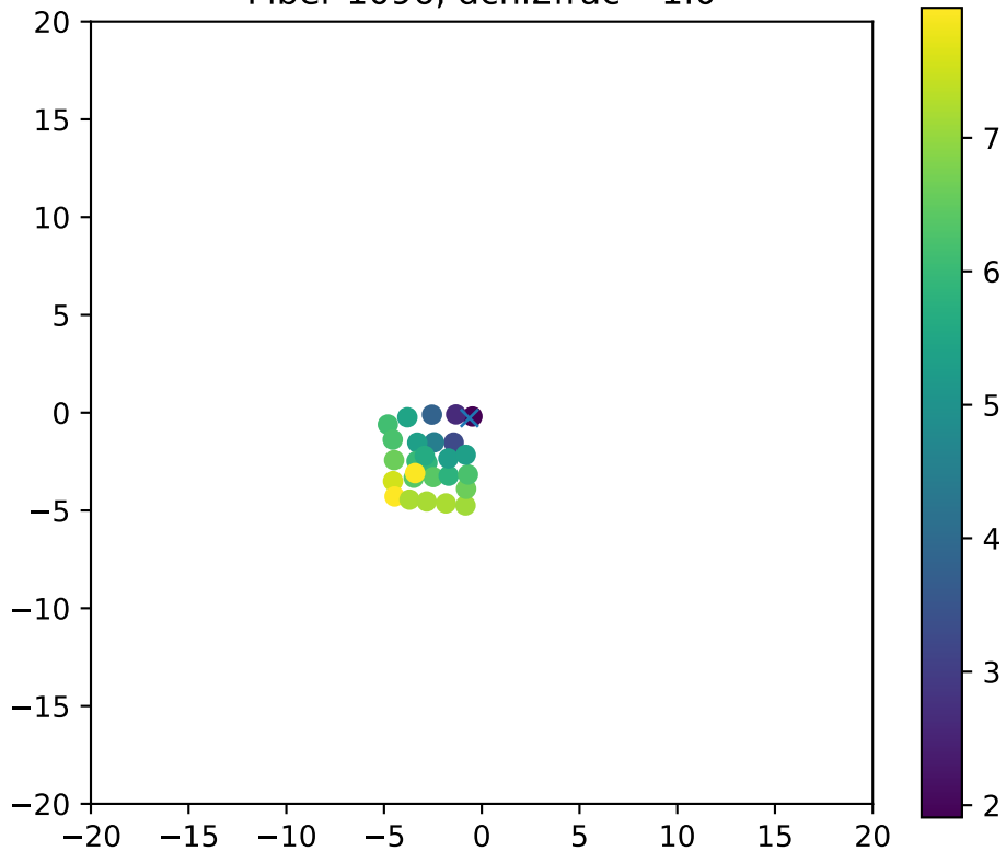
Fiber 1096, dchi2frac= 1.0
