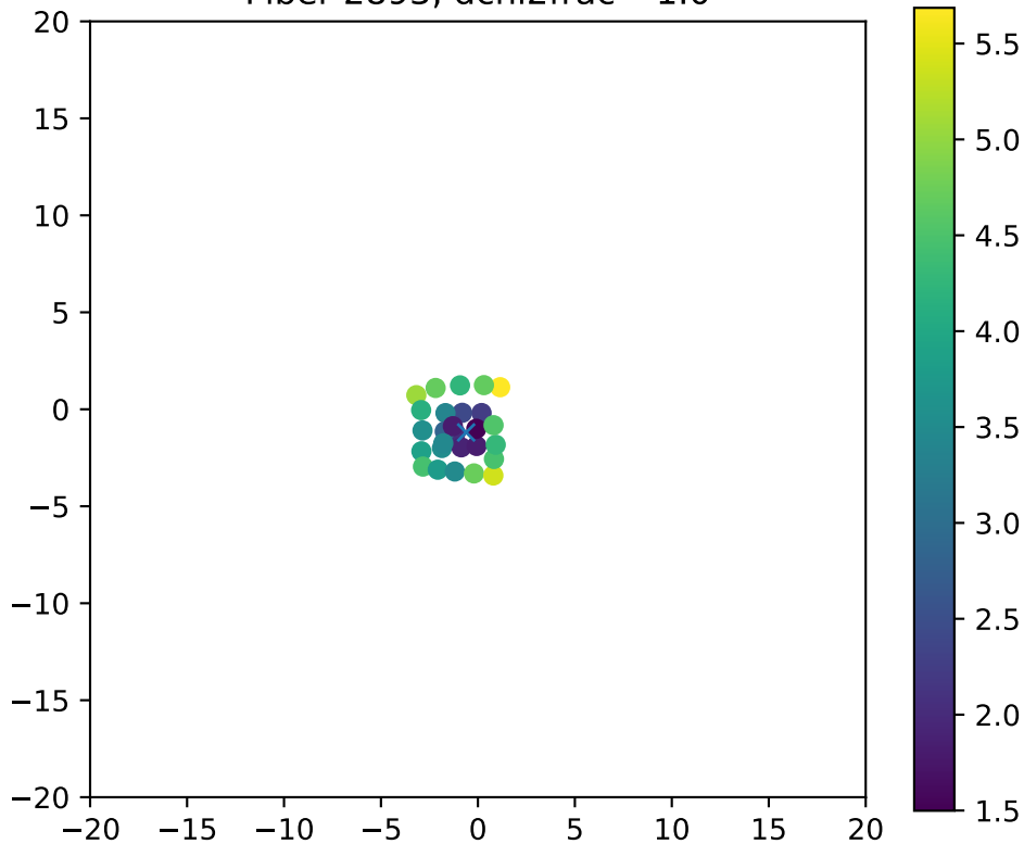
Fiber 2893, dchi2frac= 1.0
