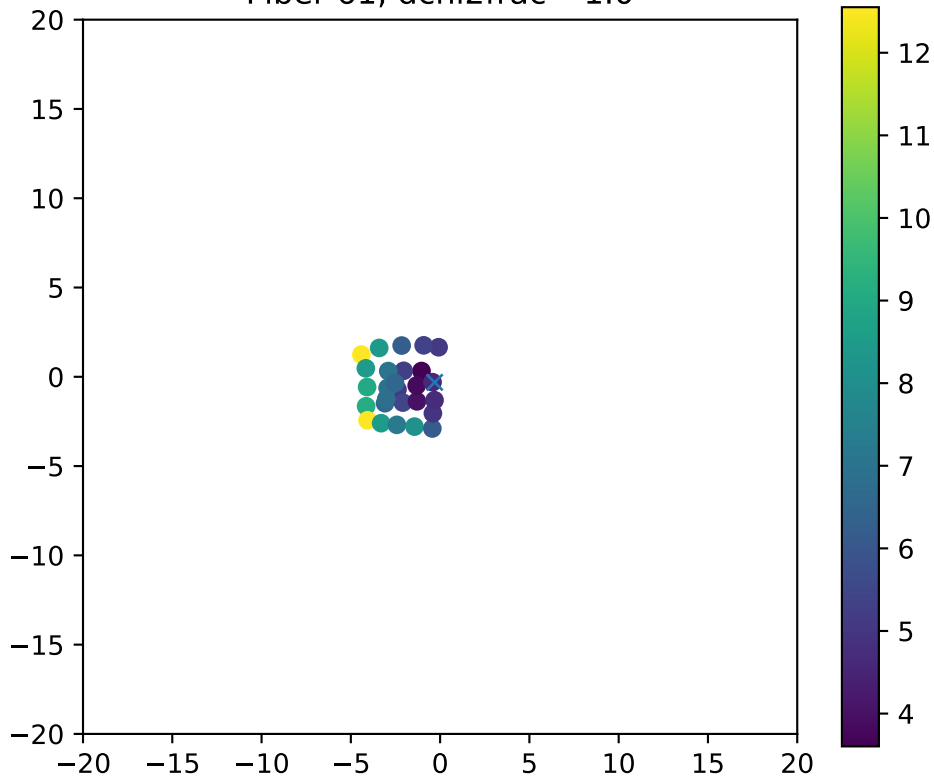
Fiber 61, dchi2frac= 1.0
