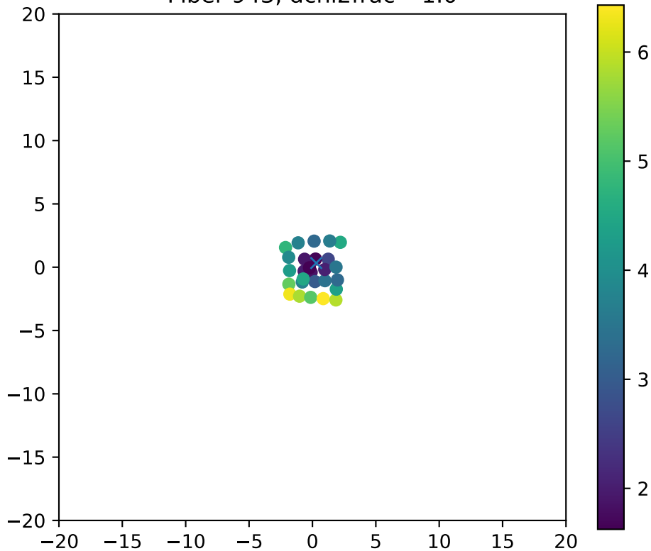
Fiber 943, dchi2frac= 1.0
