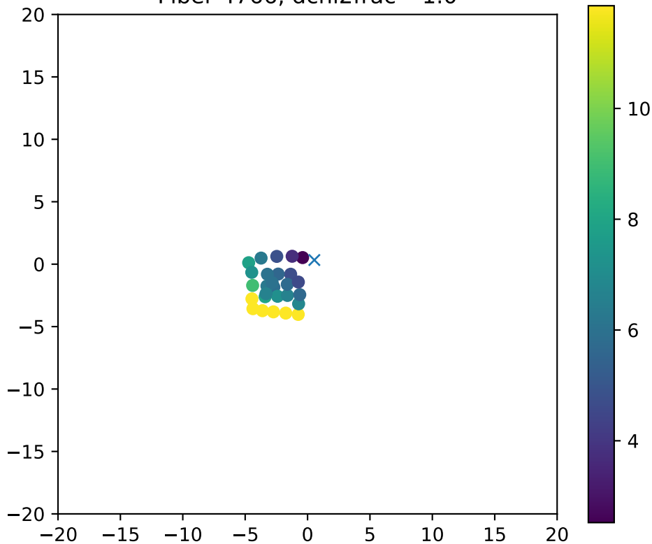
Fiber 4766, dchi2frac= 1.0
