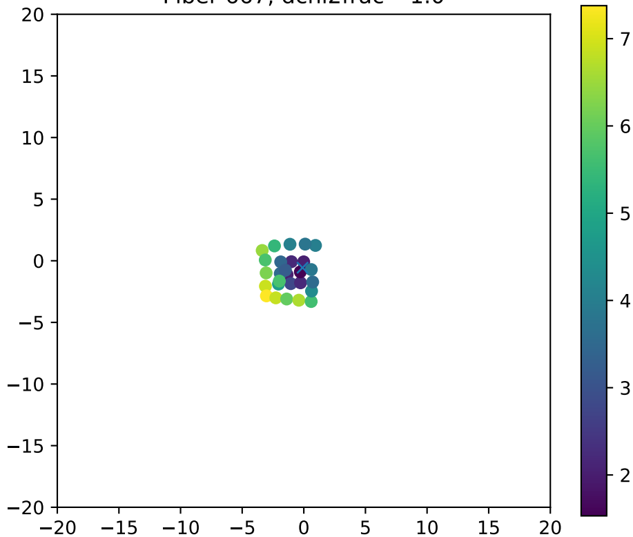
Fiber 667, dchi2frac= 1.0
