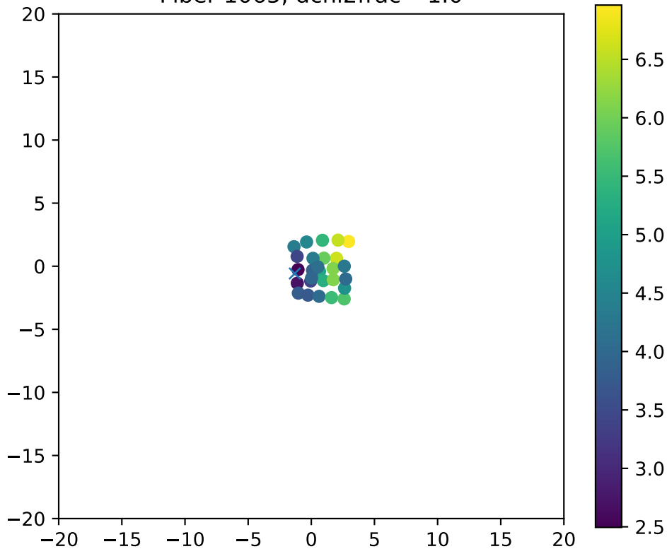
Fiber 1065, dchi2frac= 1.0
