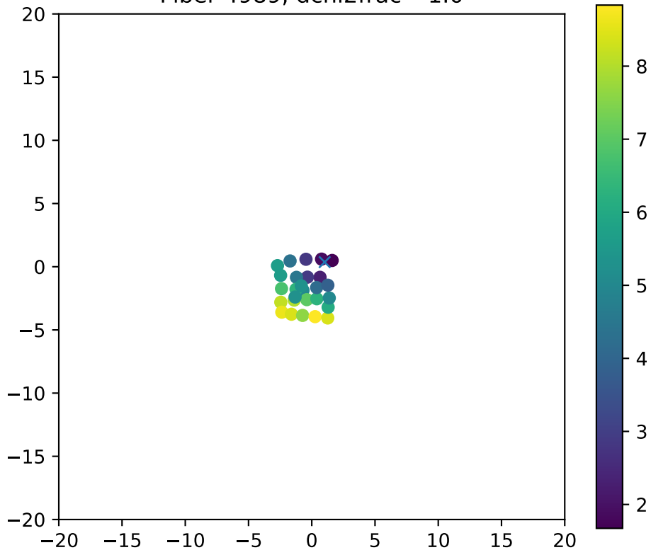
Fiber 4989, dchi2frac= 1.0
