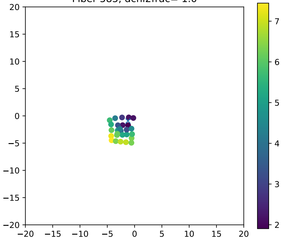
Fiber 585, dchi2frac= 1.0
