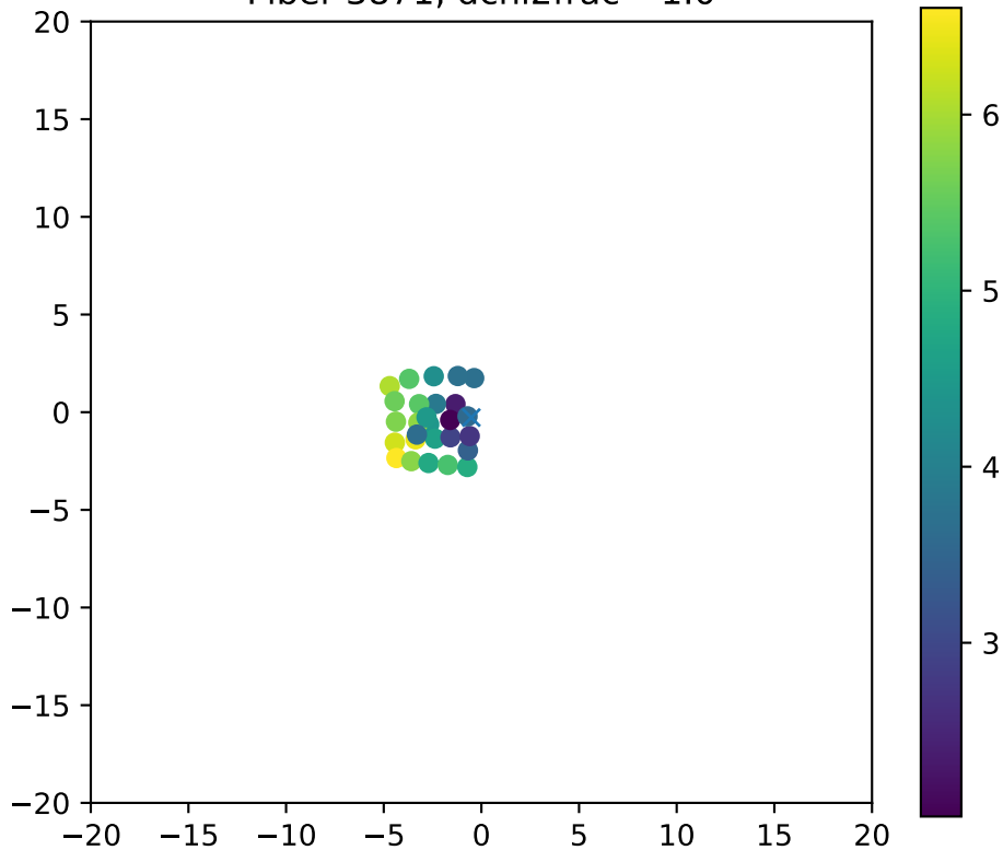
Fiber 3871, dchi2frac= 1.0
