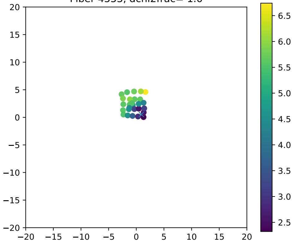
Fiber 4553, dchi2frac= 1.0
