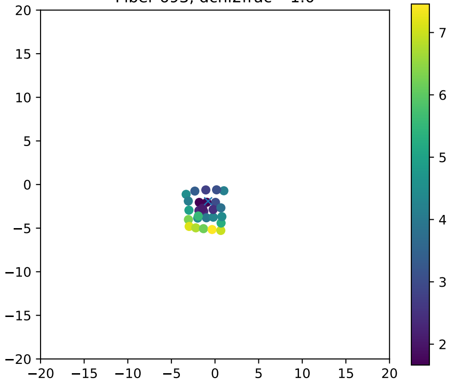
Fiber 693, dchi2frac= 1.0
