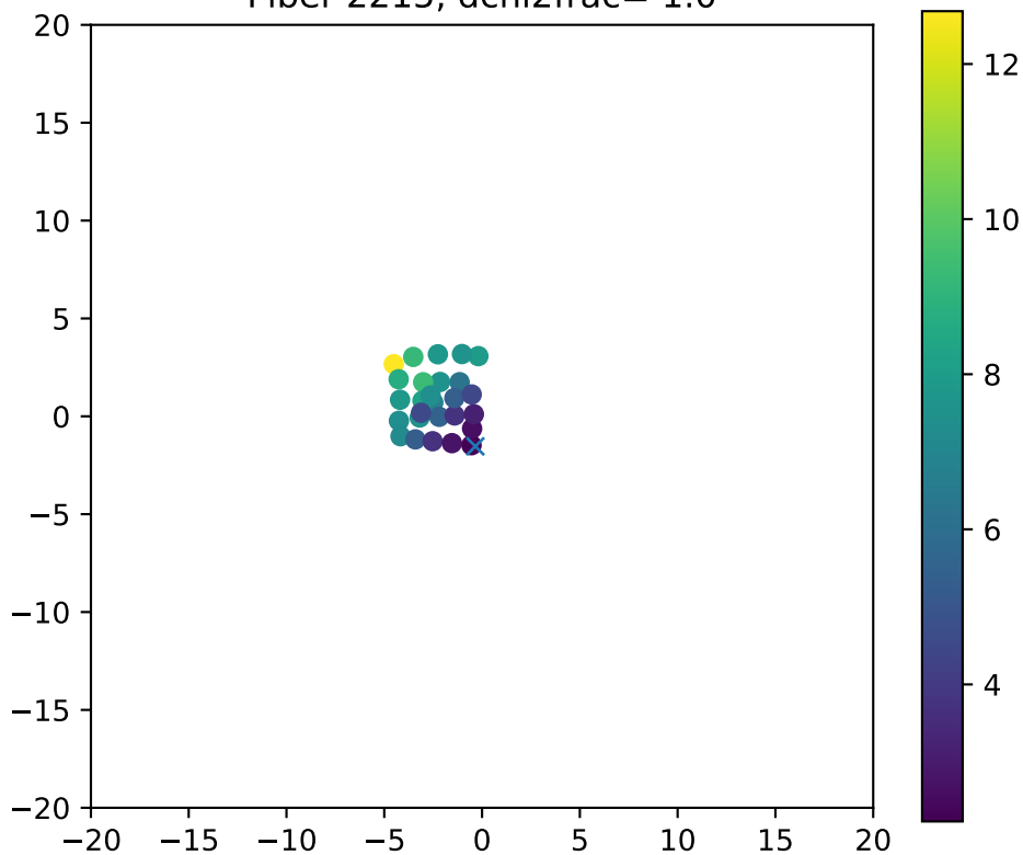
Fiber 2215, dchi2frac= 1.0
