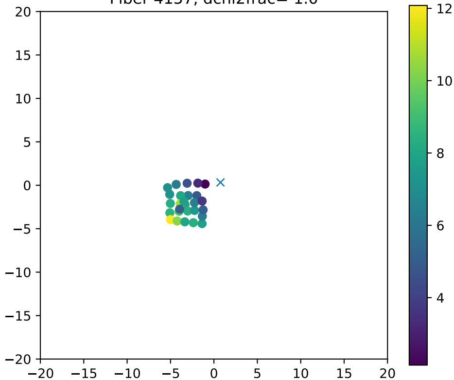
Fiber 4157, dchi2frac= 1.0
