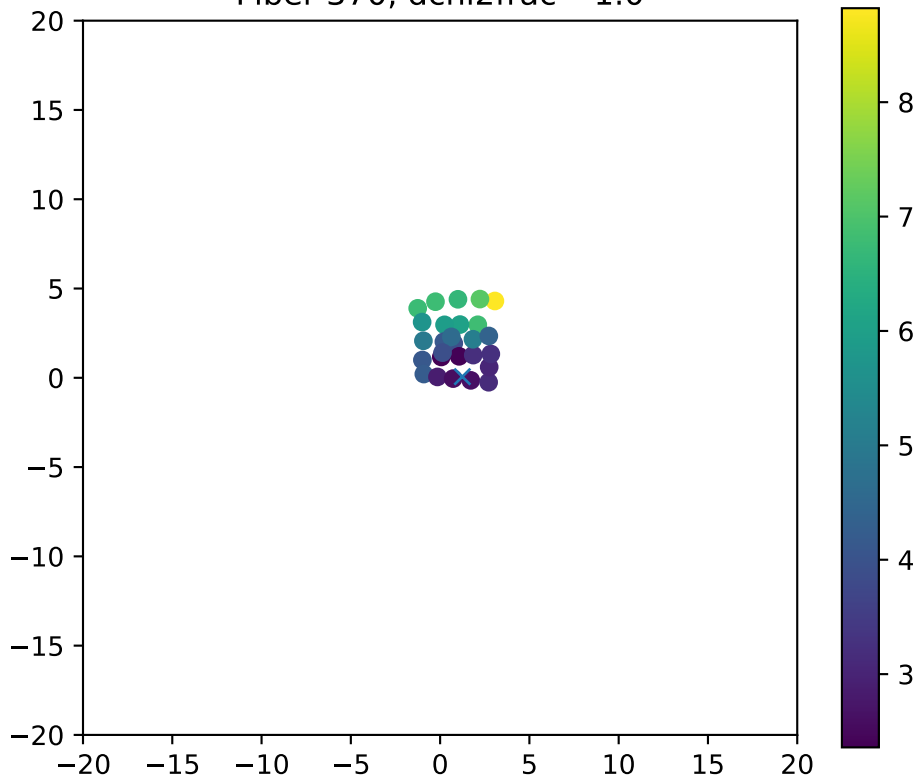
Fiber 370, dchi2frac= 1.0
