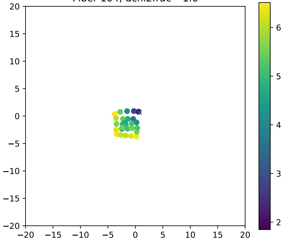
Fiber 104, dchi2frac= 1.0
