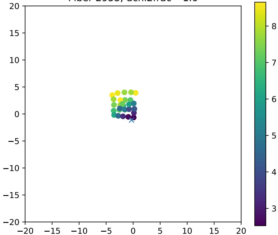
Fiber 2953, dchi2frac= 1.0
