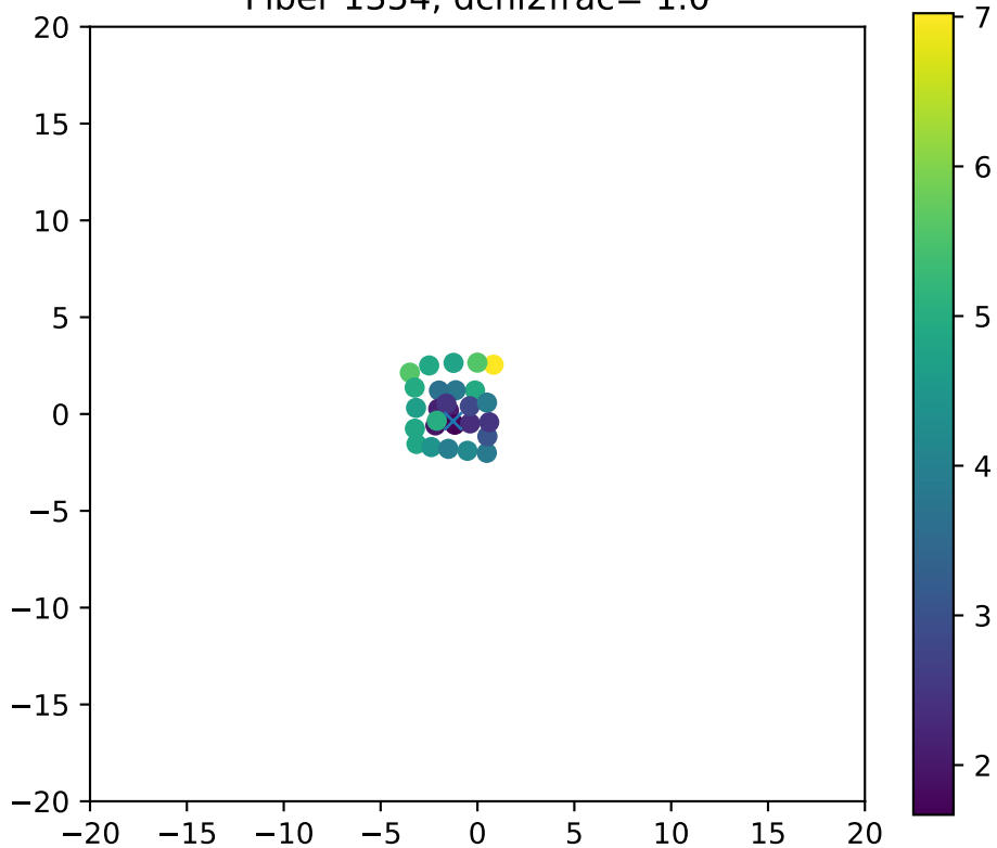
Fiber 1354, dchi2frac= 1.0
