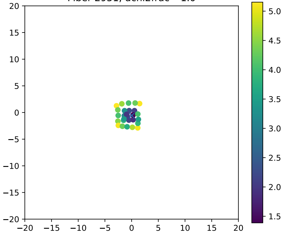
Fiber 2951, dchi2frac= 1.0
