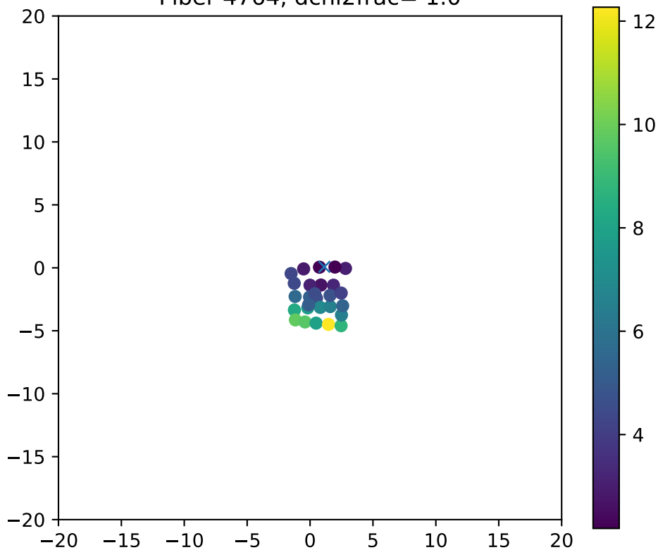
Fiber 4764, dchi2frac= 1.0
