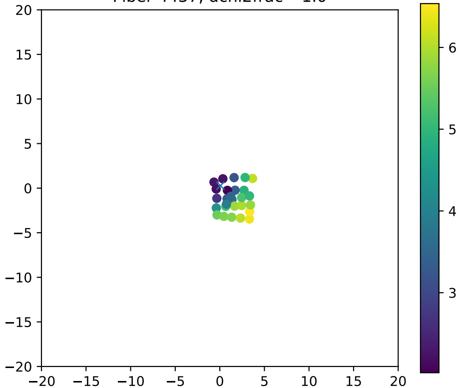
Fiber 4437, dchi2frac= 1.0
