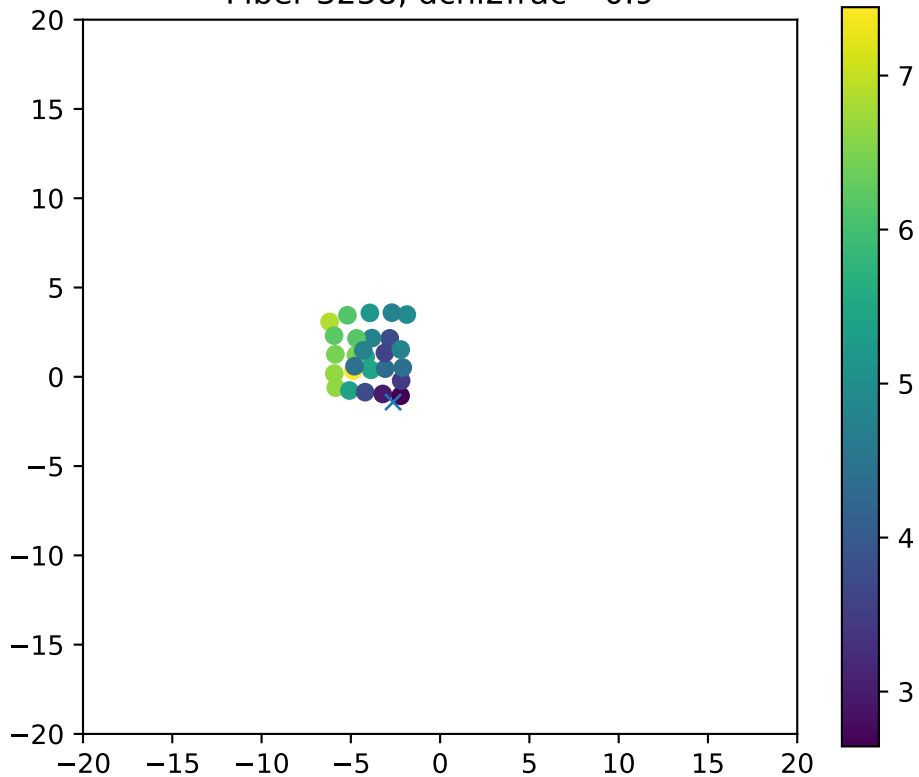
Fiber 3258, dchi2frac= 0.9
