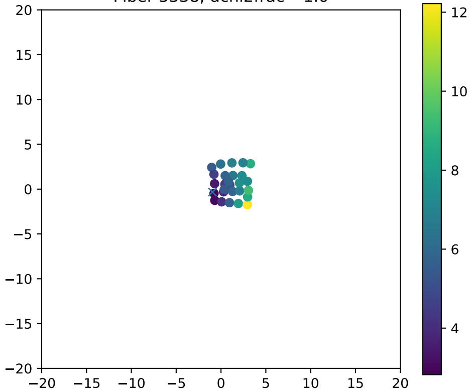
Fiber 3338, dchi2frac= 1.0
