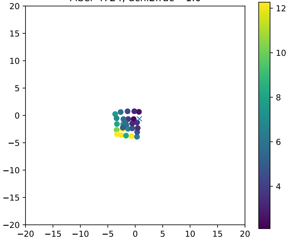
Fiber 4724, dchi2frac= 1.0
