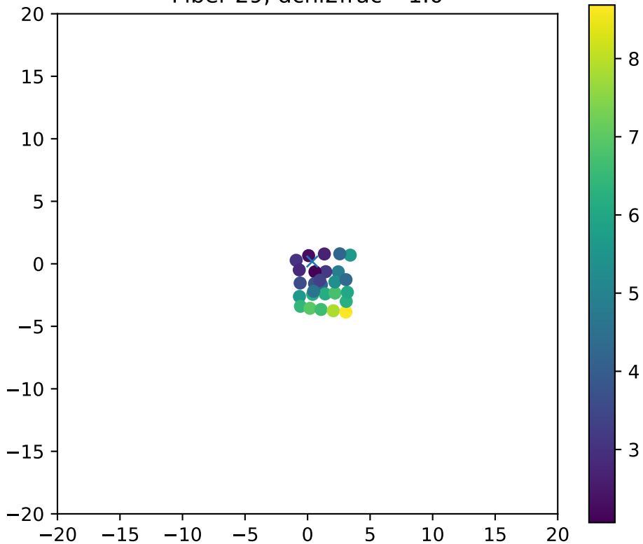
Fiber 29, dchi2frac= 1.0
