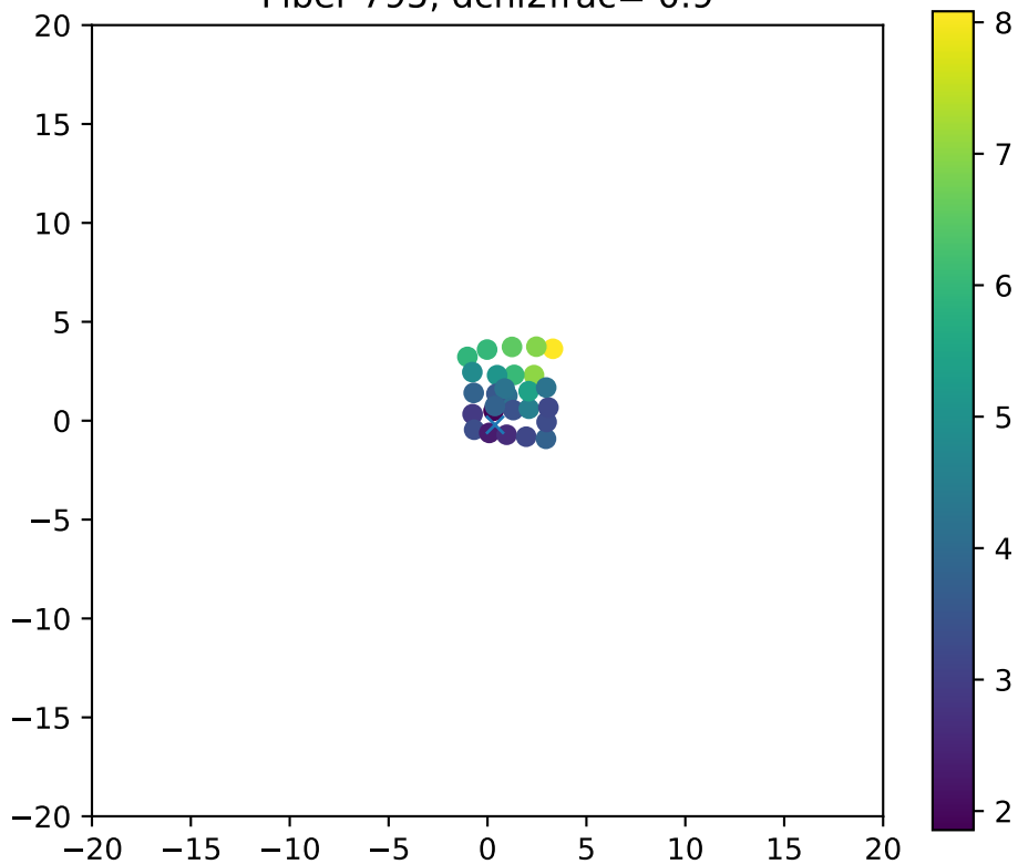
Fiber 795, dchi2frac= 0.9
