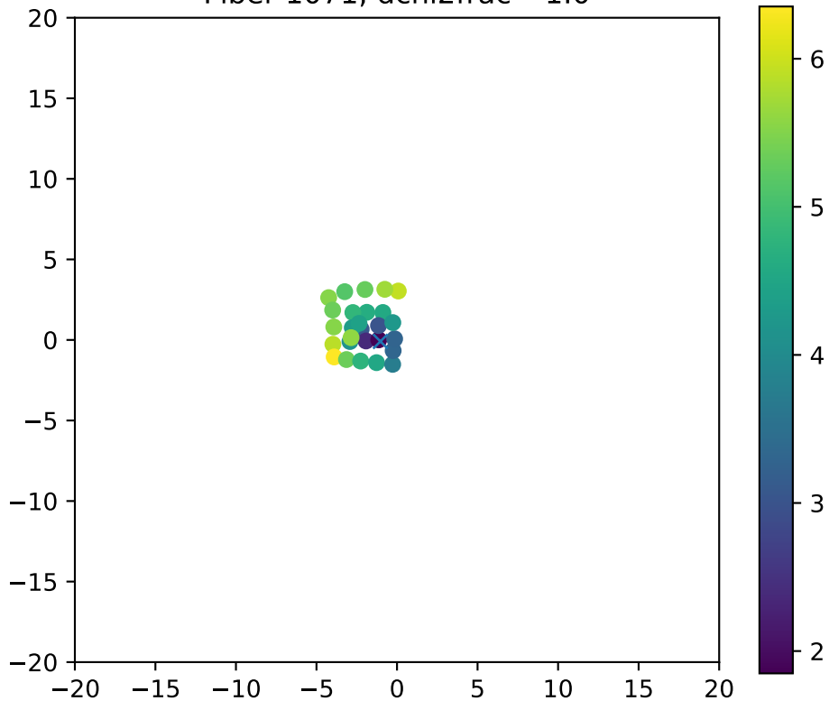
Fiber 1071, dchi2frac= 1.0
