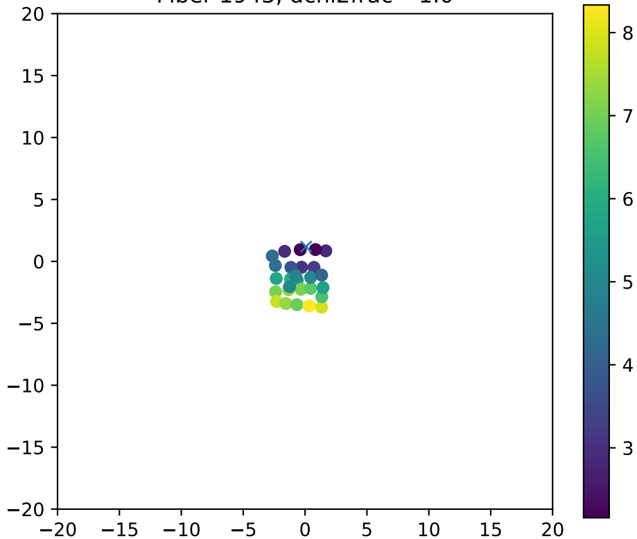
Fiber 1943, dchi2frac= 1.0
