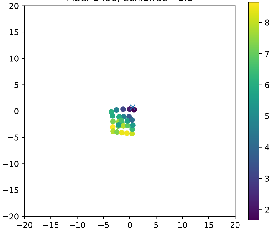
Fiber 2490, dchi2frac= 1.0
