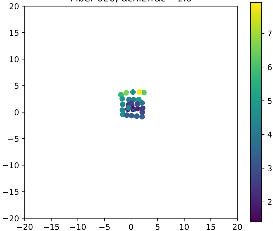
Fiber 620, dchi2frac= 1.0
