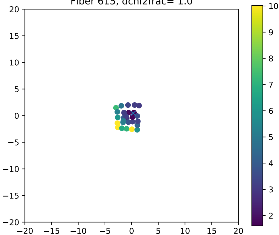
Fiber 615, dchi2frac= 1.0
