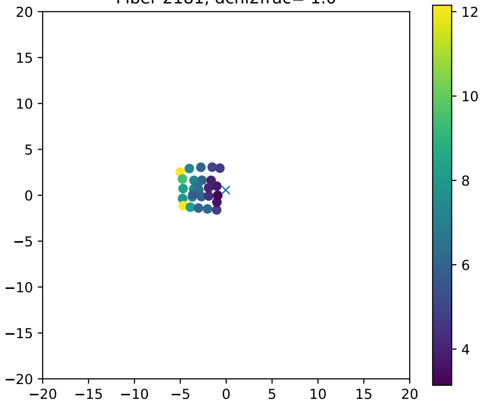
Fiber 2181, dchi2frac= 1.0
