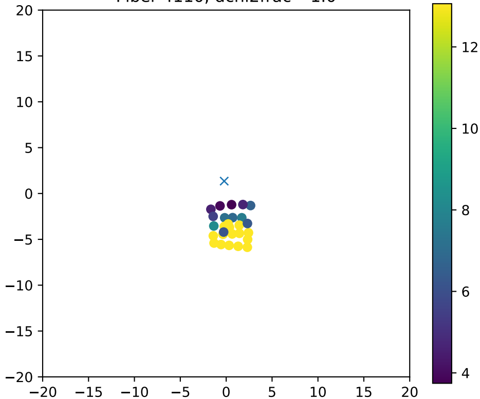
Fiber 4110, dchi2frac= 1.0
