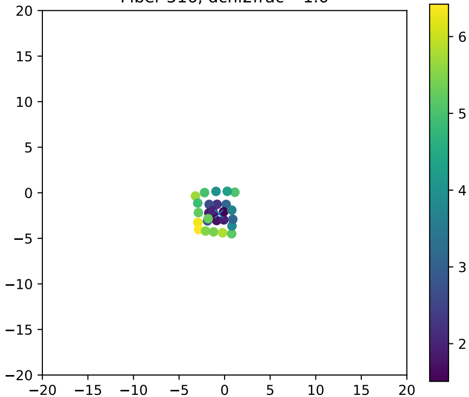
Fiber 516, dchi2frac= 1.0
