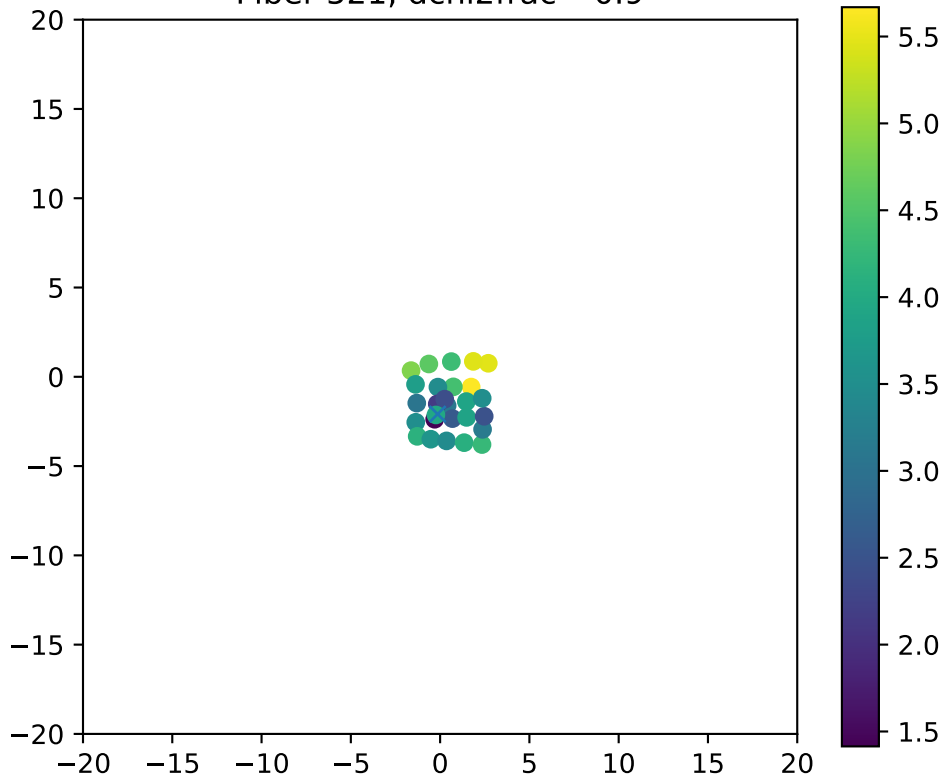
Fiber 521, dchi2frac= 0.9
