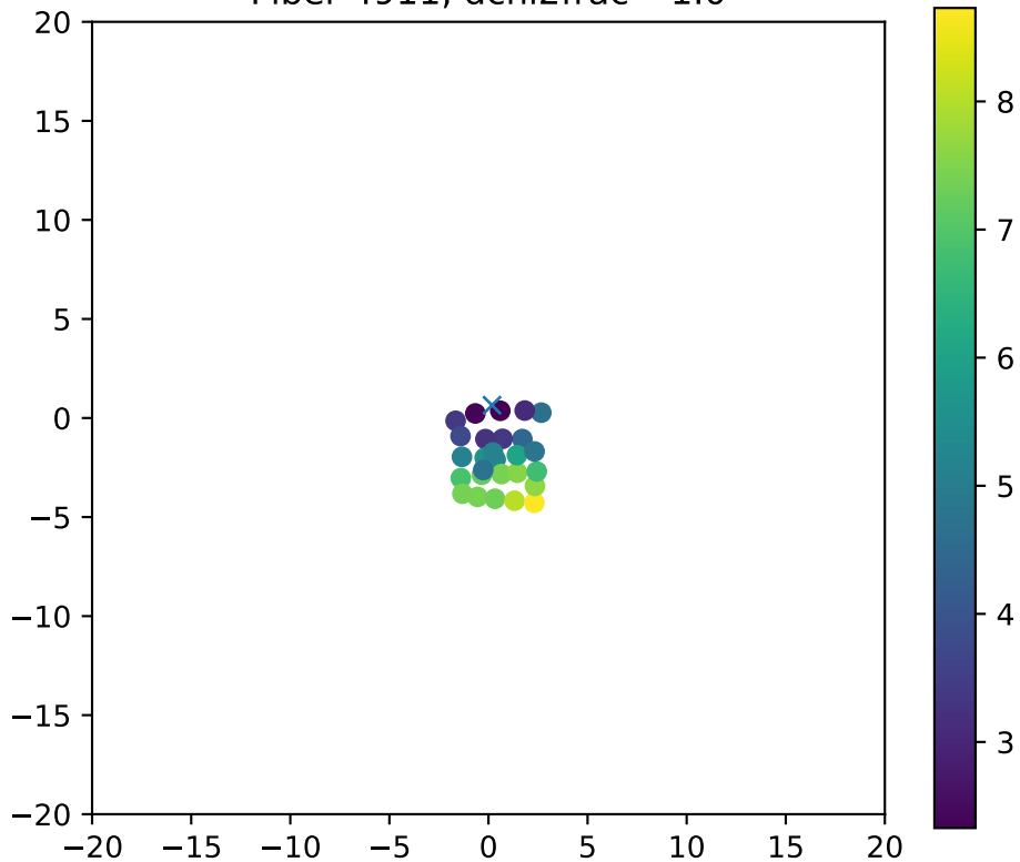
Fiber 4911, dchi2frac= 1.0
