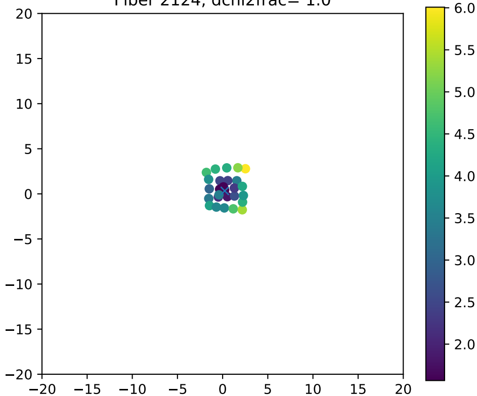
Fiber 2124, dchi2frac= 1.0
