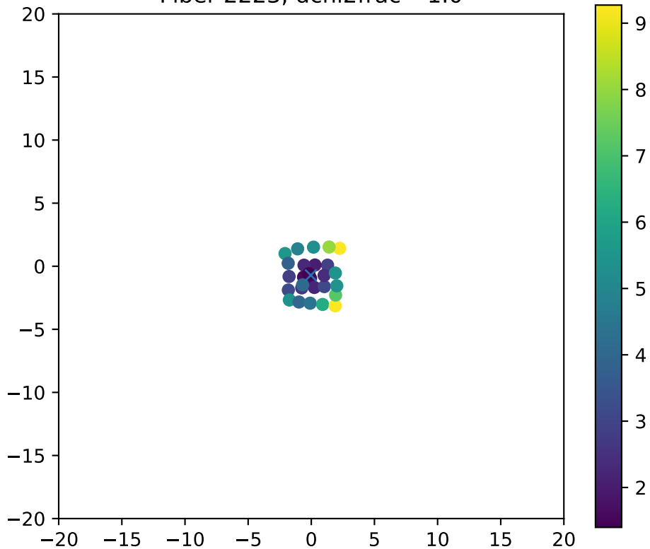
Fiber 2223, dchi2frac= 1.0
