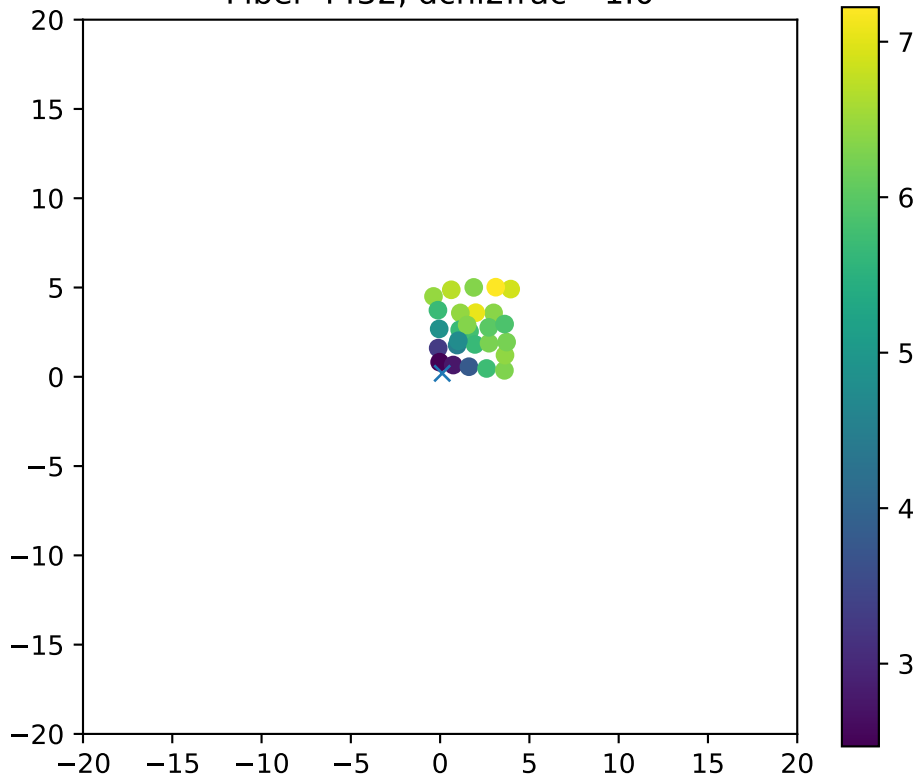
Fiber 4432, dchi2frac= 1.0
