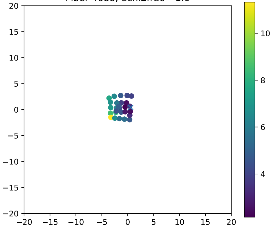
Fiber 4688, dchi2frac= 1.0
