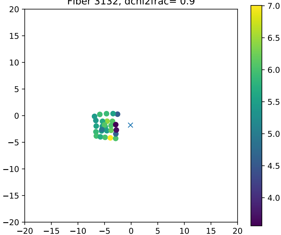
Fiber 3132, dchi2frac= 0.9
