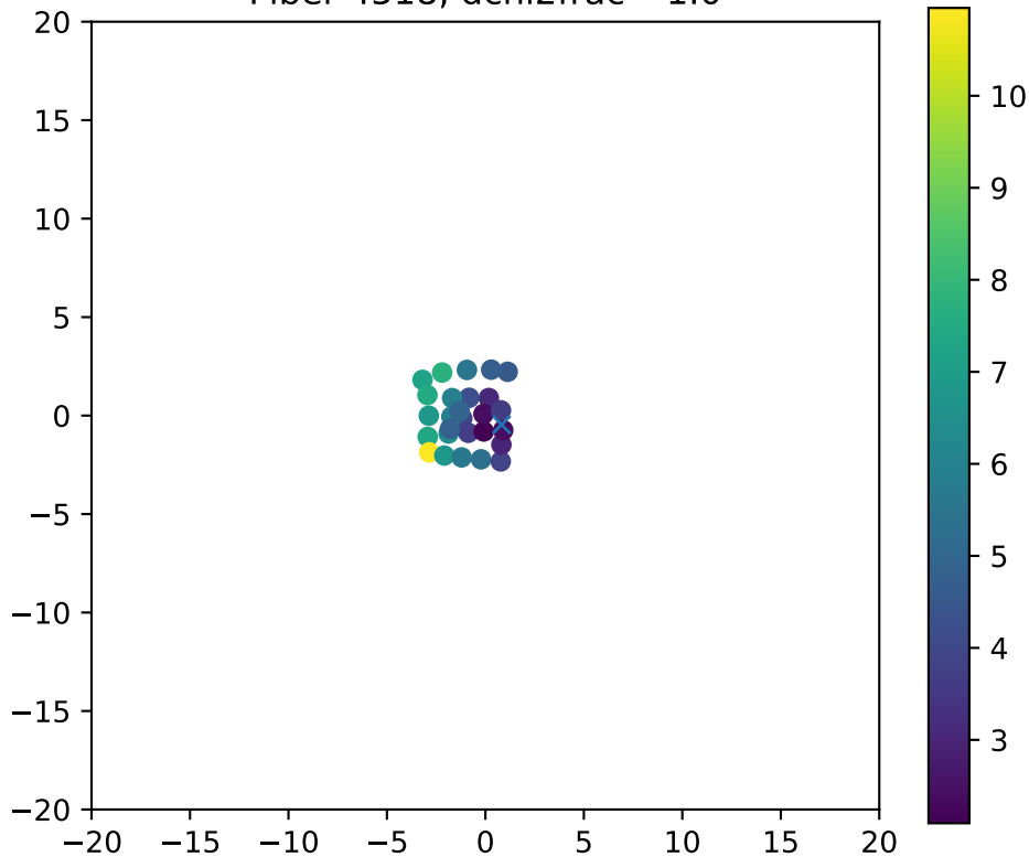
Fiber 4518, dchi2frac= 1.0
