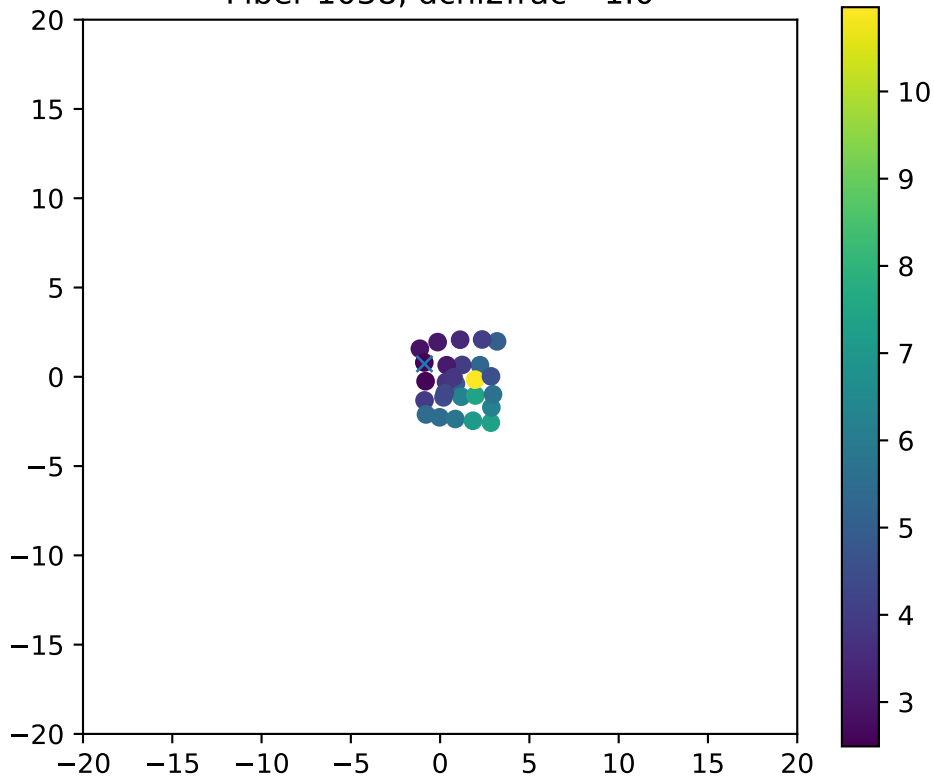
Fiber 1038, dchi2frac= 1.0
