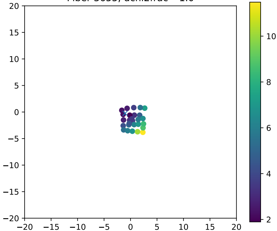
Fiber 3655, dchi2frac= 1.0
