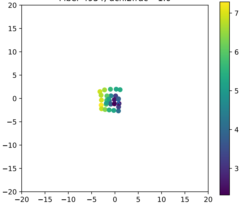
Fiber 4934, dchi2frac= 1.0
