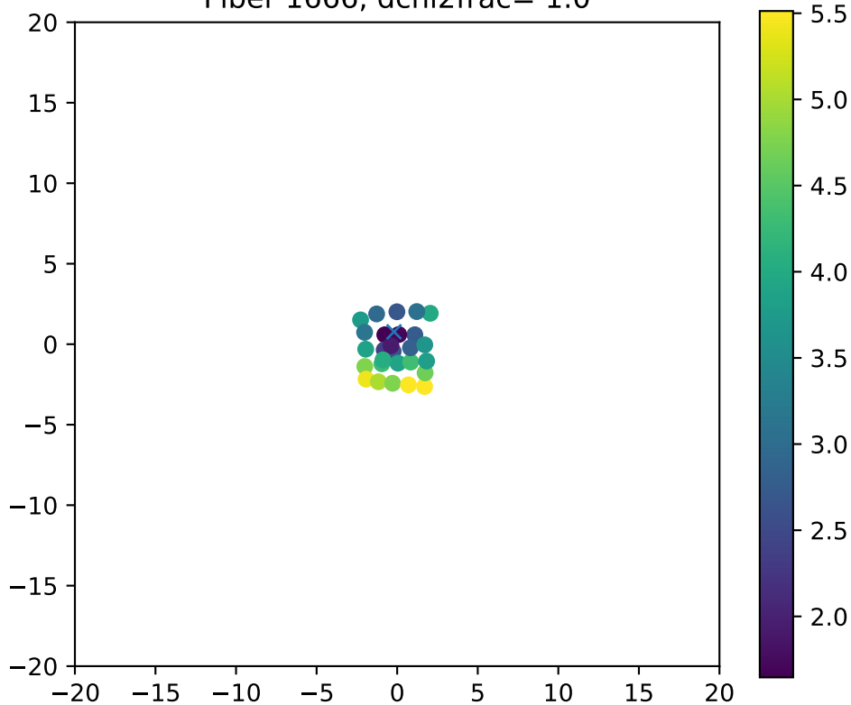
Fiber 1666, dchi2frac= 1.0
