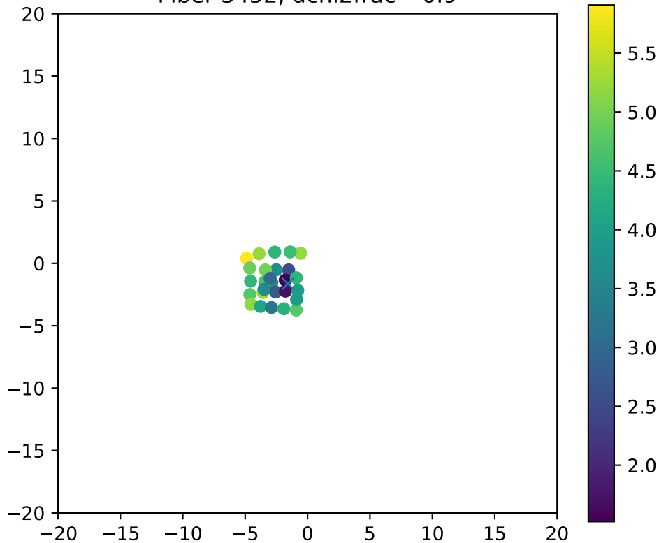
Fiber 3452, dchi2frac= 0.9
