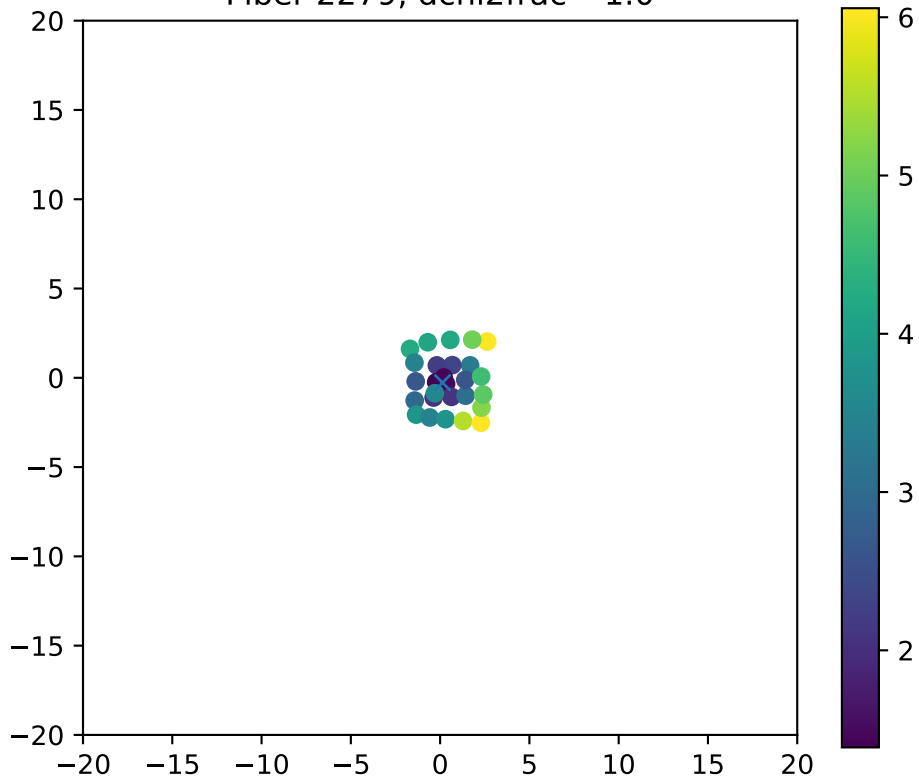
Fiber 2279, dchi2frac= 1.0
