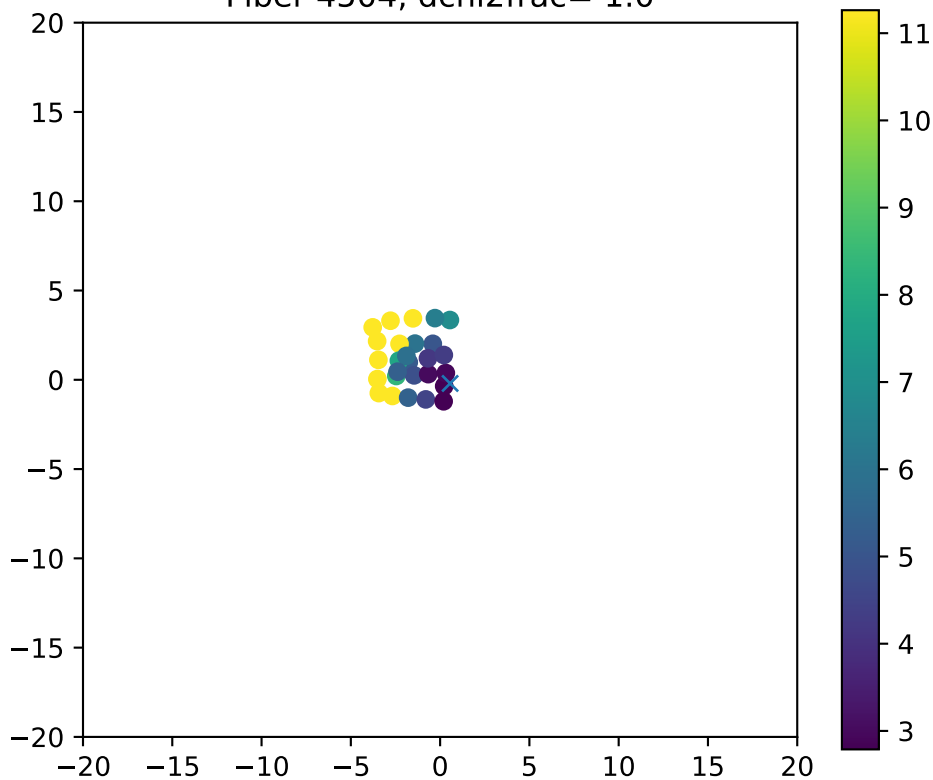
Fiber 4504, dchi2frac= 1.0
