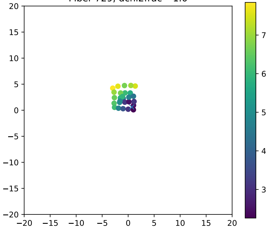
Fiber 729, dchi2frac= 1.0
