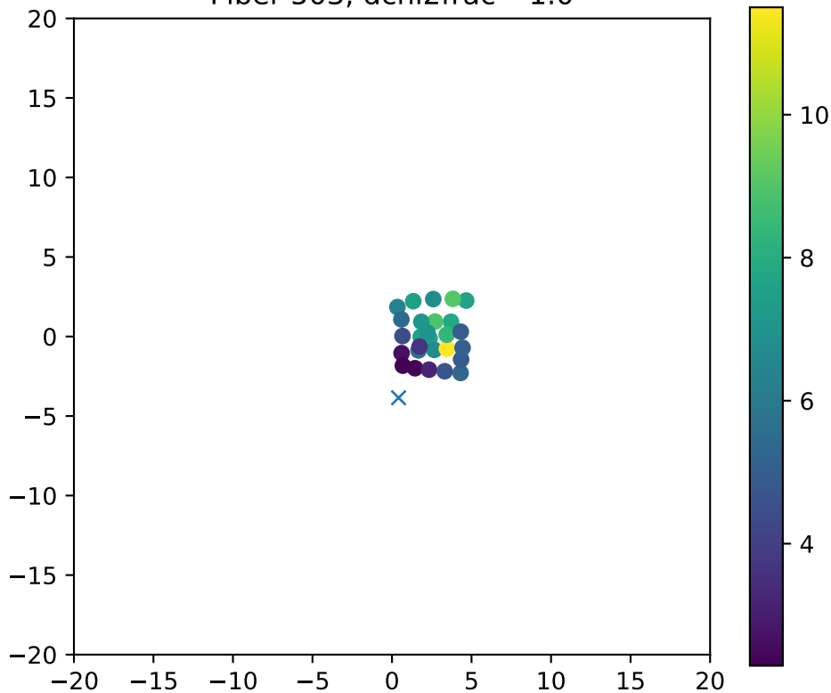
Fiber 503, dchi2frac= 1.0
