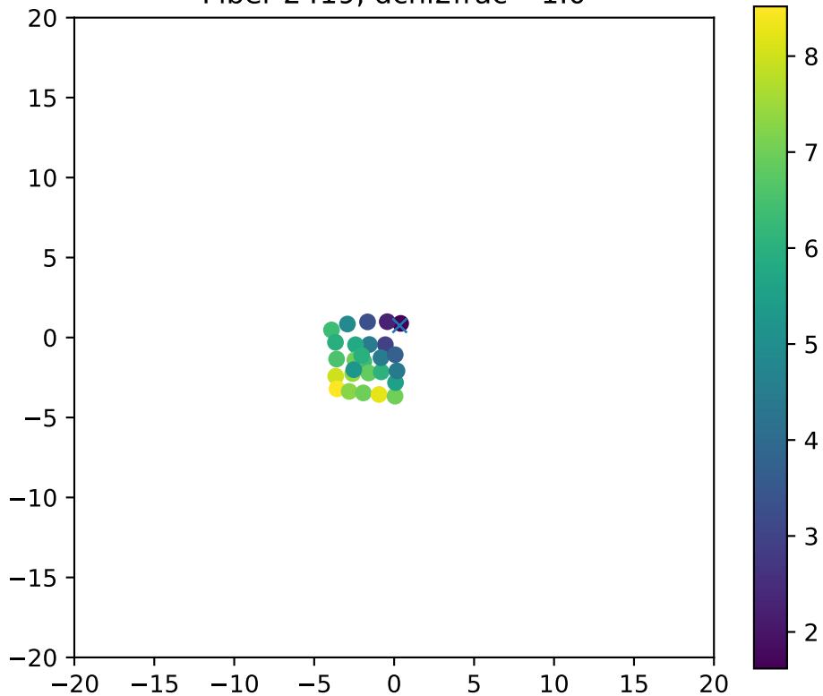
Fiber 2419, dchi2frac= 1.0
