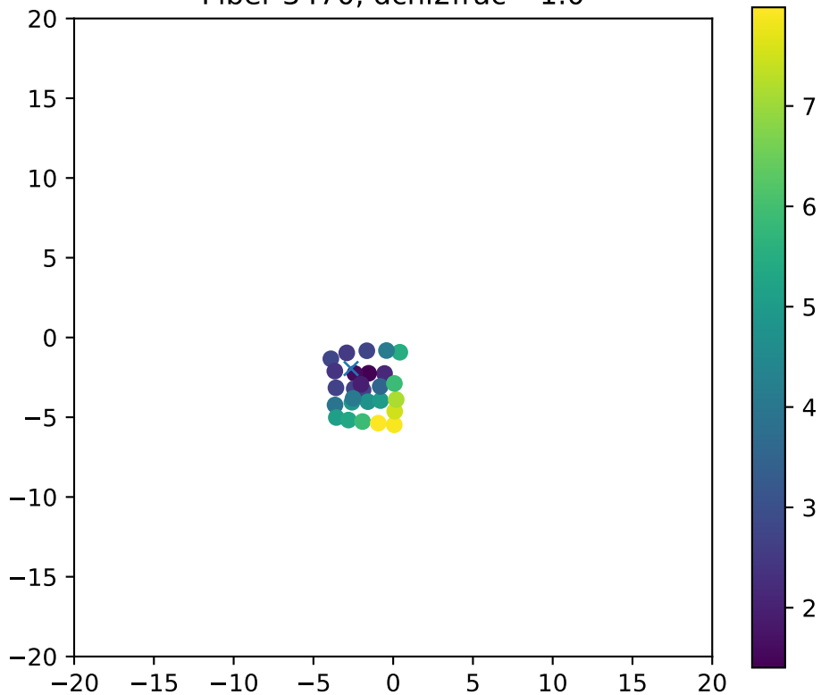
Fiber 3470, dchi2frac= 1.0
