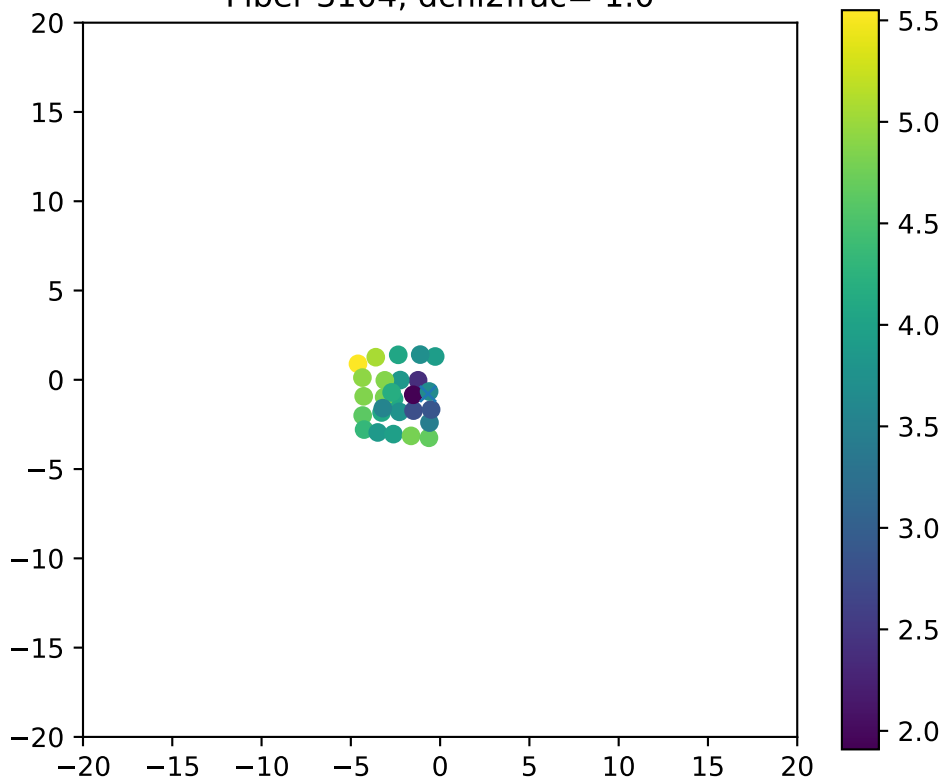
Fiber 3104, dchi2frac= 1.0
