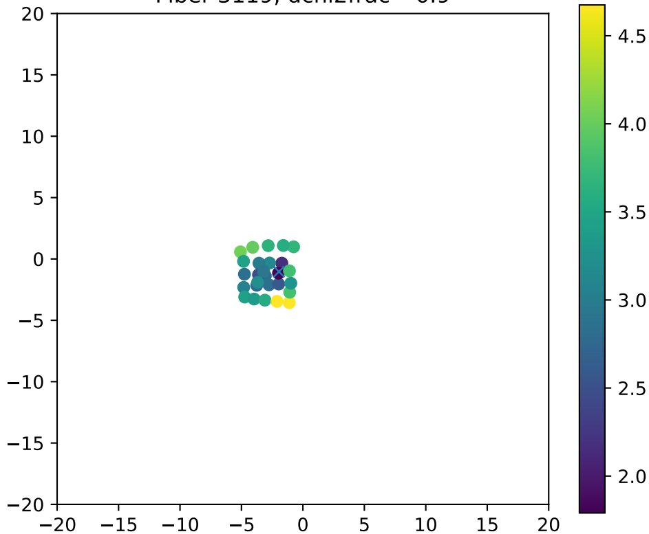
Fiber 3119, dchi2frac= 0.9
