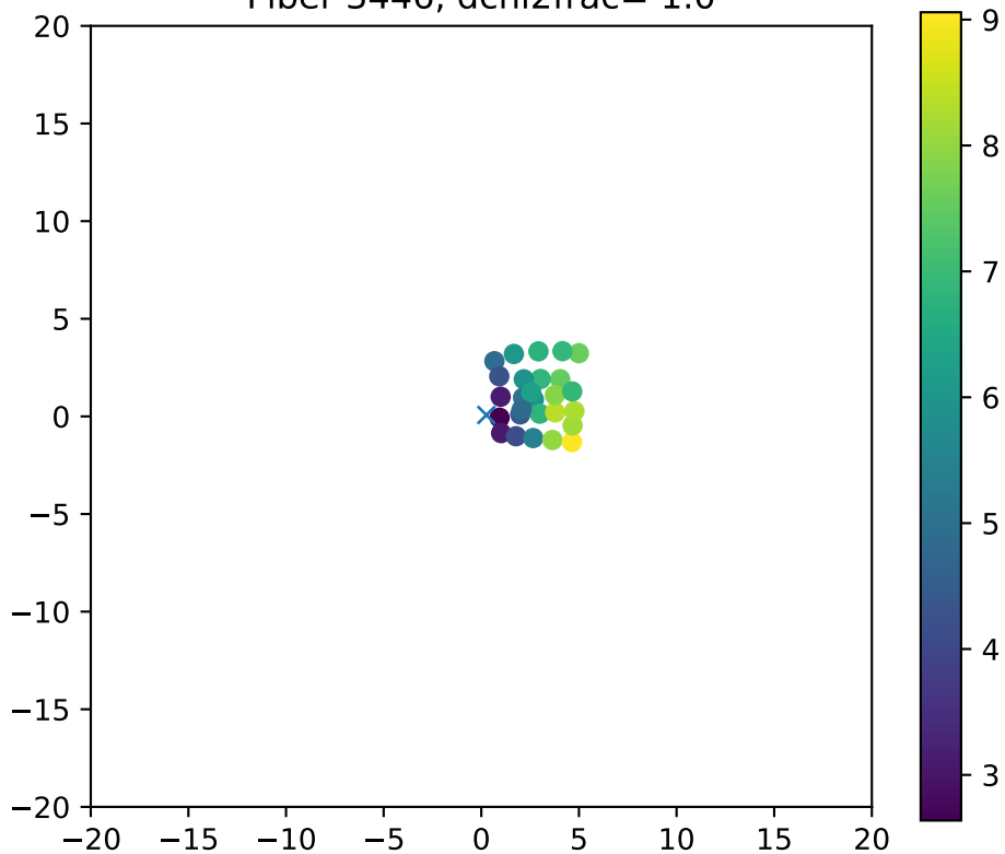
Fiber 3446, dchi2frac= 1.0
