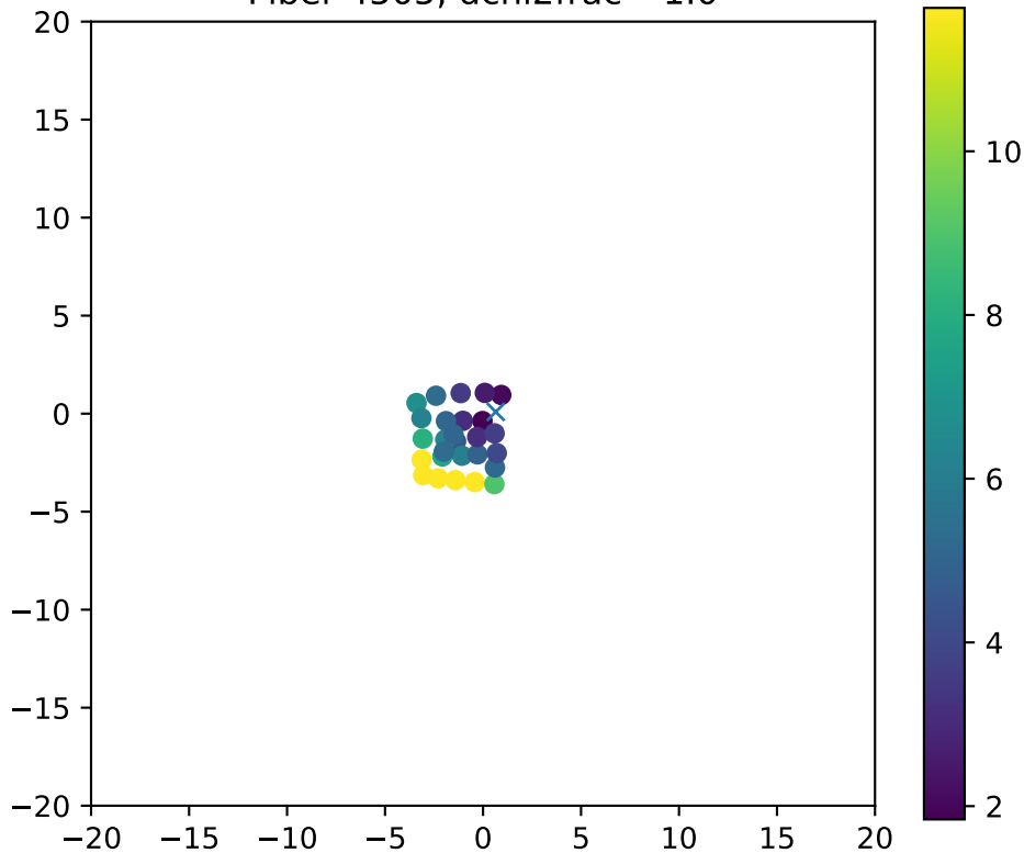
Fiber 4505, dchi2frac= 1.0
