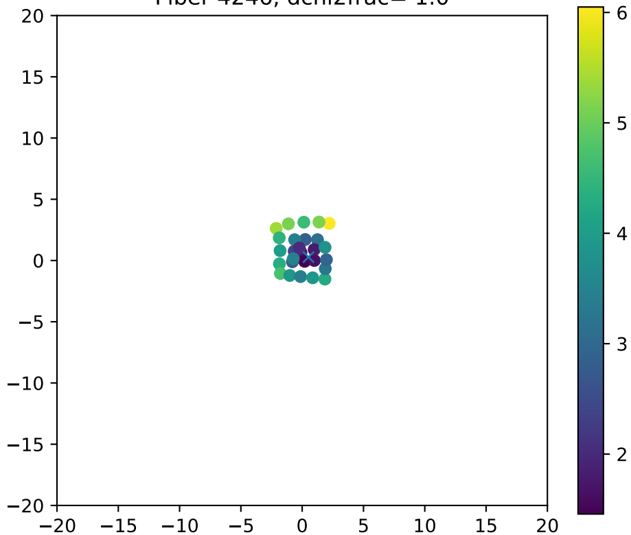
Fiber 4246, dchi2frac= 1.0
