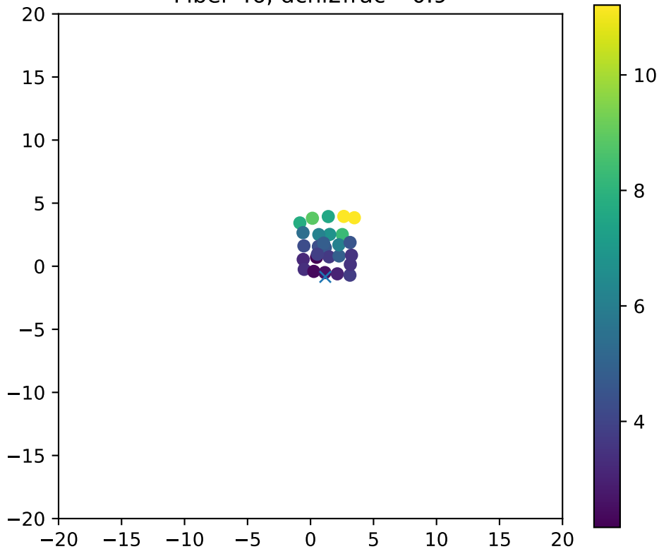
Fiber 46, dchi2frac= 0.9
