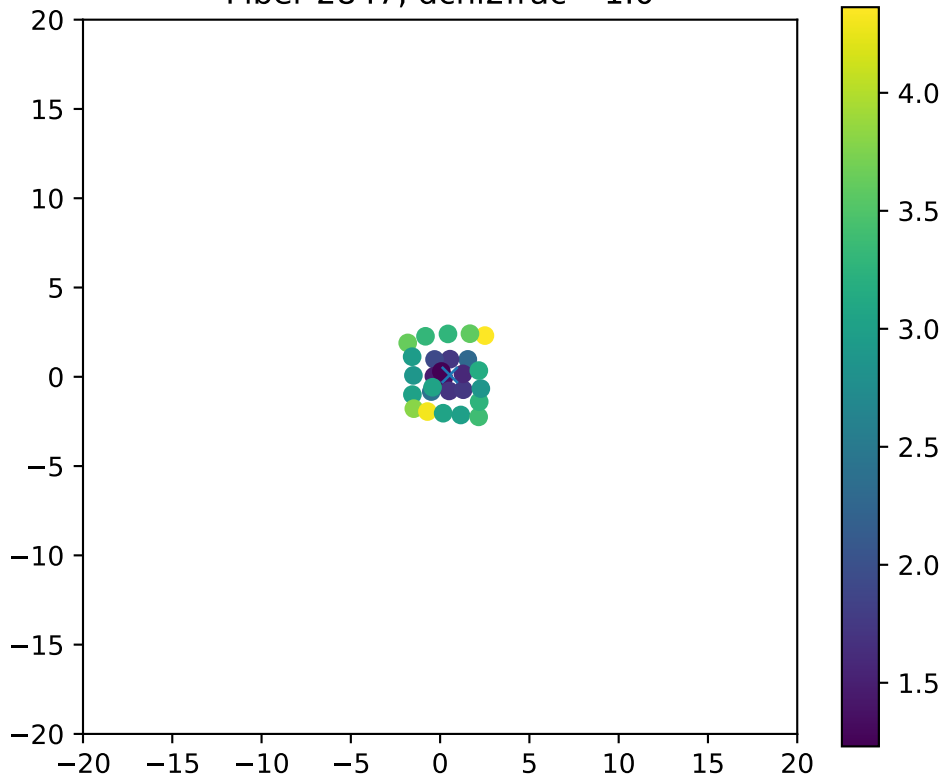
Fiber 2847, dchi2frac= 1.0
