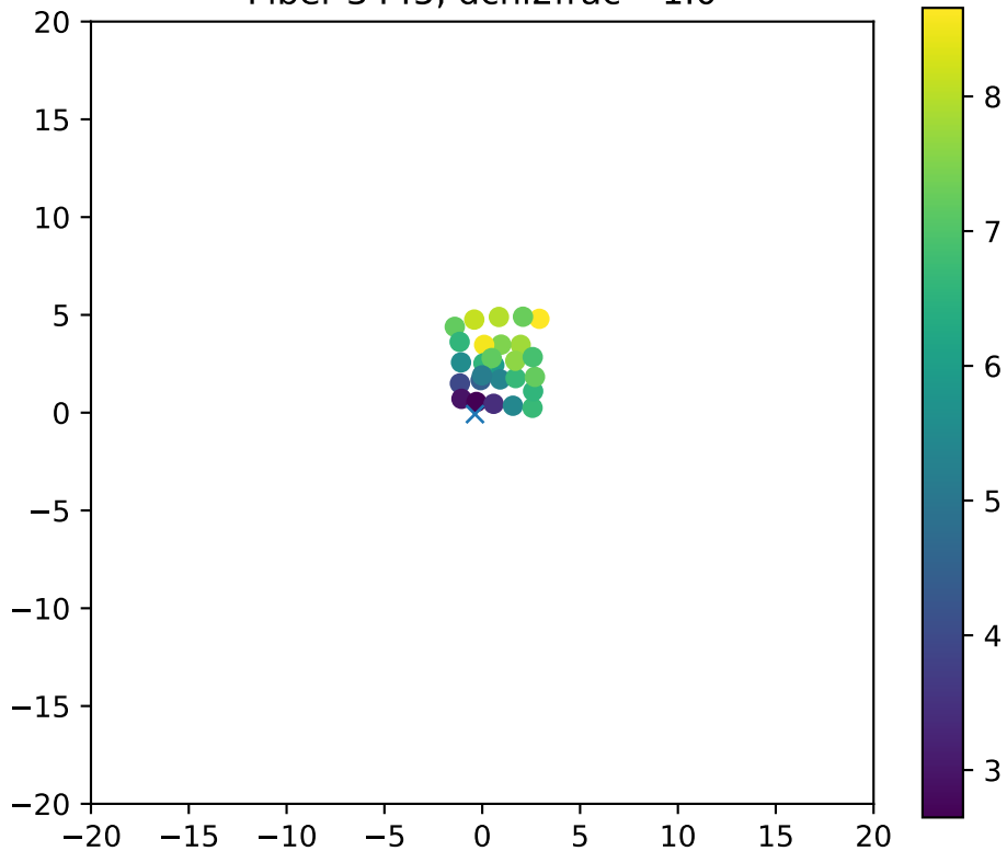
Fiber 3445, dchi2frac= 1.0
