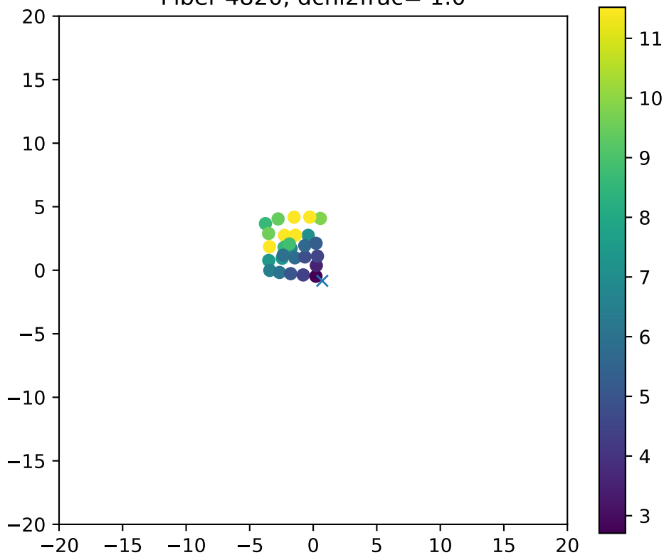
Fiber 4820, dchi2frac= 1.0
