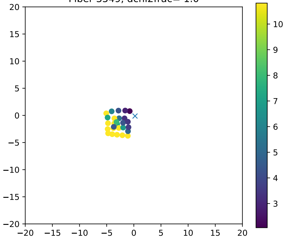
Fiber 3549, dchi2frac= 1.0
