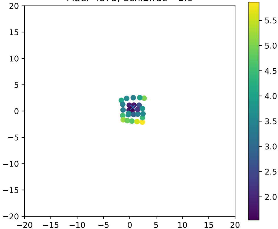
Fiber 4873, dchi2frac= 1.0
