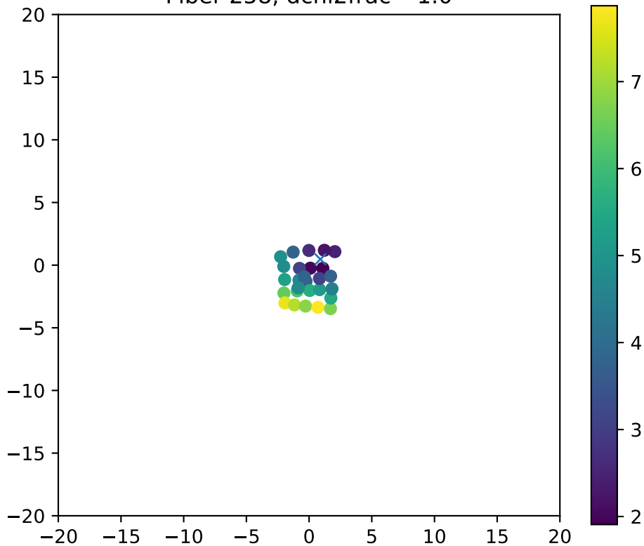
Fiber 258, dchi2frac= 1.0
