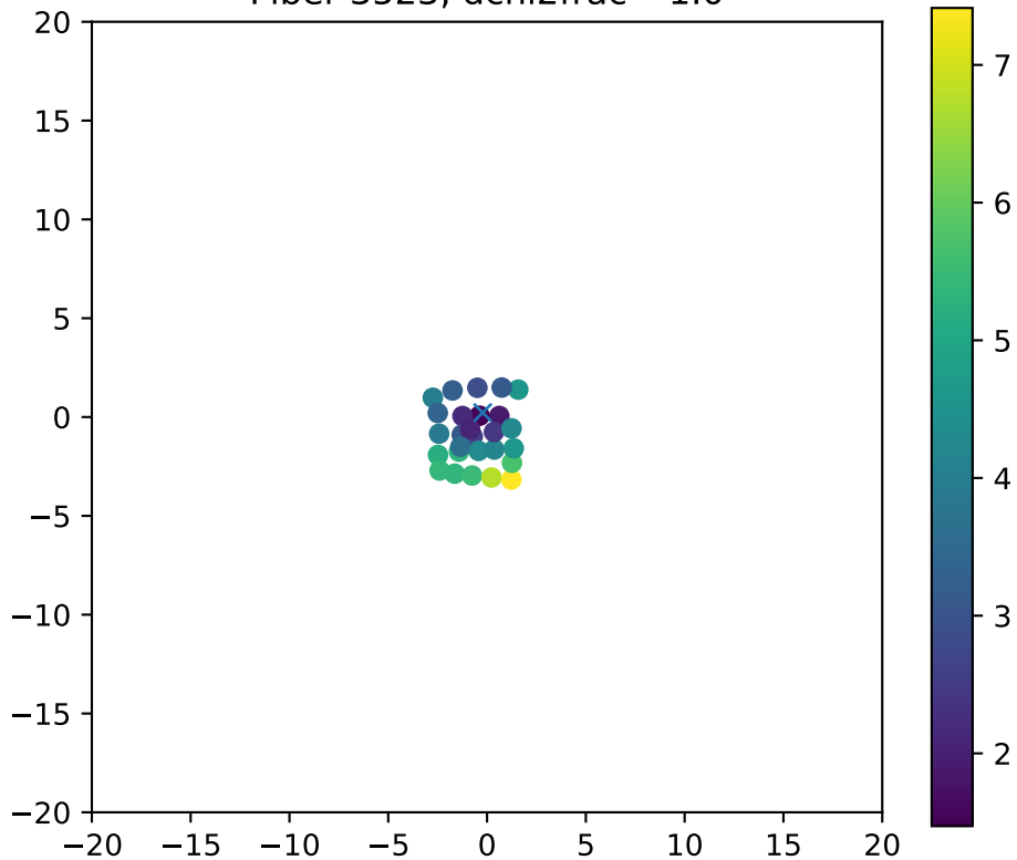
Fiber 3523, dchi2frac= 1.0
