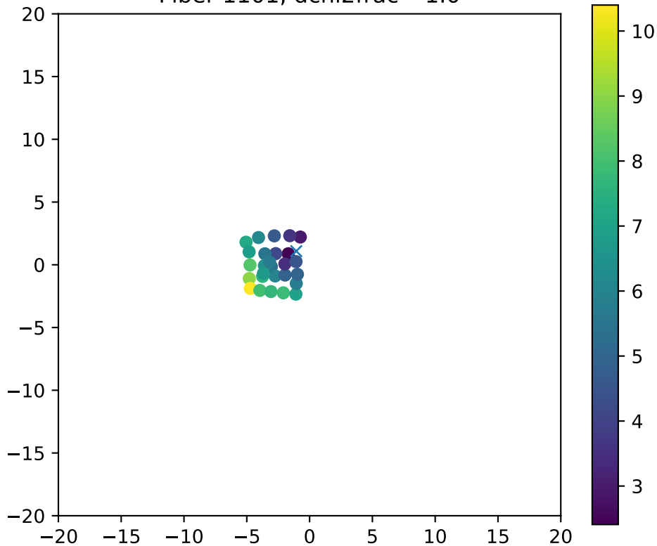
Fiber 1101, dchi2frac= 1.0
