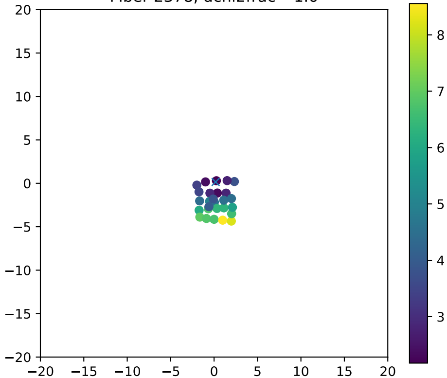
Fiber 2378, dchi2frac= 1.0
