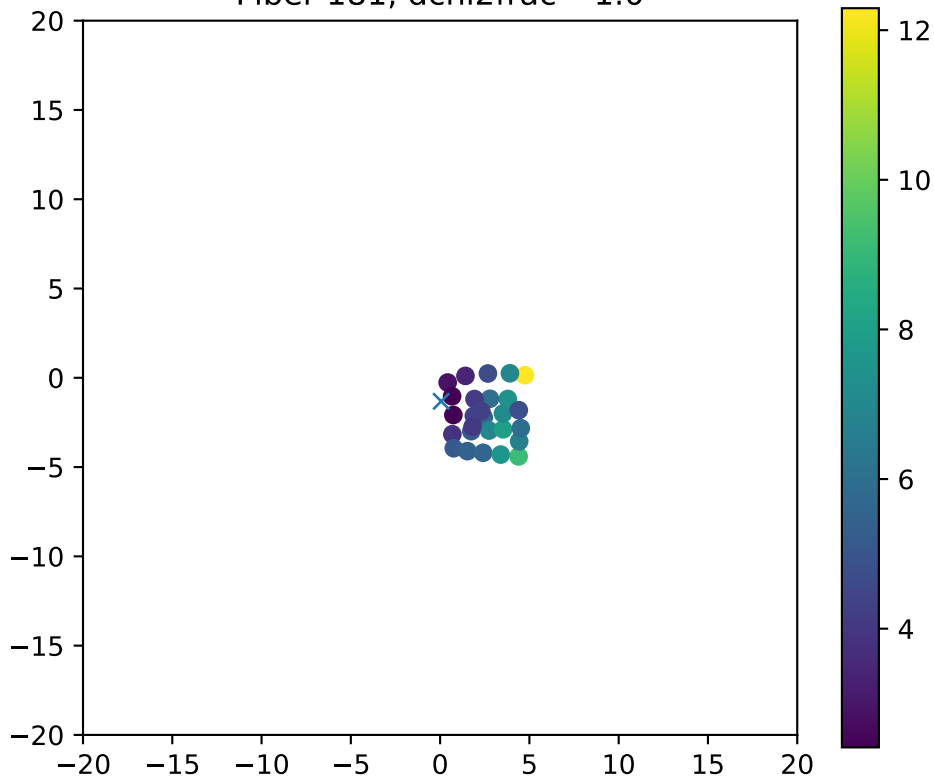
Fiber 181, dchi2frac= 1.0
