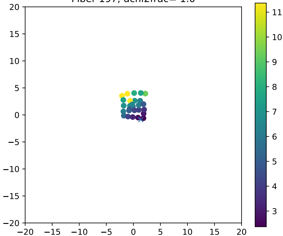
Fiber 197, dchi2frac= 1.0
