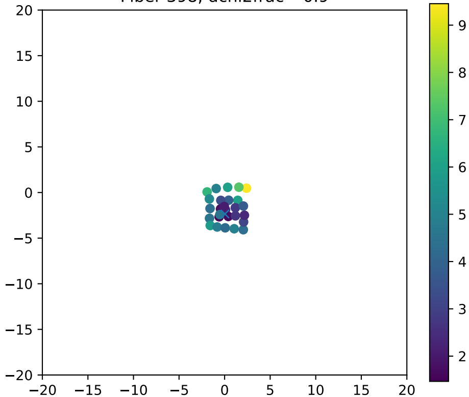
Fiber 398, dchi2frac= 0.9
