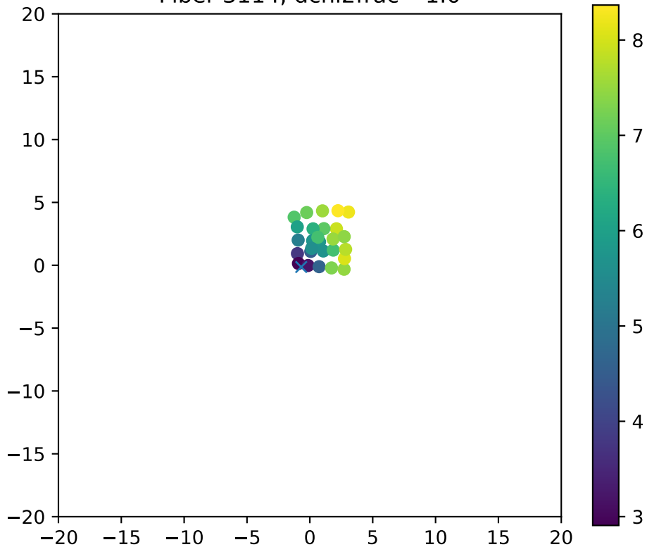
Fiber 3114, dchi2frac= 1.0
