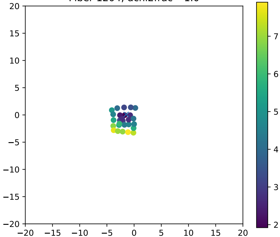
Fiber 1204, dchi2frac= 1.0
