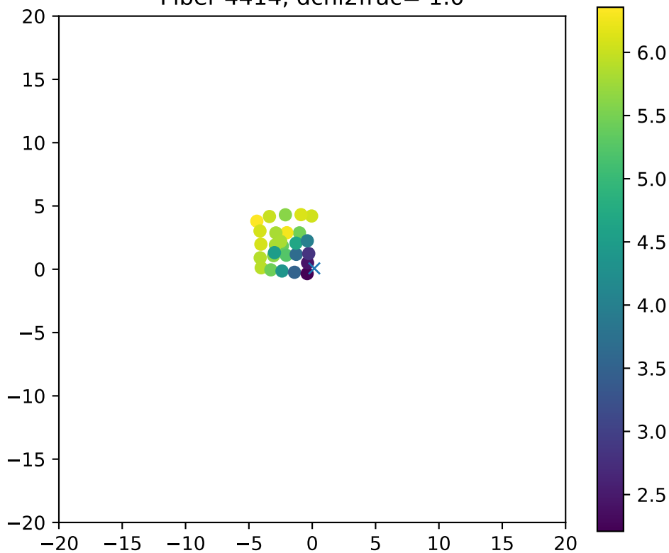
Fiber 4414, dchi2frac= 1.0
