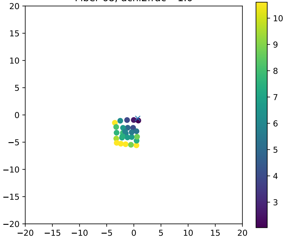
Fiber 68, dchi2frac= 1.0
