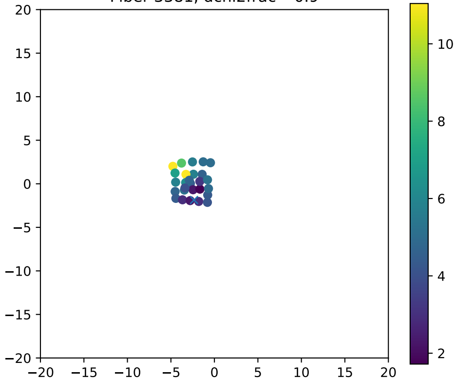
Fiber 3381, dchi2frac= 0.9
