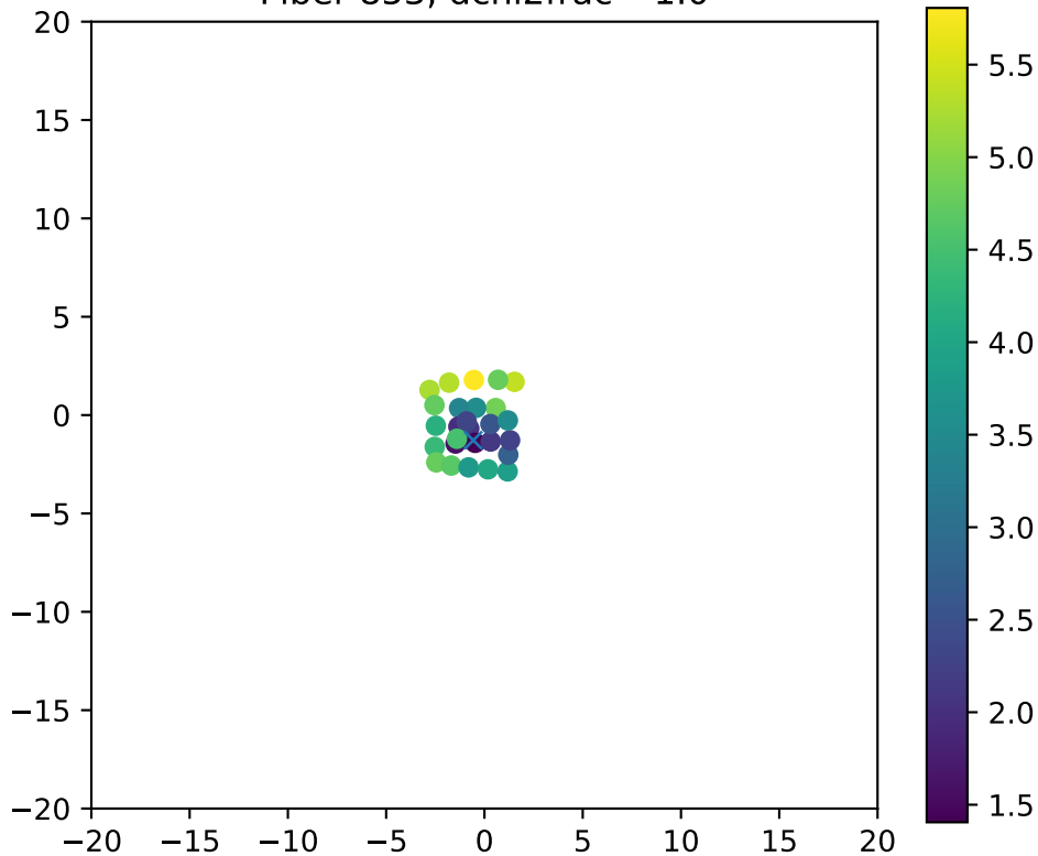
Fiber 853, dchi2frac= 1.0
