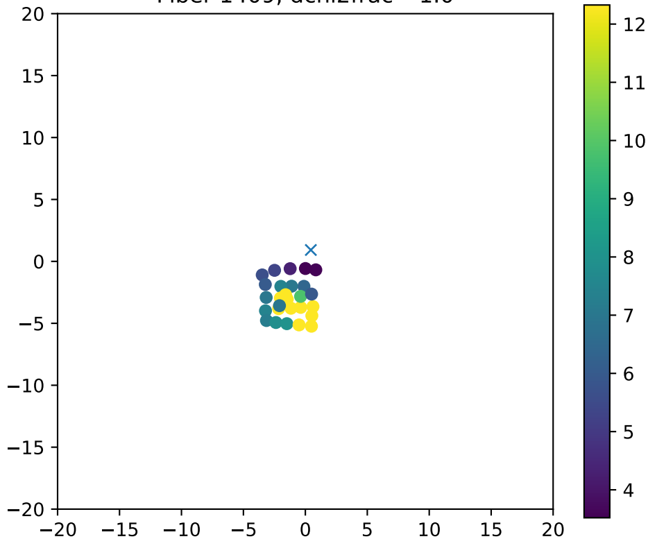
Fiber 1409, dchi2frac= 1.0
