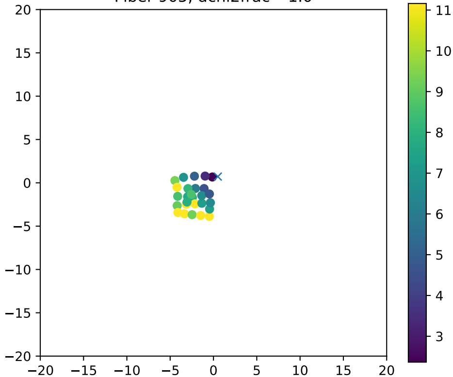
Fiber 905, dchi2frac= 1.0
