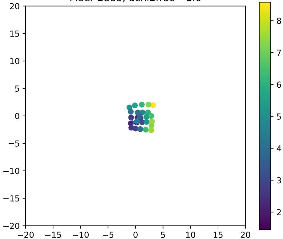
Fiber 2885, dchi2frac= 1.0
