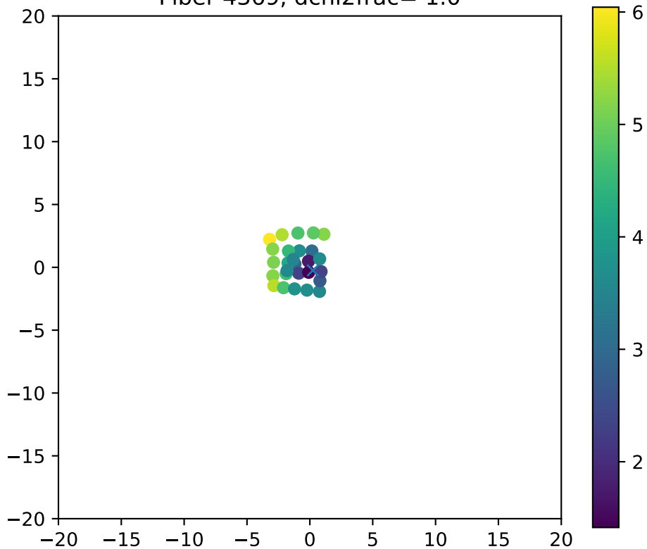
Fiber 4369, dchi2frac= 1.0
