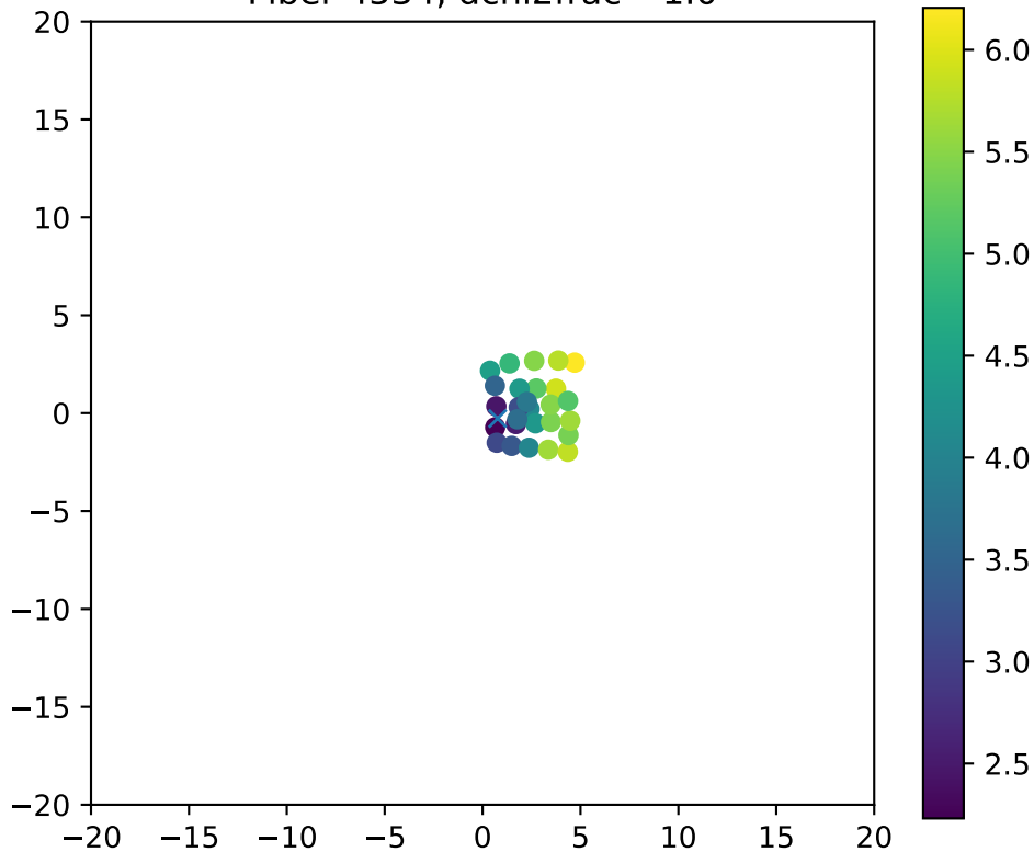
Fiber 4534, dchi2frac= 1.0
