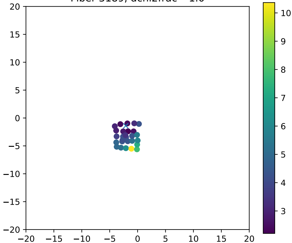
Fiber 3189, dchi2frac= 1.0
