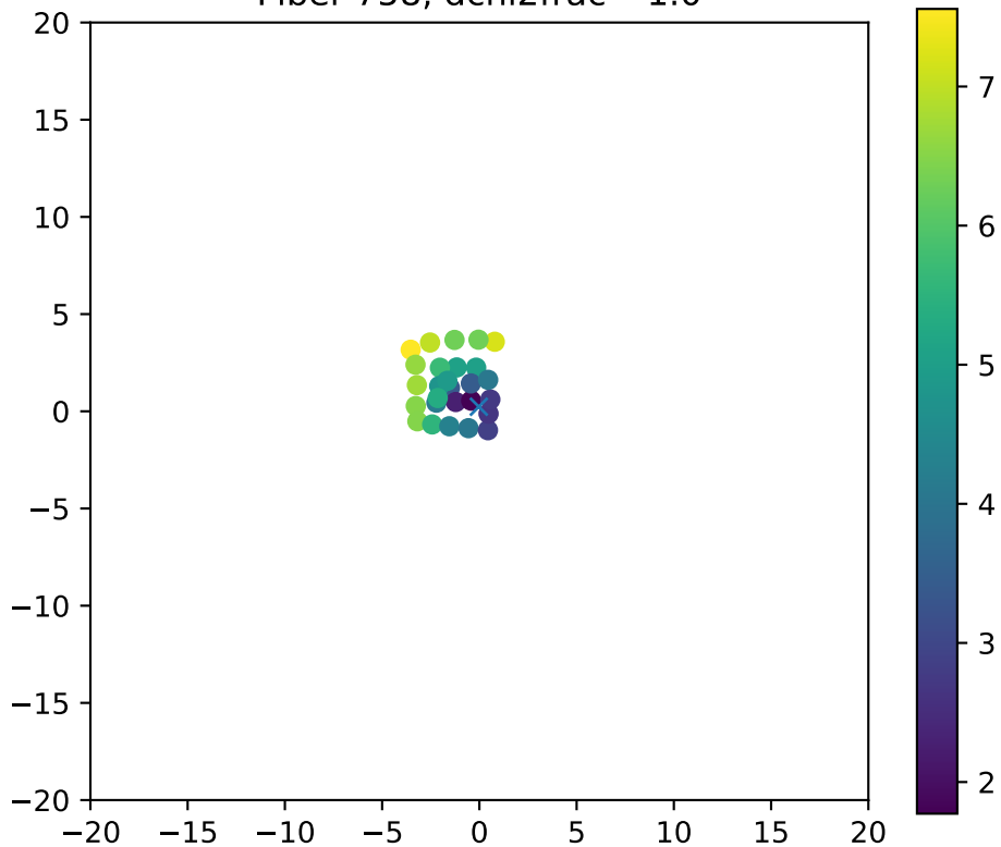
Fiber 758, dchi2frac= 1.0
