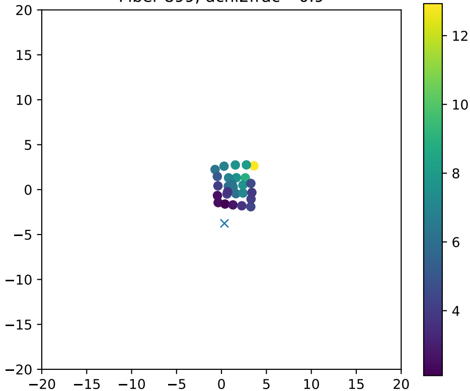
Fiber 899, dchi2frac= 0.9
