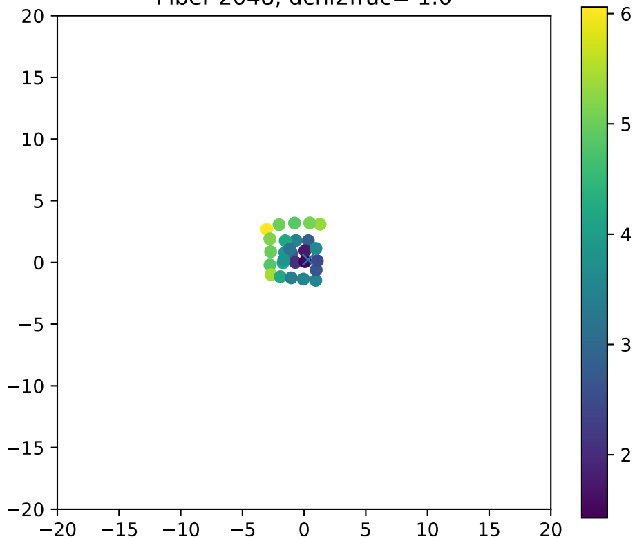
Fiber 2048, dchi2frac= 1.0
