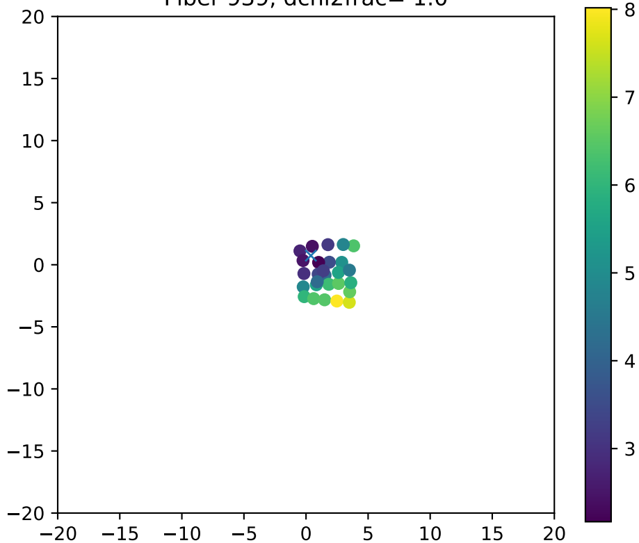
Fiber 939, dchi2frac= 1.0
