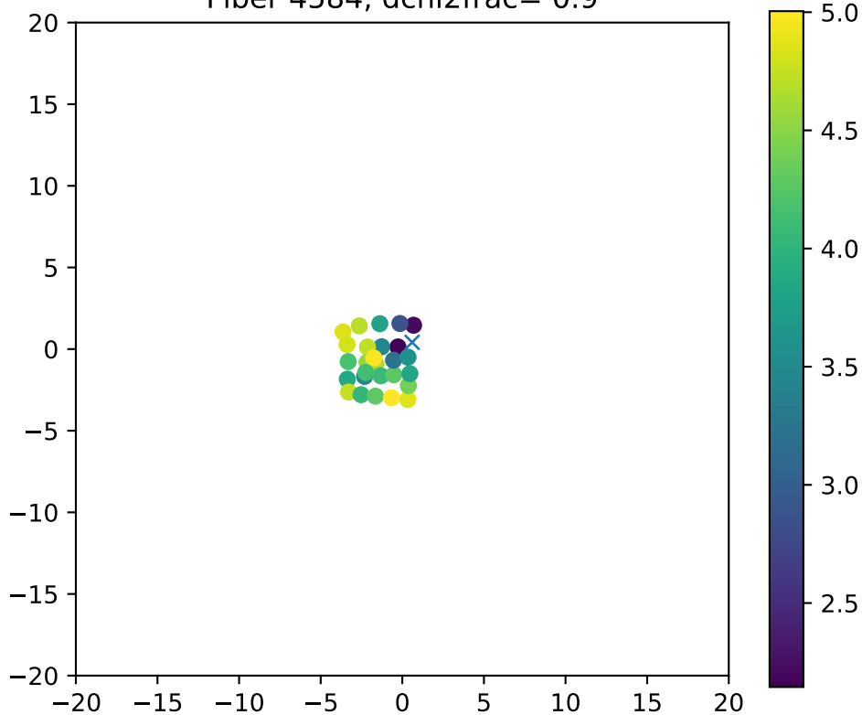
Fiber 4584, dchi2frac= 0.9
