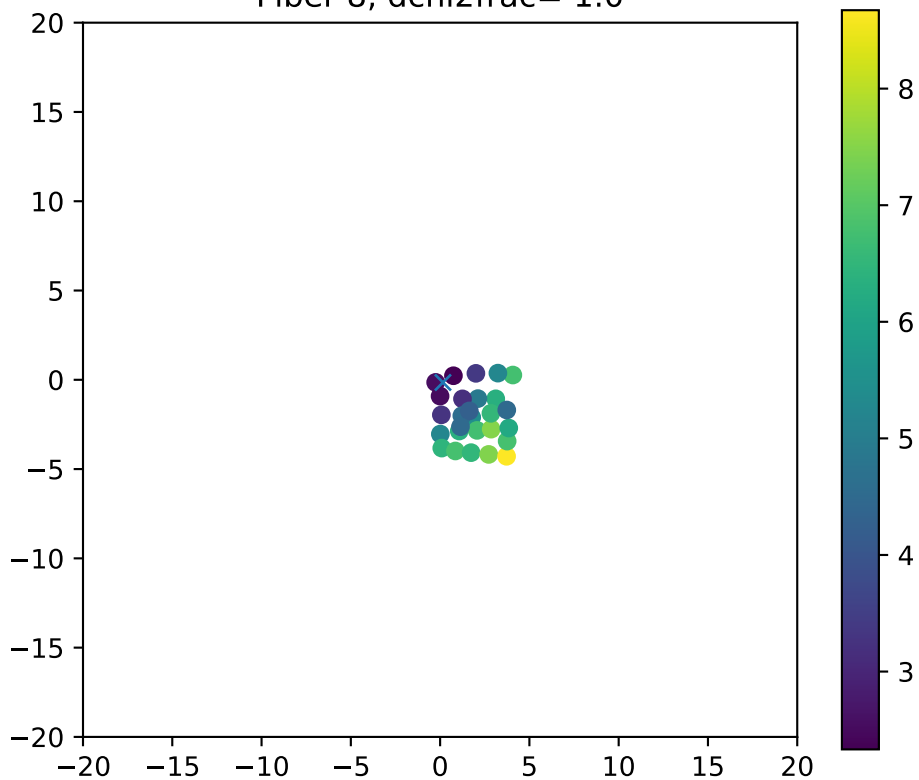
Fiber 8, dchi2frac= 1.0
