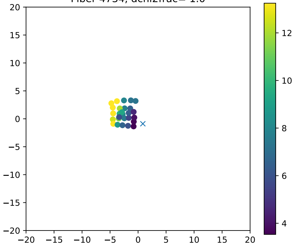
Fiber 4734, dchi2frac= 1.0
