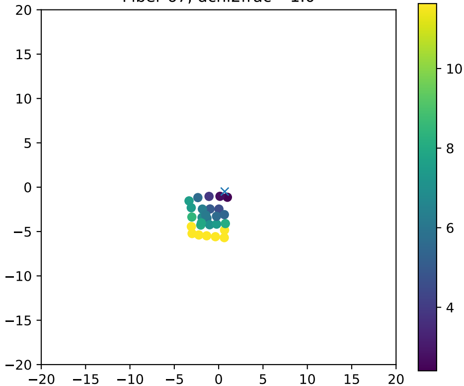
Fiber 67, dchi2frac= 1.0
