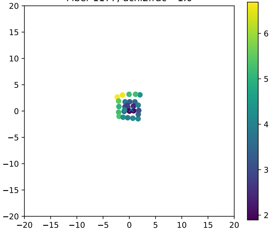
Fiber 1177, dchi2frac= 1.0
