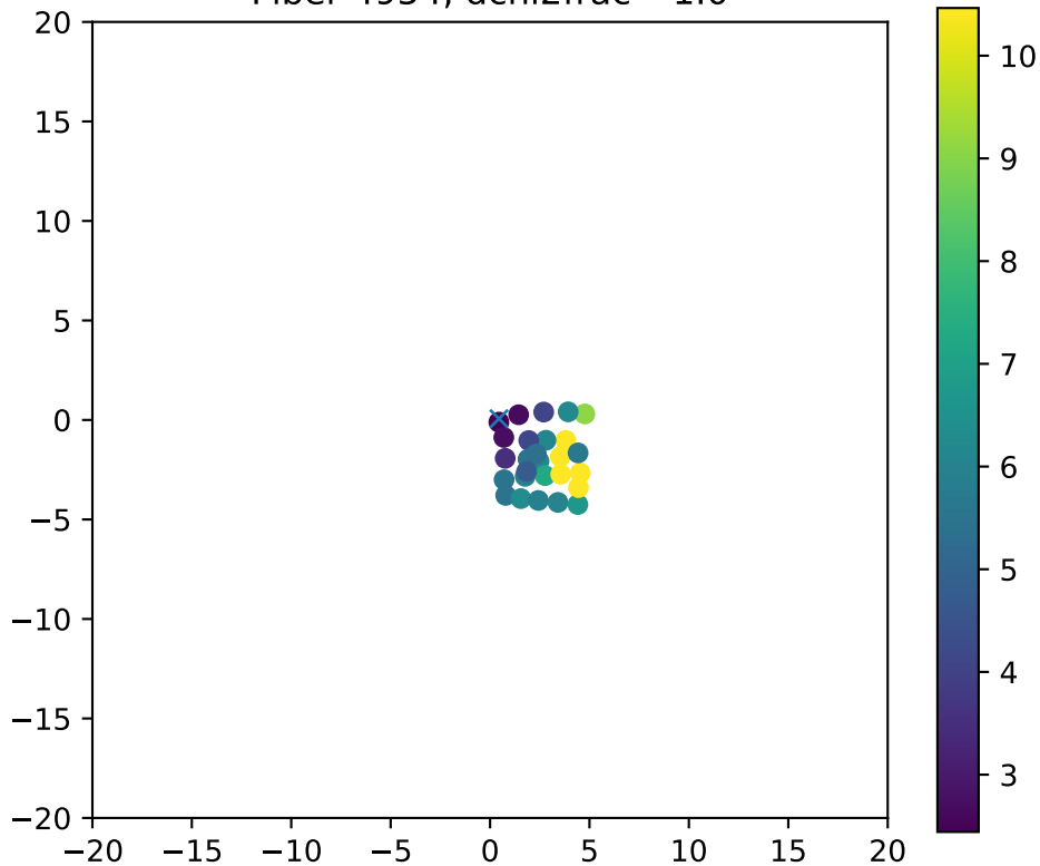
Fiber 4954, dchi2frac= 1.0
