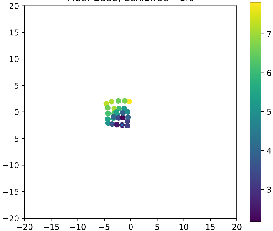
Fiber 2880, dchi2frac= 1.0
