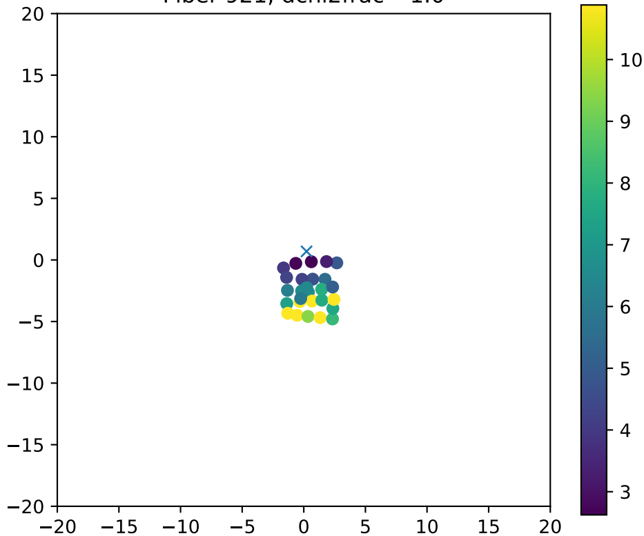
Fiber 921, dchi2frac= 1.0
