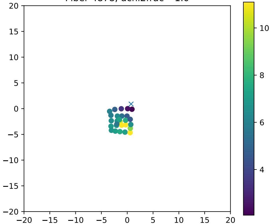
Fiber 4878, dchi2frac= 1.0
