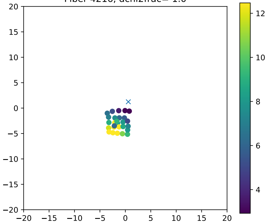
Fiber 4216, dchi2frac= 1.0
