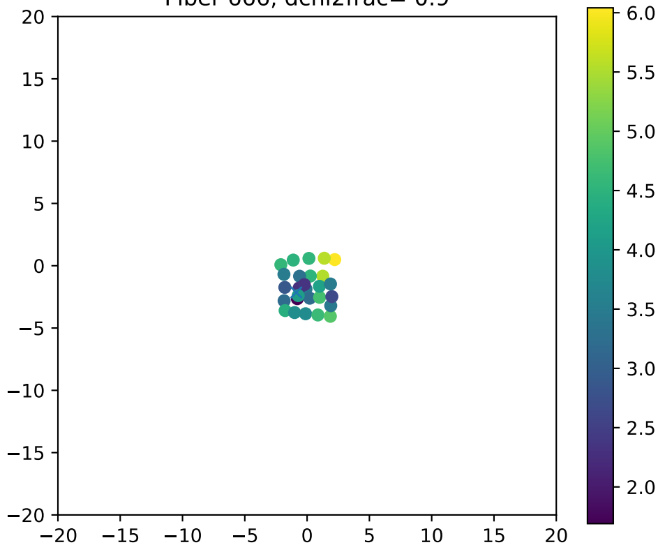
Fiber 666, dchi2frac= 0.9
