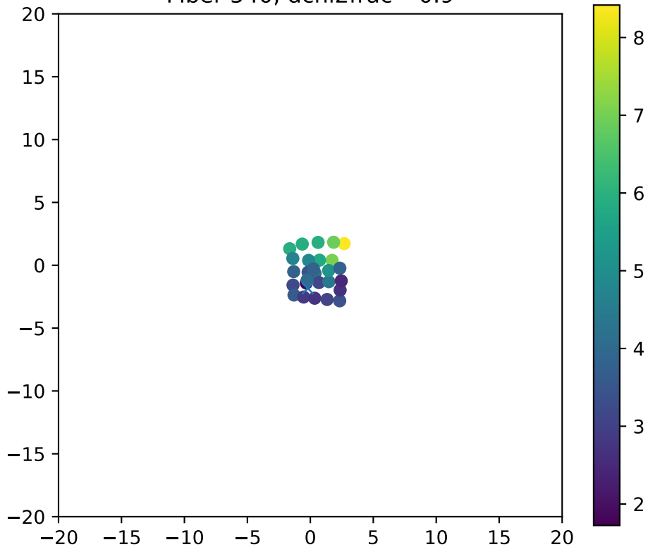
Fiber 540, dchi2frac= 0.9
