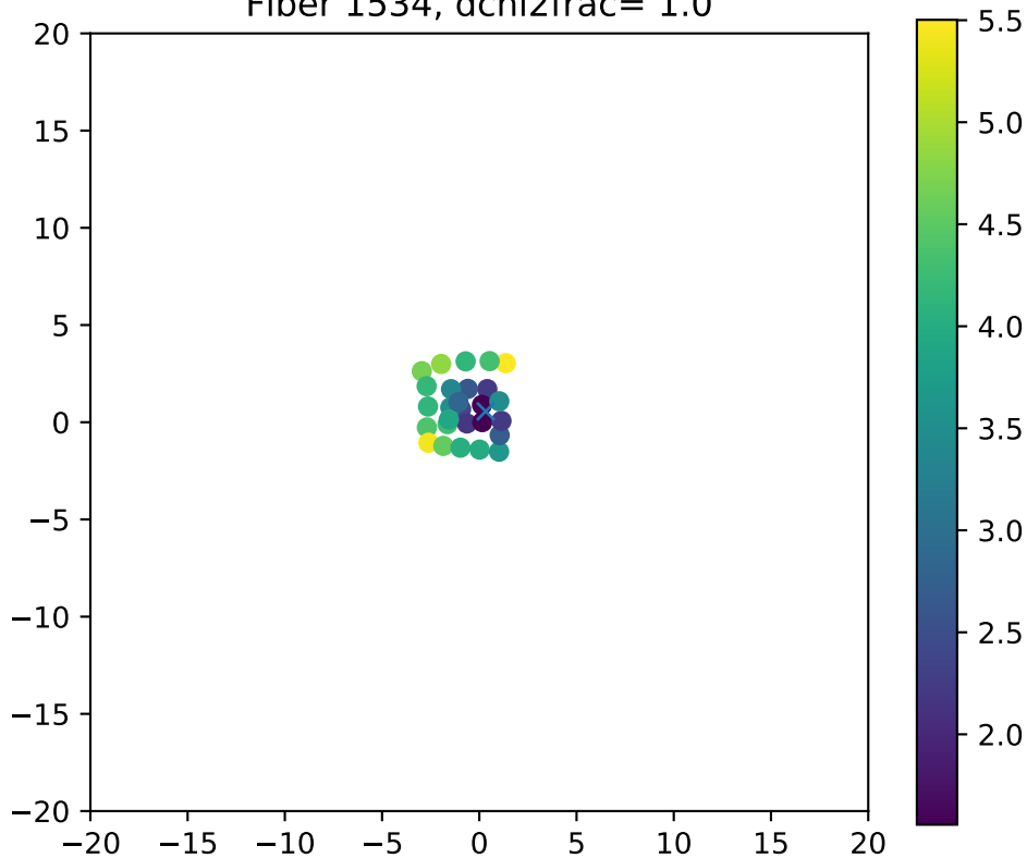
Fiber 1534, dchi2frac= 1.0
