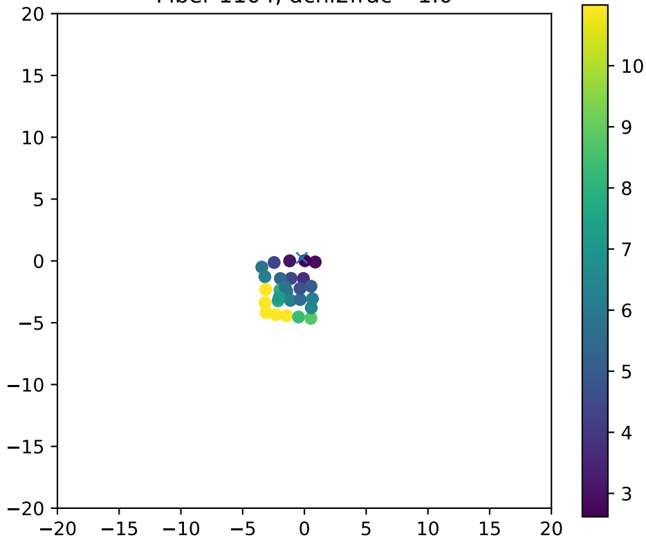
Fiber 1104, dchi2frac= 1.0
