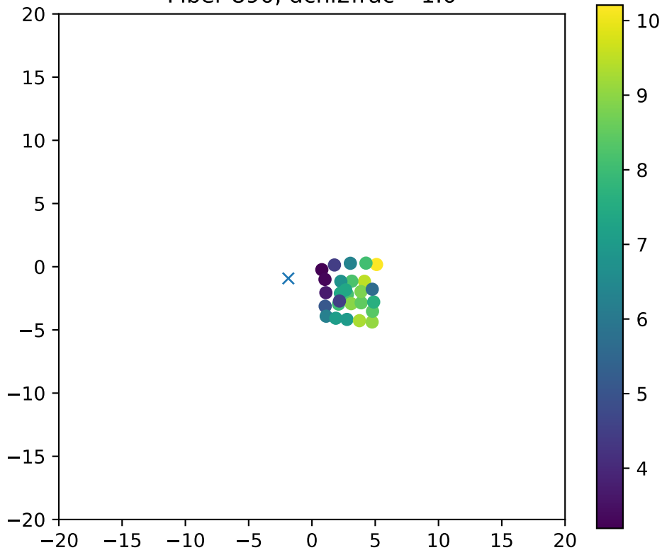
Fiber 890, dchi2frac= 1.0
