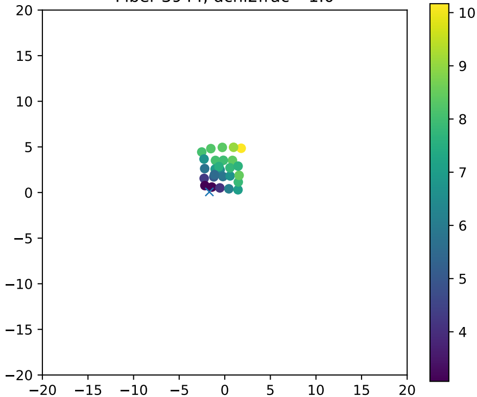
Fiber 3944, dchi2frac= 1.0
