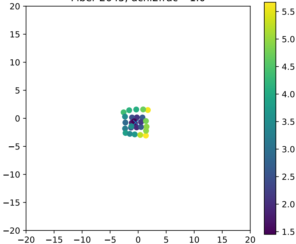
Fiber 2645, dchi2frac= 1.0
