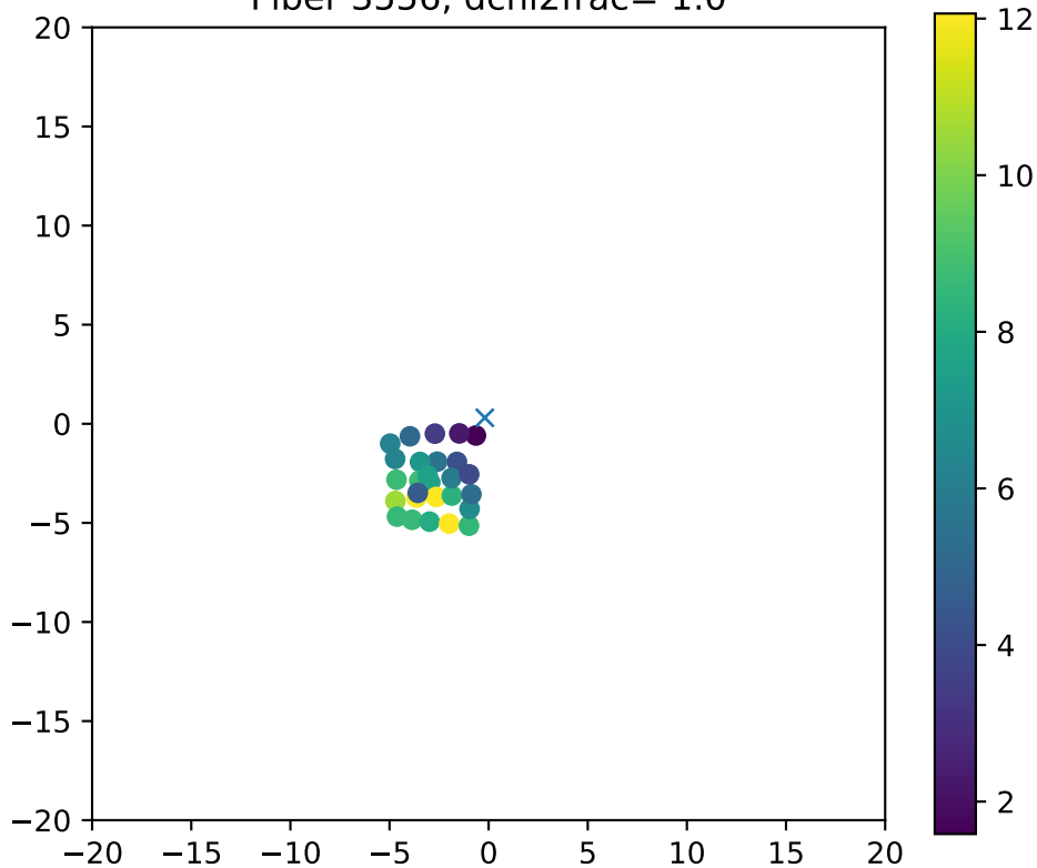
Fiber 3556, dchi2frac= 1.0
