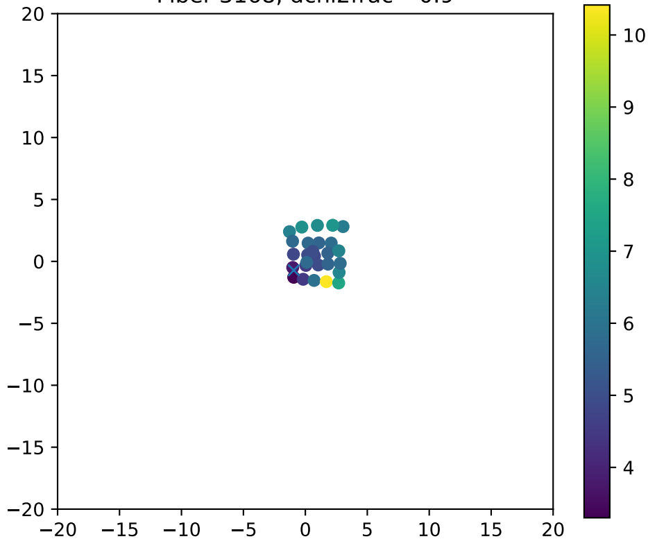
Fiber 3168, dchi2frac= 0.9
