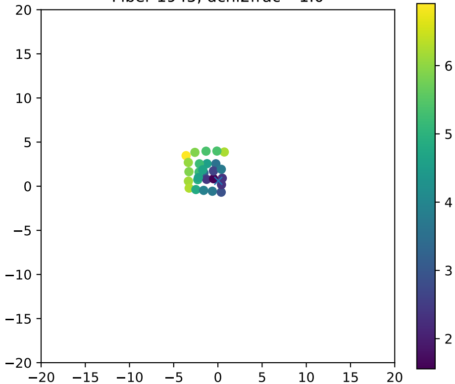
Fiber 1945, dchi2frac= 1.0
