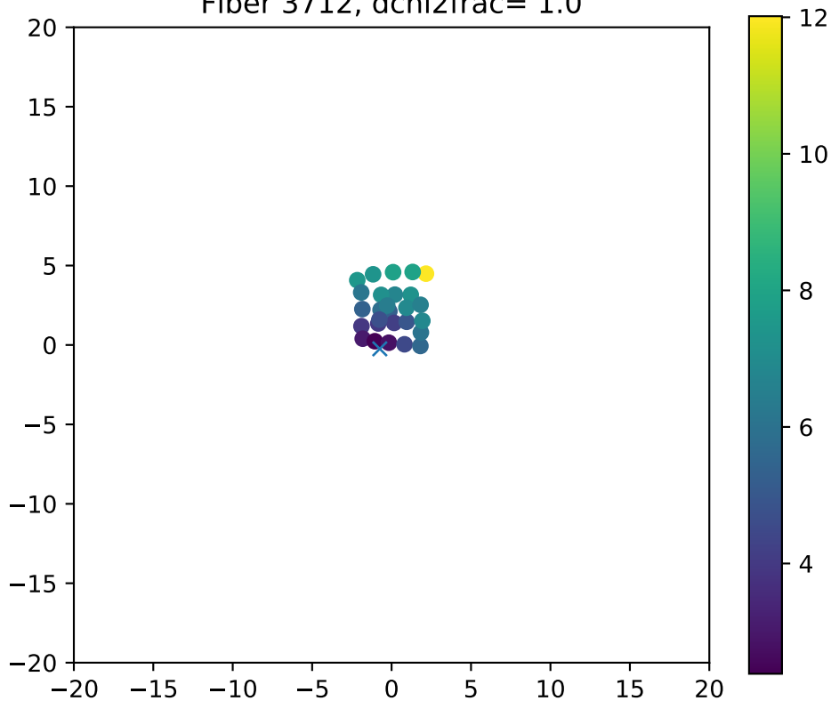
Fiber 3712, dchi2frac= 1.0
