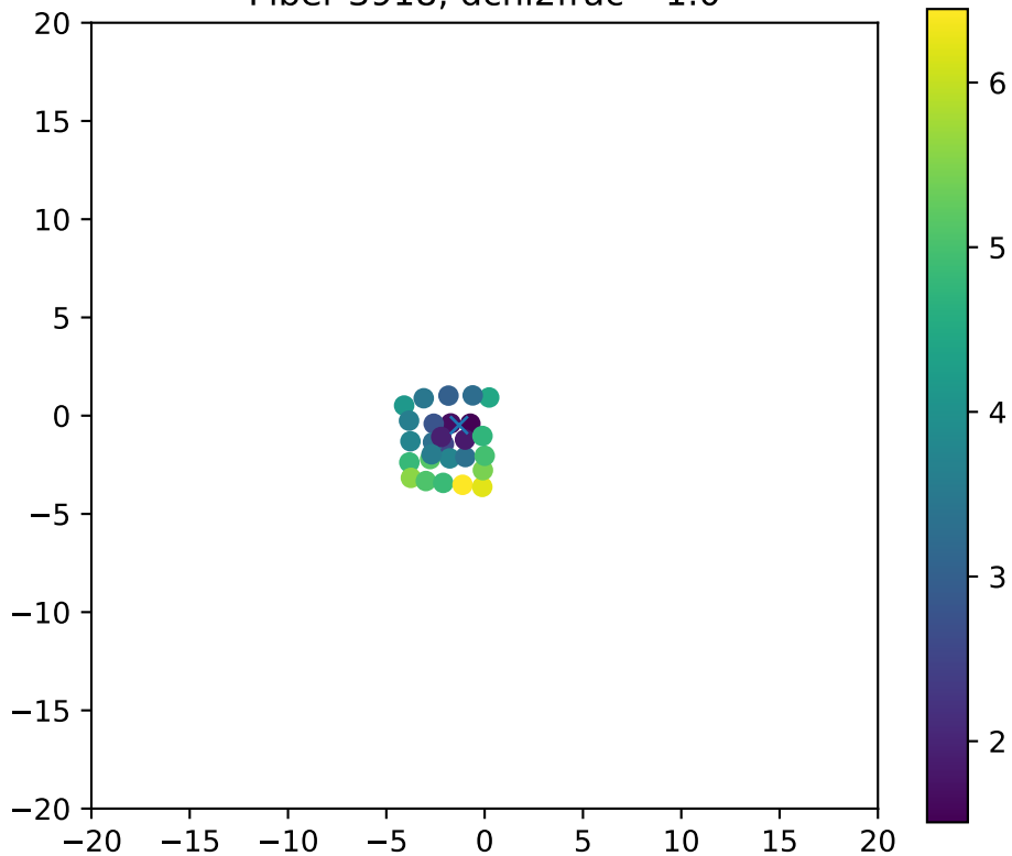
Fiber 3918, dchi2frac= 1.0
