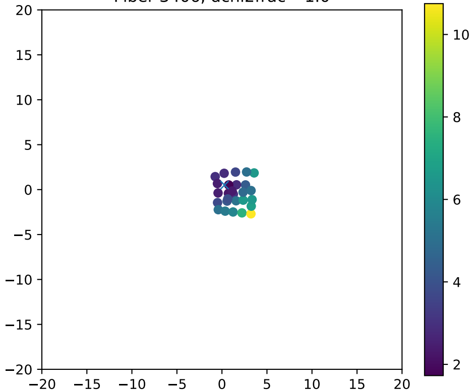
Fiber 3406, dchi2frac= 1.0
