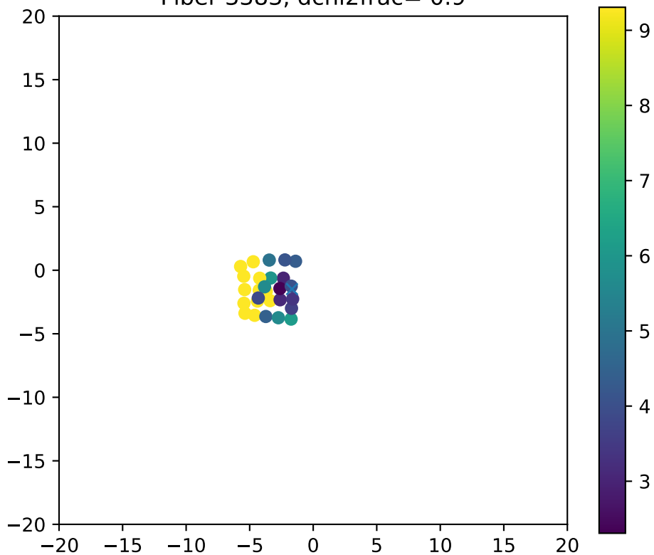
Fiber 3383, dchi2frac= 0.9
