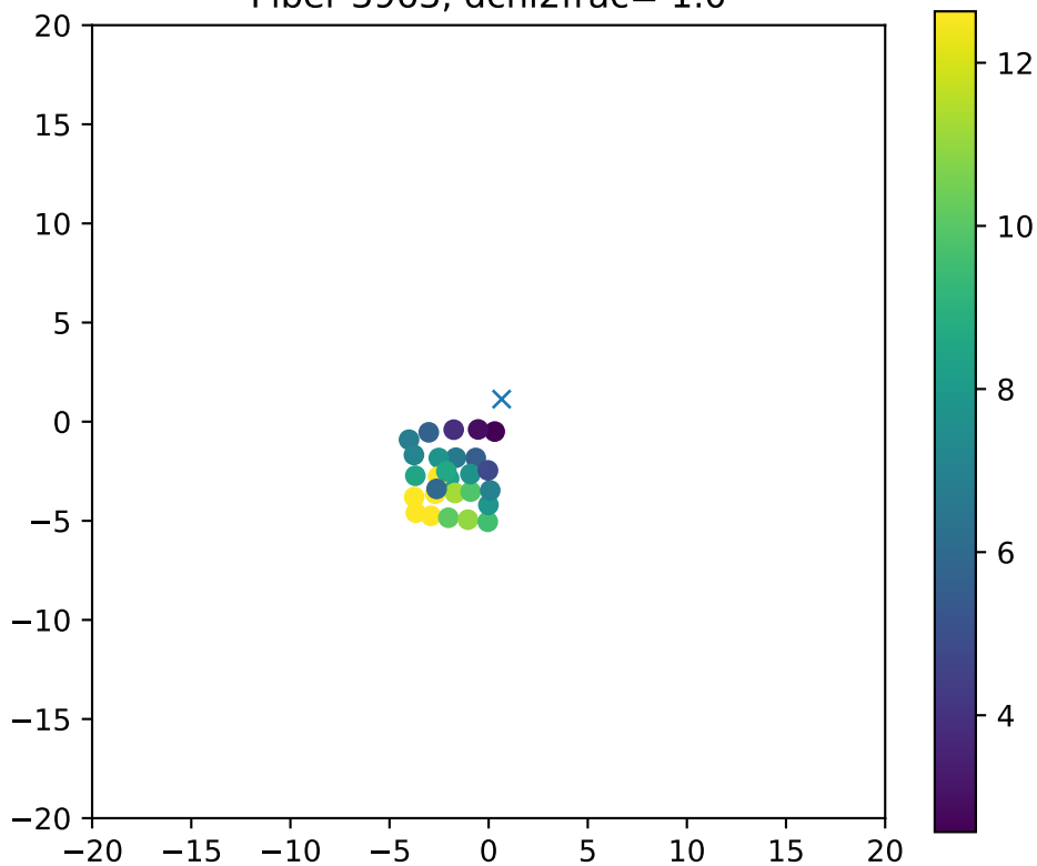
Fiber 3963, dchi2frac= 1.0
