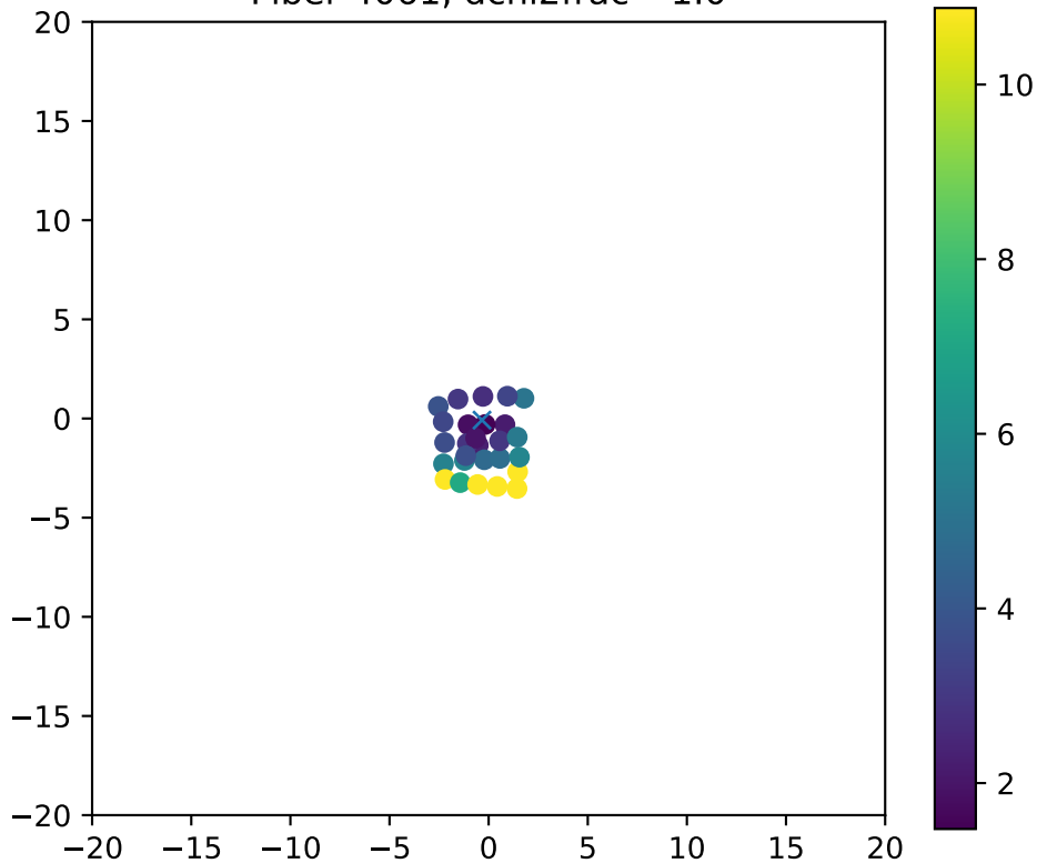
Fiber 4061, dchi2frac= 1.0
