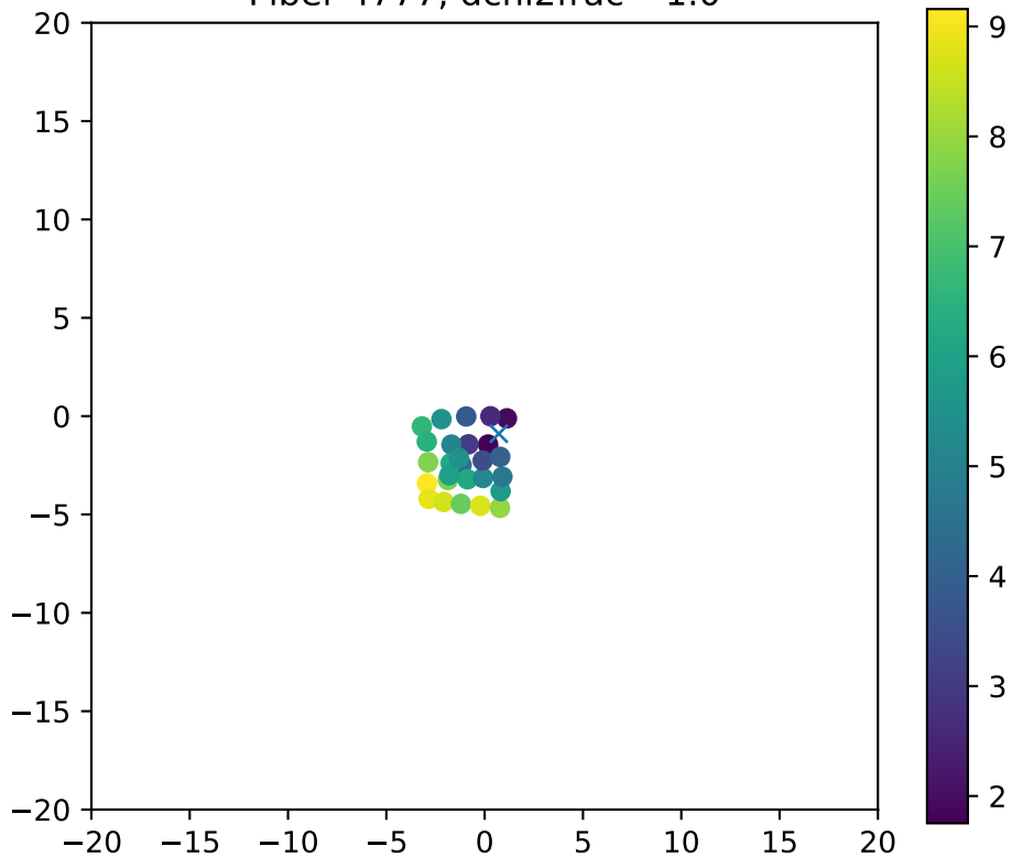
Fiber 4777, dchi2frac= 1.0
