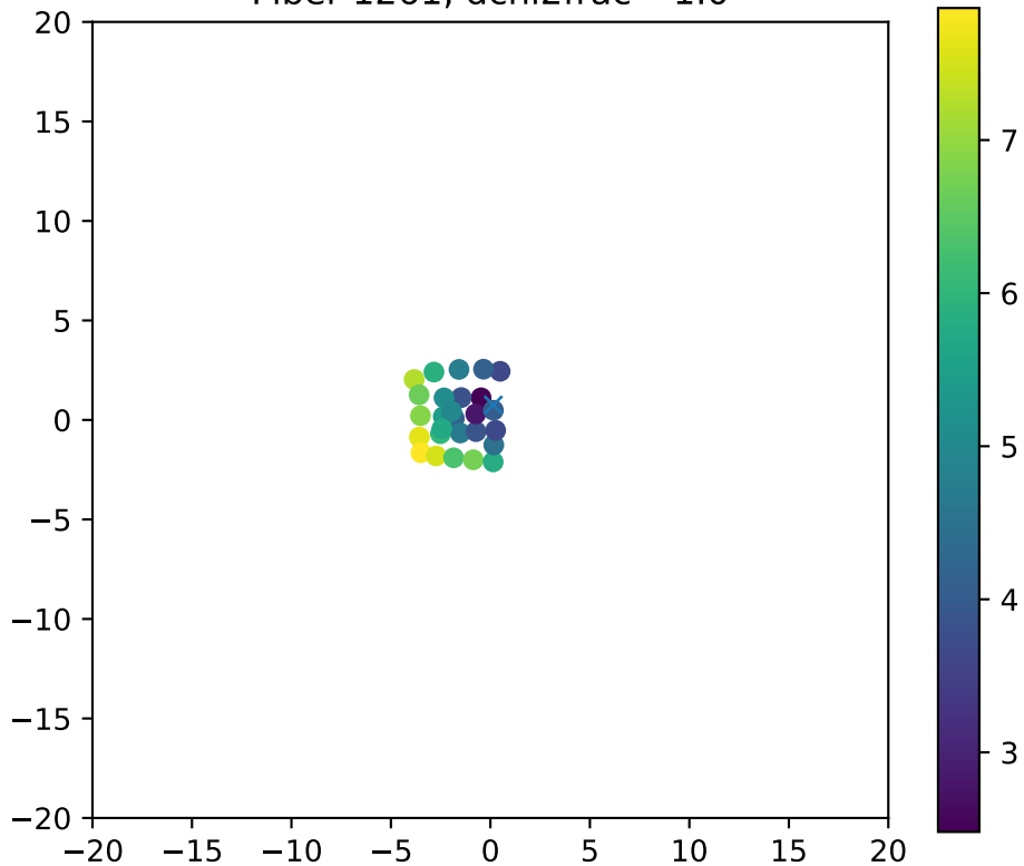
Fiber 1261, dchi2frac= 1.0
