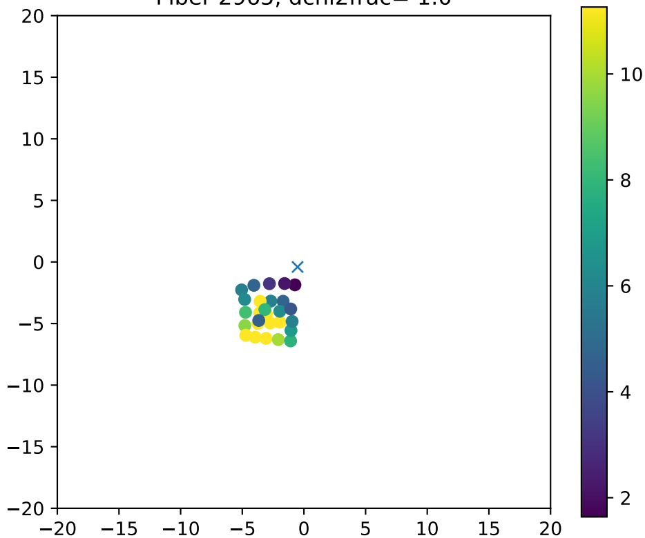
Fiber 2965, dchi2frac= 1.0
