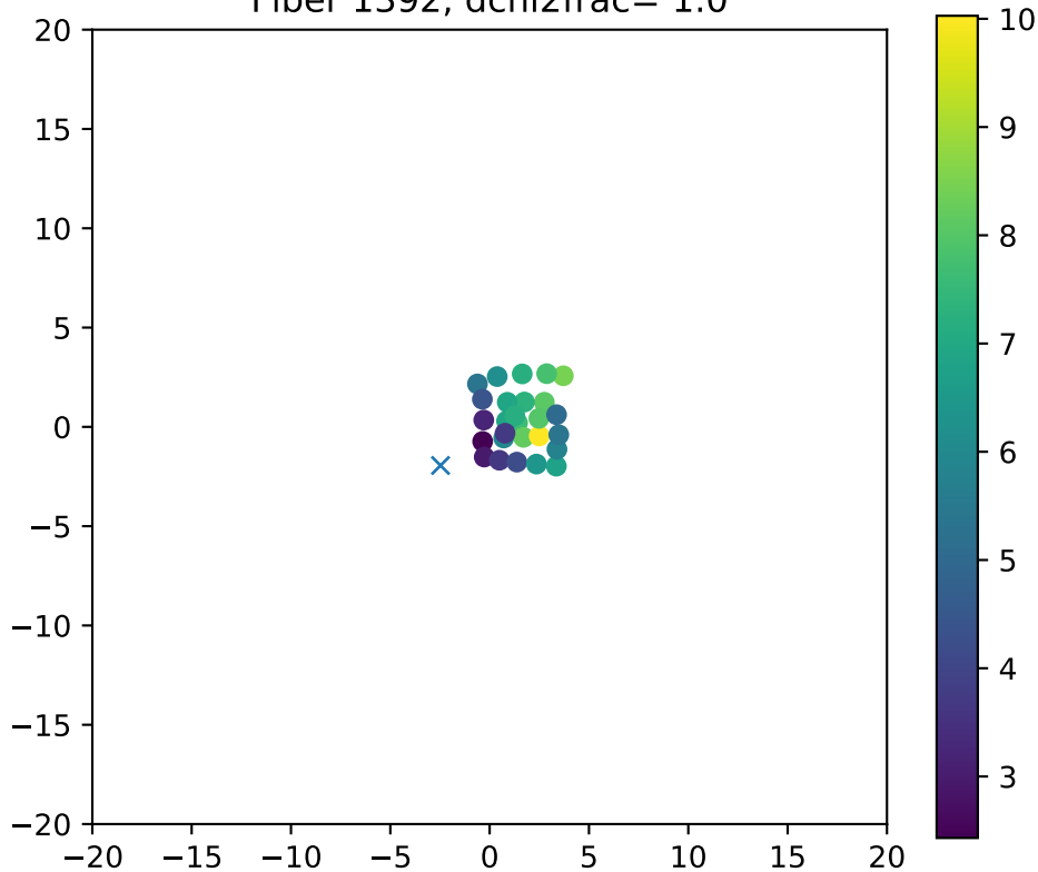
Fiber 1392, dchi2frac= 1.0
