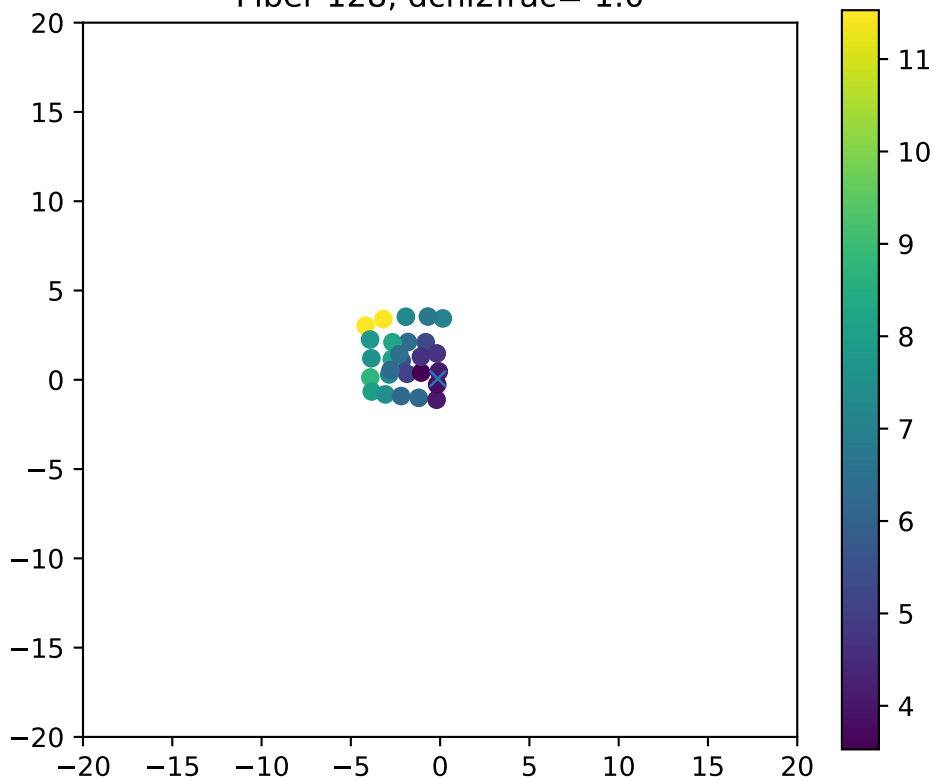
Fiber 128, dchi2frac= 1.0
