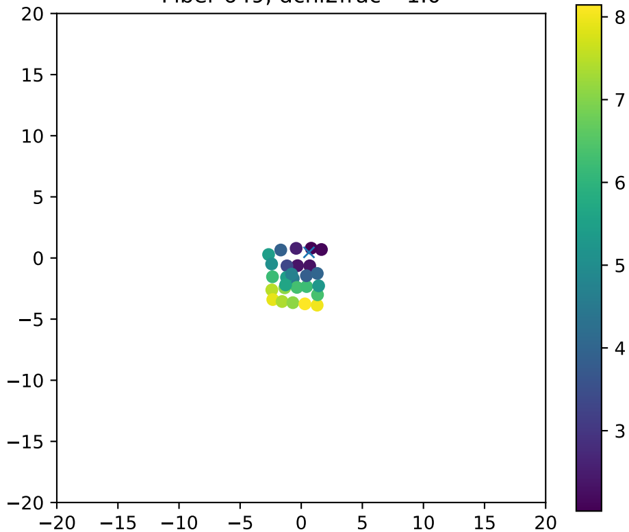
Fiber 649, dchi2frac= 1.0
