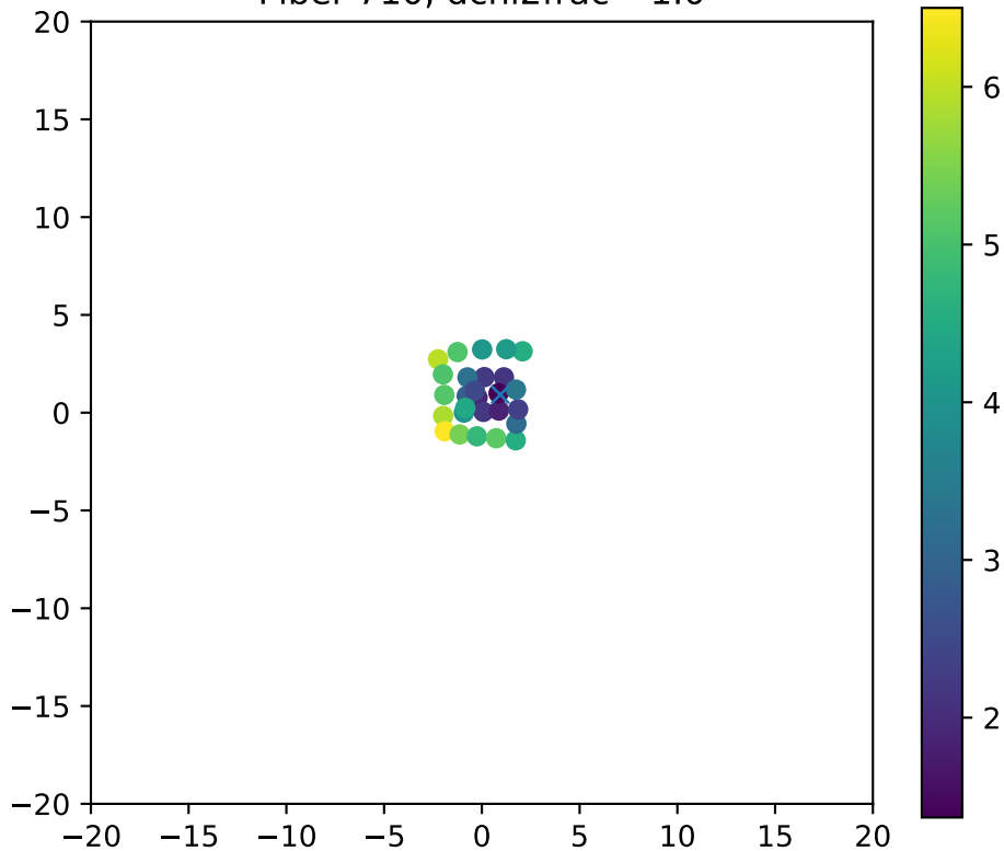
Fiber 710, dchi2frac= 1.0
