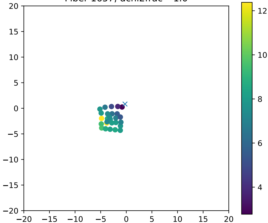
Fiber 1657, dchi2frac= 1.0
