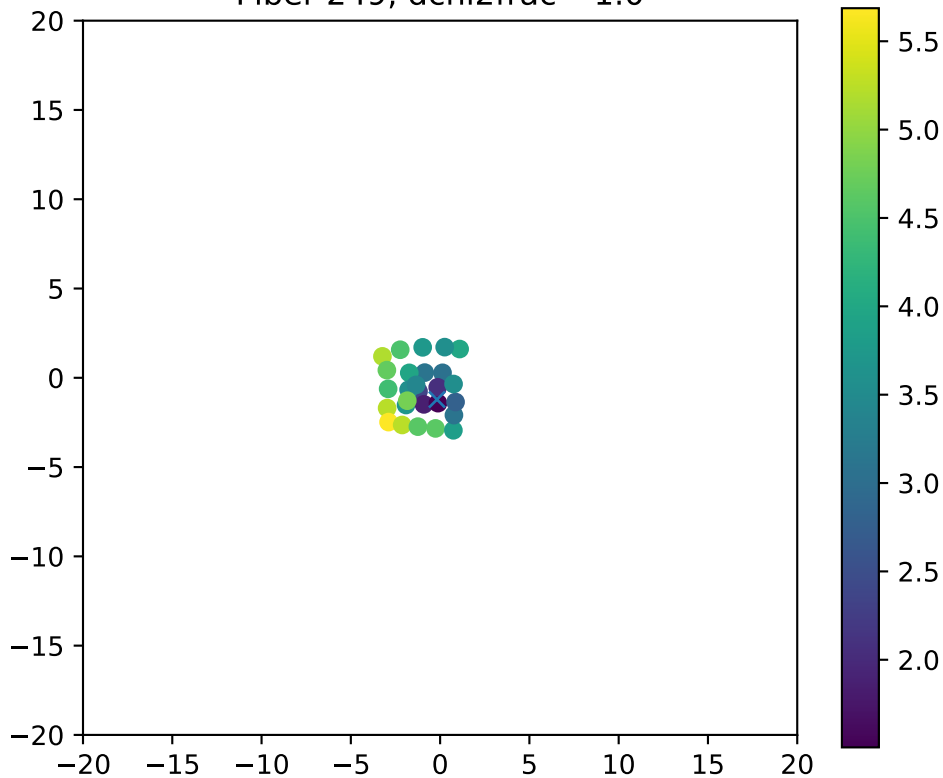
Fiber 249, dchi2frac= 1.0
