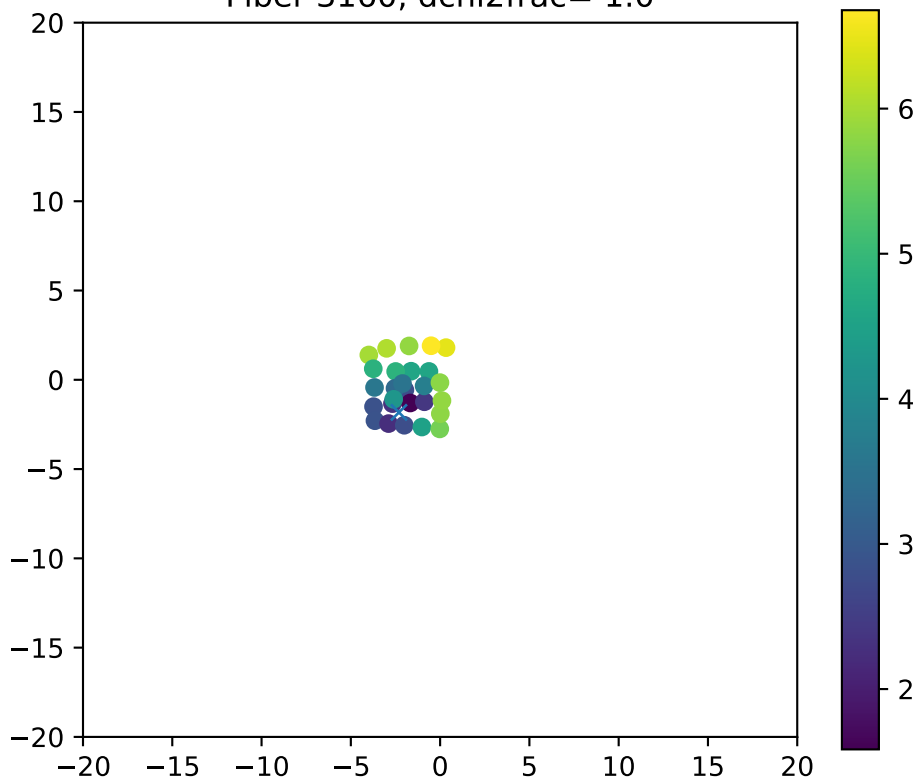
Fiber 3160, dchi2frac= 1.0
