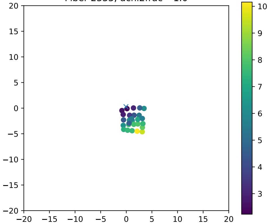
Fiber 2333, dchi2frac= 1.0
