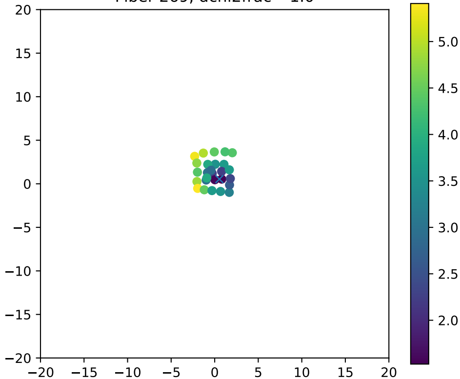
Fiber 269, dchi2frac= 1.0
