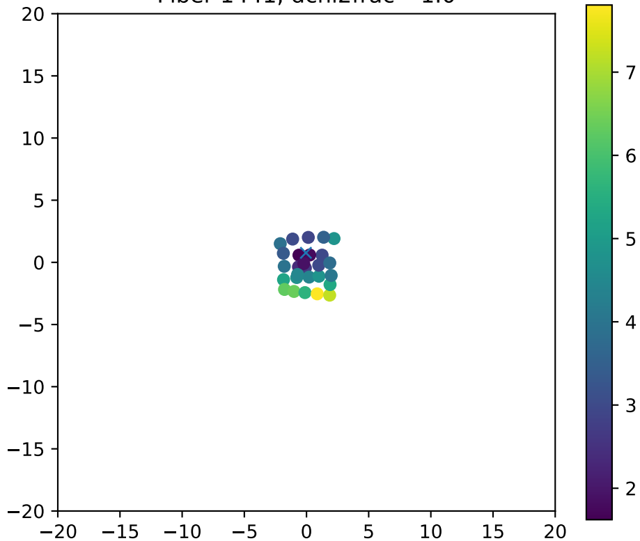
Fiber 1441, dchi2frac= 1.0
