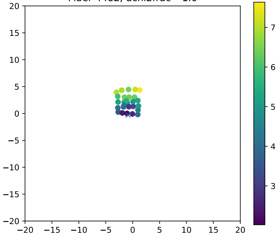
Fiber 4482, dchi2frac= 1.0
