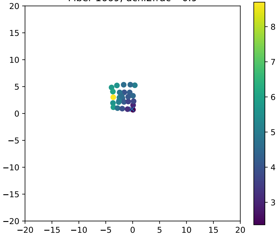
Fiber 1669, dchi2frac= 0.9
