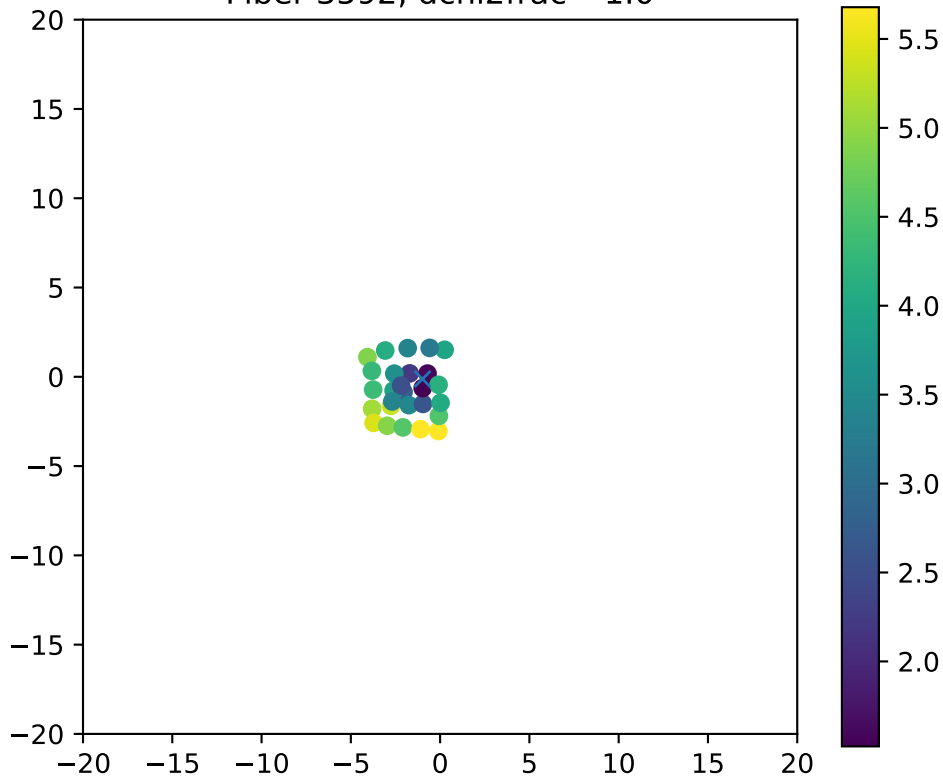
Fiber 3592, dchi2frac= 1.0
