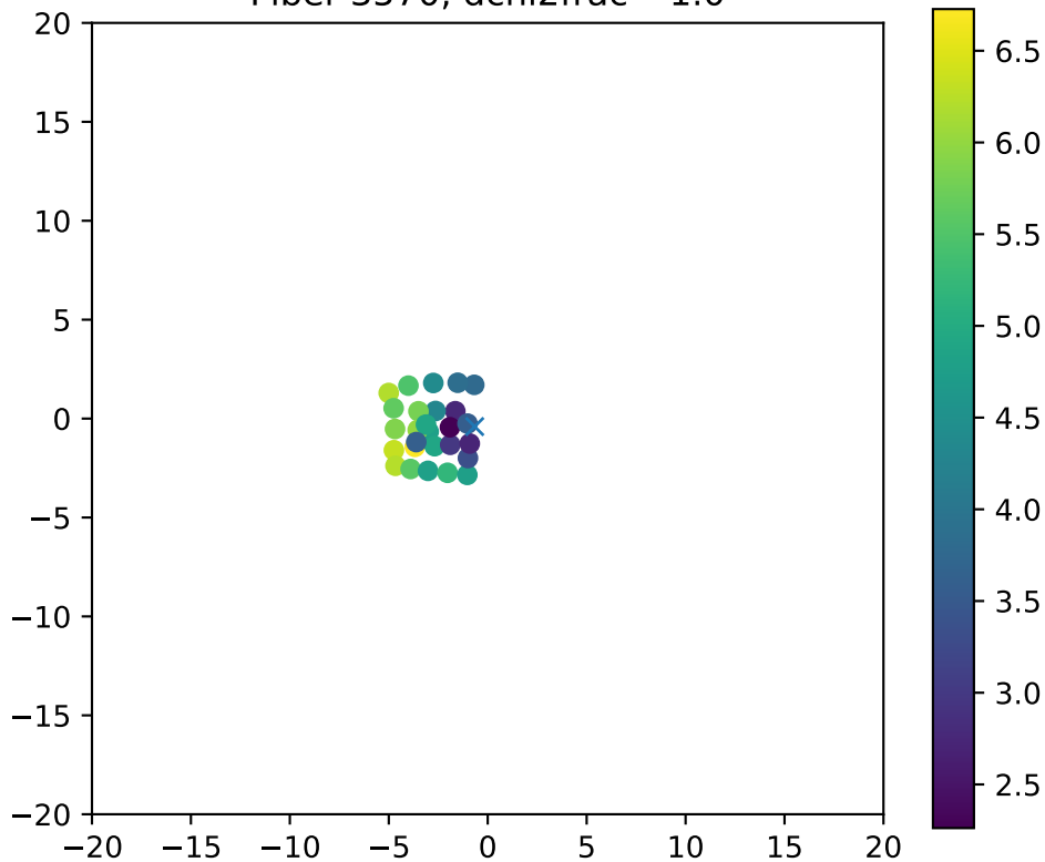
Fiber 3570, dchi2frac= 1.0
