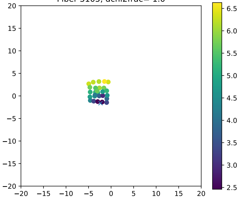
Fiber 3105, dchi2frac= 1.0
