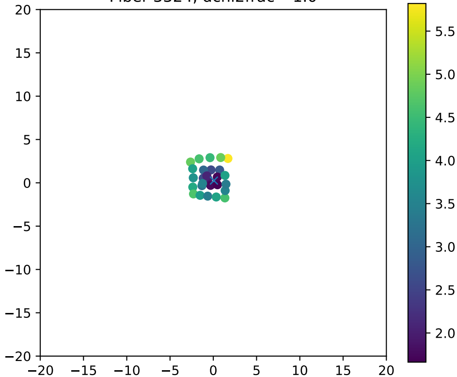
Fiber 3324, dchi2frac= 1.0
