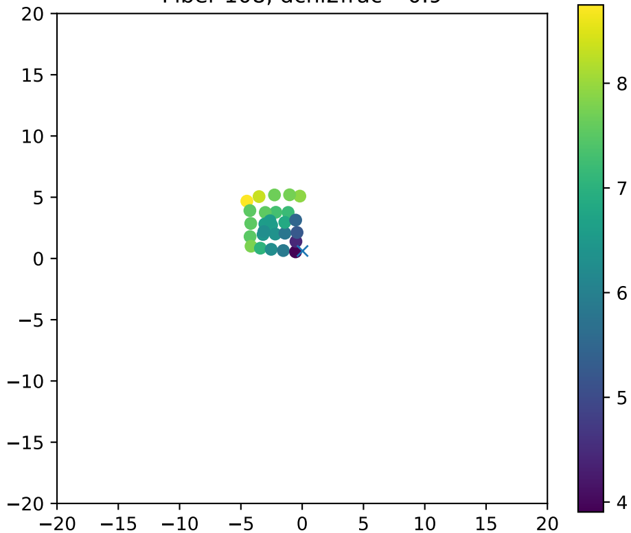
Fiber 108, dchi2frac= 0.9
