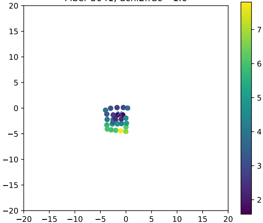
Fiber 3041, dchi2frac= 1.0
