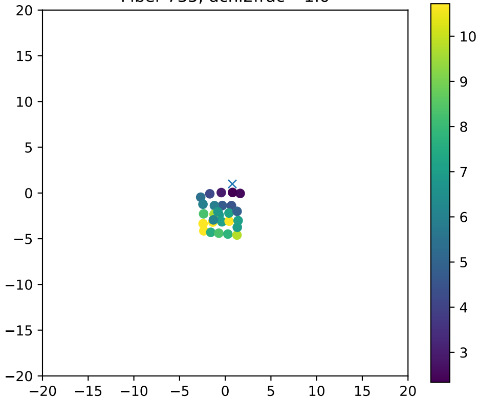
Fiber 735, dchi2frac= 1.0
