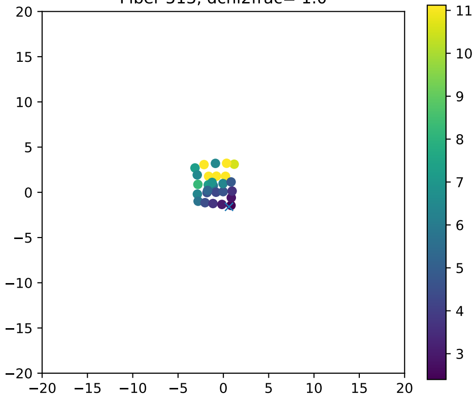
Fiber 513, dchi2frac= 1.0
