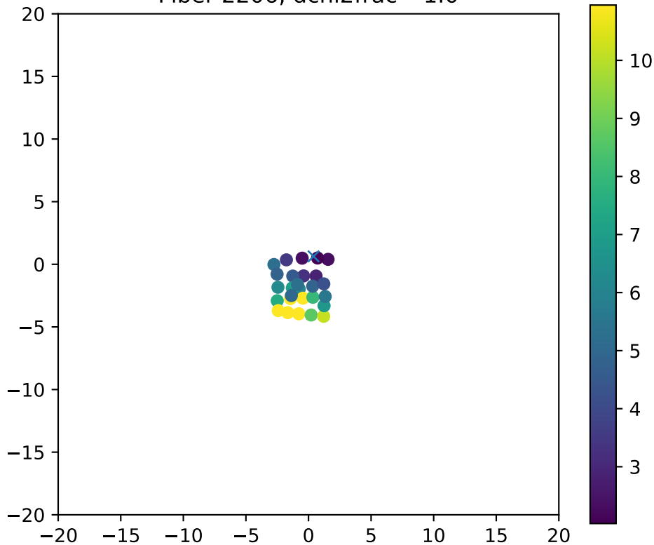
Fiber 2206, dchi2frac= 1.0
