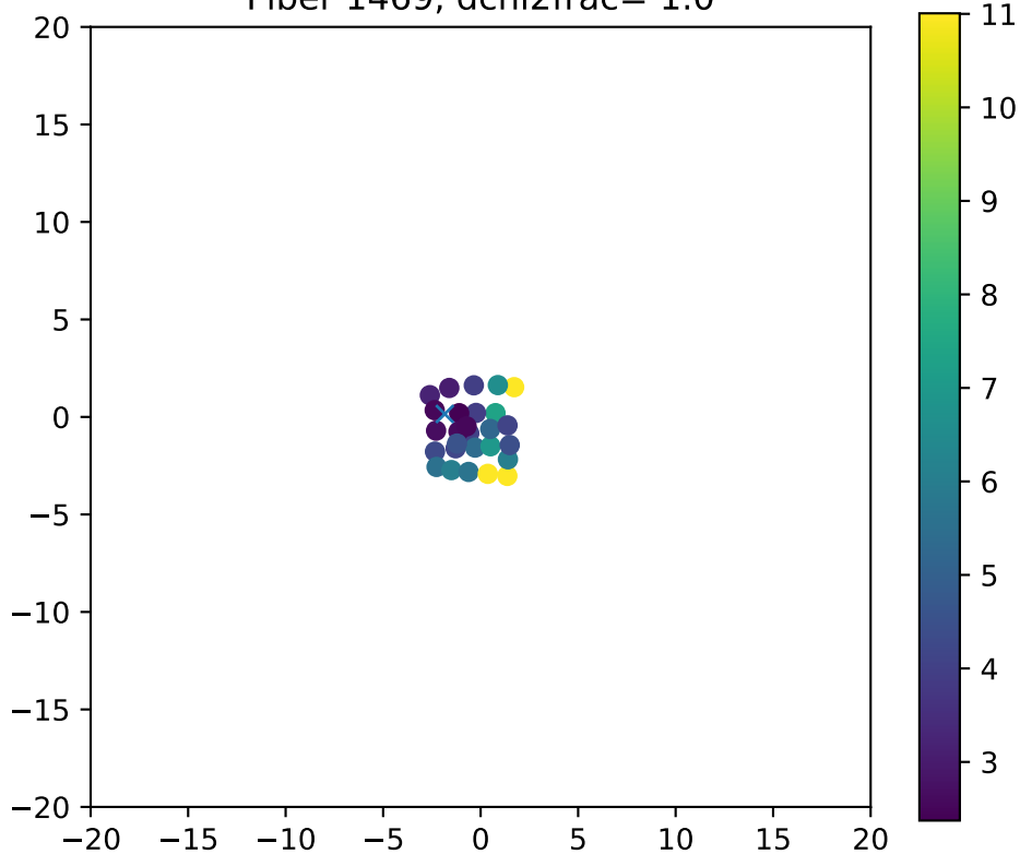
Fiber 1469, dchi2frac= 1.0
