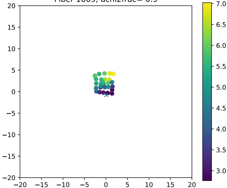
Fiber 1069, dchi2frac= 0.9
