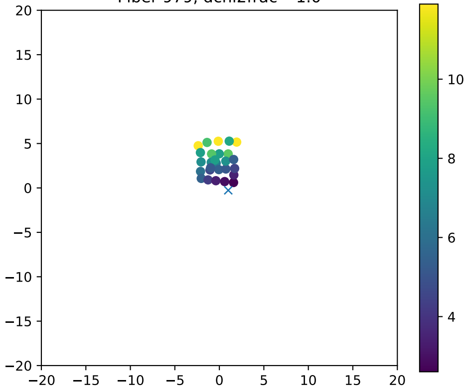
Fiber 979, dchi2frac= 1.0
