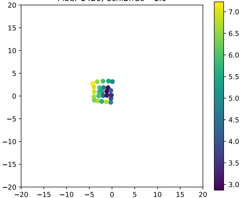
Fiber 1426, dchi2frac= 1.0
