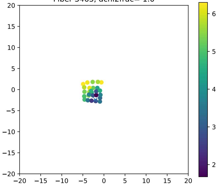
Fiber 3463, dchi2frac= 1.0
