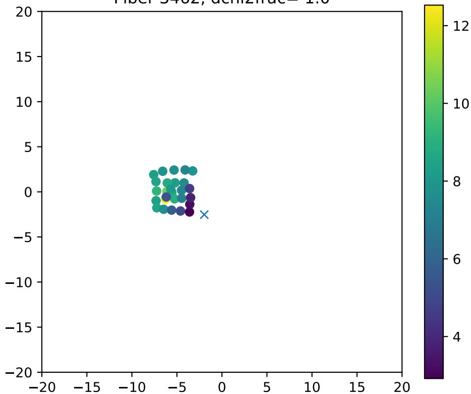
Fiber 3462, dchi2frac= 1.0
