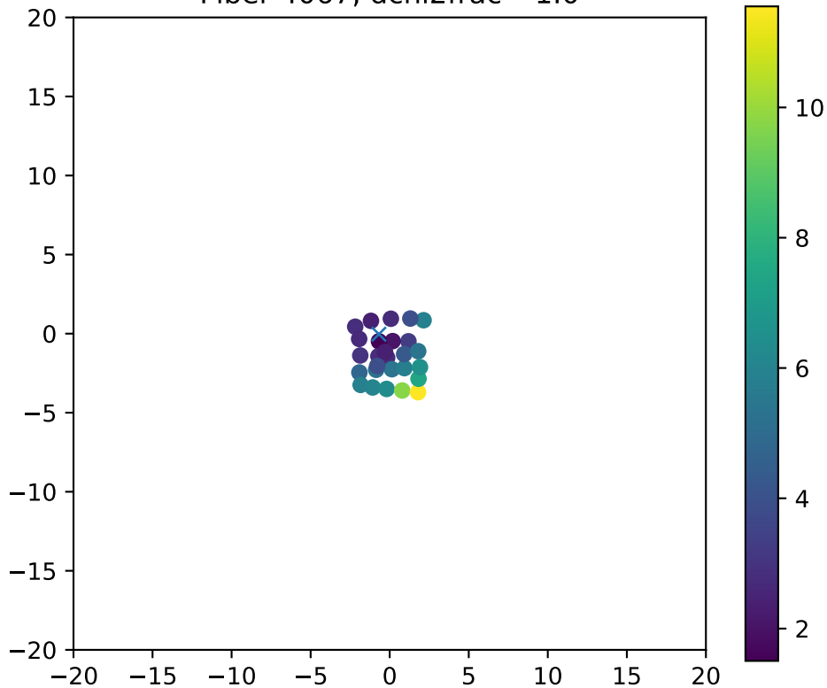
Fiber 4067, dchi2frac= 1.0
