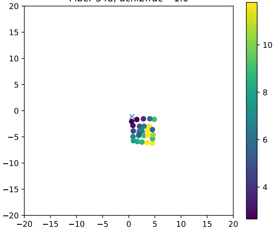
Fiber 348, dchi2frac= 1.0
