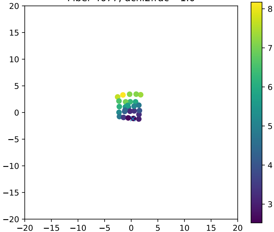
Fiber 4677, dchi2frac= 1.0
