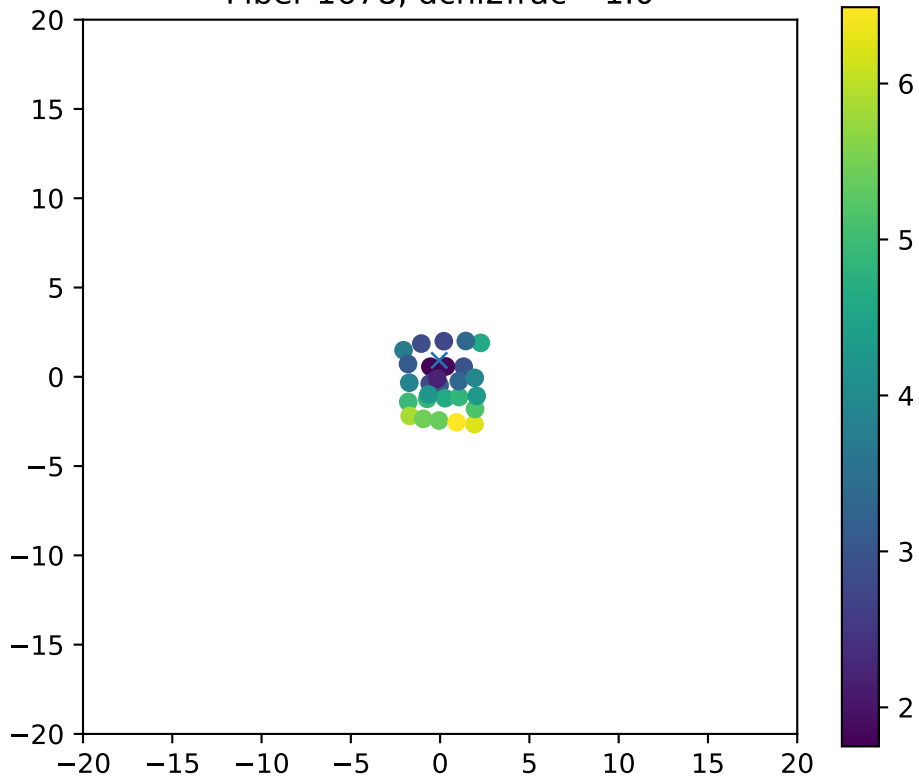
Fiber 1678, dchi2frac= 1.0
