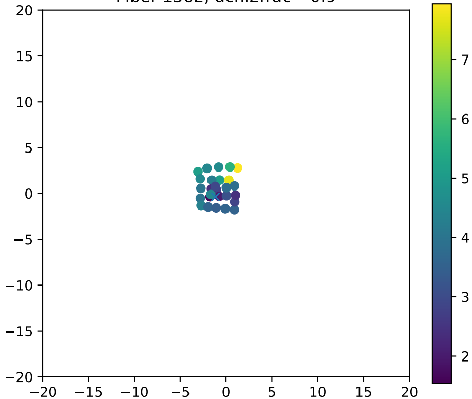
Fiber 1362, dchi2frac= 0.9
