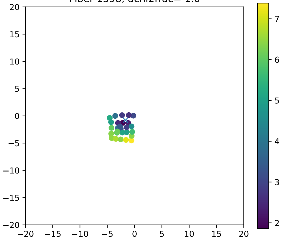
Fiber 1398, dchi2frac= 1.0
