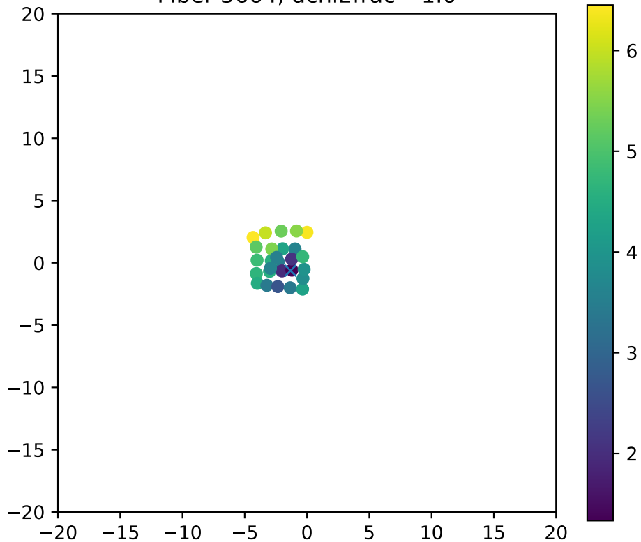
Fiber 3664, dchi2frac= 1.0
