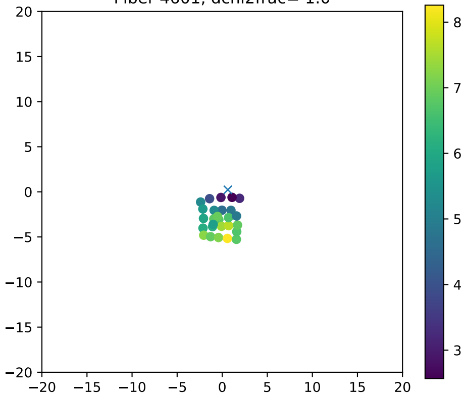
Fiber 4601, dchi2frac= 1.0
