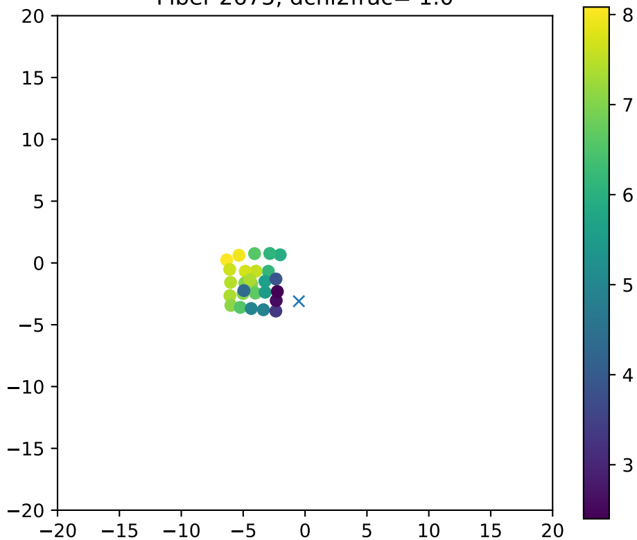
Fiber 2675, dchi2frac= 1.0
