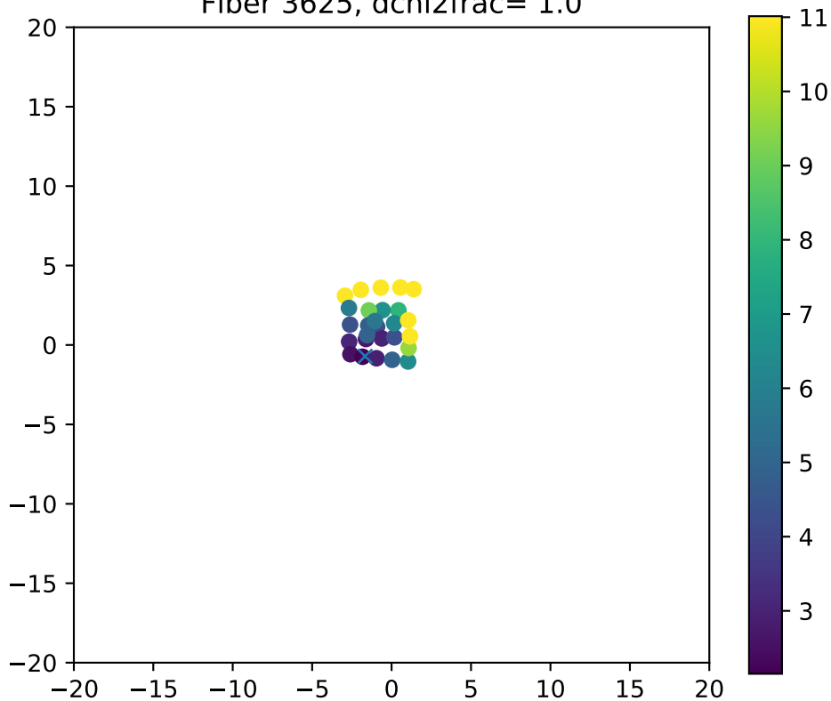
Fiber 3625, dchi2frac= 1.0
