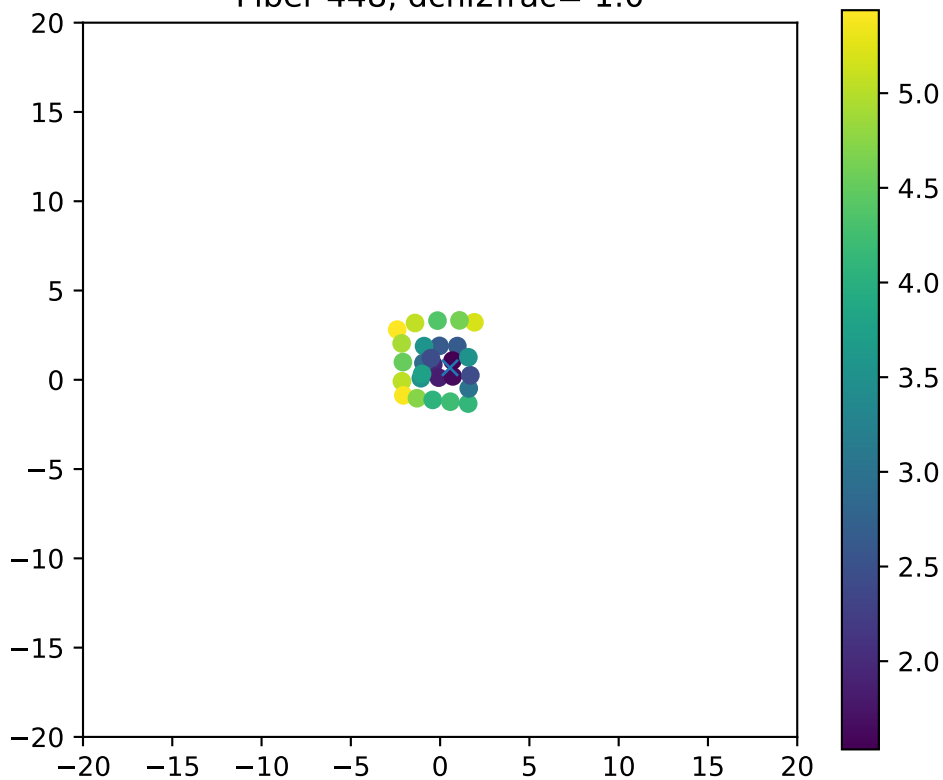
Fiber 448, dchi2frac= 1.0
