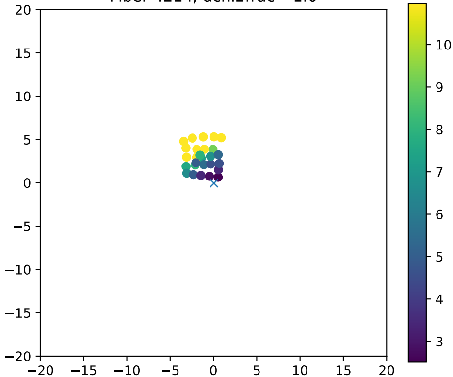
Fiber 4214, dchi2frac= 1.0
