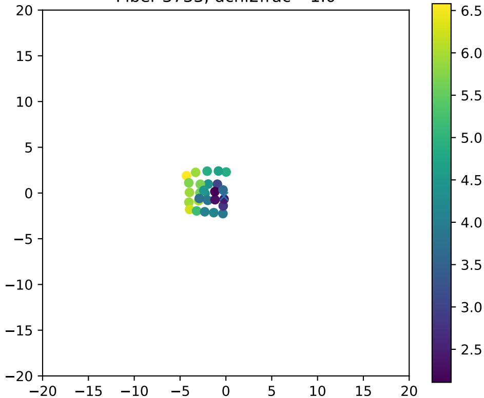
Fiber 3733, dchi2frac= 1.0
