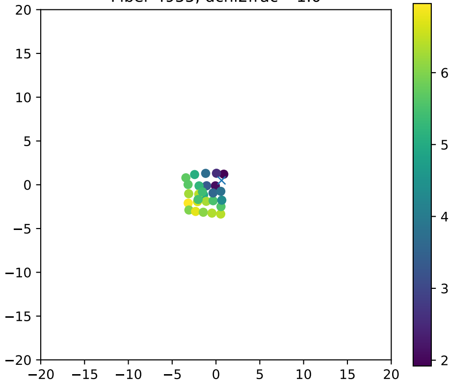
Fiber 4955, dchi2frac= 1.0
