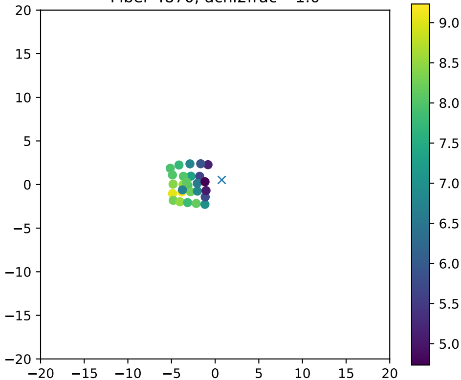
Fiber 4870, dchi2frac= 1.0
