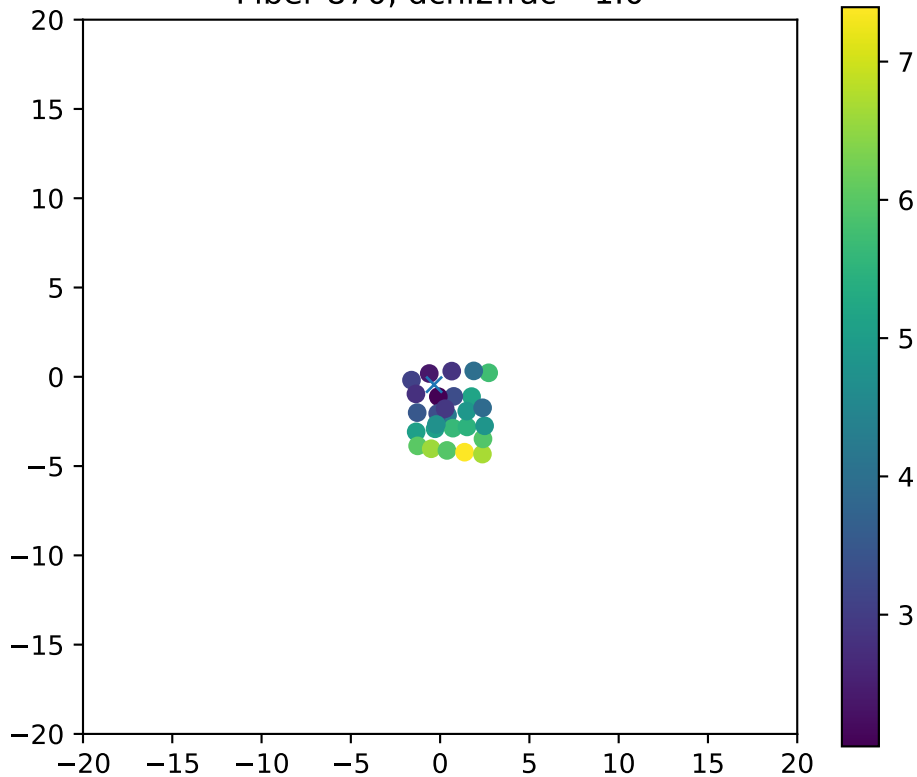
Fiber 870, dchi2frac= 1.0
