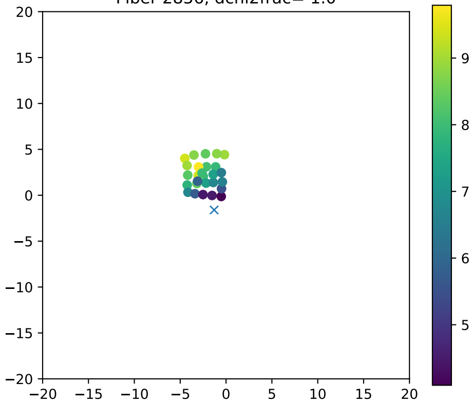
Fiber 2856, dchi2frac= 1.0
