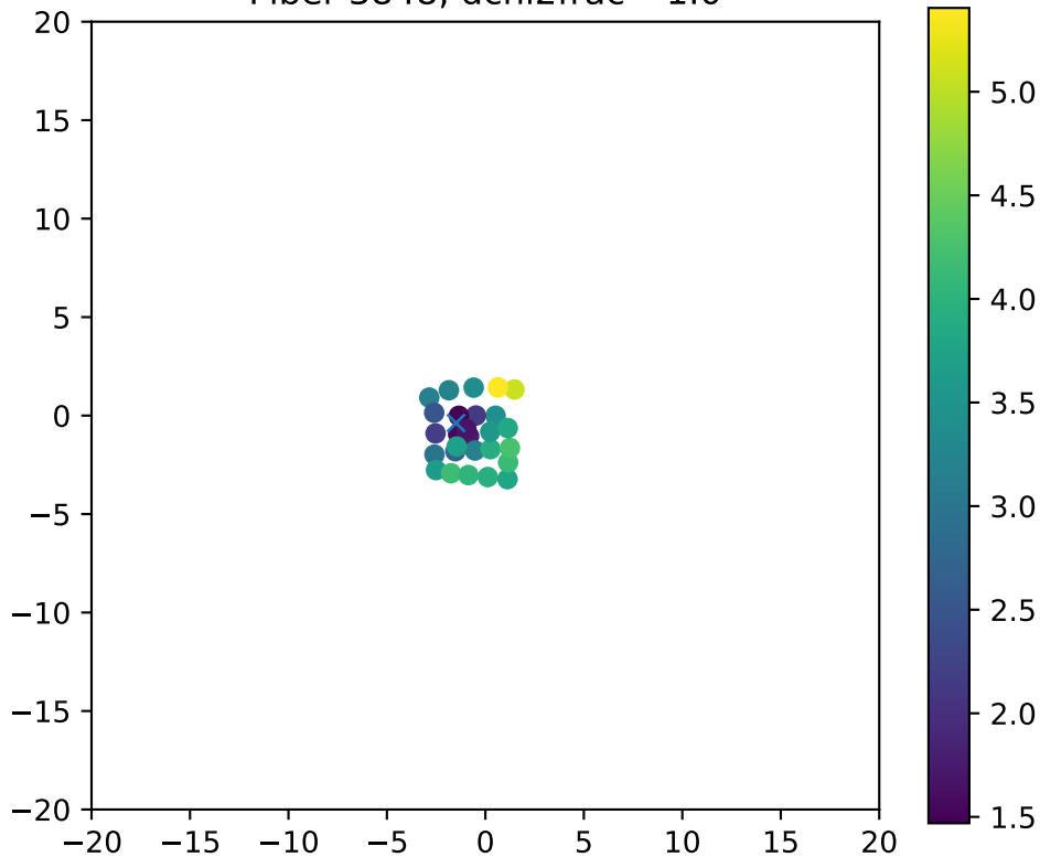
Fiber 3848, dchi2frac= 1.0
