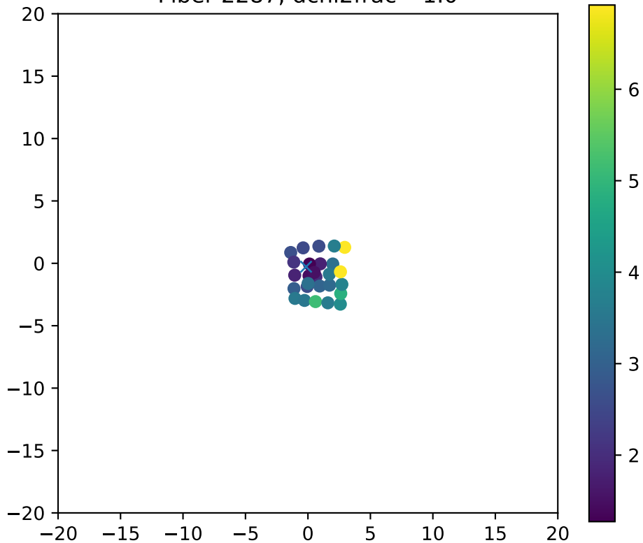
Fiber 2287, dchi2frac= 1.0
