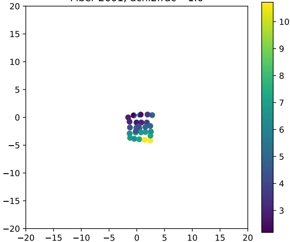
Fiber 2601, dchi2frac= 1.0
