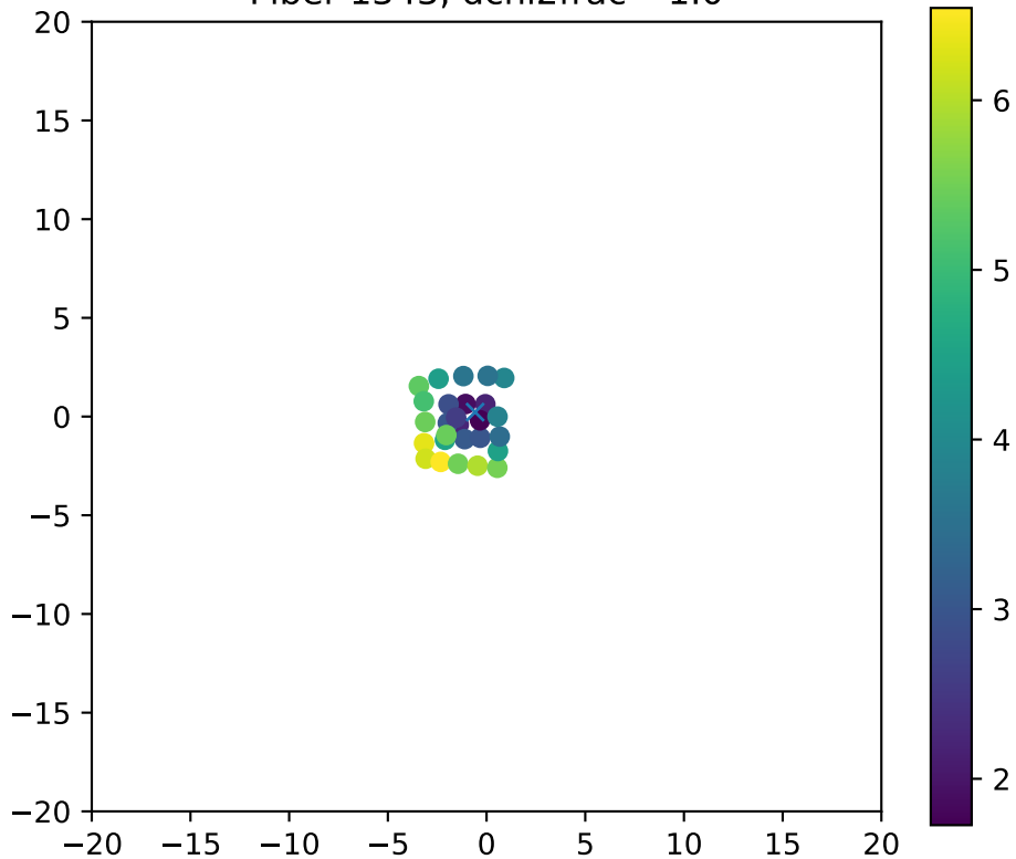
Fiber 1343, dchi2frac= 1.0
