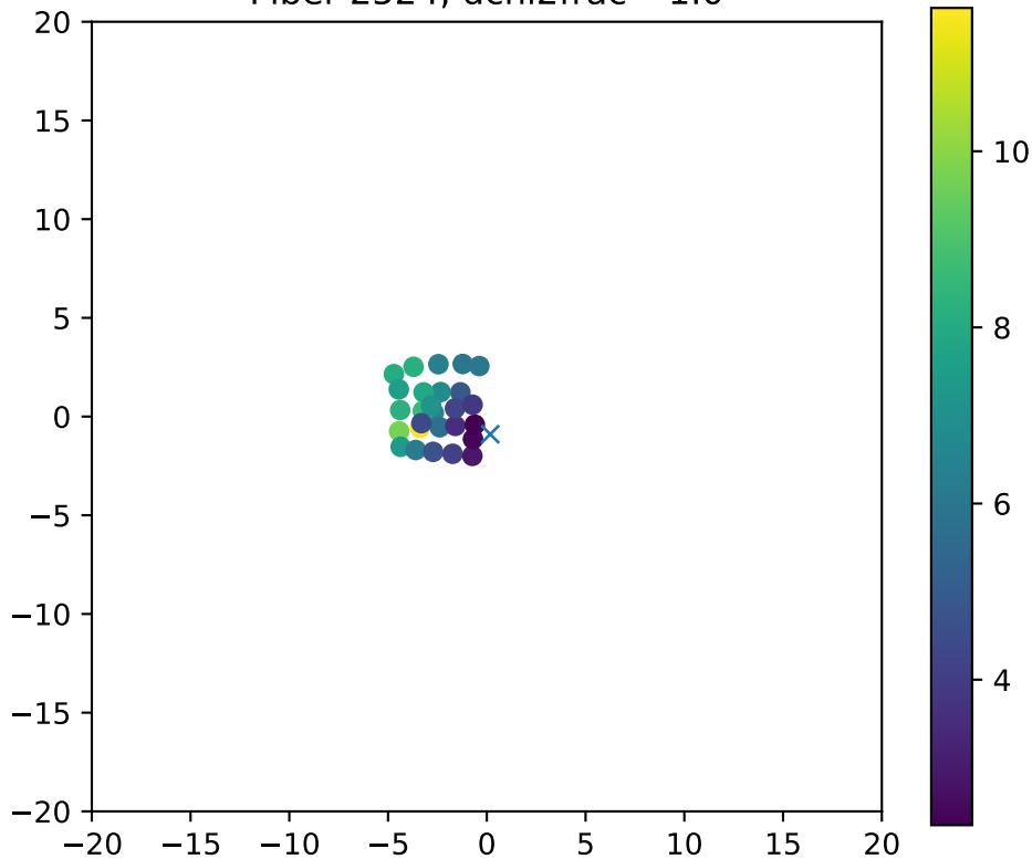
Fiber 2524, dchi2frac= 1.0
