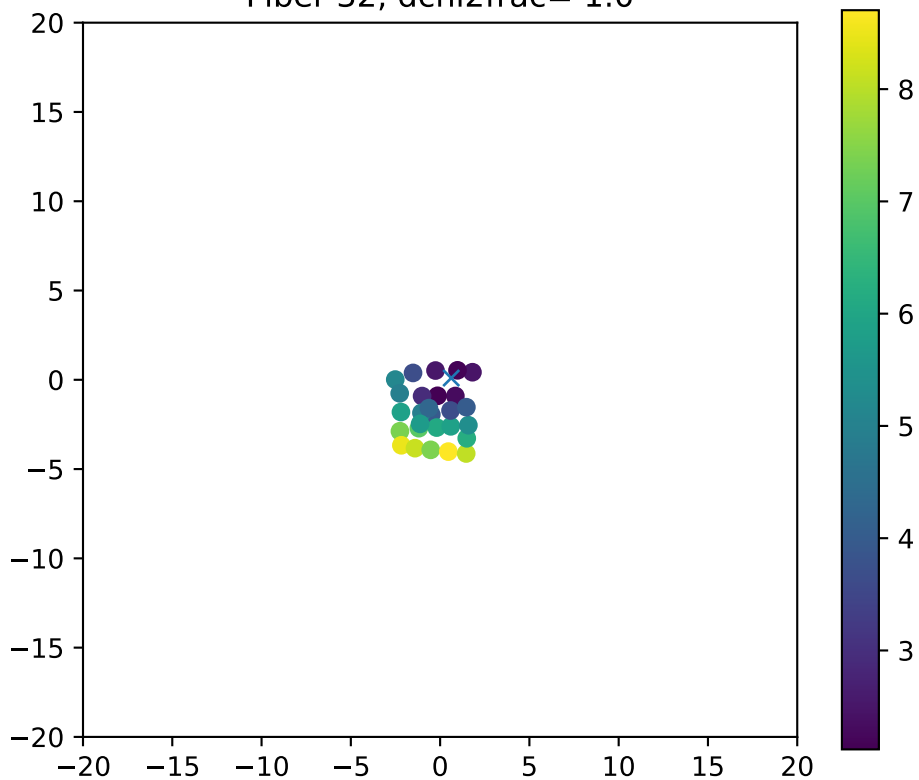
Fiber 32, dchi2frac= 1.0
