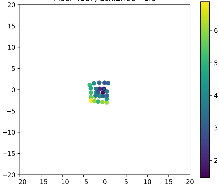
Fiber 4187, dchi2frac= 1.0
