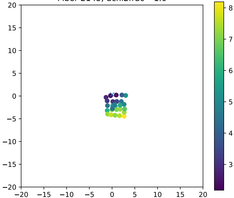
Fiber 2145, dchi2frac= 1.0
