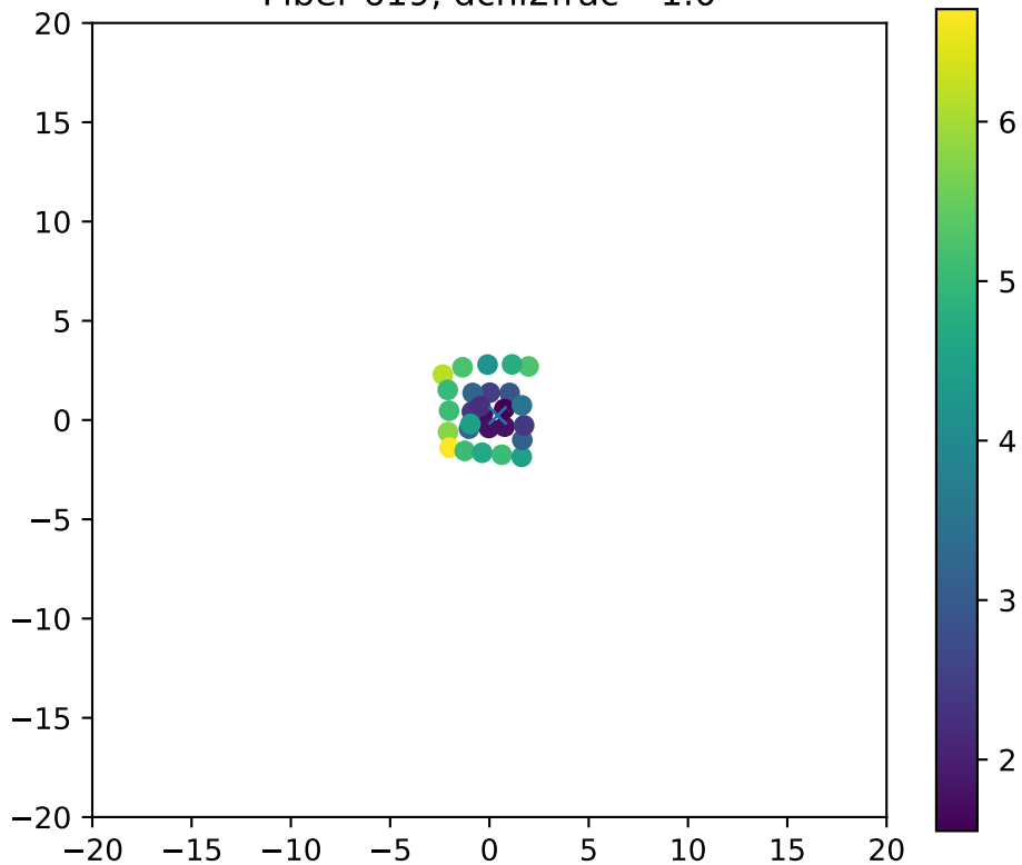
Fiber 619, dchi2frac= 1.0
