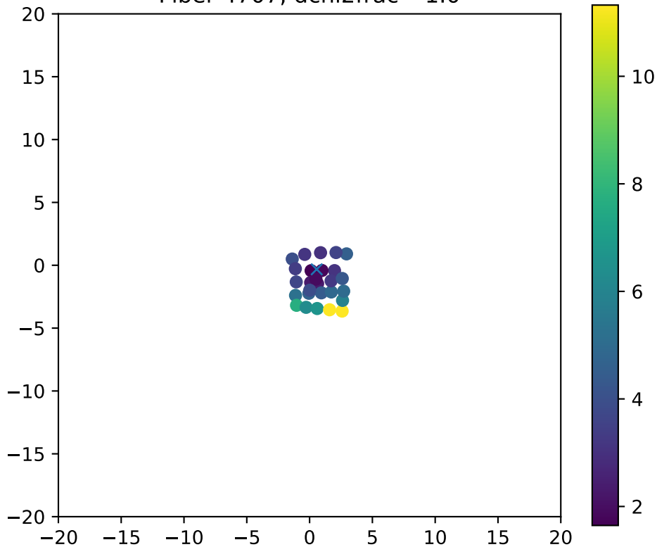
Fiber 4707, dchi2frac= 1.0
