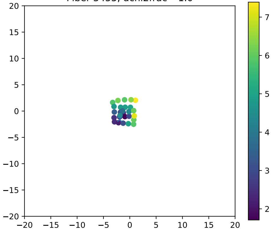
Fiber 3455, dchi2frac= 1.0
