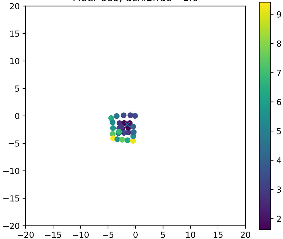
Fiber 669, dchi2frac= 1.0
