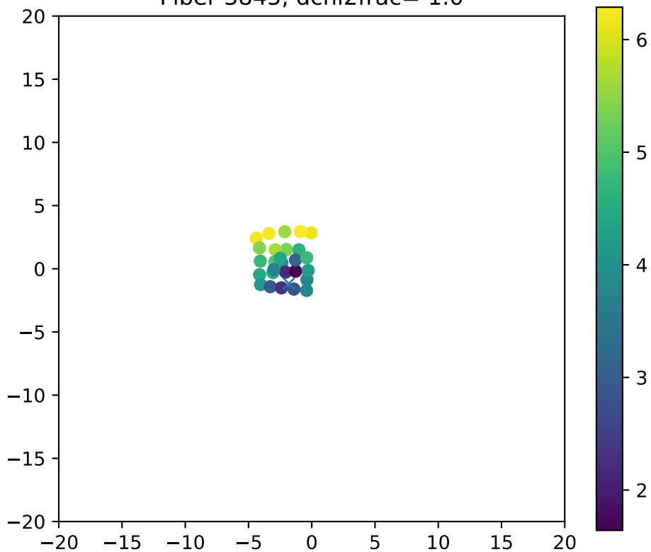
Fiber 3845, dchi2frac= 1.0
