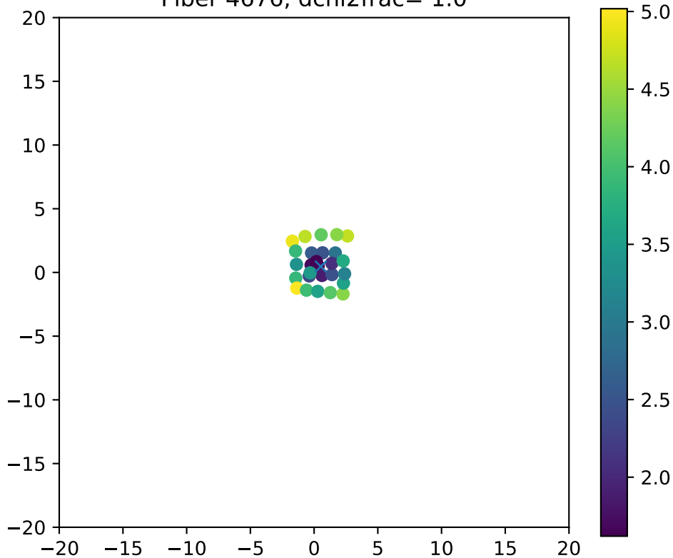
Fiber 4676, dchi2frac= 1.0
