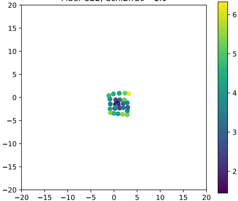
Fiber 322, dchi2frac= 1.0
