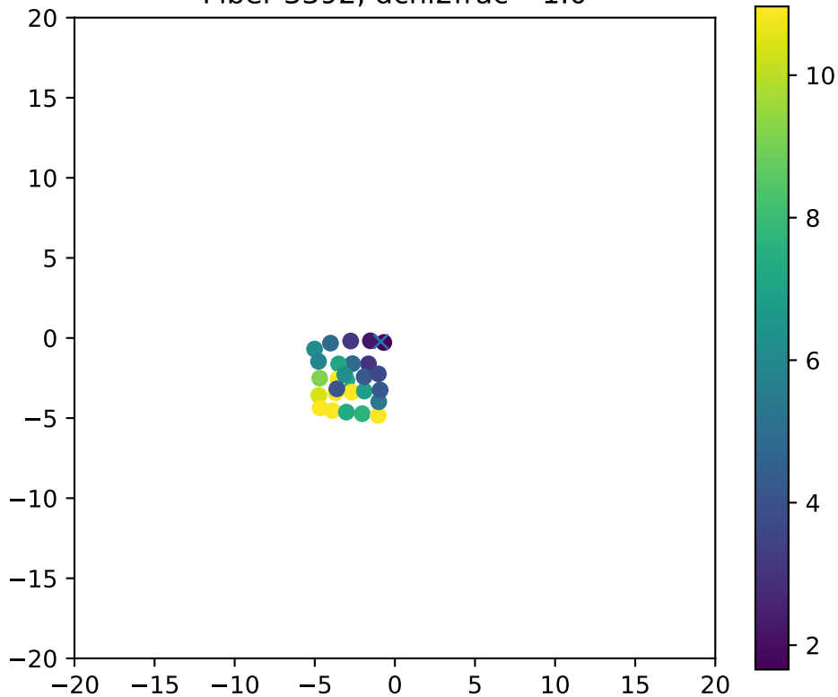
Fiber 3392, dchi2frac= 1.0
