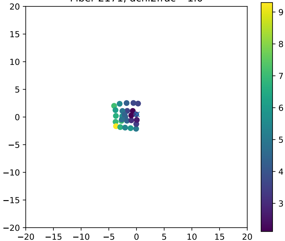
Fiber 2171, dchi2frac= 1.0
