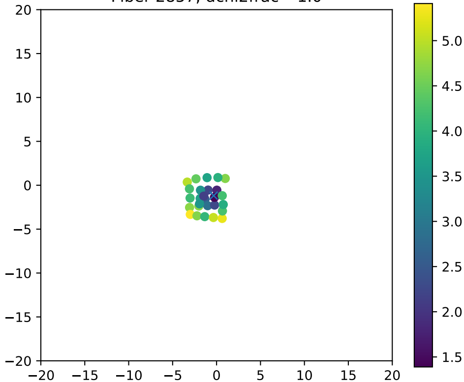
Fiber 2857, dchi2frac= 1.0
