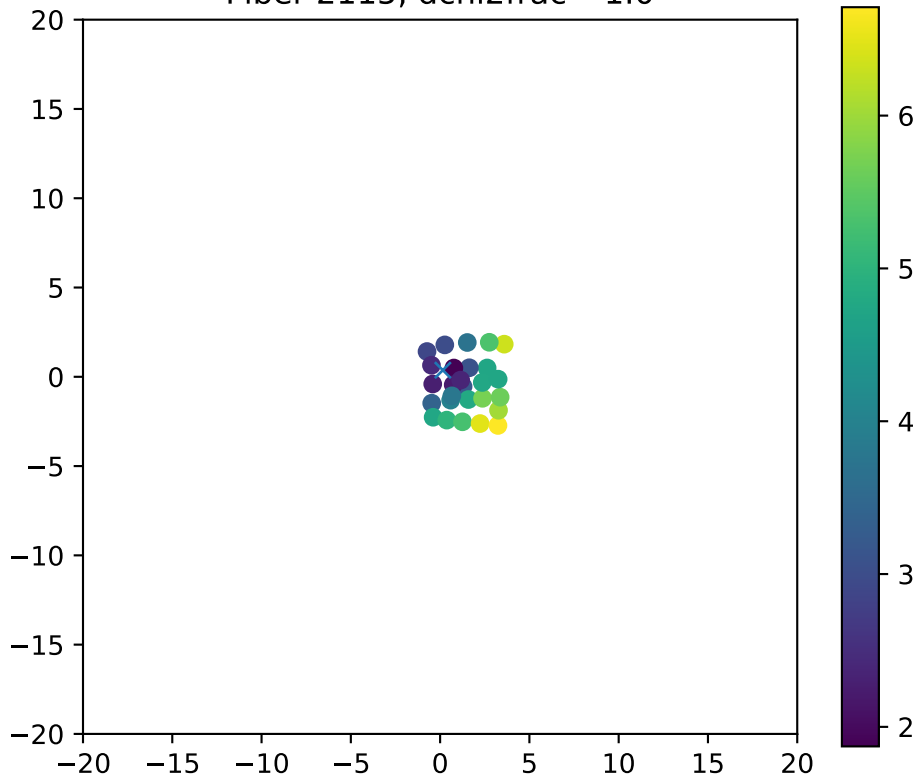
Fiber 2115, dchi2frac= 1.0
