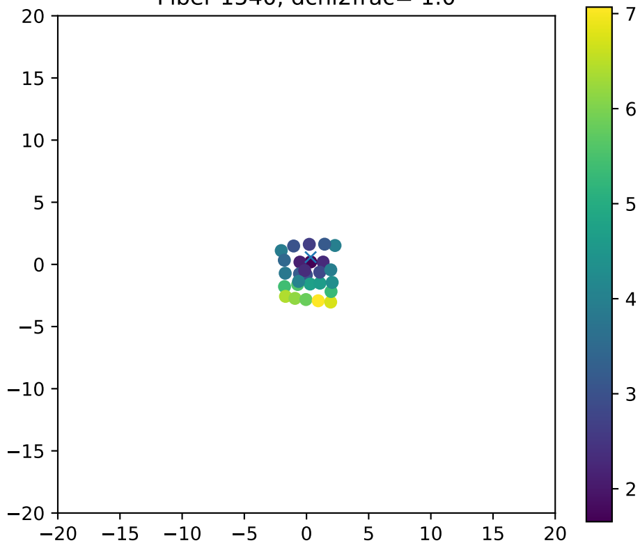
Fiber 1540, dchi2frac= 1.0
