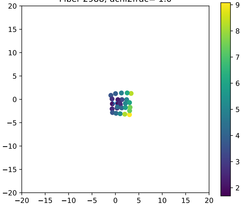
Fiber 2988, dchi2frac= 1.0
