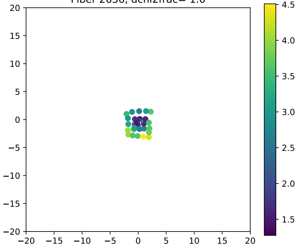
Fiber 2636, dchi2frac= 1.0
