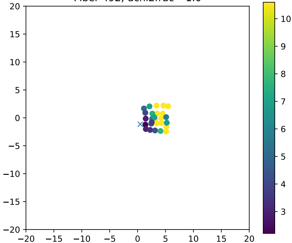
Fiber 492, dchi2frac= 1.0
