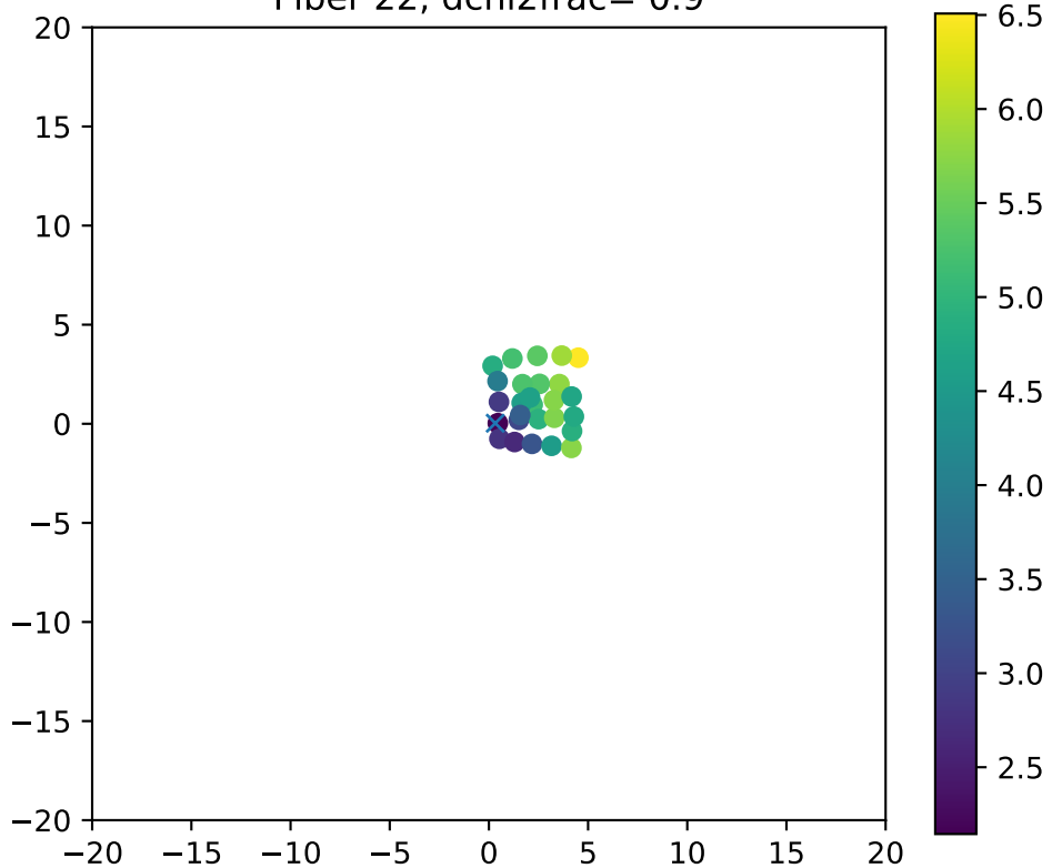
Fiber 22, dchi2frac= 0.9
