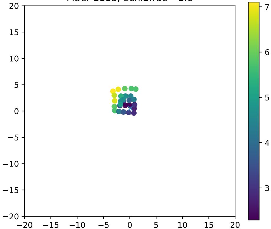
Fiber 1113, dchi2frac= 1.0
