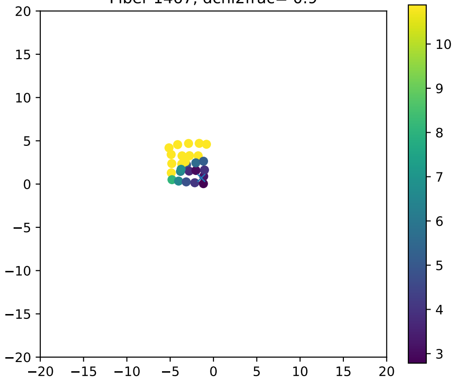
Fiber 1467, dchi2frac= 0.9
