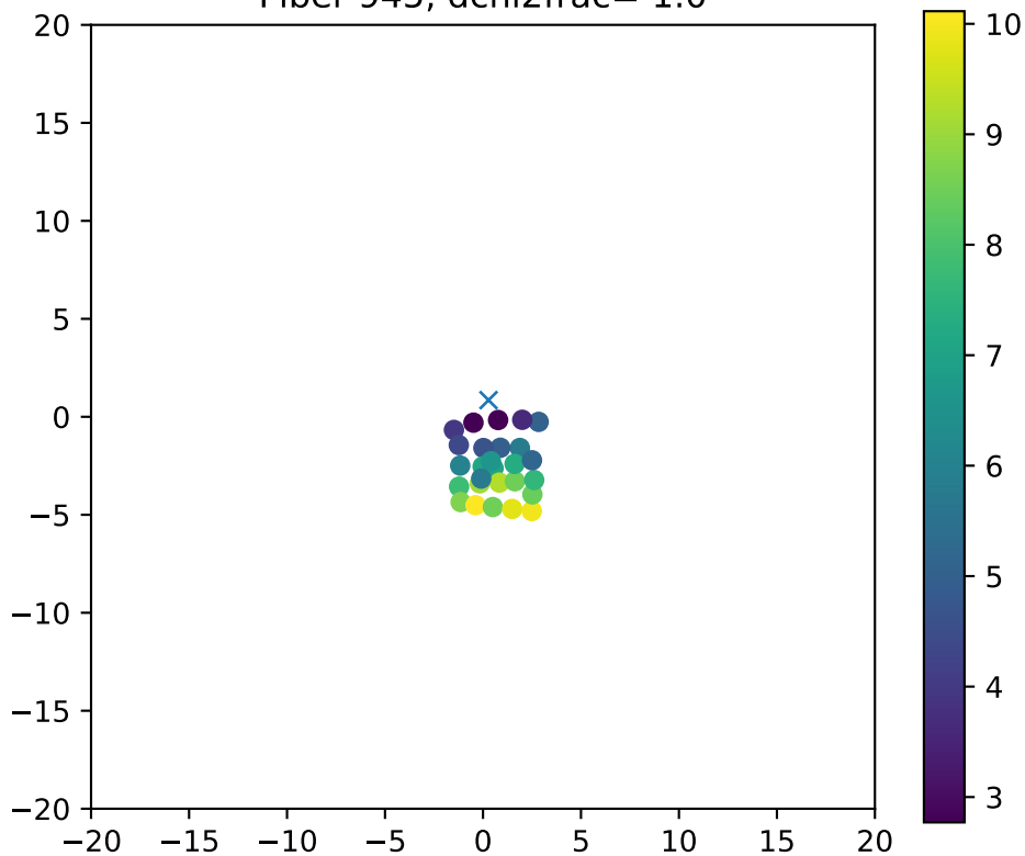
Fiber 945, dchi2frac= 1.0
