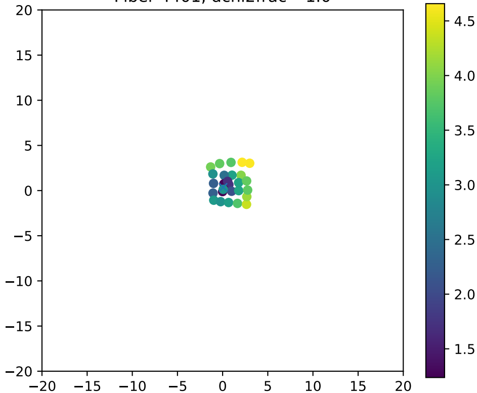
Fiber 4401, dchi2frac= 1.0
