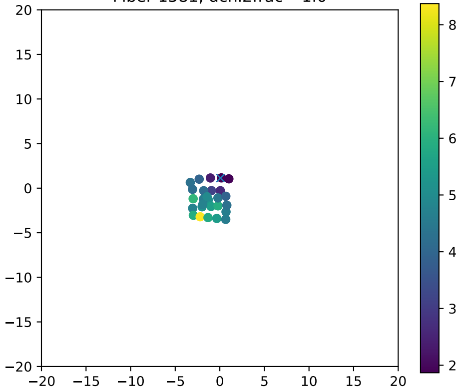
Fiber 1581, dchi2frac= 1.0
