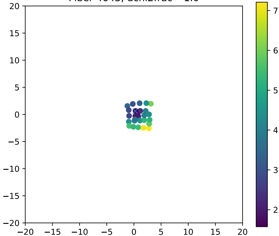
Fiber 4643, dchi2frac= 1.0
