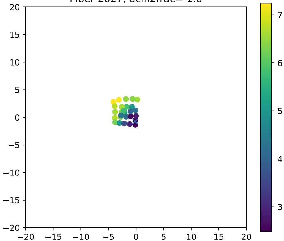
Fiber 2627, dchi2frac= 1.0
