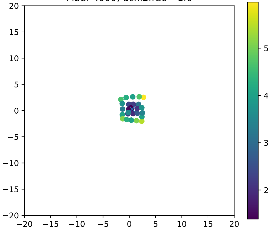
Fiber 4999, dchi2frac= 1.0
