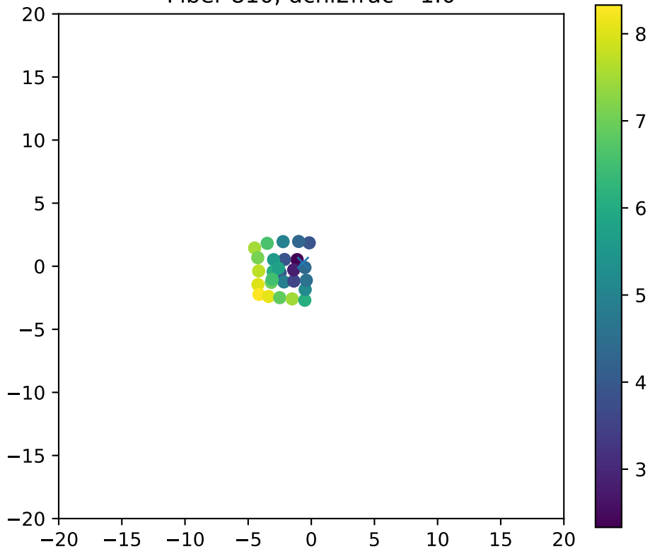
Fiber 810, dchi2frac= 1.0
