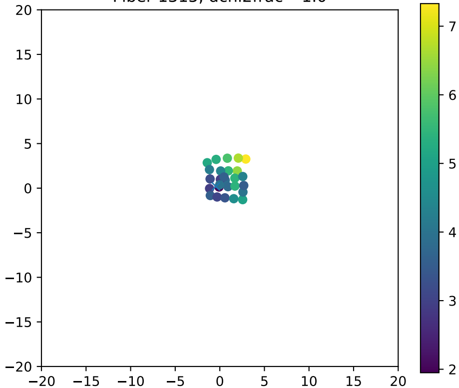
Fiber 1315, dchi2frac= 1.0
