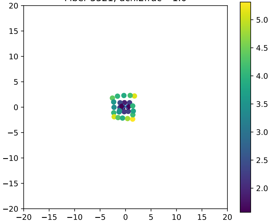
Fiber 3321, dchi2frac= 1.0
