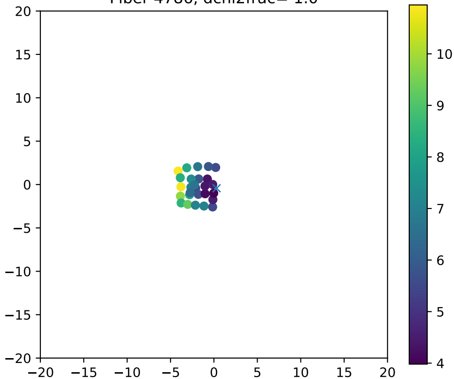
Fiber 4786, dchi2frac= 1.0
