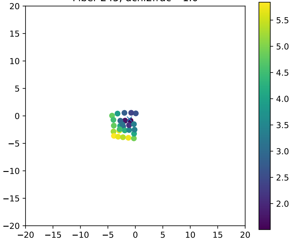
Fiber 245, dchi2frac= 1.0
