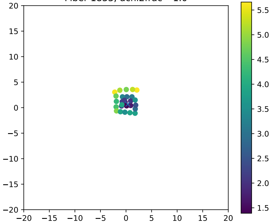
Fiber 1833, dchi2frac= 1.0
