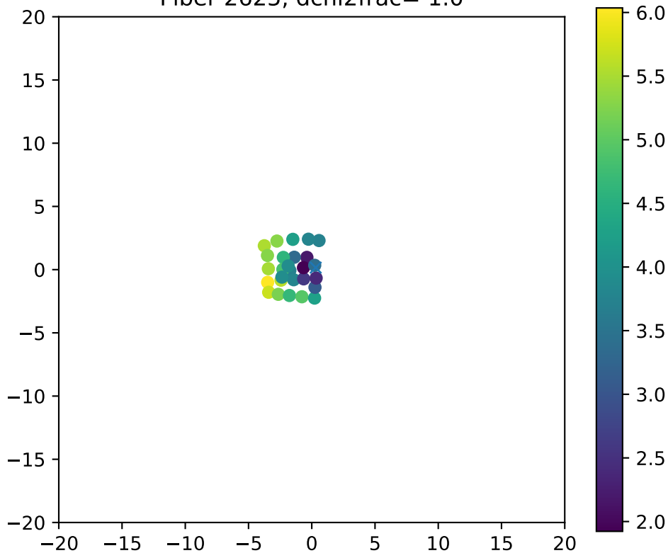
Fiber 2625, dchi2frac= 1.0
