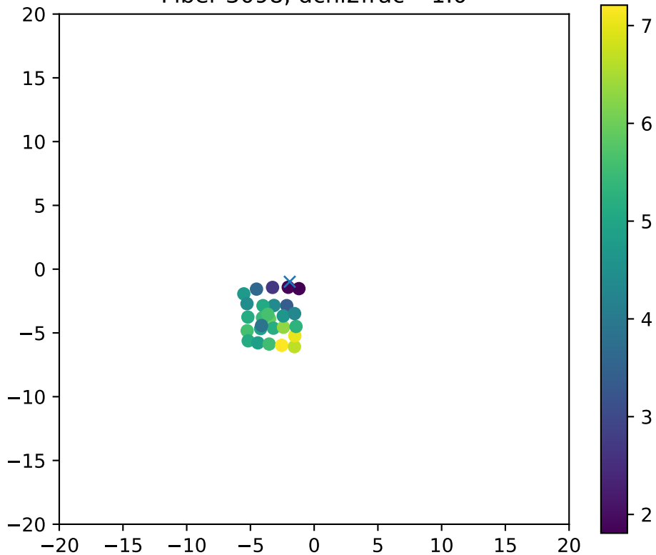
Fiber 3098, dchi2frac= 1.0
