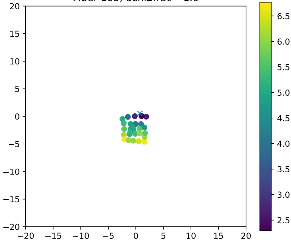
Fiber 105, dchi2frac= 1.0
