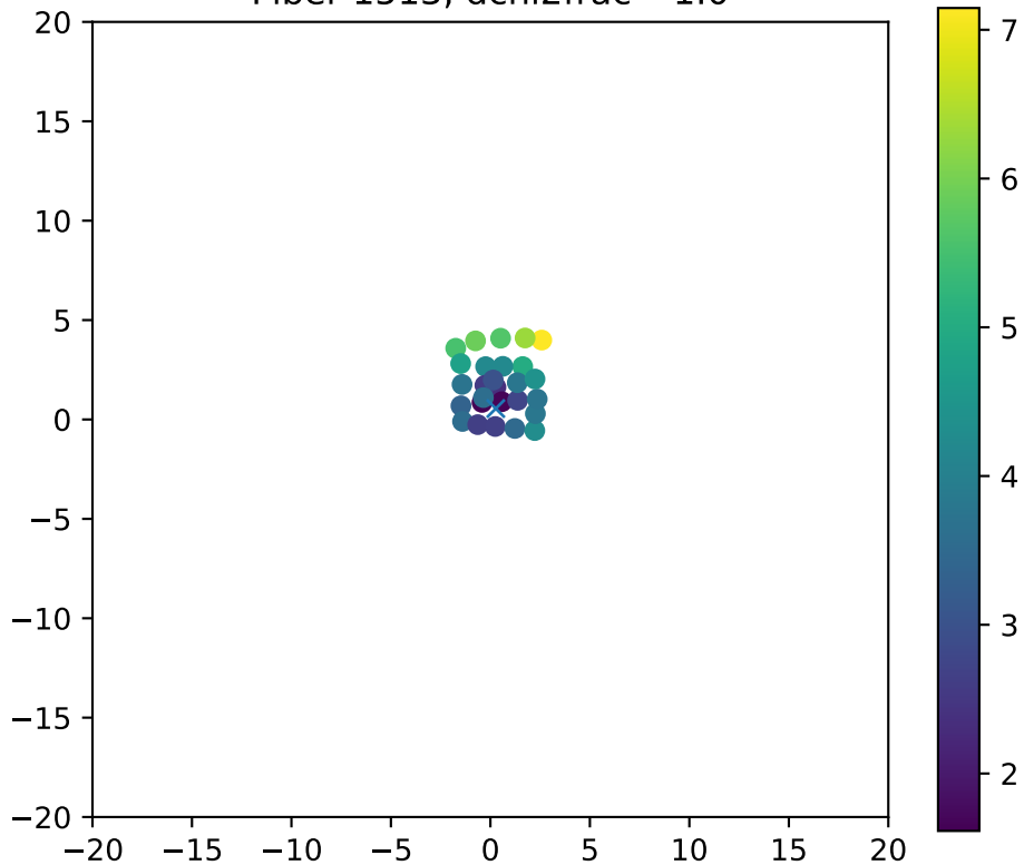
Fiber 1513, dchi2frac= 1.0
