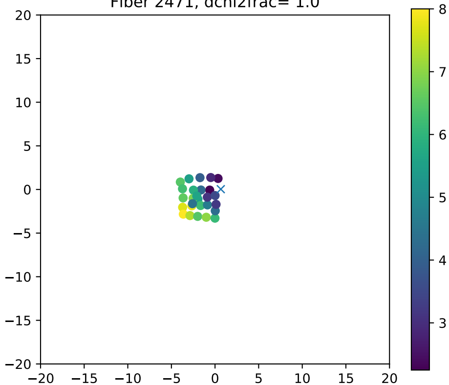
Fiber 2471, dchi2frac= 1.0
