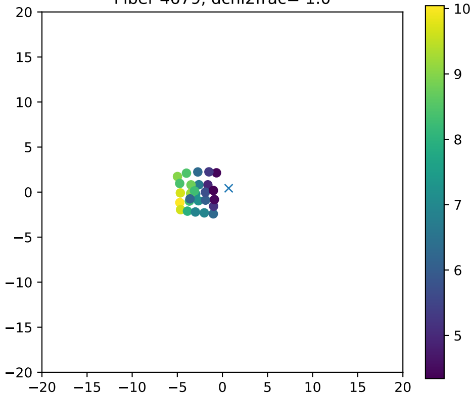
Fiber 4679, dchi2frac= 1.0
