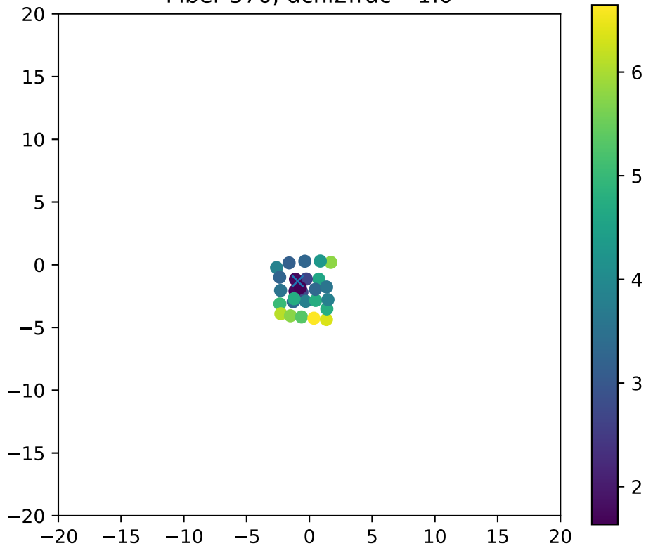
Fiber 570, dchi2frac= 1.0
