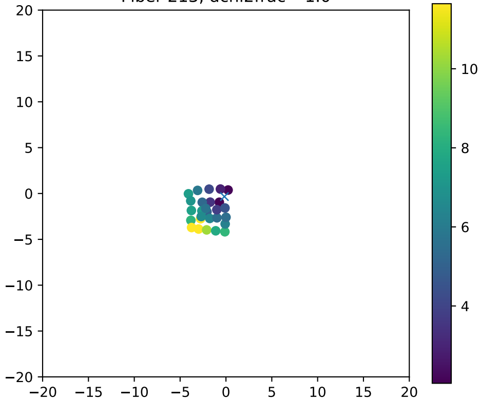
Fiber 213, dchi2frac= 1.0
