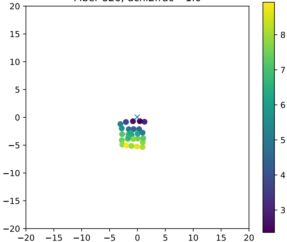
Fiber 826, dchi2frac= 1.0
