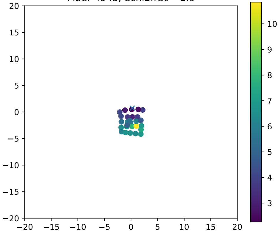
Fiber 4943, dchi2frac= 1.0
