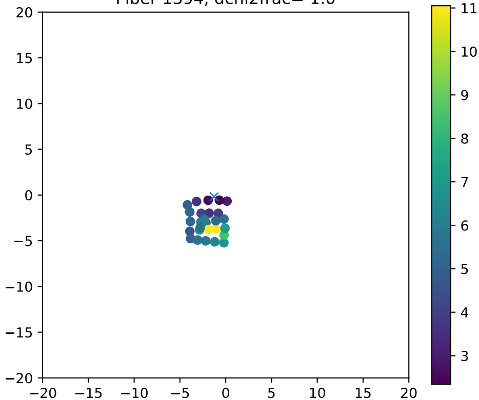
Fiber 1394, dchi2frac= 1.0
