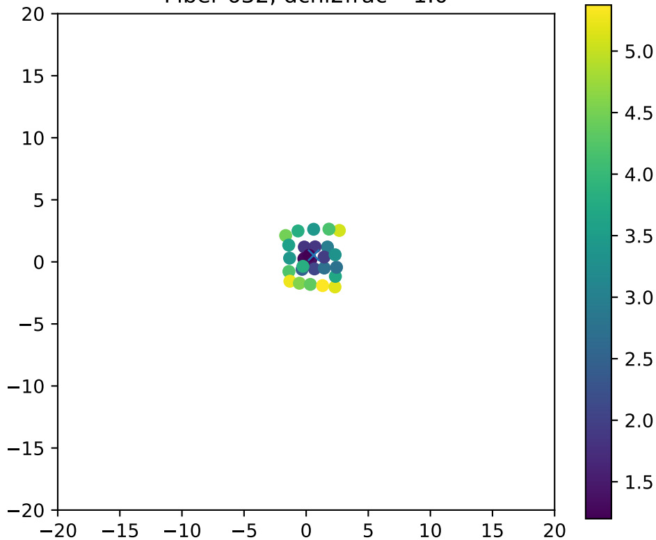
Fiber 632, dchi2frac= 1.0
