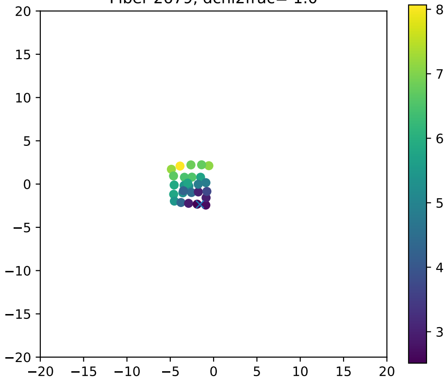
Fiber 2679, dchi2frac= 1.0
