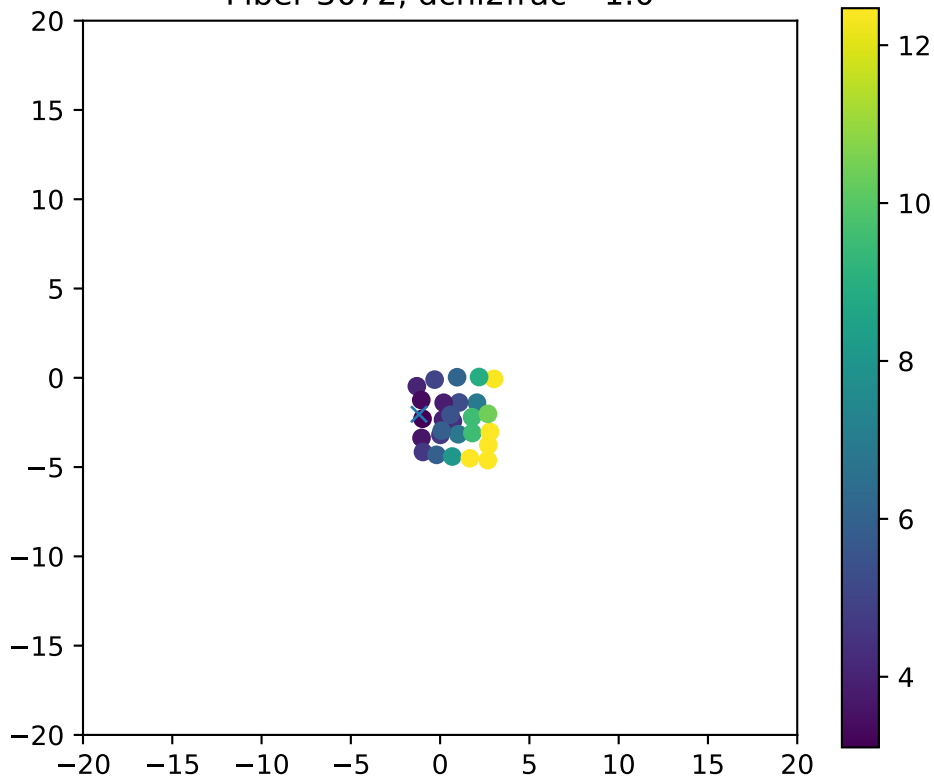
Fiber 3072, dchi2frac= 1.0
