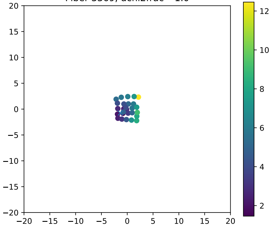
Fiber 3369, dchi2frac= 1.0
