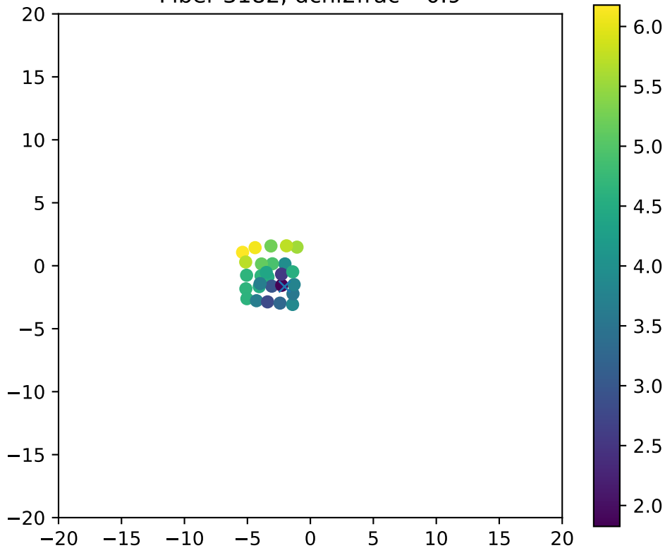
Fiber 3182, dchi2frac= 0.9
