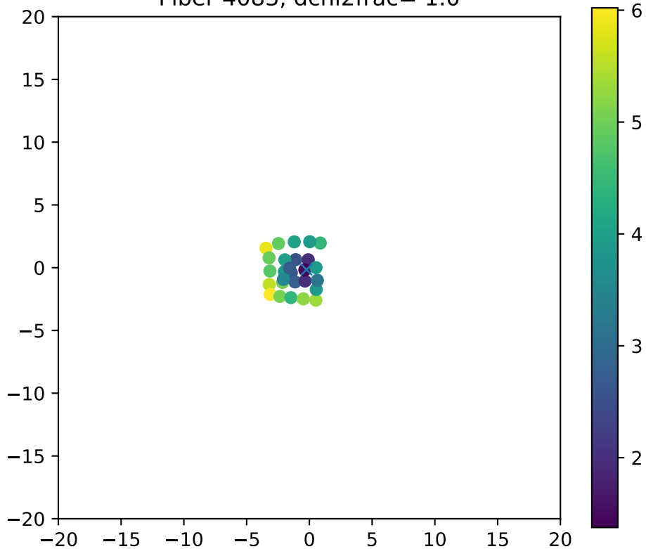
Fiber 4083, dchi2frac= 1.0
