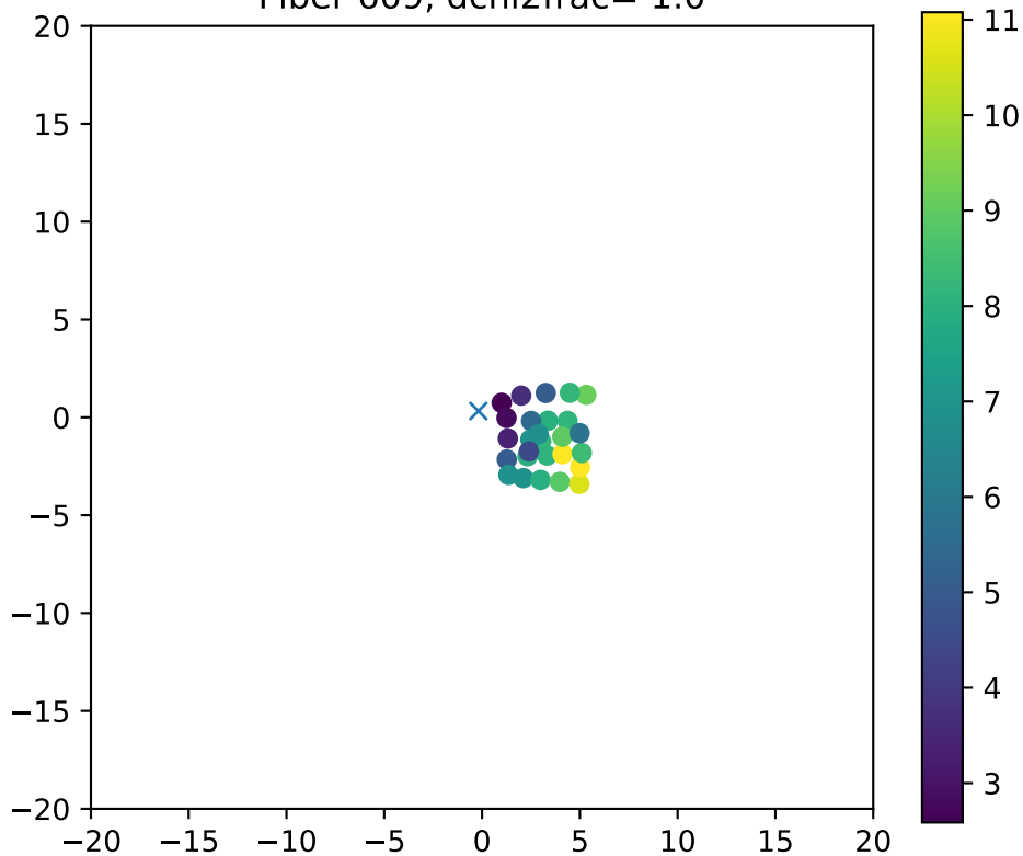
Fiber 609, dchi2frac= 1.0
