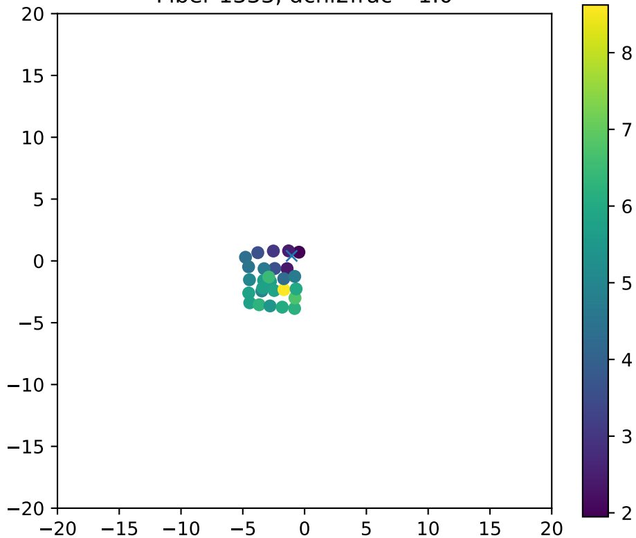
Fiber 1333, dchi2frac= 1.0
