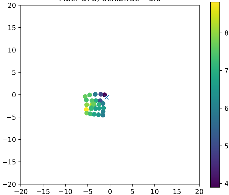
Fiber 578, dchi2frac= 1.0
