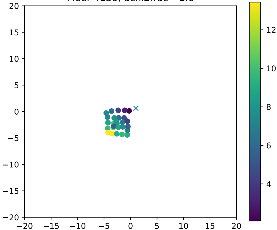
Fiber 4130, dchi2frac= 1.0
