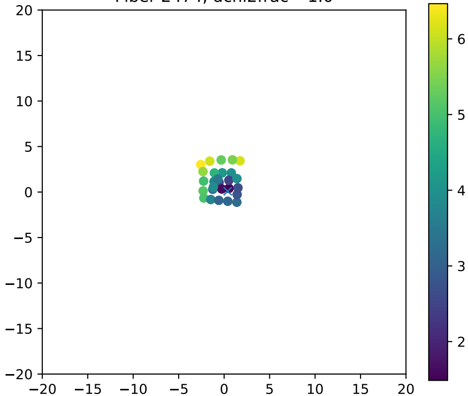
Fiber 2474, dchi2frac= 1.0
