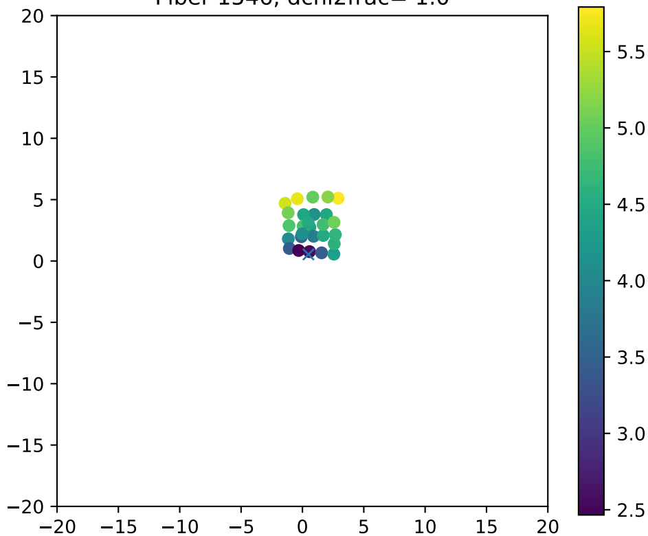
Fiber 1546, dchi2frac= 1.0
