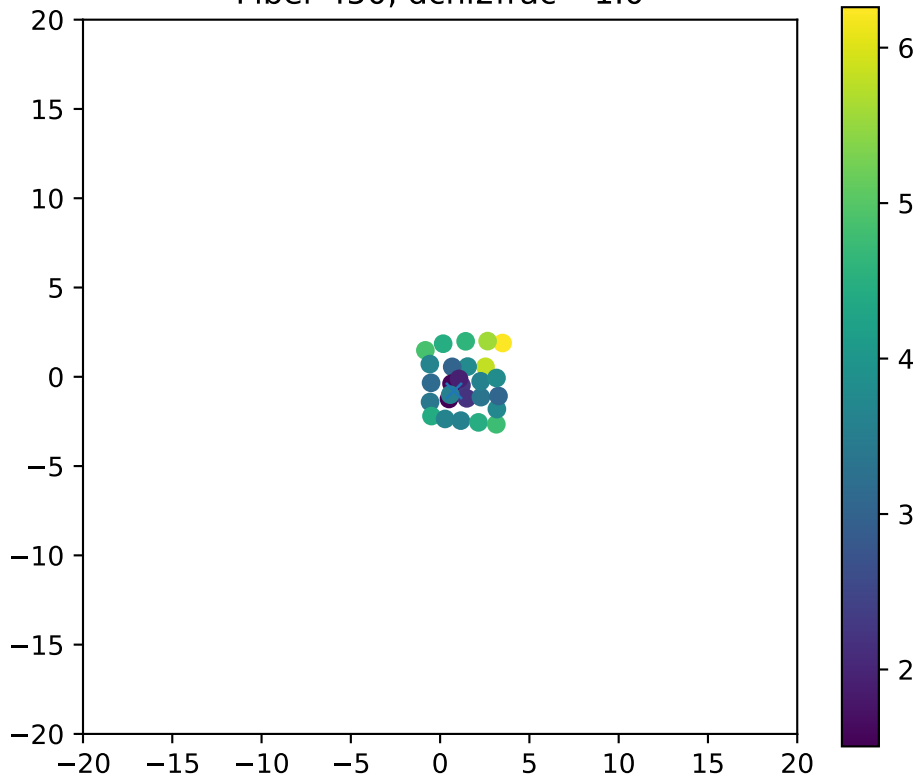
Fiber 450, dchi2frac= 1.0
