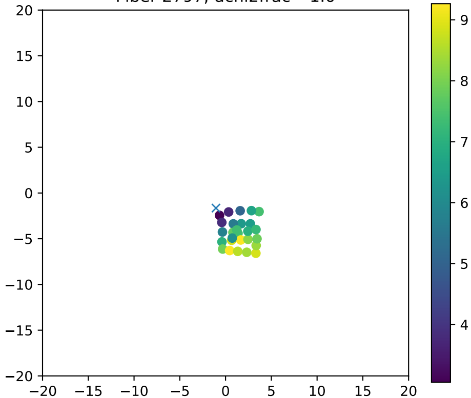
Fiber 2797, dchi2frac= 1.0
