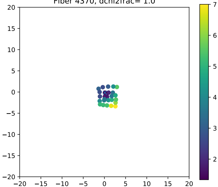
Fiber 4370, dchi2frac= 1.0
