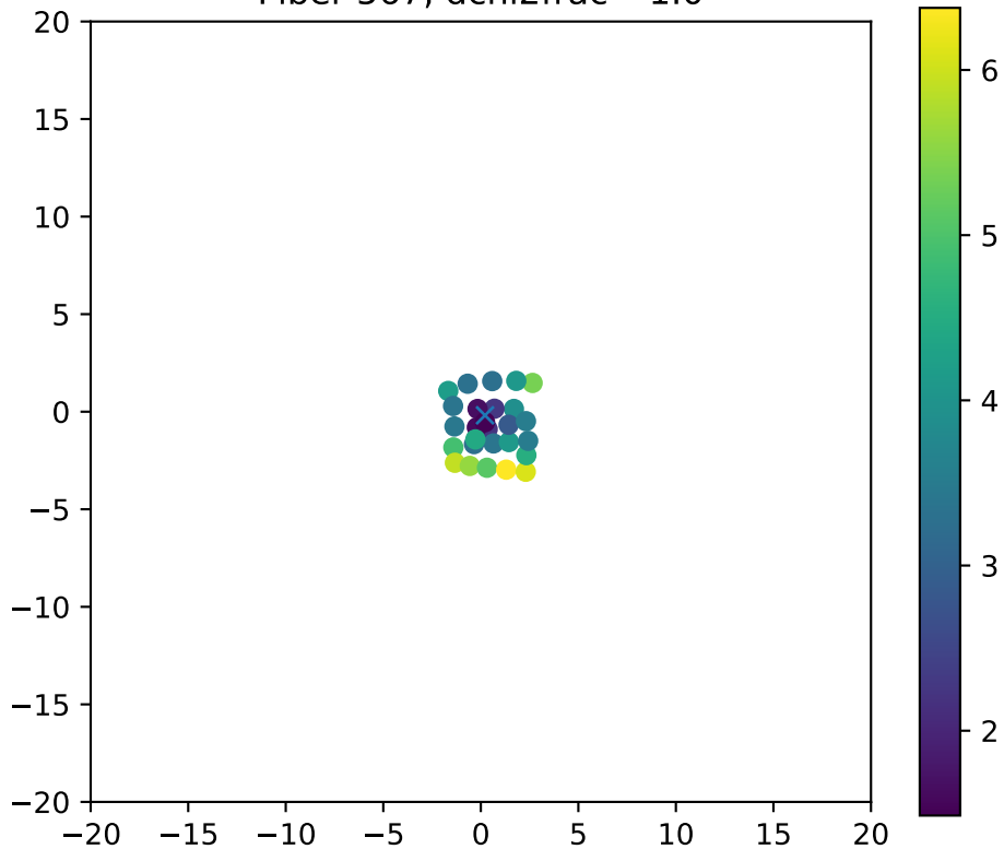
Fiber 567, dchi2frac= 1.0
