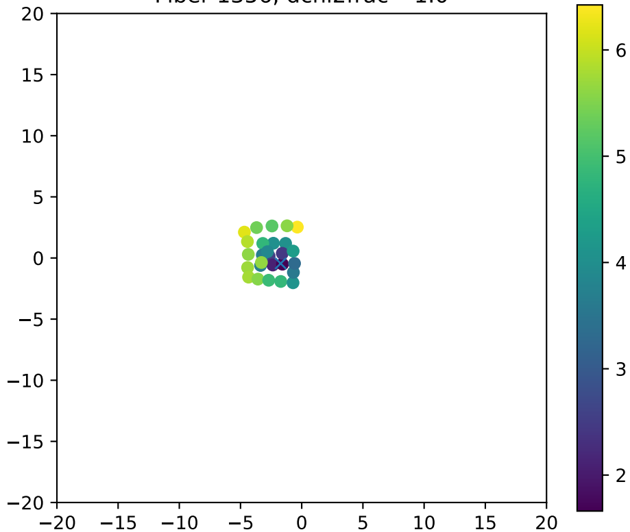
Fiber 1356, dchi2frac= 1.0
