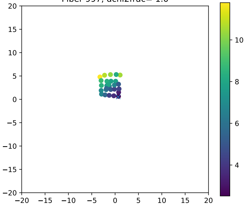
Fiber 997, dchi2frac= 1.0
