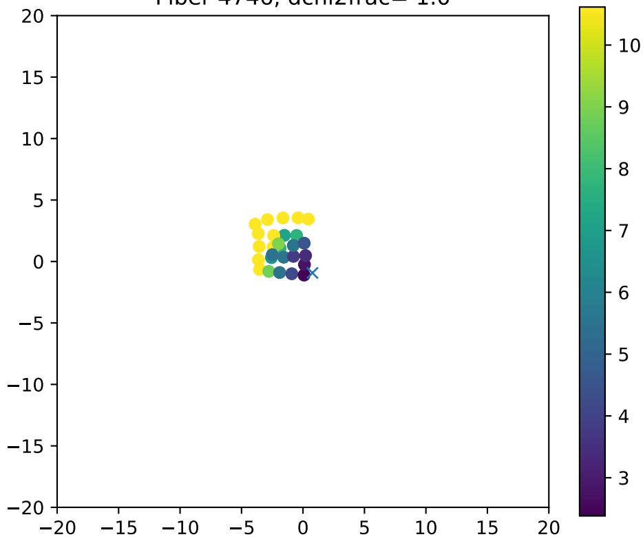
Fiber 4746, dchi2frac= 1.0
