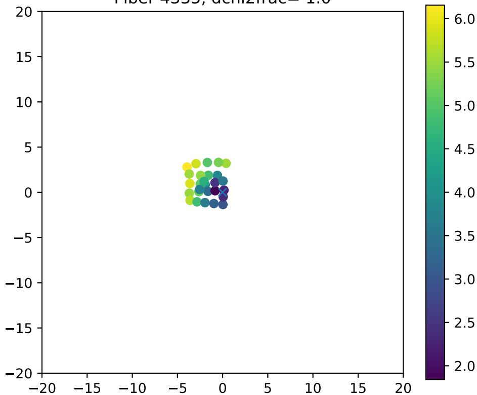
Fiber 4335, dchi2frac= 1.0
