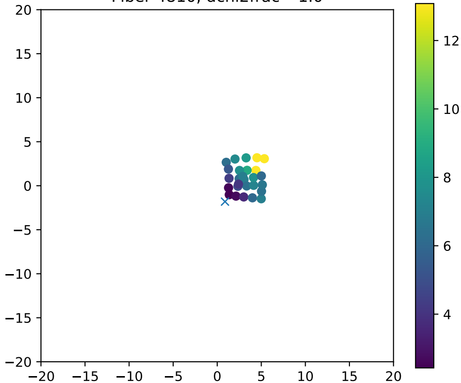
Fiber 4810, dchi2frac= 1.0
