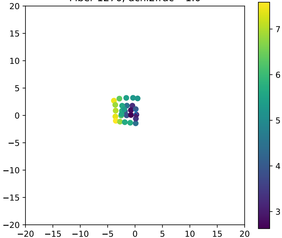
Fiber 1276, dchi2frac= 1.0
