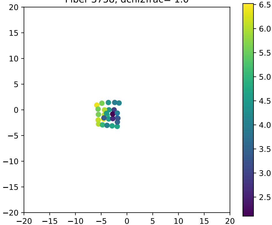
Fiber 3758, dchi2frac= 1.0
