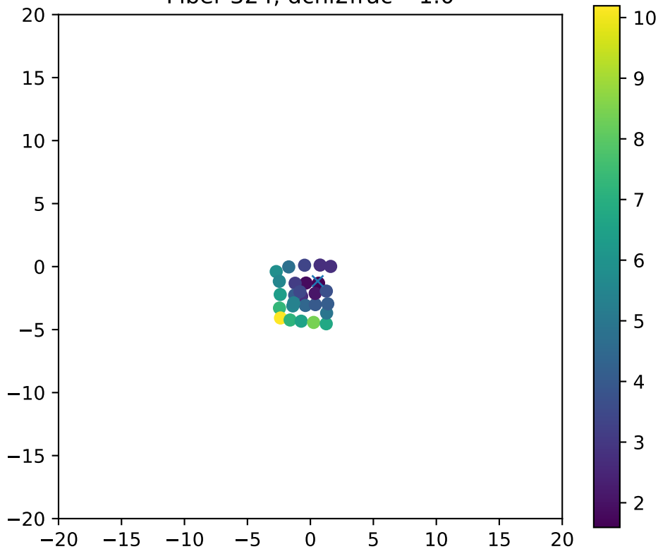
Fiber 324, dchi2frac= 1.0
