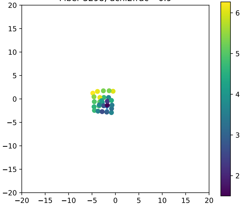
Fiber 3298, dchi2frac= 0.9
