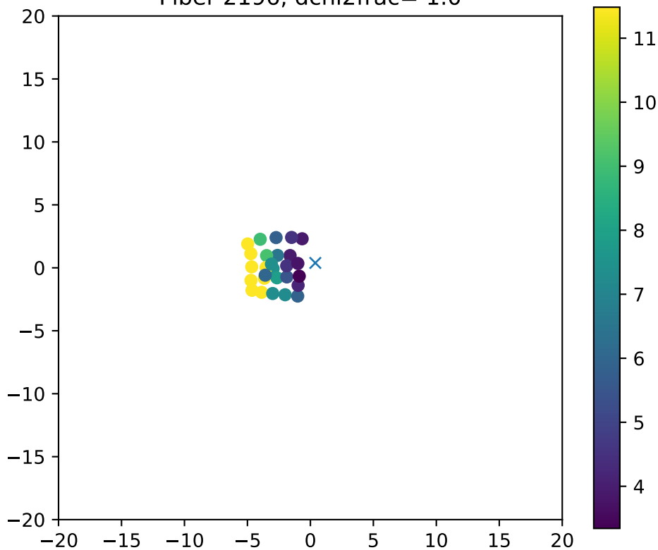
Fiber 2196, dchi2frac= 1.0
