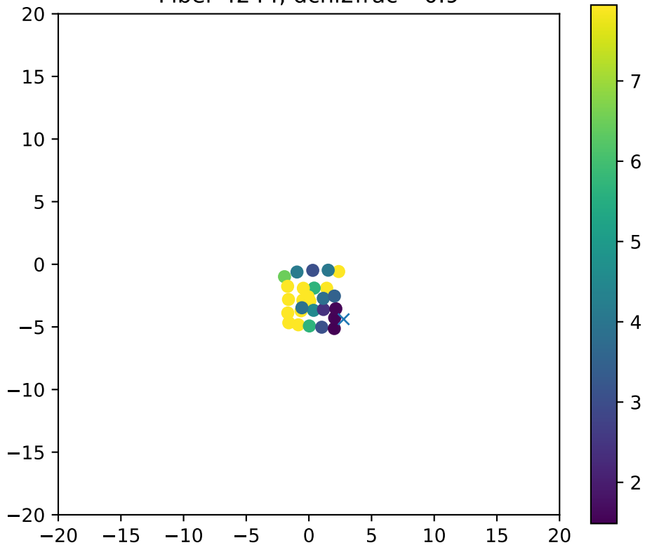
Fiber 4244, dchi2frac= 0.9
