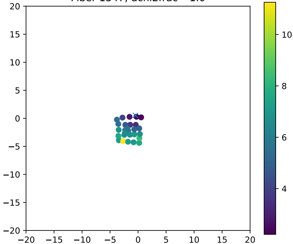
Fiber 1347, dchi2frac= 1.0
