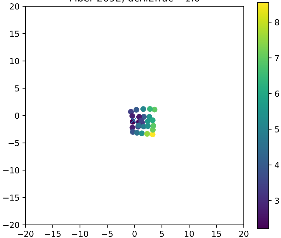
Fiber 2692, dchi2frac= 1.0
