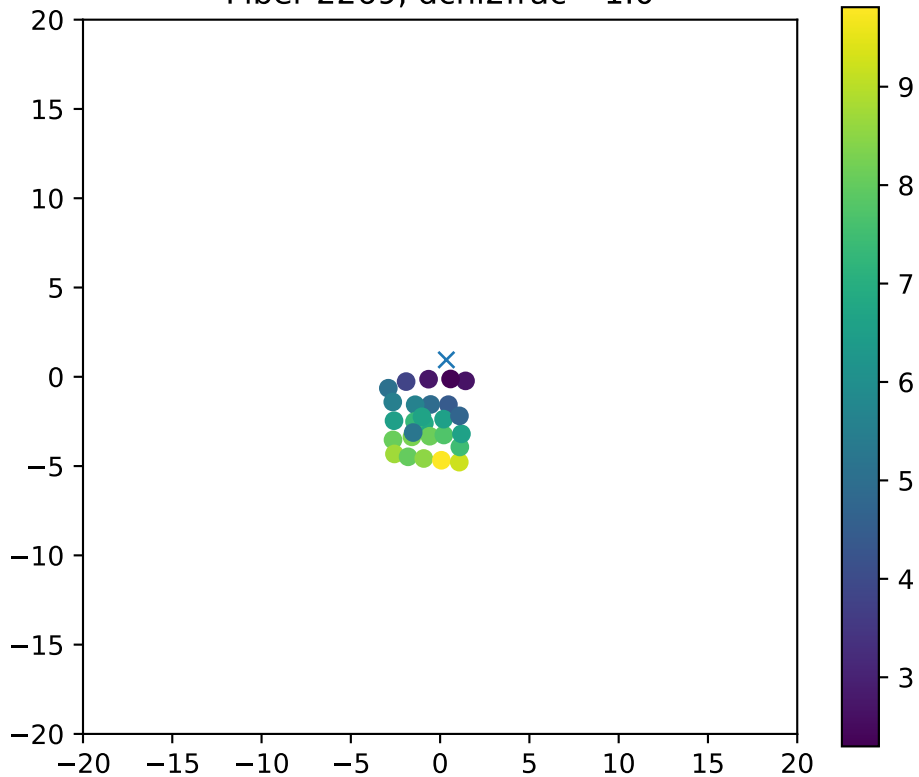
Fiber 2269, dchi2frac= 1.0
