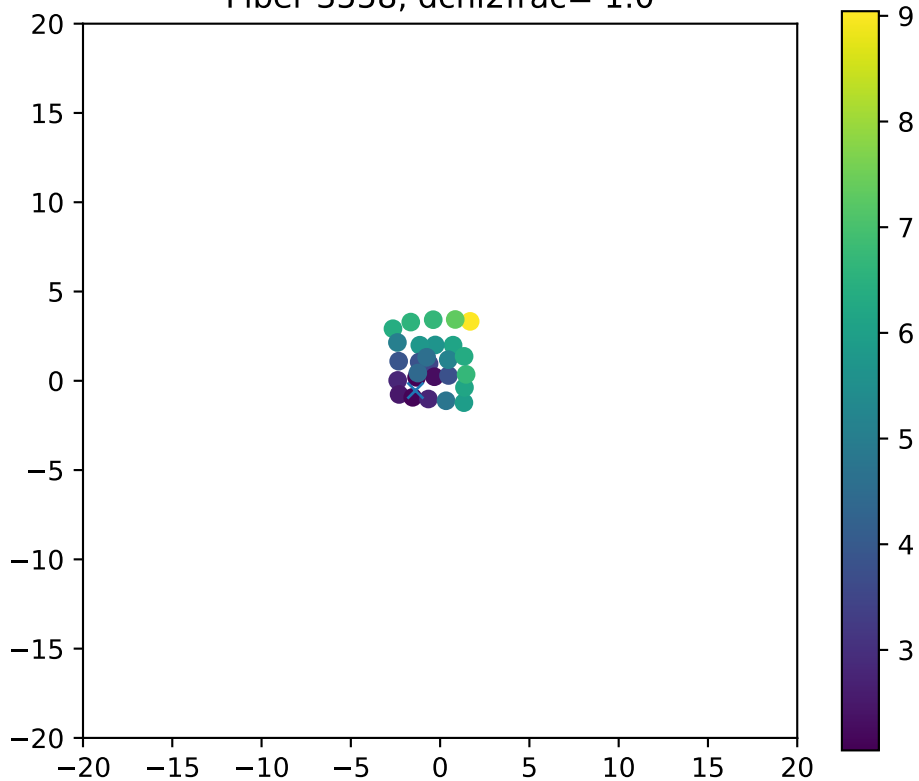
Fiber 3558, dchi2frac= 1.0
