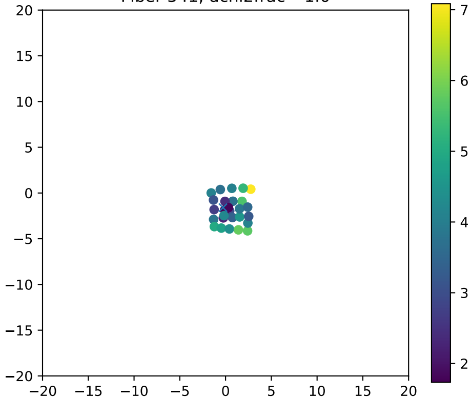
Fiber 541, dchi2frac= 1.0
