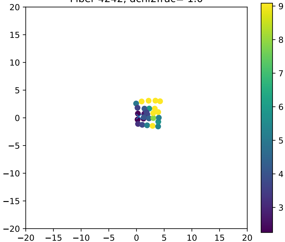
Fiber 4242, dchi2frac= 1.0
