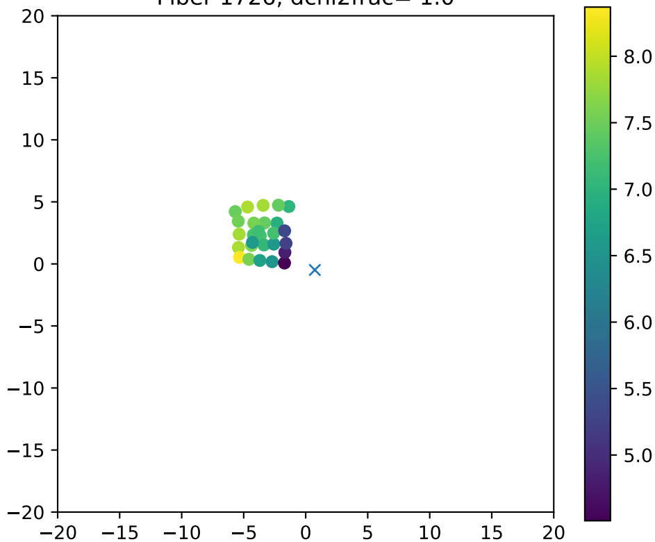
Fiber 1726, dchi2frac= 1.0
