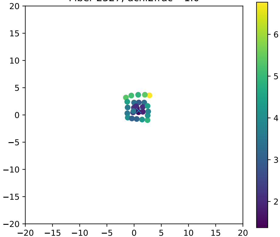
Fiber 2327, dchi2frac= 1.0
