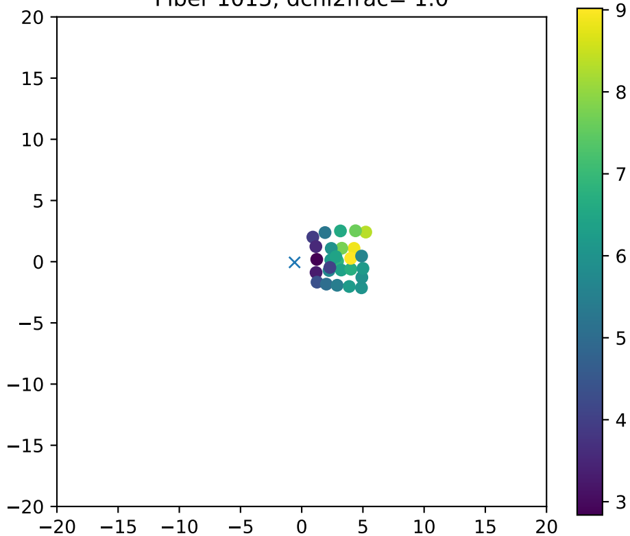
Fiber 1015, dchi2frac= 1.0
