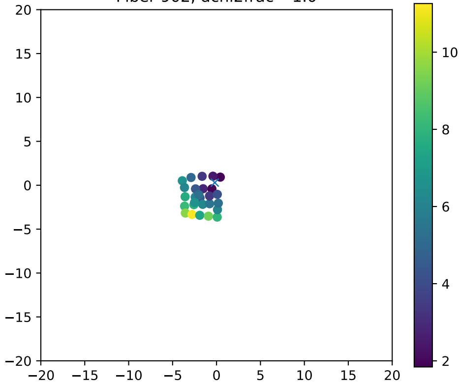
Fiber 902, dchi2frac= 1.0
