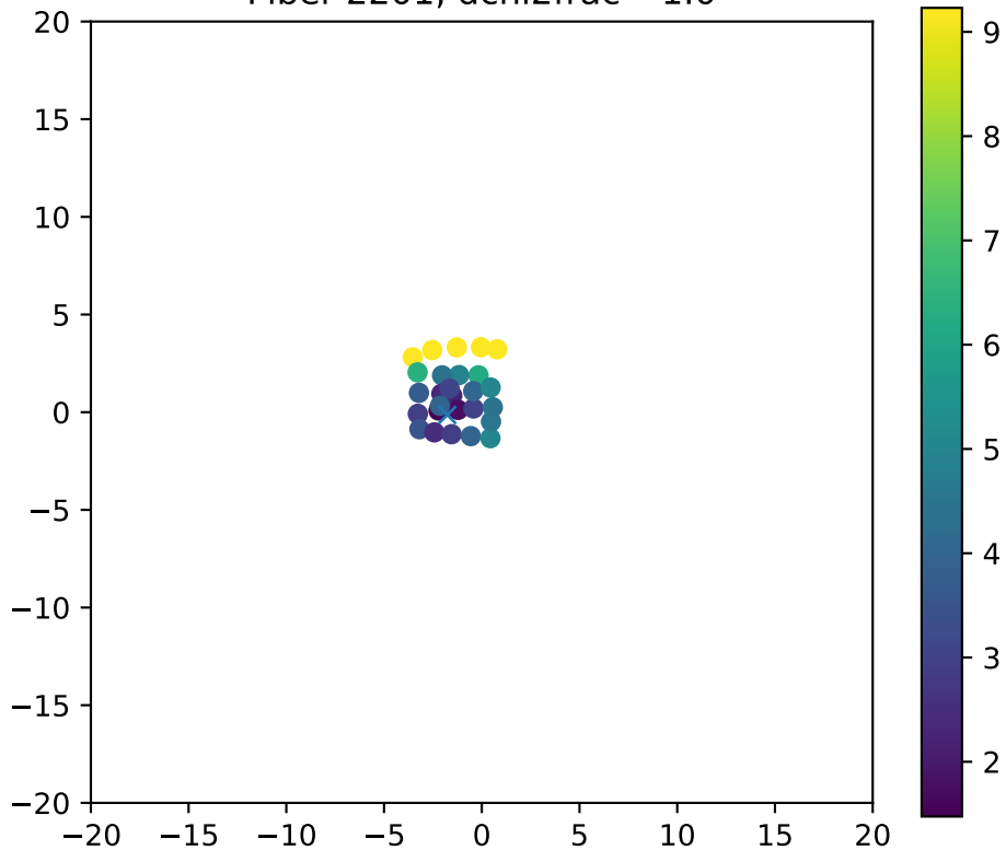
Fiber 2201, dchi2frac= 1.0
