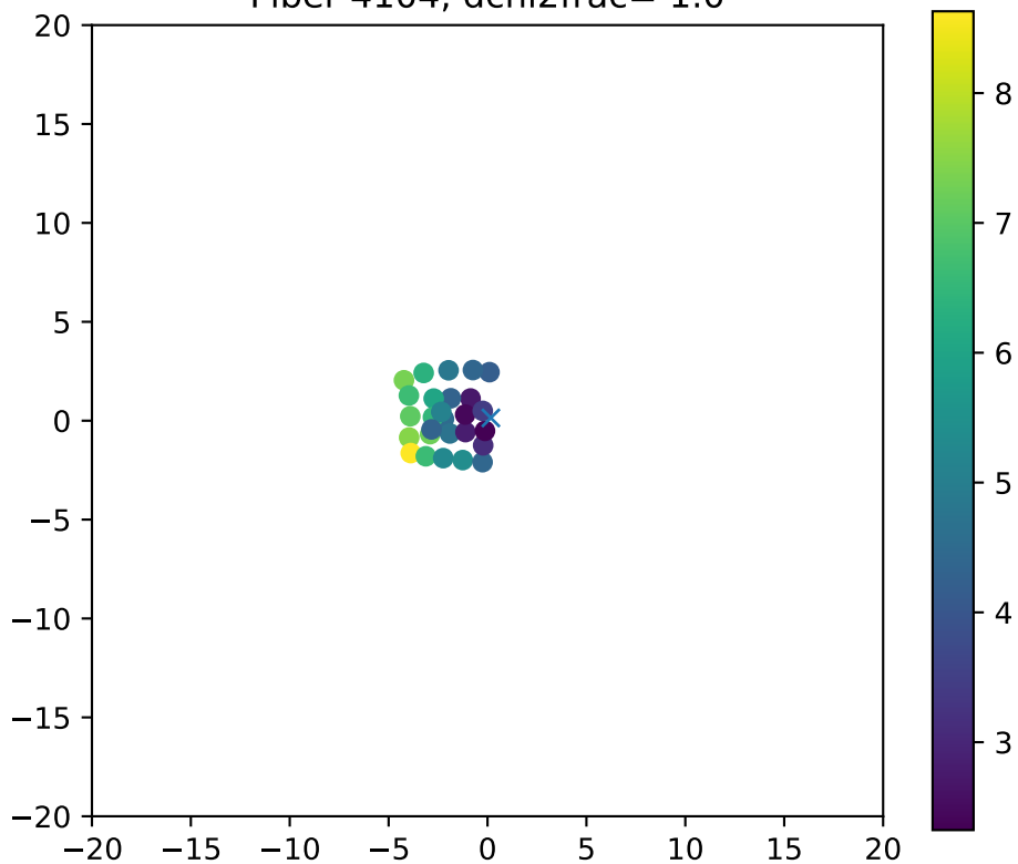
Fiber 4104, dchi2frac= 1.0
