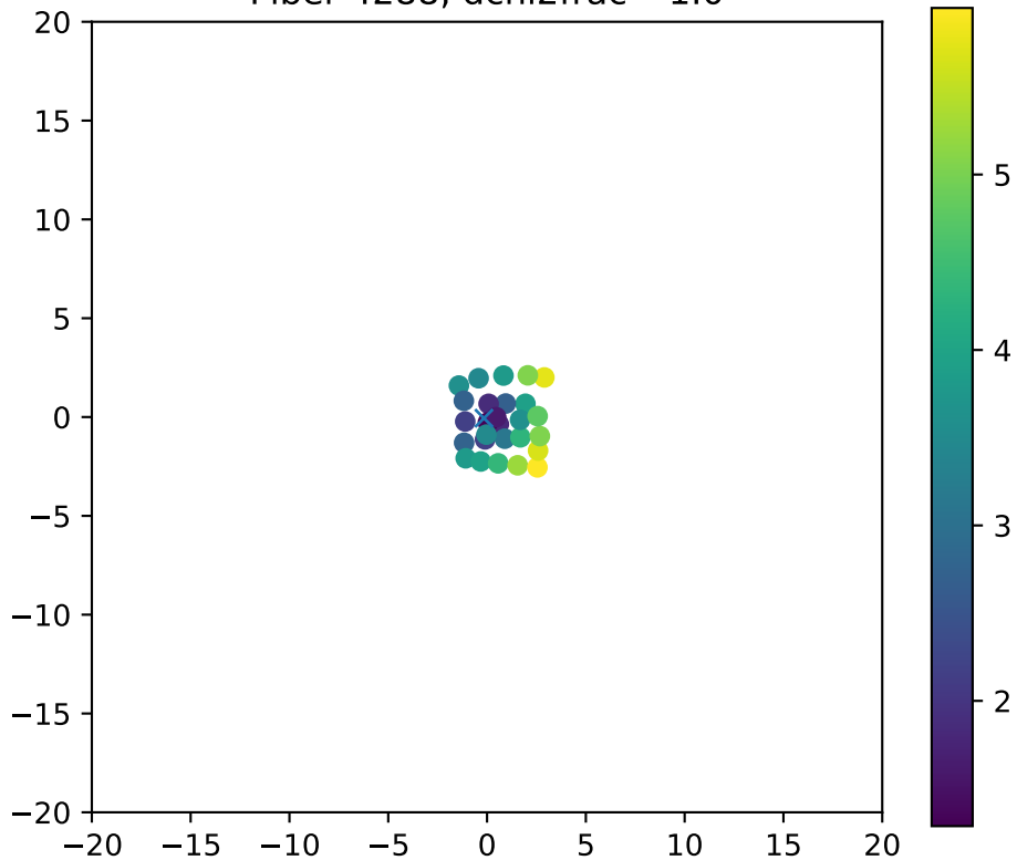
Fiber 4288, dchi2frac= 1.0
