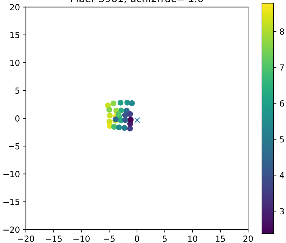
Fiber 3961, dchi2frac= 1.0
