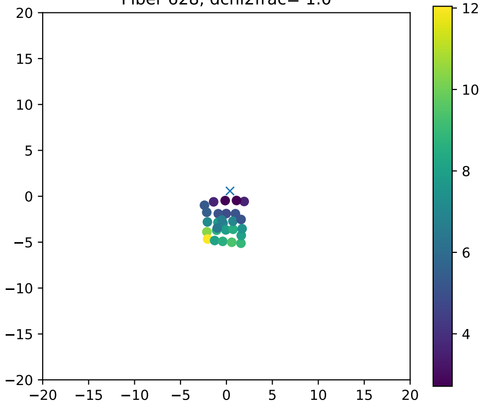
Fiber 628, dchi2frac= 1.0
