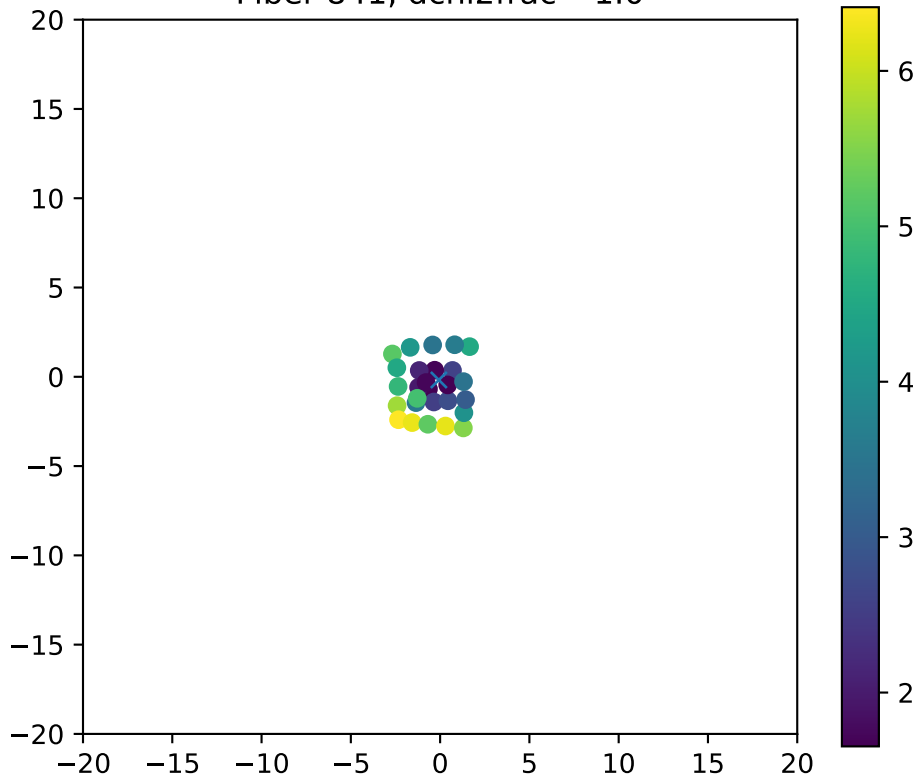
Fiber 841, dchi2frac= 1.0
