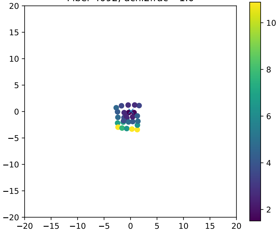
Fiber 4092, dchi2frac= 1.0
