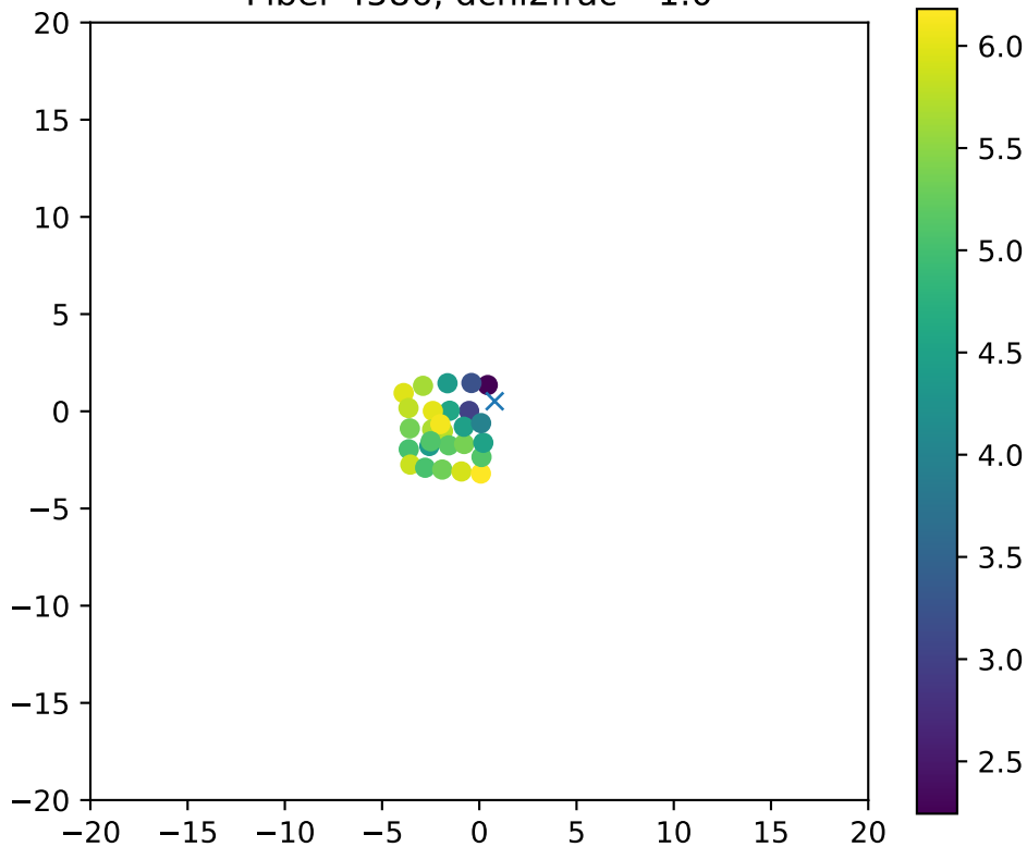
Fiber 4586, dchi2frac= 1.0
