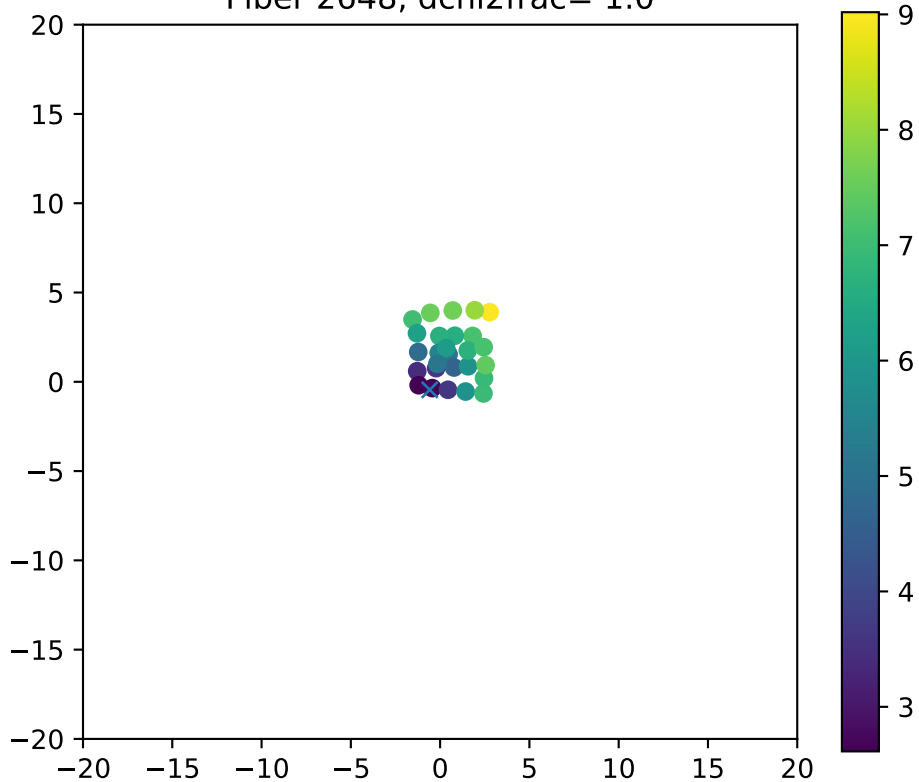
Fiber 2648, dchi2frac= 1.0
