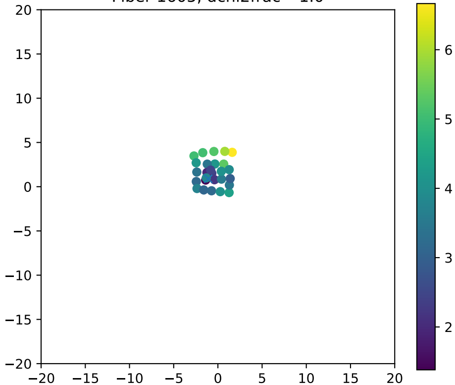
Fiber 1605, dchi2frac= 1.0
