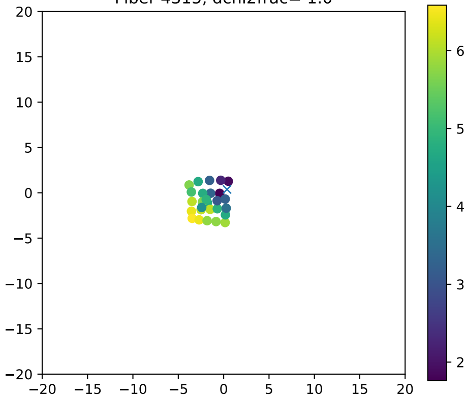
Fiber 4315, dchi2frac= 1.0
