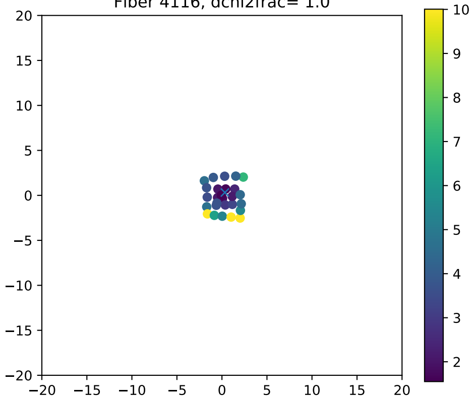
Fiber 4116, dchi2frac= 1.0
