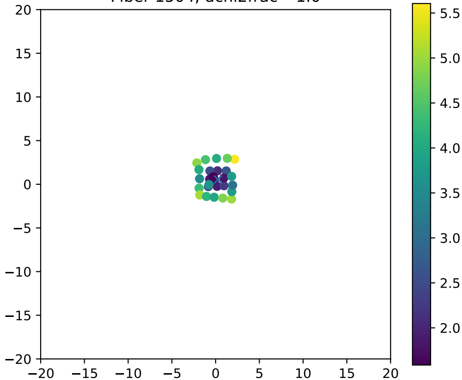
Fiber 1504, dchi2frac= 1.0
