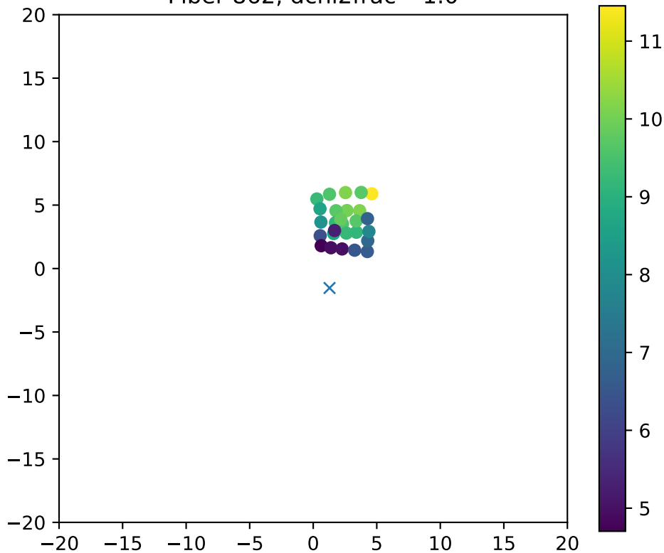
Fiber 862, dchi2frac= 1.0
