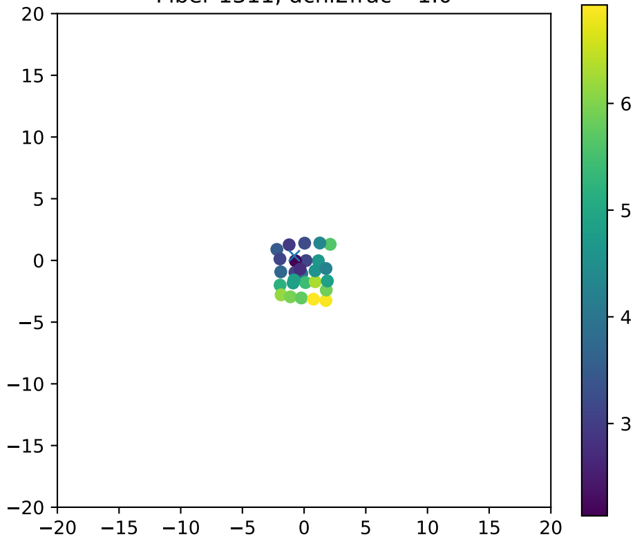
Fiber 1311, dchi2frac= 1.0
