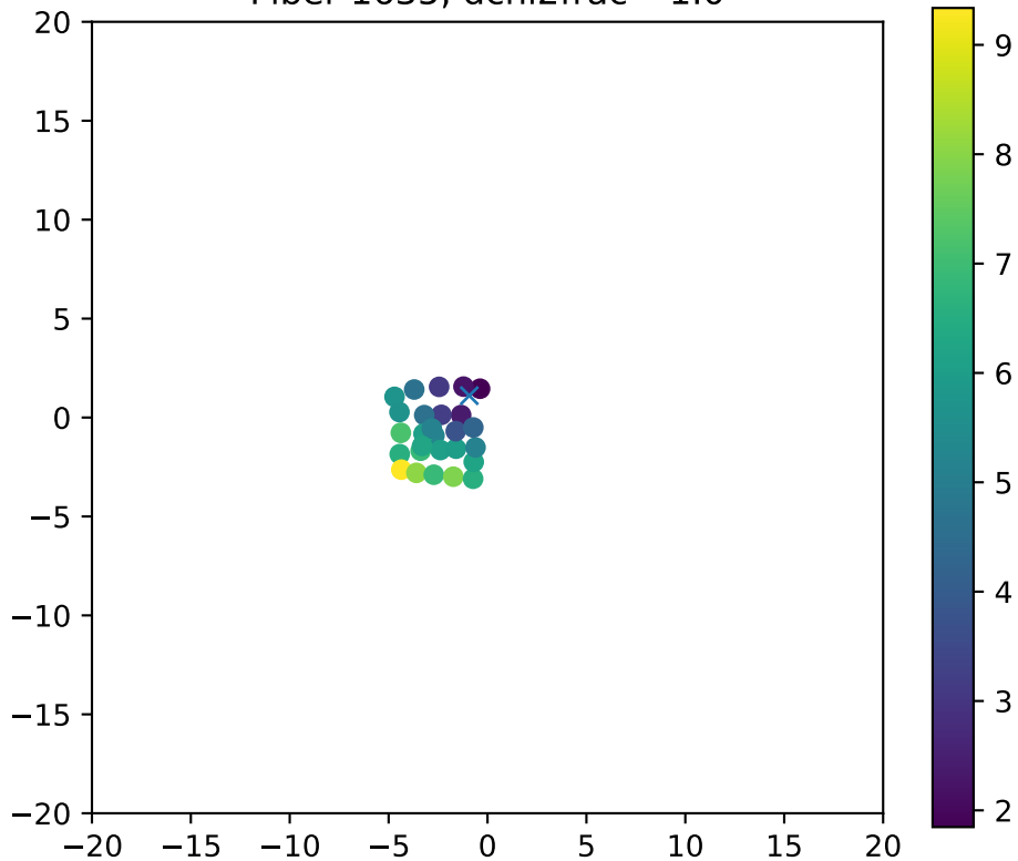
Fiber 1635, dchi2frac= 1.0
