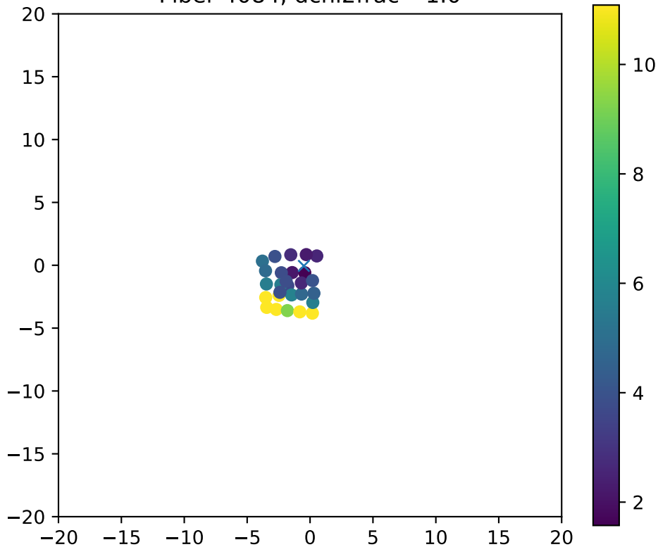
Fiber 4084, dchi2frac= 1.0
