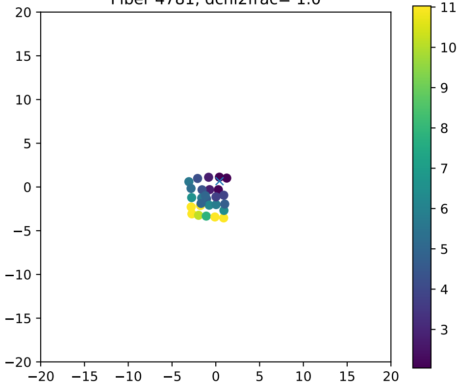
Fiber 4781, dchi2frac= 1.0
