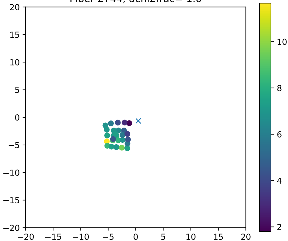
Fiber 2744, dchi2frac= 1.0
