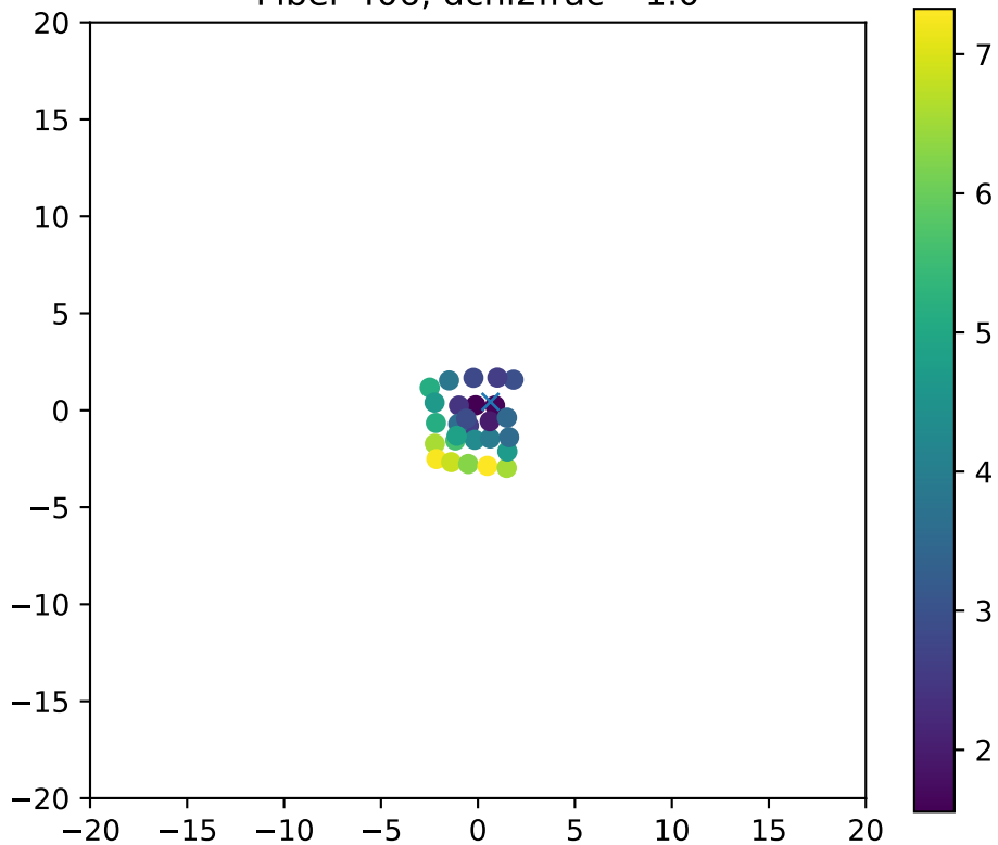
Fiber 406, dchi2frac= 1.0
