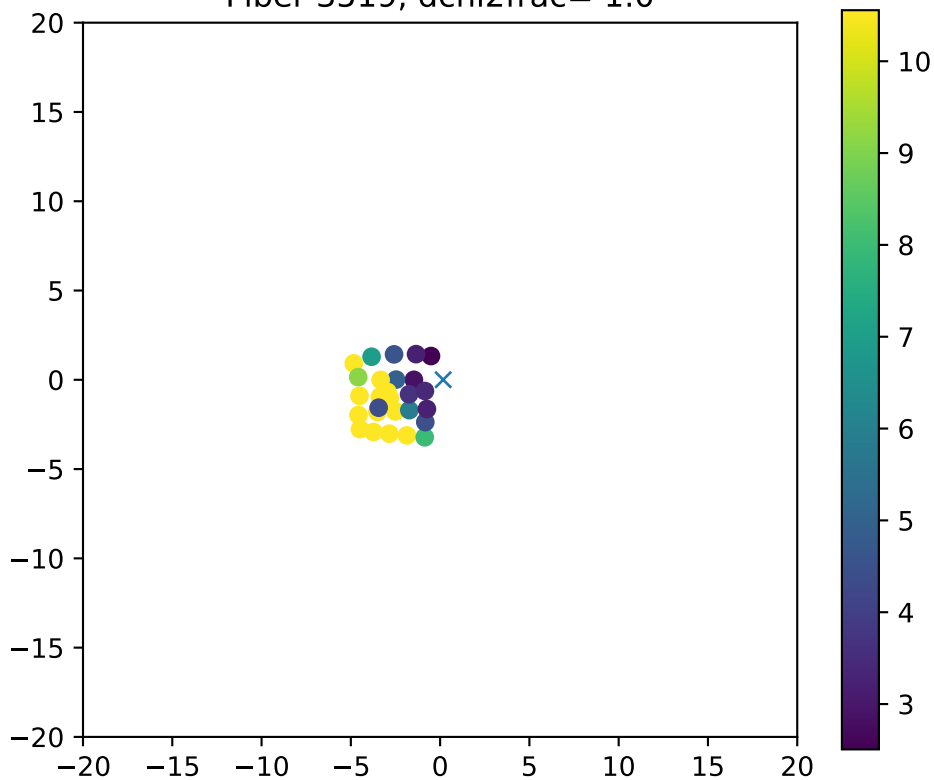
Fiber 3519, dchi2frac= 1.0
