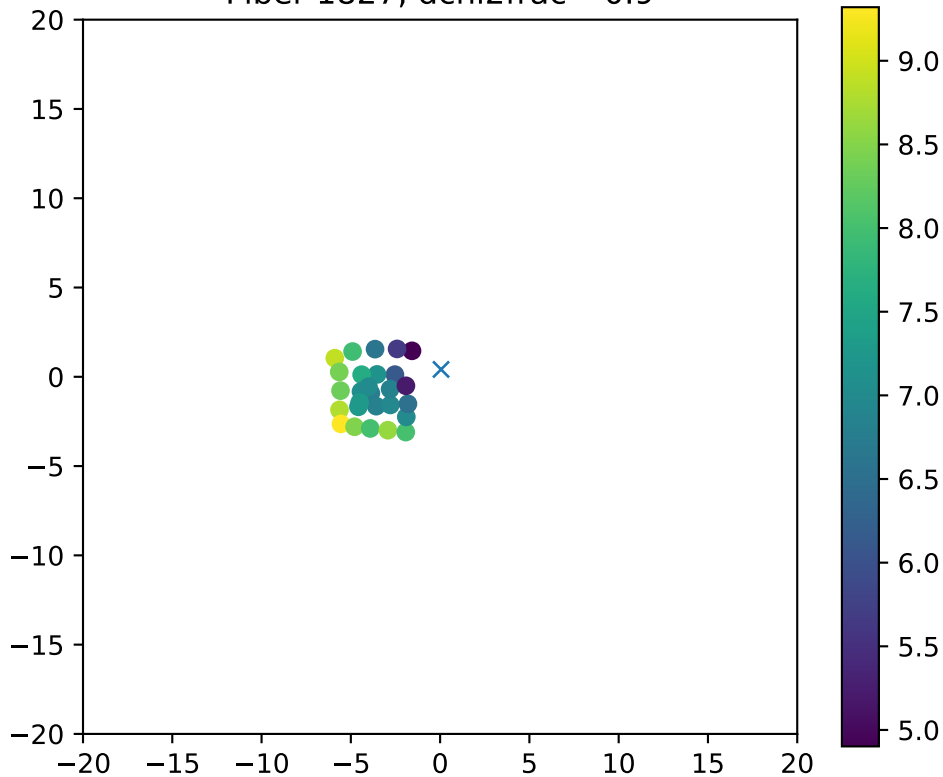
Fiber 1827, dchi2frac= 0.9
