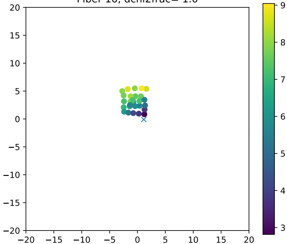
Fiber 10, dchi2frac= 1.0
