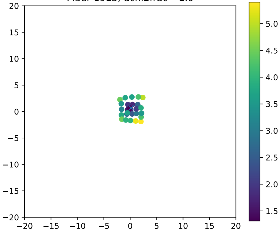
Fiber 1913, dchi2frac= 1.0
