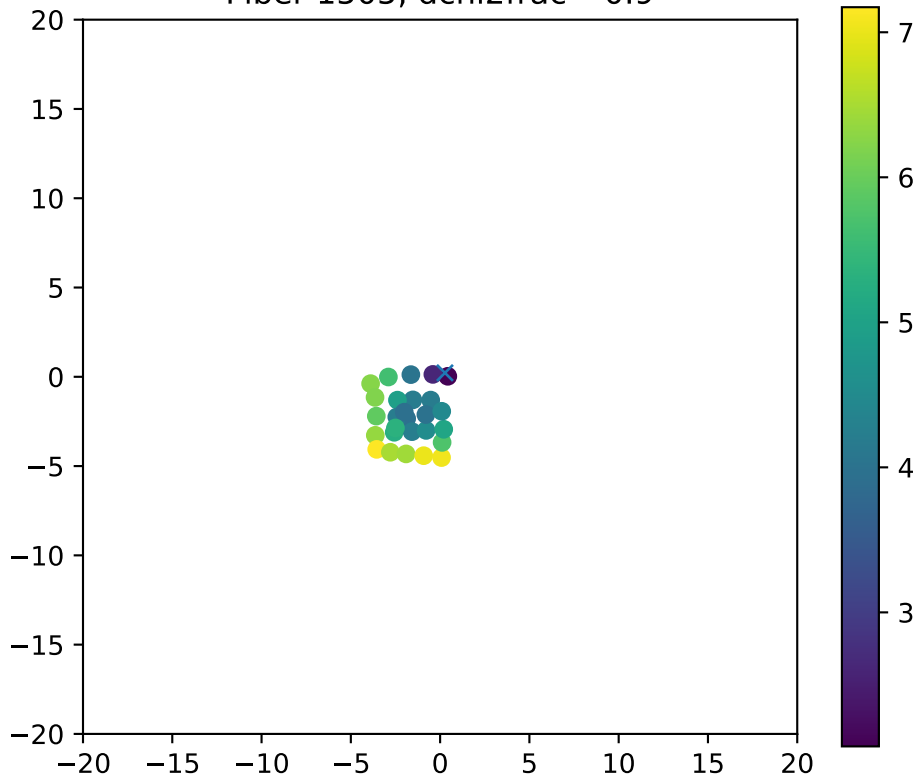
Fiber 1505, dchi2frac= 0.9
