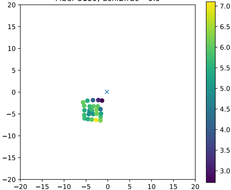
Fiber 3139, dchi2frac= 0.9
