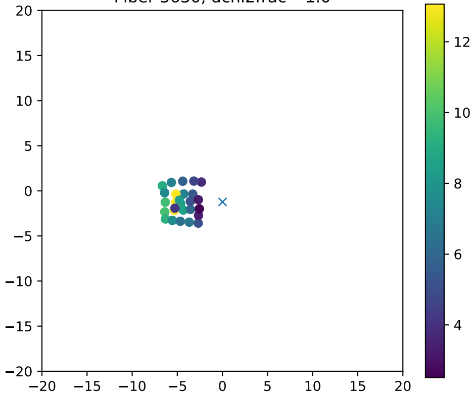
Fiber 3630, dchi2frac= 1.0
