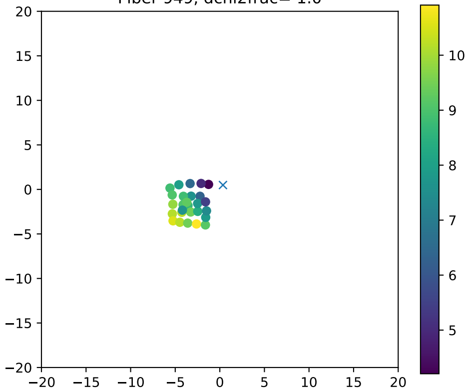
Fiber 949, dchi2frac= 1.0
