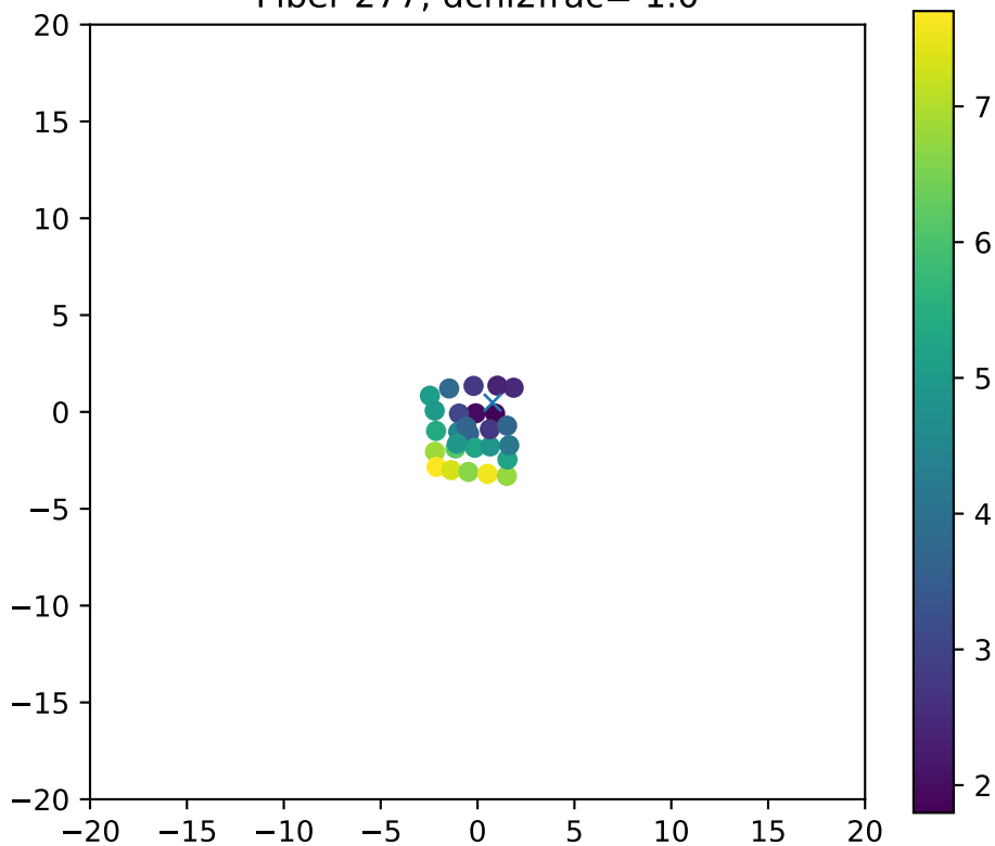
Fiber 277, dchi2frac= 1.0
