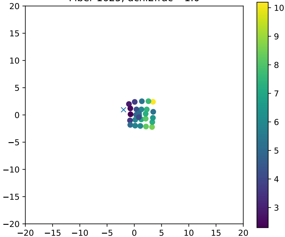
Fiber 1625, dchi2frac= 1.0
