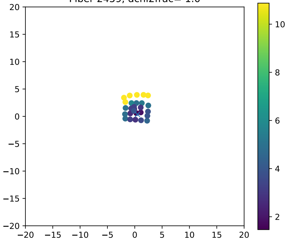
Fiber 2459, dchi2frac= 1.0
