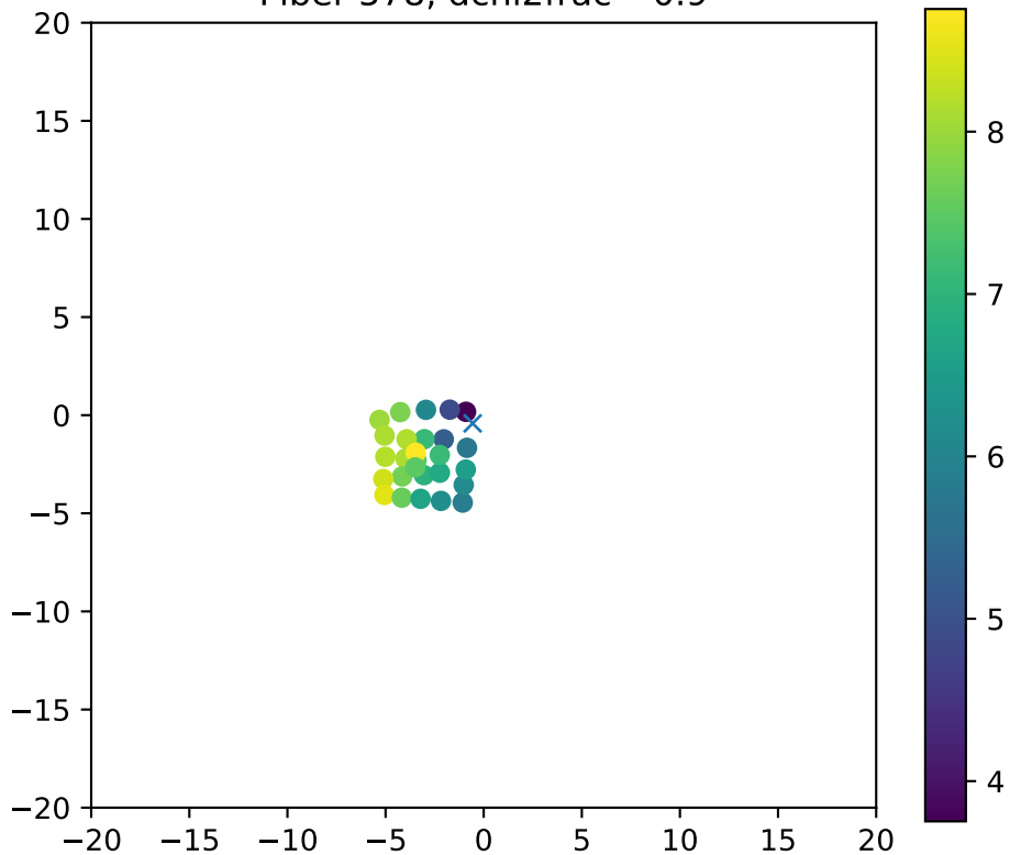
Fiber 578, dchi2frac= 0.9
