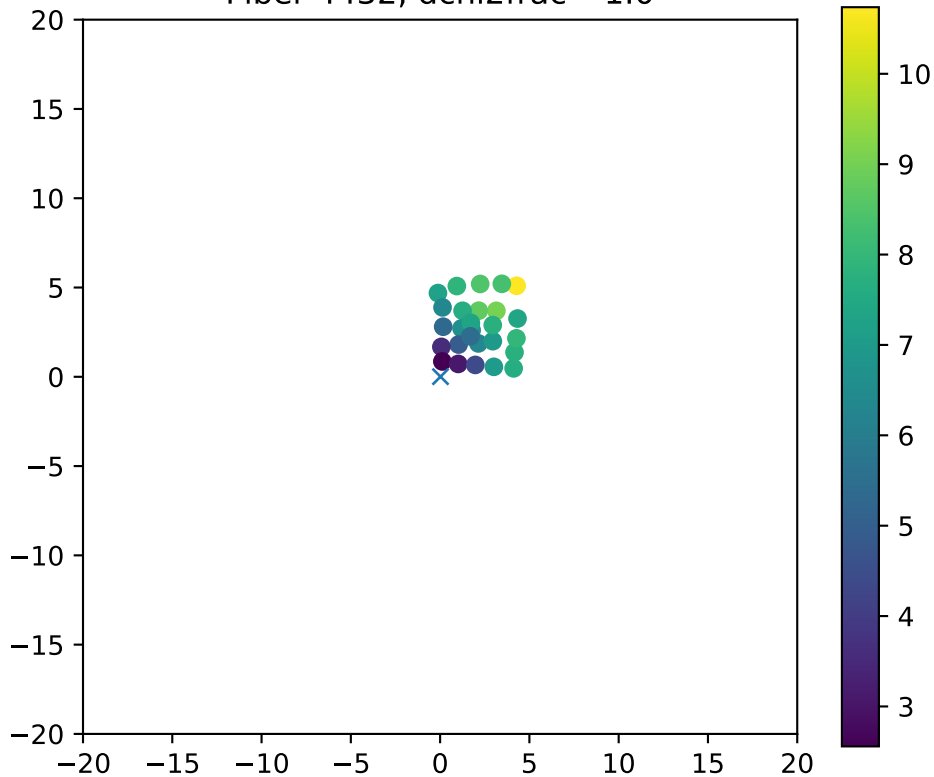
Fiber 4432, dchi2frac= 1.0
