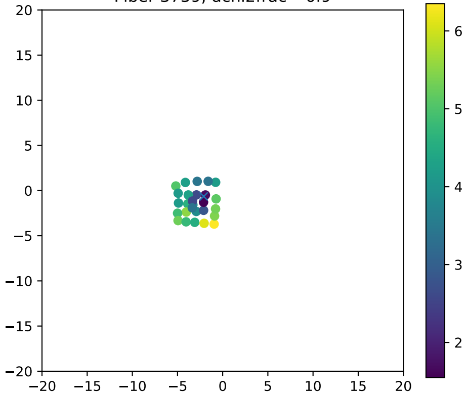
Fiber 3759, dchi2frac= 0.9
