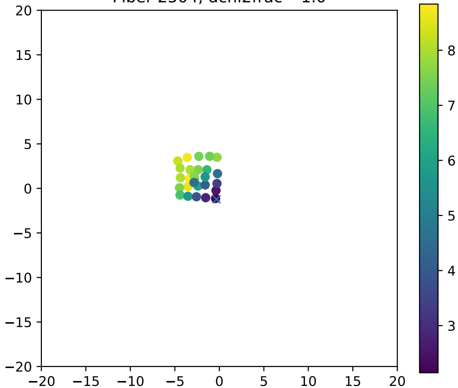
Fiber 2504, dchi2frac= 1.0
