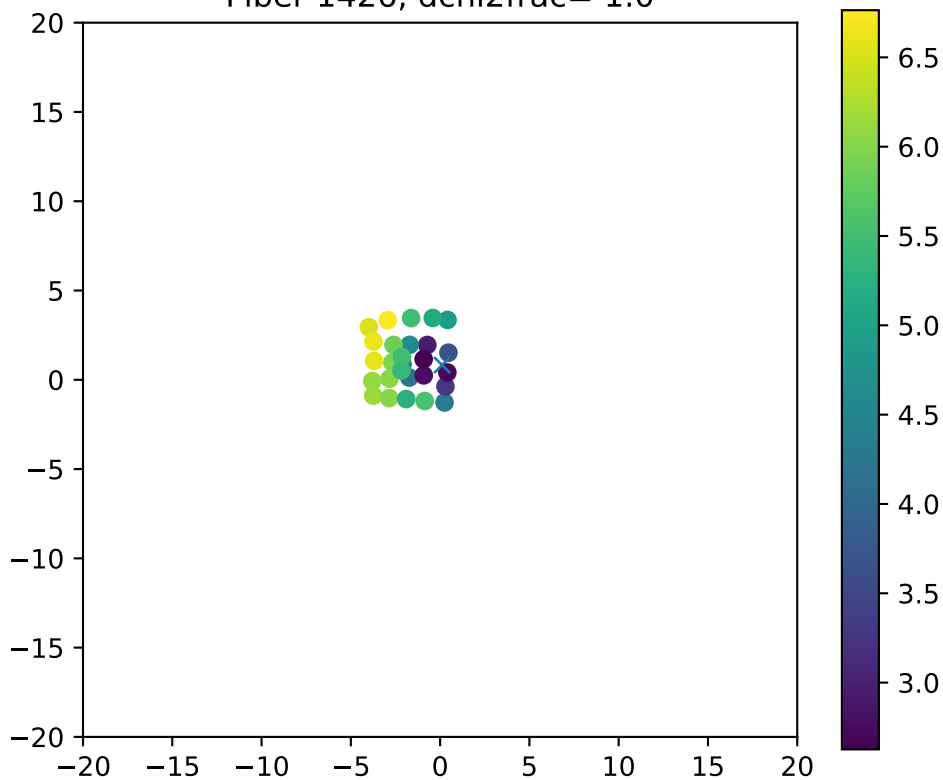
Fiber 1426, dchi2frac= 1.0
