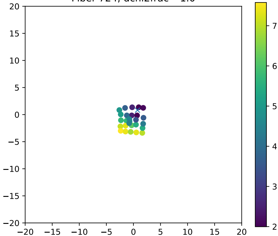
Fiber 724, dchi2frac= 1.0
