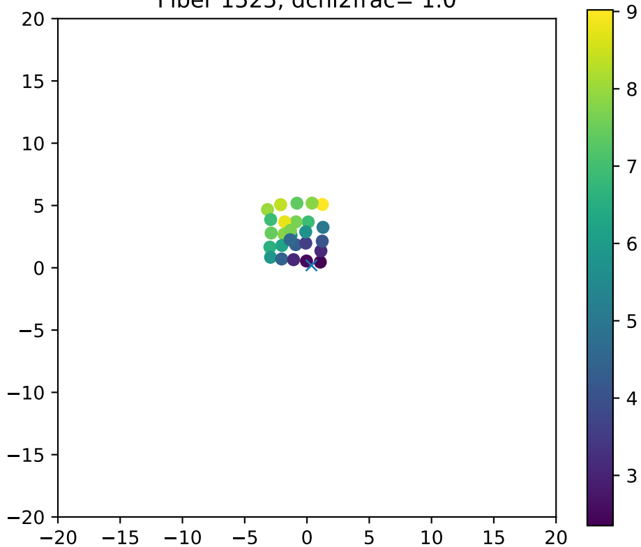
Fiber 1525, dchi2frac= 1.0
