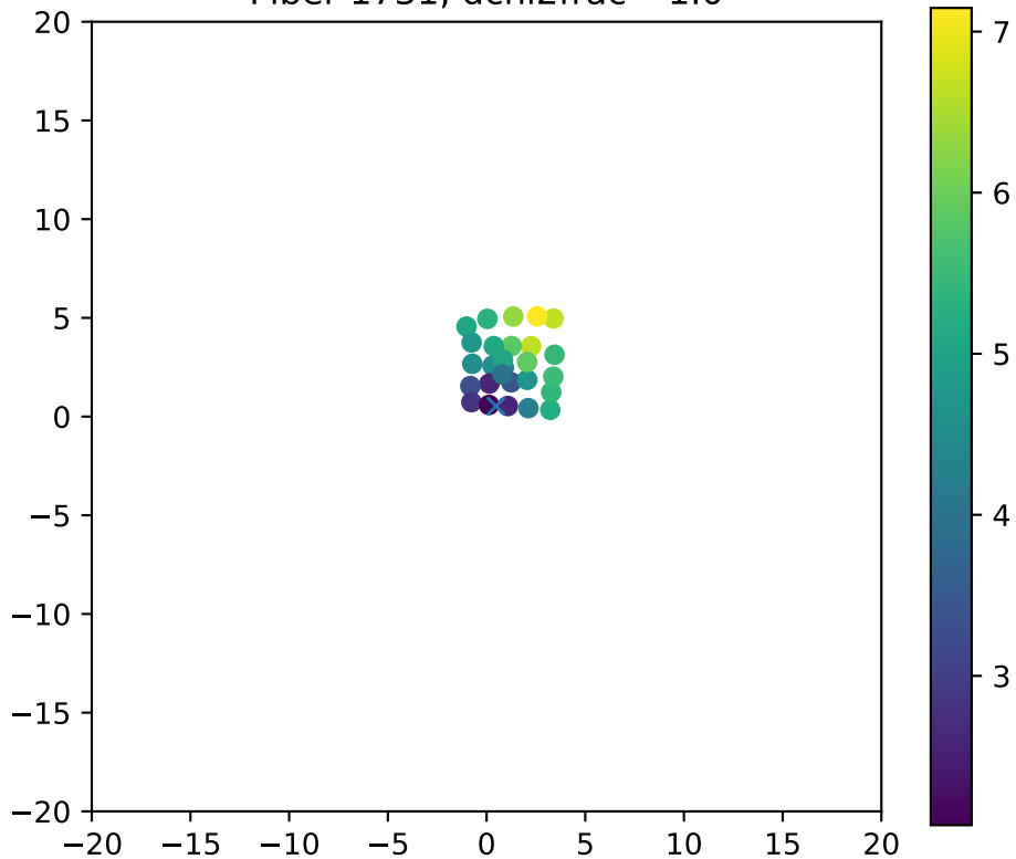
Fiber 1731, dchi2frac= 1.0
