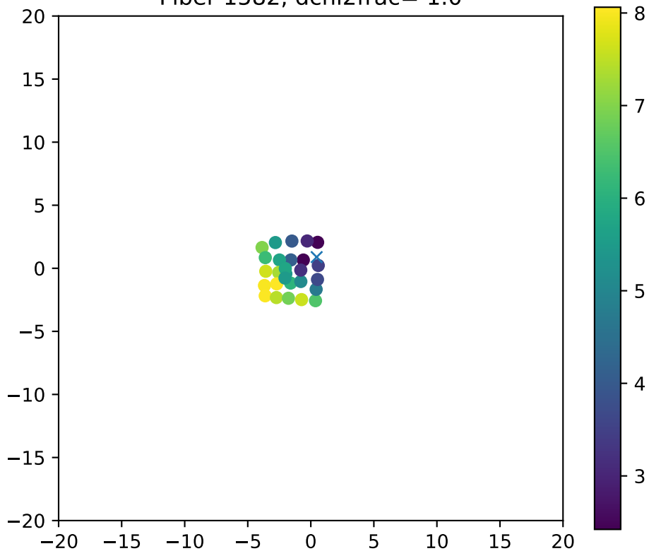
Fiber 1582, dchi2frac= 1.0
