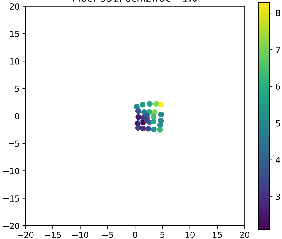
Fiber 331, dchi2frac= 1.0
