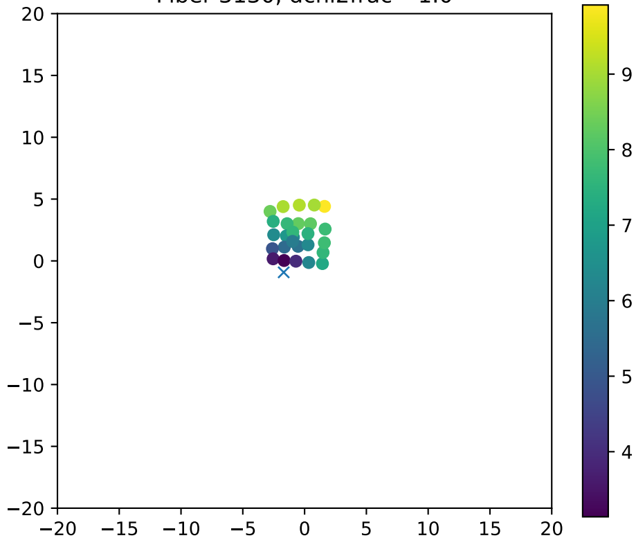
Fiber 3130, dchi2frac= 1.0
