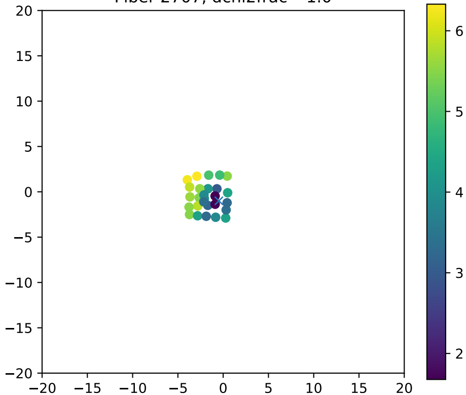
Fiber 2707, dchi2frac= 1.0
