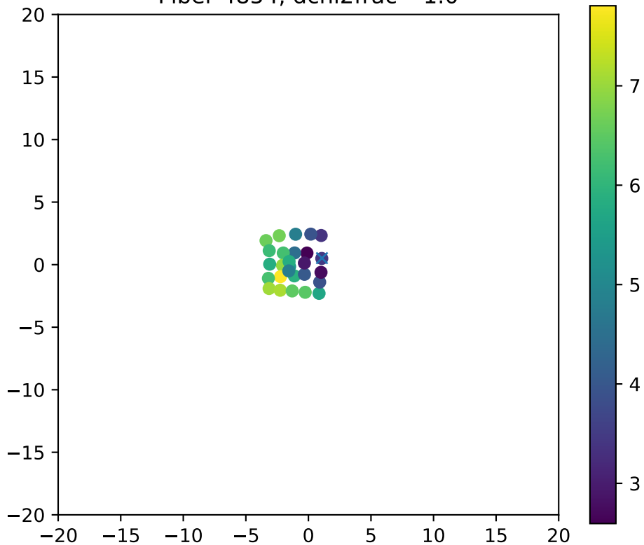
Fiber 4854, dchi2frac= 1.0
