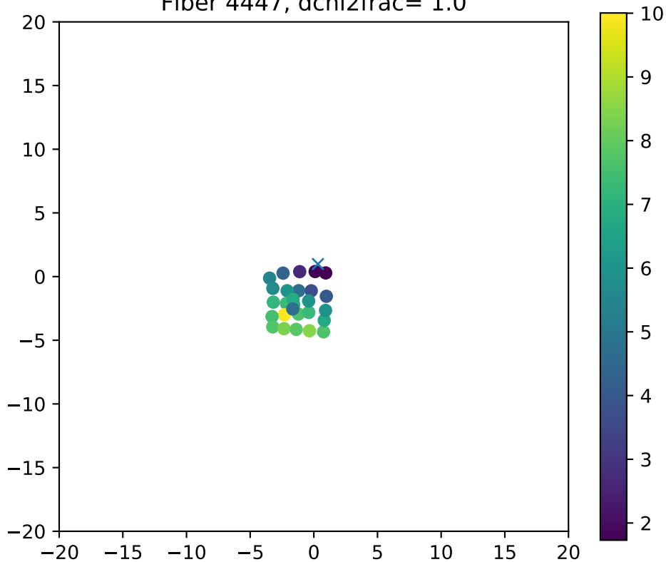
Fiber 4447, dchi2frac= 1.0
