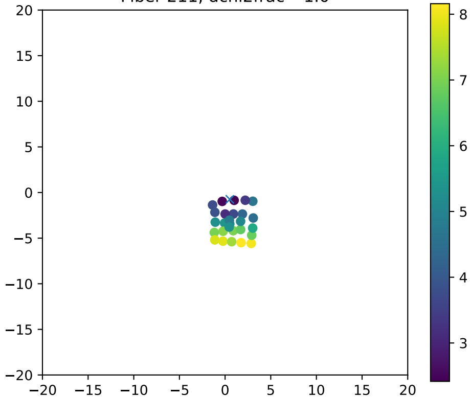
Fiber 211, dchi2frac= 1.0
