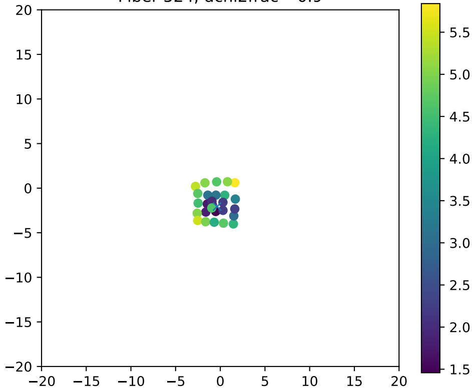
Fiber 524, dchi2frac= 0.9
