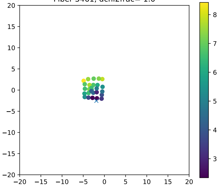
Fiber 3461, dchi2frac= 1.0
