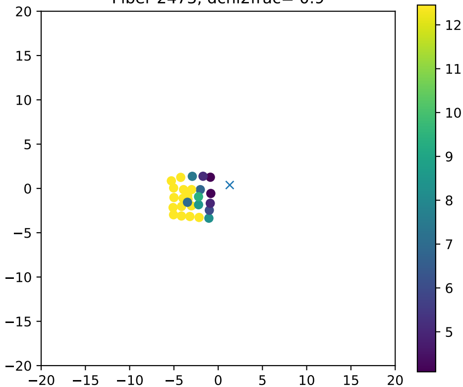
Fiber 2473, dchi2frac= 0.9
