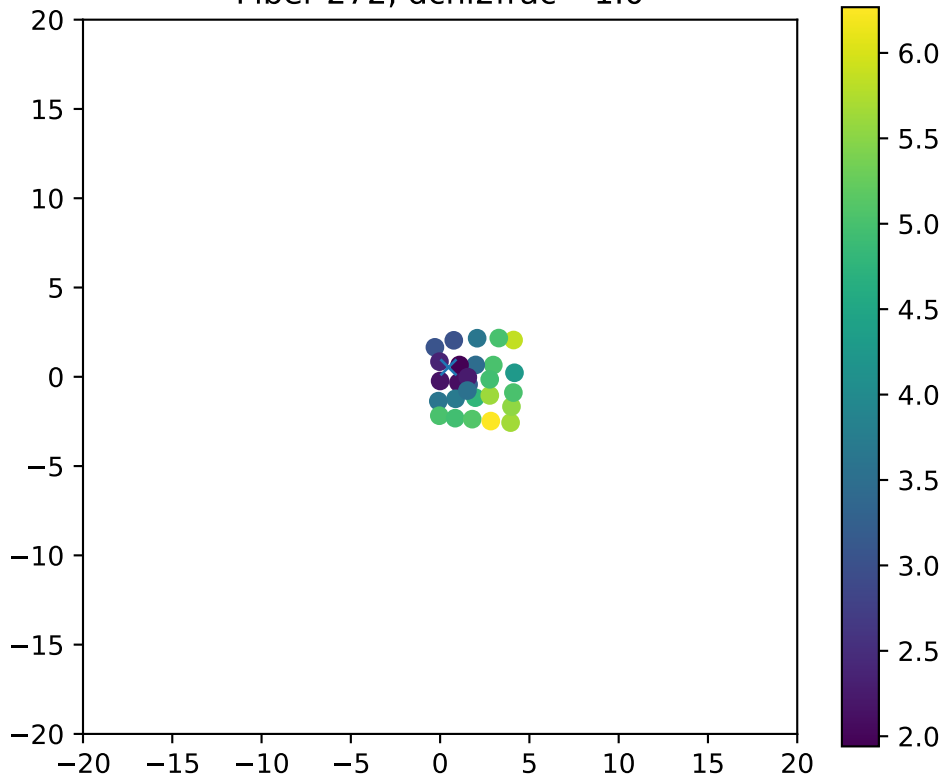
Fiber 272, dchi2frac= 1.0
