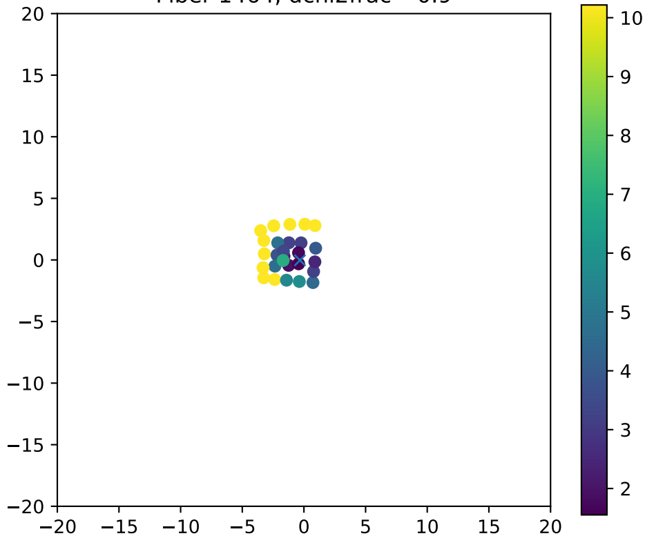
Fiber 1464, dchi2frac= 0.9
