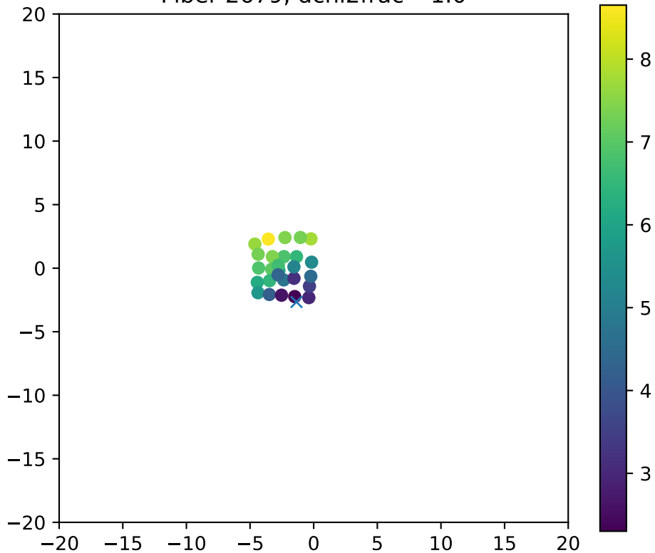
Fiber 2679, dchi2frac= 1.0
