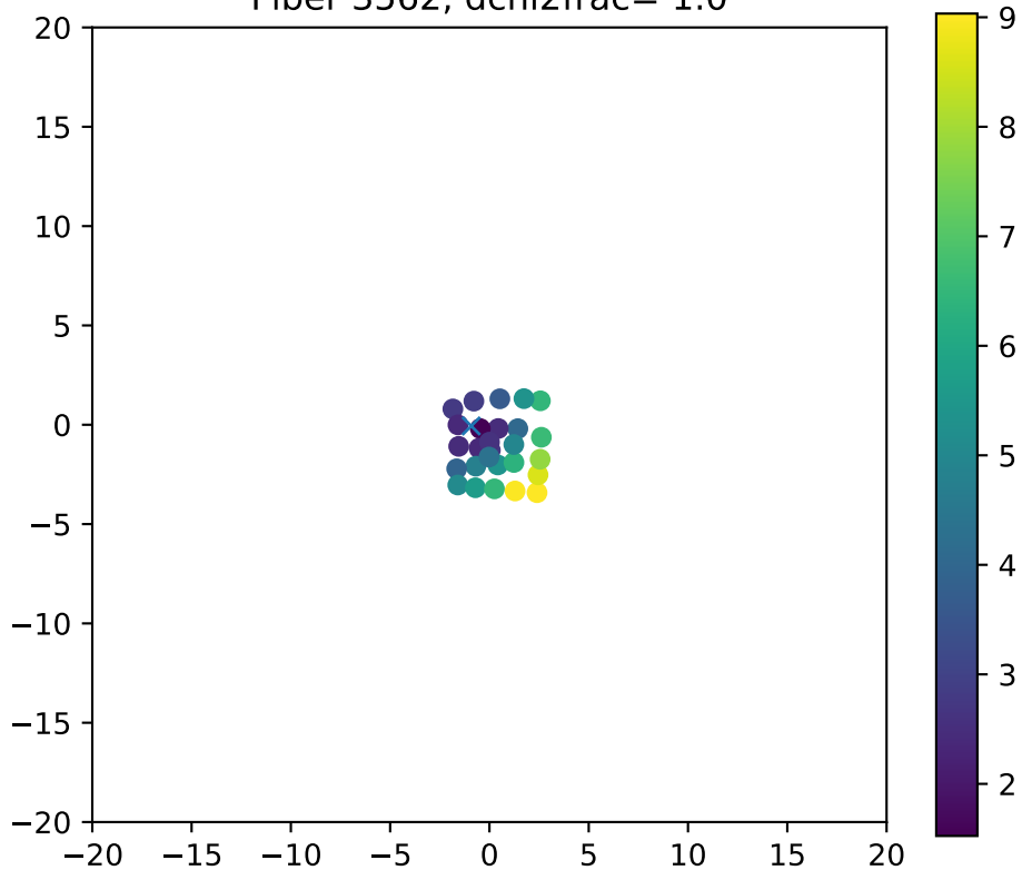
Fiber 3562, dchi2frac= 1.0
