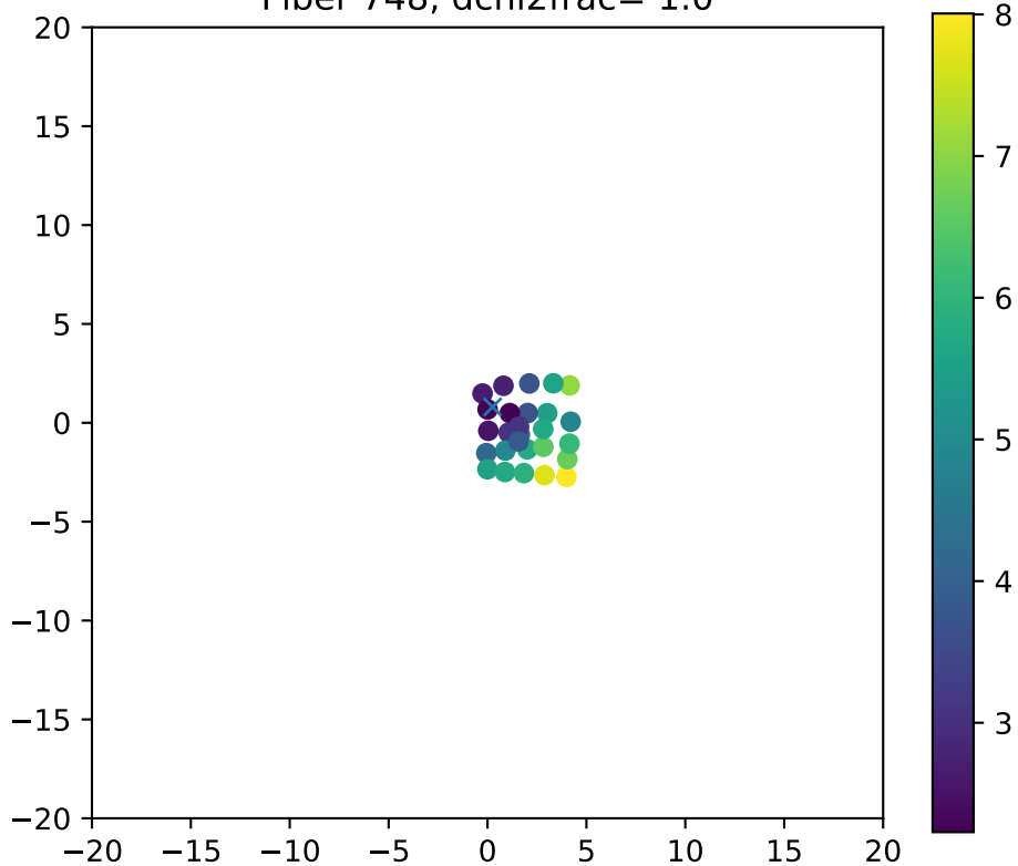
Fiber 748, dchi2frac= 1.0
