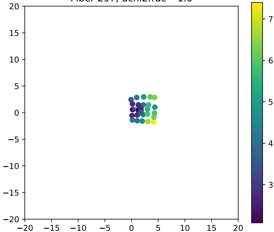
Fiber 297, dchi2frac= 1.0
