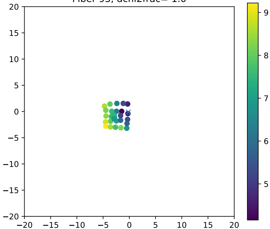
Fiber 93, dchi2frac= 1.0
