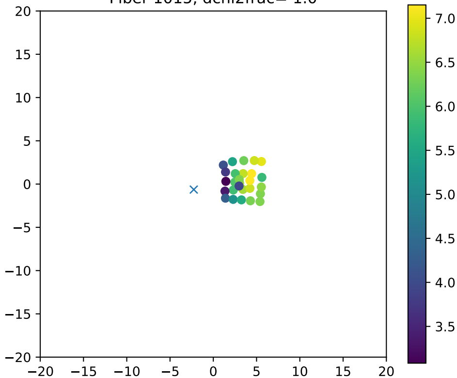
Fiber 1015, dchi2frac= 1.0
