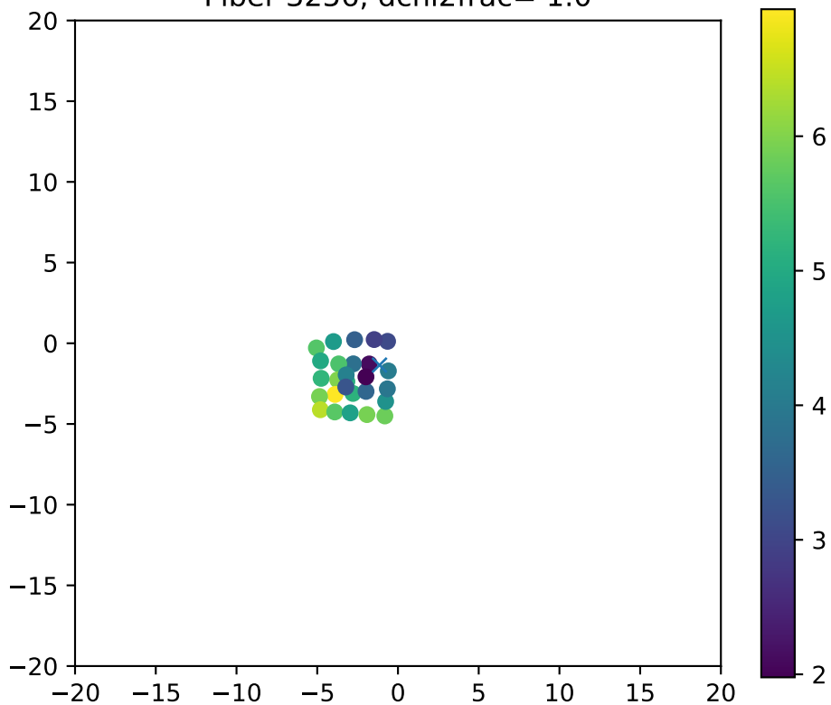
Fiber 3256, dchi2frac= 1.0
