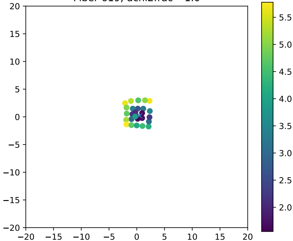
Fiber 619, dchi2frac= 1.0
