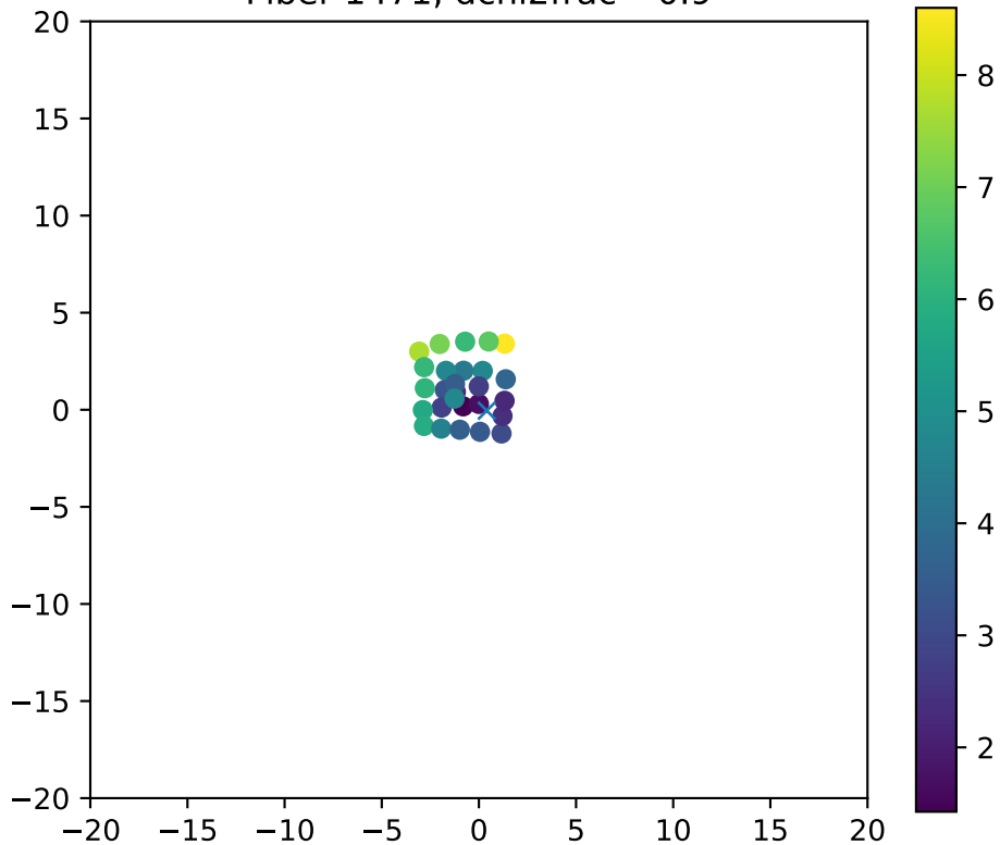
Fiber 1471, dchi2frac= 0.9
