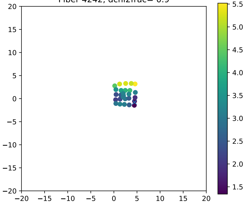
Fiber 4242, dchi2frac= 0.9
