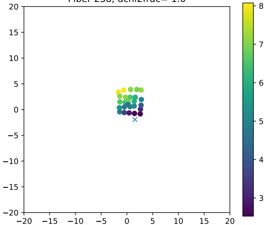
Fiber 238, dchi2frac= 1.0
