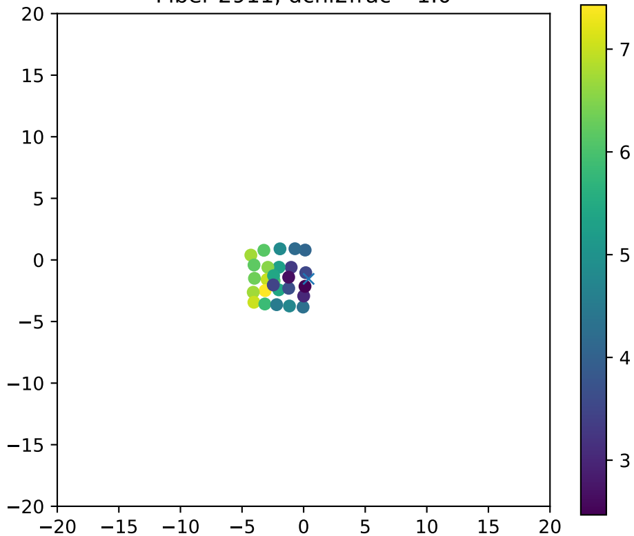
Fiber 2911, dchi2frac= 1.0
