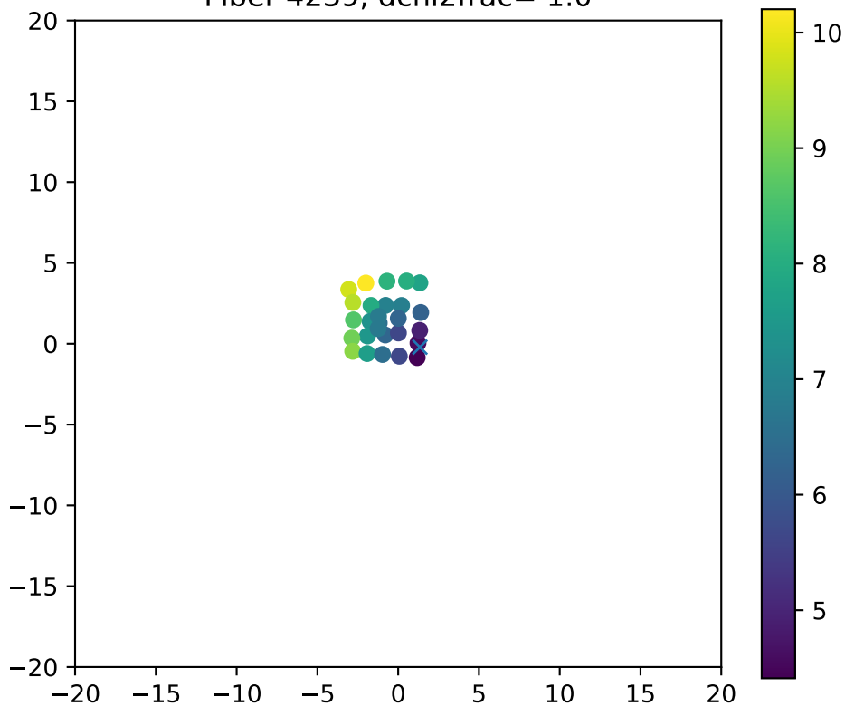
Fiber 4239, dchi2frac= 1.0
