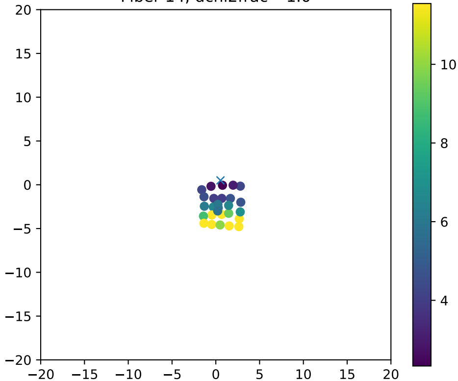
Fiber 14, dchi2frac= 1.0
