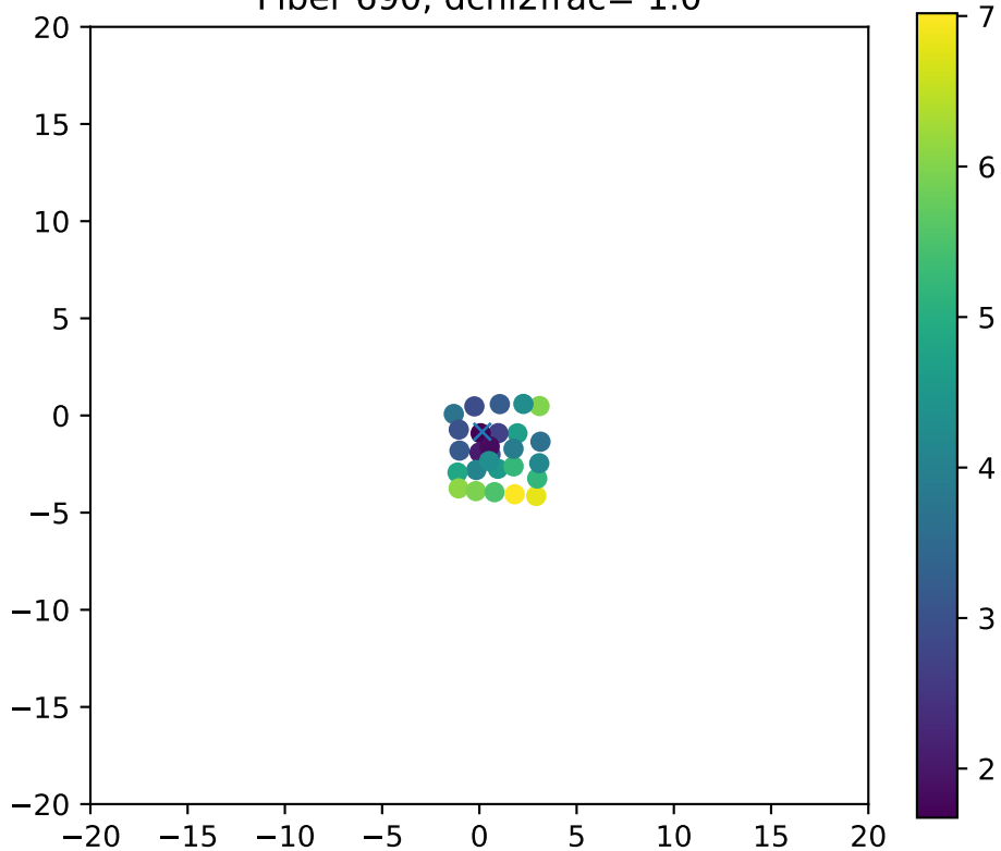
Fiber 690, dchi2frac= 1.0
