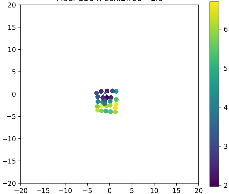
Fiber 3564, dchi2frac= 1.0
