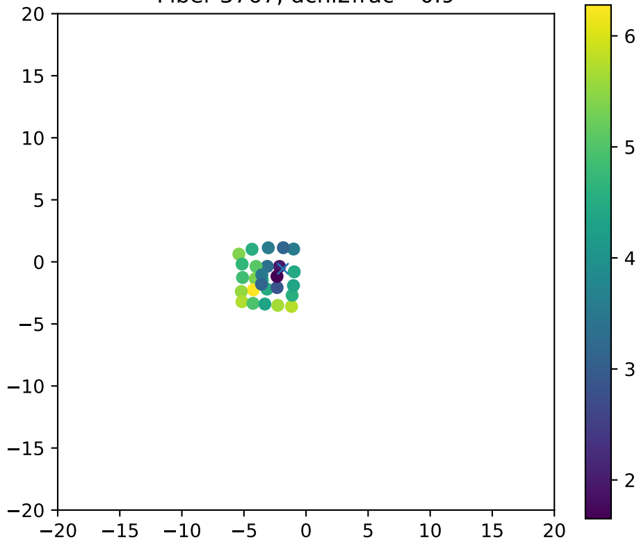
Fiber 3767, dchi2frac= 0.9
