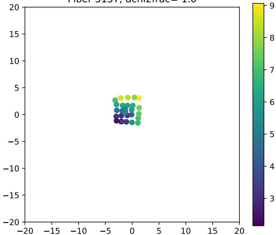
Fiber 3157, dchi2frac= 1.0
