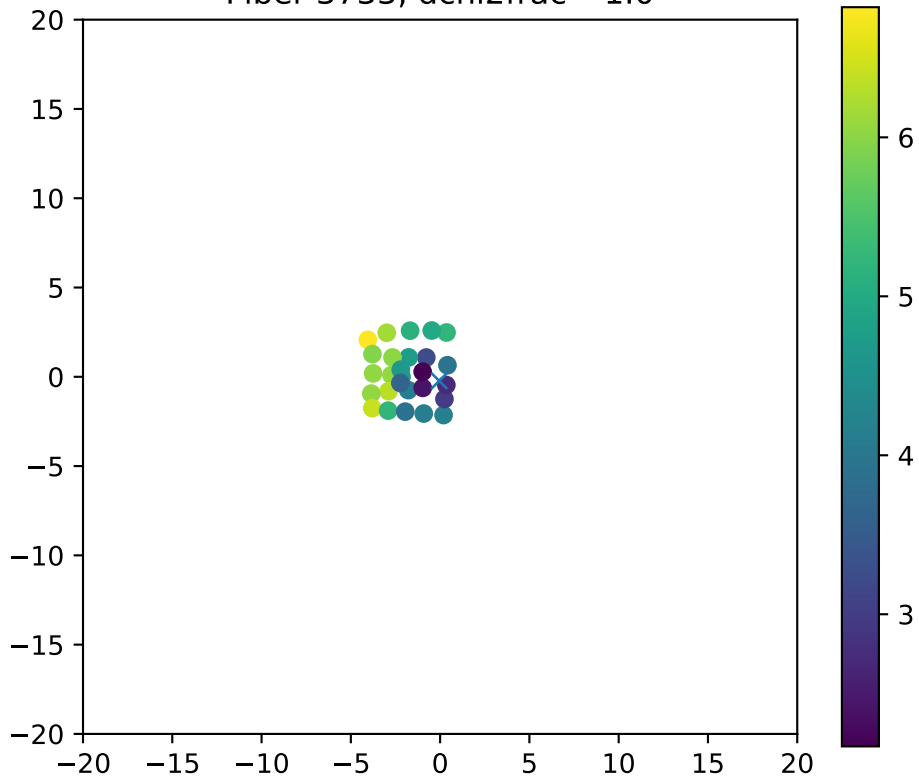
Fiber 3733, dchi2frac= 1.0
