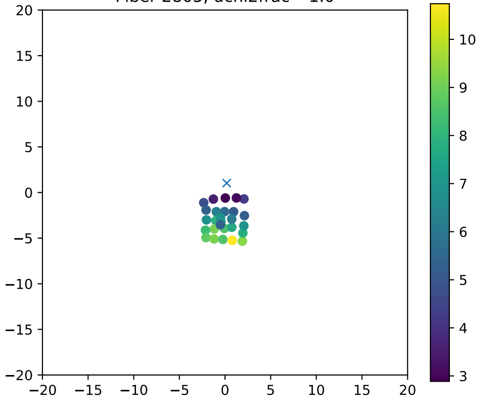
Fiber 2805, dchi2frac= 1.0
