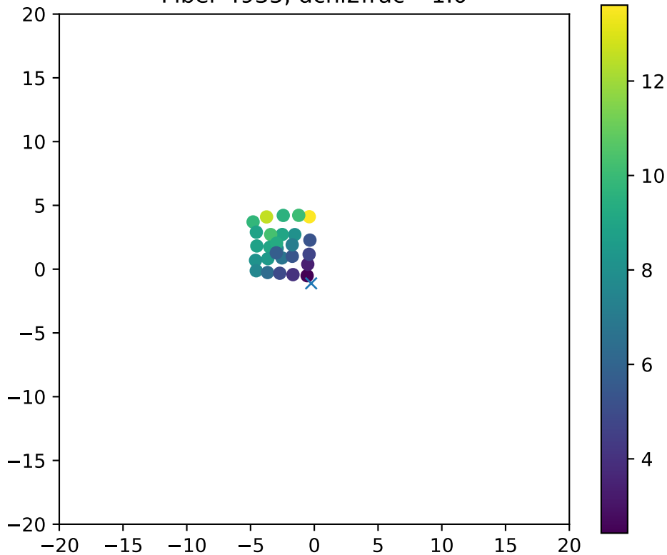
Fiber 4935, dchi2frac= 1.0
