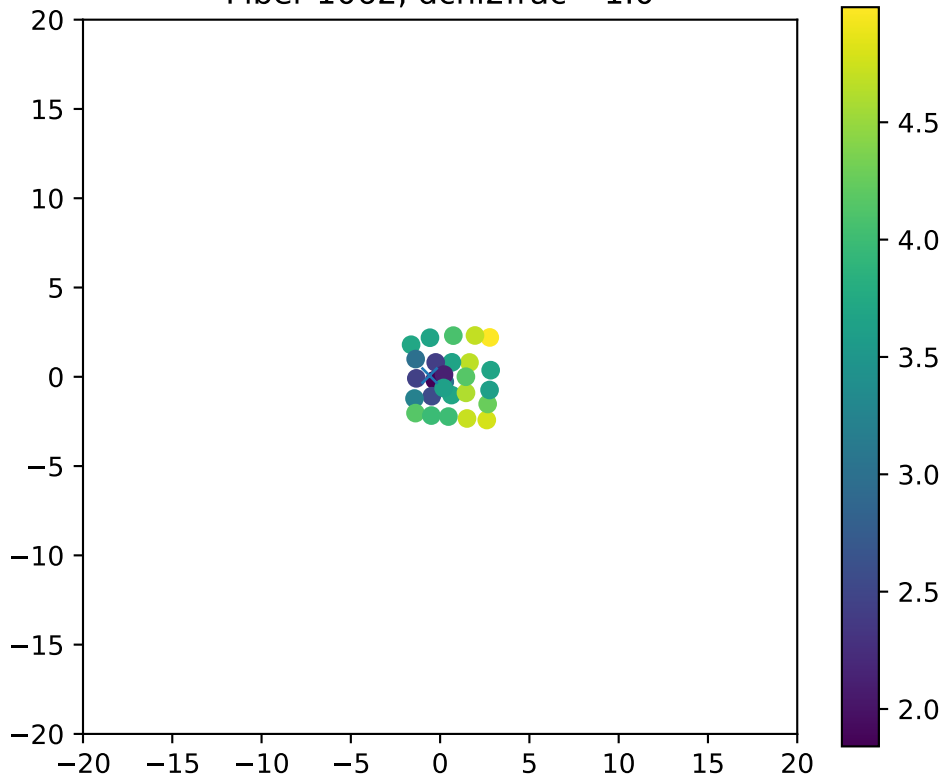
Fiber 1062, dchi2frac= 1.0
