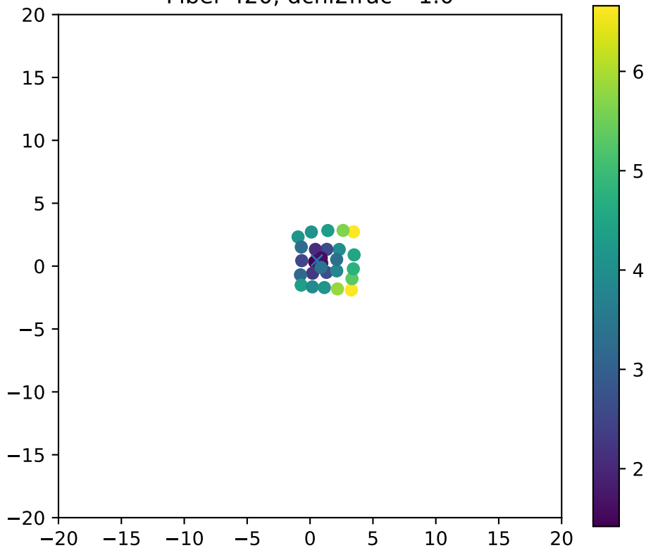
Fiber 420, dchi2frac= 1.0
