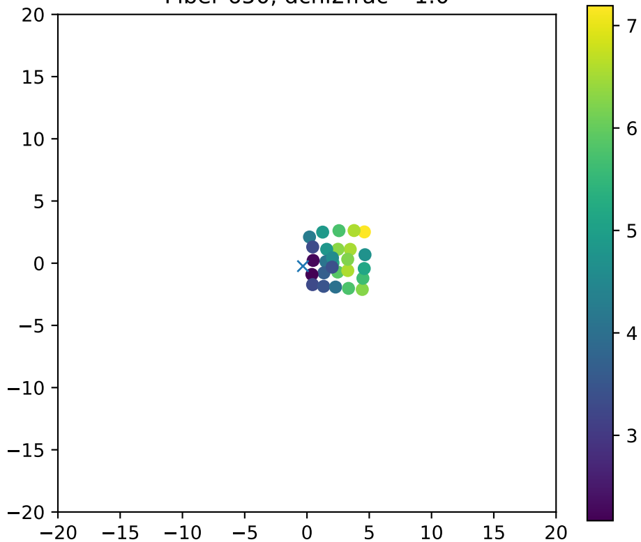
Fiber 650, dchi2frac= 1.0
