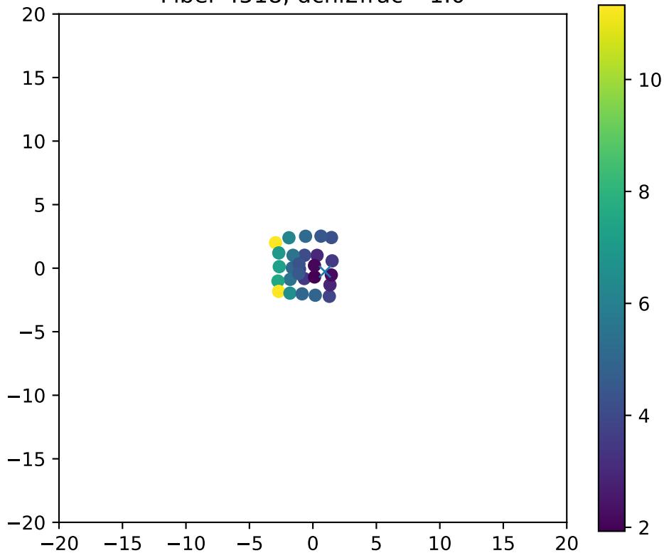
Fiber 4518, dchi2frac= 1.0
