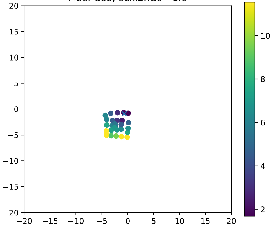
Fiber 888, dchi2frac= 1.0
