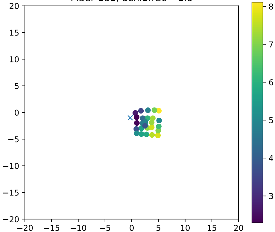
Fiber 181, dchi2frac= 1.0
