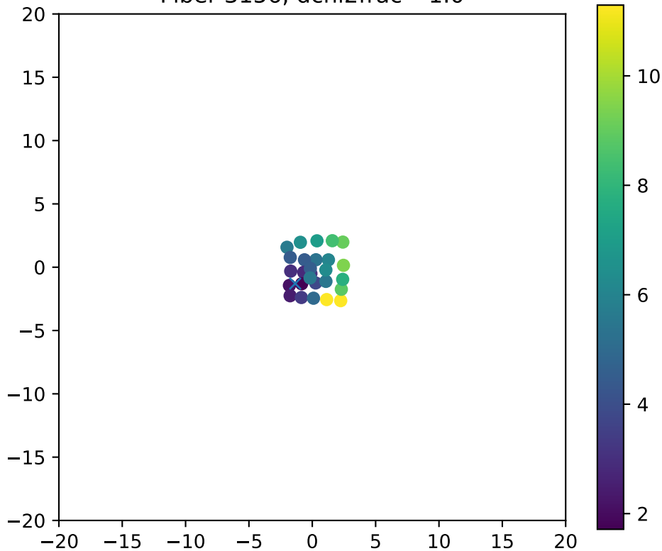
Fiber 3156, dchi2frac= 1.0
