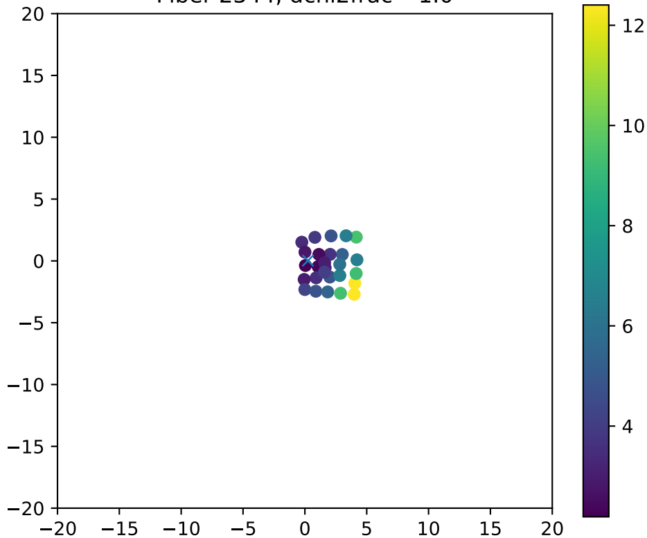
Fiber 2344, dchi2frac= 1.0
