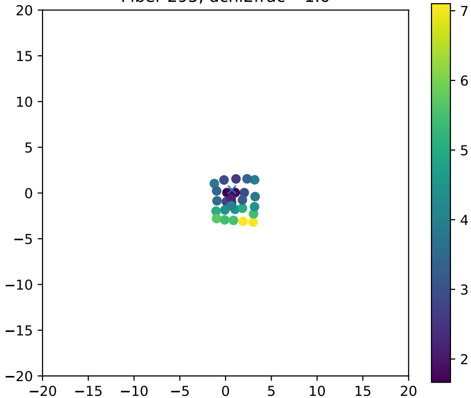
Fiber 295, dchi2frac= 1.0
