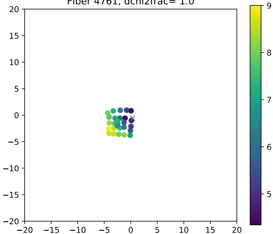
Fiber 4761, dchi2frac= 1.0
