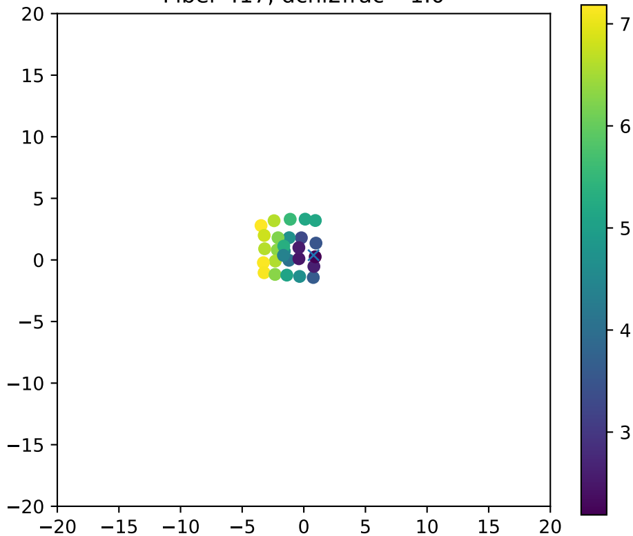
Fiber 417, dchi2frac= 1.0
