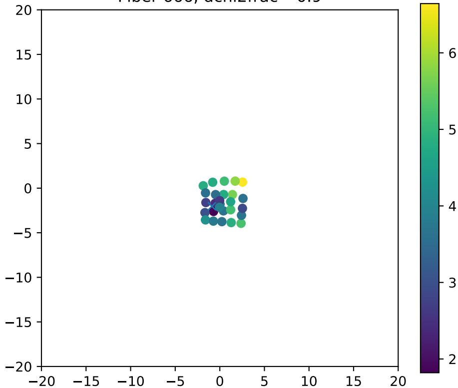
Fiber 666, dchi2frac= 0.9
