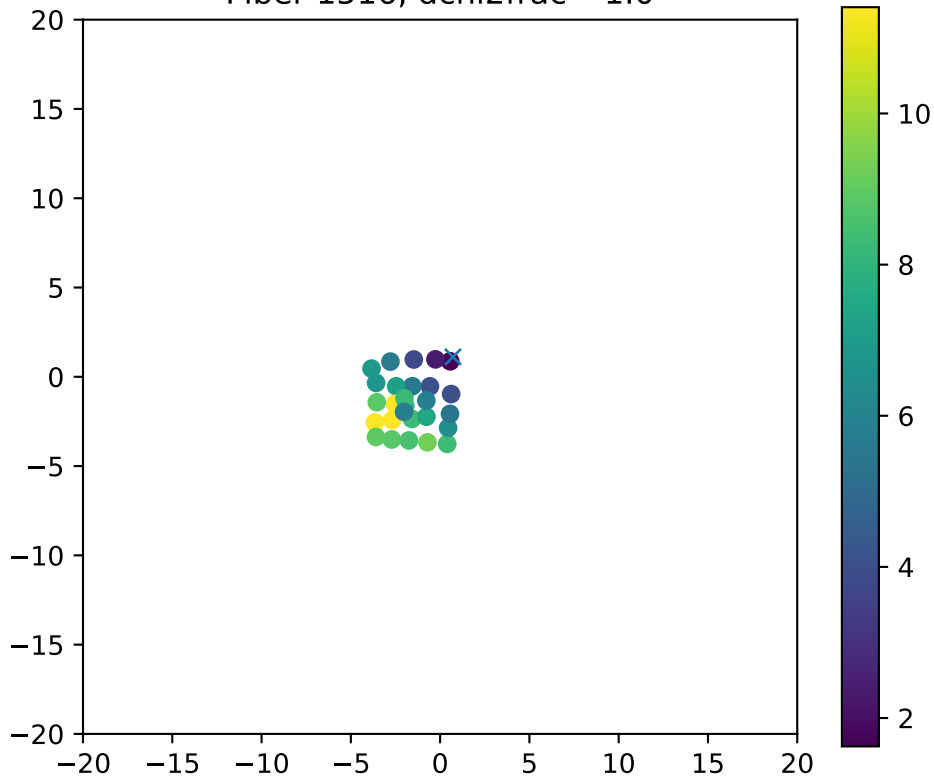
Fiber 1516, dchi2frac= 1.0
