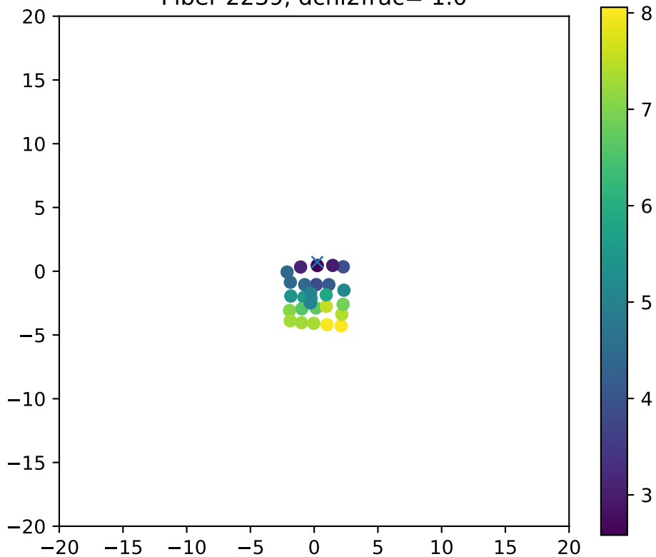
Fiber 2239, dchi2frac= 1.0
