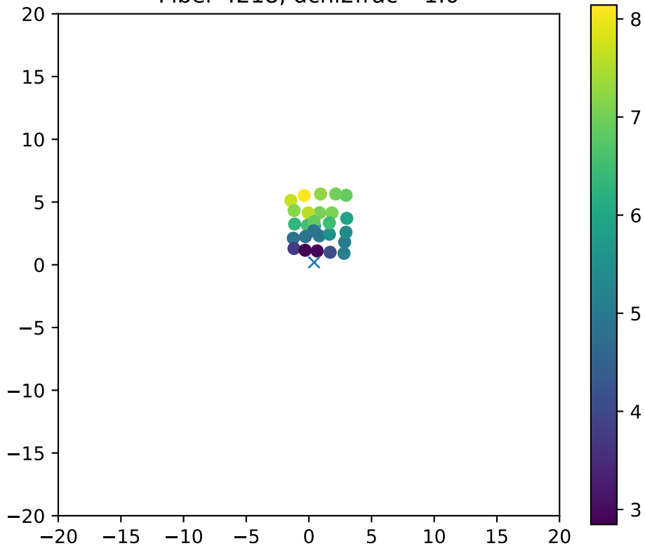
Fiber 4218, dchi2frac= 1.0
