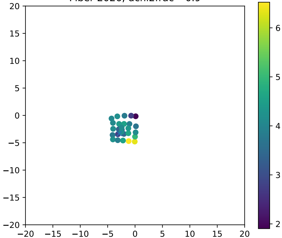
Fiber 2026, dchi2frac= 0.9
