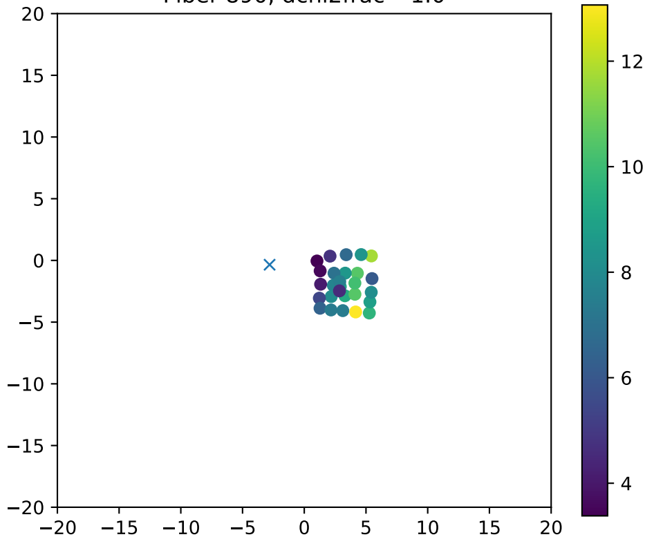
Fiber 890, dchi2frac= 1.0
