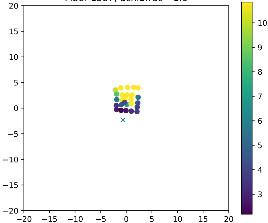
Fiber 1387, dchi2frac= 1.0
