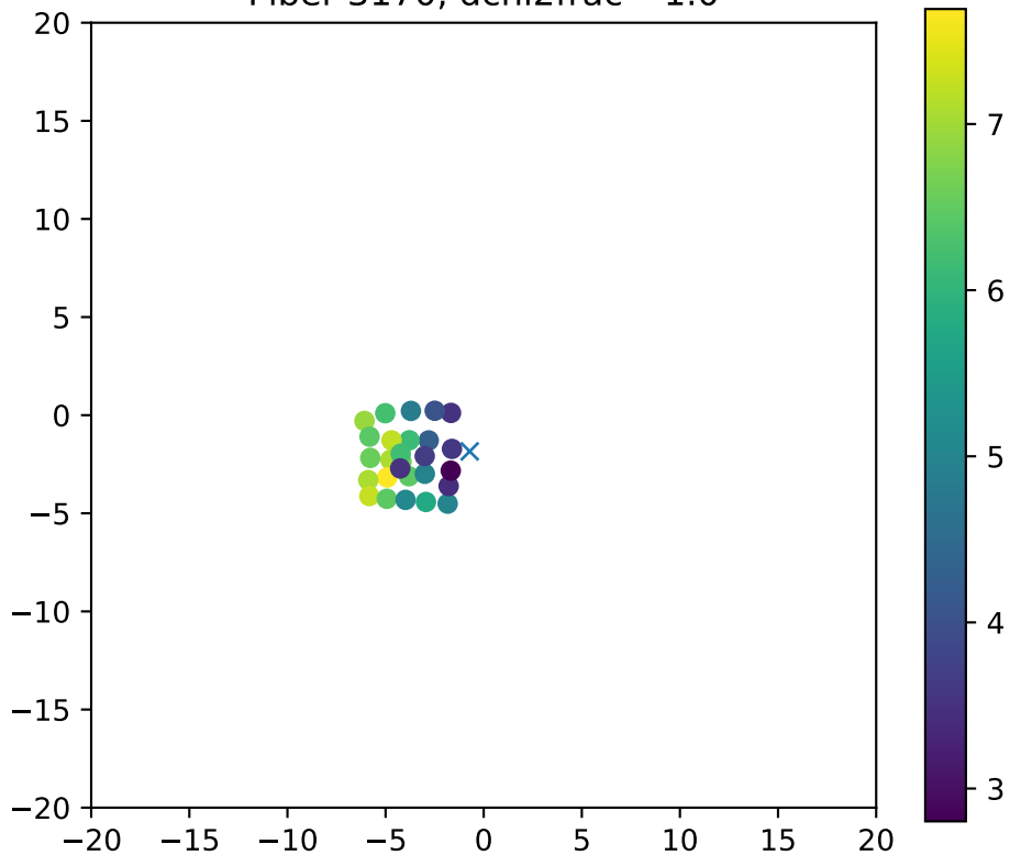
Fiber 3170, dchi2frac= 1.0
