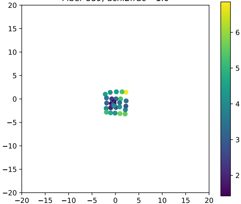
Fiber 889, dchi2frac= 1.0
