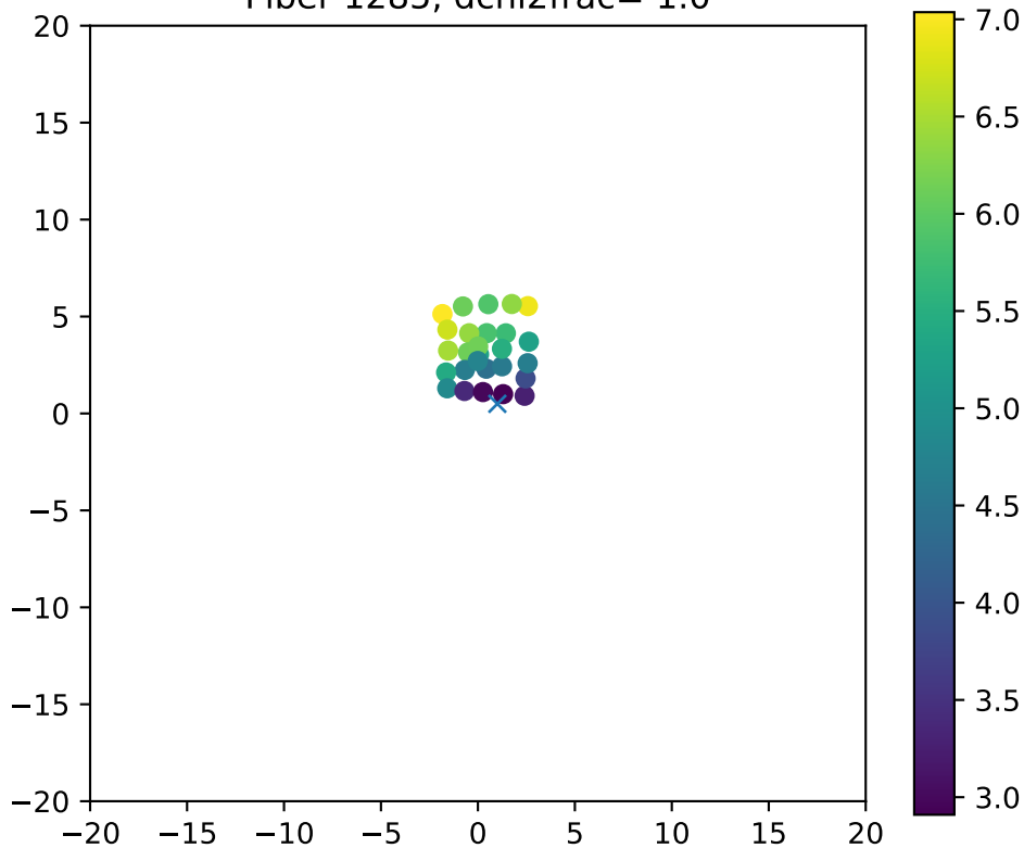
Fiber 1285, dchi2frac= 1.0
