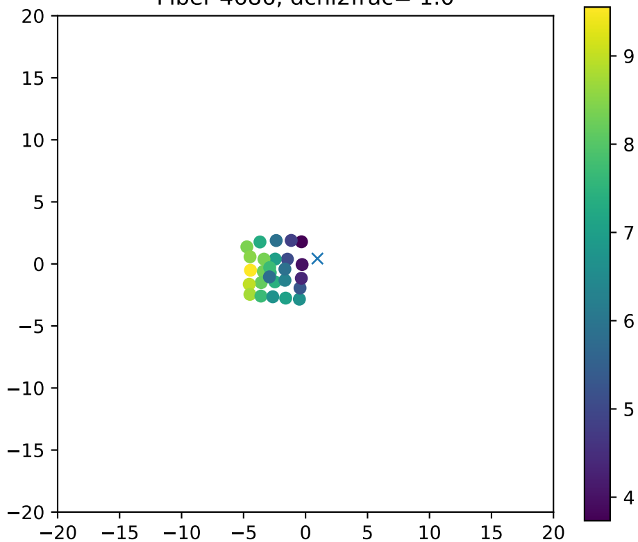
Fiber 4686, dchi2frac= 1.0
