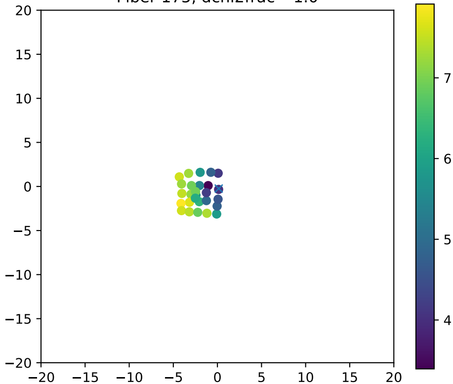
Fiber 175, dchi2frac= 1.0
