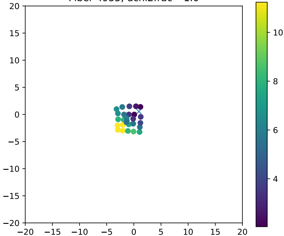
Fiber 4955, dchi2frac= 1.0
