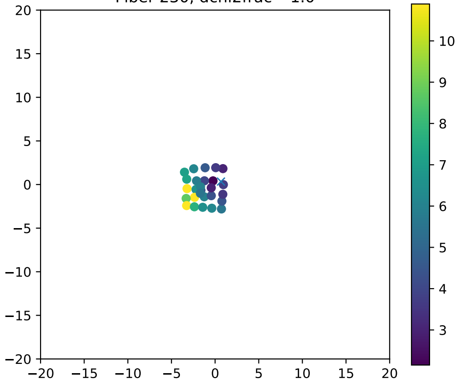
Fiber 230, dchi2frac= 1.0
