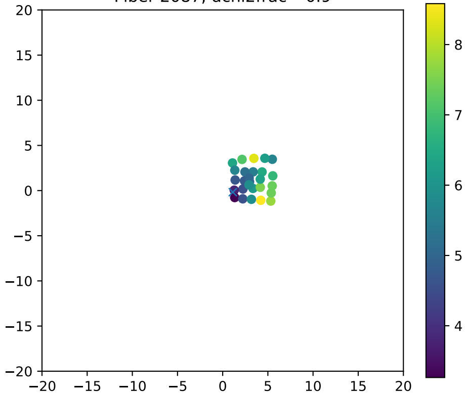
Fiber 2087, dchi2frac= 0.9
