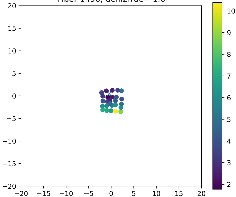
Fiber 1490, dchi2frac= 1.0
