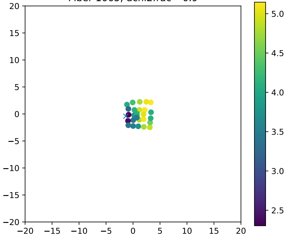
Fiber 1065, dchi2frac= 0.9
