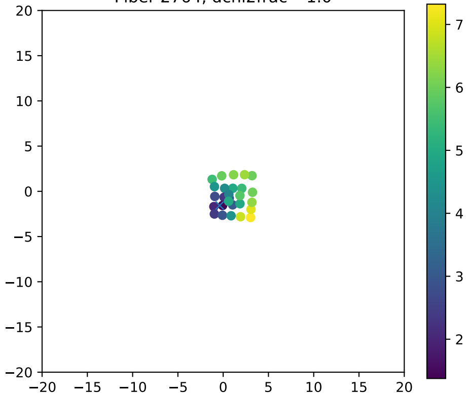
Fiber 2764, dchi2frac= 1.0
