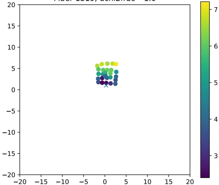
Fiber 1319, dchi2frac= 1.0
