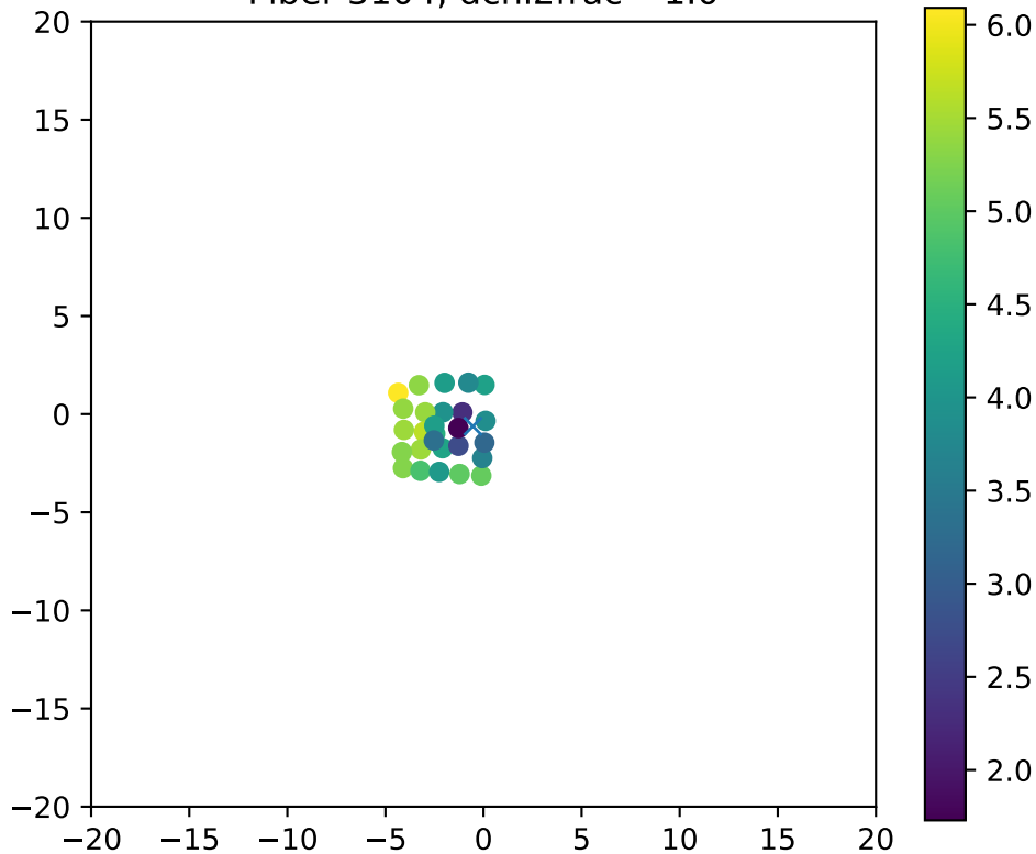
Fiber 3104, dchi2frac= 1.0
