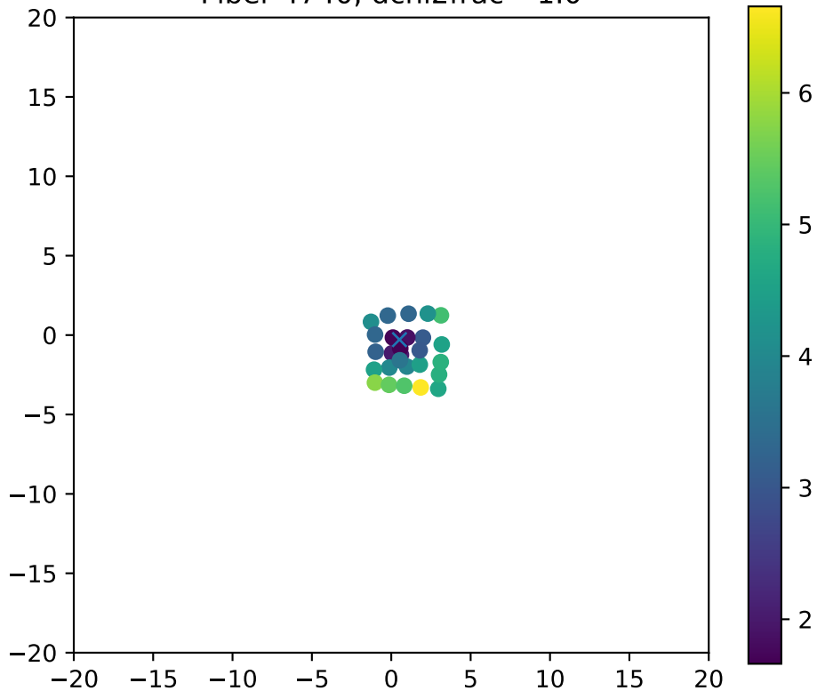
Fiber 4740, dchi2frac= 1.0
