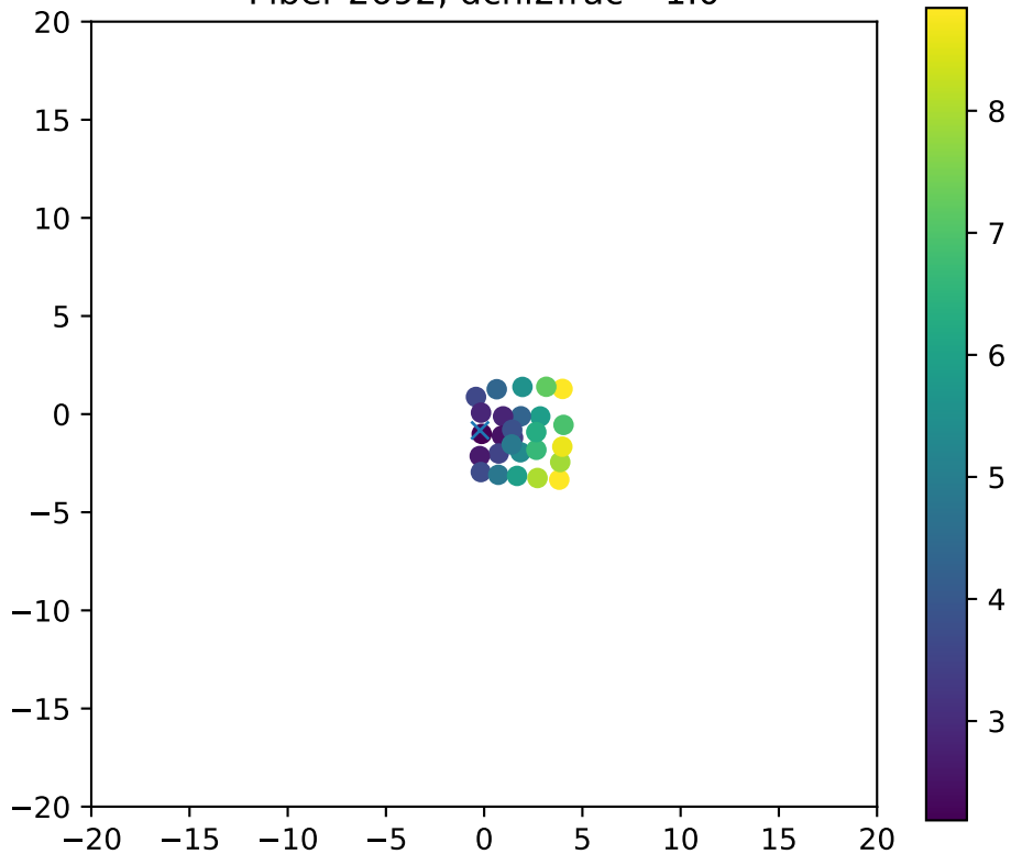
Fiber 2692, dchi2frac= 1.0
