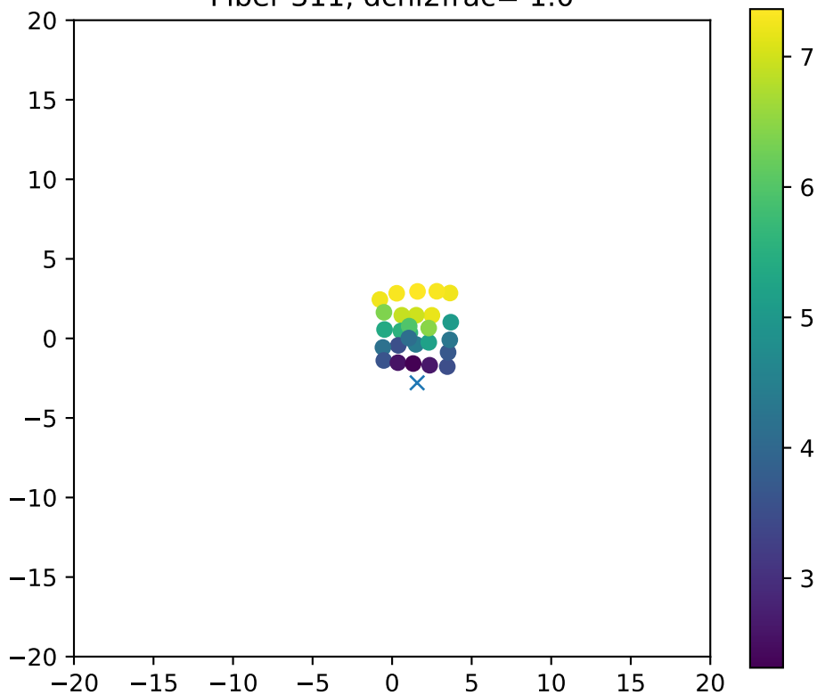
Fiber 311, dchi2frac= 1.0
