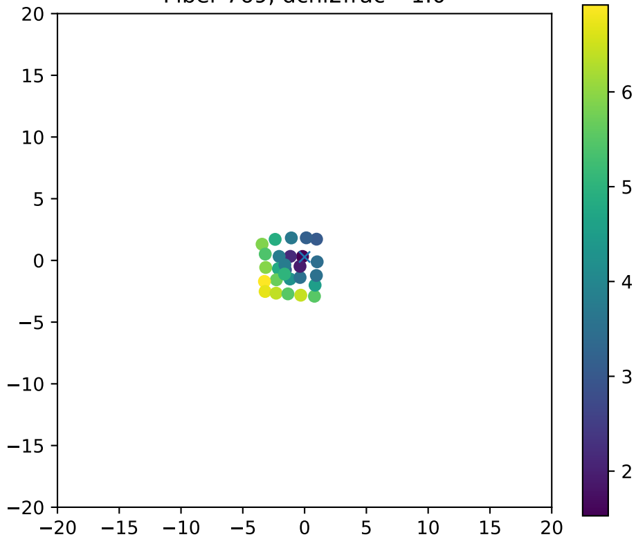
Fiber 769, dchi2frac= 1.0
