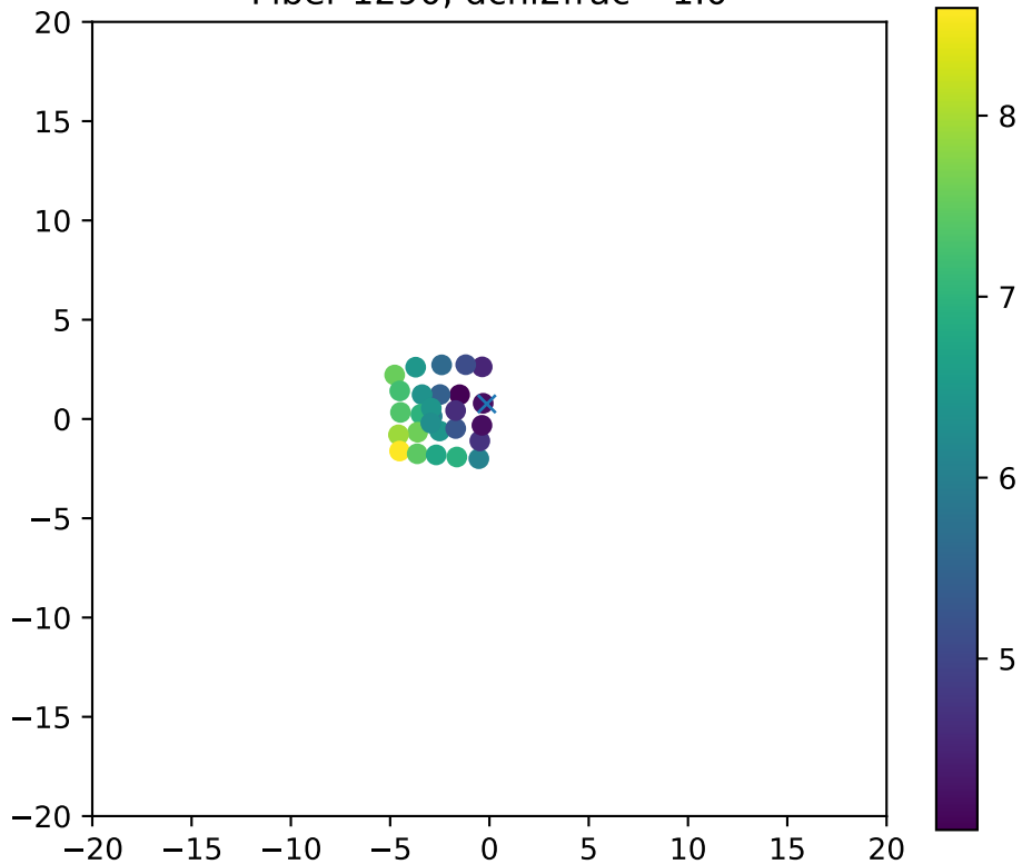
Fiber 1290, dchi2frac= 1.0
