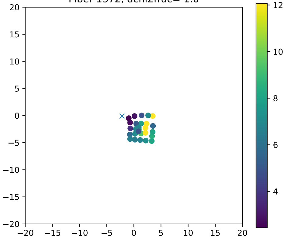
Fiber 1372, dchi2frac= 1.0
