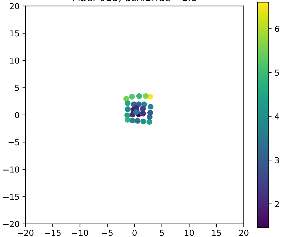
Fiber 925, dchi2frac= 1.0
