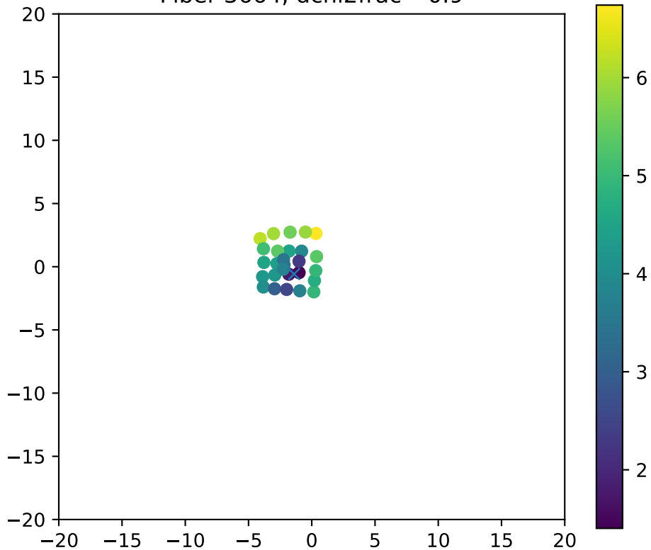
Fiber 3664, dchi2frac= 0.9
