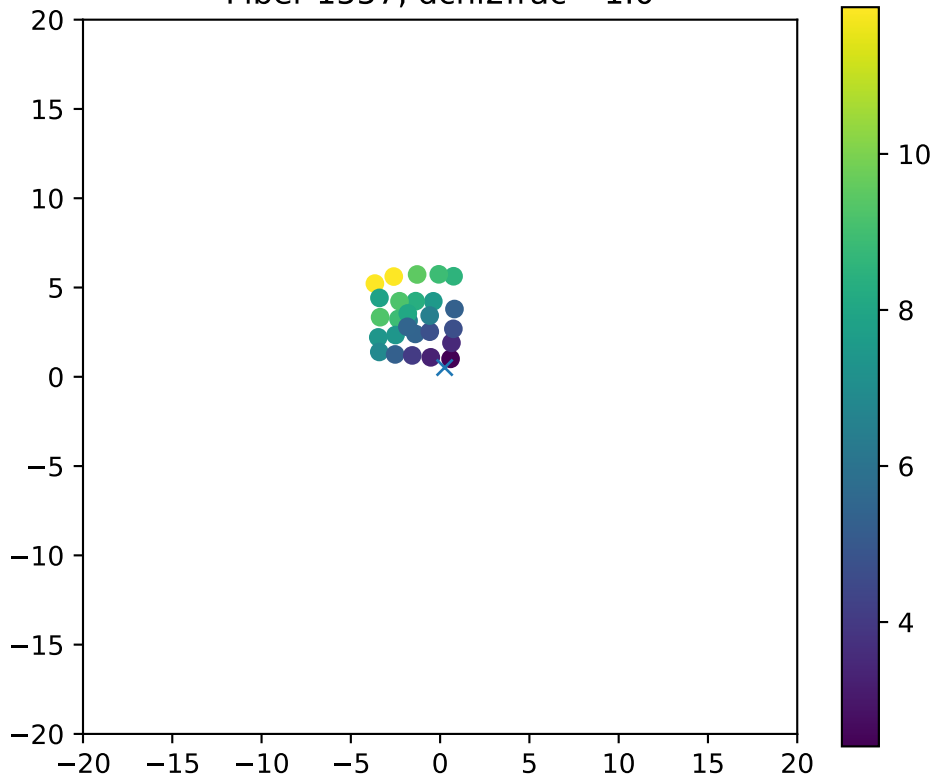
Fiber 1557, dchi2frac= 1.0
