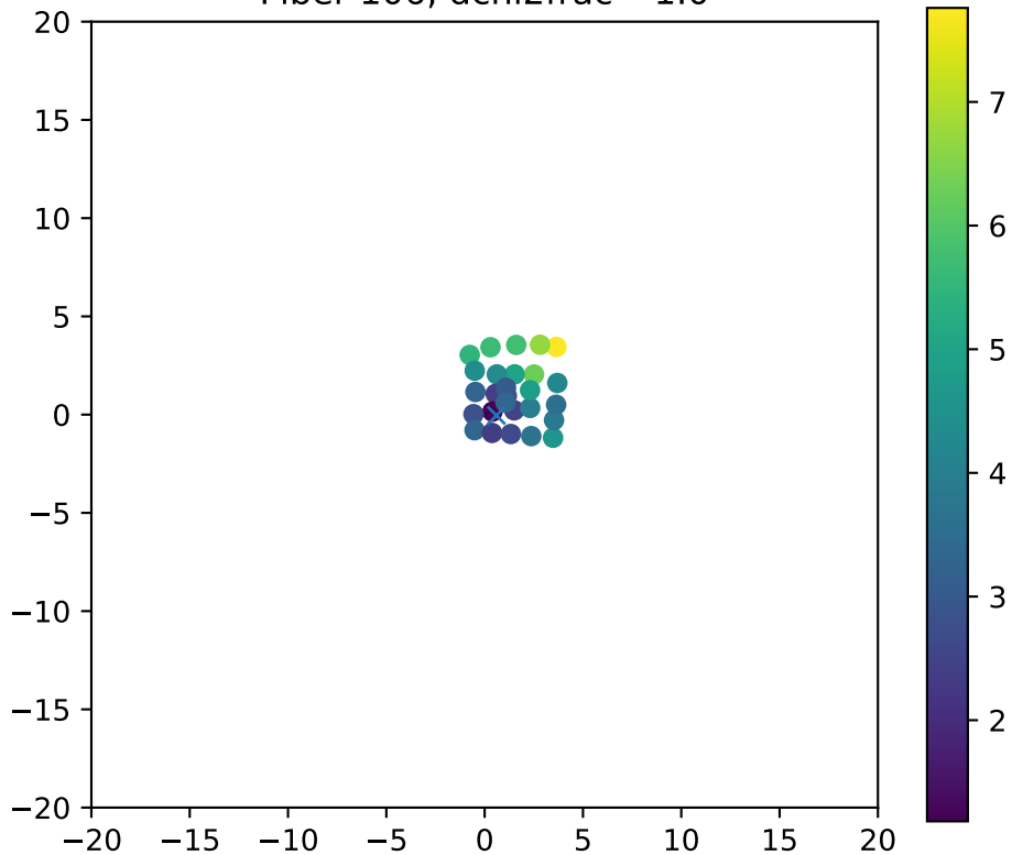
Fiber 106, dchi2frac= 1.0
