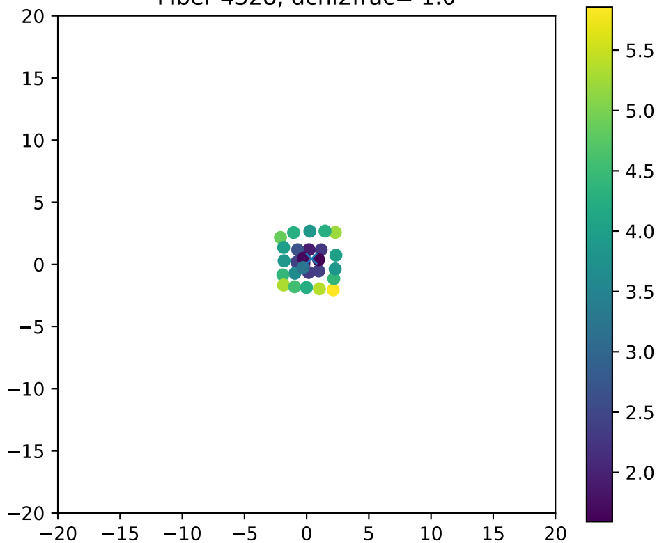
Fiber 4328, dchi2frac= 1.0
