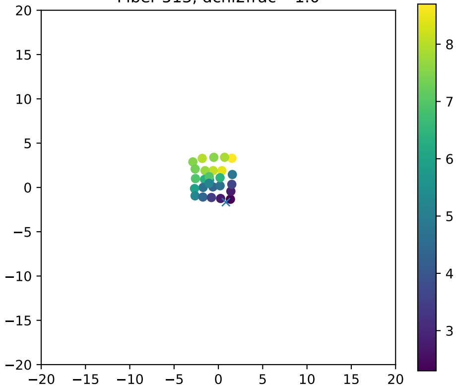
Fiber 513, dchi2frac= 1.0
