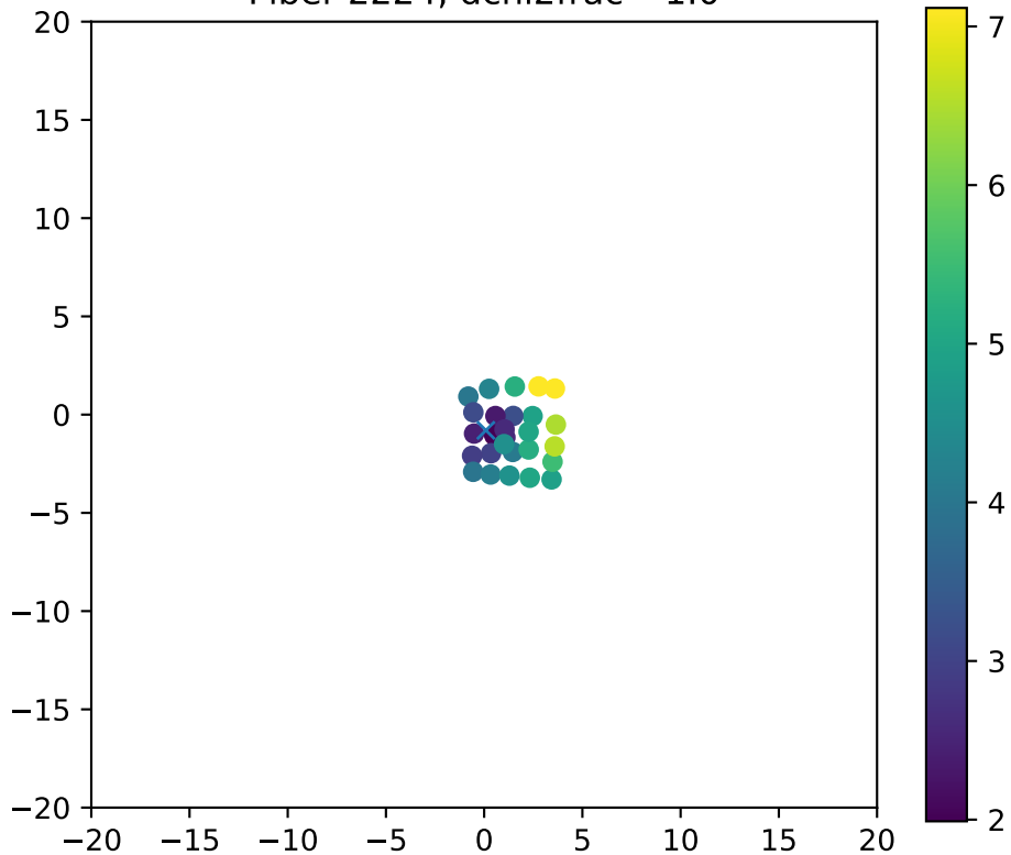
Fiber 2224, dchi2frac= 1.0
