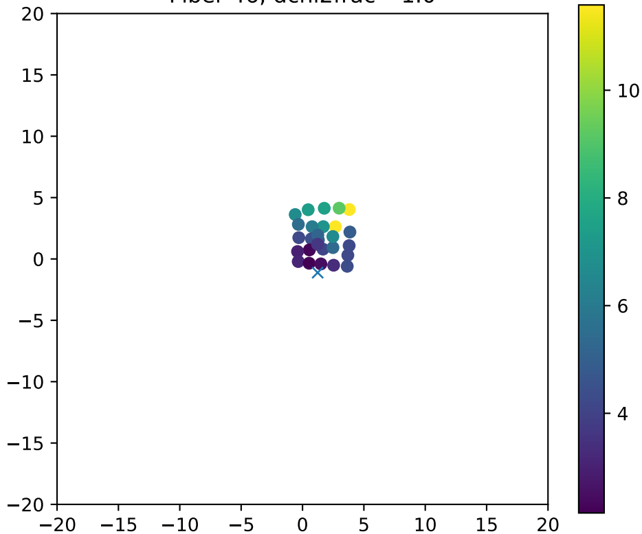
Fiber 46, dchi2frac= 1.0
