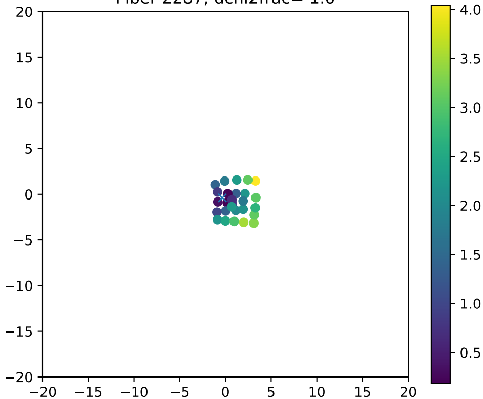
Fiber 2287, dchi2frac= 1.0
