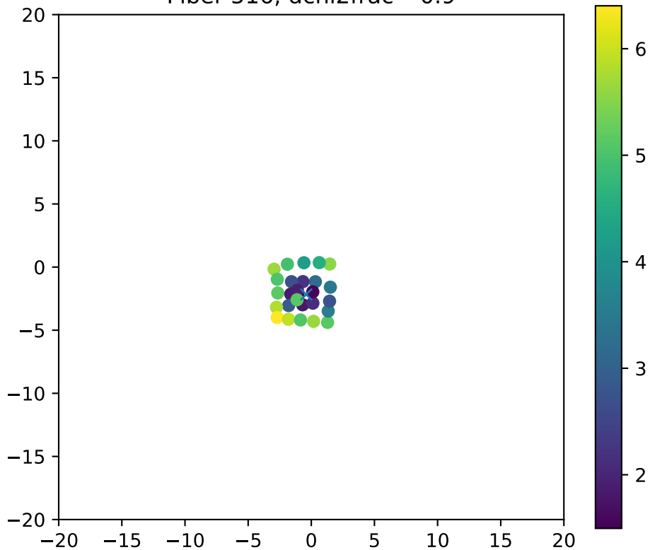
Fiber 516, dchi2frac= 0.9
