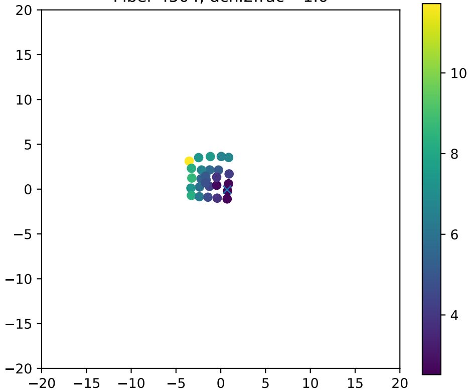
Fiber 4504, dchi2frac= 1.0
