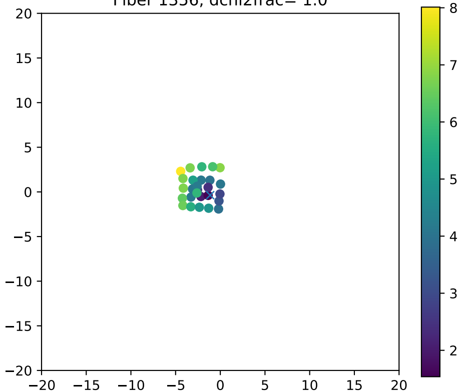
Fiber 1356, dchi2frac= 1.0
