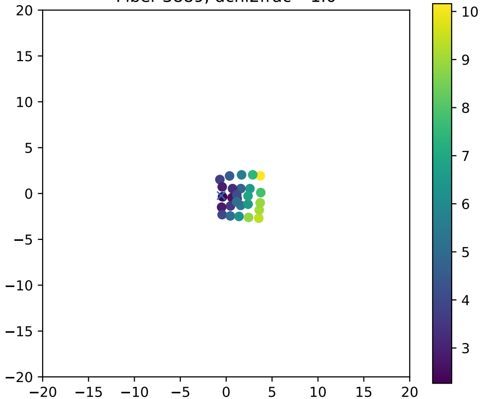
Fiber 3889, dchi2frac= 1.0
