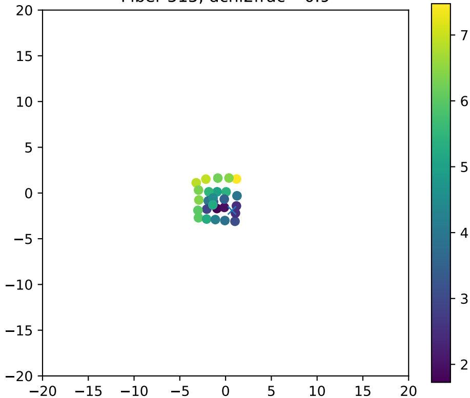
Fiber 515, dchi2frac= 0.9
