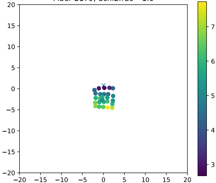
Fiber 2179, dchi2frac= 1.0
