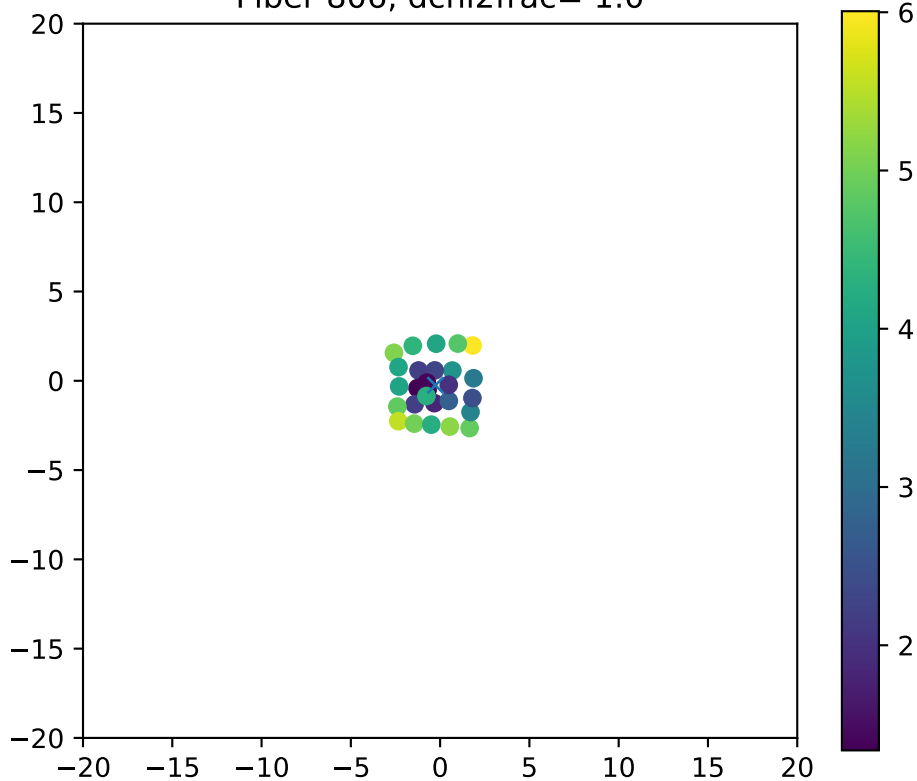
Fiber 806, dchi2frac= 1.0
