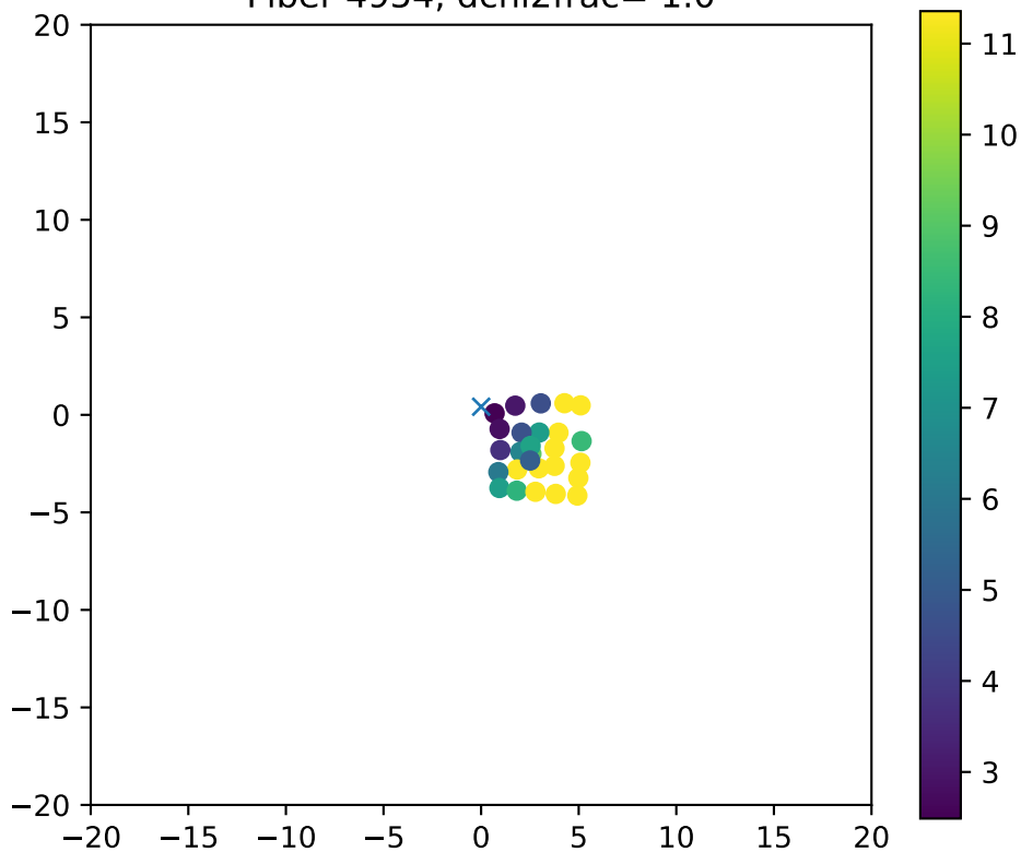
Fiber 4954, dchi2frac= 1.0
