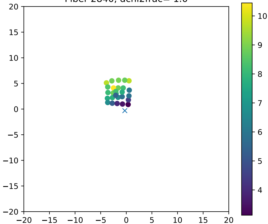
Fiber 2840, dchi2frac= 1.0
