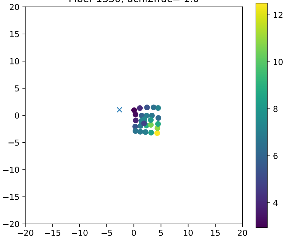
Fiber 1330, dchi2frac= 1.0
