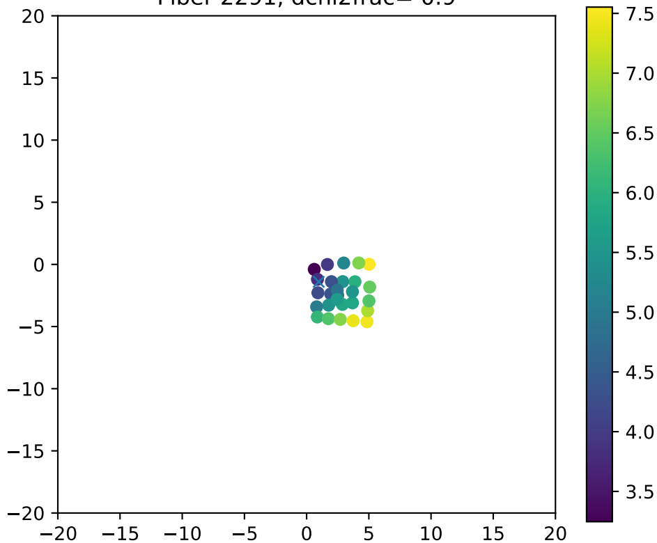
Fiber 2291, dchi2frac= 0.9
