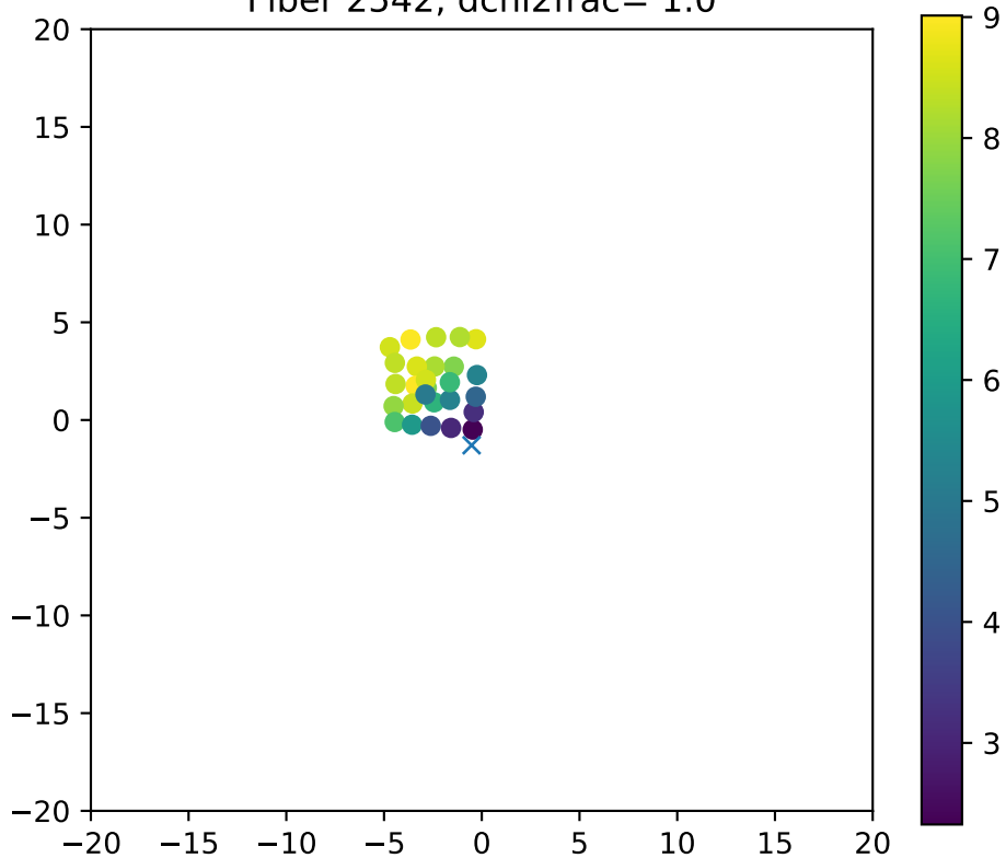
Fiber 2542, dchi2frac= 1.0
