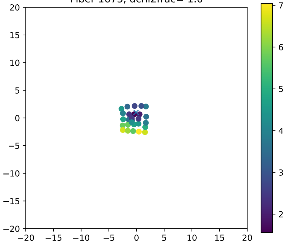
Fiber 1675, dchi2frac= 1.0
