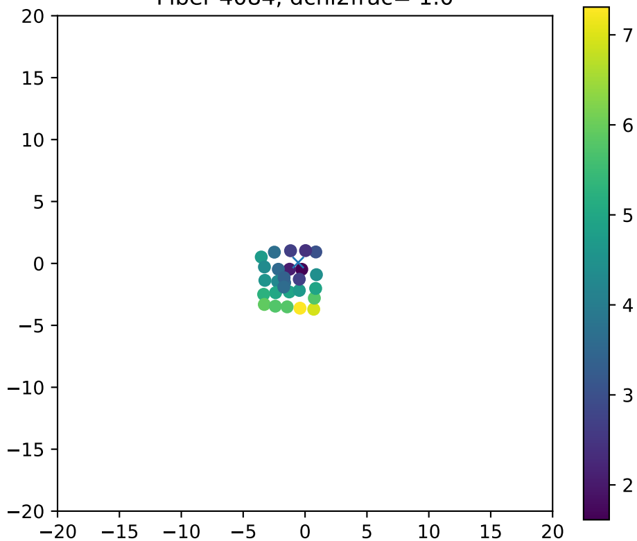
Fiber 4084, dchi2frac= 1.0
