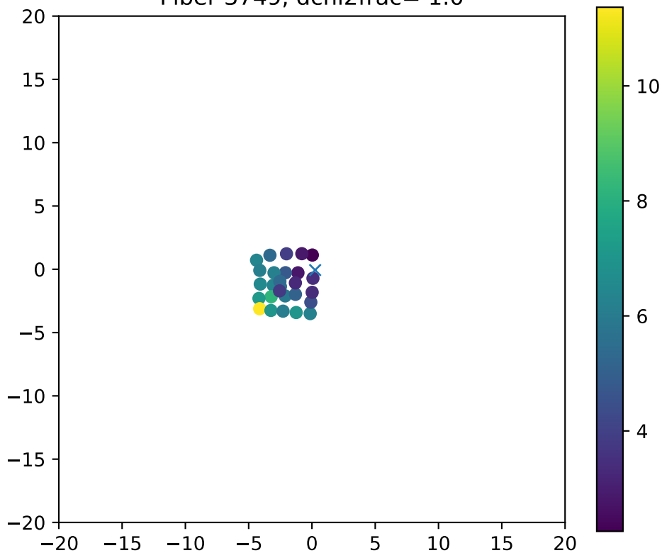
Fiber 3749, dchi2frac= 1.0
