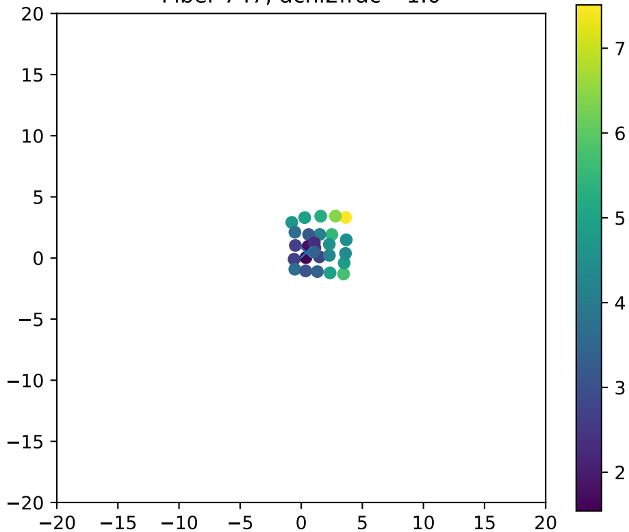
Fiber 747, dchi2frac= 1.0
