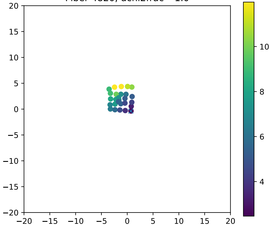
Fiber 4820, dchi2frac= 1.0
