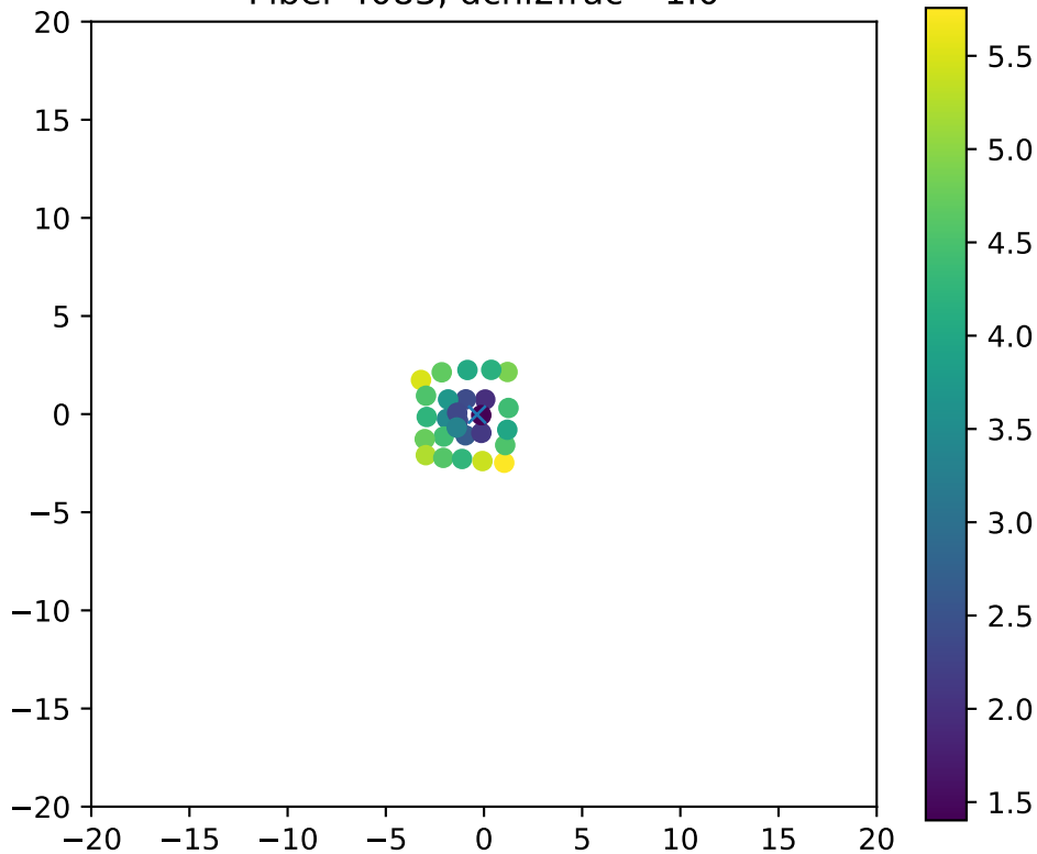
Fiber 4083, dchi2frac= 1.0
