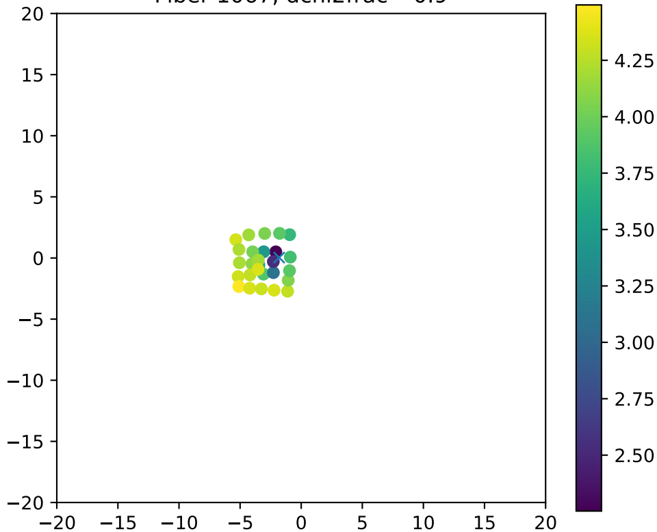
Fiber 1067, dchi2frac= 0.9
