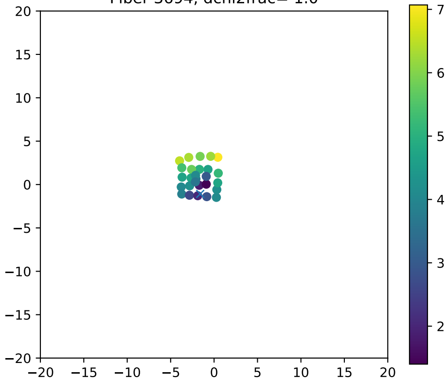
Fiber 3694, dchi2frac= 1.0
