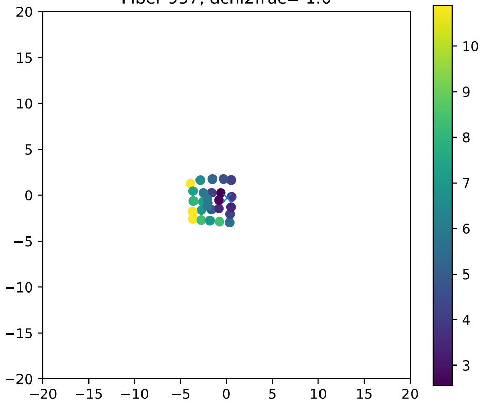
Fiber 957, dchi2frac= 1.0
