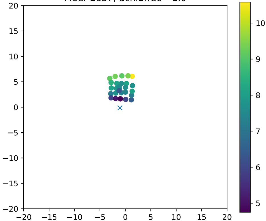
Fiber 2637, dchi2frac= 1.0
