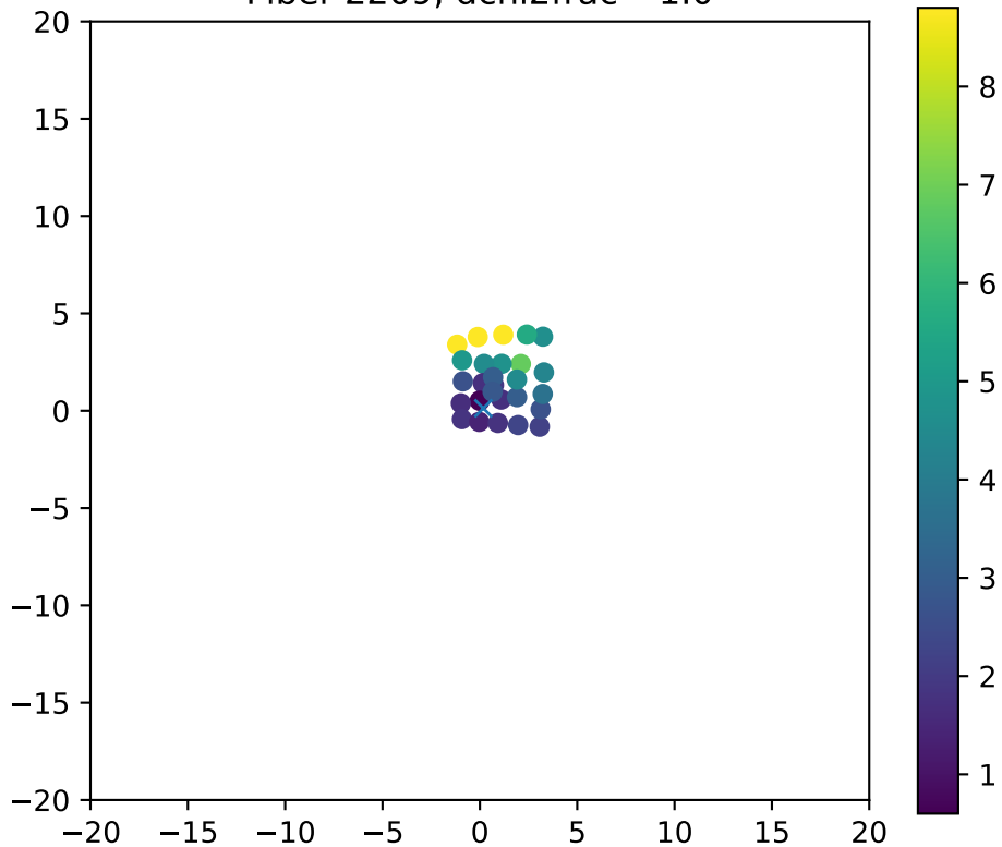
Fiber 2209, dchi2frac= 1.0
