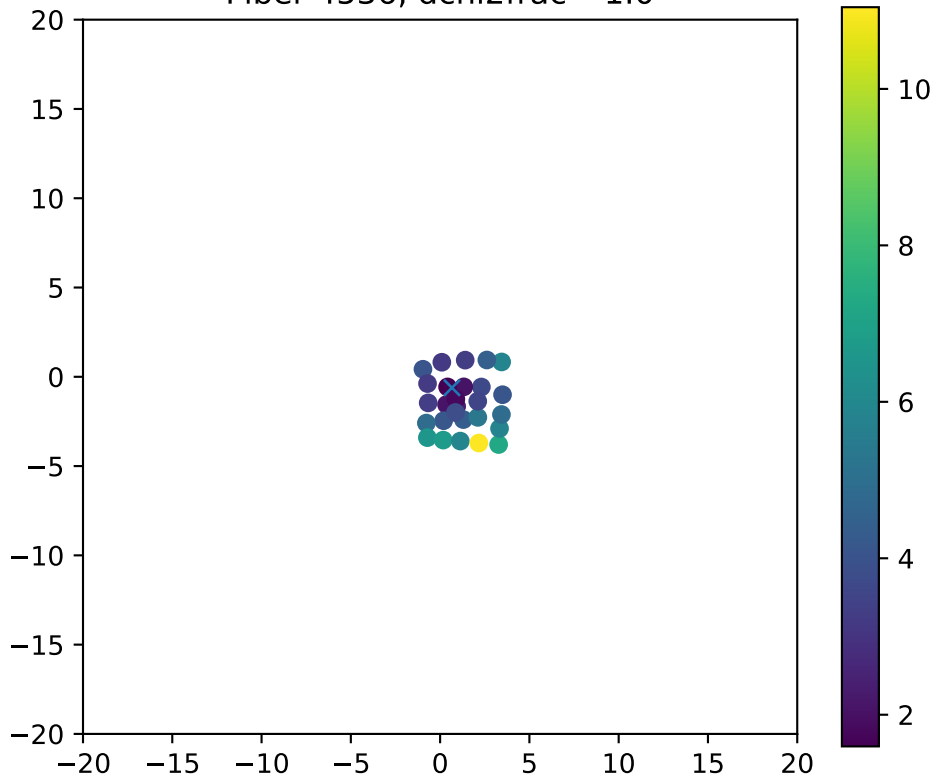
Fiber 4536, dchi2frac= 1.0
