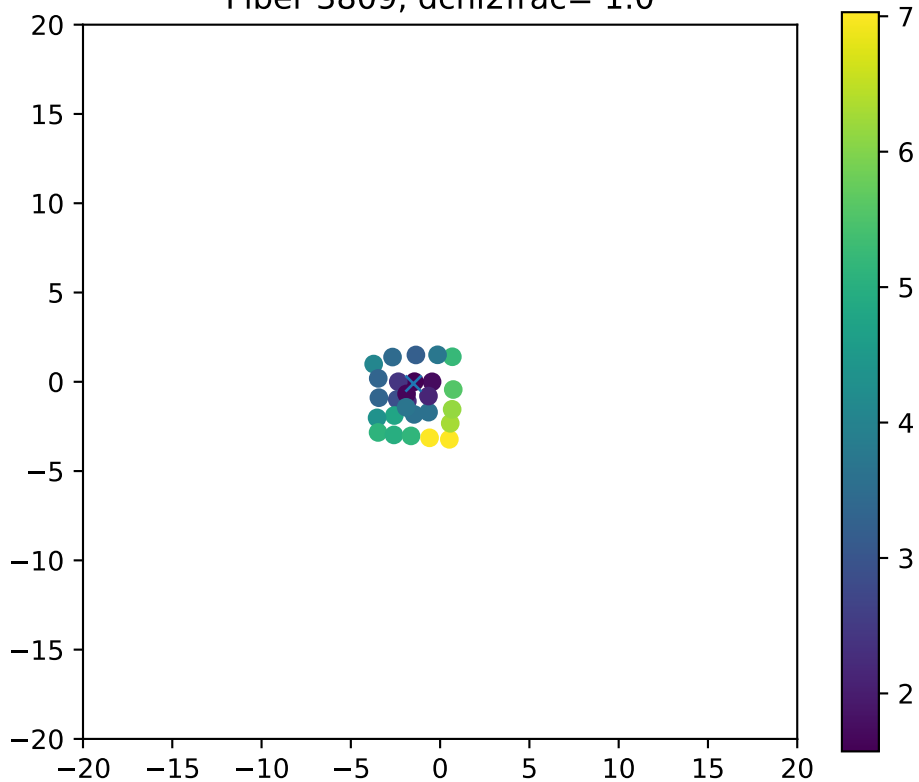
Fiber 3809, dchi2frac= 1.0
