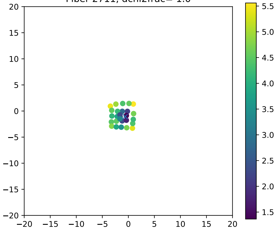
Fiber 2711, dchi2frac= 1.0
