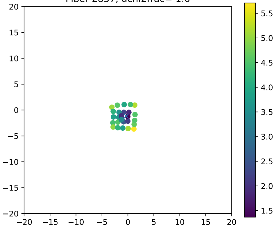
Fiber 2857, dchi2frac= 1.0
