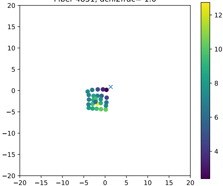
Fiber 4851, dchi2frac= 1.0
