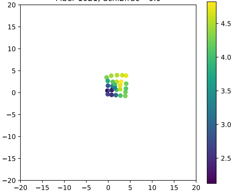
Fiber 1021, dchi2frac= 0.9
