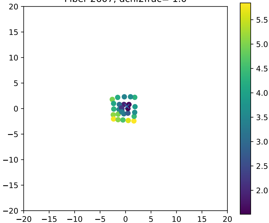
Fiber 2607, dchi2frac= 1.0
