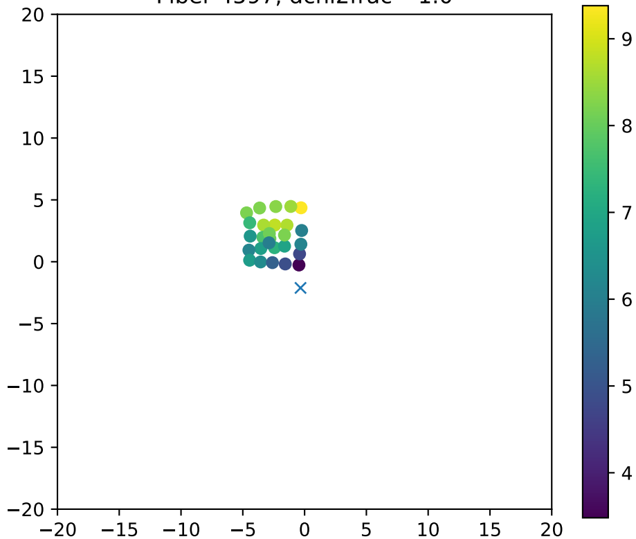
Fiber 4597, dchi2frac= 1.0
