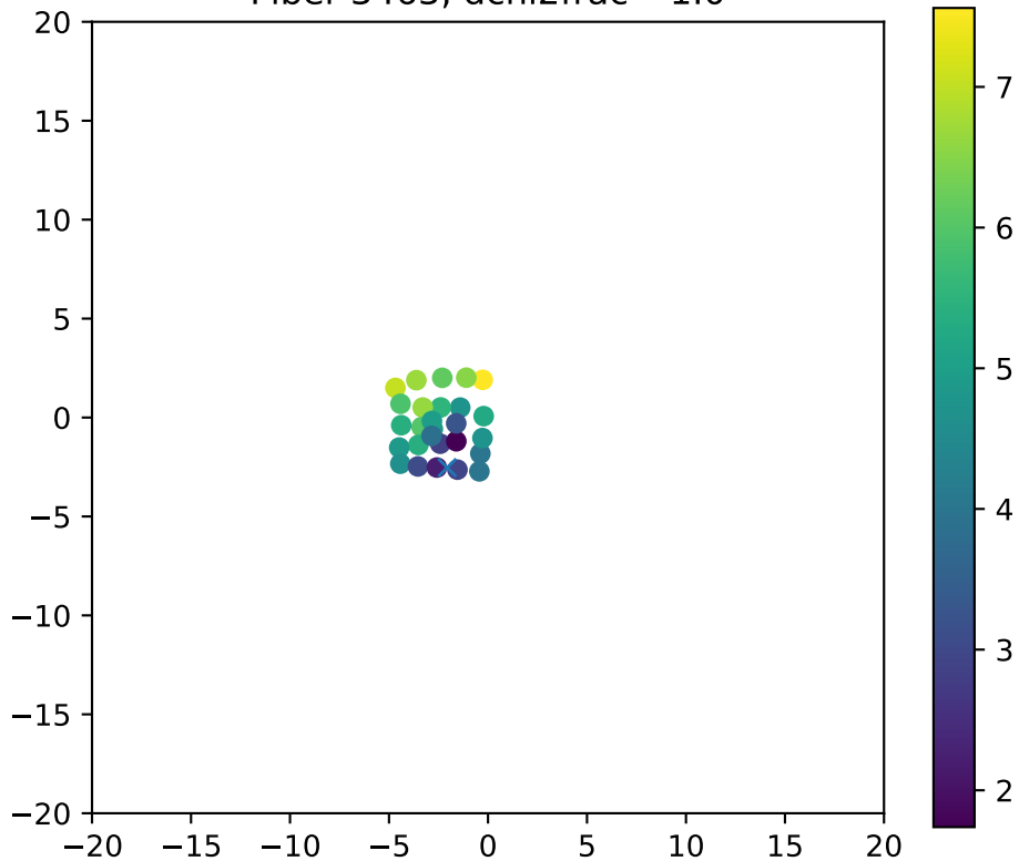
Fiber 3463, dchi2frac= 1.0
