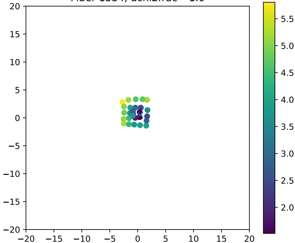
Fiber 1534, dchi2frac= 1.0
