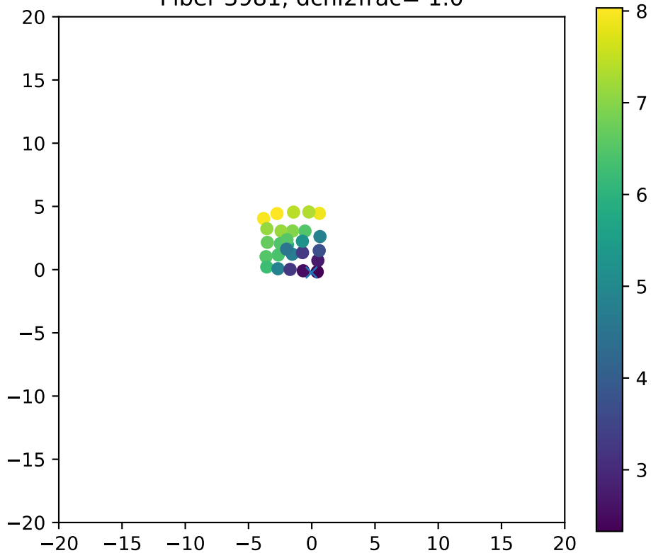
Fiber 3981, dchi2frac= 1.0
