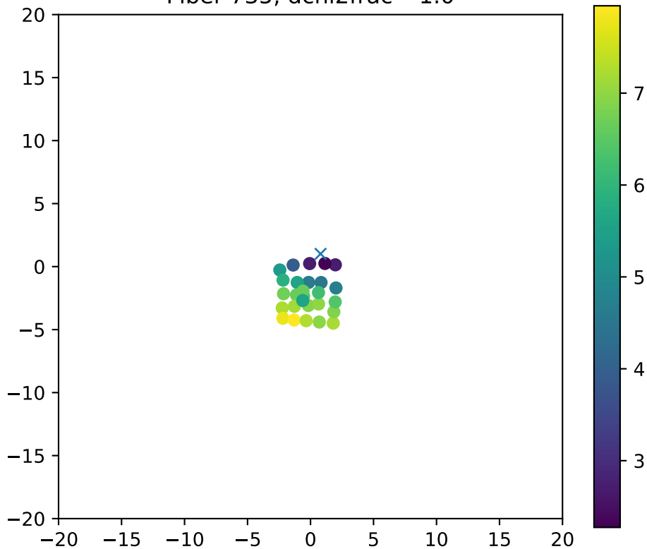
Fiber 735, dchi2frac= 1.0
