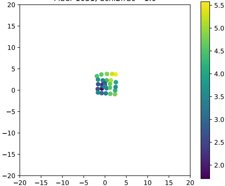
Fiber 1031, dchi2frac= 1.0
