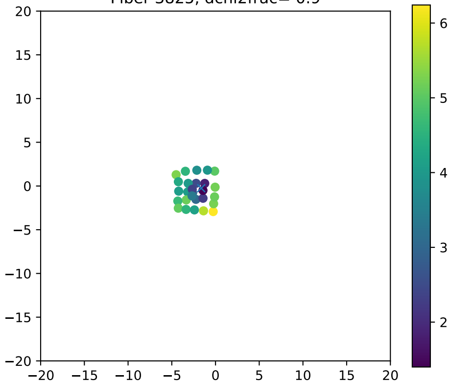
Fiber 3825, dchi2frac= 0.9
