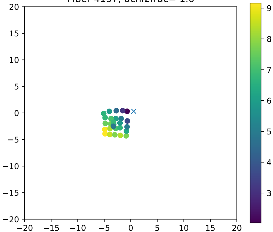
Fiber 4157, dchi2frac= 1.0
