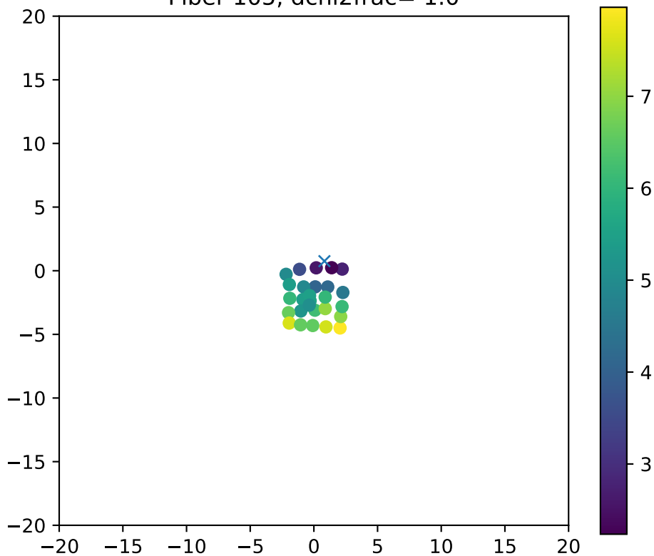
Fiber 105, dchi2frac= 1.0
