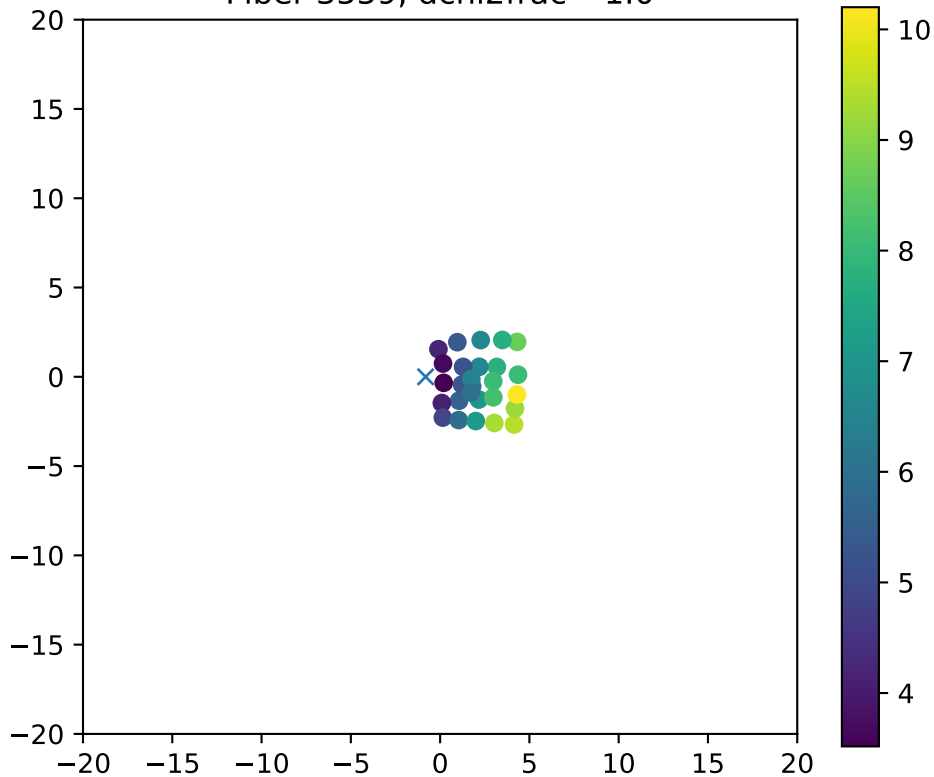
Fiber 3559, dchi2frac= 1.0
