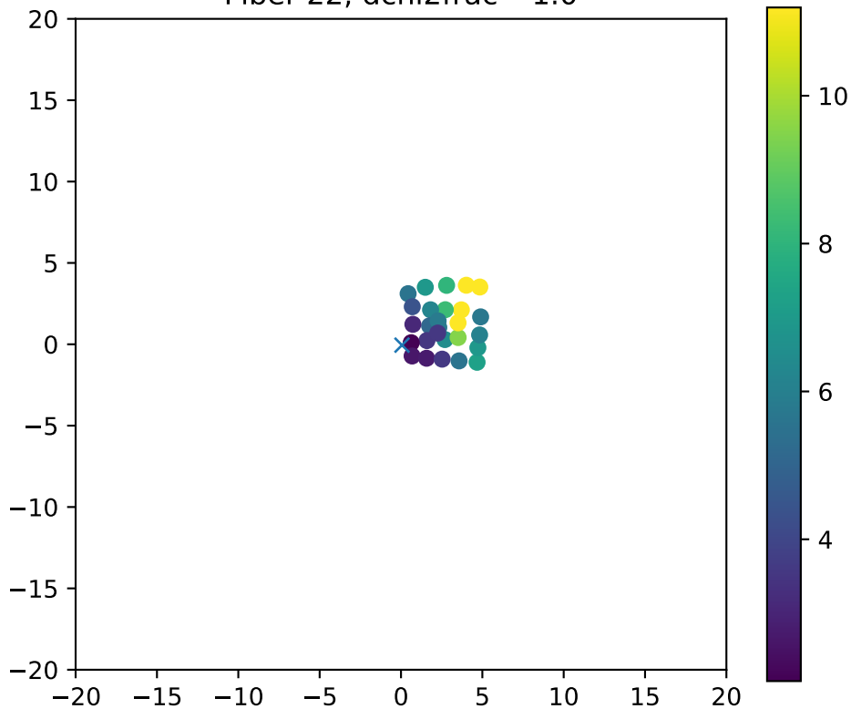
Fiber 22, dchi2frac= 1.0
