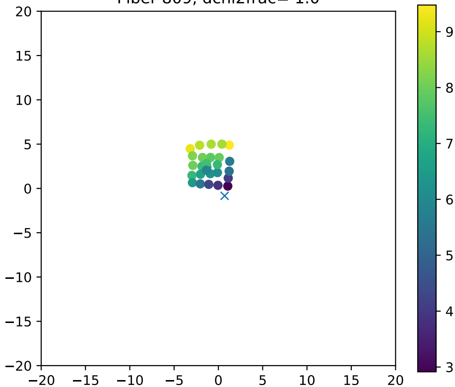
Fiber 809, dchi2frac= 1.0
