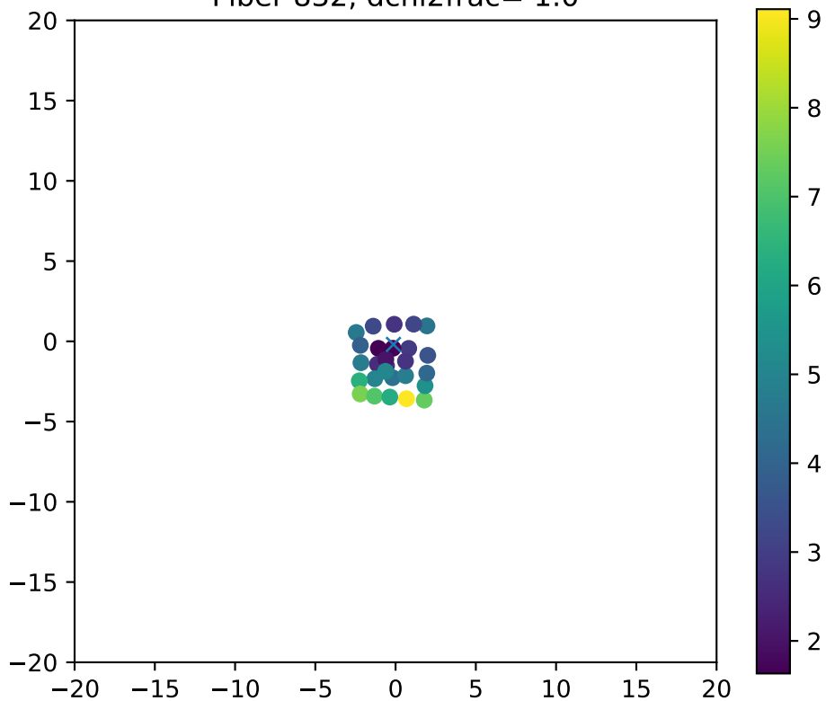
Fiber 832, dchi2frac= 1.0
