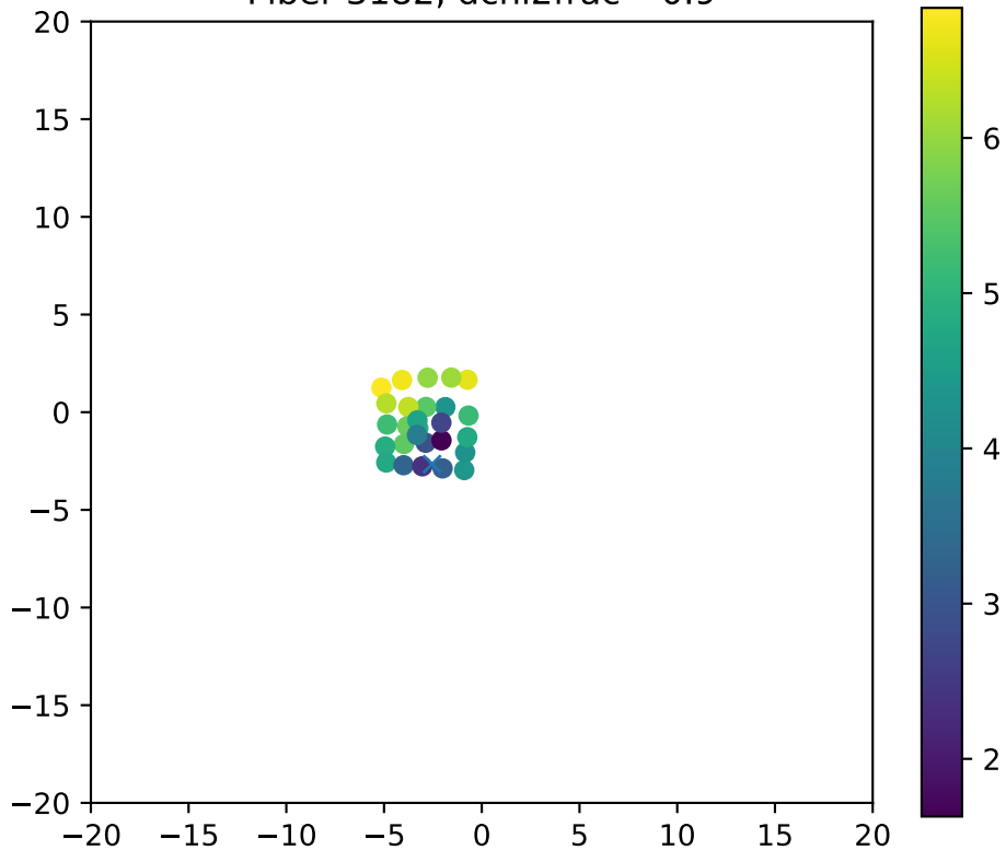
Fiber 3182, dchi2frac= 0.9
