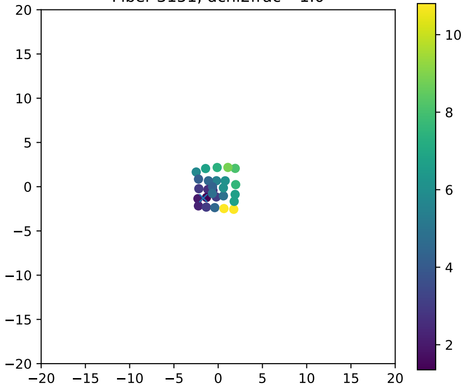
Fiber 3151, dchi2frac= 1.0
