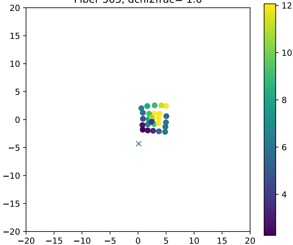
Fiber 503, dchi2frac= 1.0
