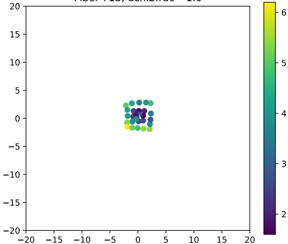
Fiber 713, dchi2frac= 1.0
