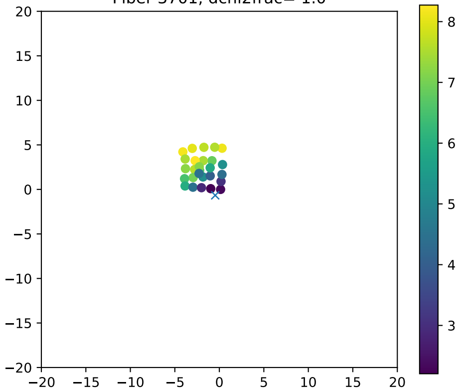
Fiber 3701, dchi2frac= 1.0
