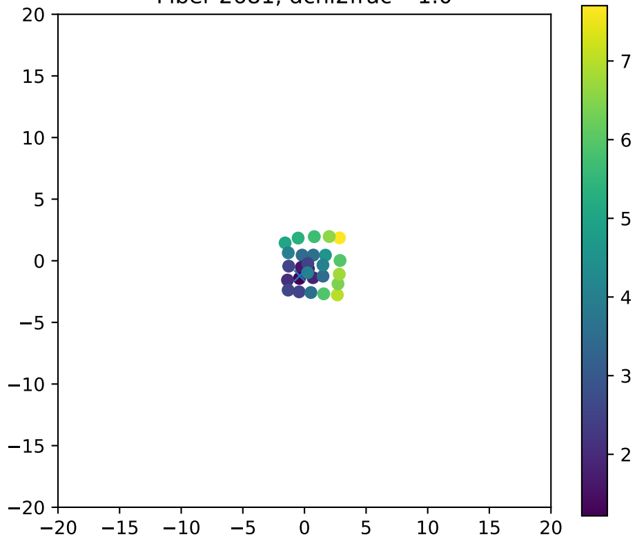
Fiber 2681, dchi2frac= 1.0
