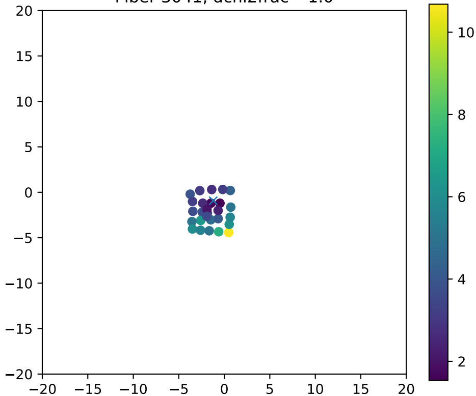
Fiber 3041, dchi2frac= 1.0
