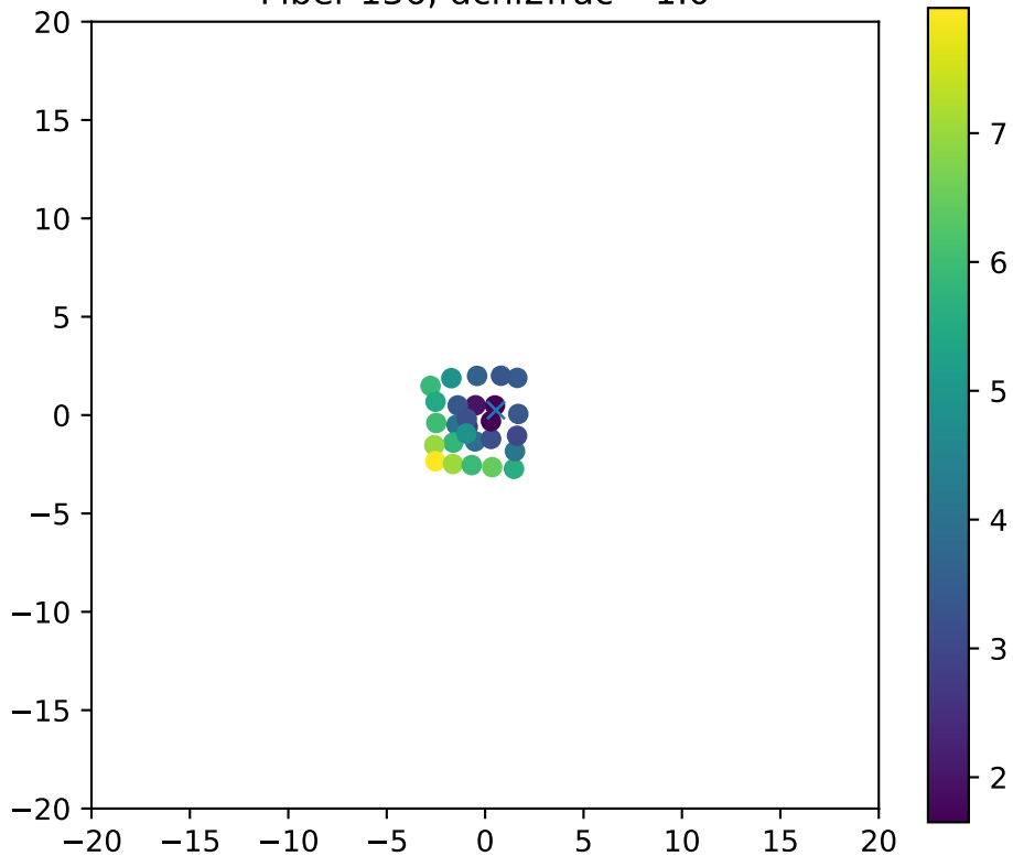
Fiber 136, dchi2frac= 1.0
