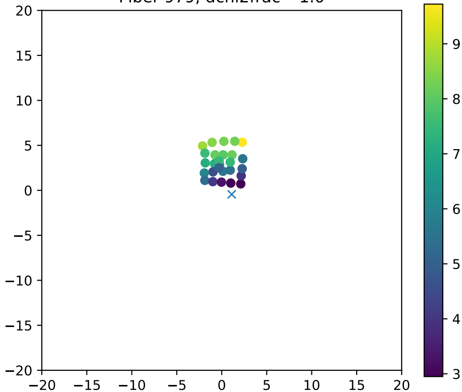
Fiber 979, dchi2frac= 1.0
