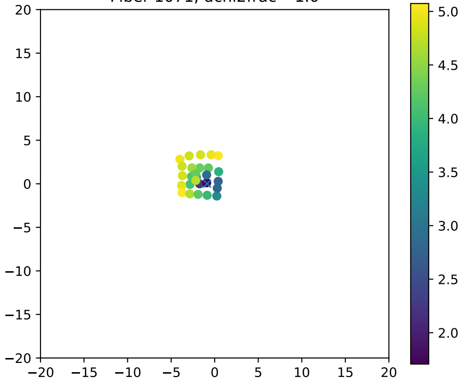
Fiber 1071, dchi2frac= 1.0
