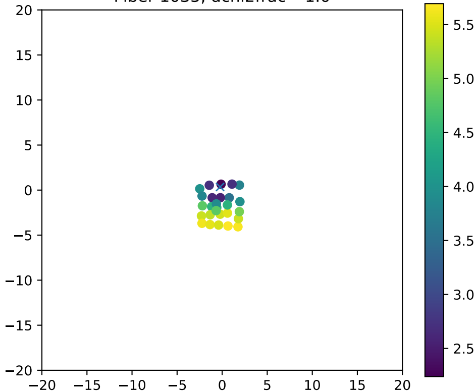
Fiber 1035, dchi2frac= 1.0
