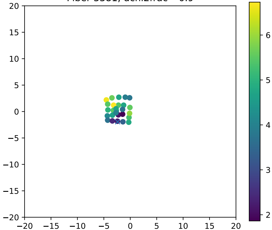
Fiber 3381, dchi2frac= 0.9
