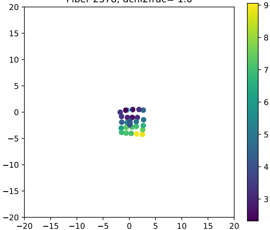
Fiber 2378, dchi2frac= 1.0
