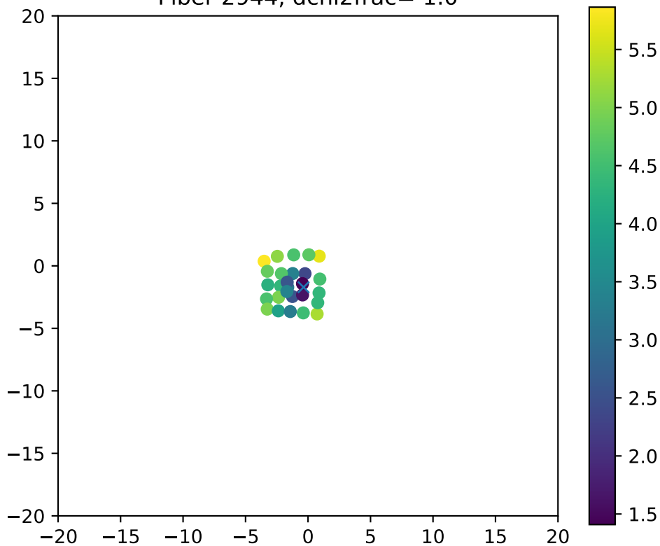
Fiber 2944, dchi2frac= 1.0
