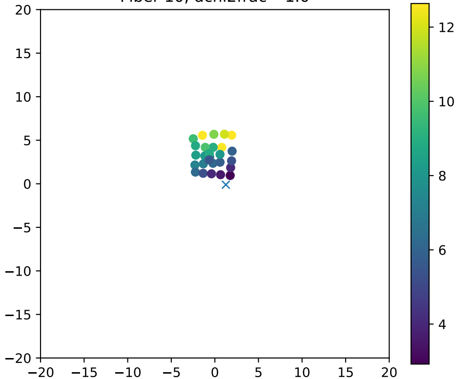
Fiber 10, dchi2frac= 1.0
