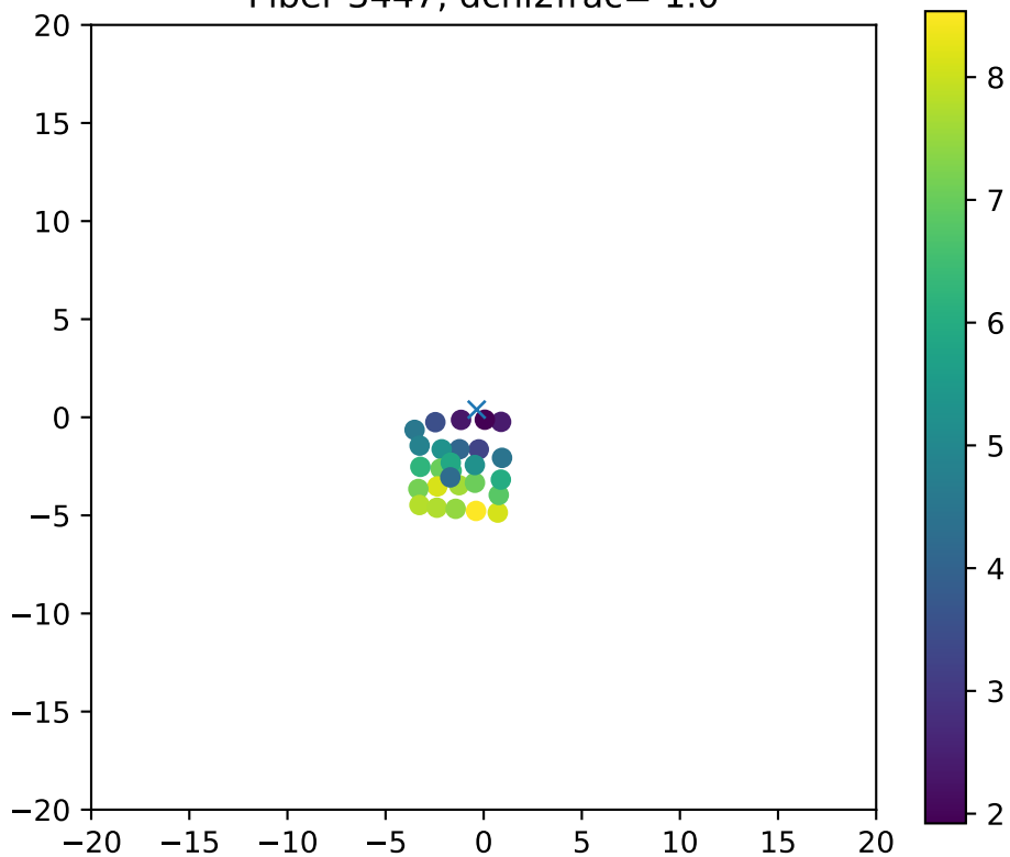
Fiber 3447, dchi2frac= 1.0
