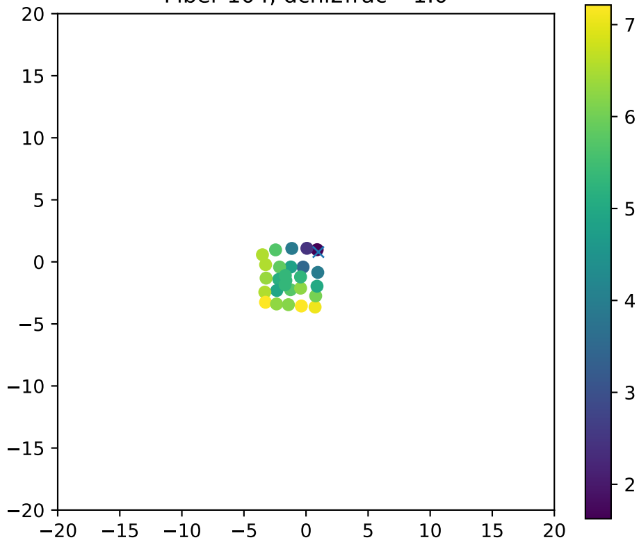
Fiber 104, dchi2frac= 1.0
