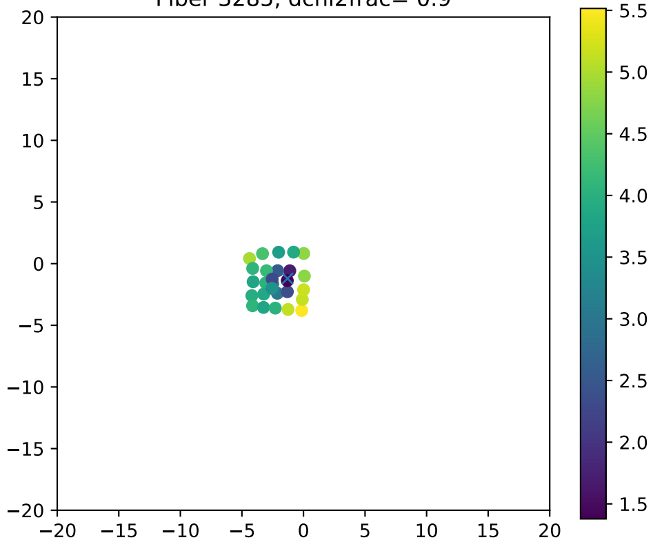
Fiber 3285, dchi2frac= 0.9
