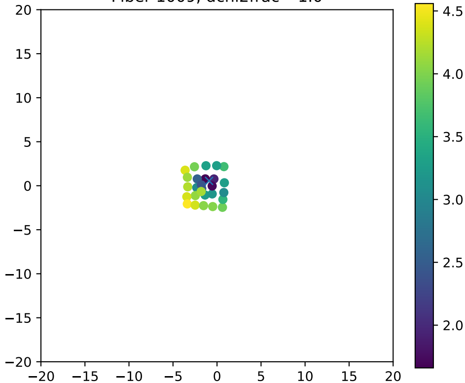
Fiber 1009, dchi2frac= 1.0
