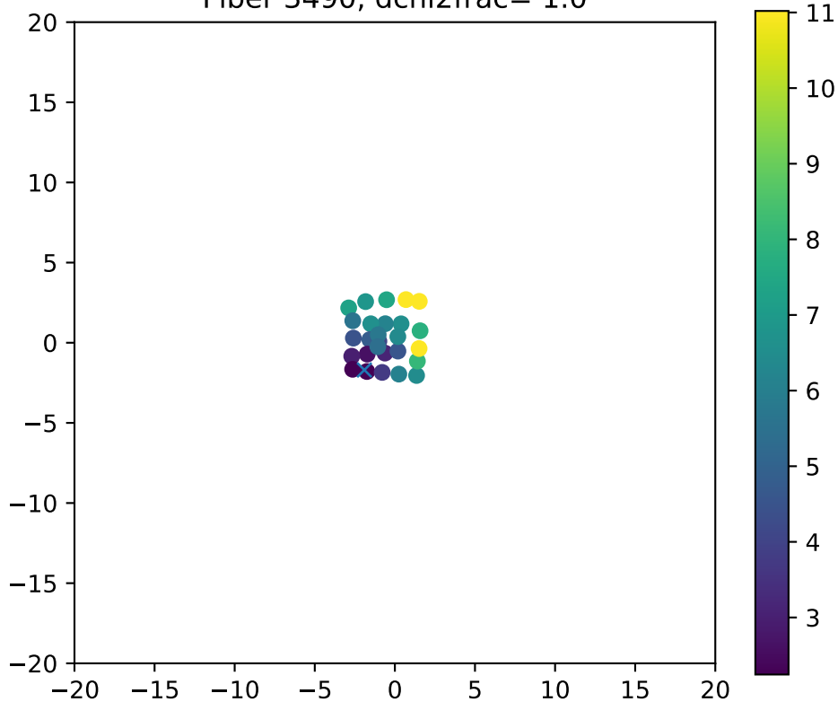
Fiber 3490, dchi2frac= 1.0
