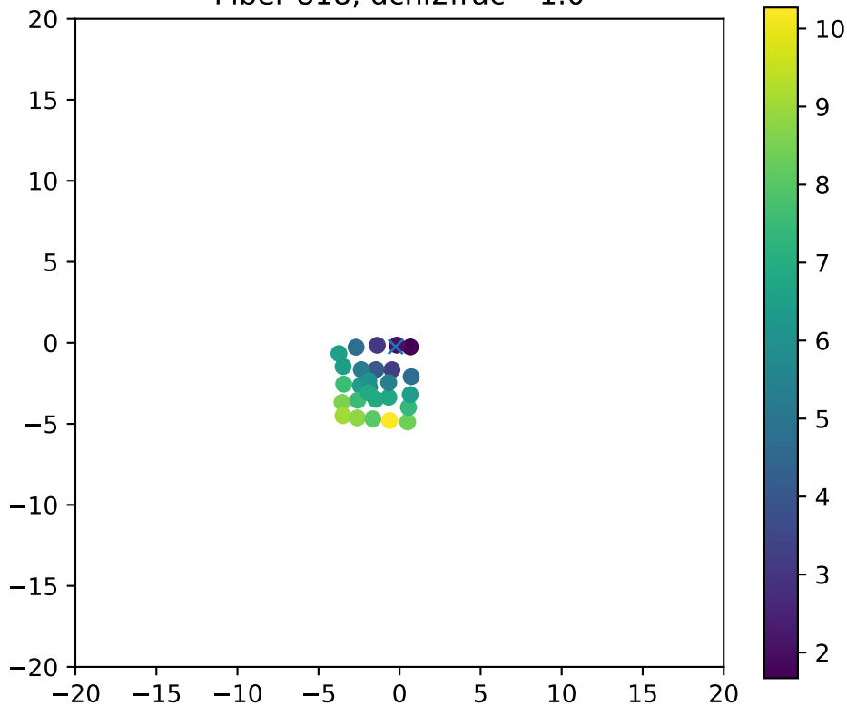
Fiber 818, dchi2frac= 1.0
