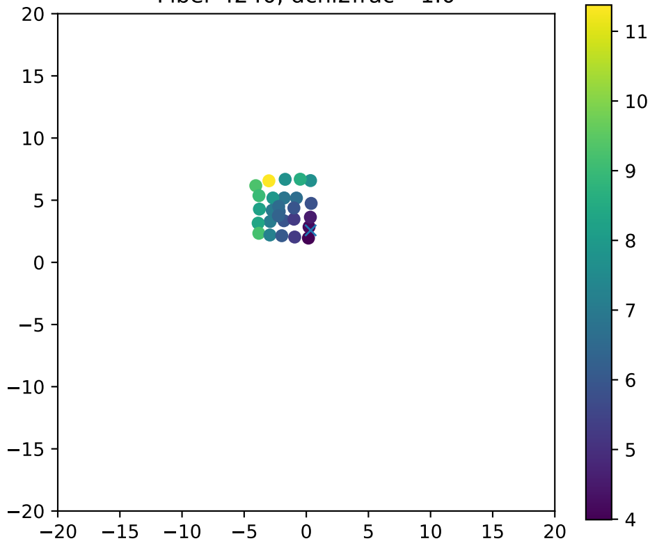
Fiber 4240, dchi2frac= 1.0
