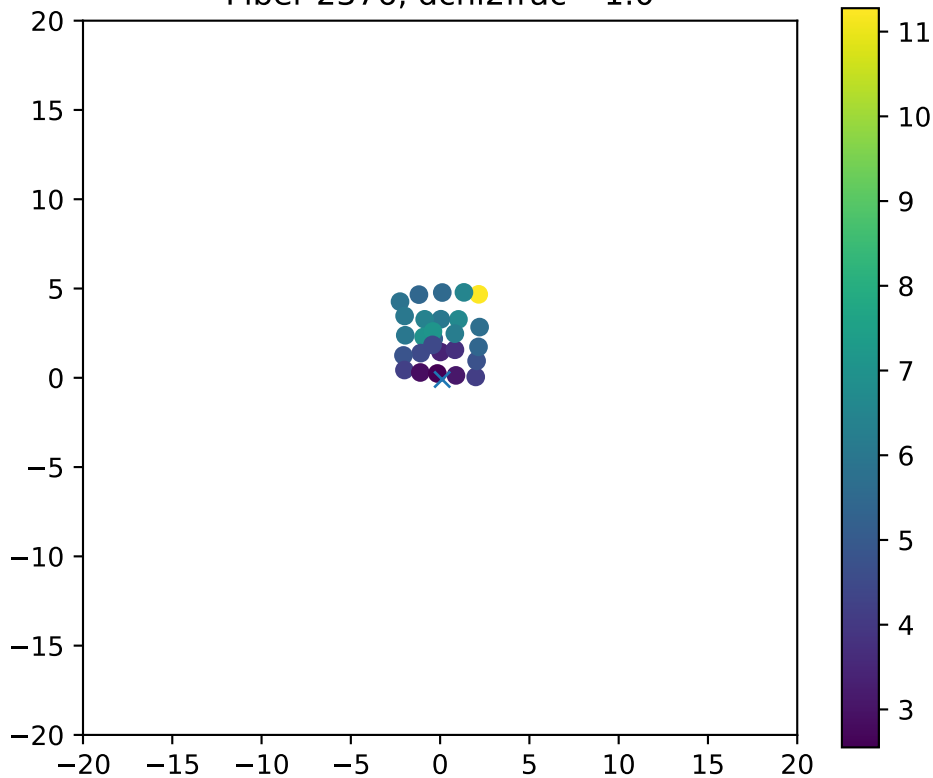
Fiber 2376, dchi2frac= 1.0
