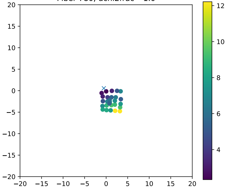
Fiber 780, dchi2frac= 1.0
