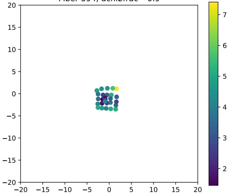
Fiber 594, dchi2frac= 0.9
