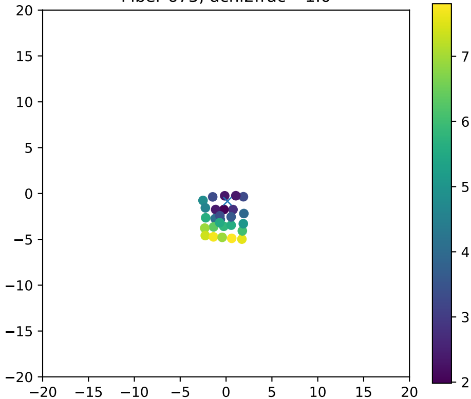
Fiber 675, dchi2frac= 1.0
