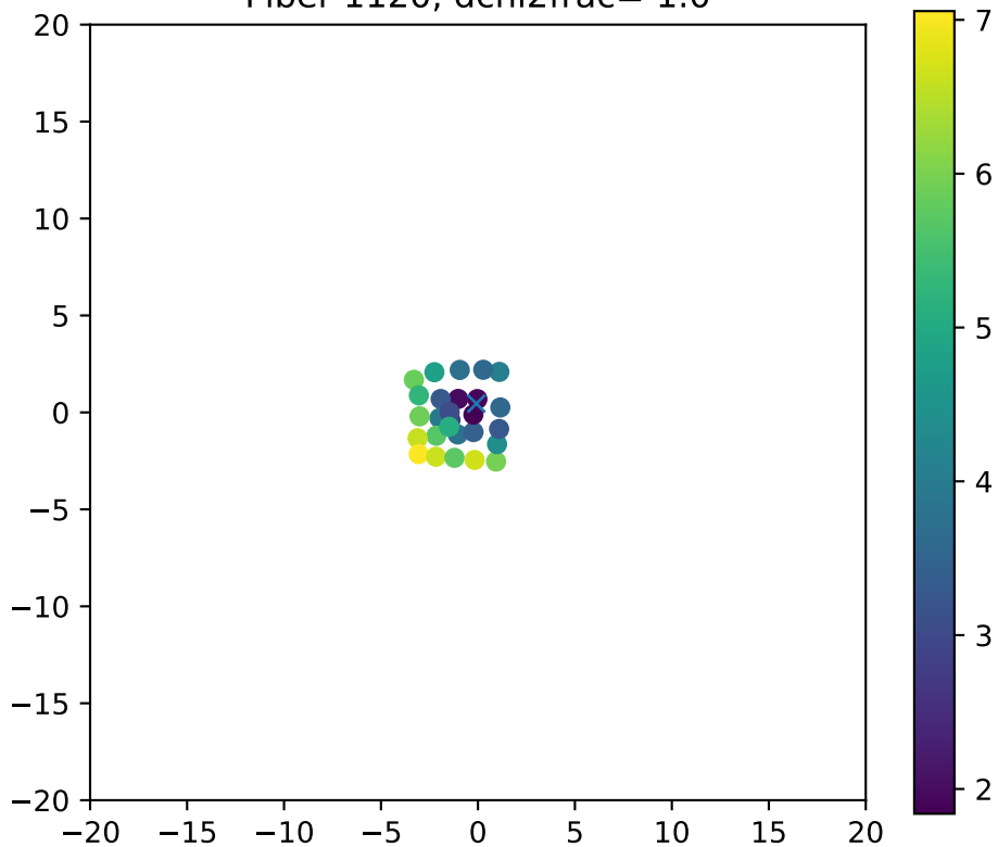
Fiber 1120, dchi2frac= 1.0
