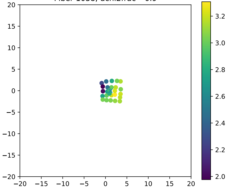
Fiber 1038, dchi2frac= 0.9
