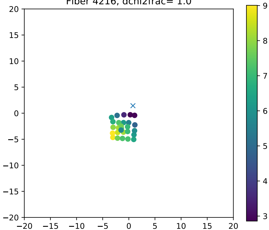
Fiber 4216, dchi2frac= 1.0
