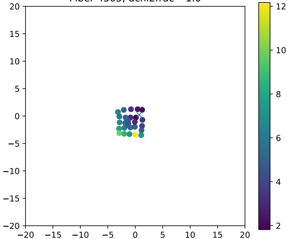
Fiber 4505, dchi2frac= 1.0
