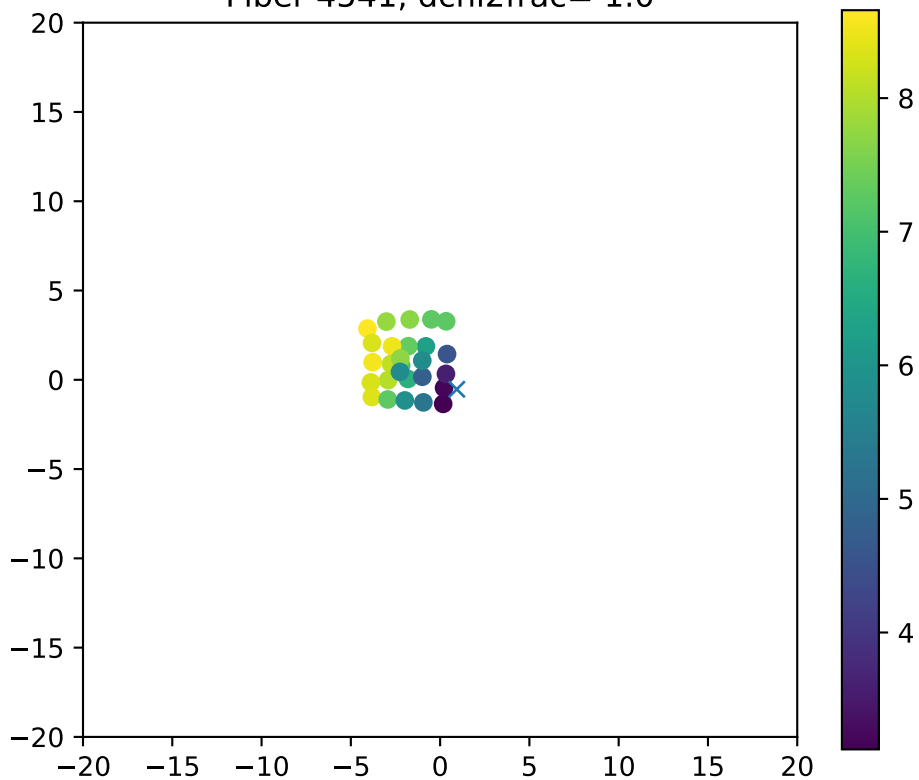
Fiber 4541, dchi2frac= 1.0
