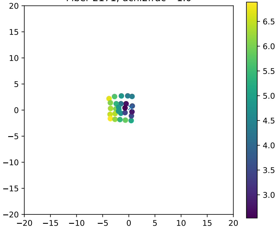
Fiber 2171, dchi2frac= 1.0
