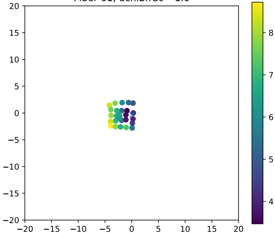
Fiber 61, dchi2frac= 1.0
