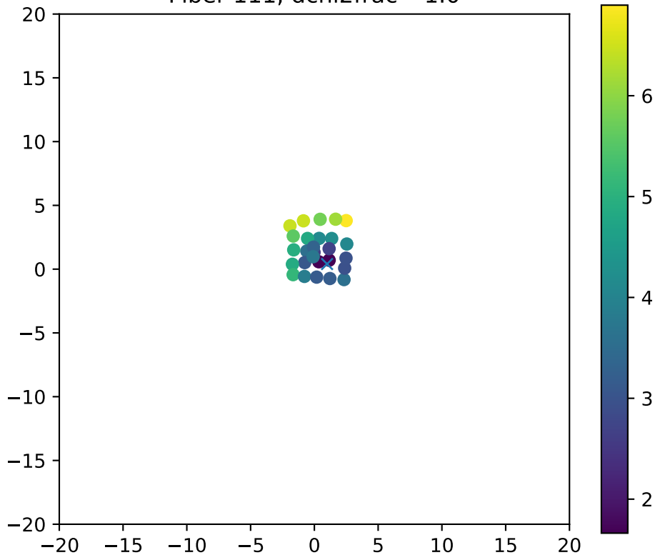
Fiber 111, dchi2frac= 1.0
