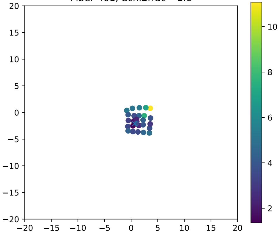
Fiber 461, dchi2frac= 1.0
