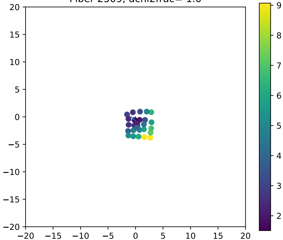
Fiber 2509, dchi2frac= 1.0
