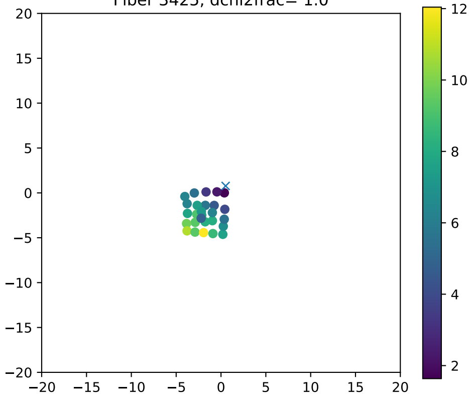
Fiber 3425, dchi2frac= 1.0
