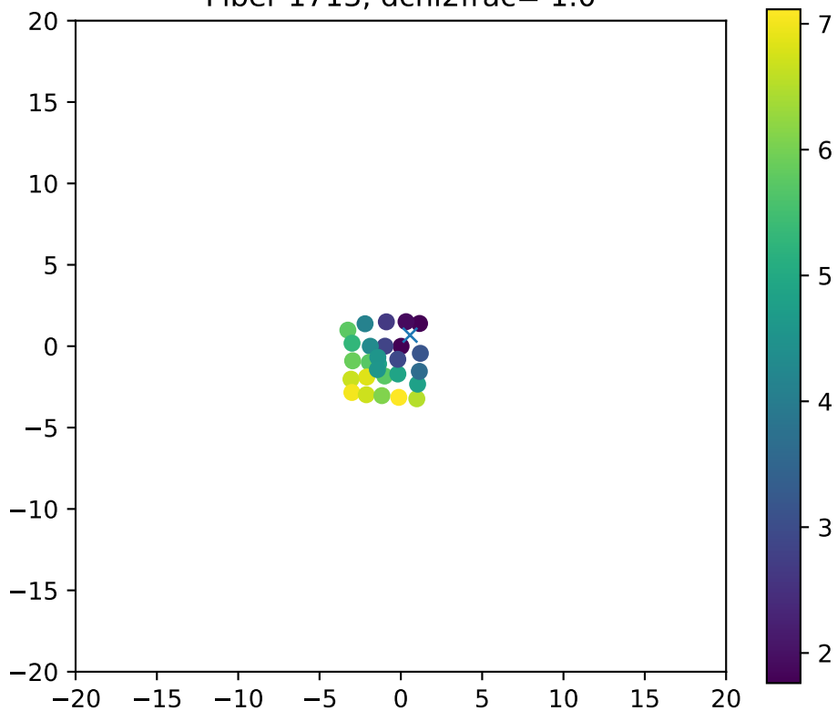
Fiber 1713, dchi2frac= 1.0
