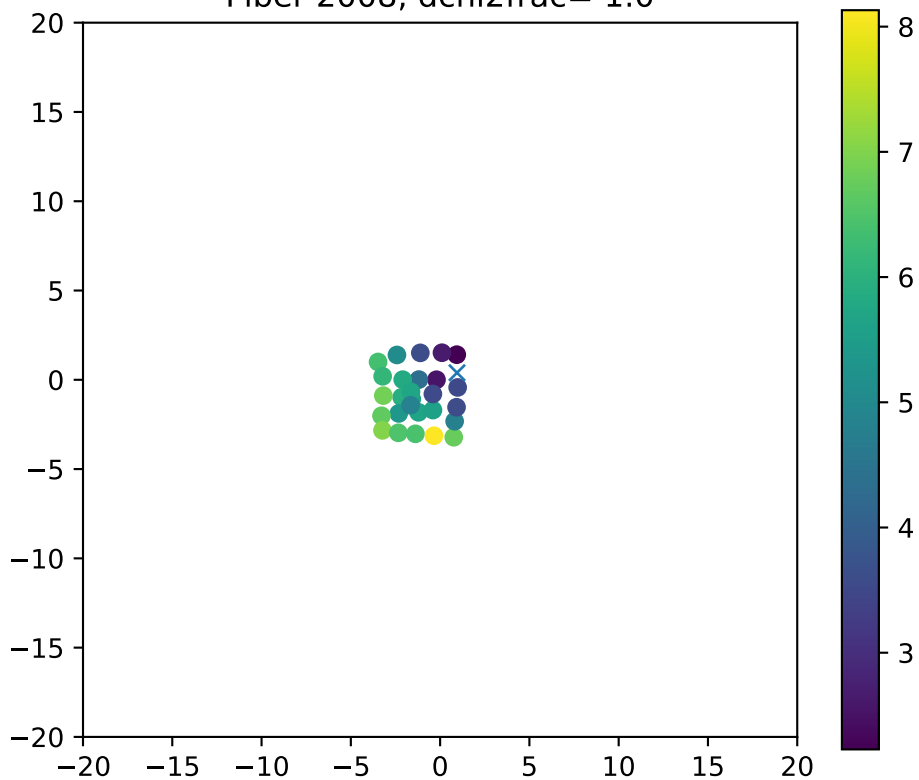
Fiber 2008, dchi2frac= 1.0
