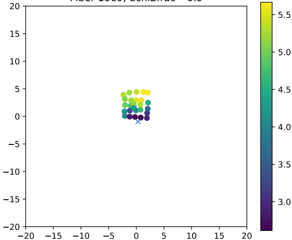
Fiber 1069, dchi2frac= 0.9
