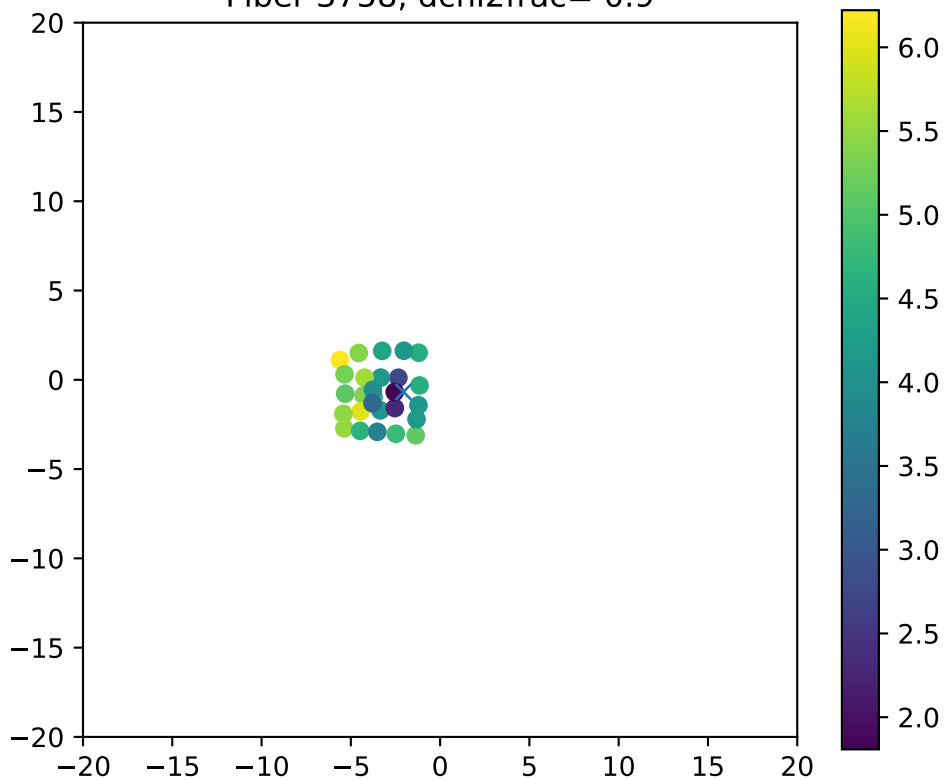
Fiber 3758, dchi2frac= 0.9
