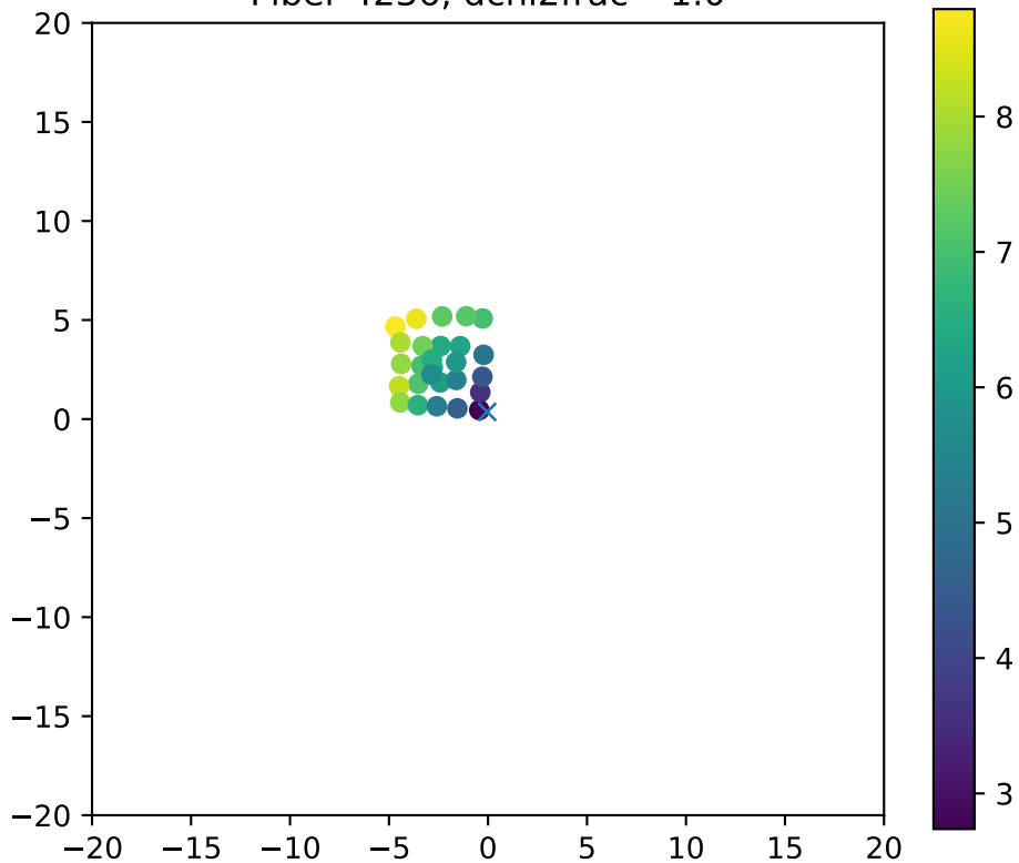
Fiber 4236, dchi2frac= 1.0
