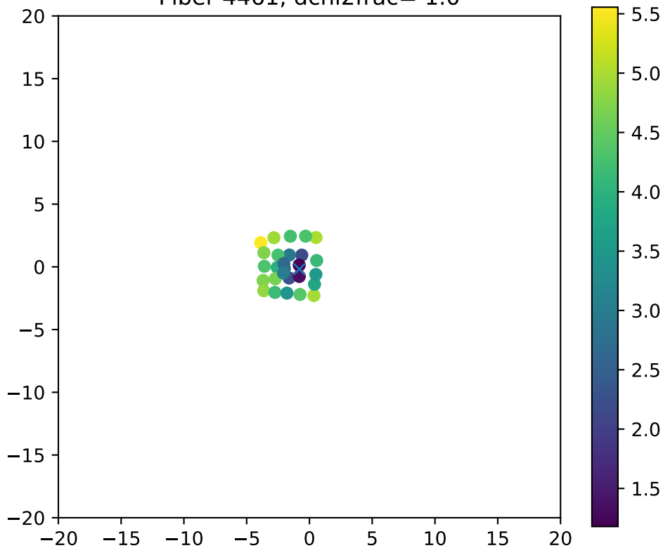
Fiber 4461, dchi2frac= 1.0
