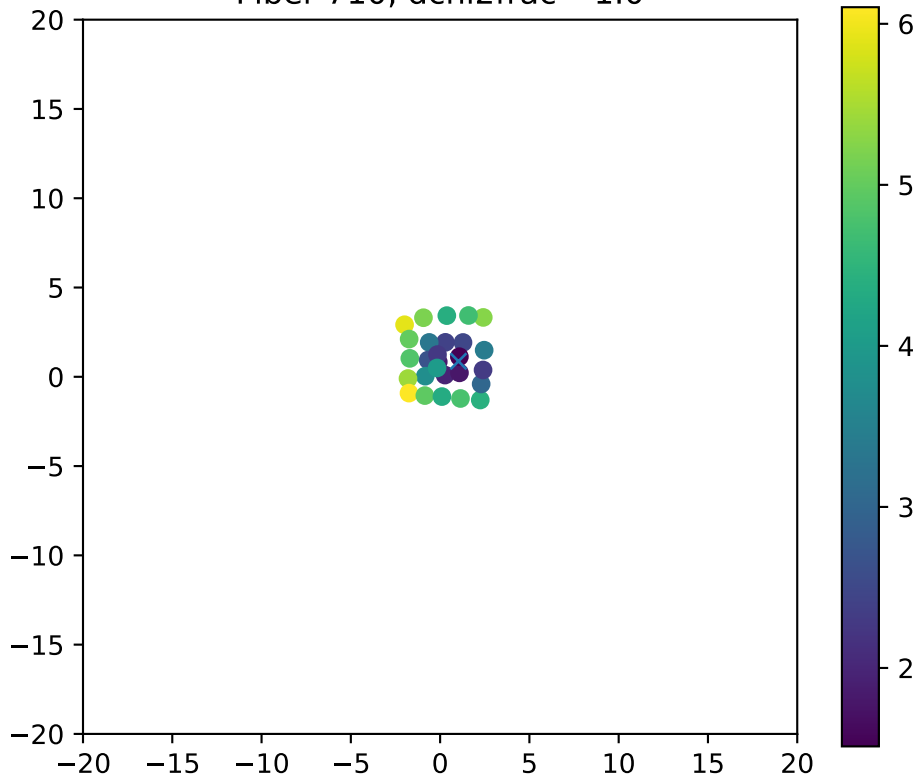
Fiber 710, dchi2frac= 1.0
