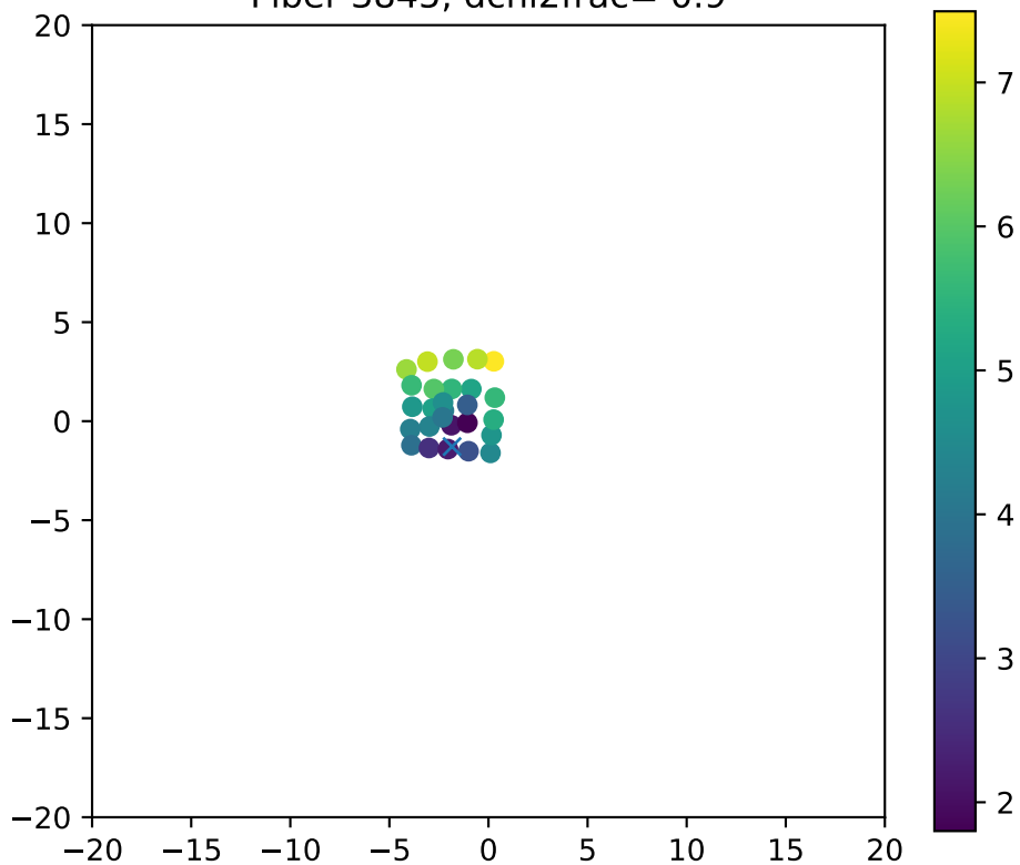
Fiber 3845, dchi2frac= 0.9
