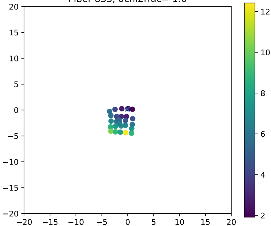
Fiber 833, dchi2frac= 1.0
