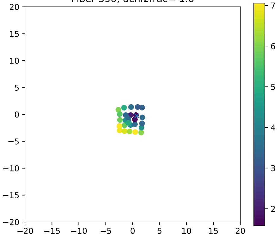
Fiber 390, dchi2frac= 1.0
