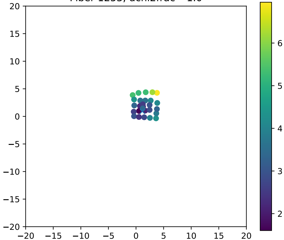
Fiber 1253, dchi2frac= 1.0
