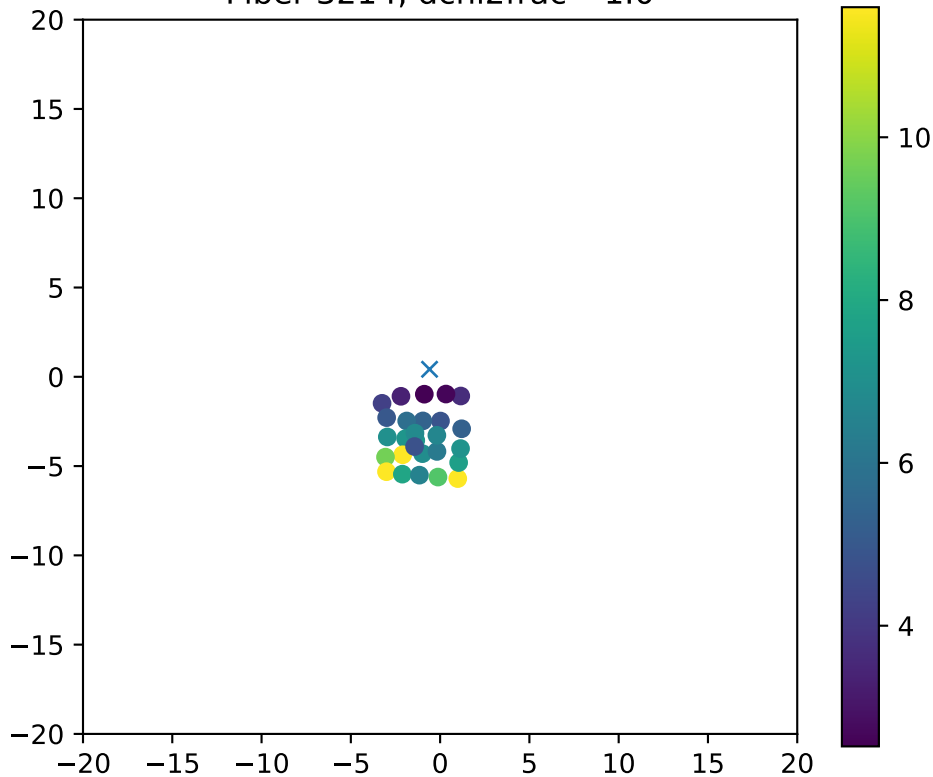
Fiber 3214, dchi2frac= 1.0
