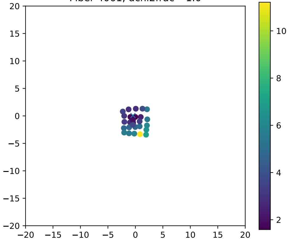
Fiber 4061, dchi2frac= 1.0
