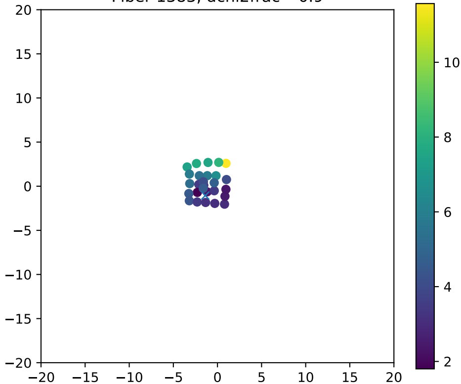
Fiber 1383, dchi2frac= 0.9
