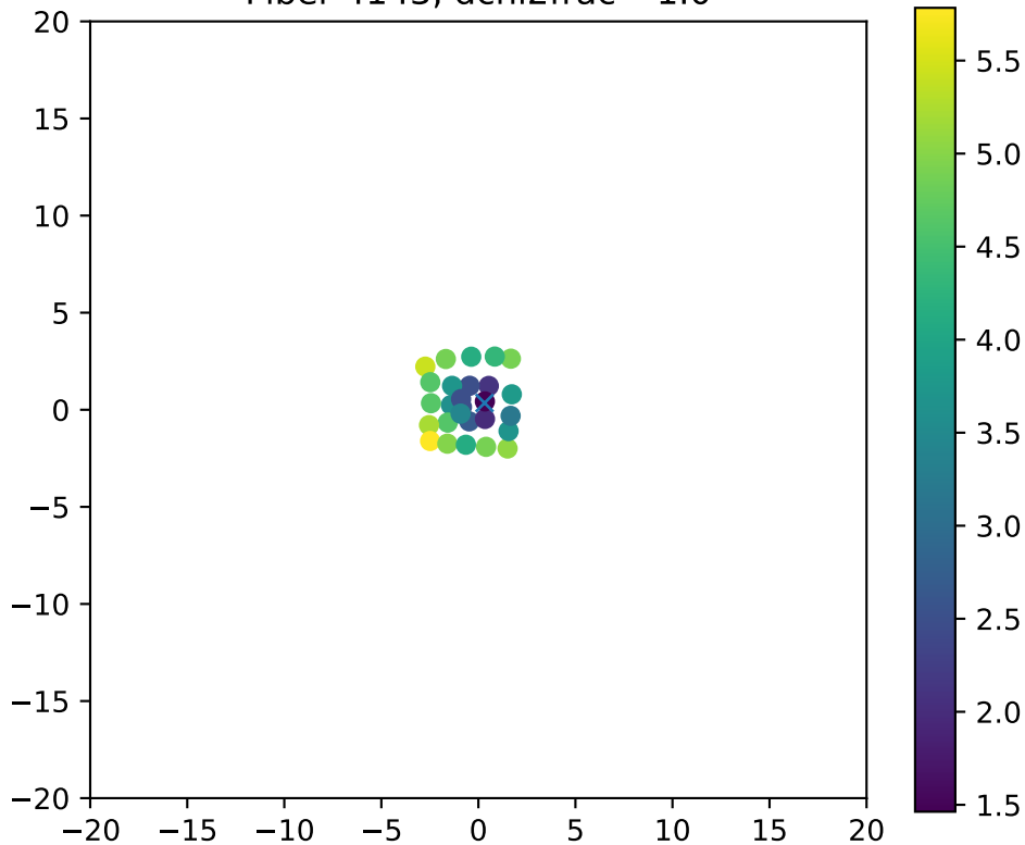
Fiber 4143, dchi2frac= 1.0
