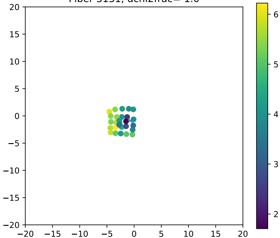
Fiber 3131, dchi2frac= 1.0
