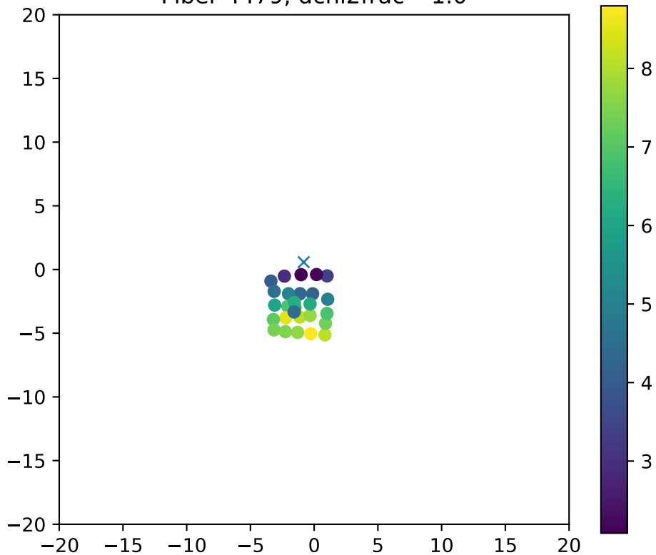
Fiber 4479, dchi2frac= 1.0
