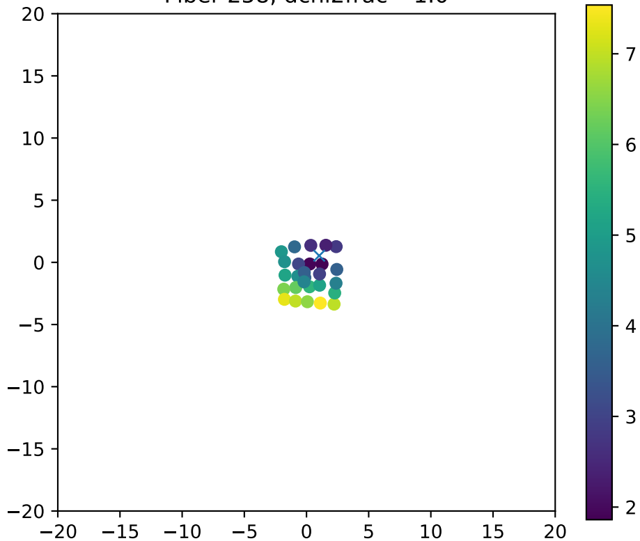
Fiber 258, dchi2frac= 1.0
