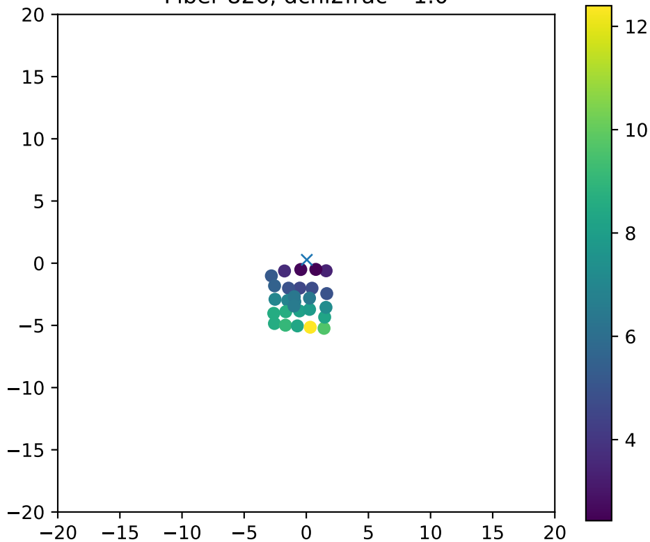
Fiber 826, dchi2frac= 1.0
