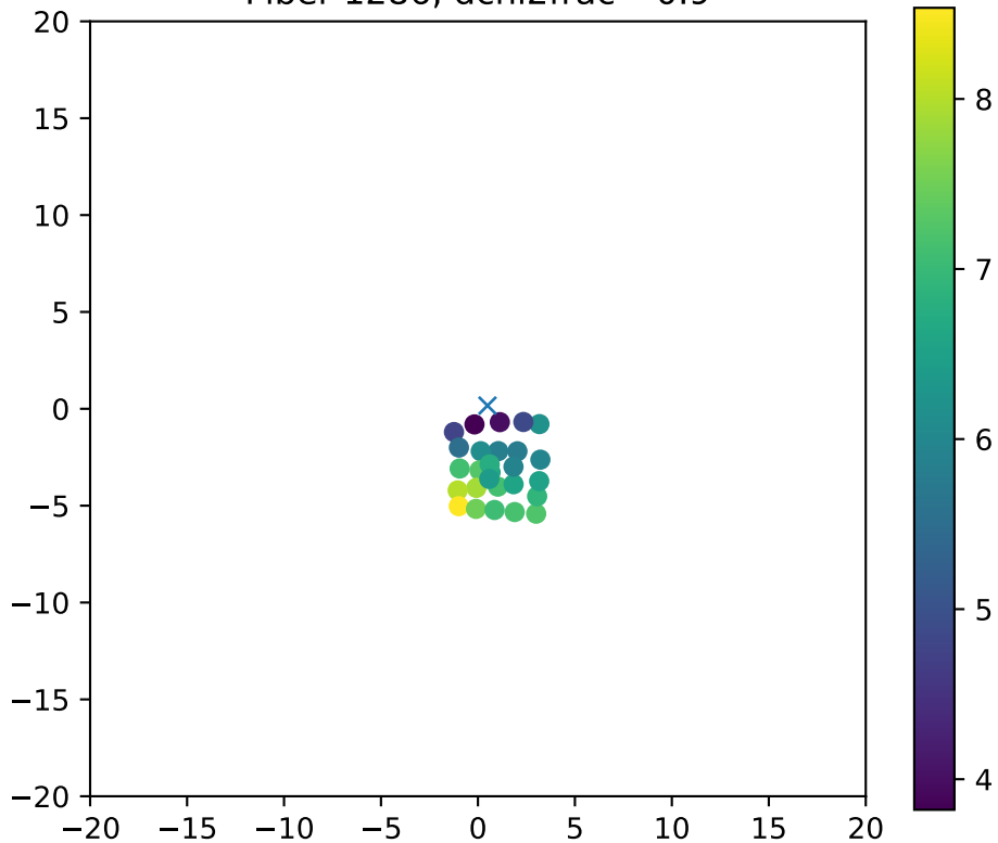
Fiber 1286, dchi2frac= 0.9
