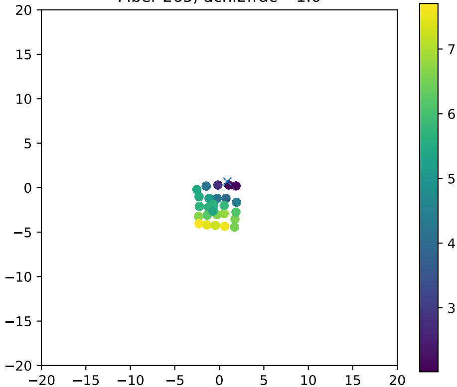
Fiber 265, dchi2frac= 1.0
