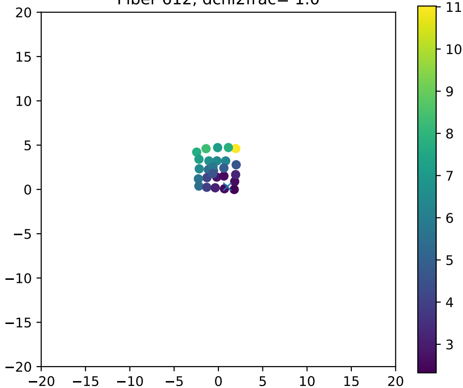
Fiber 612, dchi2frac= 1.0
