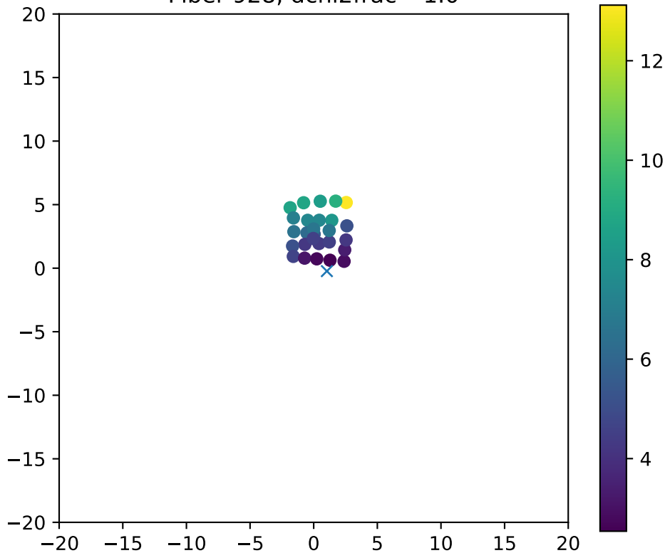
Fiber 928, dchi2frac= 1.0
