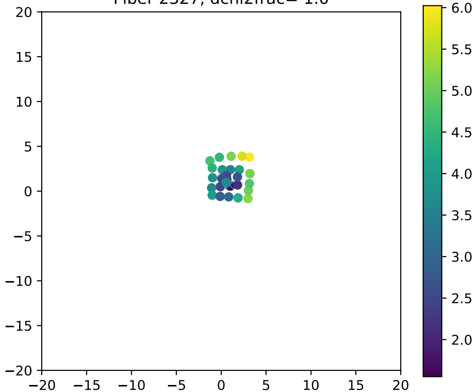
Fiber 2327, dchi2frac= 1.0
