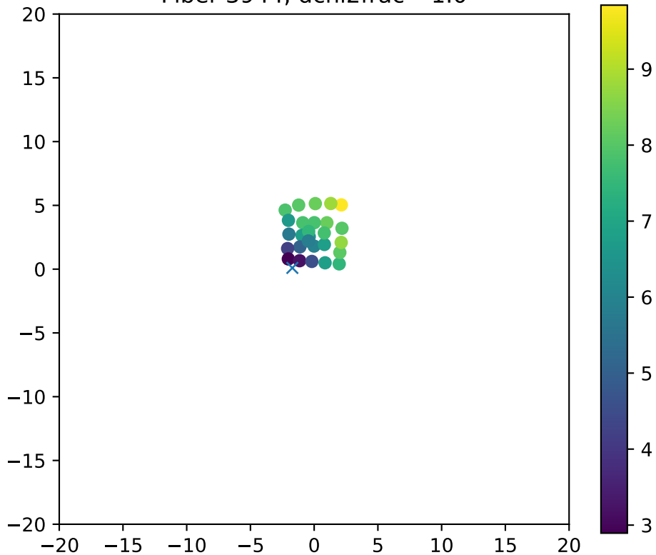
Fiber 3944, dchi2frac= 1.0
