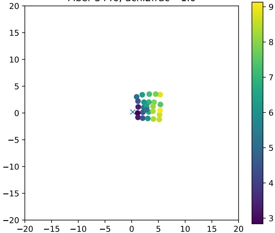
Fiber 3446, dchi2frac= 1.0
