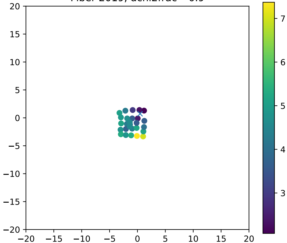
Fiber 2019, dchi2frac= 0.9
