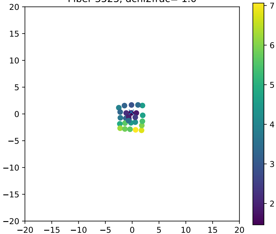
Fiber 3523, dchi2frac= 1.0
