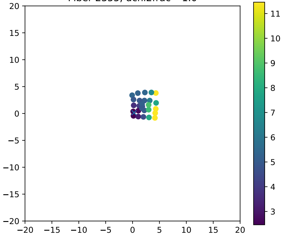
Fiber 2355, dchi2frac= 1.0
