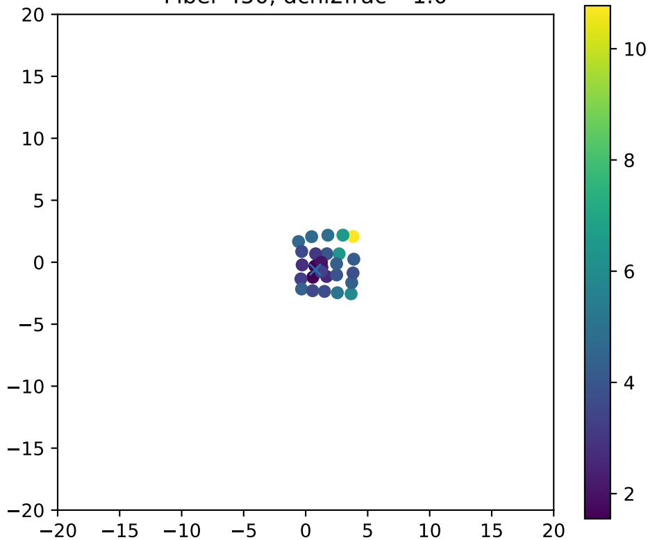
Fiber 450, dchi2frac= 1.0
