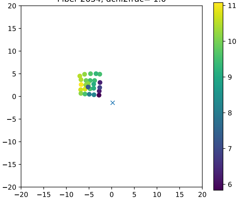
Fiber 2634, dchi2frac= 1.0
