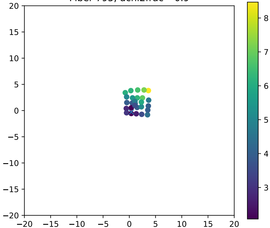
Fiber 795, dchi2frac= 0.9
