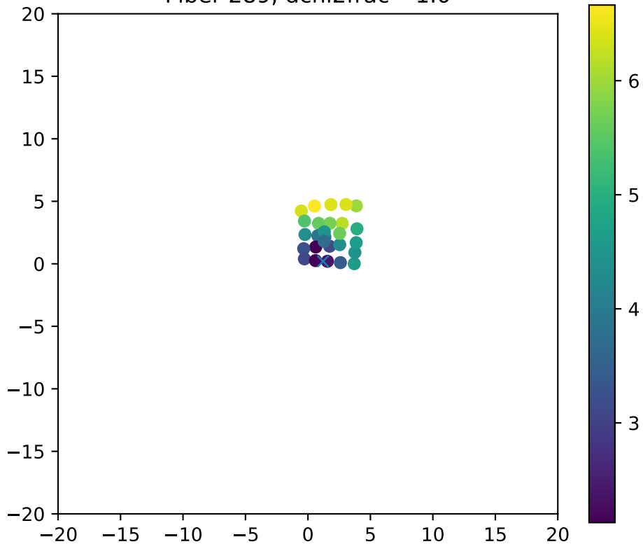
Fiber 289, dchi2frac= 1.0
