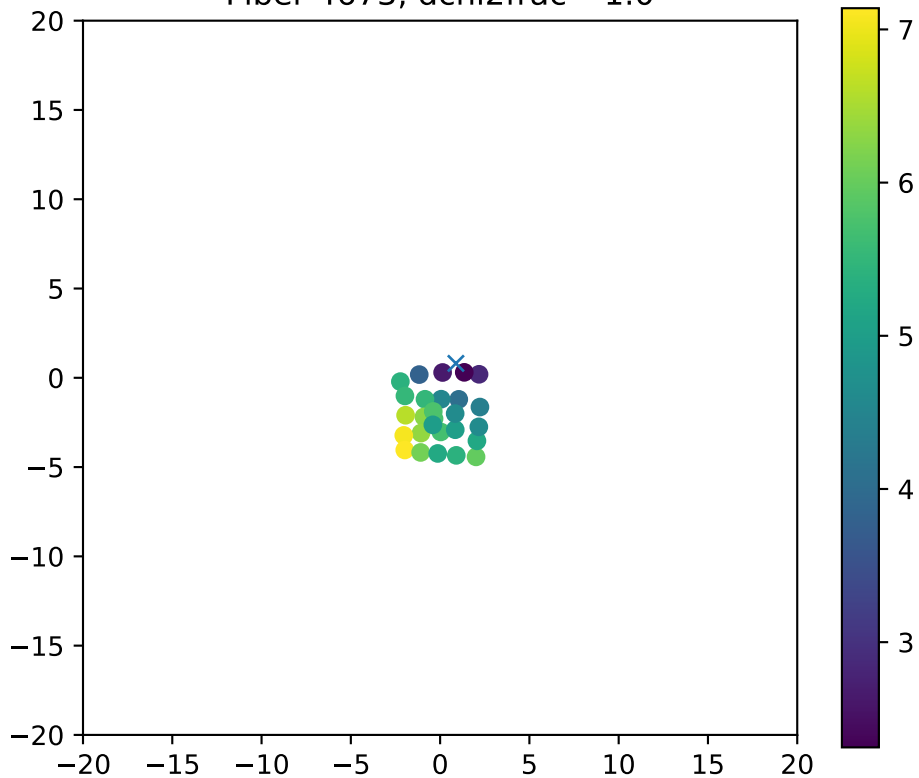
Fiber 4673, dchi2frac= 1.0
