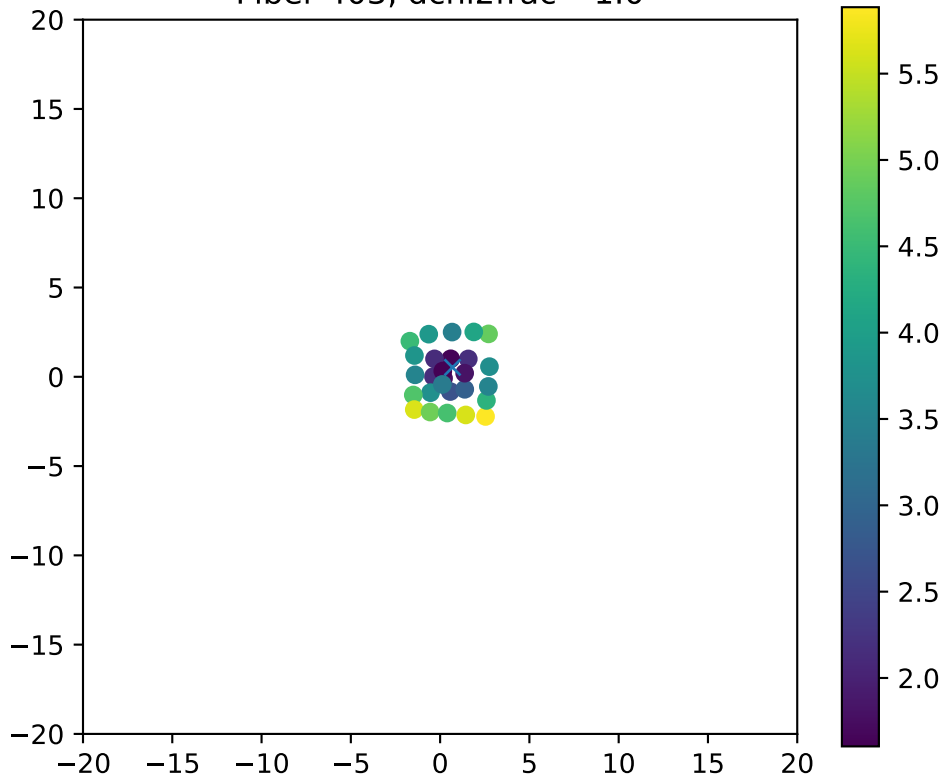
Fiber 403, dchi2frac= 1.0
