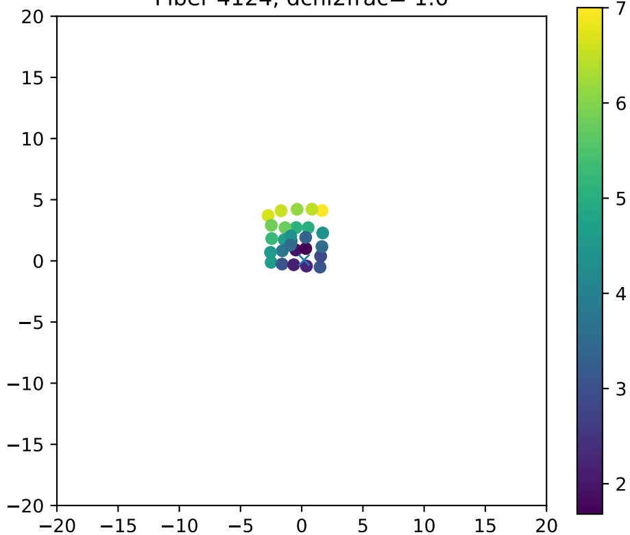
Fiber 4124, dchi2frac= 1.0
