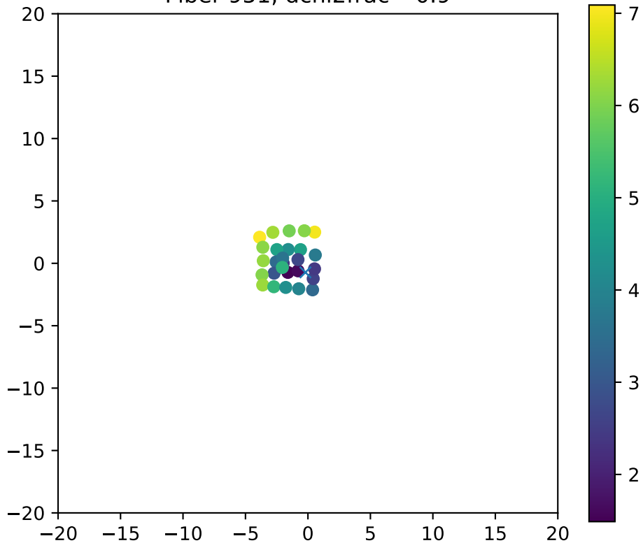
Fiber 951, dchi2frac= 0.9
