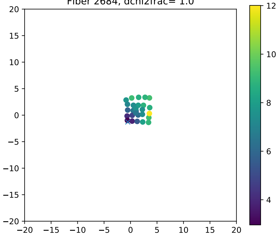
Fiber 2684, dchi2frac= 1.0
