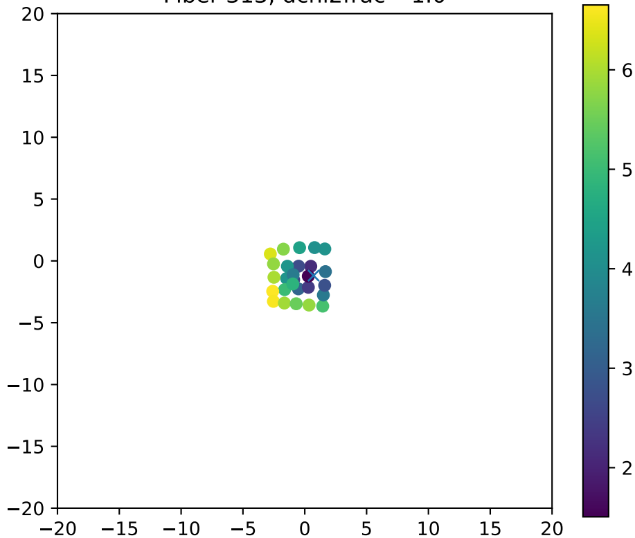
Fiber 313, dchi2frac= 1.0
