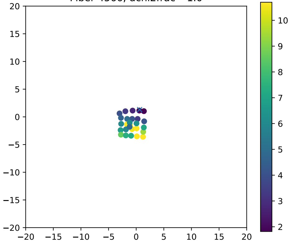
Fiber 4566, dchi2frac= 1.0
