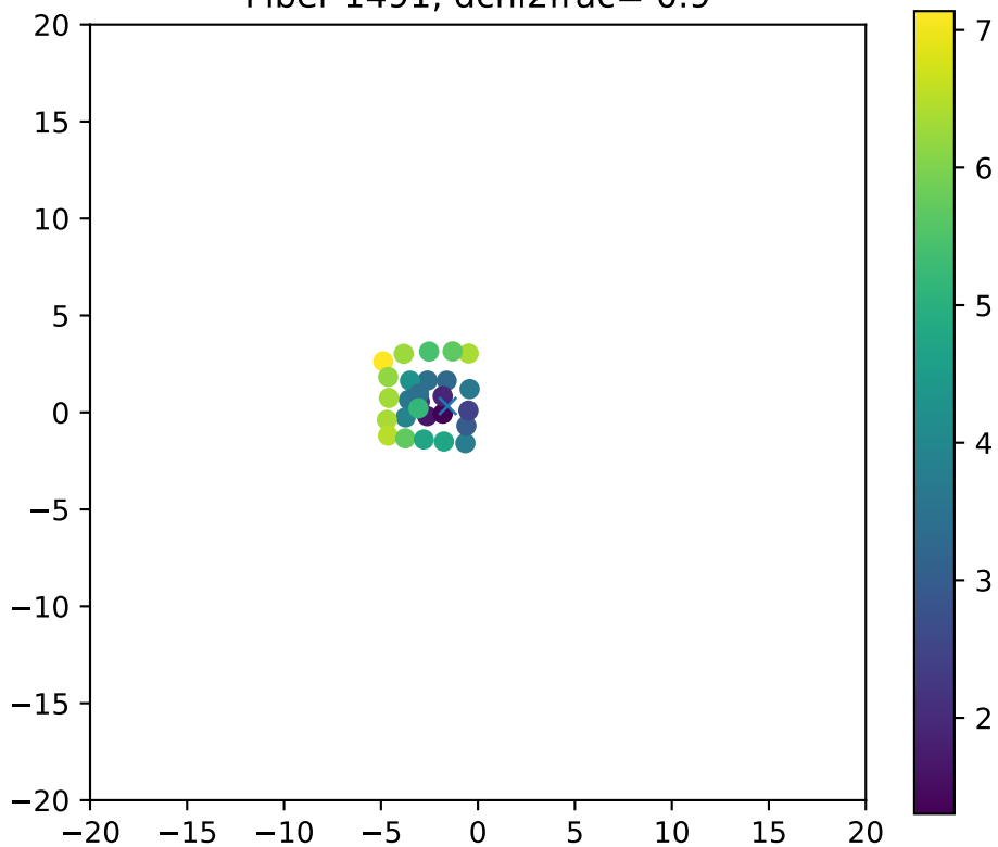
Fiber 1491, dchi2frac= 0.9
