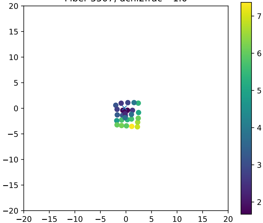
Fiber 3507, dchi2frac= 1.0
