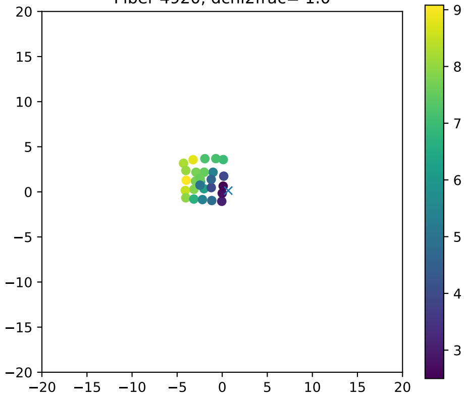
Fiber 4920, dchi2frac= 1.0
