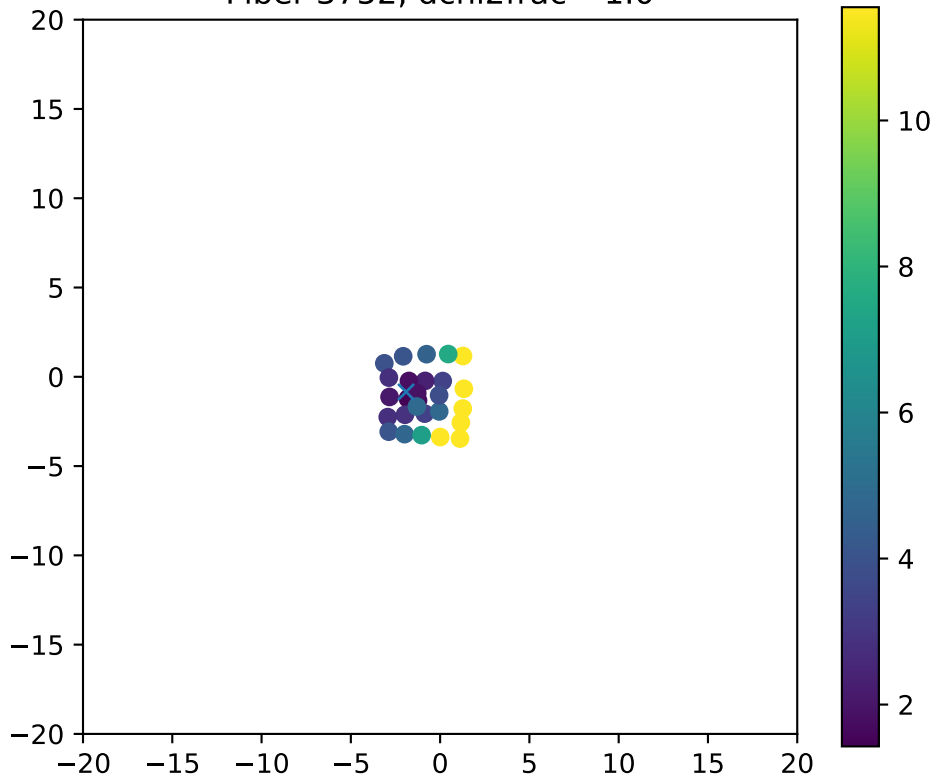
Fiber 3752, dchi2frac= 1.0
