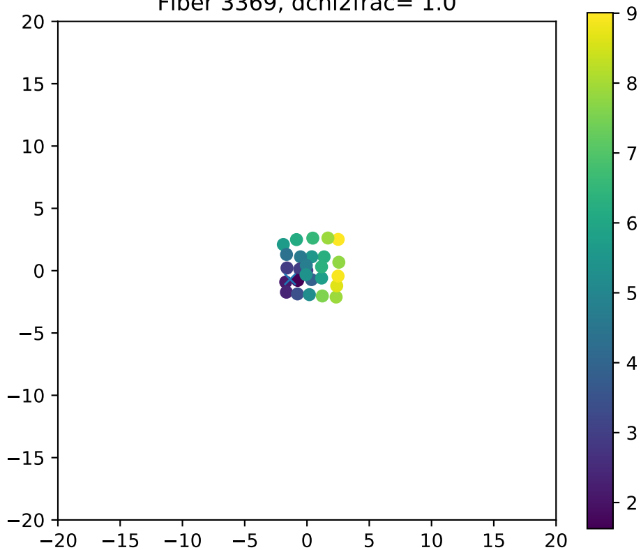
Fiber 3369, dchi2frac= 1.0
