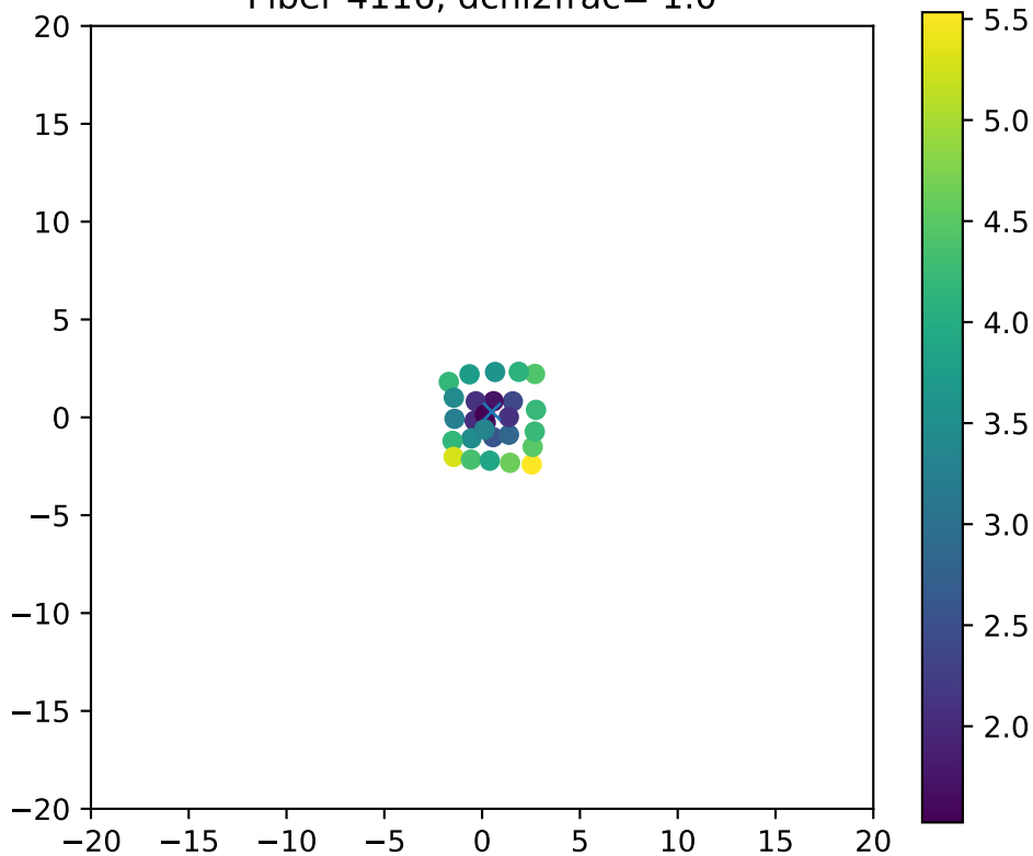
Fiber 4116, dchi2frac= 1.0
