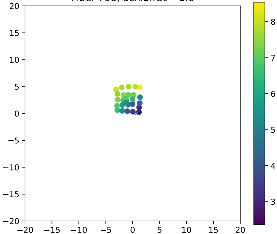
Fiber 798, dchi2frac= 1.0
