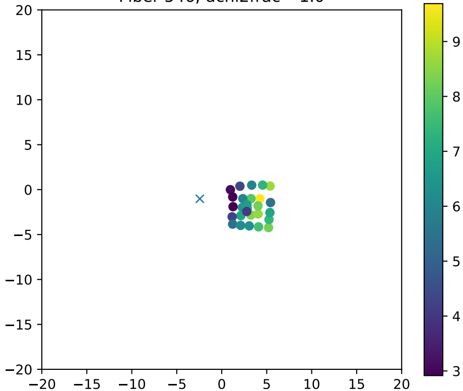
Fiber 546, dchi2frac= 1.0
