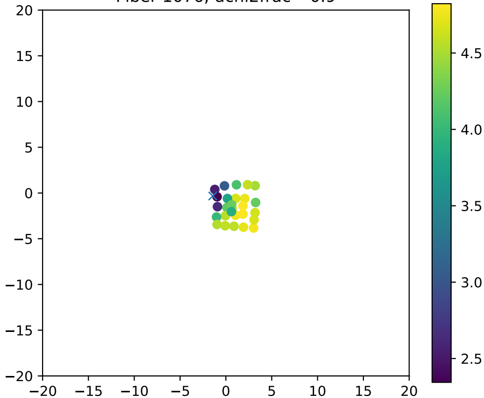
Fiber 1076, dchi2frac= 0.9
