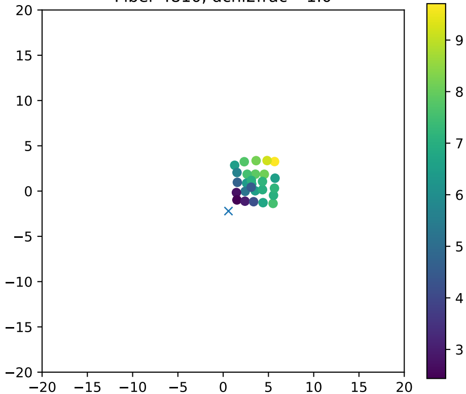
Fiber 4810, dchi2frac= 1.0
