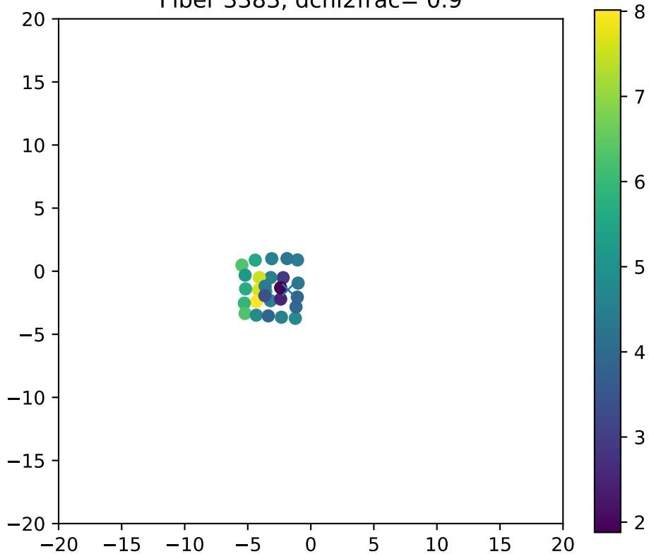
Fiber 3383, dchi2frac= 0.9
