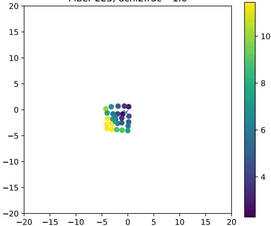
Fiber 223, dchi2frac= 1.0
