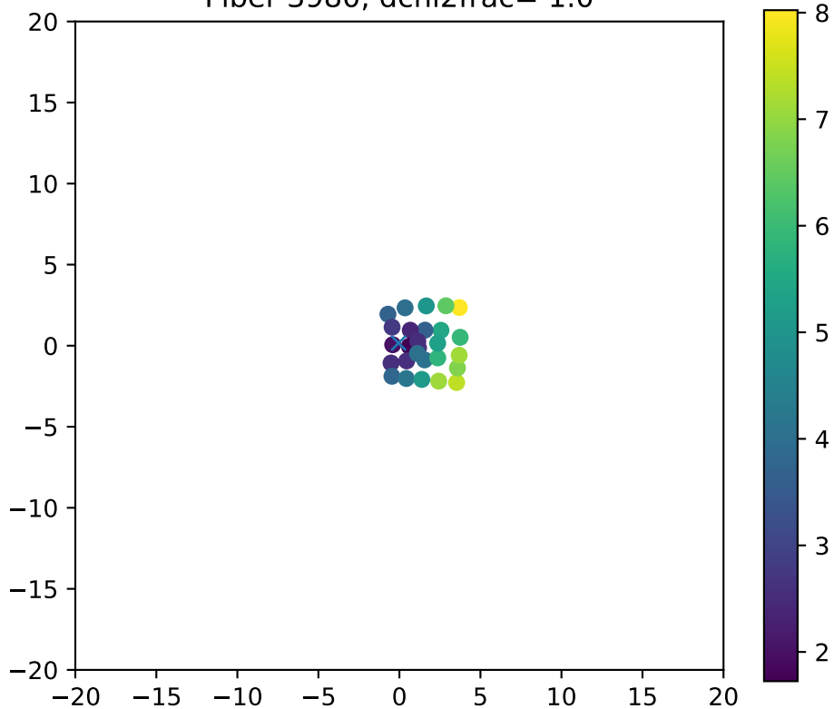
Fiber 3980, dchi2frac= 1.0
