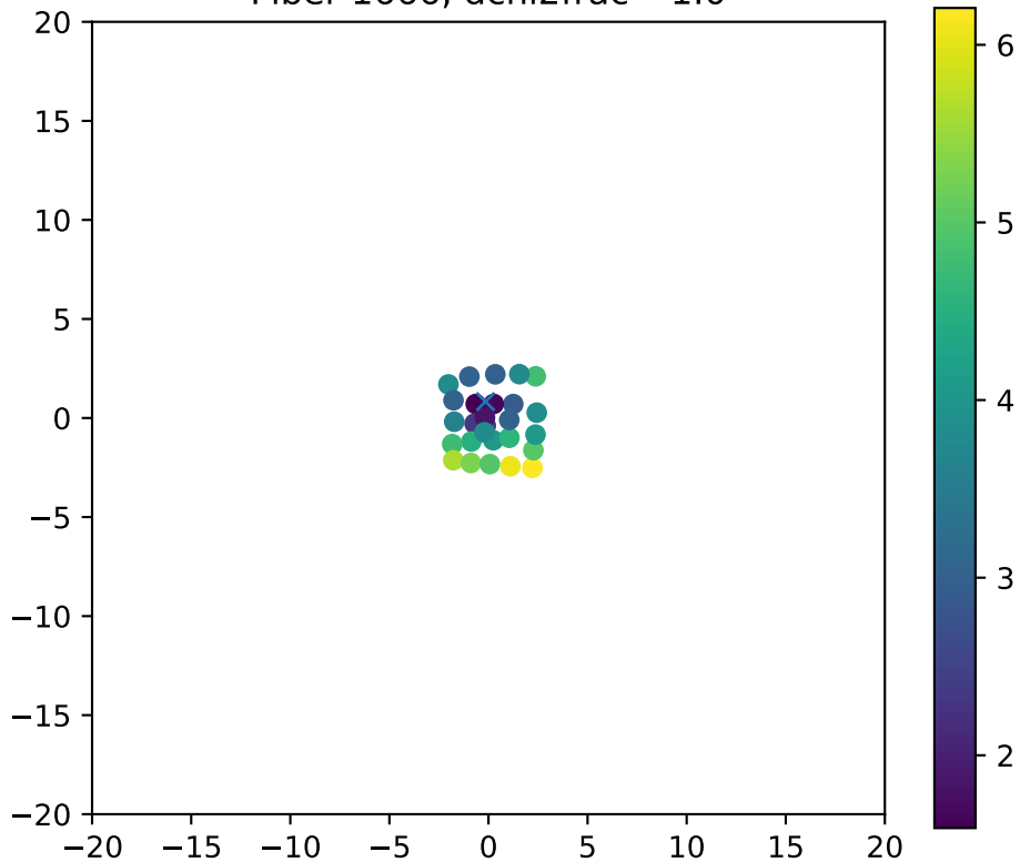
Fiber 1666, dchi2frac= 1.0
