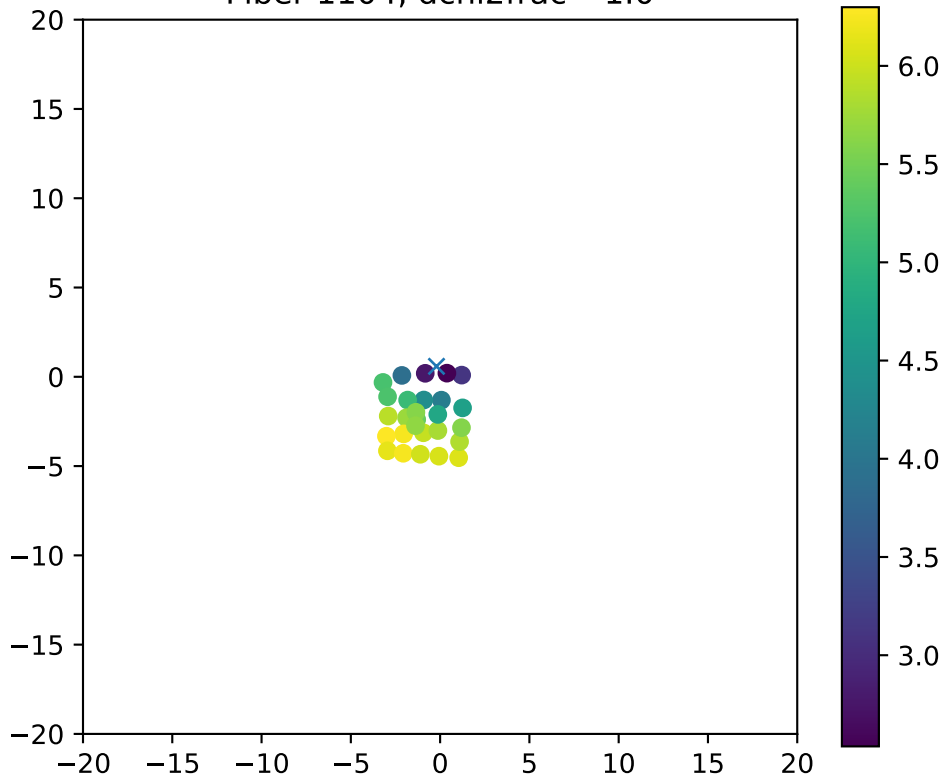
Fiber 1104, dchi2frac= 1.0
