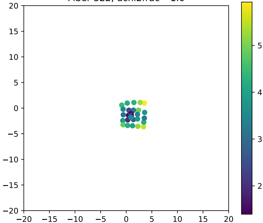
Fiber 322, dchi2frac= 1.0
