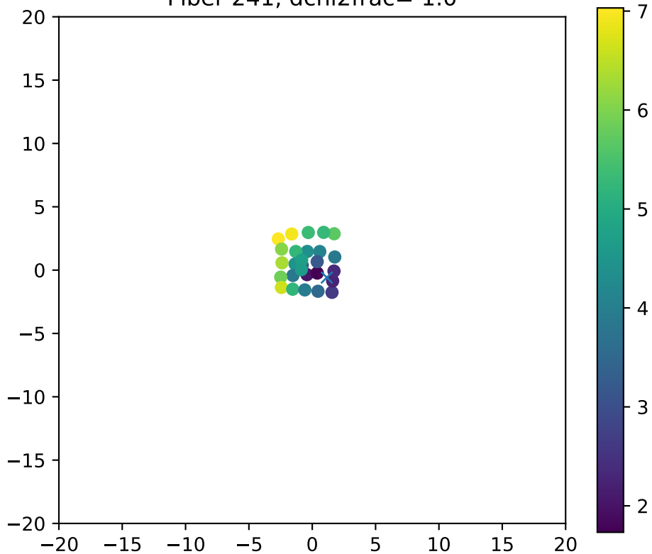
Fiber 241, dchi2frac= 1.0
