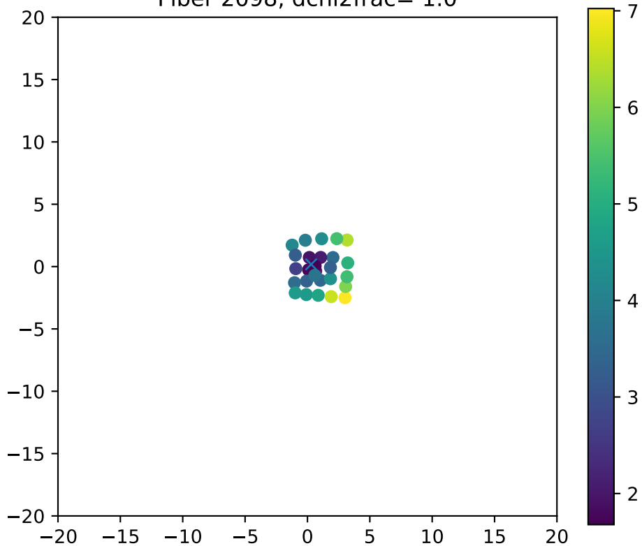
Fiber 2098, dchi2frac= 1.0
