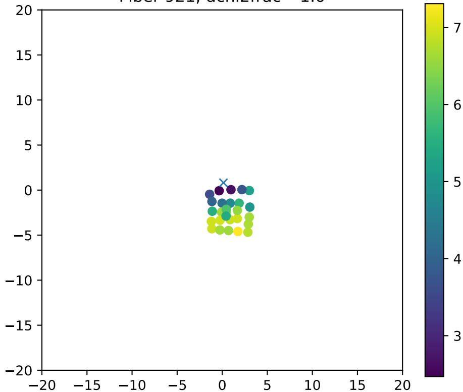
Fiber 921, dchi2frac= 1.0
