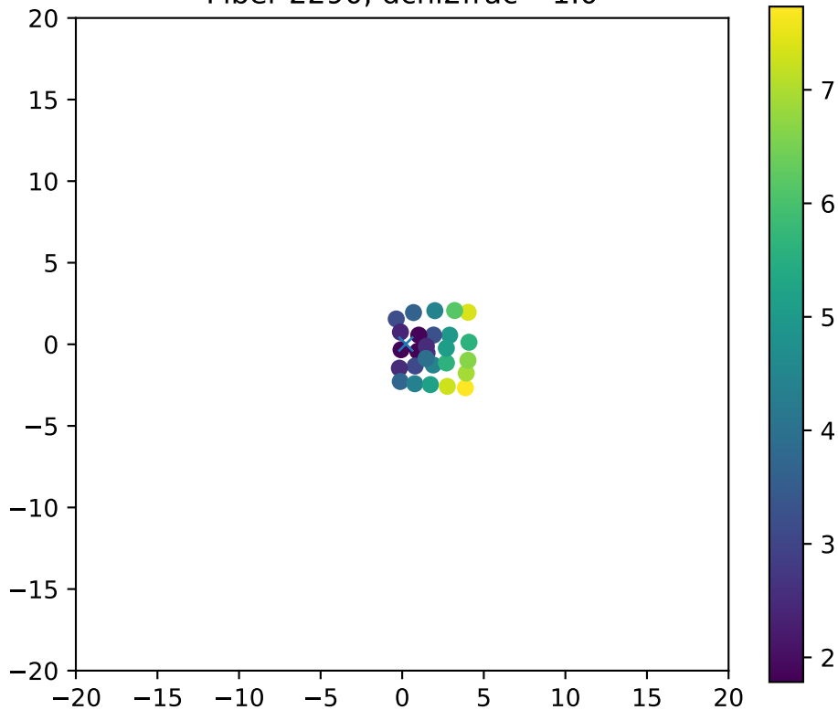
Fiber 2290, dchi2frac= 1.0
