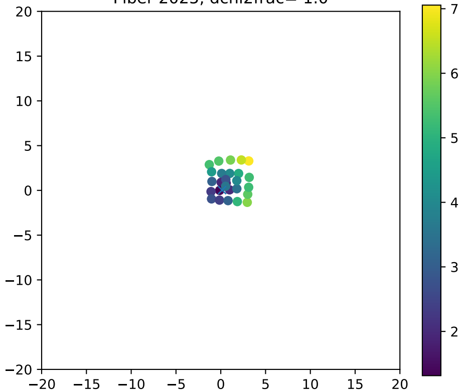
Fiber 2025, dchi2frac= 1.0
