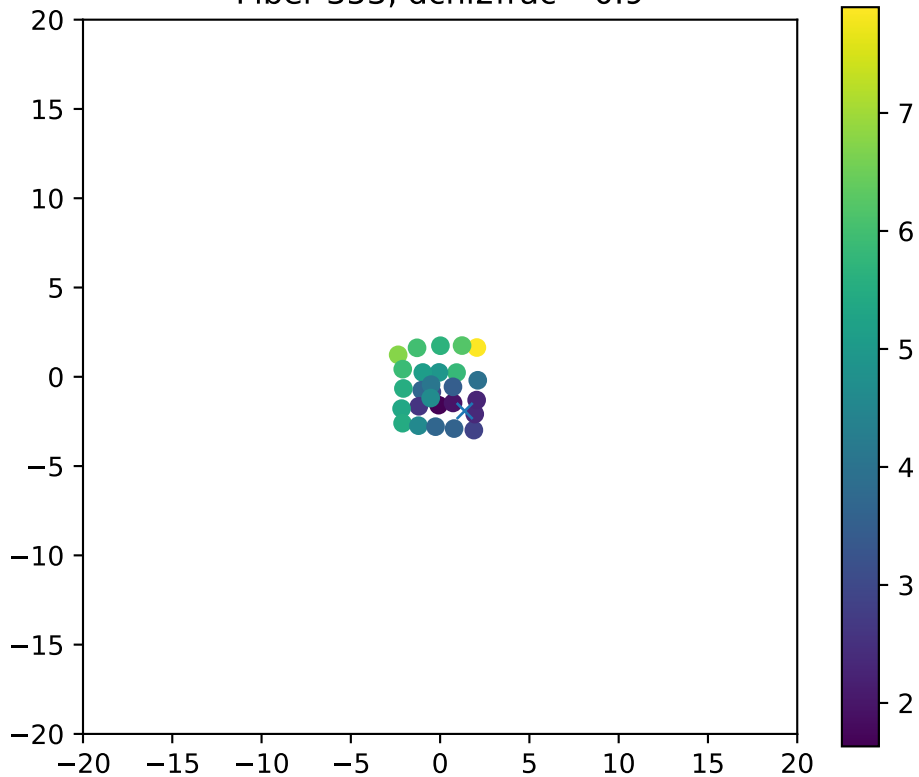
Fiber 353, dchi2frac= 0.9
