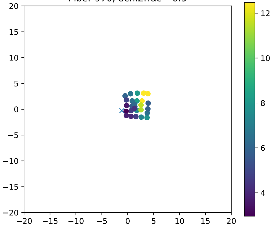
Fiber 970, dchi2frac= 0.9
