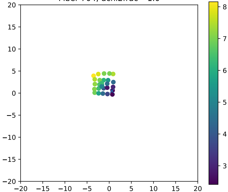
Fiber 704, dchi2frac= 1.0
