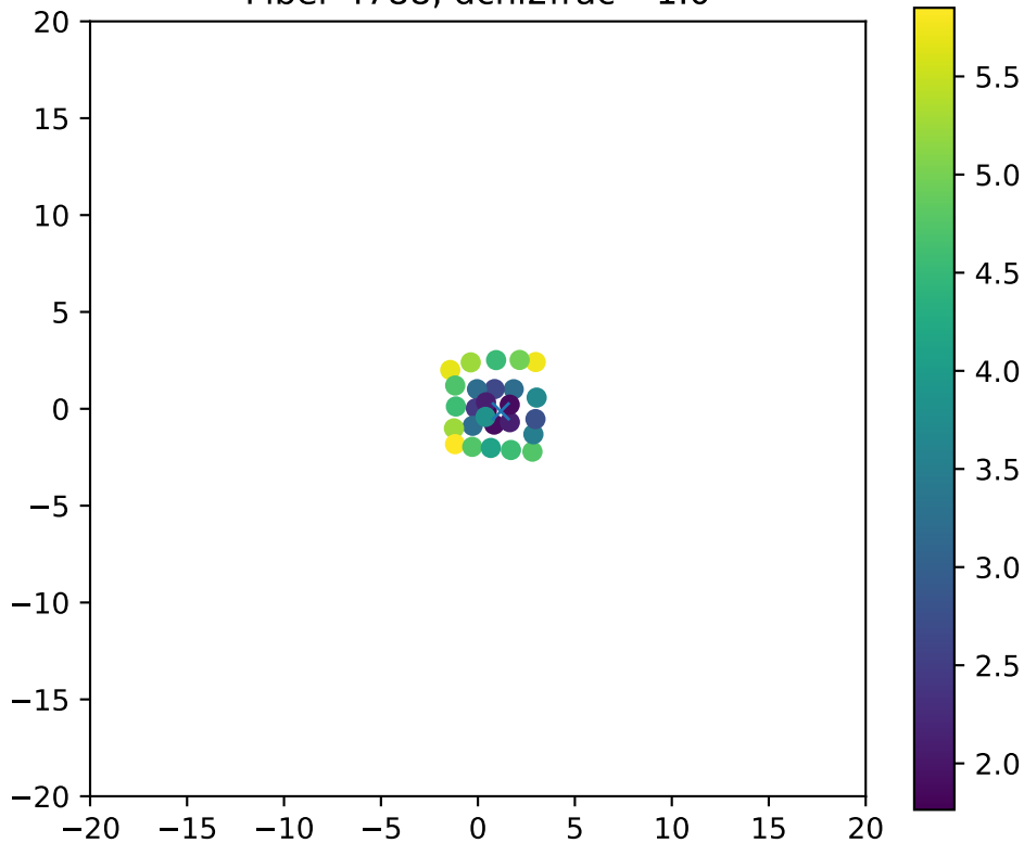
Fiber 4788, dchi2frac= 1.0
