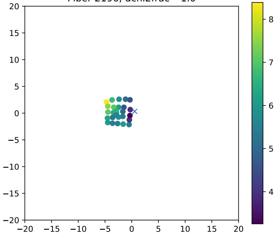
Fiber 2196, dchi2frac= 1.0
