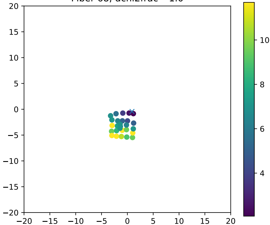
Fiber 68, dchi2frac= 1.0
