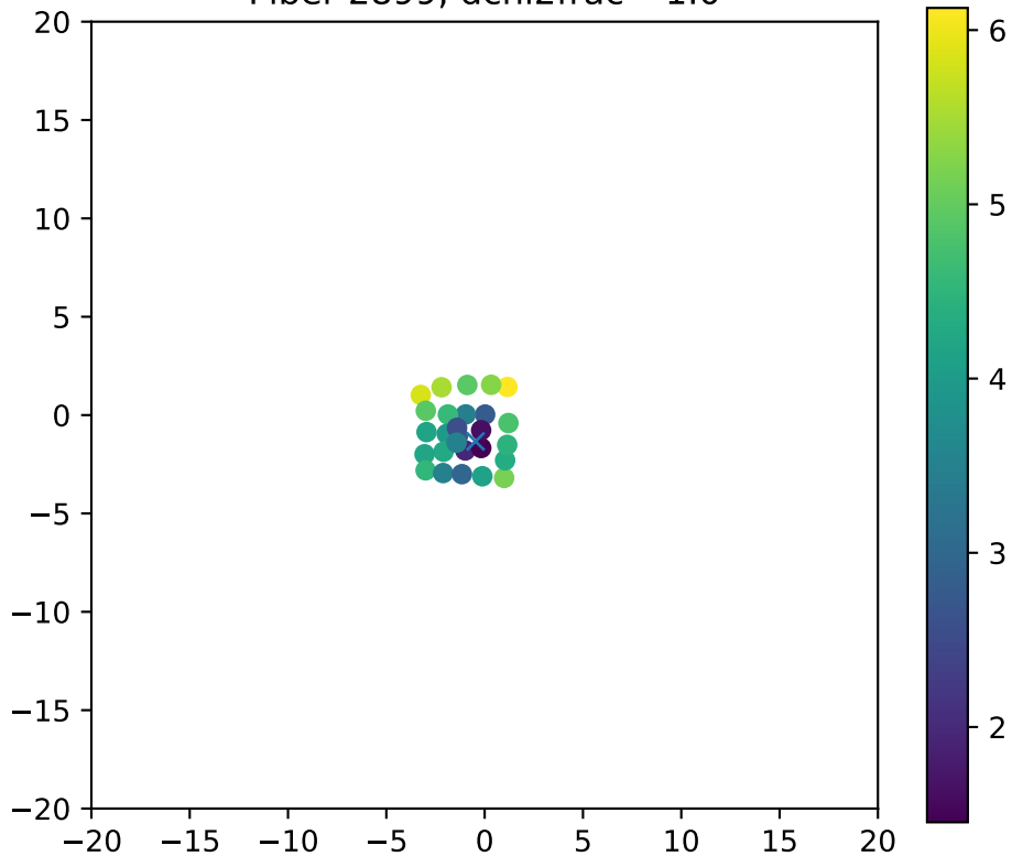
Fiber 2899, dchi2frac= 1.0
