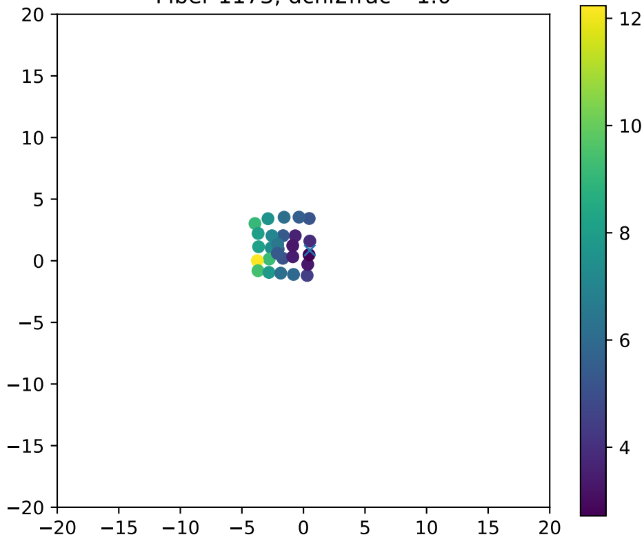
Fiber 1173, dchi2frac= 1.0
