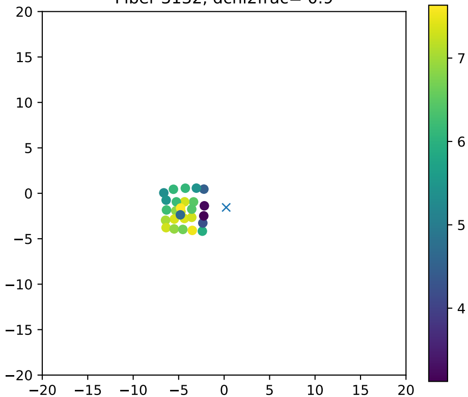
Fiber 3132, dchi2frac= 0.9
