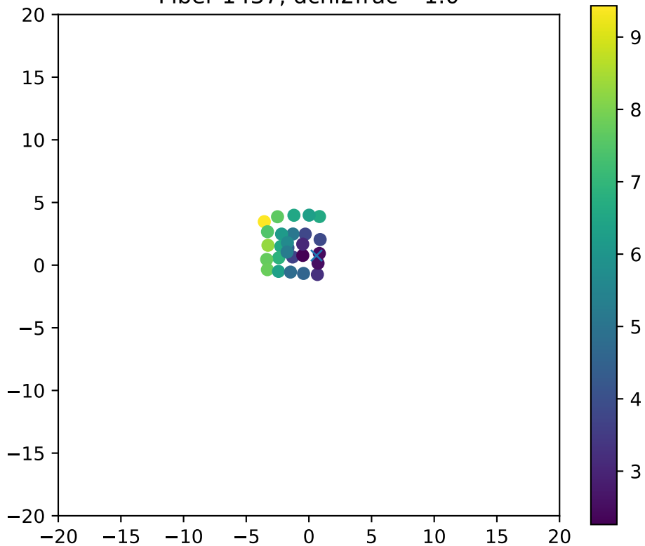
Fiber 1437, dchi2frac= 1.0
