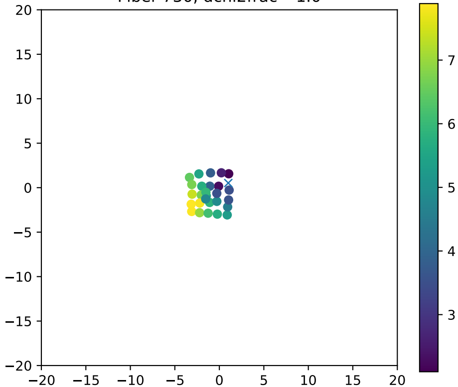
Fiber 730, dchi2frac= 1.0
