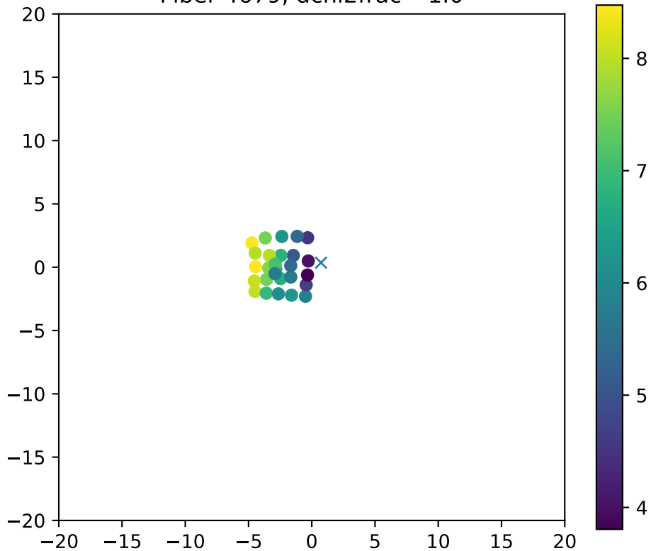
Fiber 4679, dchi2frac= 1.0
