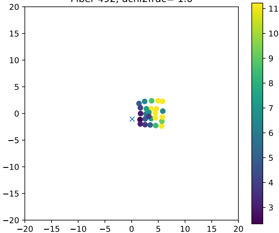
Fiber 492, dchi2frac= 1.0
