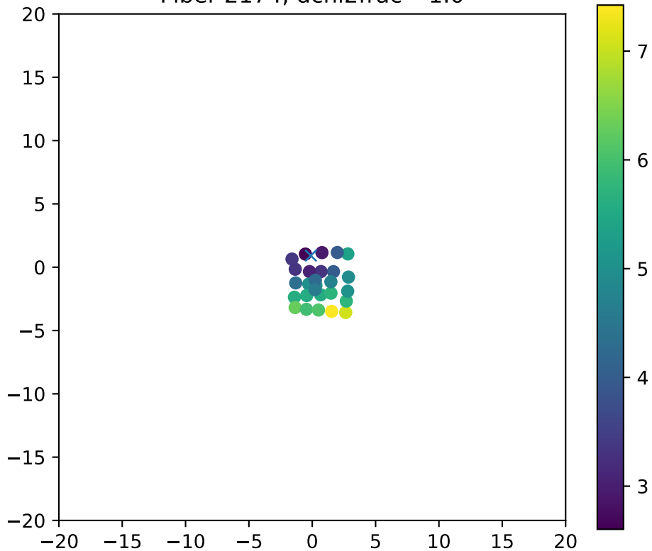
Fiber 2174, dchi2frac= 1.0
