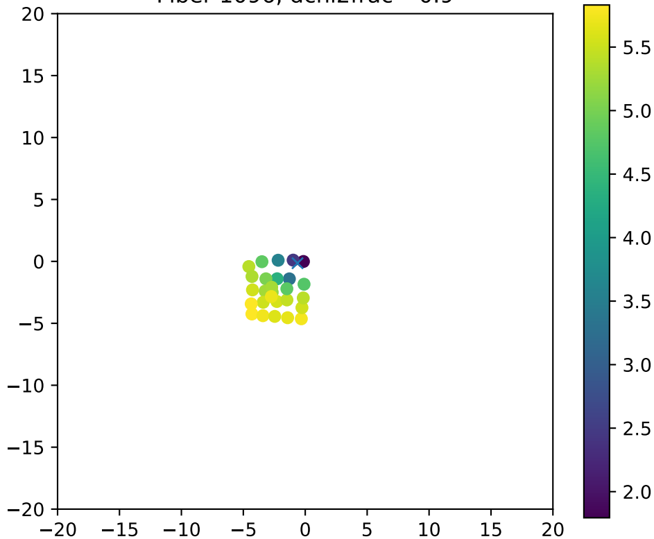
Fiber 1096, dchi2frac= 0.9
