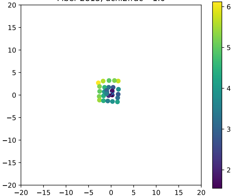
Fiber 2813, dchi2frac= 1.0
