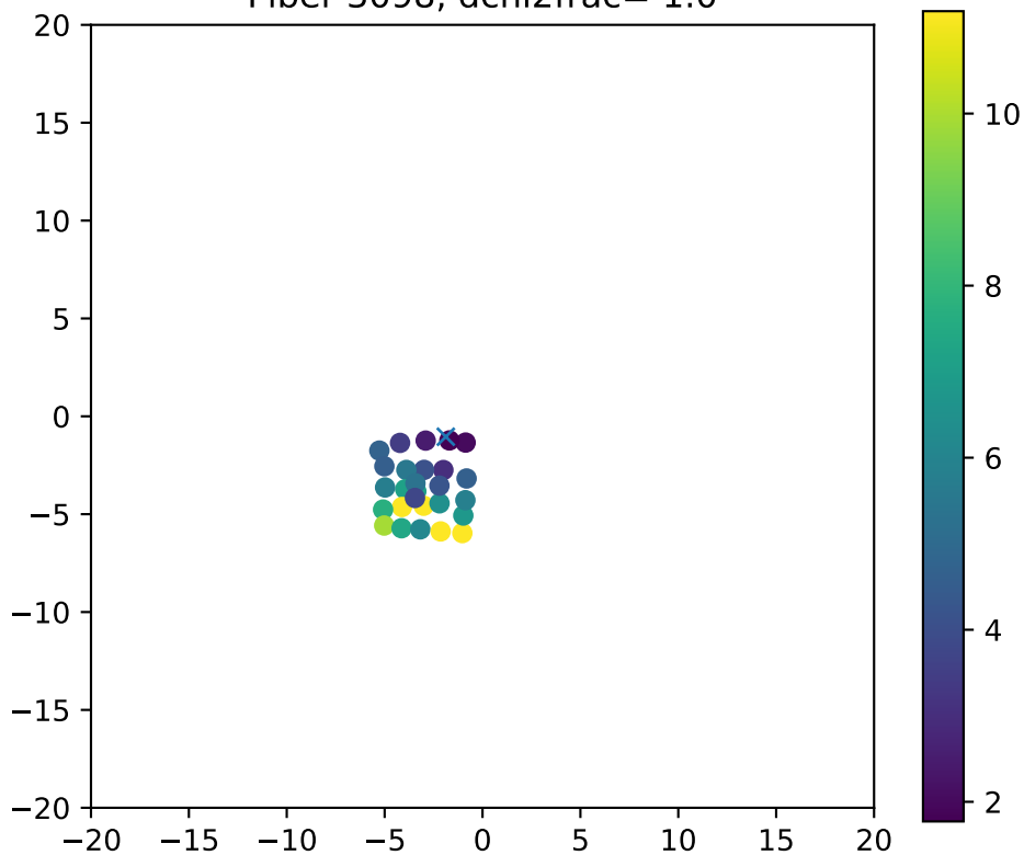
Fiber 3098, dchi2frac= 1.0
