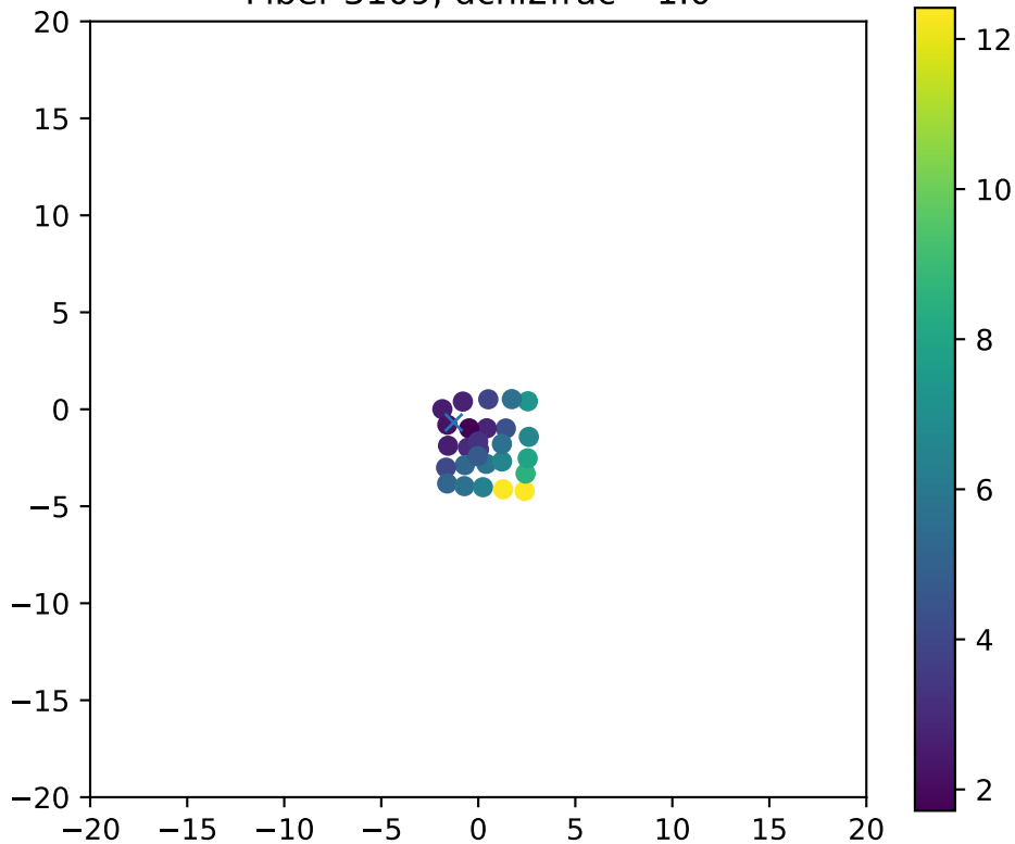
Fiber 3109, dchi2frac= 1.0
