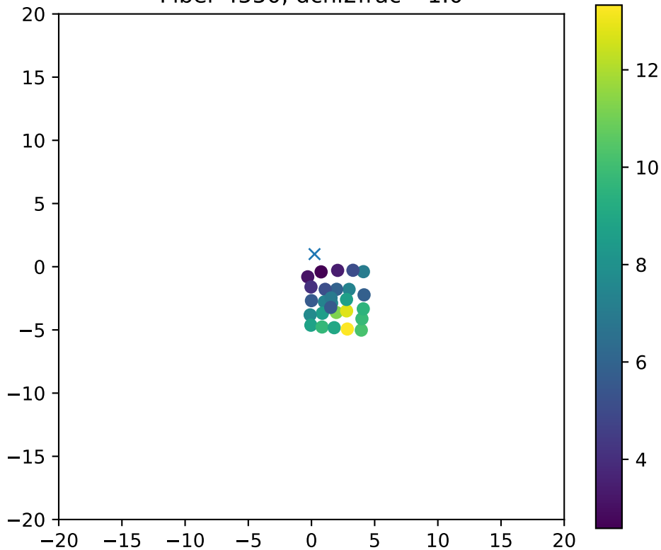
Fiber 4550, dchi2frac= 1.0
