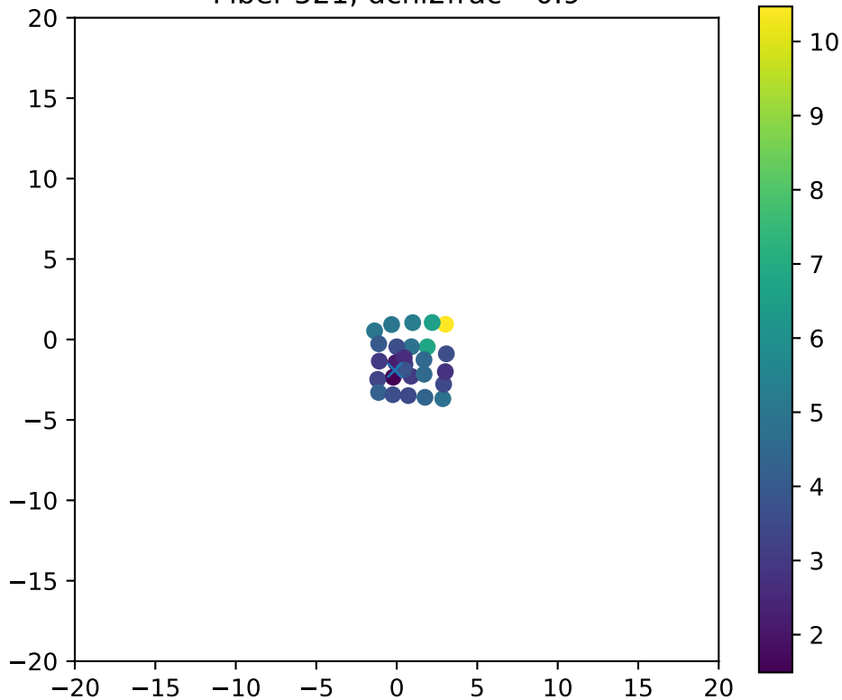
Fiber 521, dchi2frac= 0.9
