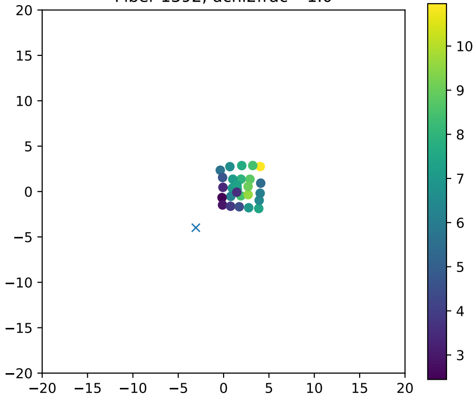
Fiber 1392, dchi2frac= 1.0
