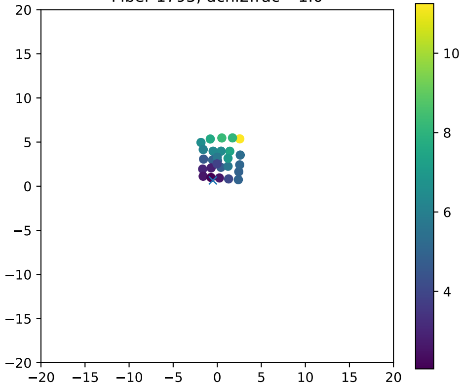
Fiber 1795, dchi2frac= 1.0
