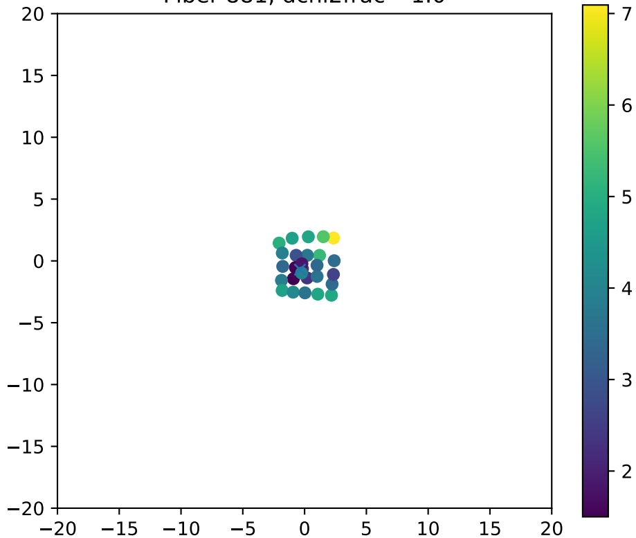
Fiber 881, dchi2frac= 1.0
