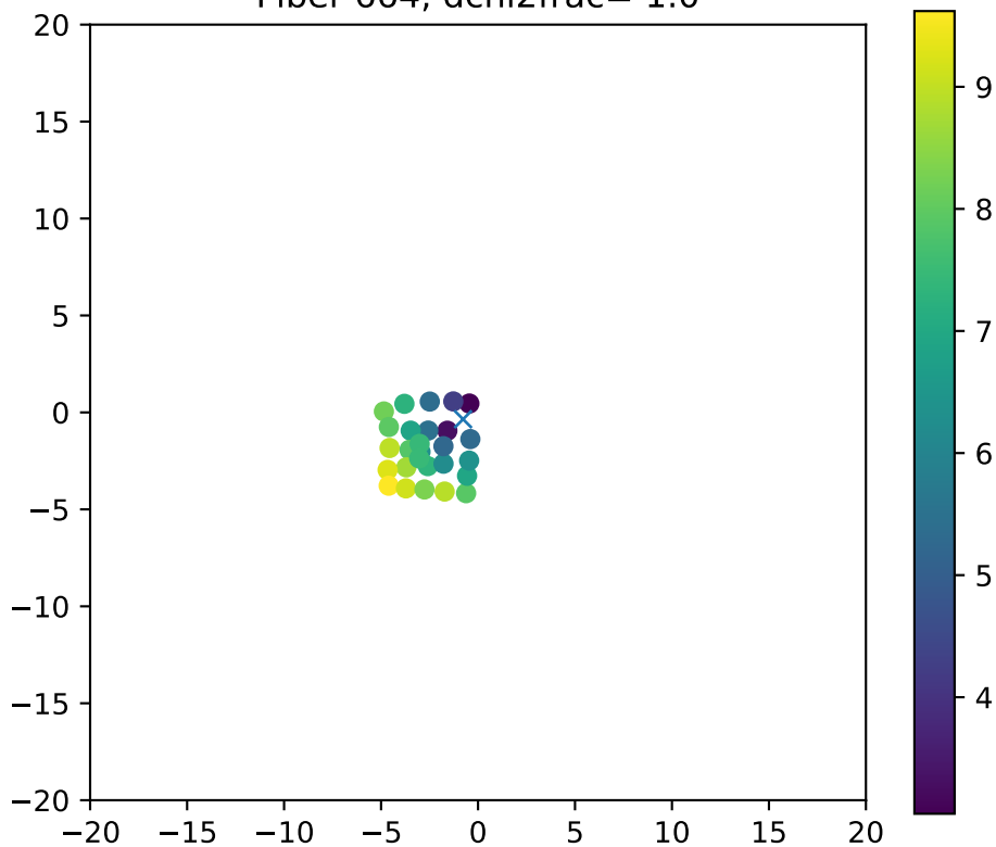
Fiber 664, dchi2frac= 1.0
