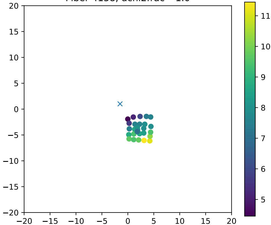
Fiber 4158, dchi2frac= 1.0
