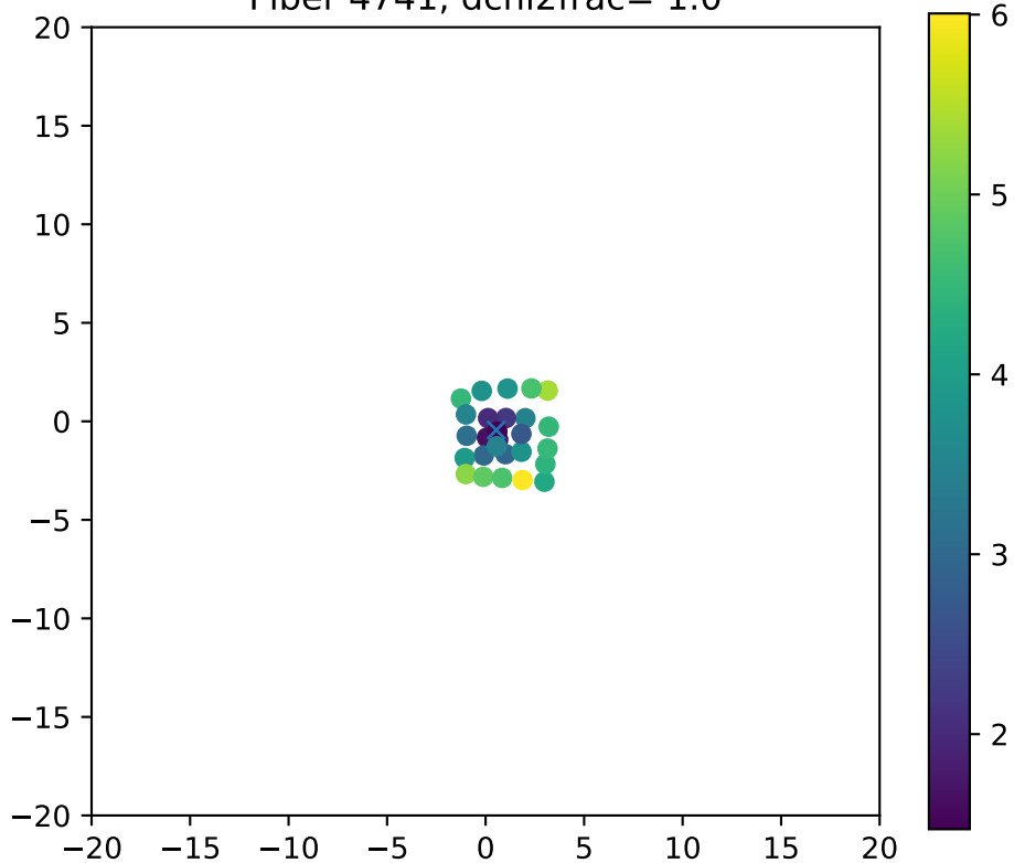
Fiber 4741, dchi2frac= 1.0
