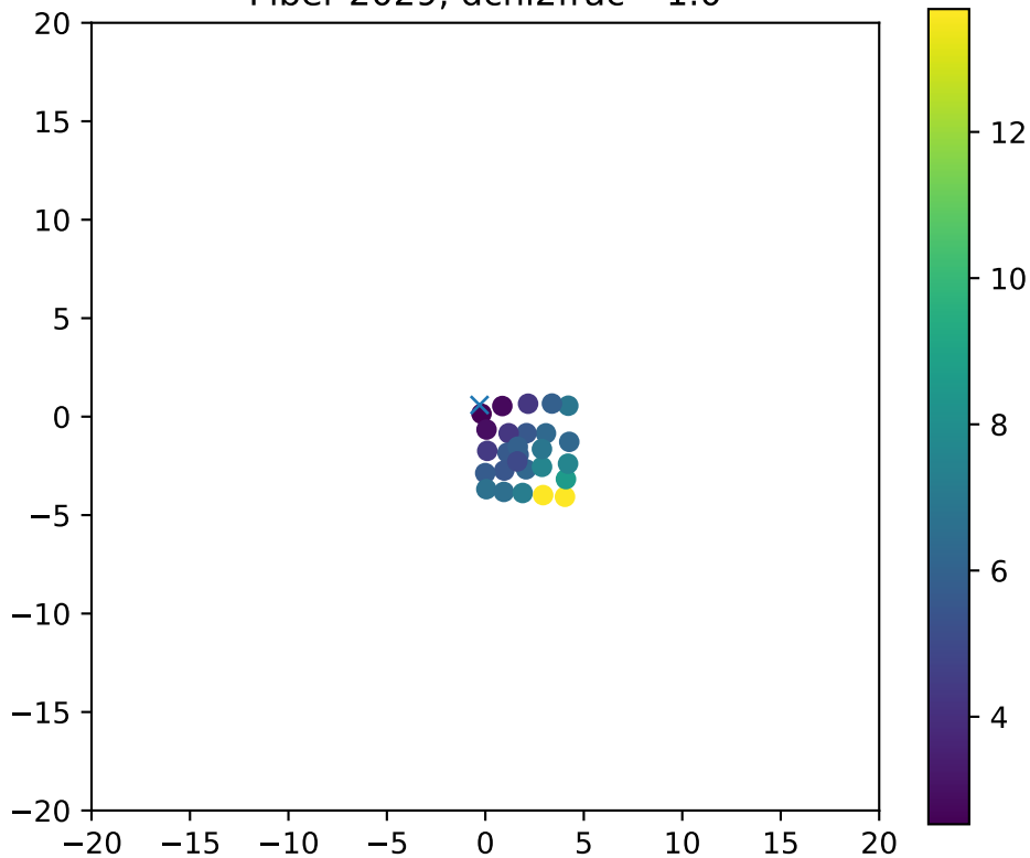
Fiber 2029, dchi2frac= 1.0
