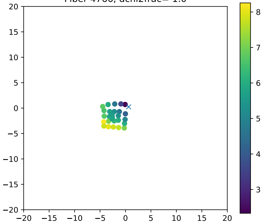
Fiber 4766, dchi2frac= 1.0
