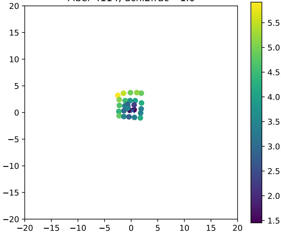
Fiber 4114, dchi2frac= 1.0
