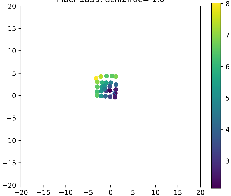
Fiber 1839, dchi2frac= 1.0
