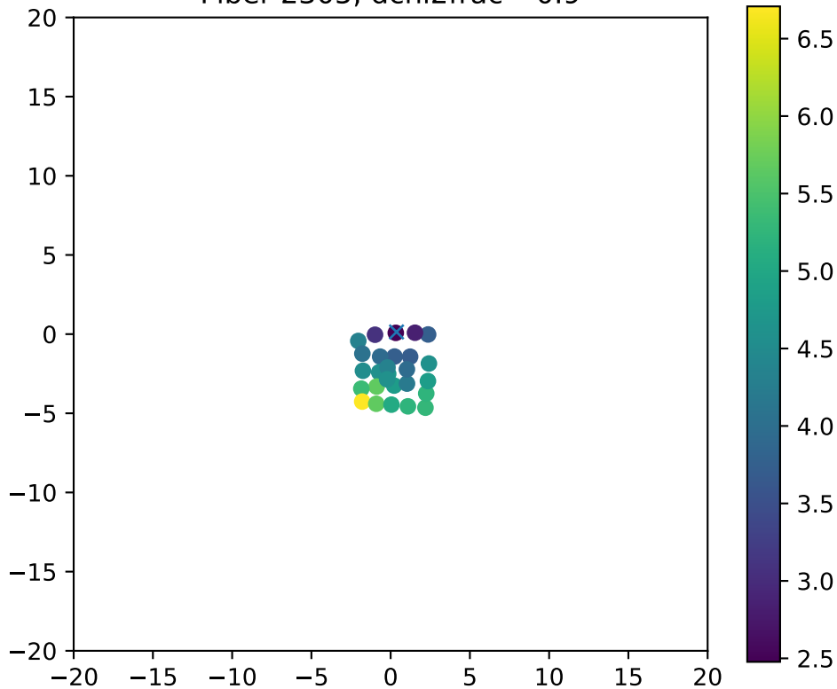
Fiber 2305, dchi2frac= 0.9
