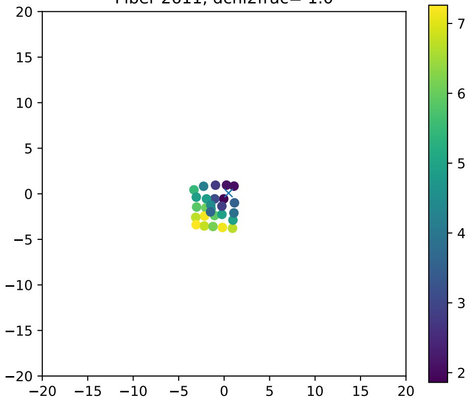
Fiber 2611, dchi2frac= 1.0
