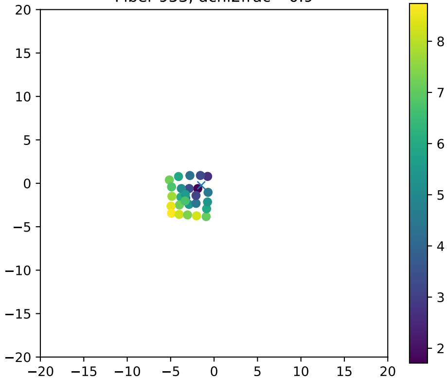
Fiber 953, dchi2frac= 0.9
