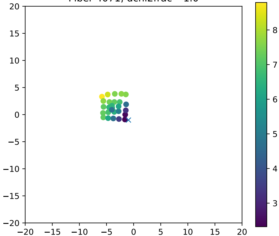
Fiber 4071, dchi2frac= 1.0
