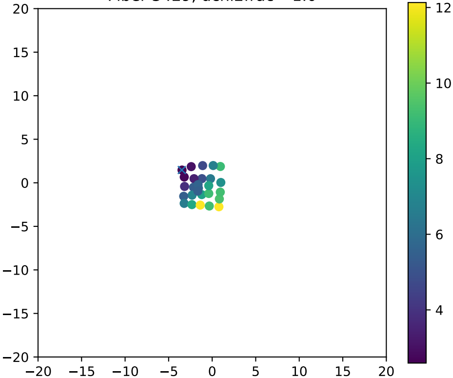
Fiber 3429, dchi2frac= 1.0
