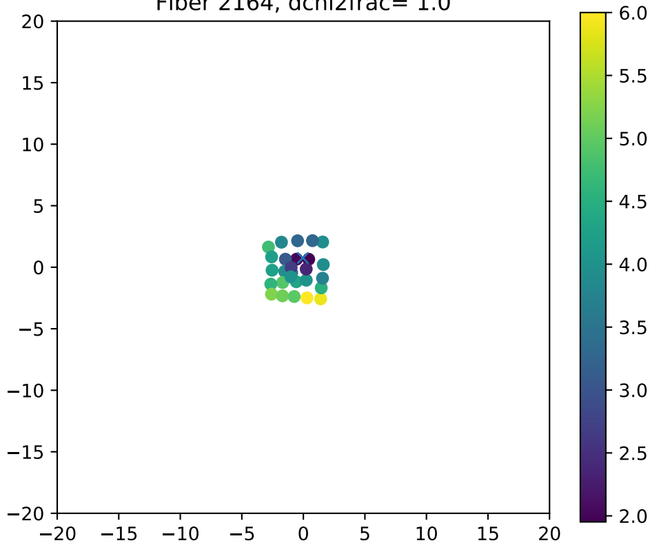
Fiber 2164, dchi2frac= 1.0
