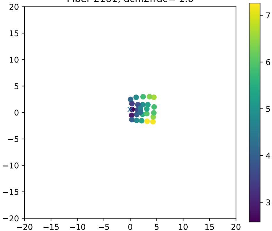
Fiber 2161, dchi2frac= 1.0
