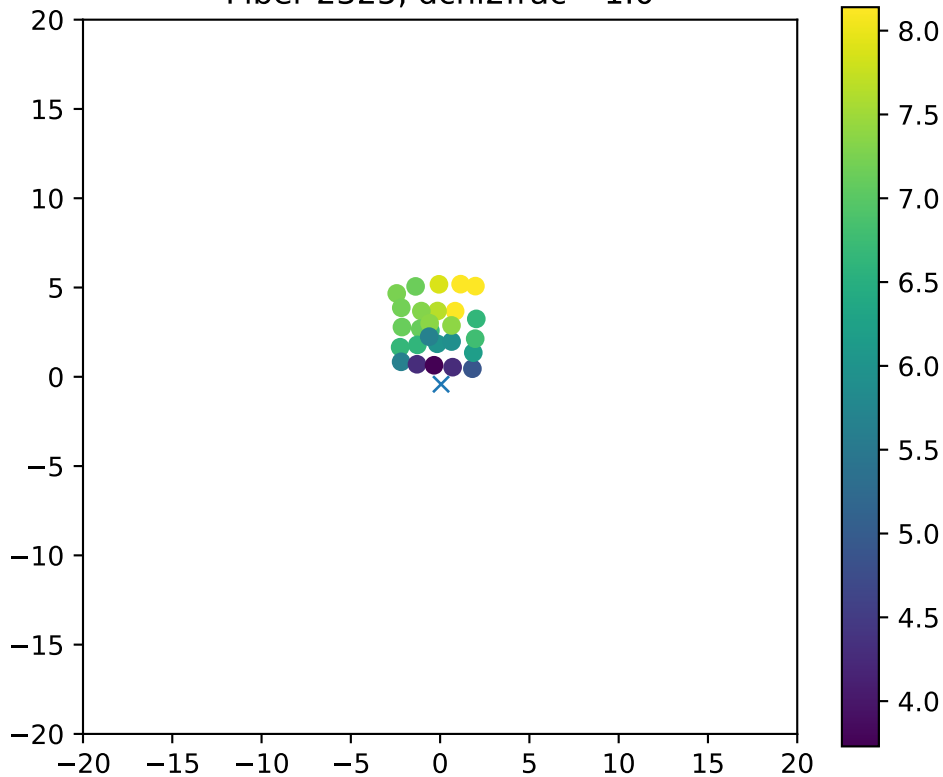
Fiber 2325, dchi2frac= 1.0
