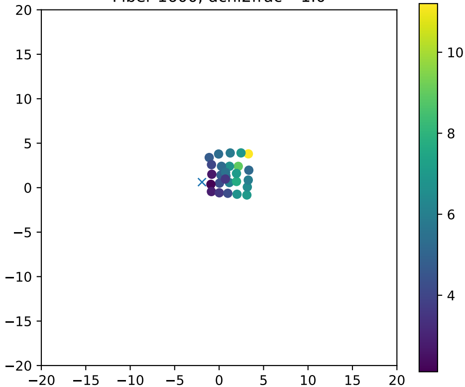
Fiber 1600, dchi2frac= 1.0
