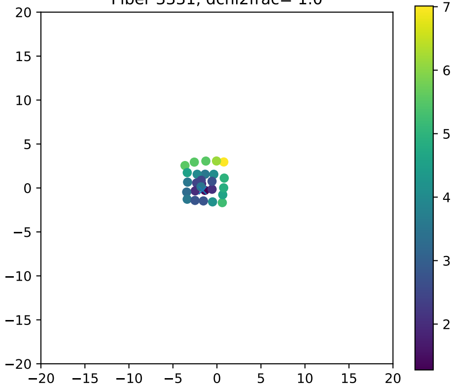
Fiber 3331, dchi2frac= 1.0
