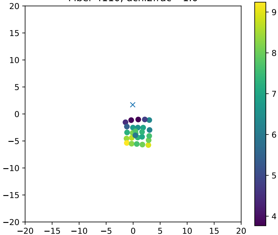
Fiber 4110, dchi2frac= 1.0
