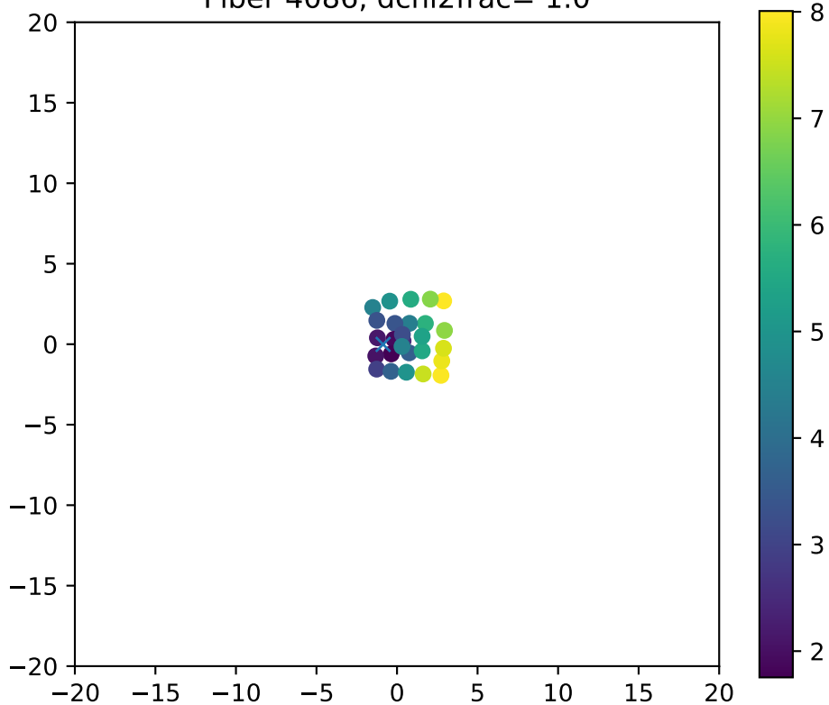
Fiber 4086, dchi2frac= 1.0
