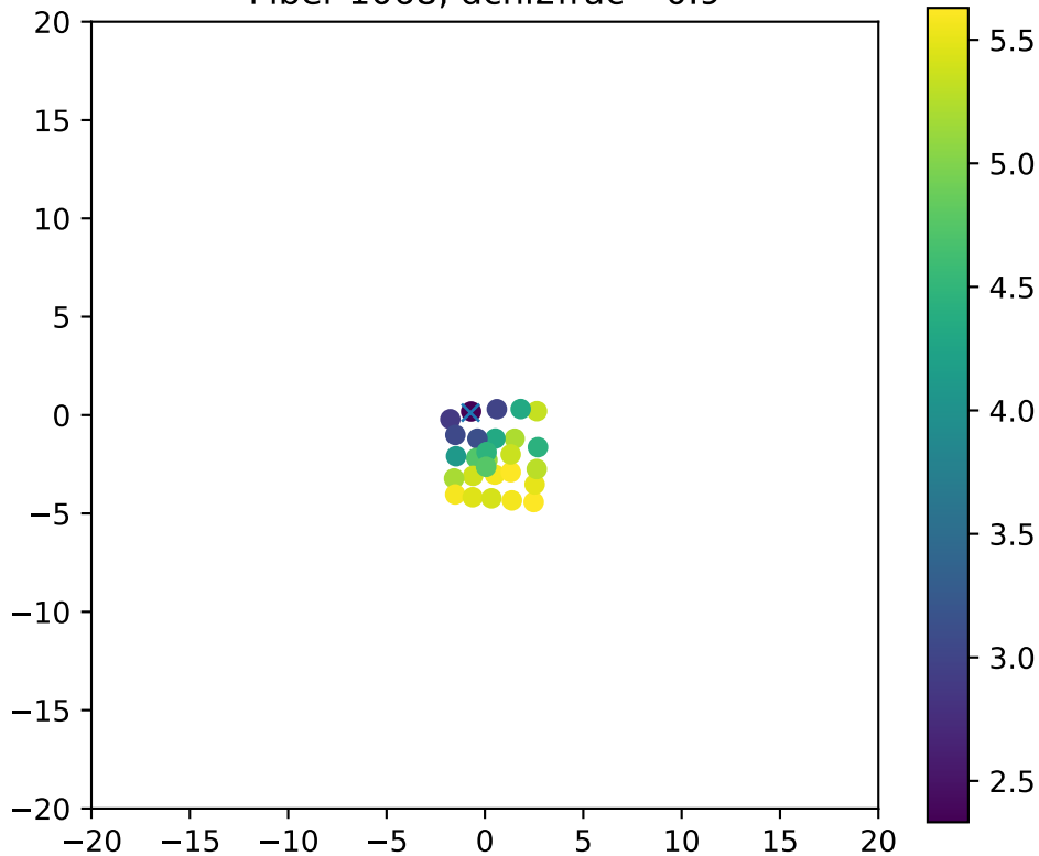
Fiber 1068, dchi2frac= 0.9
