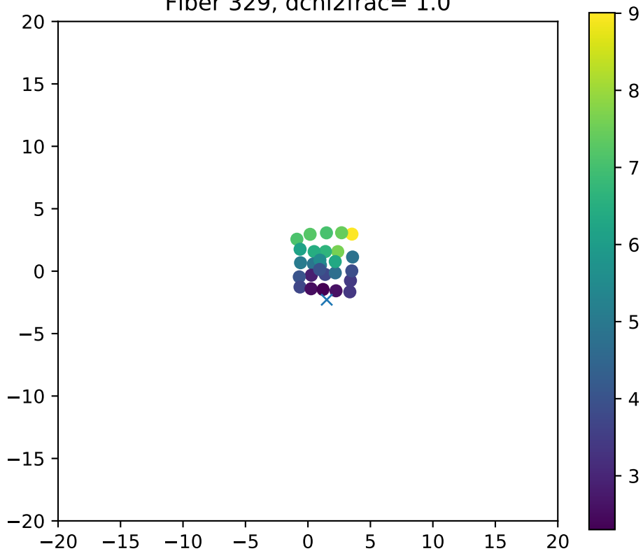
Fiber 329, dchi2frac= 1.0
