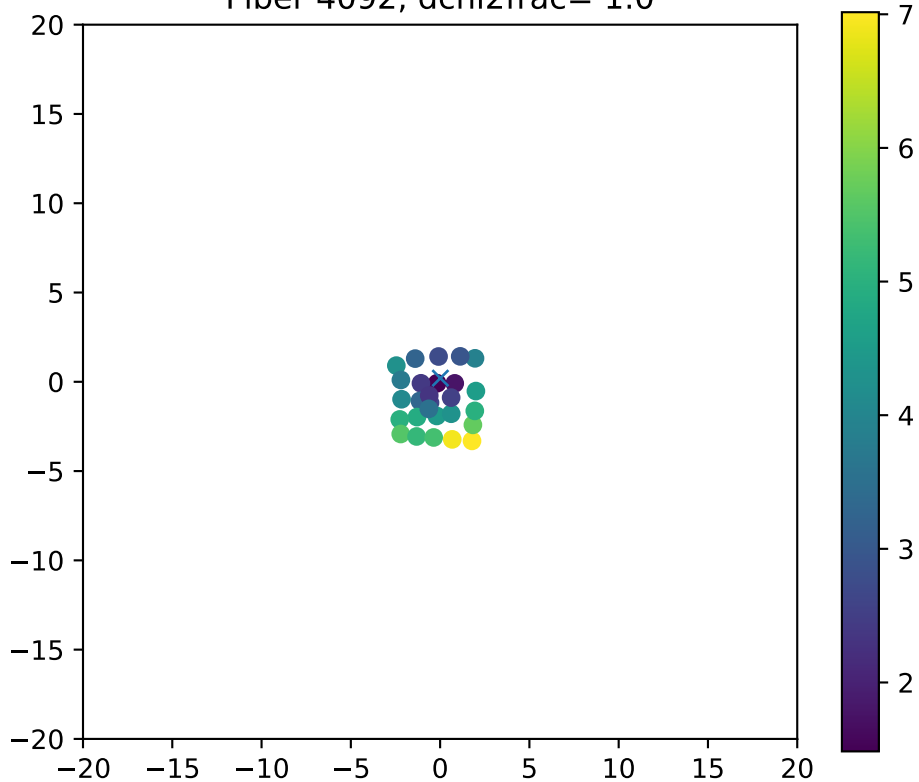
Fiber 4092, dchi2frac= 1.0
