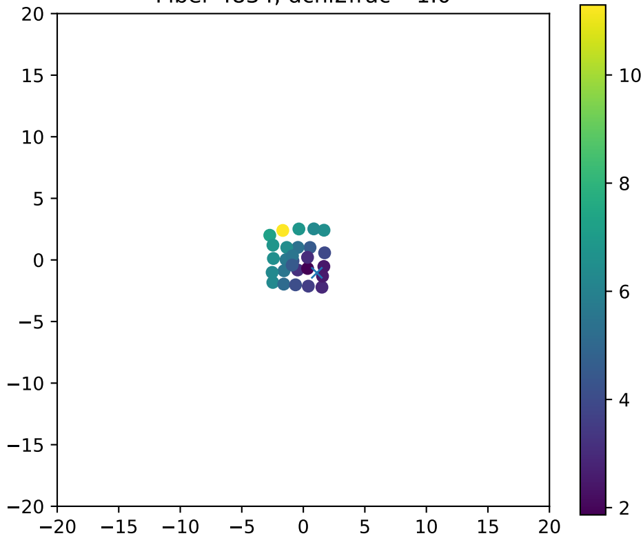
Fiber 4834, dchi2frac= 1.0
