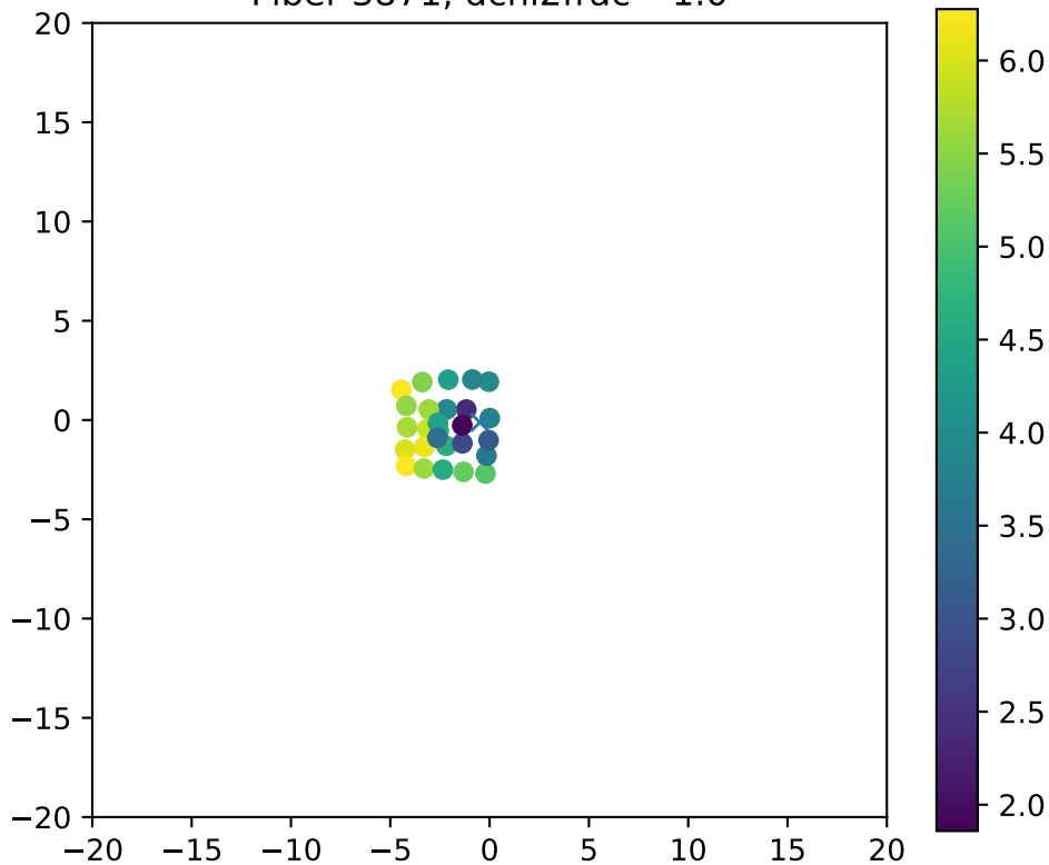
Fiber 3871, dchi2frac= 1.0
