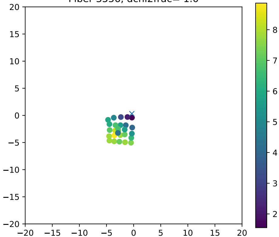
Fiber 3556, dchi2frac= 1.0
