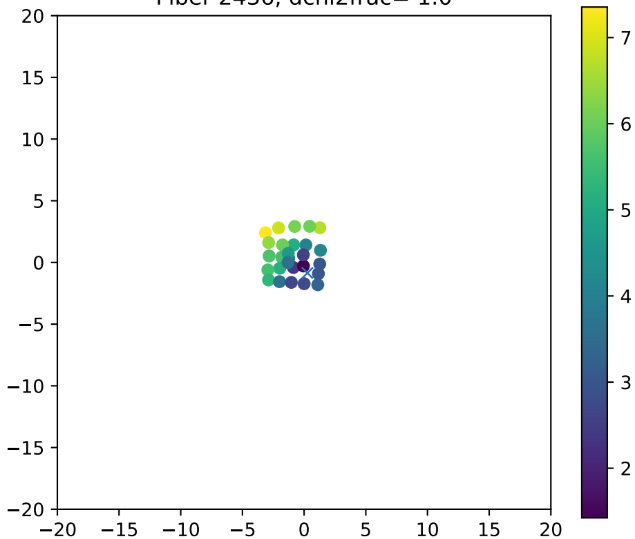
Fiber 2436, dchi2frac= 1.0
