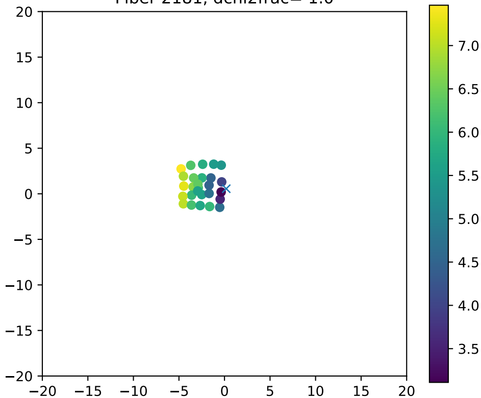
Fiber 2181, dchi2frac= 1.0
