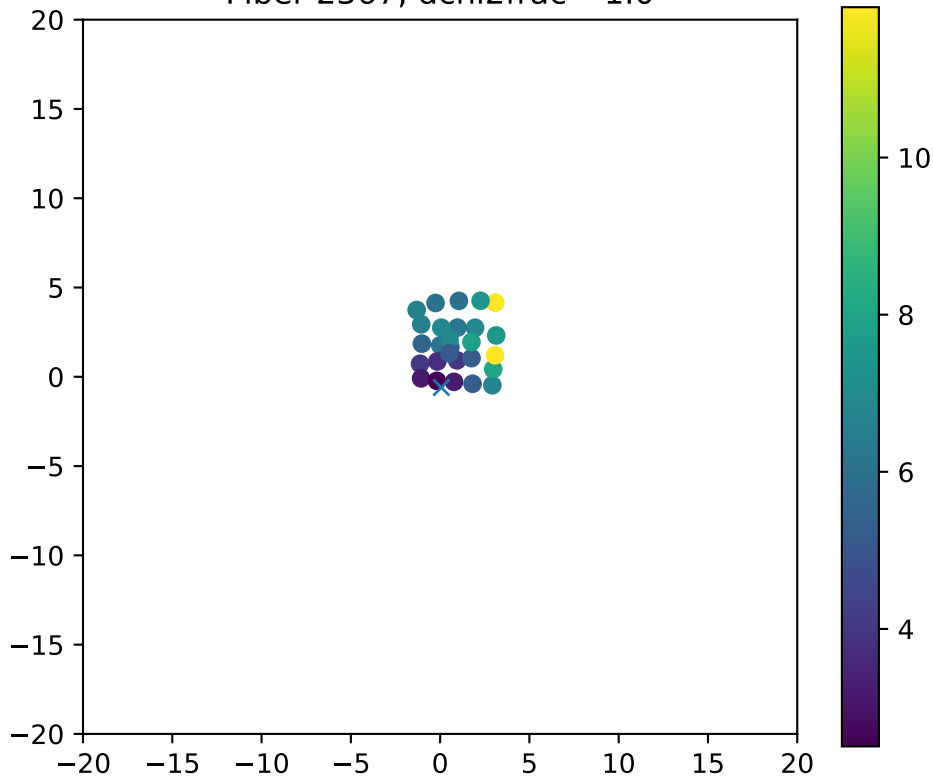
Fiber 2367, dchi2frac= 1.0
