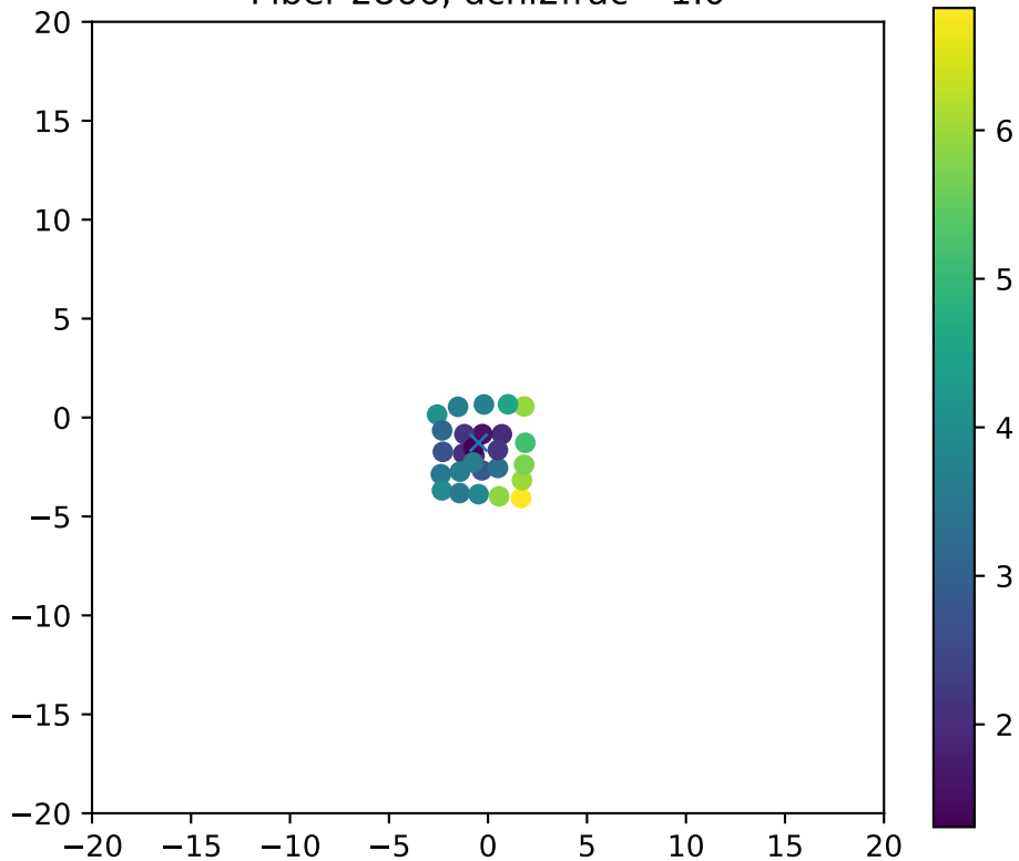
Fiber 2866, dchi2frac= 1.0
