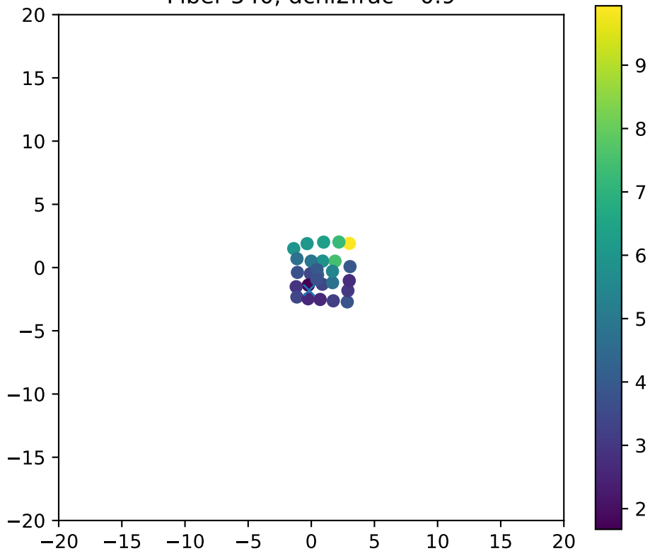
Fiber 540, dchi2frac= 0.9
