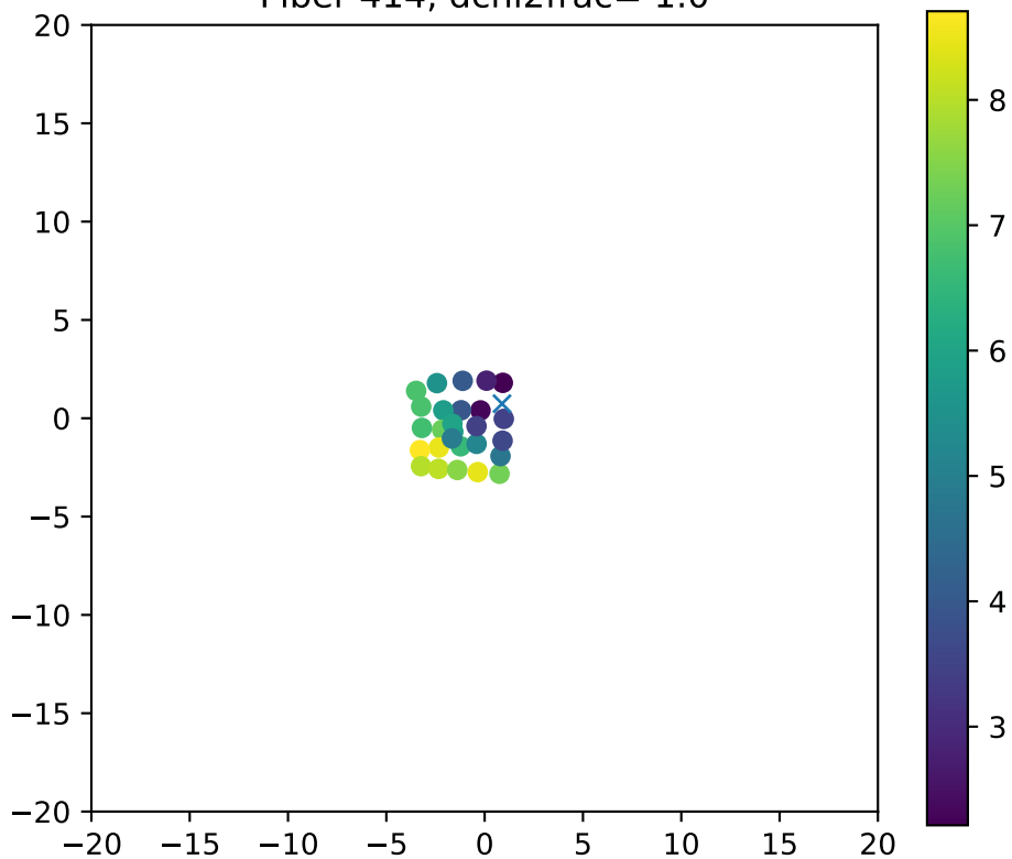
Fiber 414, dchi2frac= 1.0
