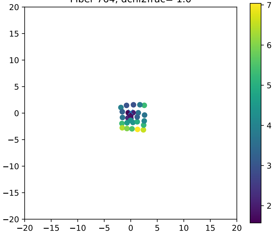
Fiber 764, dchi2frac= 1.0
