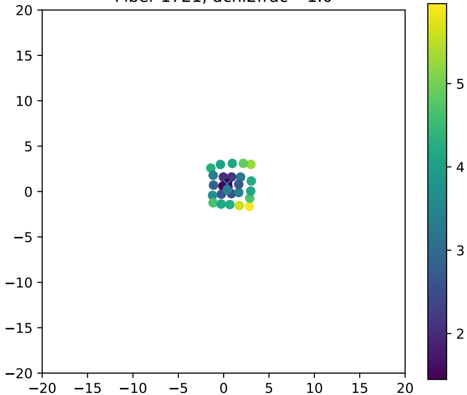
Fiber 1721, dchi2frac= 1.0
