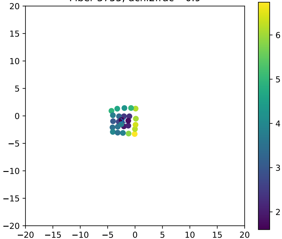
Fiber 3755, dchi2frac= 0.9
