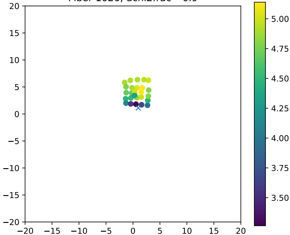
Fiber 1026, dchi2frac= 0.9
