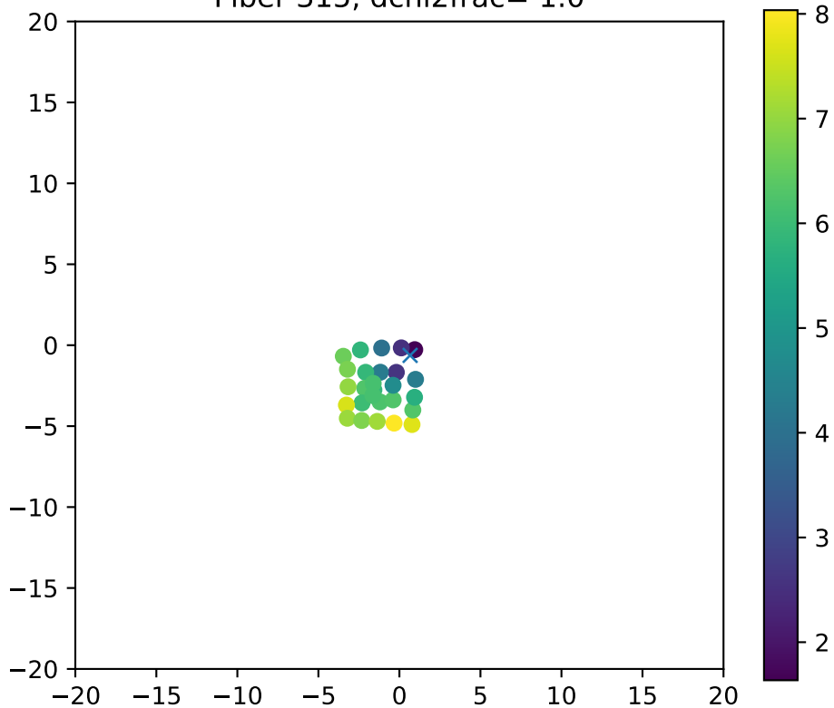
Fiber 315, dchi2frac= 1.0
