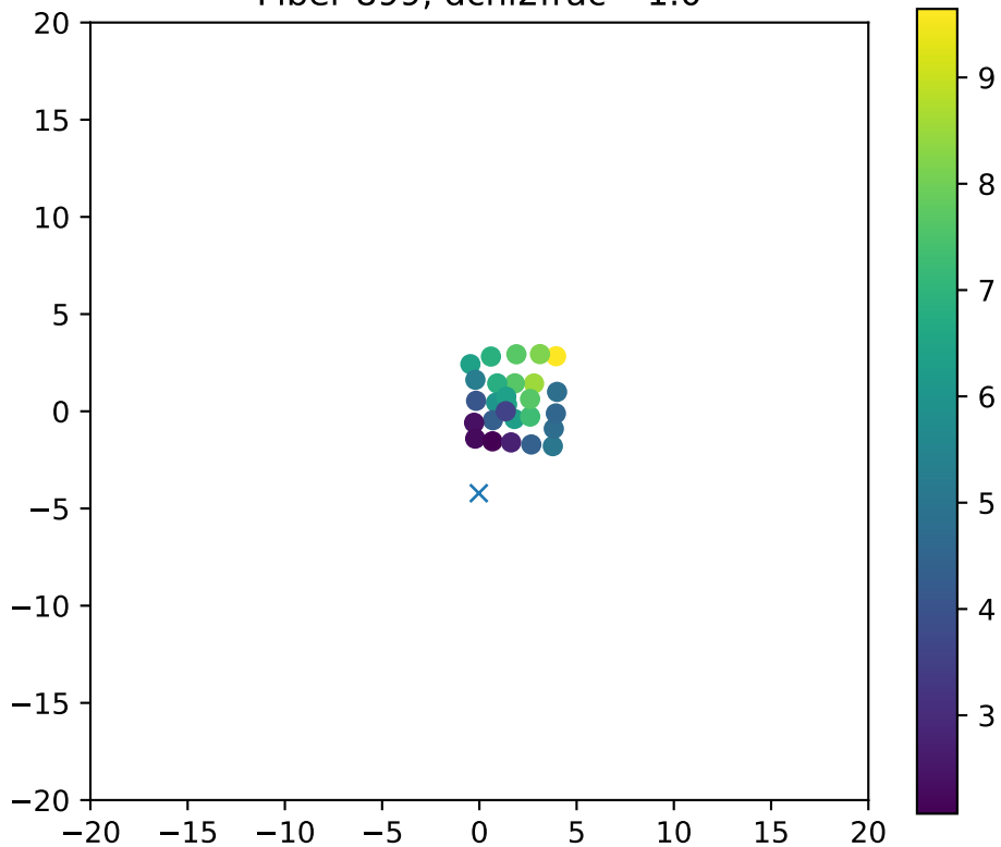
Fiber 899, dchi2frac= 1.0
