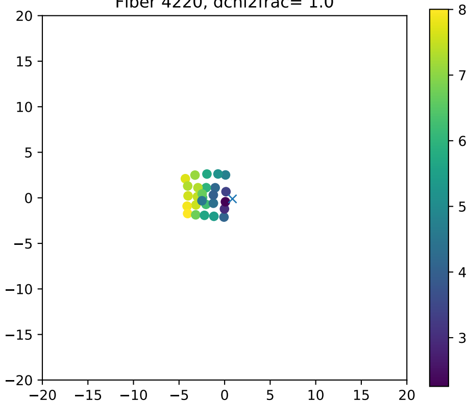
Fiber 4220, dchi2frac= 1.0
