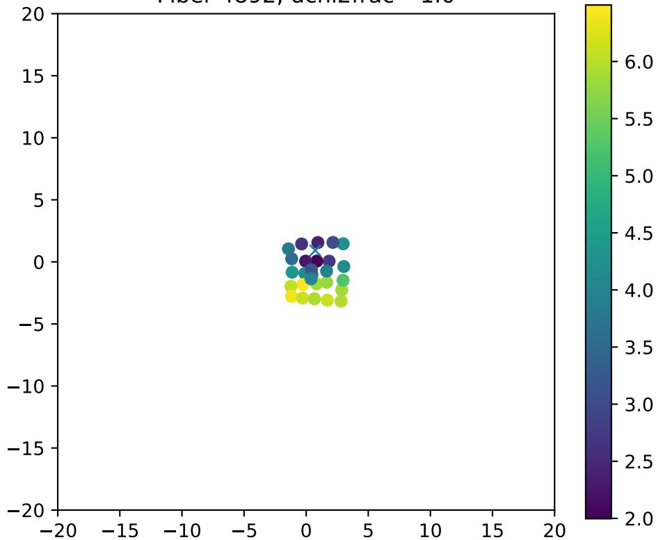
Fiber 4892, dchi2frac= 1.0
