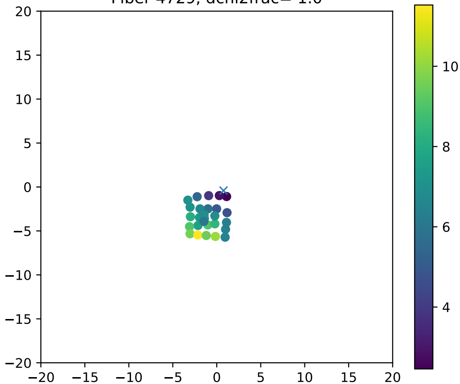
Fiber 4729, dchi2frac= 1.0
