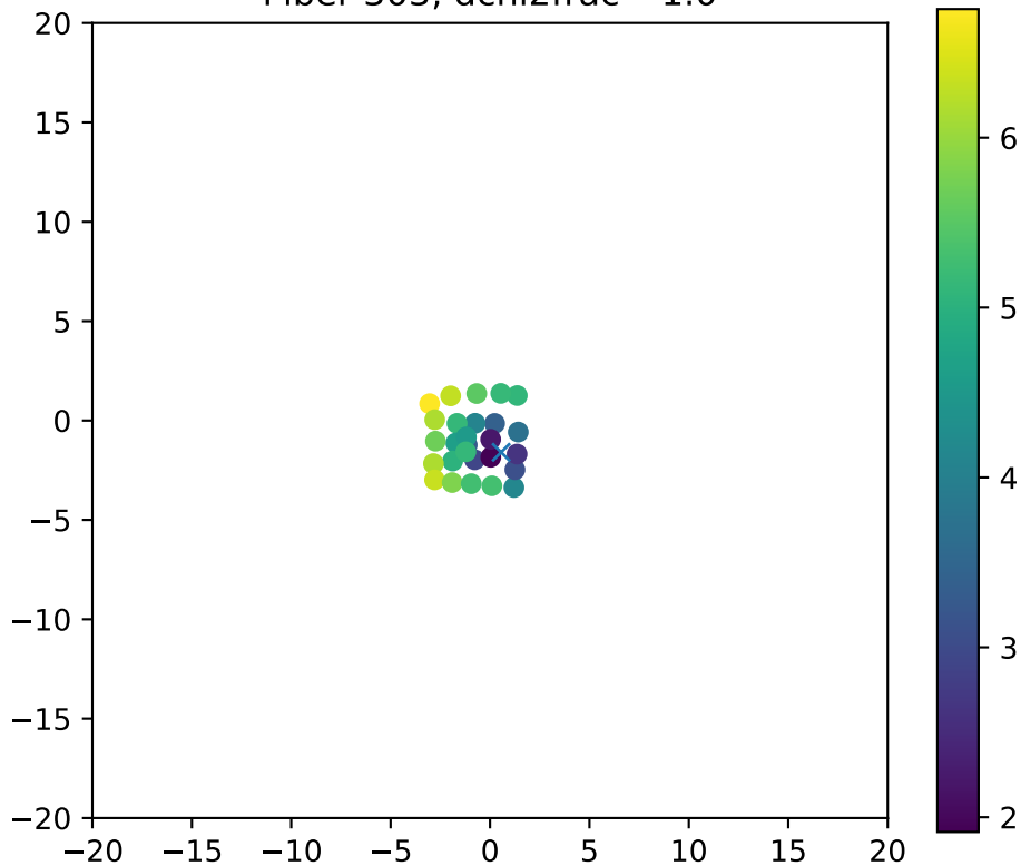
Fiber 303, dchi2frac= 1.0
