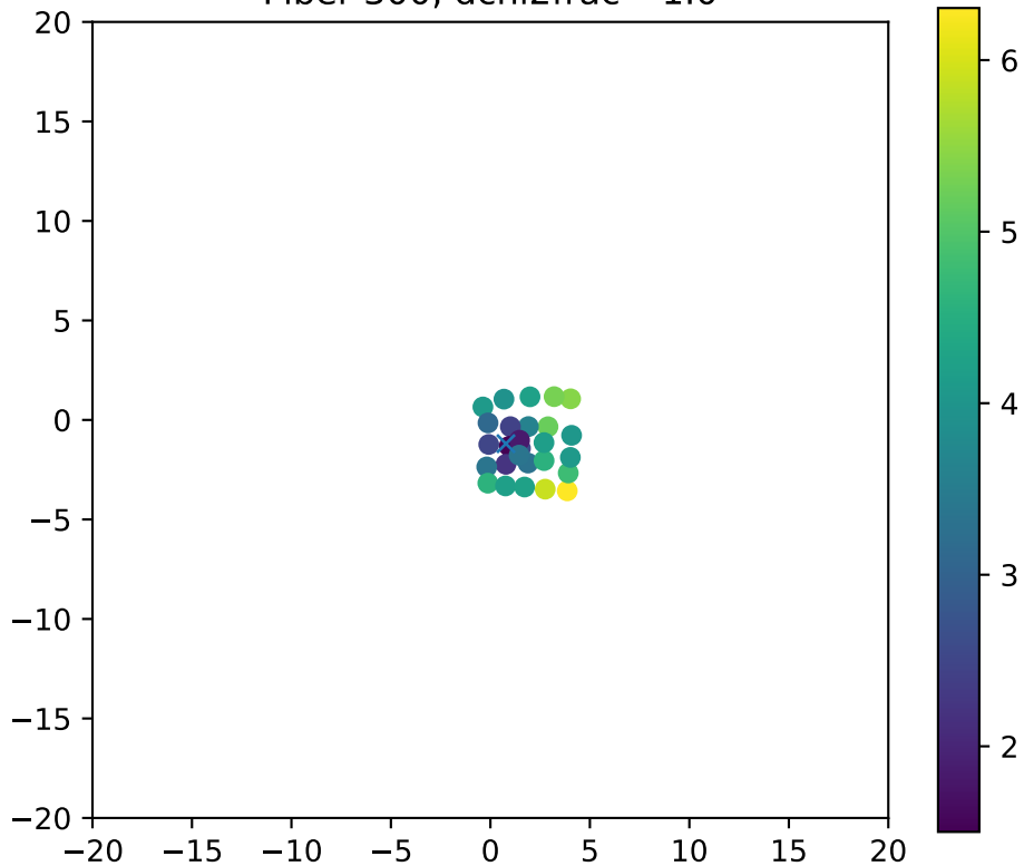
Fiber 300, dchi2frac= 1.0
