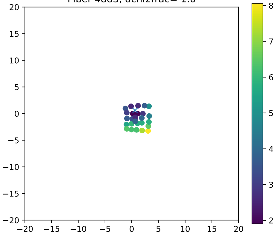
Fiber 4883, dchi2frac= 1.0
