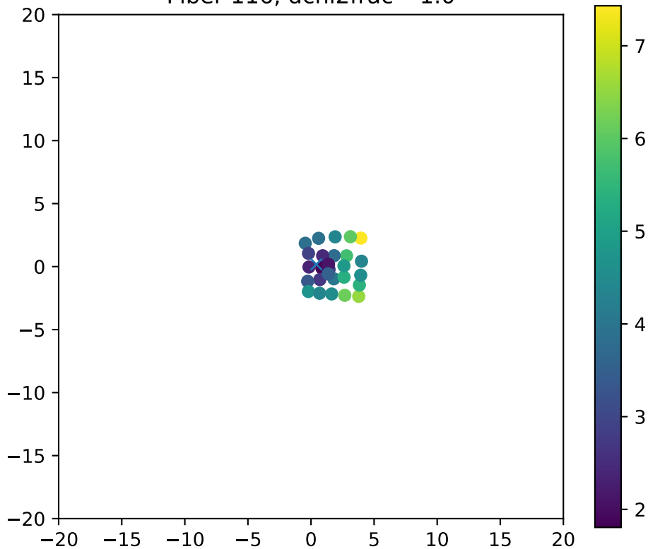
Fiber 116, dchi2frac= 1.0
