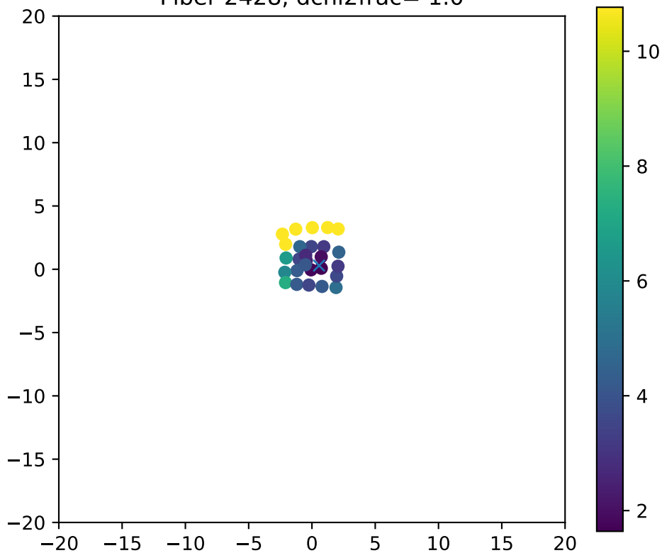
Fiber 2428, dchi2frac= 1.0
