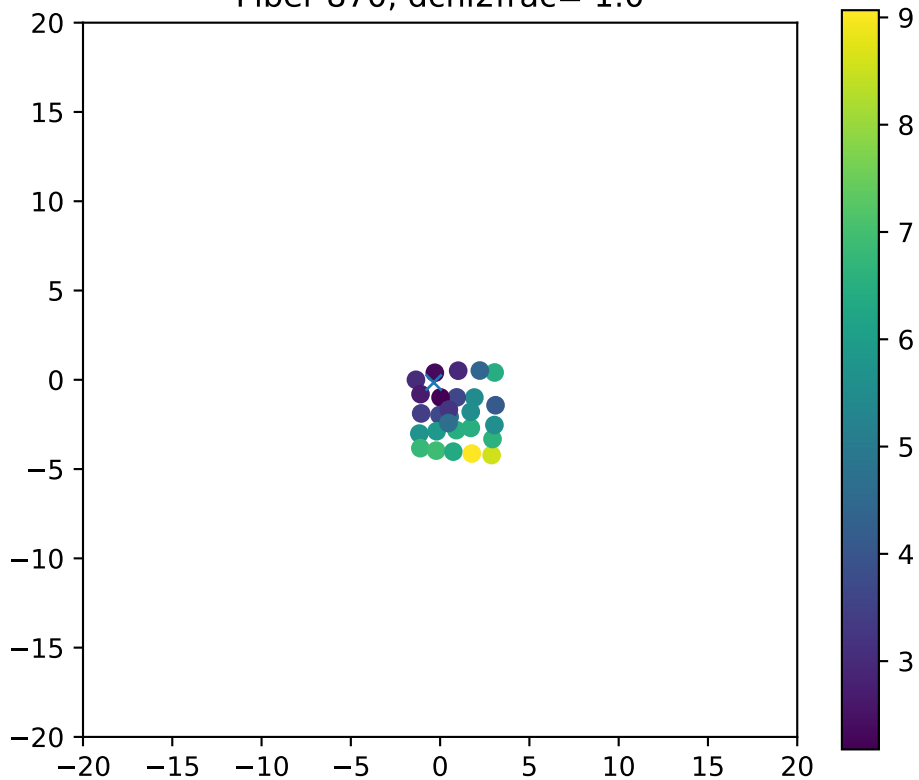
Fiber 870, dchi2frac= 1.0
