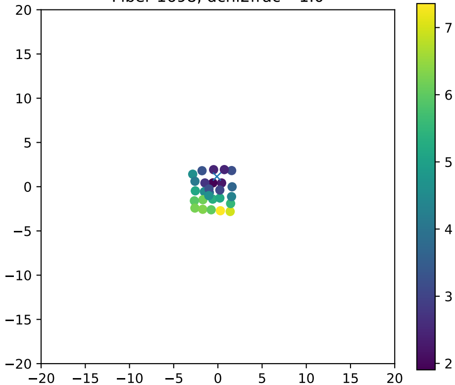
Fiber 1698, dchi2frac= 1.0
