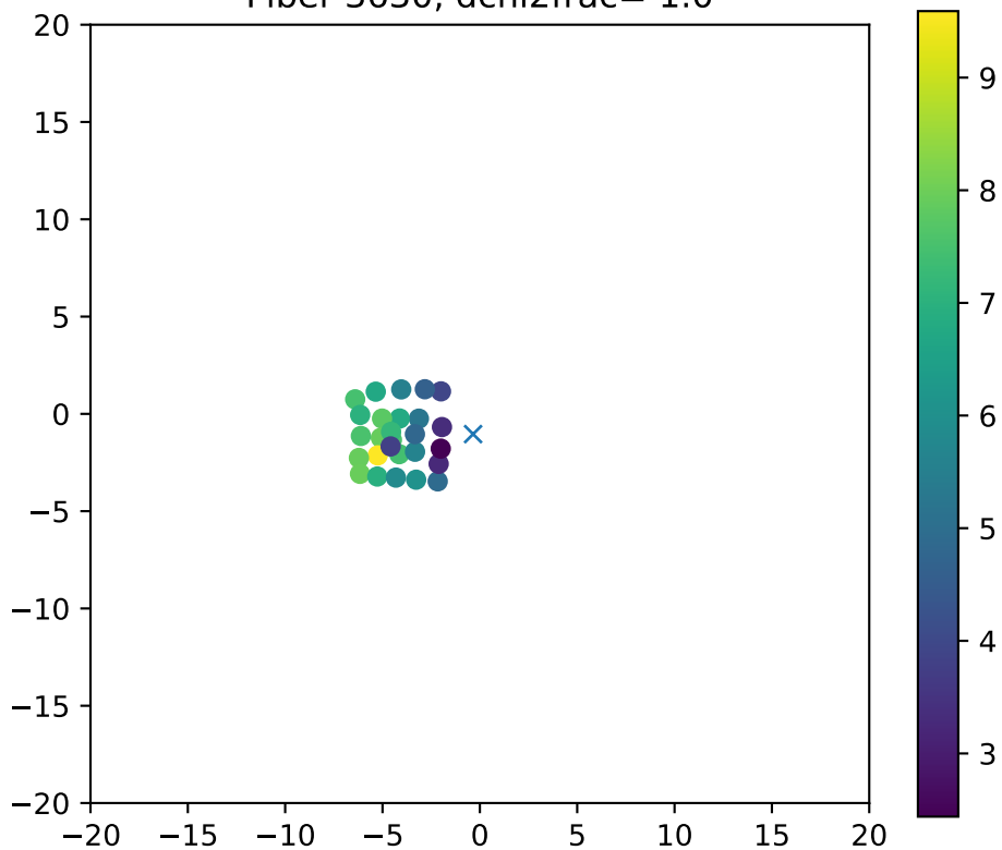
Fiber 3630, dchi2frac= 1.0
