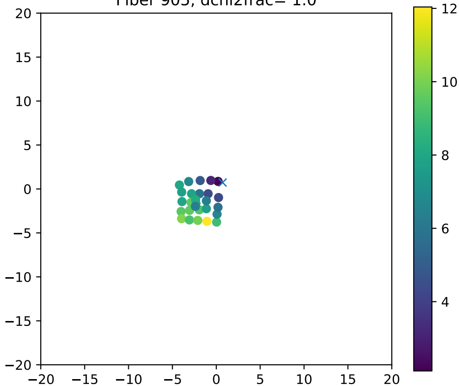
Fiber 905, dchi2frac= 1.0
