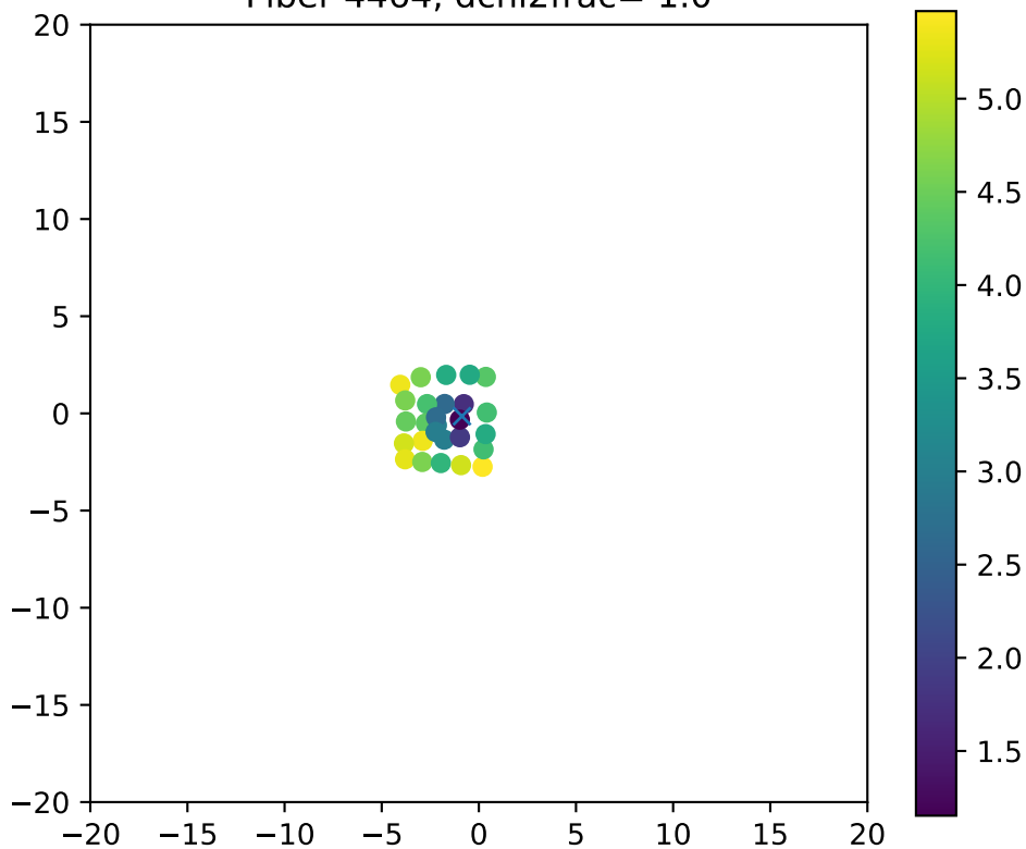
Fiber 4464, dchi2frac= 1.0
