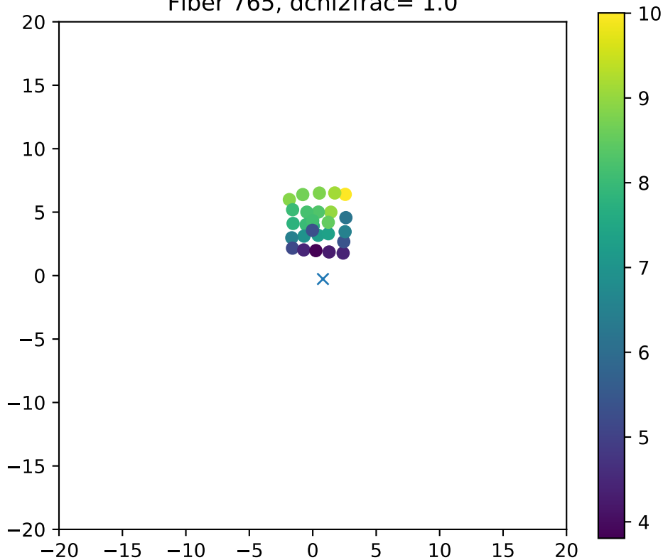
Fiber 765, dchi2frac= 1.0
