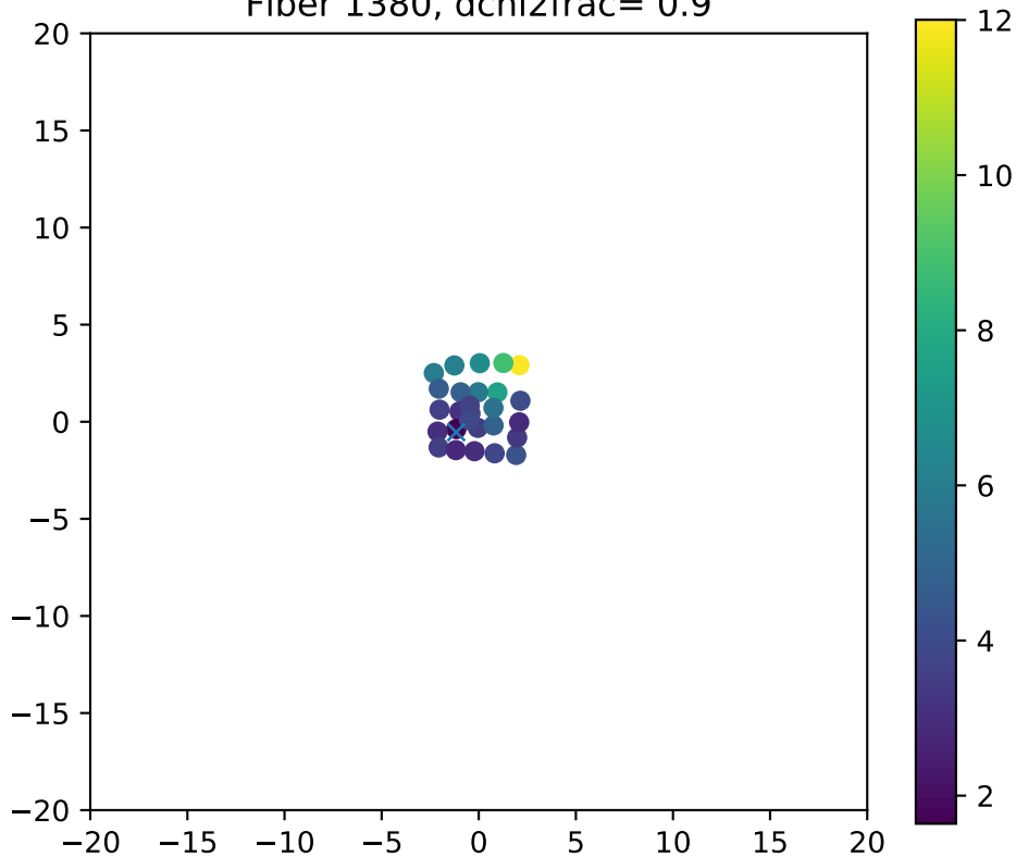
Fiber 1380, dchi2frac= 0.9
