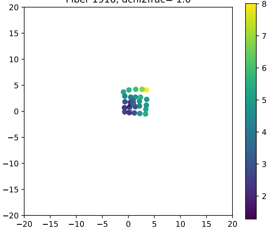
Fiber 1916, dchi2frac= 1.0
