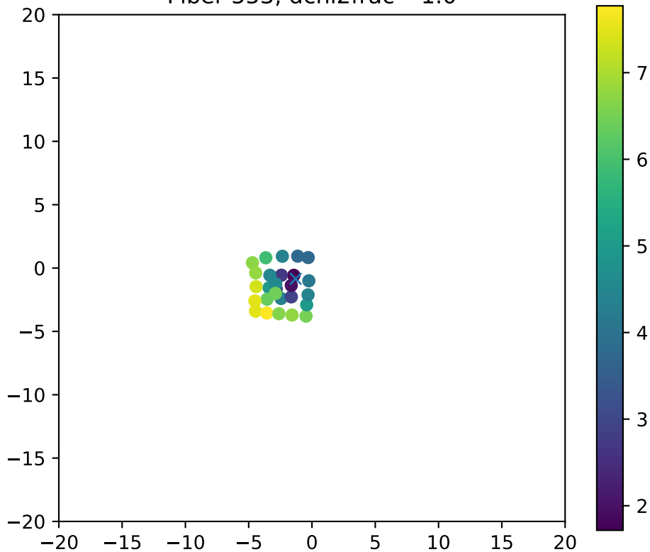
Fiber 553, dchi2frac= 1.0
