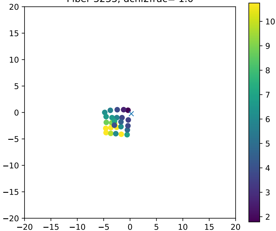
Fiber 3233, dchi2frac= 1.0
