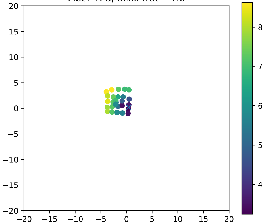
Fiber 128, dchi2frac= 1.0
