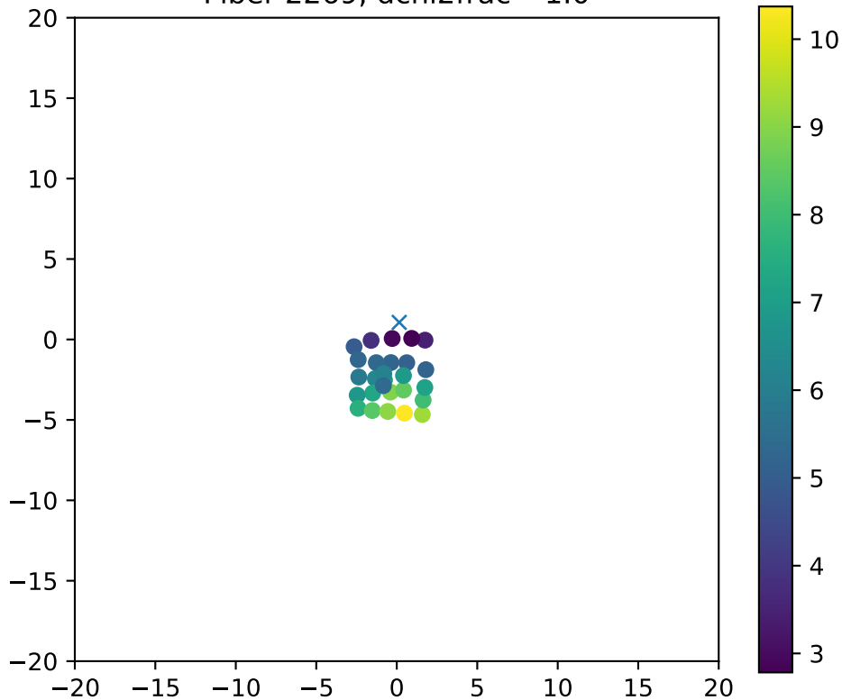
Fiber 2269, dchi2frac= 1.0
