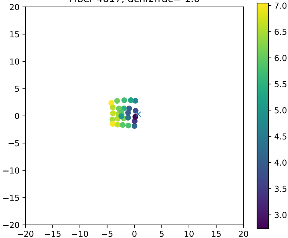
Fiber 4617, dchi2frac= 1.0
