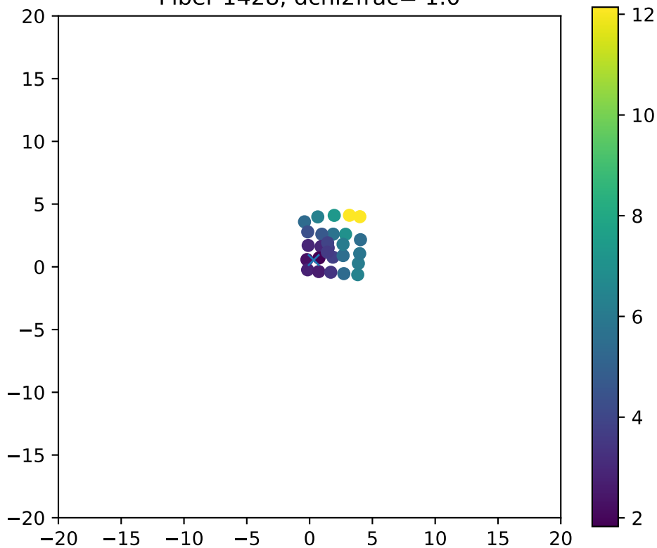
Fiber 1428, dchi2frac= 1.0
