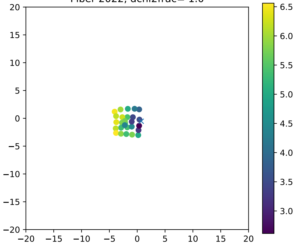
Fiber 2022, dchi2frac= 1.0
