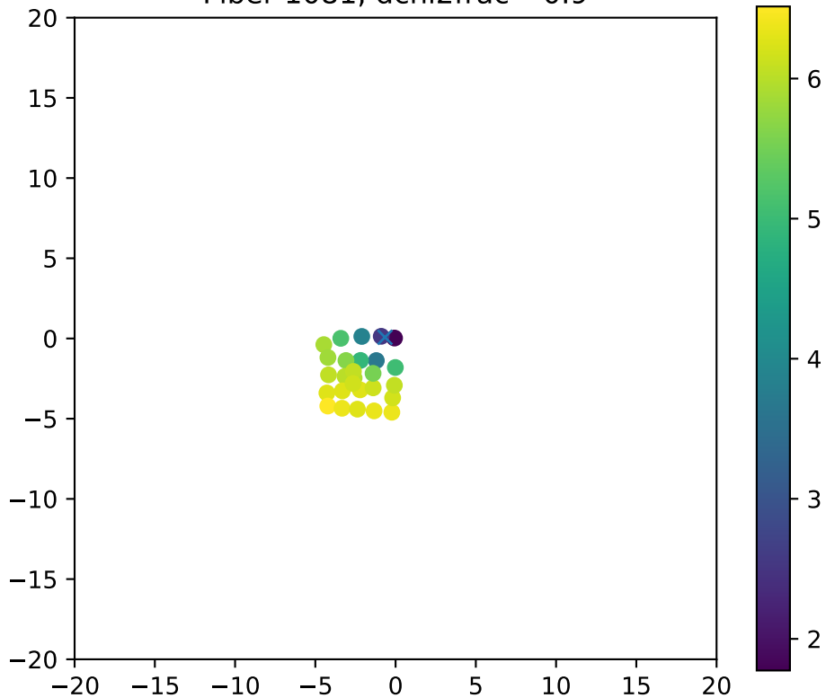
Fiber 1081, dchi2frac= 0.9
