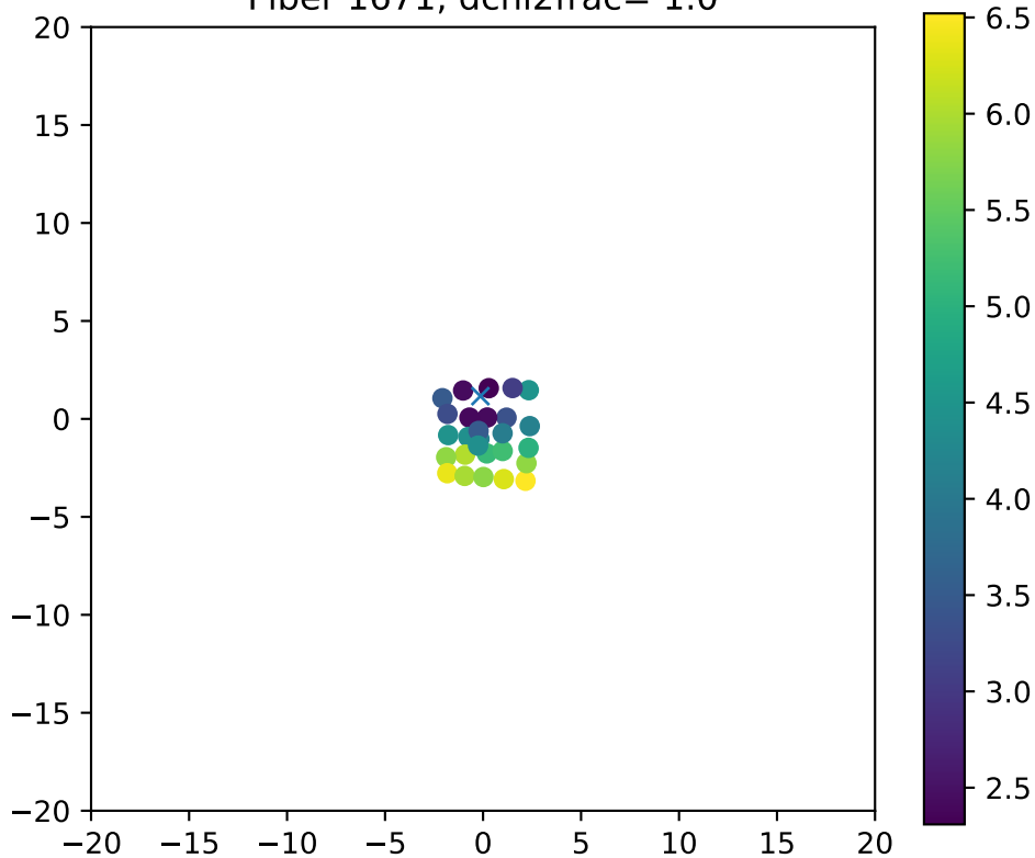
Fiber 1671, dchi2frac= 1.0
