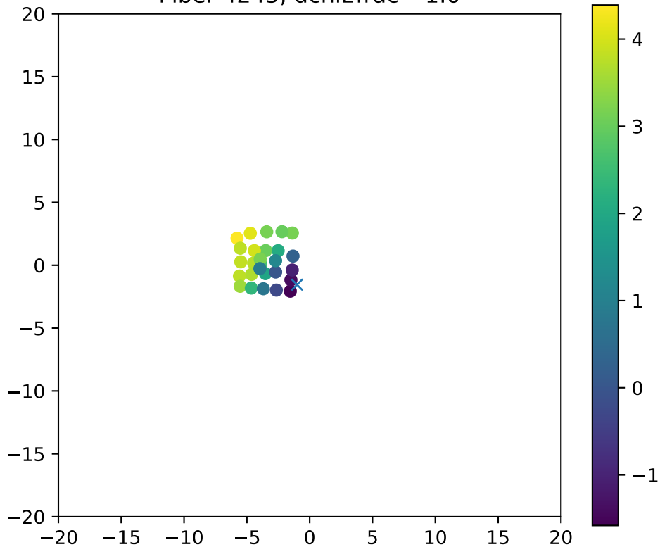
Fiber 4245, dchi2frac= 1.0
