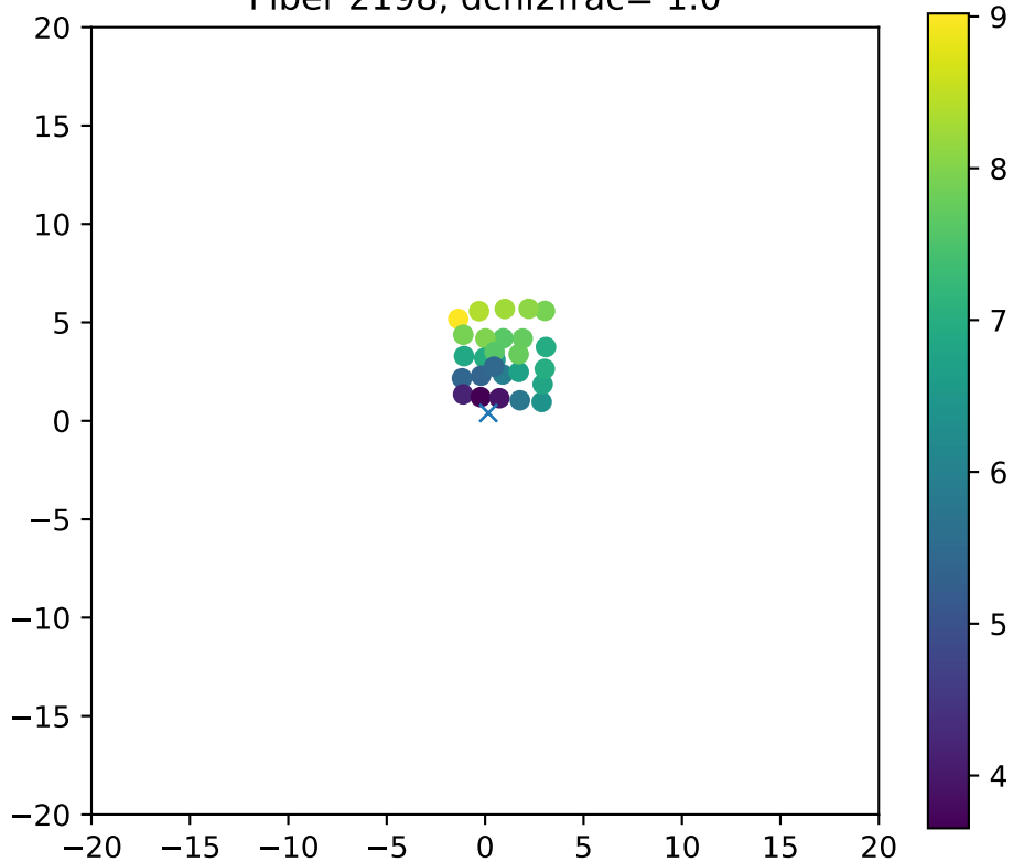
Fiber 2198, dchi2frac= 1.0
