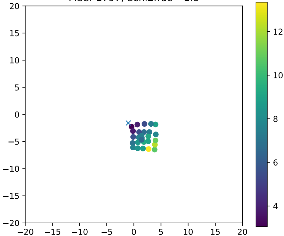
Fiber 2797, dchi2frac= 1.0
