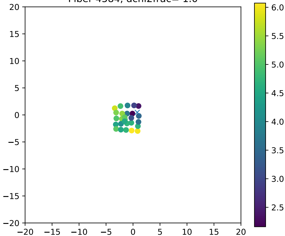
Fiber 4584, dchi2frac= 1.0
