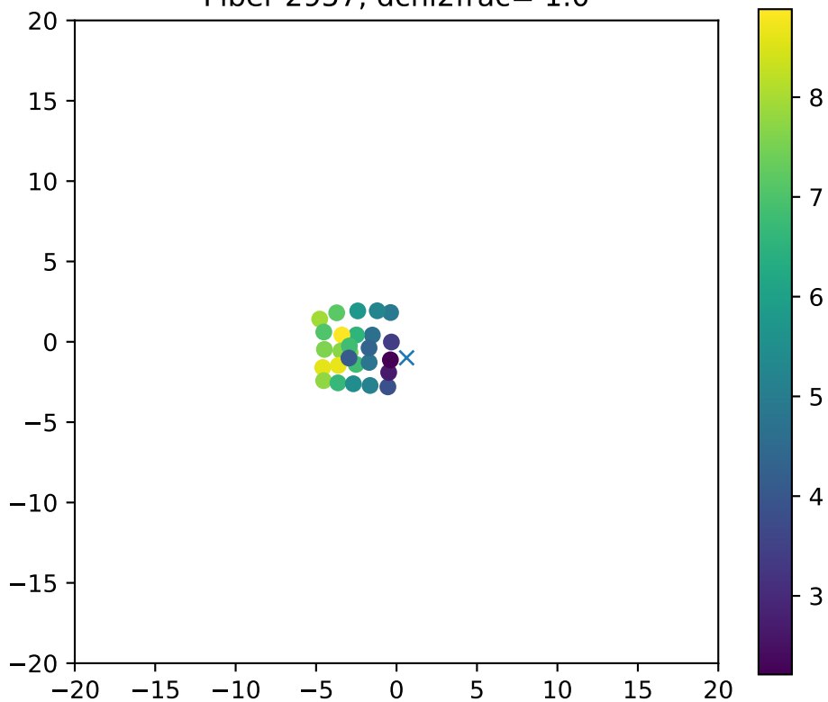
Fiber 2957, dchi2frac= 1.0
