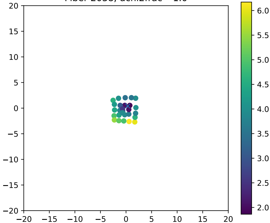
Fiber 2038, dchi2frac= 1.0
