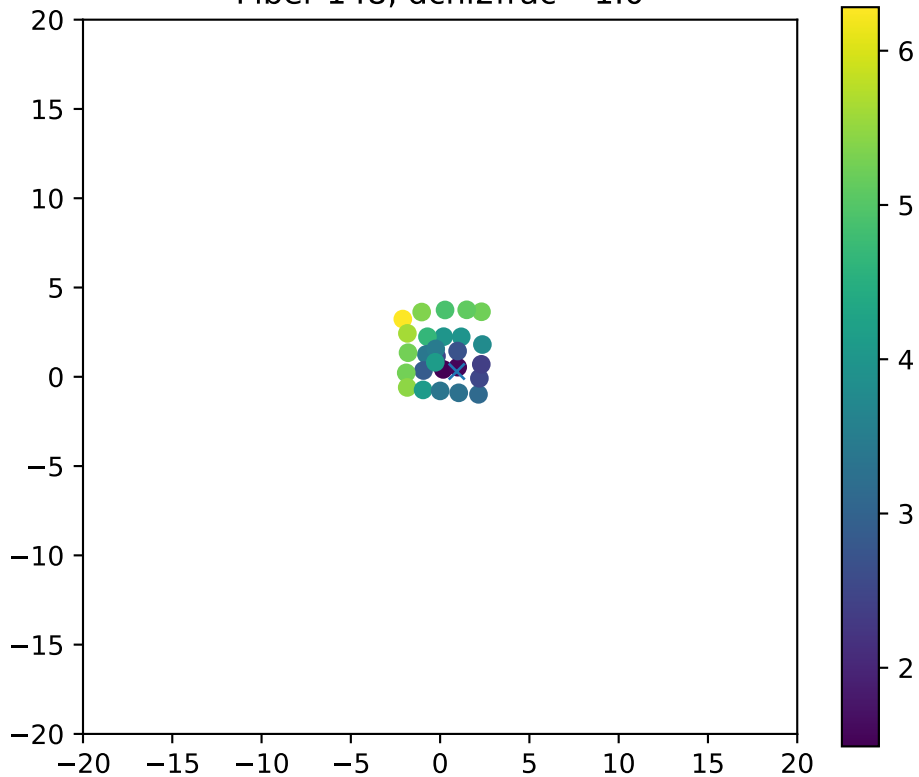
Fiber 148, dchi2frac= 1.0
