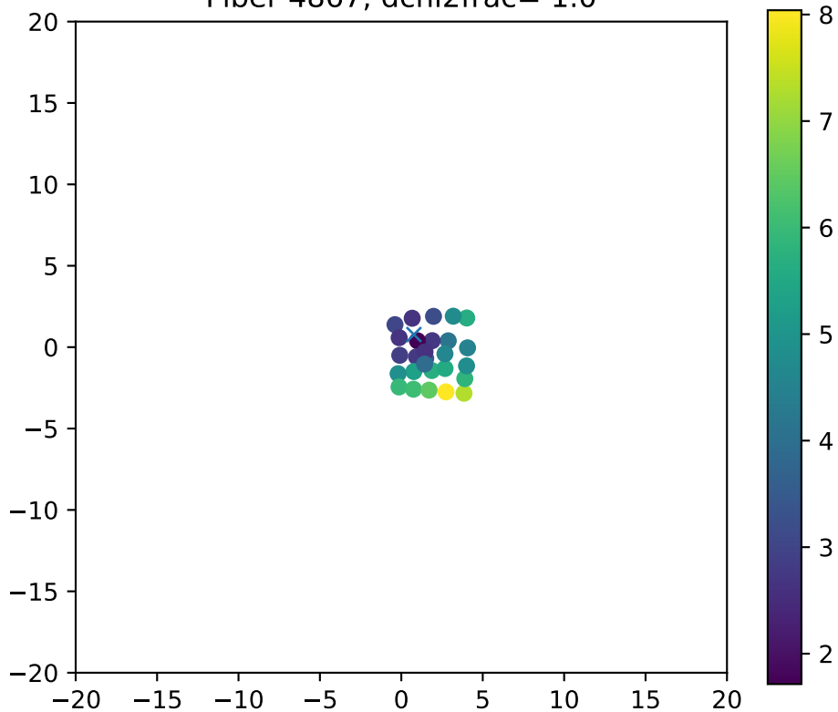
Fiber 4867, dchi2frac= 1.0
