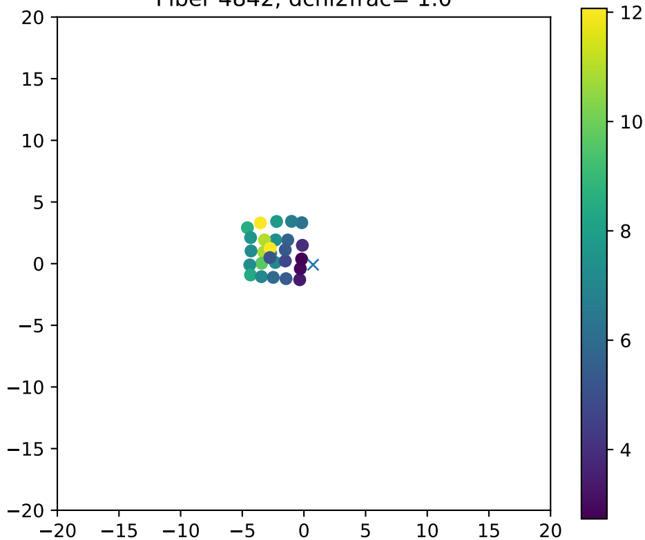
Fiber 4842, dchi2frac= 1.0
