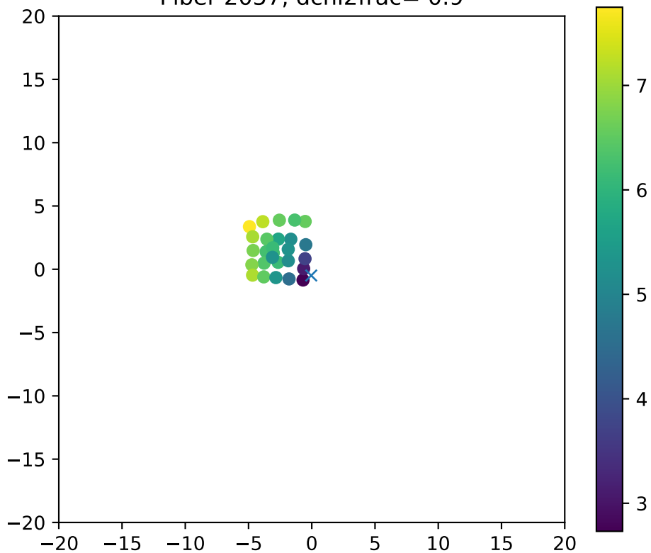
Fiber 2057, dchi2frac= 0.9
