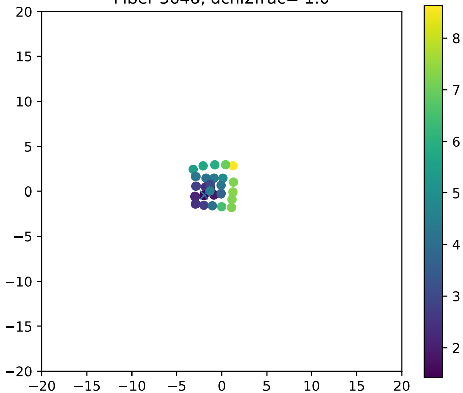
Fiber 3646, dchi2frac= 1.0
