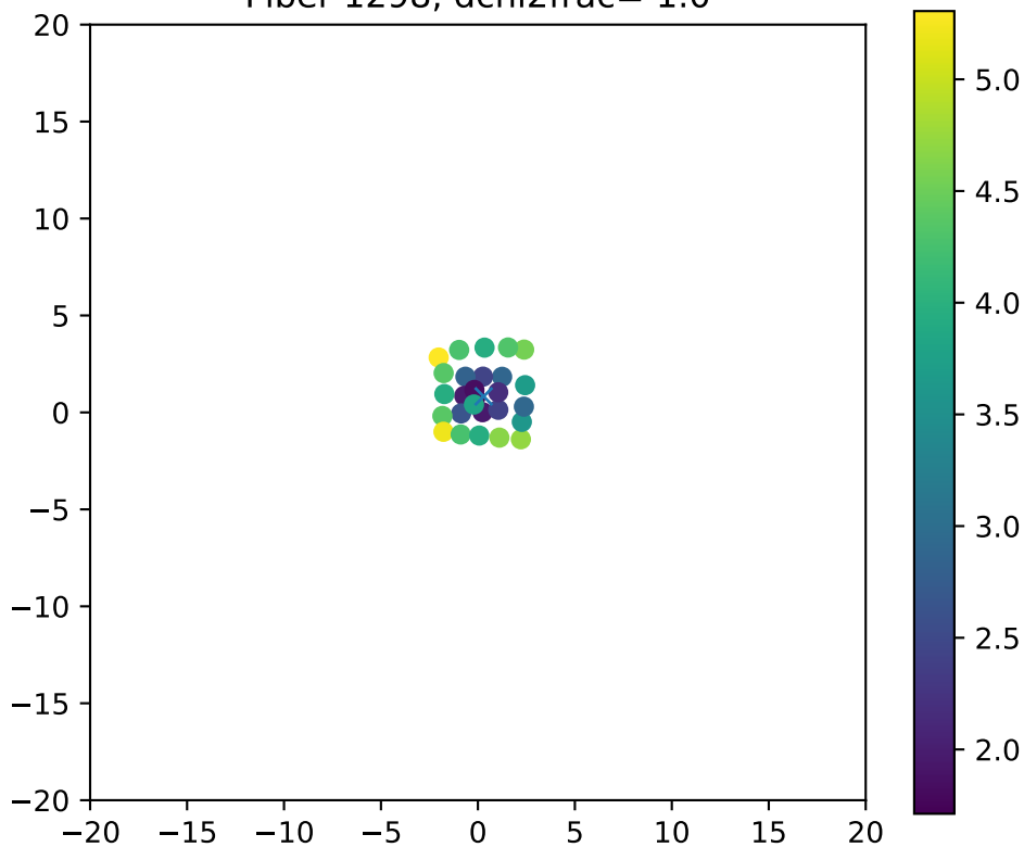
Fiber 1298, dchi2frac= 1.0
