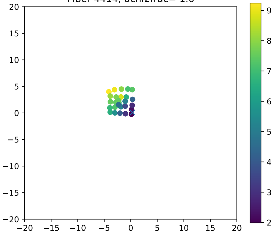
Fiber 4414, dchi2frac= 1.0
