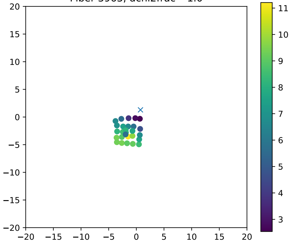
Fiber 3963, dchi2frac= 1.0
