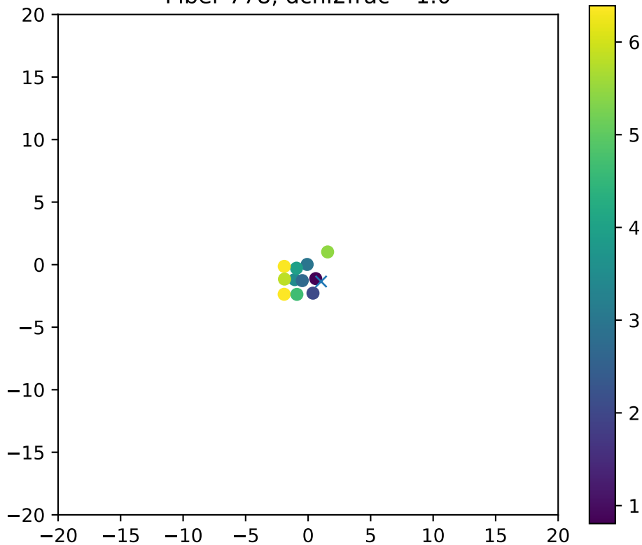
Fiber 778, dchi2frac= 1.0
