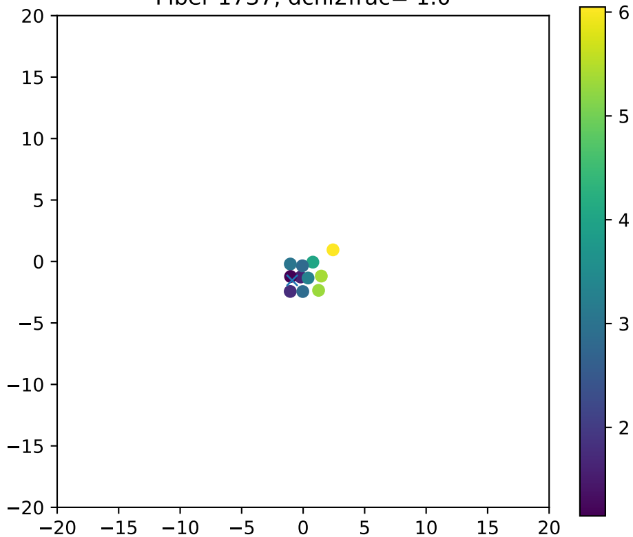
Fiber 1737, dchi2frac= 1.0
