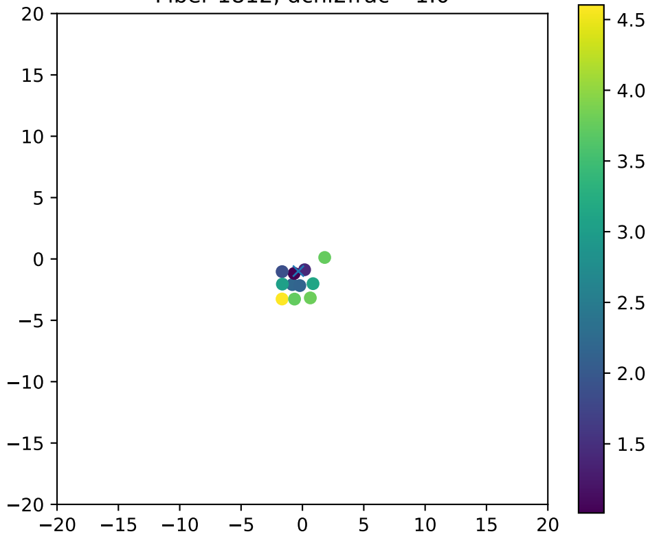
Fiber 1812, dchi2frac= 1.0
