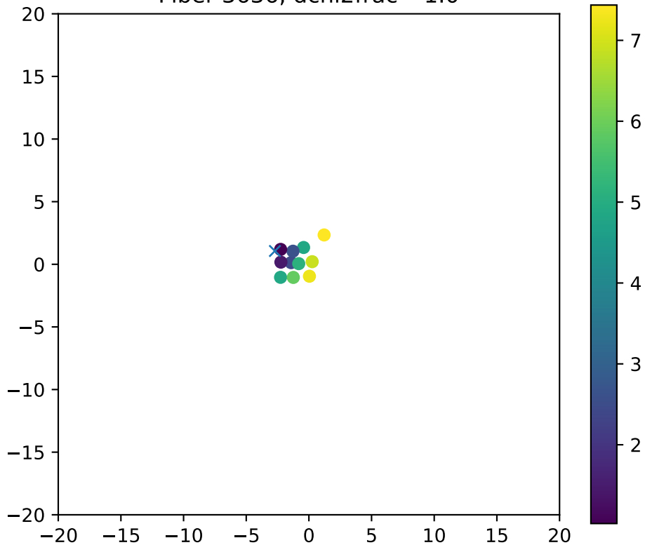
Fiber 3636, dchi2frac= 1.0
