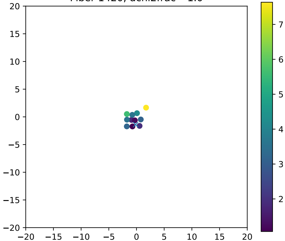
Fiber 1420, dchi2frac= 1.0
