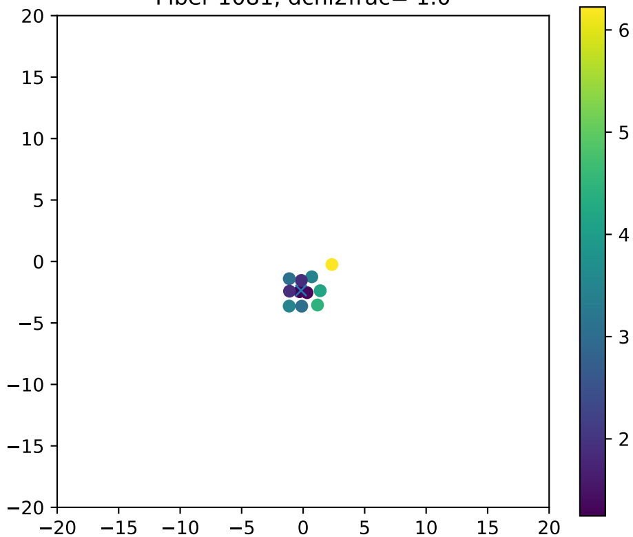
Fiber 1081, dchi2frac= 1.0
