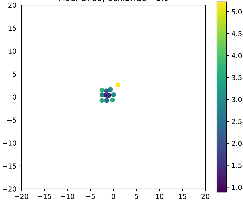
Fiber 3705, dchi2frac= 1.0
