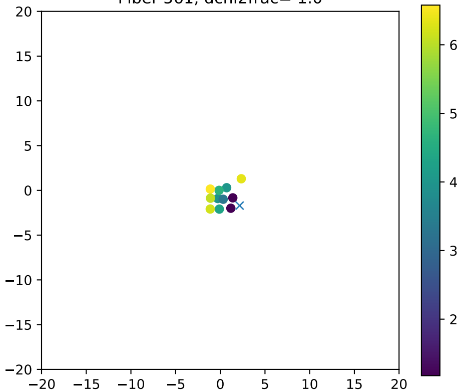
Fiber 561, dchi2frac= 1.0
