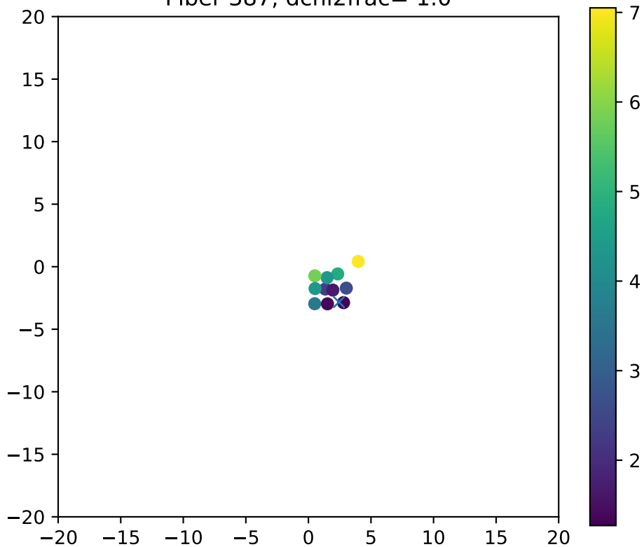
Fiber 387, dchi2frac= 1.0
