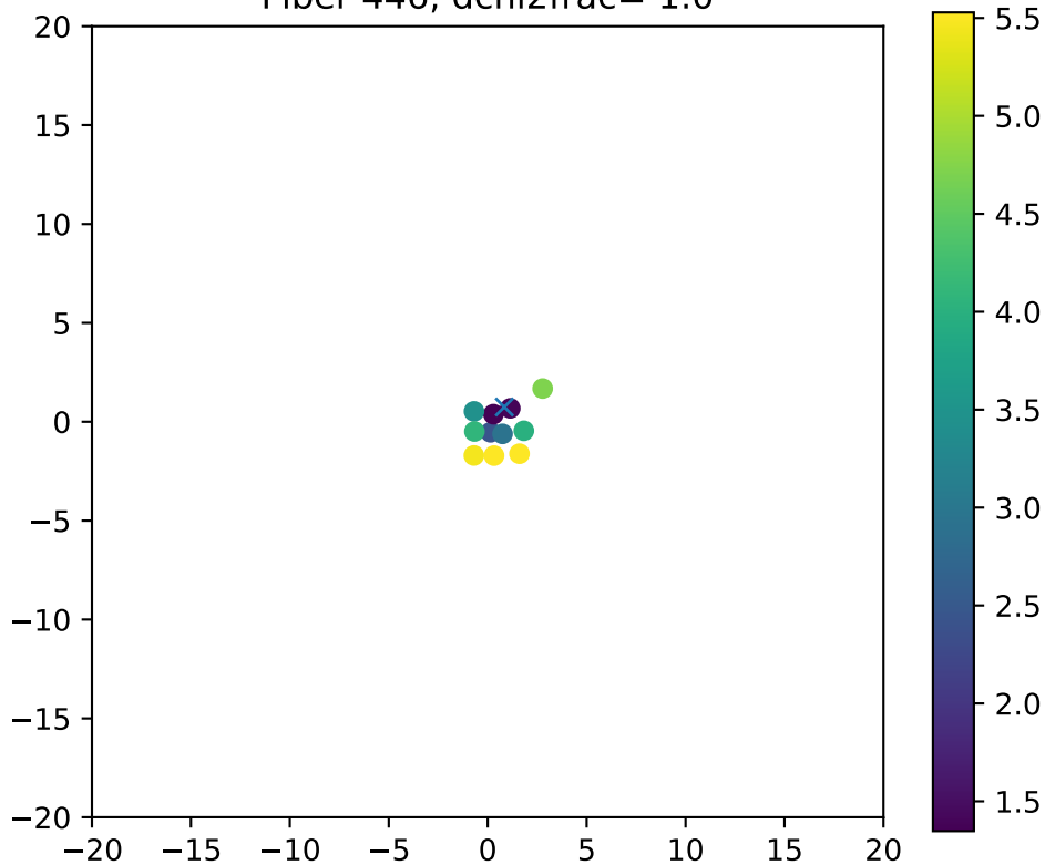
Fiber 446, dchi2frac= 1.0
