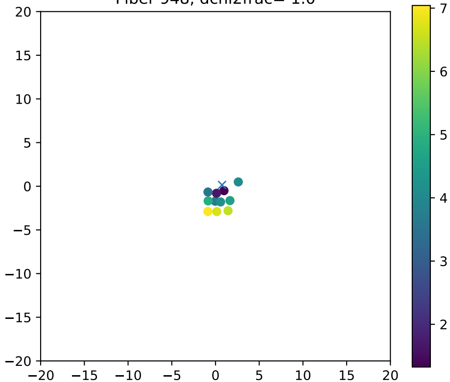
Fiber 948, dchi2frac= 1.0
