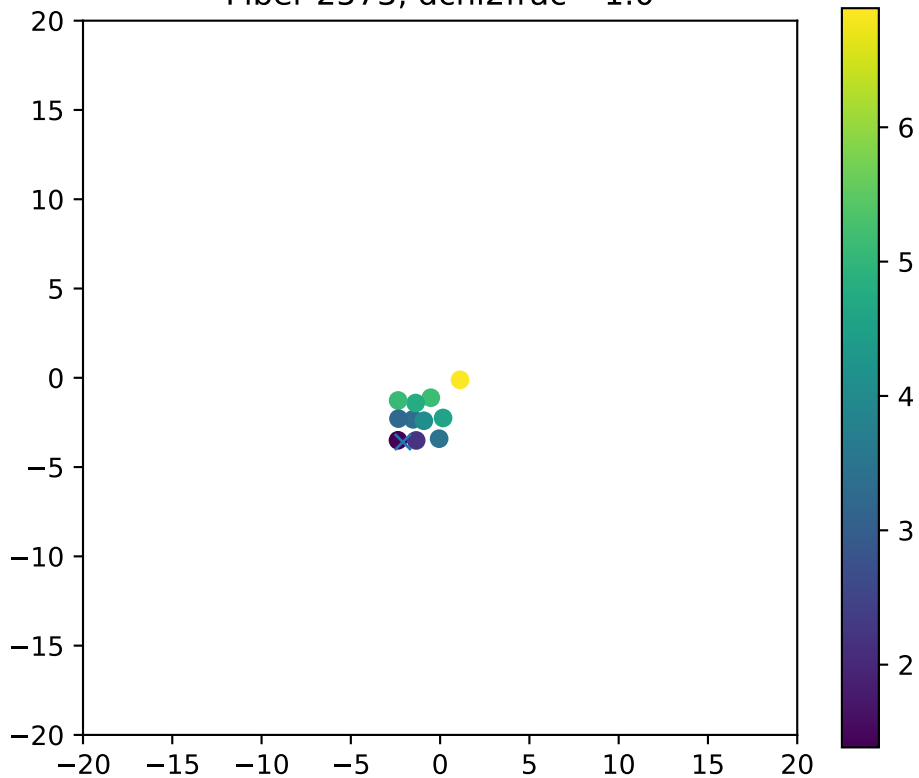
Fiber 2573, dchi2frac= 1.0
