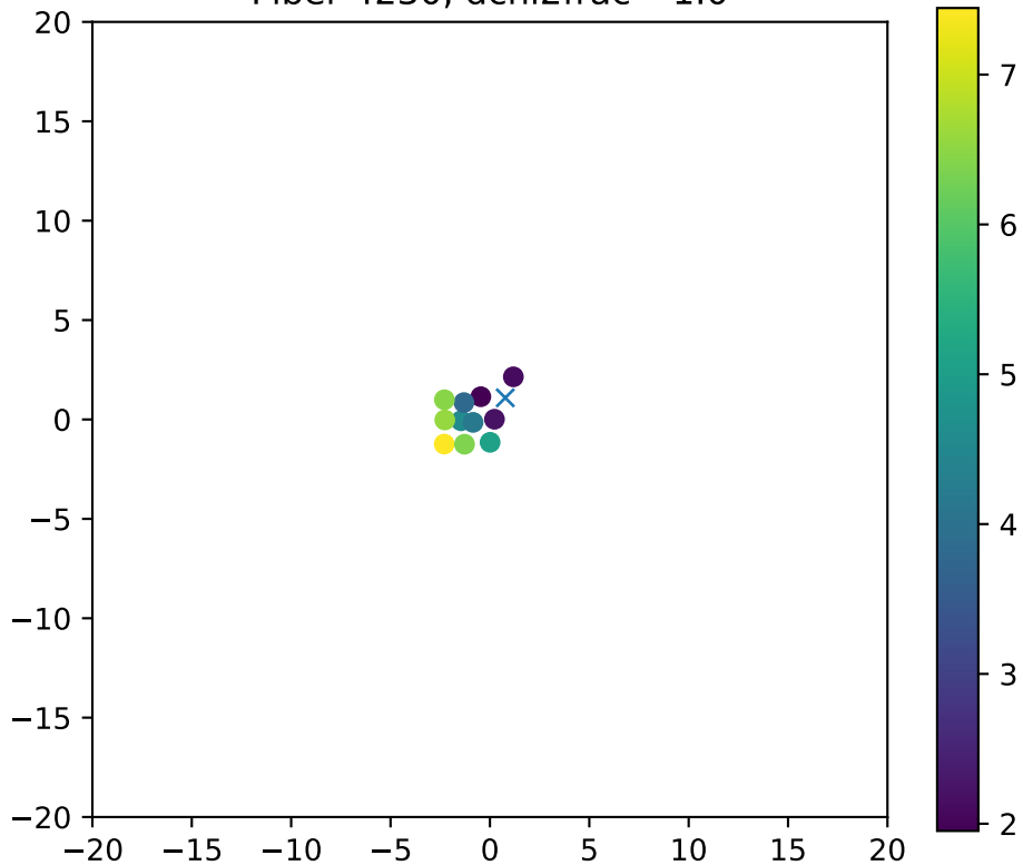
Fiber 4230, dchi2frac= 1.0
