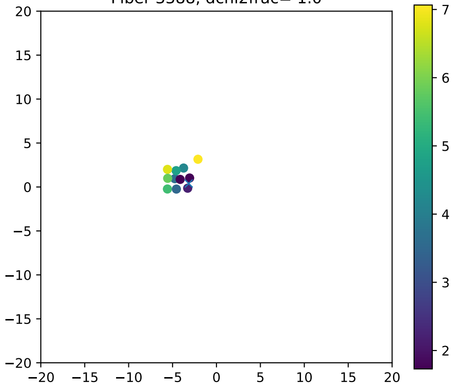
Fiber 3388, dchi2frac= 1.0
