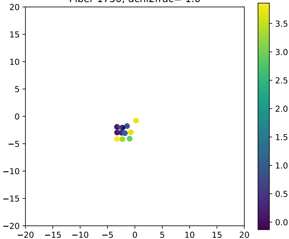
Fiber 1750, dchi2frac= 1.0
