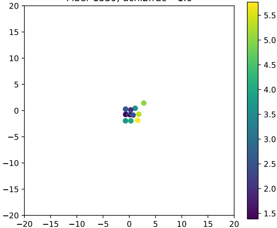
Fiber 1539, dchi2frac= 1.0
