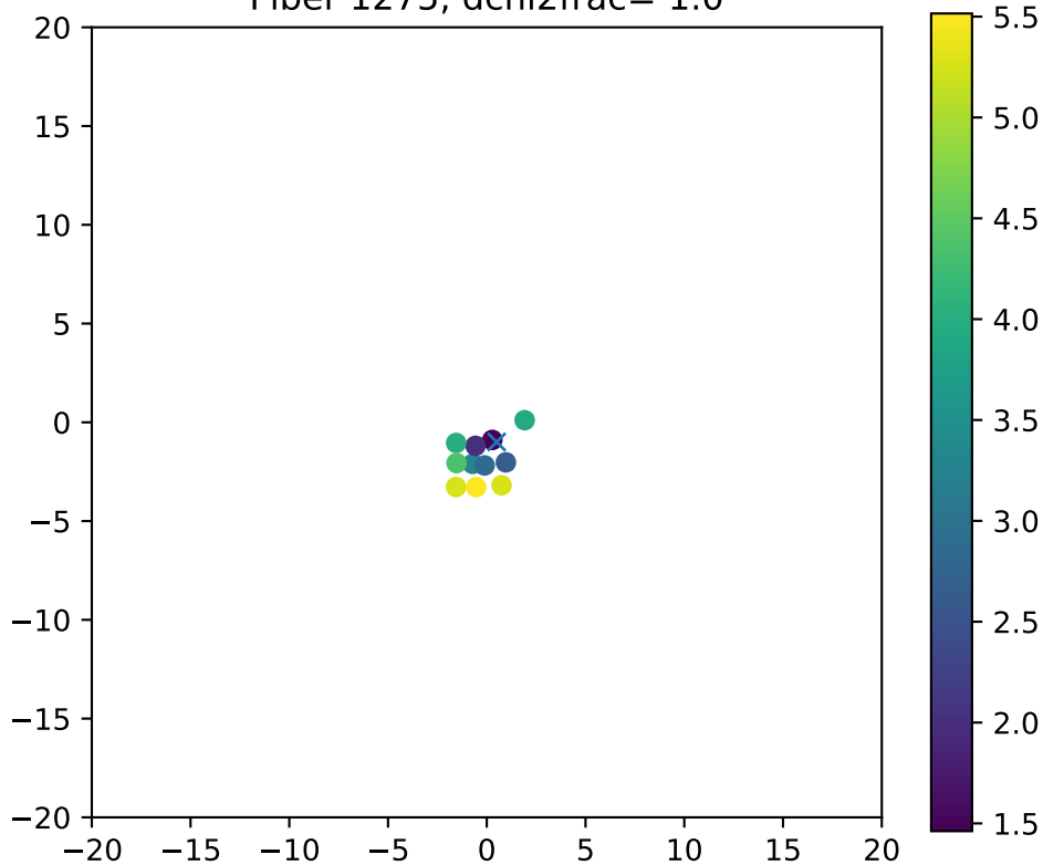
Fiber 1275, dchi2frac= 1.0
