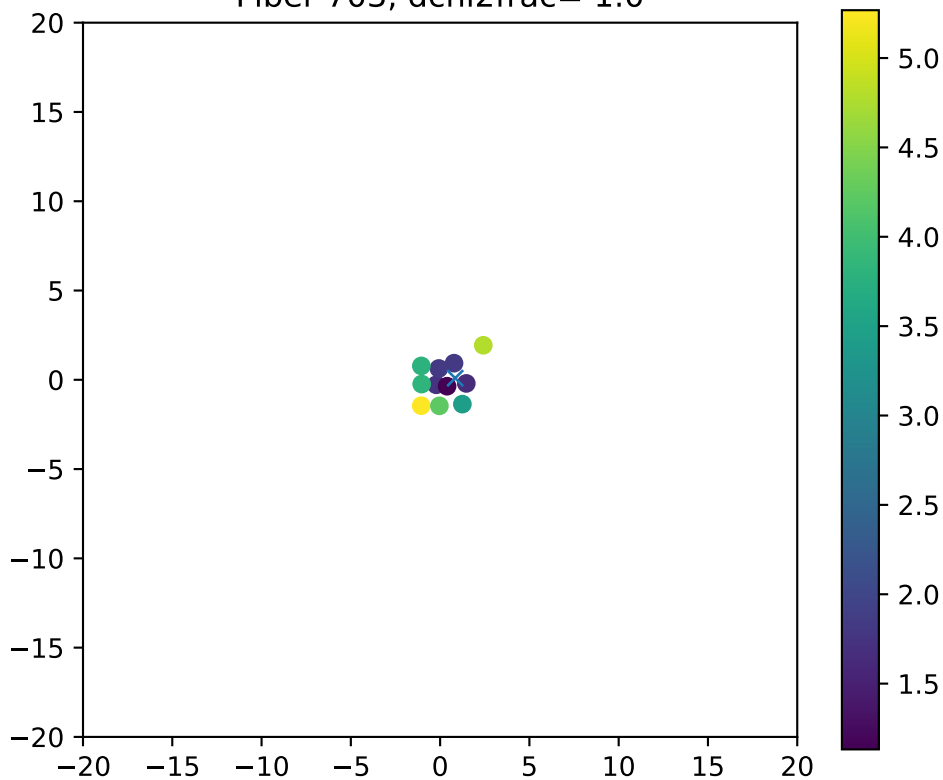
Fiber 703, dchi2frac= 1.0
