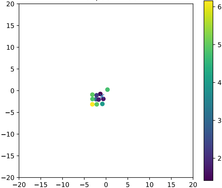
Fiber 2458, dchi2frac= 1.0
