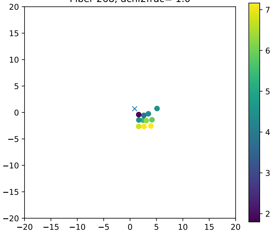
Fiber 268, dchi2frac= 1.0
