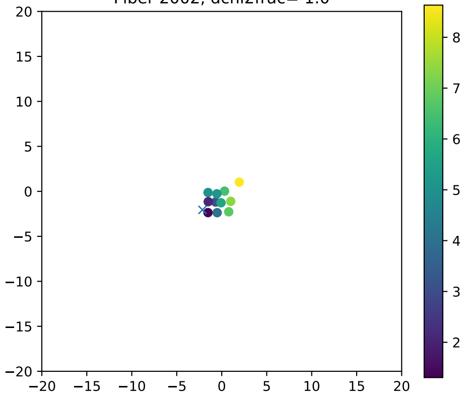
Fiber 2002, dchi2frac= 1.0
