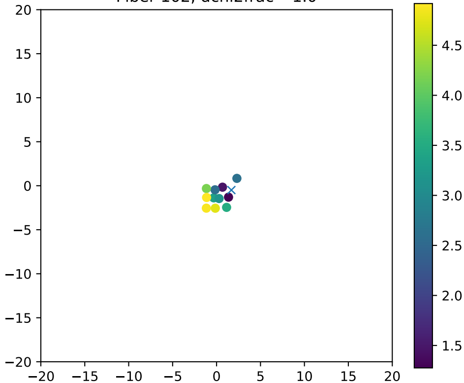
Fiber 102, dchi2frac= 1.0
