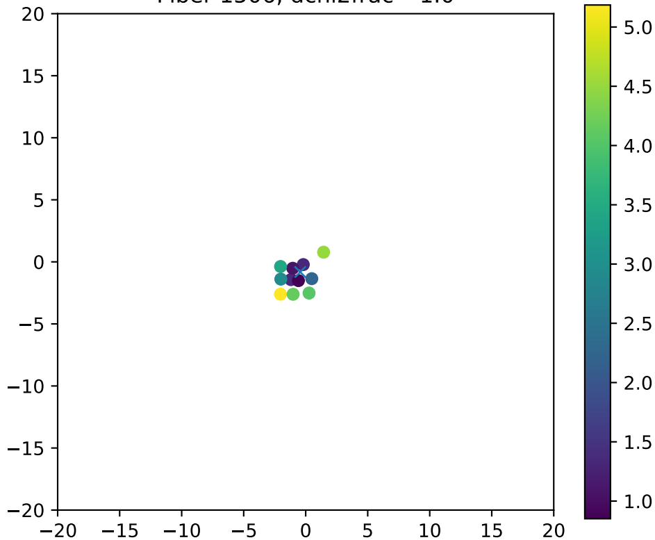
Fiber 1506, dchi2frac= 1.0
