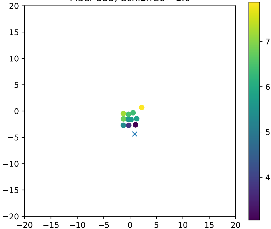
Fiber 533, dchi2frac= 1.0
