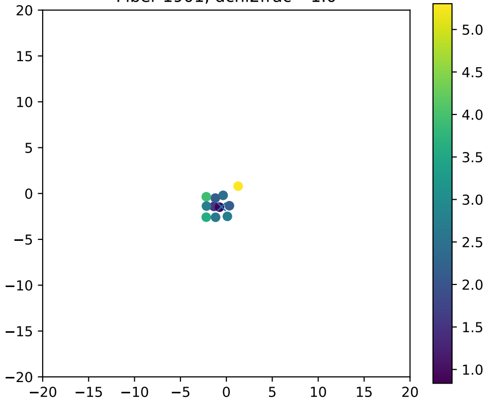
Fiber 1901, dchi2frac= 1.0
