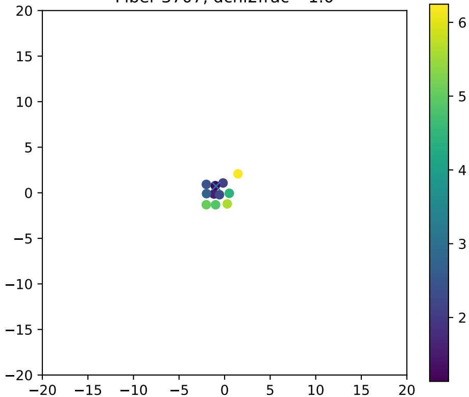
Fiber 3707, dchi2frac= 1.0
