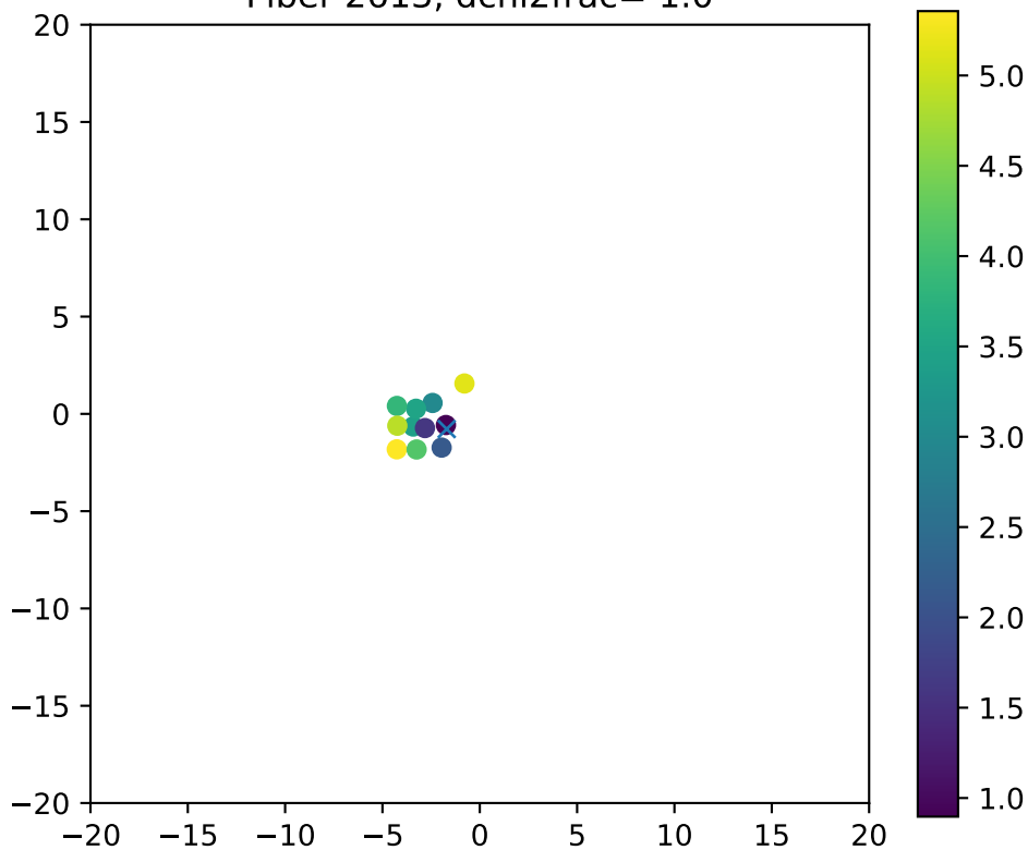
Fiber 2613, dchi2frac= 1.0
