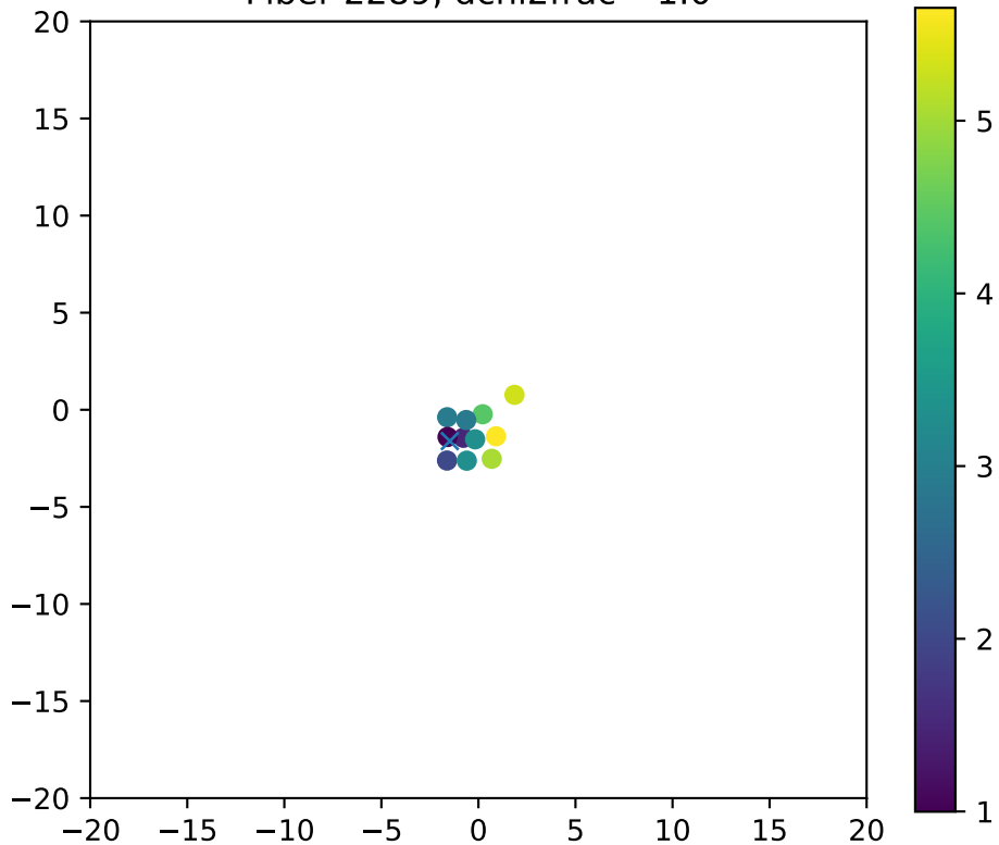
Fiber 2289, dchi2frac= 1.0
