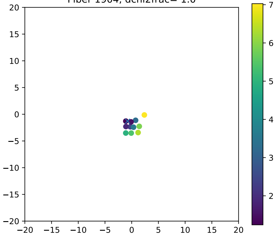
Fiber 1904, dchi2frac= 1.0
