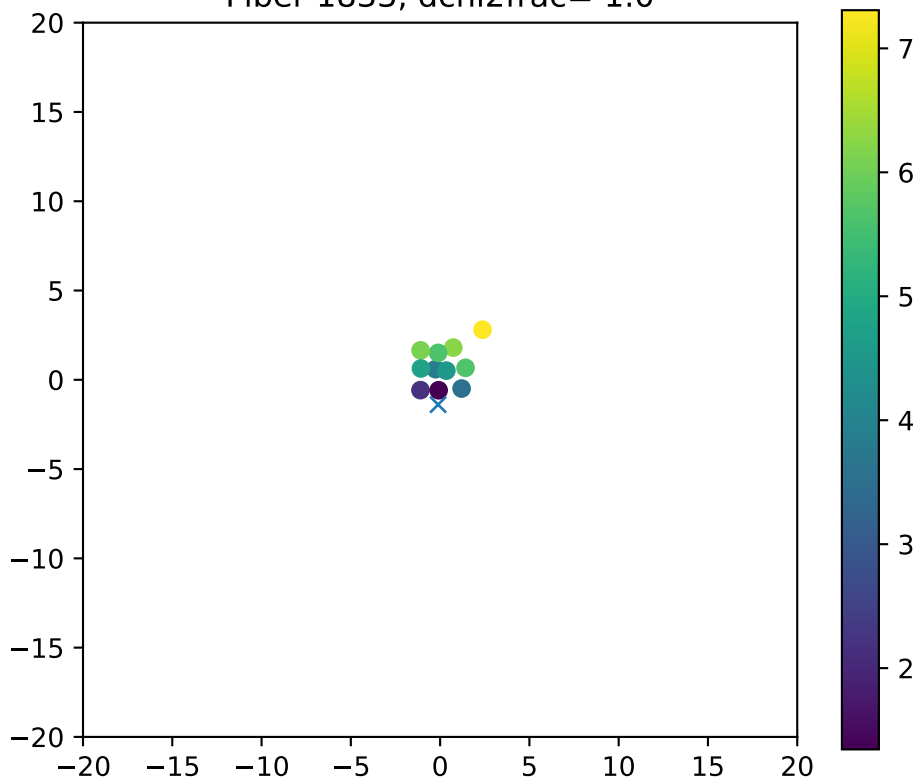
Fiber 1833, dchi2frac= 1.0
