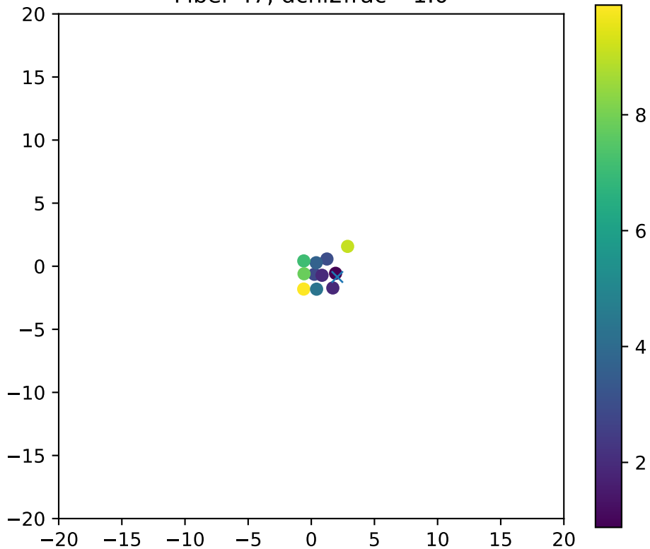
Fiber 47, dchi2frac= 1.0
