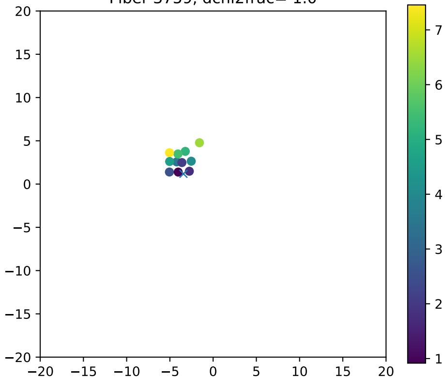
Fiber 3759, dchi2frac= 1.0
