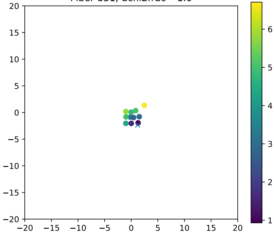
Fiber 831, dchi2frac= 1.0
