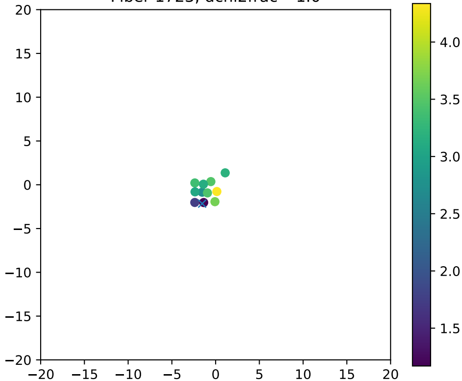
Fiber 1723, dchi2frac= 1.0
