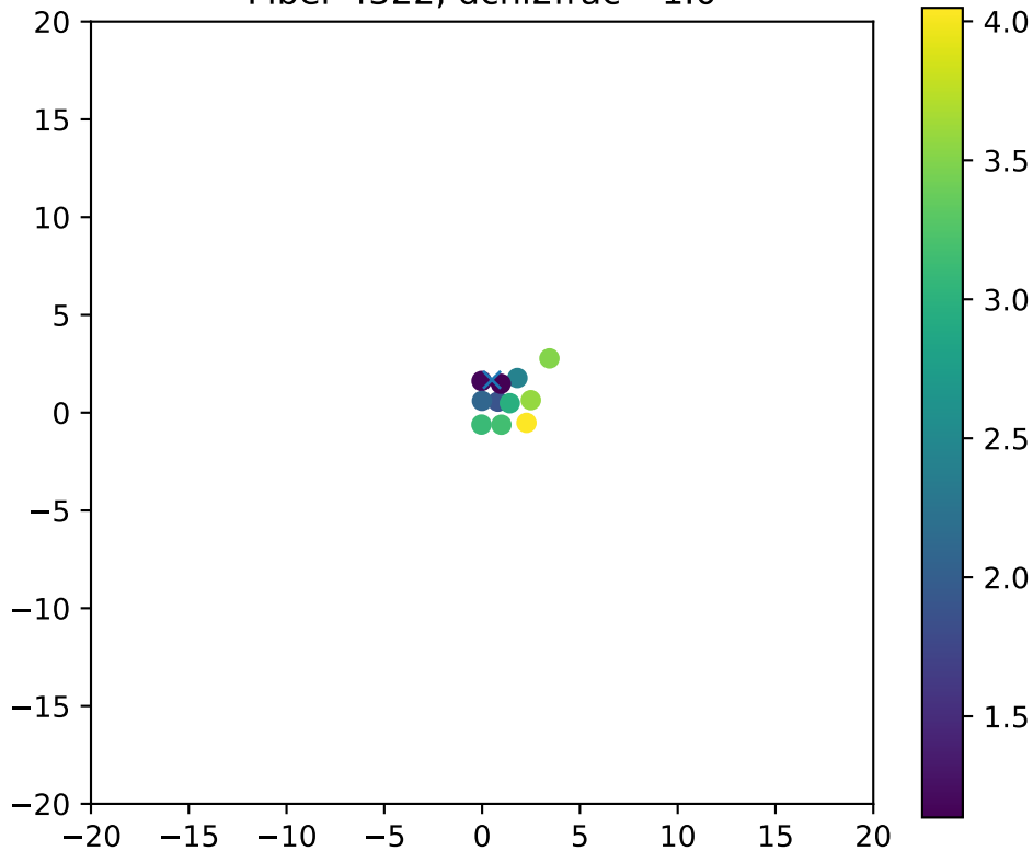
Fiber 4322, dchi2frac= 1.0
