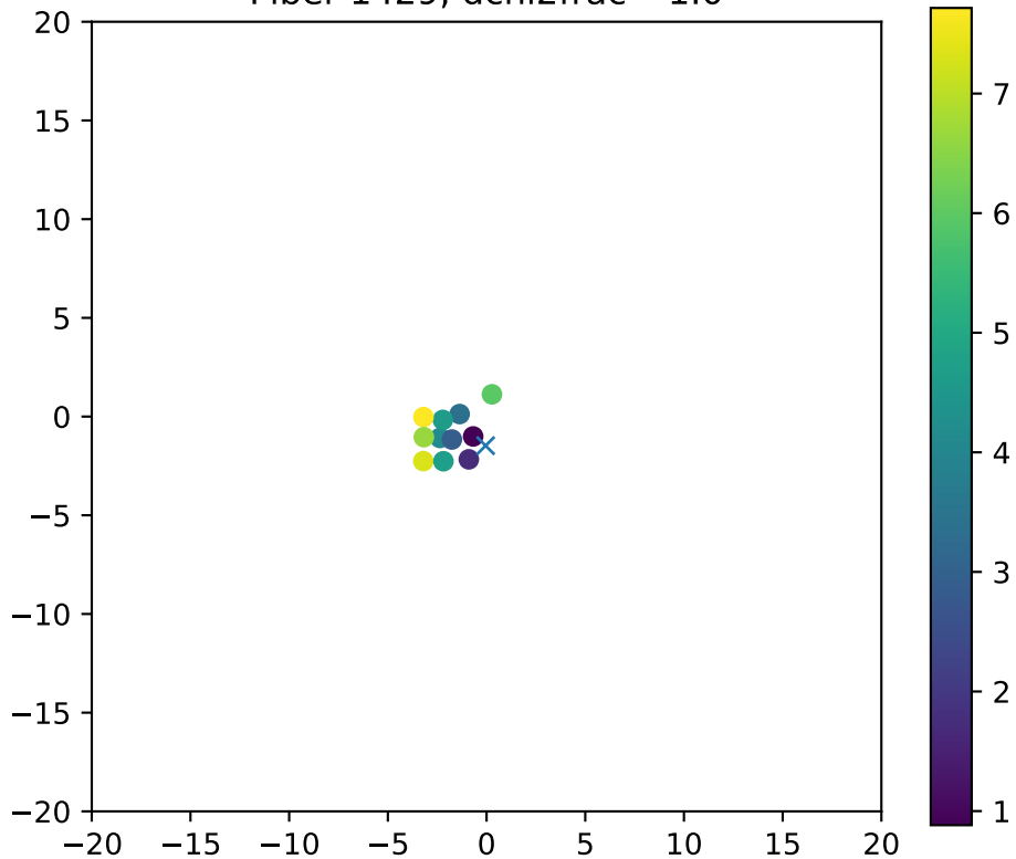
Fiber 1429, dchi2frac= 1.0
