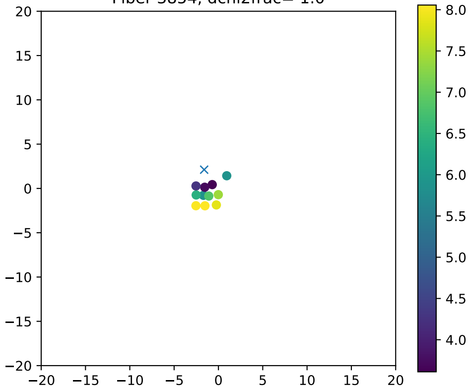
Fiber 3854, dchi2frac= 1.0
