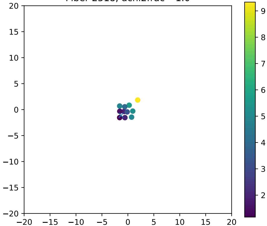
Fiber 2518, dchi2frac= 1.0
