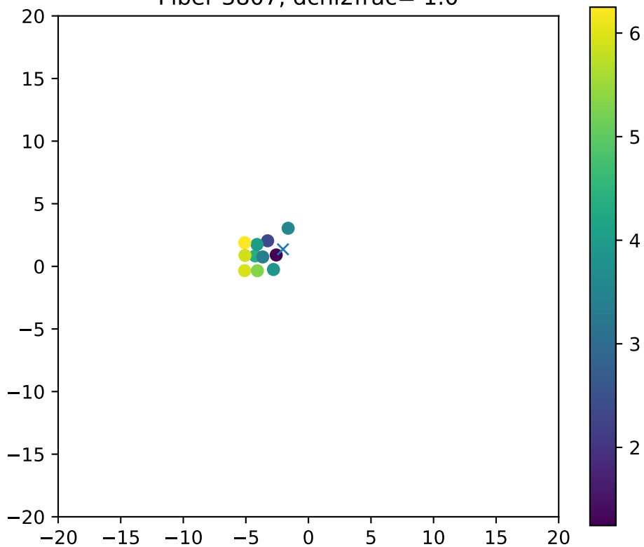
Fiber 3807, dchi2frac= 1.0
