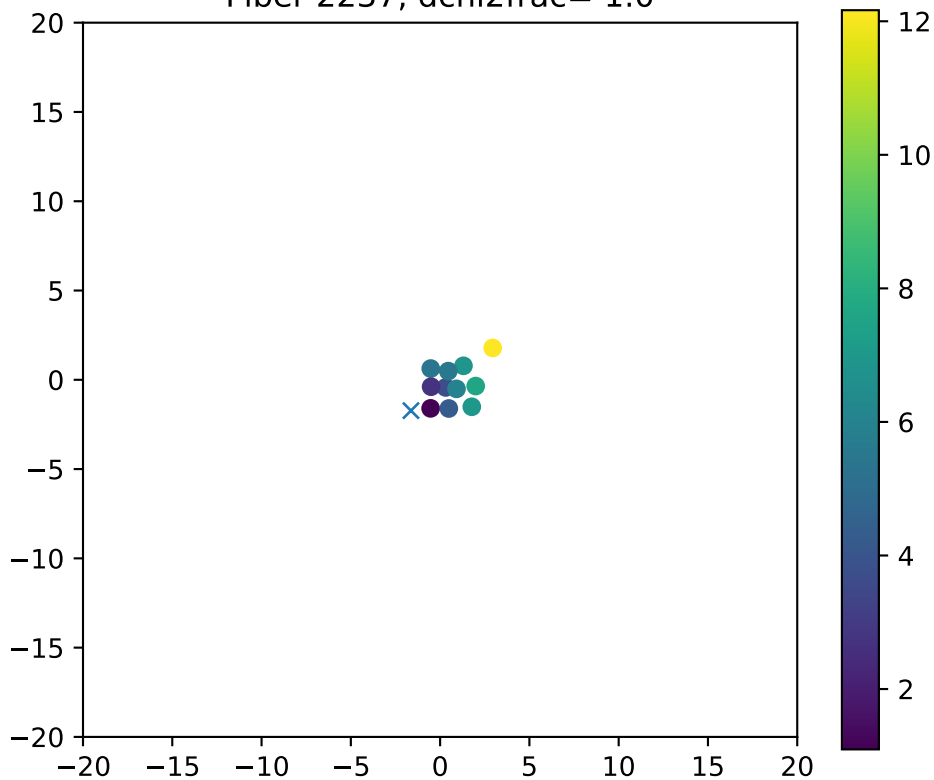
Fiber 2237, dchi2frac= 1.0
