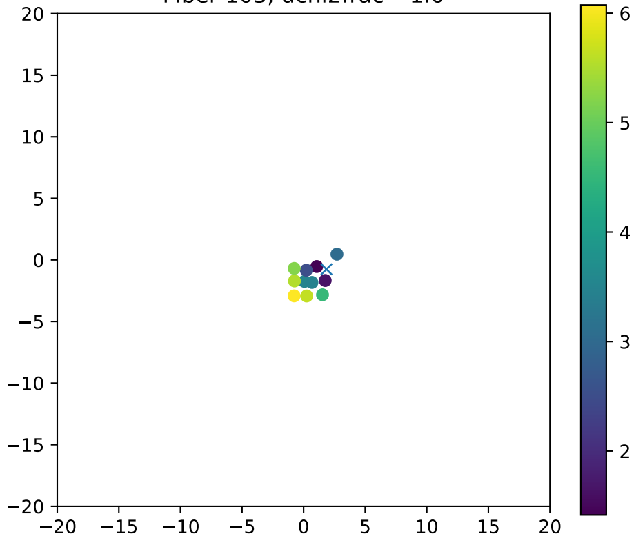
Fiber 103, dchi2frac= 1.0
