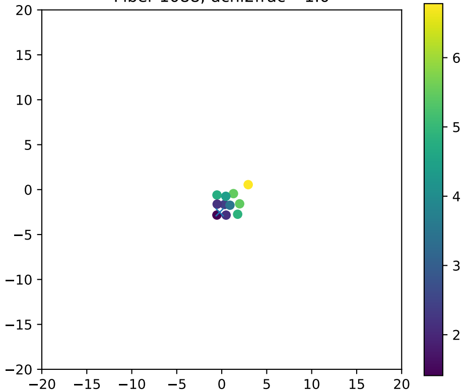
Fiber 1088, dchi2frac= 1.0
