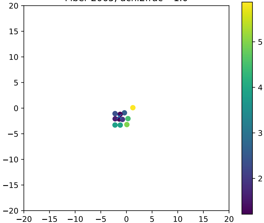
Fiber 2065, dchi2frac= 1.0
