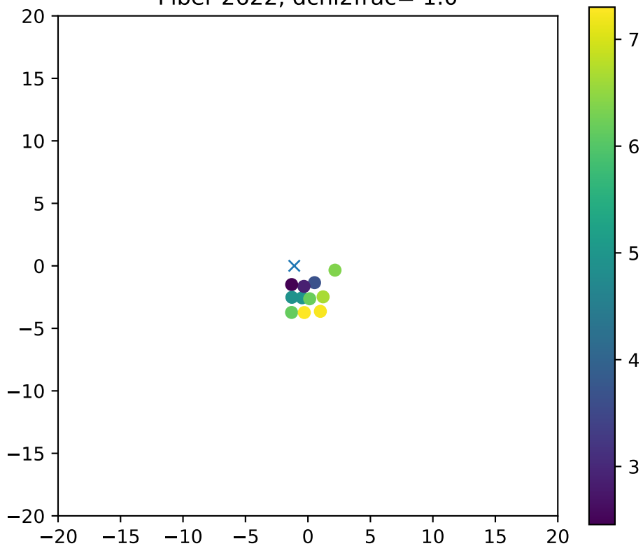
Fiber 2622, dchi2frac= 1.0
