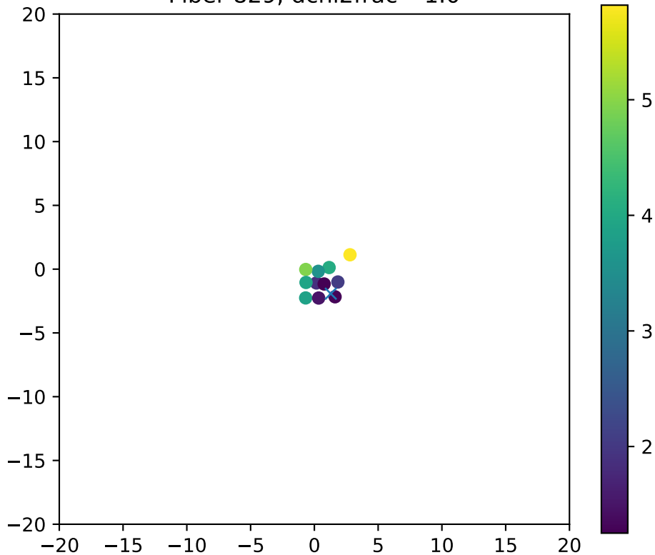
Fiber 829, dchi2frac= 1.0
