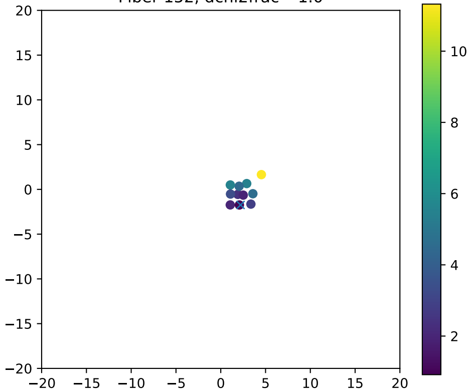
Fiber 152, dchi2frac= 1.0
