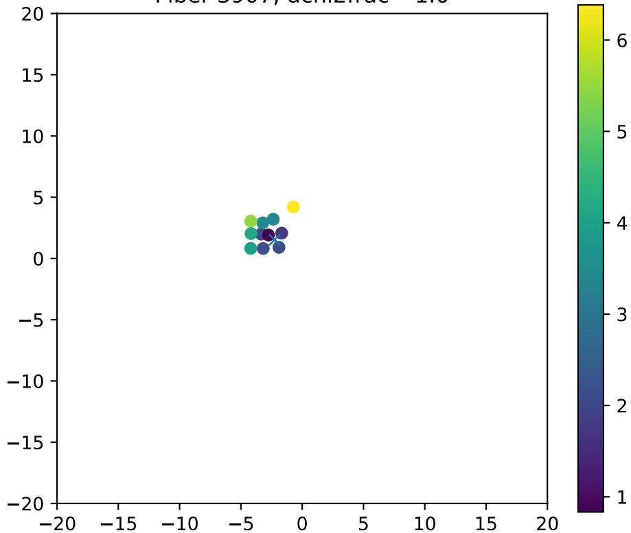
Fiber 3907, dchi2frac= 1.0
