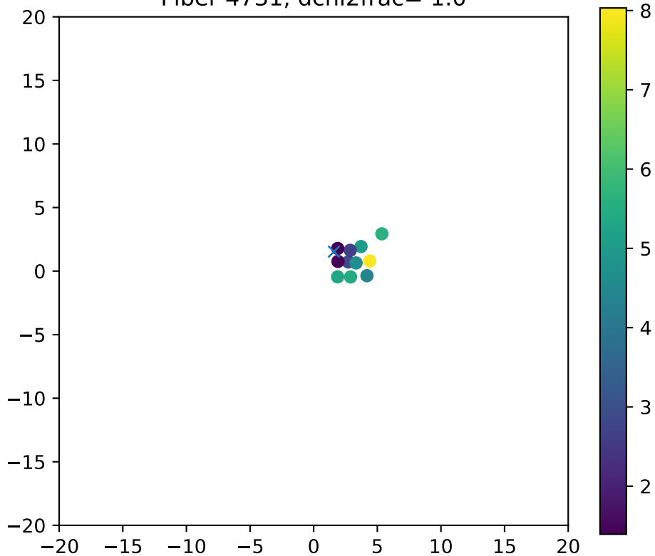
Fiber 4731, dchi2frac= 1.0
