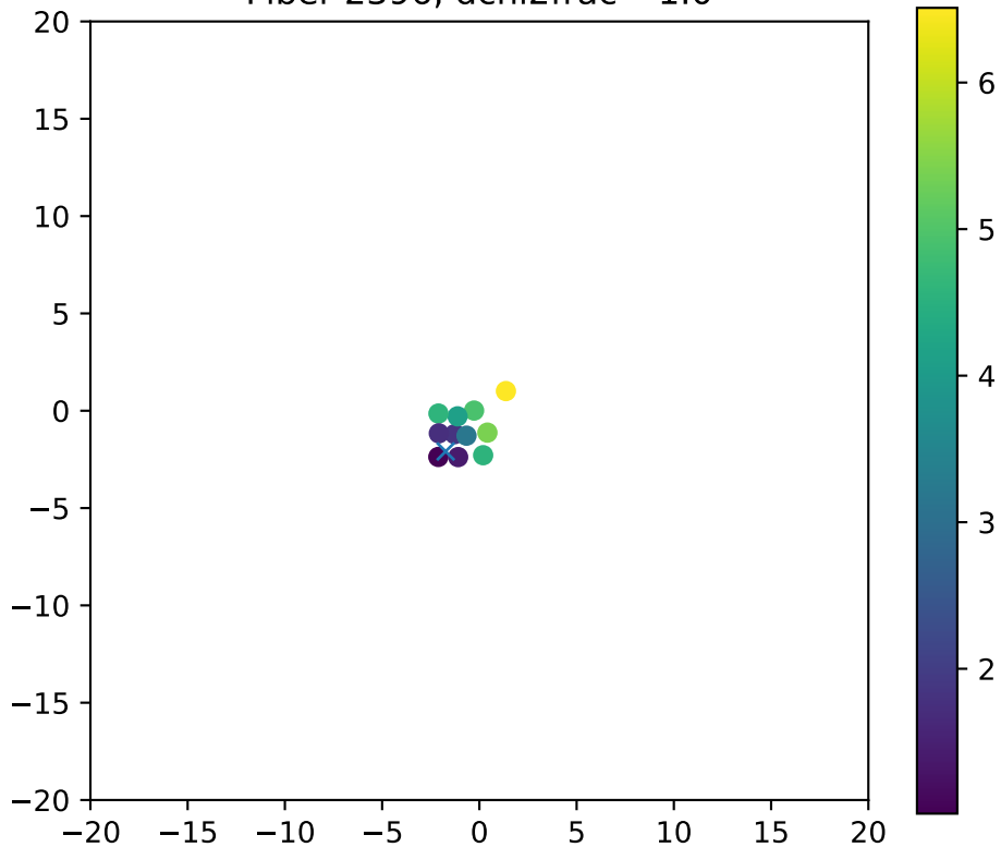
Fiber 2396, dchi2frac= 1.0
