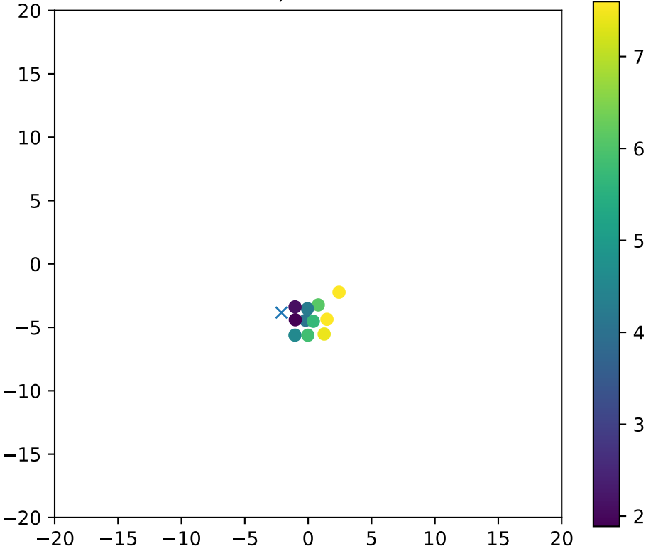
Fiber 1351, dchi2frac= 1.0
