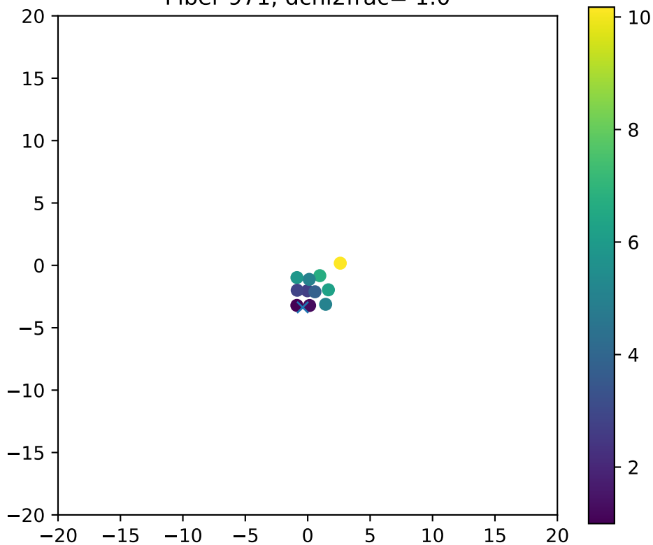
Fiber 971, dchi2frac= 1.0
