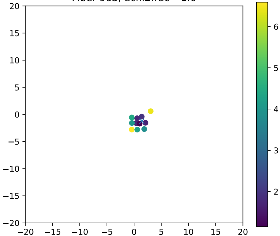
Fiber 963, dchi2frac= 1.0
