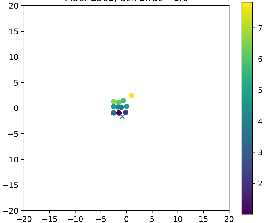
Fiber 2361, dchi2frac= 1.0
