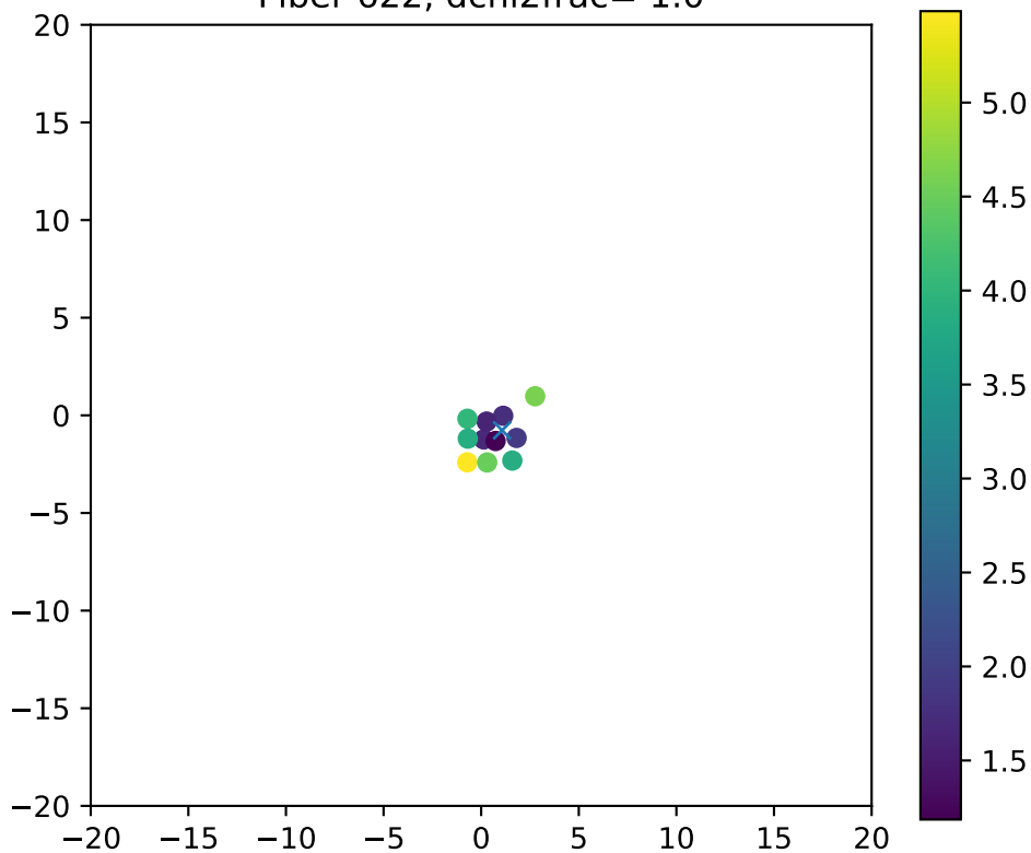
Fiber 622, dchi2frac= 1.0
