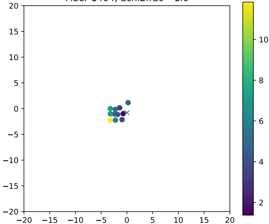
Fiber 1404, dchi2frac= 1.0
