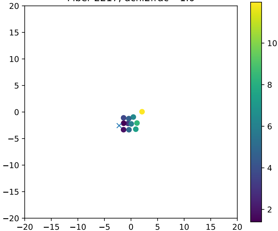
Fiber 2217, dchi2frac= 1.0
