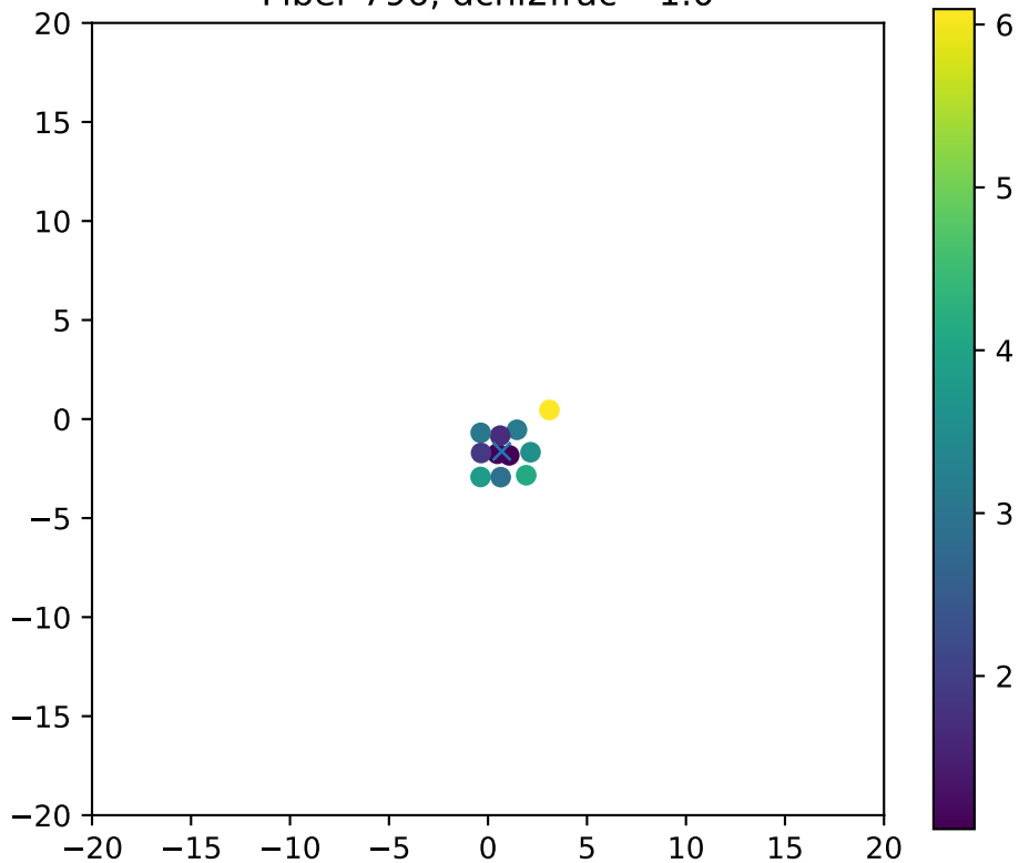
Fiber 796, dchi2frac= 1.0
