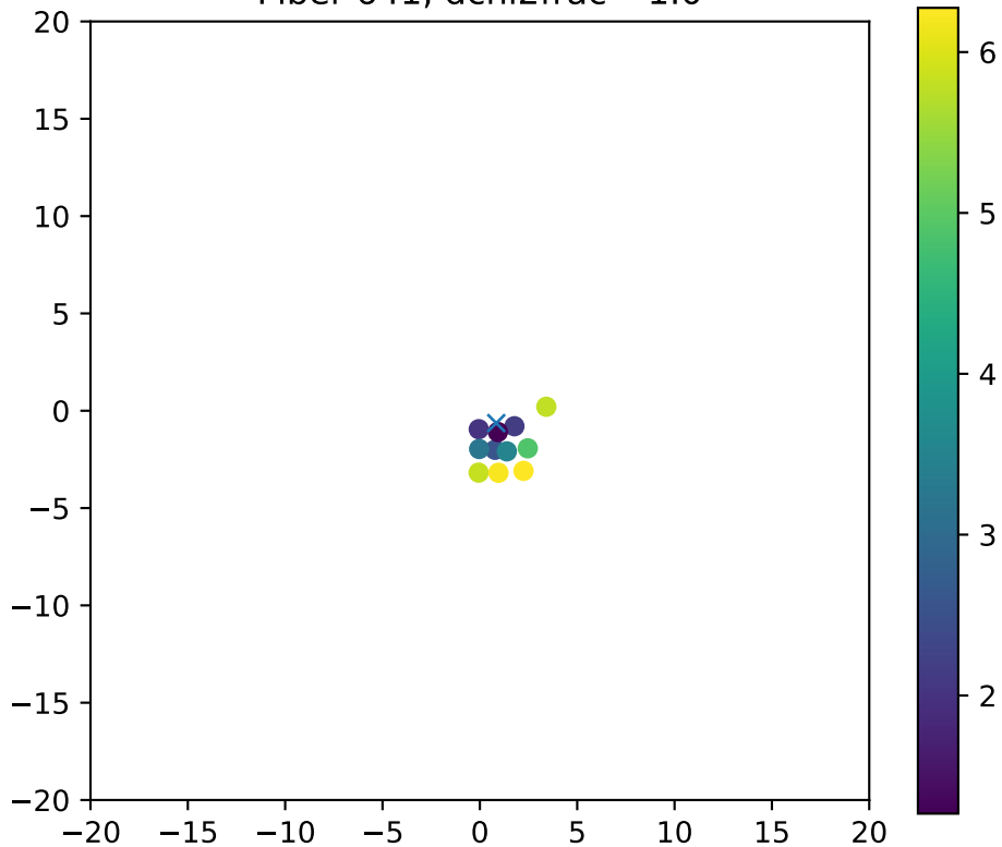
Fiber 641, dchi2frac= 1.0
