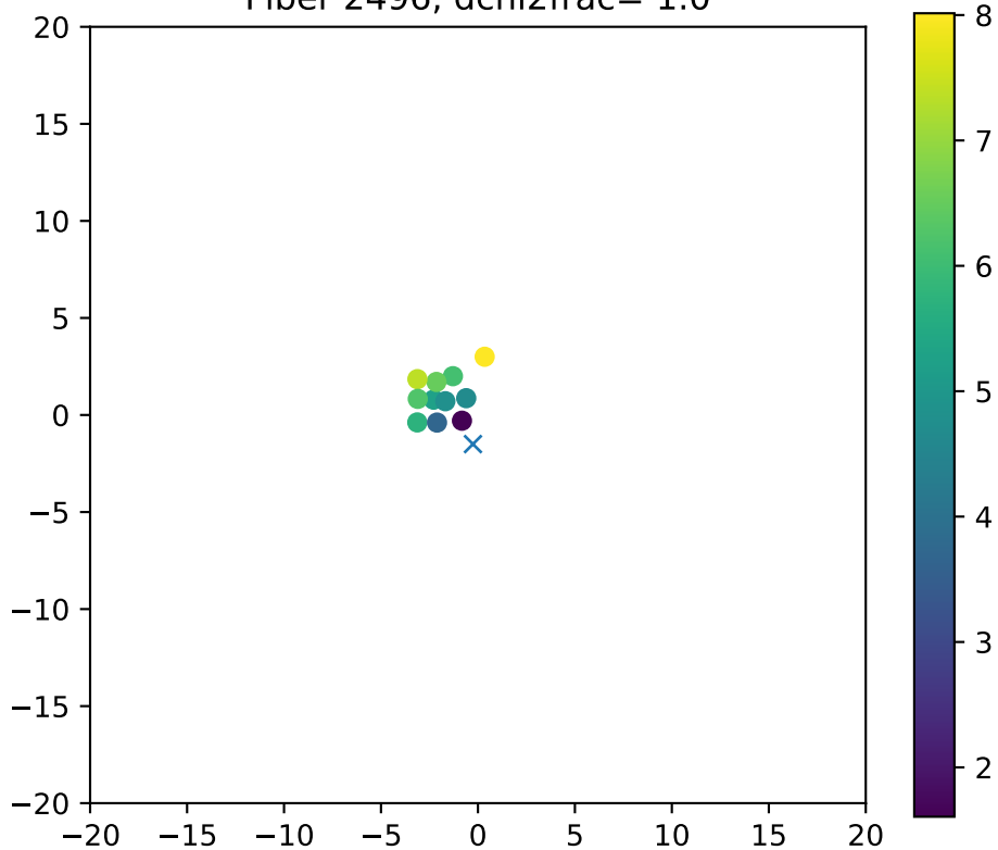
Fiber 2496, dchi2frac= 1.0
