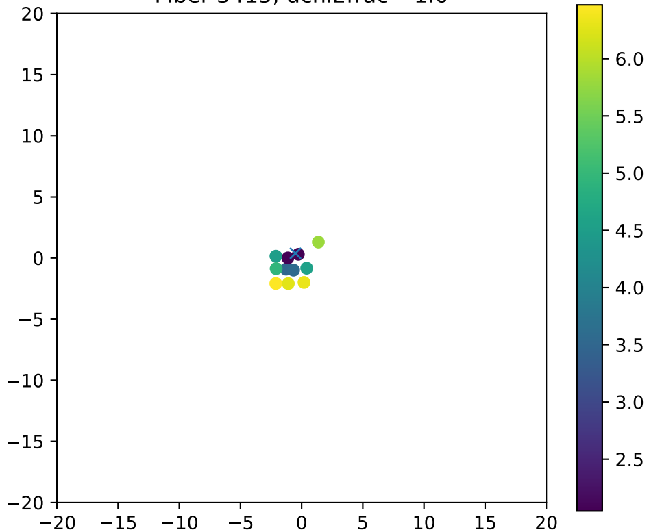
Fiber 3415, dchi2frac= 1.0
