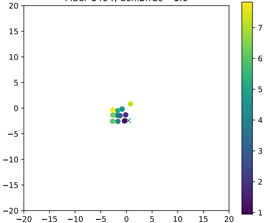
Fiber 1494, dchi2frac= 1.0
