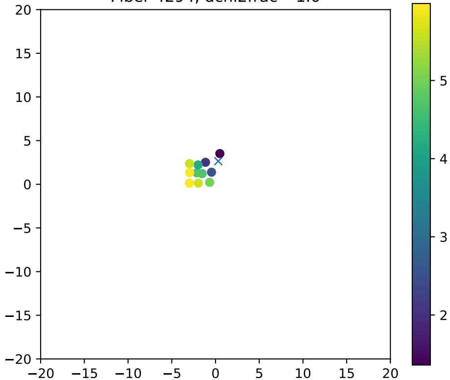
Fiber 4294, dchi2frac= 1.0
