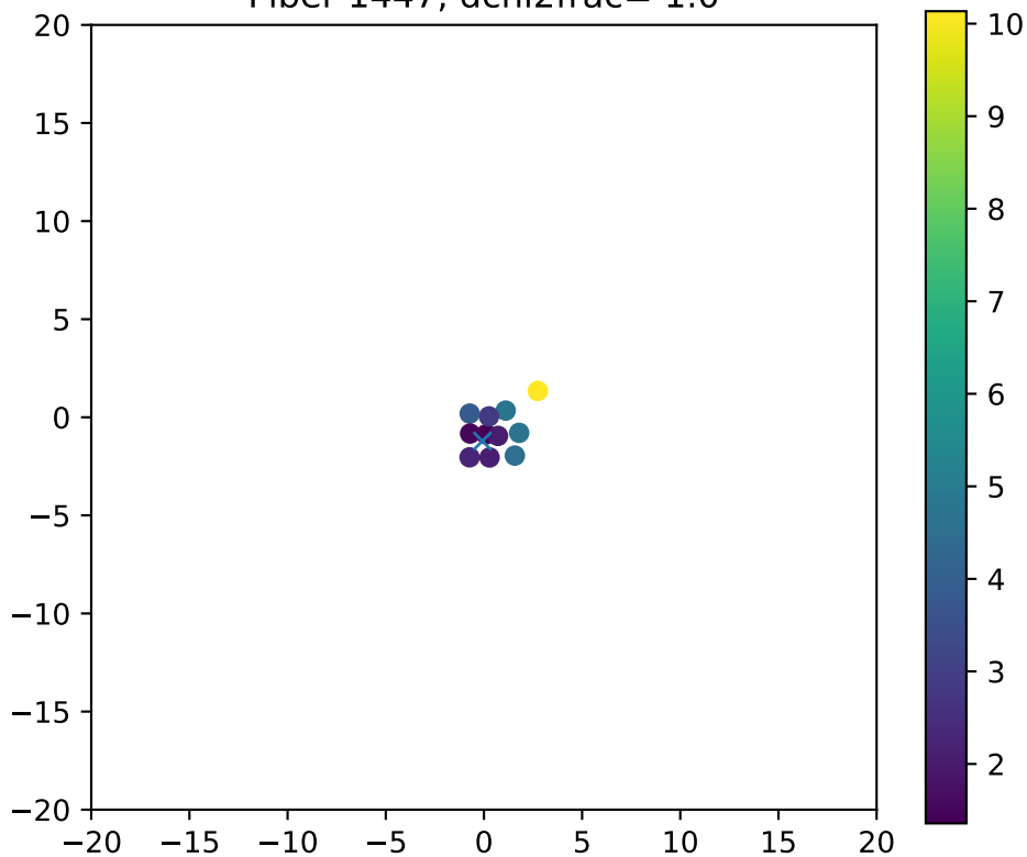
Fiber 1447, dchi2frac= 1.0
