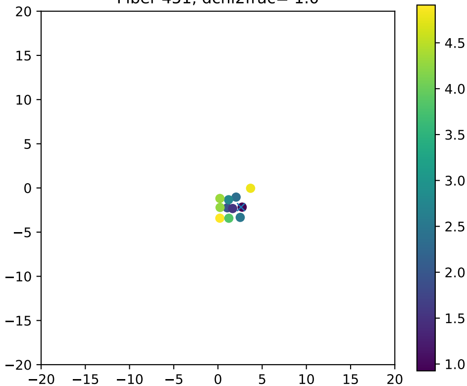
Fiber 451, dchi2frac= 1.0
