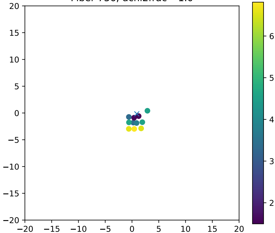
Fiber 736, dchi2frac= 1.0
