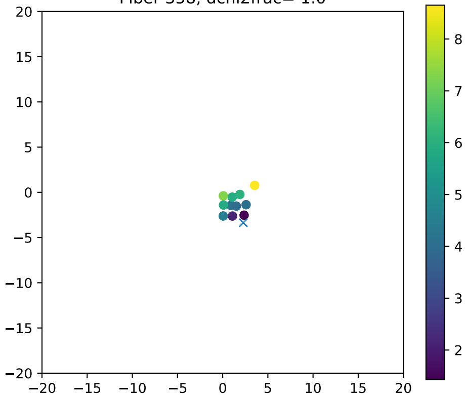
Fiber 358, dchi2frac= 1.0
