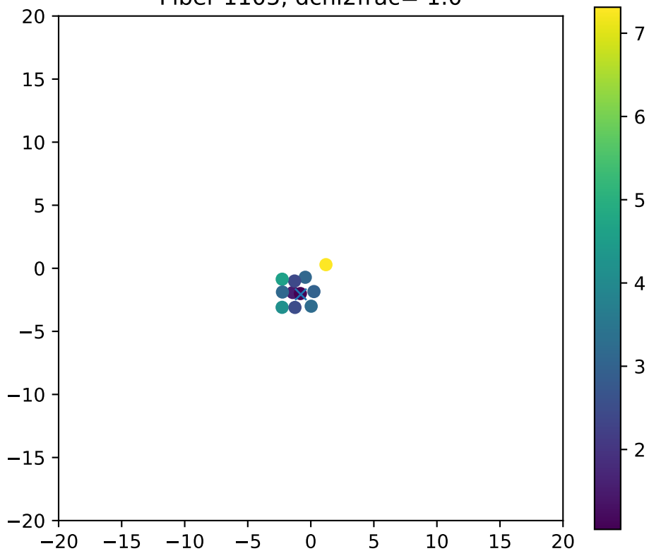
Fiber 1105, dchi2frac= 1.0
