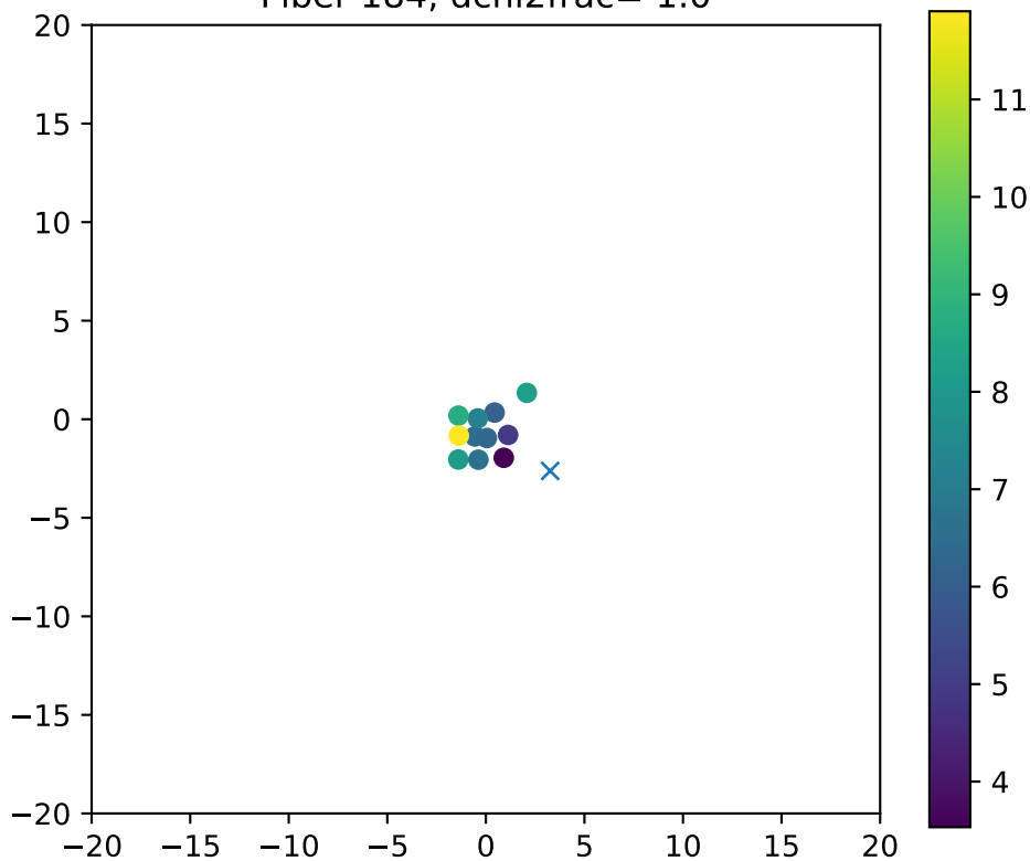
Fiber 184, dchi2frac= 1.0
