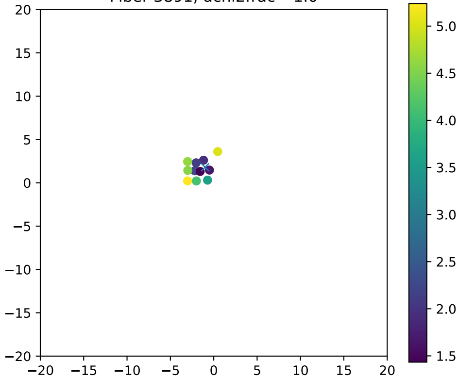
Fiber 3891, dchi2frac= 1.0
