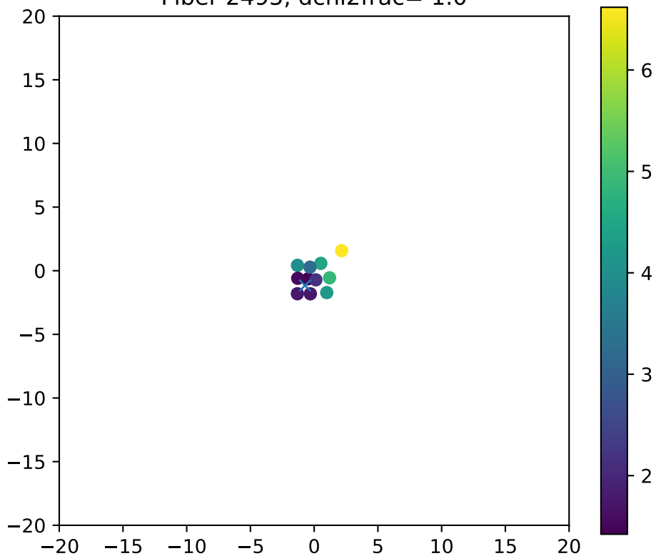
Fiber 2495, dchi2frac= 1.0
