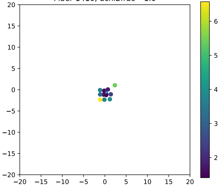
Fiber 1410, dchi2frac= 1.0
