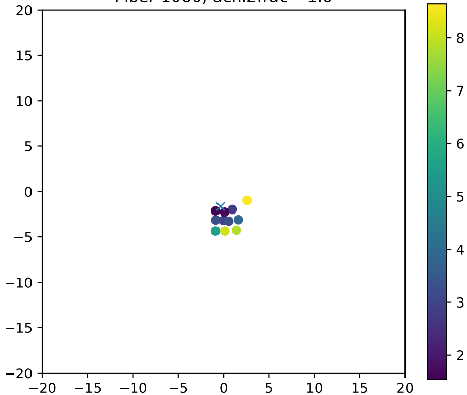
Fiber 1000, dchi2frac= 1.0
