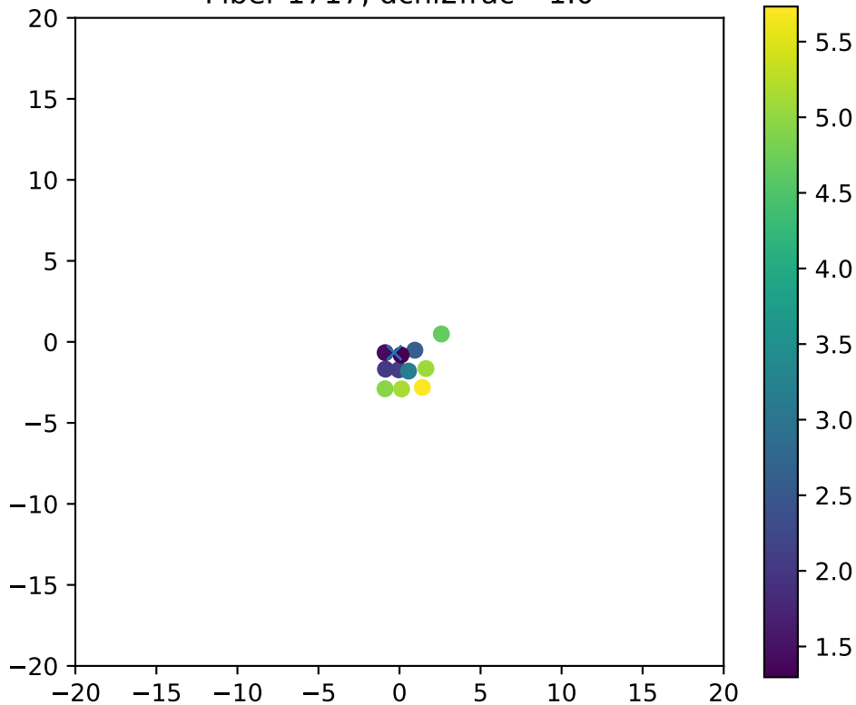
Fiber 1717, dchi2frac= 1.0
