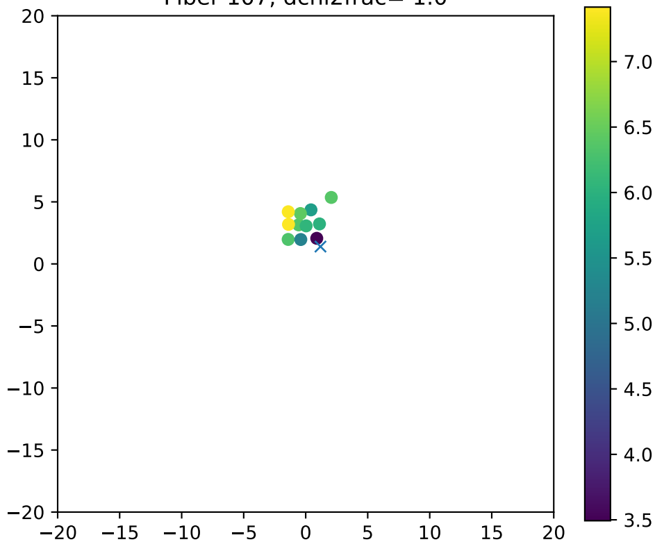
Fiber 107, dchi2frac= 1.0
