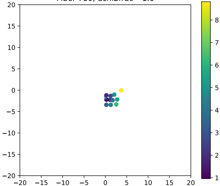
Fiber 780, dchi2frac= 1.0
