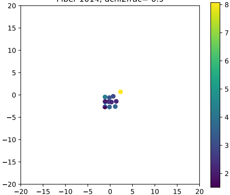
Fiber 1014, dchi2frac= 0.9
