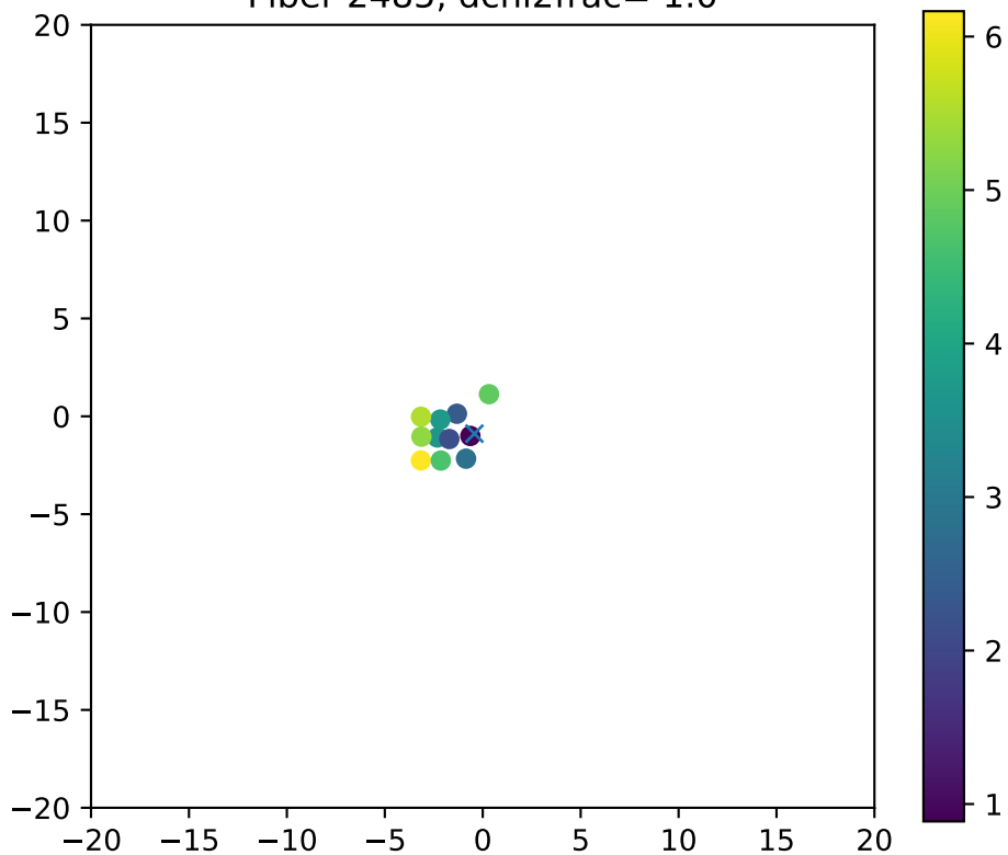
Fiber 2485, dchi2frac= 1.0
