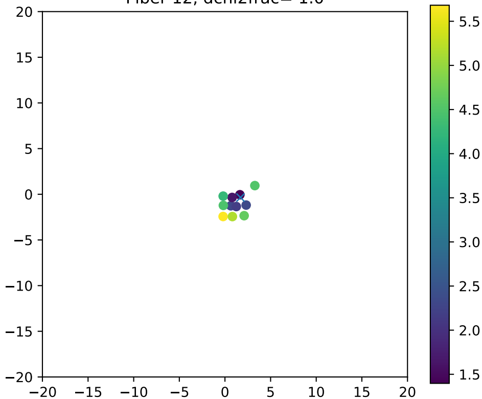
Fiber 12, dchi2frac= 1.0
