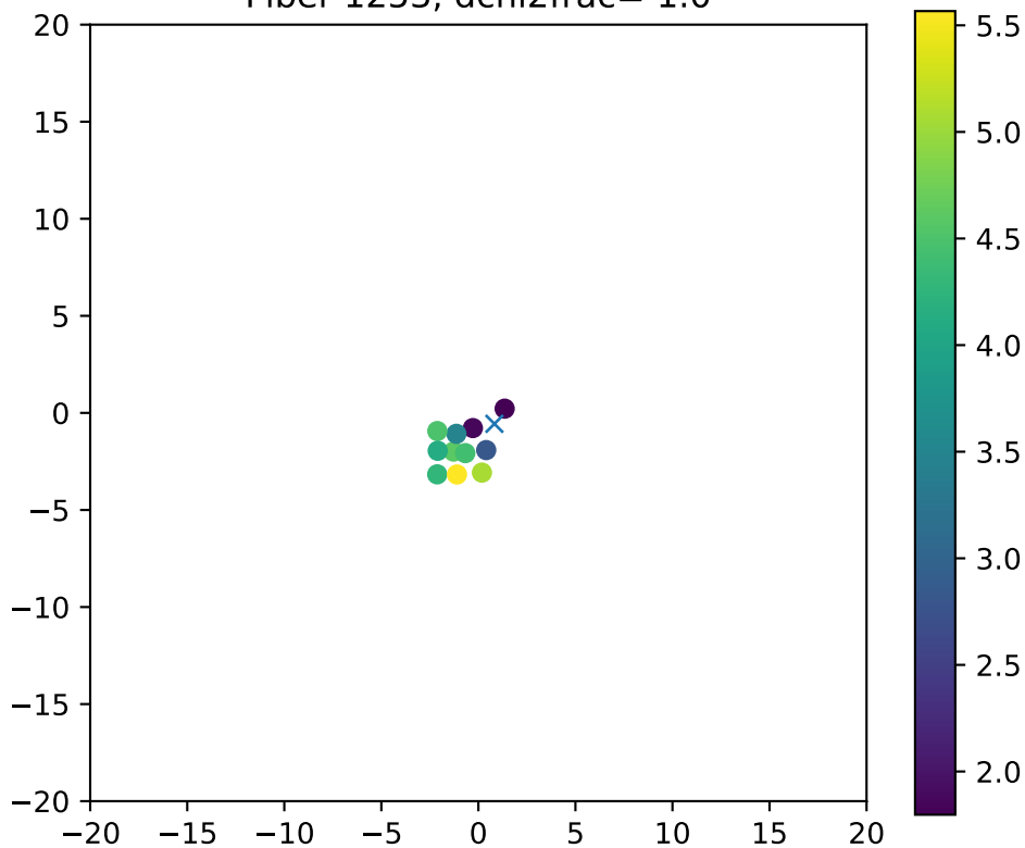
Fiber 1253, dchi2frac= 1.0
