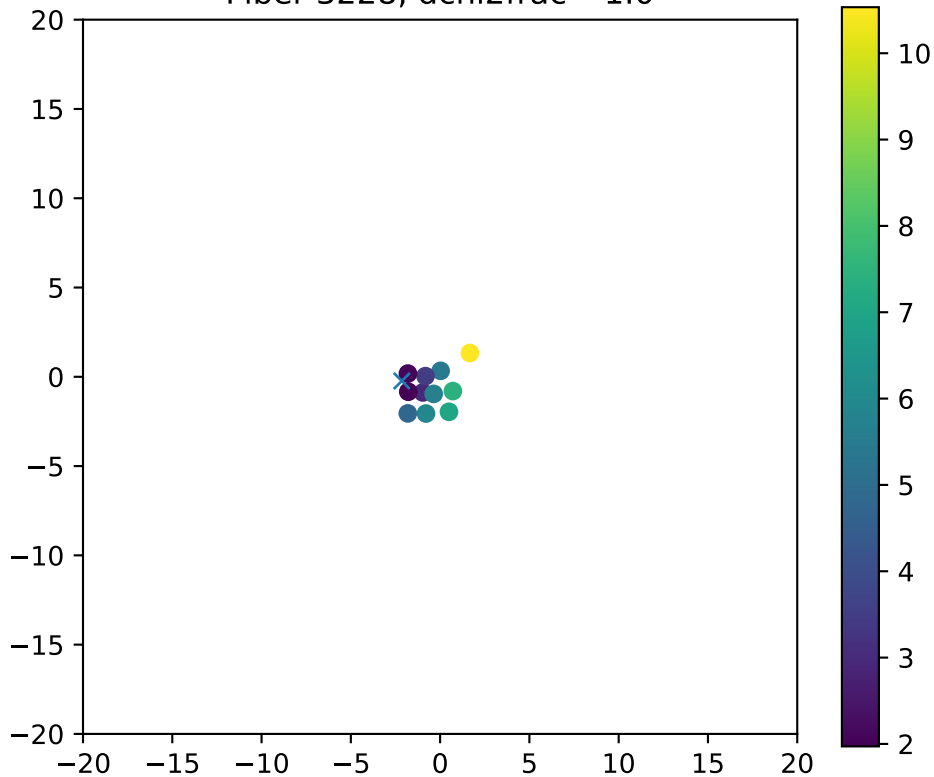
Fiber 3228, dchi2frac= 1.0
