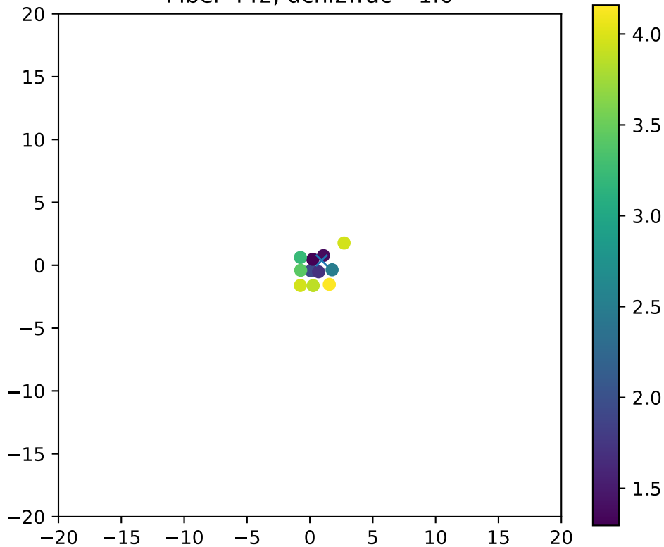
Fiber 442, dchi2frac= 1.0
