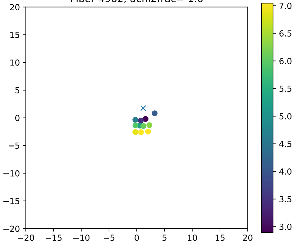
Fiber 4962, dchi2frac= 1.0
