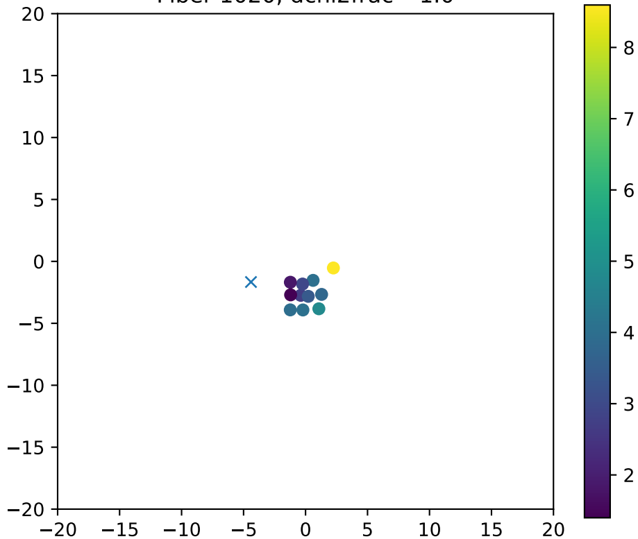
Fiber 1020, dchi2frac= 1.0
