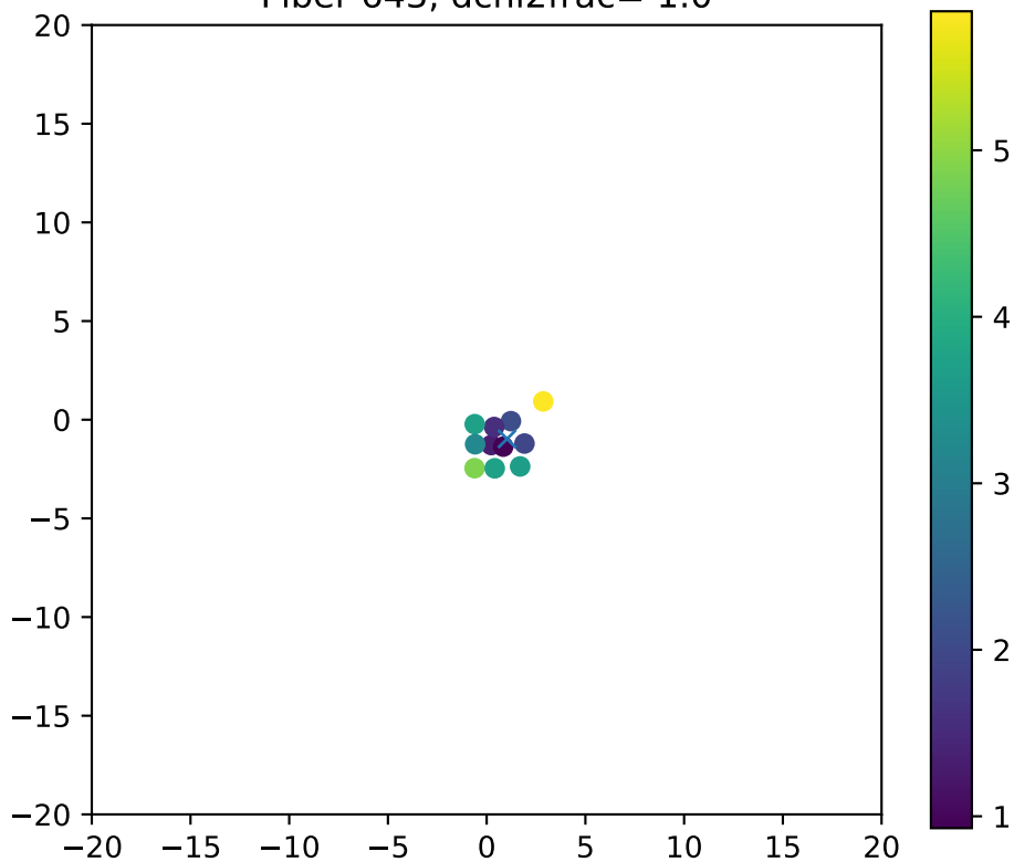
Fiber 643, dchi2frac= 1.0
