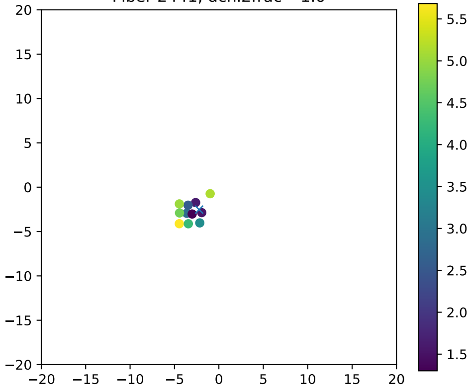
Fiber 2441, dchi2frac= 1.0
