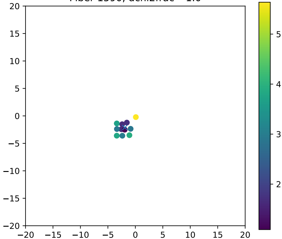
Fiber 1590, dchi2frac= 1.0
