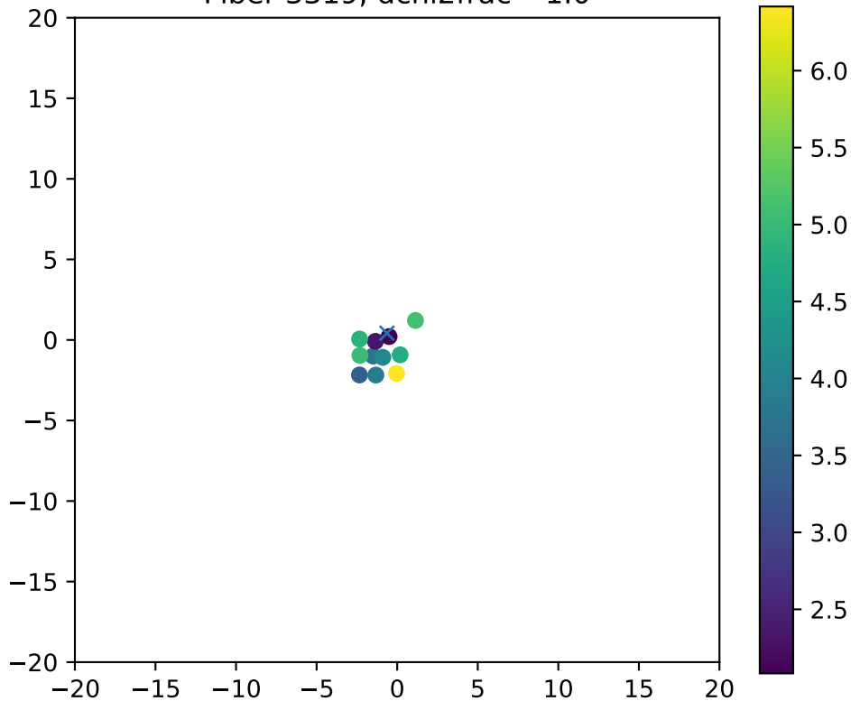
Fiber 3319, dchi2frac= 1.0
