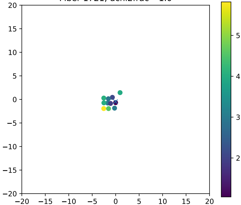
Fiber 1721, dchi2frac= 1.0
