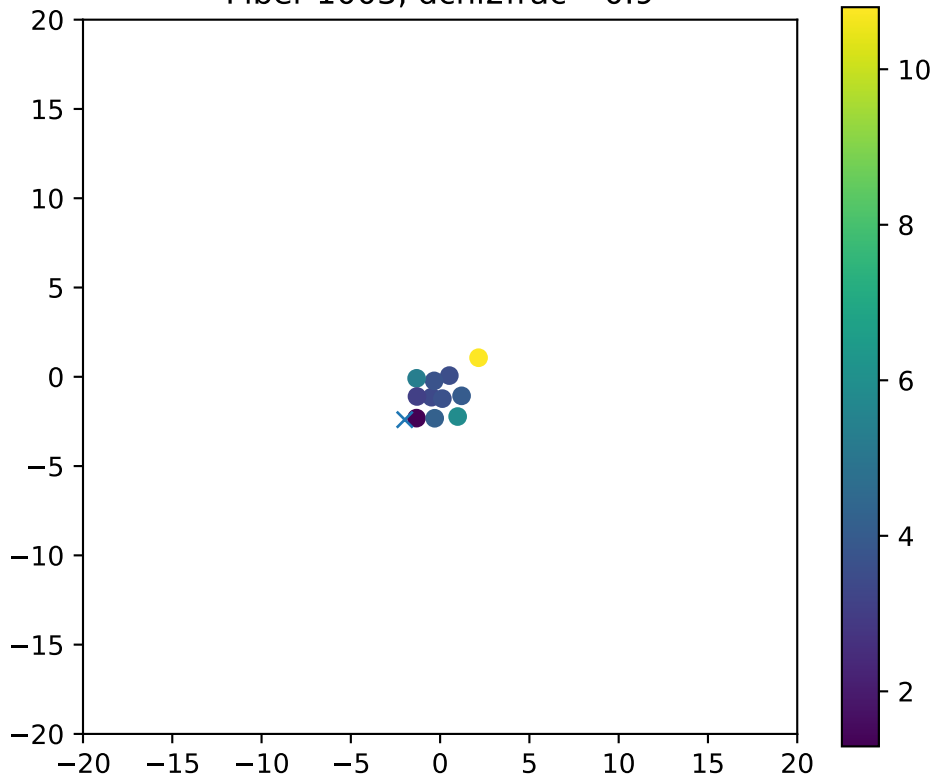
Fiber 1003, dchi2frac= 0.9
