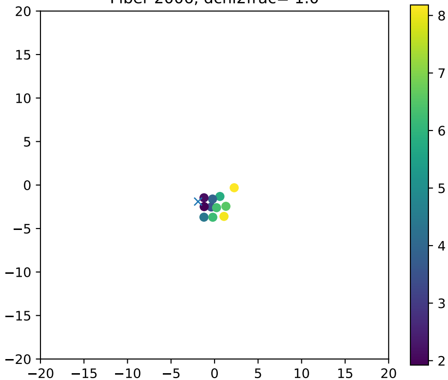
Fiber 2006, dchi2frac= 1.0
