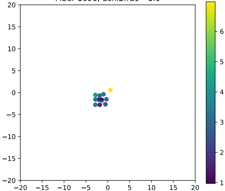
Fiber 1696, dchi2frac= 1.0
