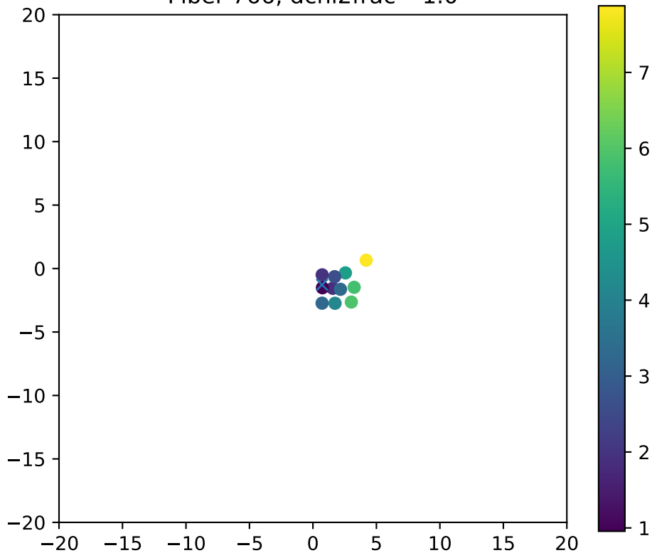
Fiber 766, dchi2frac= 1.0
