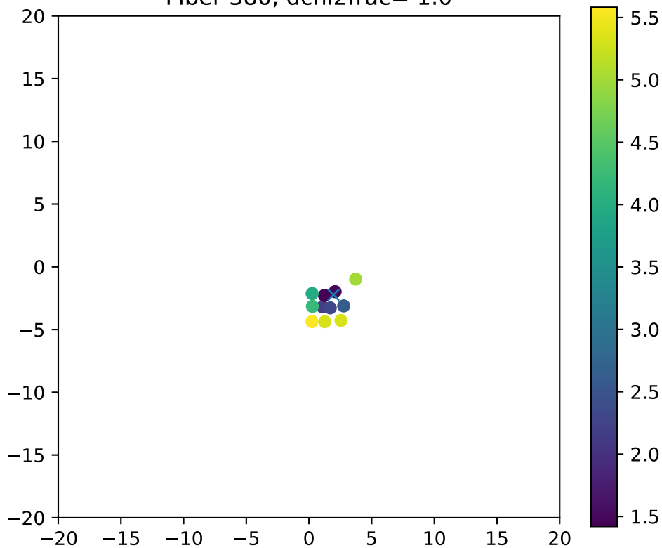
Fiber 380, dchi2frac= 1.0
