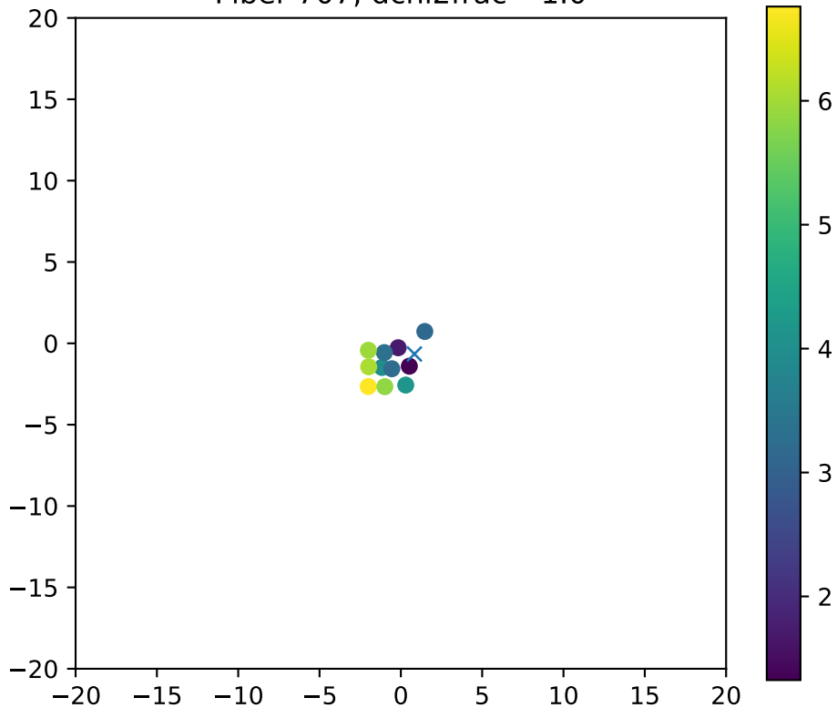
Fiber 707, dchi2frac= 1.0
