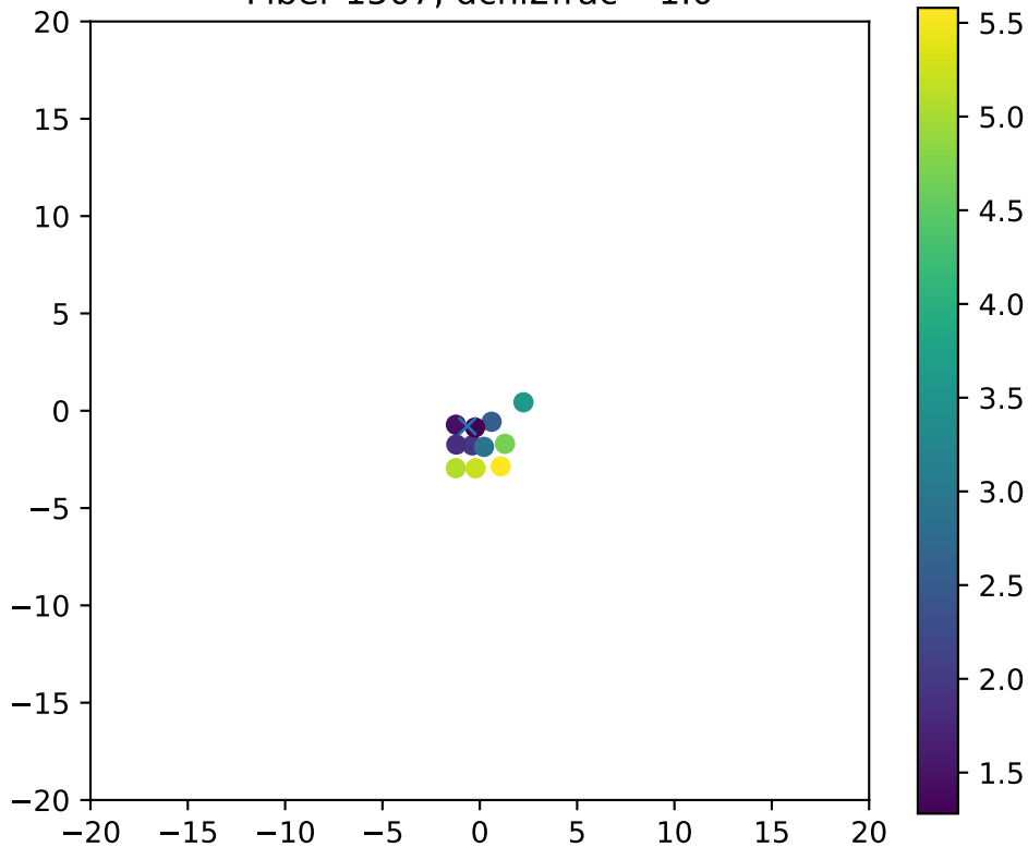
Fiber 1507, dchi2frac= 1.0
