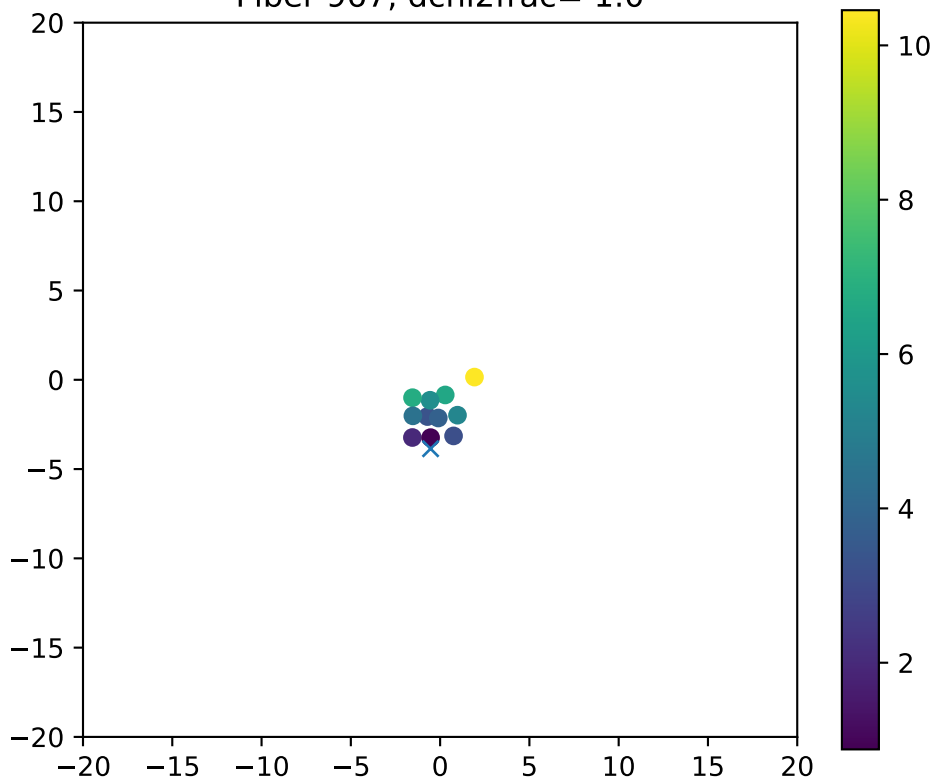
Fiber 967, dchi2frac= 1.0
