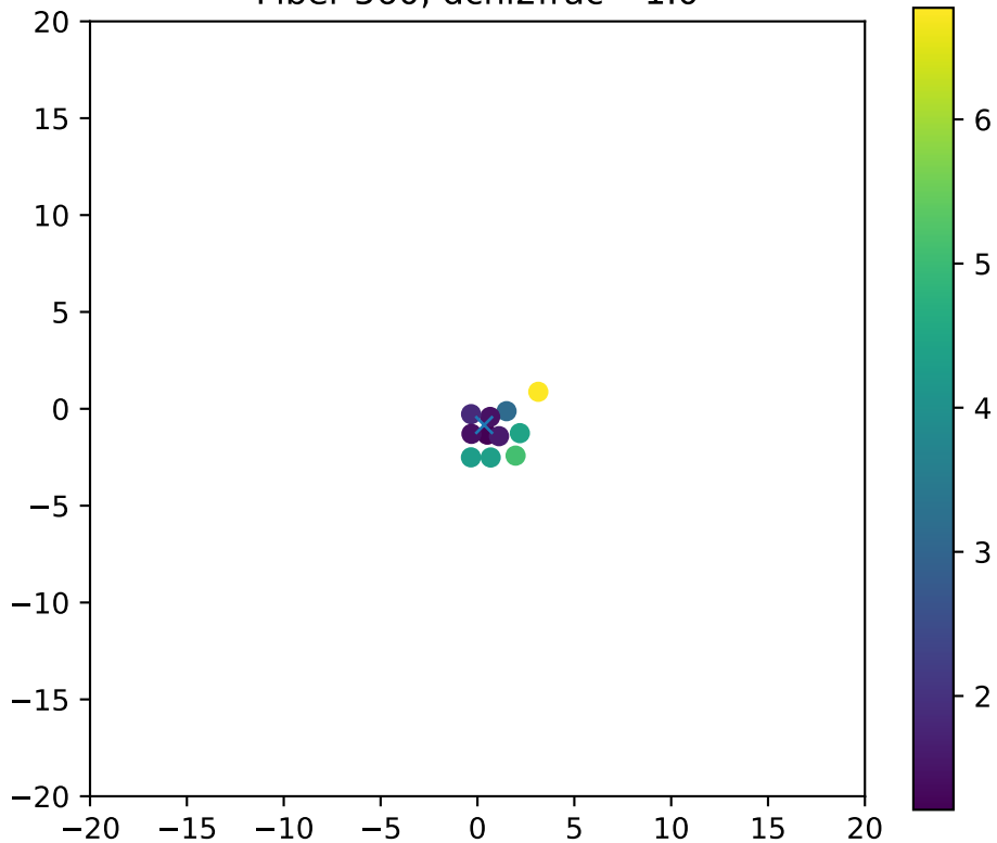
Fiber 560, dchi2frac= 1.0
