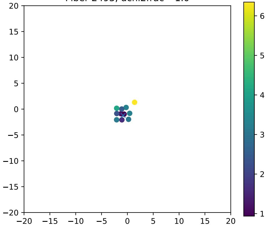
Fiber 2493, dchi2frac= 1.0
