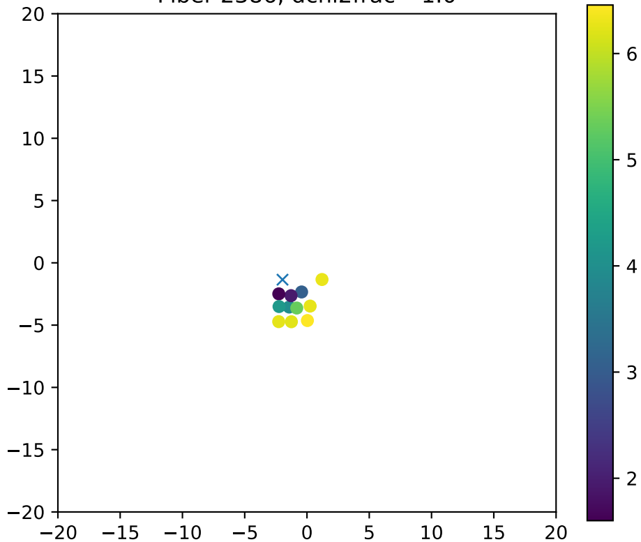
Fiber 2386, dchi2frac= 1.0
