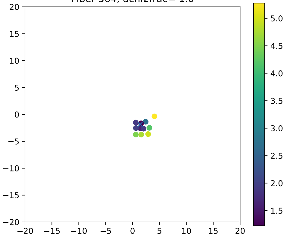
Fiber 564, dchi2frac= 1.0
