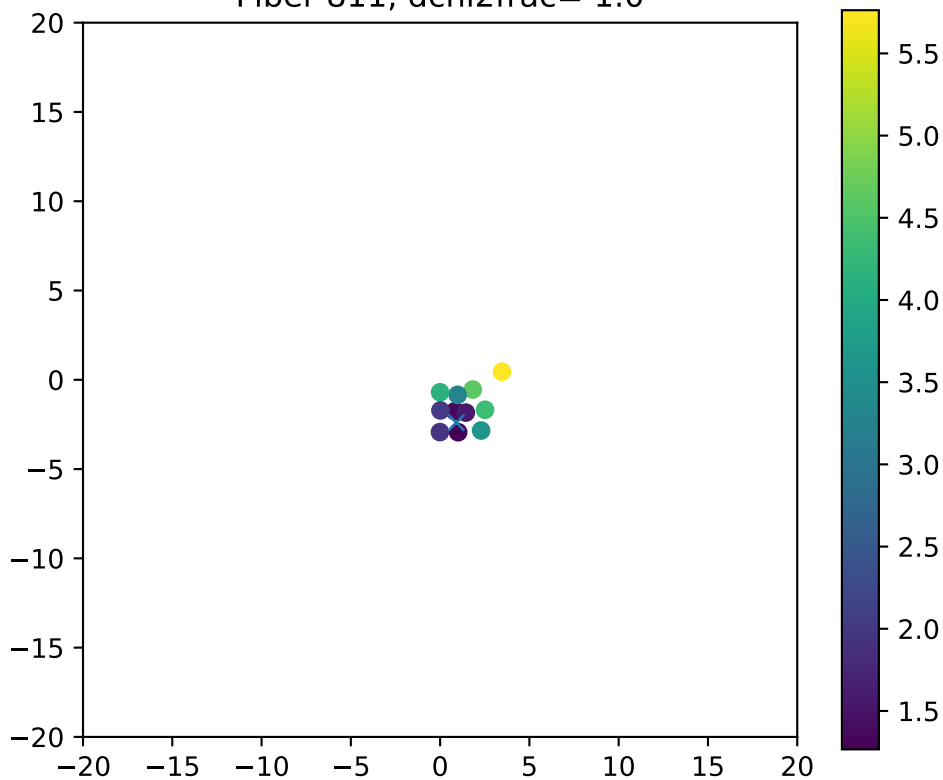
Fiber 811, dchi2frac= 1.0
