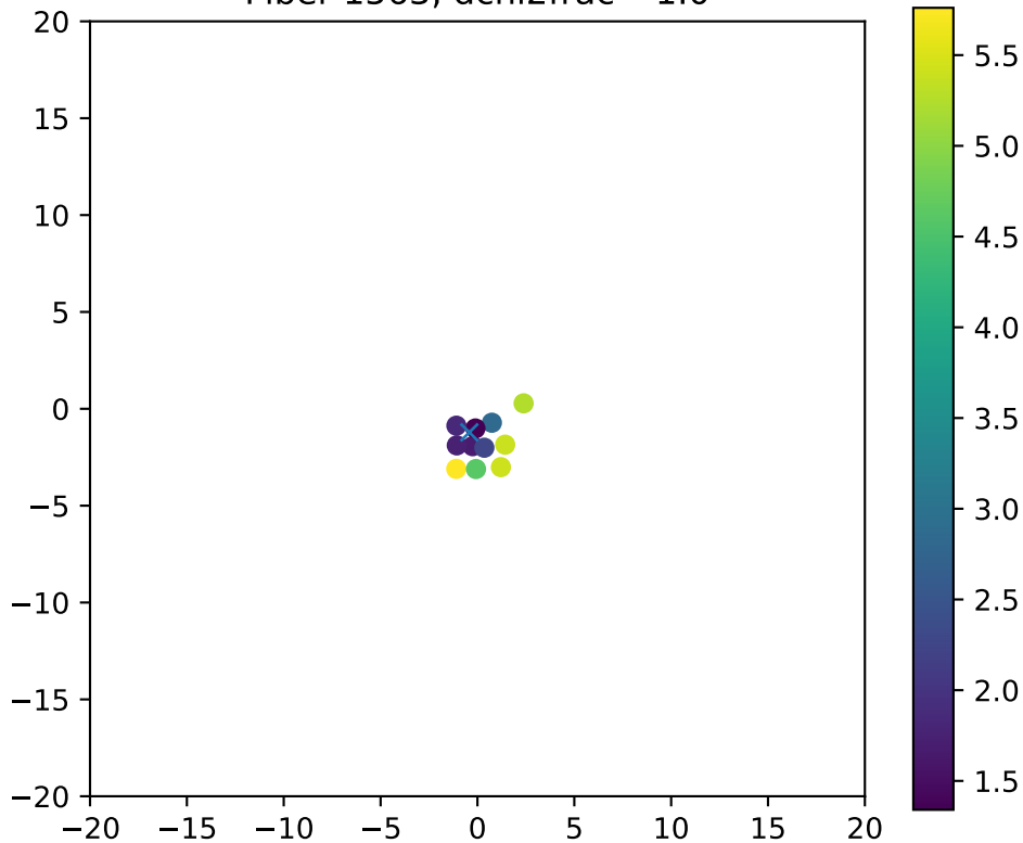
Fiber 1563, dchi2frac= 1.0
