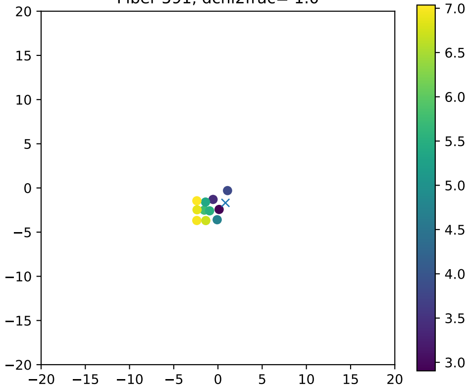
Fiber 591, dchi2frac= 1.0
