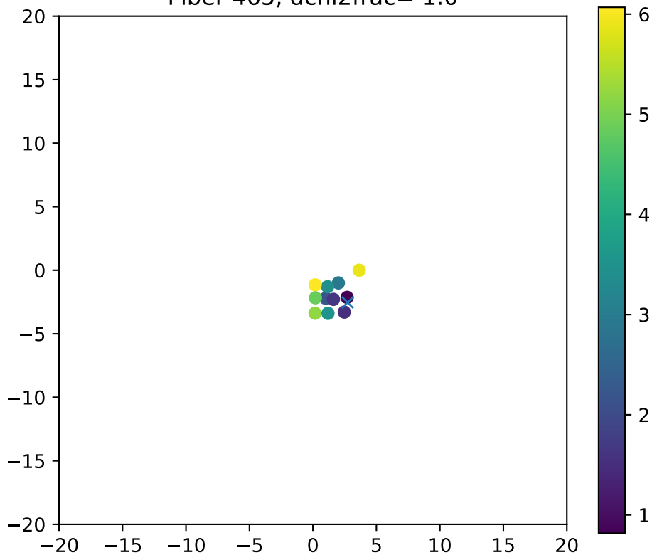
Fiber 465, dchi2frac= 1.0
