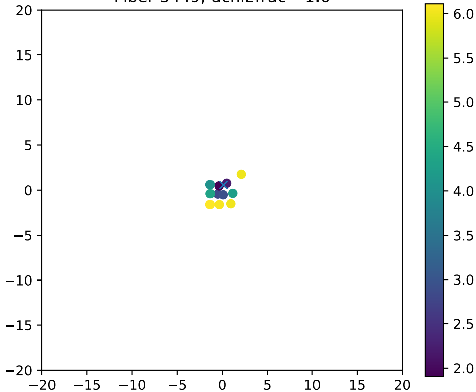
Fiber 3449, dchi2frac= 1.0
