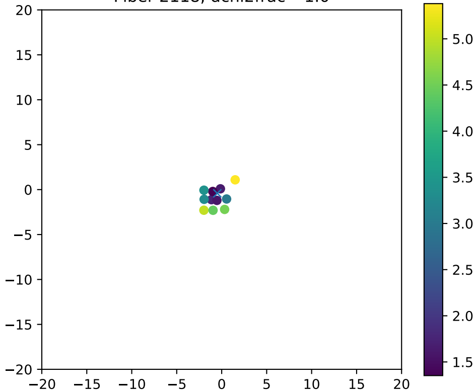
Fiber 2118, dchi2frac= 1.0
