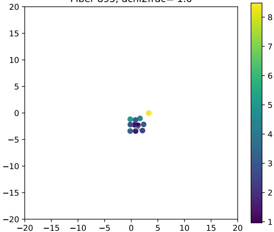
Fiber 895, dchi2frac= 1.0
