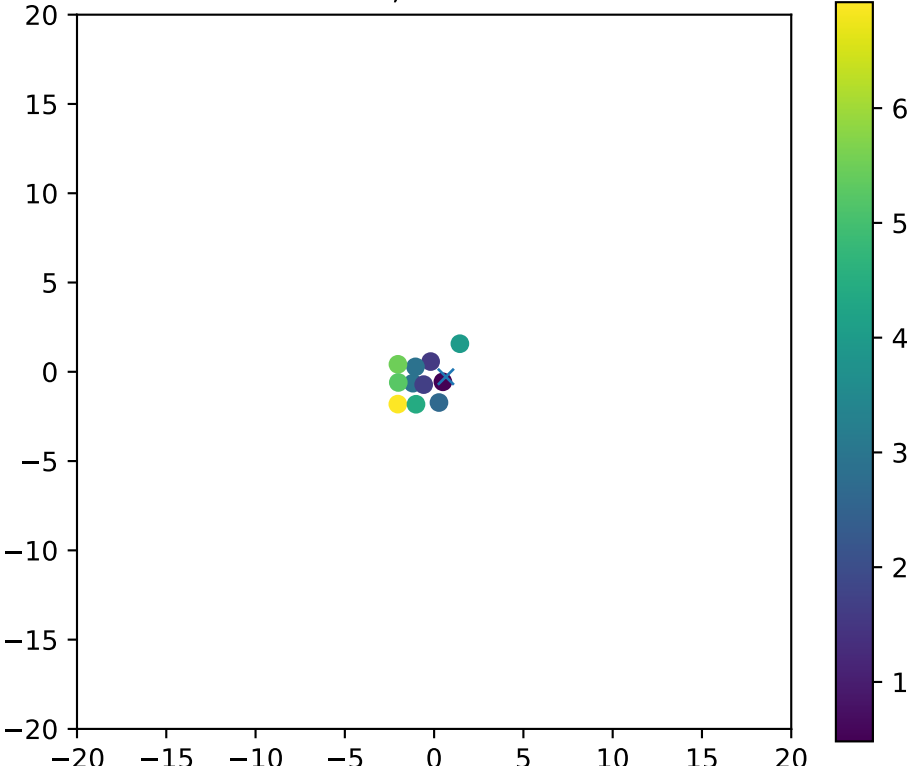
Fiber 1406, dchi2frac= 1.0
