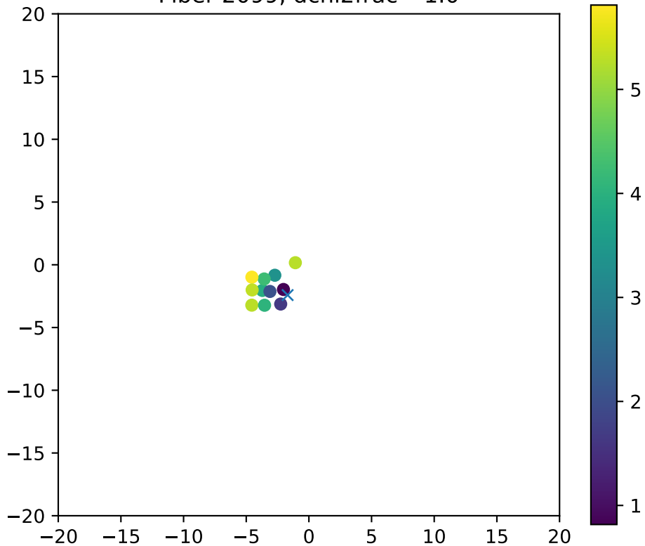
Fiber 2099, dchi2frac= 1.0
