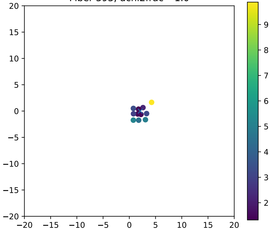
Fiber 393, dchi2frac= 1.0
