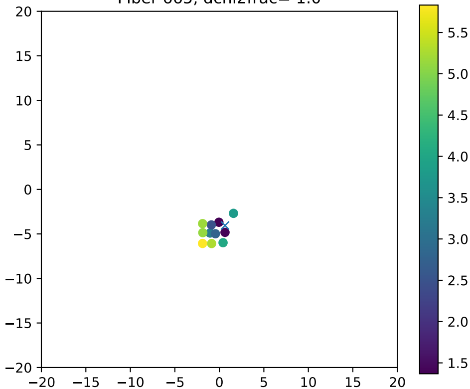
Fiber 665, dchi2frac= 1.0
