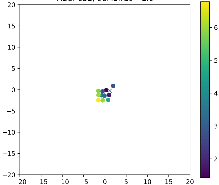
Fiber 632, dchi2frac= 1.0
