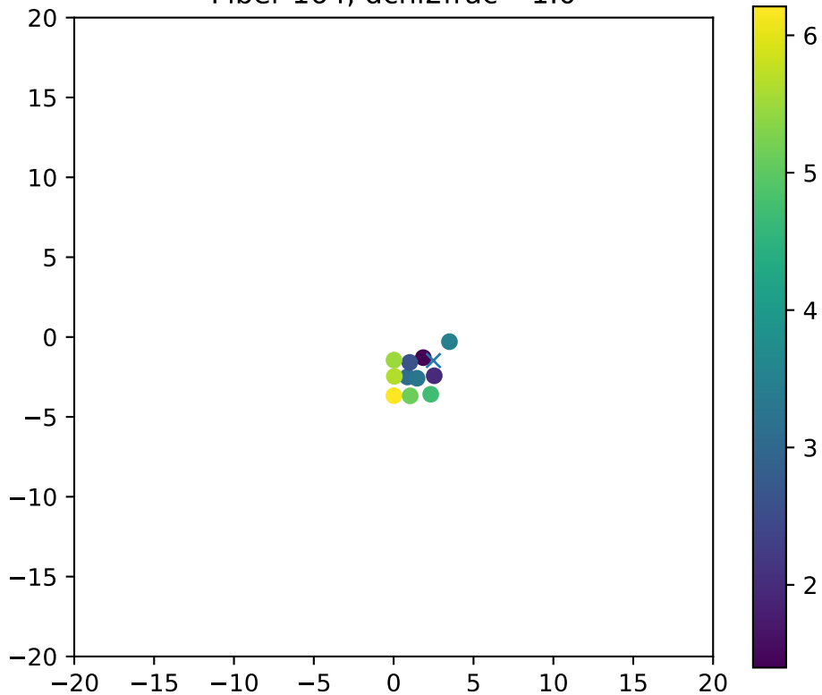
Fiber 164, dchi2frac= 1.0
