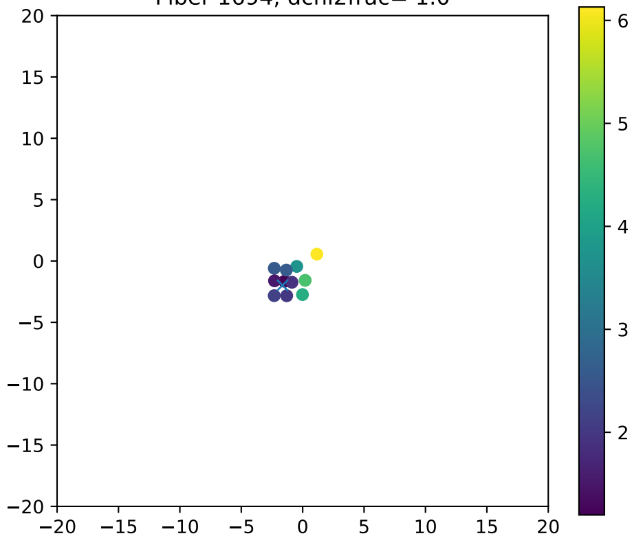
Fiber 1694, dchi2frac= 1.0
