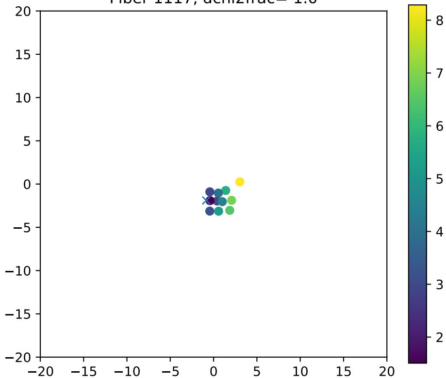
Fiber 1117, dchi2frac= 1.0
