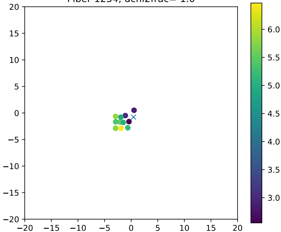
Fiber 1254, dchi2frac= 1.0
