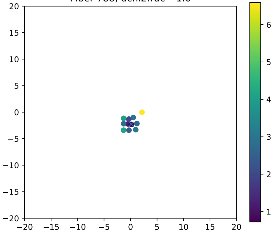
Fiber 788, dchi2frac= 1.0
