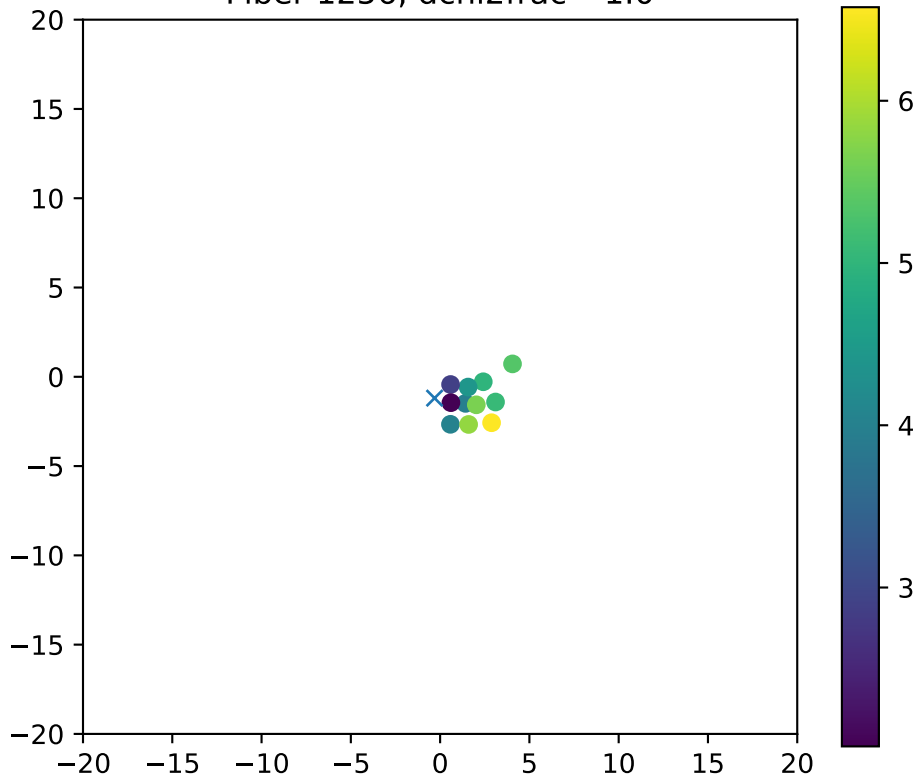
Fiber 1256, dchi2frac= 1.0
