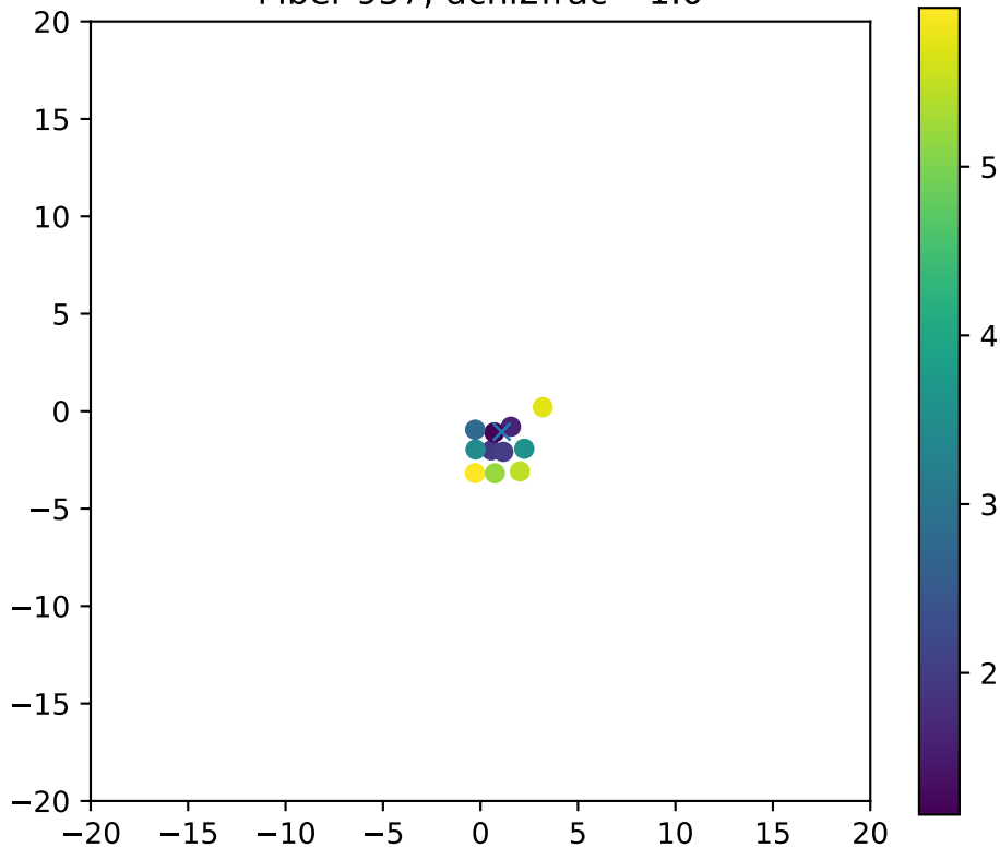
Fiber 957, dchi2frac= 1.0
