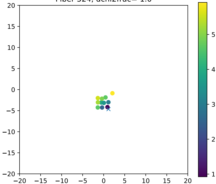
Fiber 524, dchi2frac= 1.0
