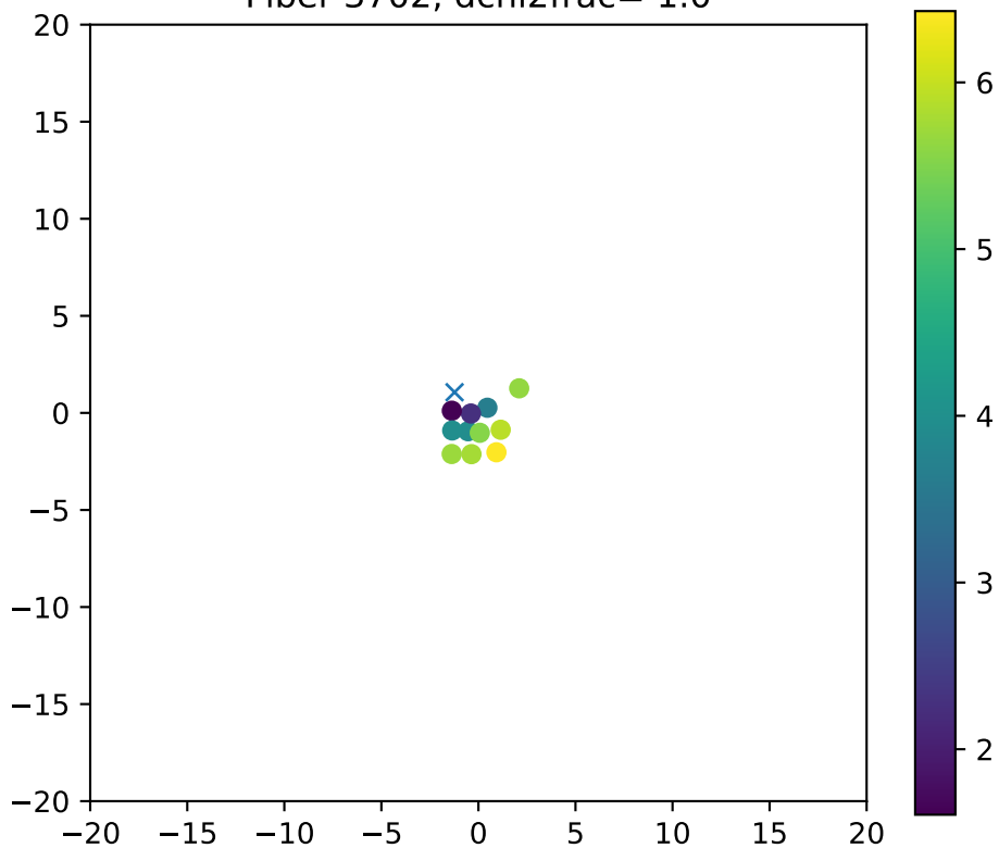
Fiber 3702, dchi2frac= 1.0
