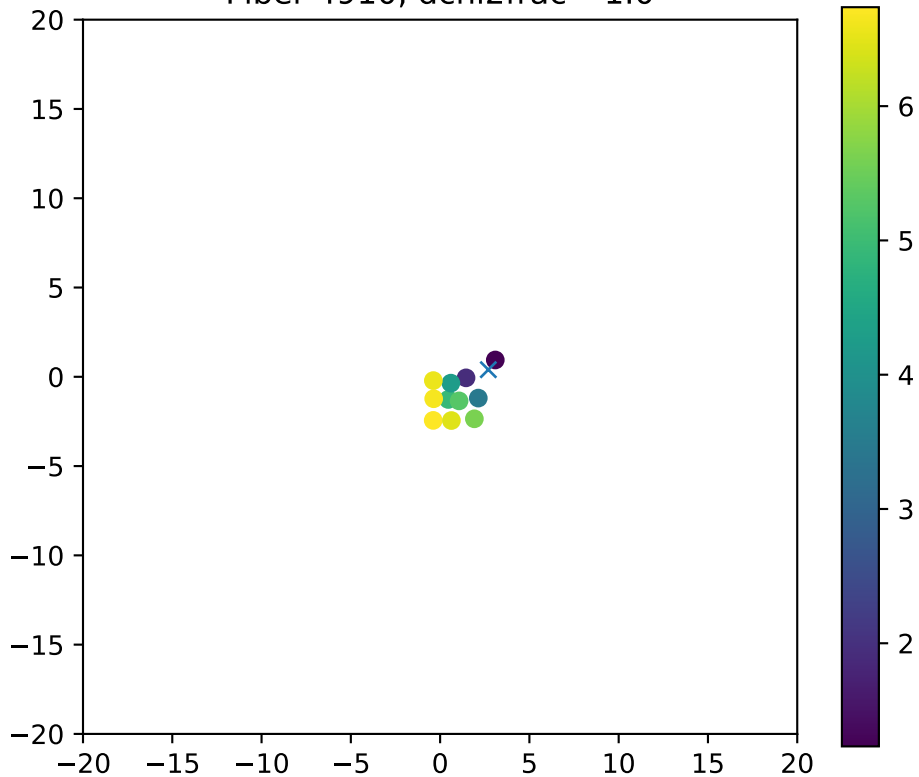
Fiber 4910, dchi2frac= 1.0
