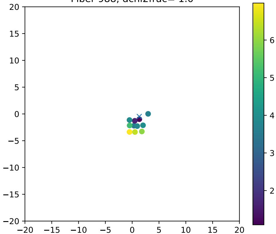
Fiber 988, dchi2frac= 1.0
