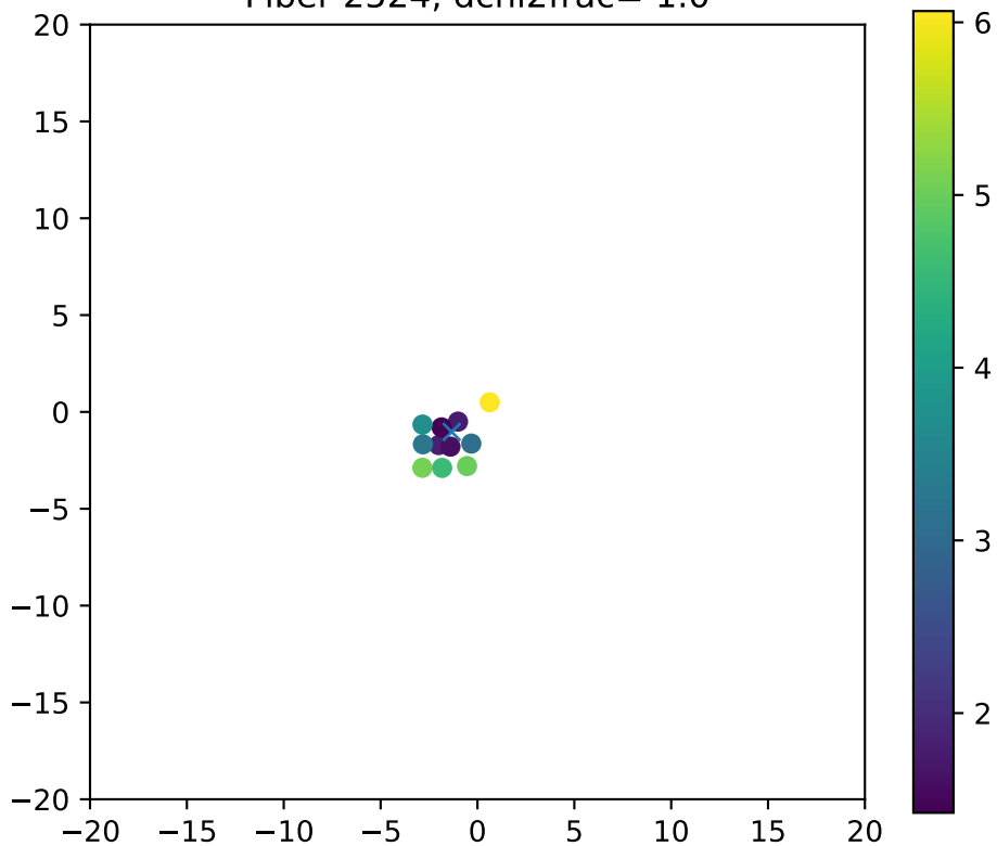
Fiber 2524, dchi2frac= 1.0
