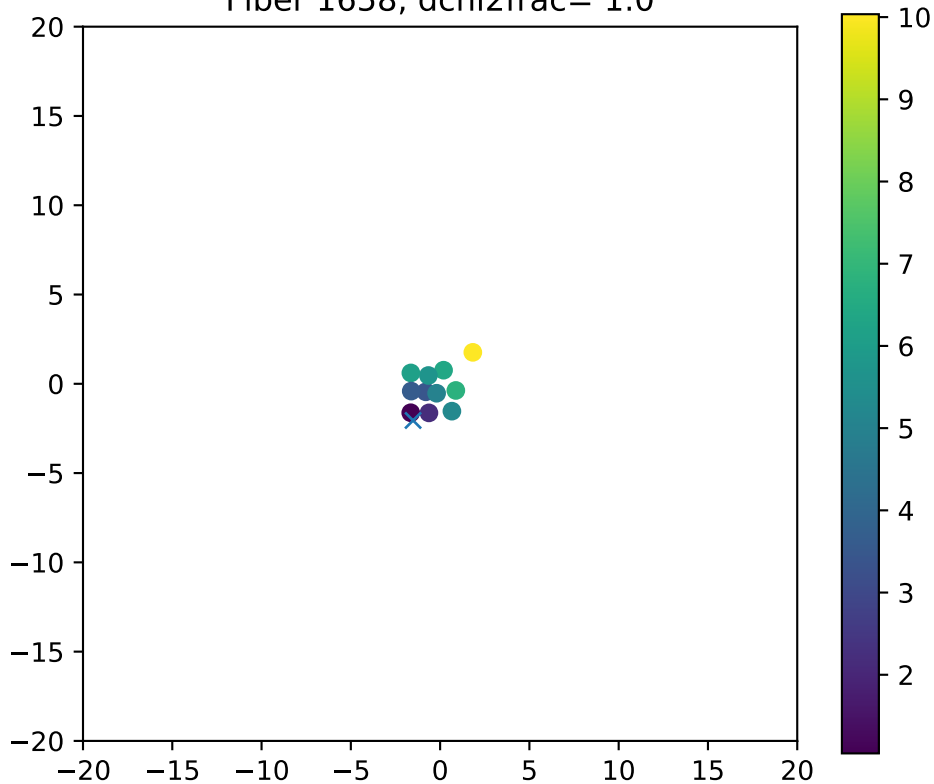
Fiber 1658, dchi2frac= 1.0
