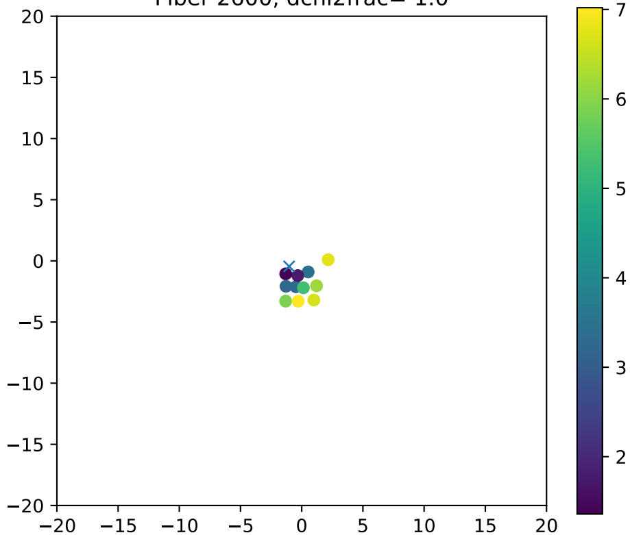
Fiber 2600, dchi2frac= 1.0
