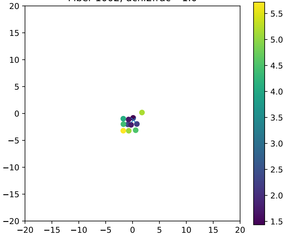
Fiber 1002, dchi2frac= 1.0
