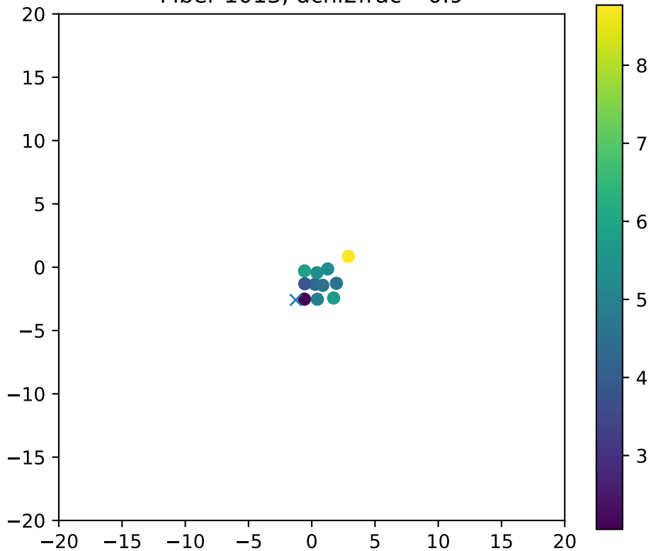
Fiber 1013, dchi2frac= 0.9
