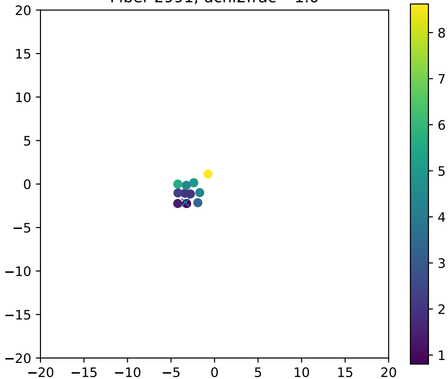
Fiber 2991, dchi2frac= 1.0
