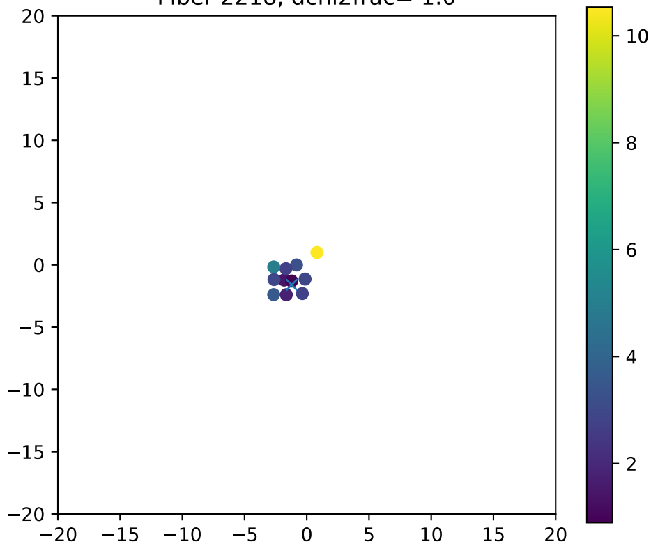
Fiber 2218, dchi2frac= 1.0
