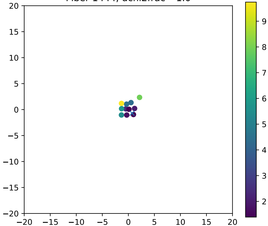
Fiber 1444, dchi2frac= 1.0
