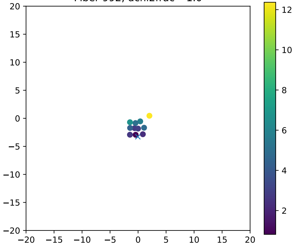
Fiber 992, dchi2frac= 1.0
