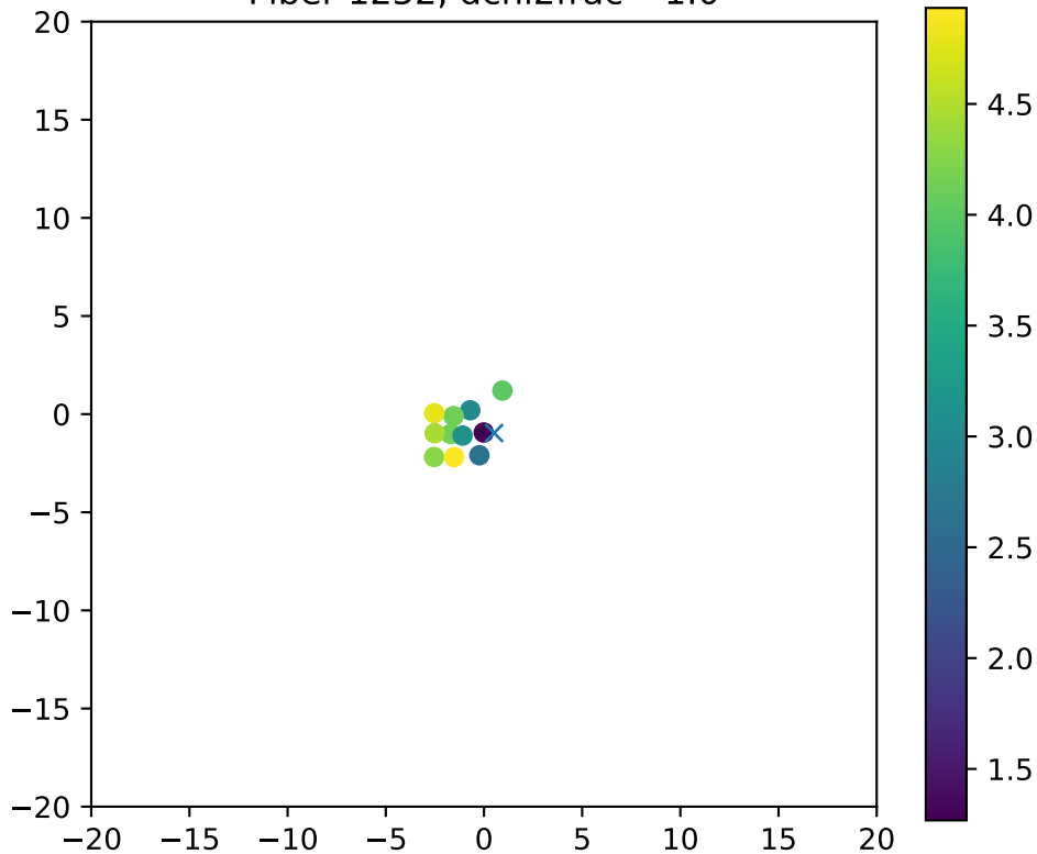
Fiber 1252, dchi2frac= 1.0
