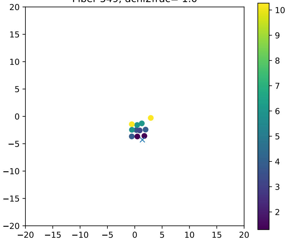
Fiber 549, dchi2frac= 1.0
