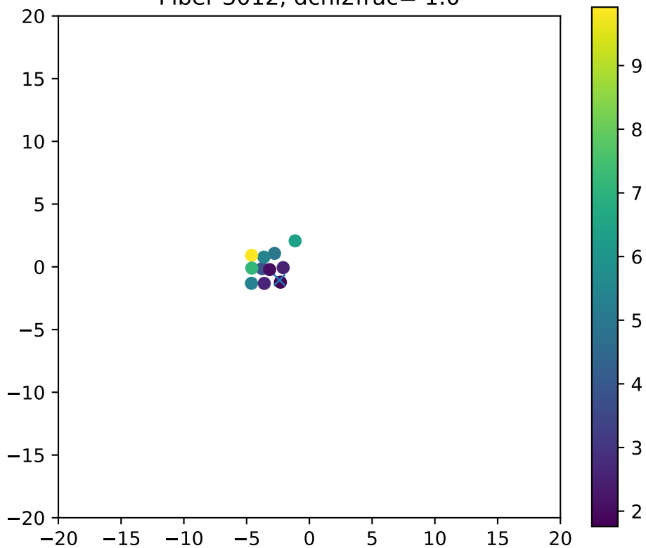
Fiber 3012, dchi2frac= 1.0
