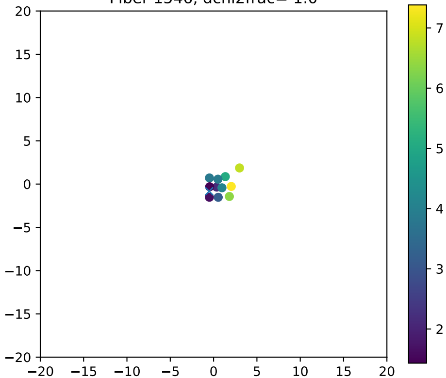
Fiber 1546, dchi2frac= 1.0
