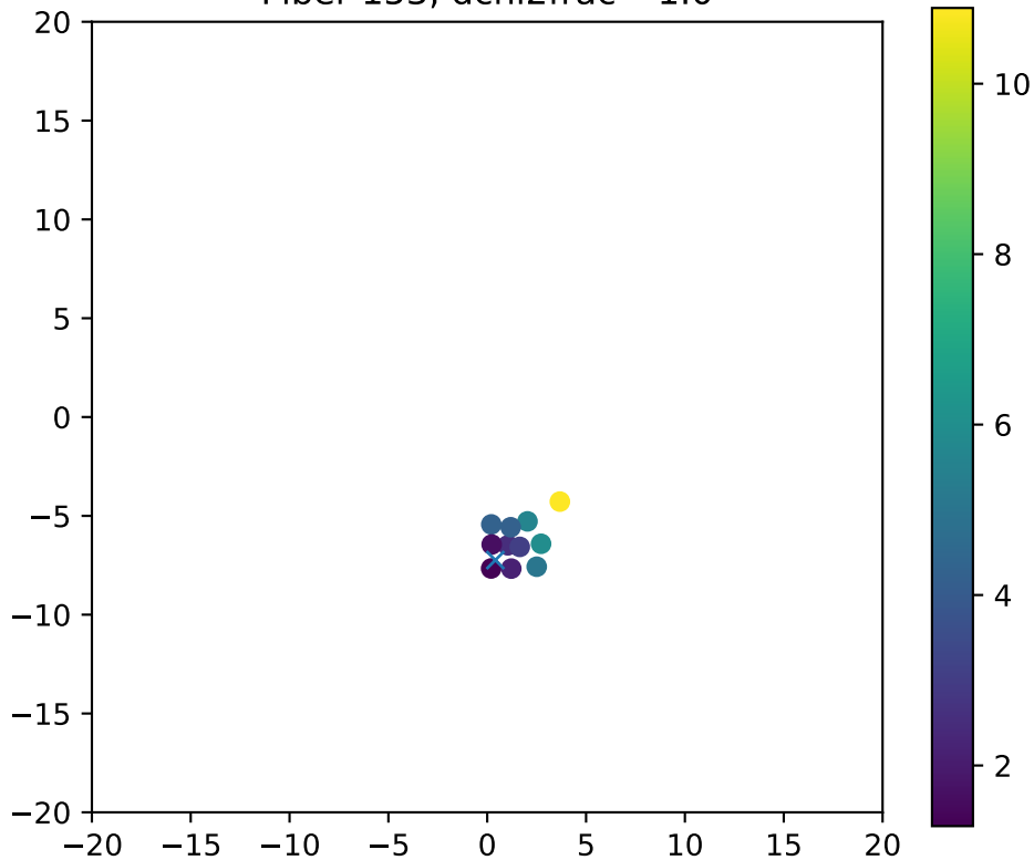
Fiber 153, dchi2frac= 1.0
