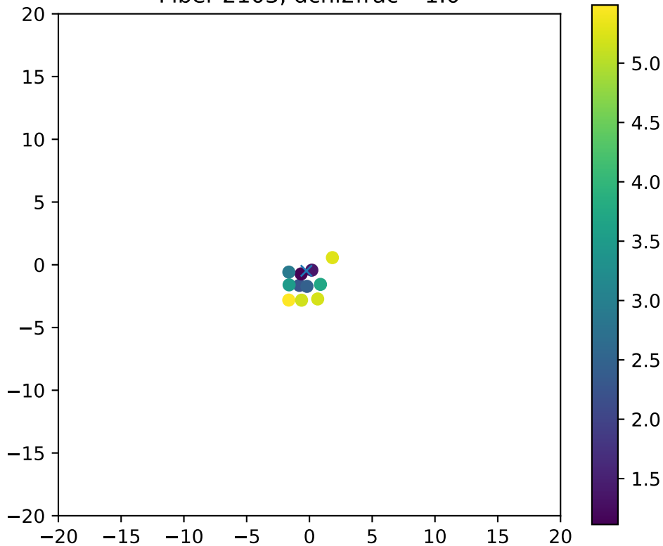
Fiber 2103, dchi2frac= 1.0
