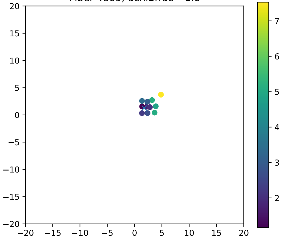
Fiber 4809, dchi2frac= 1.0
