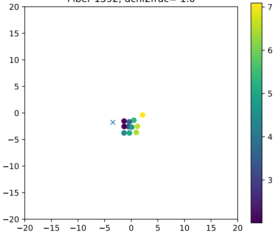
Fiber 1592, dchi2frac= 1.0
