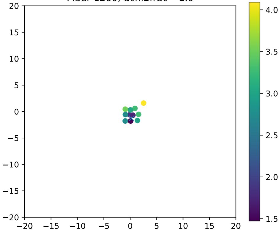
Fiber 1260, dchi2frac= 1.0
