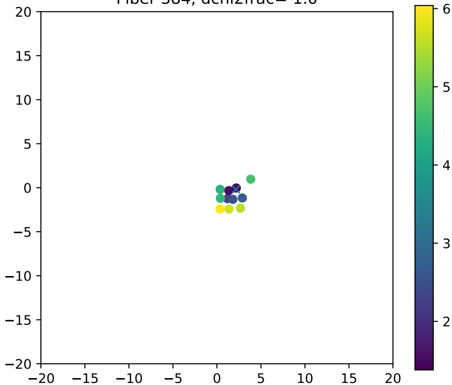
Fiber 384, dchi2frac= 1.0
