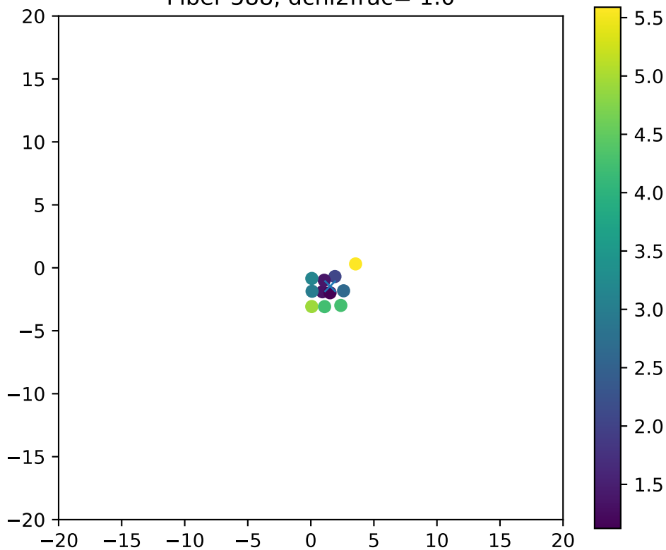
Fiber 588, dchi2frac= 1.0
