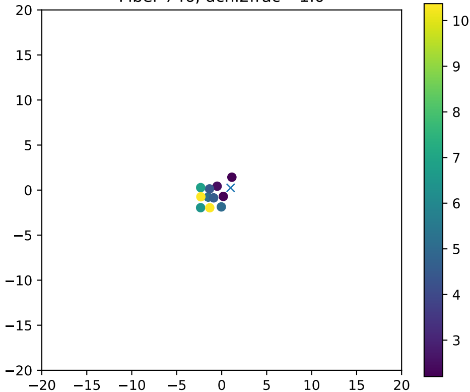
Fiber 746, dchi2frac= 1.0
