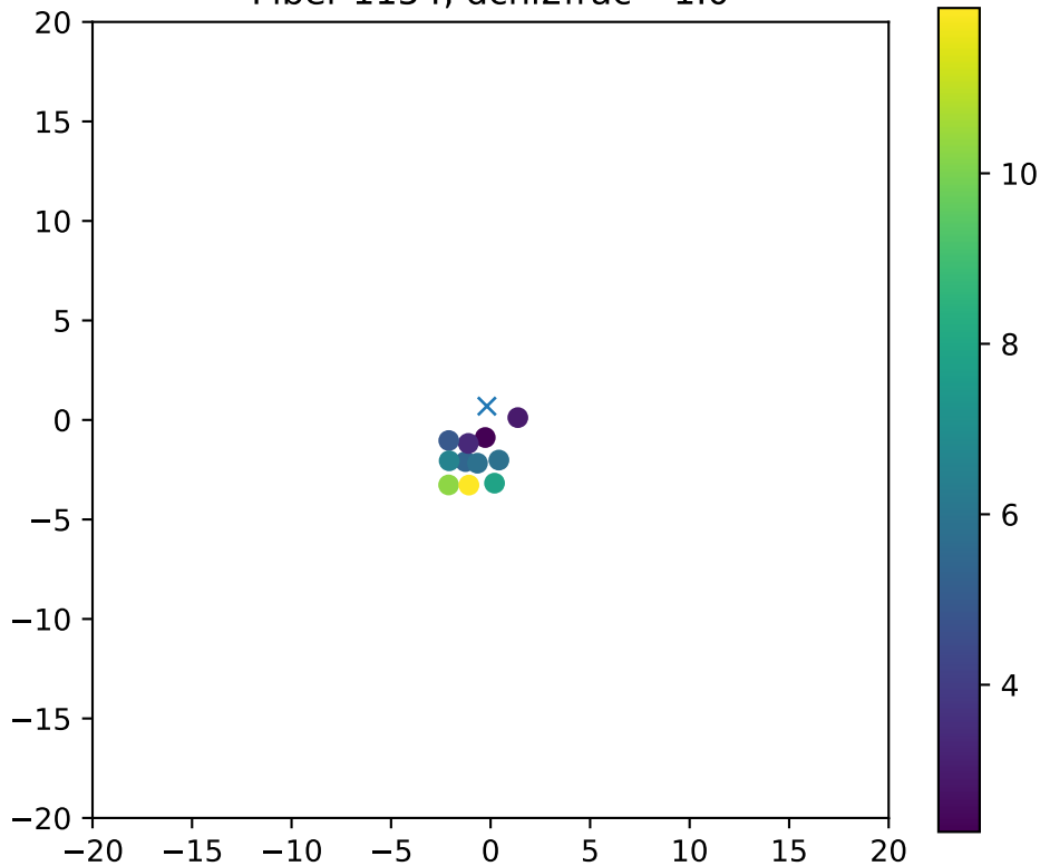
Fiber 1154, dchi2frac= 1.0
