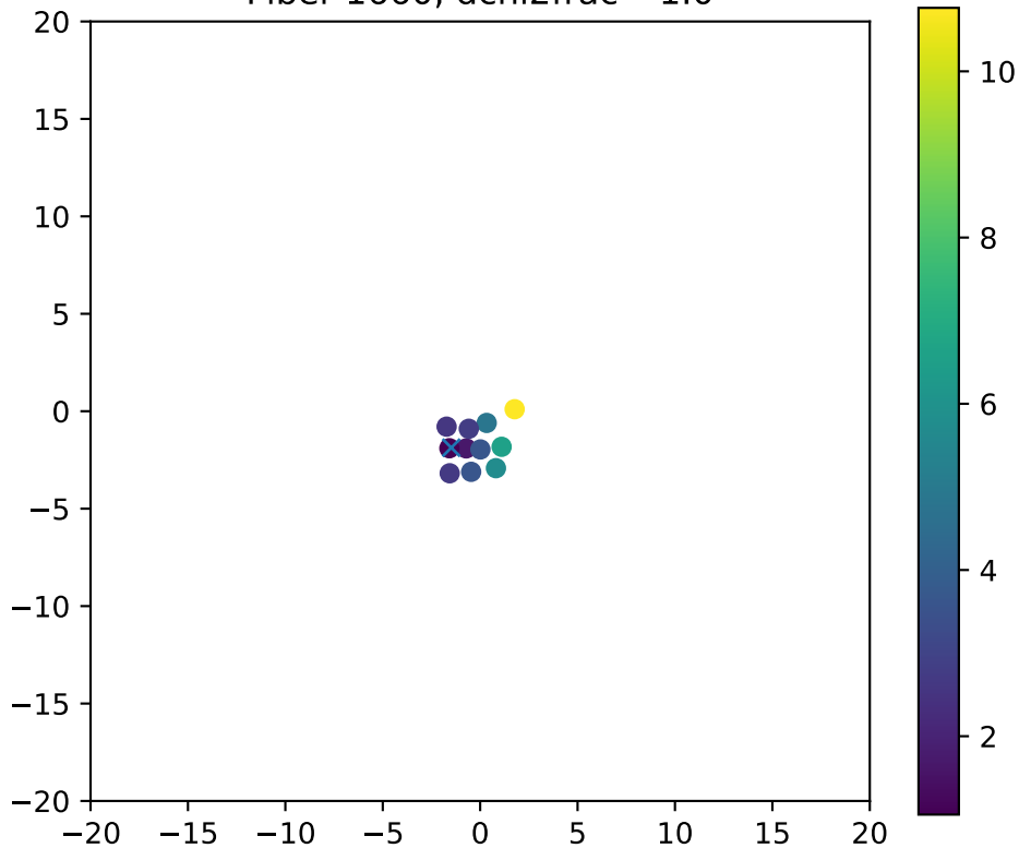
Fiber 1660, dchi2frac= 1.0
