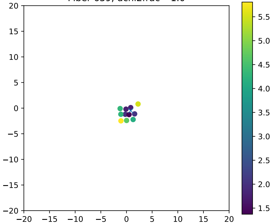
Fiber 639, dchi2frac= 1.0
