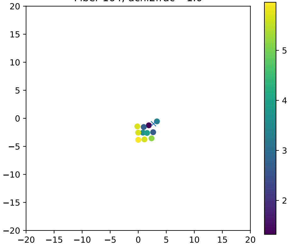
Fiber 164, dchi2frac= 1.0
