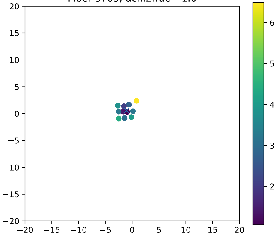
Fiber 3705, dchi2frac= 1.0
