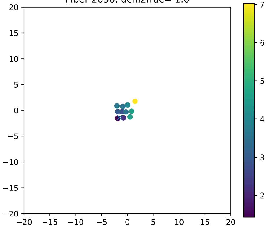
Fiber 2096, dchi2frac= 1.0
