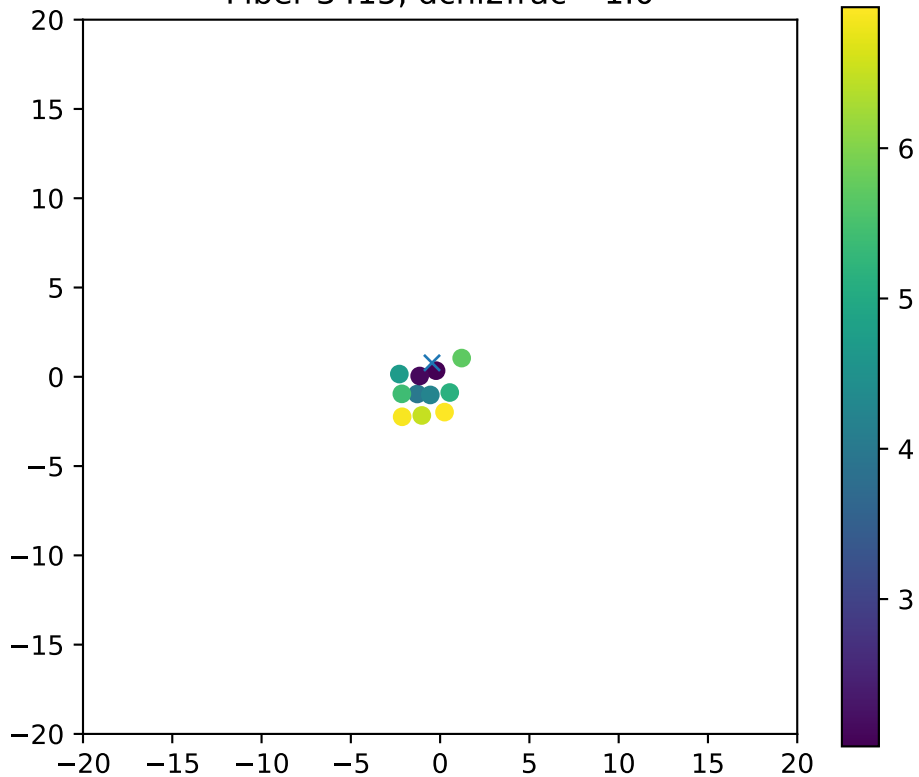
Fiber 3415, dchi2frac= 1.0
