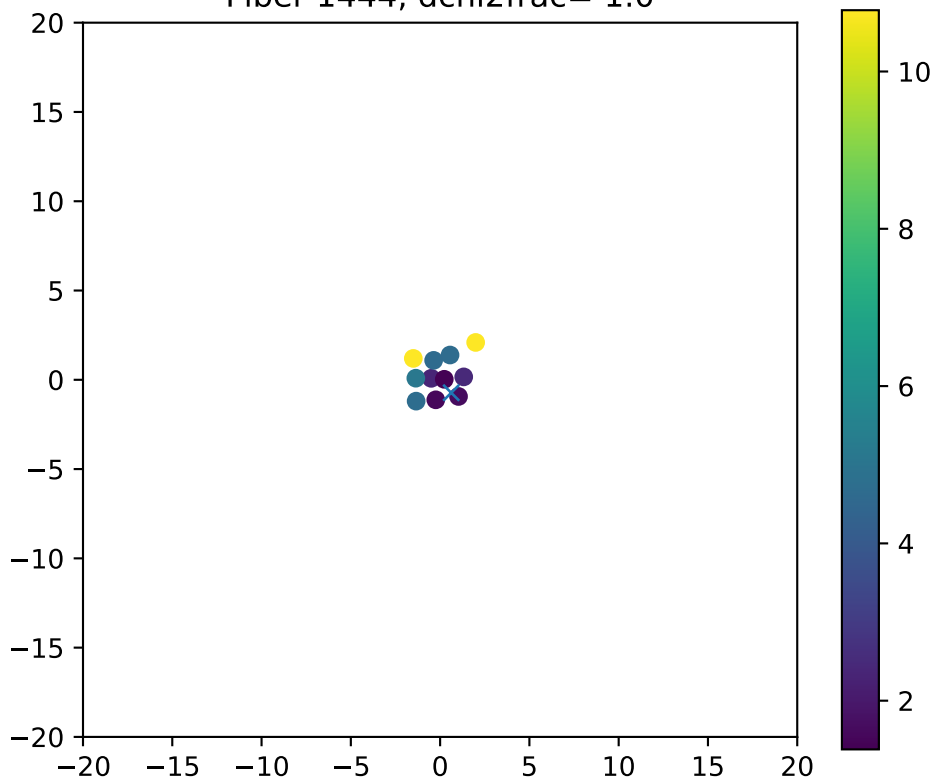
Fiber 1444, dchi2frac= 1.0
