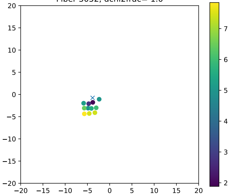
Fiber 3052, dchi2frac= 1.0
