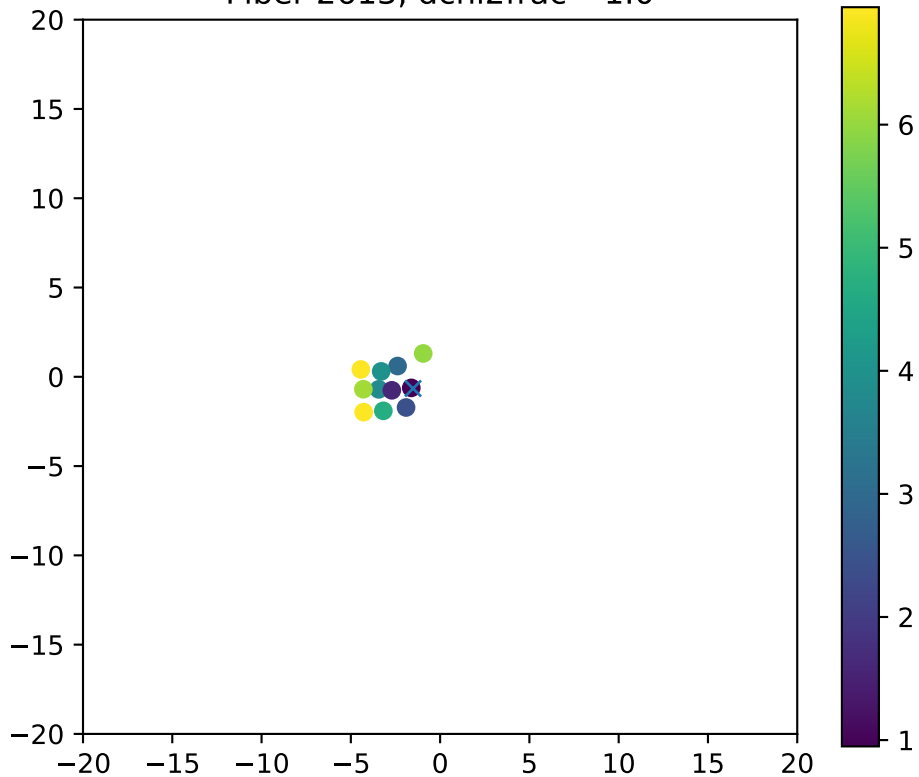
Fiber 2613, dchi2frac= 1.0
