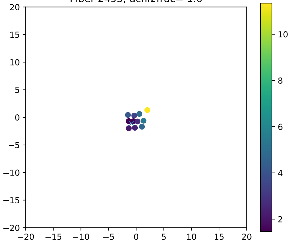
Fiber 2495, dchi2frac= 1.0
