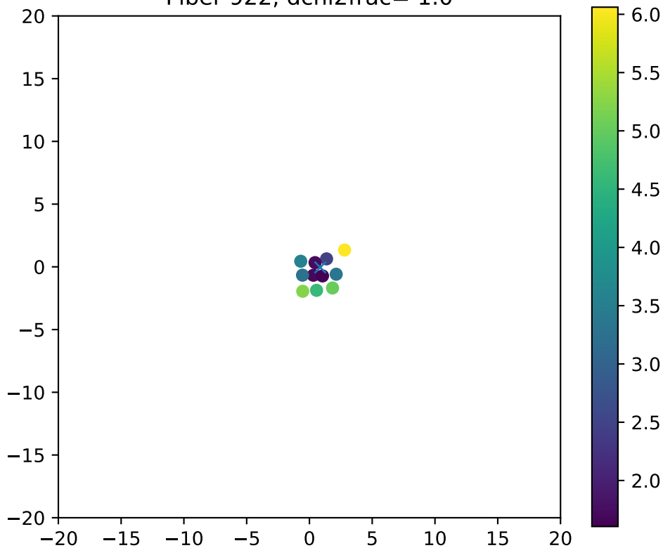
Fiber 922, dchi2frac= 1.0
