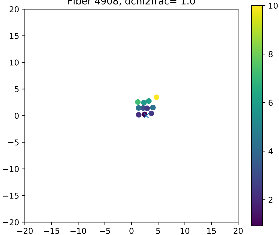
Fiber 4908, dchi2frac= 1.0
