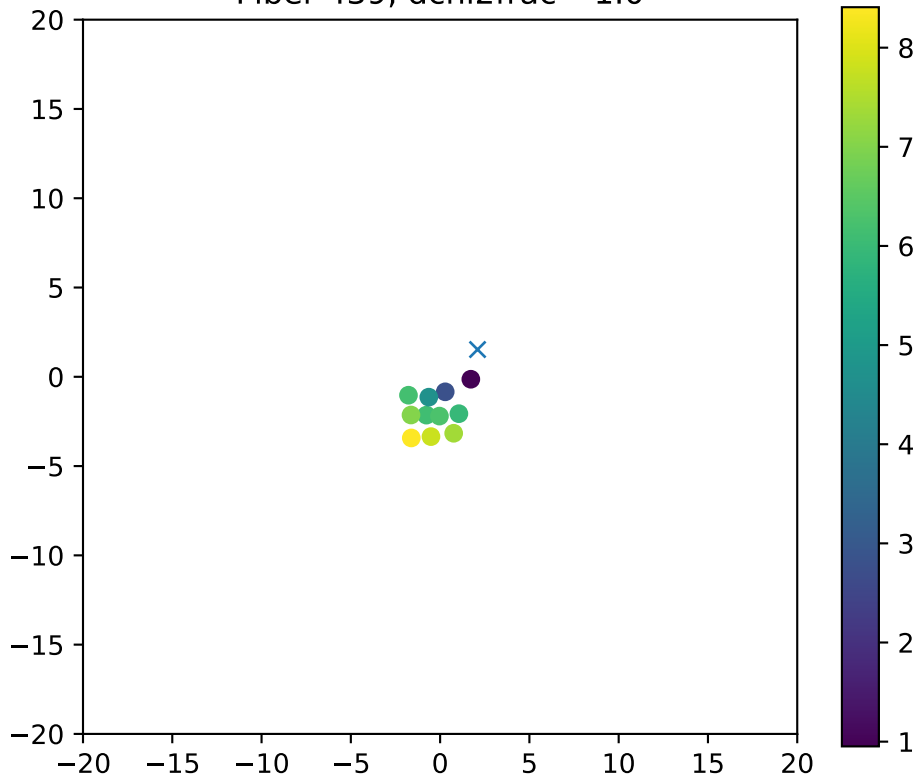
Fiber 439, dchi2frac= 1.0
