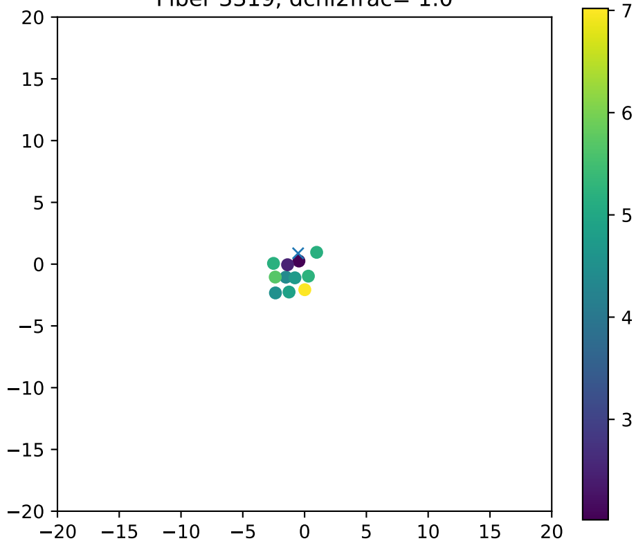
Fiber 3319, dchi2frac= 1.0
