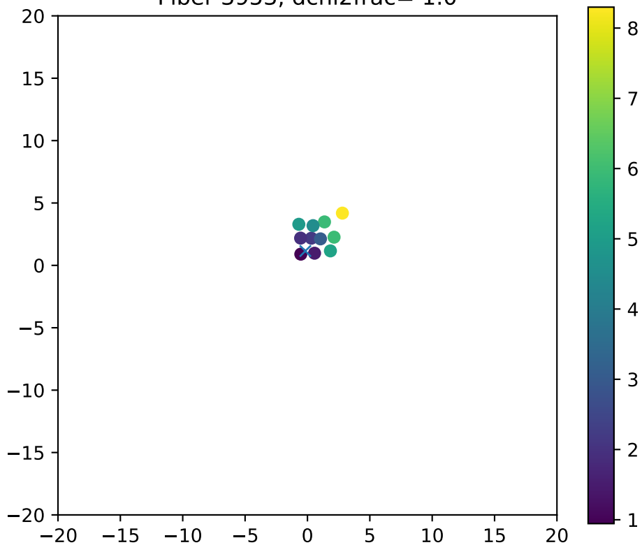
Fiber 3953, dchi2frac= 1.0
