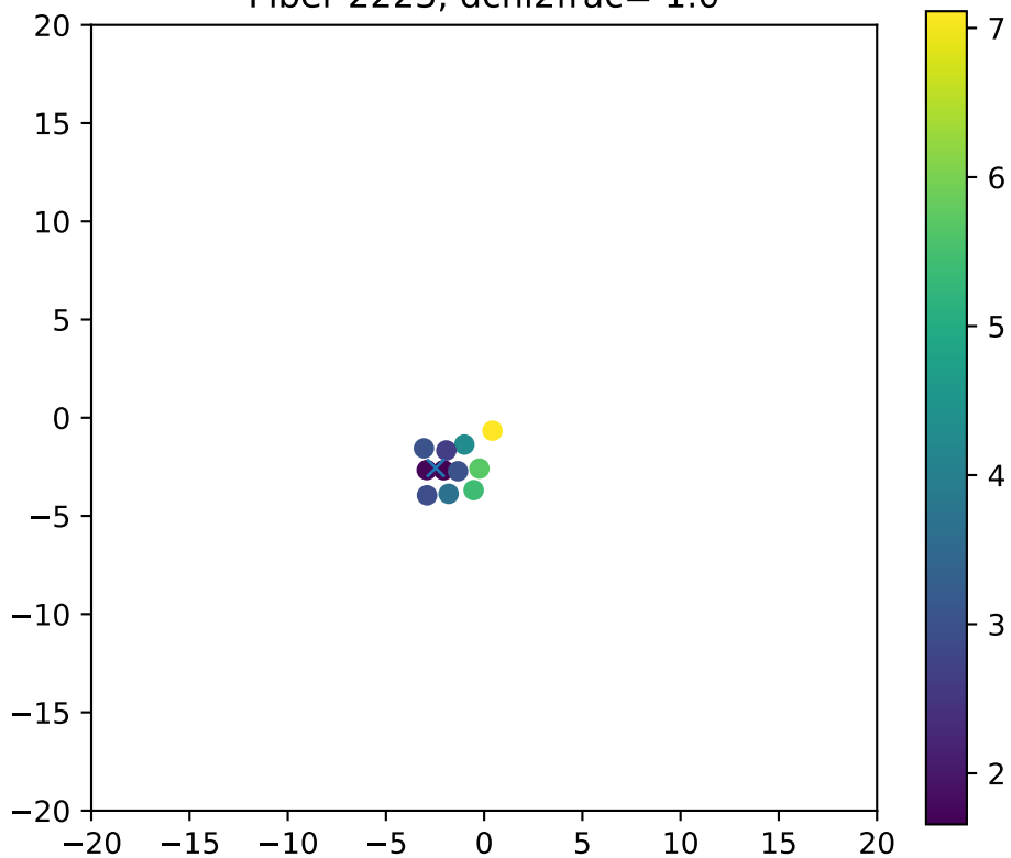
Fiber 2223, dchi2frac= 1.0
