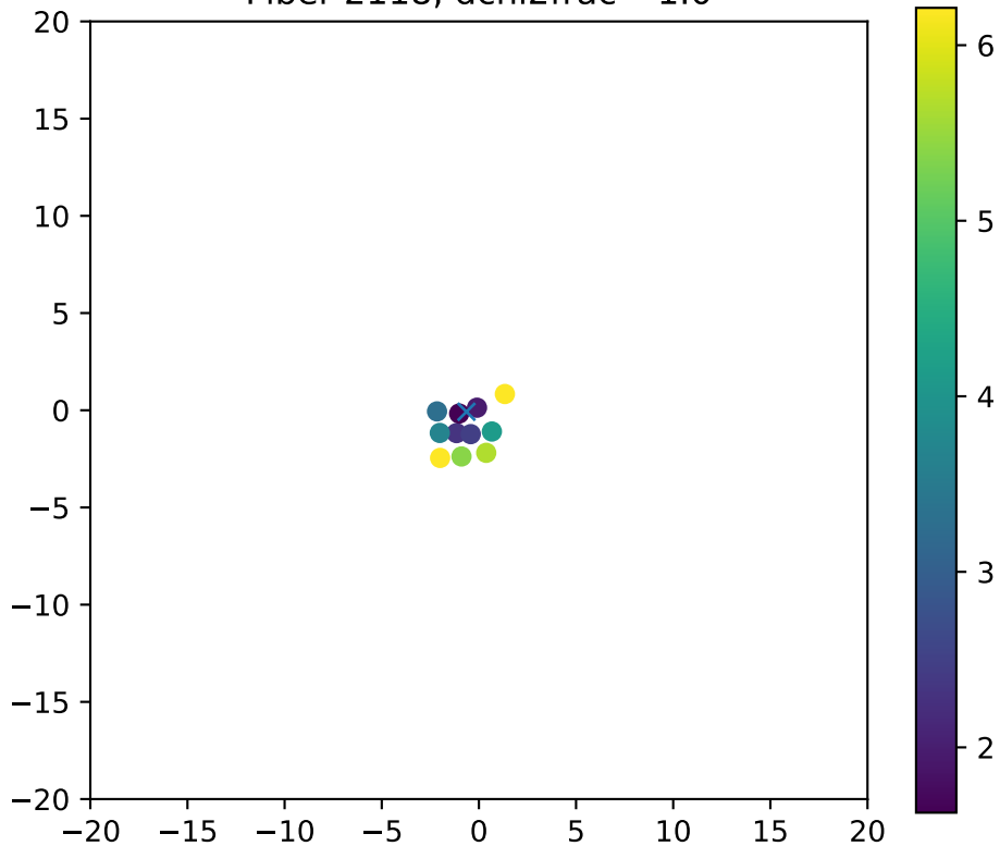
Fiber 2118, dchi2frac= 1.0
