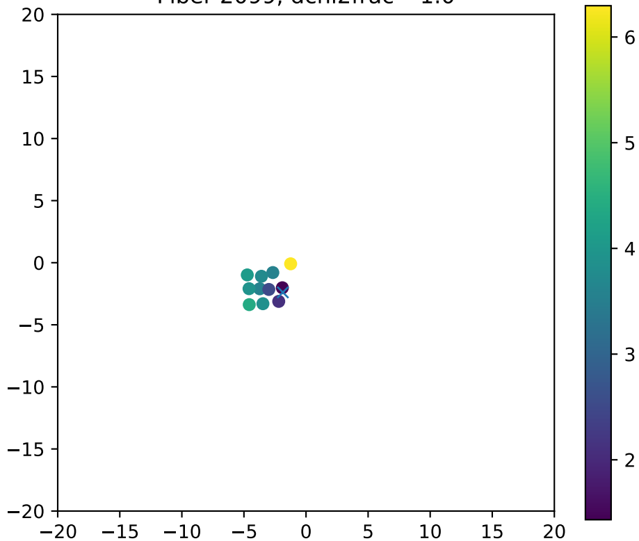
Fiber 2099, dchi2frac= 1.0
