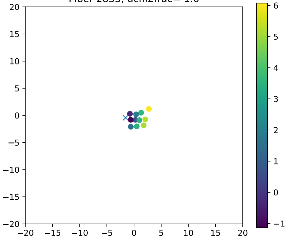
Fiber 2833, dchi2frac= 1.0
