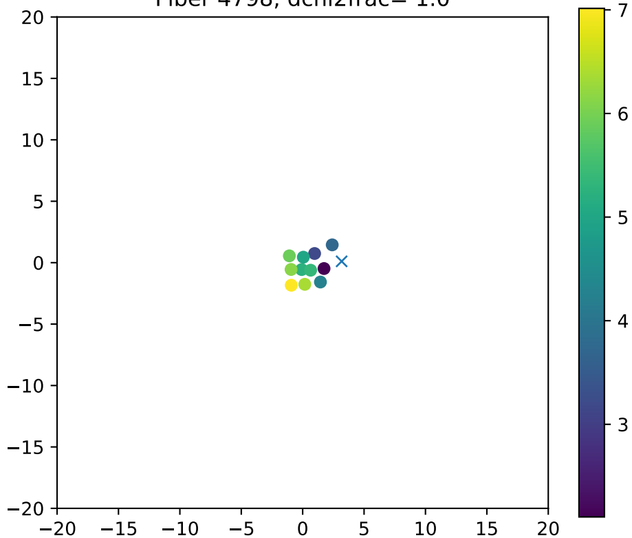
Fiber 4798, dchi2frac= 1.0
