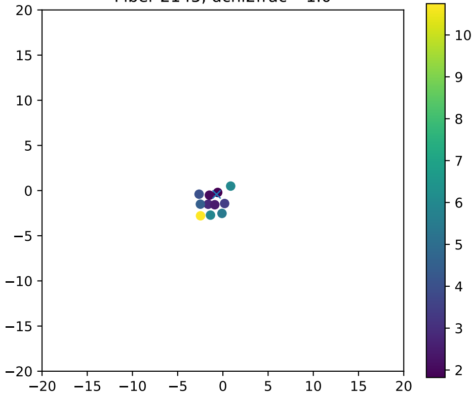
Fiber 2145, dchi2frac= 1.0
