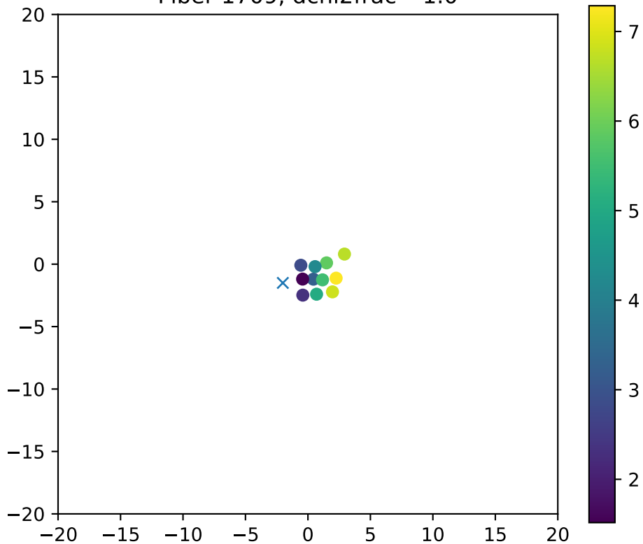
Fiber 1709, dchi2frac= 1.0
