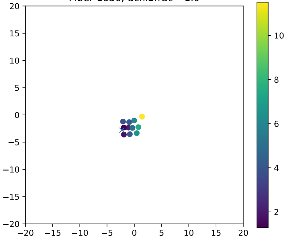
Fiber 1636, dchi2frac= 1.0
