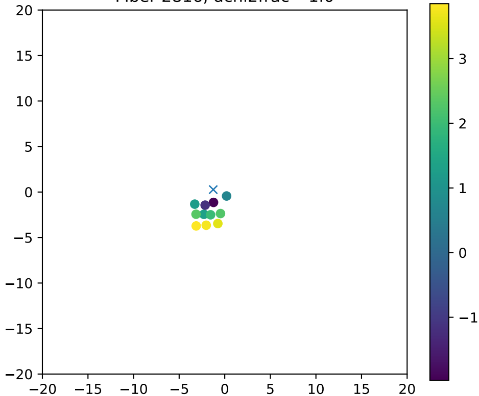
Fiber 2816, dchi2frac= 1.0
