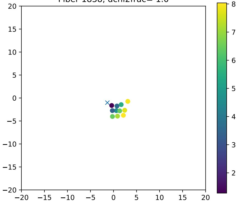
Fiber 1838, dchi2frac= 1.0
