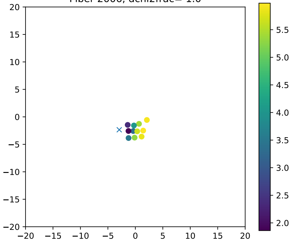
Fiber 2006, dchi2frac= 1.0
