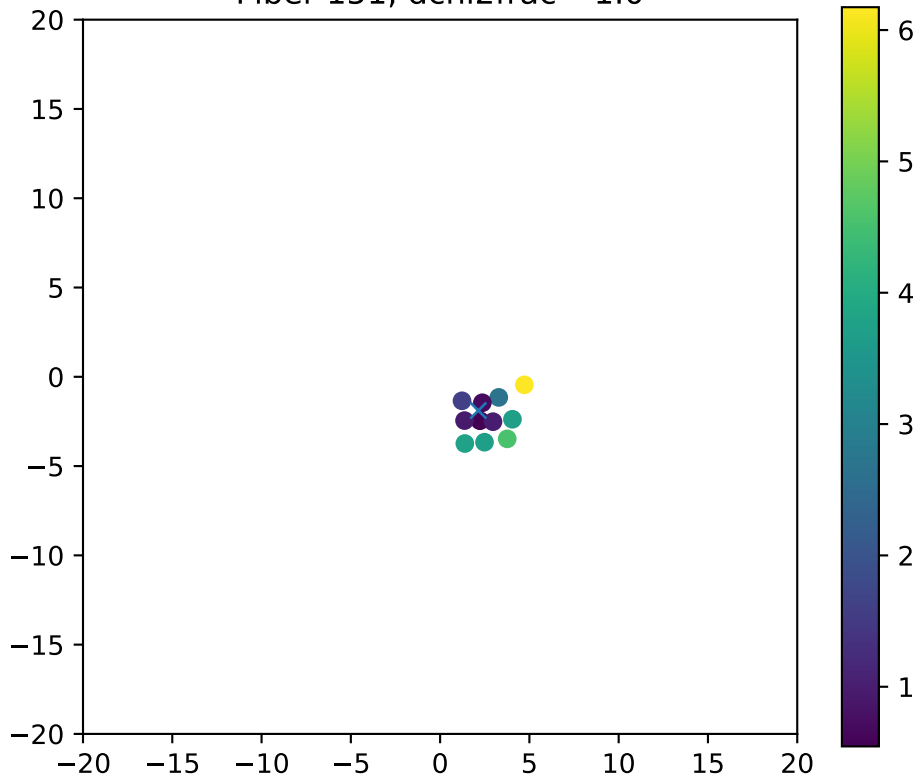
Fiber 151, dchi2frac= 1.0
