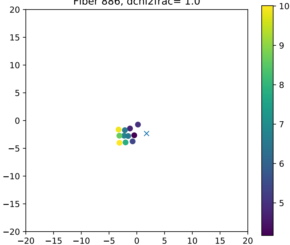
Fiber 886, dchi2frac= 1.0
