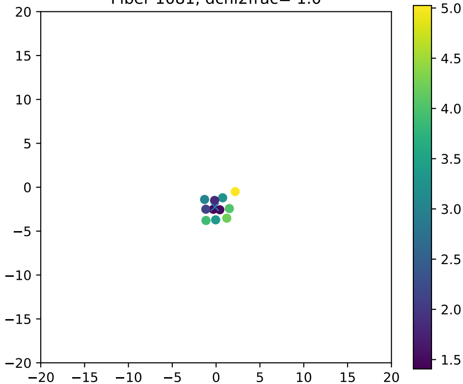
Fiber 1081, dchi2frac= 1.0
