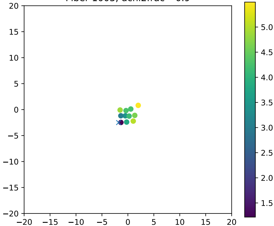
Fiber 1003, dchi2frac= 0.9
