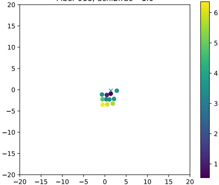
Fiber 988, dchi2frac= 1.0
