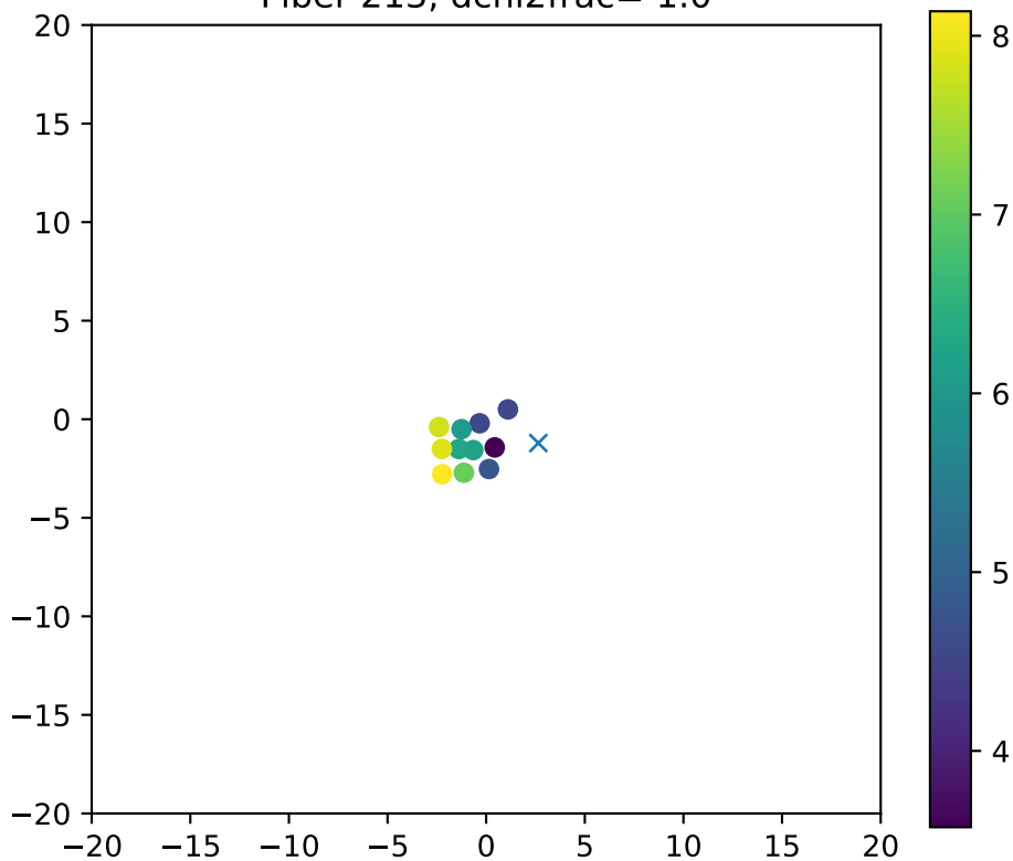
Fiber 213, dchi2frac= 1.0
