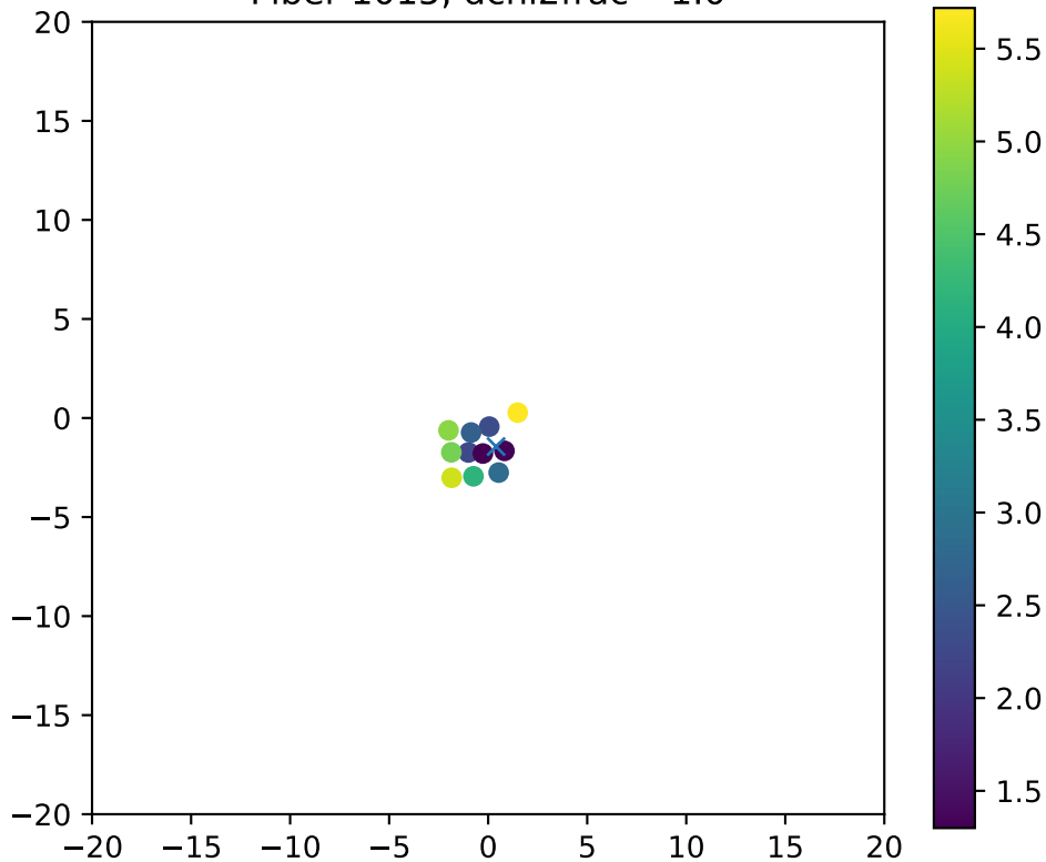
Fiber 1015, dchi2frac= 1.0
