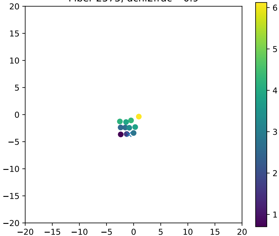
Fiber 2573, dchi2frac= 0.9
