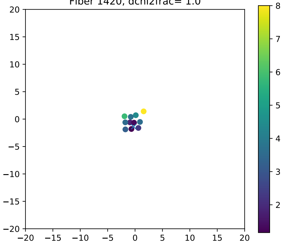
Fiber 1420, dchi2frac= 1.0
