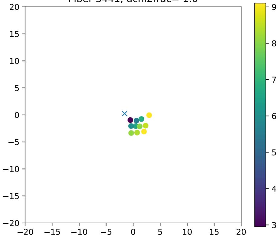
Fiber 3441, dchi2frac= 1.0
