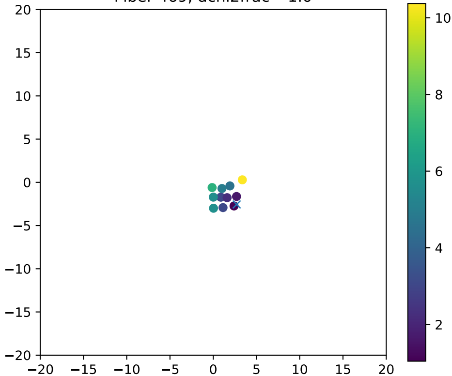
Fiber 469, dchi2frac= 1.0
