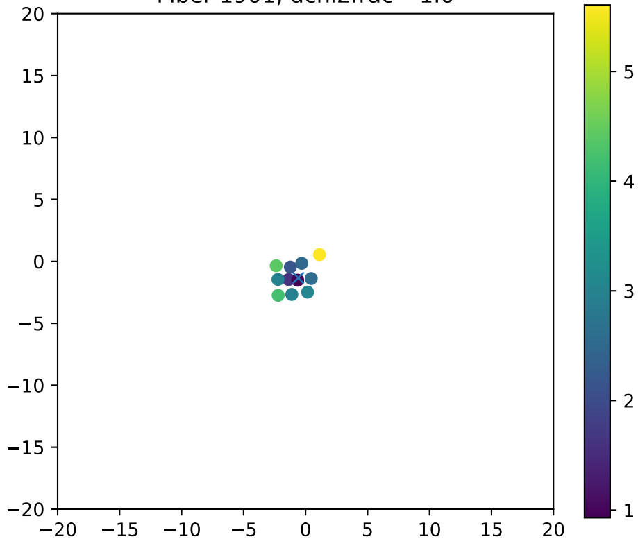
Fiber 1901, dchi2frac= 1.0
