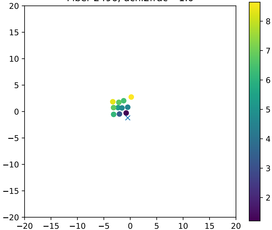
Fiber 2496, dchi2frac= 1.0
