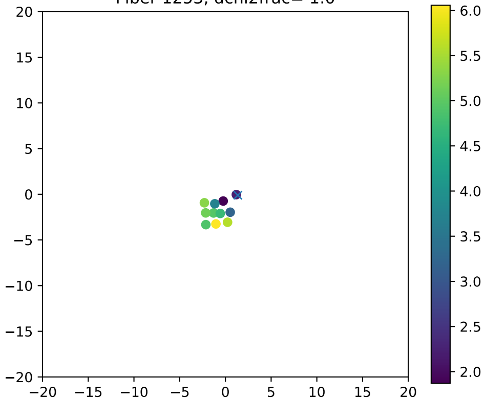
Fiber 1253, dchi2frac= 1.0
