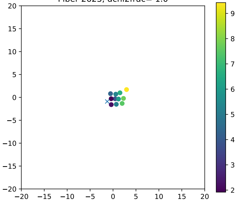
Fiber 2623, dchi2frac= 1.0
