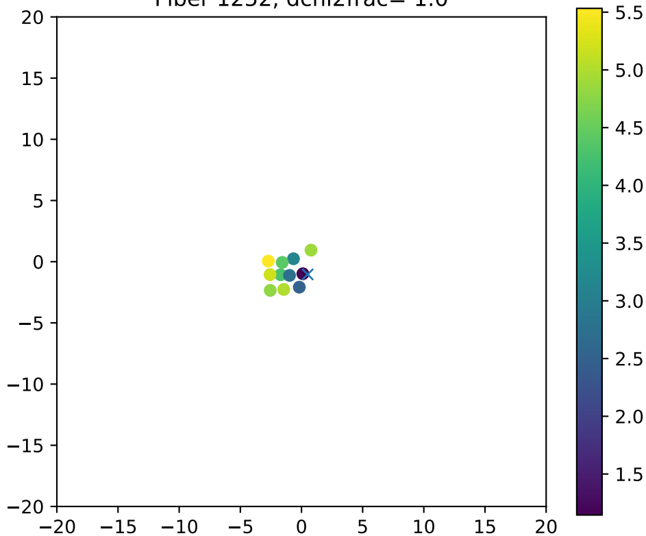
Fiber 1252, dchi2frac= 1.0
