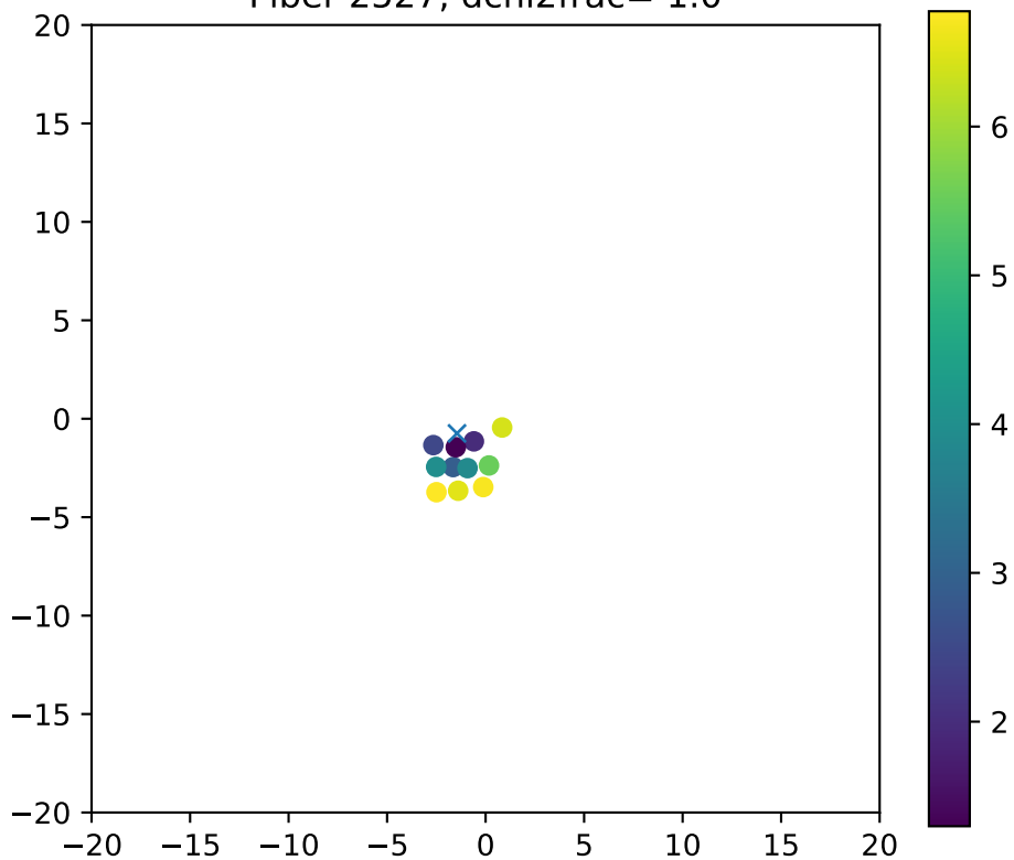
Fiber 2527, dchi2frac= 1.0
