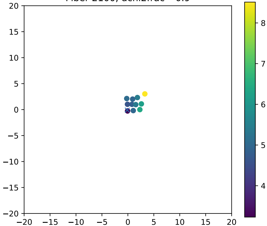
Fiber 2100, dchi2frac= 0.9
