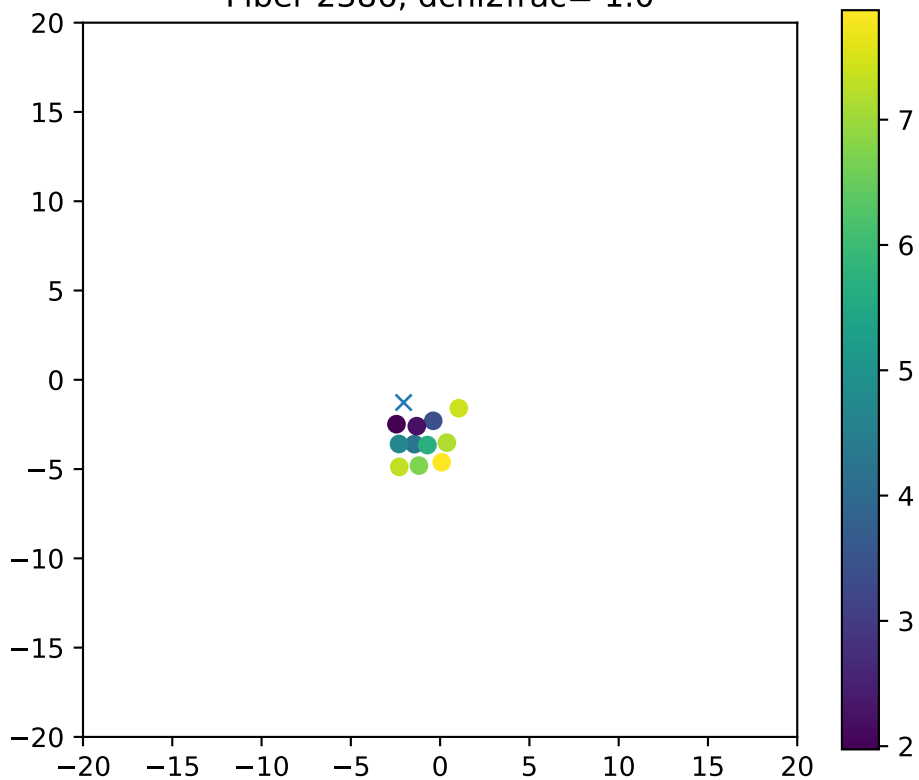
Fiber 2386, dchi2frac= 1.0
