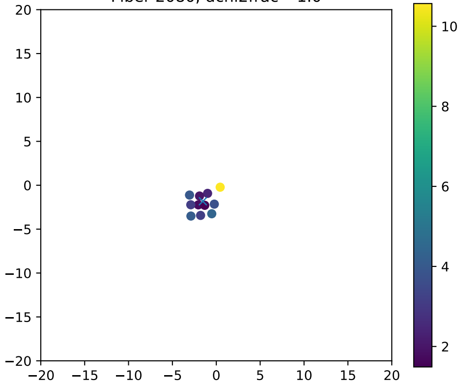
Fiber 2080, dchi2frac= 1.0
