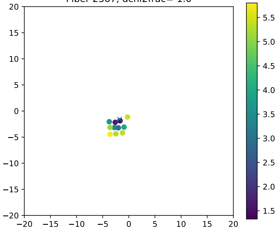
Fiber 2367, dchi2frac= 1.0
