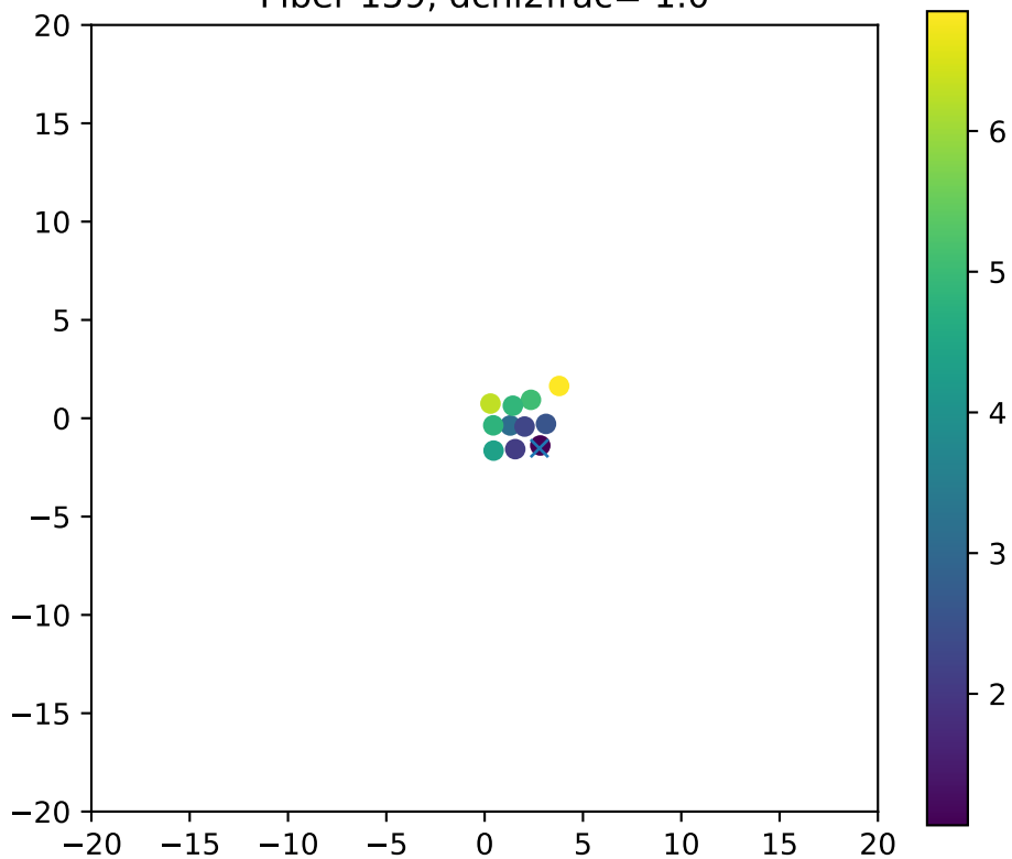
Fiber 159, dchi2frac= 1.0
