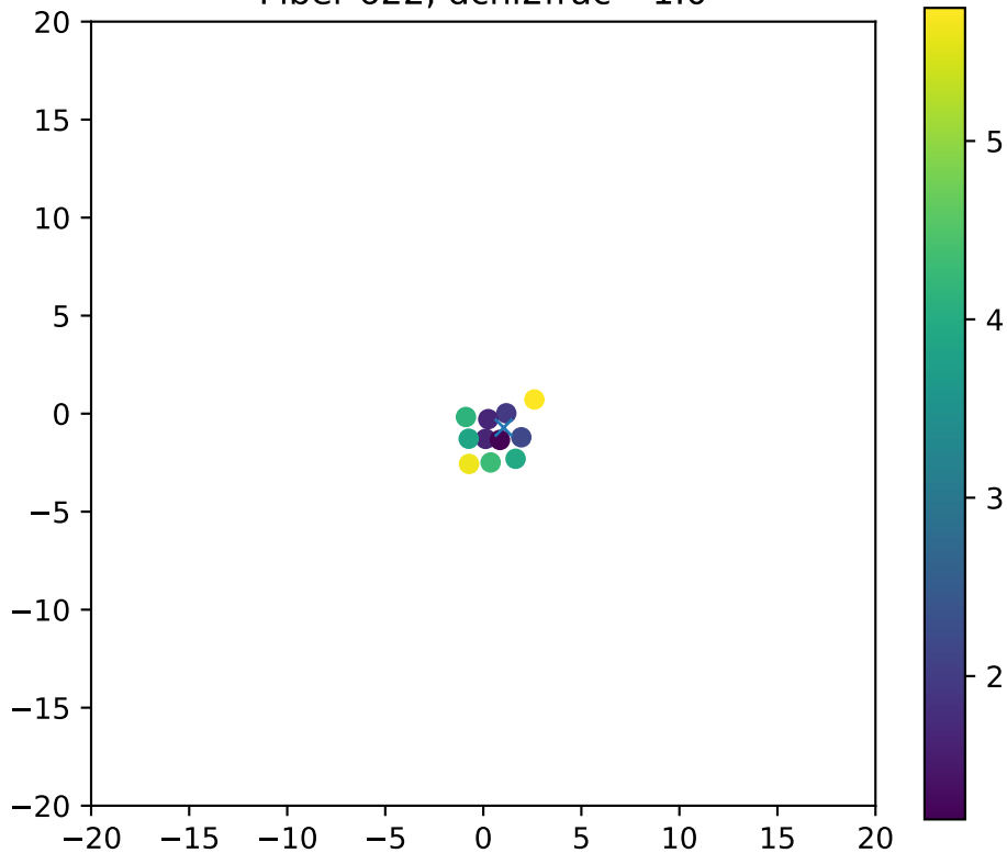
Fiber 622, dchi2frac= 1.0
