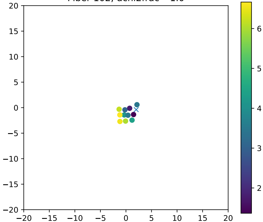
Fiber 102, dchi2frac= 1.0
