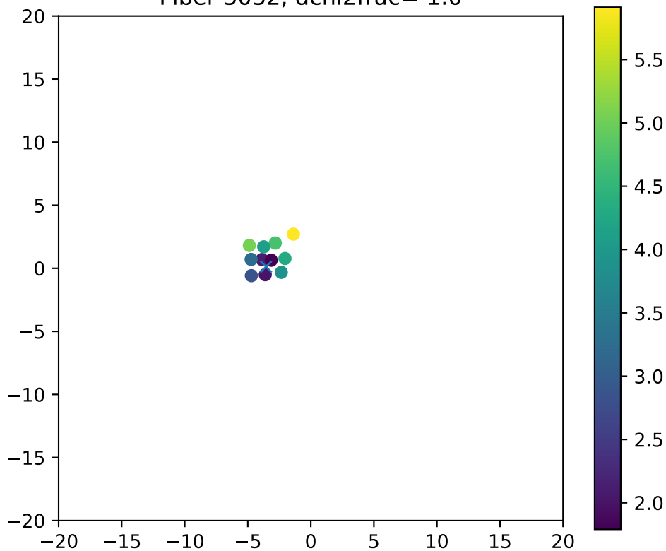
Fiber 3032, dchi2frac= 1.0
