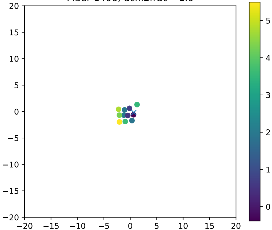
Fiber 1406, dchi2frac= 1.0
