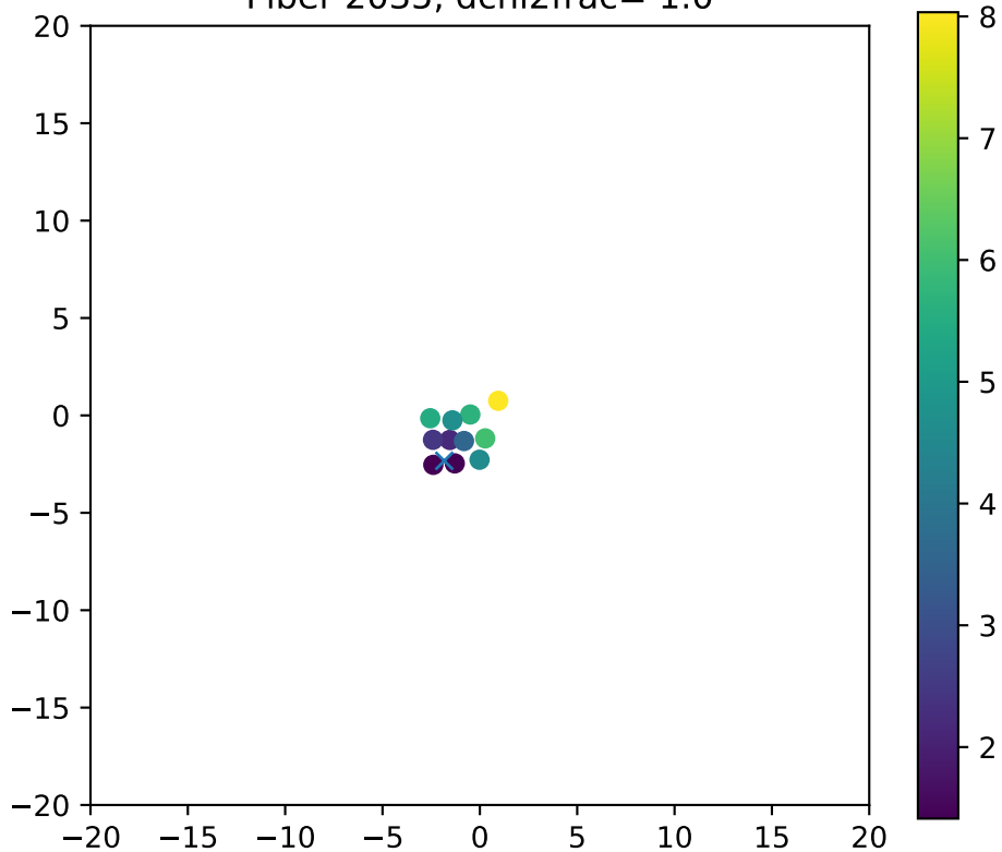
Fiber 2035, dchi2frac= 1.0
