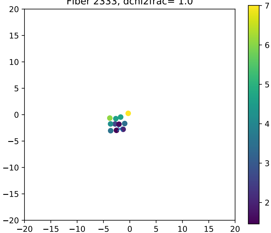
Fiber 2333, dchi2frac= 1.0
