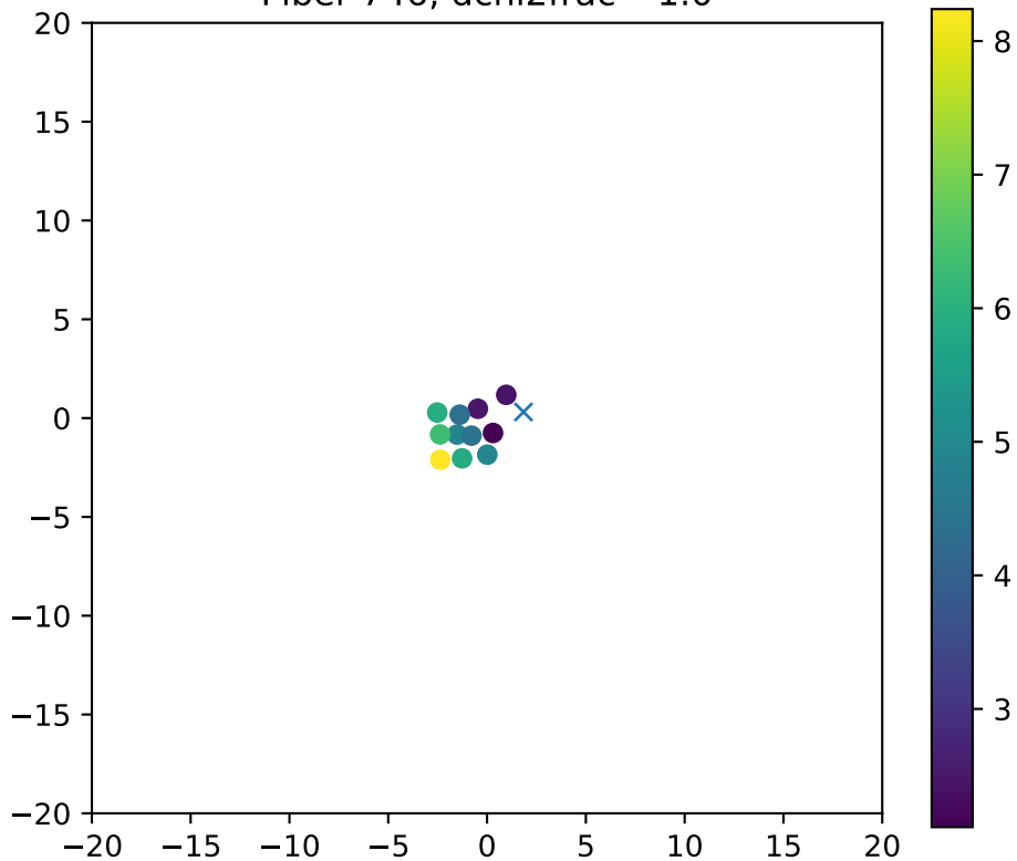
Fiber 746, dchi2frac= 1.0
