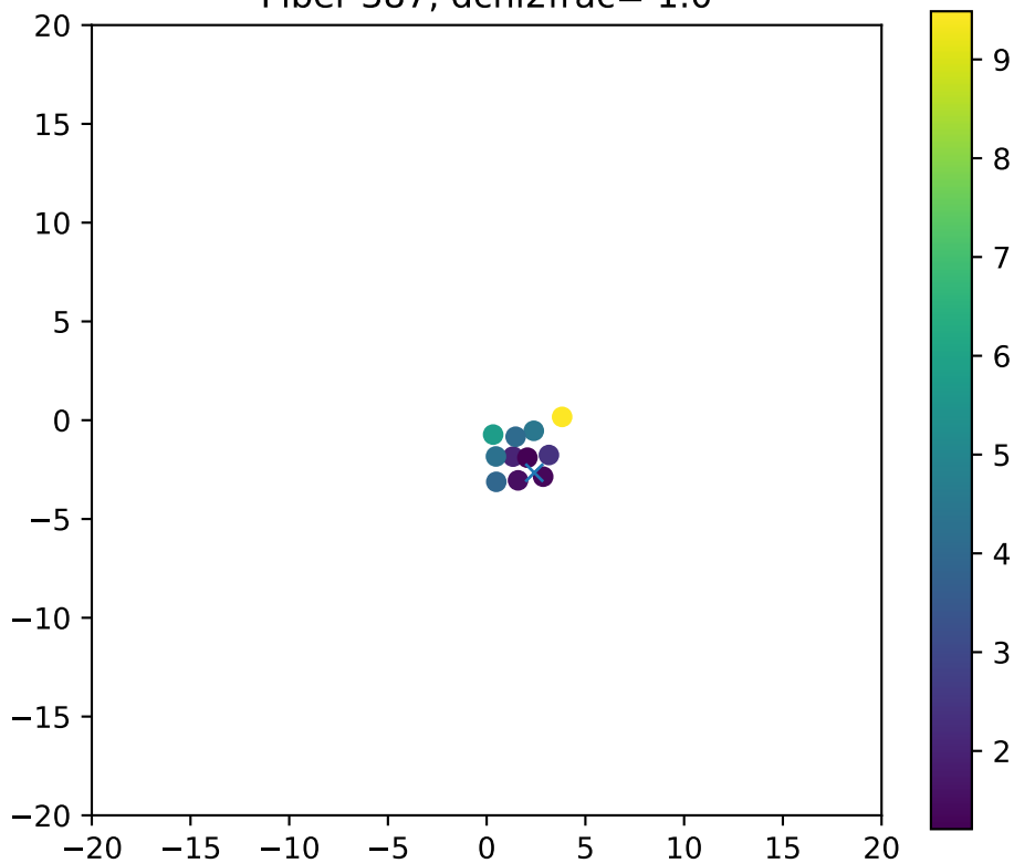
Fiber 387, dchi2frac= 1.0
