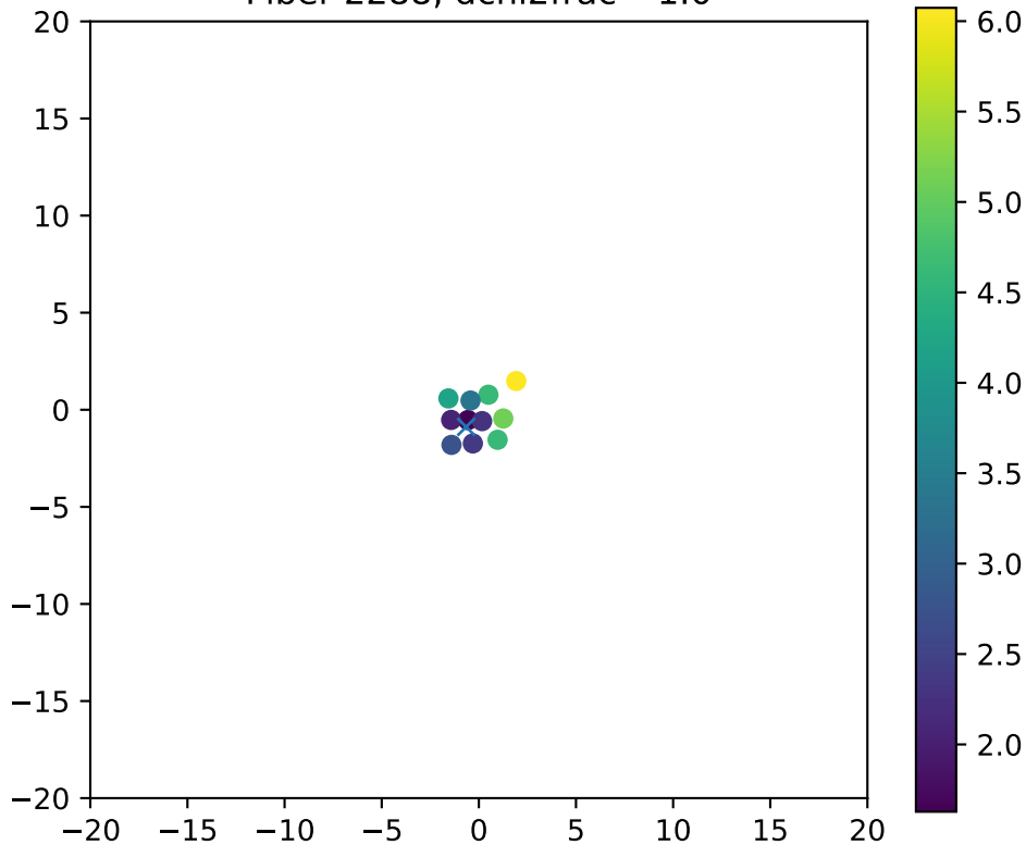
Fiber 2288, dchi2frac= 1.0
