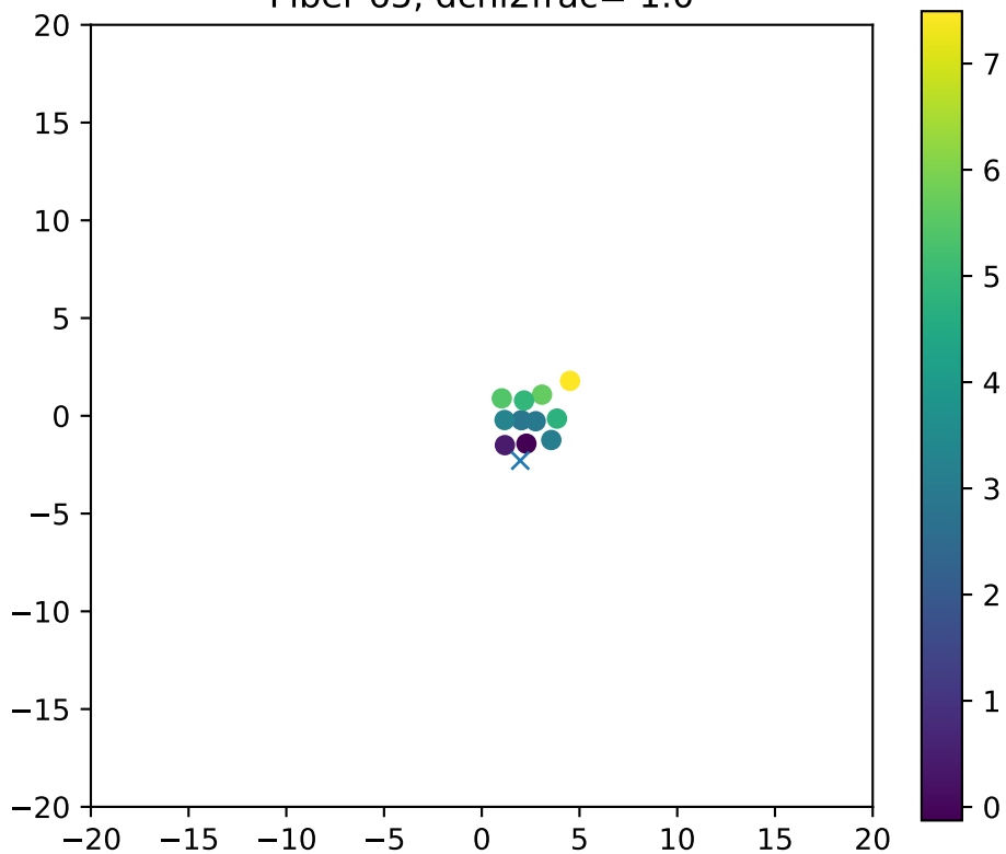
Fiber 65, dchi2frac= 1.0
