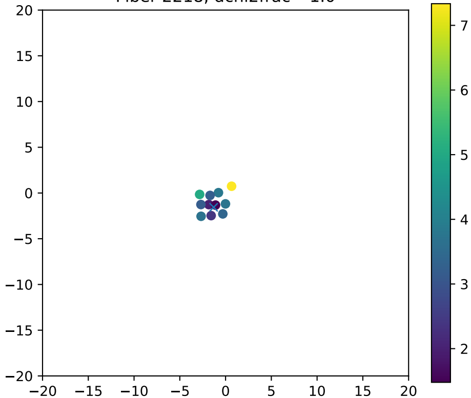
Fiber 2218, dchi2frac= 1.0
