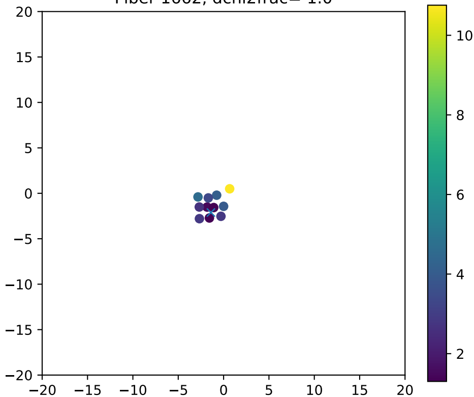
Fiber 1662, dchi2frac= 1.0
