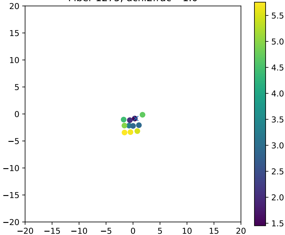
Fiber 1275, dchi2frac= 1.0
