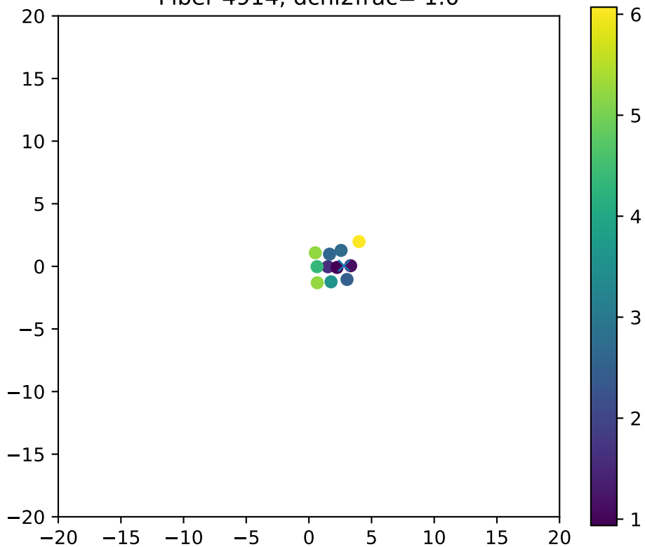
Fiber 4914, dchi2frac= 1.0
