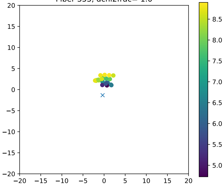
Fiber 353, dchi2frac= 1.0
