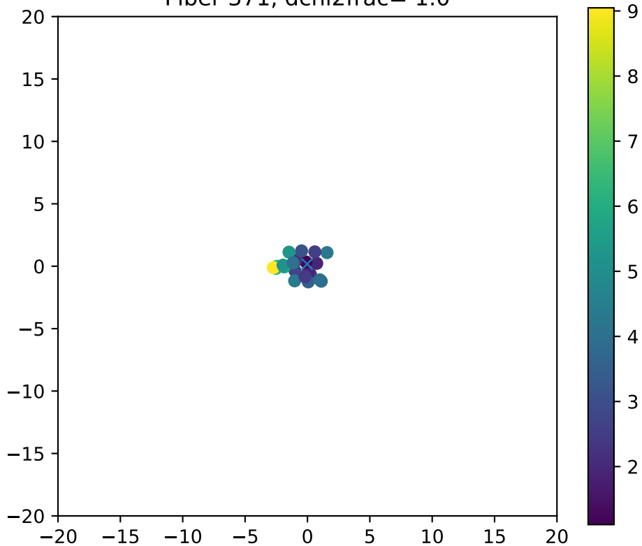
Fiber 371, dchi2frac= 1.0
