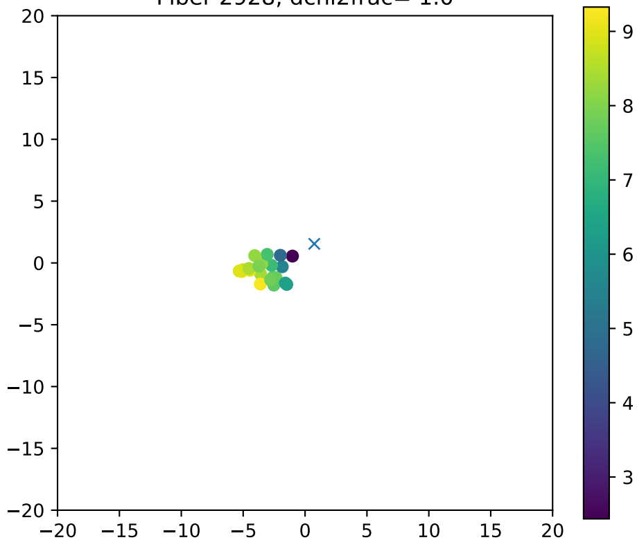
Fiber 2928, dchi2frac= 1.0
