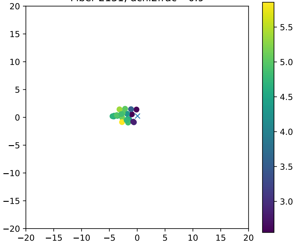
Fiber 2131, dchi2frac= 0.9
