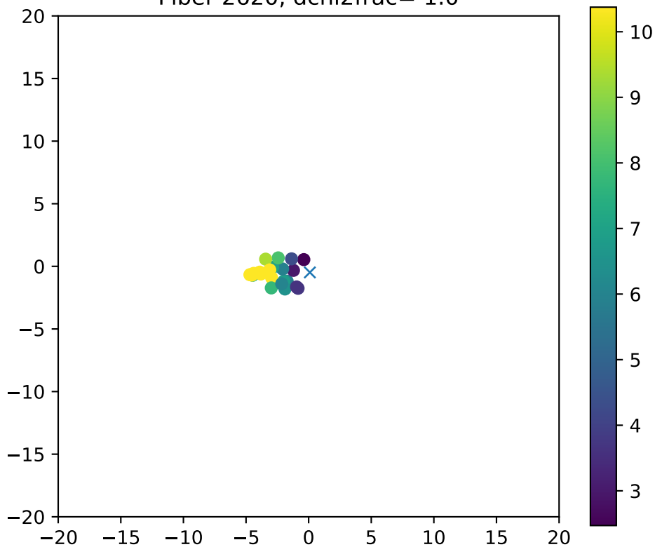
Fiber 2620, dchi2frac= 1.0
