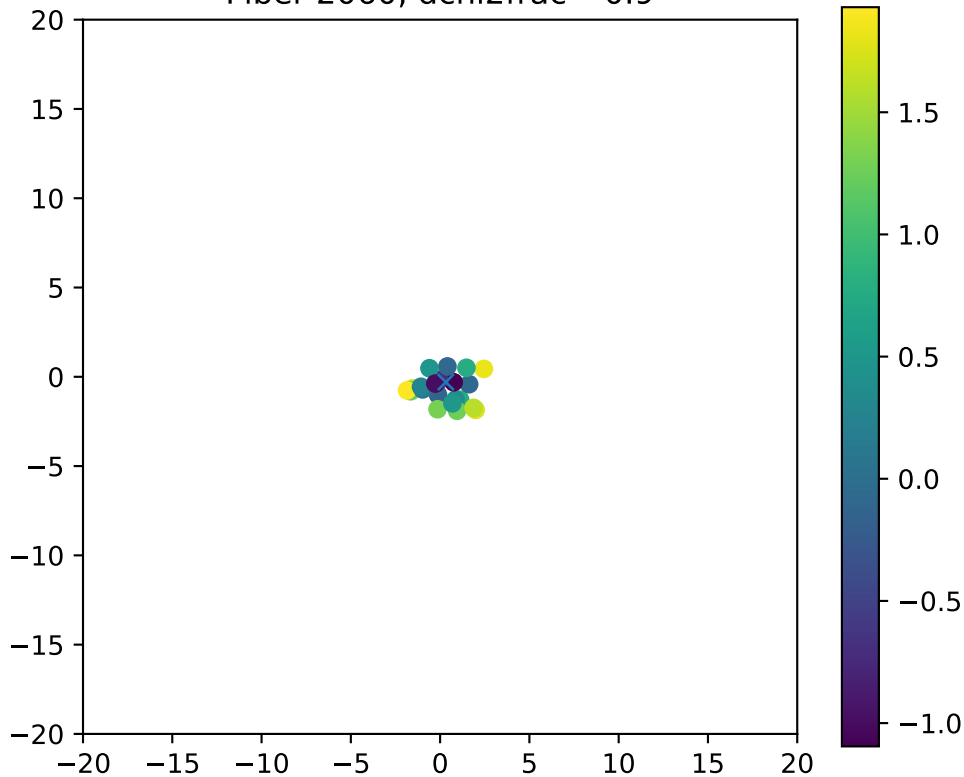
Fiber 2060, dchi2frac= 0.9
