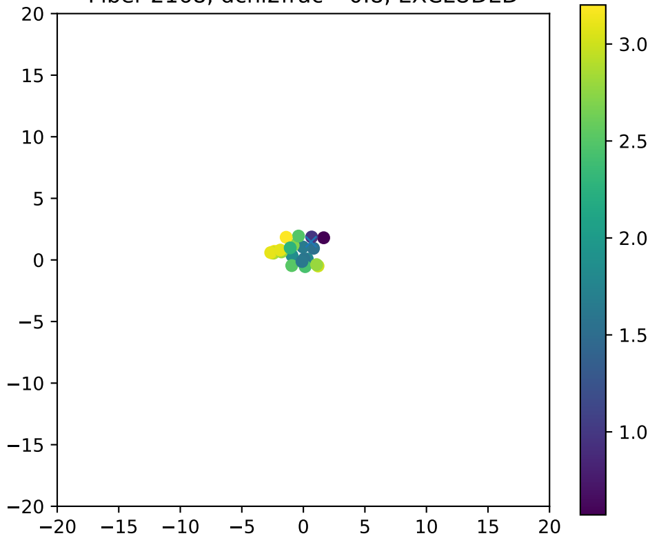
Fiber 2168, dchi2frac= 0.8, EXCLUDED
