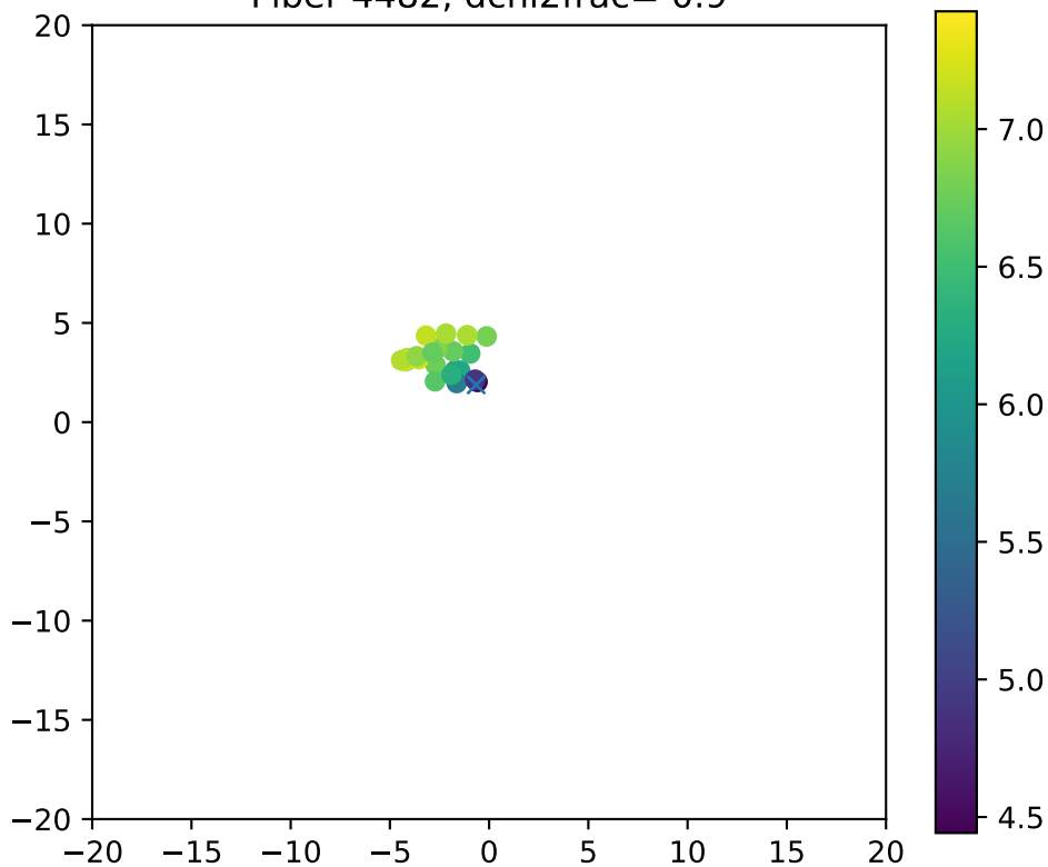
Fiber 4482, dchi2frac= 0.9
