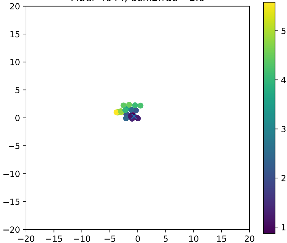
Fiber 4644, dchi2frac= 1.0
