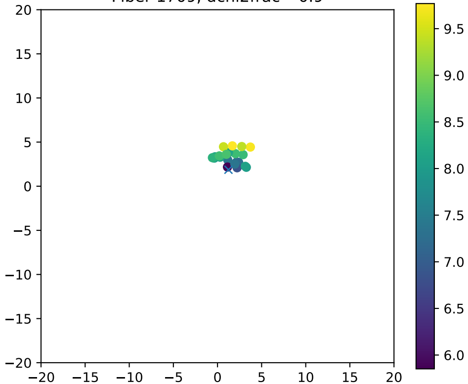
Fiber 1709, dchi2frac= 0.9
