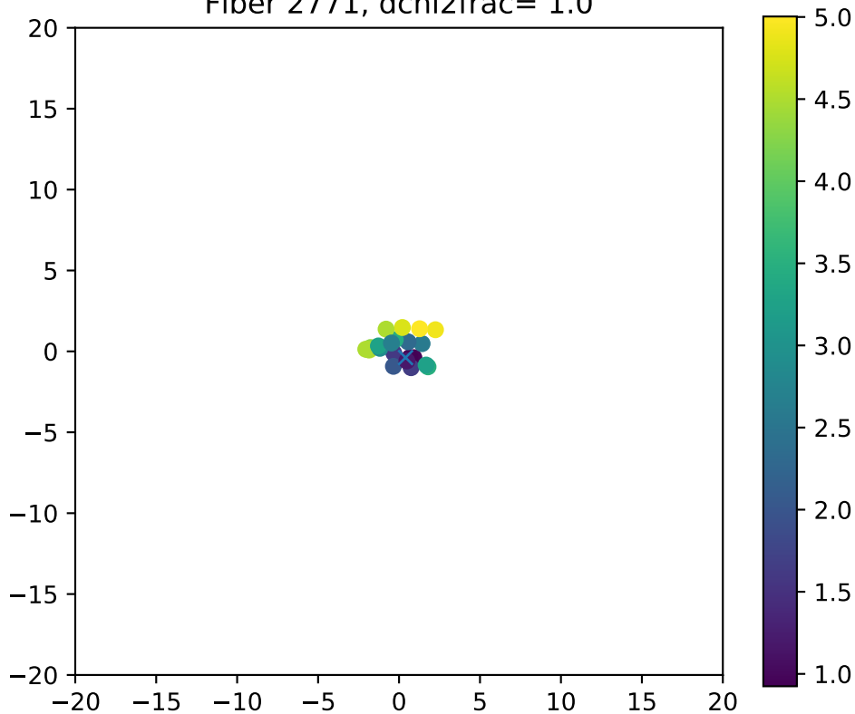
Fiber 2771, dchi2frac= 1.0
