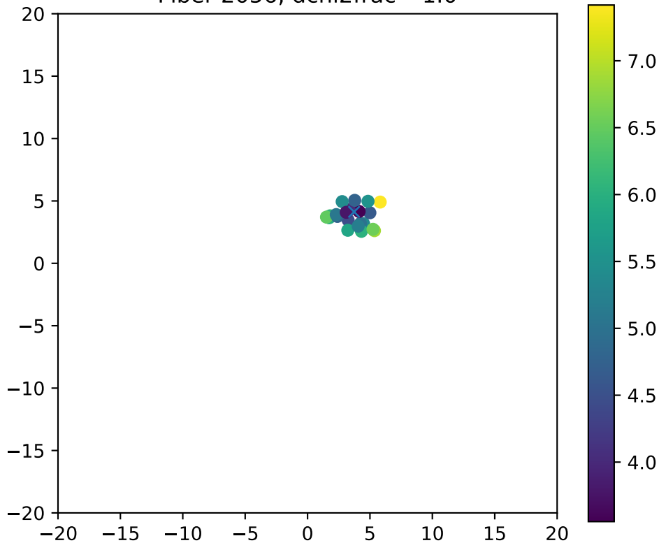
Fiber 2056, dchi2frac= 1.0
