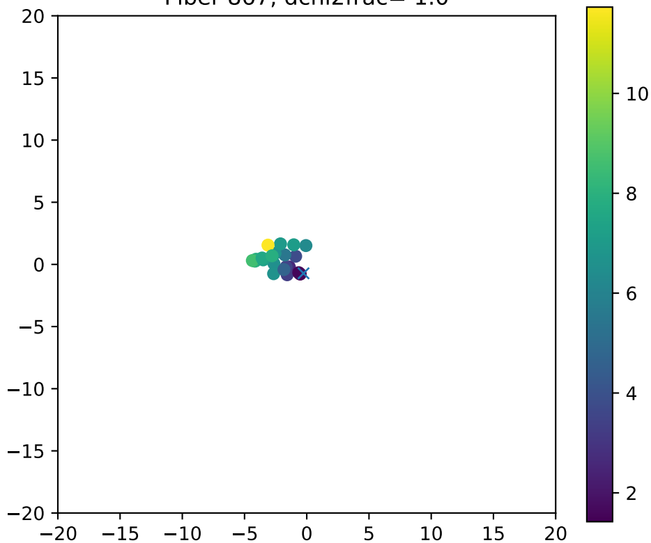
Fiber 867, dchi2frac= 1.0
