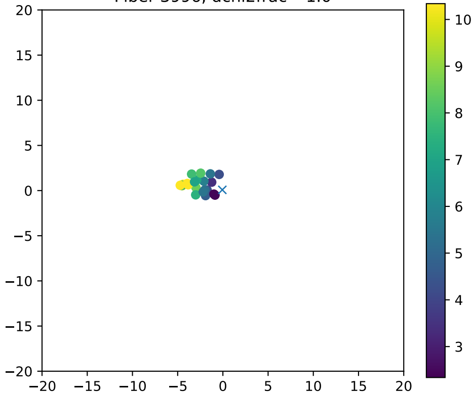
Fiber 3996, dchi2frac= 1.0
