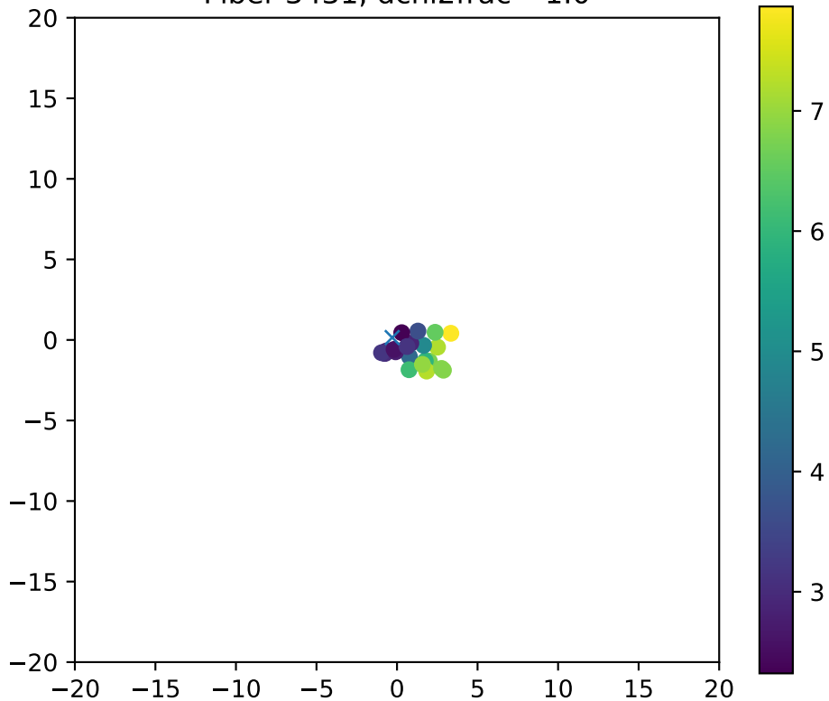
Fiber 3431, dchi2frac= 1.0
