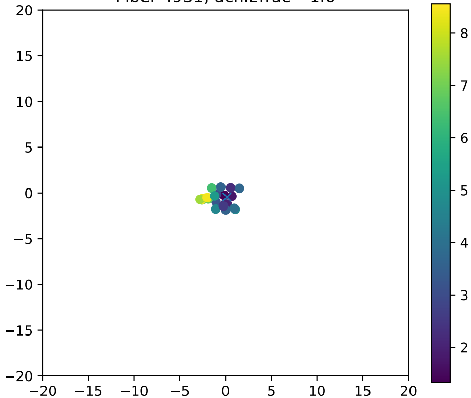
Fiber 4931, dchi2frac= 1.0
