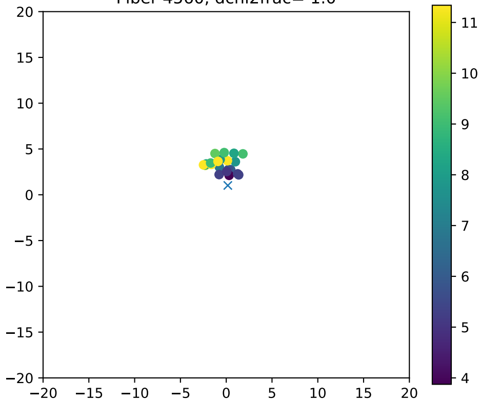
Fiber 4560, dchi2frac= 1.0
