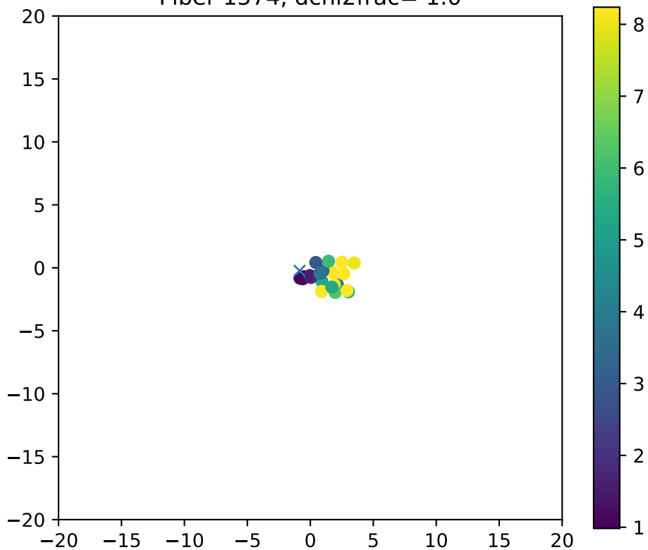
Fiber 1574, dchi2frac= 1.0
