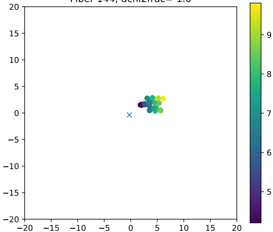
Fiber 144, dchi2frac= 1.0
