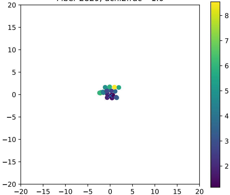
Fiber 2829, dchi2frac= 1.0
