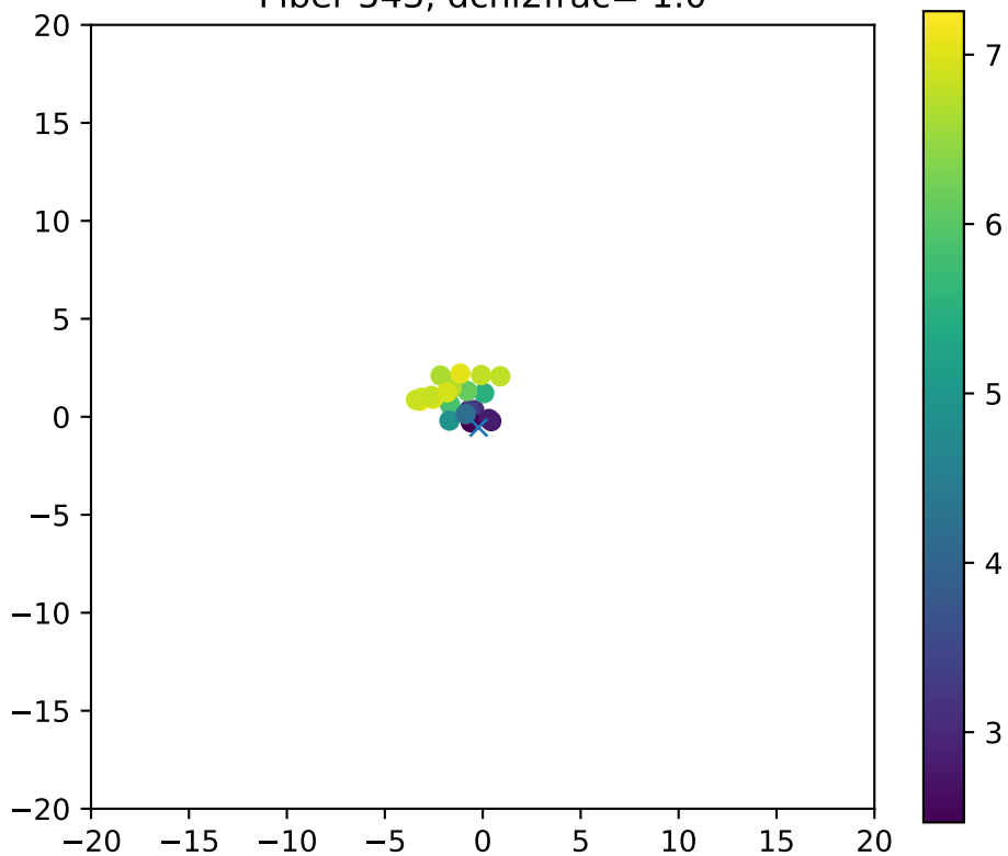
Fiber 543, dchi2frac= 1.0
