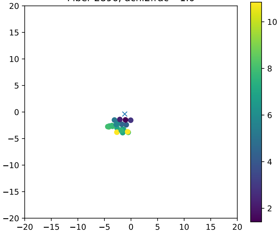
Fiber 2896, dchi2frac= 1.0
