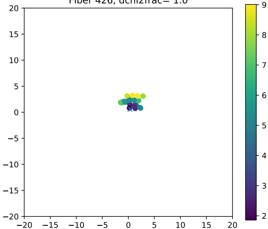
Fiber 426, dchi2frac= 1.0
