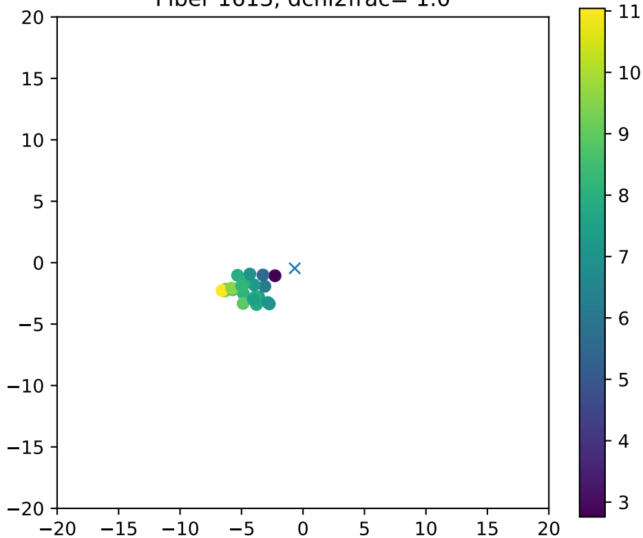
Fiber 1613, dchi2frac= 1.0
