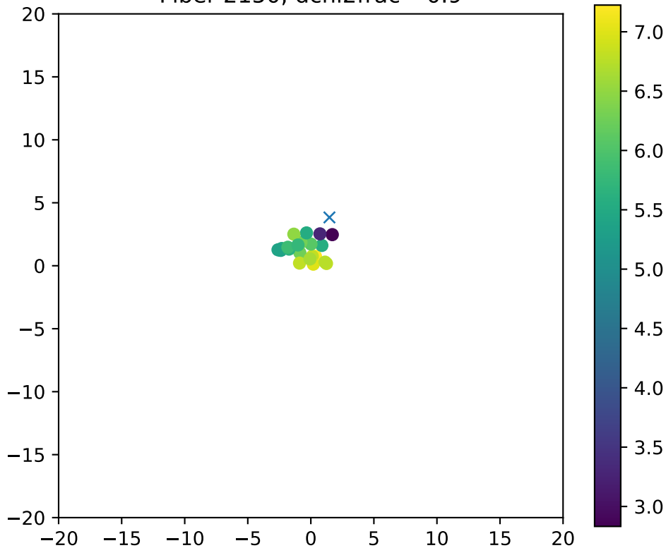
Fiber 2150, dchi2frac= 0.9
