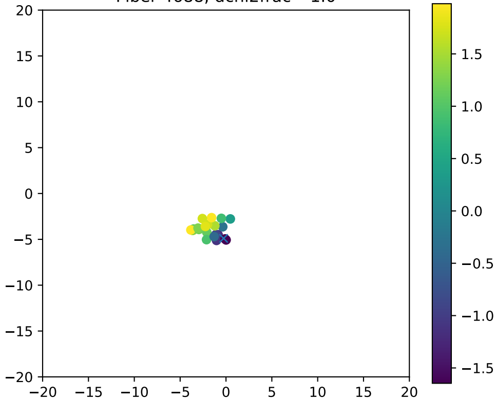
Fiber 4688, dchi2frac= 1.0
