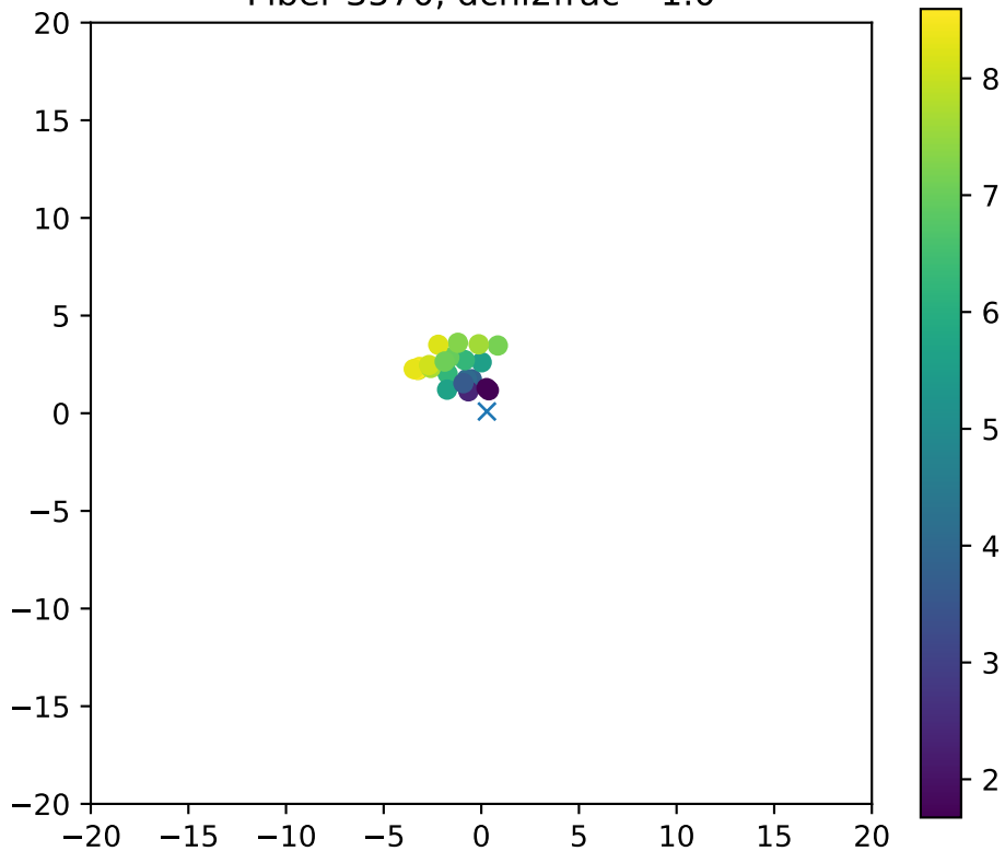
Fiber 3570, dchi2frac= 1.0
