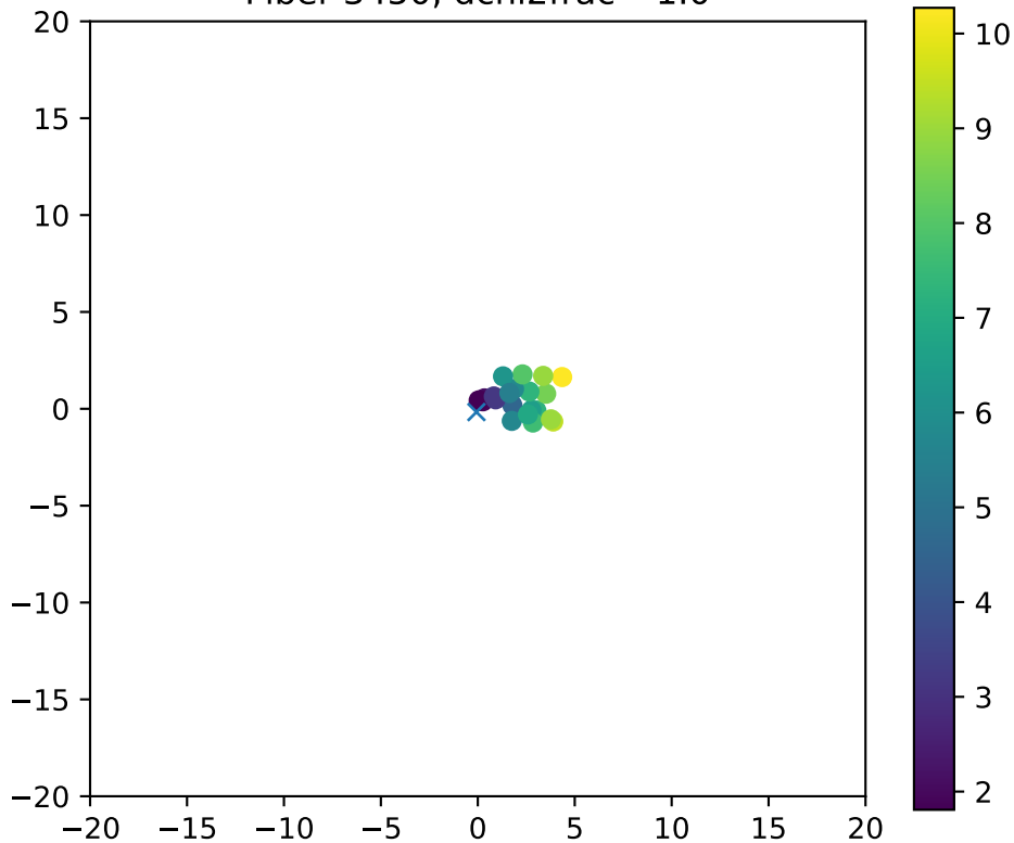
Fiber 3450, dchi2frac= 1.0
