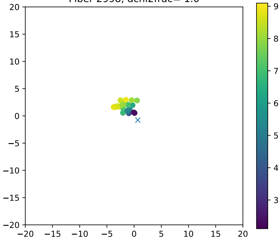
Fiber 2998, dchi2frac= 1.0
