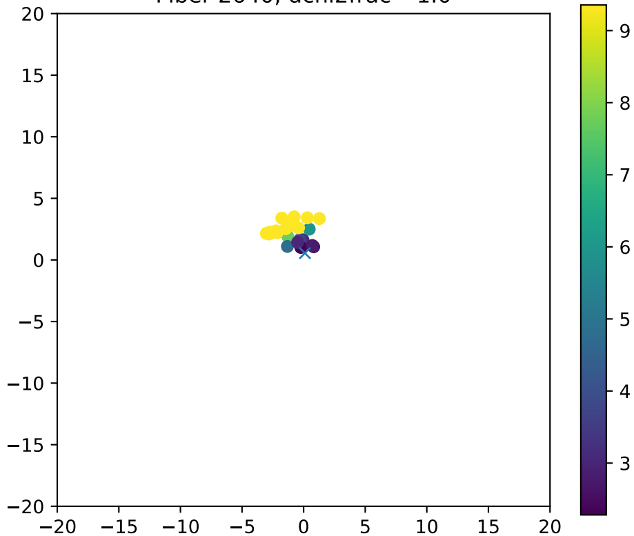
Fiber 2640, dchi2frac= 1.0
