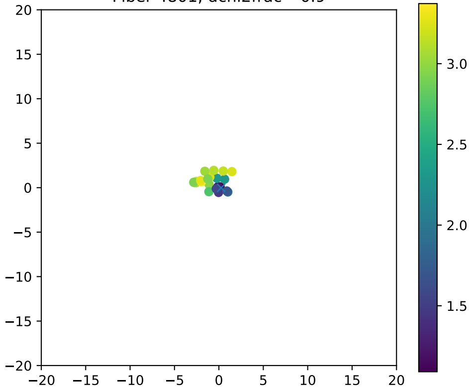
Fiber 4801, dchi2frac= 0.9
