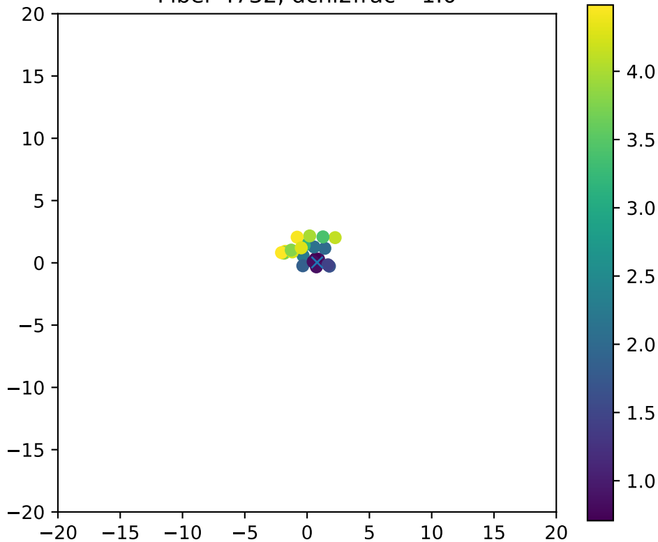
Fiber 4732, dchi2frac= 1.0
