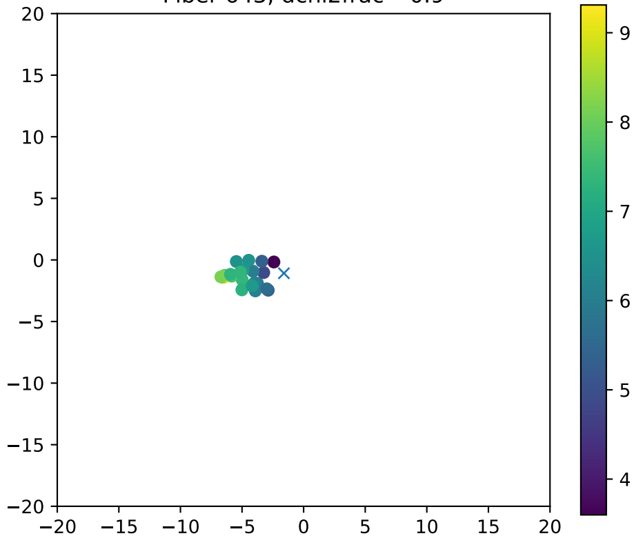
Fiber 643, dchi2frac= 0.9
