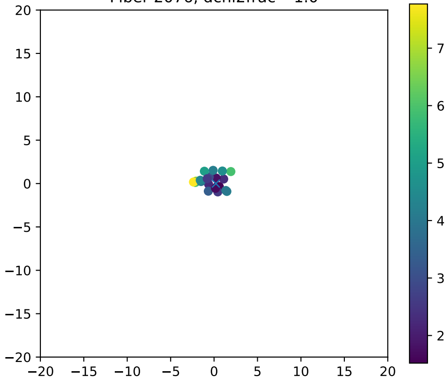
Fiber 2076, dchi2frac= 1.0
