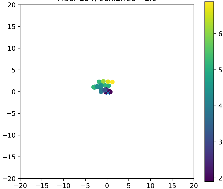
Fiber 154, dchi2frac= 1.0
