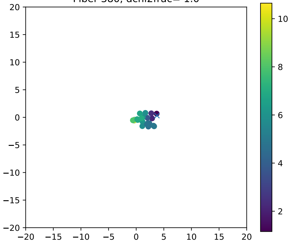
Fiber 380, dchi2frac= 1.0
