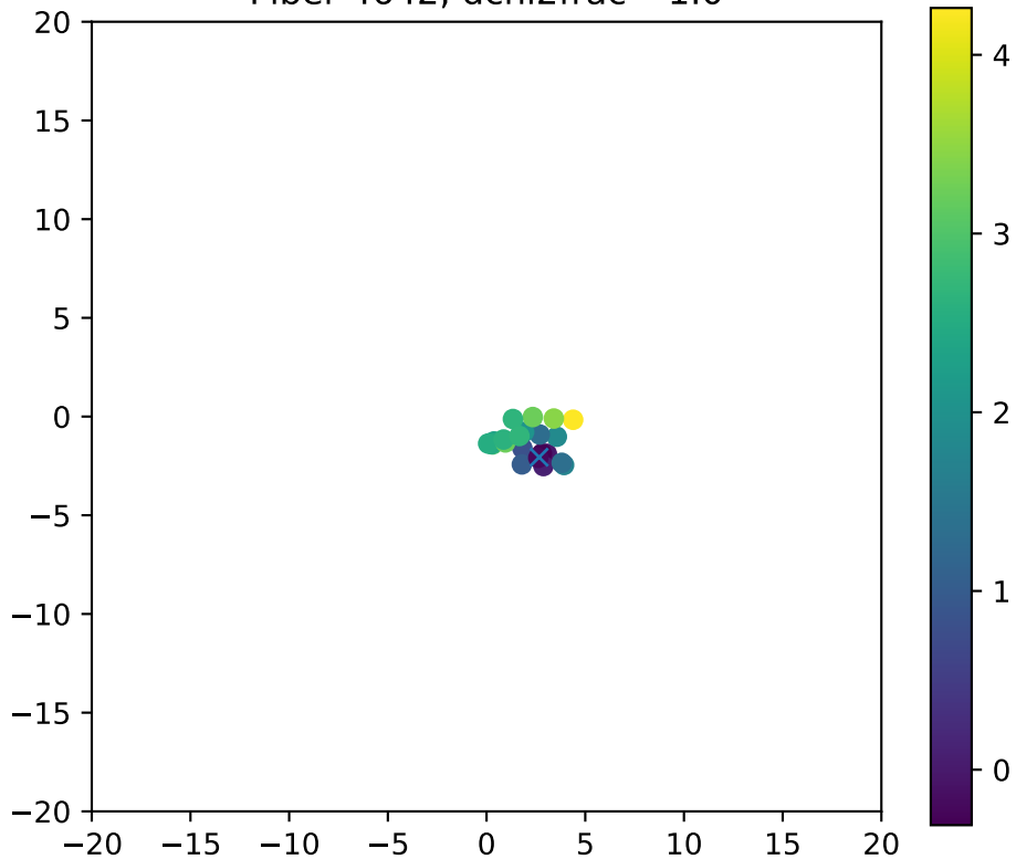
Fiber 4642, dchi2frac= 1.0
