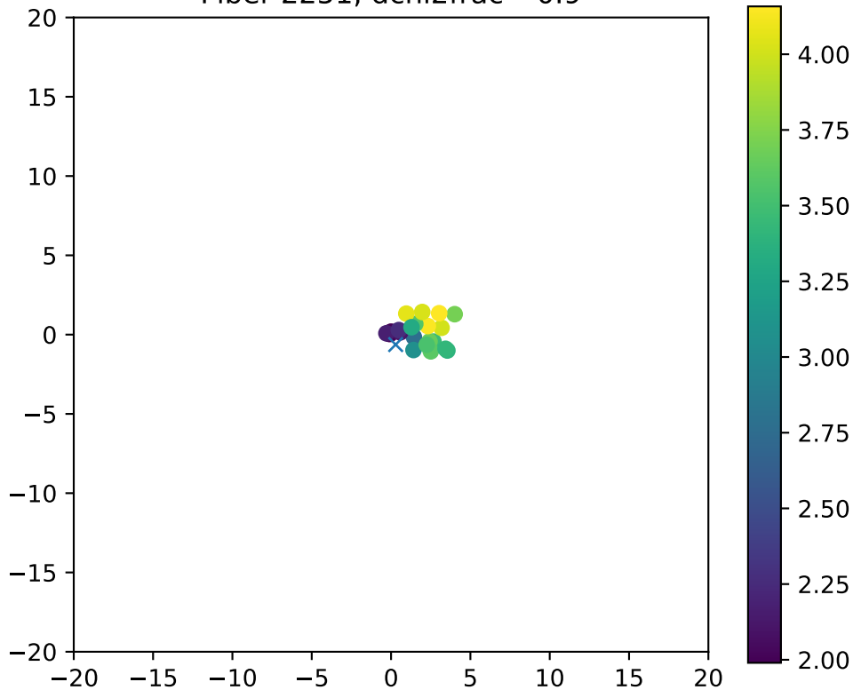
Fiber 2251, dchi2frac= 0.9
