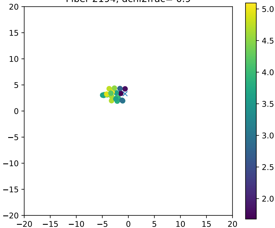
Fiber 2194, dchi2frac= 0.9
