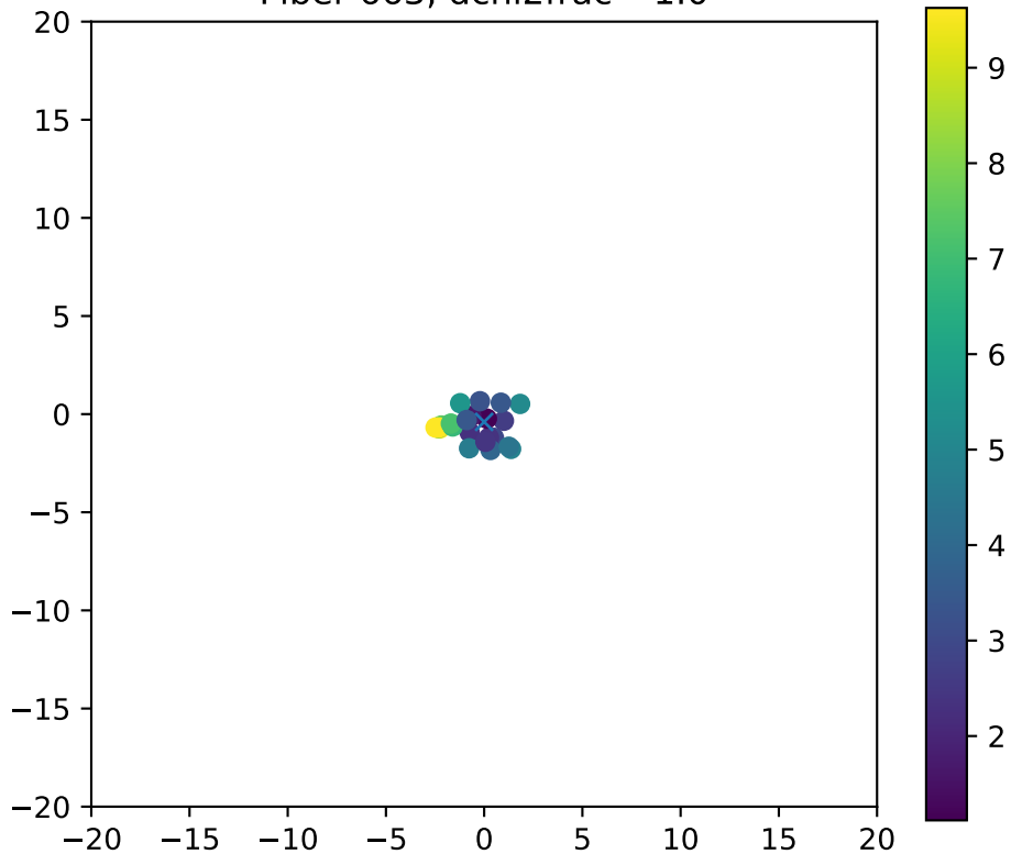
Fiber 663, dchi2frac= 1.0
