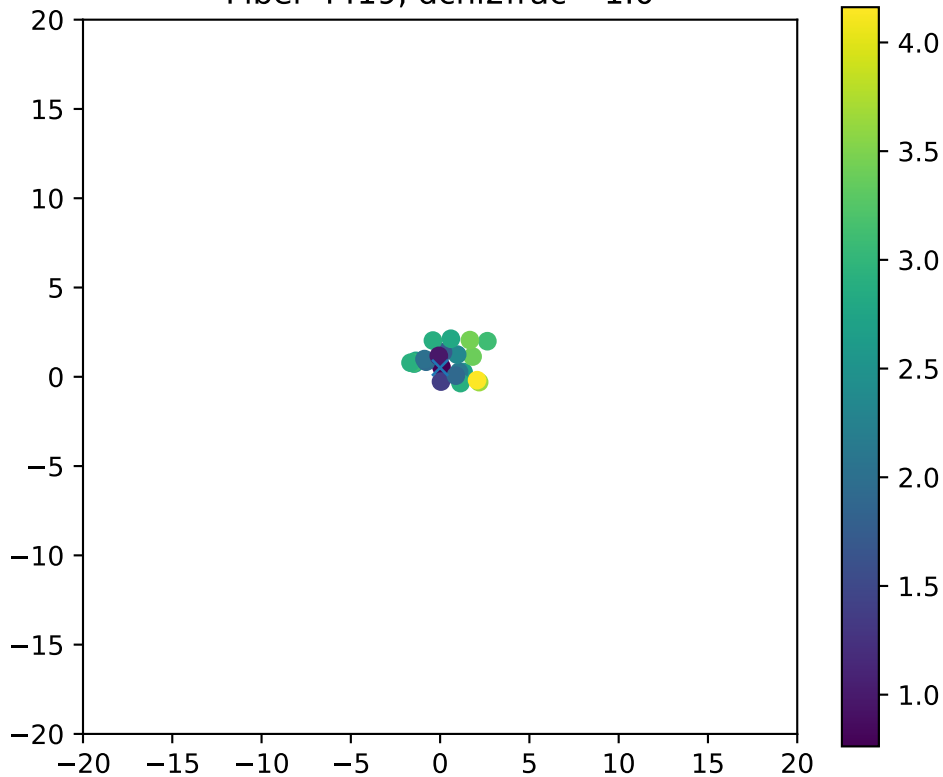
Fiber 4419, dchi2frac= 1.0
