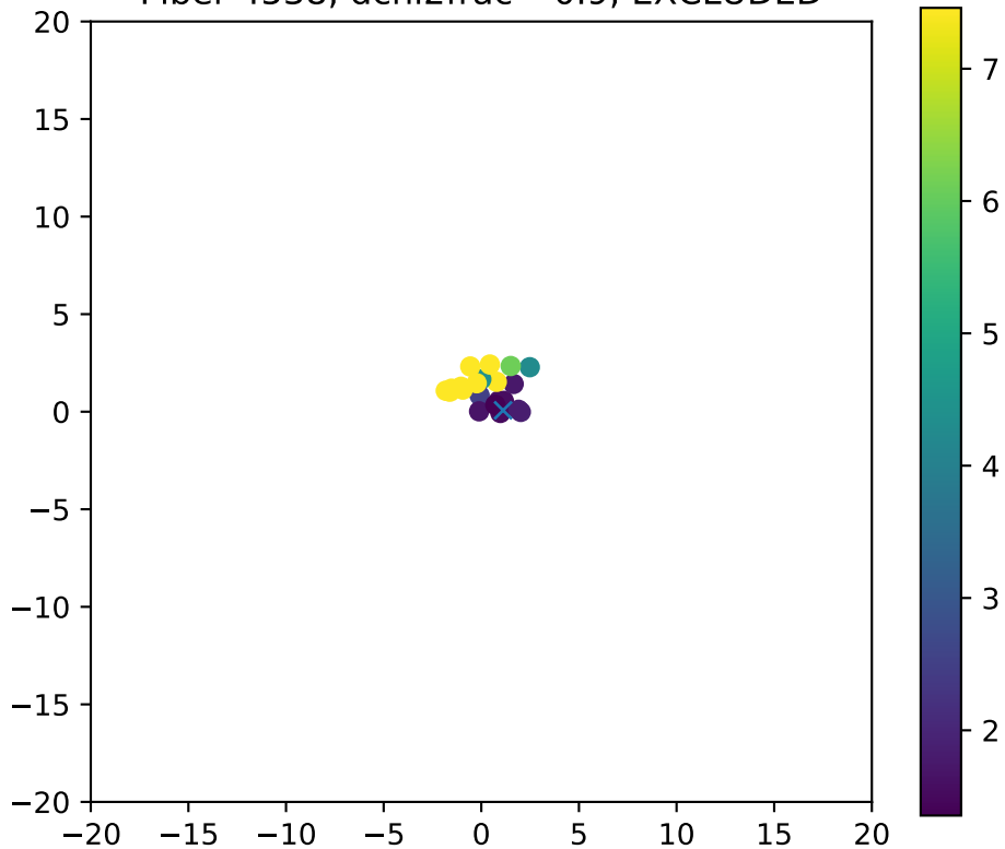
Fiber 4538, dchi2frac= 0.9, EXCLUDED
