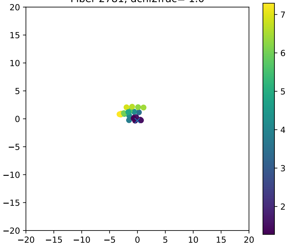
Fiber 2781, dchi2frac= 1.0
