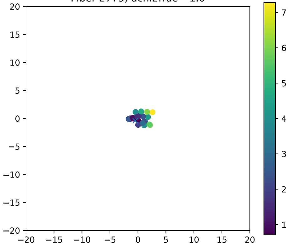
Fiber 2775, dchi2frac= 1.0
