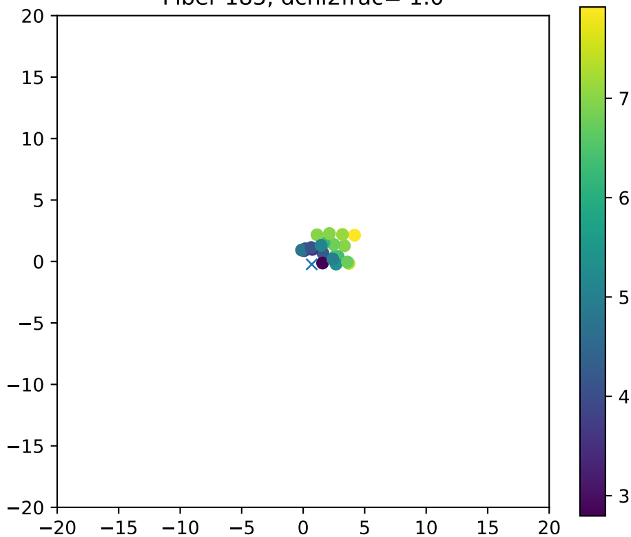
Fiber 185, dchi2frac= 1.0
