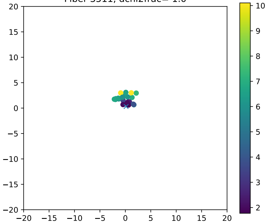
Fiber 3511, dchi2frac= 1.0
