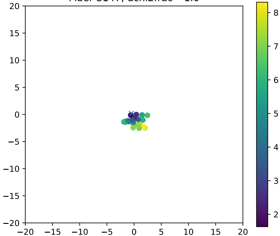
Fiber 3147, dchi2frac= 1.0
