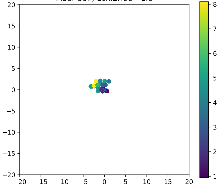
Fiber 807, dchi2frac= 1.0
