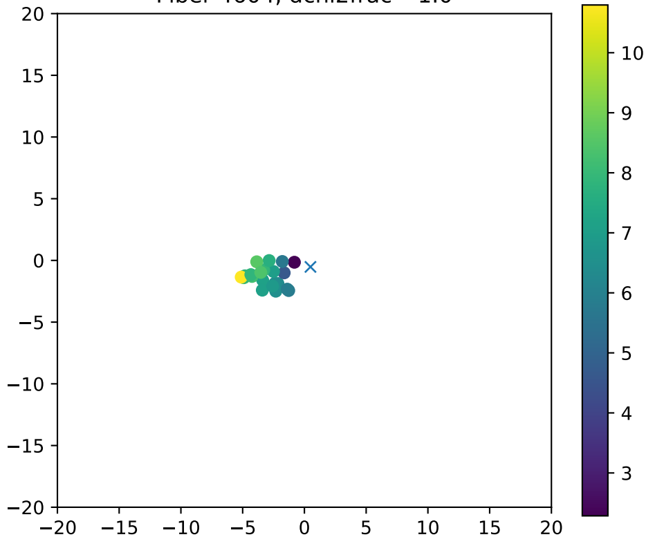
Fiber 4604, dchi2frac= 1.0
