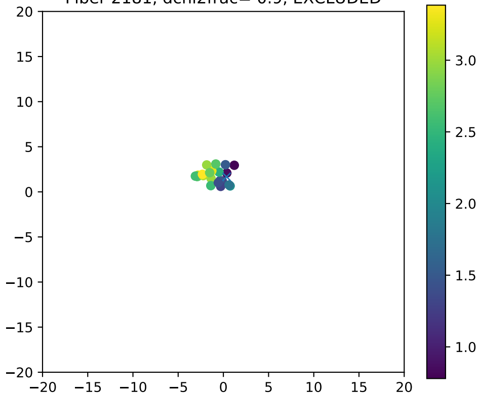
Fiber 2181, dchi2frac= 0.9, EXCLUDED
