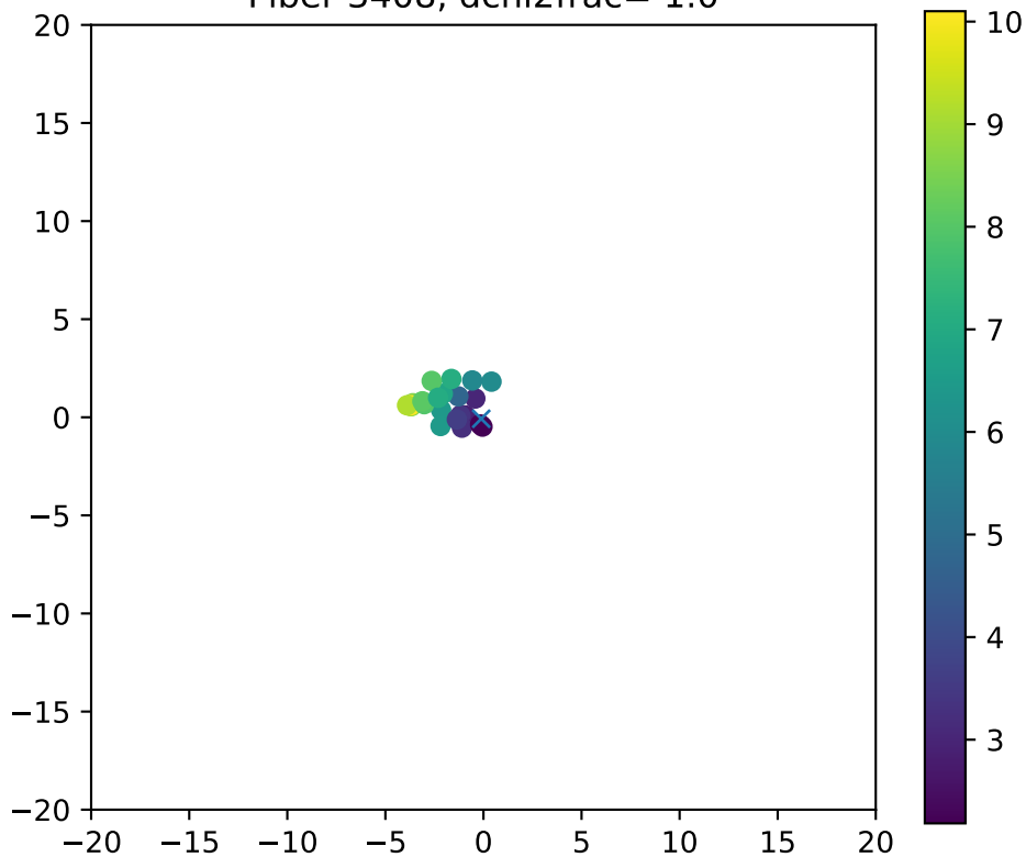
Fiber 3408, dchi2frac= 1.0
