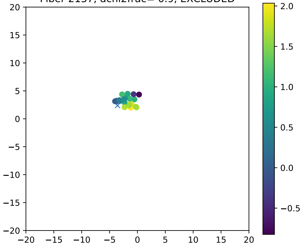
Fiber 2137, dchi2frac= 0.9, EXCLUDED
