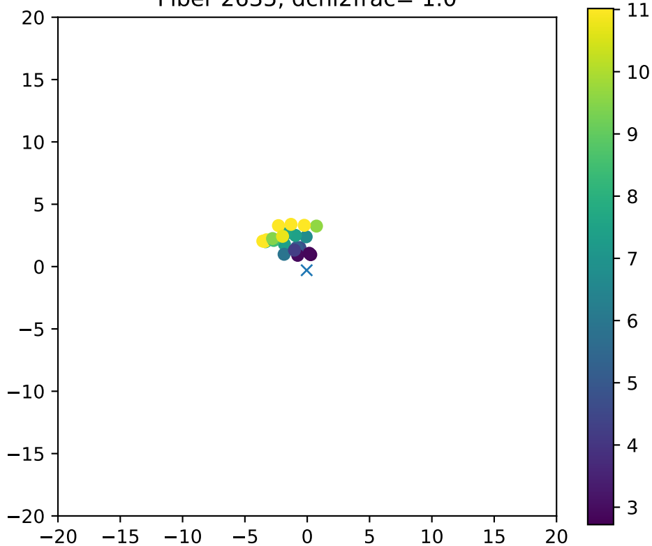
Fiber 2635, dchi2frac= 1.0
