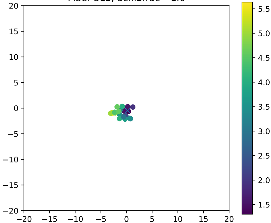
Fiber 312, dchi2frac= 1.0
