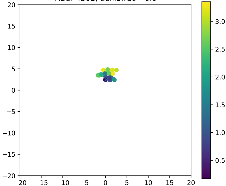
Fiber 4302, dchi2frac= 0.9
