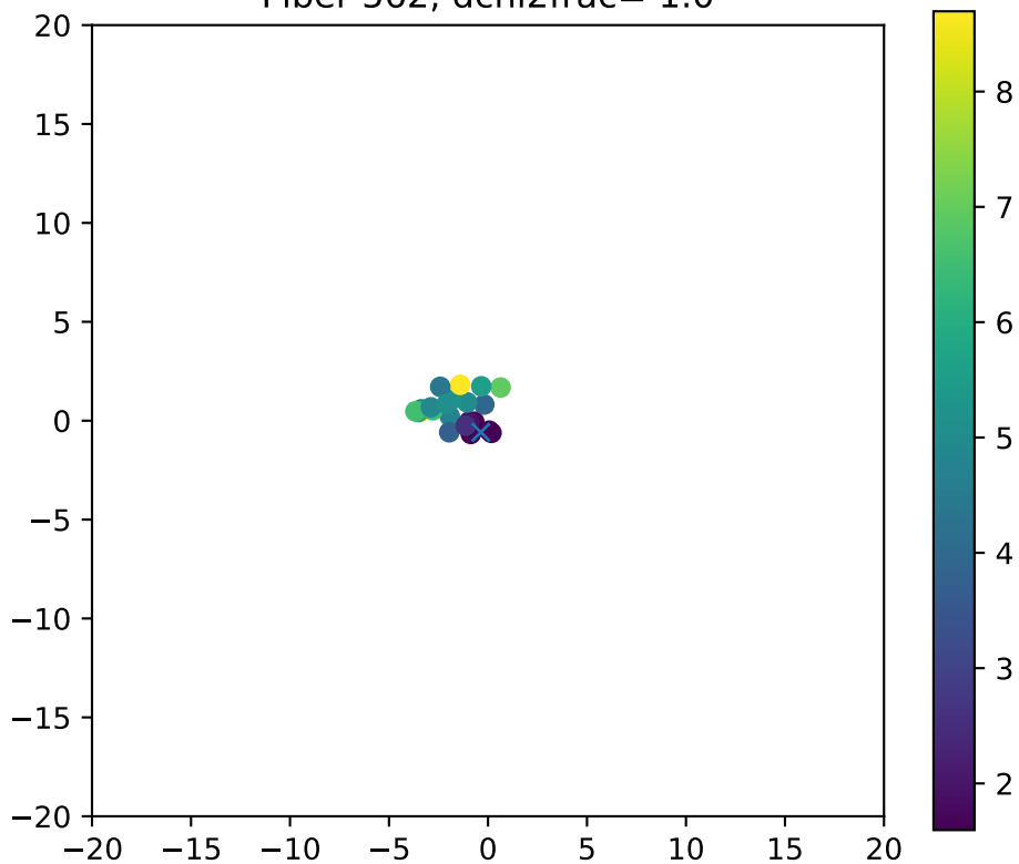
Fiber 562, dchi2frac= 1.0
