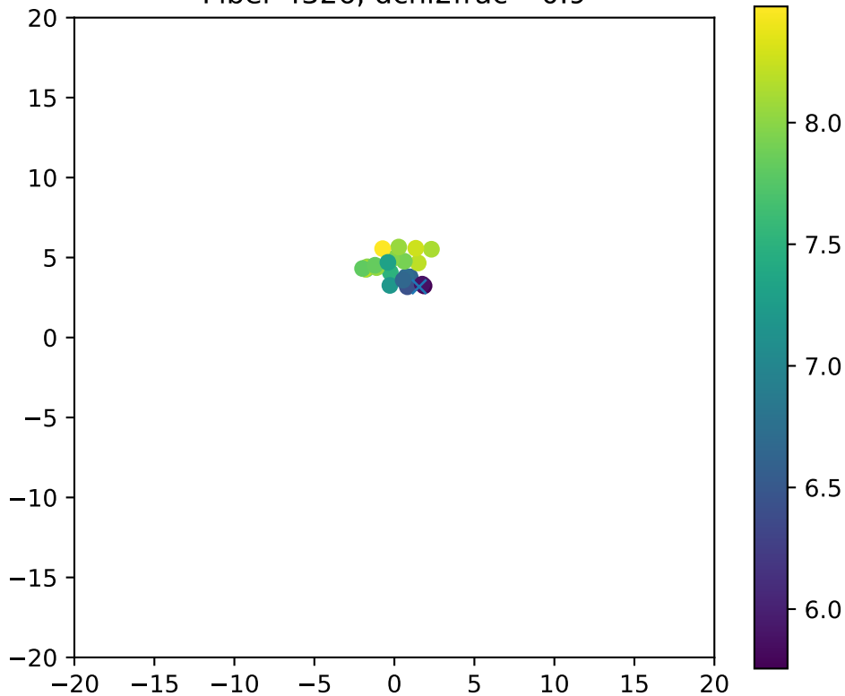
Fiber 4326, dchi2frac= 0.9
