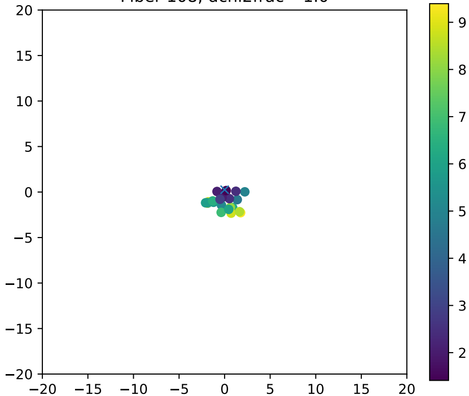
Fiber 108, dchi2frac= 1.0
