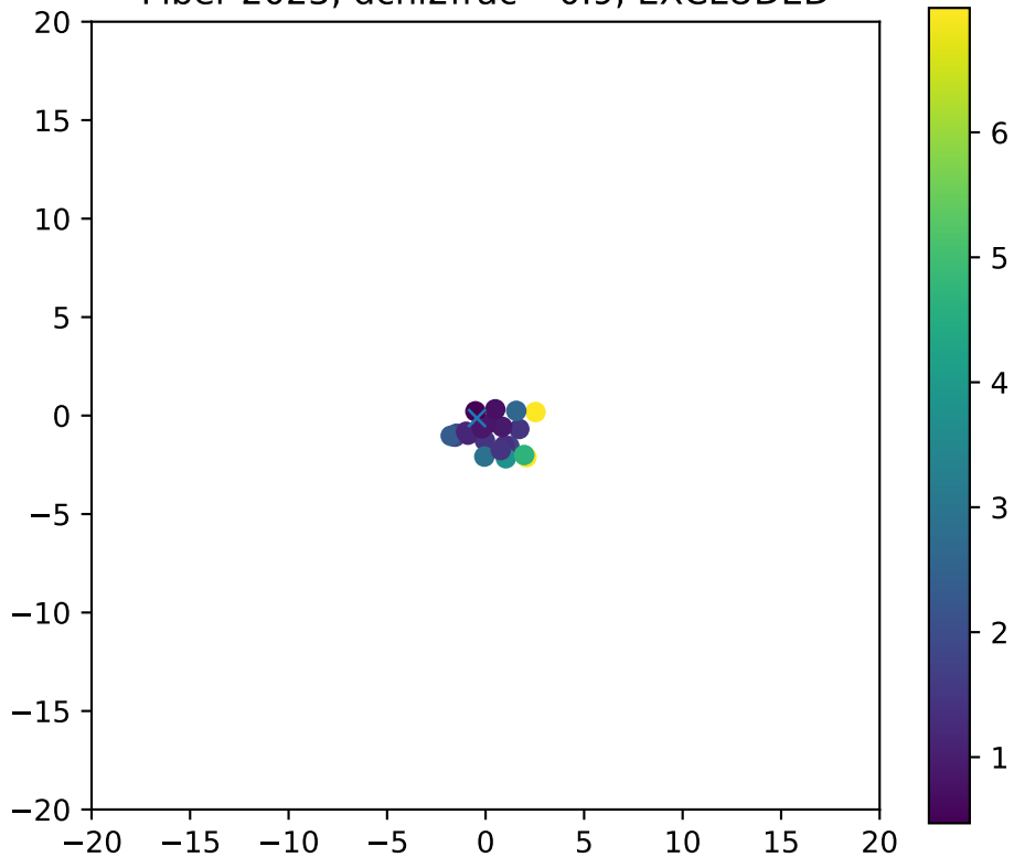
Fiber 2023, dchi2frac= 0.9, EXCLUDED
