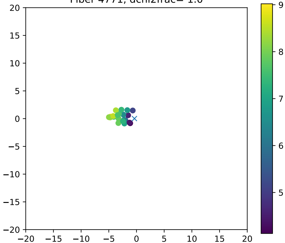
Fiber 4771, dchi2frac= 1.0
