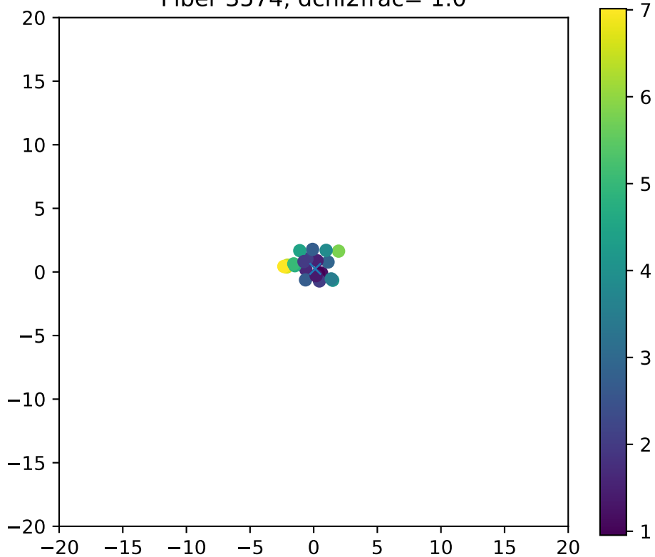
Fiber 3574, dchi2frac= 1.0
