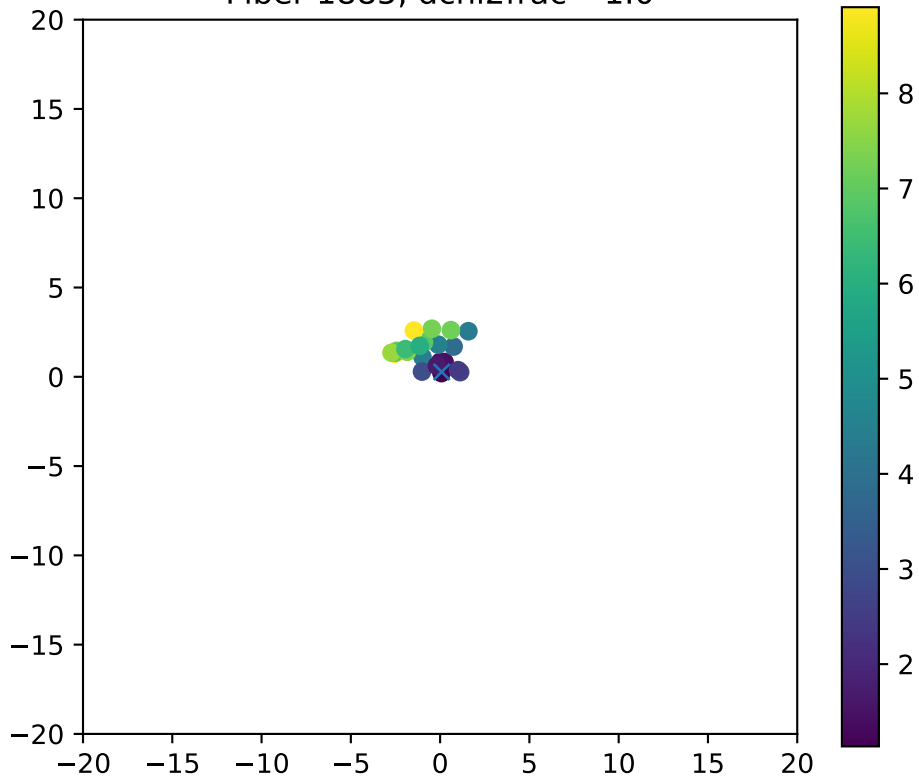
Fiber 1885, dchi2frac= 1.0
