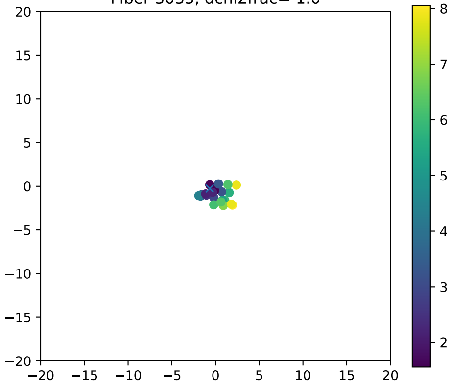
Fiber 3035, dchi2frac= 1.0
