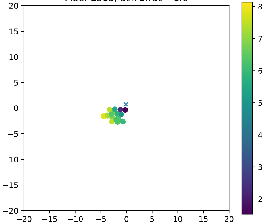
Fiber 2313, dchi2frac= 1.0
