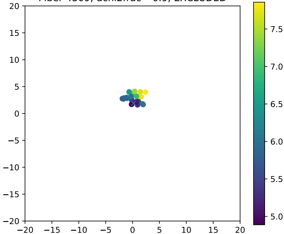
Fiber 4309, dchi2frac= 0.9, EXCLUDED
