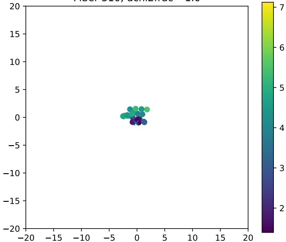
Fiber 510, dchi2frac= 1.0
