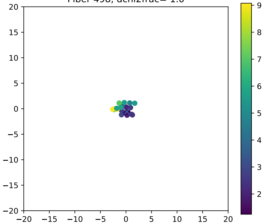
Fiber 498, dchi2frac= 1.0
