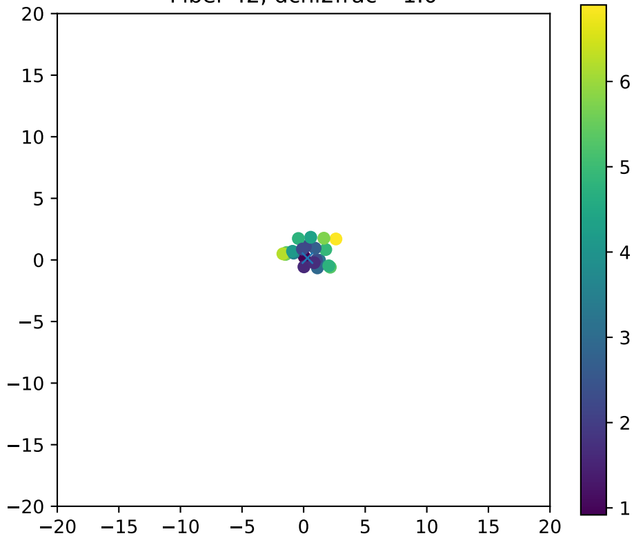
Fiber 42, dchi2frac= 1.0
