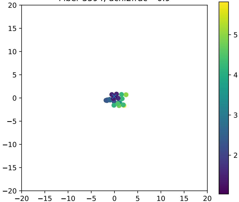
Fiber 3594, dchi2frac= 0.9
