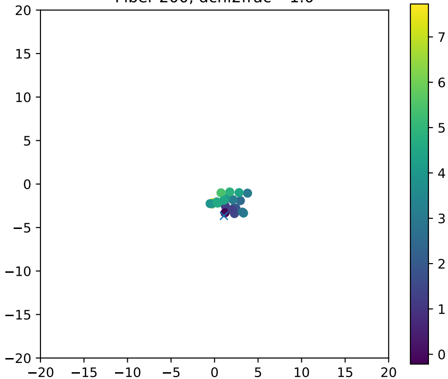
Fiber 200, dchi2frac= 1.0
