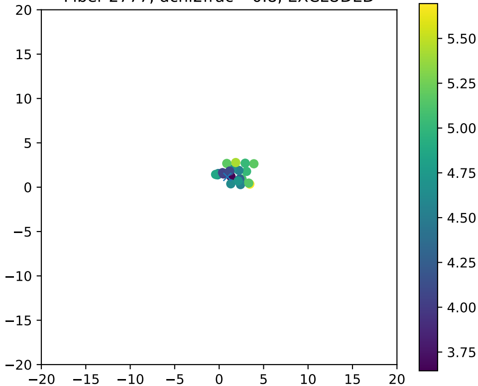
Fiber 2777, dchi2frac= 0.8, EXCLUDED
