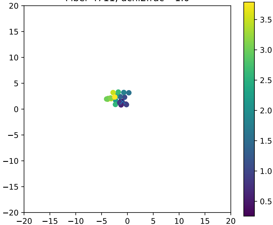
Fiber 4711, dchi2frac= 1.0
