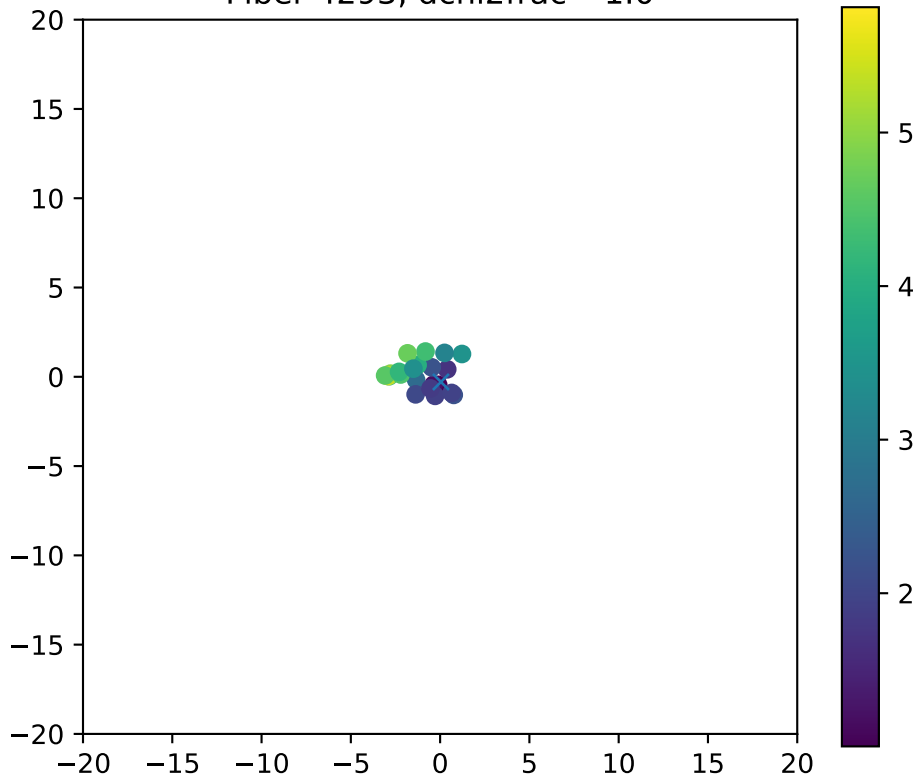
Fiber 4293, dchi2frac= 1.0
