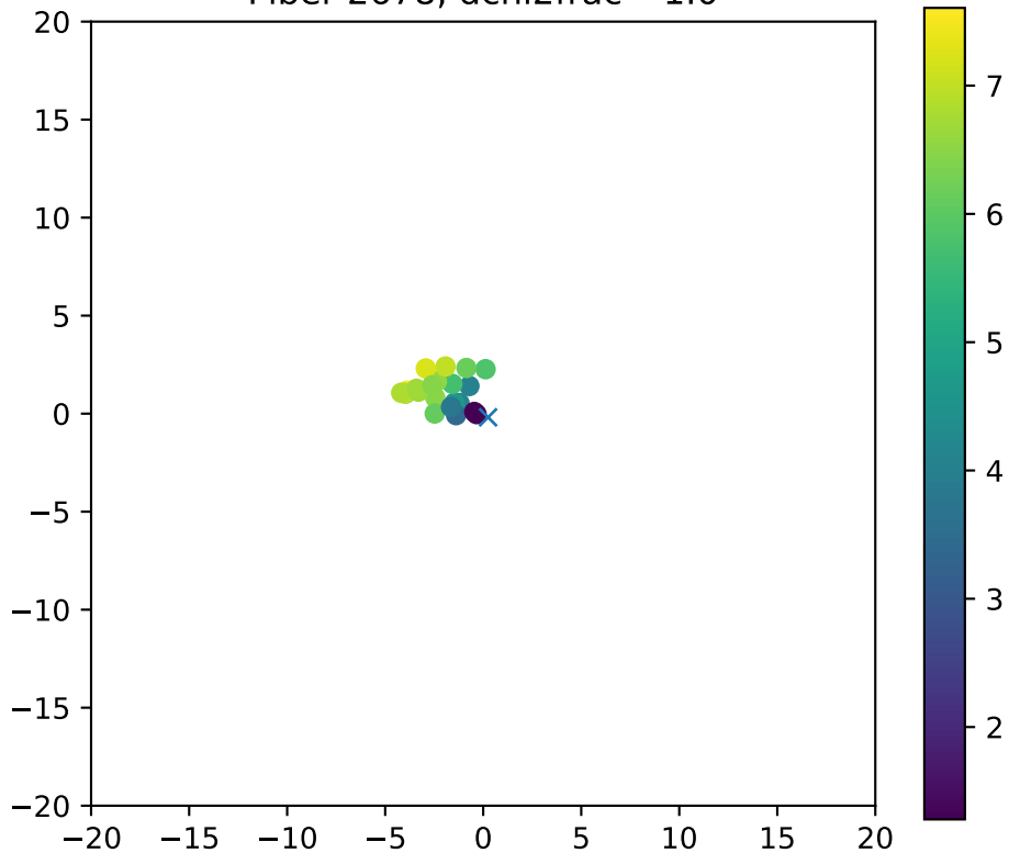
Fiber 2678, dchi2frac= 1.0
