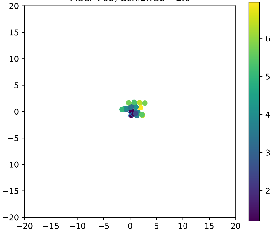
Fiber 768, dchi2frac= 1.0
