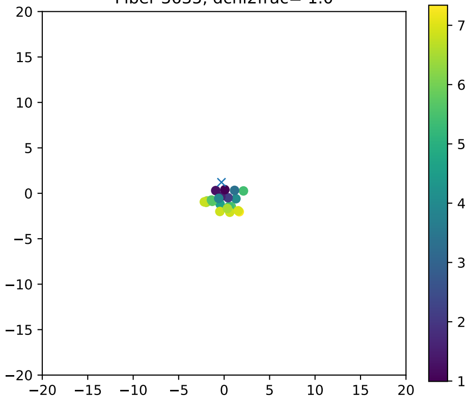
Fiber 3635, dchi2frac= 1.0
