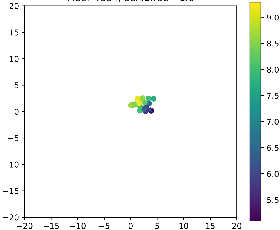
Fiber 4684, dchi2frac= 1.0
