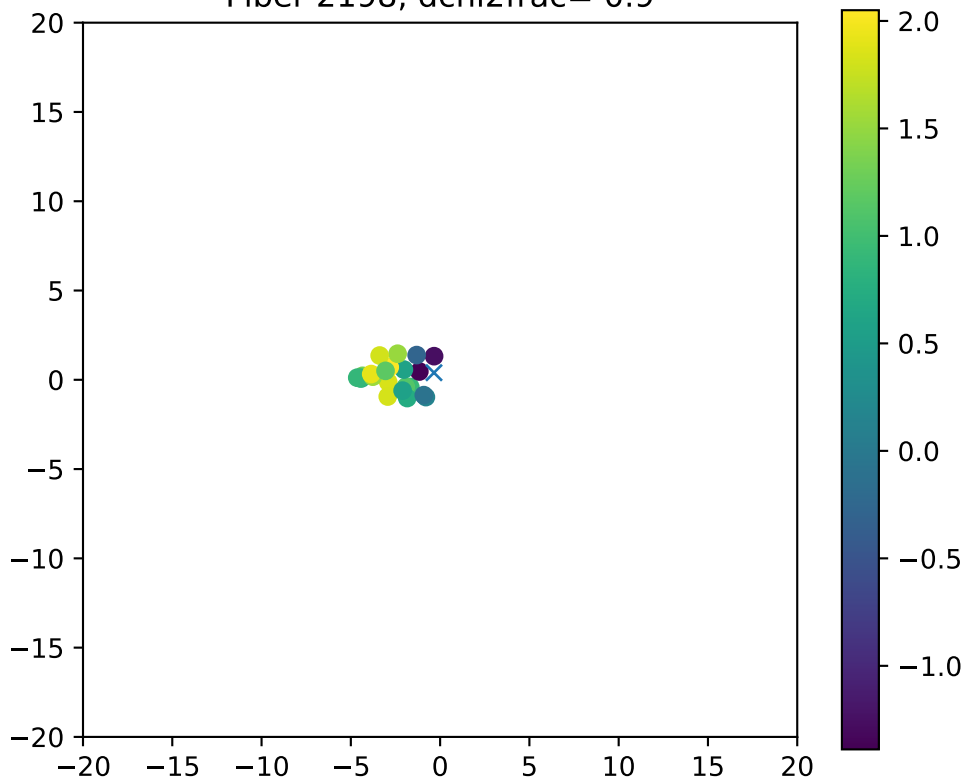
Fiber 2198, dchi2frac= 0.9
