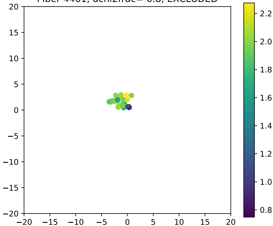
Fiber 4461, dchi2frac= 0.8, EXCLUDED
