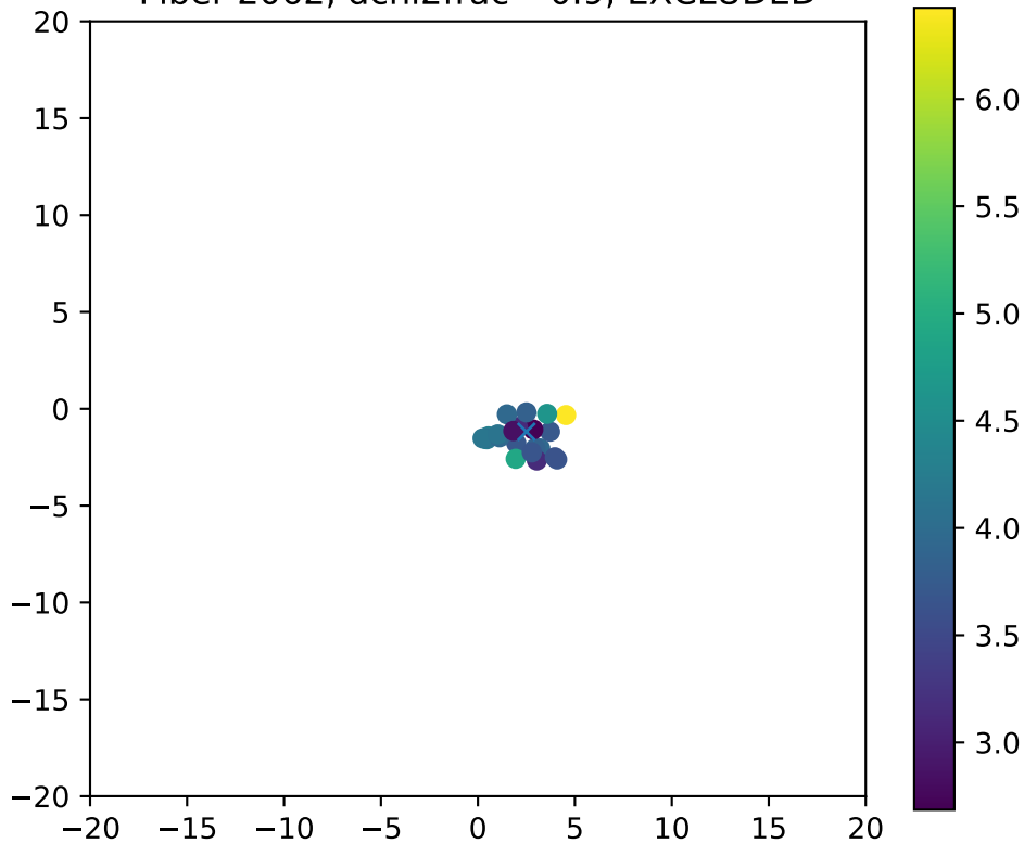
Fiber 2062, dchi2frac= 0.9, EXCLUDED
