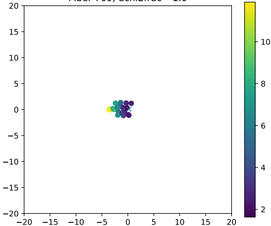
Fiber 709, dchi2frac= 1.0
