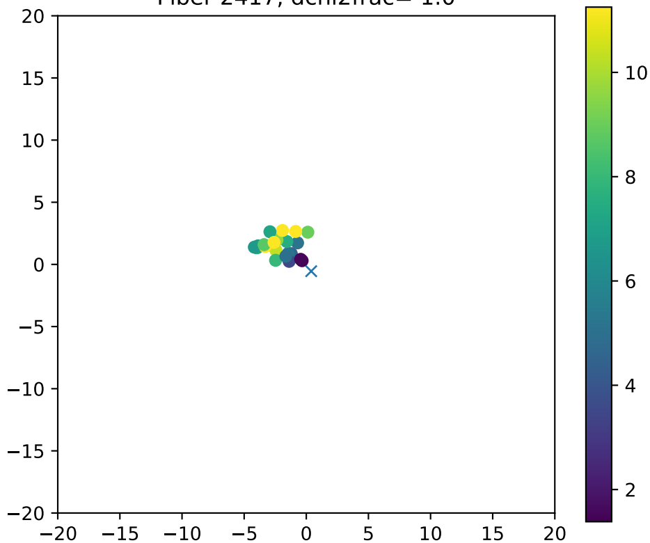
Fiber 2417, dchi2frac= 1.0
