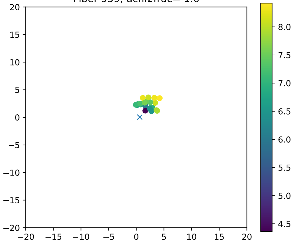
Fiber 959, dchi2frac= 1.0
