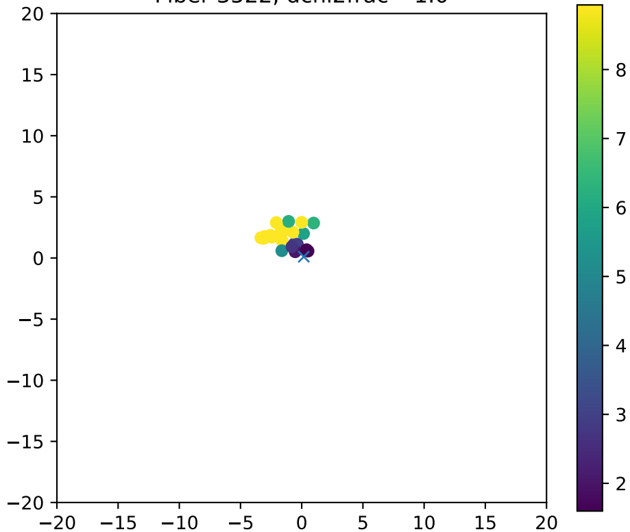
Fiber 3522, dchi2frac= 1.0
