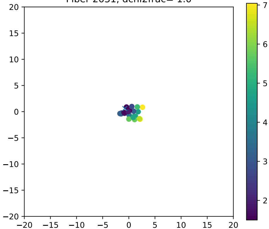
Fiber 2031, dchi2frac= 1.0
