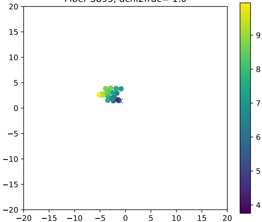
Fiber 3895, dchi2frac= 1.0
