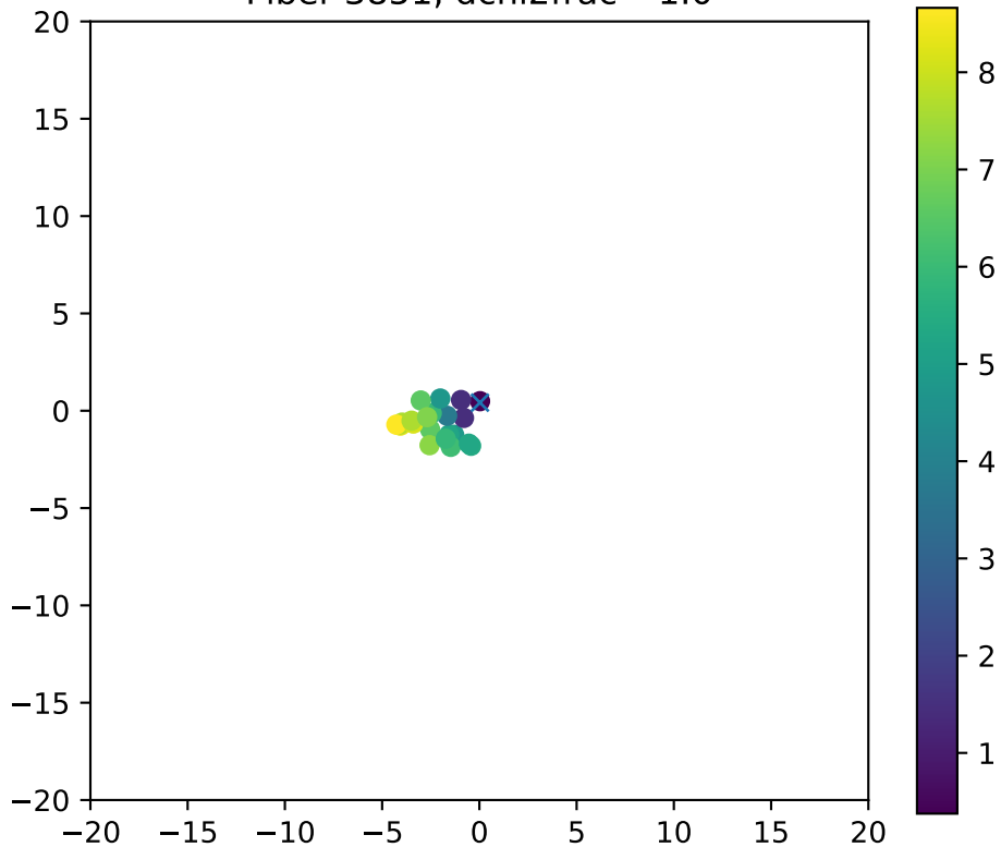
Fiber 3851, dchi2frac= 1.0
