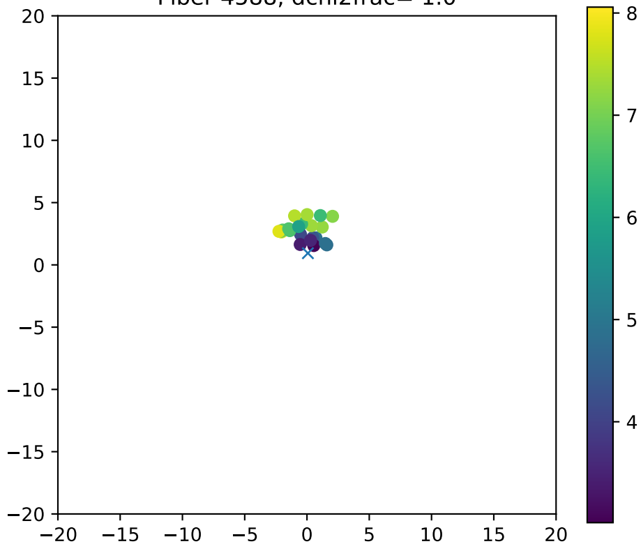
Fiber 4588, dchi2frac= 1.0
