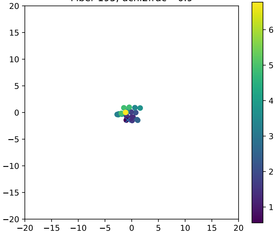
Fiber 195, dchi2frac= 0.9
