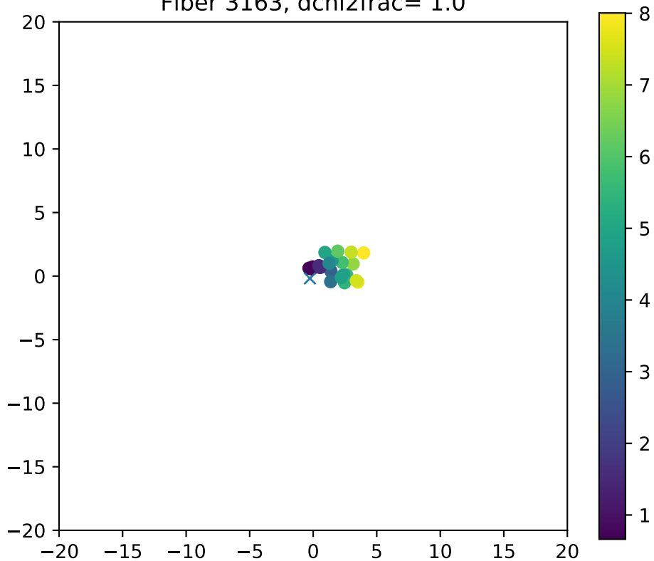
Fiber 3163, dchi2frac= 1.0
