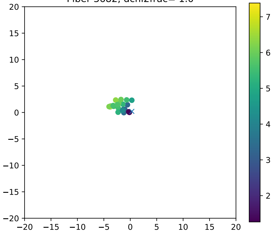
Fiber 3682, dchi2frac= 1.0
