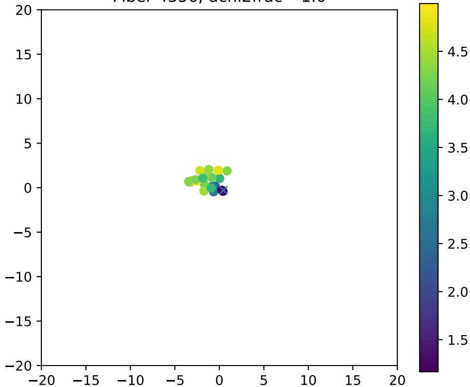
Fiber 4356, dchi2frac= 1.0
