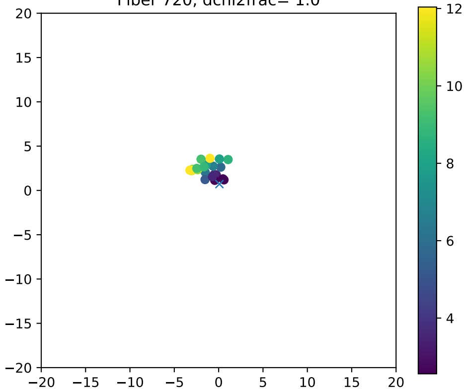
Fiber 720, dchi2frac= 1.0
