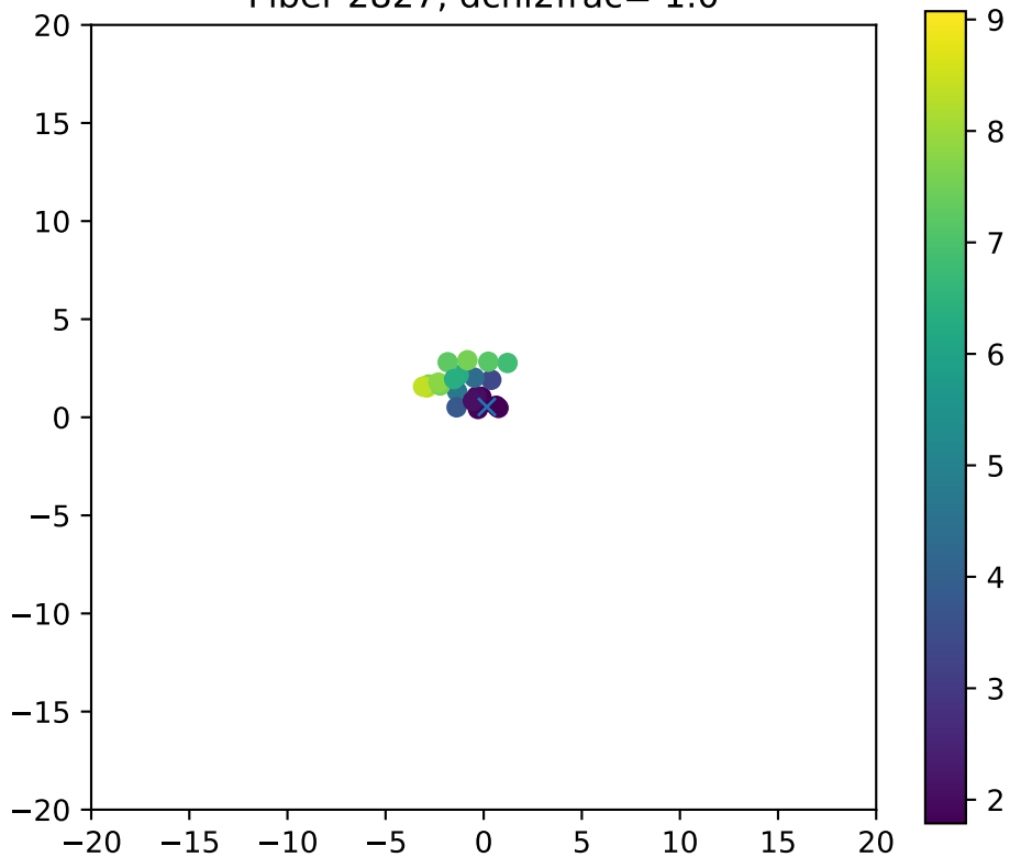
Fiber 2827, dchi2frac= 1.0
