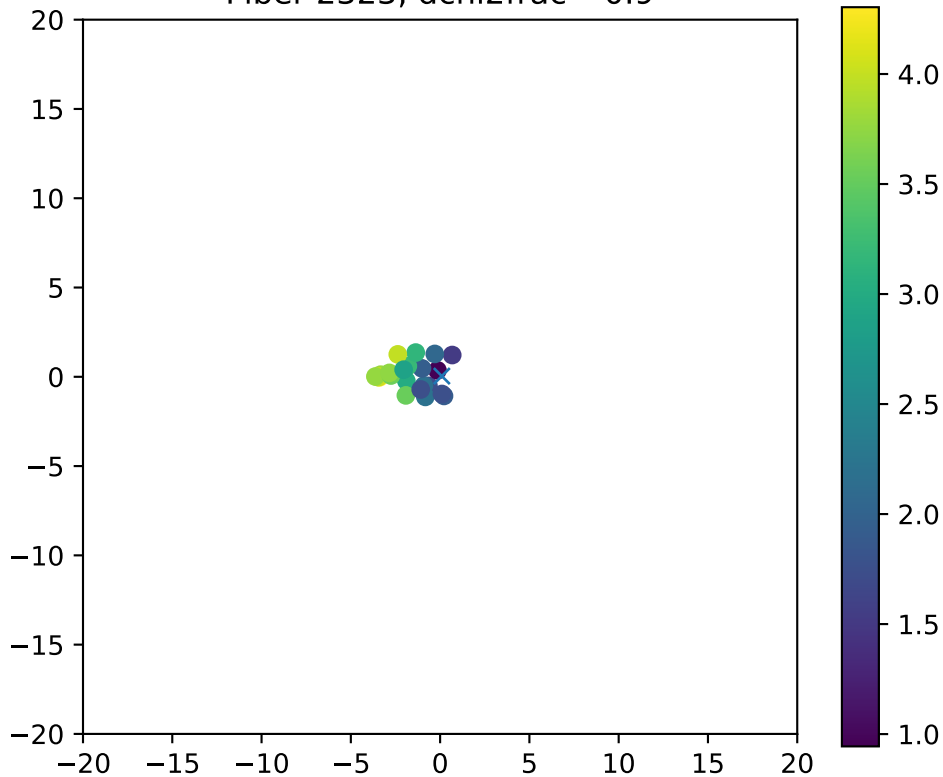
Fiber 2323, dchi2frac= 0.9
