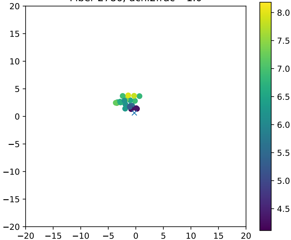
Fiber 2786, dchi2frac= 1.0
