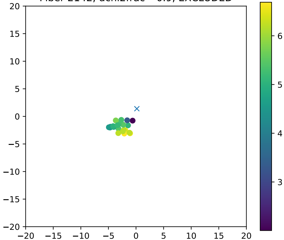
Fiber 2142, dchi2frac= 0.9, EXCLUDED
