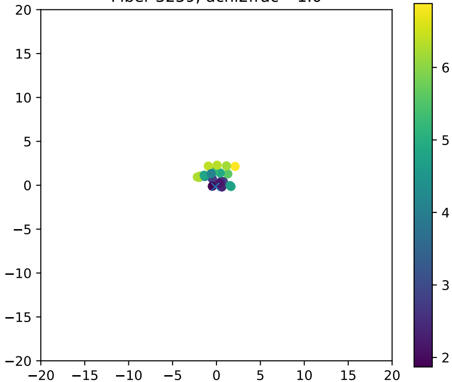
Fiber 3259, dchi2frac= 1.0
