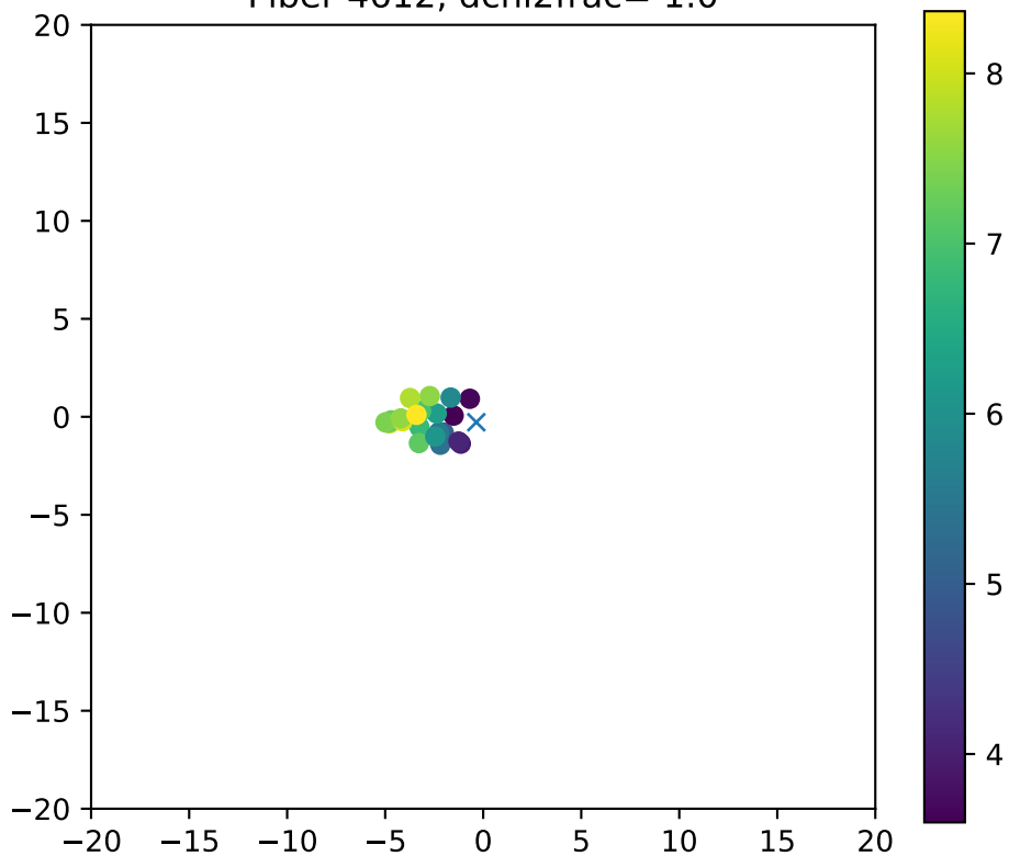
Fiber 4612, dchi2frac= 1.0
