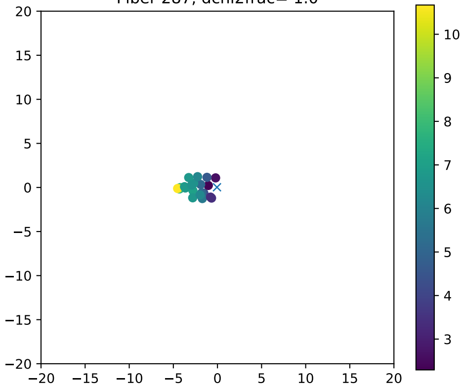
Fiber 287, dchi2frac= 1.0
