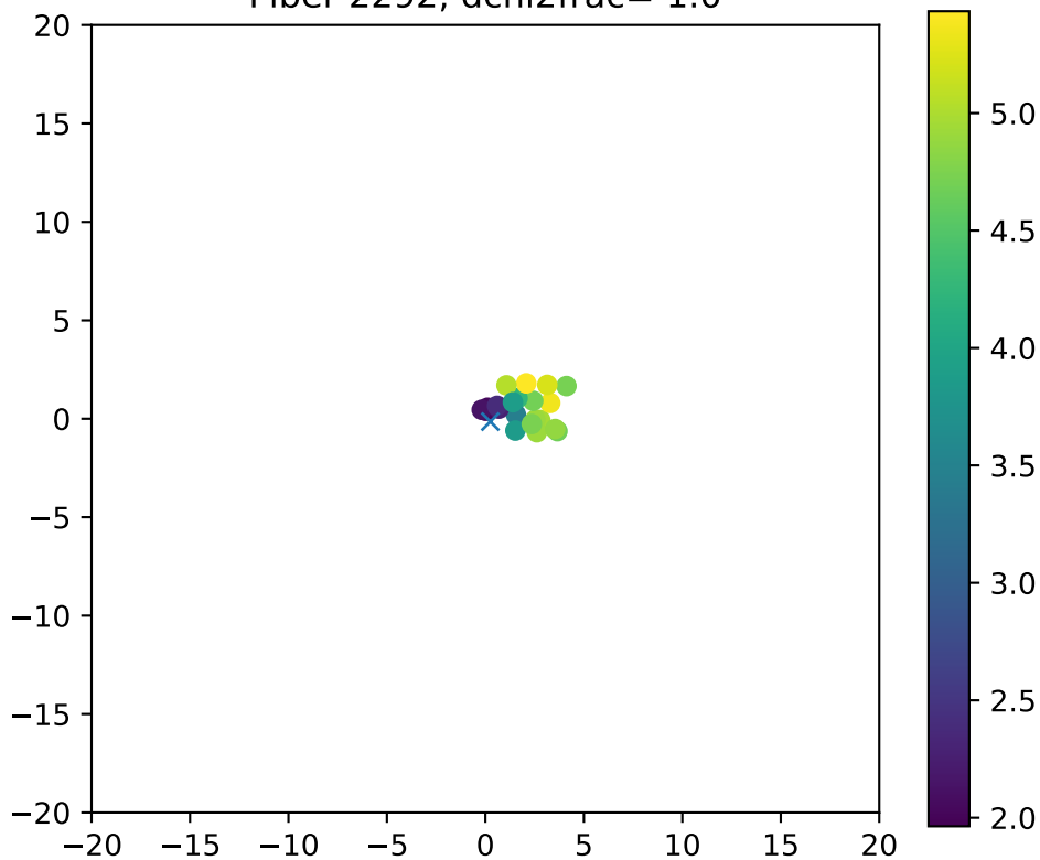
Fiber 2292, dchi2frac= 1.0
