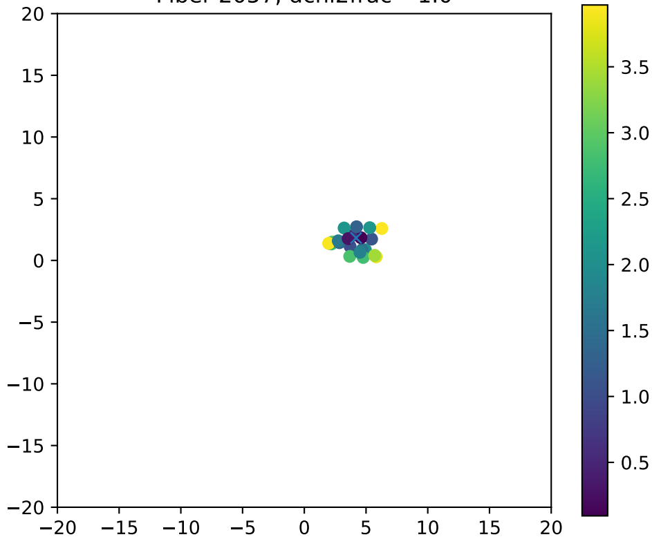
Fiber 2057, dchi2frac= 1.0
