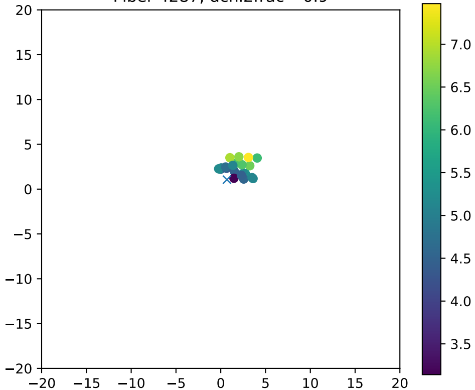
Fiber 4287, dchi2frac= 0.9
