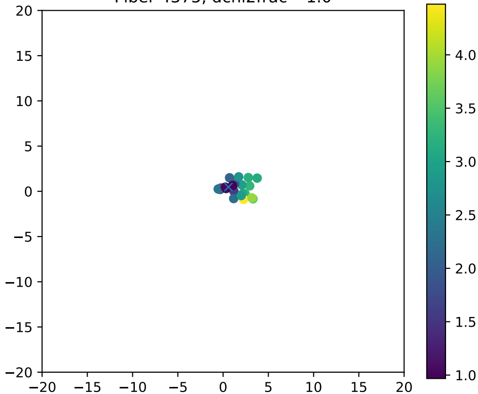
Fiber 4375, dchi2frac= 1.0
