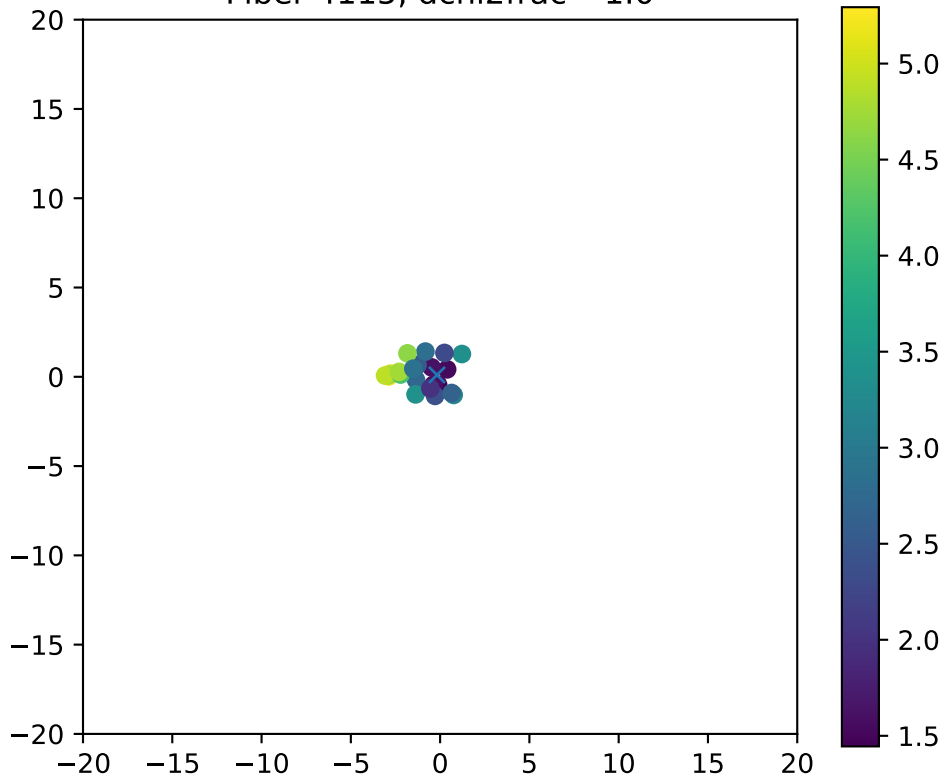
Fiber 4115, dchi2frac= 1.0
