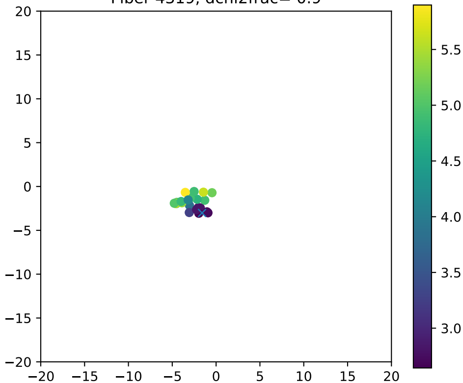
Fiber 4319, dchi2frac= 0.9
