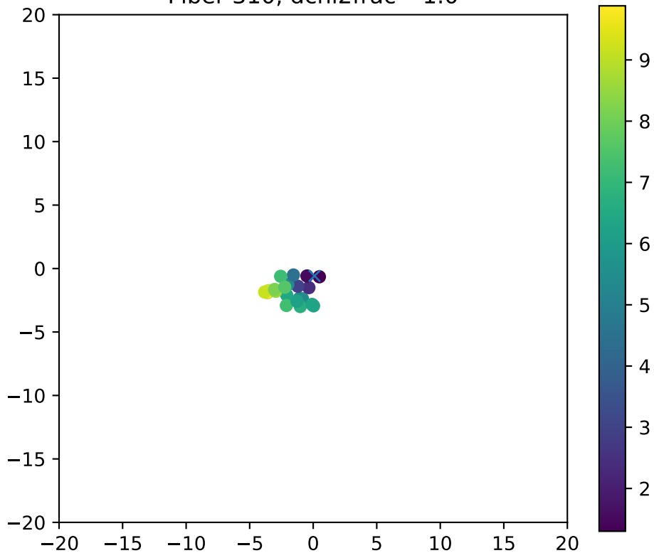
Fiber 310, dchi2frac= 1.0
