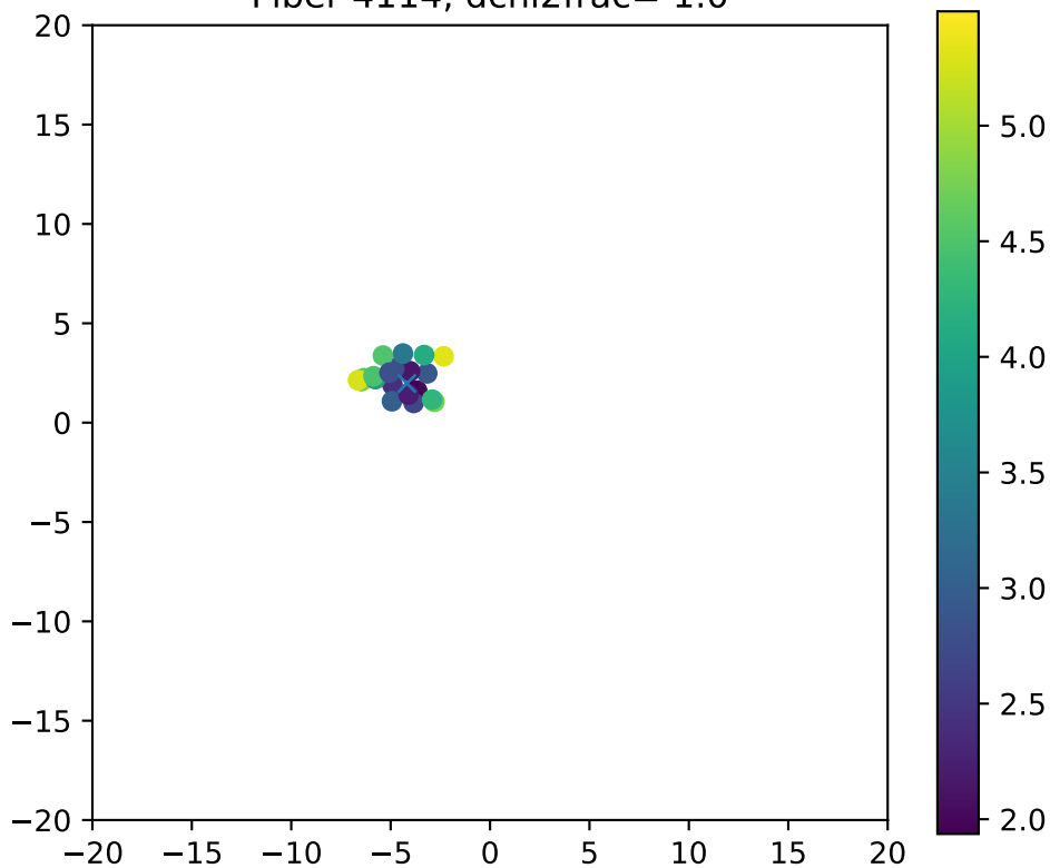
Fiber 4114, dchi2frac= 1.0
