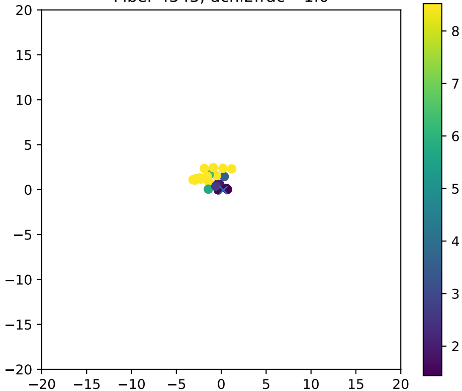
Fiber 4545, dchi2frac= 1.0
