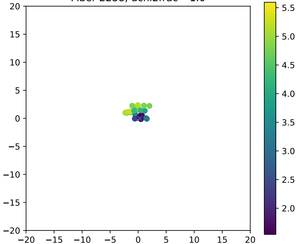
Fiber 2238, dchi2frac= 1.0
