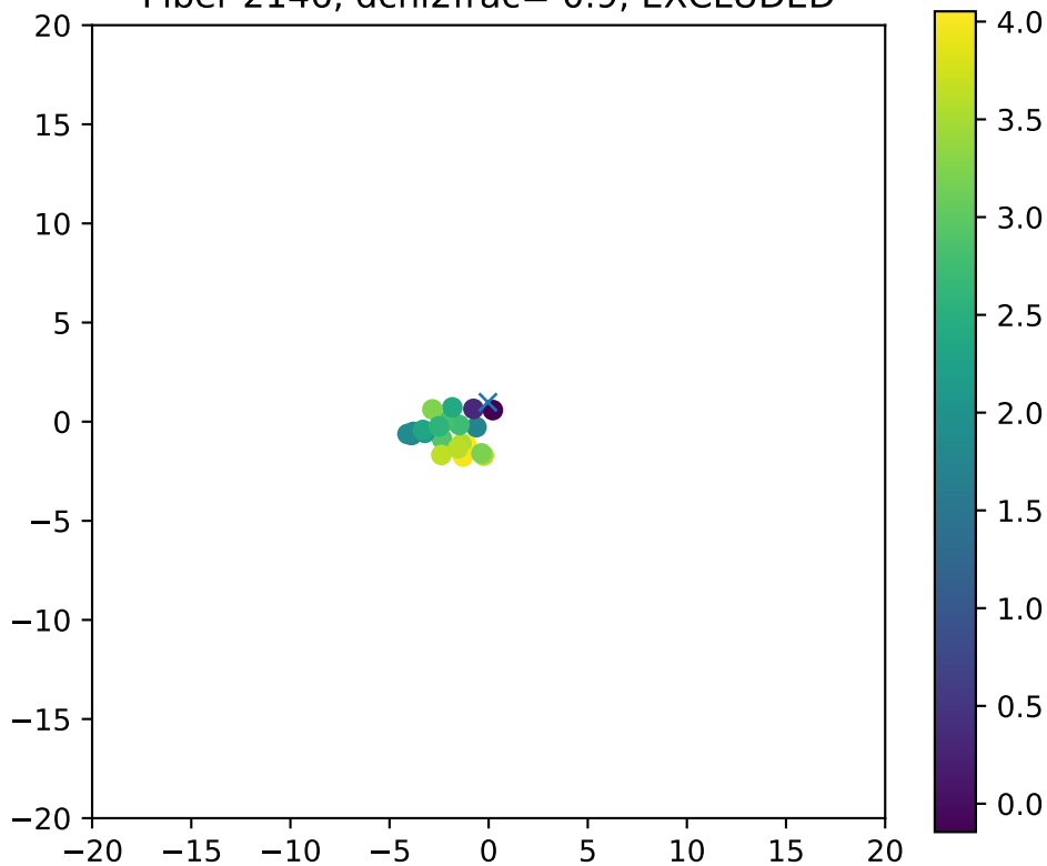
Fiber 2146, dchi2frac= 0.9, EXCLUDED
