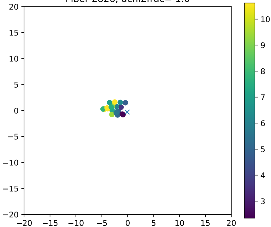
Fiber 2826, dchi2frac= 1.0
