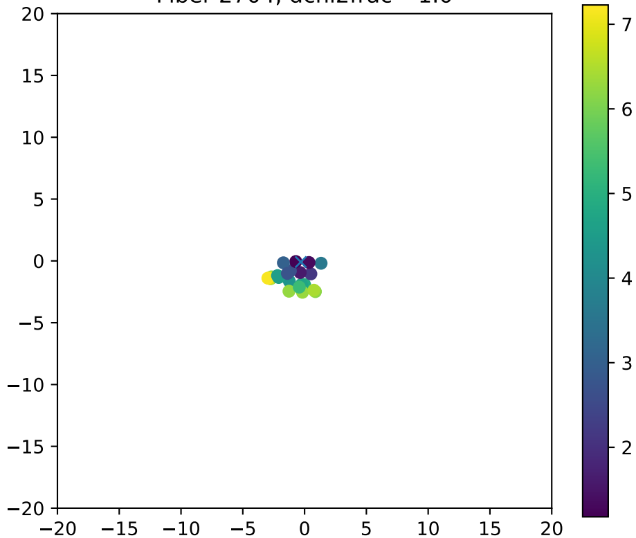
Fiber 2704, dchi2frac= 1.0
