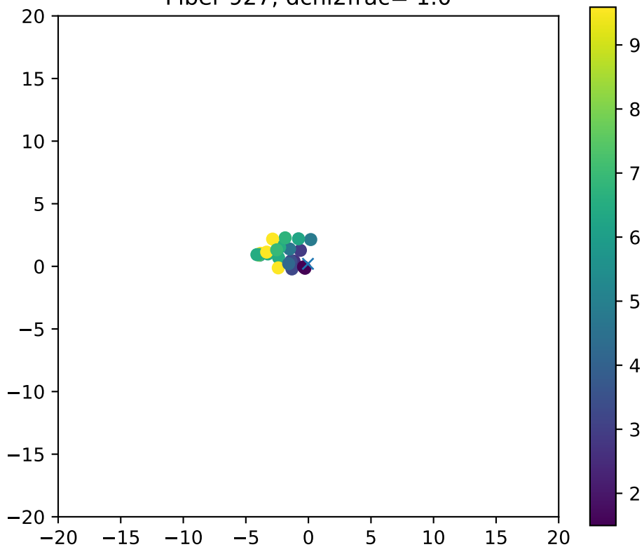
Fiber 927, dchi2frac= 1.0
