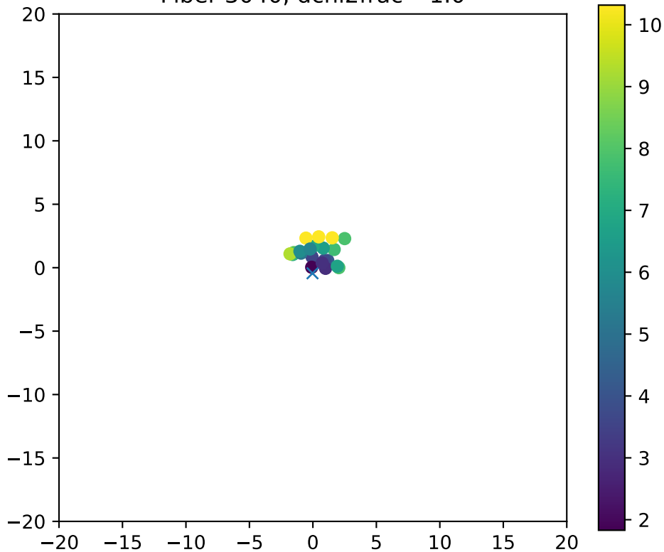
Fiber 3040, dchi2frac= 1.0
