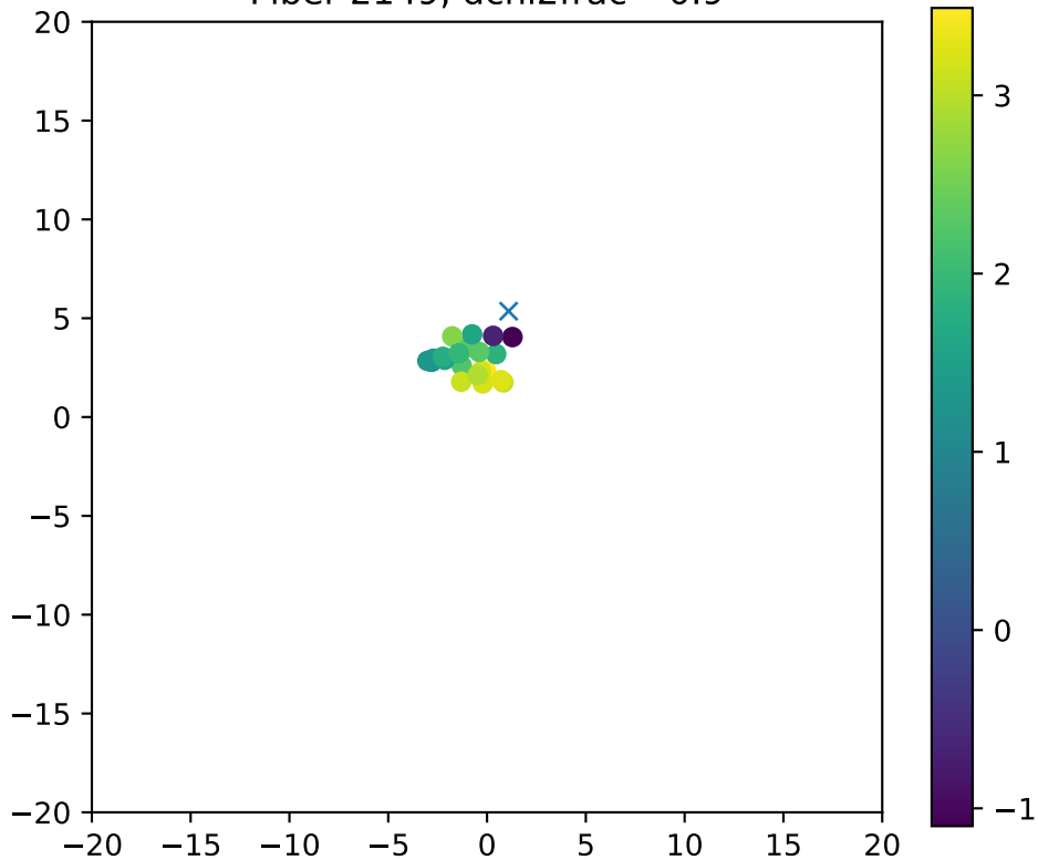
Fiber 2149, dchi2frac= 0.9
