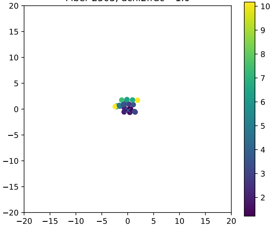
Fiber 2503, dchi2frac= 1.0
