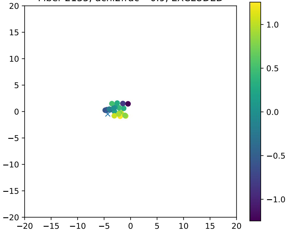
Fiber 2135, dchi2frac= 0.9, EXCLUDED
