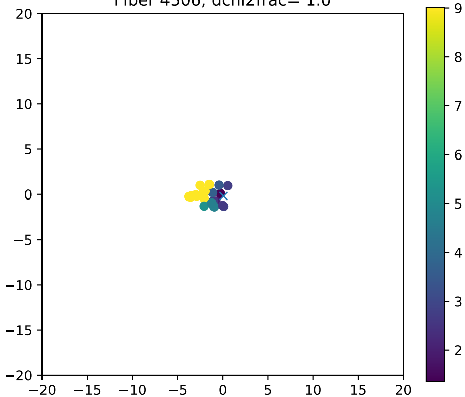
Fiber 4506, dchi2frac= 1.0
