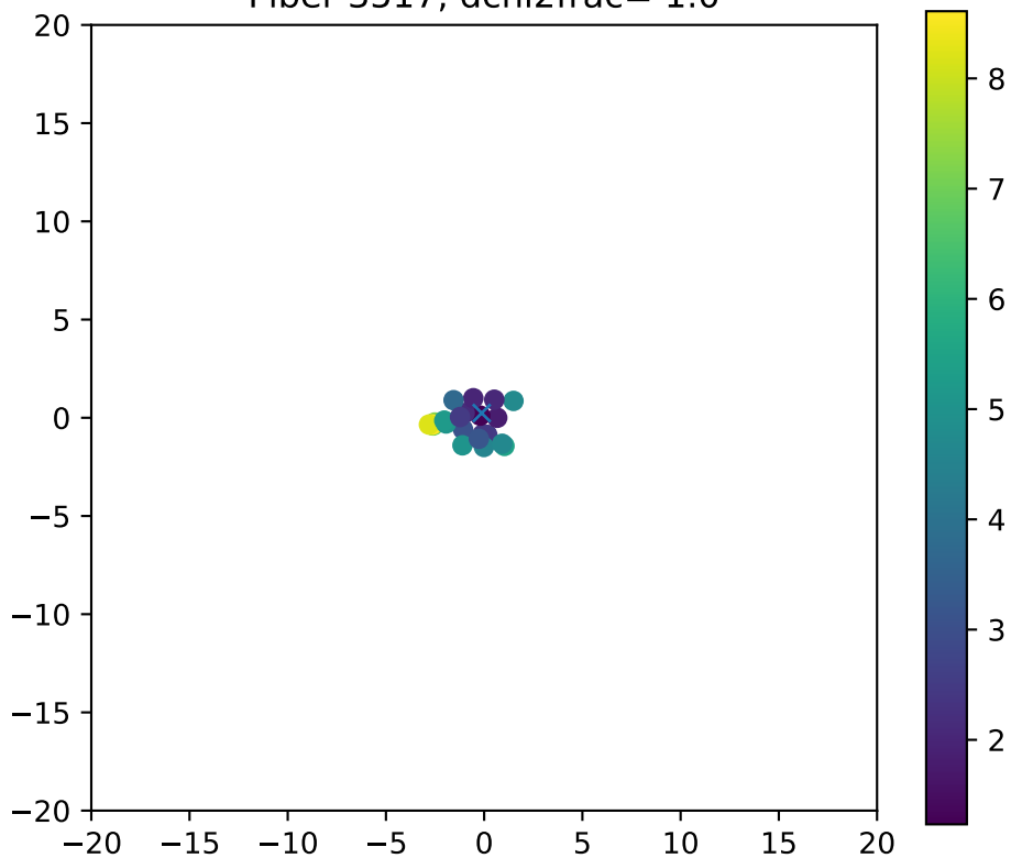
Fiber 3517, dchi2frac= 1.0
