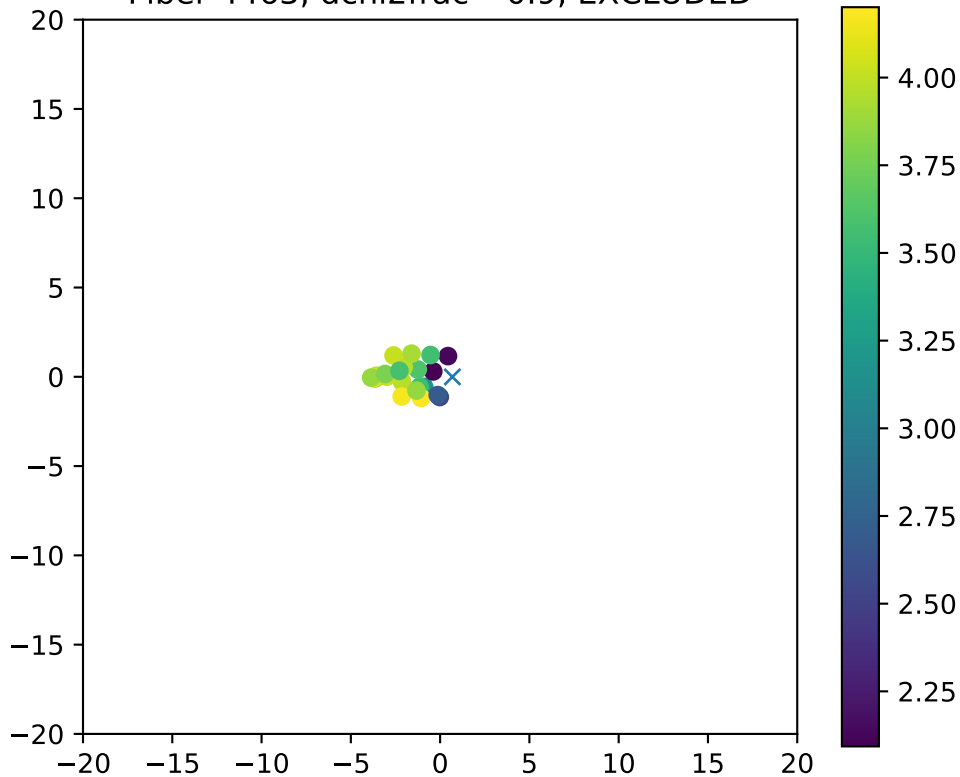
Fiber 4463, dchi2frac= 0.9, EXCLUDED
