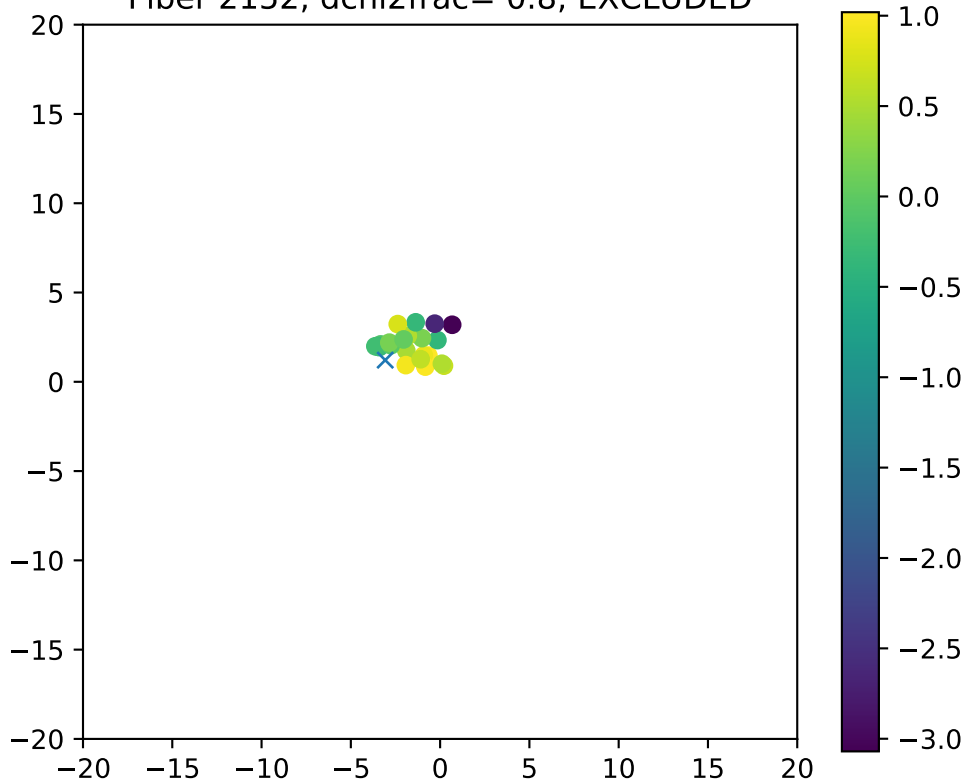
Fiber 2152, dchi2frac= 0.8, EXCLUDED
