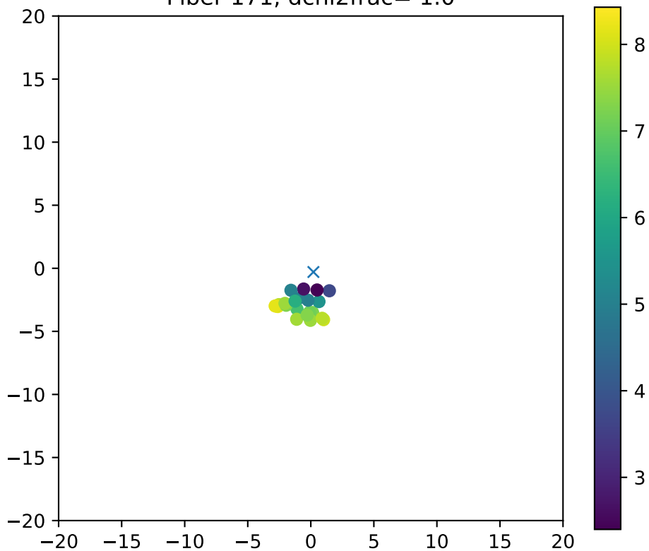
Fiber 171, dchi2frac= 1.0
