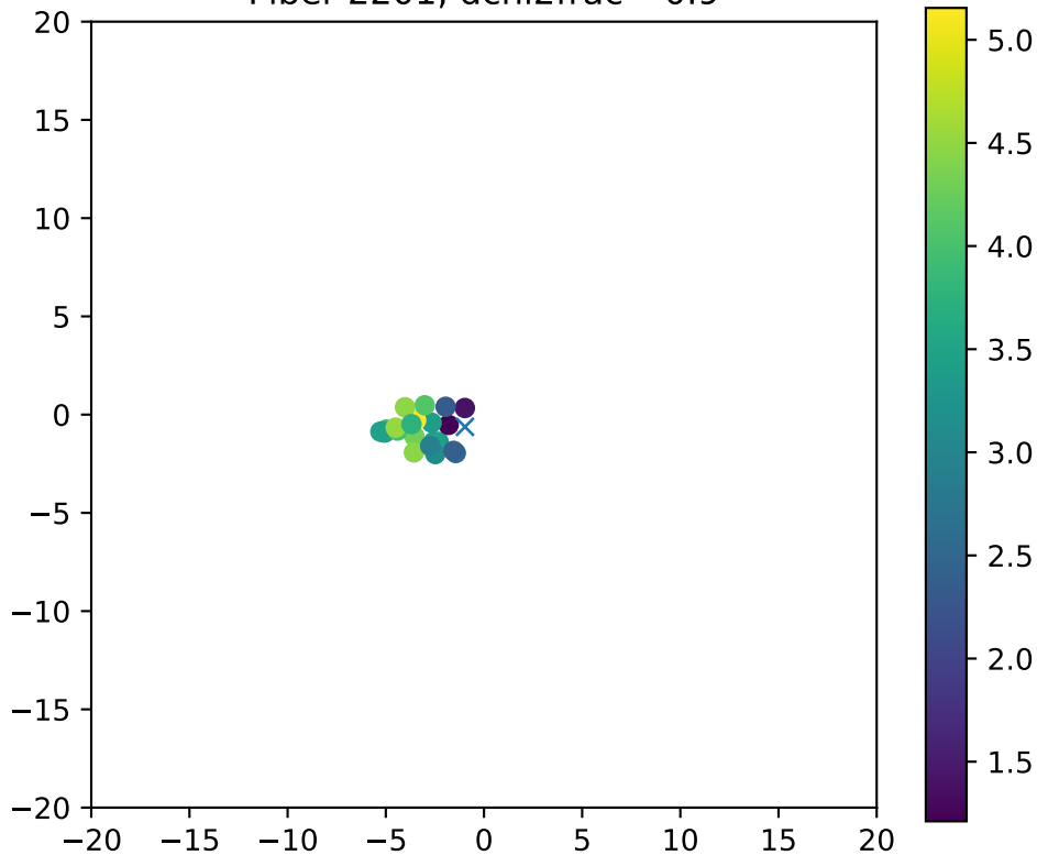
Fiber 2201, dchi2frac= 0.9
