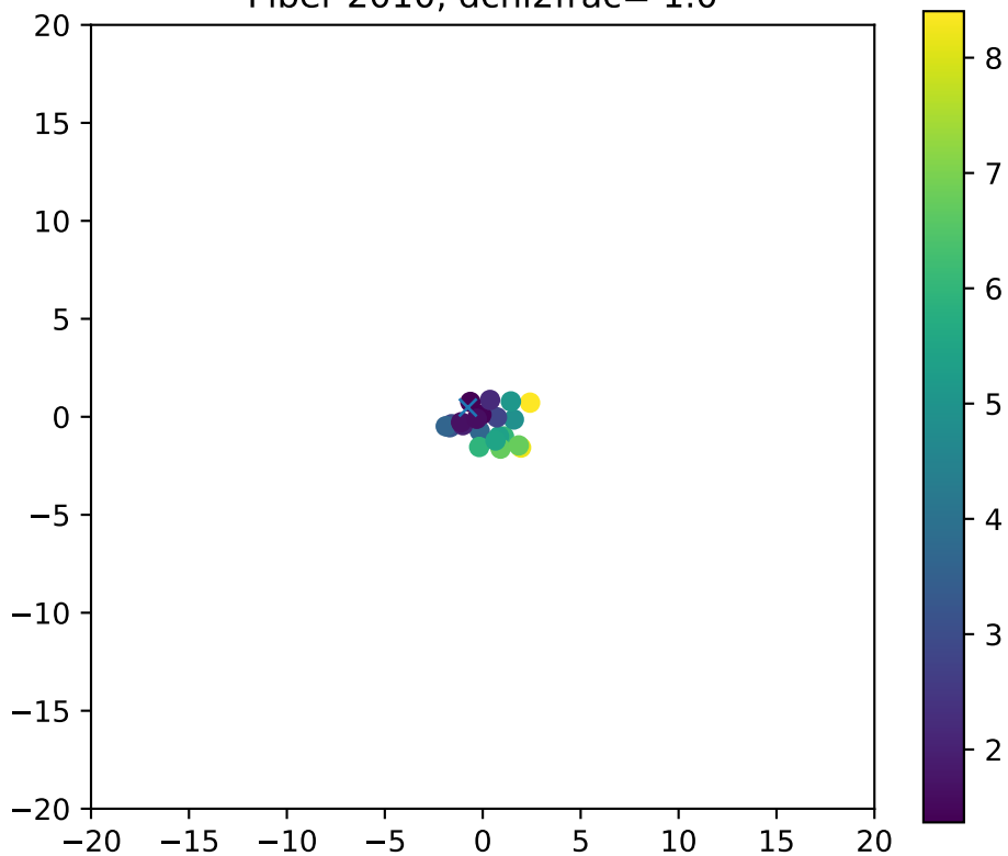
Fiber 2010, dchi2frac= 1.0
