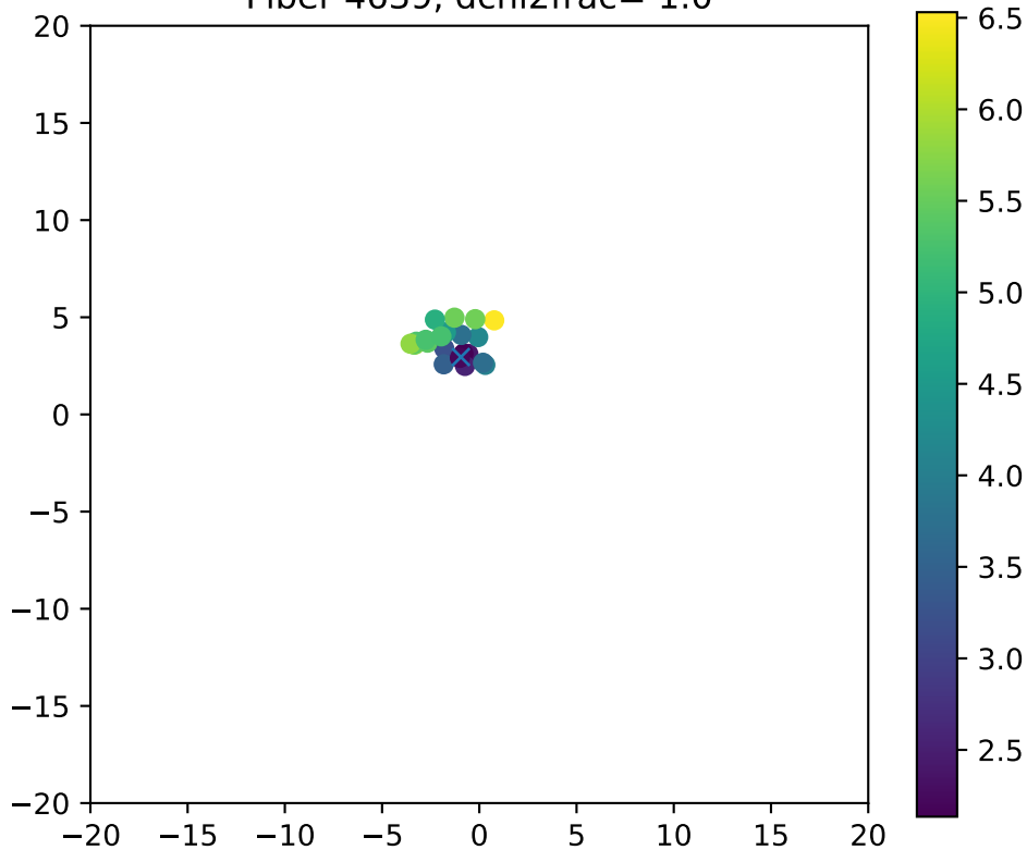
Fiber 4639, dchi2frac= 1.0
