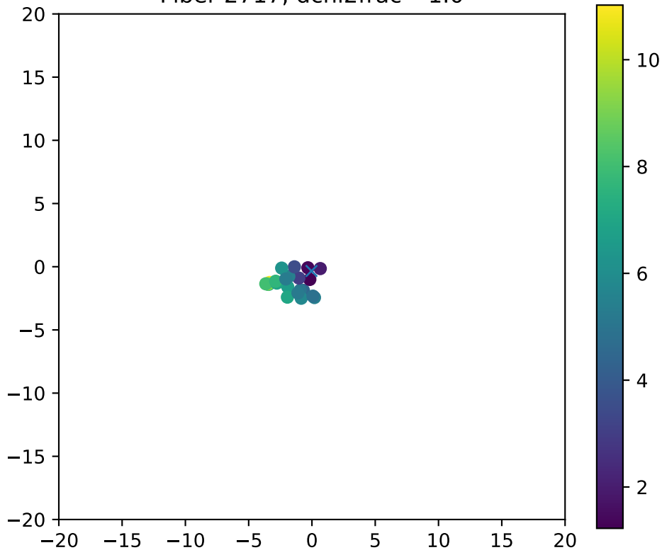
Fiber 2717, dchi2frac= 1.0
