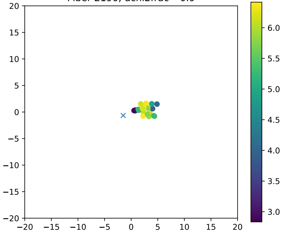
Fiber 2190, dchi2frac= 0.9
