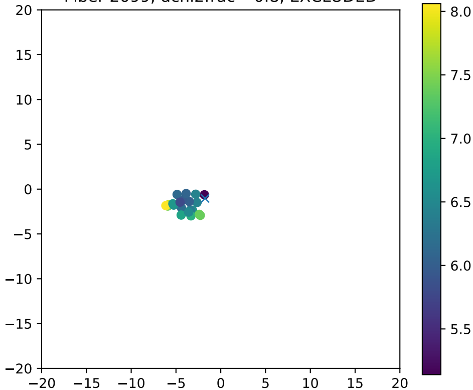
Fiber 2099, dchi2frac= 0.8, EXCLUDED
