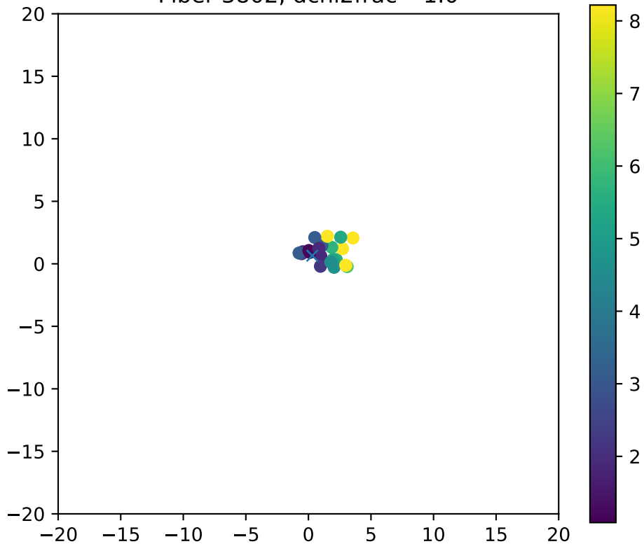
Fiber 3802, dchi2frac= 1.0
