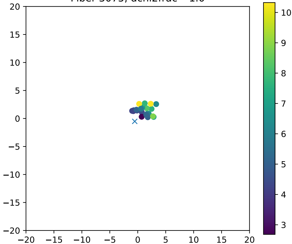
Fiber 3075, dchi2frac= 1.0
