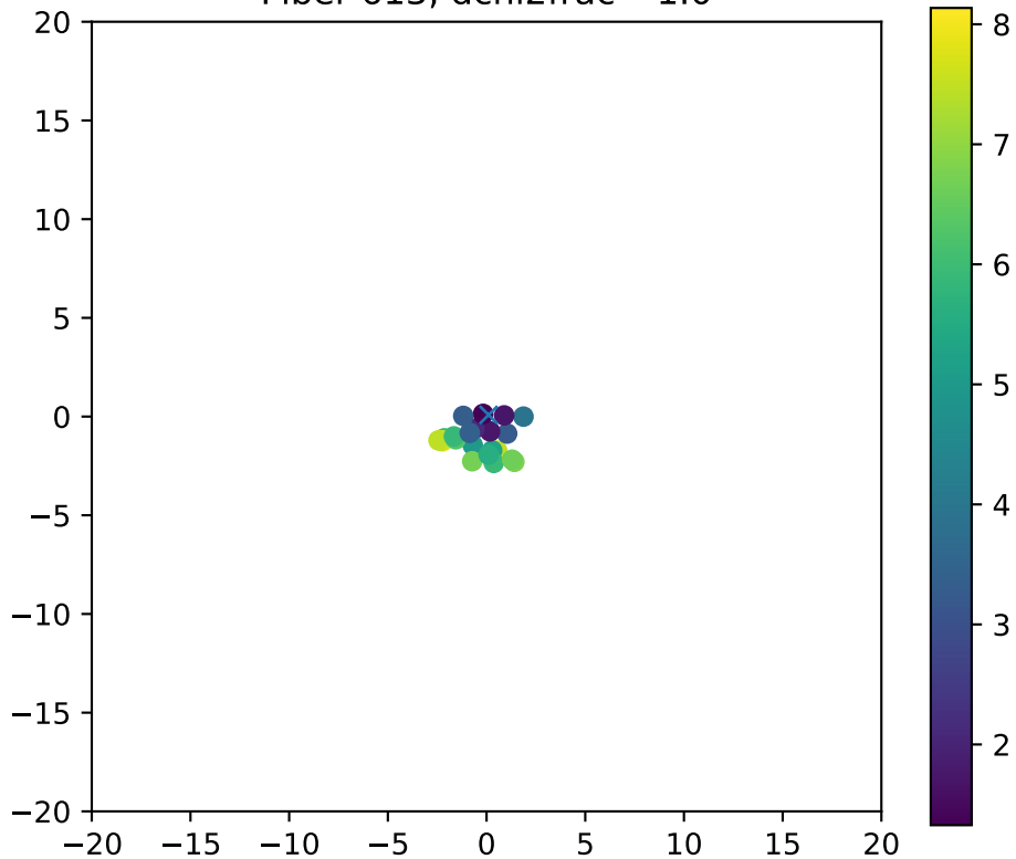
Fiber 613, dchi2frac= 1.0
