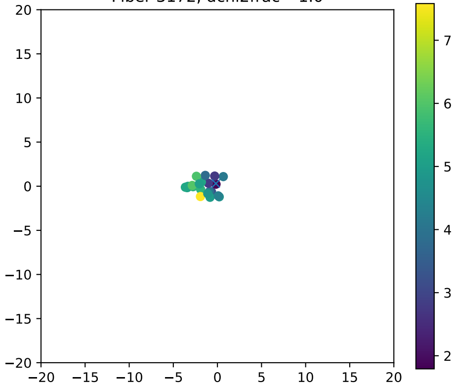
Fiber 3172, dchi2frac= 1.0
