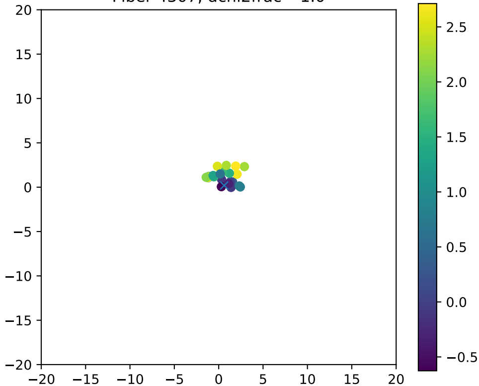
Fiber 4307, dchi2frac= 1.0
