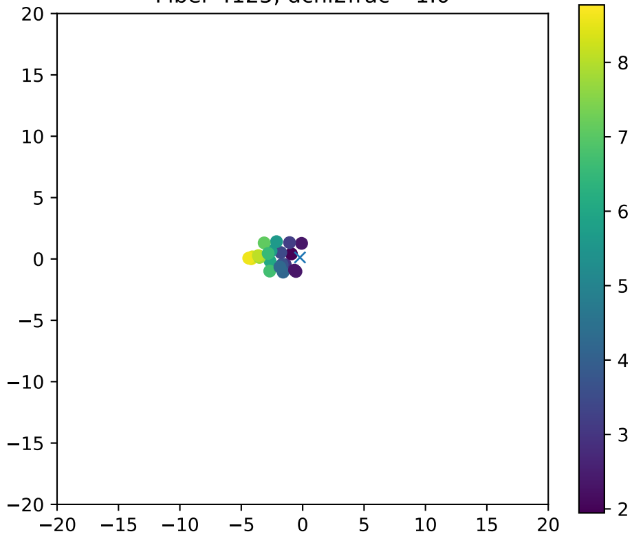
Fiber 4125, dchi2frac= 1.0
