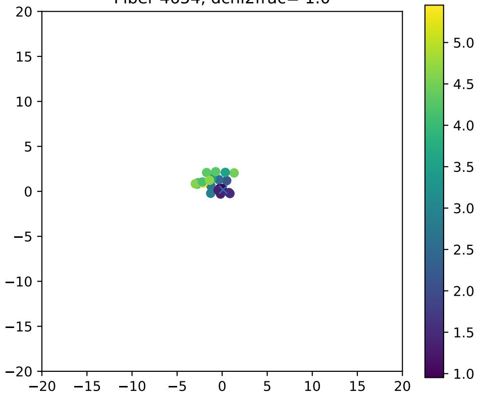
Fiber 4654, dchi2frac= 1.0
