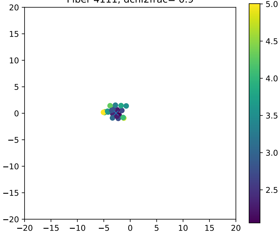
Fiber 4111, dchi2frac= 0.9
