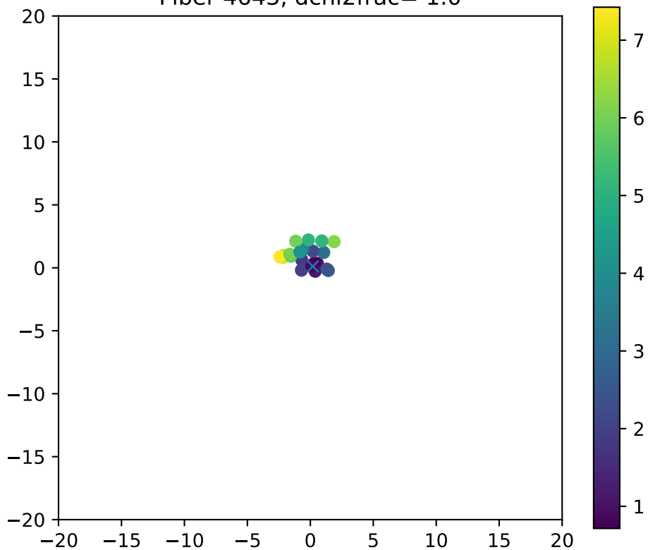
Fiber 4643, dchi2frac= 1.0
