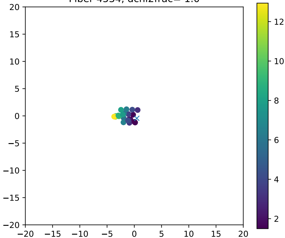
Fiber 4534, dchi2frac= 1.0
