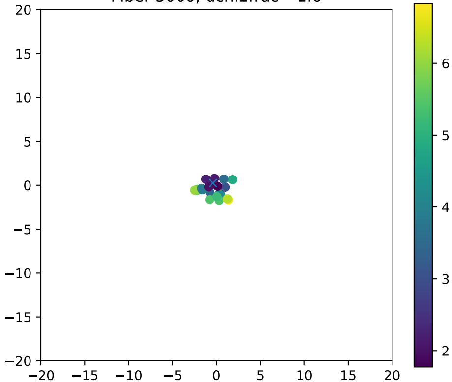
Fiber 3060, dchi2frac= 1.0
