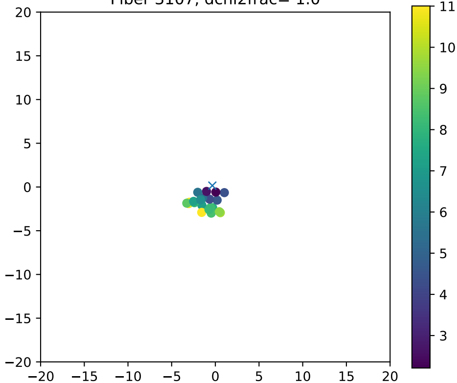
Fiber 3107, dchi2frac= 1.0
