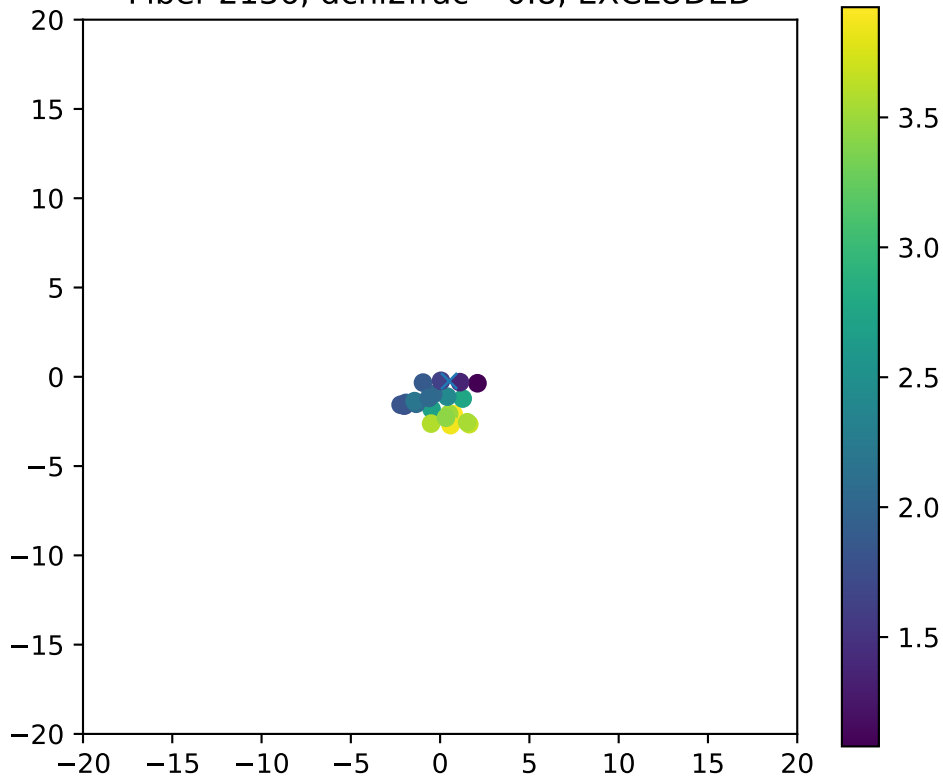
Fiber 2136, dchi2frac= 0.8, EXCLUDED
