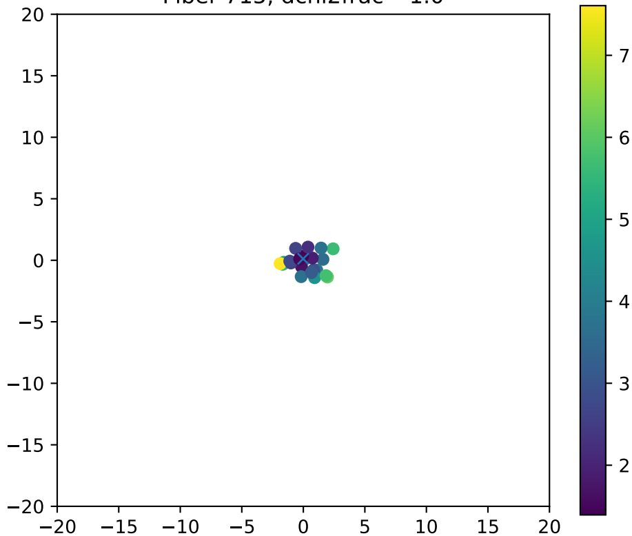
Fiber 715, dchi2frac= 1.0
