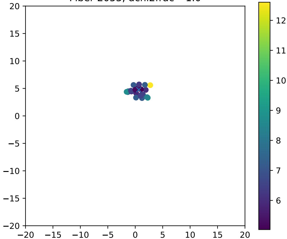
Fiber 2053, dchi2frac= 1.0
