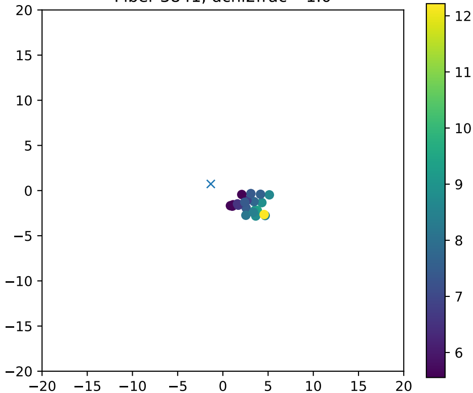
Fiber 3841, dchi2frac= 1.0
