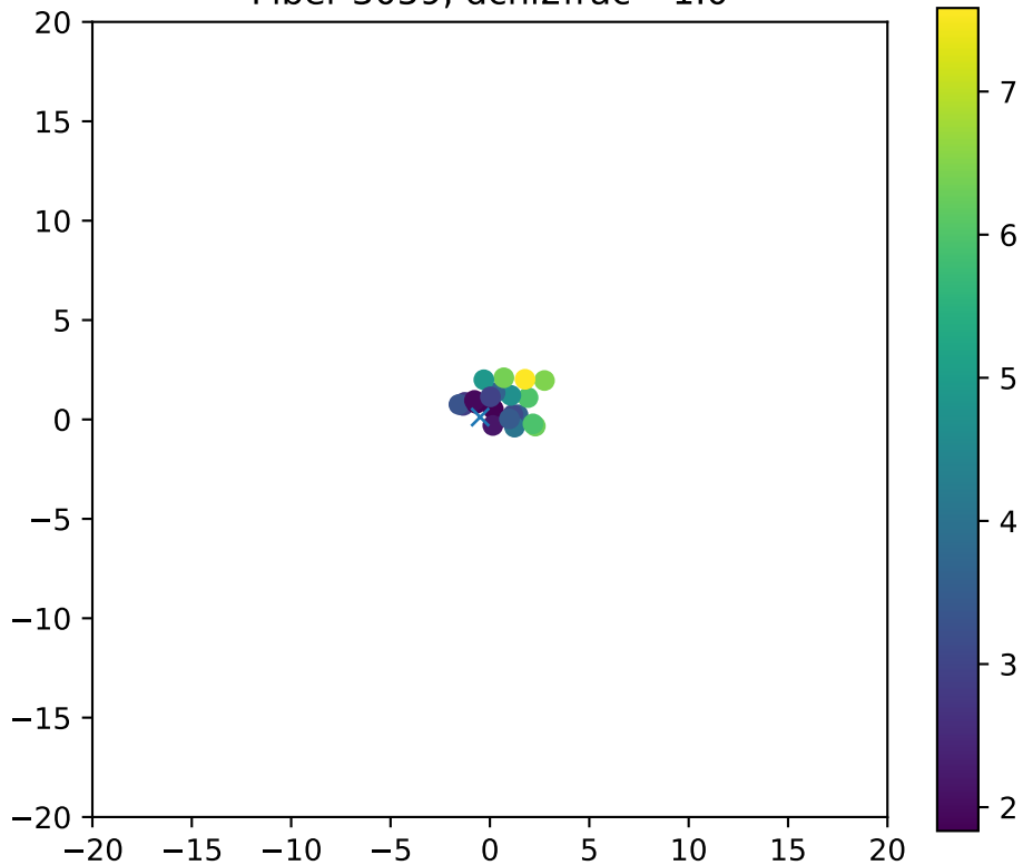
Fiber 3059, dchi2frac= 1.0
