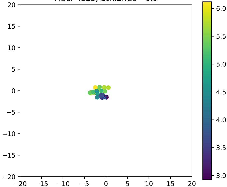
Fiber 4325, dchi2frac= 0.9
