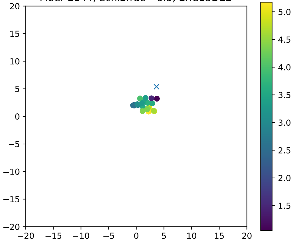
Fiber 2144, dchi2frac= 0.9, EXCLUDED
