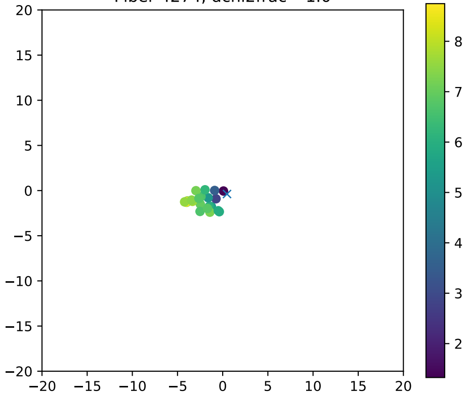
Fiber 4274, dchi2frac= 1.0
