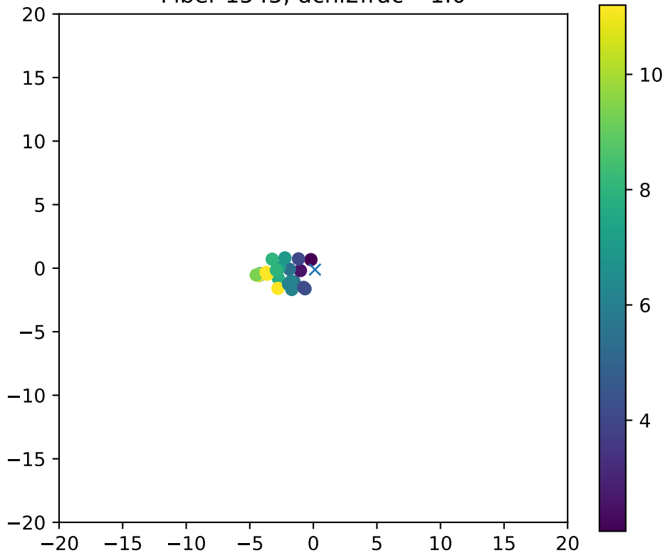
Fiber 1545, dchi2frac= 1.0
