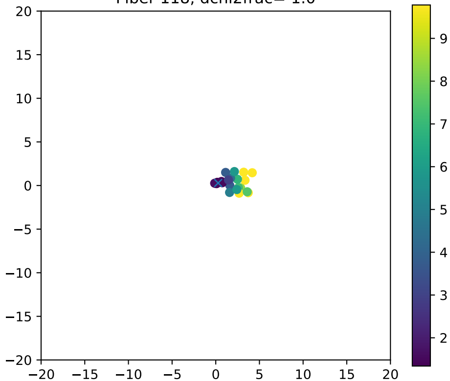
Fiber 118, dchi2frac= 1.0
