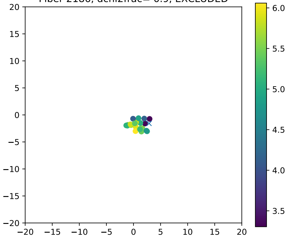
Fiber 2186, dchi2frac= 0.9, EXCLUDED
