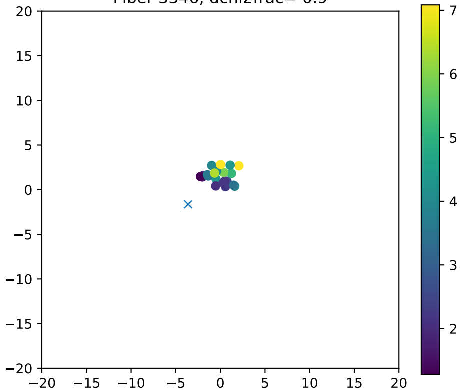
Fiber 3346, dchi2frac= 0.9
