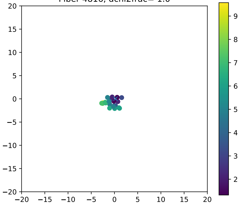
Fiber 4816, dchi2frac= 1.0
