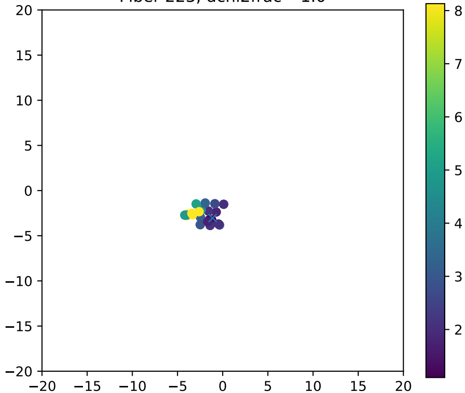
Fiber 223, dchi2frac= 1.0
