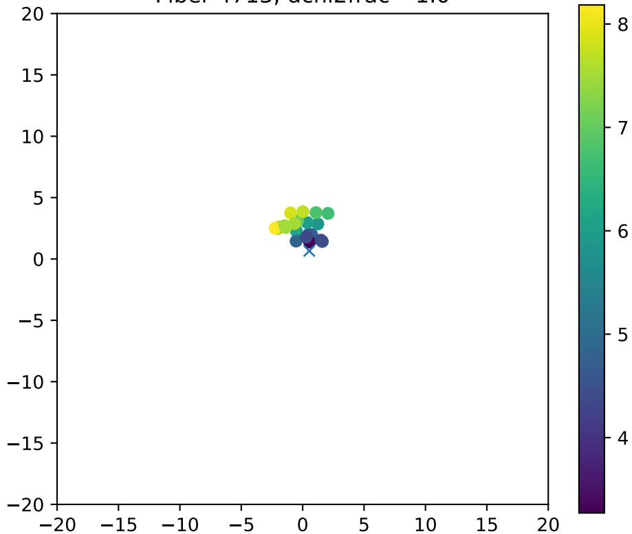
Fiber 4713, dchi2frac= 1.0
