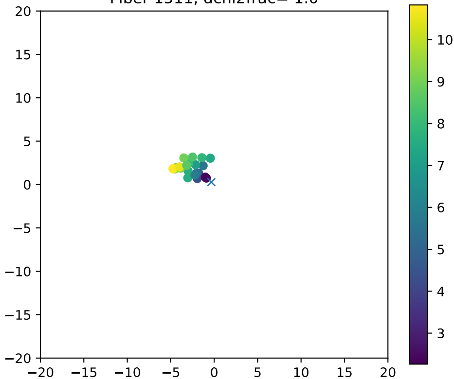
Fiber 1511, dchi2frac= 1.0
