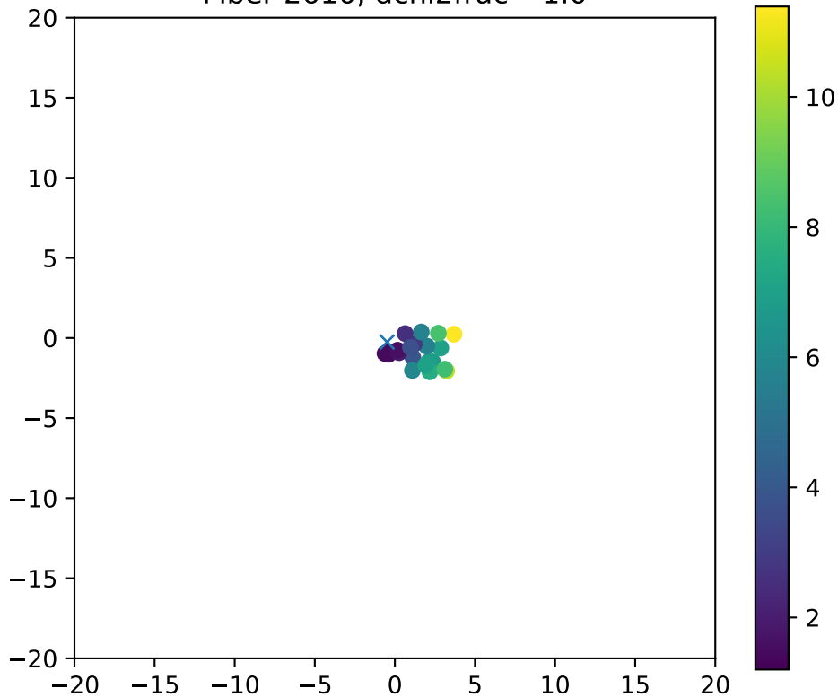
Fiber 2610, dchi2frac= 1.0
