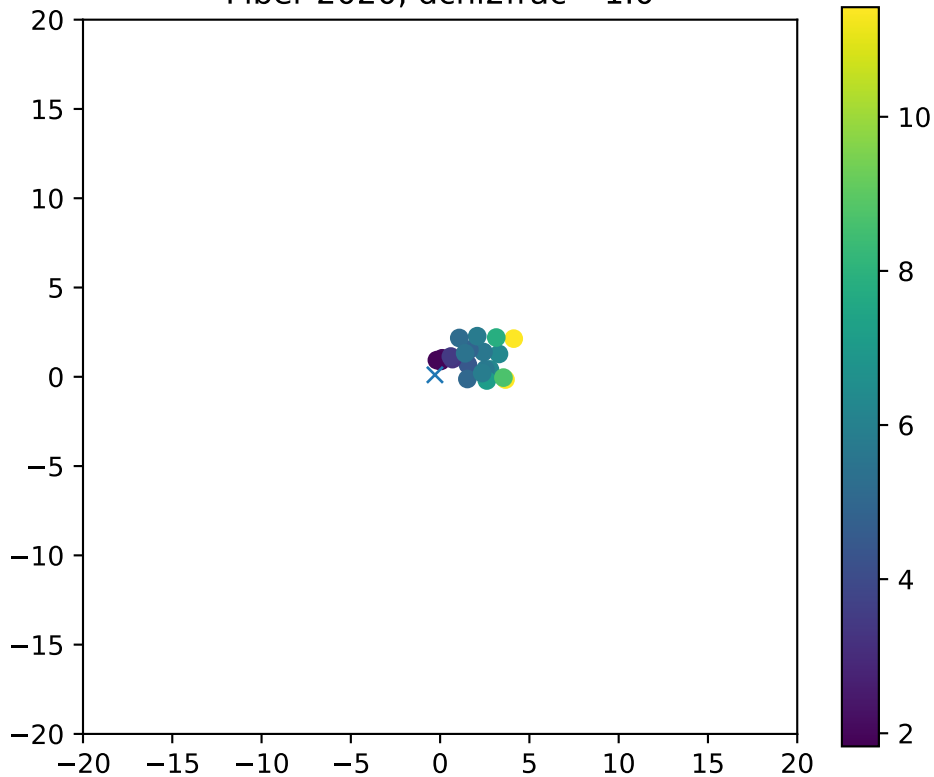
Fiber 2020, dchi2frac= 1.0
