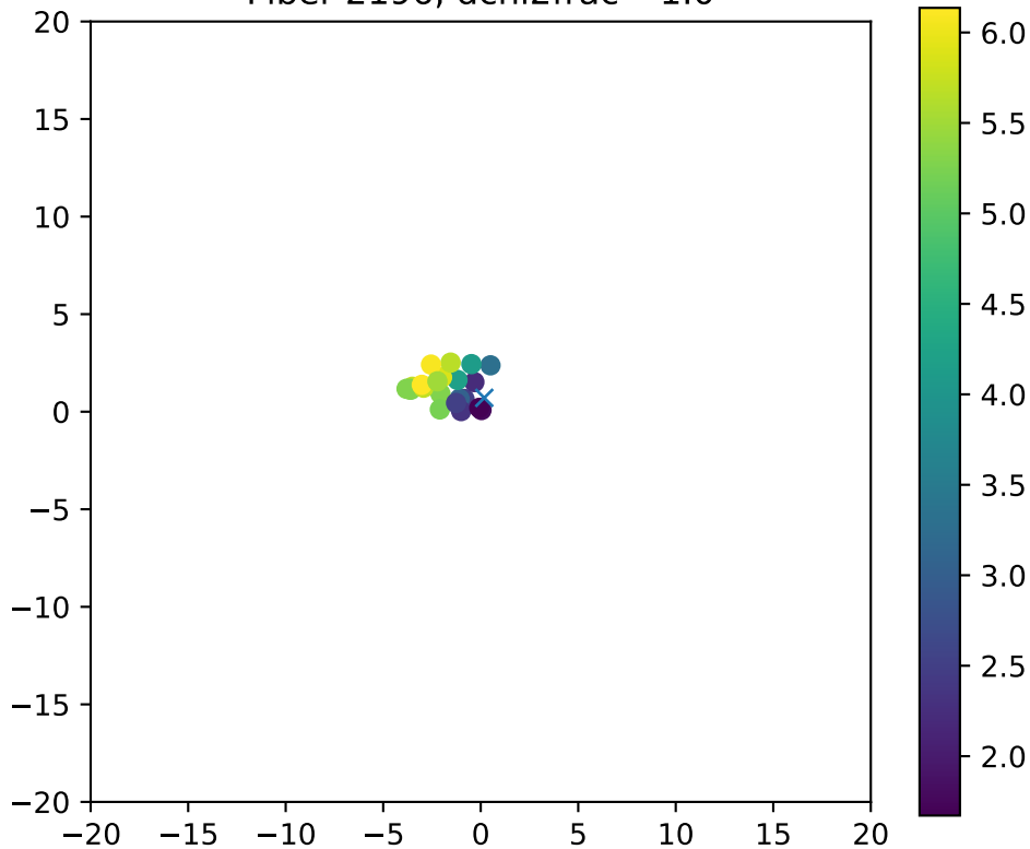
Fiber 2196, dchi2frac= 1.0
