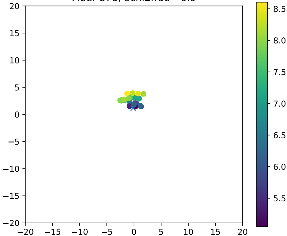
Fiber 876, dchi2frac= 0.9
