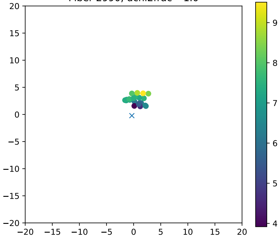
Fiber 2990, dchi2frac= 1.0
