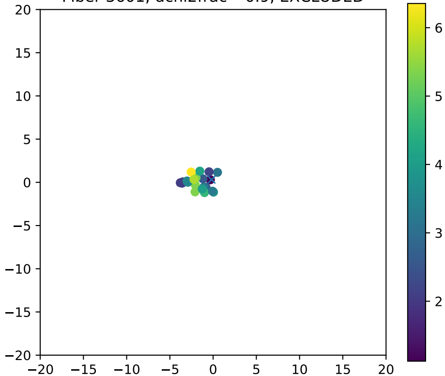
Fiber 3601, dchi2frac= 0.9, EXCLUDED
