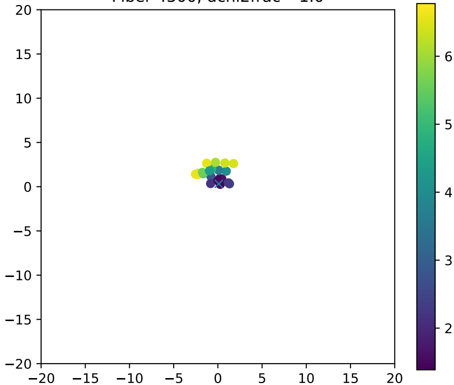
Fiber 4300, dchi2frac= 1.0
