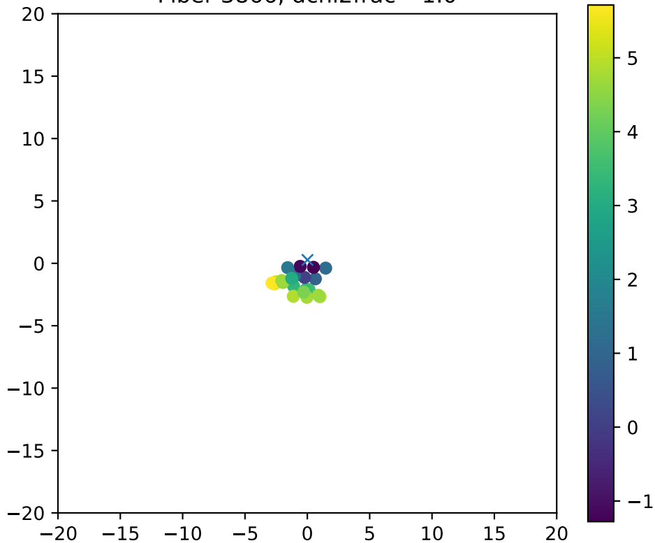
Fiber 3866, dchi2frac= 1.0
