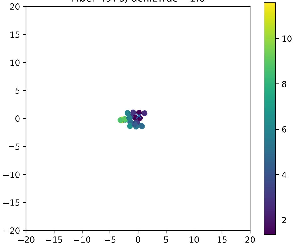
Fiber 4976, dchi2frac= 1.0
