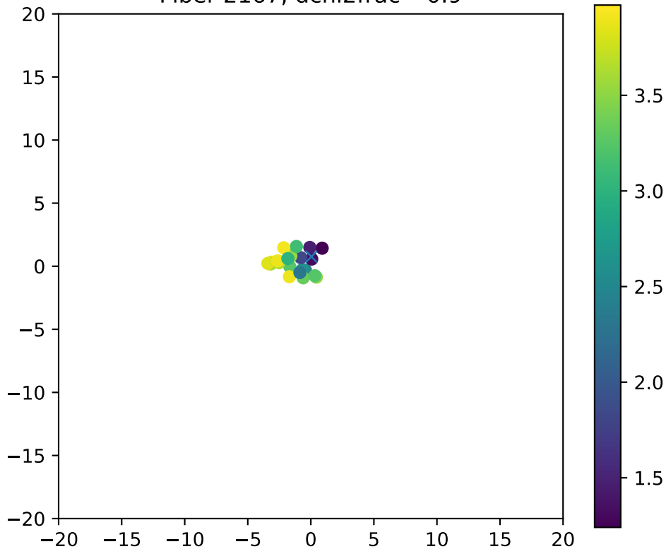
Fiber 2167, dchi2frac= 0.9
