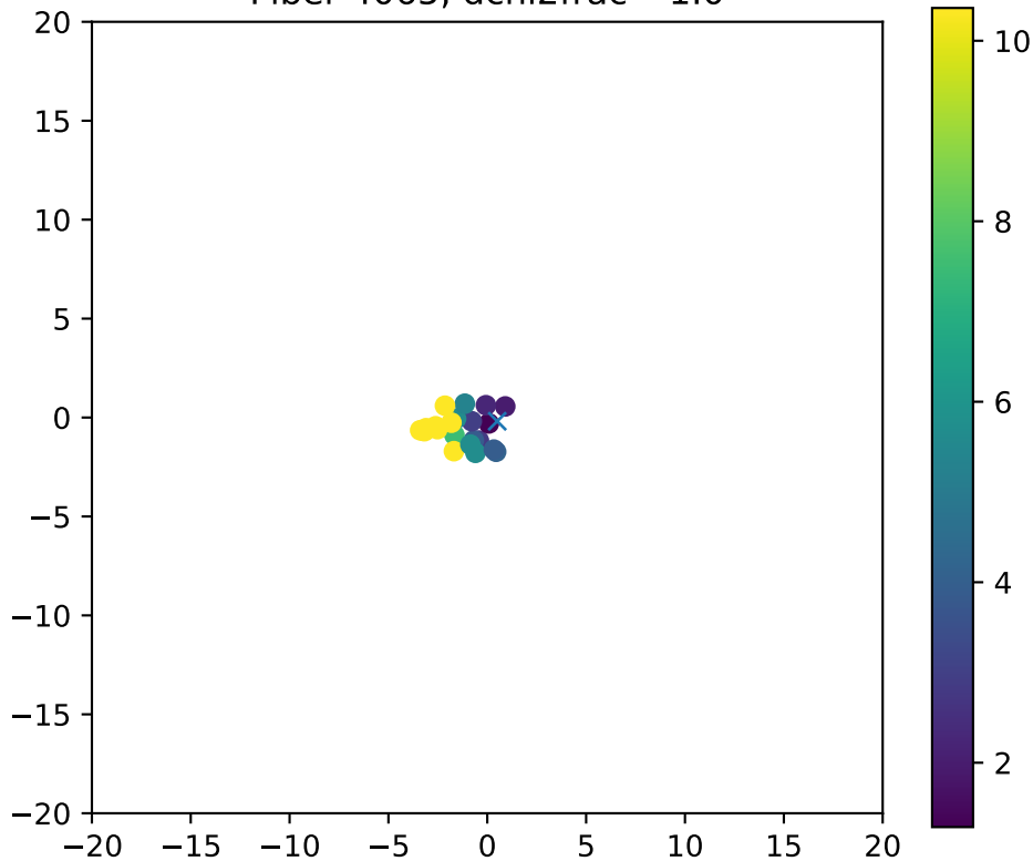
Fiber 4065, dchi2frac= 1.0
