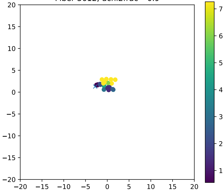
Fiber 3612, dchi2frac= 0.9
