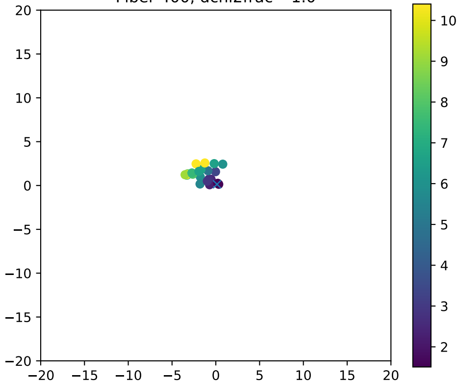
Fiber 400, dchi2frac= 1.0
