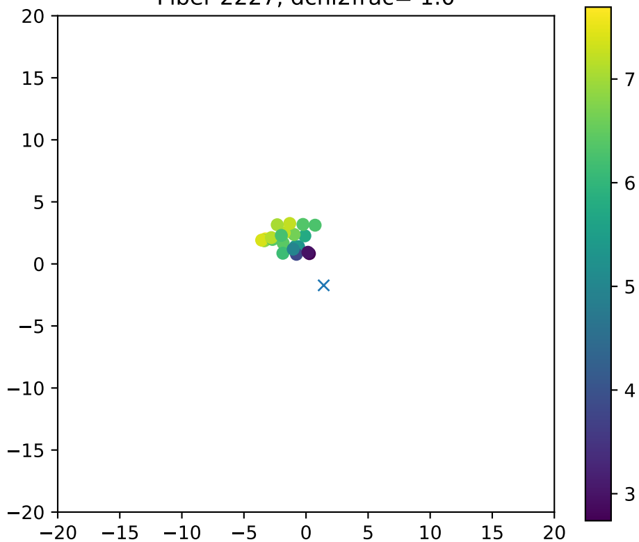
Fiber 2227, dchi2frac= 1.0
