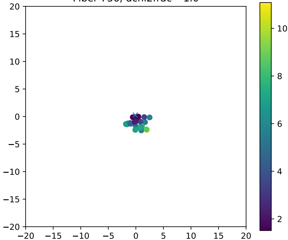
Fiber 736, dchi2frac= 1.0
