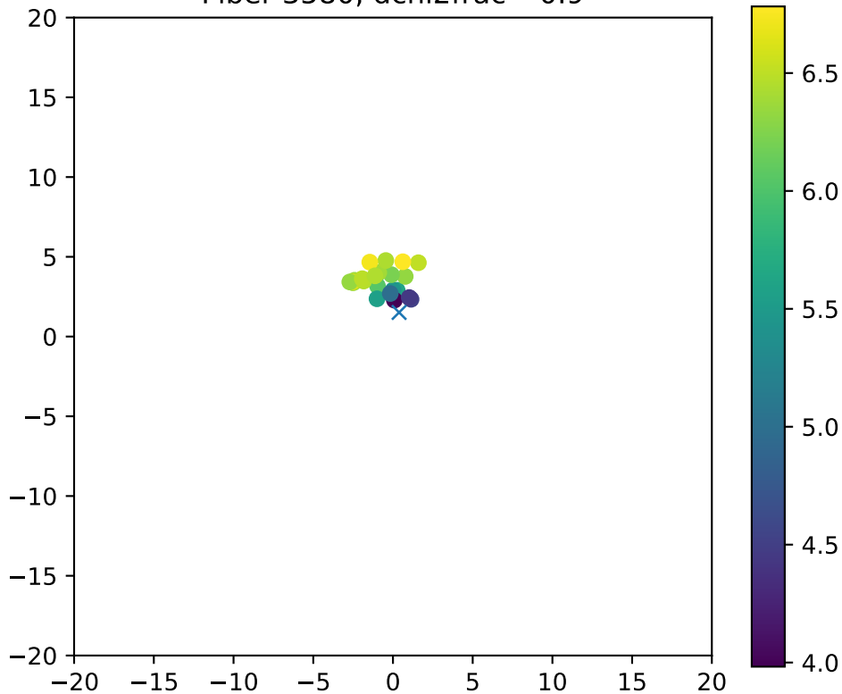
Fiber 3580, dchi2frac= 0.9
