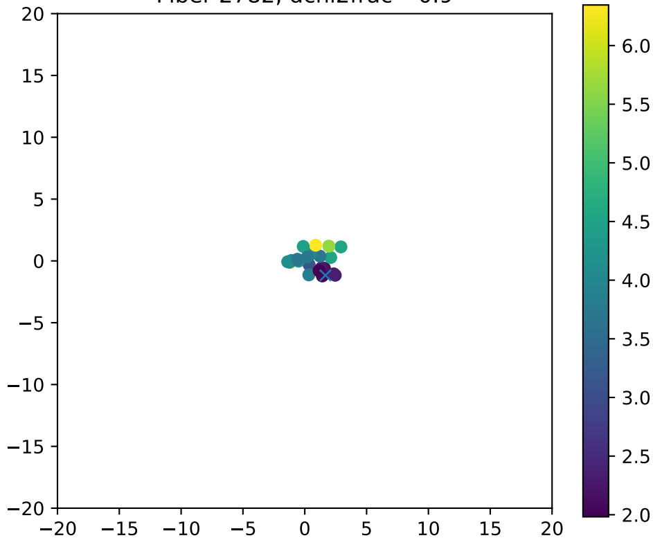
Fiber 2782, dchi2frac= 0.9
