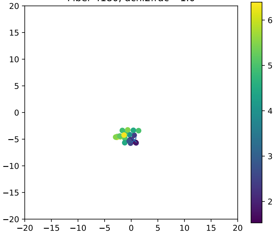
Fiber 4180, dchi2frac= 1.0
