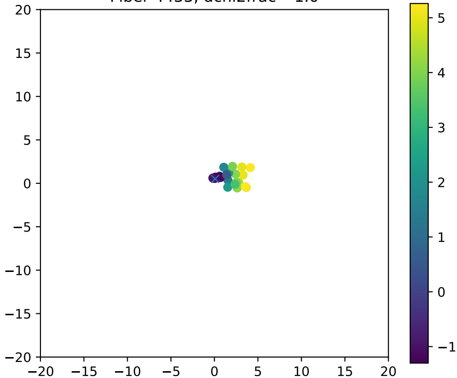
Fiber 4433, dchi2frac= 1.0
