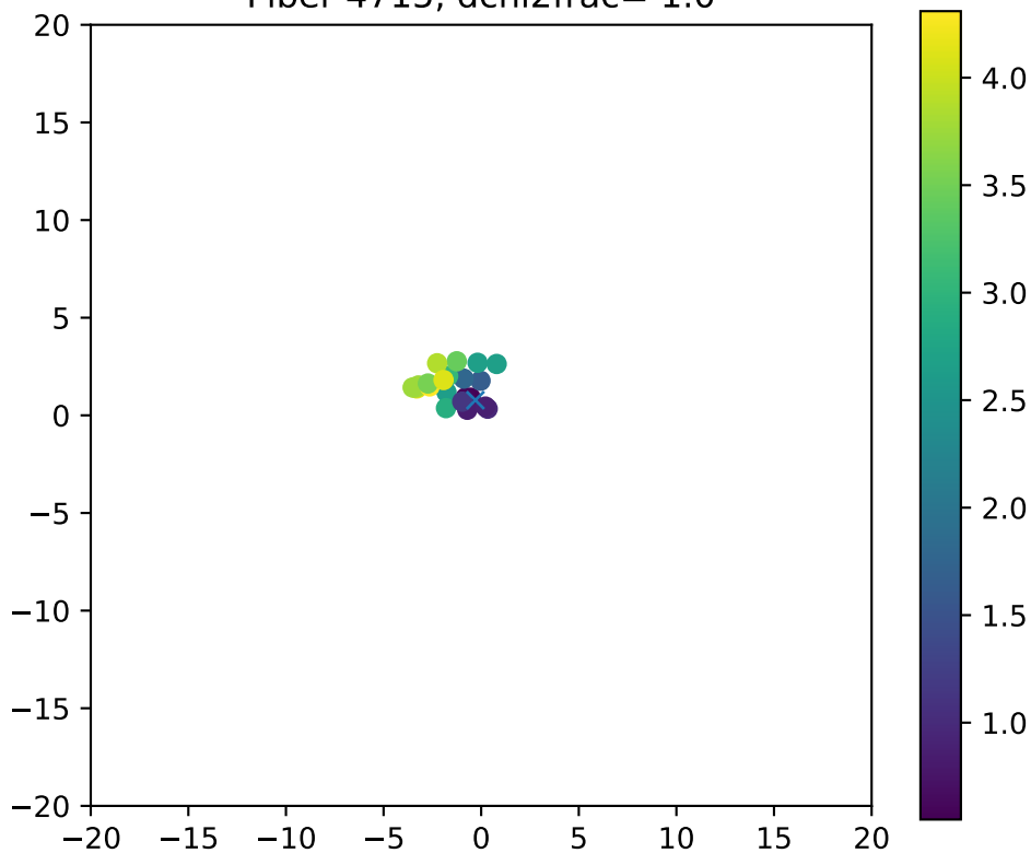
Fiber 4715, dchi2frac= 1.0
