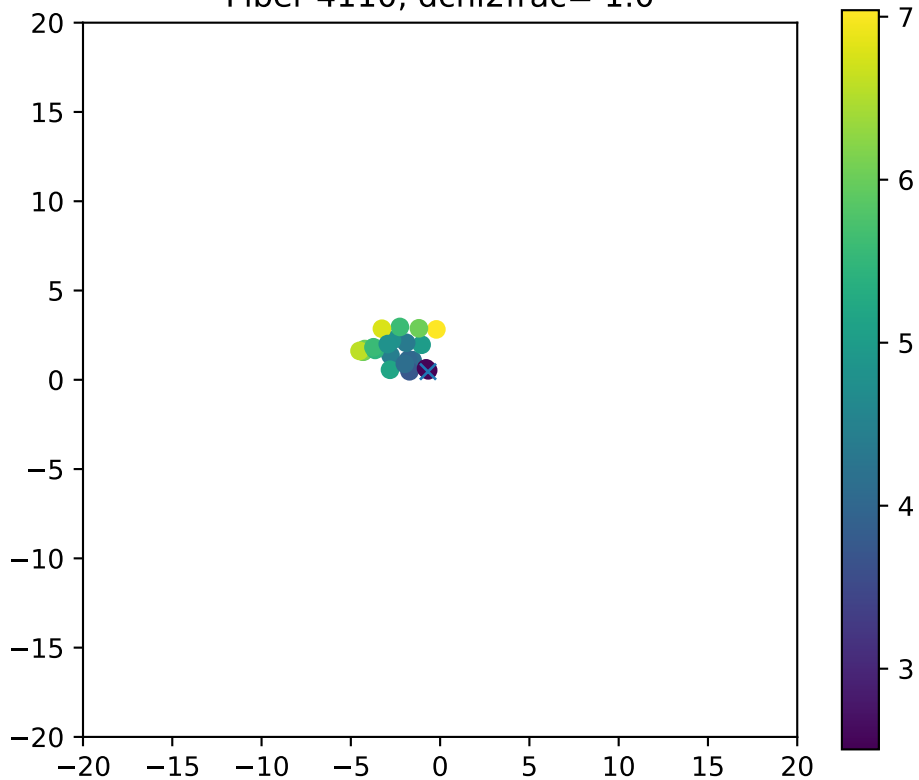
Fiber 4110, dchi2frac= 1.0
