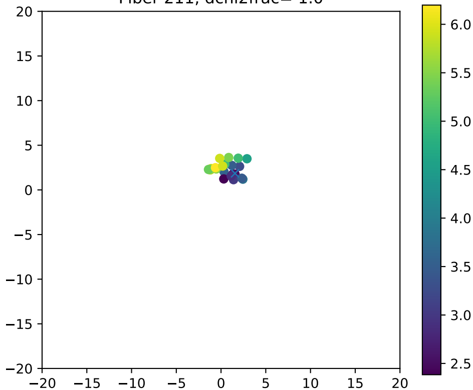
Fiber 211, dchi2frac= 1.0
