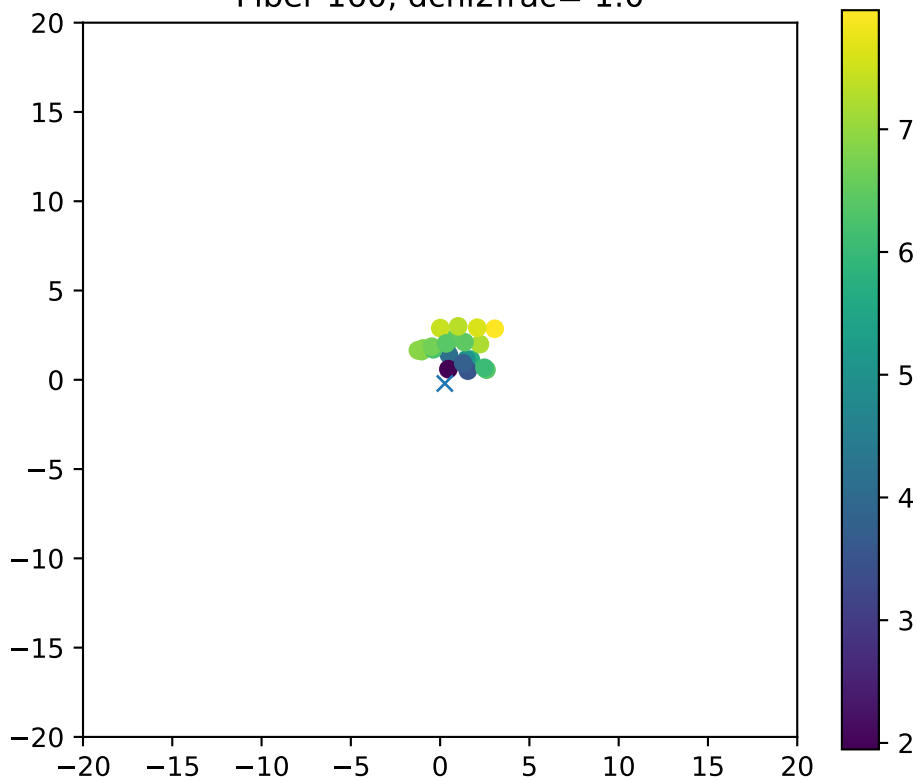
Fiber 160, dchi2frac= 1.0
