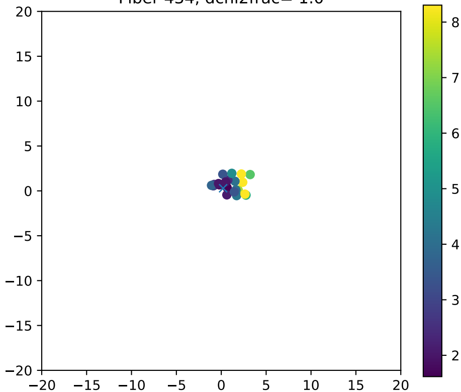
Fiber 434, dchi2frac= 1.0
