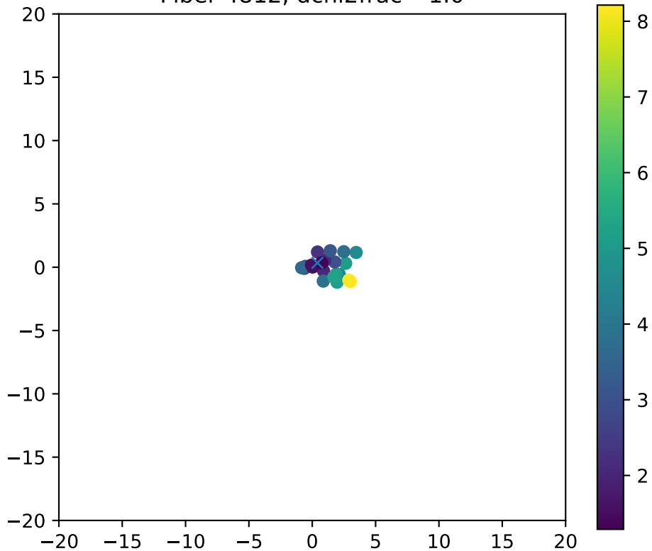
Fiber 4812, dchi2frac= 1.0
