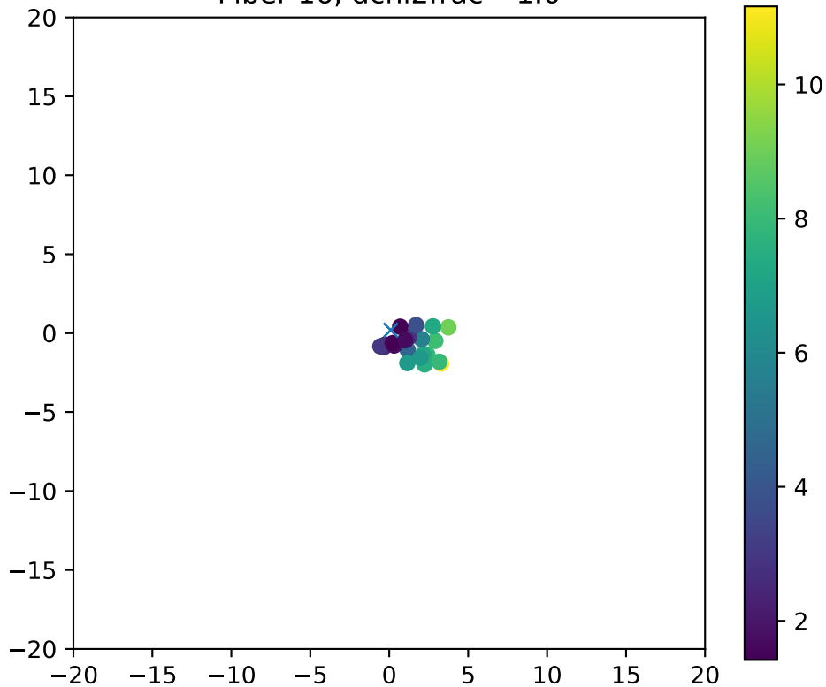
Fiber 16, dchi2frac= 1.0
