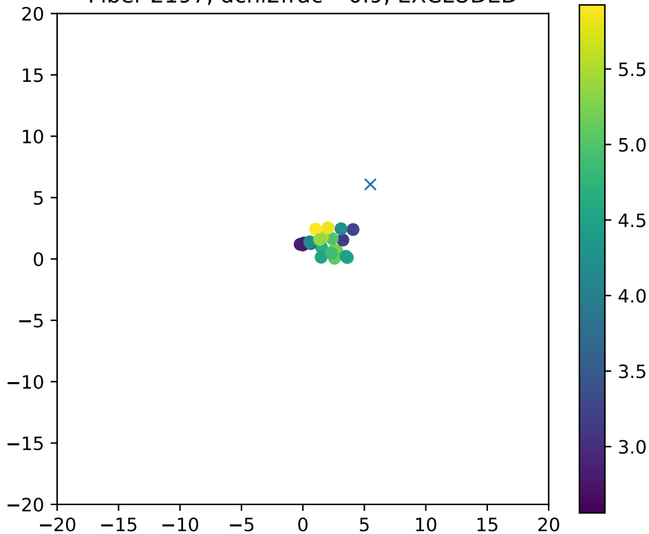
Fiber 2197, dchi2frac= 0.9, EXCLUDED
