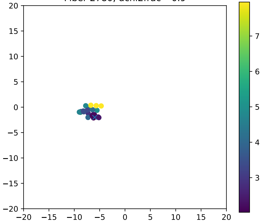
Fiber 2780, dchi2frac= 0.9
