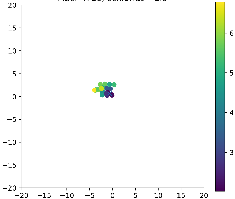
Fiber 4726, dchi2frac= 1.0
