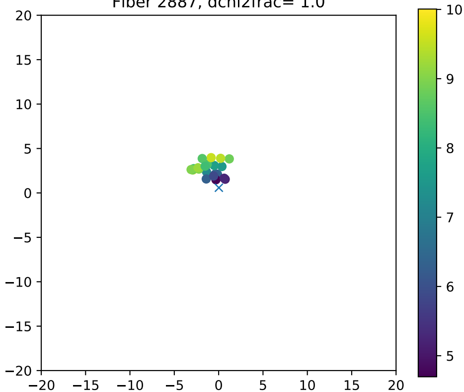
Fiber 2887, dchi2frac= 1.0
