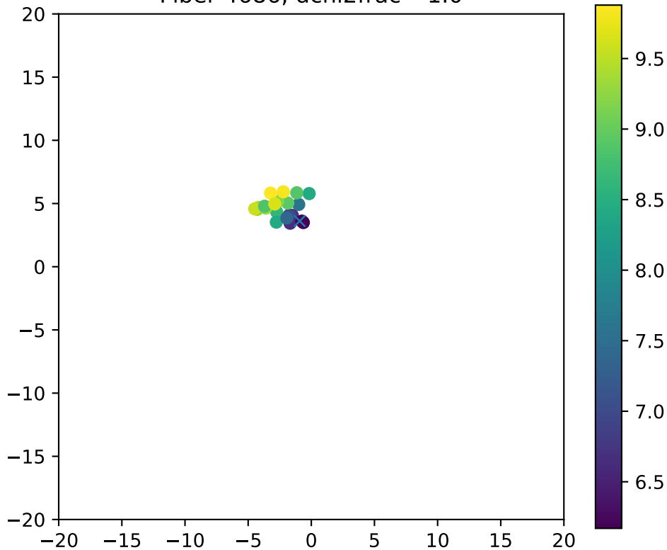
Fiber 4686, dchi2frac= 1.0
