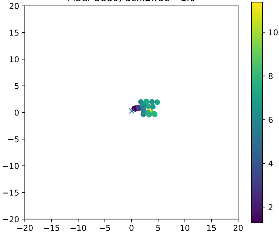
Fiber 3880, dchi2frac= 1.0
