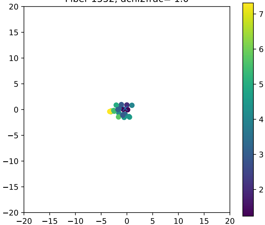
Fiber 1552, dchi2frac= 1.0
