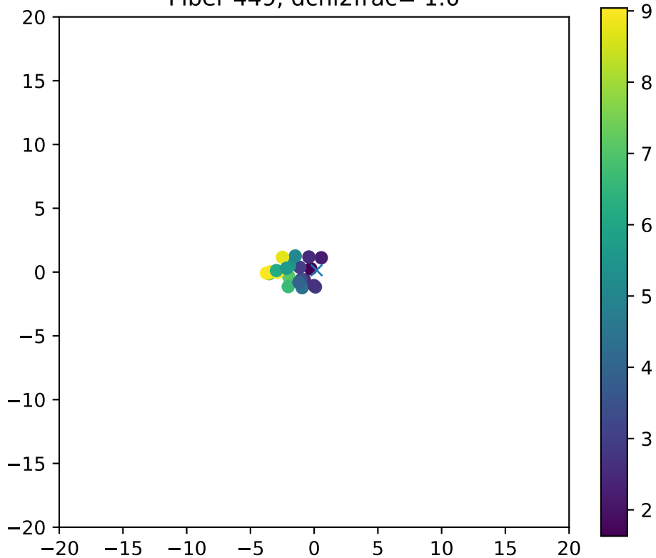
Fiber 449, dchi2frac= 1.0
