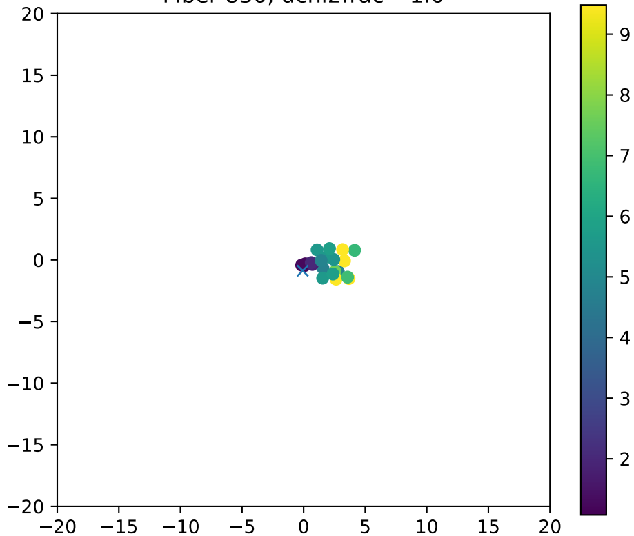
Fiber 830, dchi2frac= 1.0
