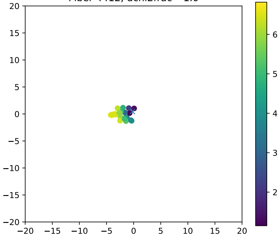
Fiber 4412, dchi2frac= 1.0
