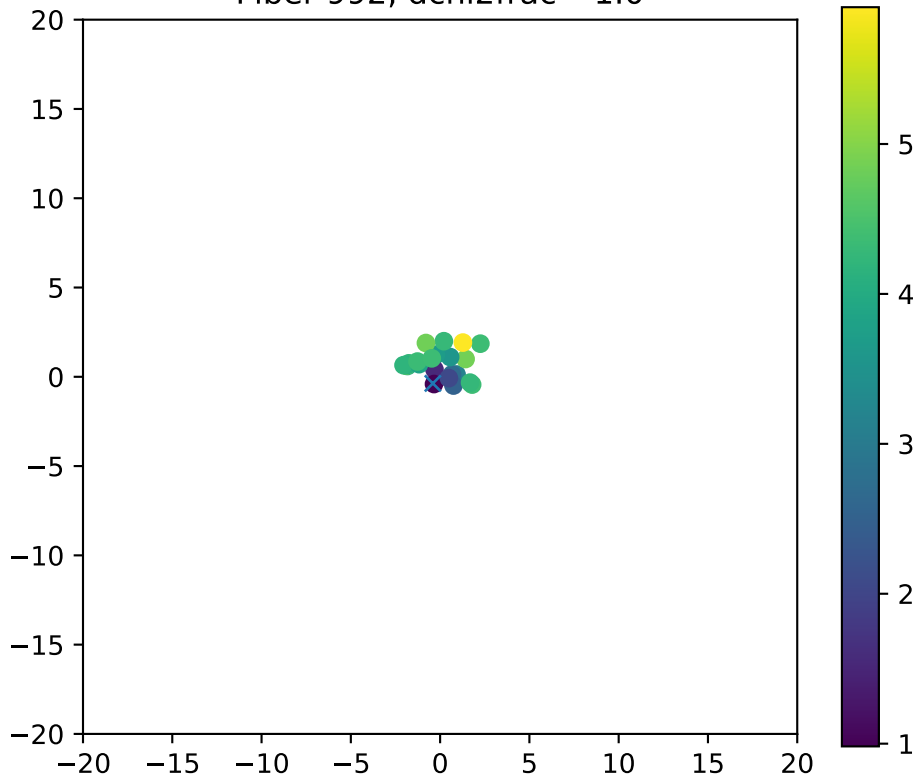
Fiber 992, dchi2frac= 1.0
