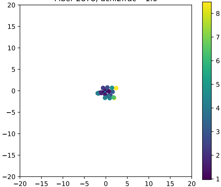
Fiber 2878, dchi2frac= 1.0
