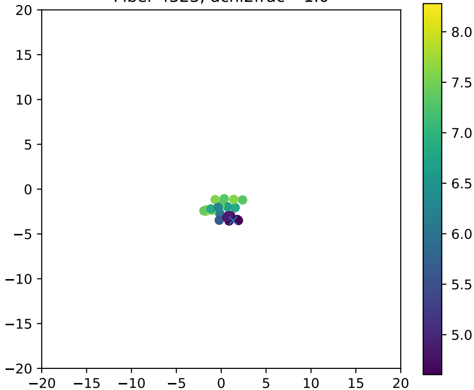
Fiber 4323, dchi2frac= 1.0
