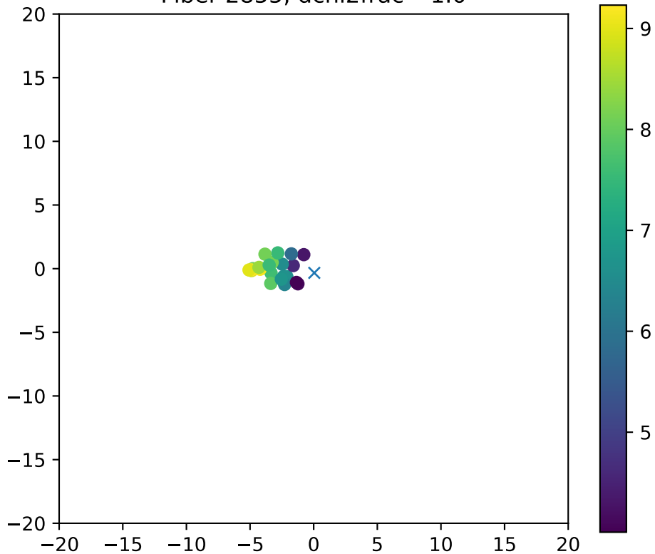
Fiber 2855, dchi2frac= 1.0
