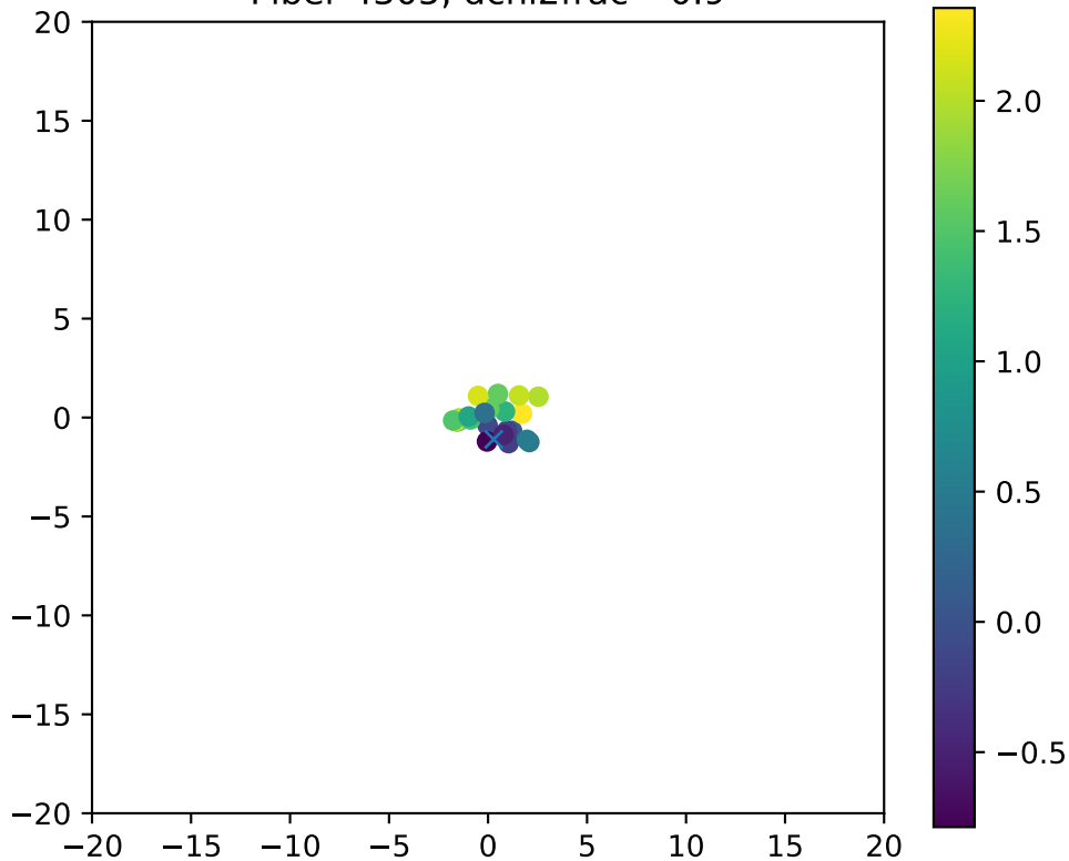
Fiber 4305, dchi2frac= 0.9
