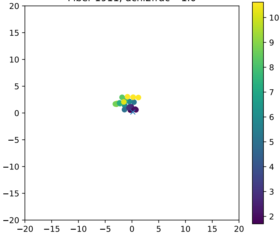
Fiber 1911, dchi2frac= 1.0
