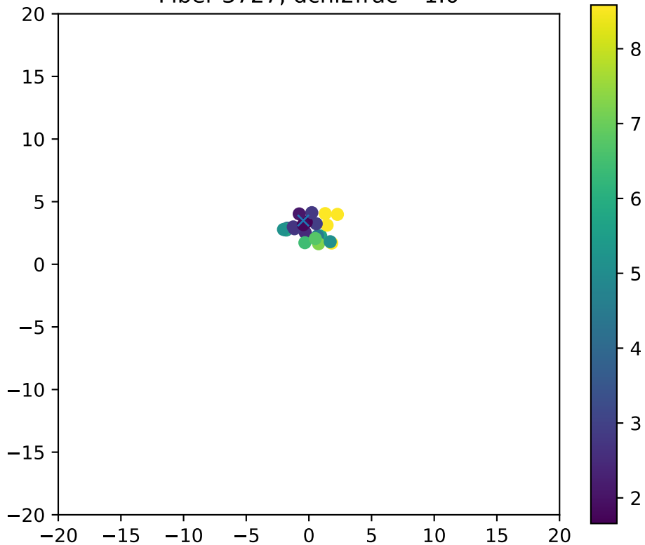
Fiber 3727, dchi2frac= 1.0
