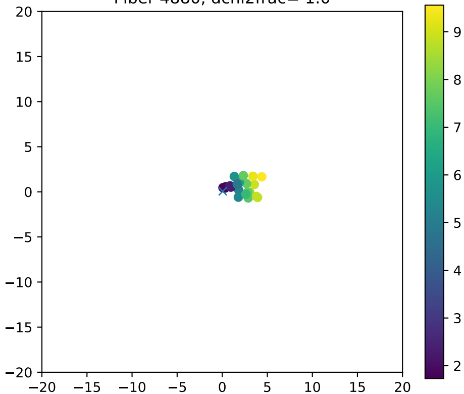
Fiber 4880, dchi2frac= 1.0
