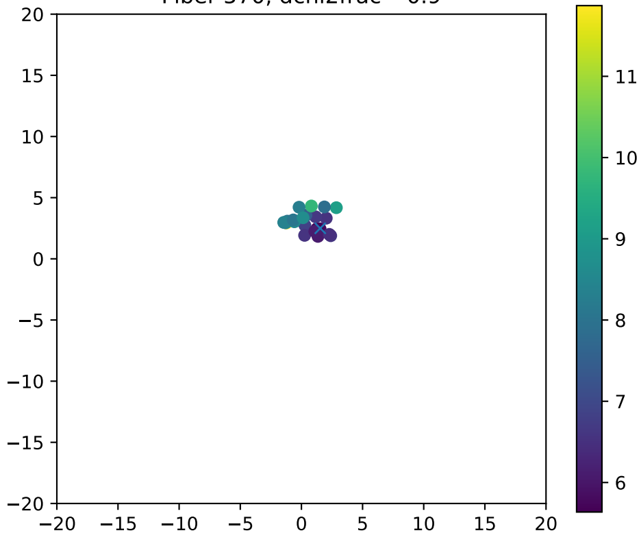
Fiber 570, dchi2frac= 0.9
