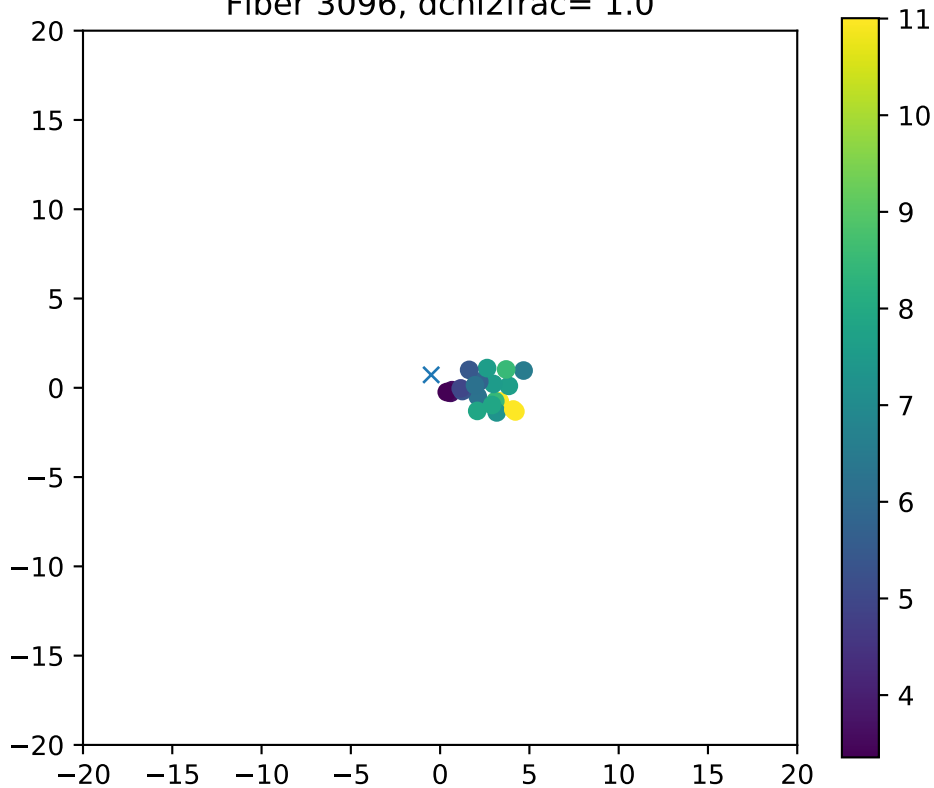
Fiber 3096, dchi2frac= 1.0
