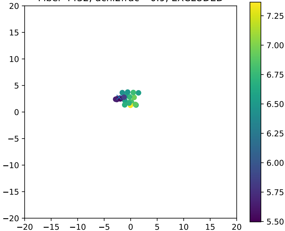
Fiber 4432, dchi2frac= 0.9, EXCLUDED
