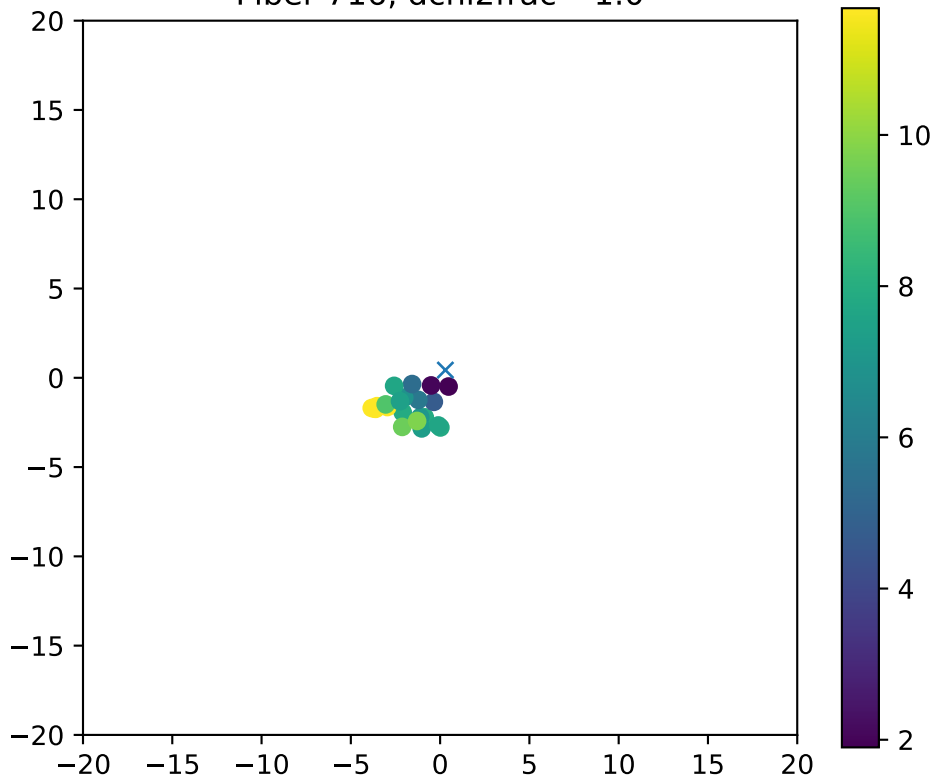
Fiber 716, dchi2frac= 1.0
