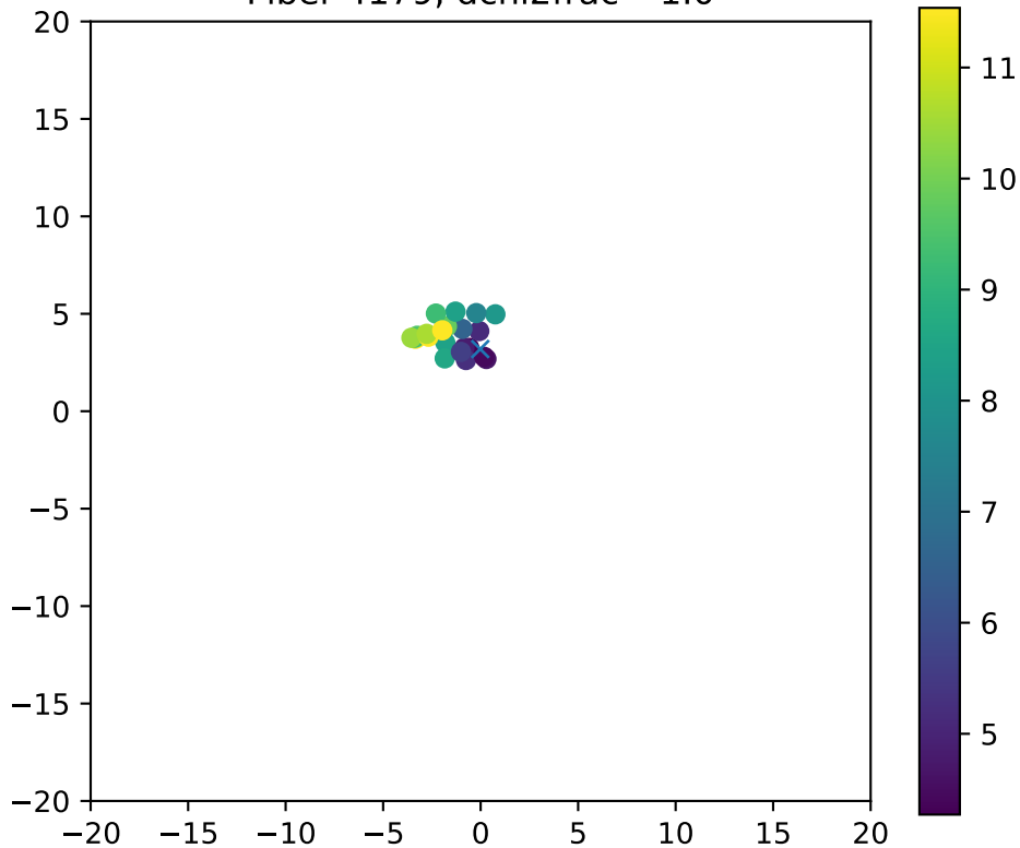
Fiber 4179, dchi2frac= 1.0
