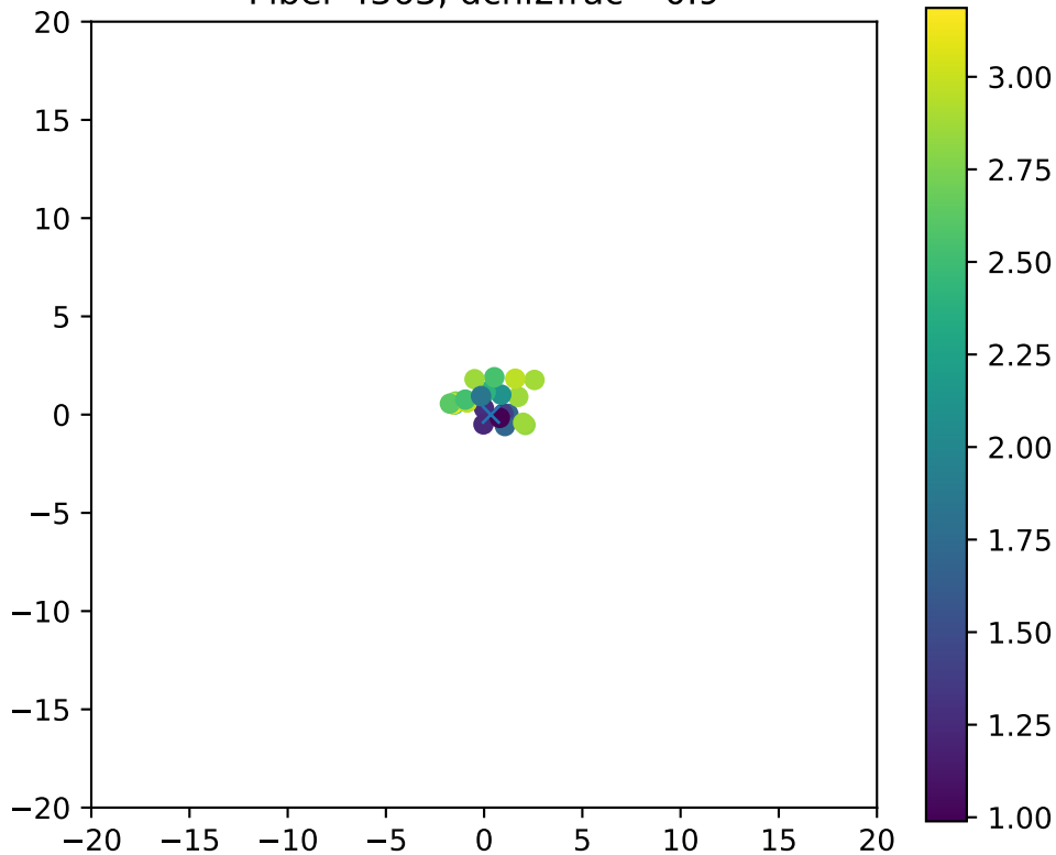
Fiber 4363, dchi2frac= 0.9
