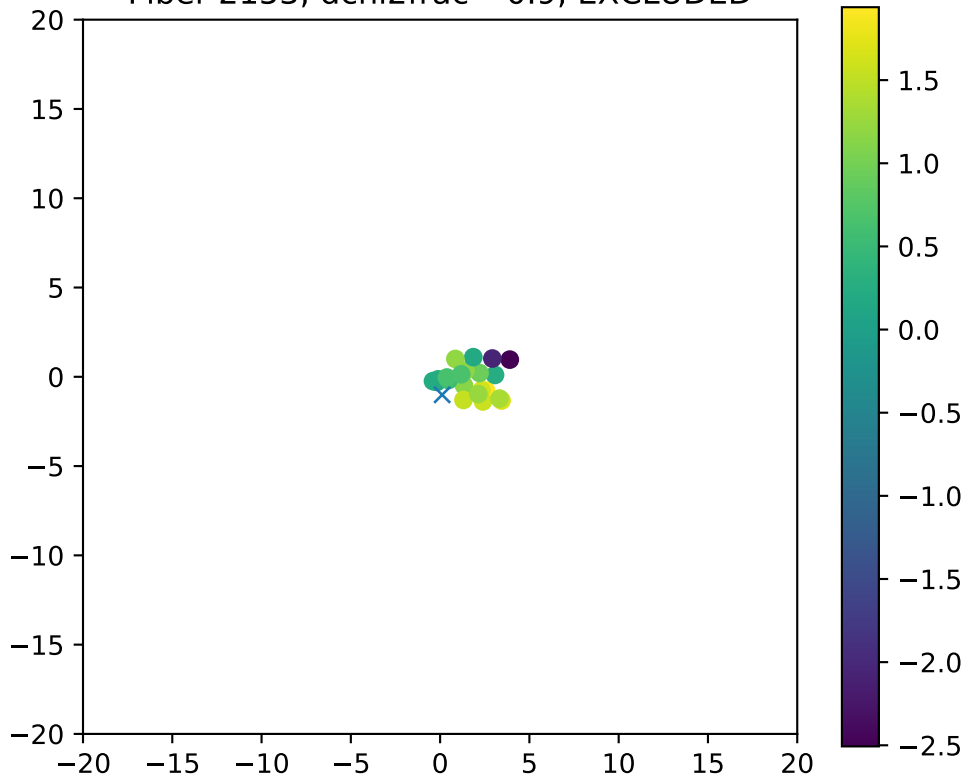
Fiber 2153, dchi2frac= 0.9, EXCLUDED
