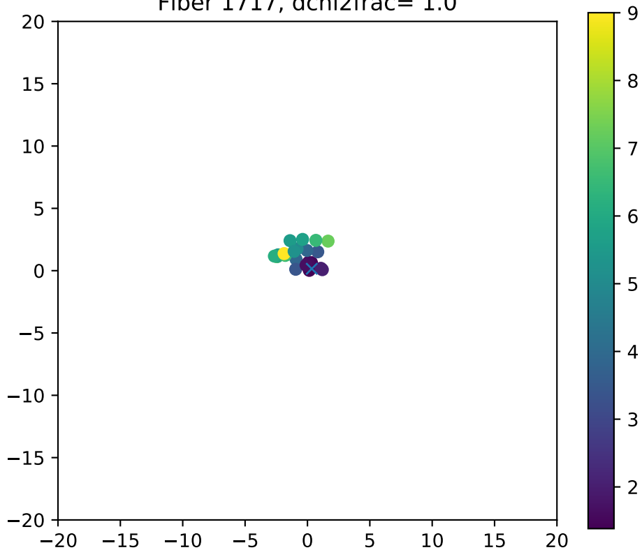
Fiber 1717, dchi2frac= 1.0
