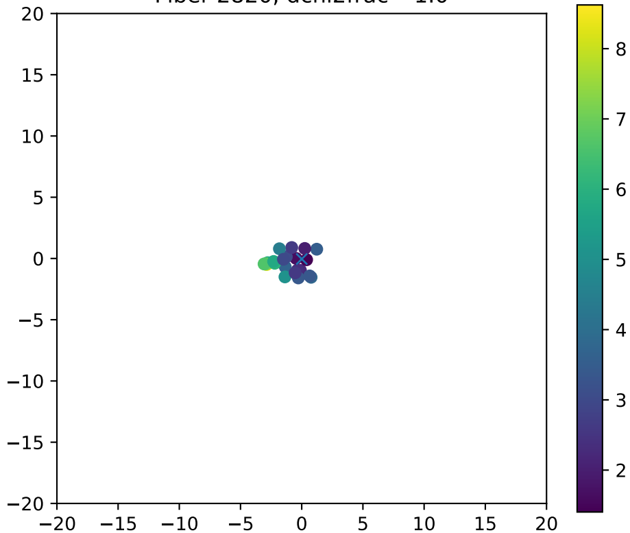
Fiber 2820, dchi2frac= 1.0
