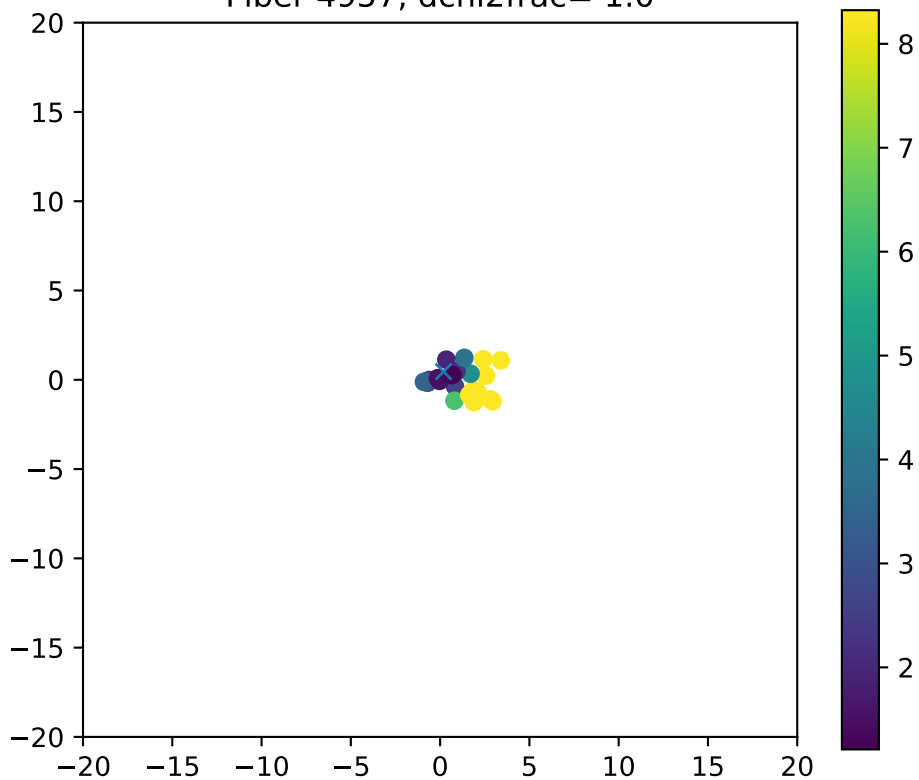
Fiber 4957, dchi2frac= 1.0
