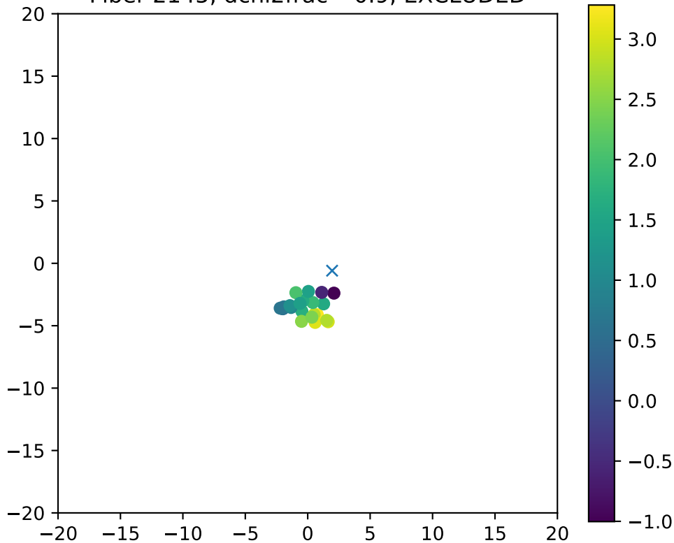
Fiber 2145, dchi2frac= 0.9, EXCLUDED
