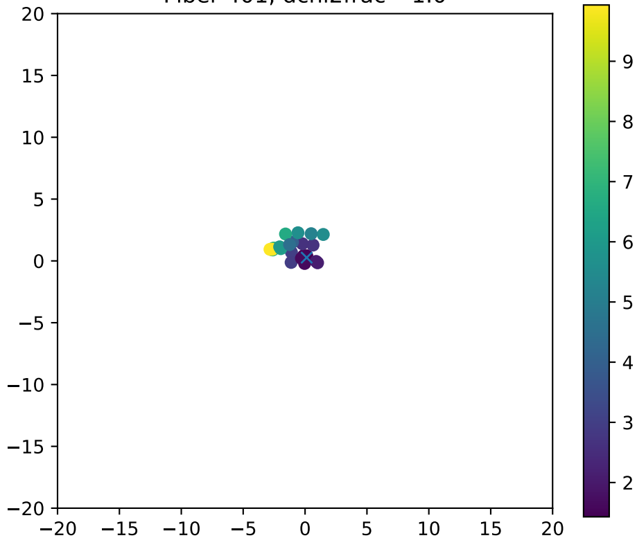
Fiber 401, dchi2frac= 1.0
