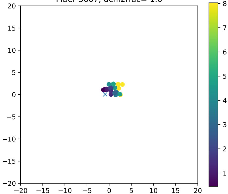
Fiber 3607, dchi2frac= 1.0
