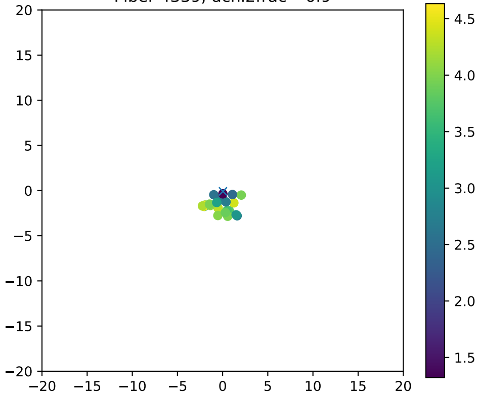
Fiber 4339, dchi2frac= 0.9
