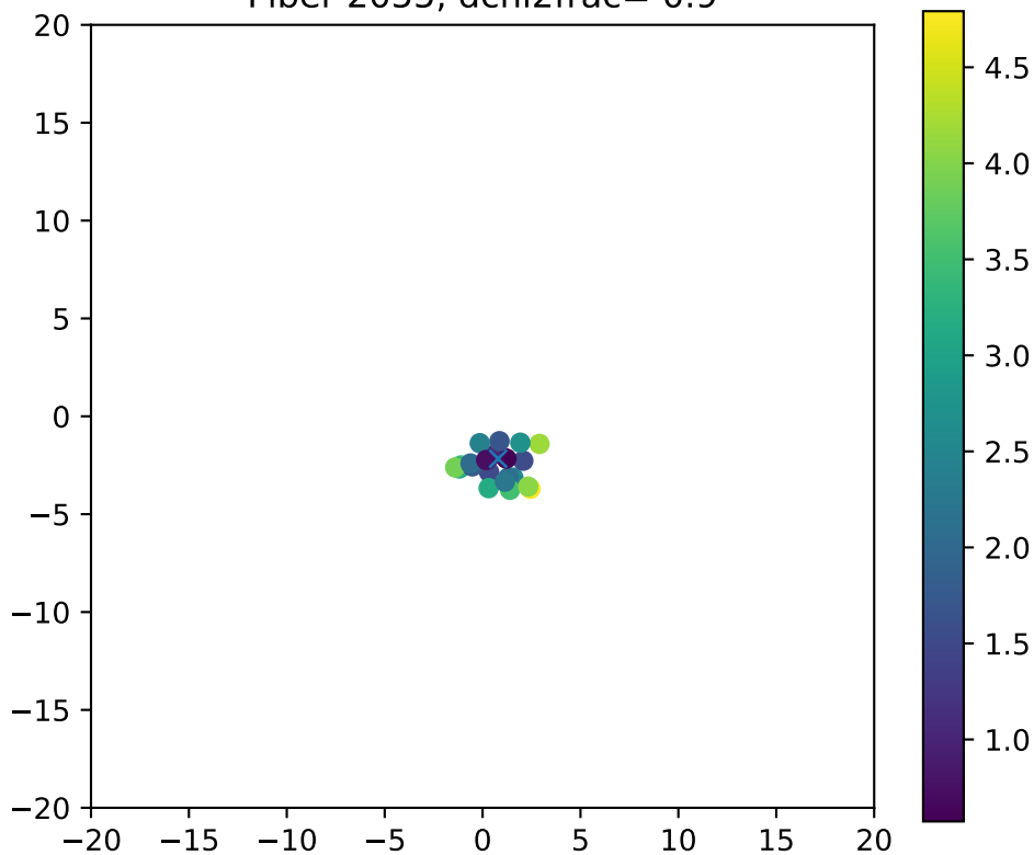
Fiber 2055, dchi2frac= 0.9
