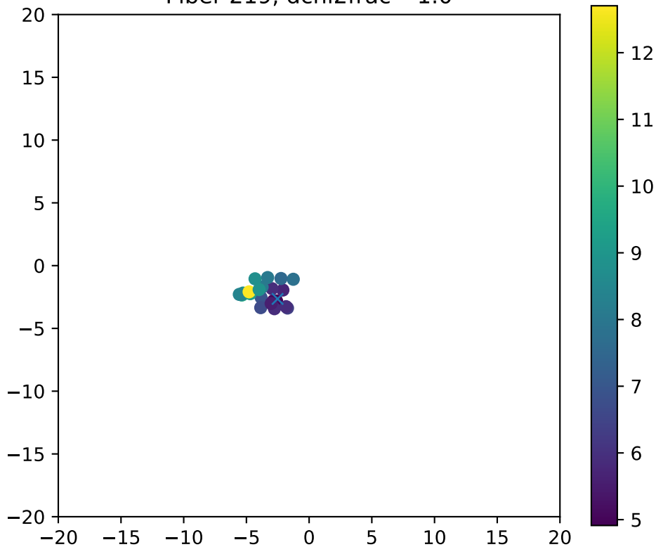
Fiber 219, dchi2frac= 1.0
