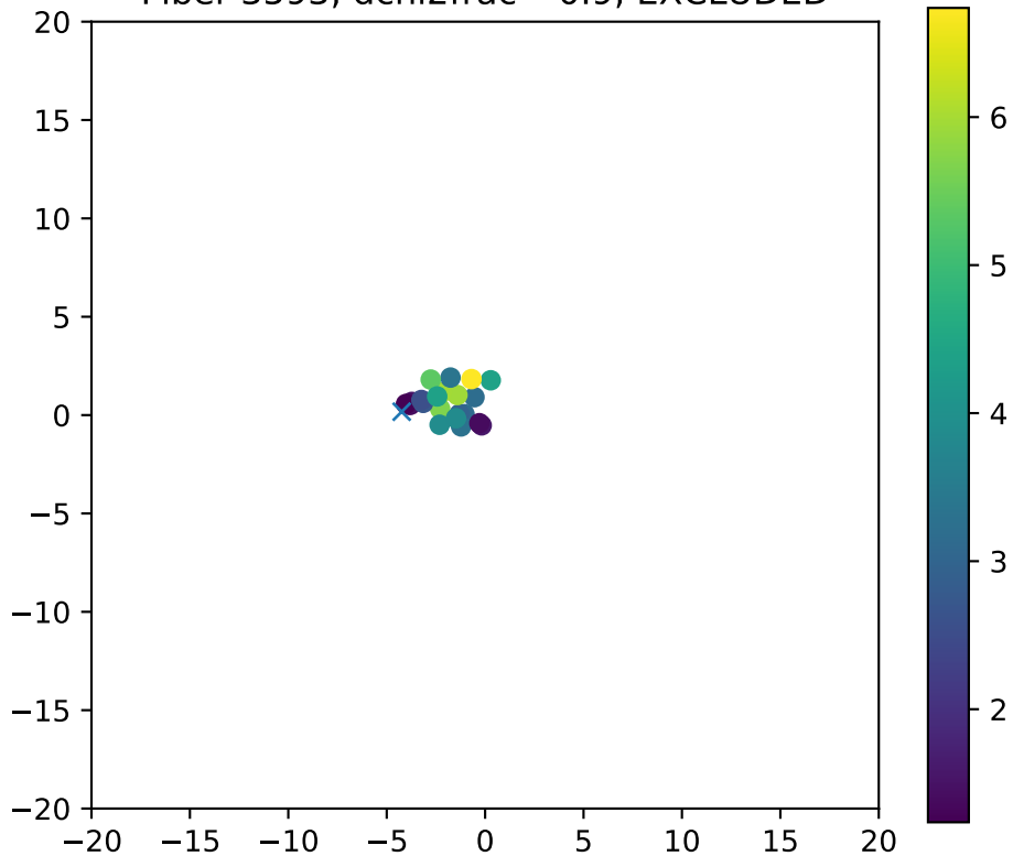
Fiber 3593, dchi2frac= 0.9, EXCLUDED
