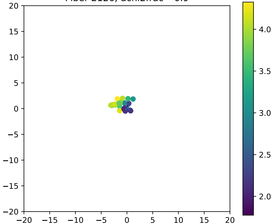
Fiber 2126, dchi2frac= 0.9
