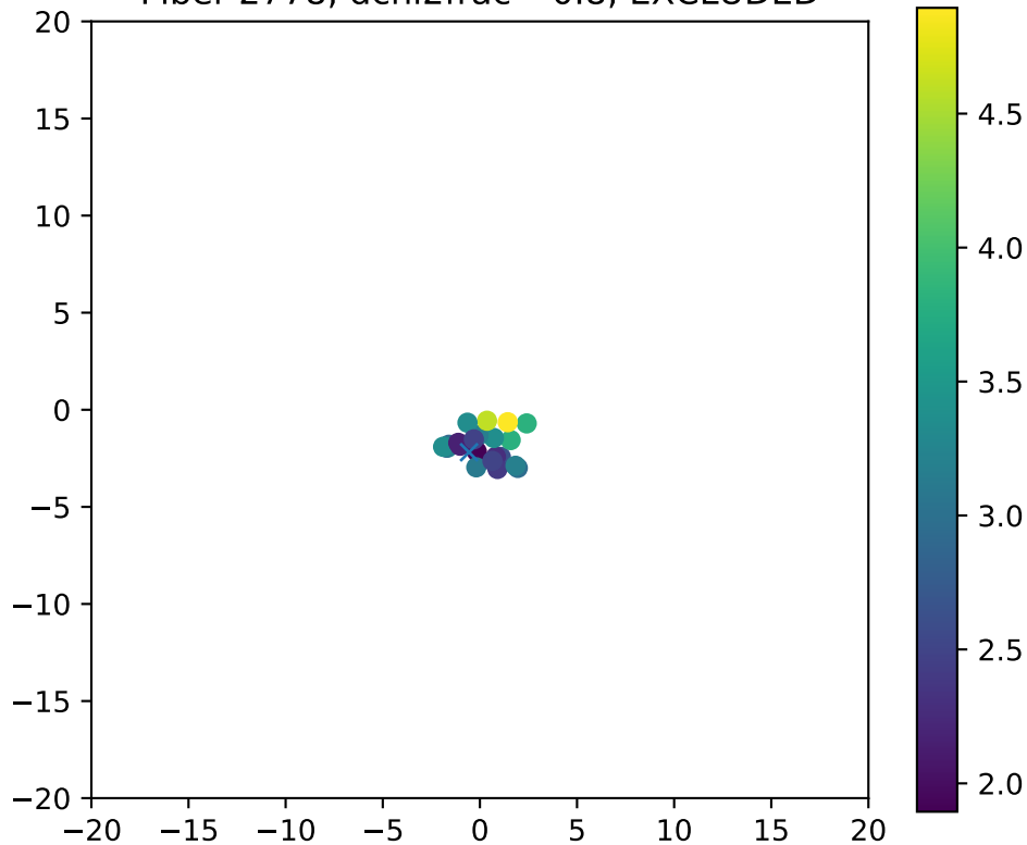
Fiber 2778, dchi2frac= 0.8, EXCLUDED
