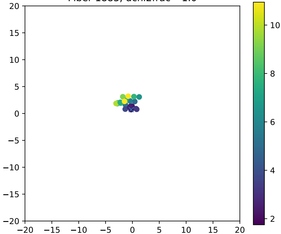
Fiber 1883, dchi2frac= 1.0
