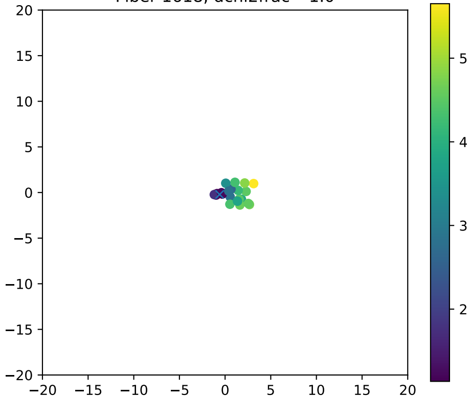
Fiber 1618, dchi2frac= 1.0
