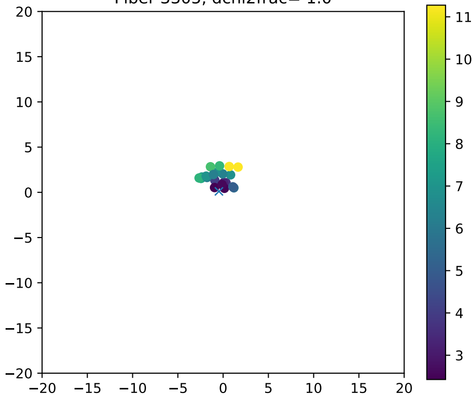
Fiber 3305, dchi2frac= 1.0
