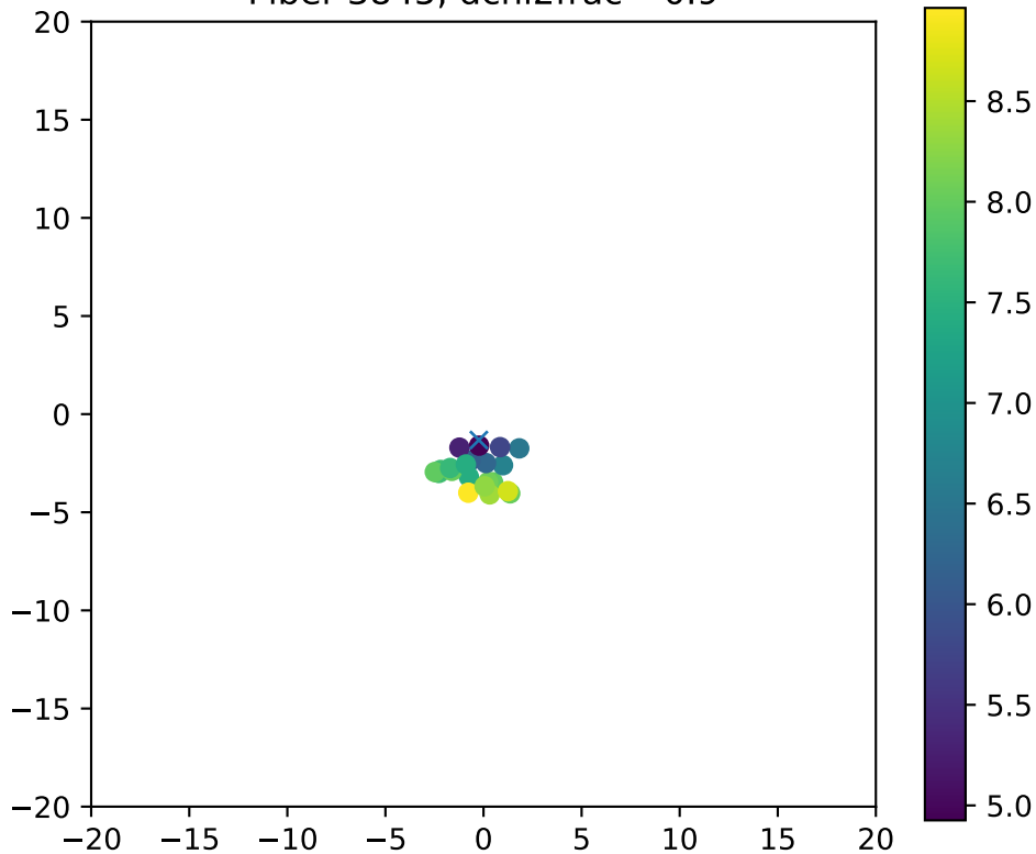
Fiber 3845, dchi2frac= 0.9
