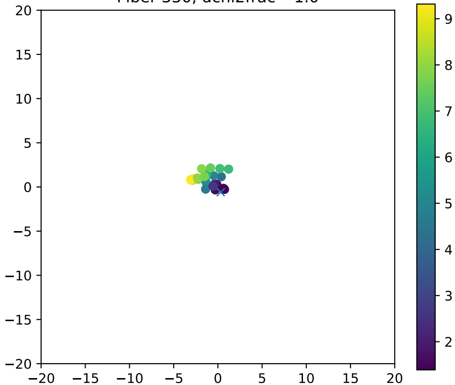
Fiber 330, dchi2frac= 1.0
