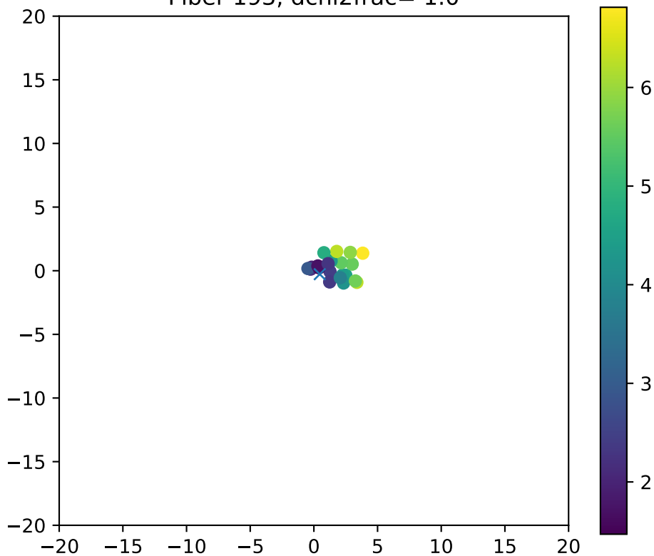
Fiber 193, dchi2frac= 1.0
