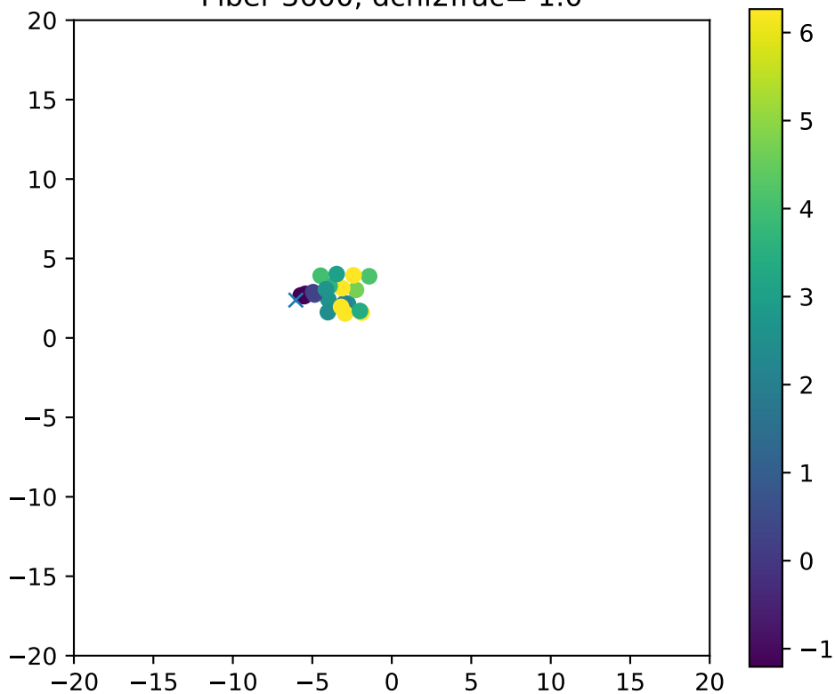
Fiber 3600, dchi2frac= 1.0
