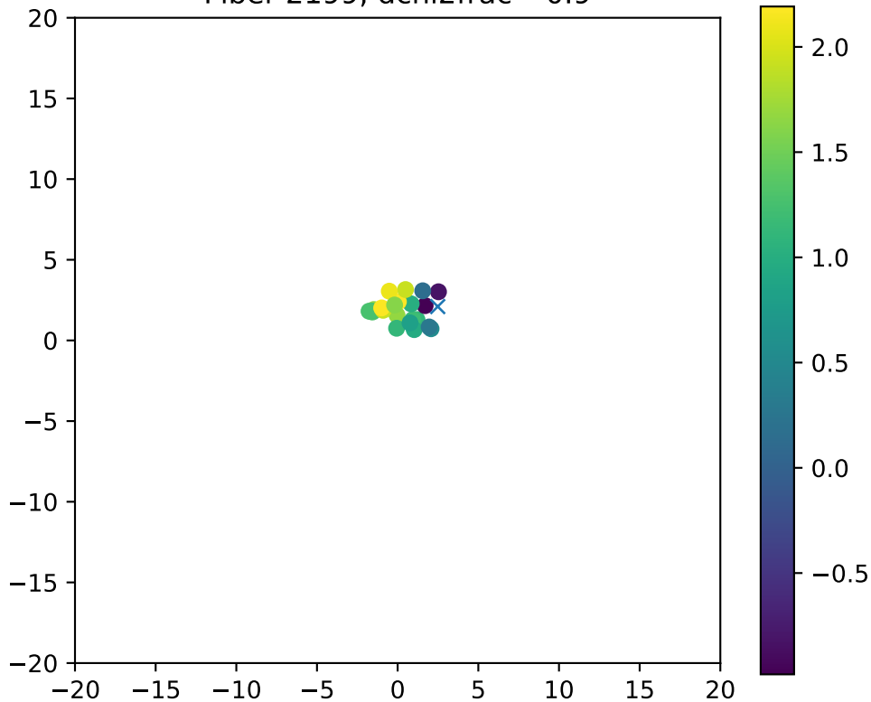
Fiber 2199, dchi2frac= 0.9
