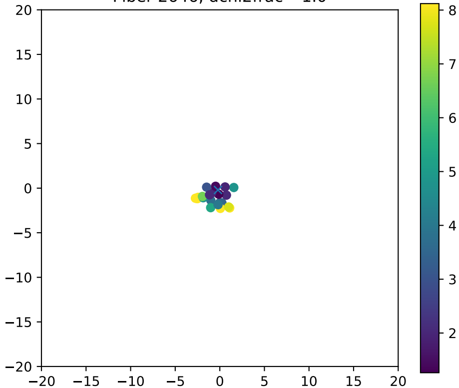
Fiber 2646, dchi2frac= 1.0
