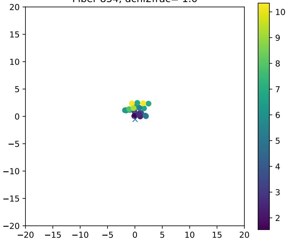
Fiber 854, dchi2frac= 1.0
