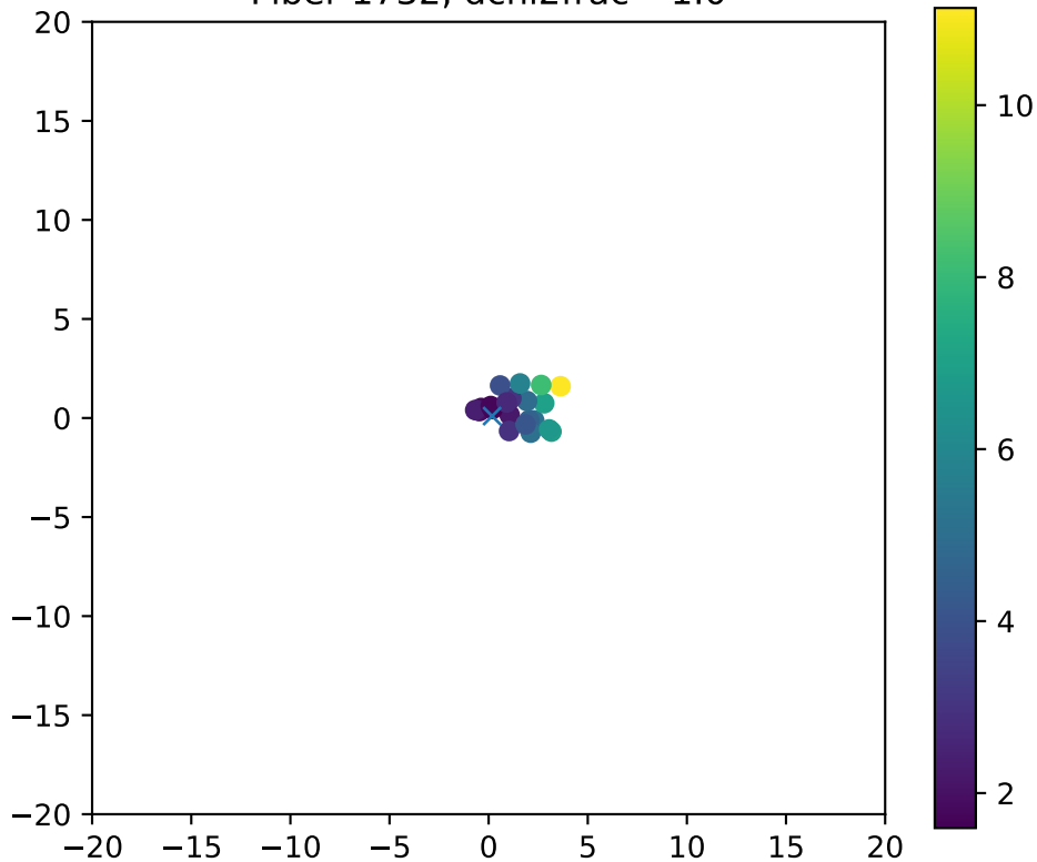
Fiber 1732, dchi2frac= 1.0
