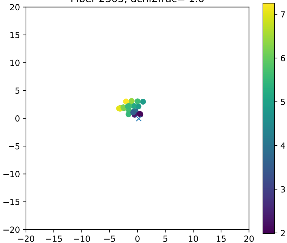
Fiber 2305, dchi2frac= 1.0
