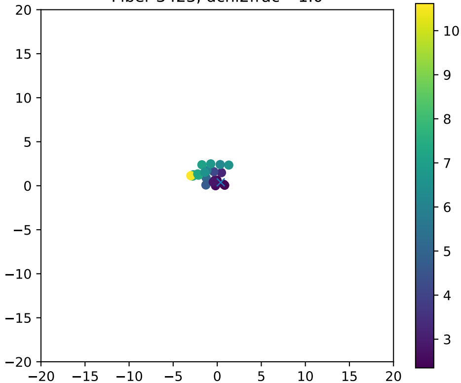
Fiber 3423, dchi2frac= 1.0
