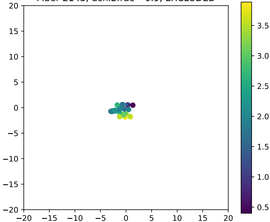
Fiber 2143, dchi2frac= 0.9, EXCLUDED
