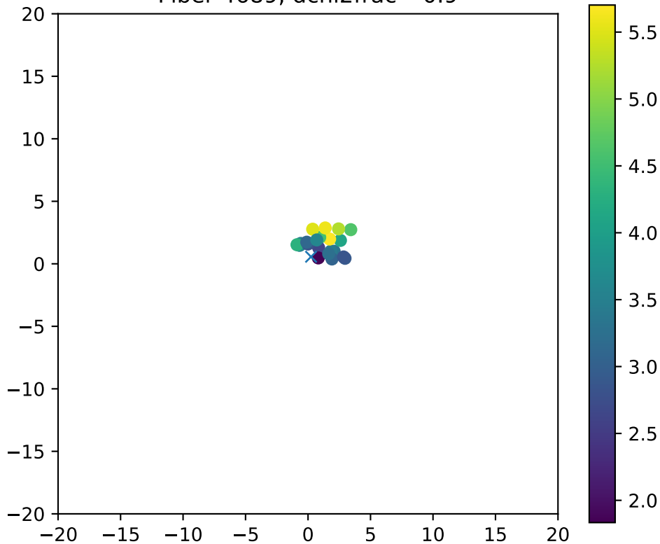
Fiber 4689, dchi2frac= 0.9
