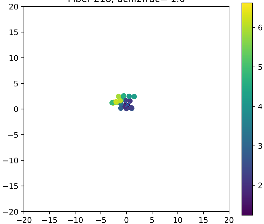
Fiber 218, dchi2frac= 1.0
