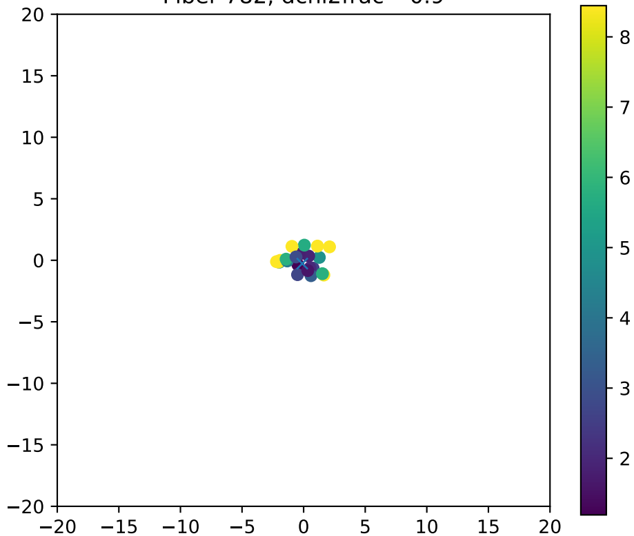
Fiber 782, dchi2frac= 0.9
