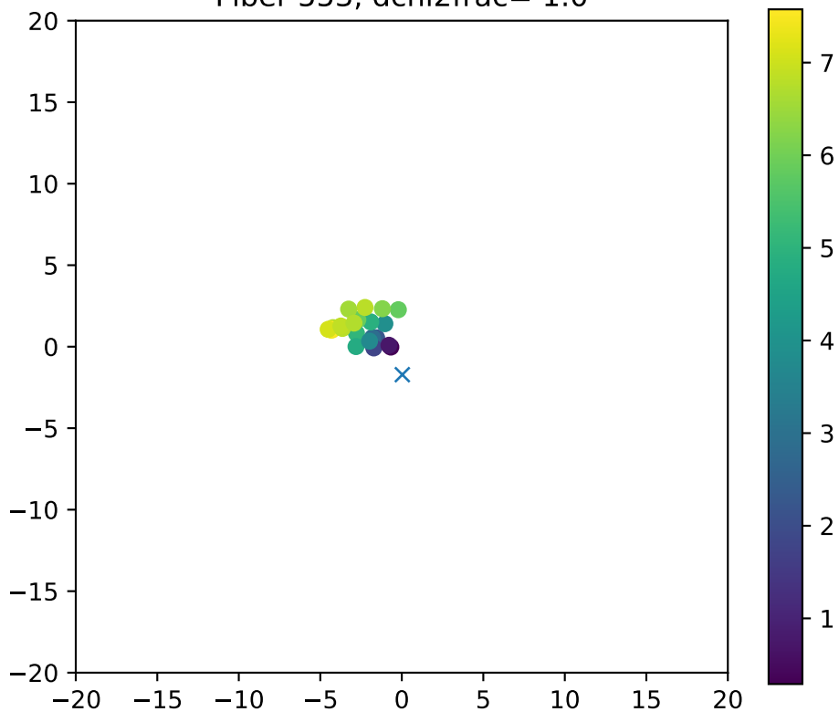
Fiber 553, dchi2frac= 1.0
