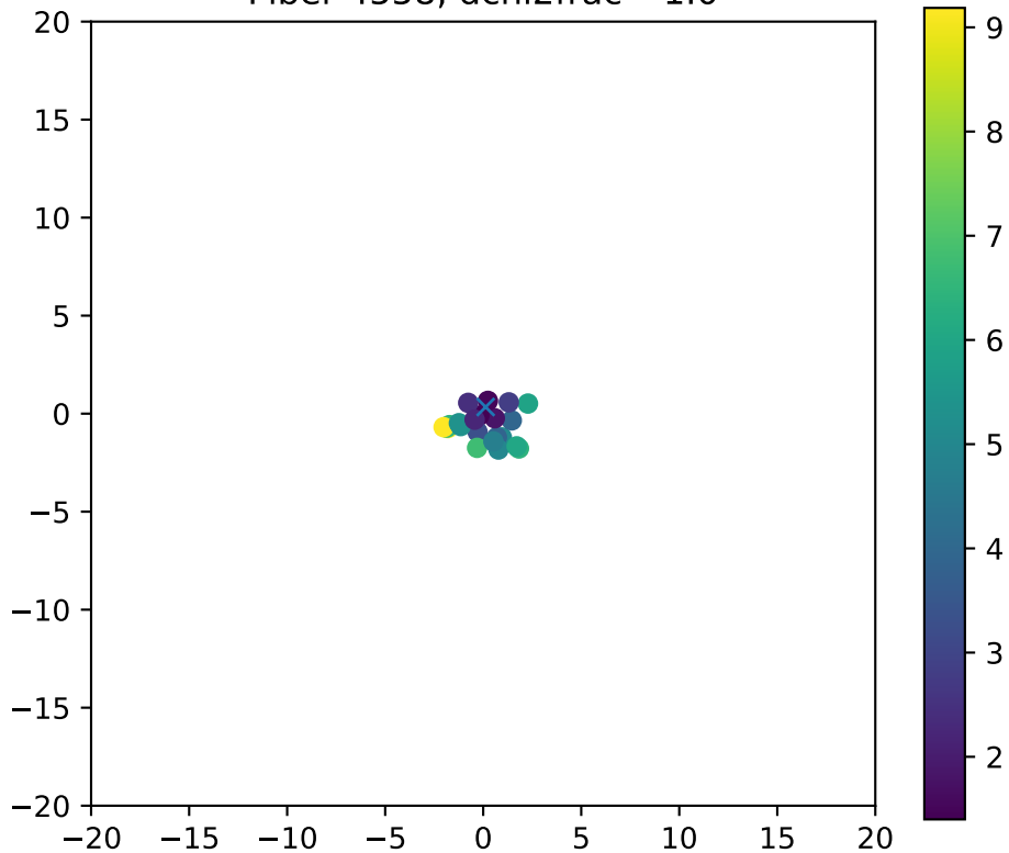
Fiber 4558, dchi2frac= 1.0
