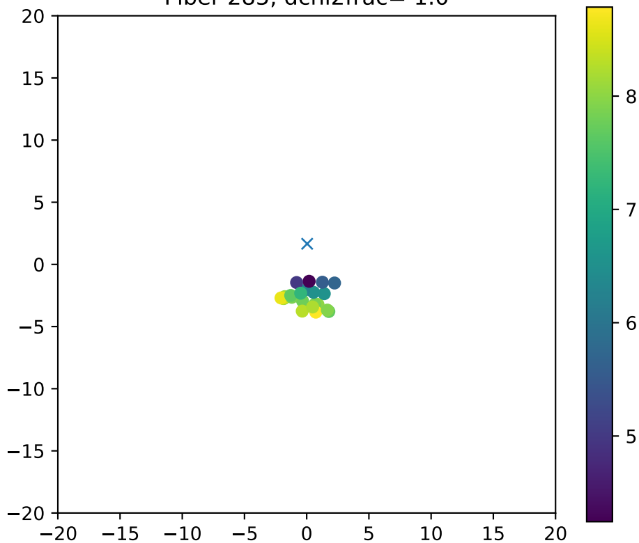
Fiber 285, dchi2frac= 1.0
