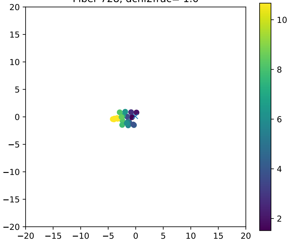
Fiber 728, dchi2frac= 1.0
