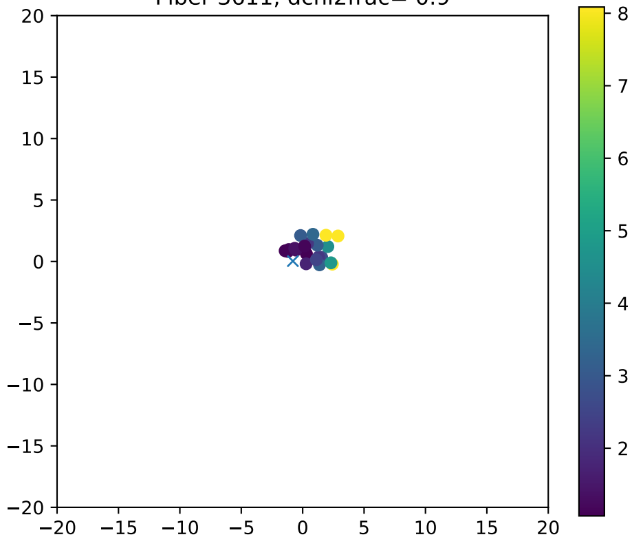
Fiber 3611, dchi2frac= 0.9
