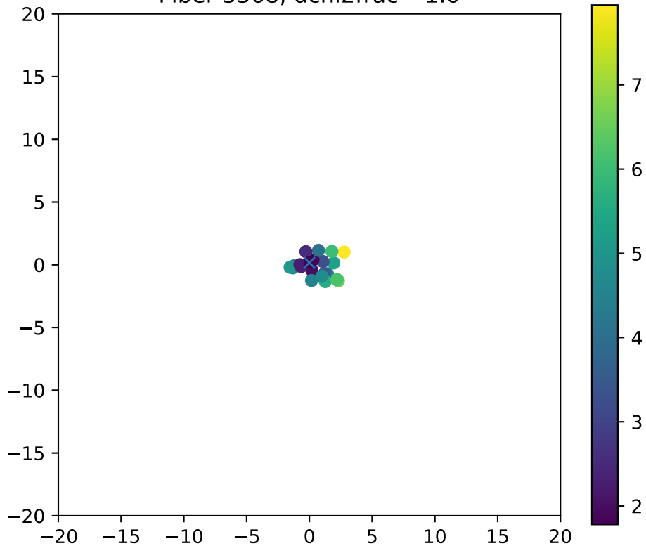
Fiber 3368, dchi2frac= 1.0
