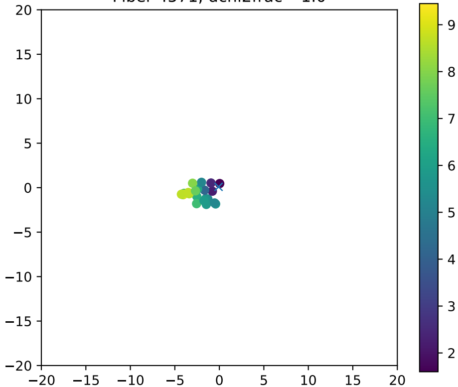
Fiber 4571, dchi2frac= 1.0
