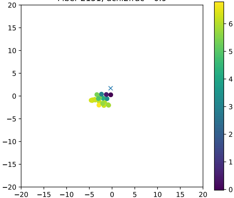
Fiber 2151, dchi2frac= 0.9
