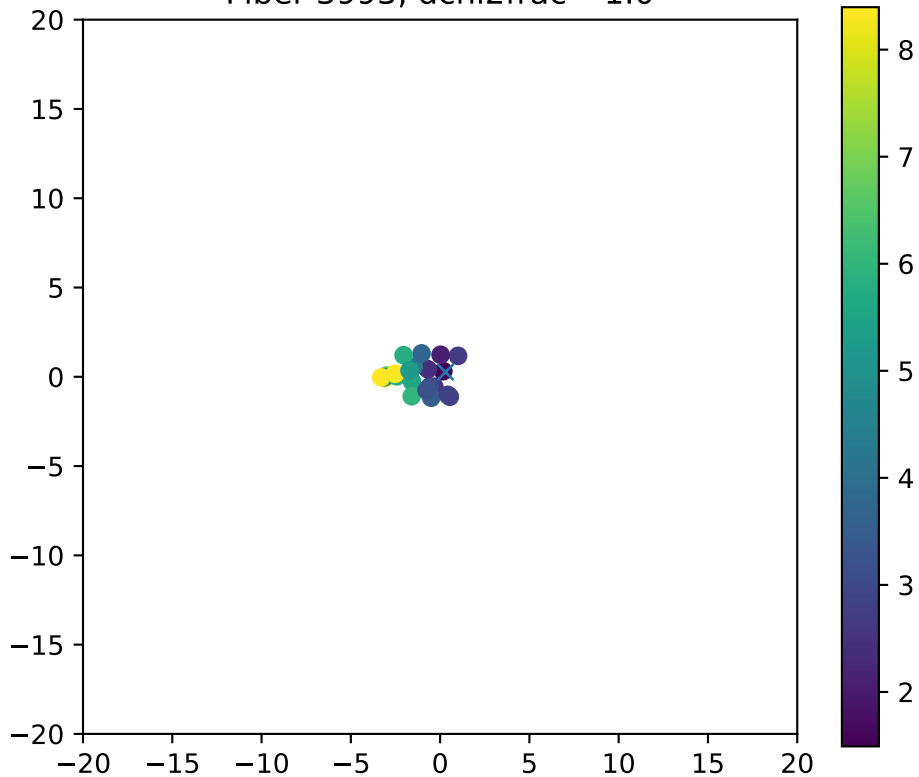
Fiber 3993, dchi2frac= 1.0
