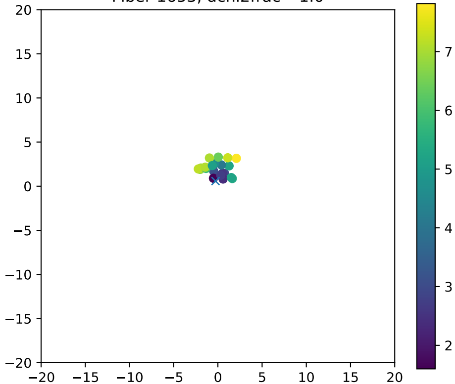
Fiber 1653, dchi2frac= 1.0
