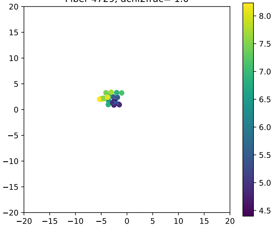
Fiber 4729, dchi2frac= 1.0
