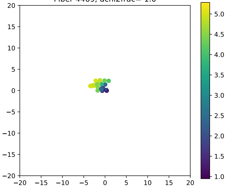
Fiber 4469, dchi2frac= 1.0
