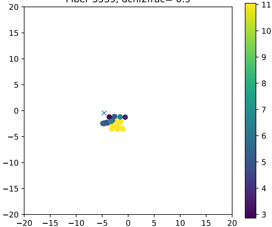
Fiber 3539, dchi2frac= 0.9
