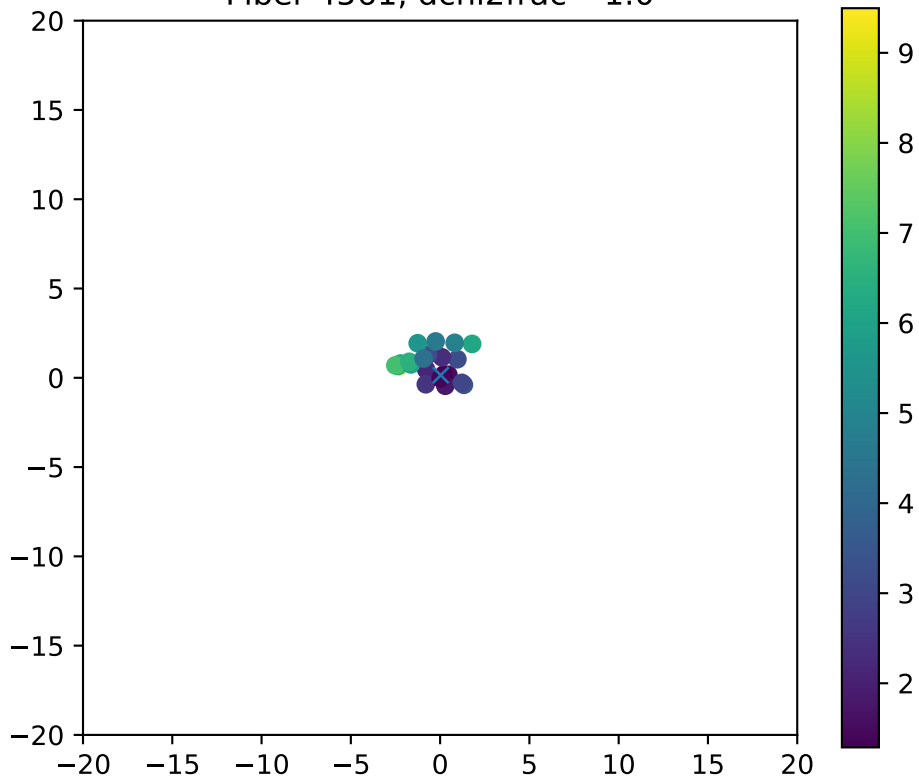
Fiber 4561, dchi2frac= 1.0
