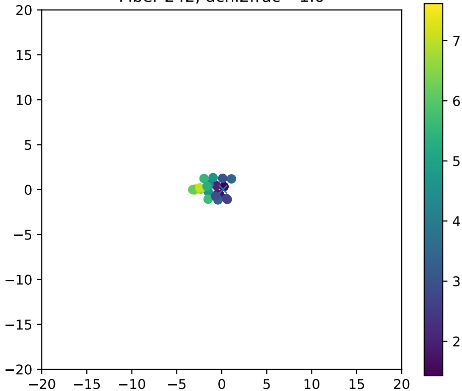
Fiber 242, dchi2frac= 1.0
