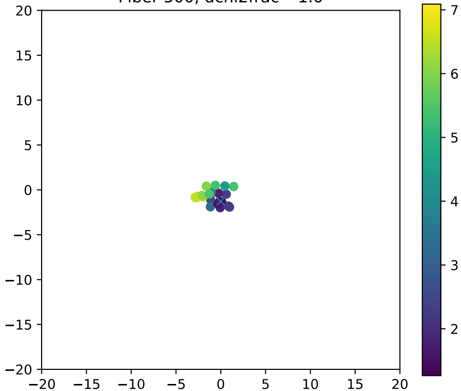
Fiber 500, dchi2frac= 1.0
