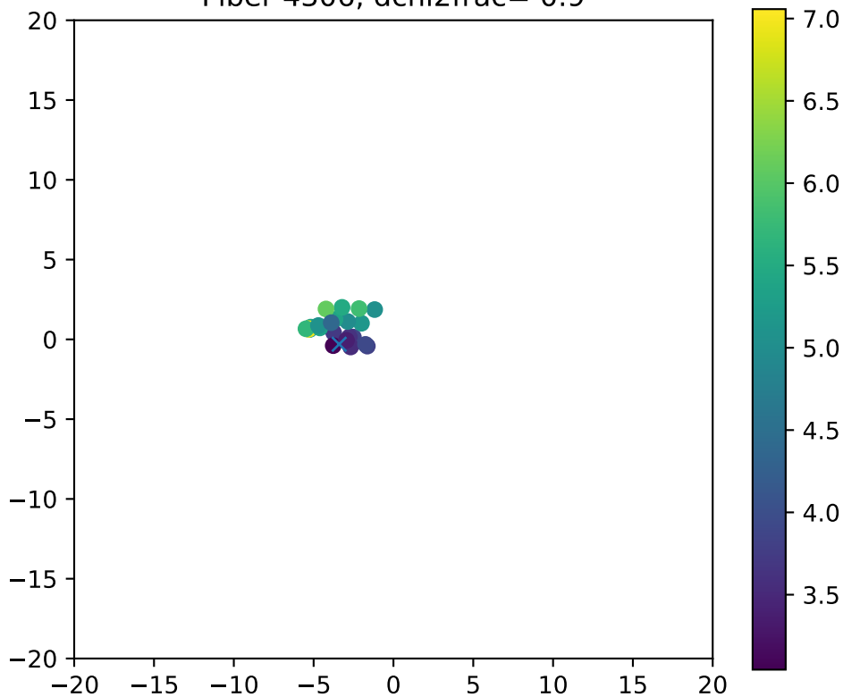
Fiber 4306, dchi2frac= 0.9
