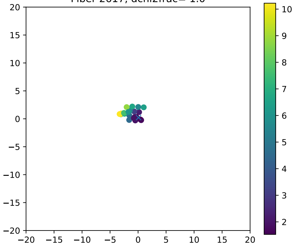
Fiber 2617, dchi2frac= 1.0
