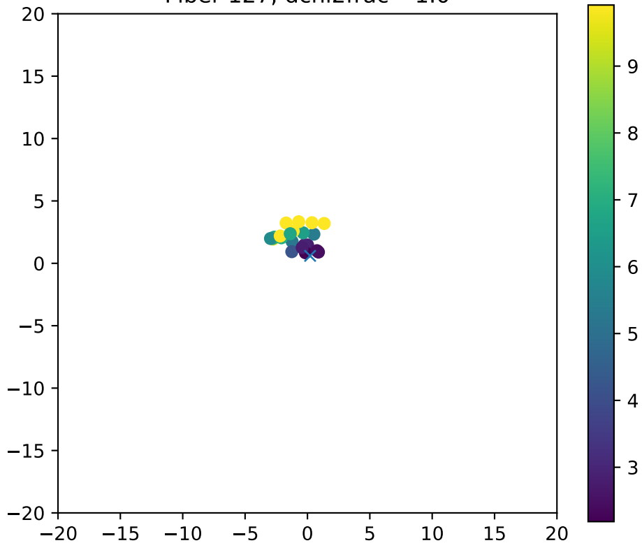
Fiber 127, dchi2frac= 1.0
