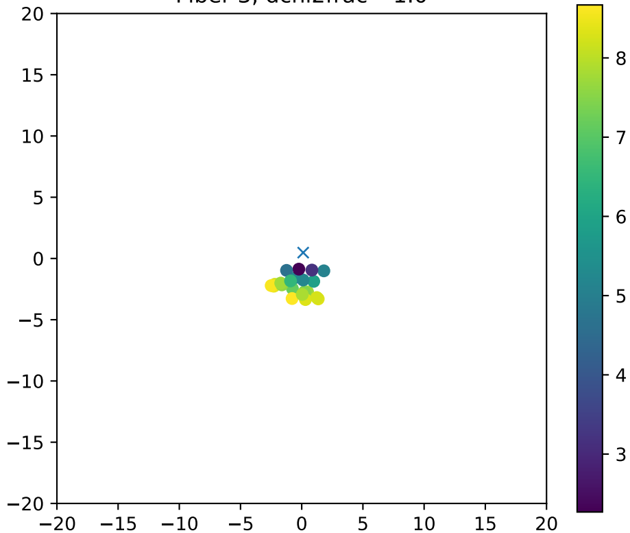
Fiber 3, dchi2frac= 1.0
