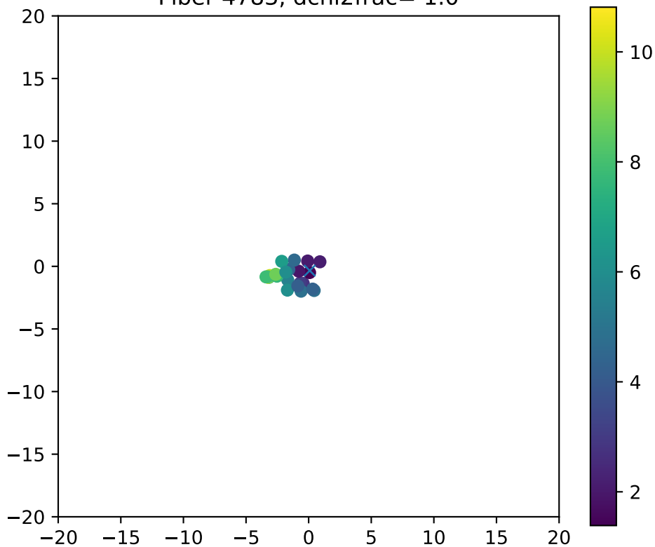
Fiber 4783, dchi2frac= 1.0
