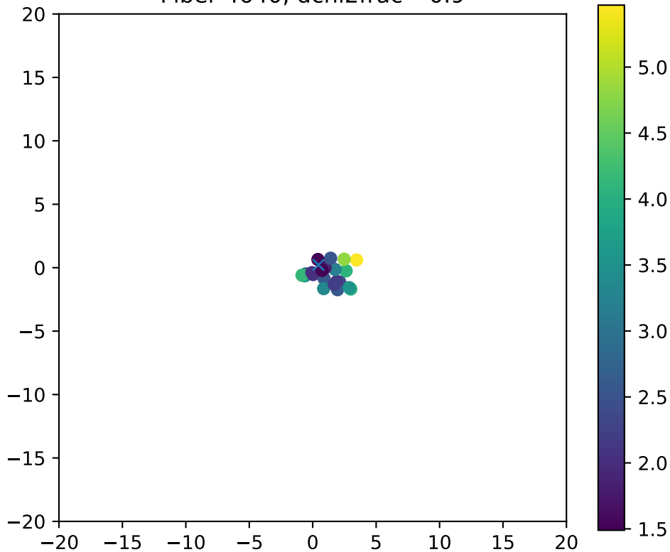
Fiber 4640, dchi2frac= 0.9
