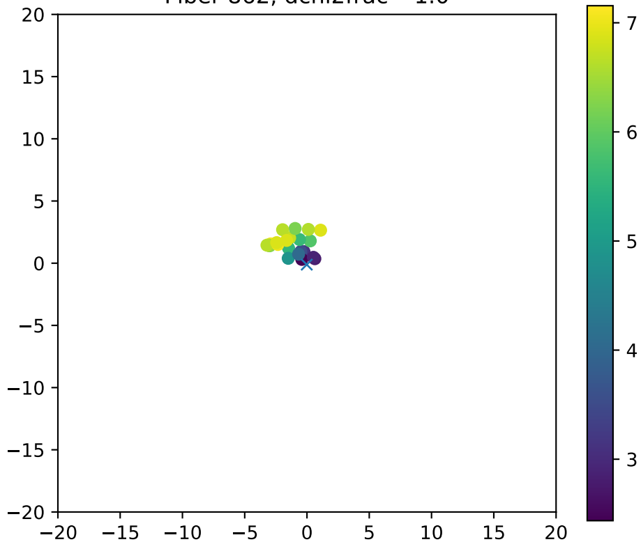
Fiber 862, dchi2frac= 1.0
