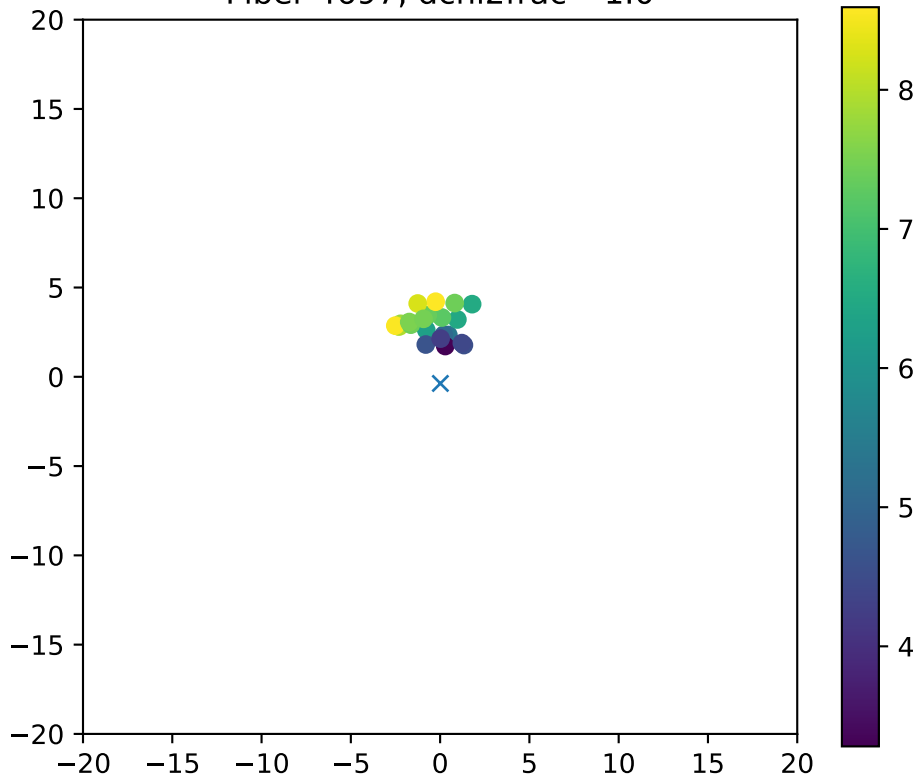
Fiber 4697, dchi2frac= 1.0
