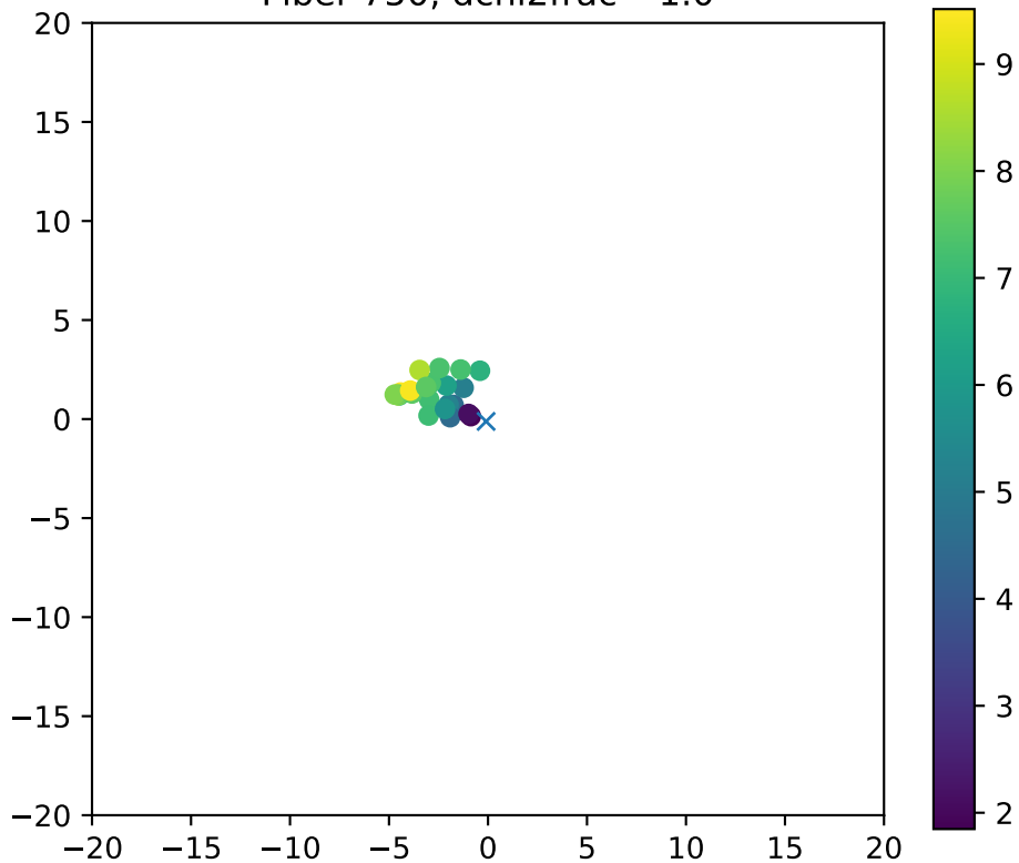
Fiber 750, dchi2frac= 1.0
