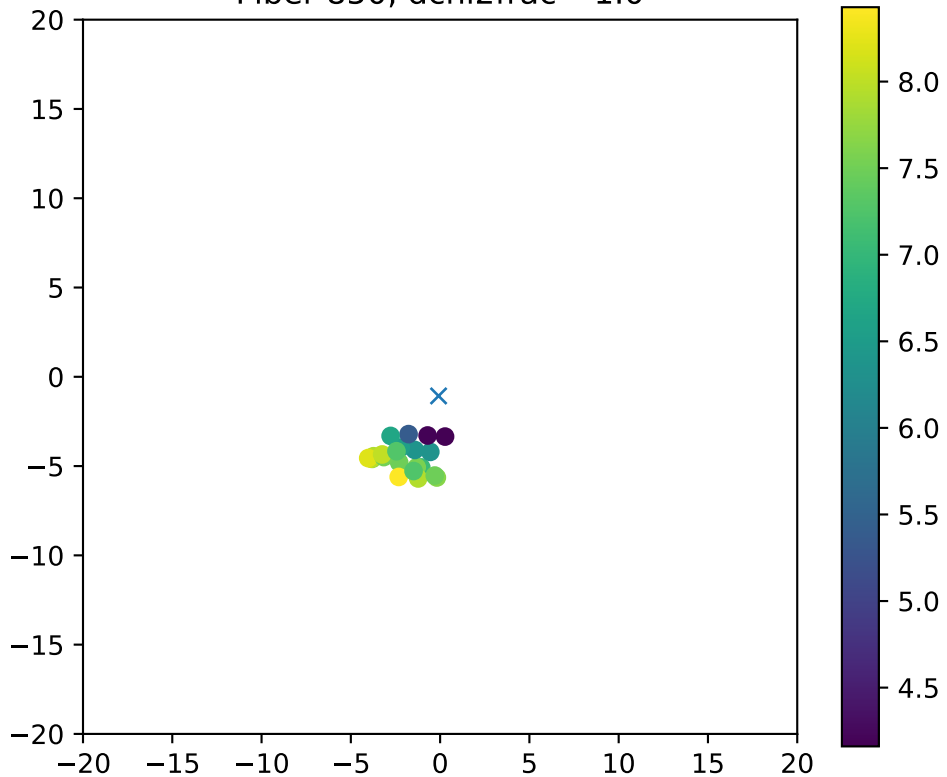
Fiber 850, dchi2frac= 1.0
