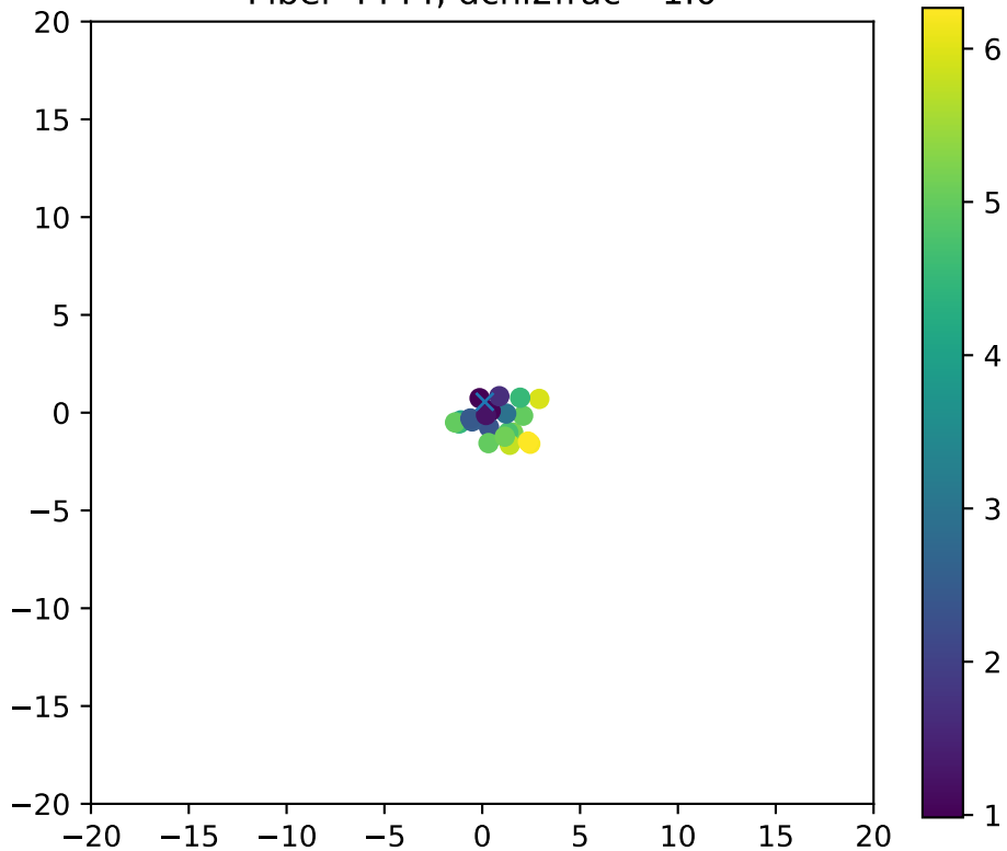
Fiber 4444, dchi2frac= 1.0
