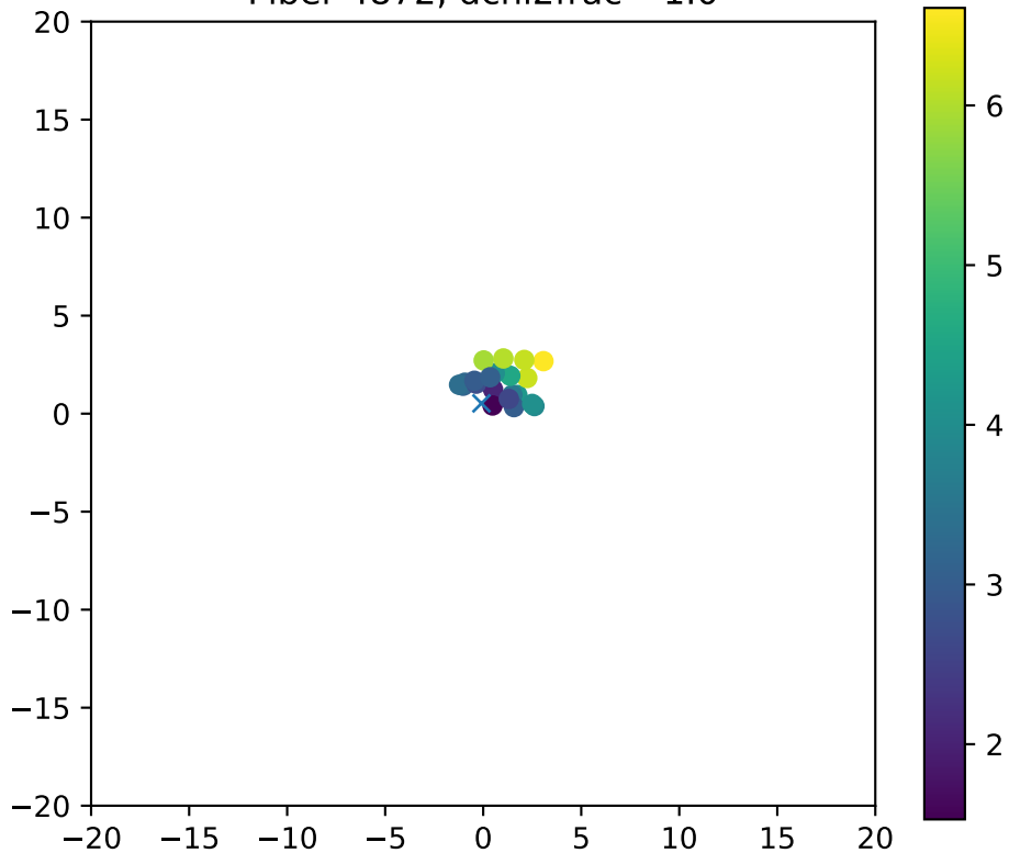
Fiber 4872, dchi2frac= 1.0
