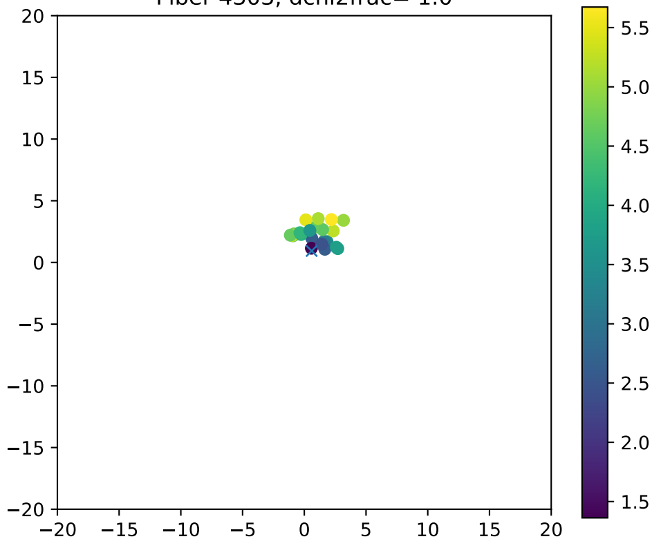
Fiber 4303, dchi2frac= 1.0
