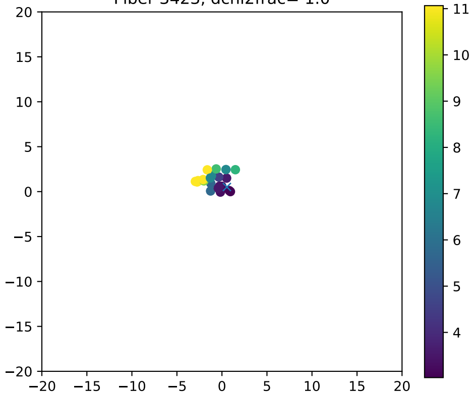
Fiber 3423, dchi2frac= 1.0
