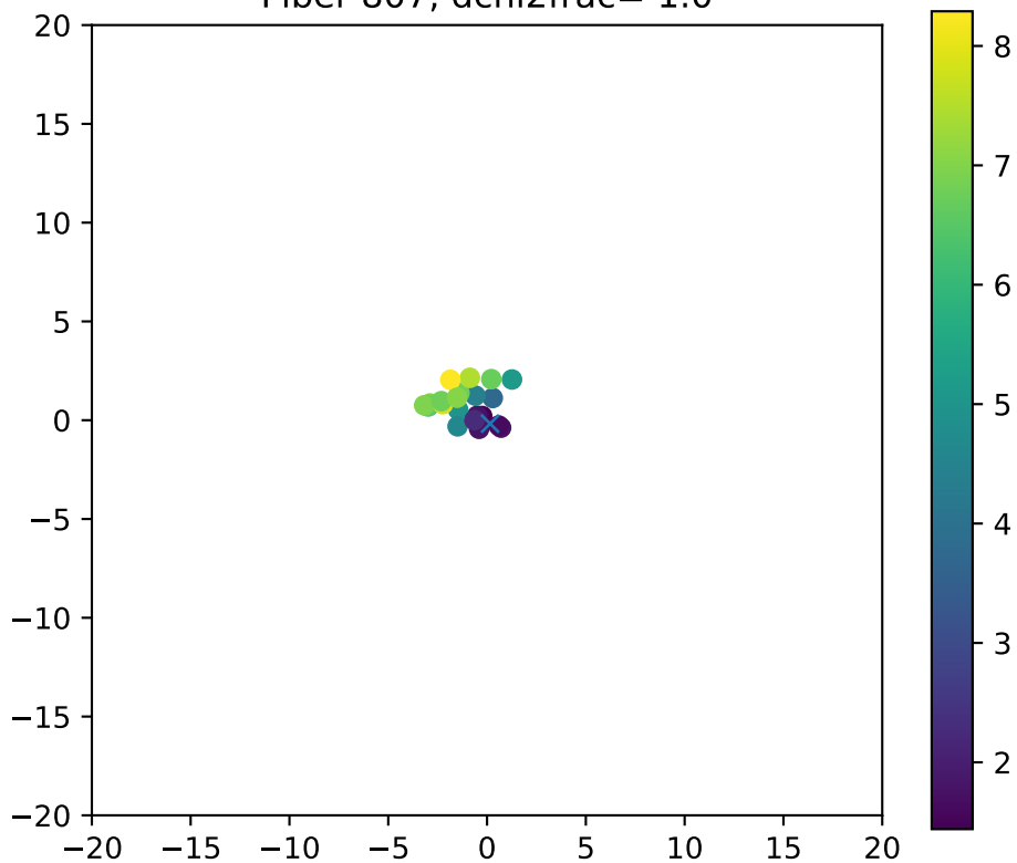
Fiber 807, dchi2frac= 1.0
