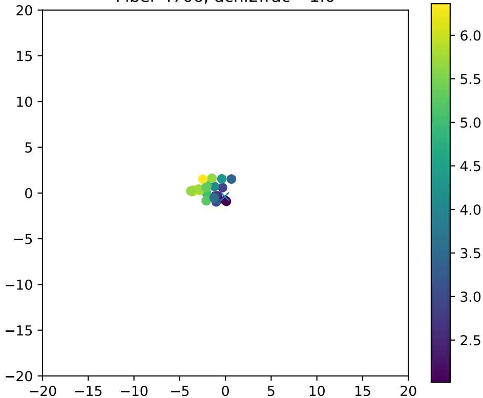
Fiber 4706, dchi2frac= 1.0
