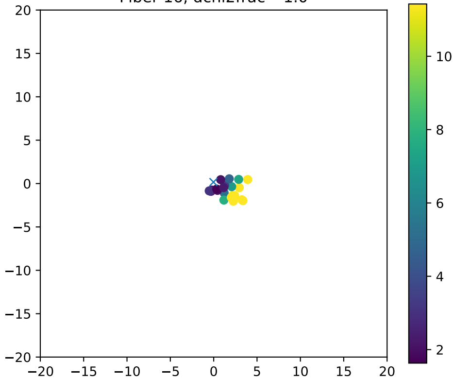
Fiber 16, dchi2frac= 1.0
