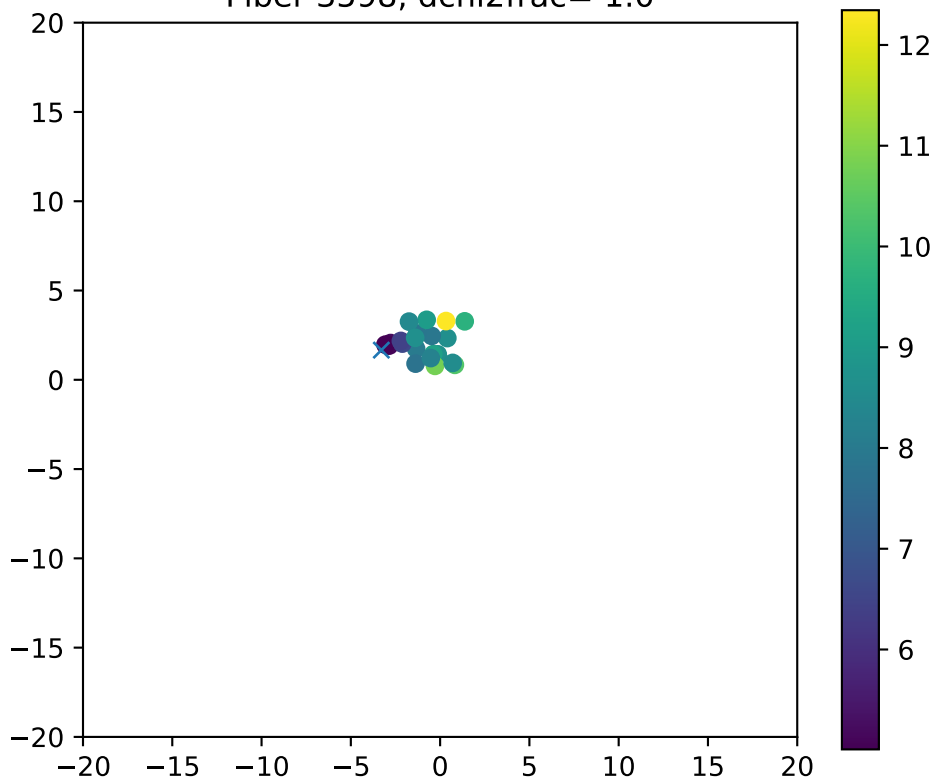
Fiber 3598, dchi2frac= 1.0
