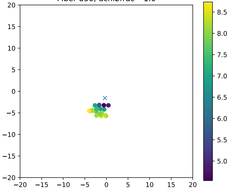
Fiber 850, dchi2frac= 1.0
