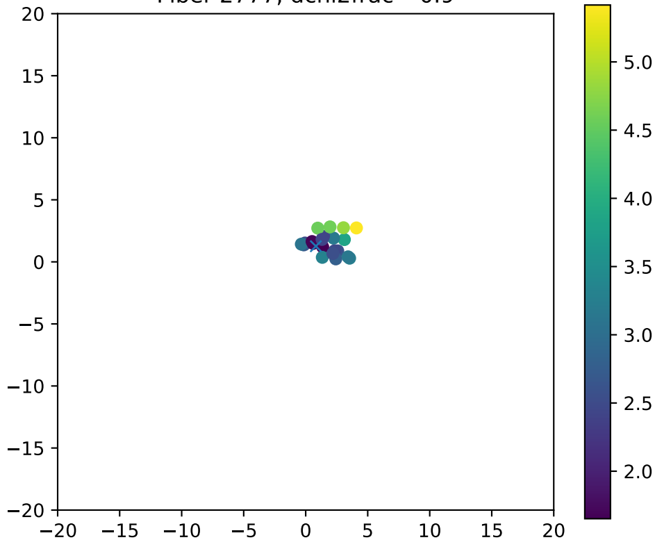
Fiber 2777, dchi2frac= 0.9
