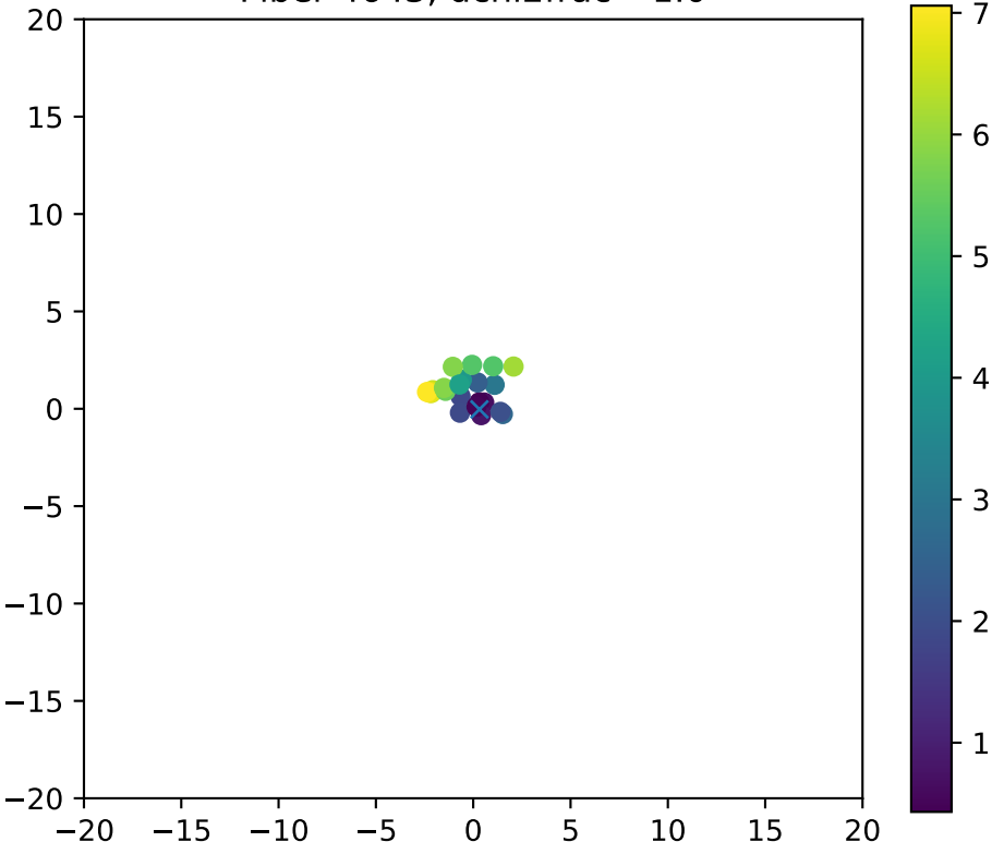
Fiber 4643, dchi2frac= 1.0
