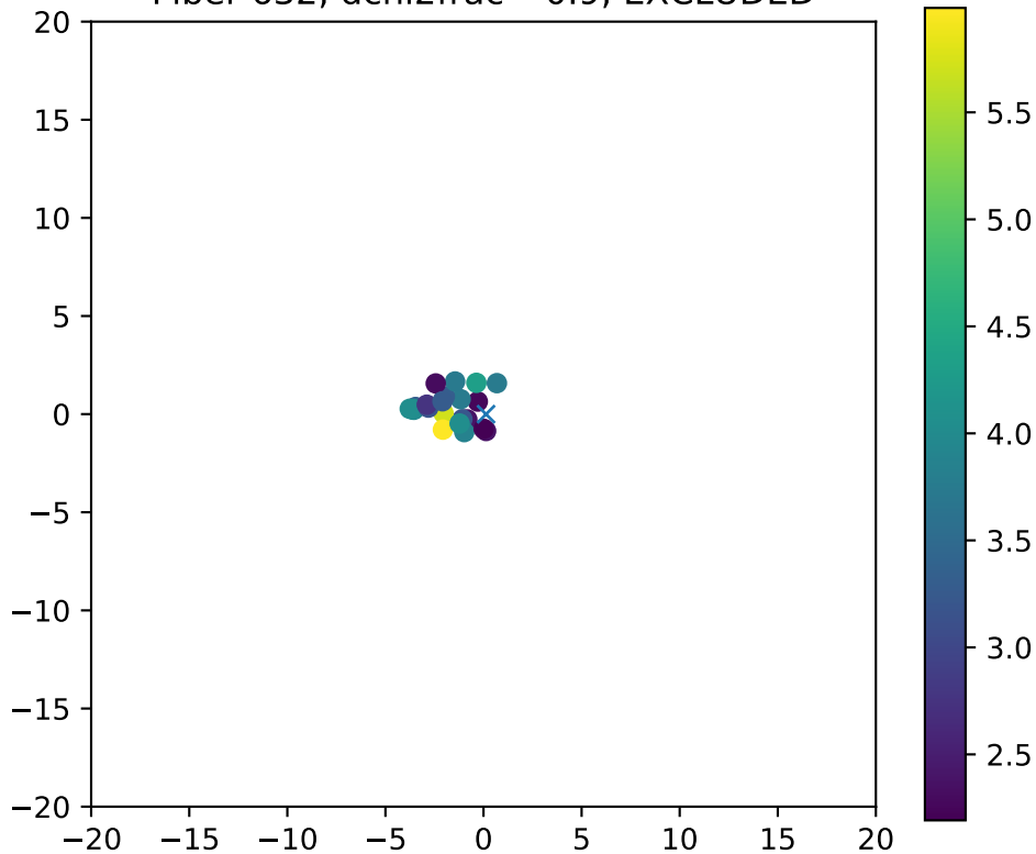
Fiber 632, dchi2frac= 0.9, EXCLUDED
