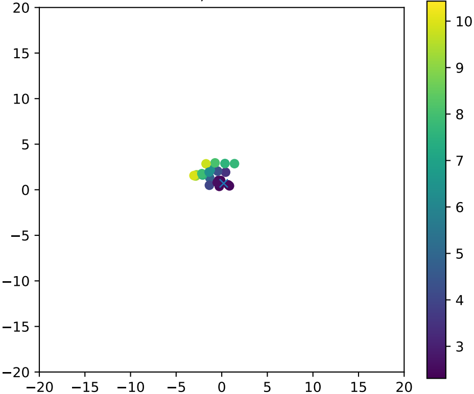
Fiber 2827, dchi2frac= 1.0
