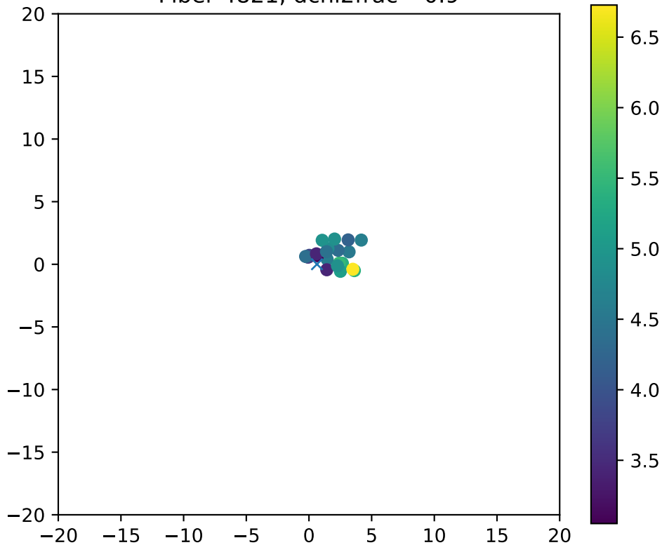
Fiber 4821, dchi2frac= 0.9
