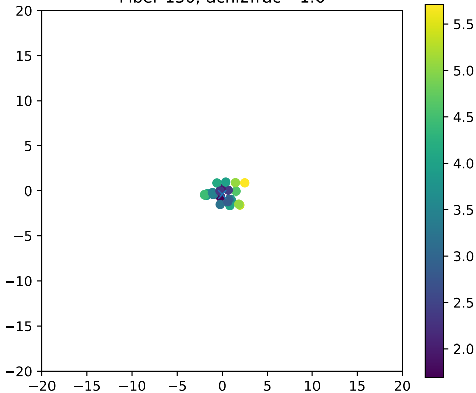
Fiber 150, dchi2frac= 1.0
