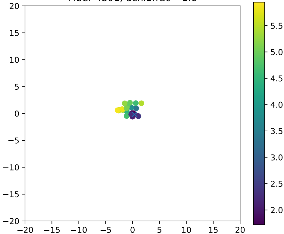
Fiber 4801, dchi2frac= 1.0
