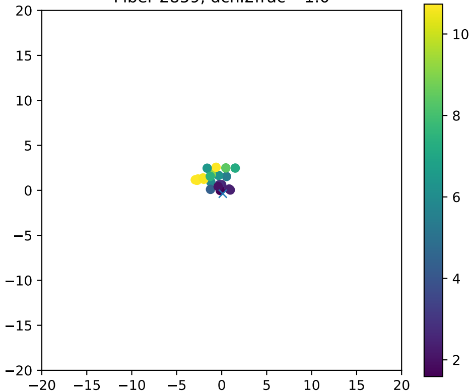
Fiber 2859, dchi2frac= 1.0
