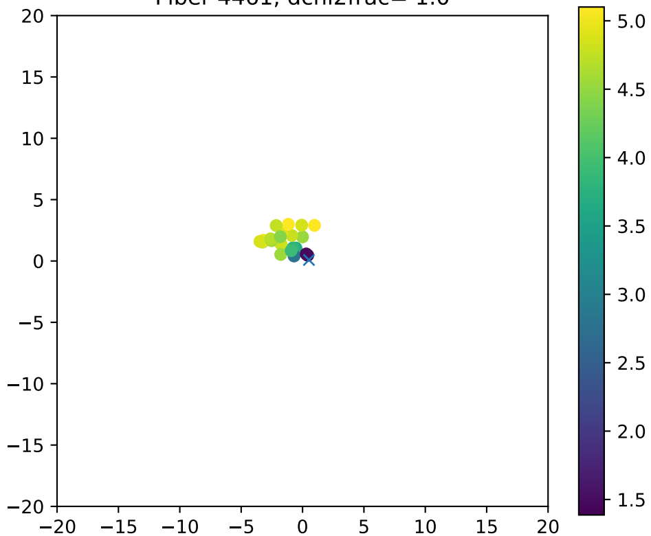
Fiber 4461, dchi2frac= 1.0
