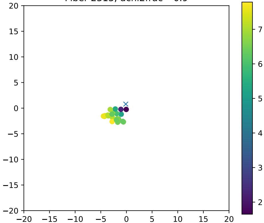
Fiber 2313, dchi2frac= 0.9
