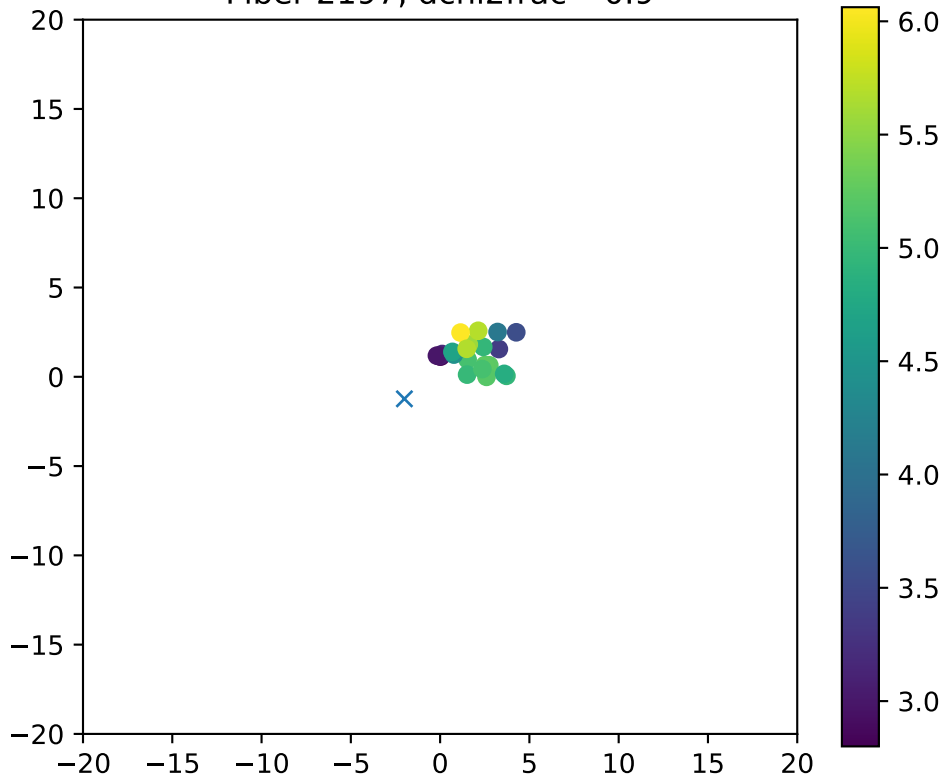
Fiber 2197, dchi2frac= 0.9
