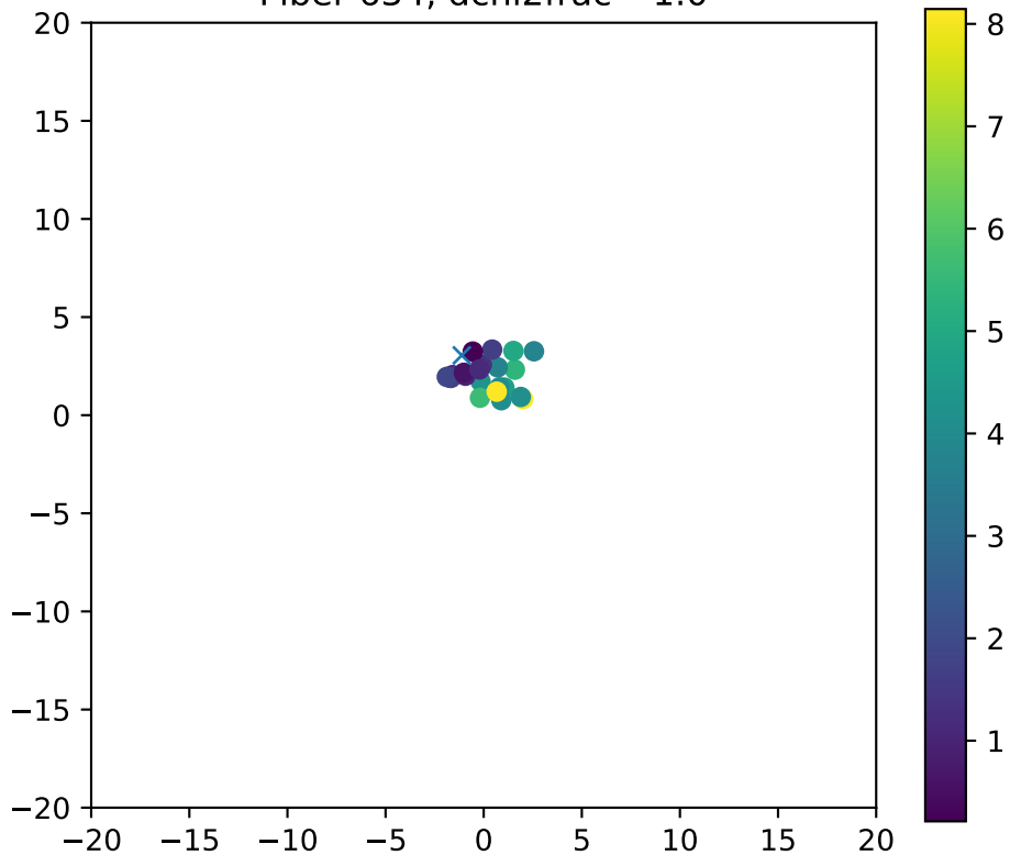
Fiber 634, dchi2frac= 1.0
