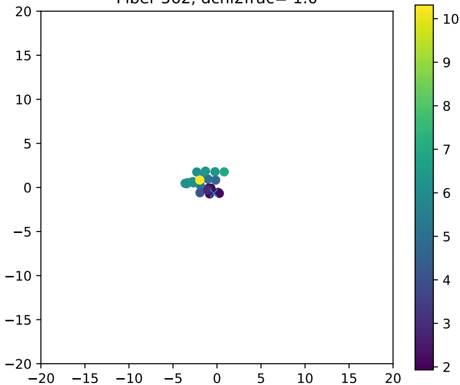
Fiber 562, dchi2frac= 1.0
