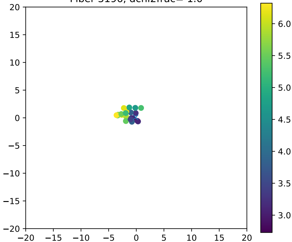
Fiber 3196, dchi2frac= 1.0
