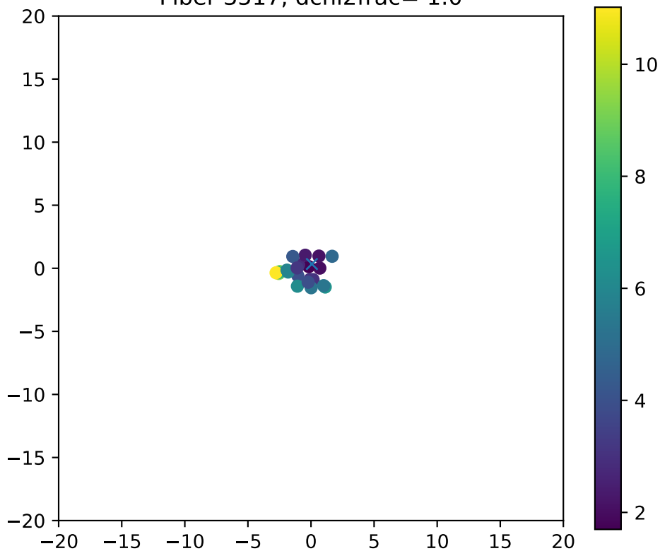
Fiber 3517, dchi2frac= 1.0
