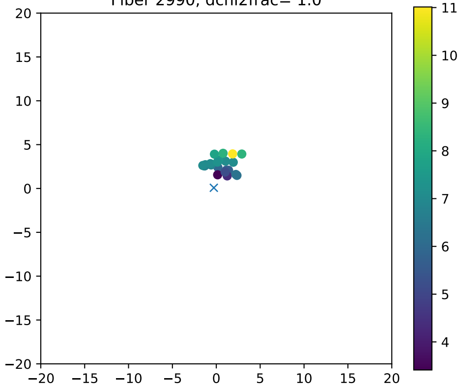
Fiber 2990, dchi2frac= 1.0
