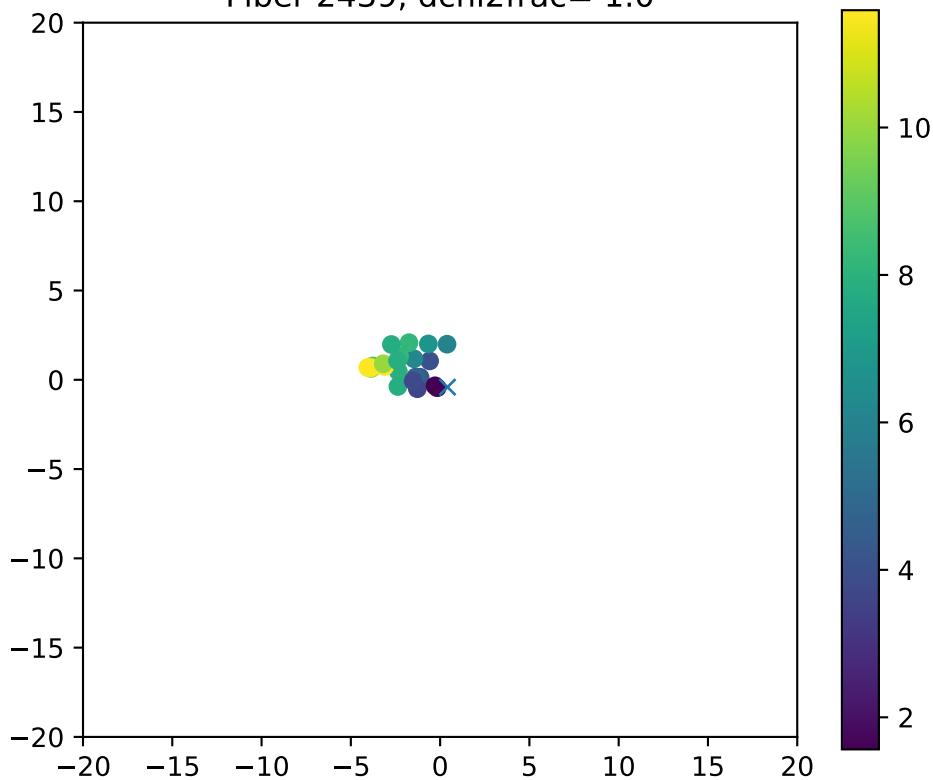
Fiber 2439, dchi2frac= 1.0
