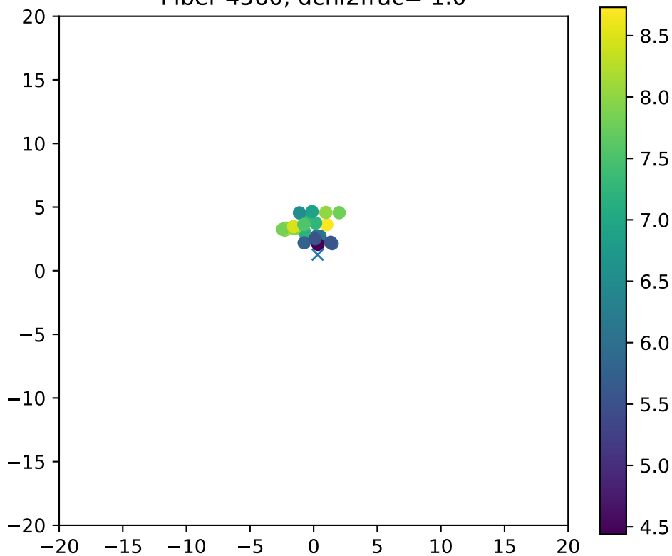
Fiber 4560, dchi2frac= 1.0
