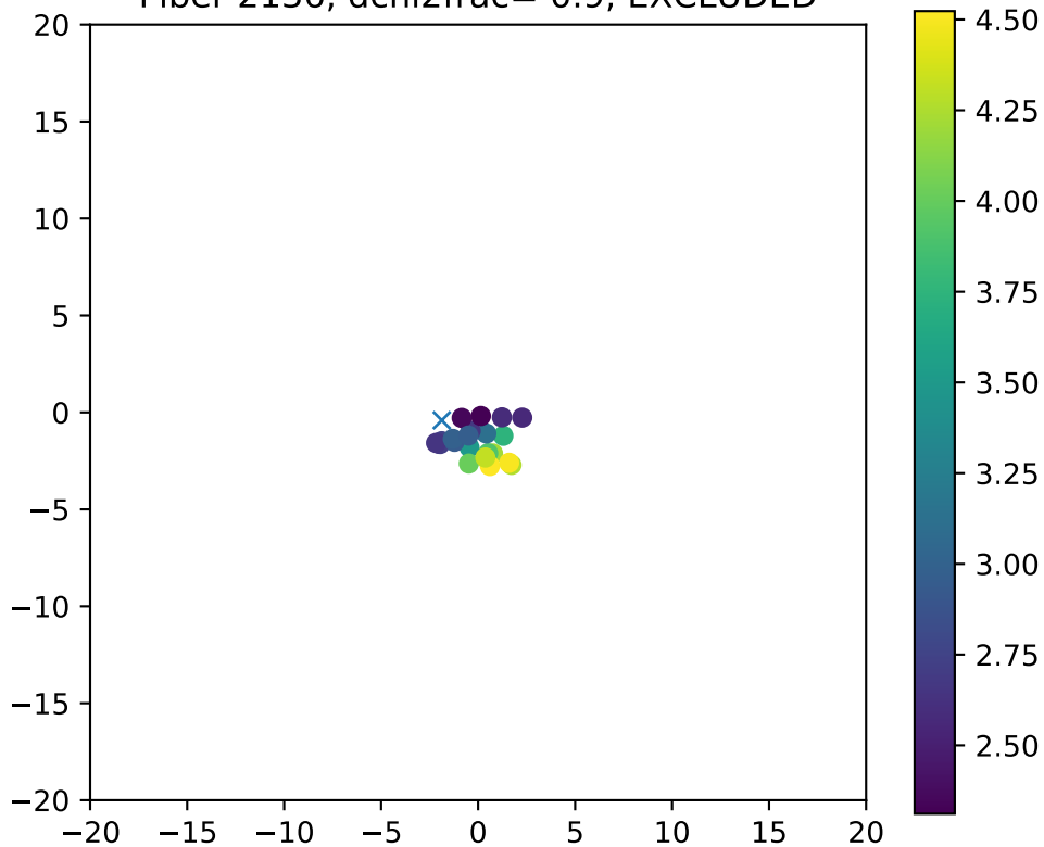
Fiber 2136, dchi2frac= 0.9, EXCLUDED
