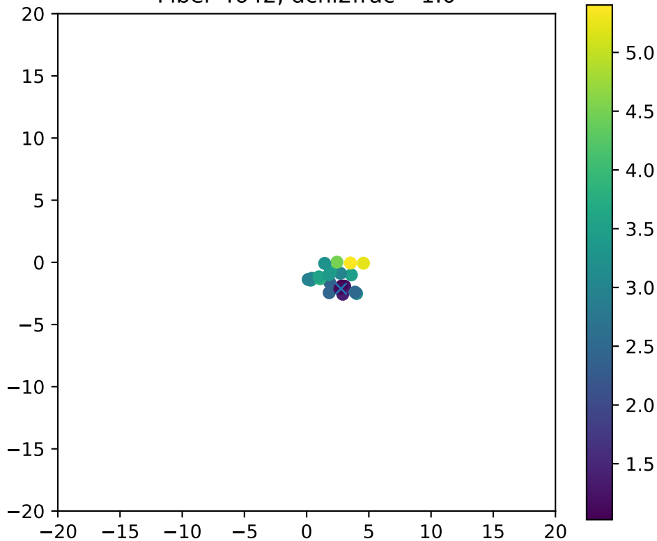
Fiber 4642, dchi2frac= 1.0
