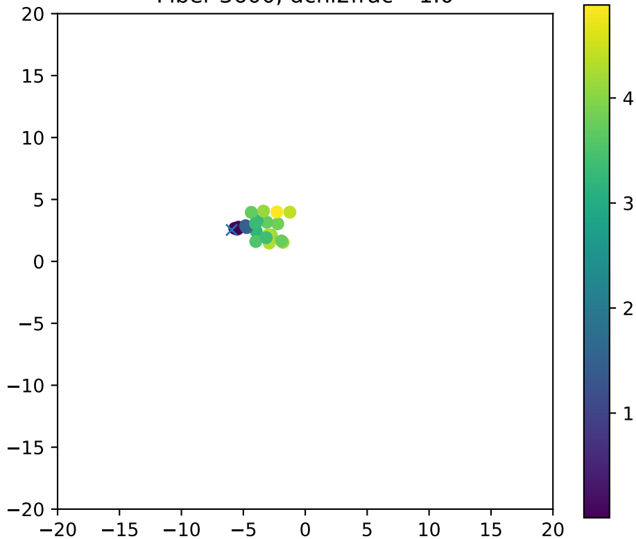
Fiber 3600, dchi2frac= 1.0
