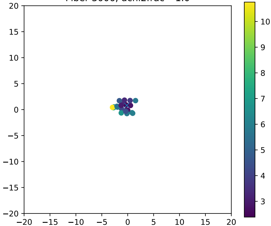
Fiber 3006, dchi2frac= 1.0
