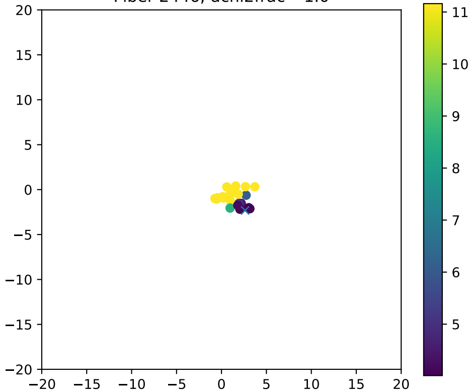
Fiber 2446, dchi2frac= 1.0
