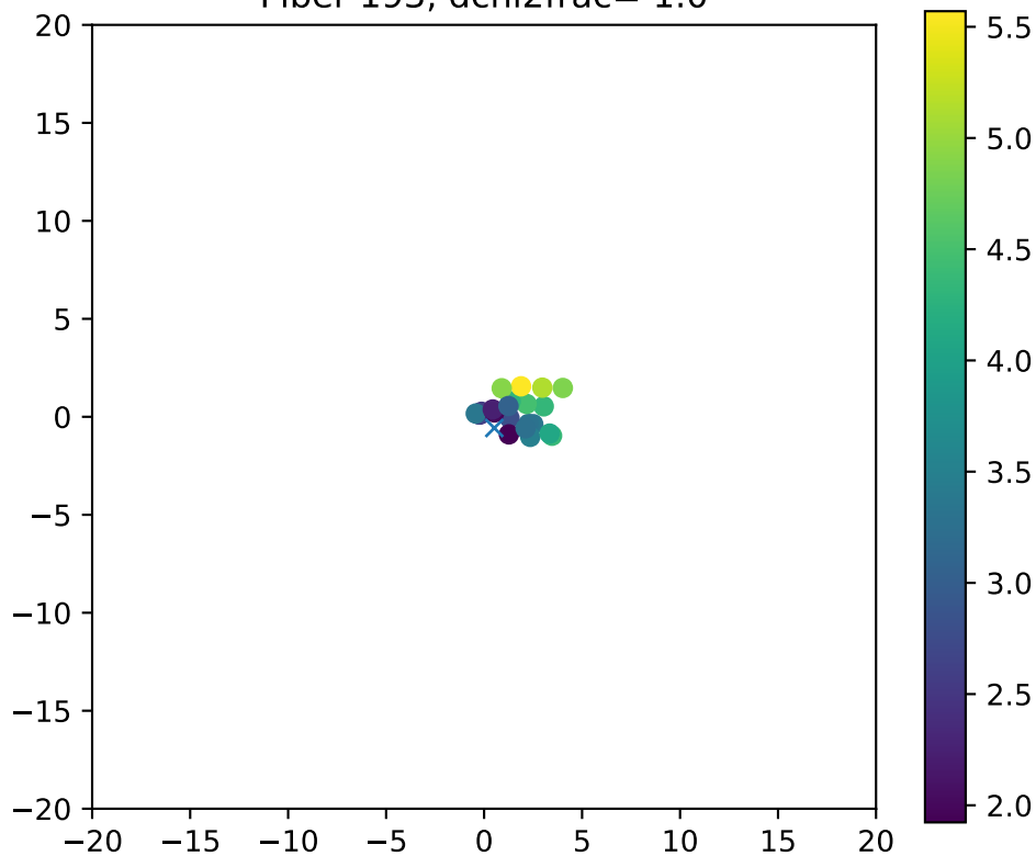
Fiber 193, dchi2frac= 1.0
