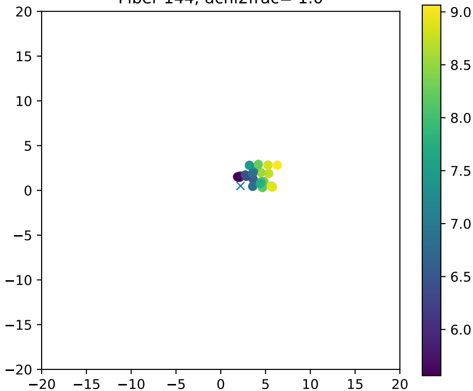
Fiber 144, dchi2frac= 1.0
