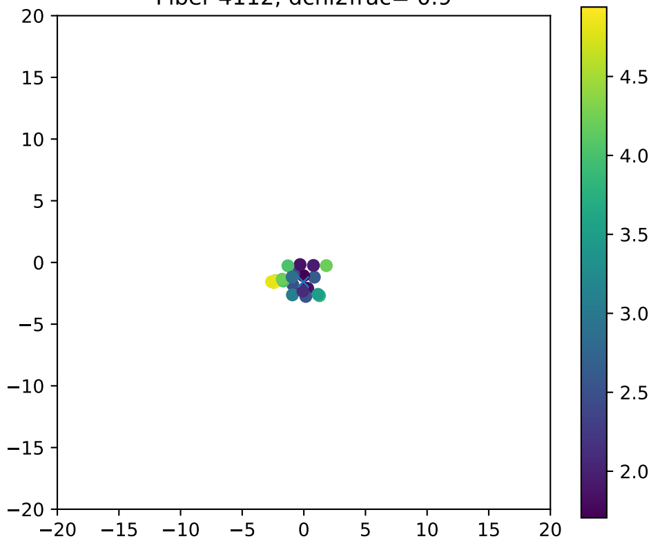
Fiber 4112, dchi2frac= 0.9
