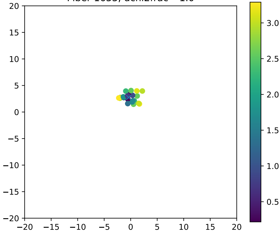
Fiber 1633, dchi2frac= 1.0
