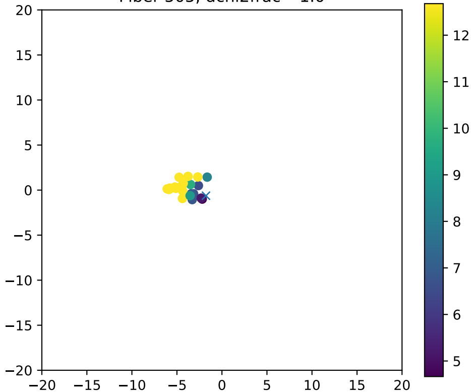
Fiber 505, dchi2frac= 1.0
