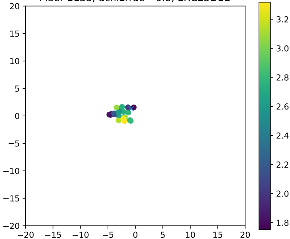
Fiber 2135, dchi2frac= 0.8, EXCLUDED
