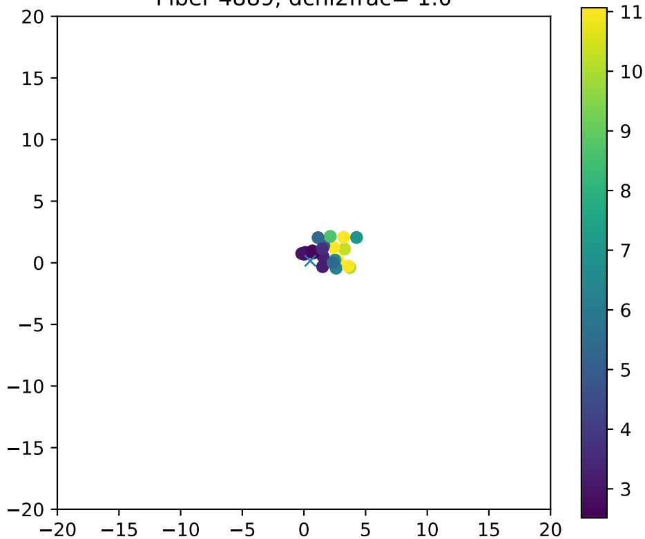
Fiber 4889, dchi2frac= 1.0
