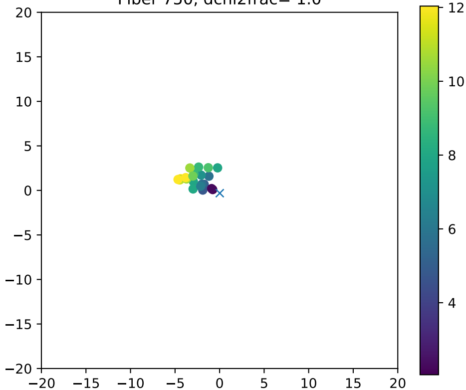
Fiber 750, dchi2frac= 1.0
