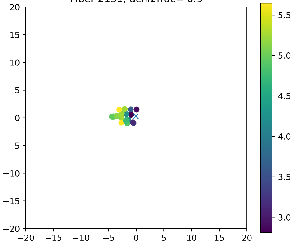
Fiber 2131, dchi2frac= 0.9
