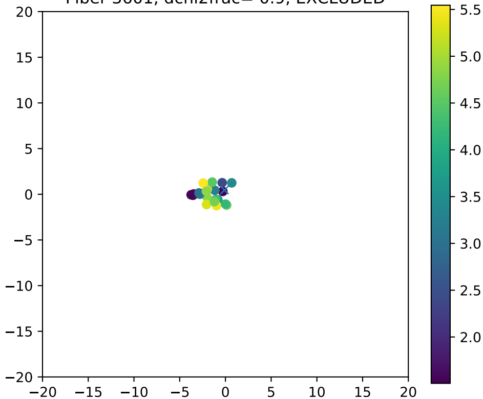
Fiber 3601, dchi2frac= 0.9, EXCLUDED
