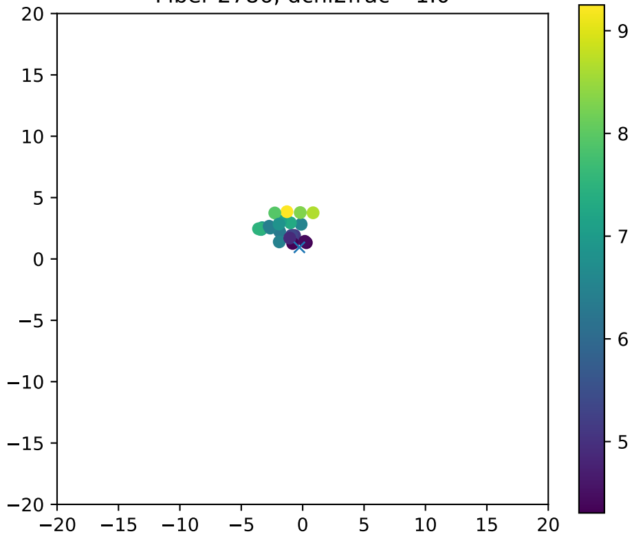
Fiber 2786, dchi2frac= 1.0
