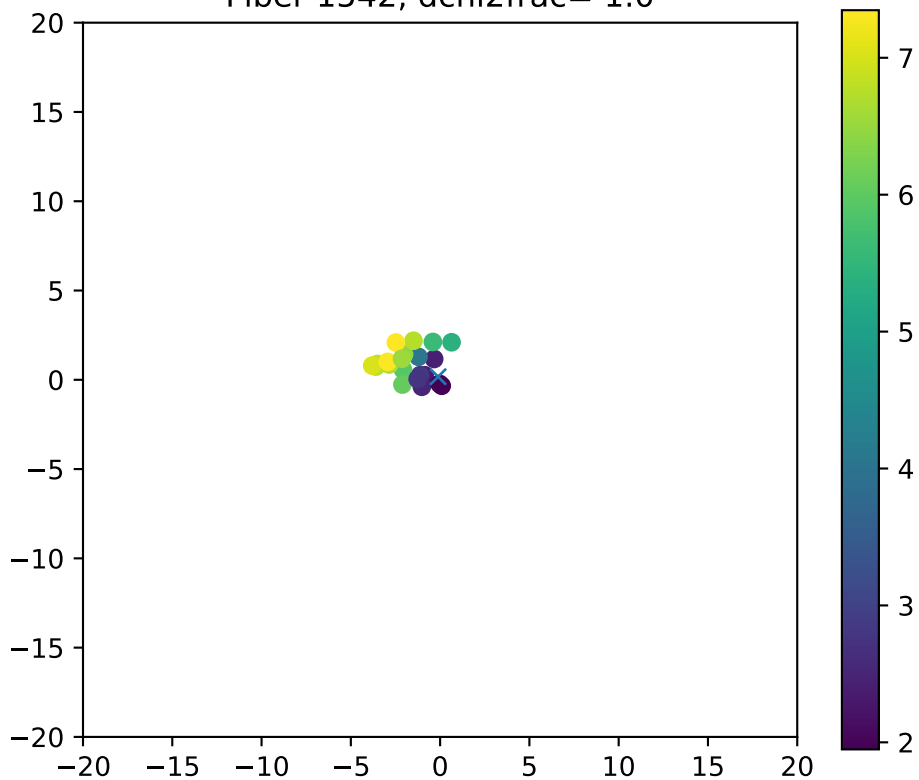
Fiber 1542, dchi2frac= 1.0
