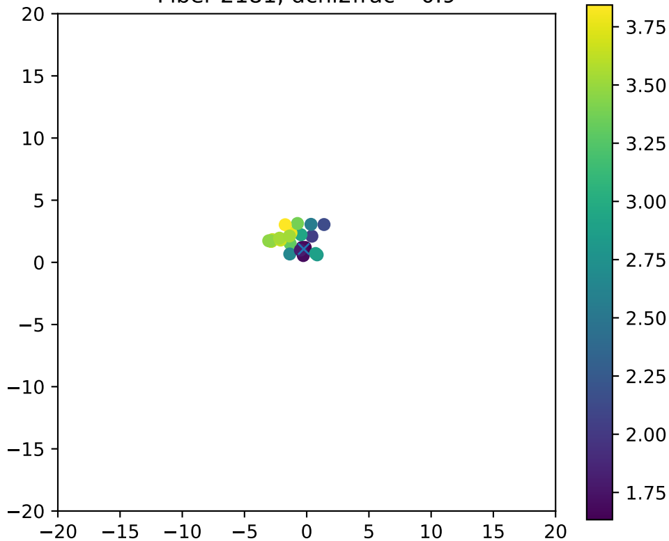
Fiber 2181, dchi2frac= 0.9
