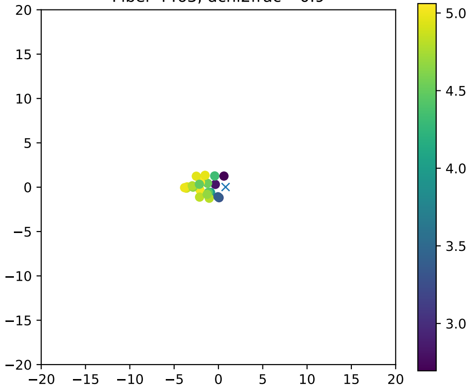
Fiber 4463, dchi2frac= 0.9
