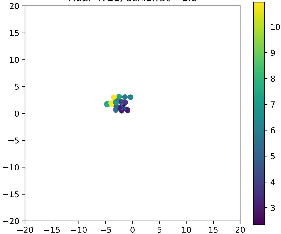
Fiber 4721, dchi2frac= 1.0
