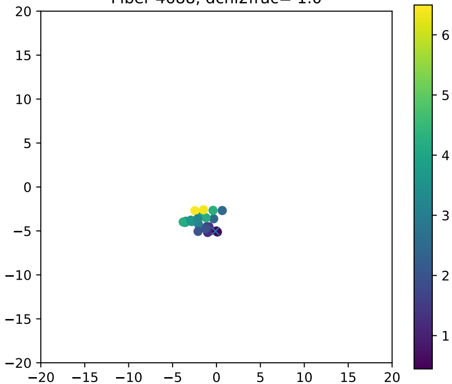
Fiber 4688, dchi2frac= 1.0
