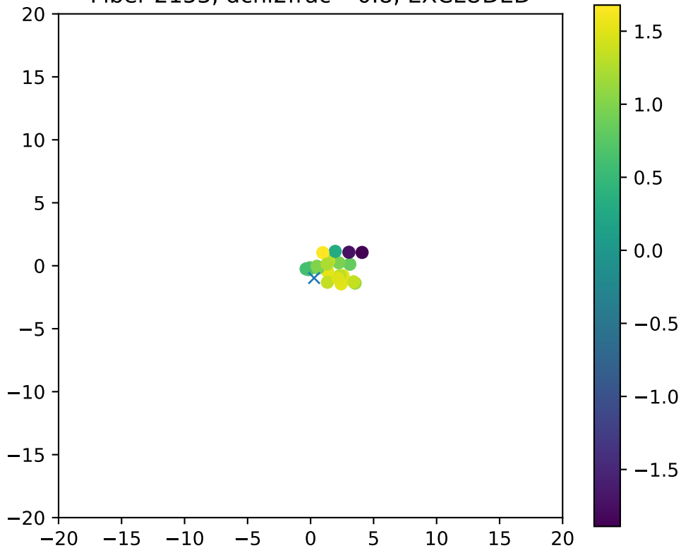
Fiber 2153, dchi2frac= 0.8, EXCLUDED
