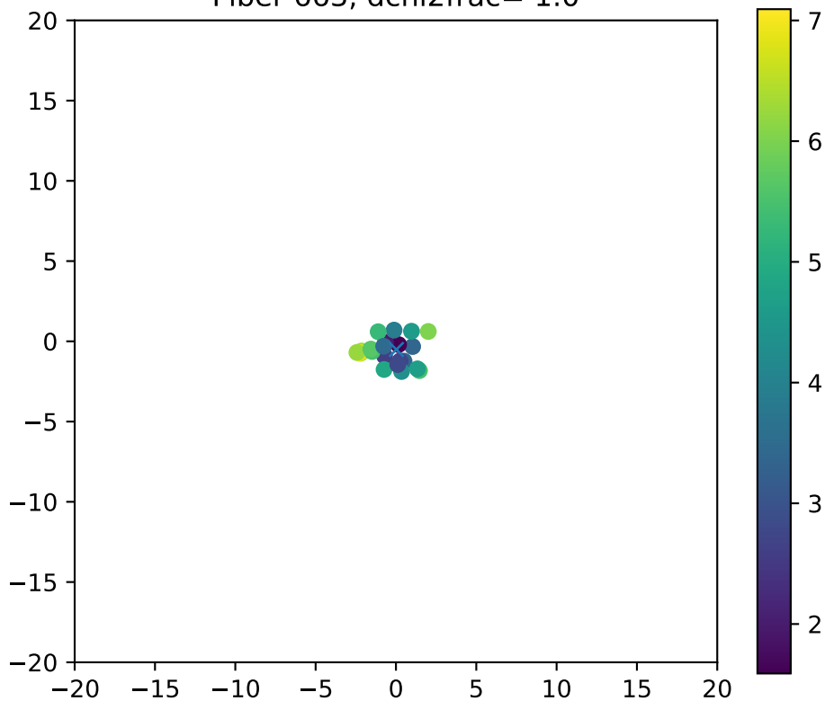
Fiber 663, dchi2frac= 1.0
