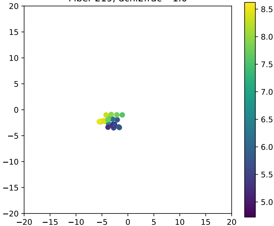
Fiber 219, dchi2frac= 1.0
