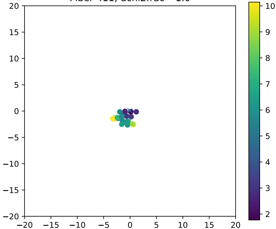
Fiber 411, dchi2frac= 1.0
