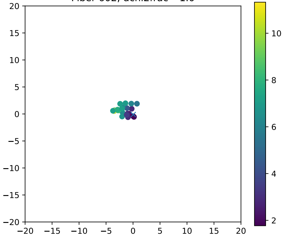
Fiber 602, dchi2frac= 1.0
