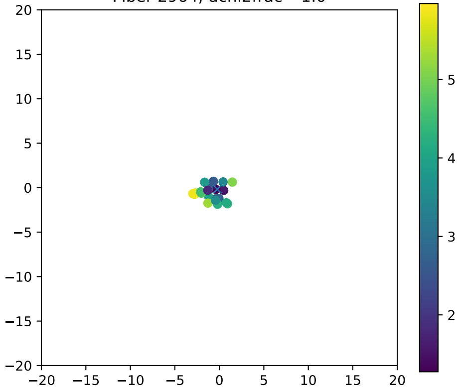
Fiber 2964, dchi2frac= 1.0
