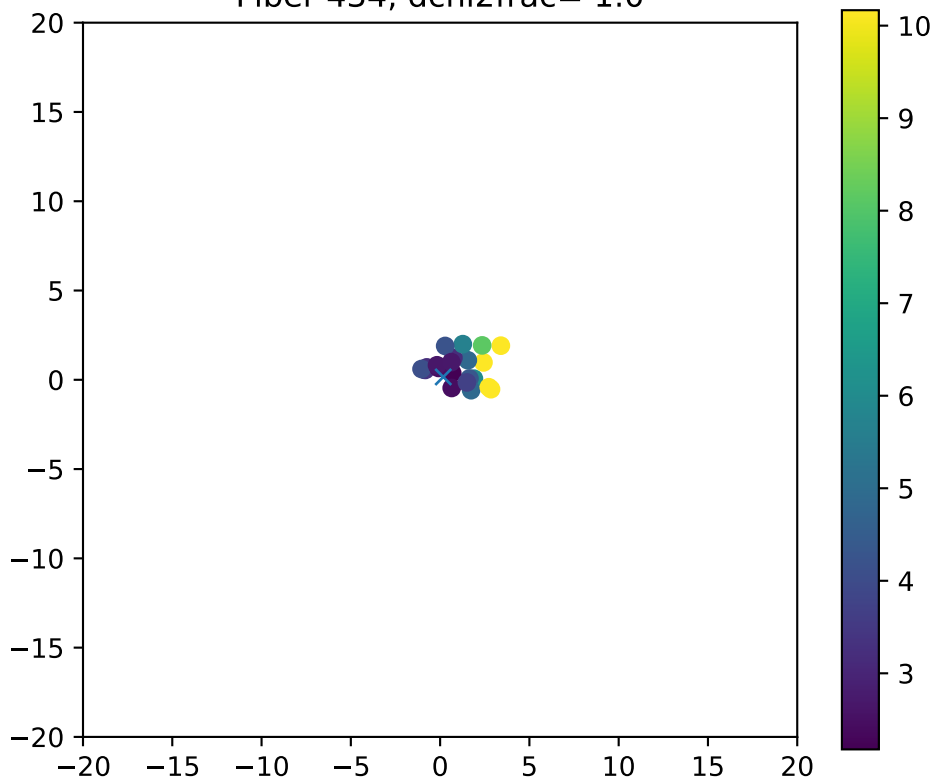
Fiber 434, dchi2frac= 1.0
