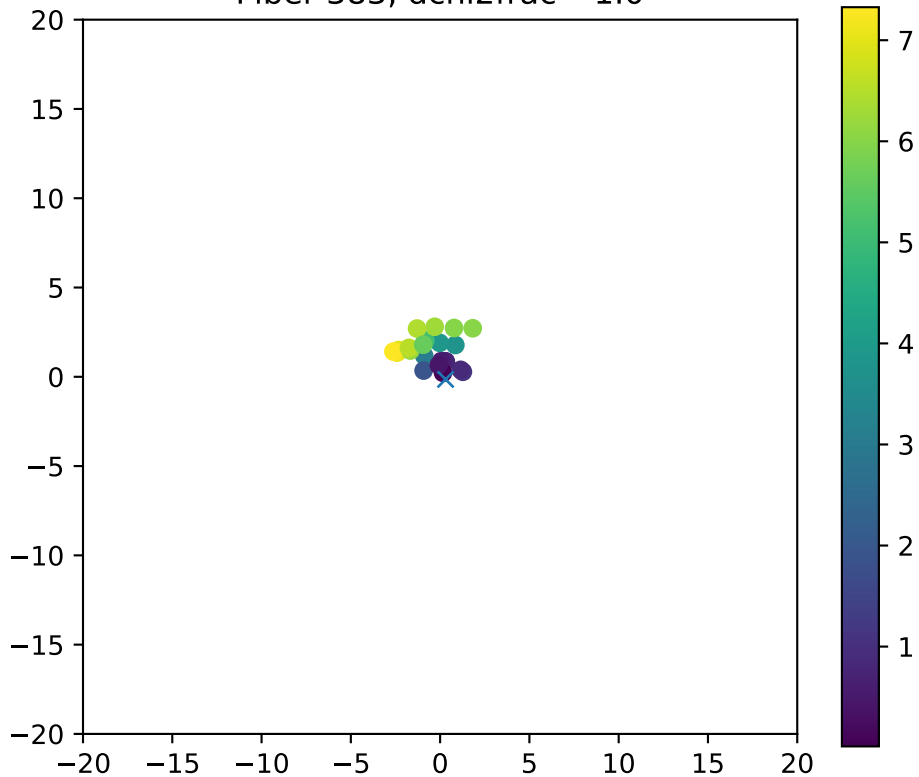
Fiber 383, dchi2frac= 1.0
