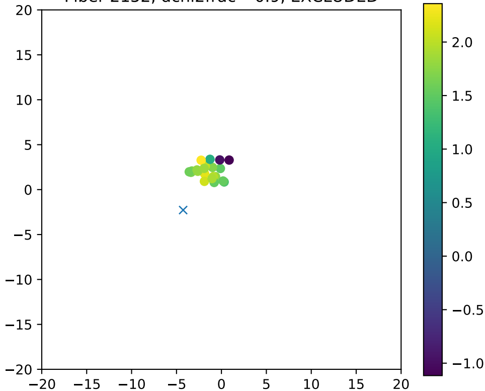
Fiber 2152, dchi2frac= 0.9, EXCLUDED
