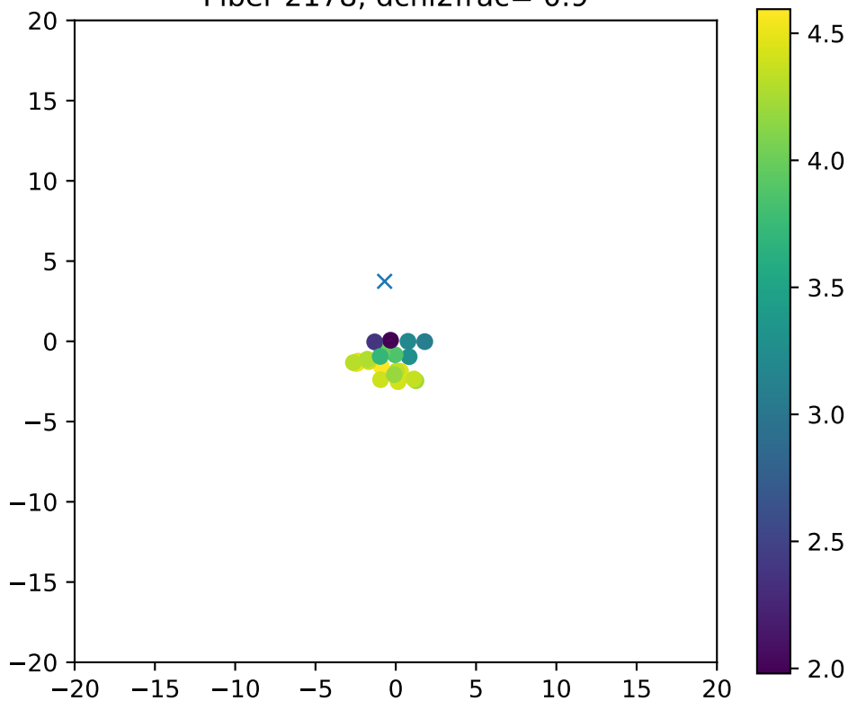
Fiber 2178, dchi2frac= 0.9
