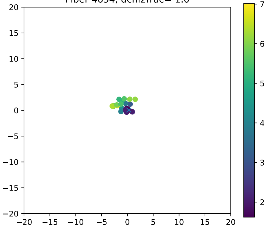
Fiber 4654, dchi2frac= 1.0
