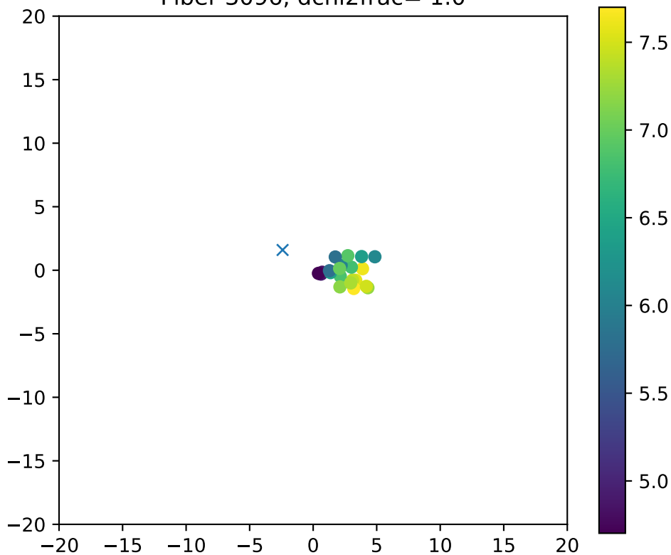
Fiber 3096, dchi2frac= 1.0
