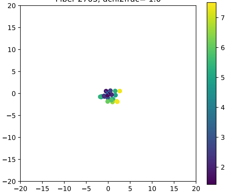
Fiber 2703, dchi2frac= 1.0
