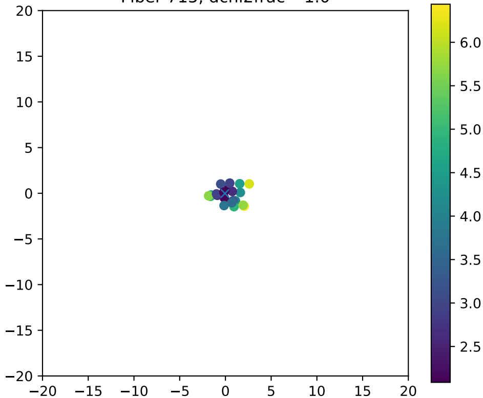
Fiber 715, dchi2frac= 1.0
