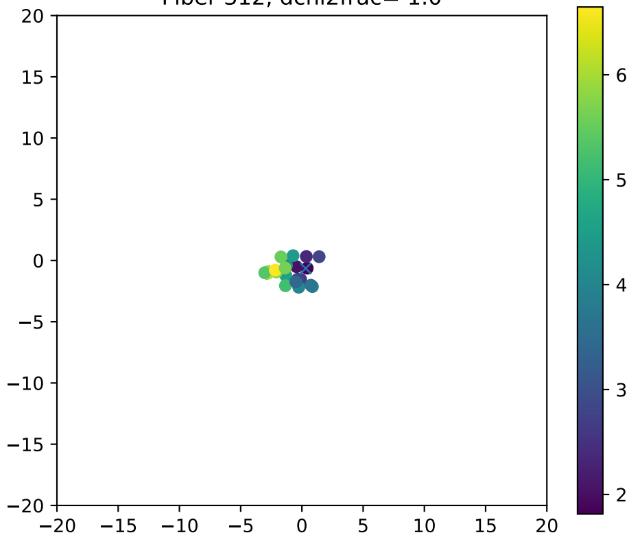
Fiber 312, dchi2frac= 1.0
