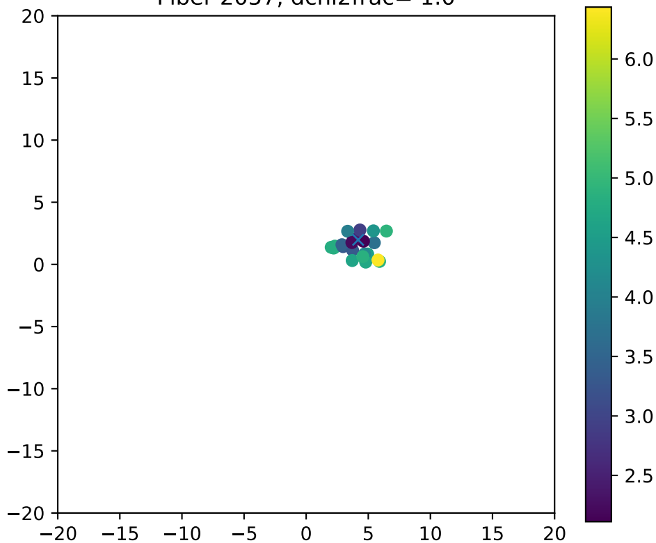
Fiber 2057, dchi2frac= 1.0
