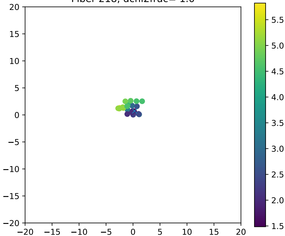
Fiber 218, dchi2frac= 1.0
