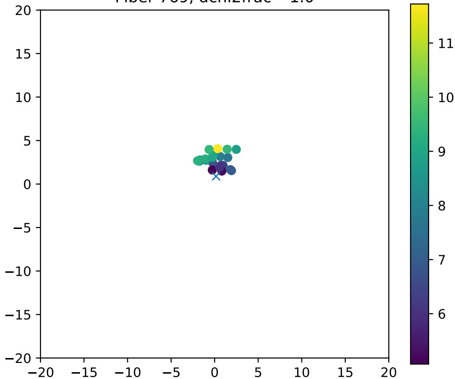
Fiber 769, dchi2frac= 1.0
