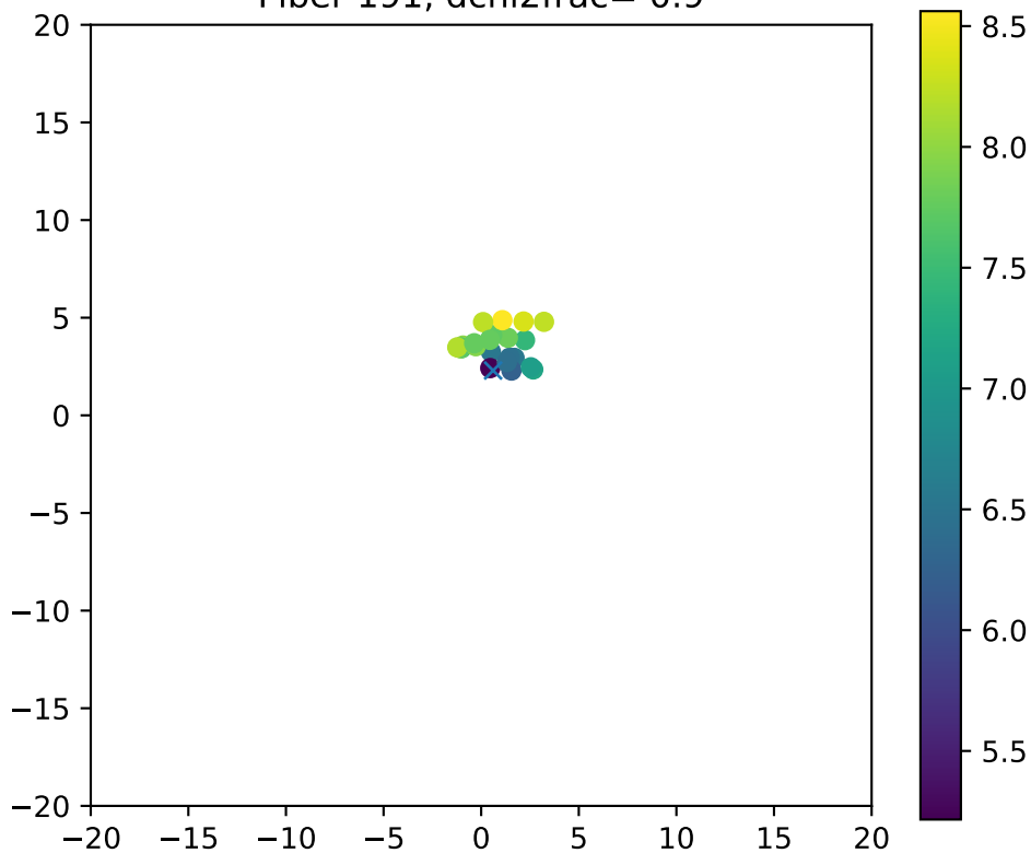
Fiber 191, dchi2frac= 0.9
