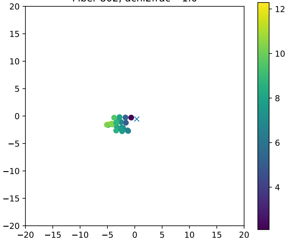
Fiber 802, dchi2frac= 1.0
