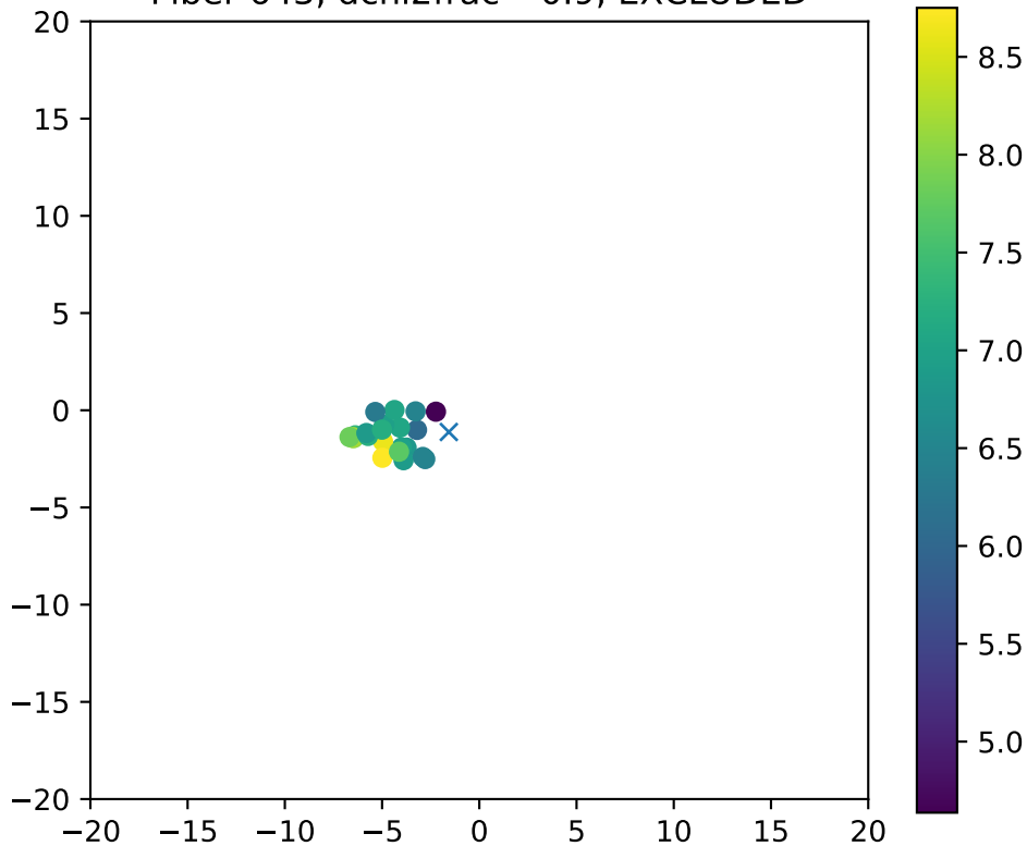
Fiber 643, dchi2frac= 0.9, EXCLUDED
