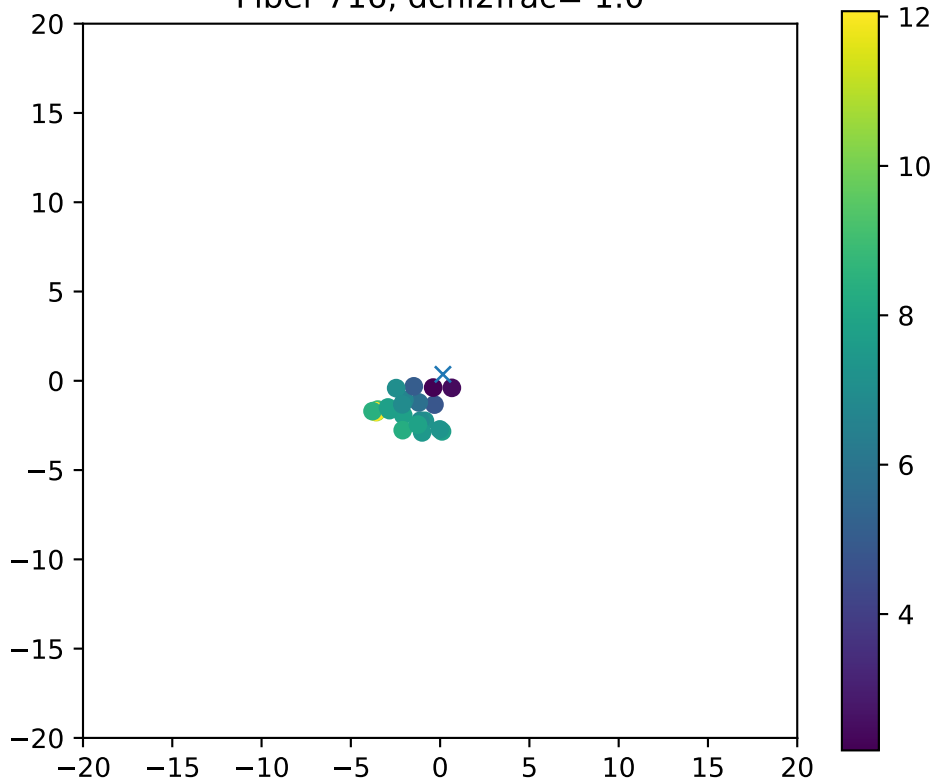
Fiber 716, dchi2frac= 1.0
