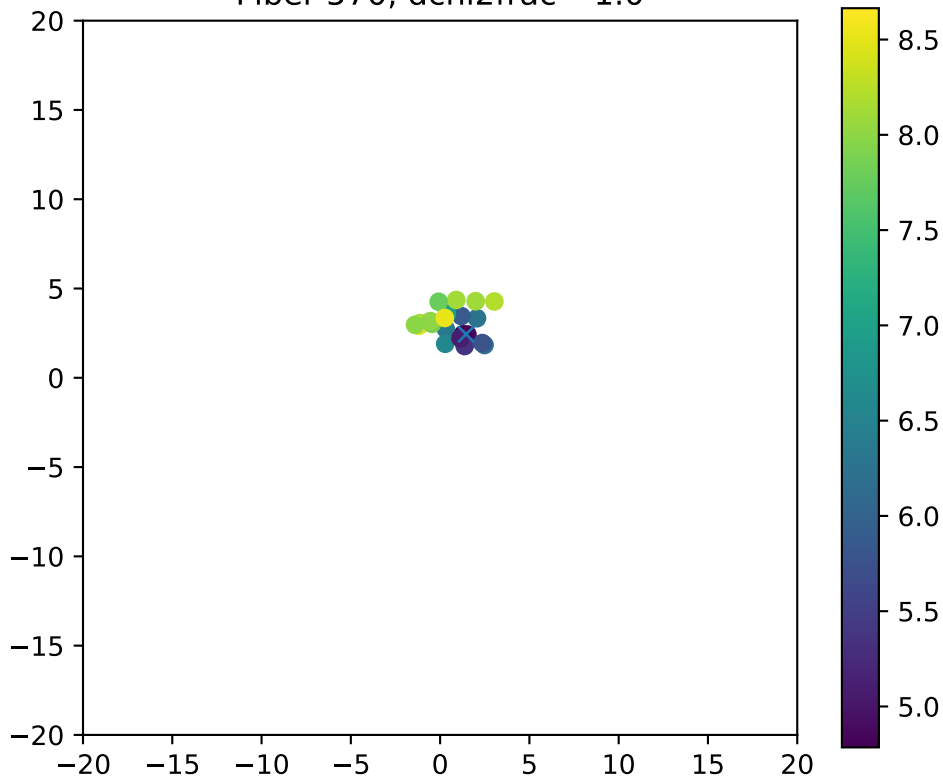
Fiber 570, dchi2frac= 1.0
