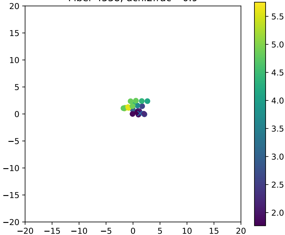
Fiber 4538, dchi2frac= 0.9
