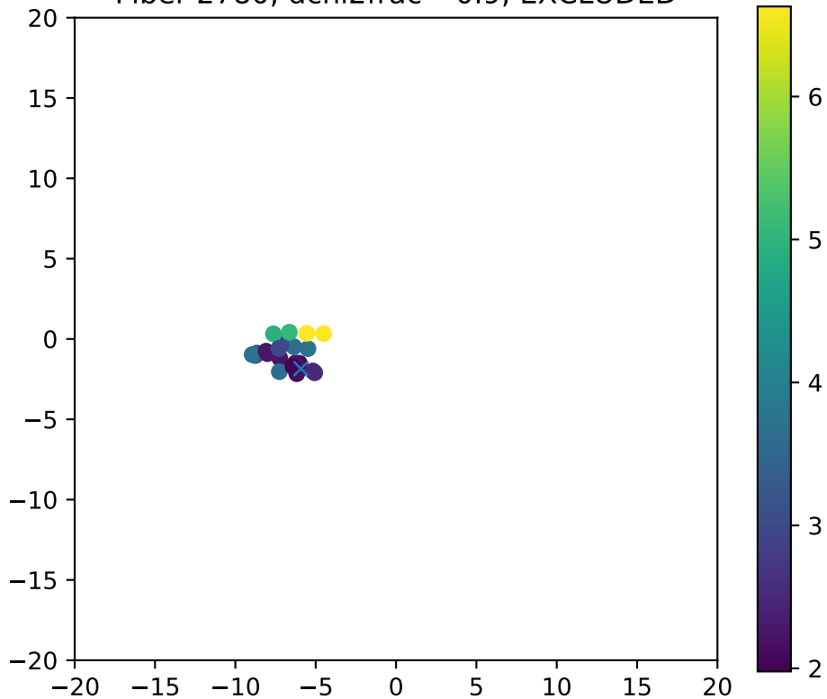
Fiber 2780, dchi2frac= 0.9, EXCLUDED
