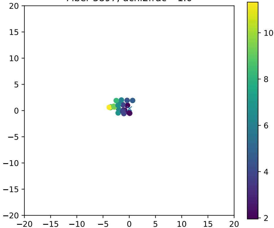
Fiber 3897, dchi2frac= 1.0
