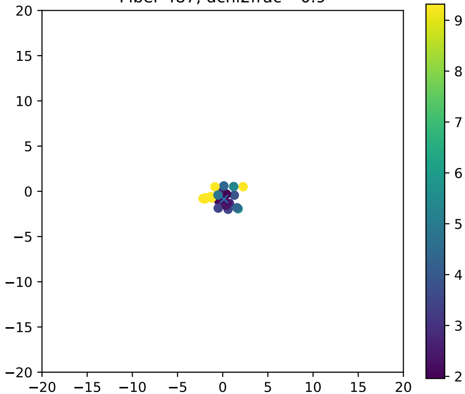
Fiber 487, dchi2frac= 0.9
