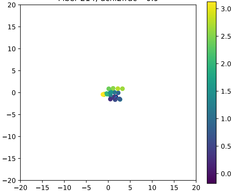
Fiber 214, dchi2frac= 0.9
