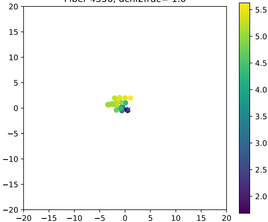
Fiber 4356, dchi2frac= 1.0
