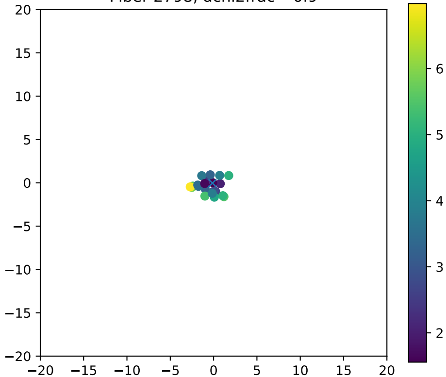
Fiber 2798, dchi2frac= 0.9
