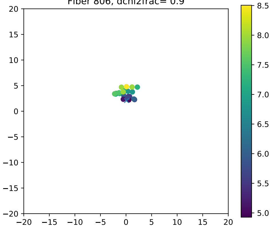
Fiber 806, dchi2frac= 0.9
