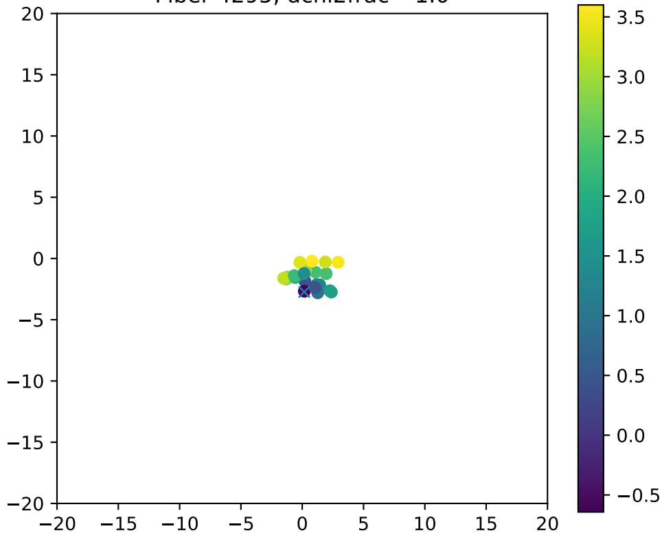
Fiber 4295, dchi2frac= 1.0
