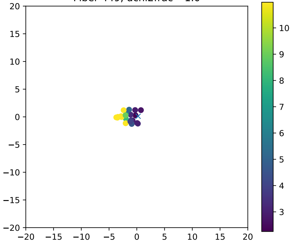
Fiber 449, dchi2frac= 1.0
