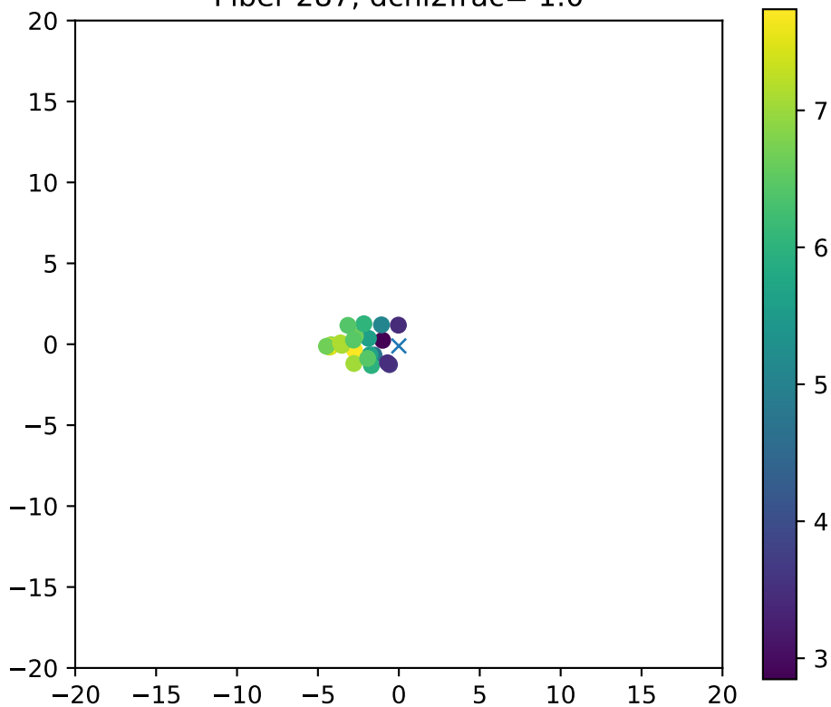
Fiber 287, dchi2frac= 1.0
