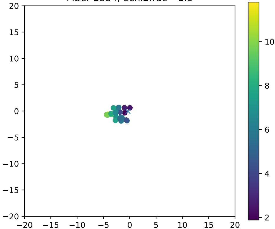
Fiber 1884, dchi2frac= 1.0
