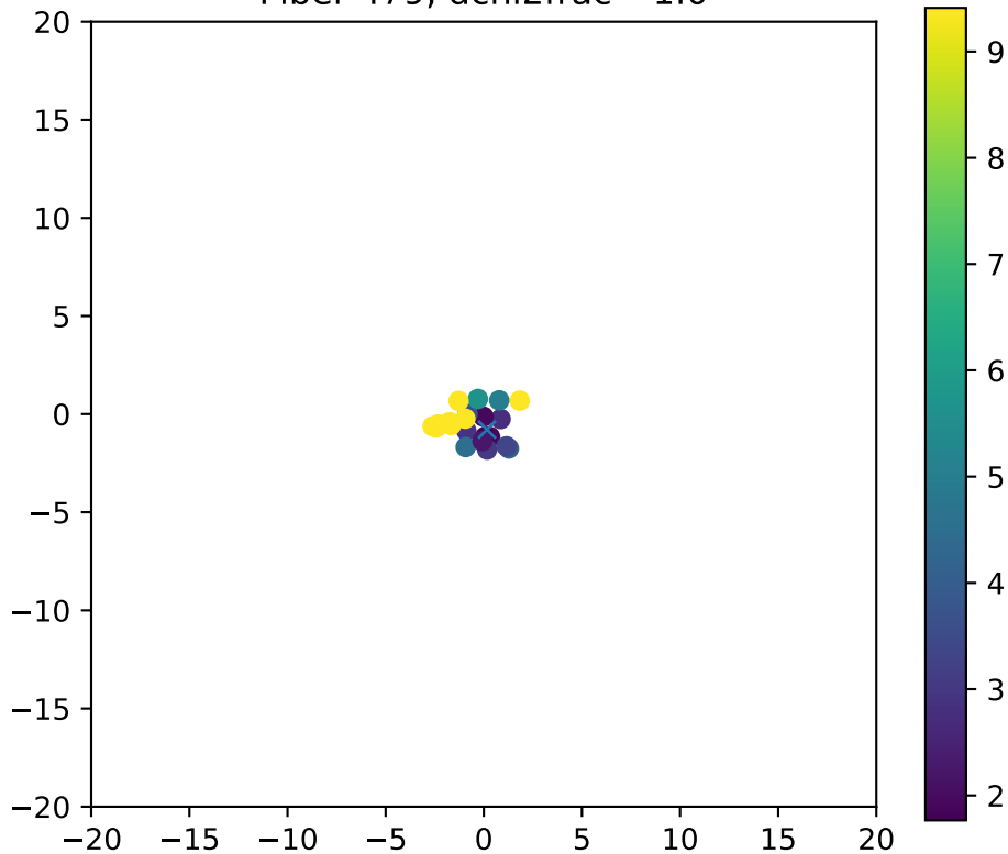
Fiber 479, dchi2frac= 1.0
