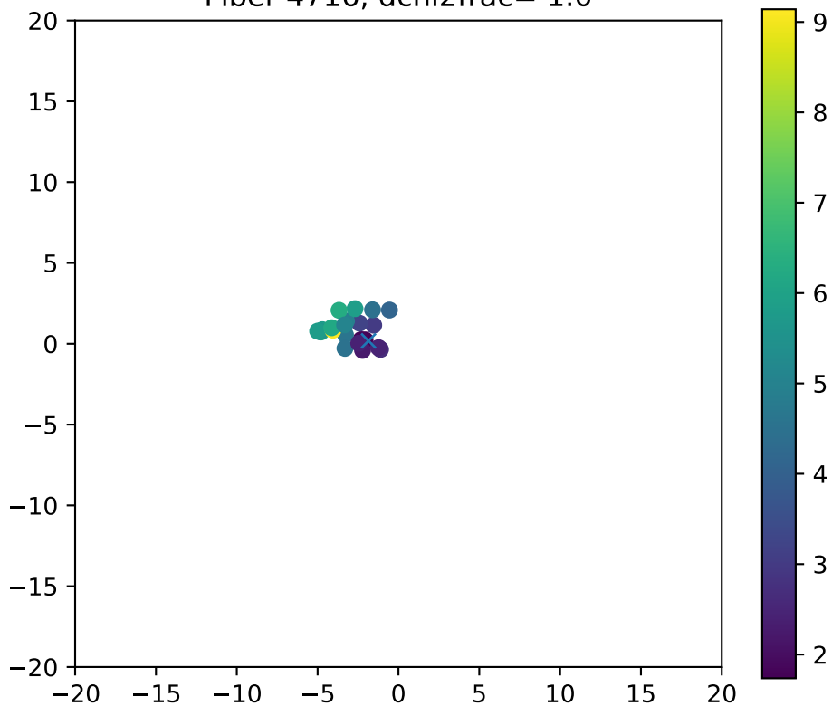
Fiber 4716, dchi2frac= 1.0
