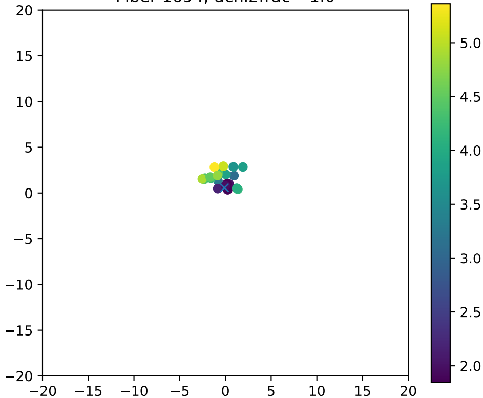
Fiber 1694, dchi2frac= 1.0
