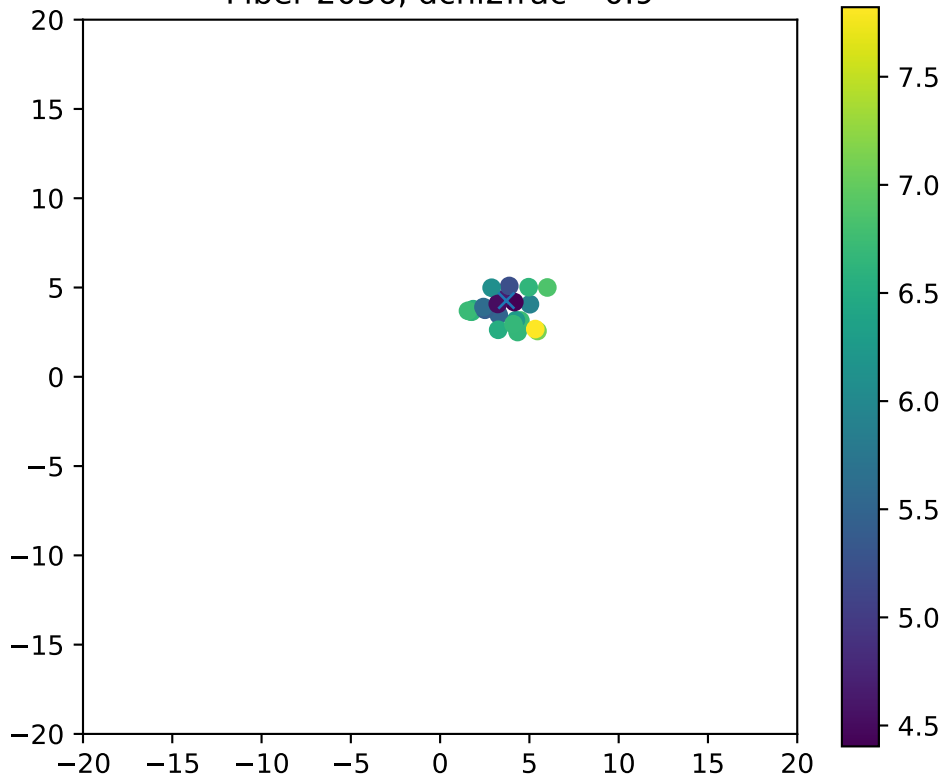
Fiber 2056, dchi2frac= 0.9
