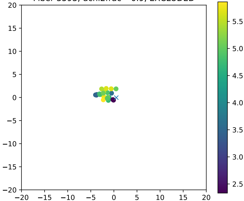
Fiber 3593, dchi2frac= 0.9, EXCLUDED
