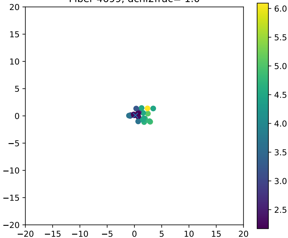
Fiber 4699, dchi2frac= 1.0
