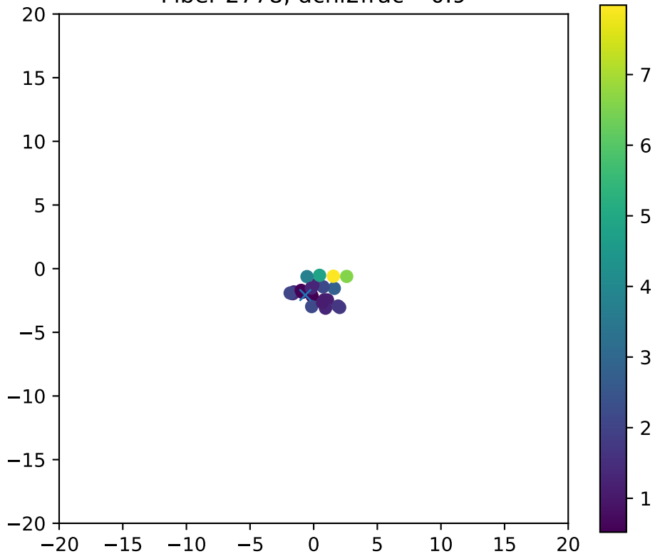
Fiber 2778, dchi2frac= 0.9
