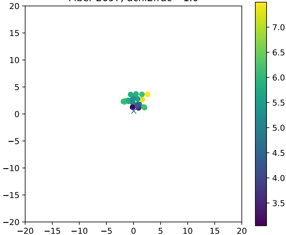
Fiber 2697, dchi2frac= 1.0
