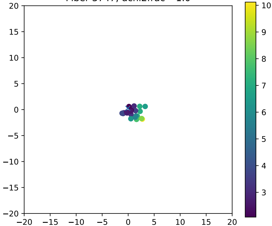
Fiber 3747, dchi2frac= 1.0
