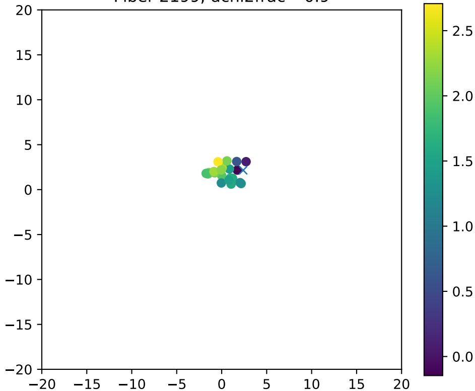
Fiber 2199, dchi2frac= 0.9
