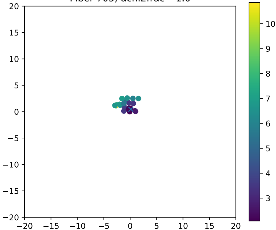
Fiber 705, dchi2frac= 1.0
