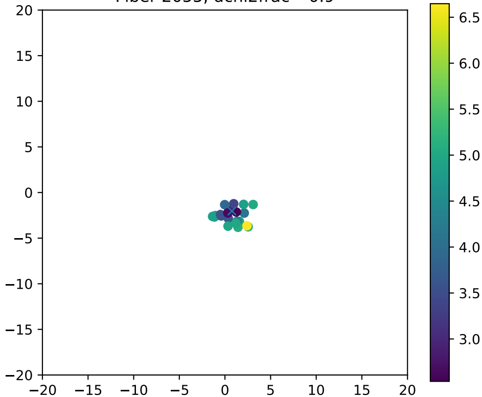
Fiber 2055, dchi2frac= 0.9
