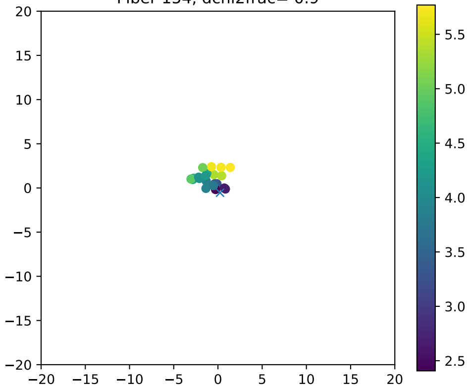
Fiber 154, dchi2frac= 0.9
