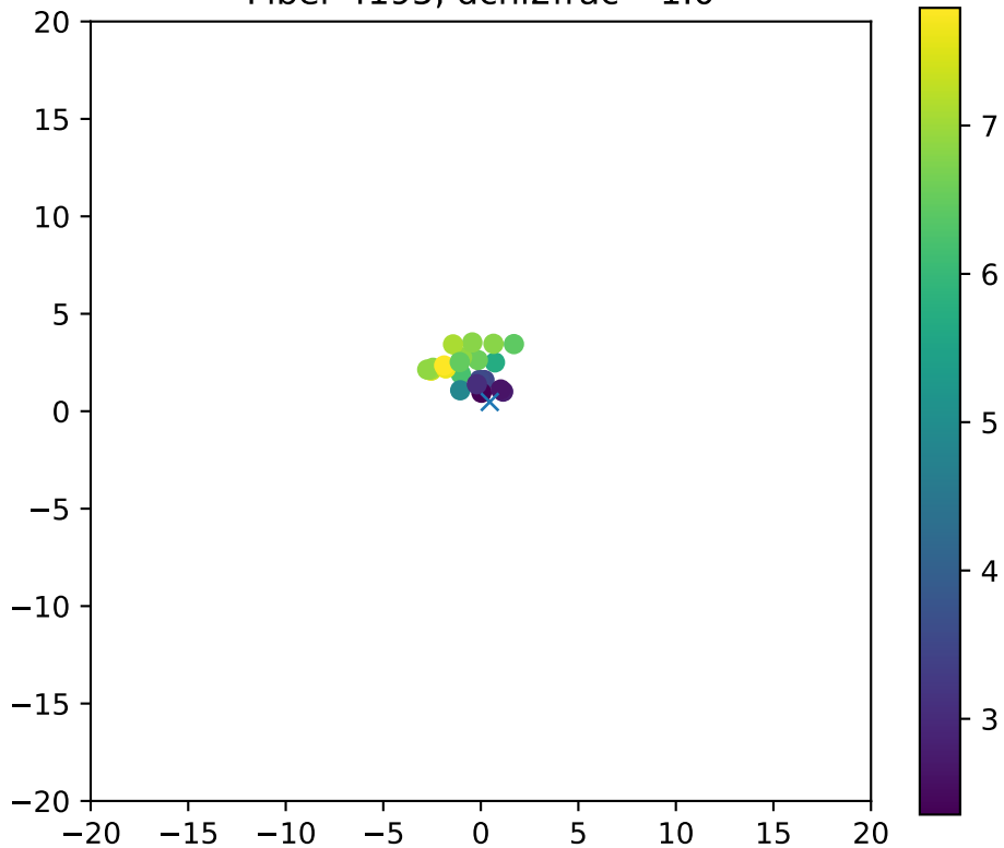
Fiber 4195, dchi2frac= 1.0
