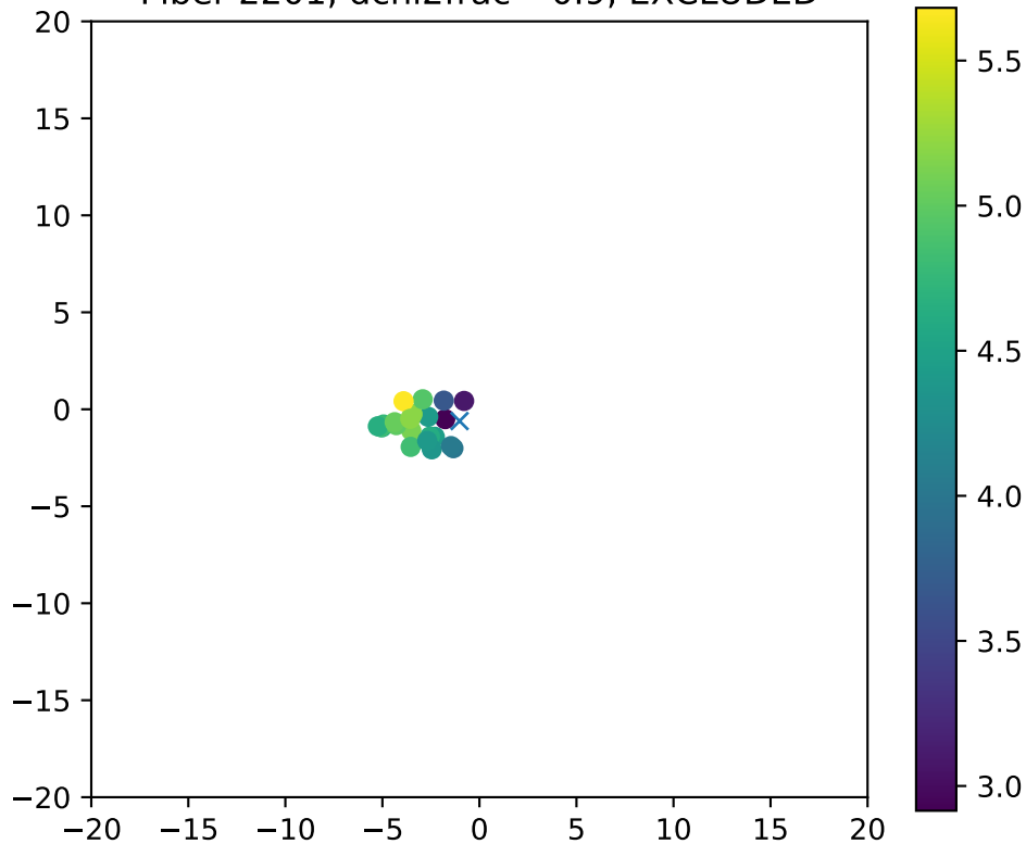
Fiber 2201, dchi2frac= 0.9, EXCLUDED
