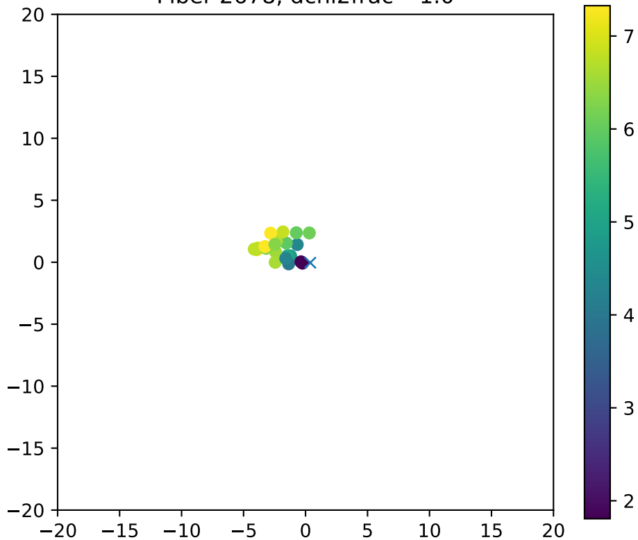
Fiber 2678, dchi2frac= 1.0
