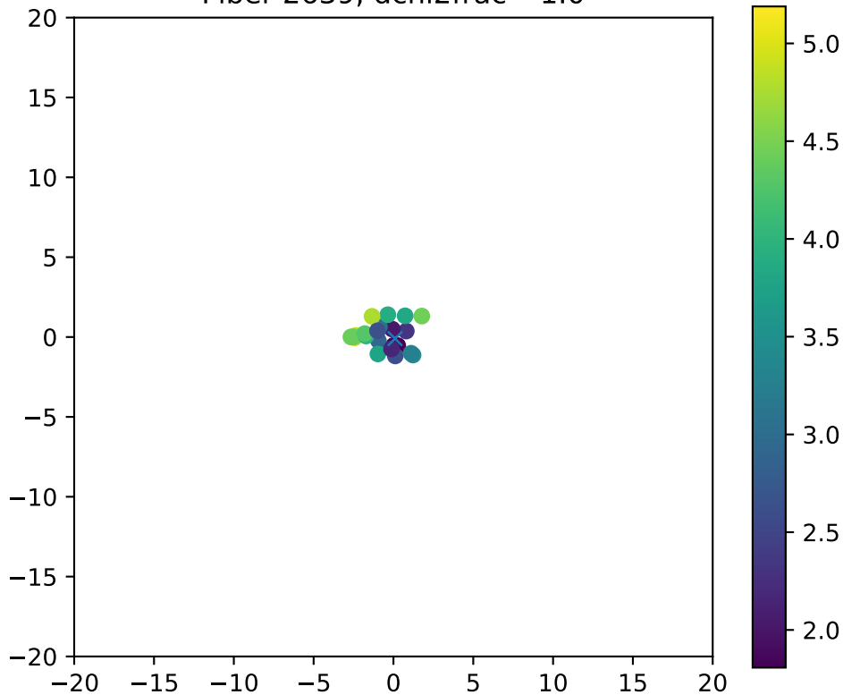
Fiber 2639, dchi2frac= 1.0
