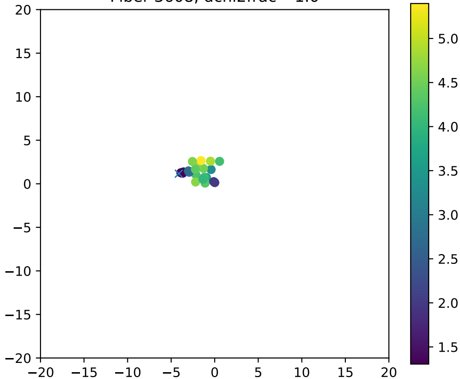
Fiber 3608, dchi2frac= 1.0
