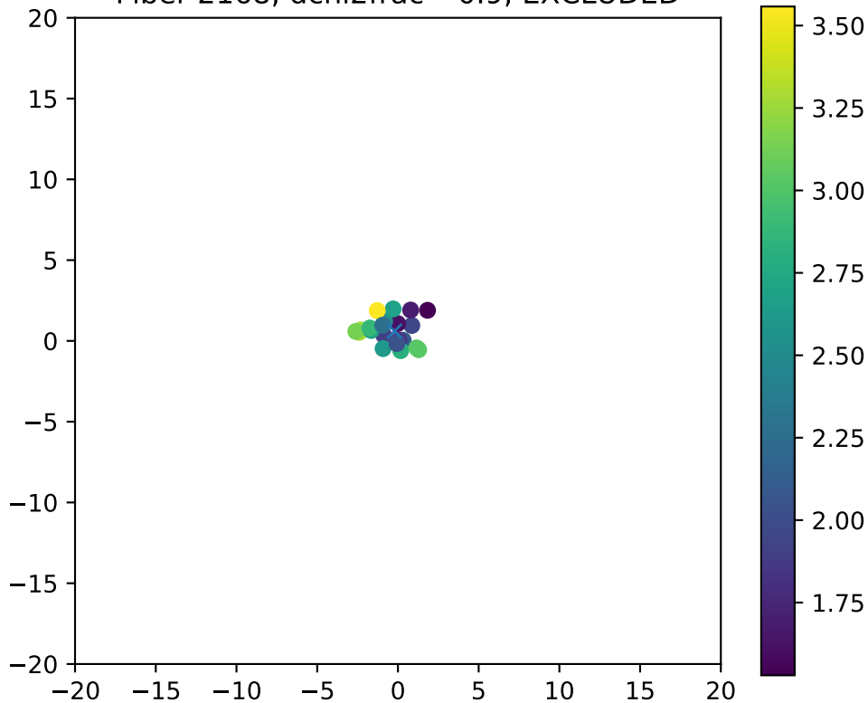
Fiber 2168, dchi2frac= 0.9, EXCLUDED
