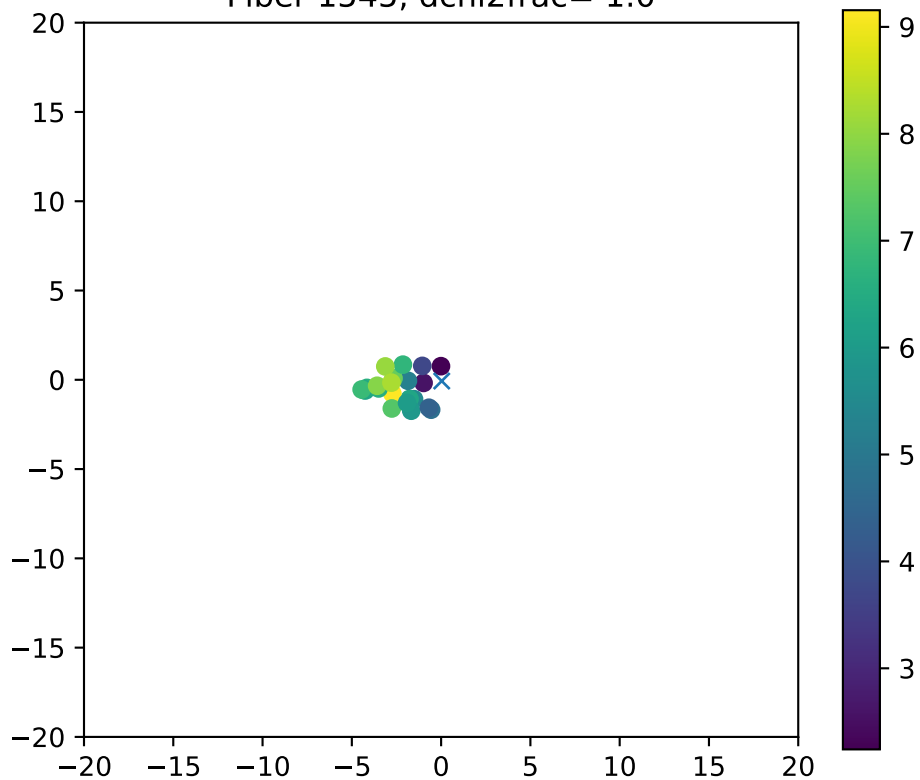
Fiber 1545, dchi2frac= 1.0
