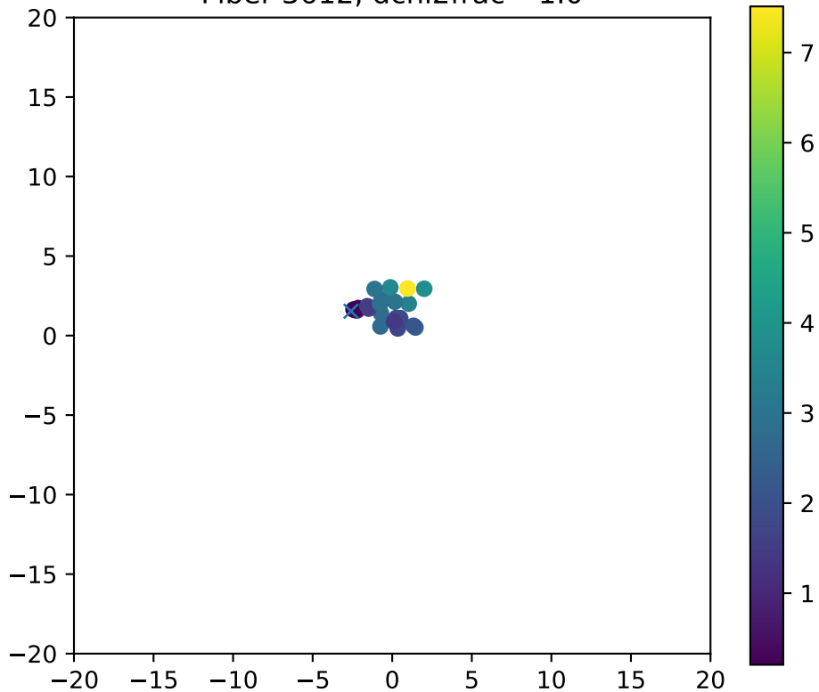
Fiber 3612, dchi2frac= 1.0
