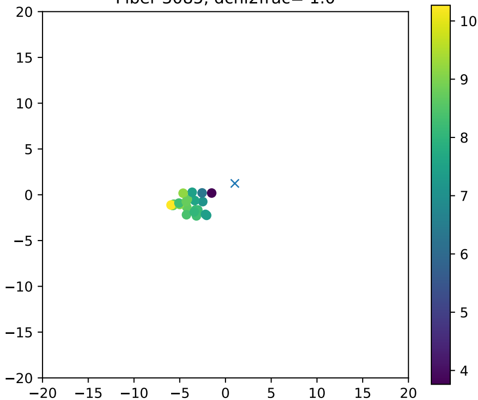
Fiber 3085, dchi2frac= 1.0
