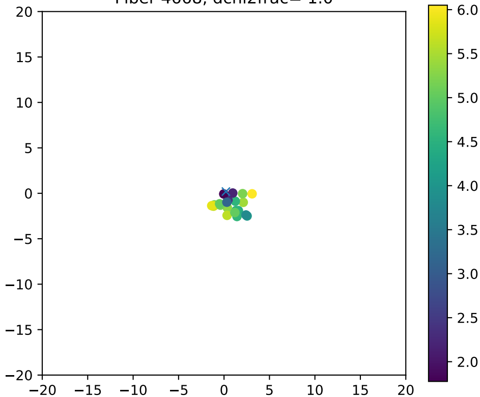
Fiber 4668, dchi2frac= 1.0
