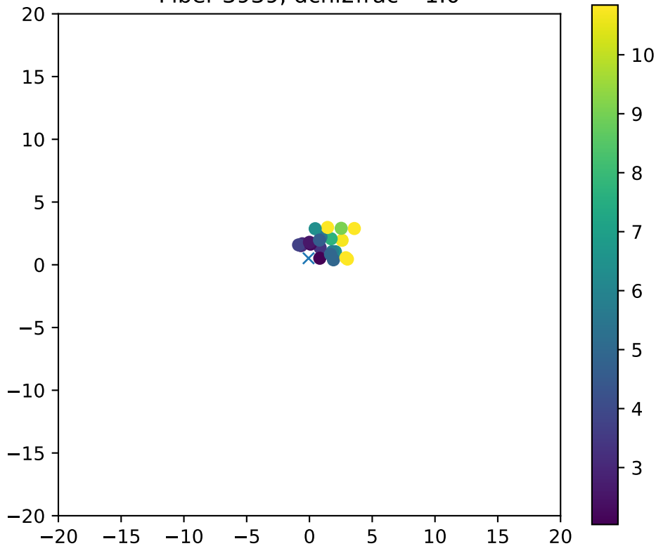
Fiber 3939, dchi2frac= 1.0
