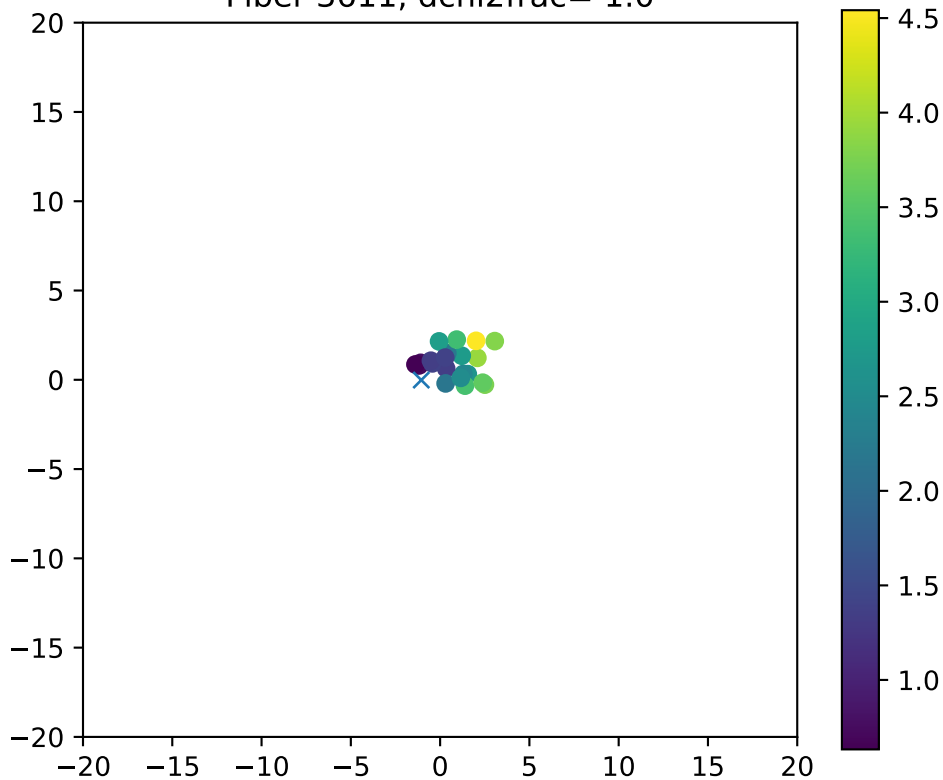
Fiber 3611, dchi2frac= 1.0
