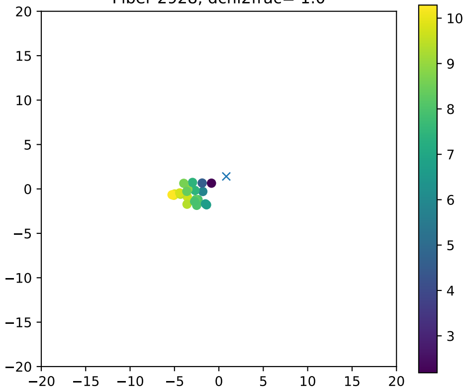
Fiber 2928, dchi2frac= 1.0
