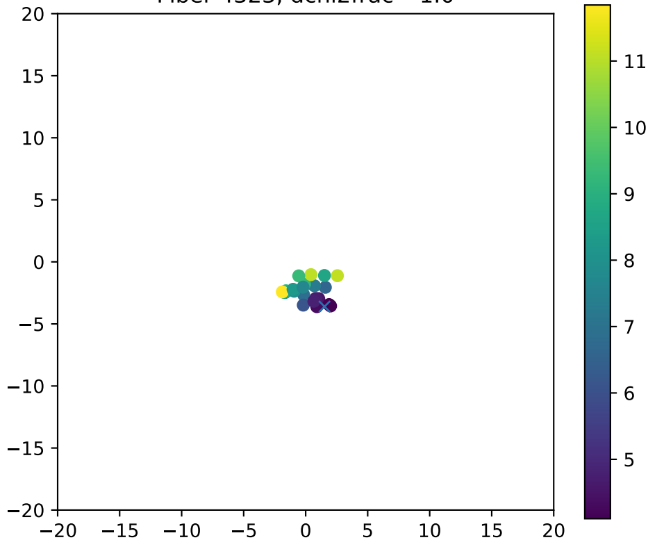
Fiber 4323, dchi2frac= 1.0
