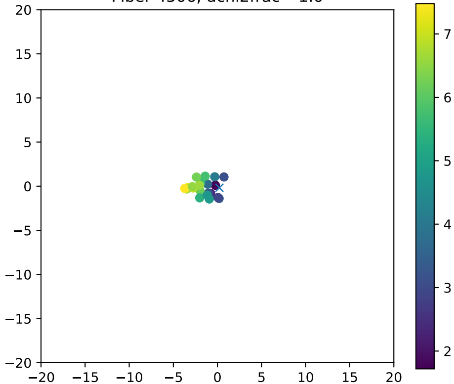
Fiber 4506, dchi2frac= 1.0
