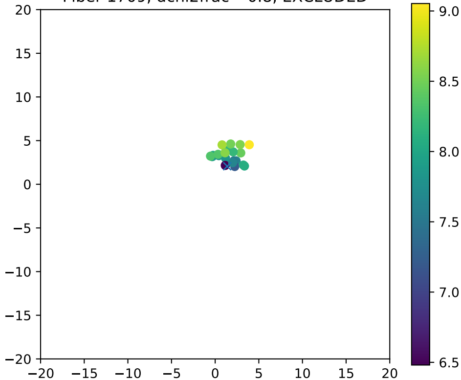
Fiber 1709, dchi2frac= 0.8, EXCLUDED
