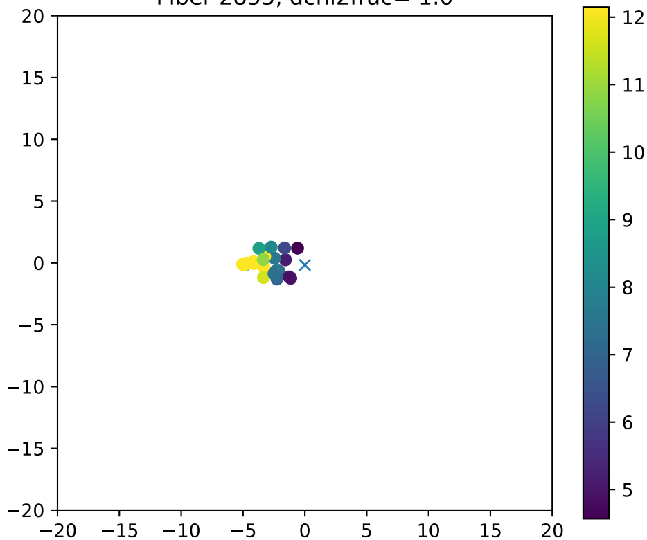
Fiber 2855, dchi2frac= 1.0
