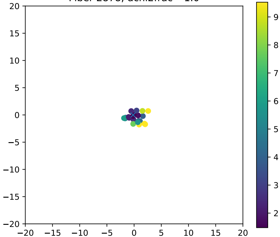
Fiber 2878, dchi2frac= 1.0
