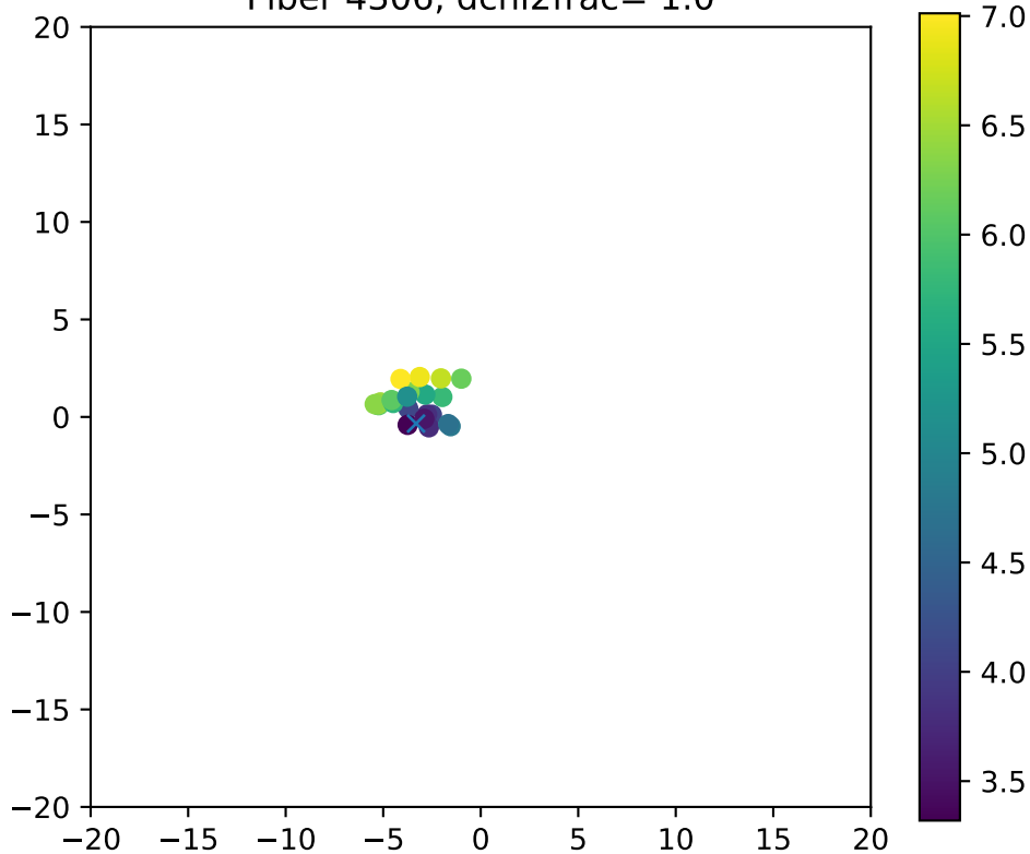
Fiber 4306, dchi2frac= 1.0
