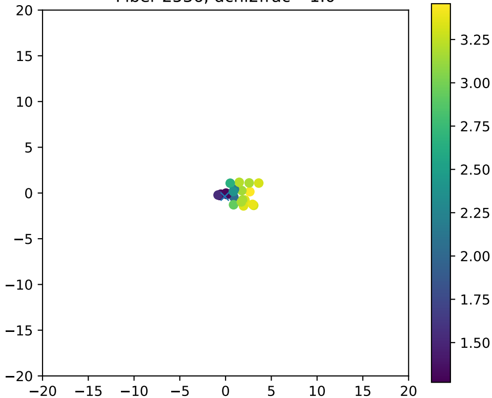
Fiber 2536, dchi2frac= 1.0
