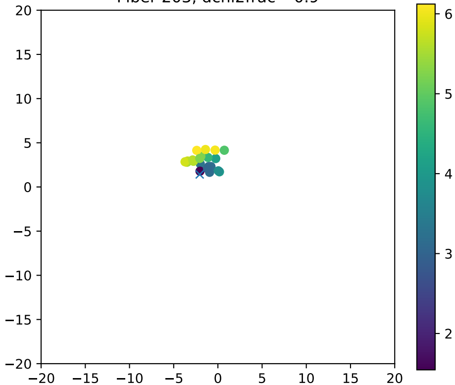
Fiber 203, dchi2frac= 0.9
