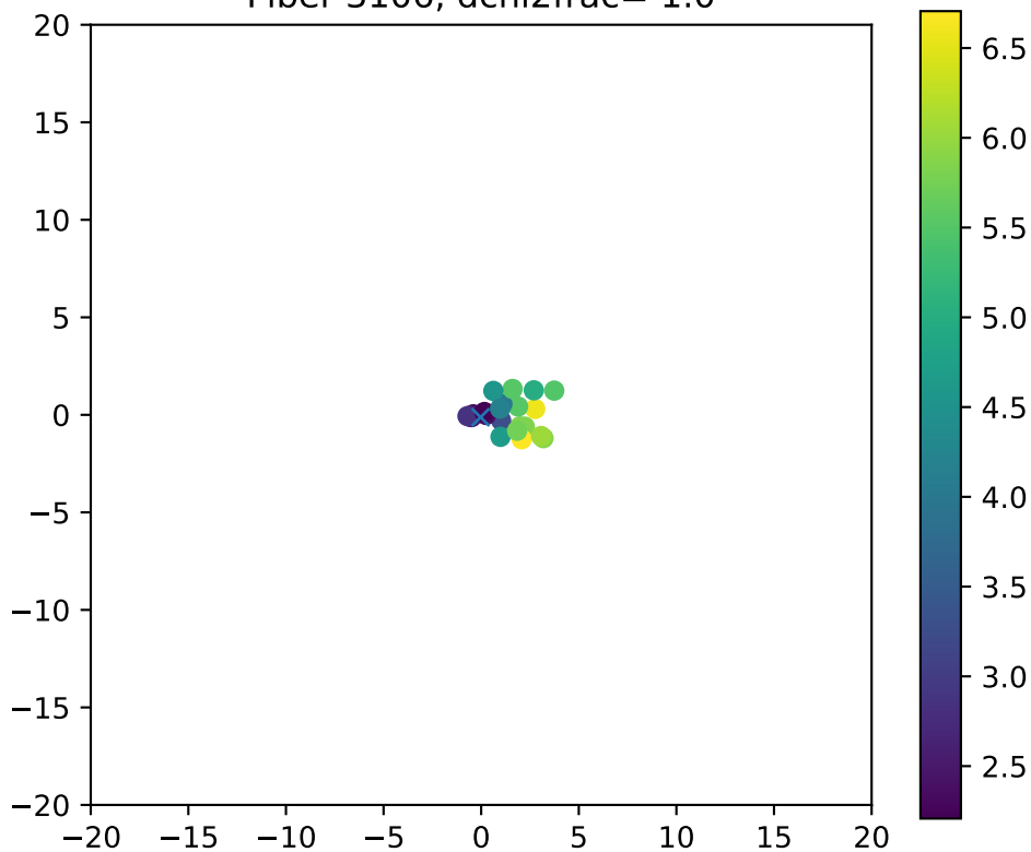
Fiber 3106, dchi2frac= 1.0
