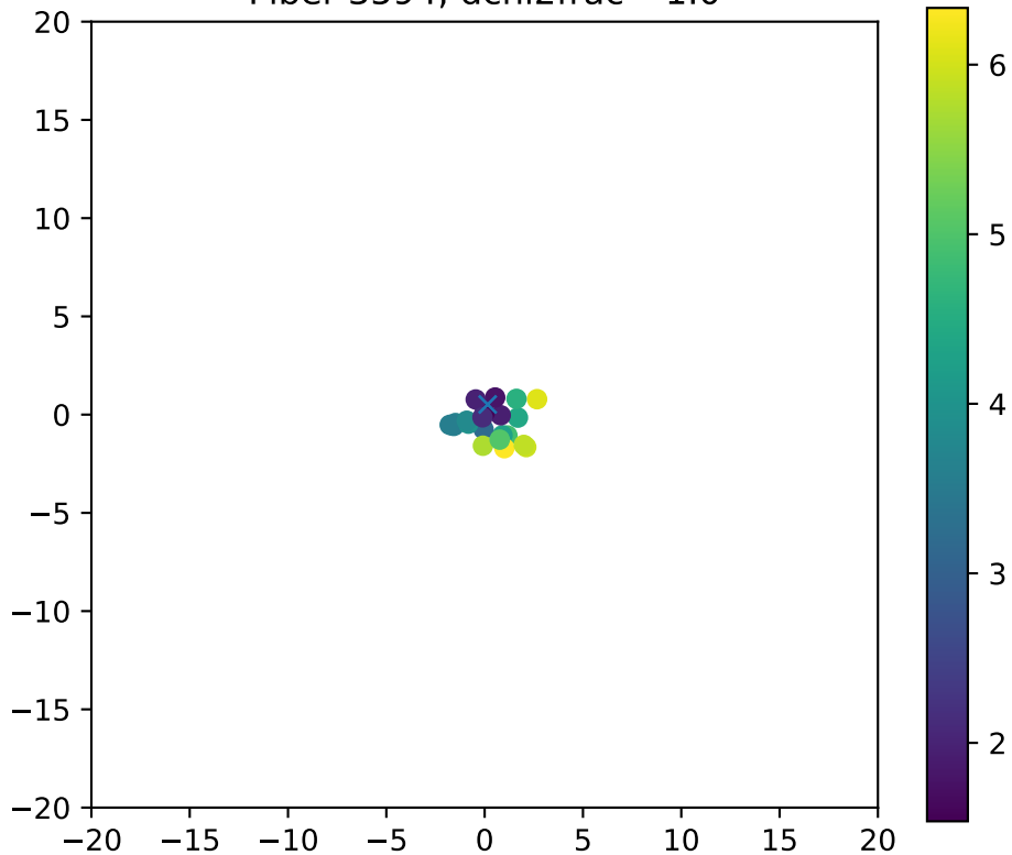
Fiber 3594, dchi2frac= 1.0
