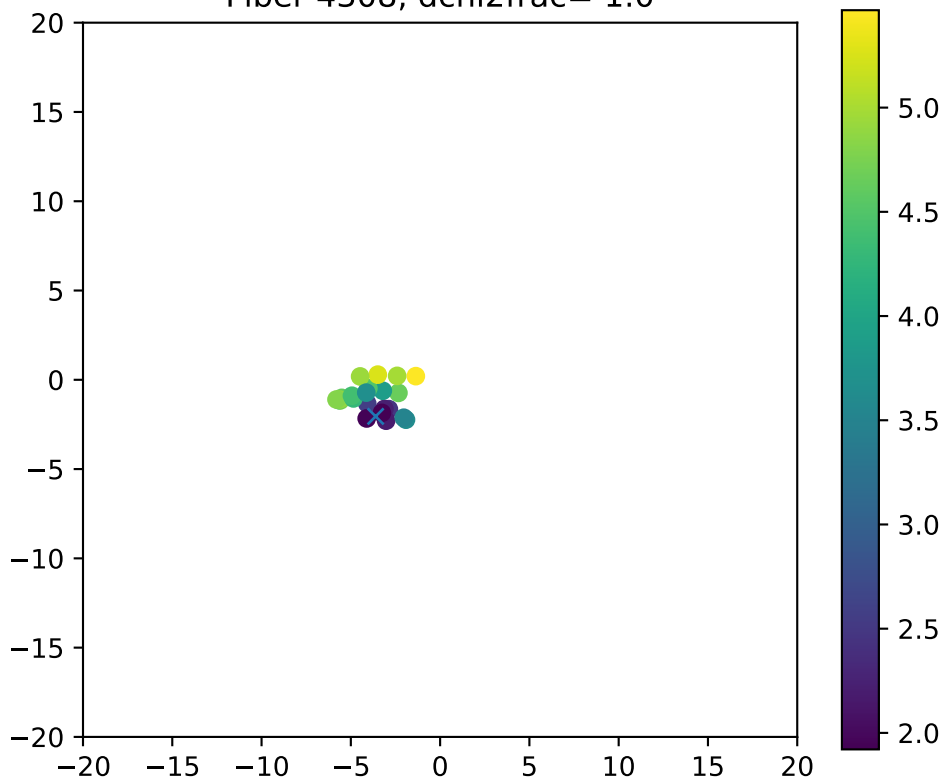
Fiber 4308, dchi2frac= 1.0
