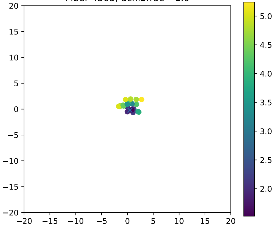
Fiber 4363, dchi2frac= 1.0
