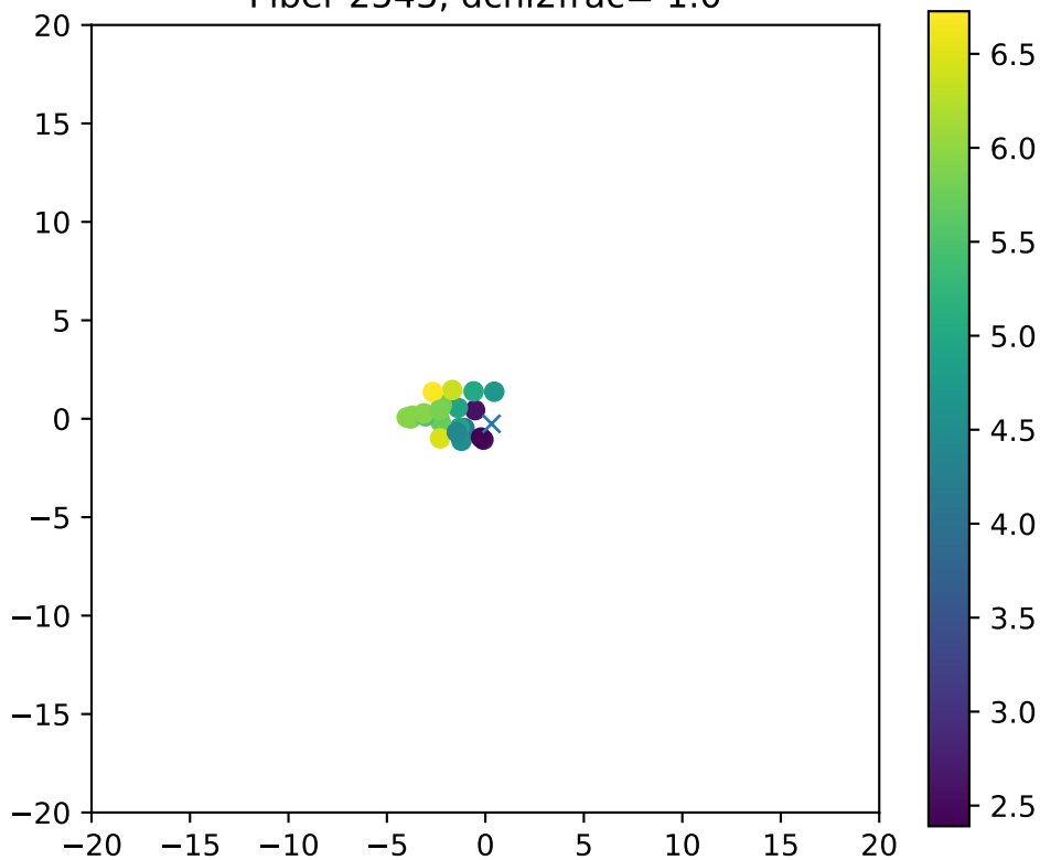
Fiber 2543, dchi2frac= 1.0
