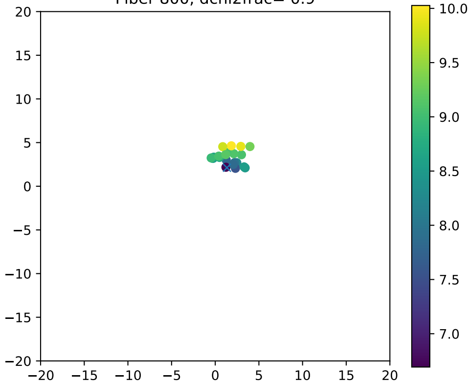
Fiber 800, dchi2frac= 0.9
