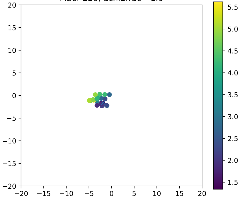
Fiber 220, dchi2frac= 1.0
