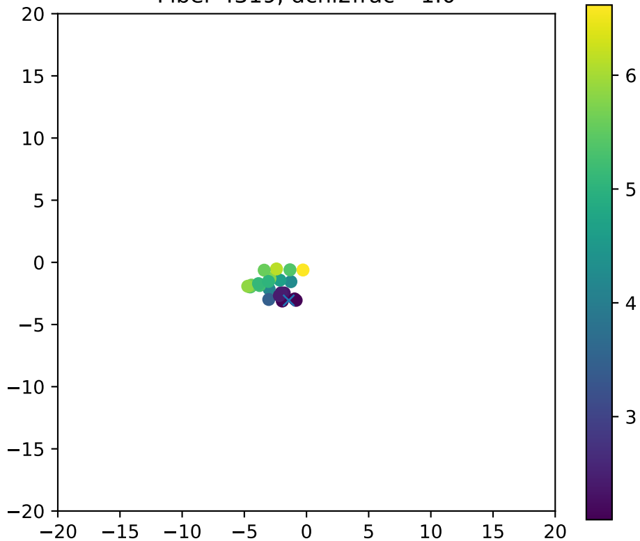
Fiber 4319, dchi2frac= 1.0
