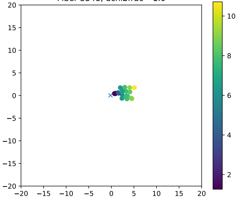
Fiber 3348, dchi2frac= 1.0
