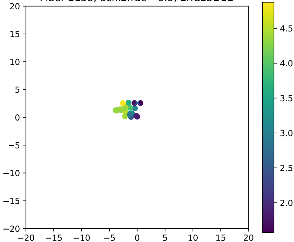
Fiber 2158, dchi2frac= 0.9, EXCLUDED
