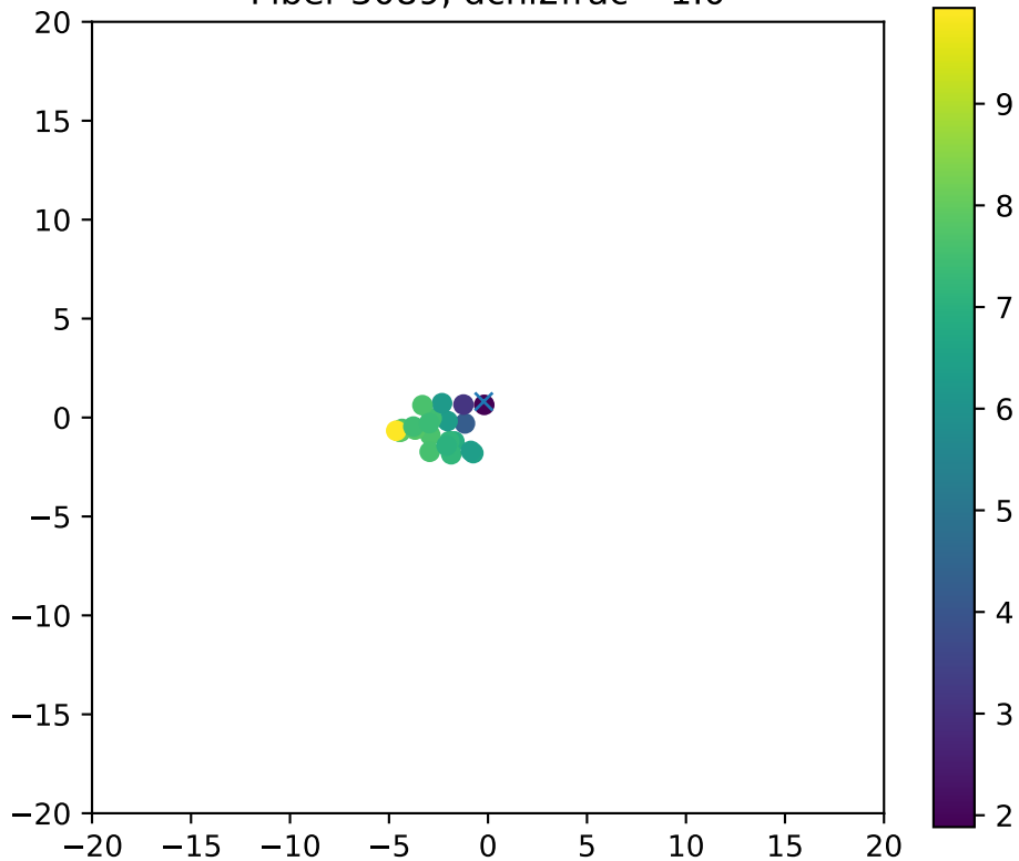
Fiber 3089, dchi2frac= 1.0
