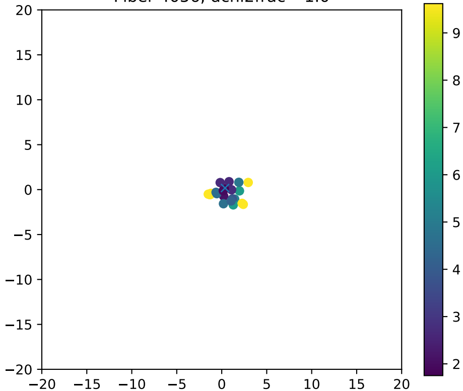
Fiber 4056, dchi2frac= 1.0
