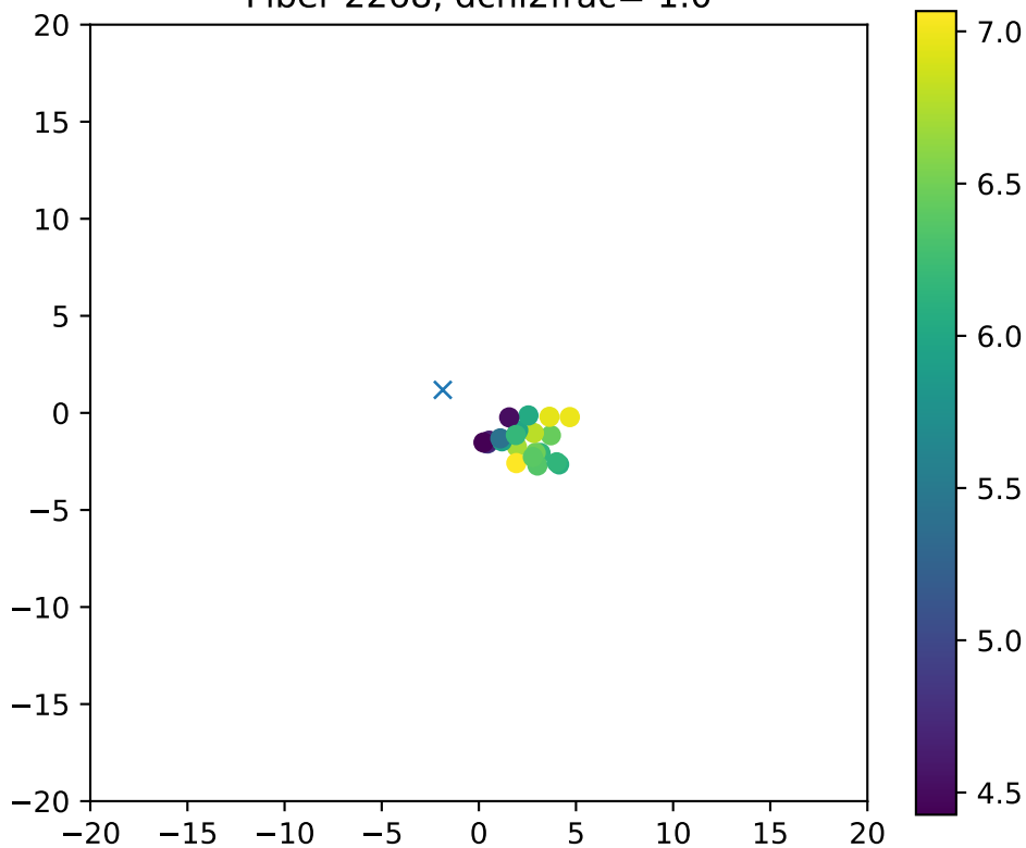
Fiber 2268, dchi2frac= 1.0
