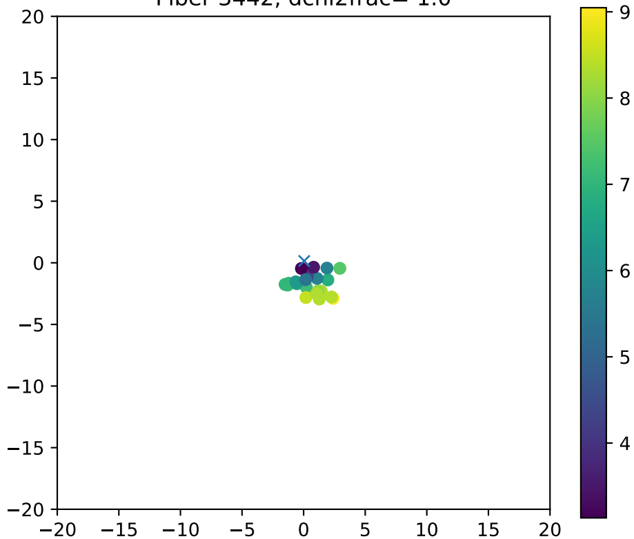
Fiber 3442, dchi2frac= 1.0
