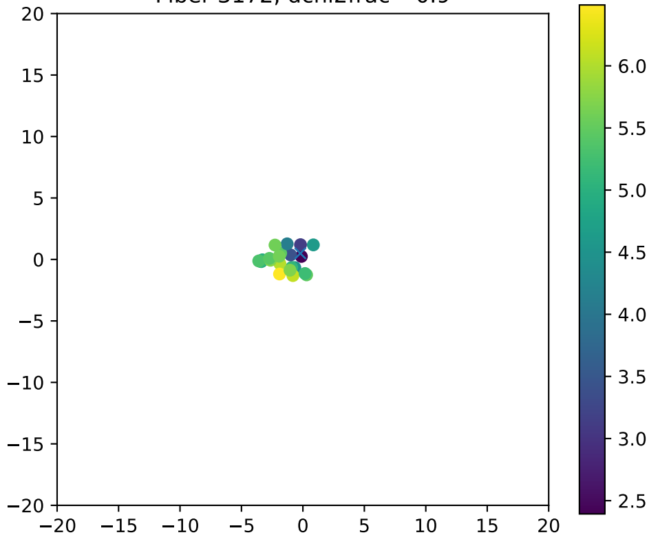
Fiber 3172, dchi2frac= 0.9
