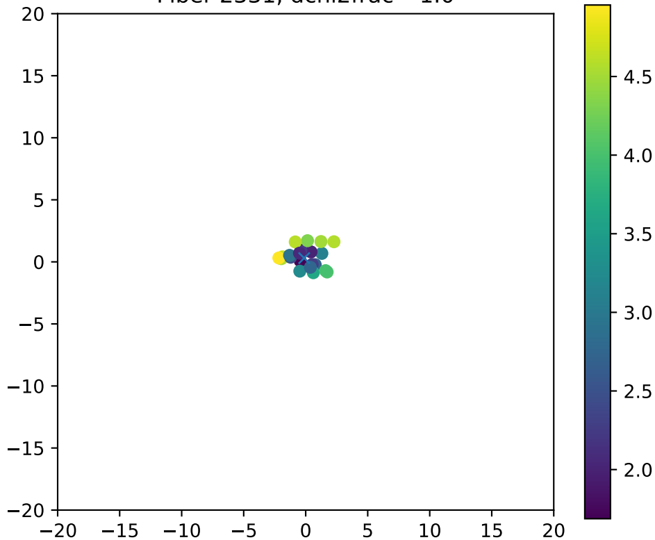
Fiber 2331, dchi2frac= 1.0
