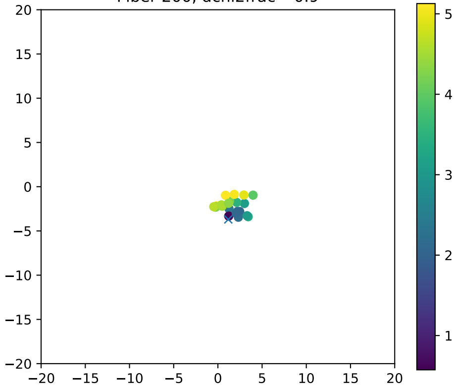
Fiber 200, dchi2frac= 0.9
