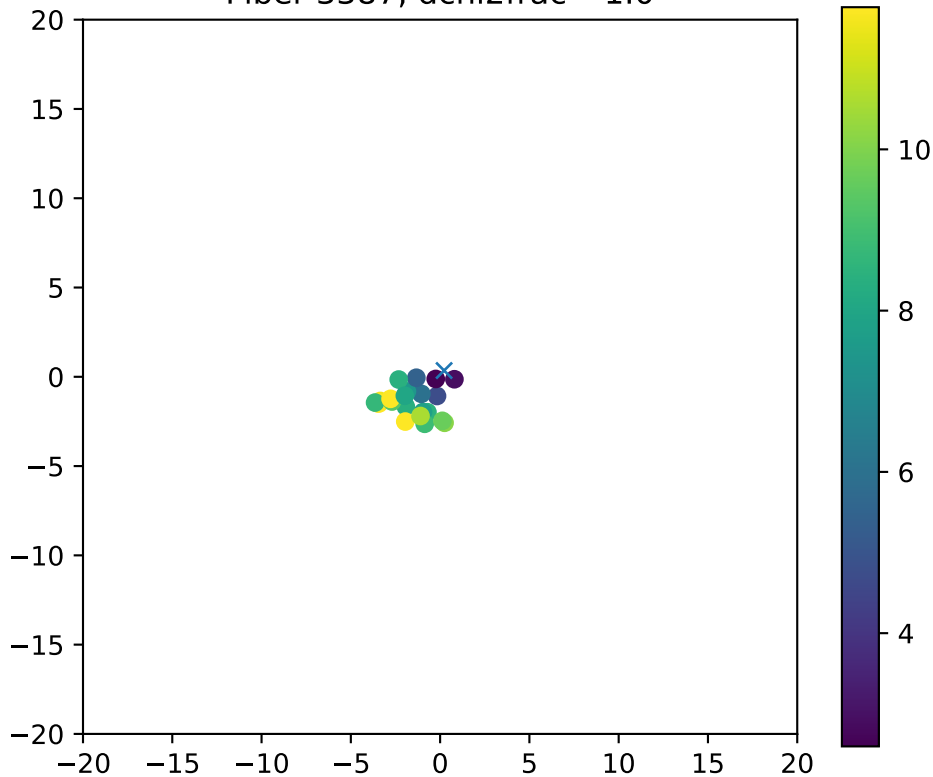
Fiber 3387, dchi2frac= 1.0
