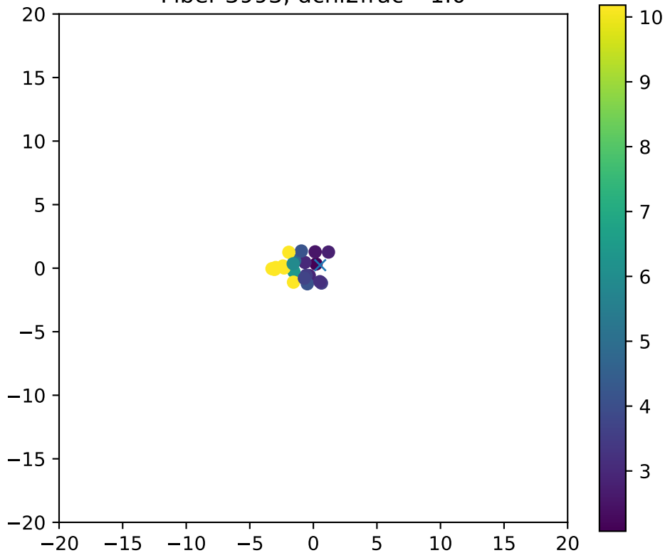
Fiber 3993, dchi2frac= 1.0
