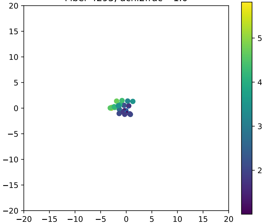
Fiber 4293, dchi2frac= 1.0
