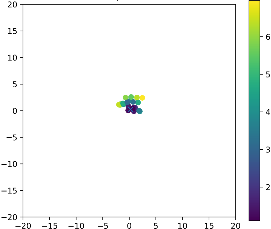
Fiber 4311, dchi2frac= 1.0
