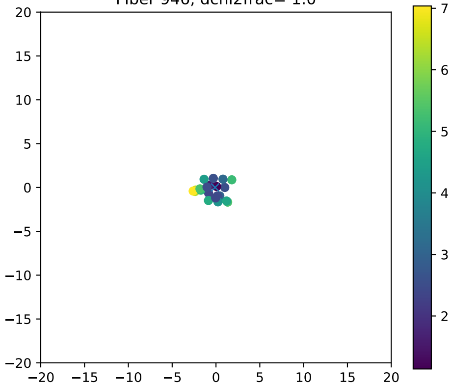
Fiber 946, dchi2frac= 1.0
