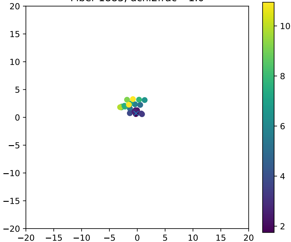
Fiber 1883, dchi2frac= 1.0
