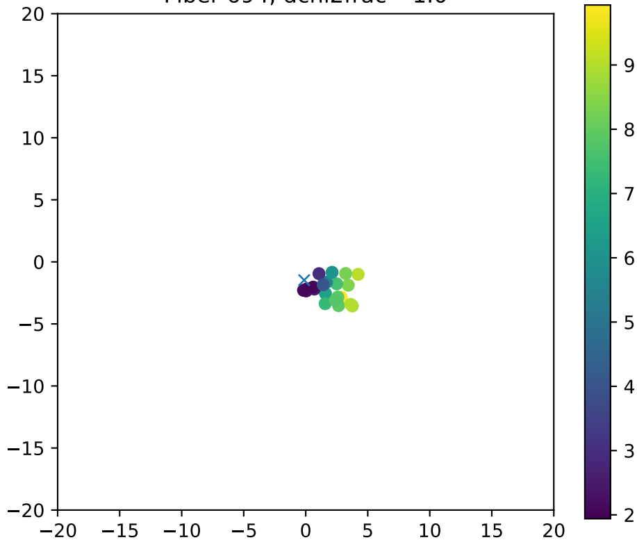
Fiber 694, dchi2frac= 1.0
