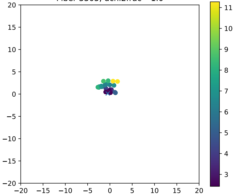
Fiber 3305, dchi2frac= 1.0
