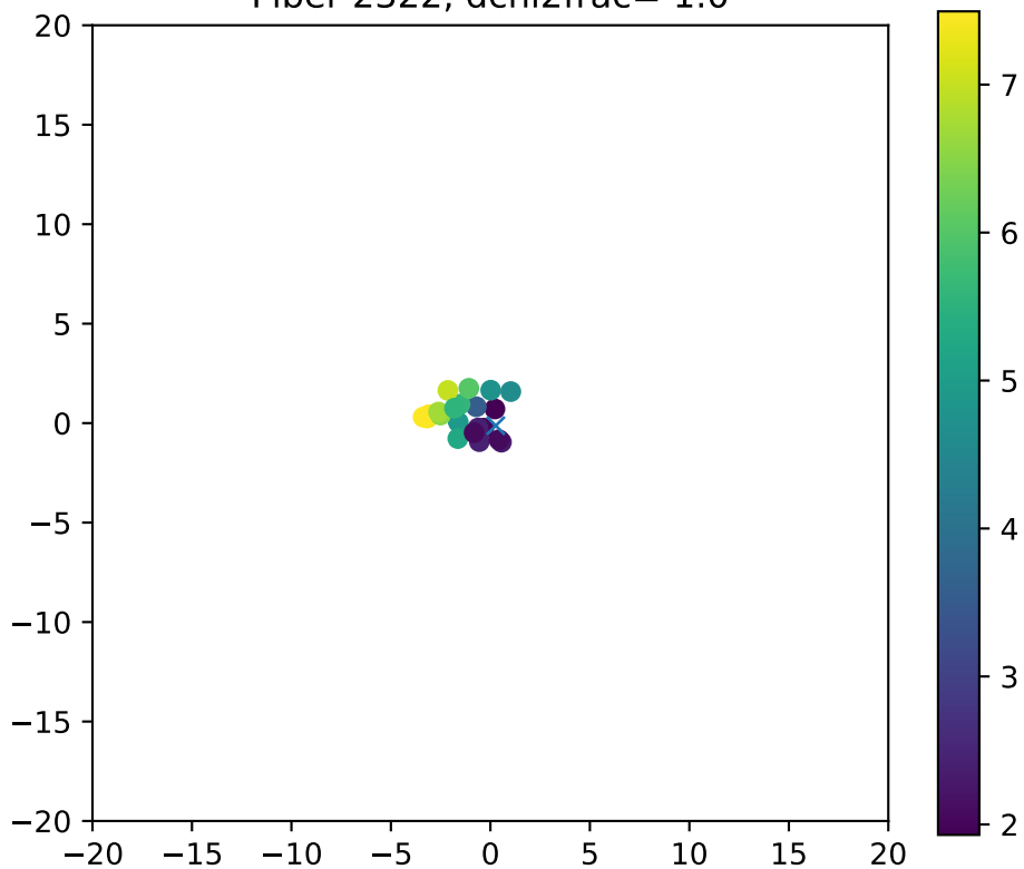
Fiber 2322, dchi2frac= 1.0
