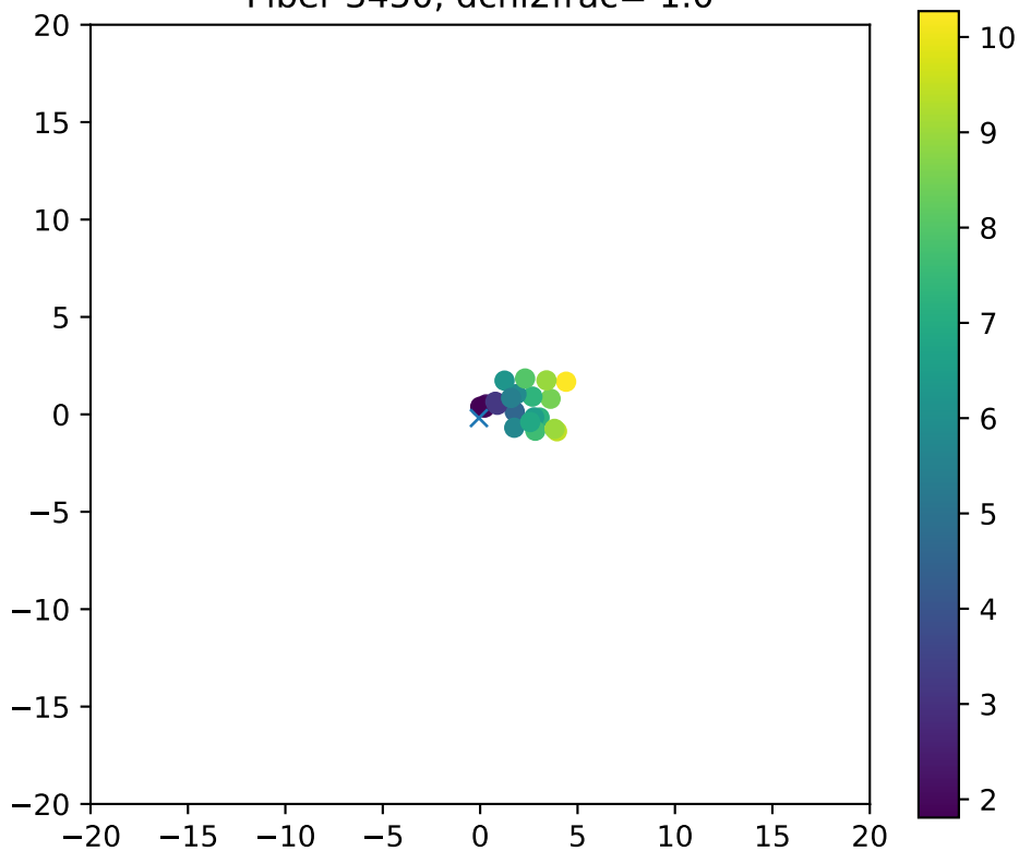
Fiber 3450, dchi2frac= 1.0
