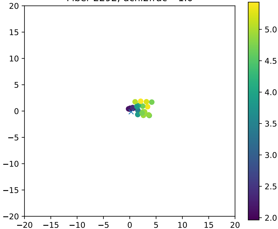
Fiber 2292, dchi2frac= 1.0
