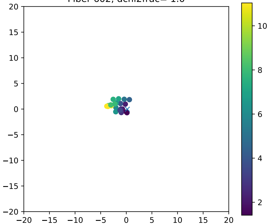
Fiber 602, dchi2frac= 1.0
