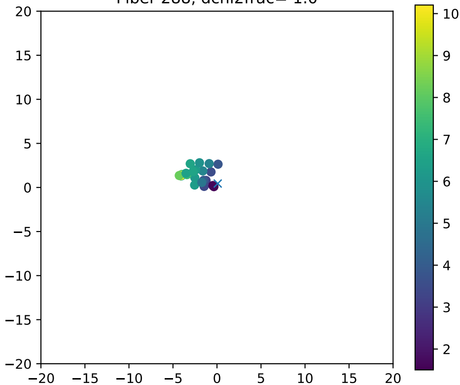
Fiber 288, dchi2frac= 1.0
