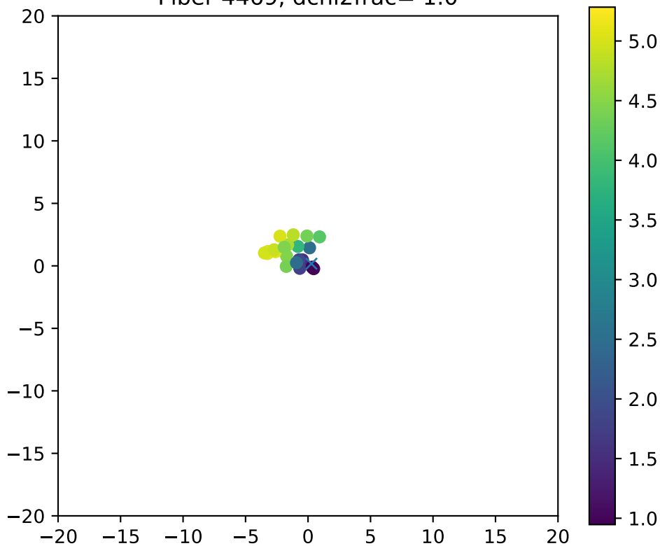
Fiber 4469, dchi2frac= 1.0
