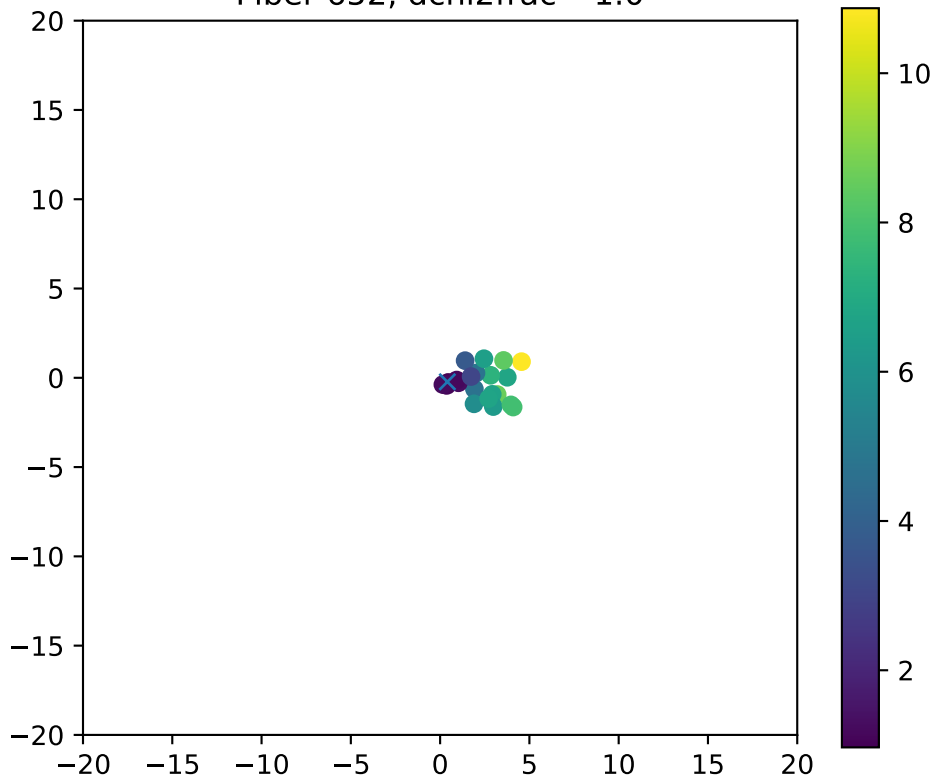
Fiber 652, dchi2frac= 1.0
