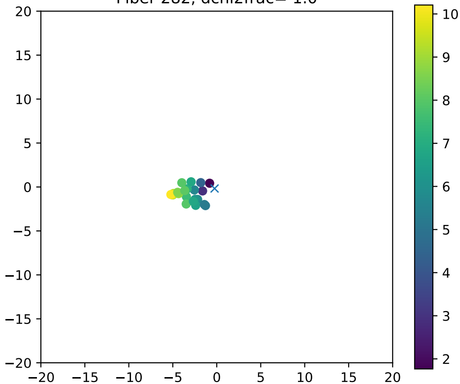
Fiber 282, dchi2frac= 1.0
