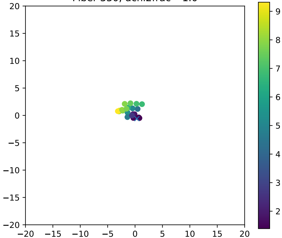
Fiber 330, dchi2frac= 1.0
