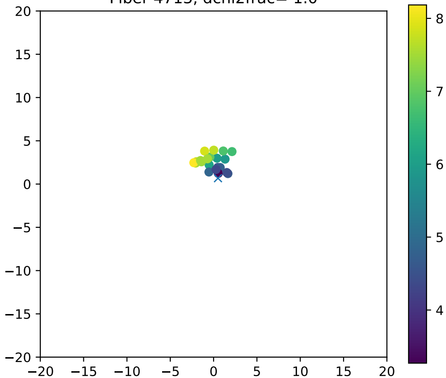
Fiber 4713, dchi2frac= 1.0
