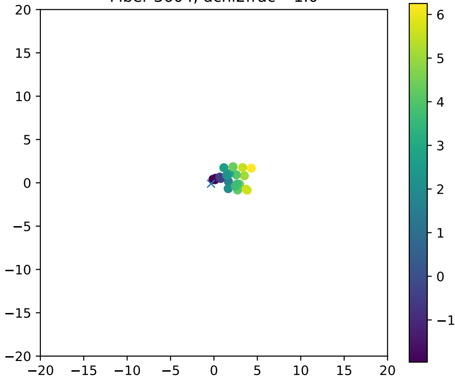
Fiber 3604, dchi2frac= 1.0
