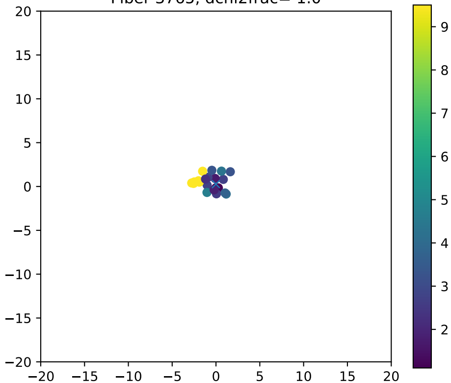
Fiber 3765, dchi2frac= 1.0
