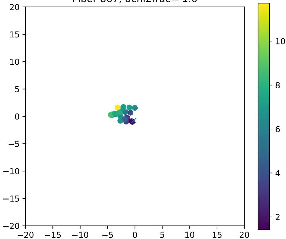
Fiber 867, dchi2frac= 1.0
