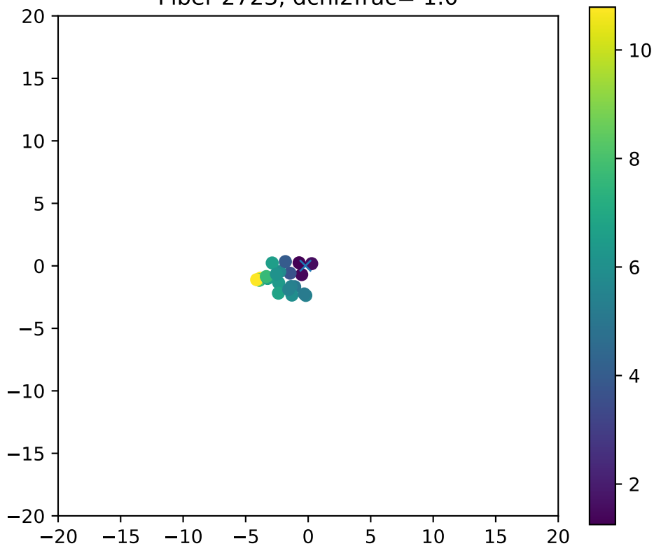
Fiber 2723, dchi2frac= 1.0
