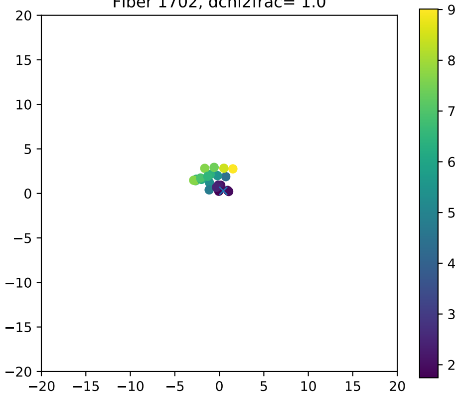
Fiber 1702, dchi2frac= 1.0
