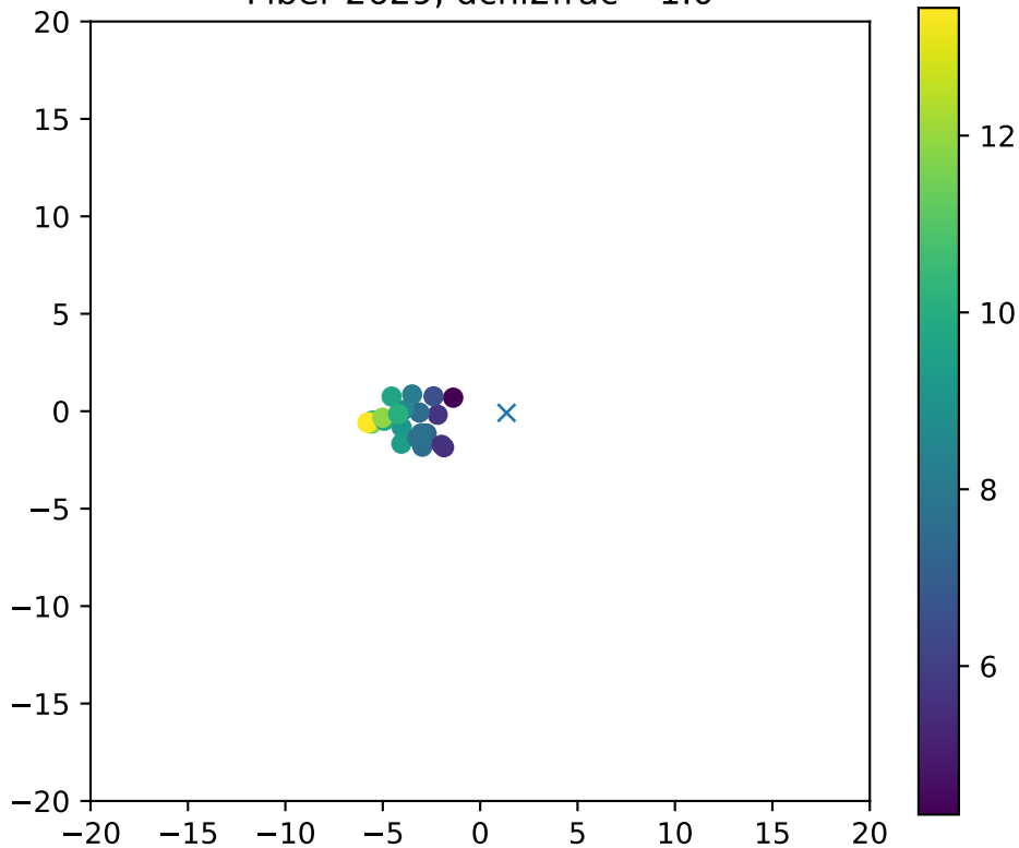
Fiber 2629, dchi2frac= 1.0
