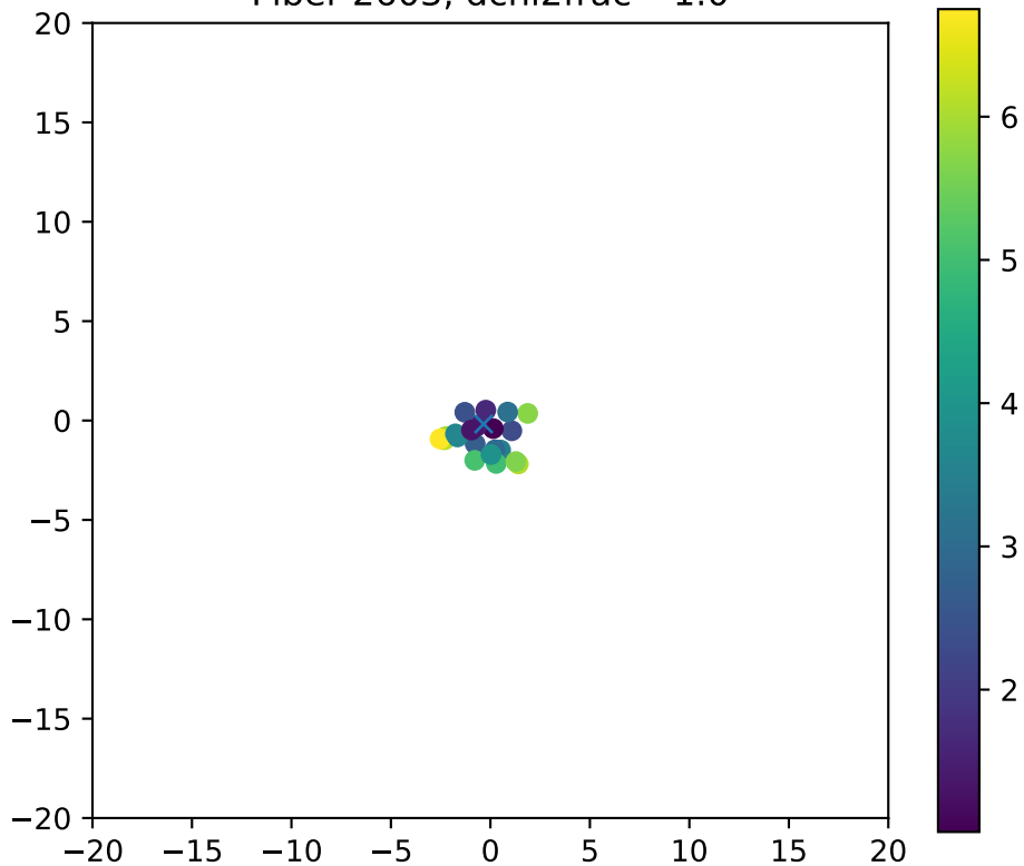
Fiber 2603, dchi2frac= 1.0
