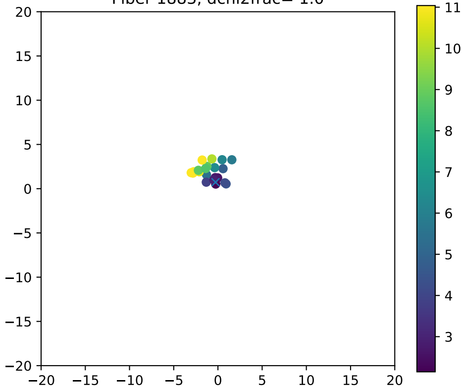
Fiber 1883, dchi2frac= 1.0
