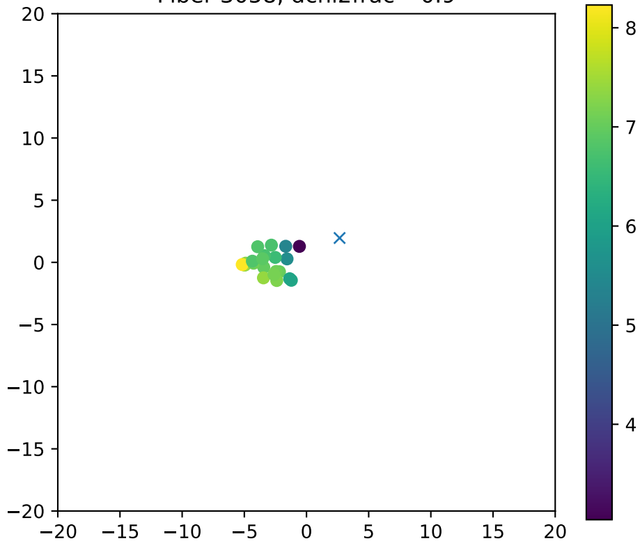
Fiber 3058, dchi2frac= 0.9
