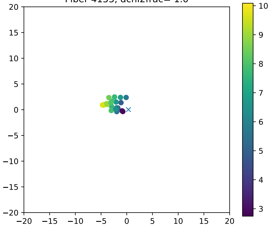
Fiber 4153, dchi2frac= 1.0
