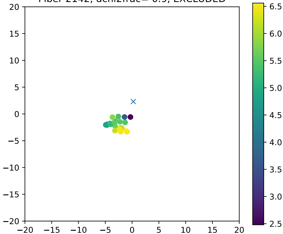
Fiber 2142, dchi2frac= 0.9, EXCLUDED
