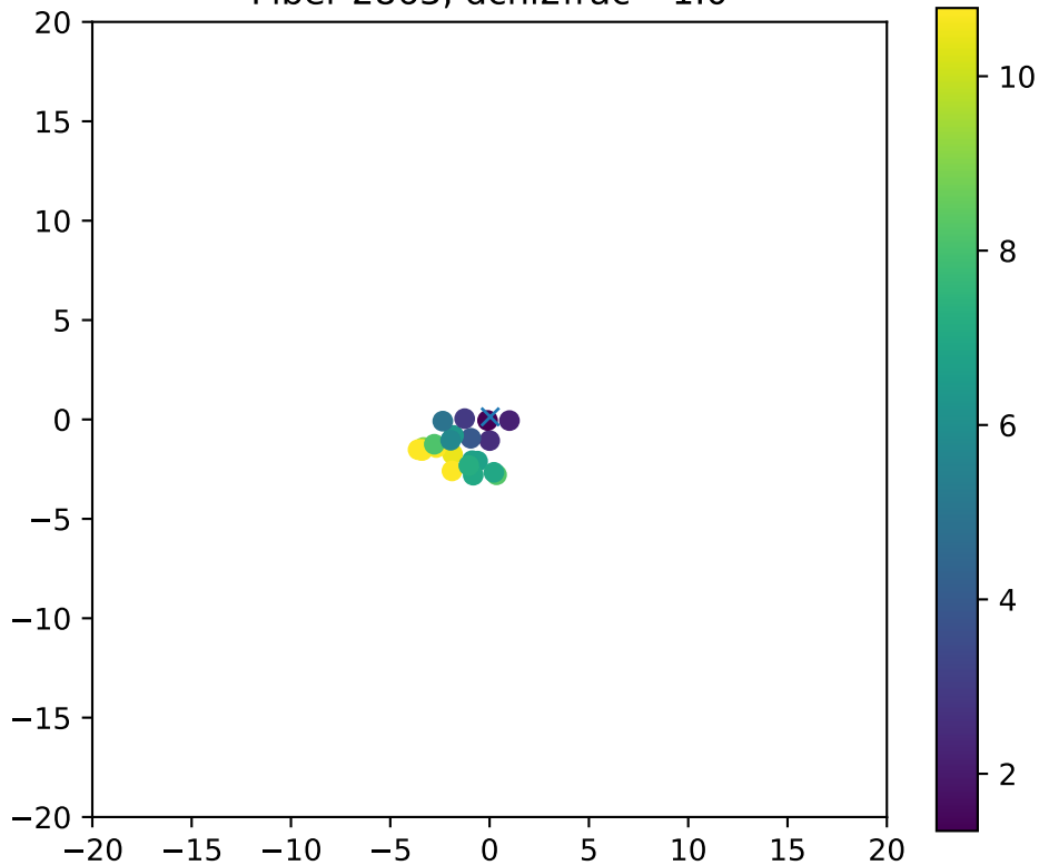
Fiber 2863, dchi2frac= 1.0
