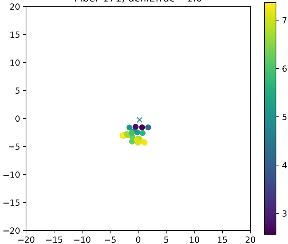
Fiber 171, dchi2frac= 1.0
