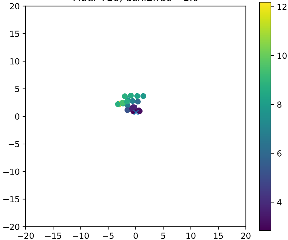
Fiber 720, dchi2frac= 1.0
