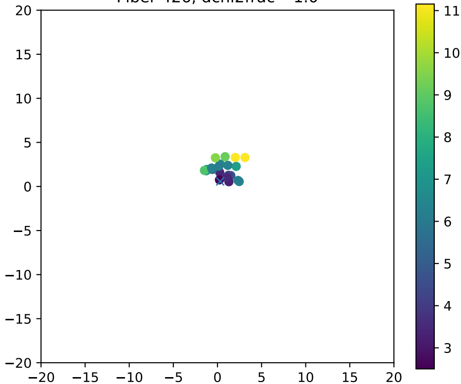
Fiber 426, dchi2frac= 1.0
