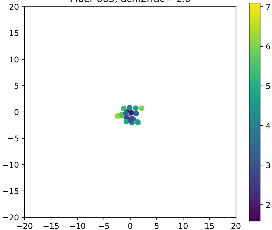
Fiber 663, dchi2frac= 1.0
