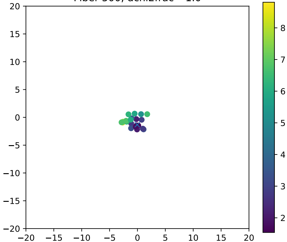
Fiber 500, dchi2frac= 1.0
