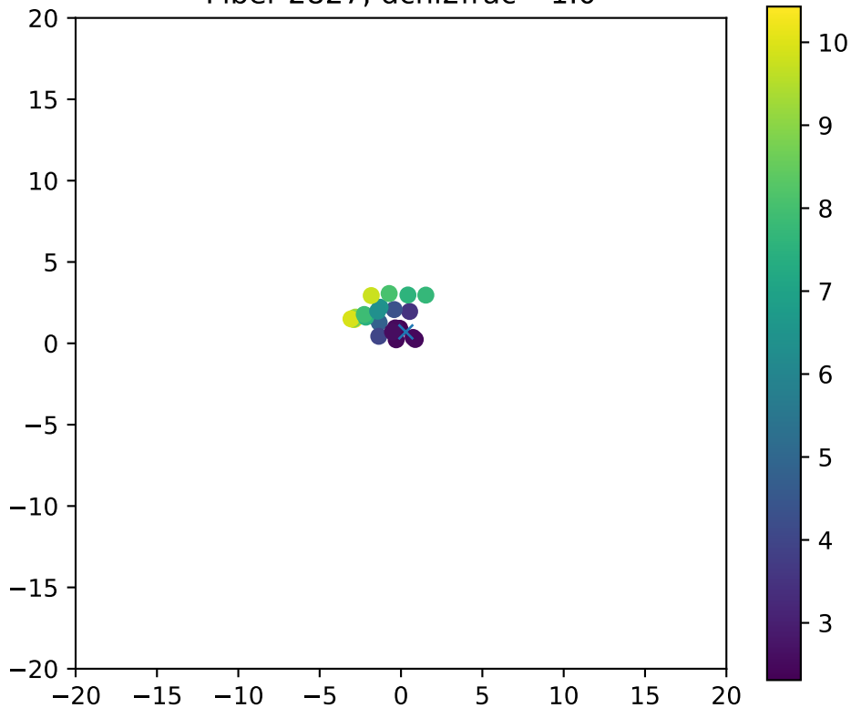
Fiber 2827, dchi2frac= 1.0
