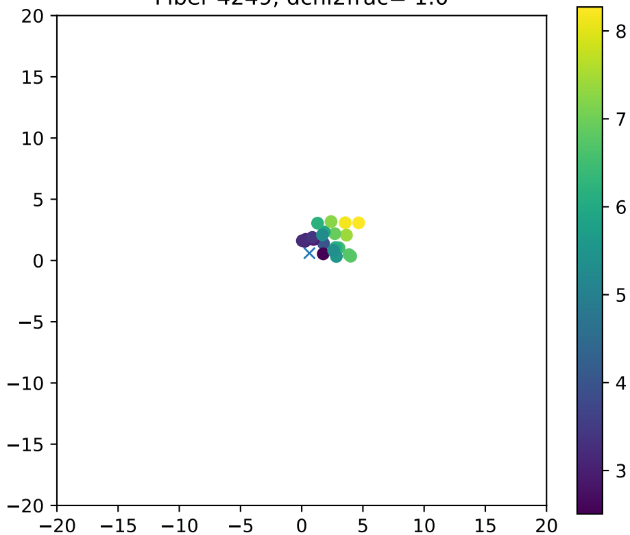
Fiber 4249, dchi2frac= 1.0
