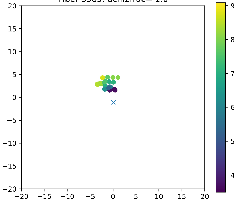
Fiber 3565, dchi2frac= 1.0
