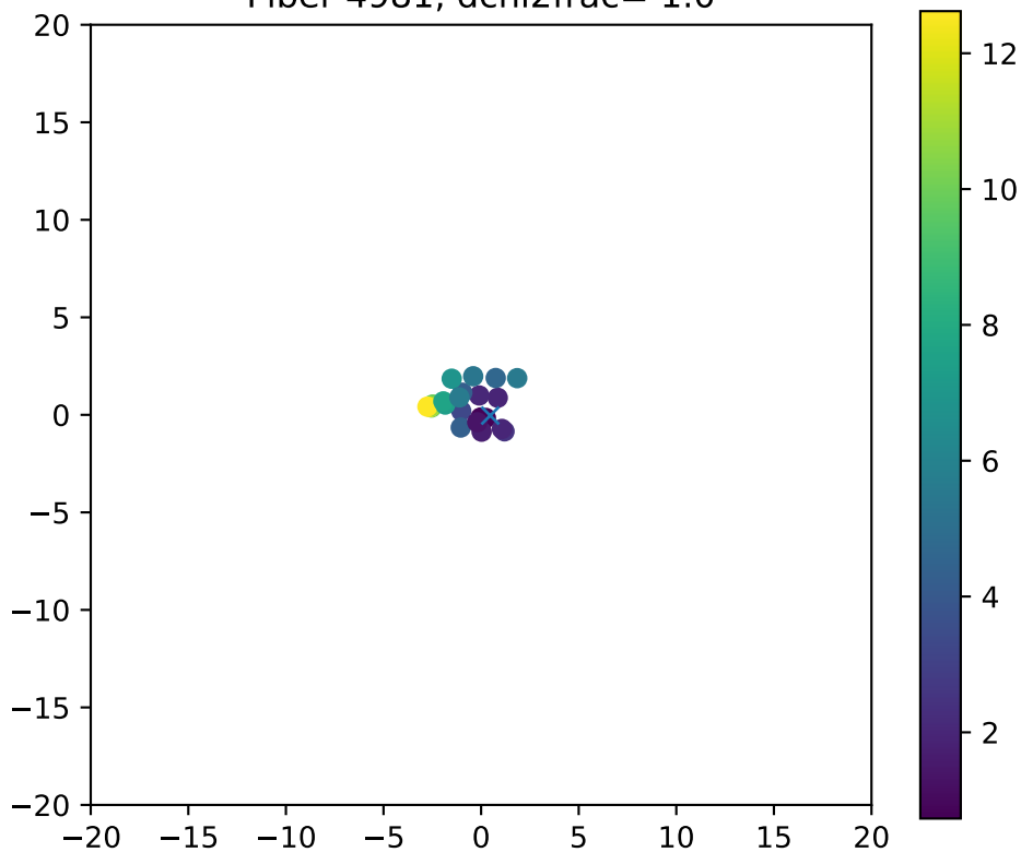
Fiber 4981, dchi2frac= 1.0
