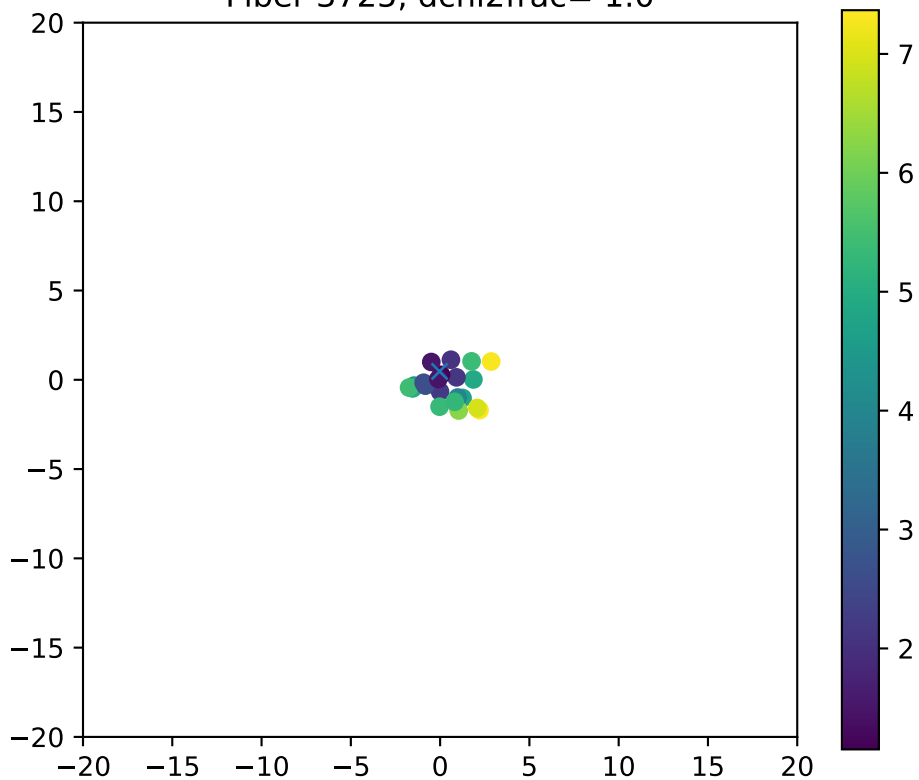
Fiber 3725, dchi2frac= 1.0
