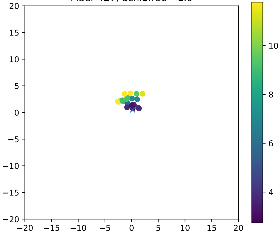
Fiber 427, dchi2frac= 1.0
