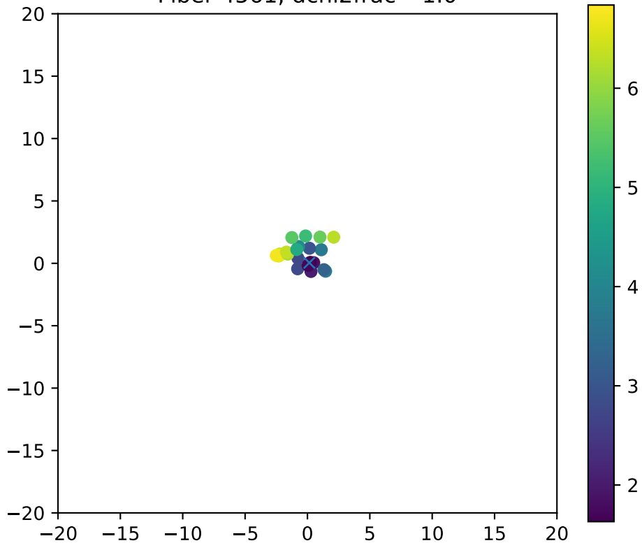
Fiber 4561, dchi2frac= 1.0
