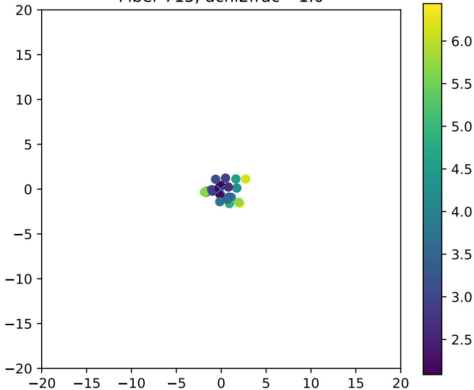
Fiber 715, dchi2frac= 1.0
