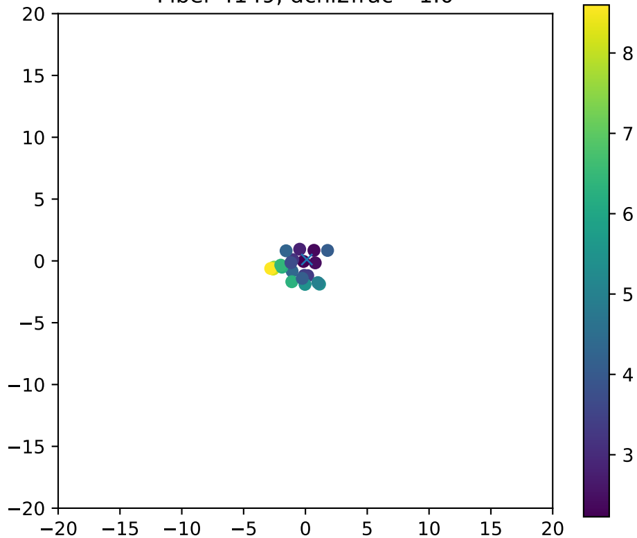
Fiber 4149, dchi2frac= 1.0
