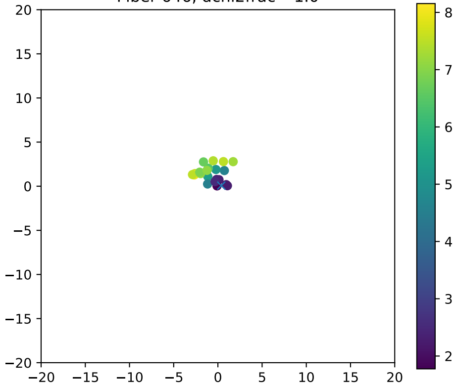
Fiber 646, dchi2frac= 1.0
