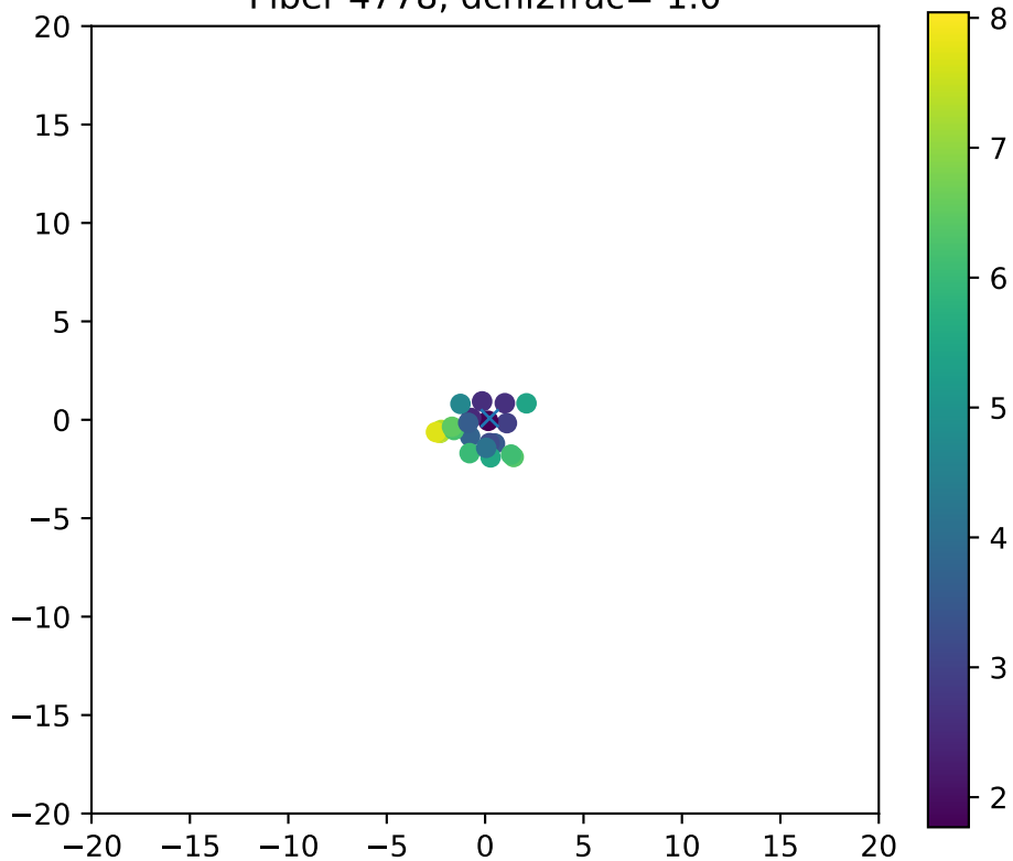
Fiber 4778, dchi2frac= 1.0
