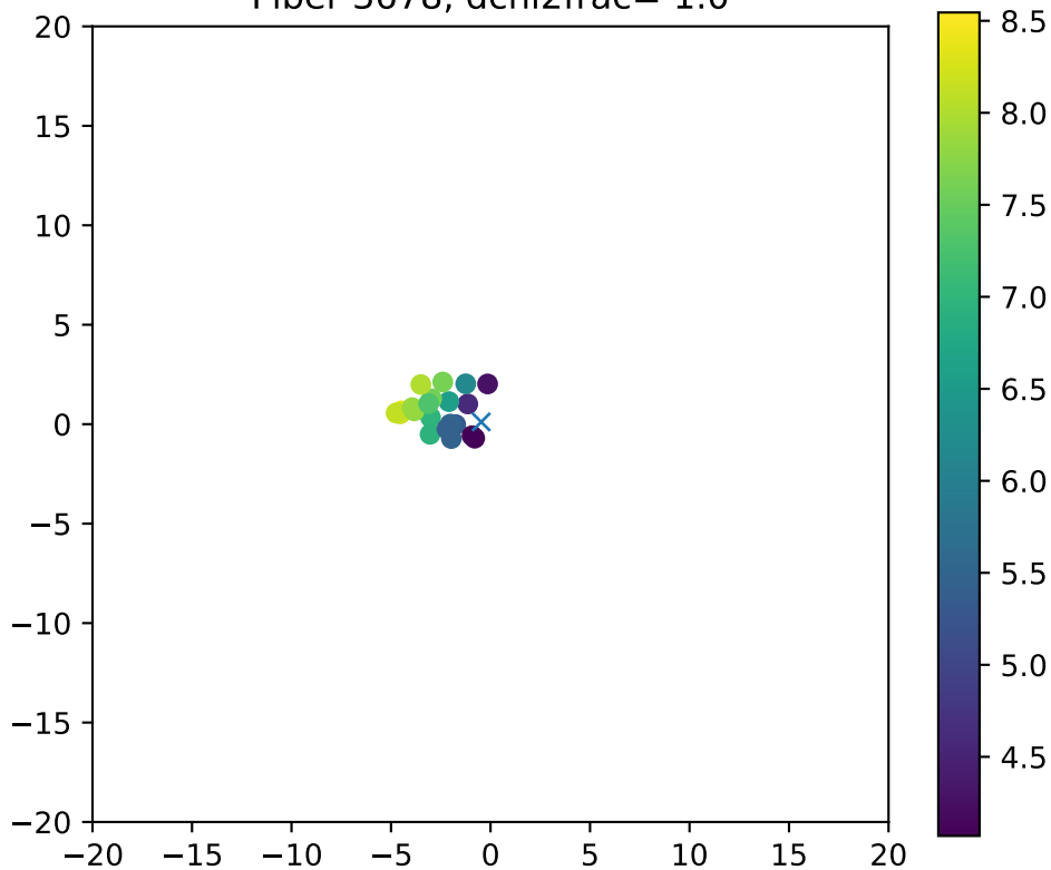
Fiber 3678, dchi2frac= 1.0
