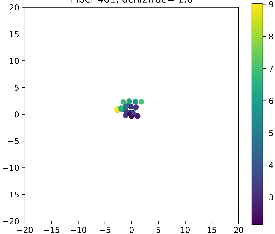
Fiber 401, dchi2frac= 1.0
