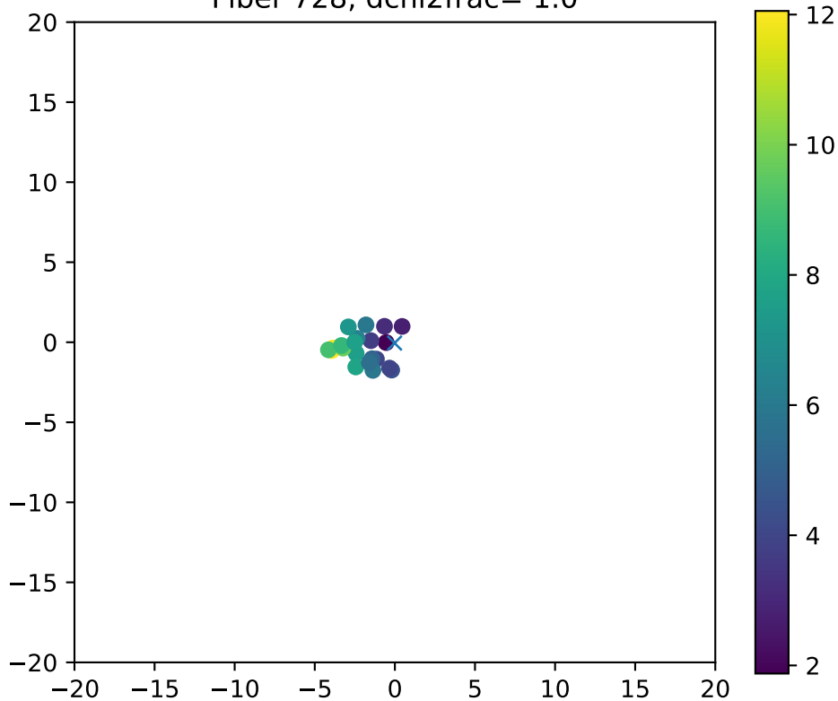
Fiber 728, dchi2frac= 1.0
