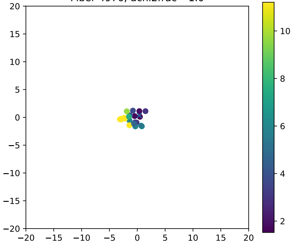
Fiber 4976, dchi2frac= 1.0
