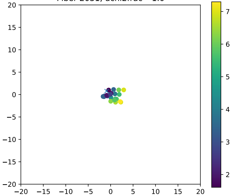
Fiber 2031, dchi2frac= 1.0
