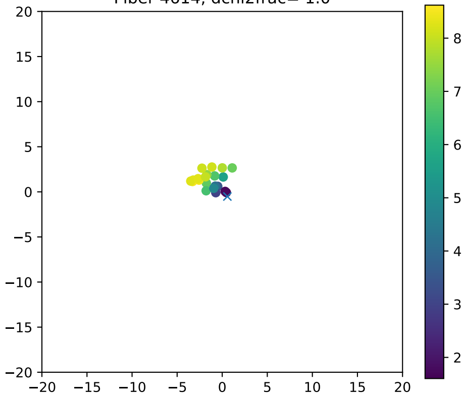
Fiber 4614, dchi2frac= 1.0
