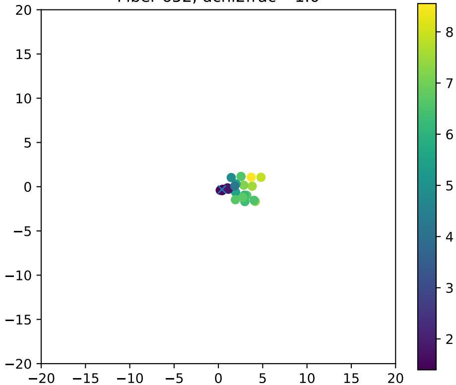
Fiber 652, dchi2frac= 1.0
