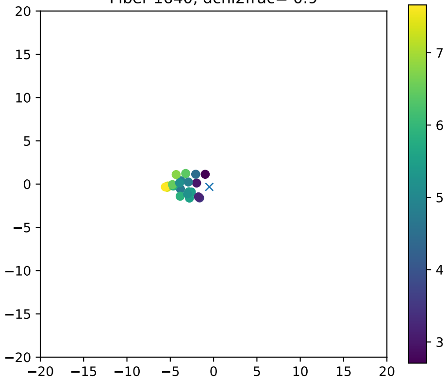
Fiber 1640, dchi2frac= 0.9
