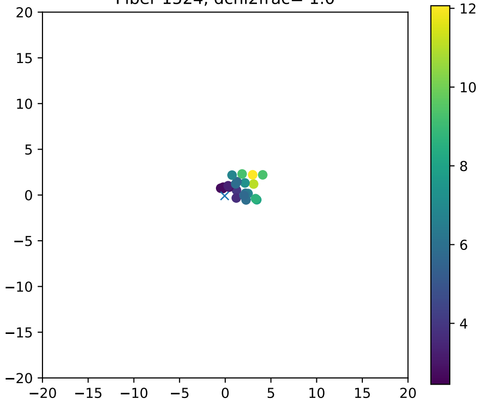
Fiber 1524, dchi2frac= 1.0
