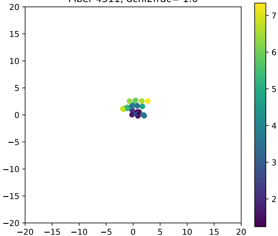
Fiber 4311, dchi2frac= 1.0
