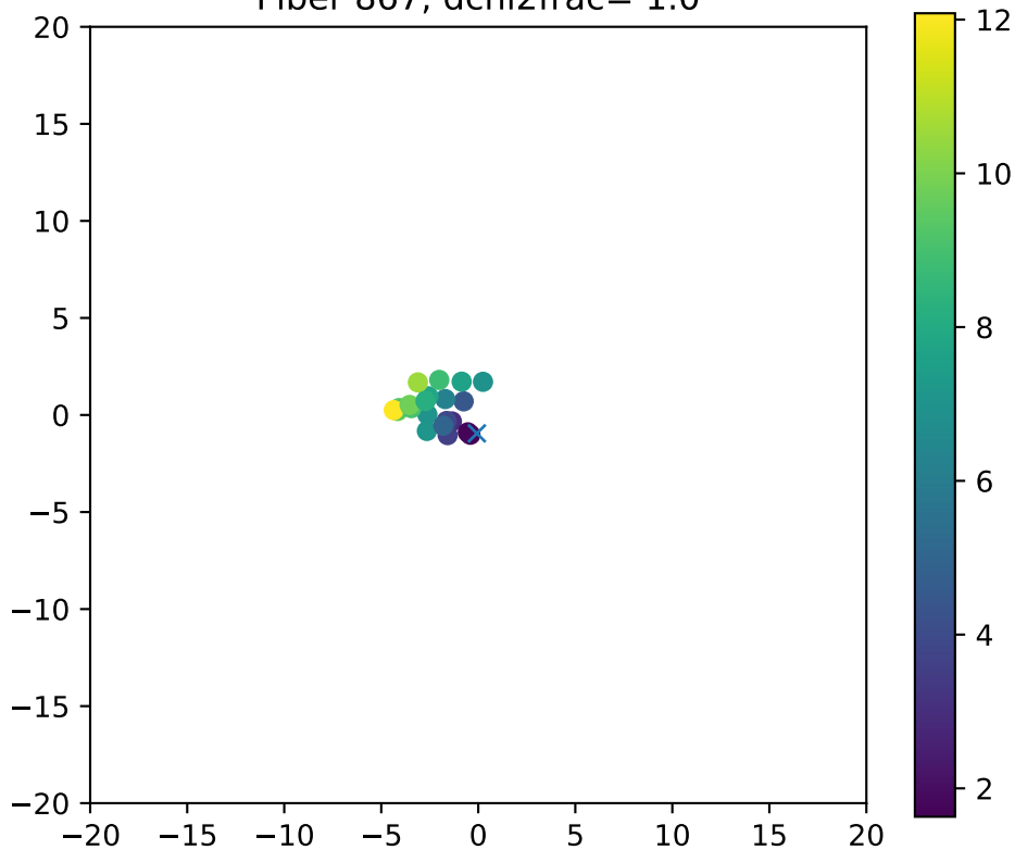
Fiber 867, dchi2frac= 1.0
