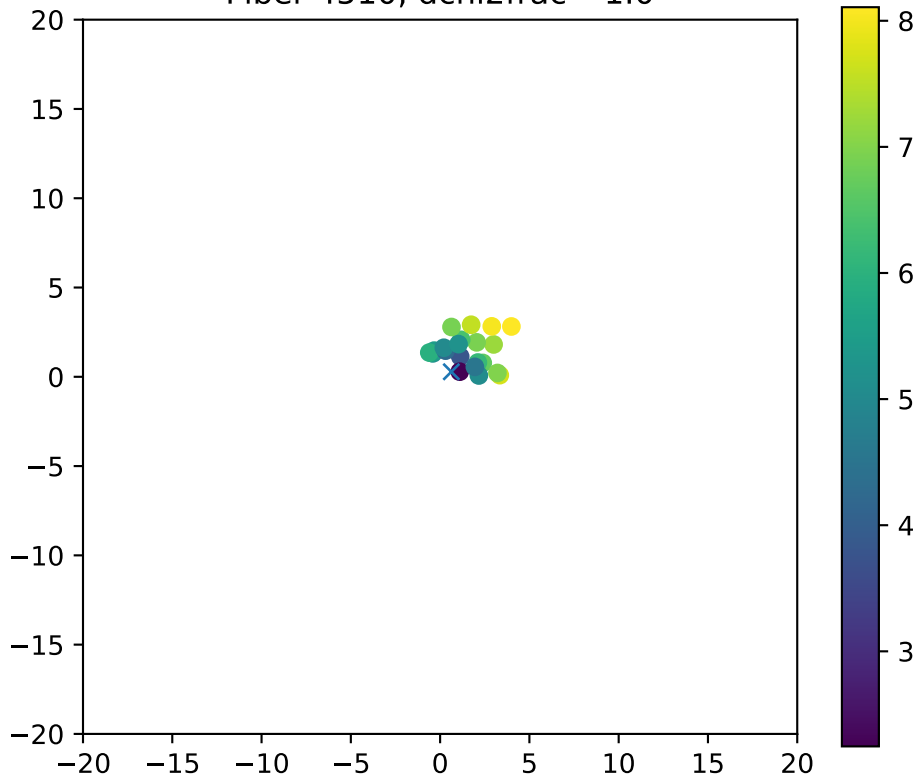
Fiber 4510, dchi2frac= 1.0
