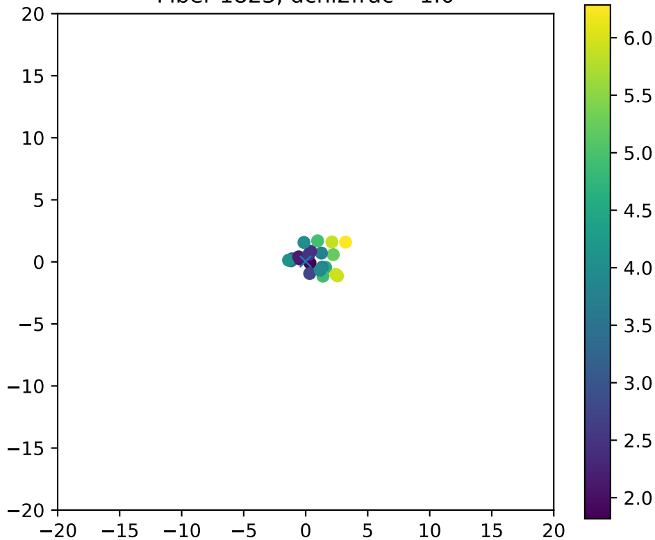
Fiber 1823, dchi2frac= 1.0
