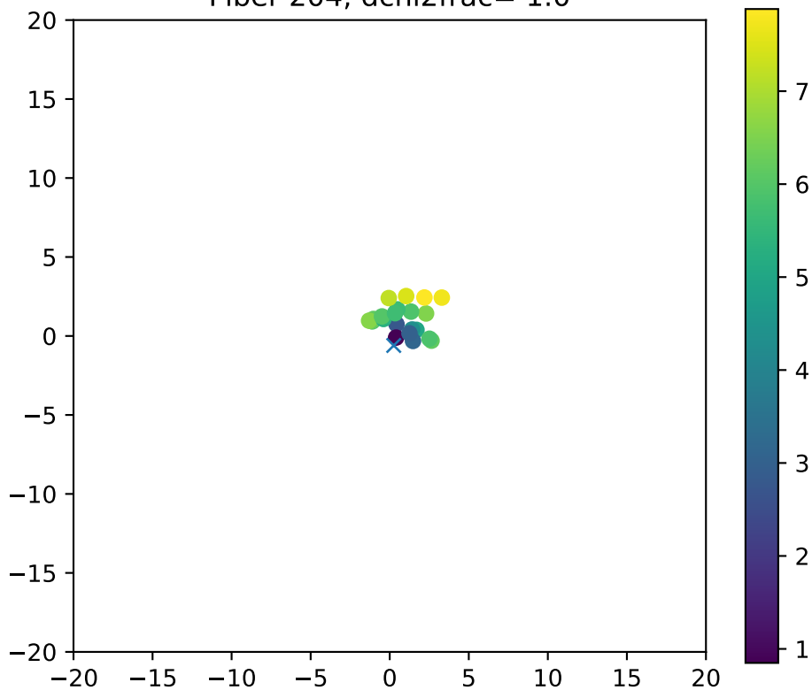
Fiber 204, dchi2frac= 1.0
