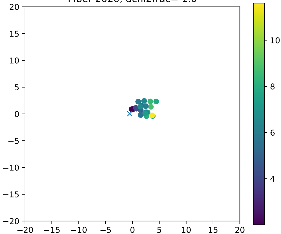
Fiber 2020, dchi2frac= 1.0
