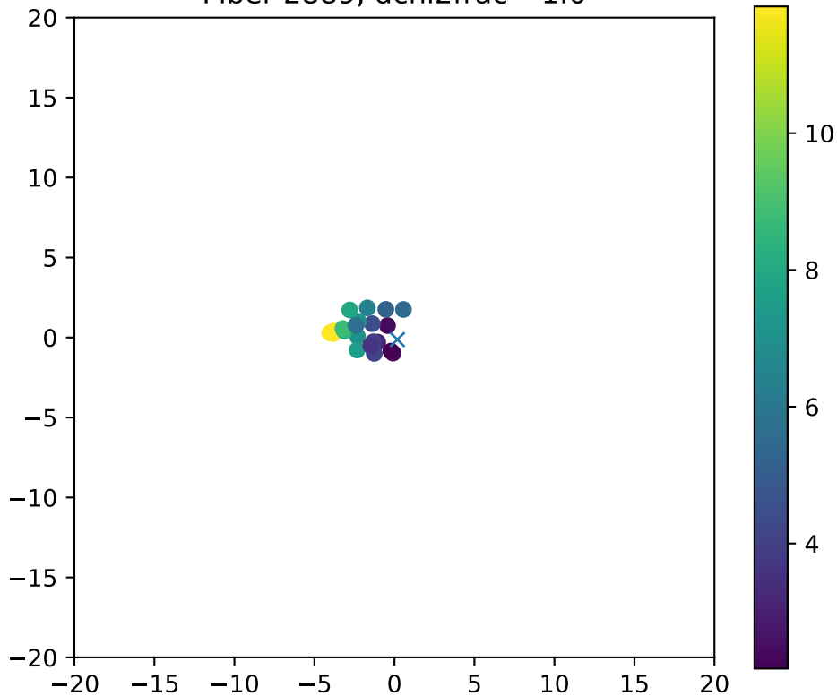
Fiber 2889, dchi2frac= 1.0
