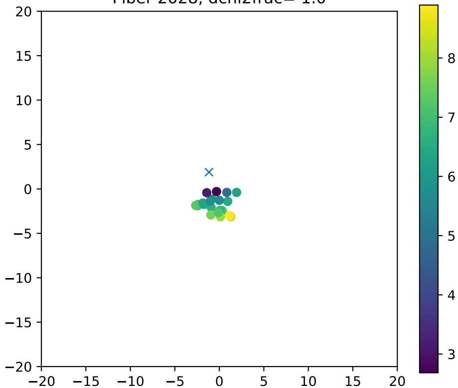
Fiber 2028, dchi2frac= 1.0
