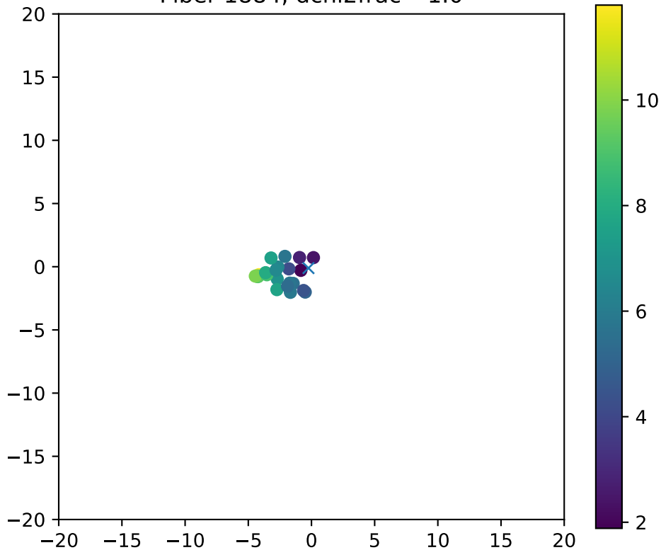
Fiber 1884, dchi2frac= 1.0
