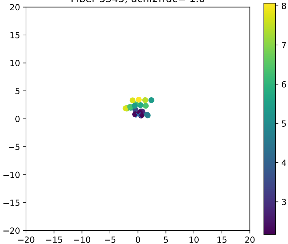
Fiber 3545, dchi2frac= 1.0
