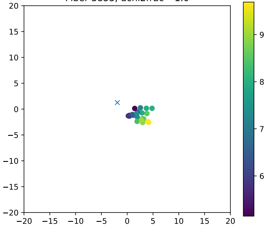
Fiber 3853, dchi2frac= 1.0
