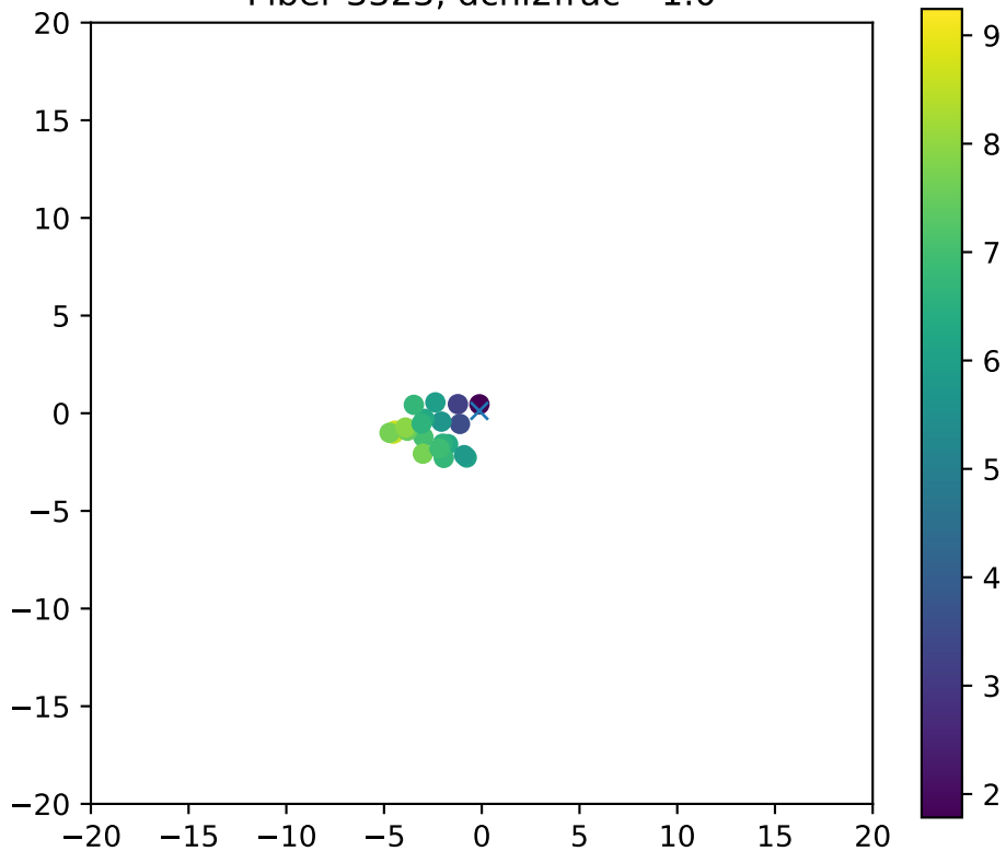
Fiber 3323, dchi2frac= 1.0
