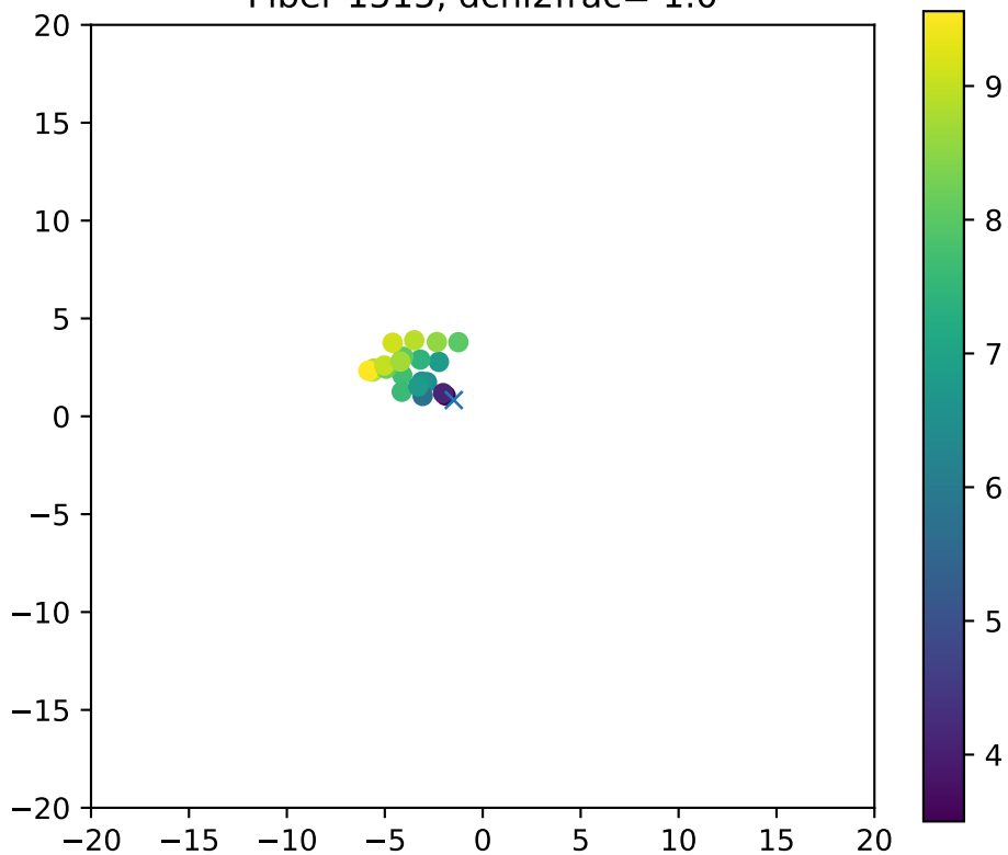
Fiber 1515, dchi2frac= 1.0
