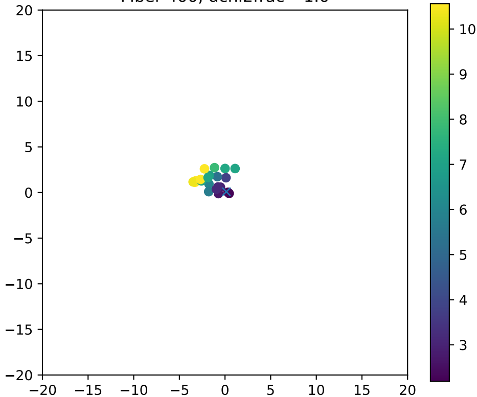
Fiber 400, dchi2frac= 1.0
