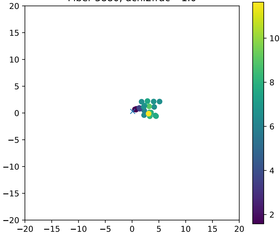
Fiber 3880, dchi2frac= 1.0
