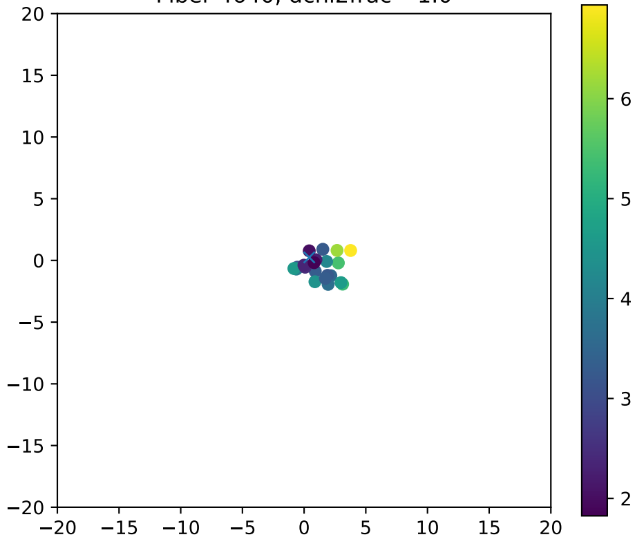
Fiber 4640, dchi2frac= 1.0
