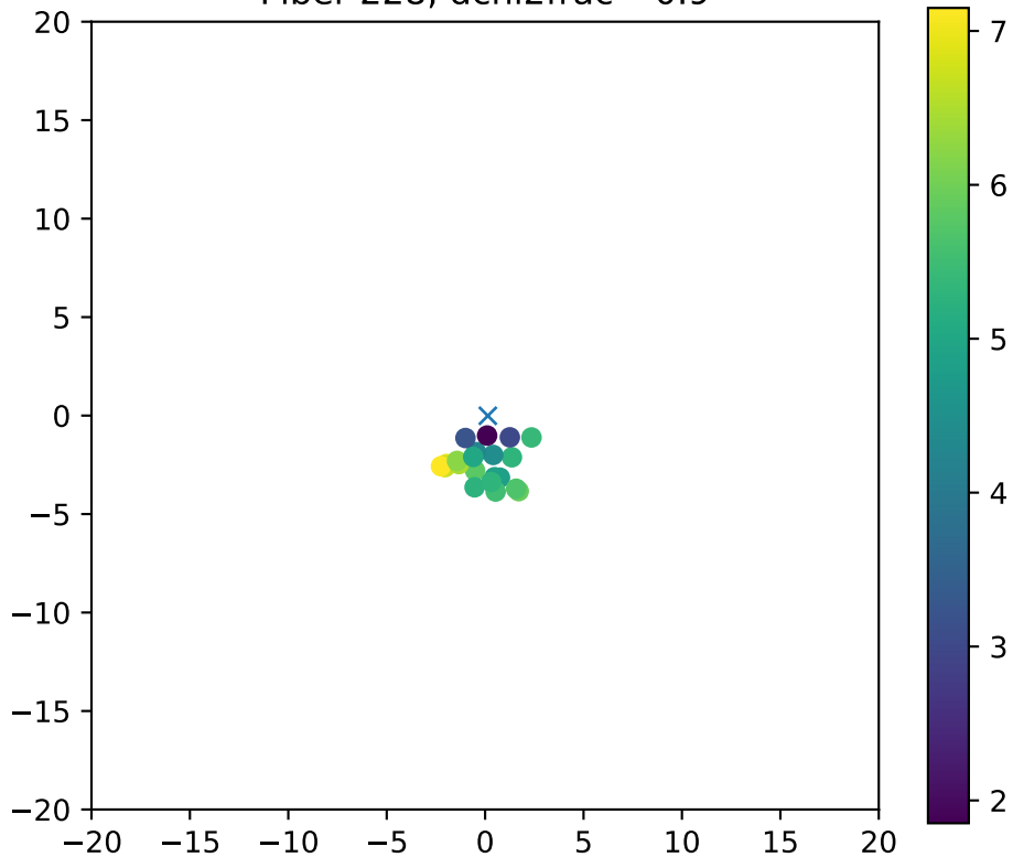
Fiber 228, dchi2frac= 0.9
