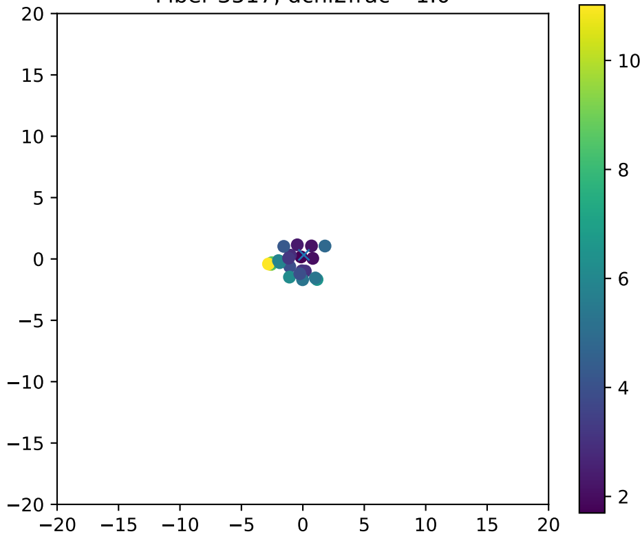
Fiber 3517, dchi2frac= 1.0
