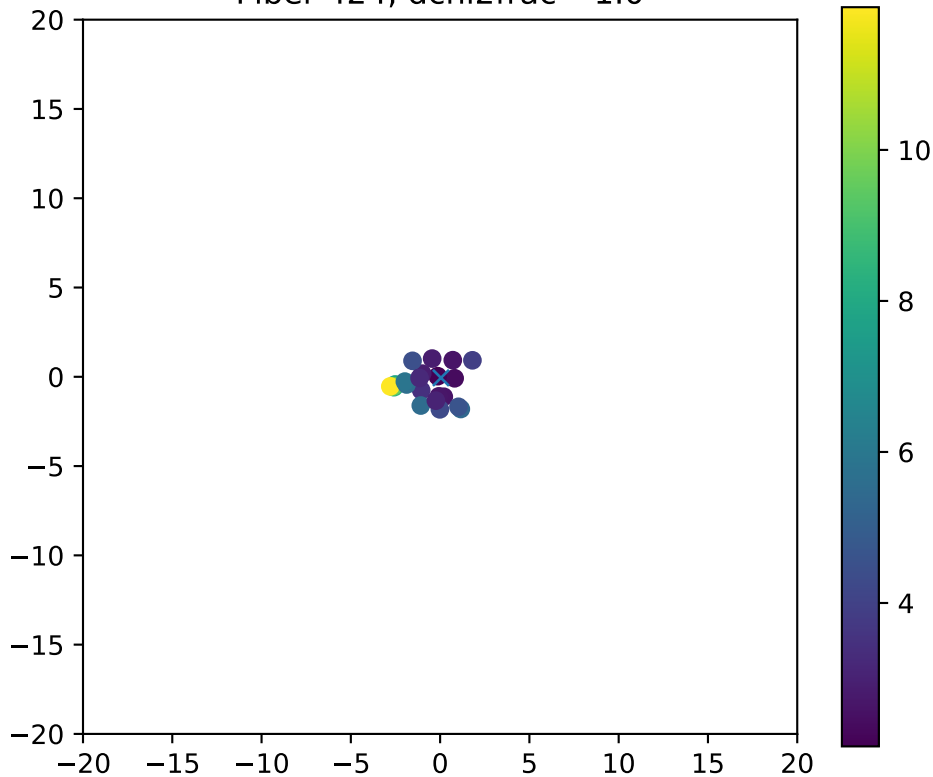
Fiber 424, dchi2frac= 1.0
