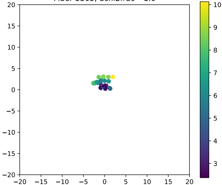
Fiber 3305, dchi2frac= 1.0
