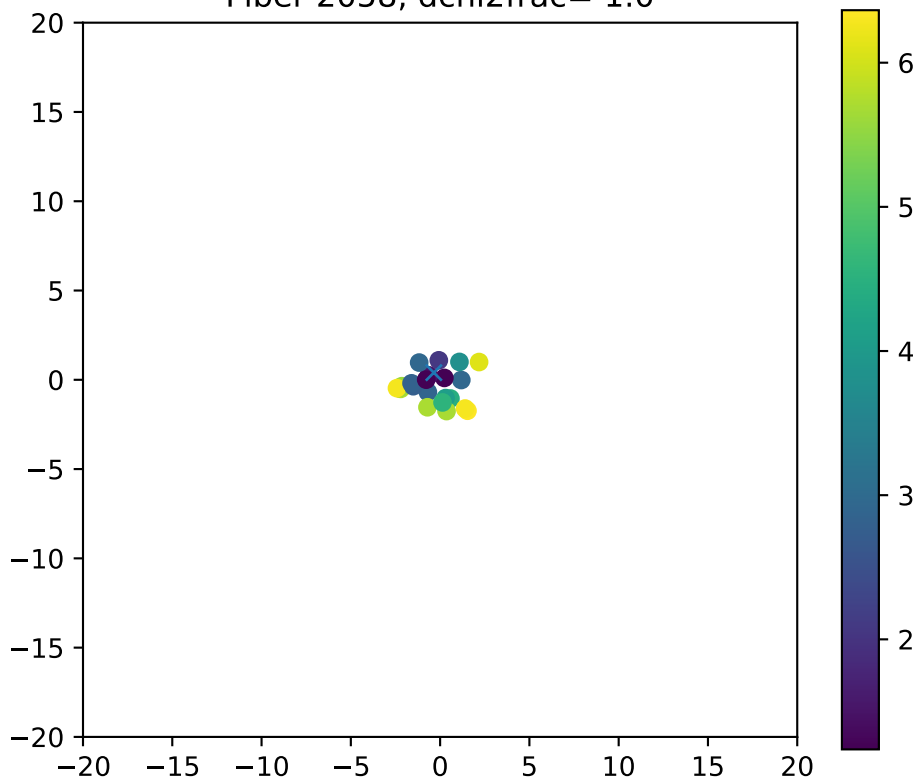
Fiber 2058, dchi2frac= 1.0
