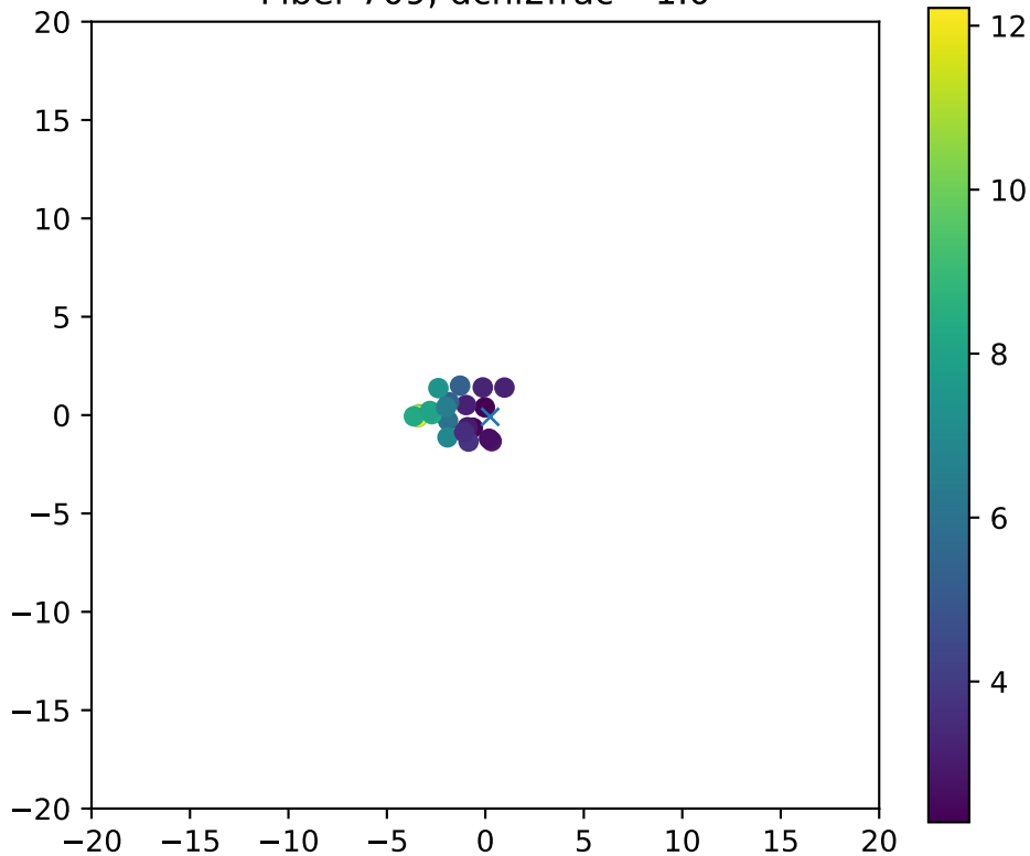
Fiber 709, dchi2frac= 1.0
