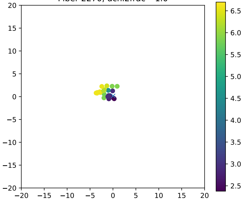
Fiber 2270, dchi2frac= 1.0
