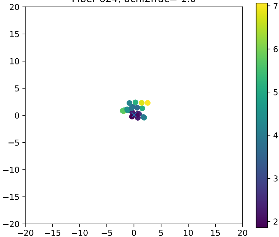
Fiber 624, dchi2frac= 1.0
