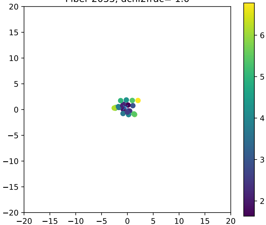
Fiber 2033, dchi2frac= 1.0
