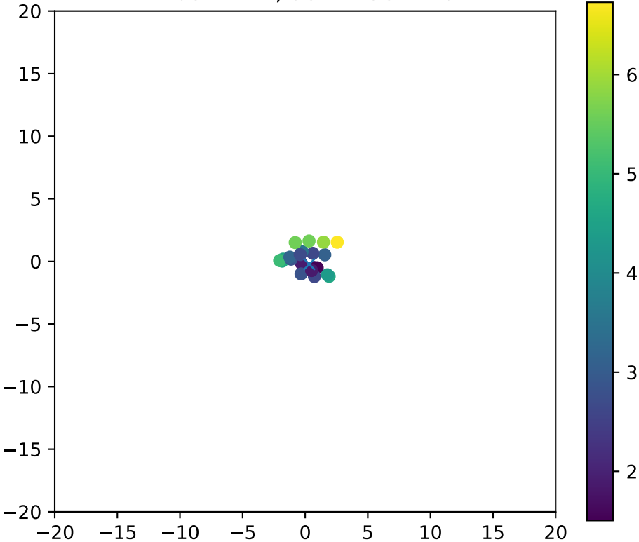
Fiber 2771, dchi2frac= 1.0
