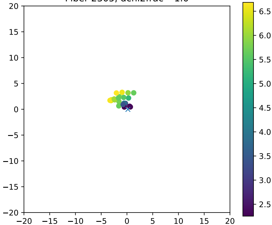
Fiber 2305, dchi2frac= 1.0
