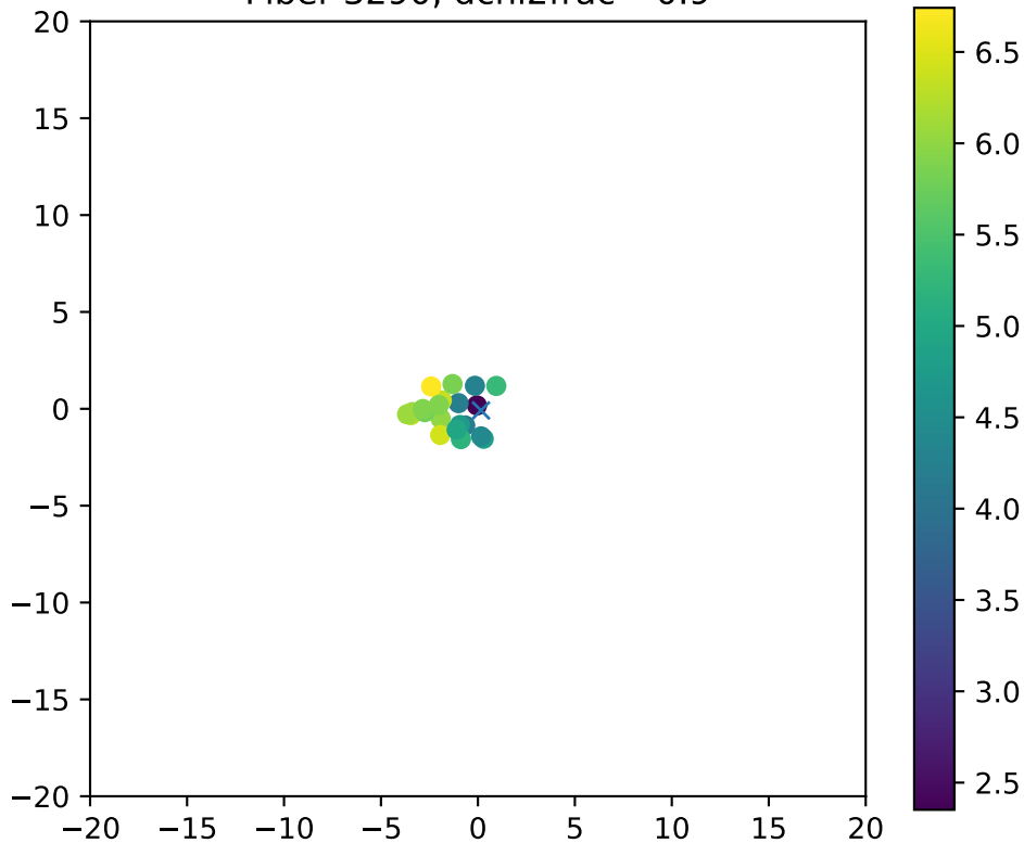
Fiber 3290, dchi2frac= 0.9
