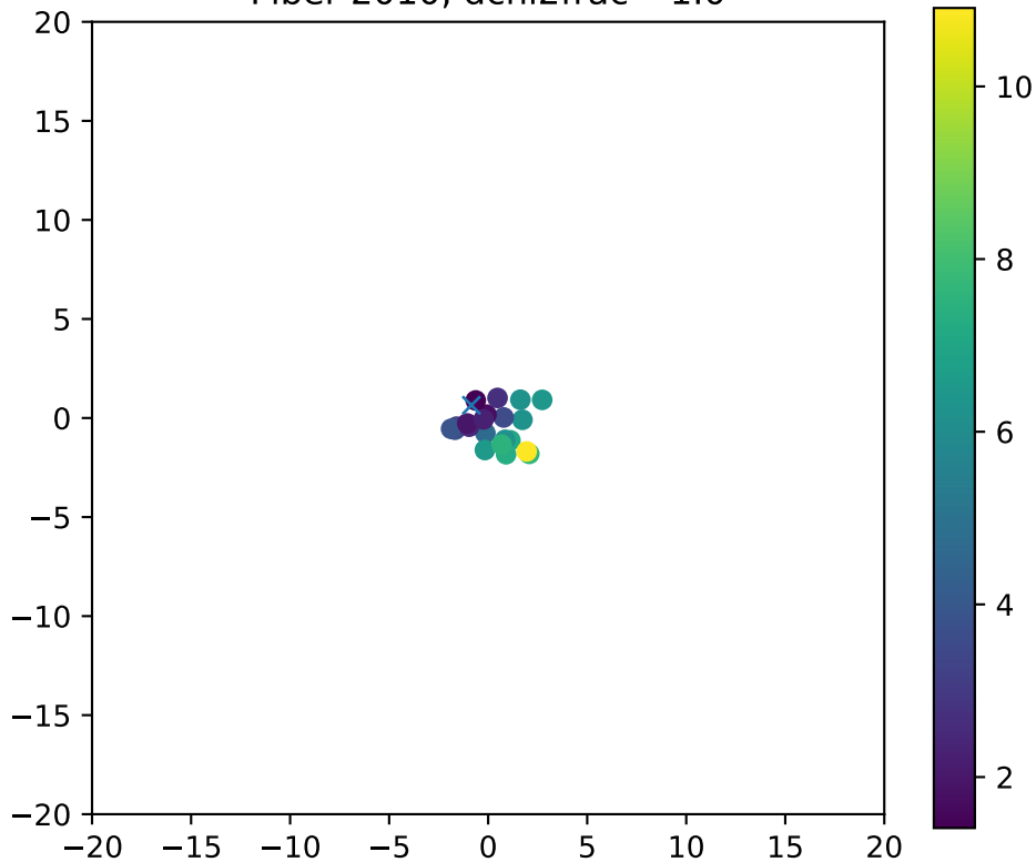
Fiber 2010, dchi2frac= 1.0
