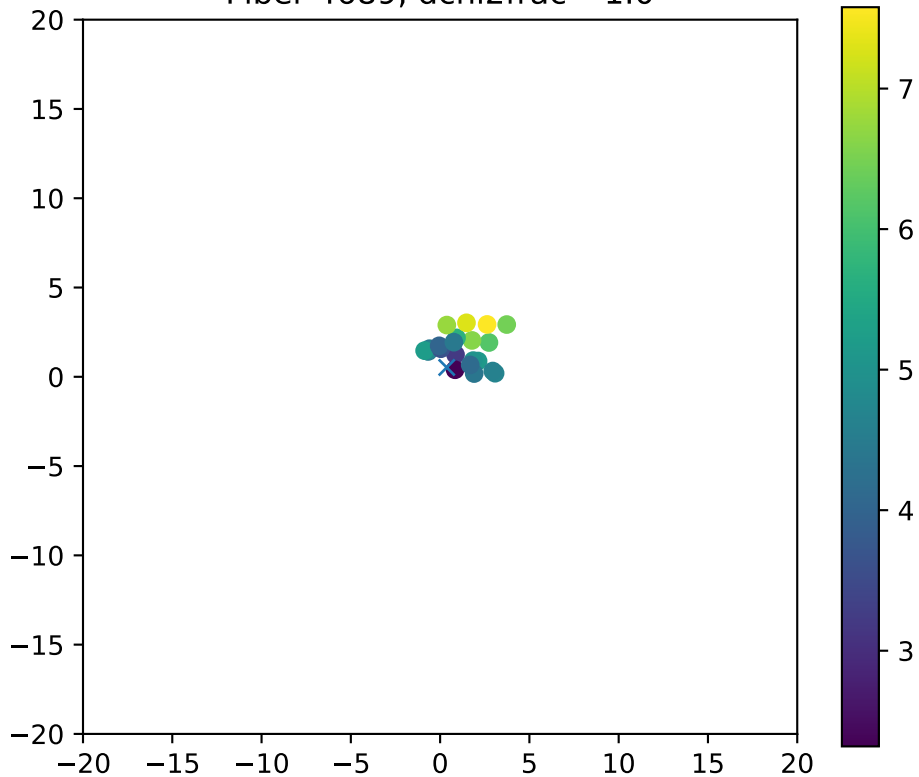
Fiber 4689, dchi2frac= 1.0
