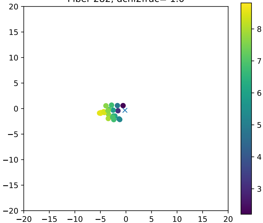
Fiber 282, dchi2frac= 1.0
