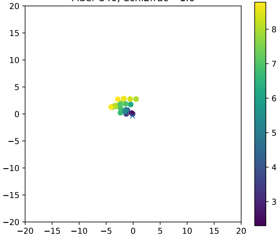
Fiber 840, dchi2frac= 1.0
