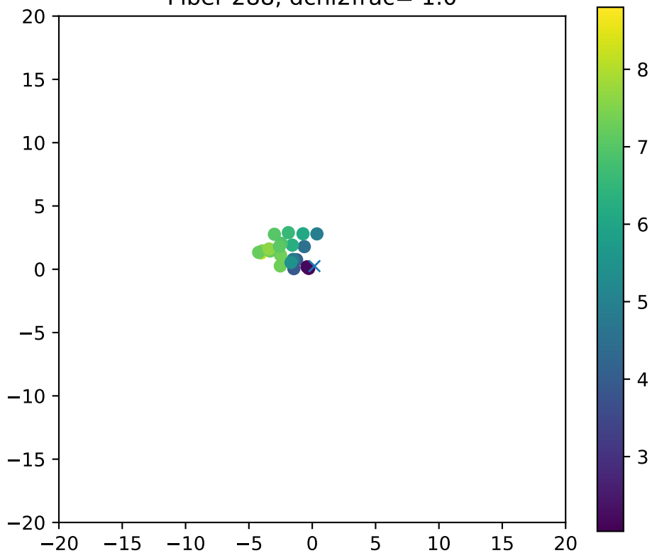
Fiber 288, dchi2frac= 1.0
