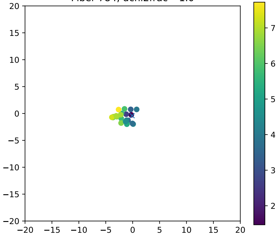
Fiber 784, dchi2frac= 1.0
