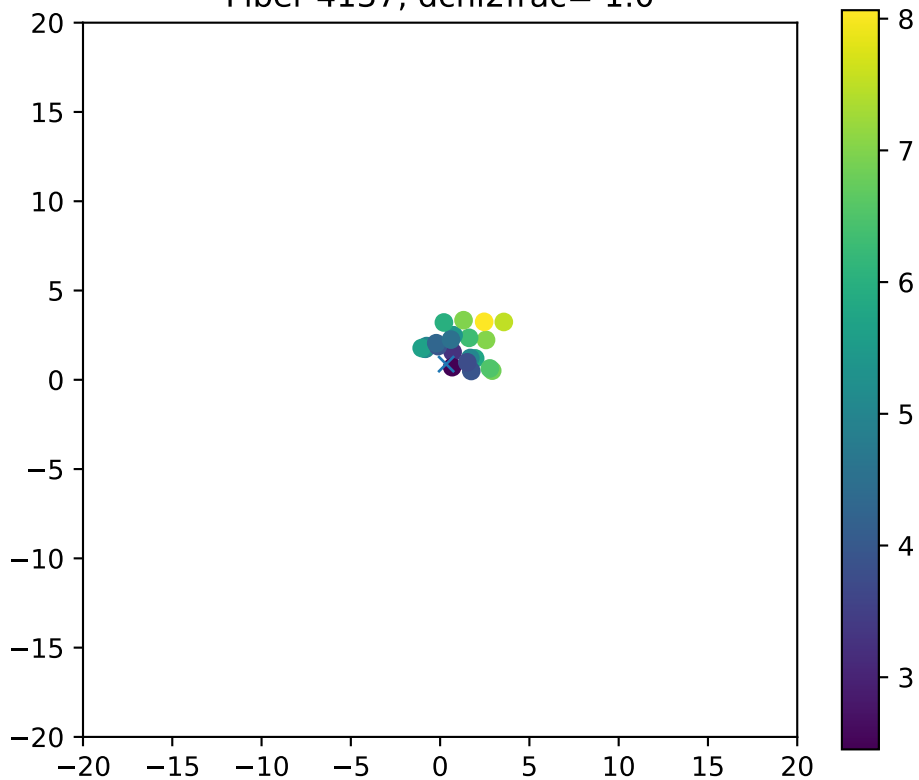
Fiber 4137, dchi2frac= 1.0
