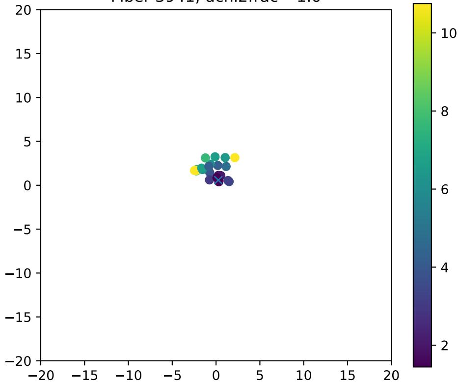
Fiber 3941, dchi2frac= 1.0
