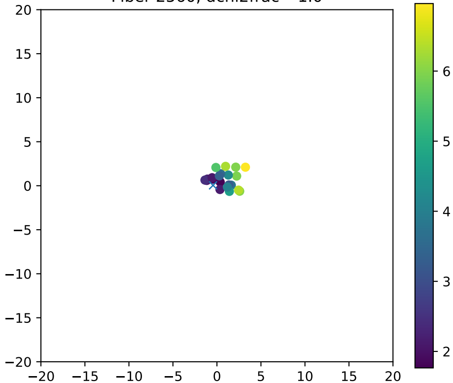
Fiber 2560, dchi2frac= 1.0
