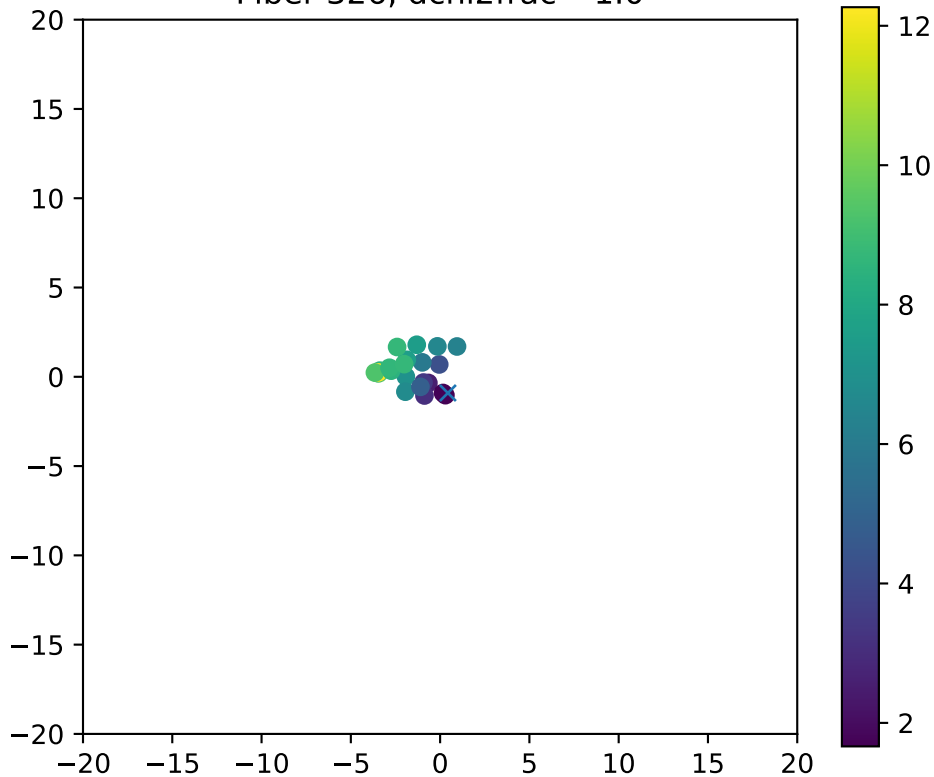
Fiber 326, dchi2frac= 1.0
