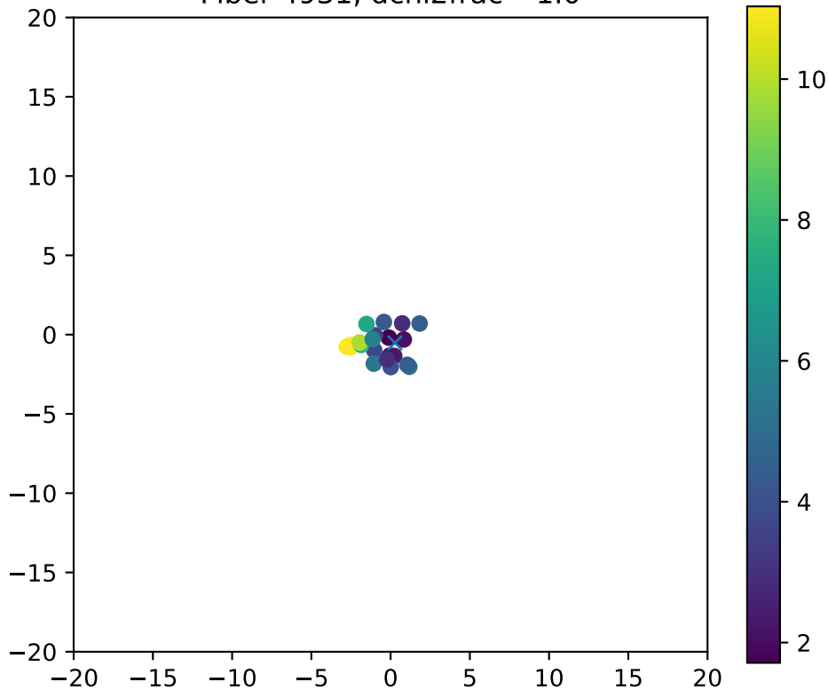
Fiber 4931, dchi2frac= 1.0
