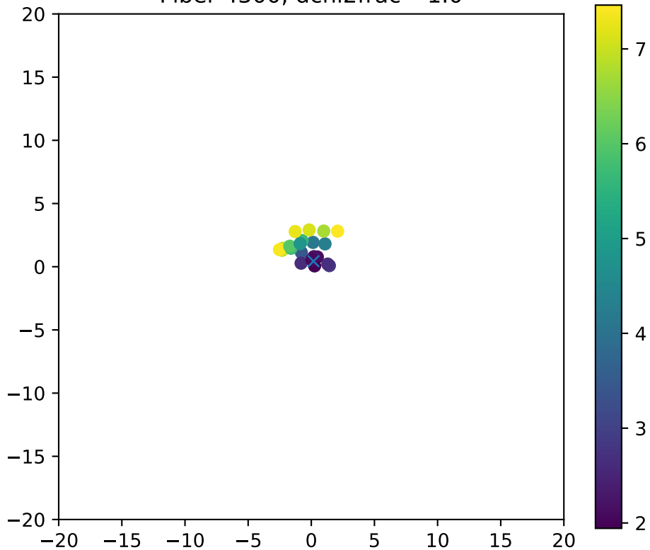
Fiber 4300, dchi2frac= 1.0
