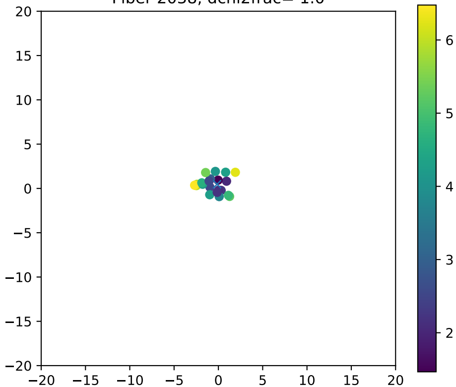
Fiber 2038, dchi2frac= 1.0
