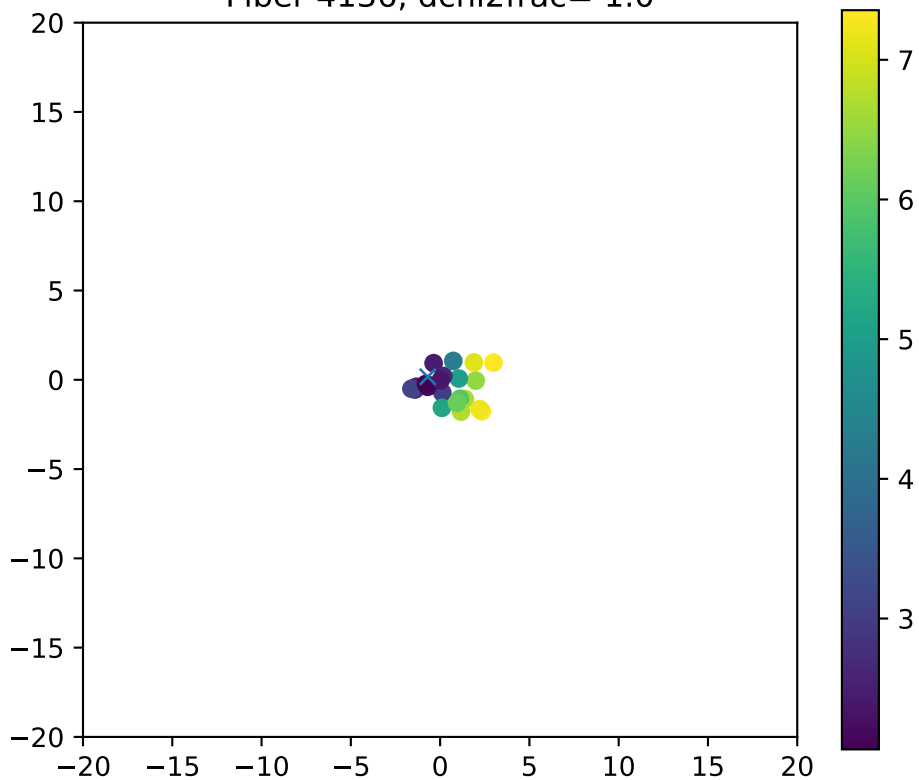
Fiber 4136, dchi2frac= 1.0
