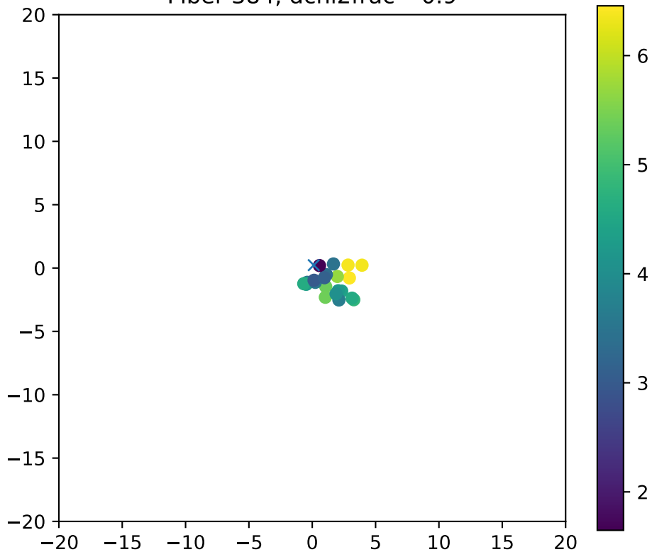
Fiber 384, dchi2frac= 0.9
