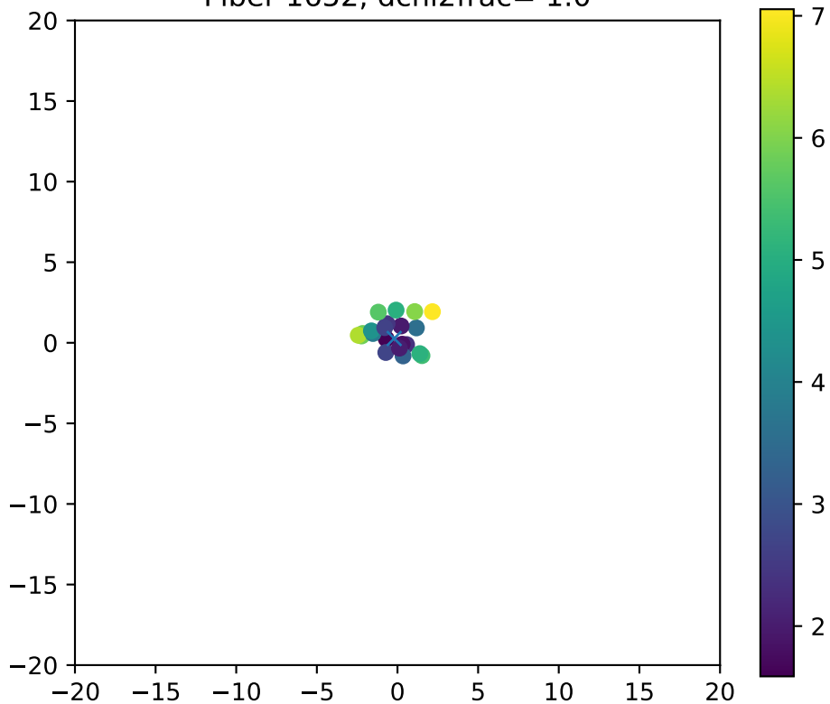
Fiber 1652, dchi2frac= 1.0
