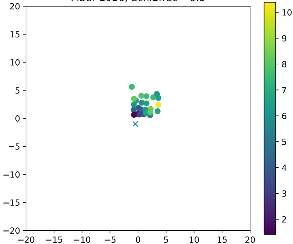
Fiber 1926, dchi2frac= 0.9
