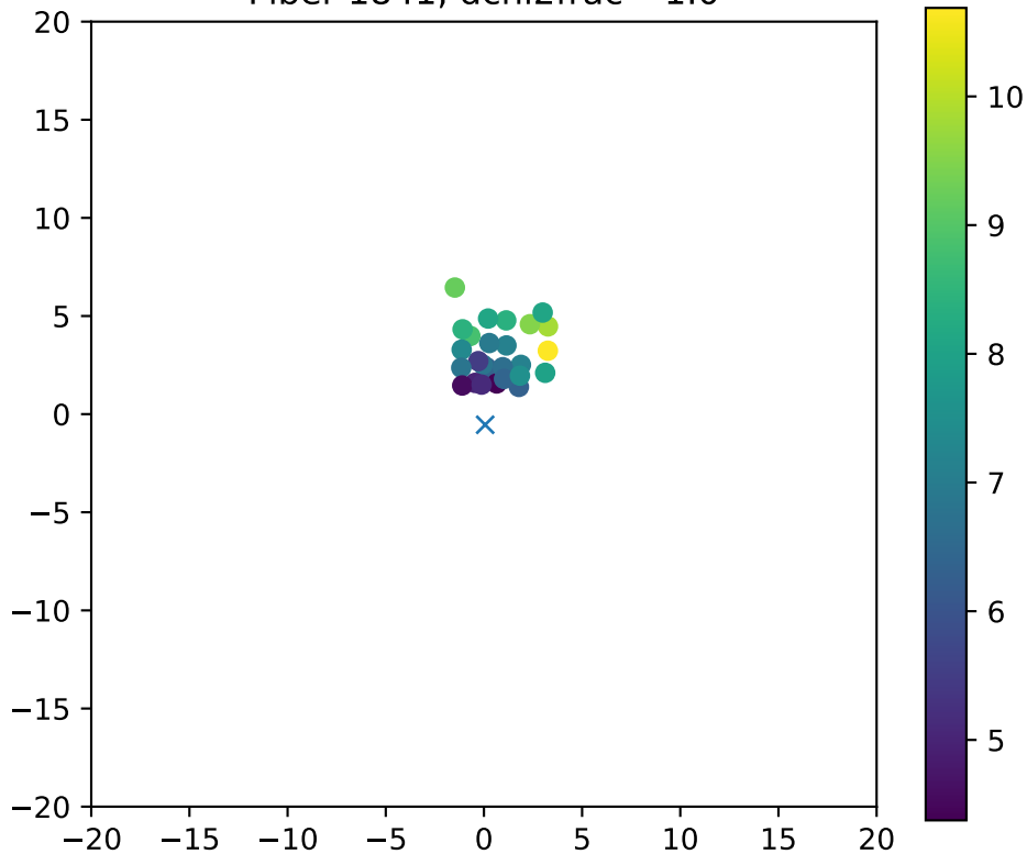
Fiber 1841, dchi2frac= 1.0
