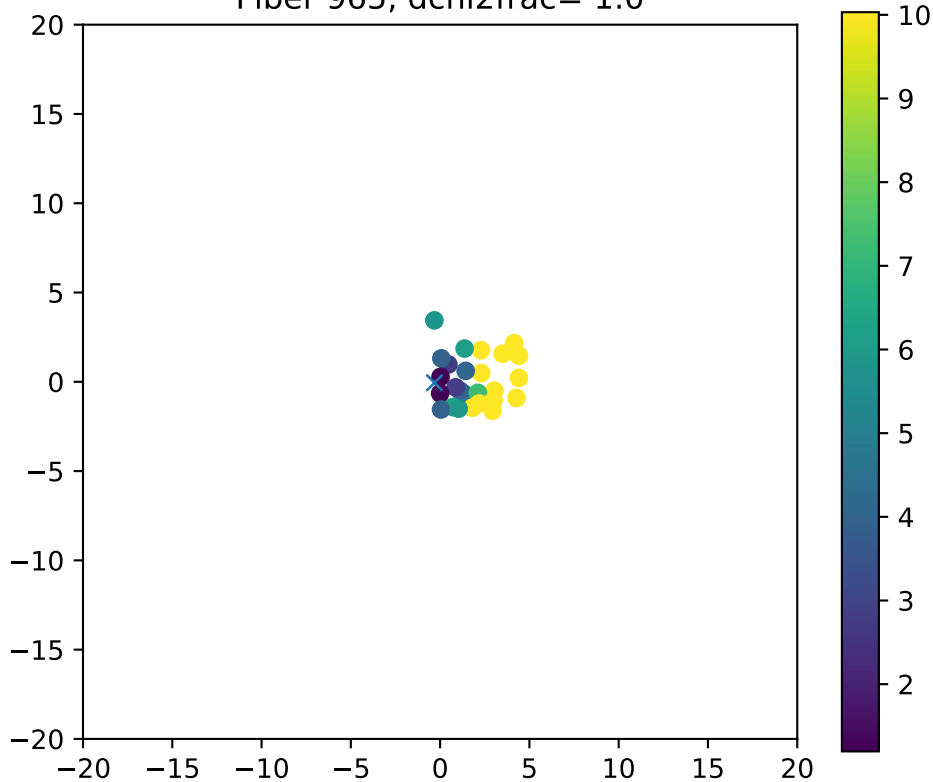
Fiber 965, dchi2frac= 1.0
