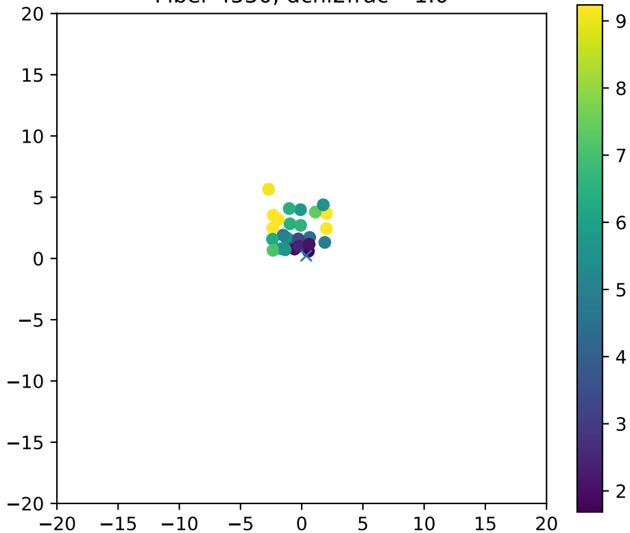
Fiber 4550, dchi2frac= 1.0
