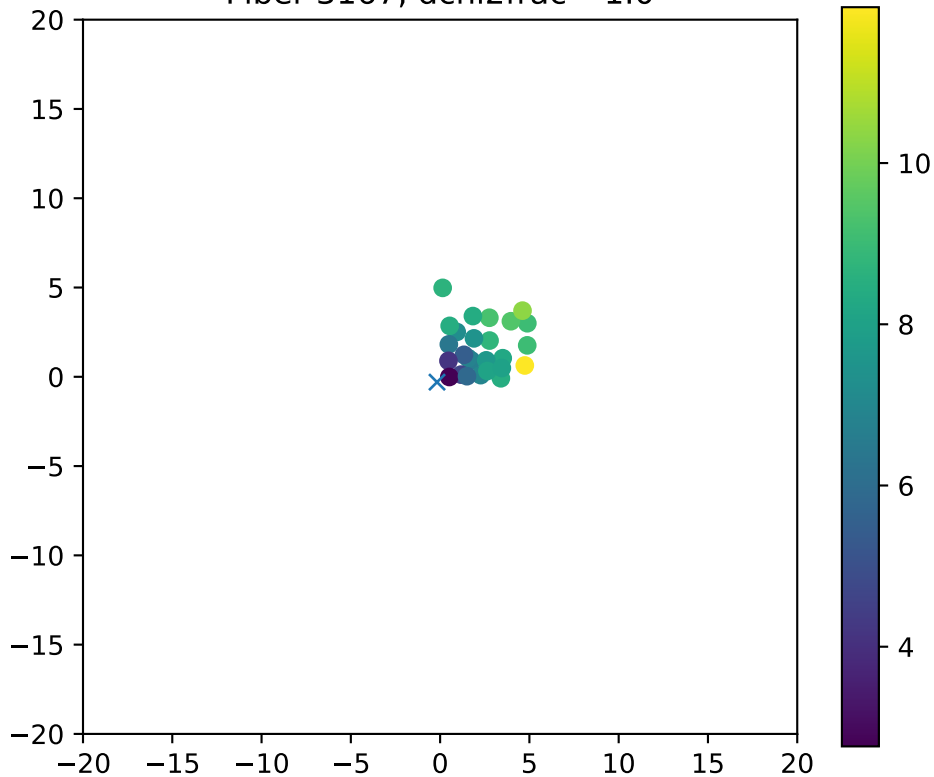
Fiber 3167, dchi2frac= 1.0
