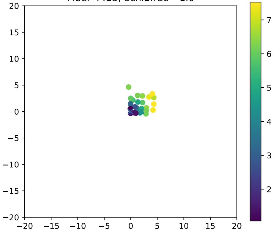
Fiber 4425, dchi2frac= 1.0
