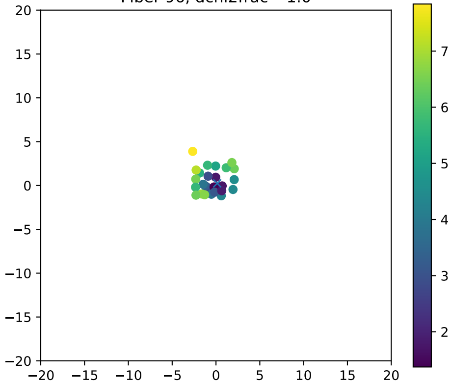
Fiber 96, dchi2frac= 1.0
