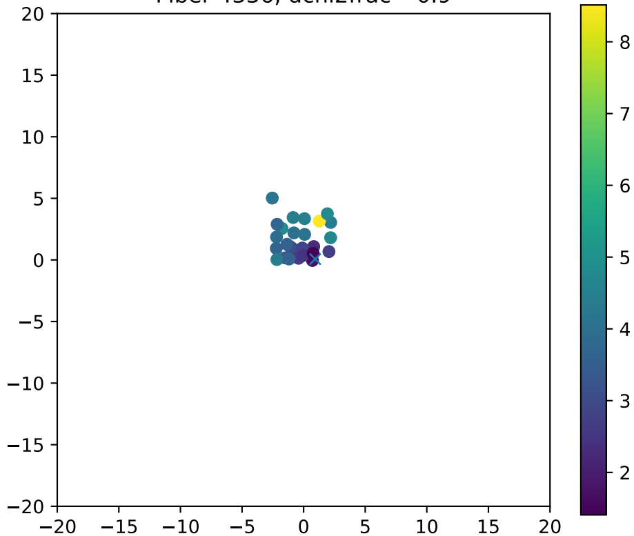
Fiber 4336, dchi2frac= 0.9
