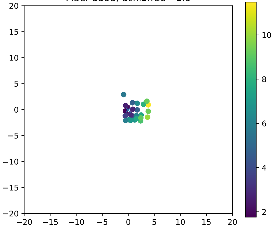
Fiber 3358, dchi2frac= 1.0
