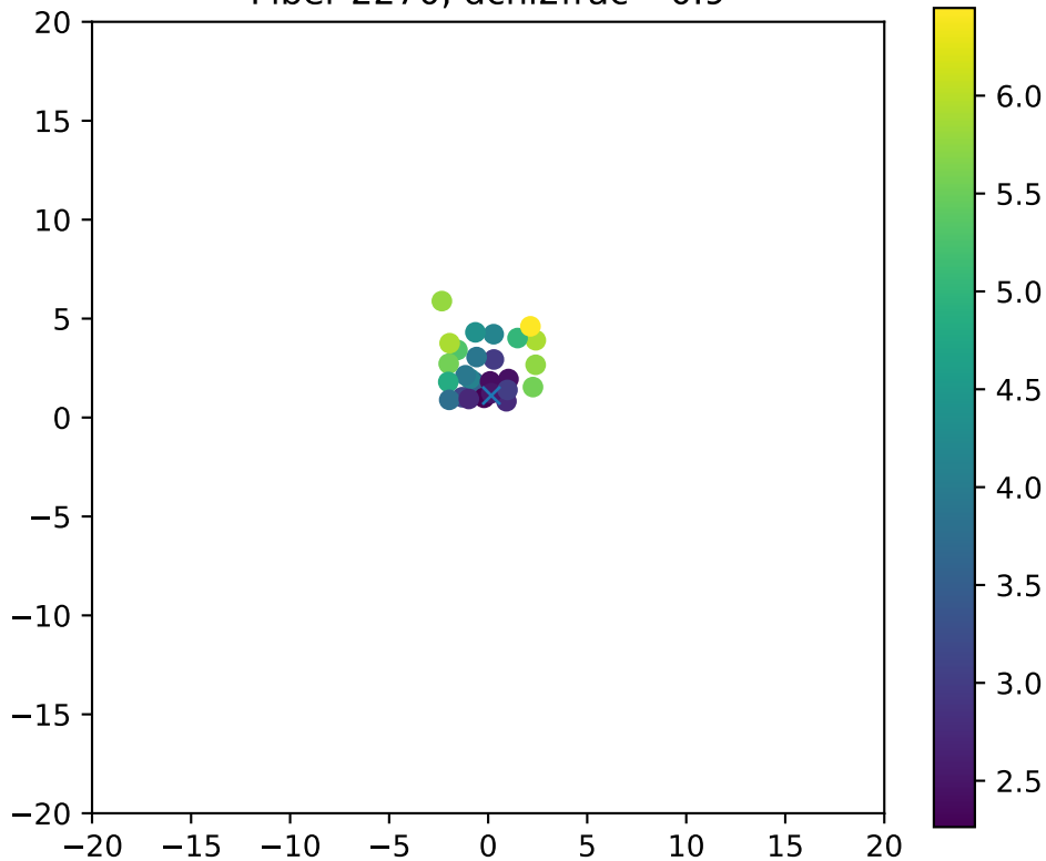
Fiber 2270, dchi2frac= 0.9
