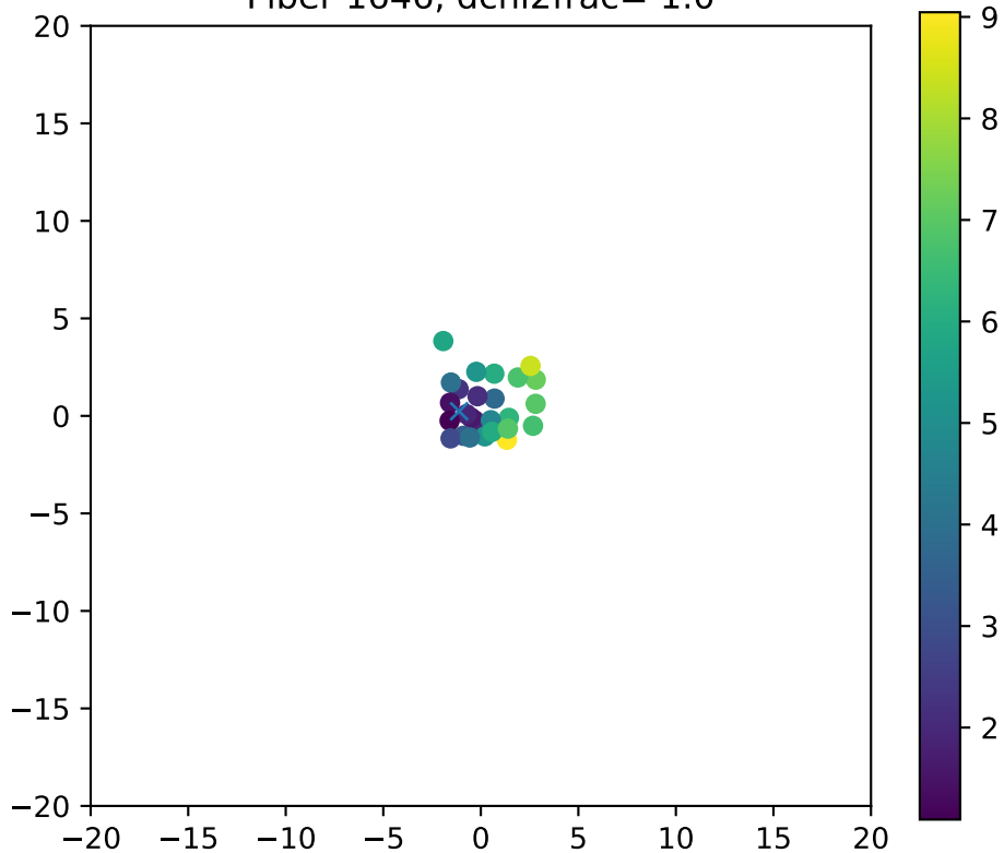
Fiber 1646, dchi2frac= 1.0
