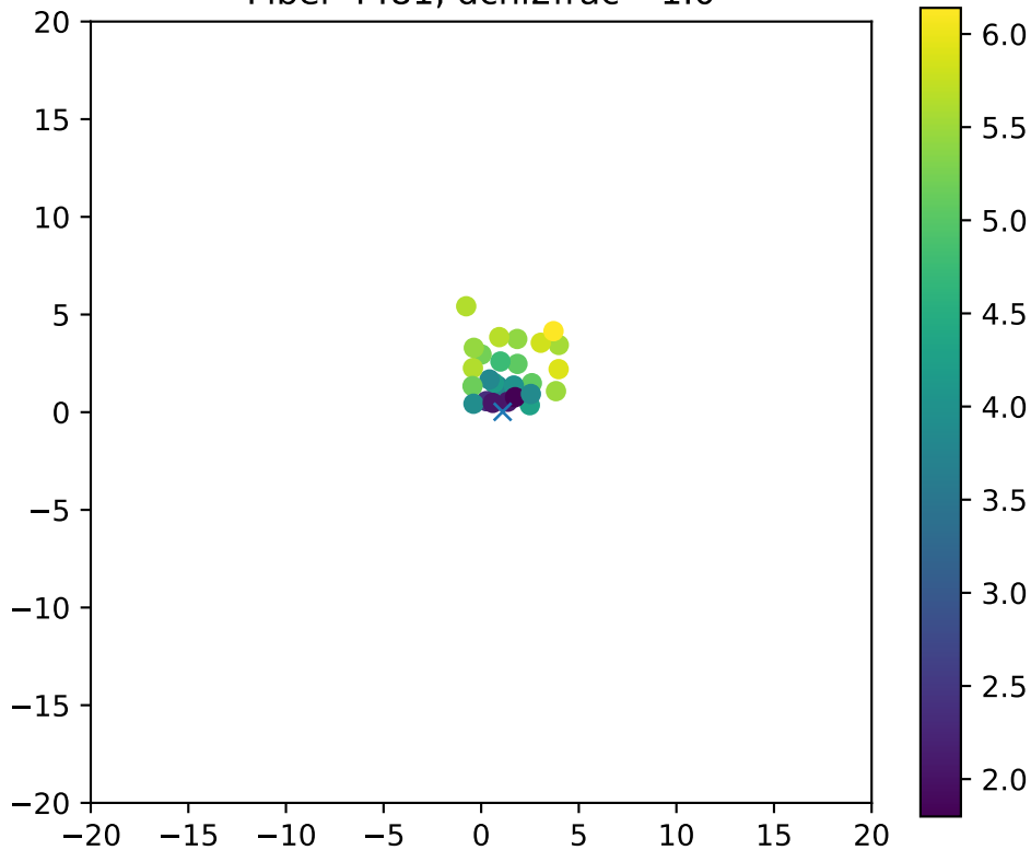
Fiber 4481, dchi2frac= 1.0
