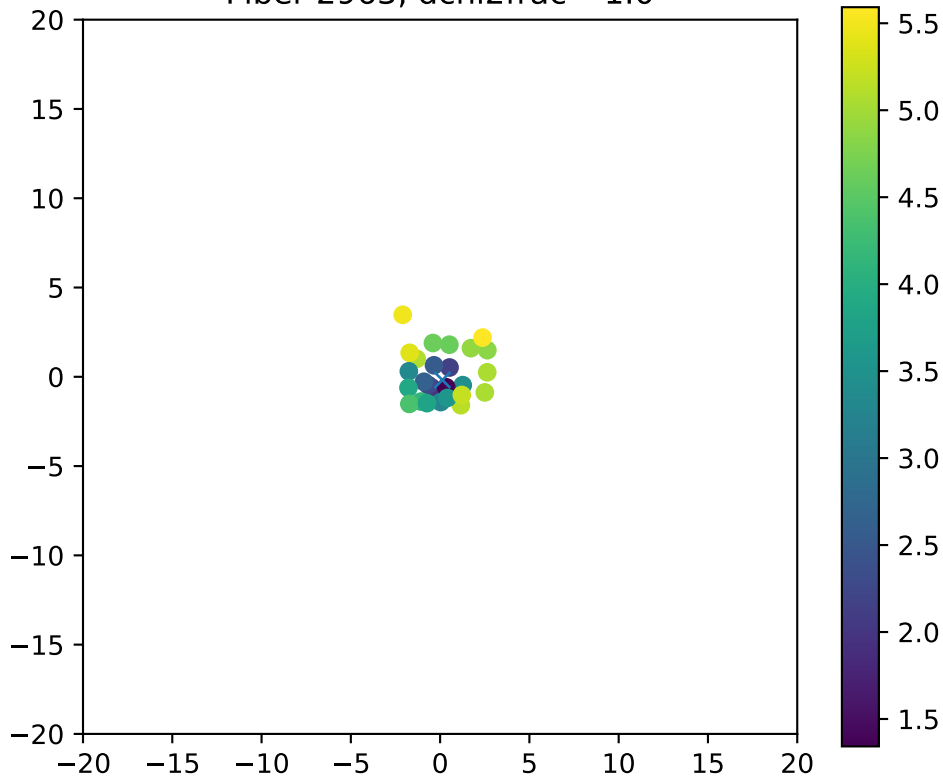
Fiber 2963, dchi2frac= 1.0
