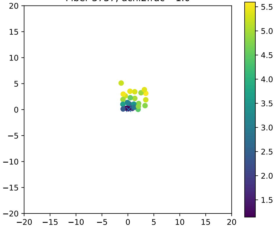
Fiber 3737, dchi2frac= 1.0
