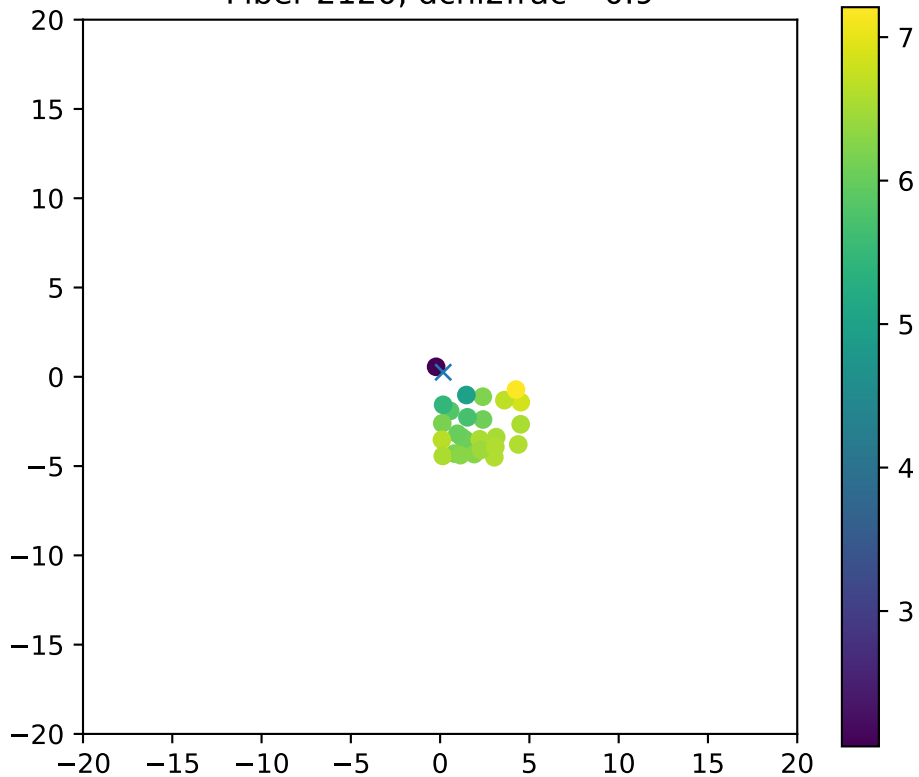
Fiber 2120, dchi2frac= 0.9
