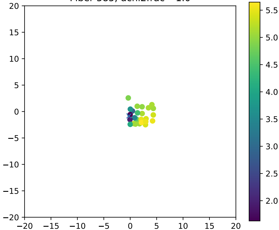
Fiber 585, dchi2frac= 1.0
