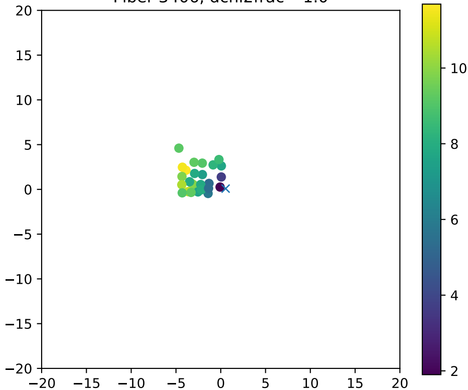
Fiber 3406, dchi2frac= 1.0
