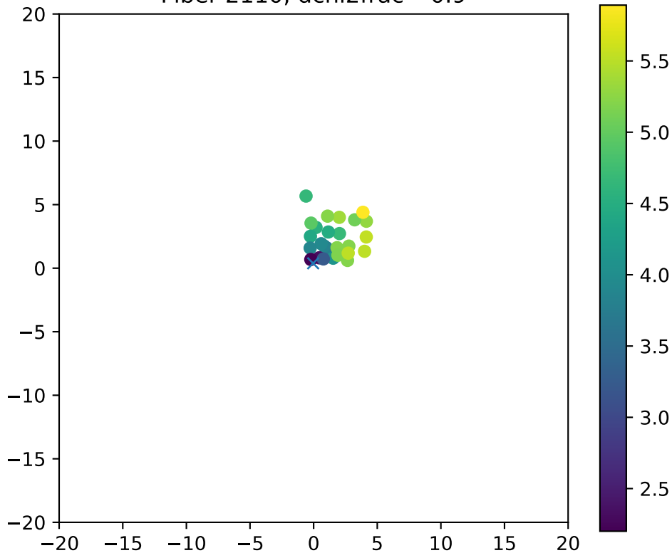
Fiber 2110, dchi2frac= 0.9
