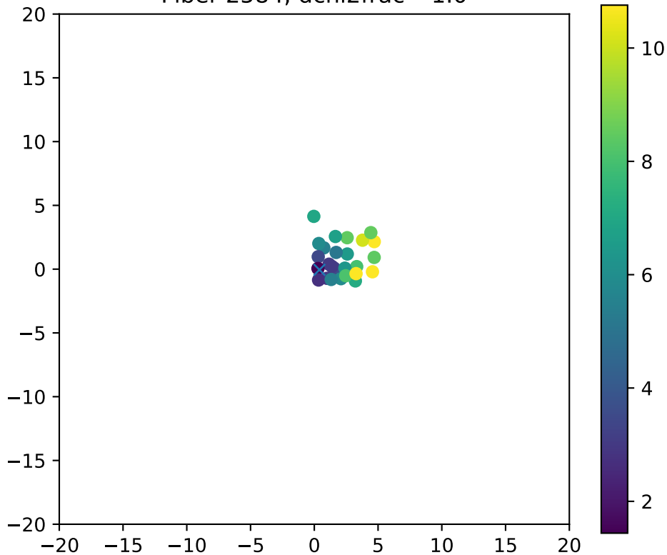
Fiber 2584, dchi2frac= 1.0
