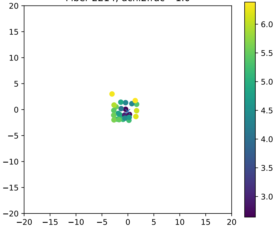
Fiber 2214, dchi2frac= 1.0
