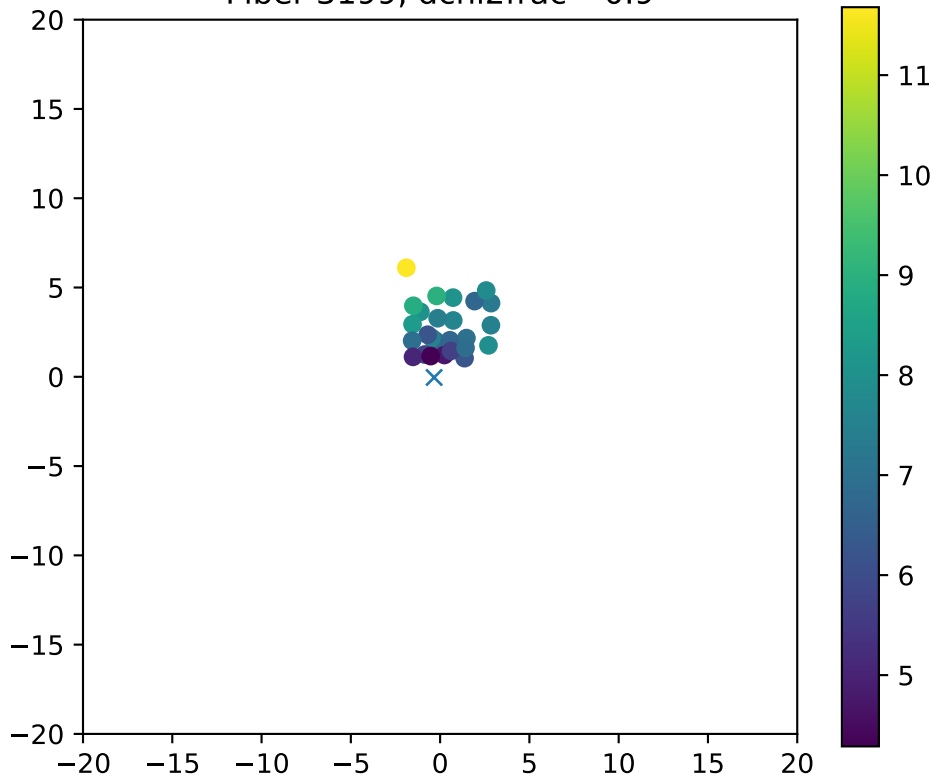
Fiber 3199, dchi2frac= 0.9
