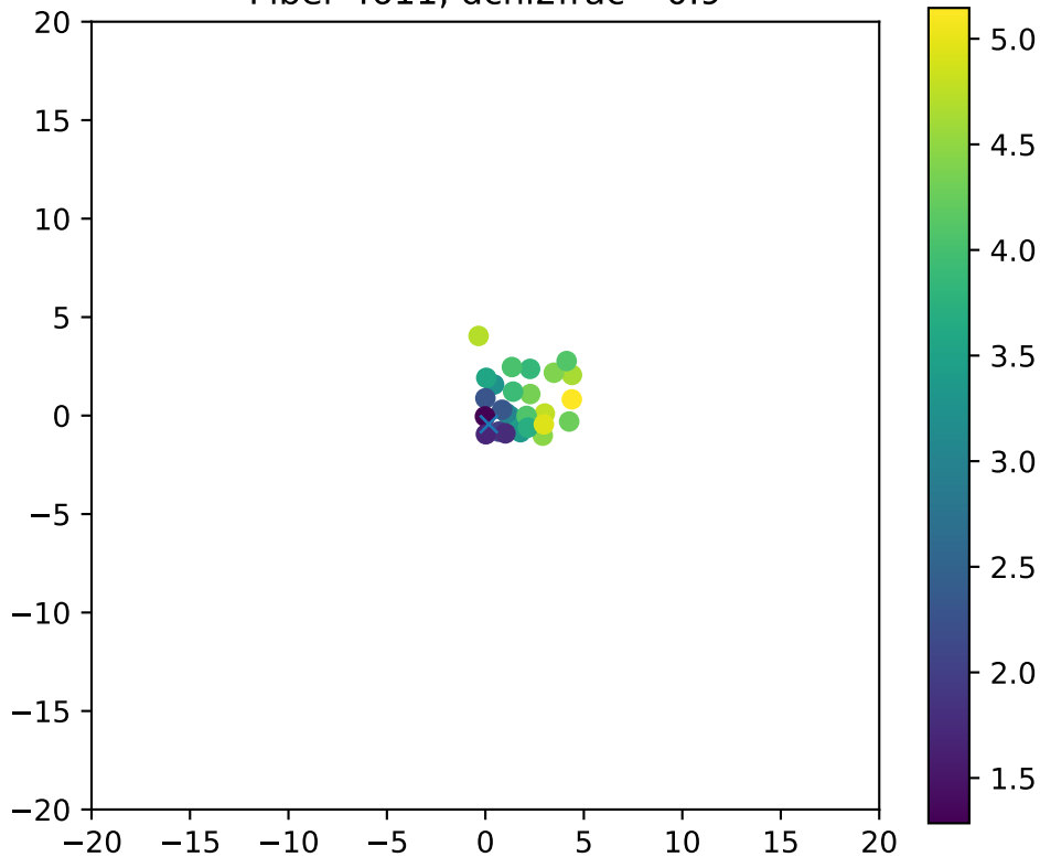
Fiber 4611, dchi2frac= 0.9
