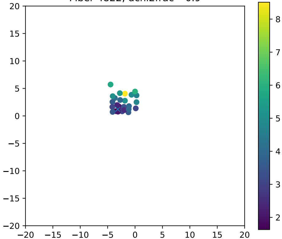
Fiber 4822, dchi2frac= 0.9
