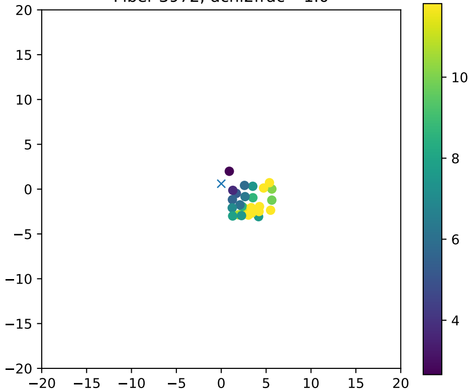
Fiber 3972, dchi2frac= 1.0
