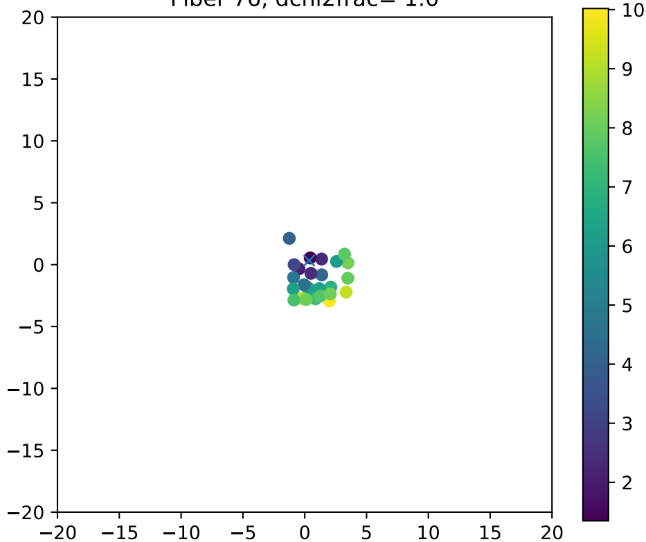
Fiber 76, dchi2frac= 1.0
