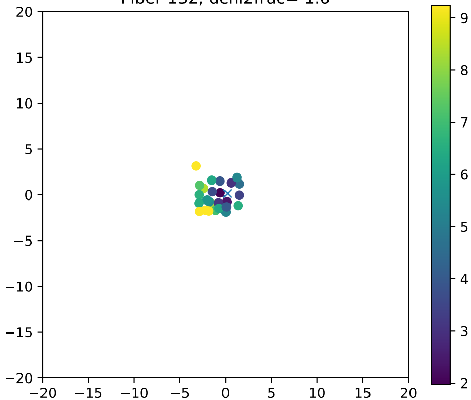
Fiber 132, dchi2frac= 1.0
