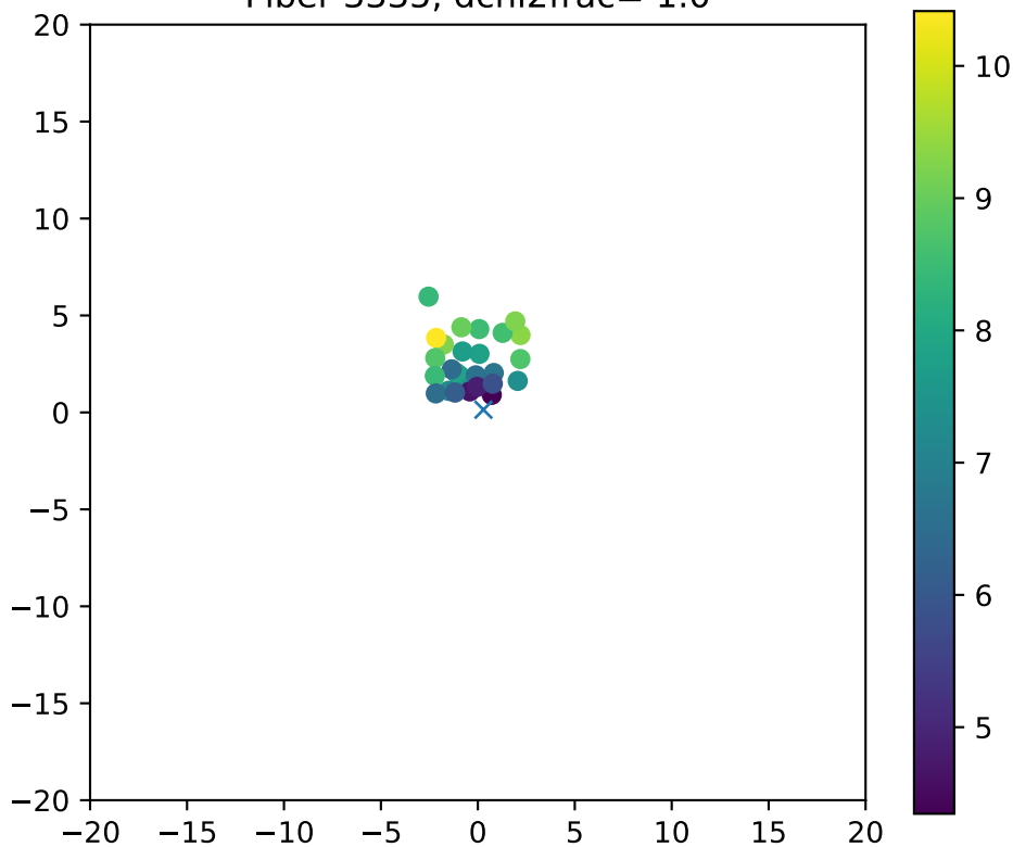
Fiber 3335, dchi2frac= 1.0
