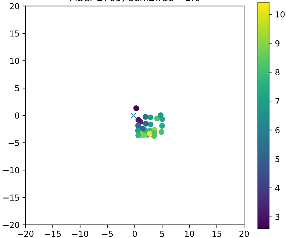
Fiber 2709, dchi2frac= 1.0
