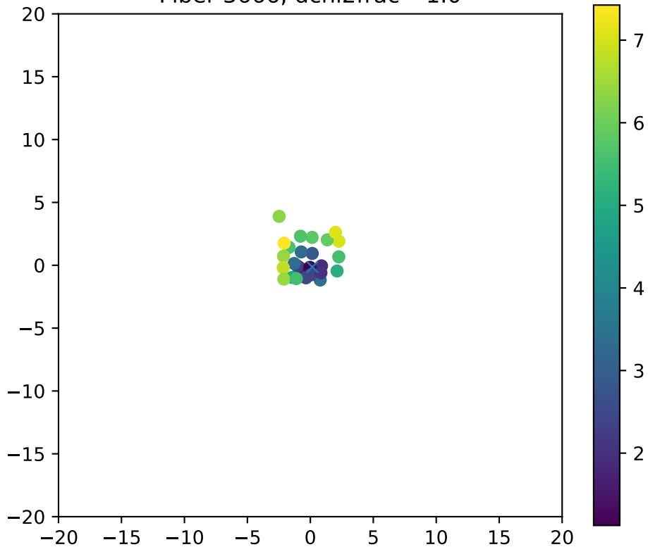
Fiber 3666, dchi2frac= 1.0
