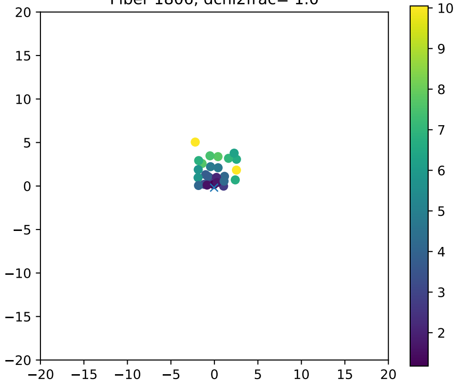
Fiber 1806, dchi2frac= 1.0
