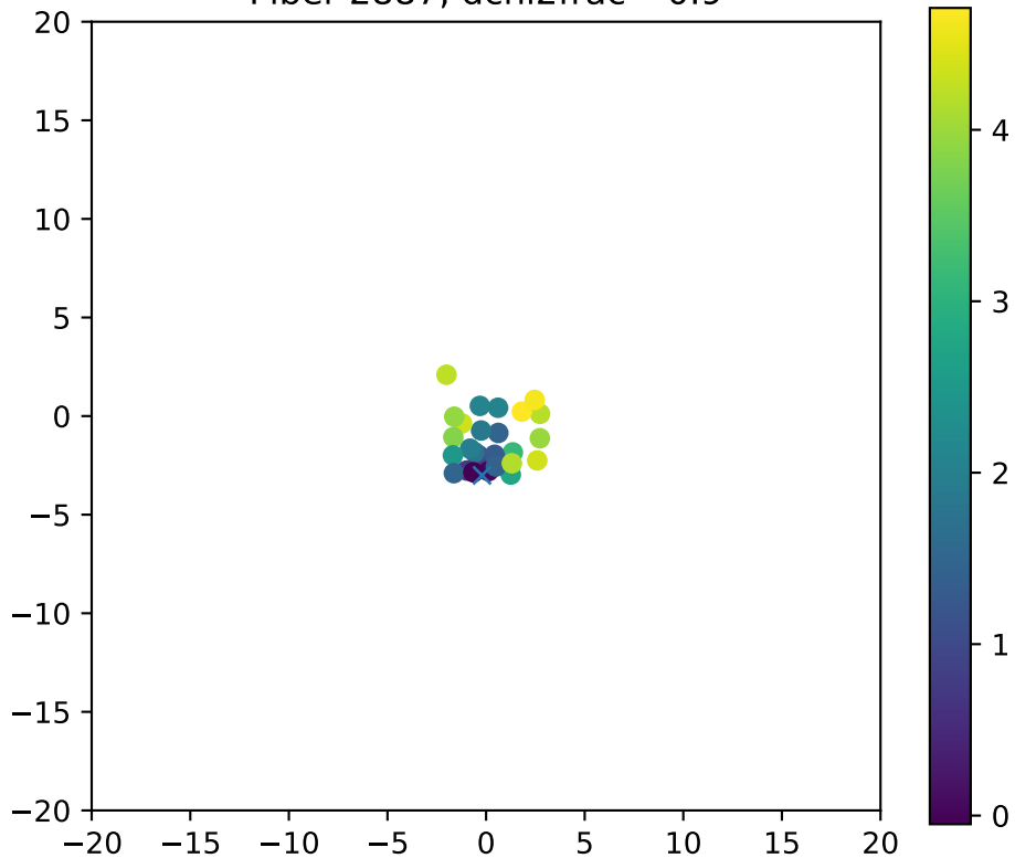
Fiber 2887, dchi2frac= 0.9
