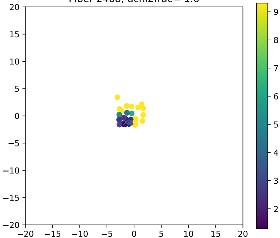
Fiber 2468, dchi2frac= 1.0
