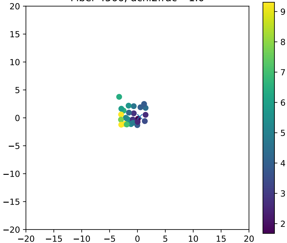
Fiber 4566, dchi2frac= 1.0
