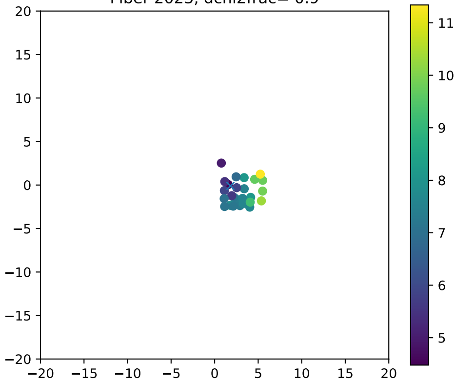
Fiber 2023, dchi2frac= 0.9
