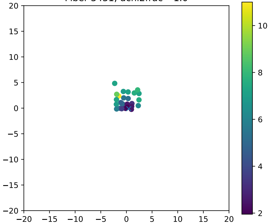
Fiber 3431, dchi2frac= 1.0
