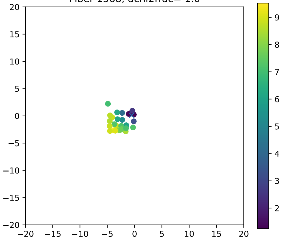
Fiber 1568, dchi2frac= 1.0
