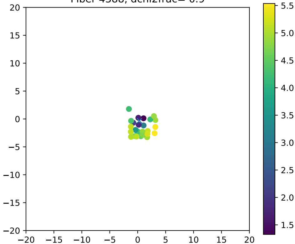
Fiber 4388, dchi2frac= 0.9
