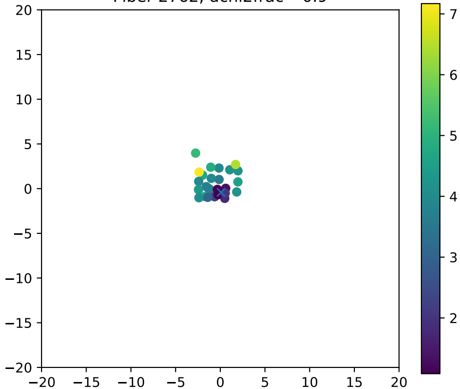
Fiber 2762, dchi2frac= 0.9
