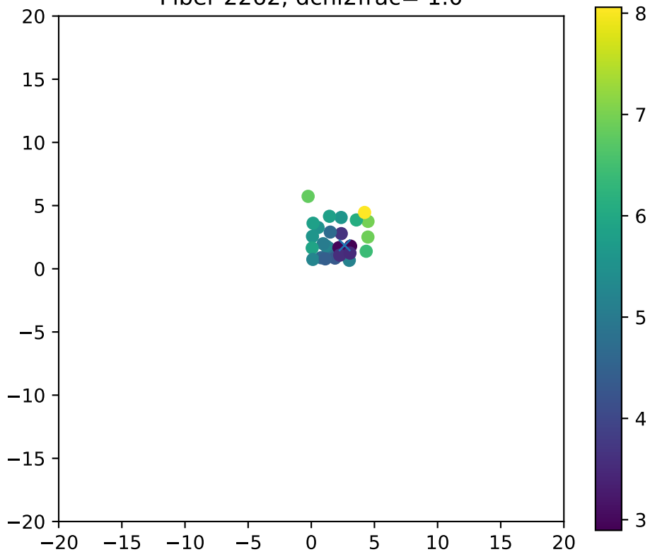
Fiber 2262, dchi2frac= 1.0
