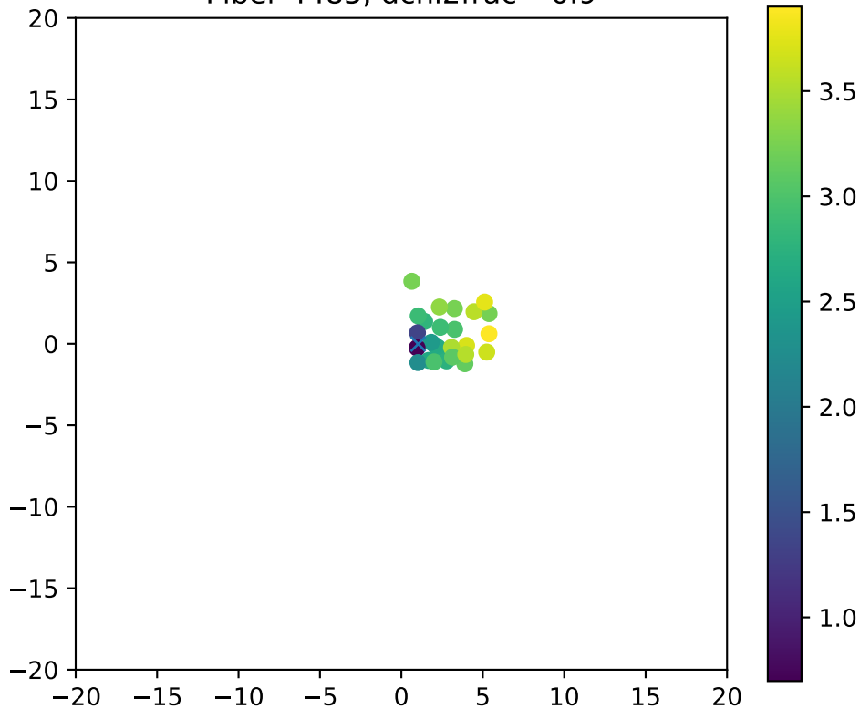
Fiber 4485, dchi2frac= 0.9
