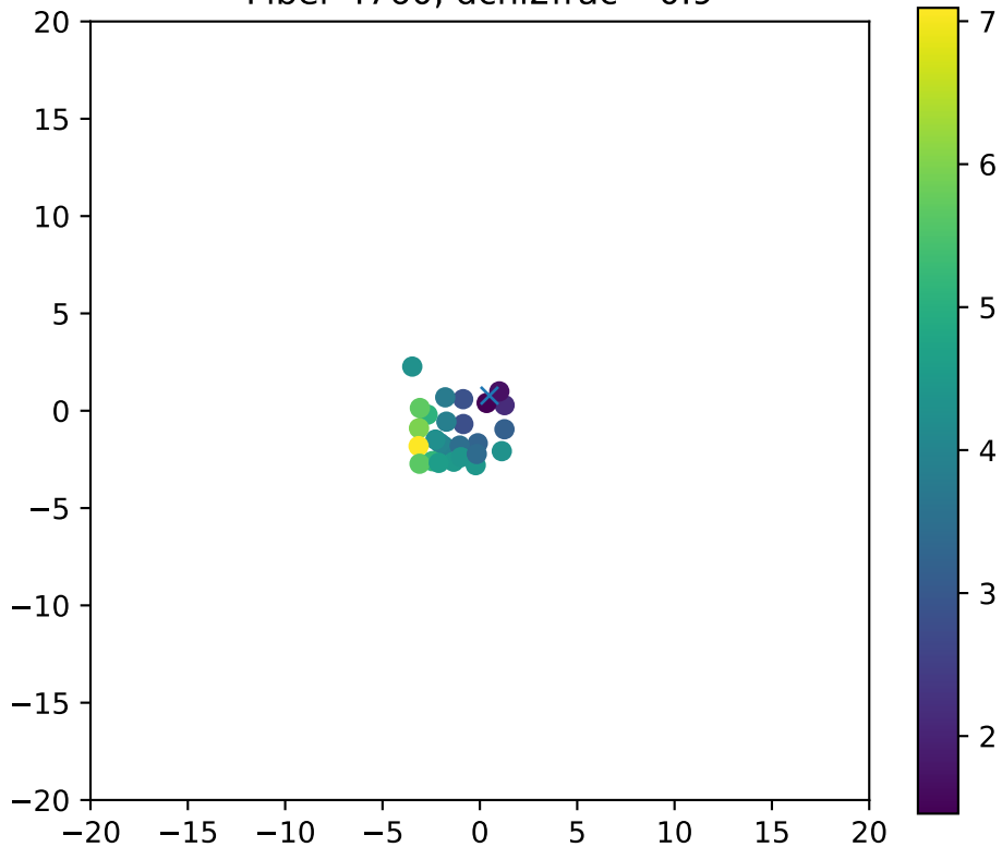
Fiber 4760, dchi2frac= 0.9
