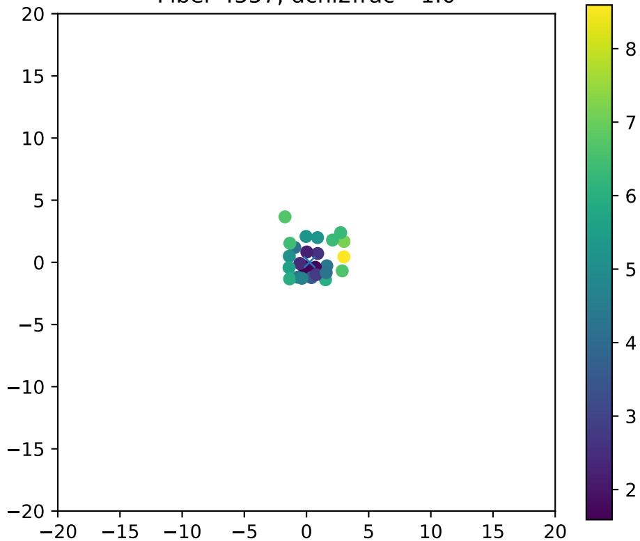
Fiber 4557, dchi2frac= 1.0
