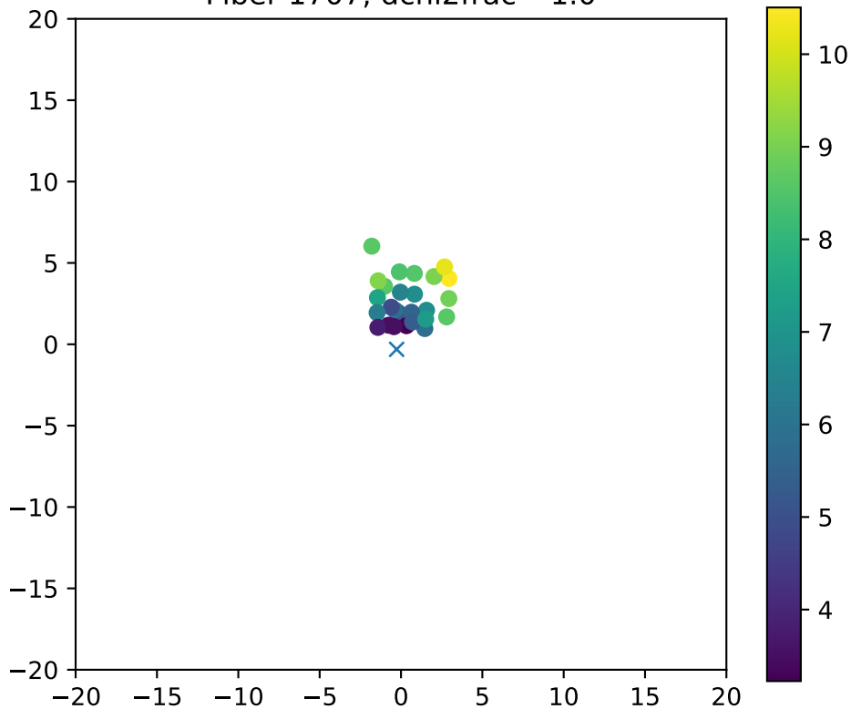
Fiber 1707, dchi2frac= 1.0
