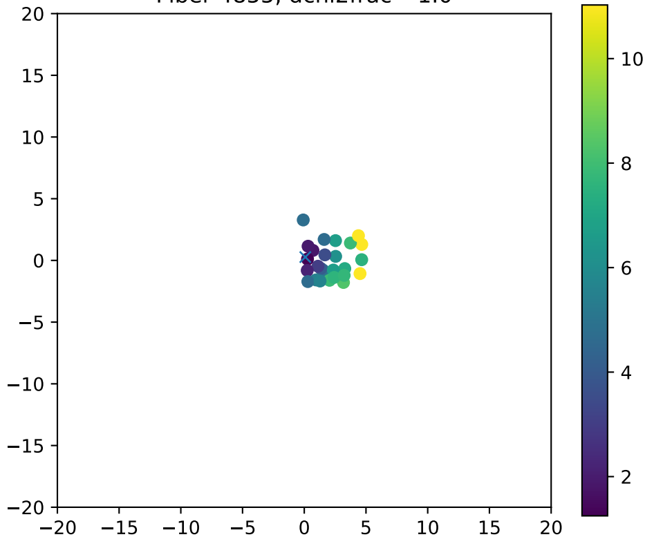
Fiber 4855, dchi2frac= 1.0
