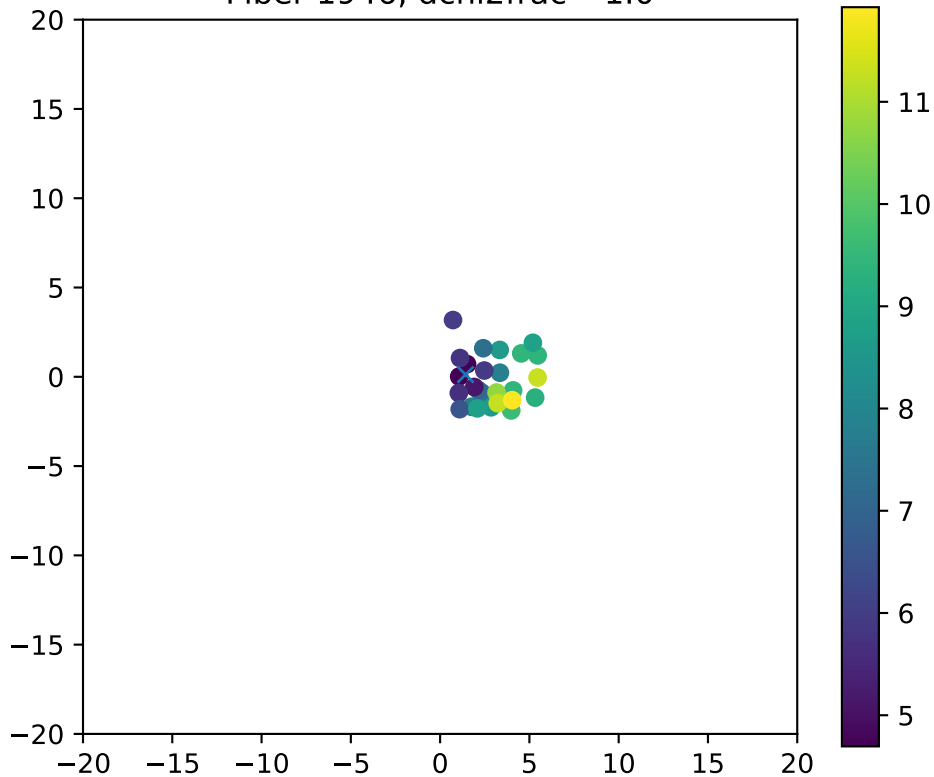
Fiber 1946, dchi2frac= 1.0
