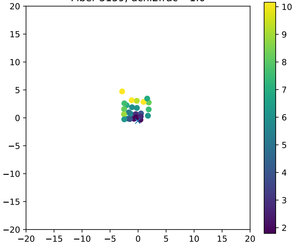
Fiber 3159, dchi2frac= 1.0
