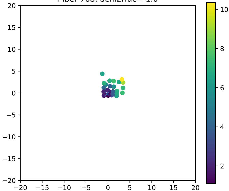
Fiber 768, dchi2frac= 1.0
