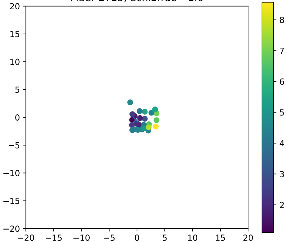
Fiber 2715, dchi2frac= 1.0
