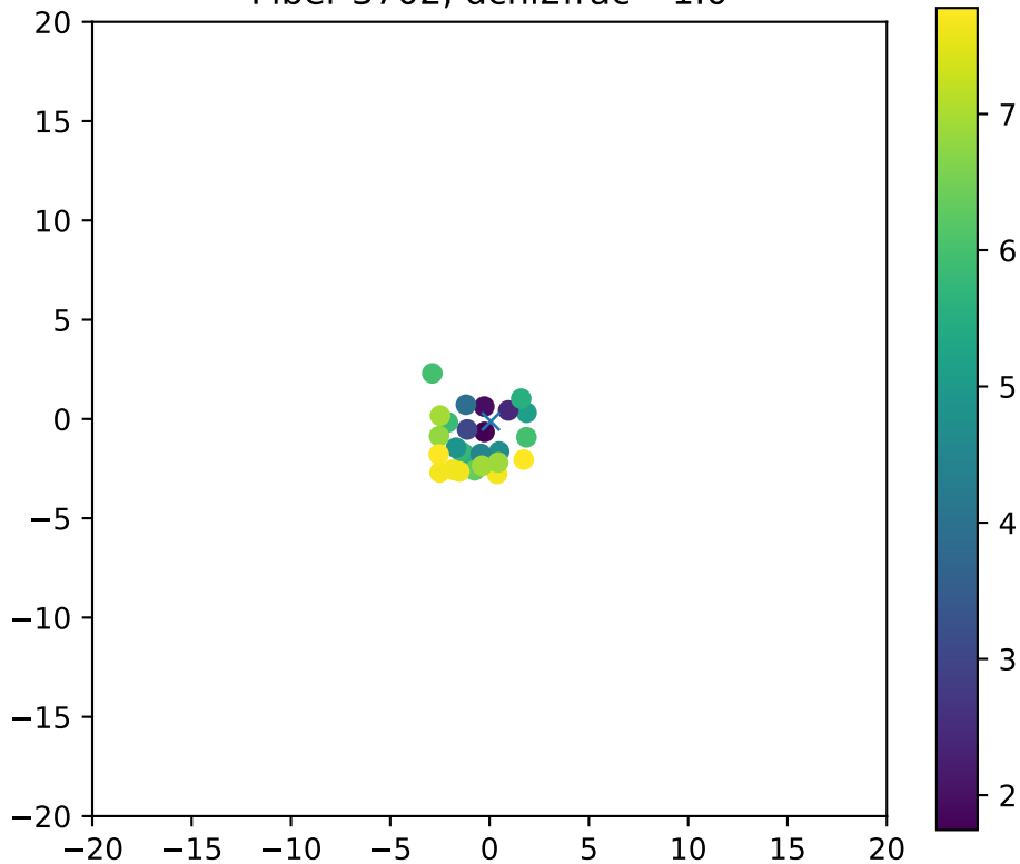
Fiber 3702, dchi2frac= 1.0
