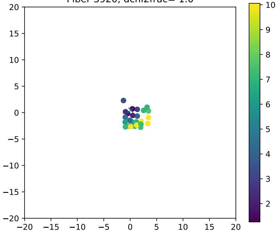
Fiber 3920, dchi2frac= 1.0
