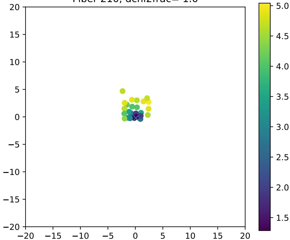
Fiber 210, dchi2frac= 1.0
