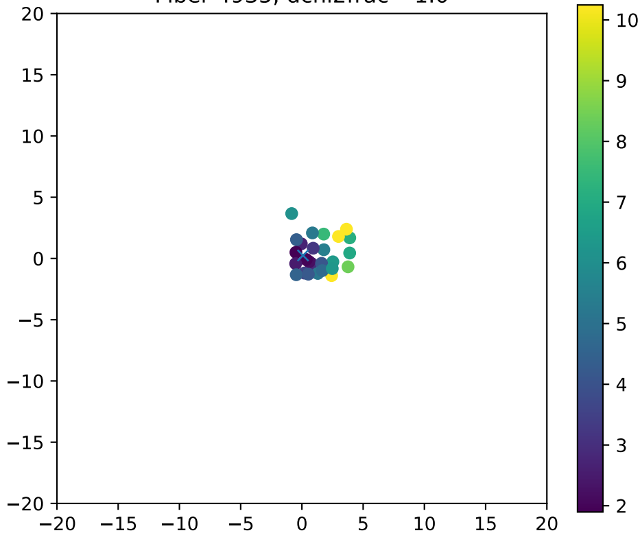
Fiber 4935, dchi2frac= 1.0
