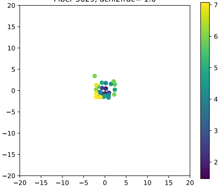
Fiber 3629, dchi2frac= 1.0
