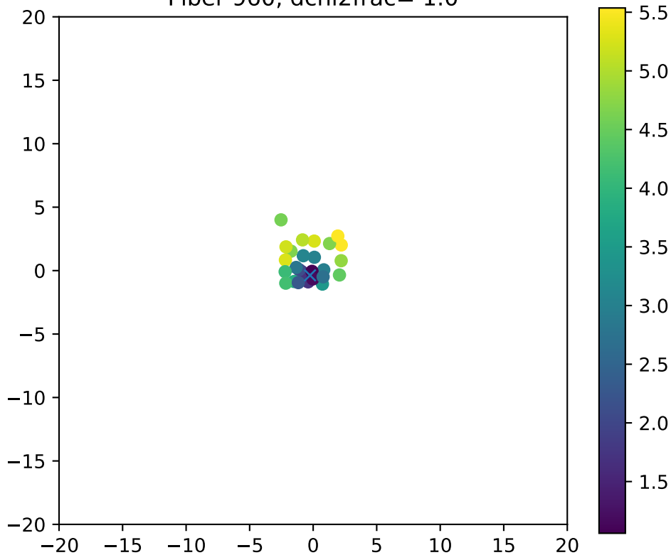
Fiber 960, dchi2frac= 1.0
