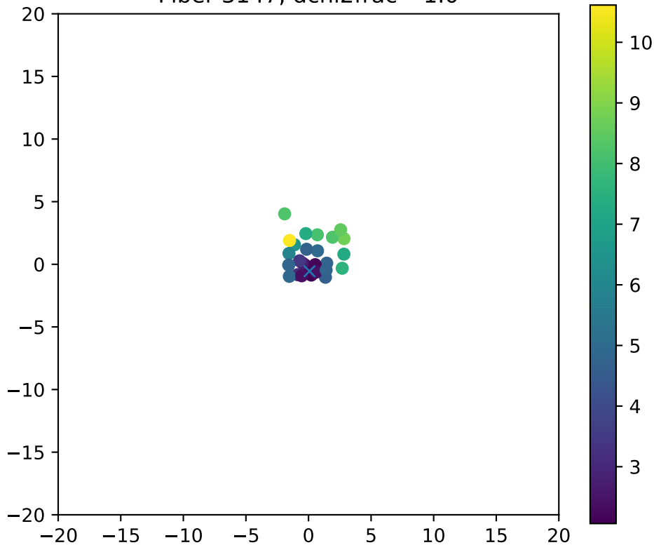
Fiber 3147, dchi2frac= 1.0
