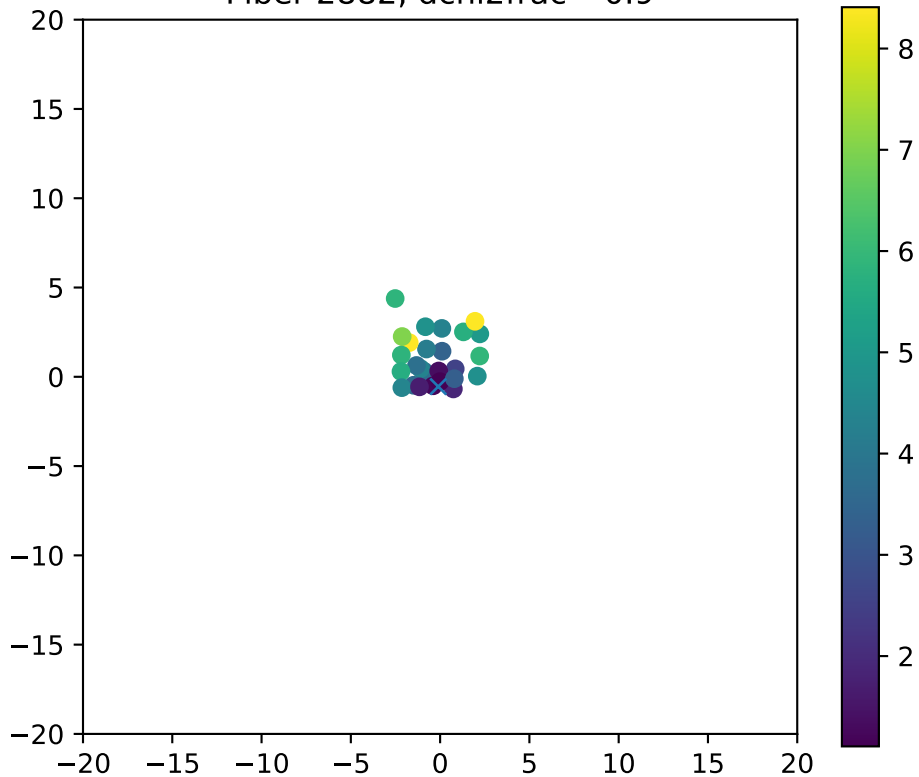
Fiber 2882, dchi2frac= 0.9
