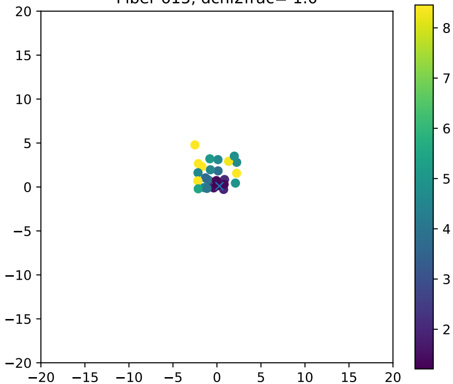
Fiber 615, dchi2frac= 1.0
