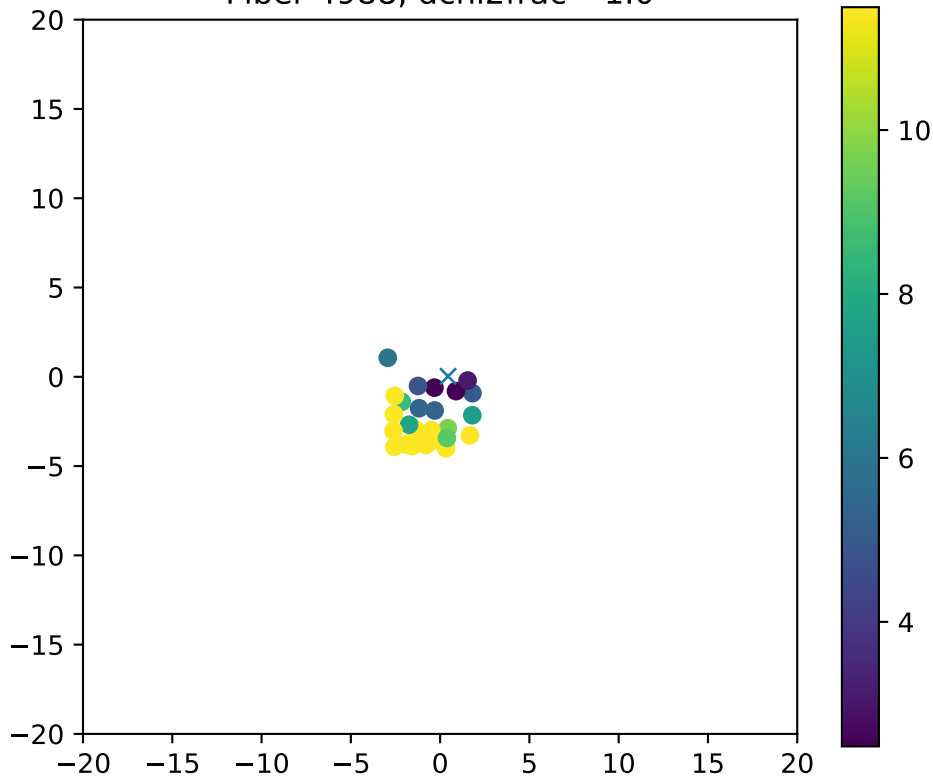
Fiber 4988, dchi2frac= 1.0
