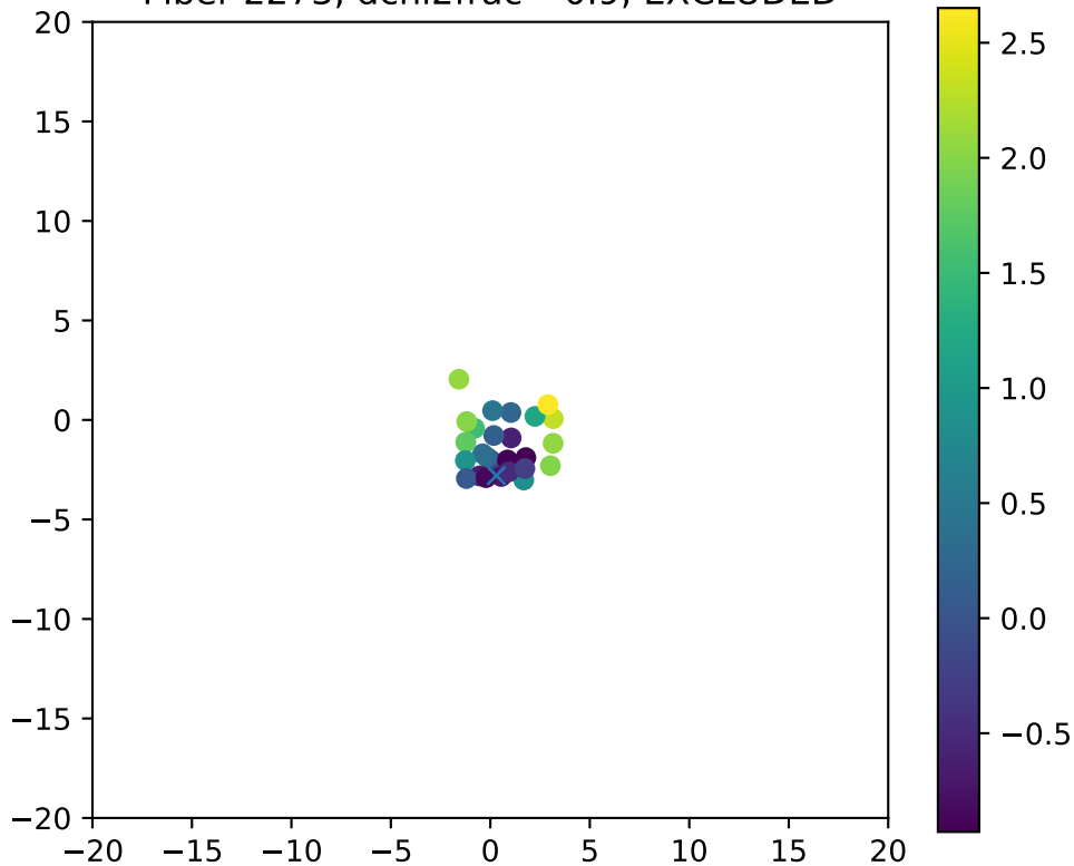
Fiber 2273, dchi2frac= 0.9, EXCLUDED
