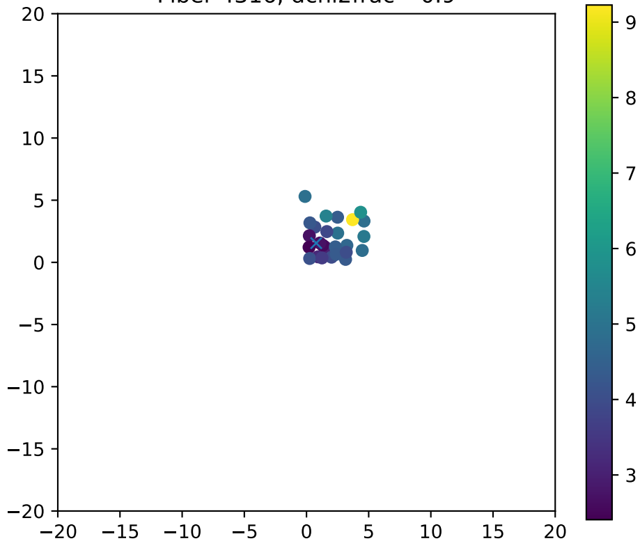
Fiber 4316, dchi2frac= 0.9
