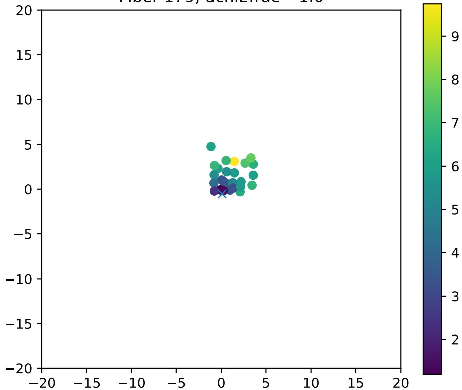
Fiber 179, dchi2frac= 1.0
