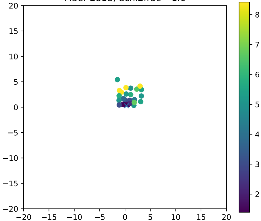
Fiber 2818, dchi2frac= 1.0
