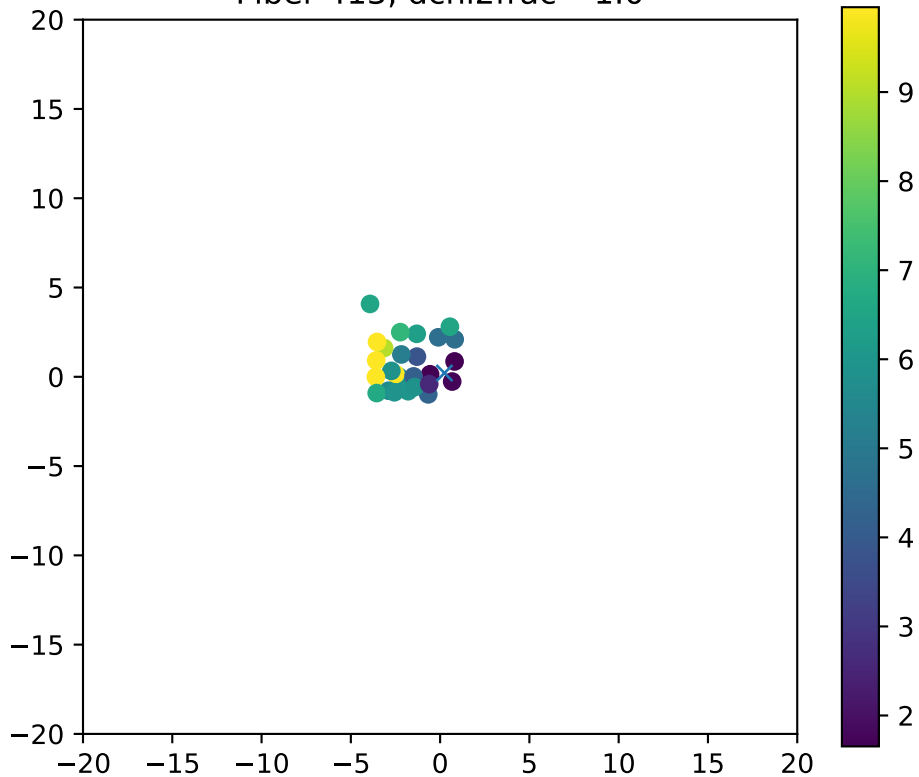
Fiber 413, dchi2frac= 1.0
