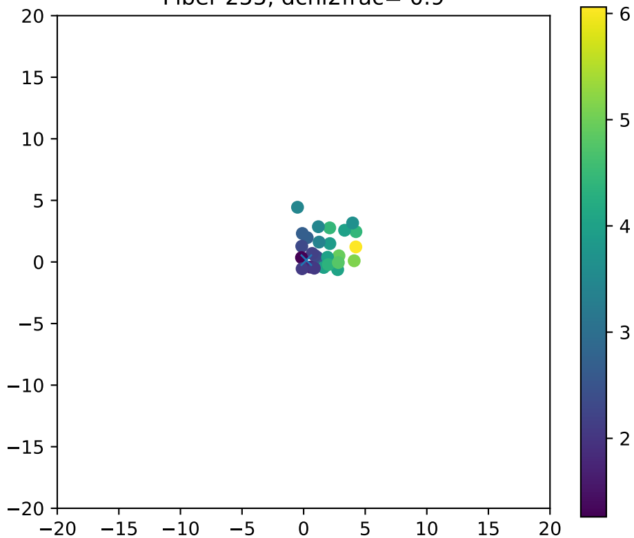
Fiber 255, dchi2frac= 0.9
