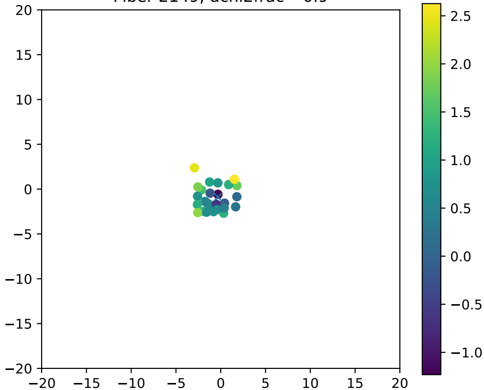
Fiber 2149, dchi2frac= 0.9
