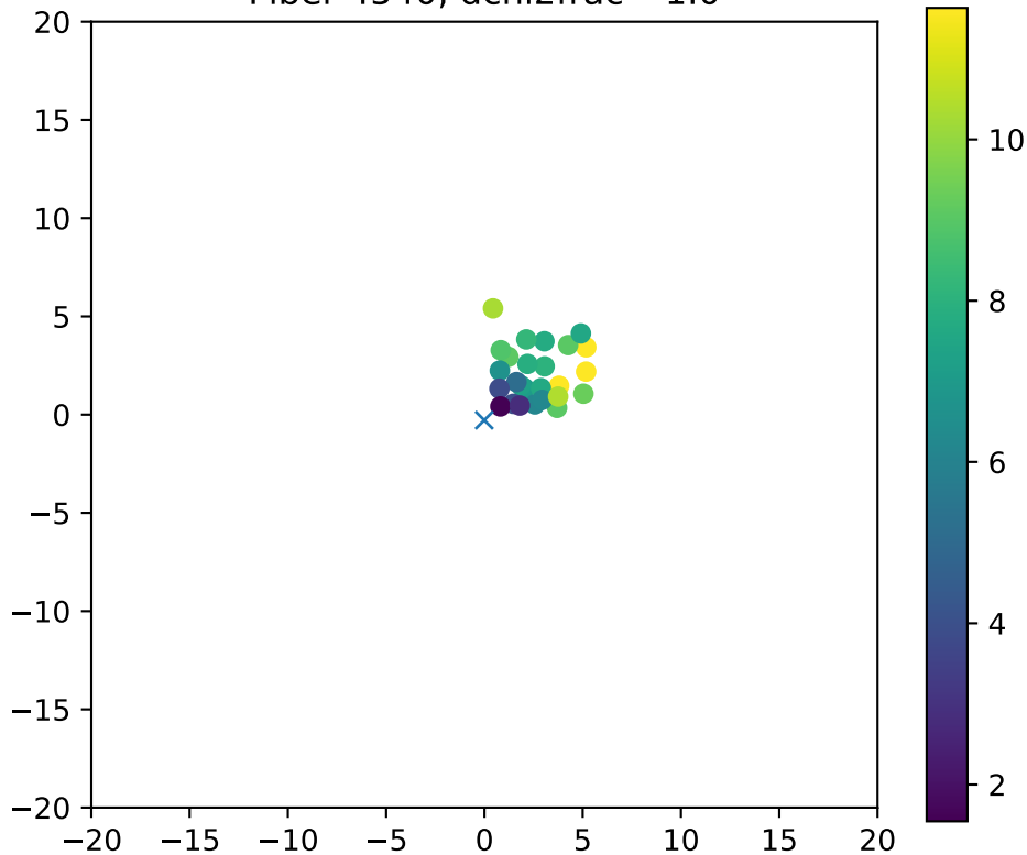
Fiber 4540, dchi2frac= 1.0
