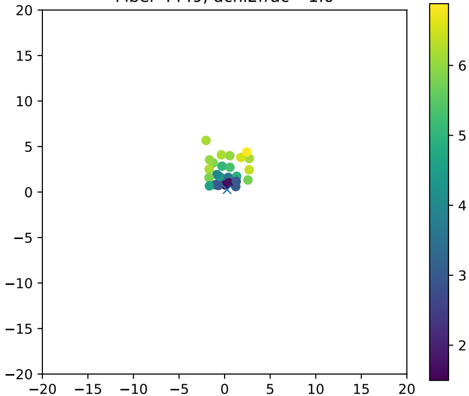
Fiber 4449, dchi2frac= 1.0
