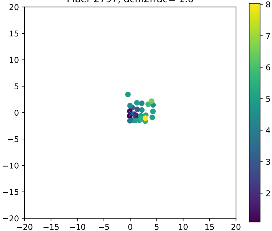
Fiber 2797, dchi2frac= 1.0
