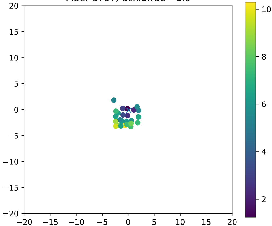
Fiber 3707, dchi2frac= 1.0
