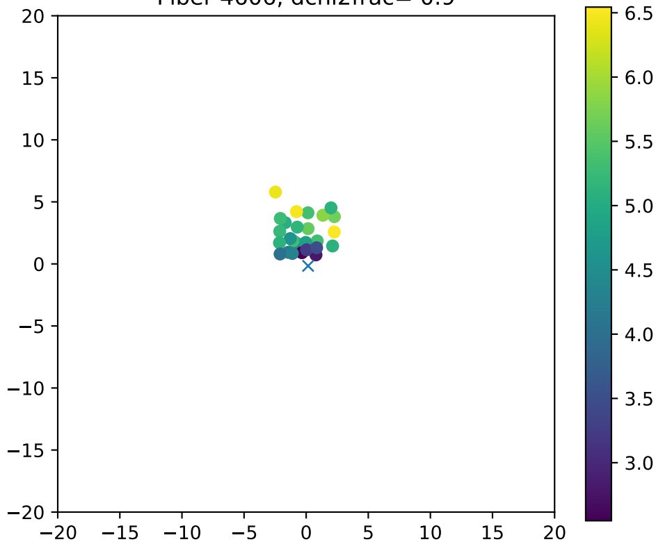
Fiber 4606, dchi2frac= 0.9
