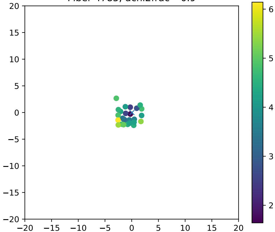
Fiber 4785, dchi2frac= 0.9
