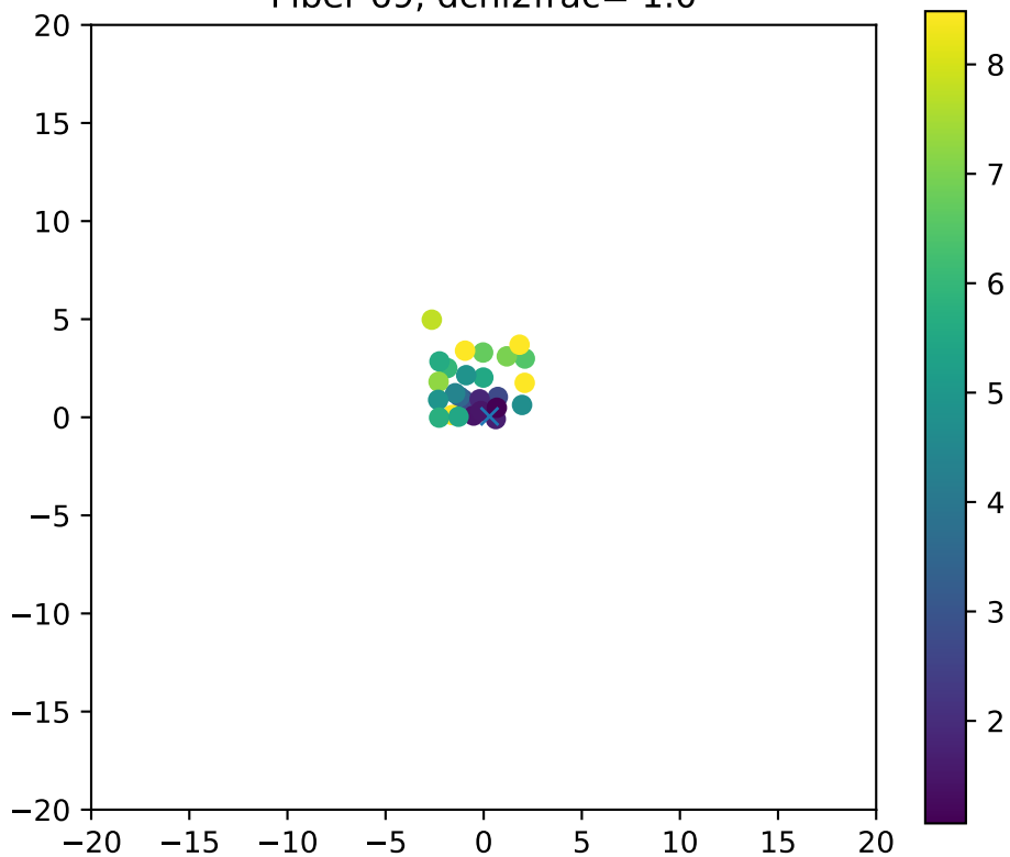
Fiber 69, dchi2frac= 1.0
