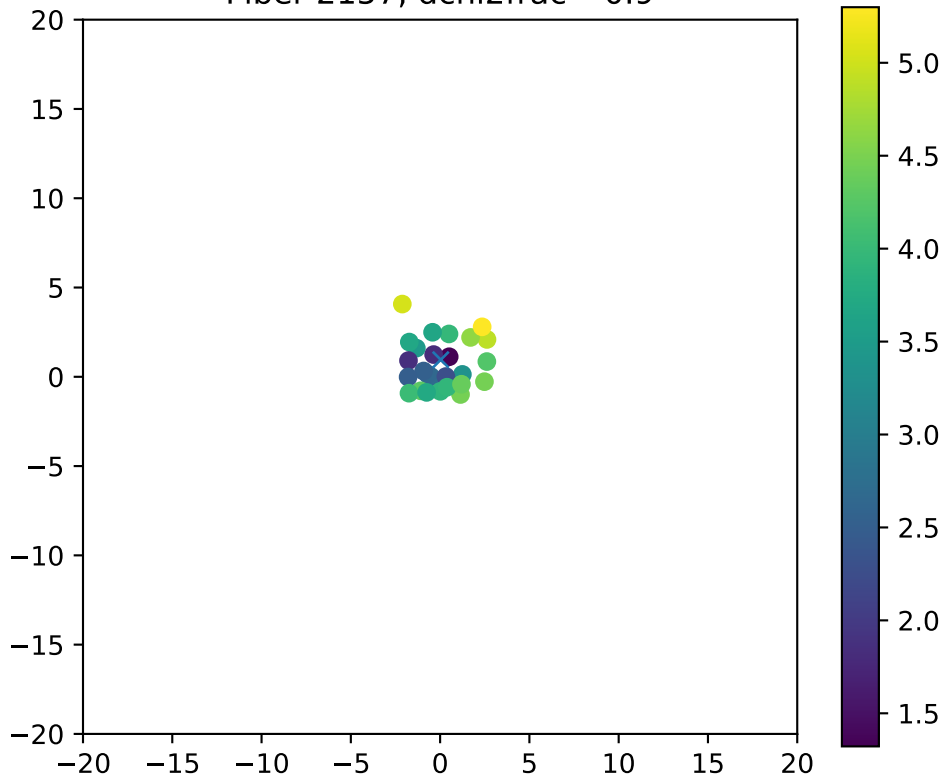
Fiber 2157, dchi2frac= 0.9
