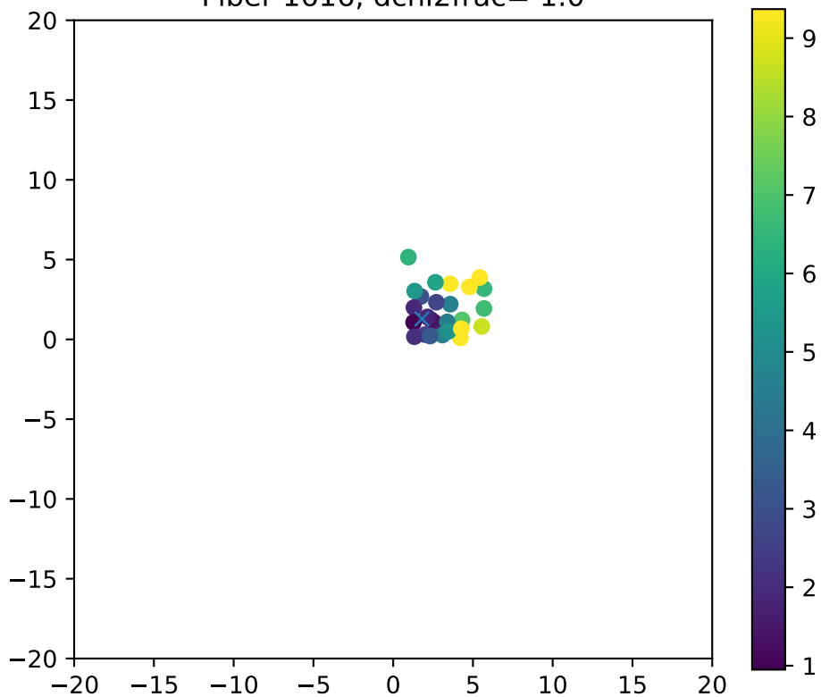
Fiber 1616, dchi2frac= 1.0
