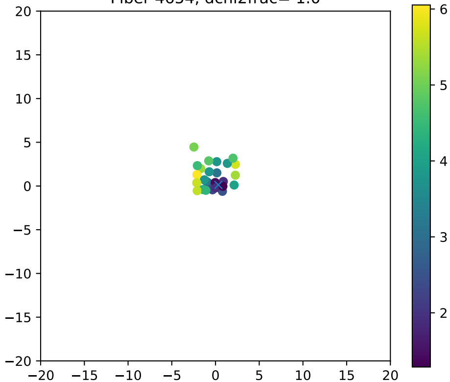
Fiber 4654, dchi2frac= 1.0
