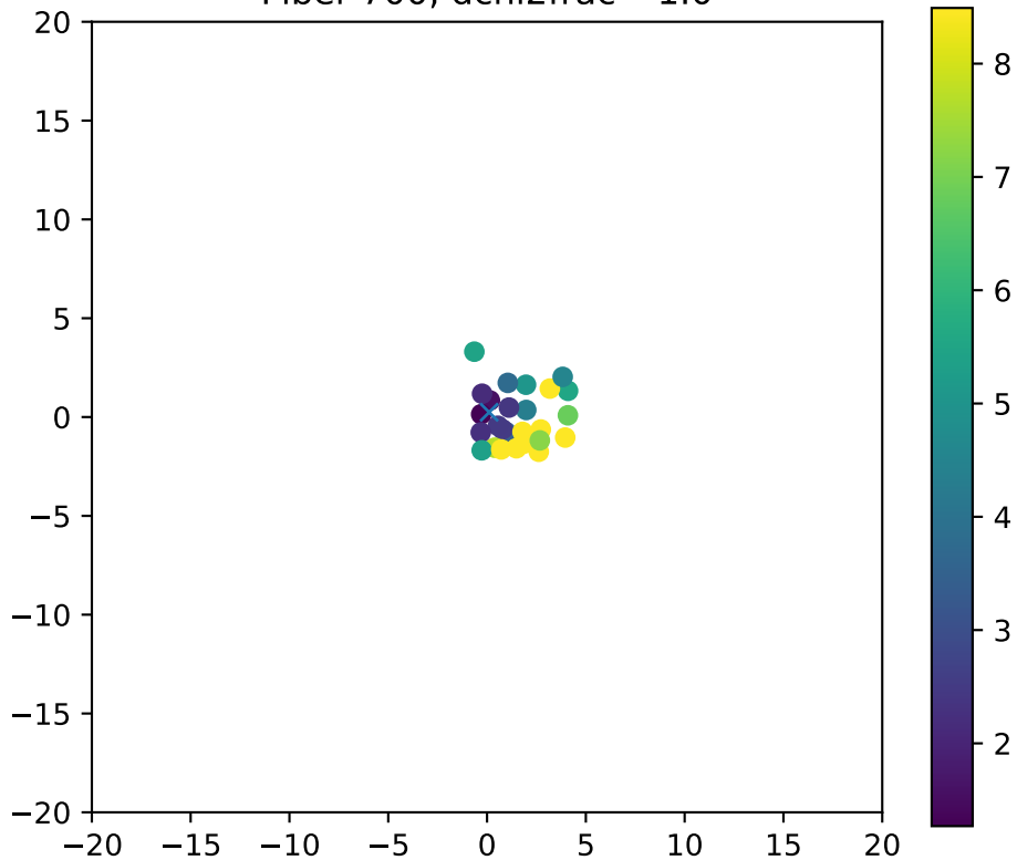
Fiber 700, dchi2frac= 1.0
