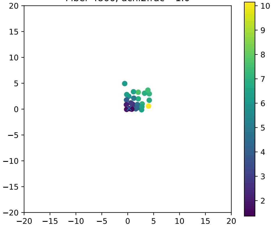
Fiber 4866, dchi2frac= 1.0
