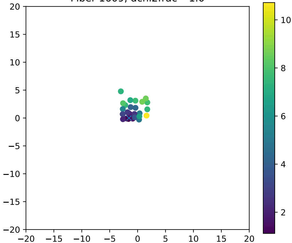
Fiber 1609, dchi2frac= 1.0
