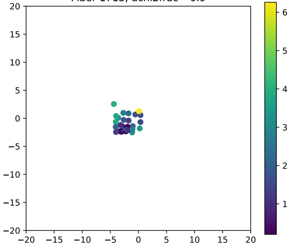
Fiber 1713, dchi2frac= 0.9
