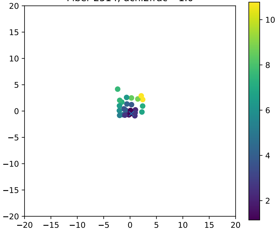
Fiber 2514, dchi2frac= 1.0
