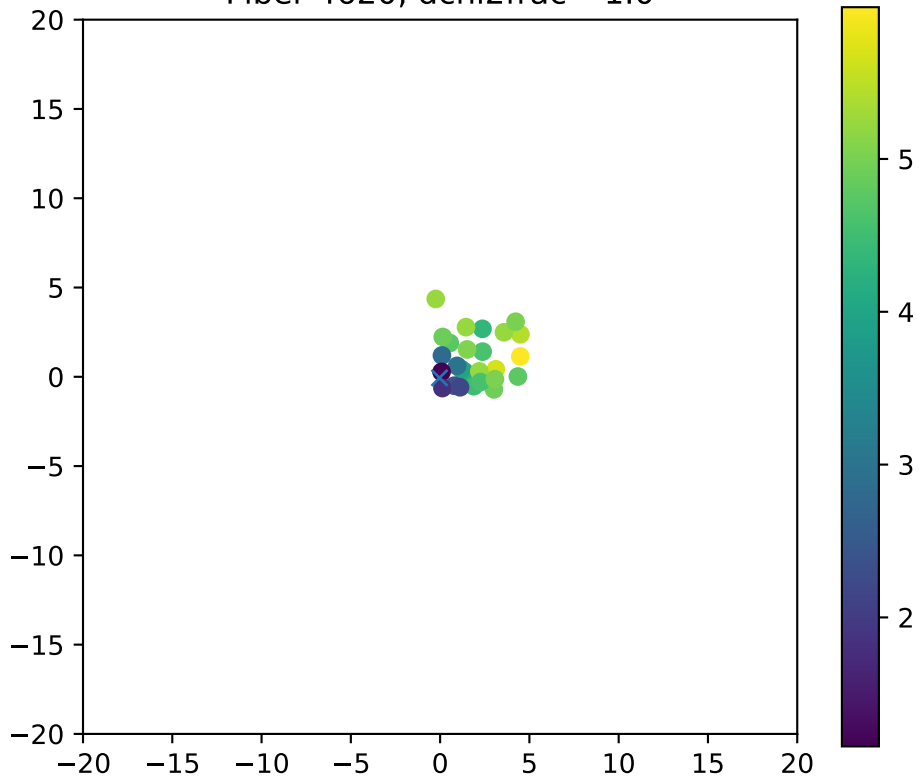
Fiber 4620, dchi2frac= 1.0
