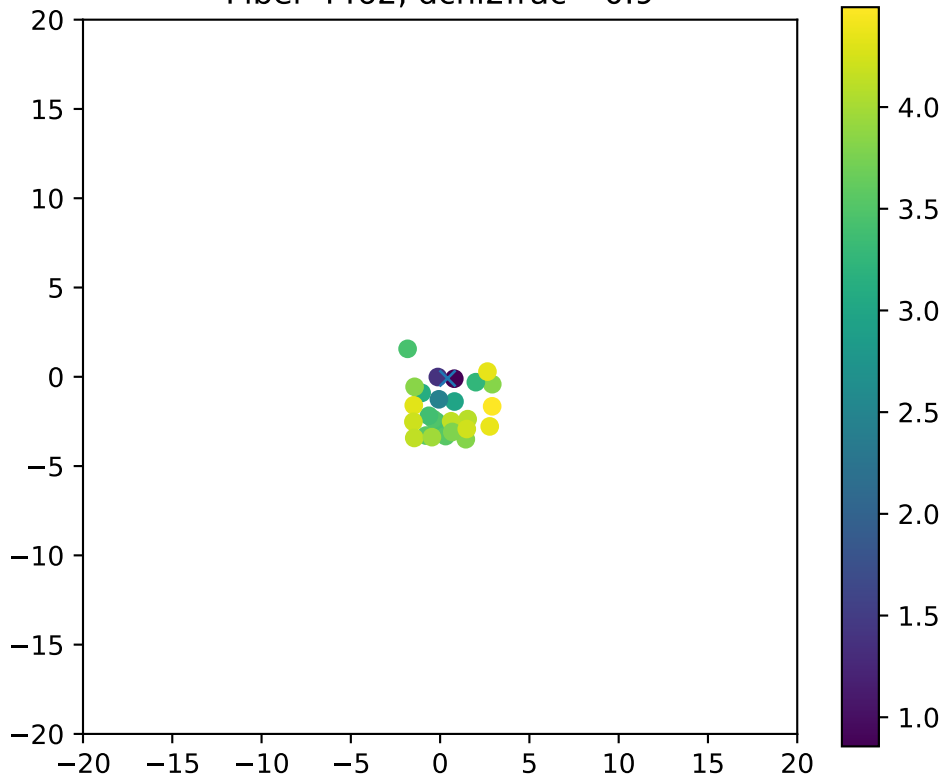
Fiber 4462, dchi2frac= 0.9
