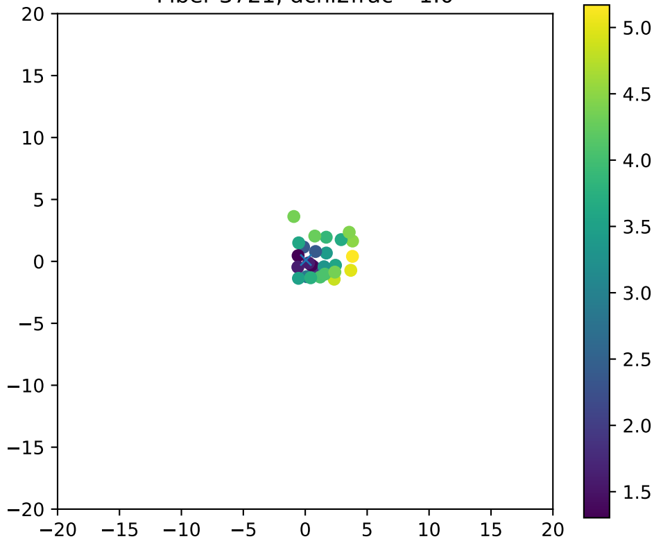
Fiber 3721, dchi2frac= 1.0
