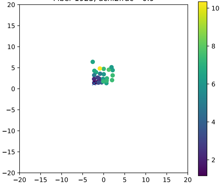
Fiber 1923, dchi2frac= 0.9
