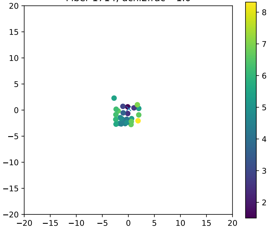
Fiber 1714, dchi2frac= 1.0
