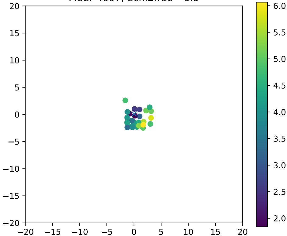
Fiber 4607, dchi2frac= 0.9
