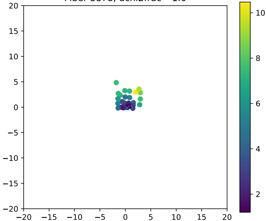
Fiber 3878, dchi2frac= 1.0
