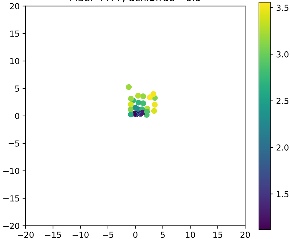
Fiber 4477, dchi2frac= 0.9
