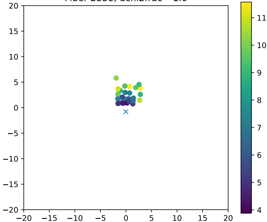
Fiber 2538, dchi2frac= 1.0
