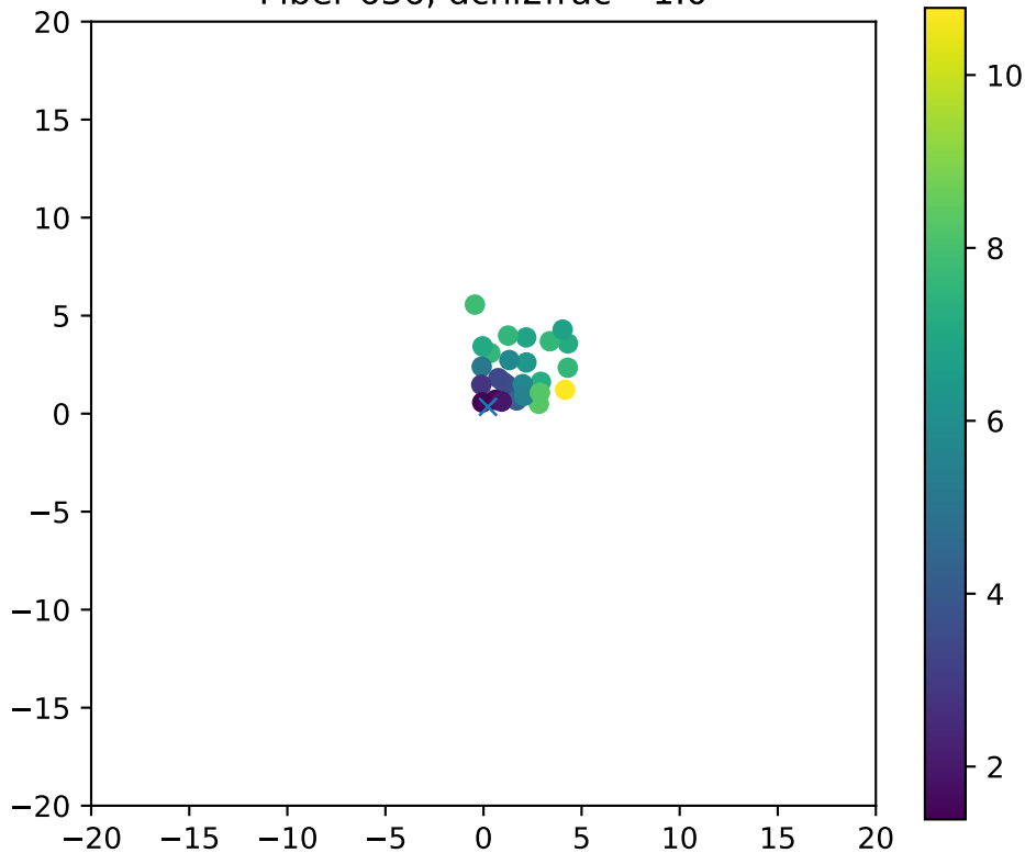
Fiber 636, dchi2frac= 1.0
