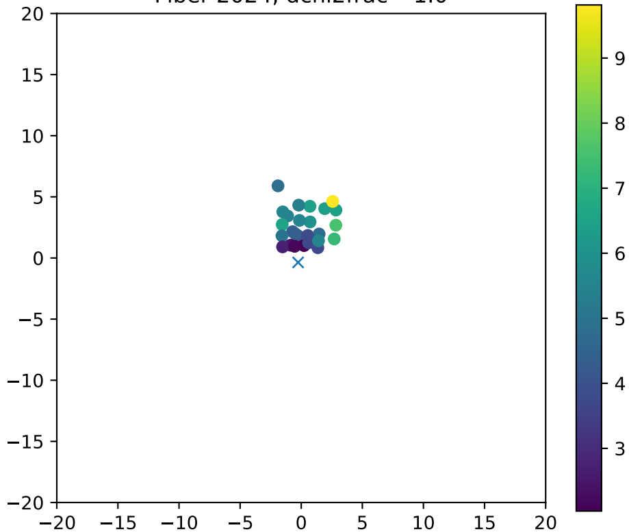
Fiber 2024, dchi2frac= 1.0
