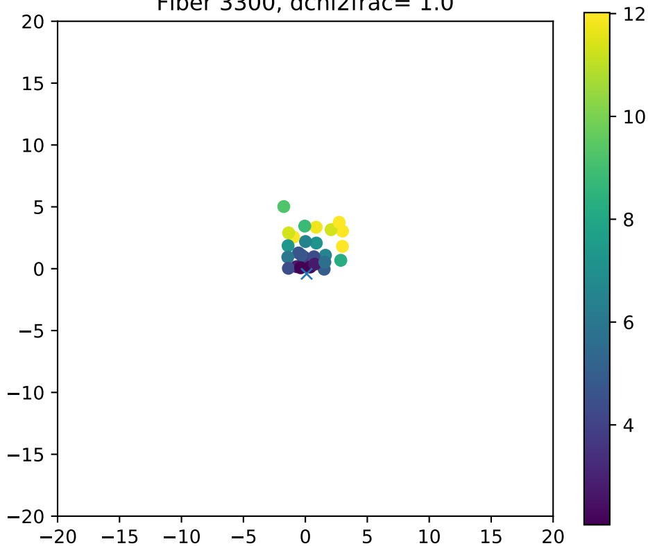
Fiber 3300, dchi2frac= 1.0
