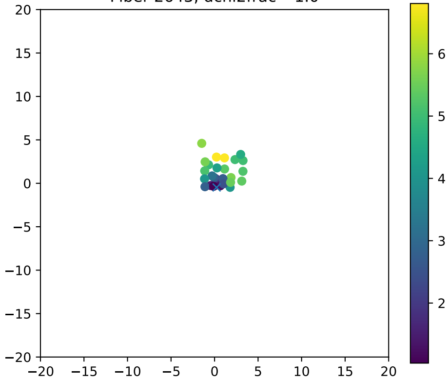
Fiber 2643, dchi2frac= 1.0
