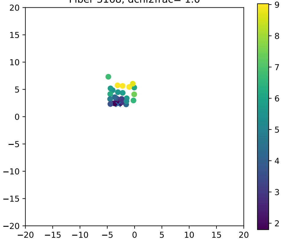
Fiber 3168, dchi2frac= 1.0
