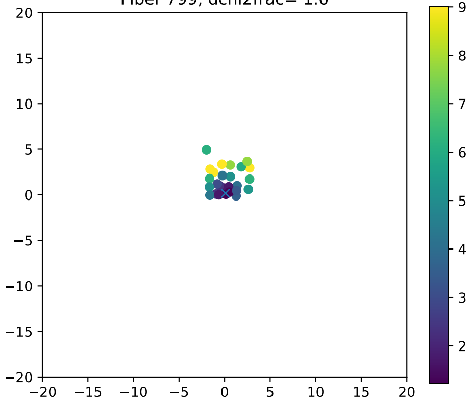
Fiber 799, dchi2frac= 1.0
