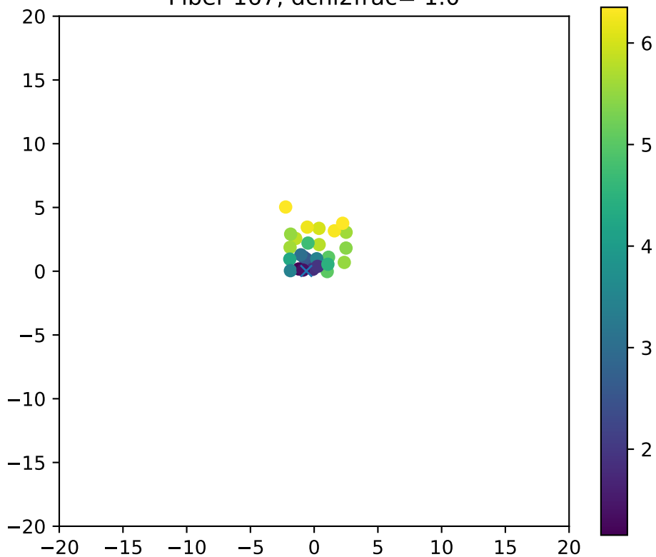
Fiber 167, dchi2frac= 1.0
