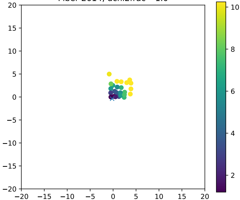
Fiber 2614, dchi2frac= 1.0
