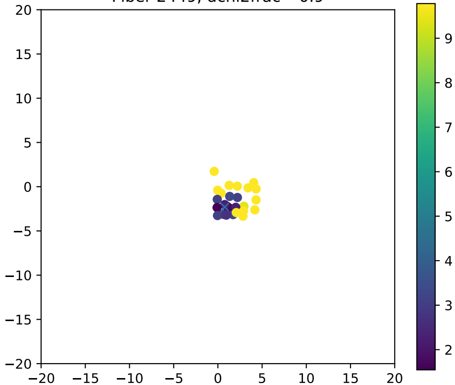
Fiber 2449, dchi2frac= 0.9
