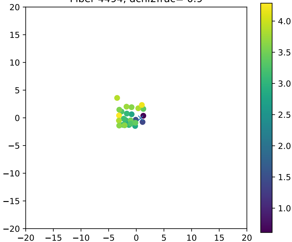
Fiber 4494, dchi2frac= 0.9
