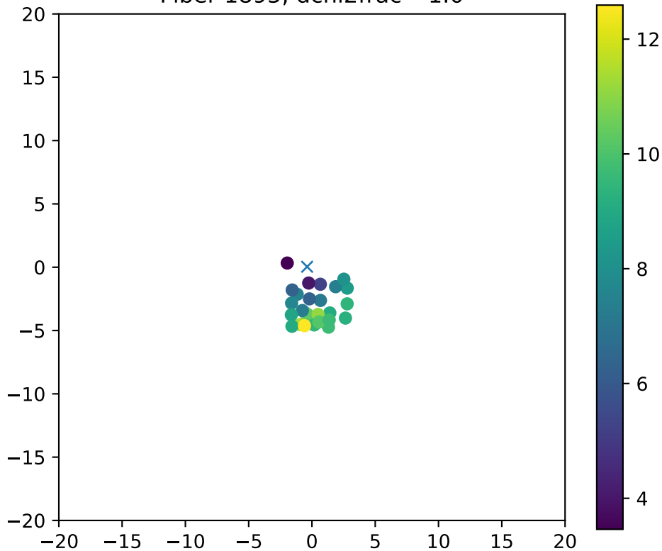
Fiber 1895, dchi2frac= 1.0
