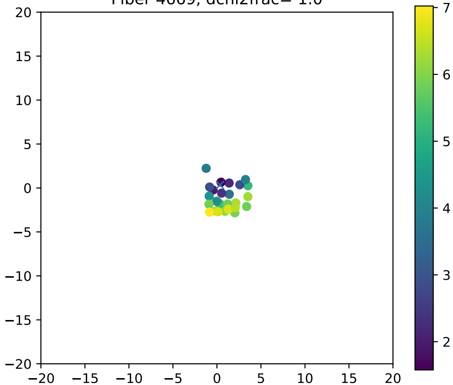
Fiber 4669, dchi2frac= 1.0
