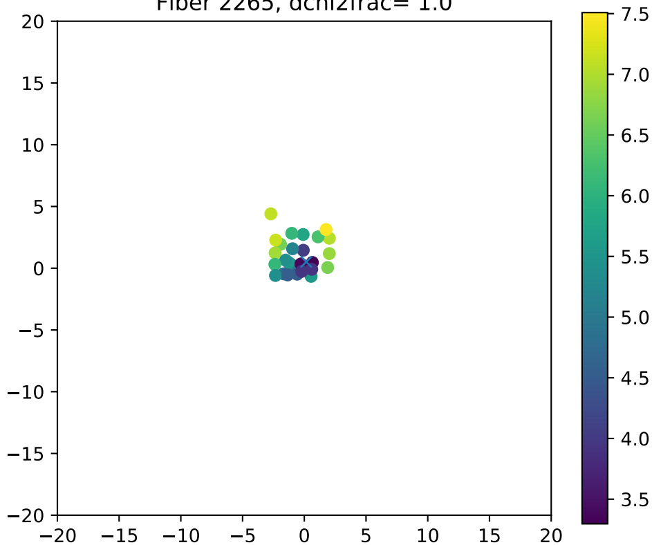
Fiber 2265, dchi2frac= 1.0
