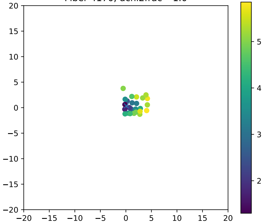
Fiber 4170, dchi2frac= 1.0
