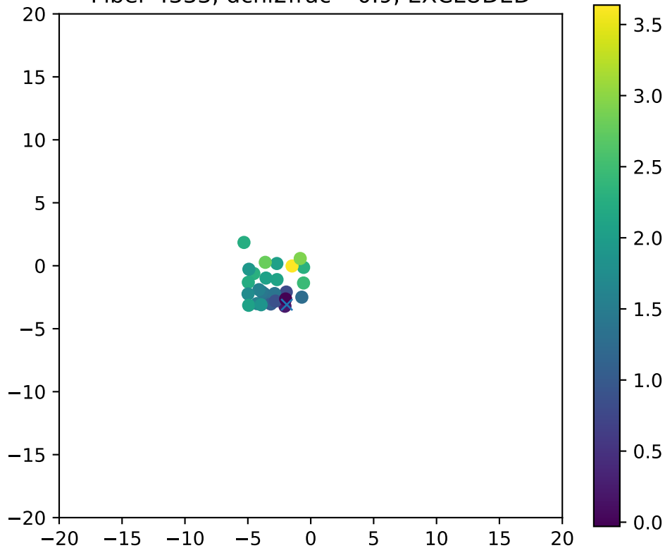
Fiber 4333, dchi2frac= 0.9, EXCLUDED
