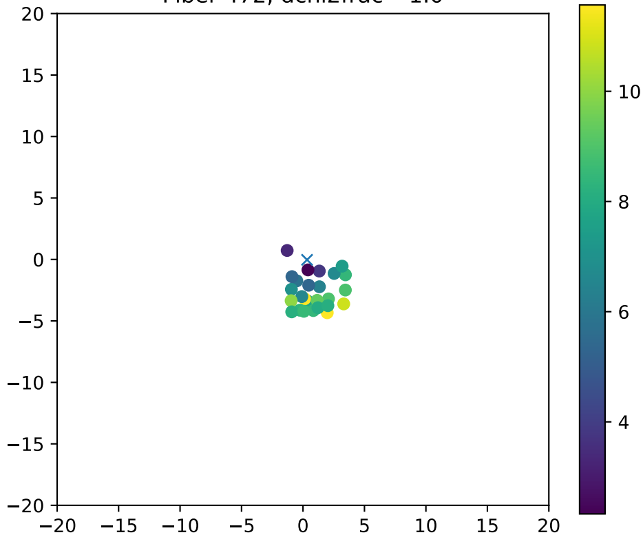
Fiber 472, dchi2frac= 1.0
