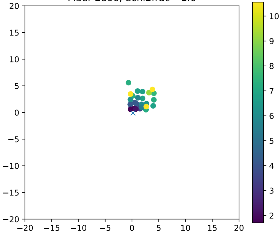
Fiber 2806, dchi2frac= 1.0
