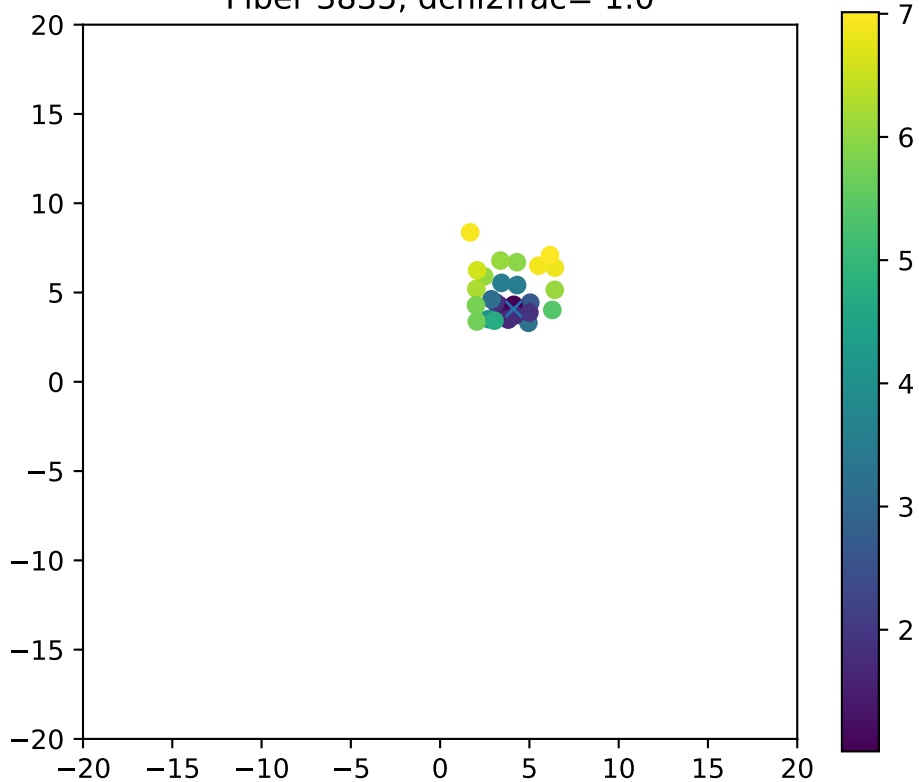
Fiber 3835, dchi2frac= 1.0
