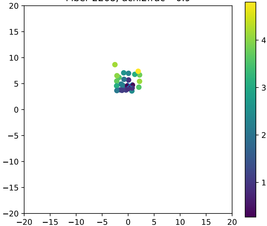
Fiber 2268, dchi2frac= 0.9
