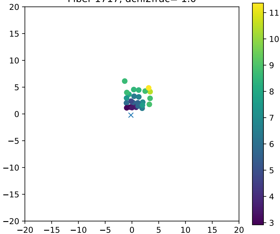
Fiber 1717, dchi2frac= 1.0
