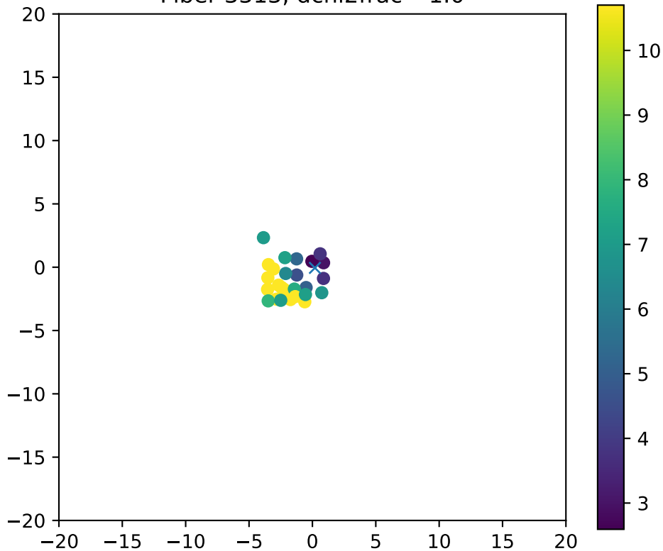
Fiber 3313, dchi2frac= 1.0
