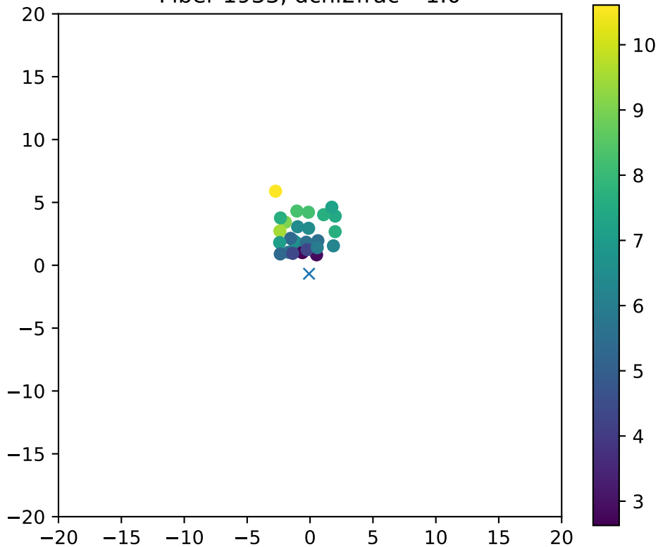
Fiber 1933, dchi2frac= 1.0
