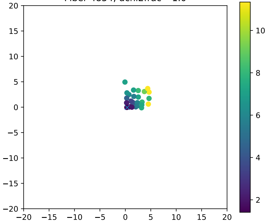
Fiber 4854, dchi2frac= 1.0
