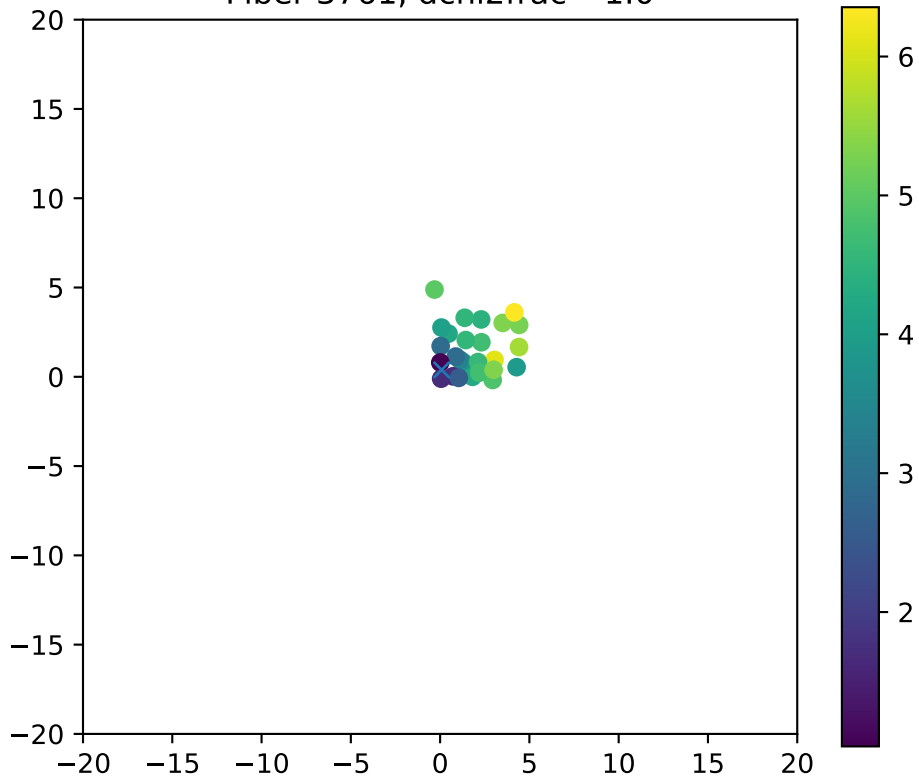
Fiber 3761, dchi2frac= 1.0
