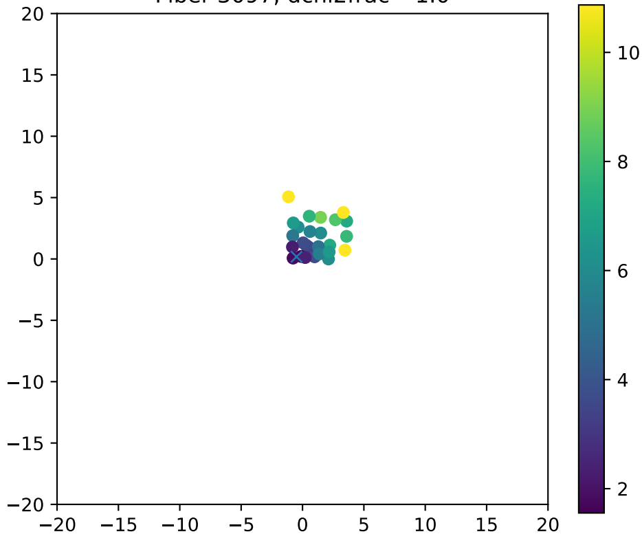
Fiber 3097, dchi2frac= 1.0
