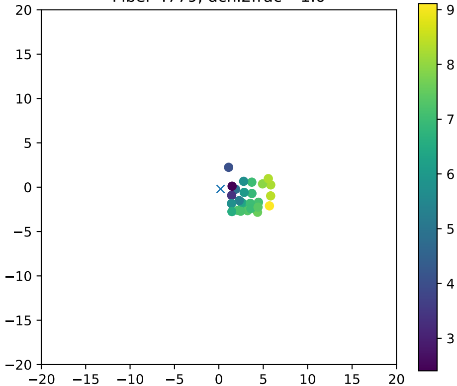
Fiber 4779, dchi2frac= 1.0
