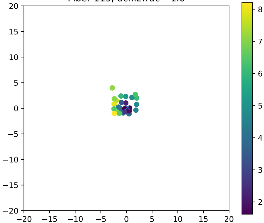
Fiber 119, dchi2frac= 1.0
