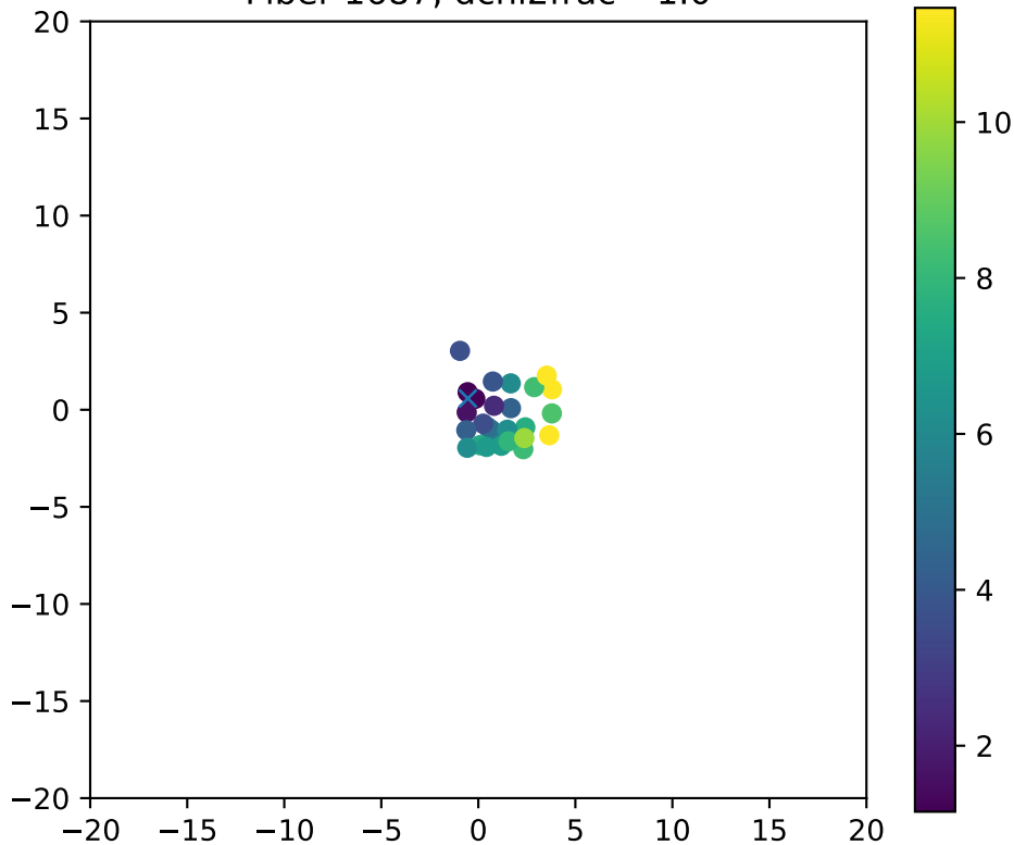
Fiber 1687, dchi2frac= 1.0
