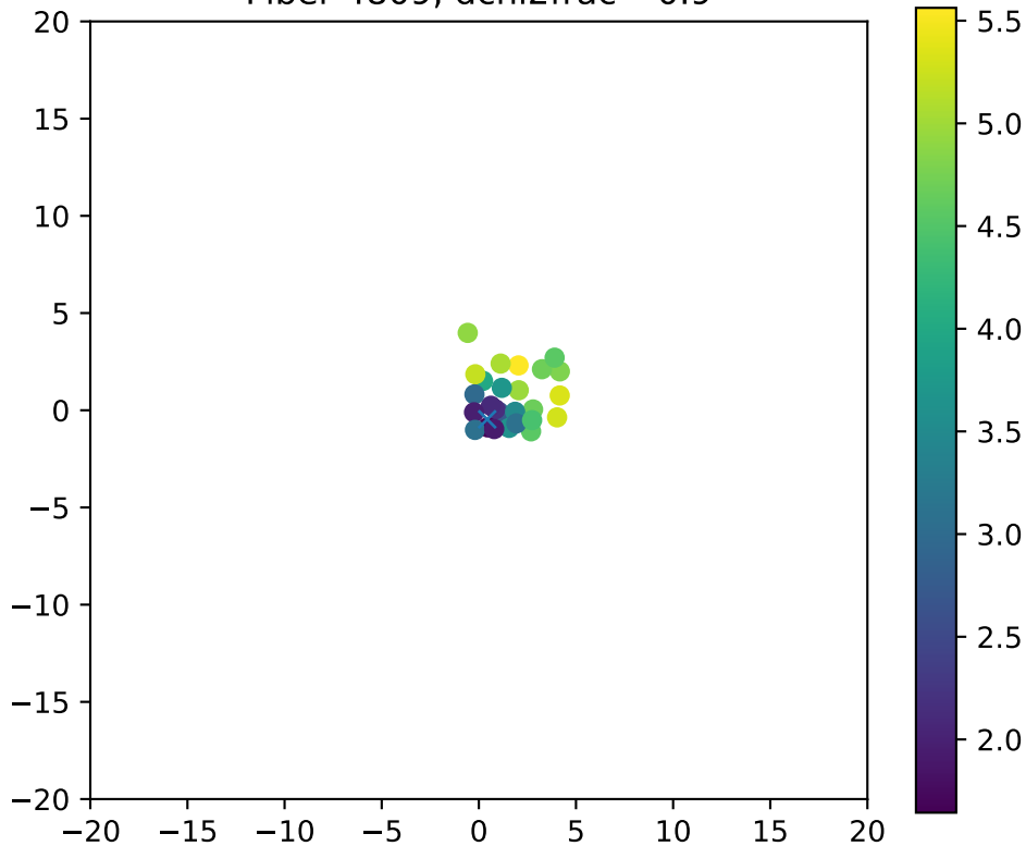
Fiber 4809, dchi2frac= 0.9
