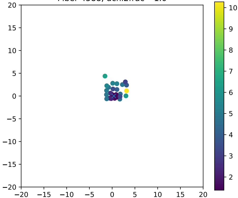
Fiber 4588, dchi2frac= 1.0
