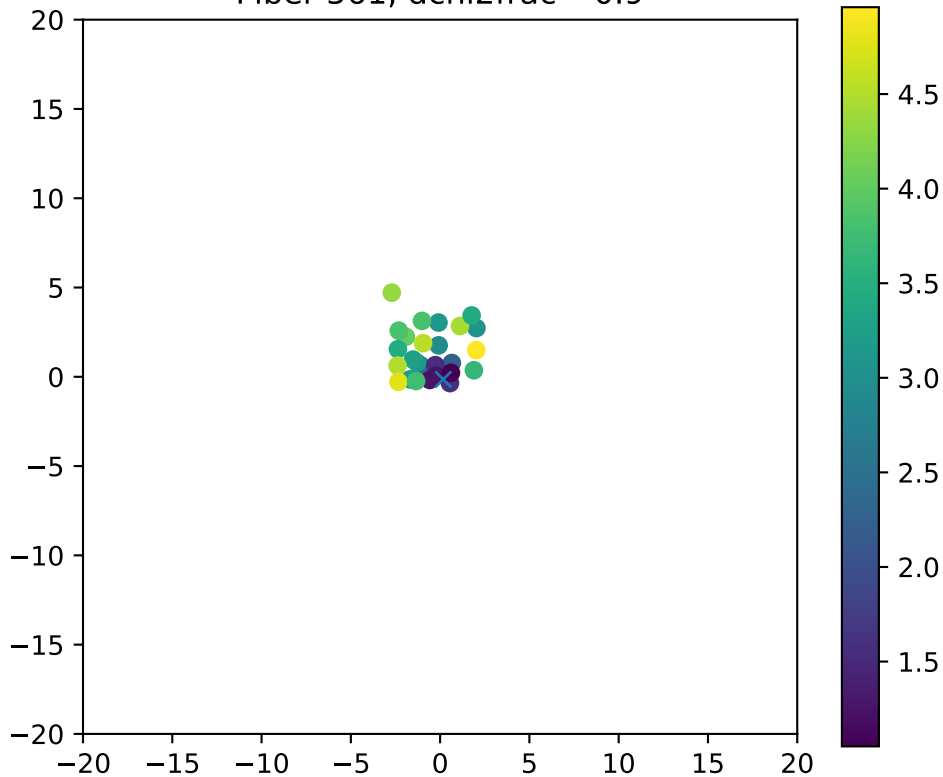
Fiber 561, dchi2frac= 0.9
