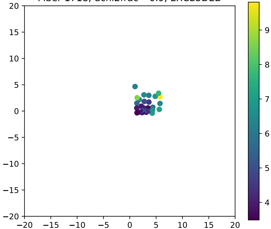
Fiber 1718, dchi2frac= 0.9, EXCLUDED
