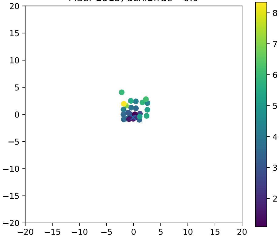
Fiber 2915, dchi2frac= 0.9
