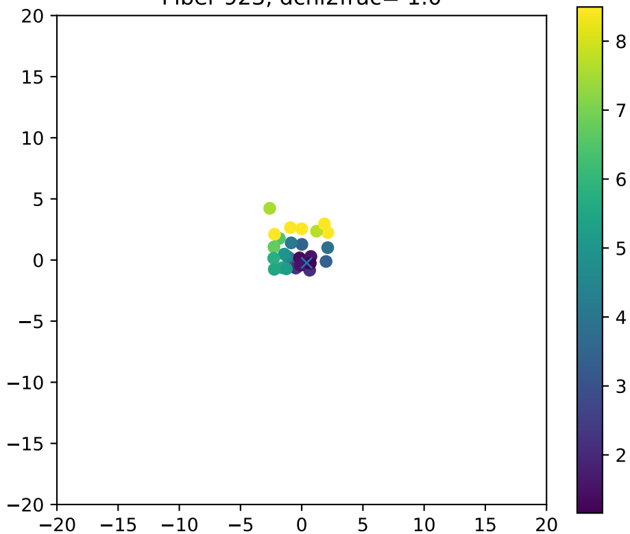
Fiber 923, dchi2frac= 1.0
