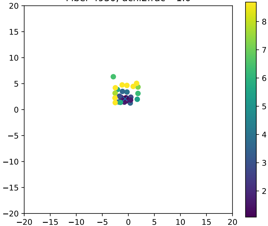
Fiber 4930, dchi2frac= 1.0
