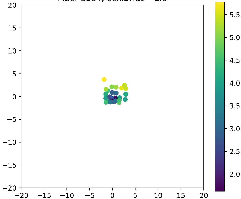
Fiber 3234, dchi2frac= 1.0
