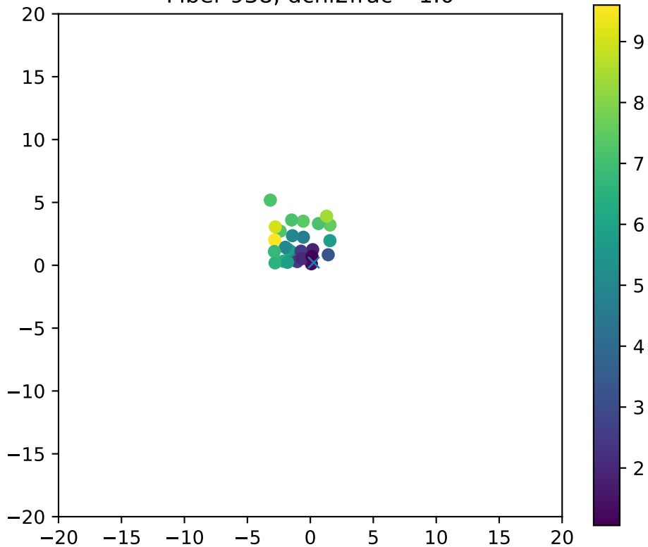
Fiber 938, dchi2frac= 1.0
