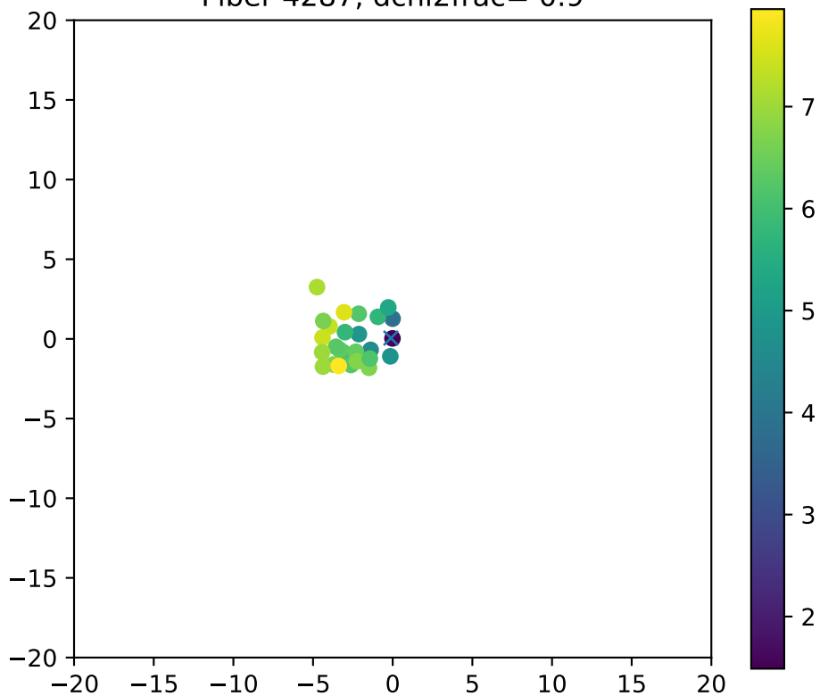
Fiber 4287, dchi2frac= 0.9
