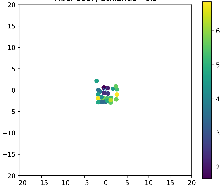
Fiber 1817, dchi2frac= 0.9
