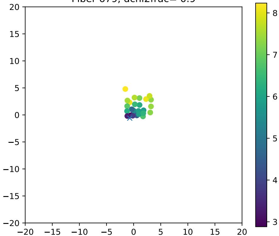
Fiber 679, dchi2frac= 0.9
