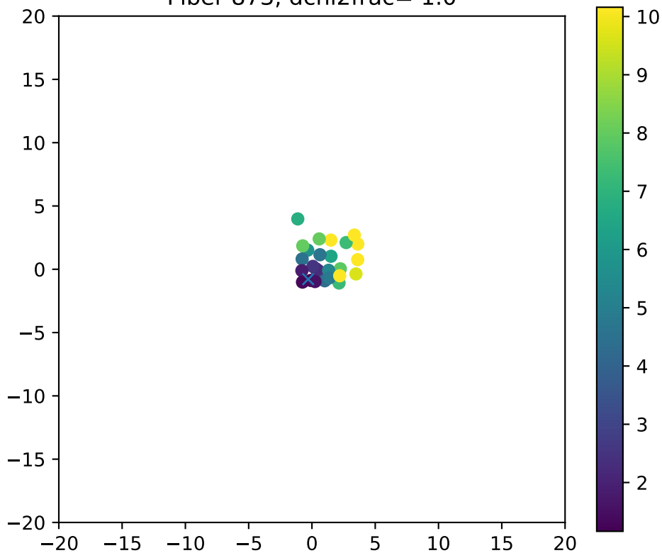
Fiber 873, dchi2frac= 1.0
