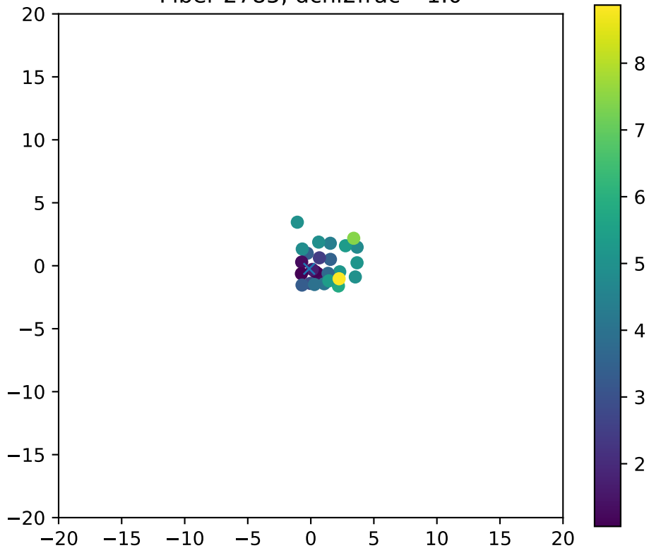
Fiber 2785, dchi2frac= 1.0
