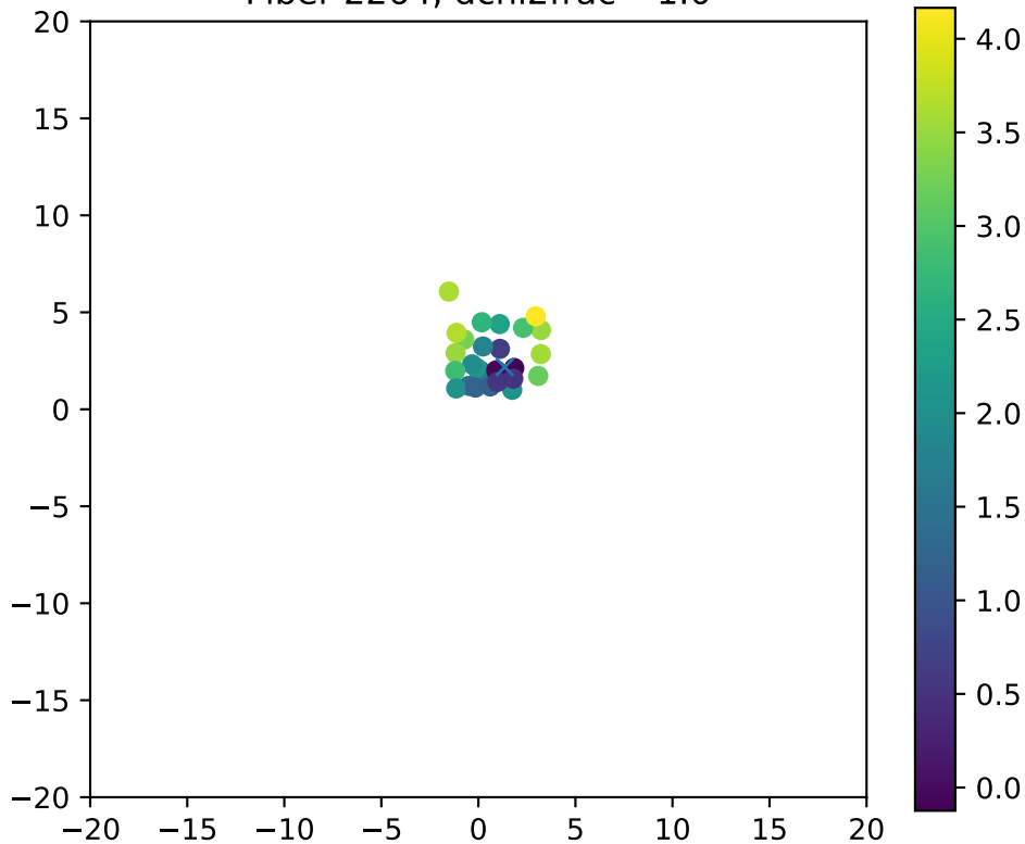
Fiber 2264, dchi2frac= 1.0
