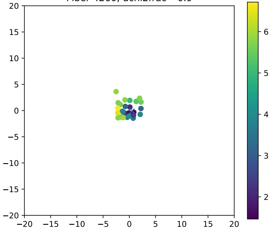
Fiber 4260, dchi2frac= 0.9
