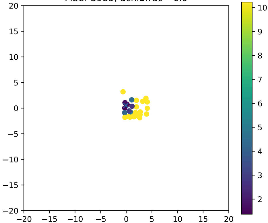
Fiber 3985, dchi2frac= 0.9
