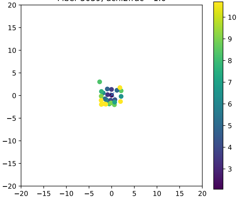
Fiber 3039, dchi2frac= 1.0
