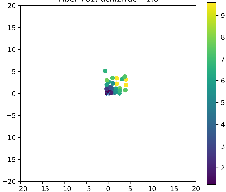
Fiber 781, dchi2frac= 1.0
