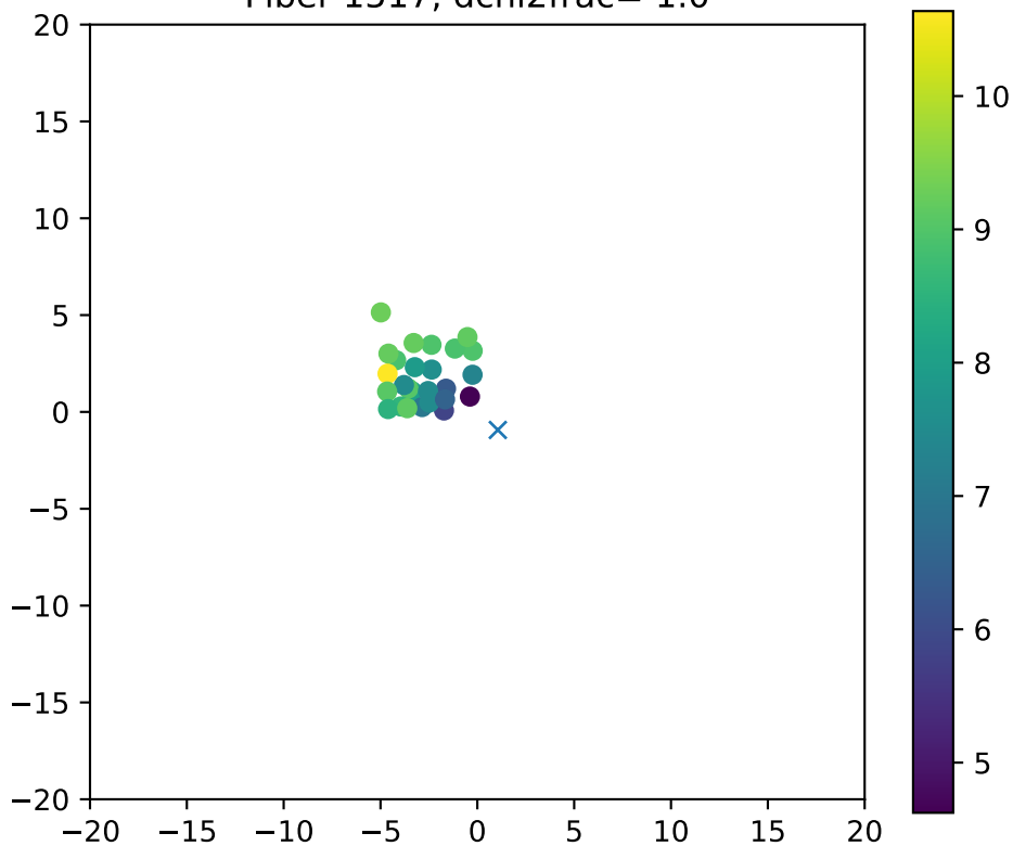
Fiber 1517, dchi2frac= 1.0
