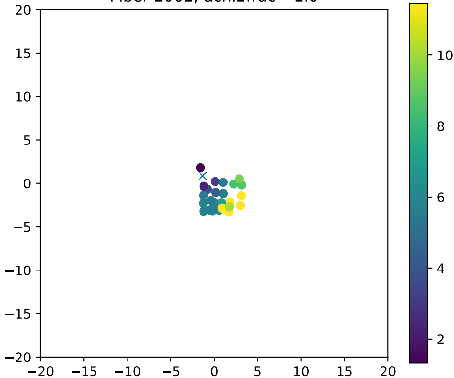
Fiber 2001, dchi2frac= 1.0
