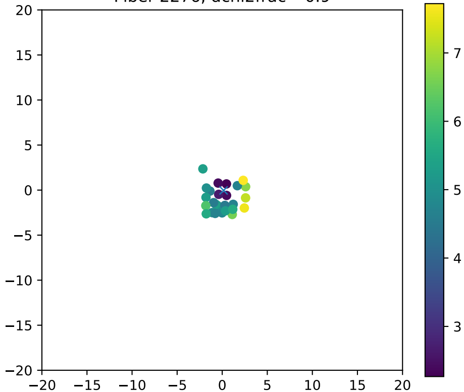
Fiber 2276, dchi2frac= 0.9
