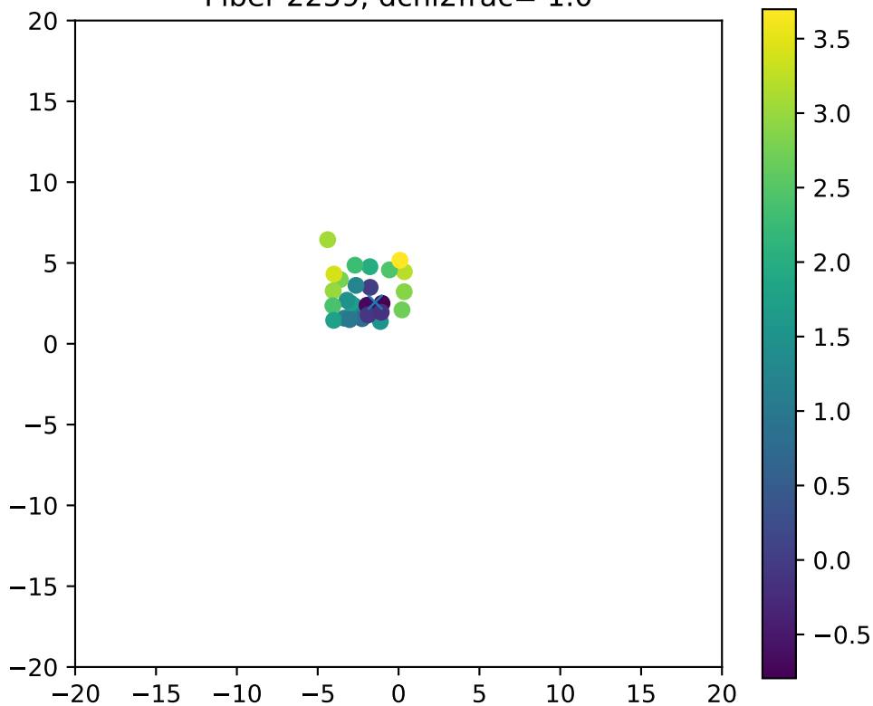
Fiber 2259, dchi2frac= 1.0
