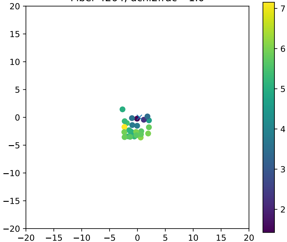
Fiber 4264, dchi2frac= 1.0
