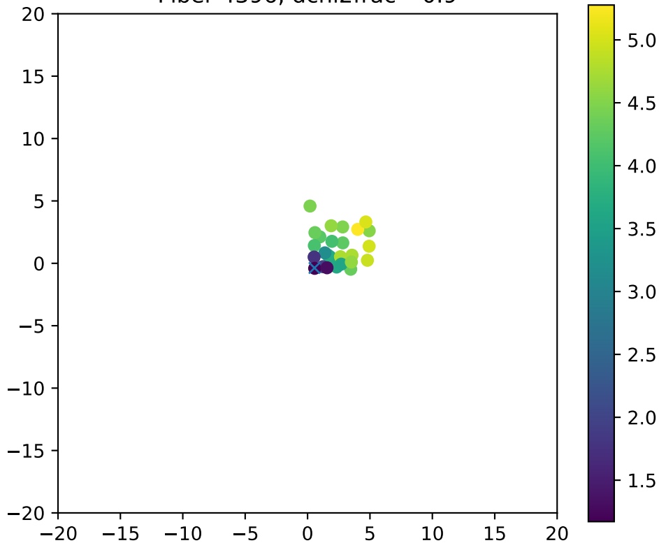
Fiber 4396, dchi2frac= 0.9
