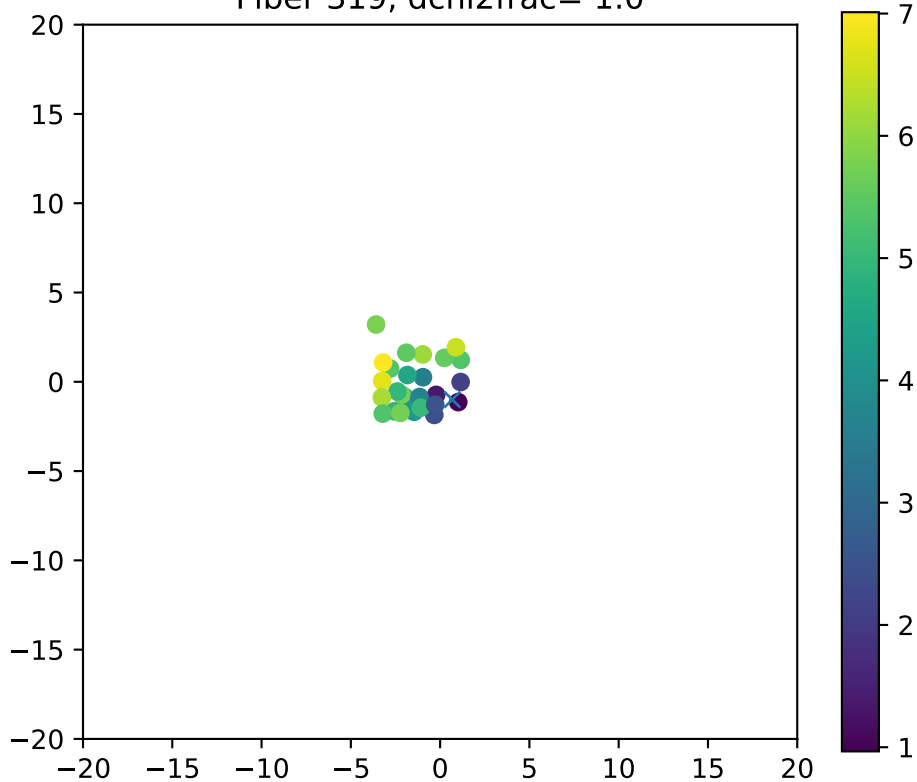
Fiber 319, dchi2frac= 1.0
