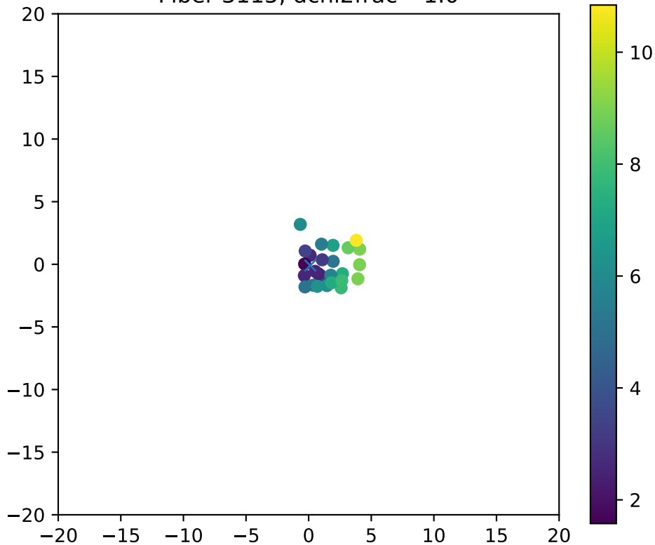
Fiber 3115, dchi2frac= 1.0
