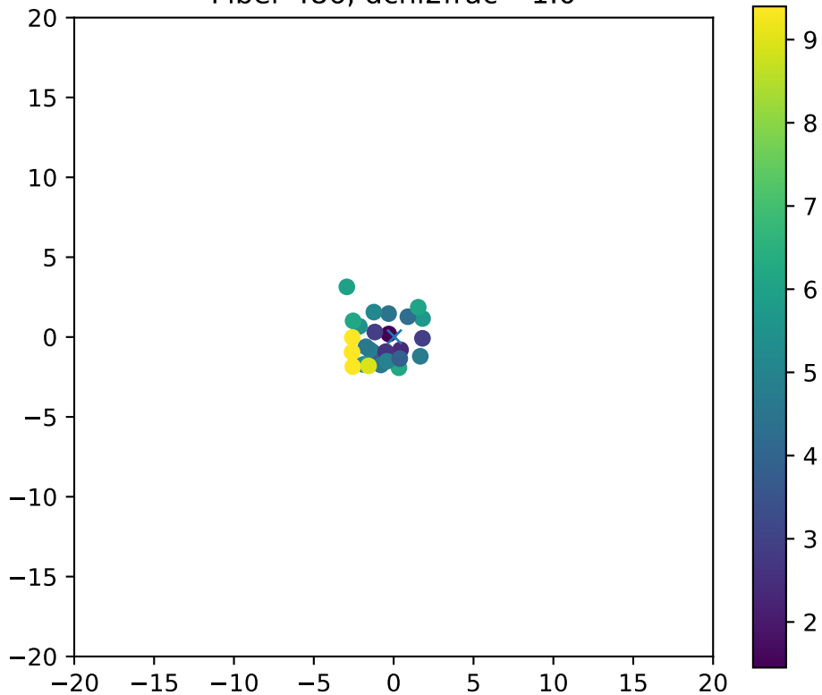
Fiber 486, dchi2frac= 1.0
