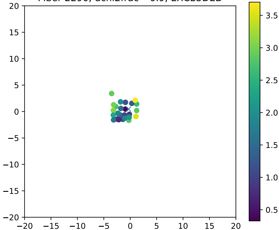
Fiber 2290, dchi2frac= 0.9, EXCLUDED
