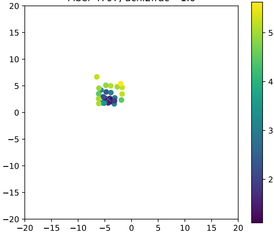
Fiber 4797, dchi2frac= 1.0
