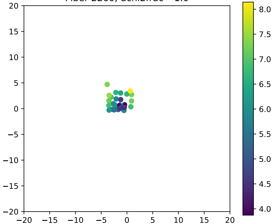
Fiber 2260, dchi2frac= 1.0
