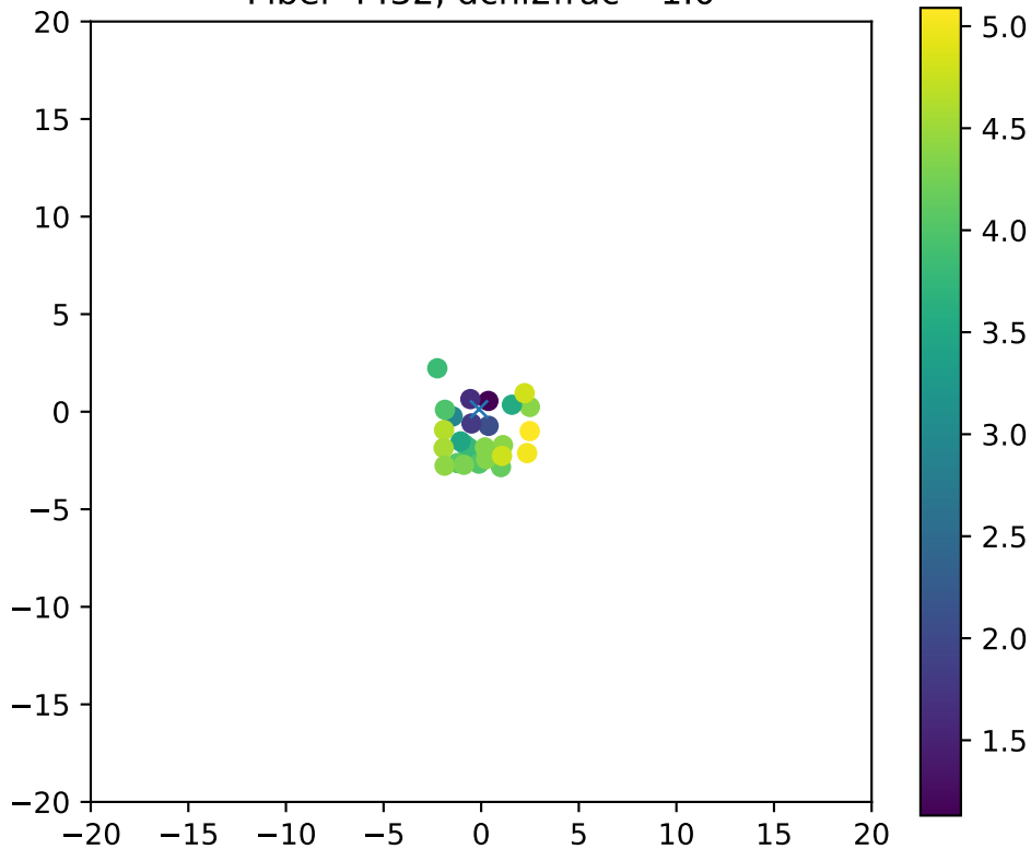
Fiber 4432, dchi2frac= 1.0
