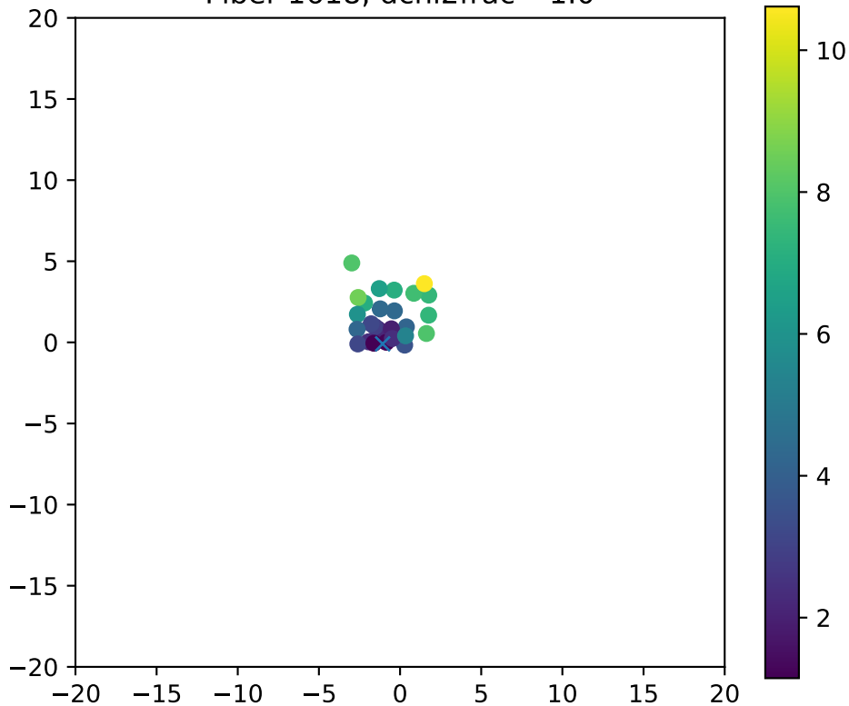
Fiber 1618, dchi2frac= 1.0
