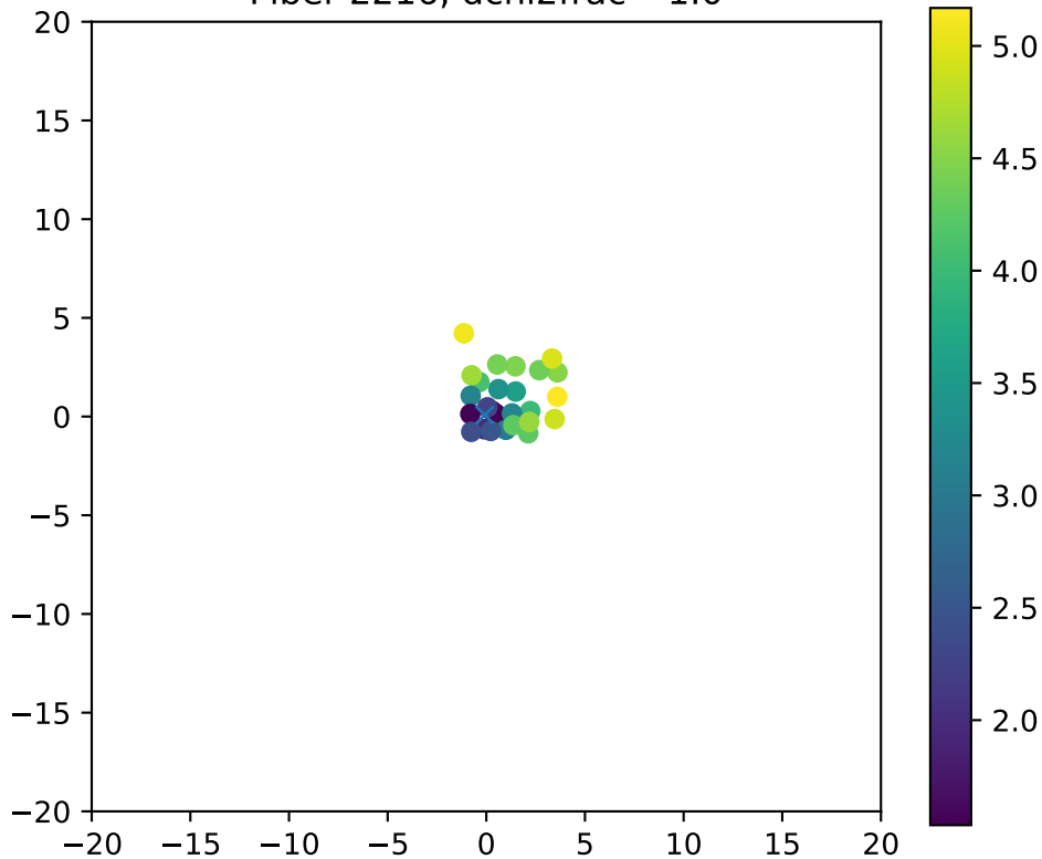
Fiber 2216, dchi2frac= 1.0
