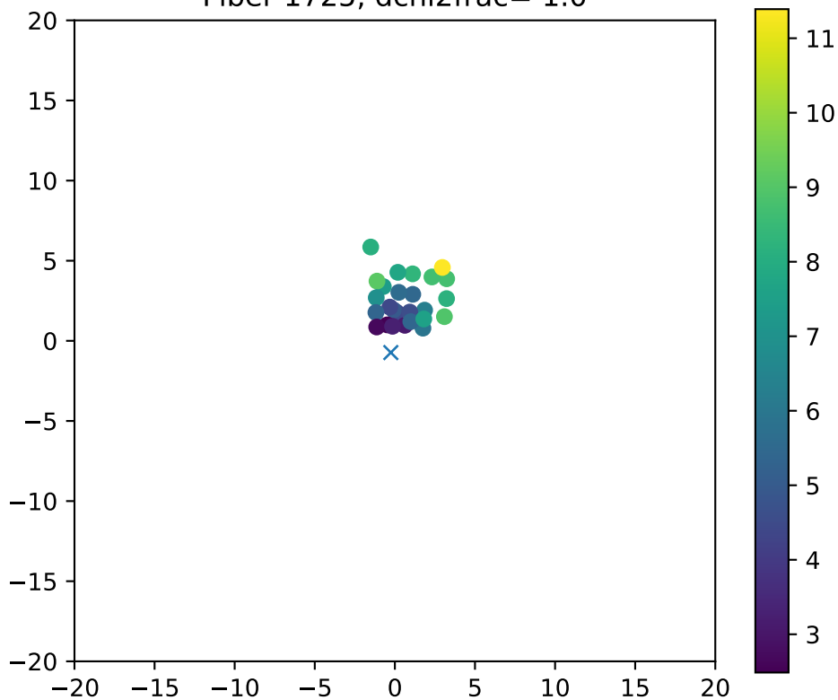
Fiber 1725, dchi2frac= 1.0
