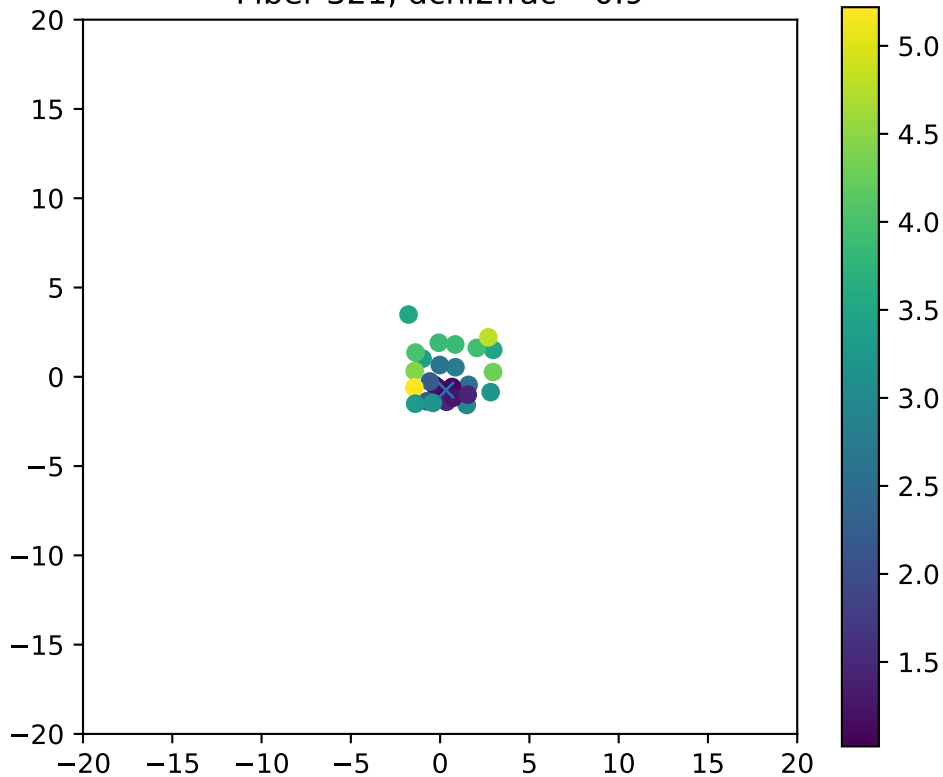
Fiber 321, dchi2frac= 0.9
