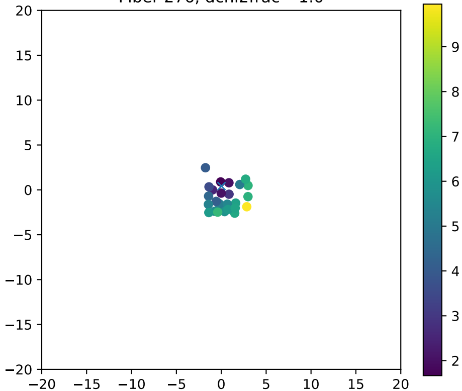
Fiber 276, dchi2frac= 1.0
