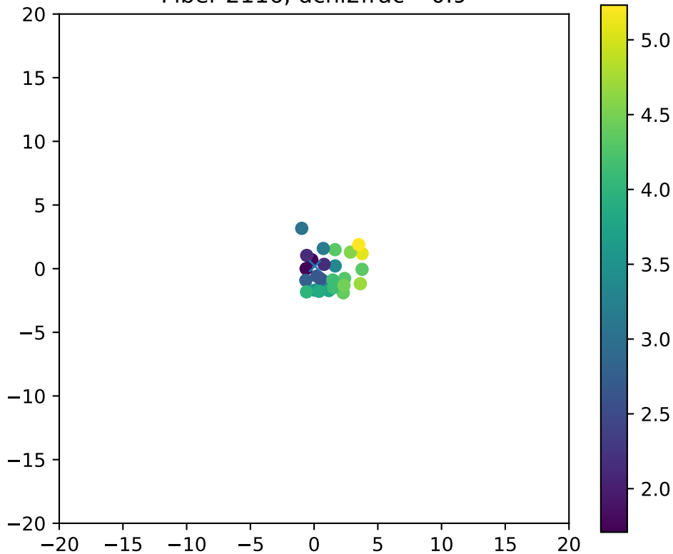
Fiber 2116, dchi2frac= 0.9
