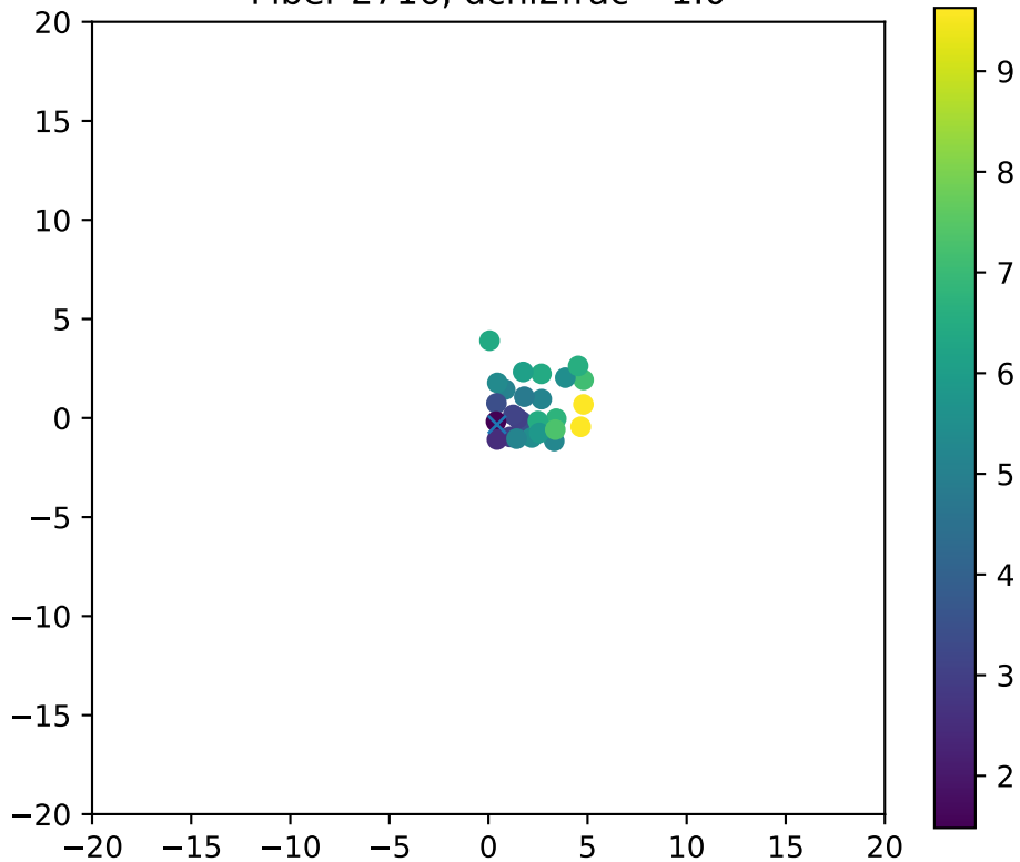
Fiber 2716, dchi2frac= 1.0
