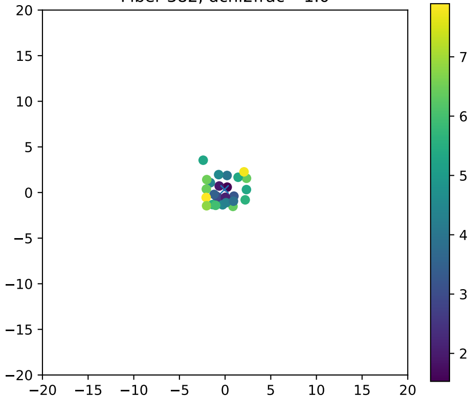
Fiber 382, dchi2frac= 1.0
