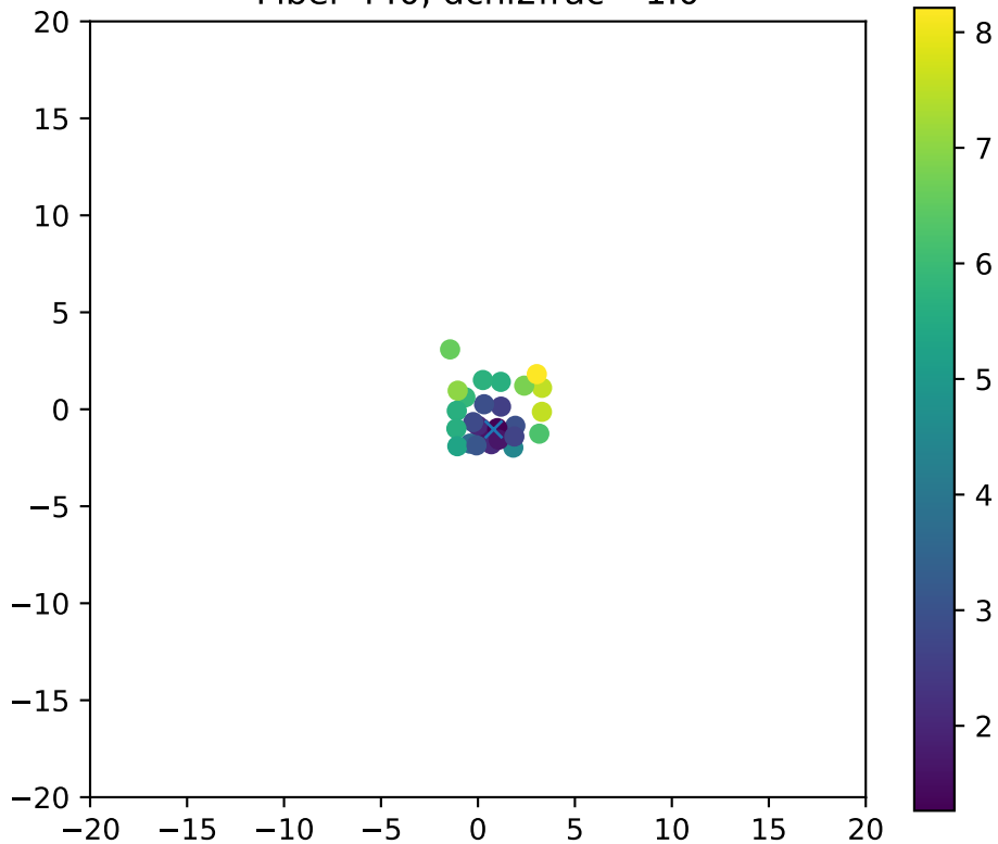
Fiber 440, dchi2frac= 1.0
