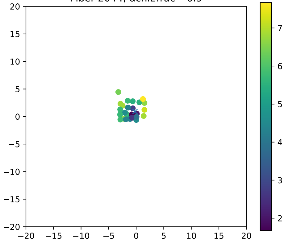
Fiber 2044, dchi2frac= 0.9
