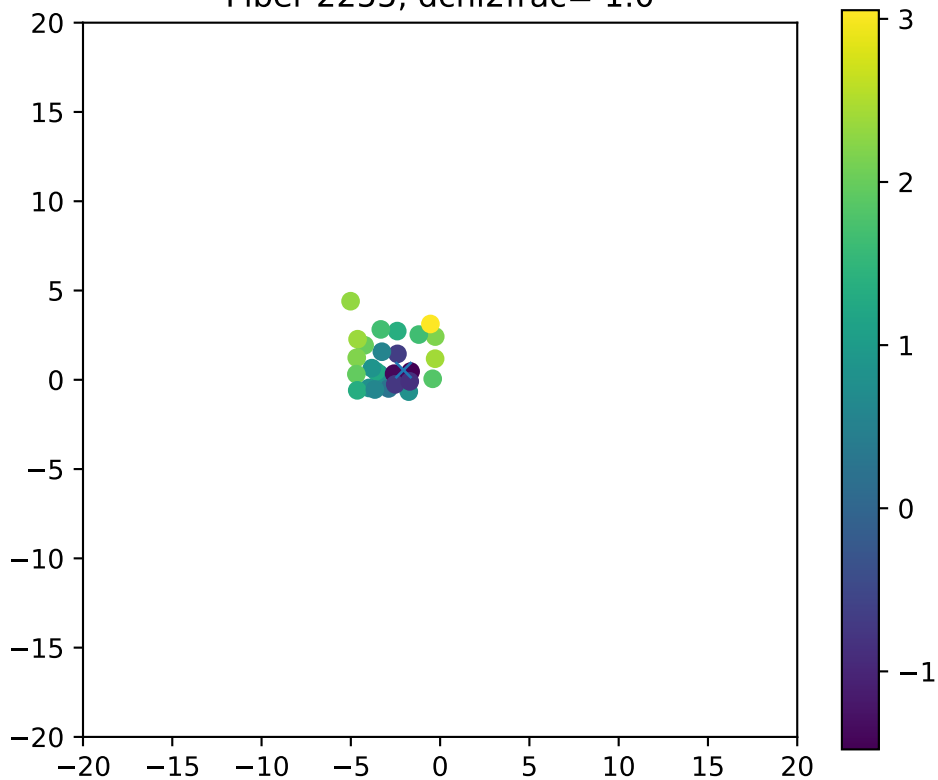
Fiber 2255, dchi2frac= 1.0
