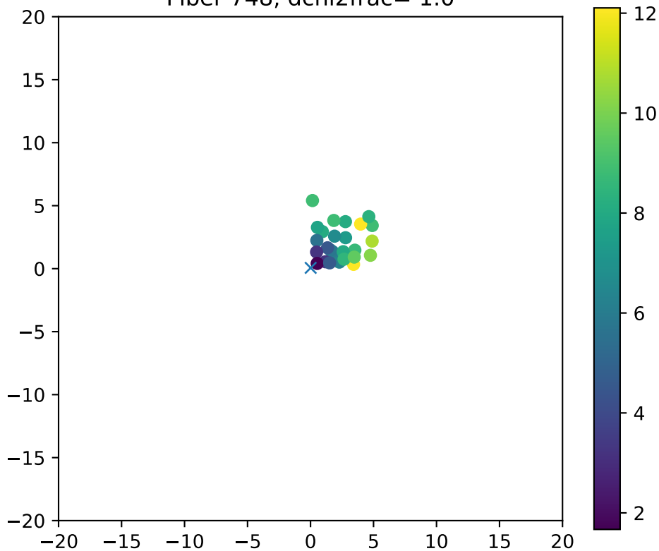
Fiber 748, dchi2frac= 1.0
