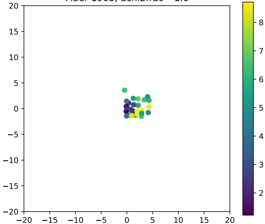
Fiber 1903, dchi2frac= 1.0
