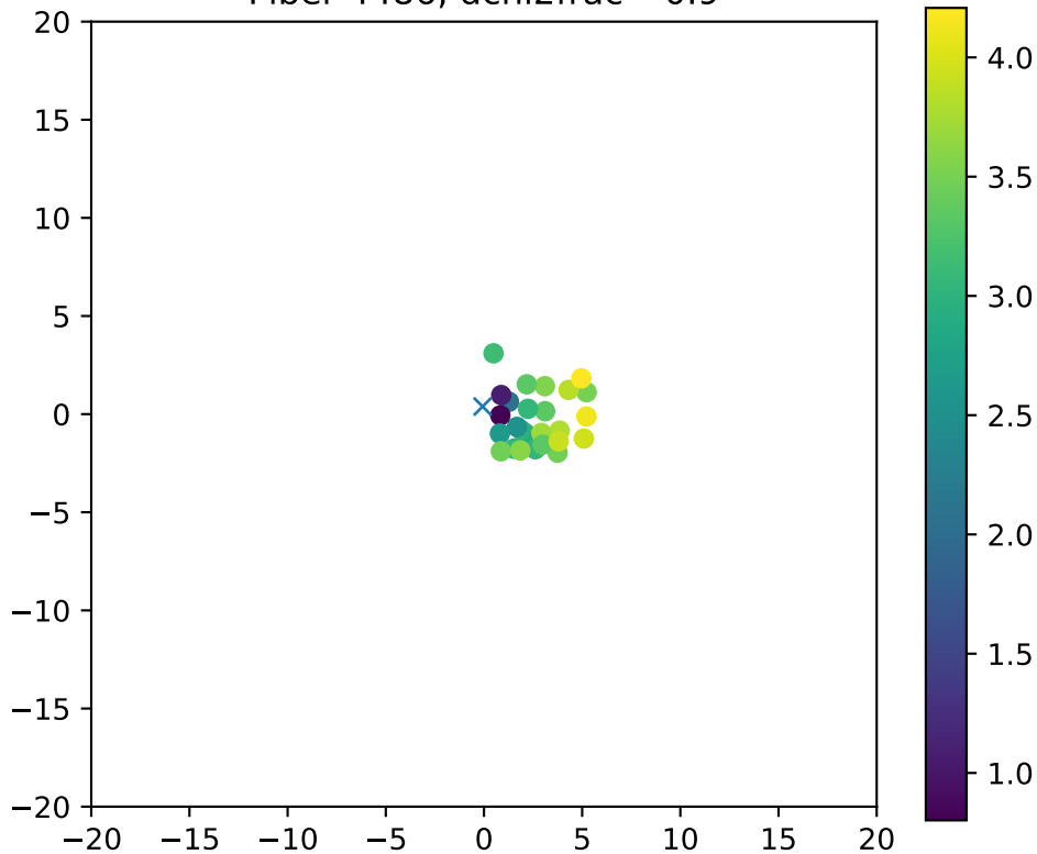
Fiber 4486, dchi2frac= 0.9
