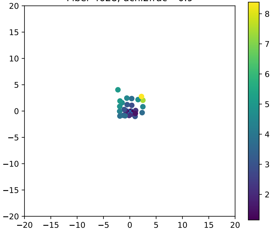
Fiber 4628, dchi2frac= 0.9
