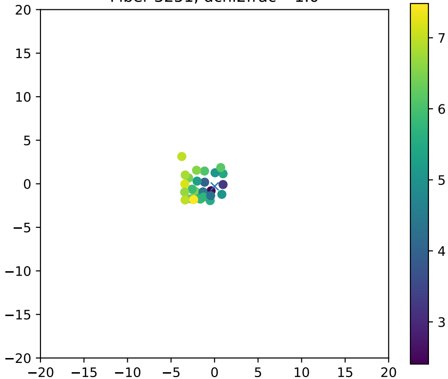
Fiber 3251, dchi2frac= 1.0
