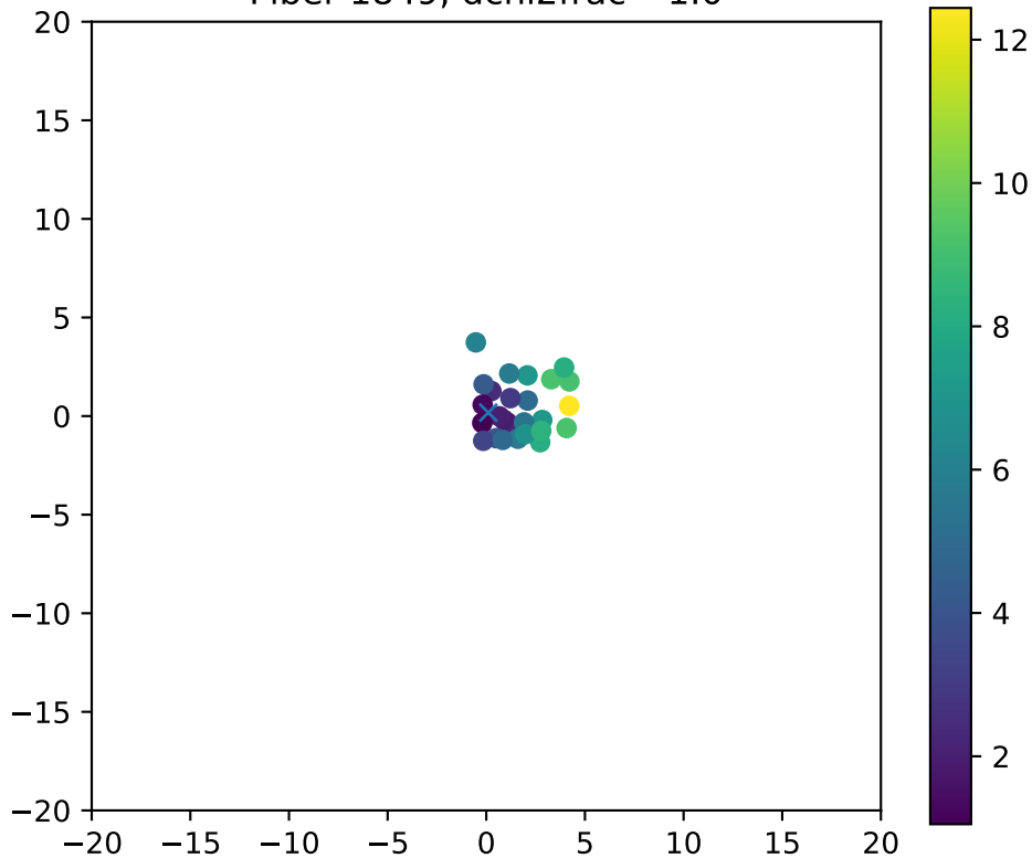
Fiber 1849, dchi2frac= 1.0
