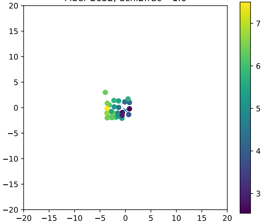
Fiber 2652, dchi2frac= 1.0
