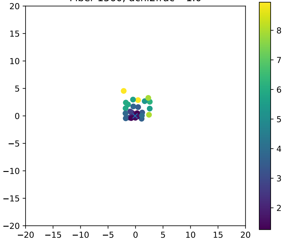
Fiber 1560, dchi2frac= 1.0
