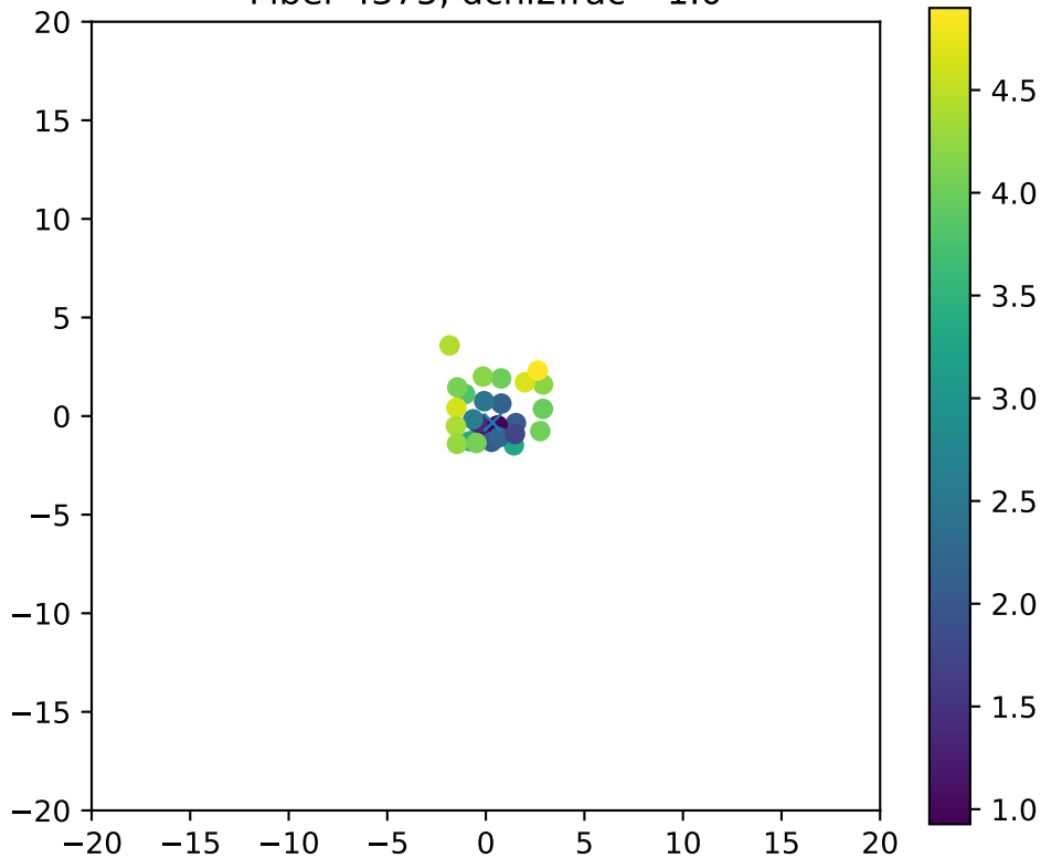
Fiber 4375, dchi2frac= 1.0
