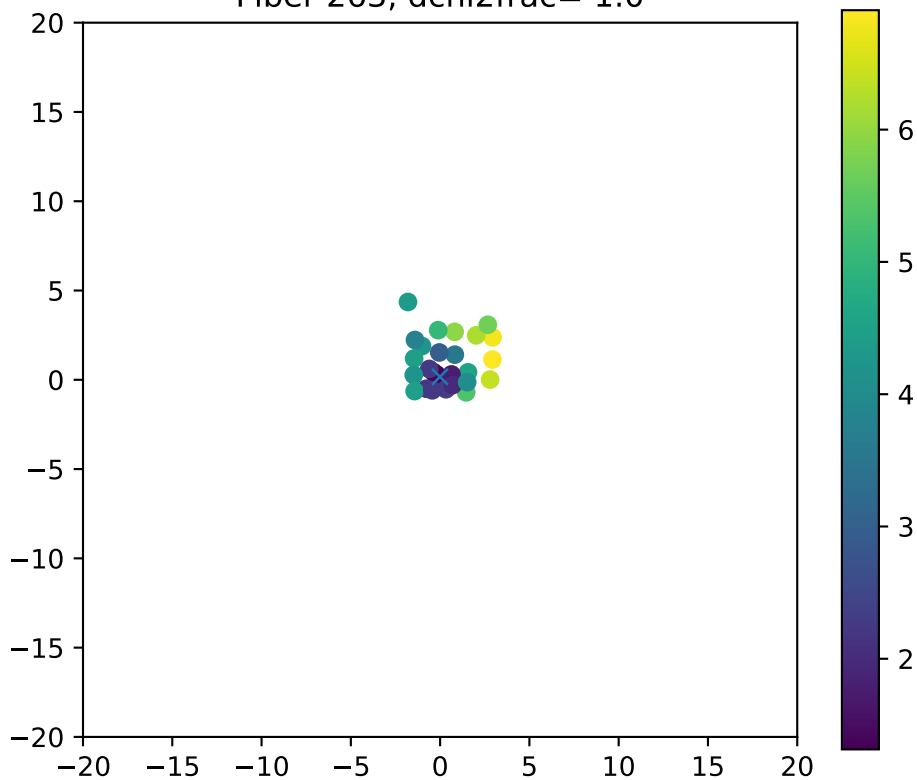
Fiber 263, dchi2frac= 1.0
