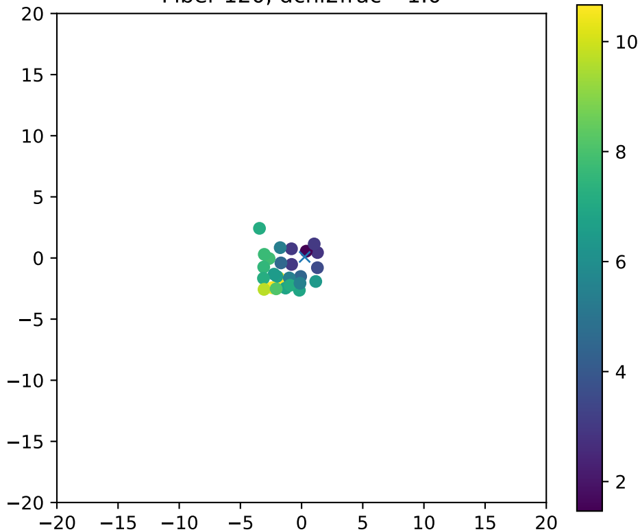
Fiber 120, dchi2frac= 1.0
