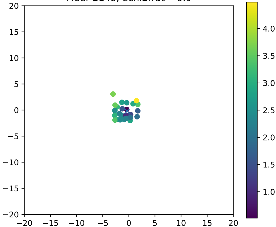
Fiber 2148, dchi2frac= 0.9
