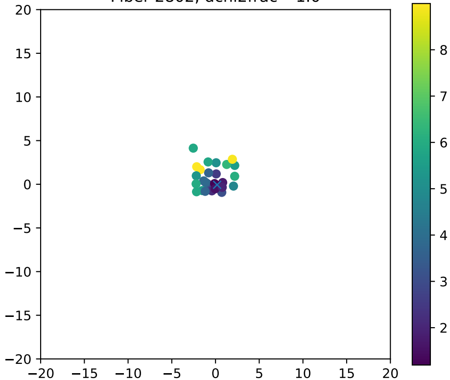
Fiber 2802, dchi2frac= 1.0
