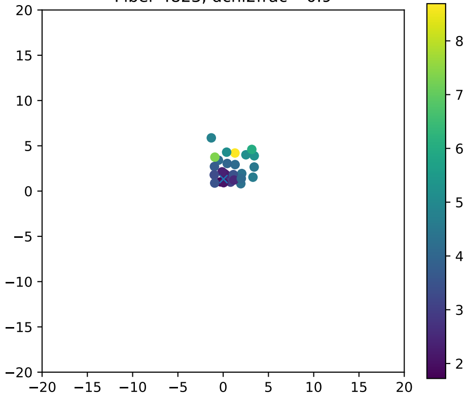
Fiber 4823, dchi2frac= 0.9
