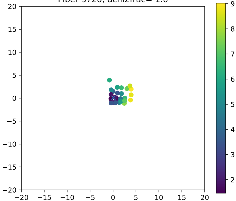
Fiber 3720, dchi2frac= 1.0
