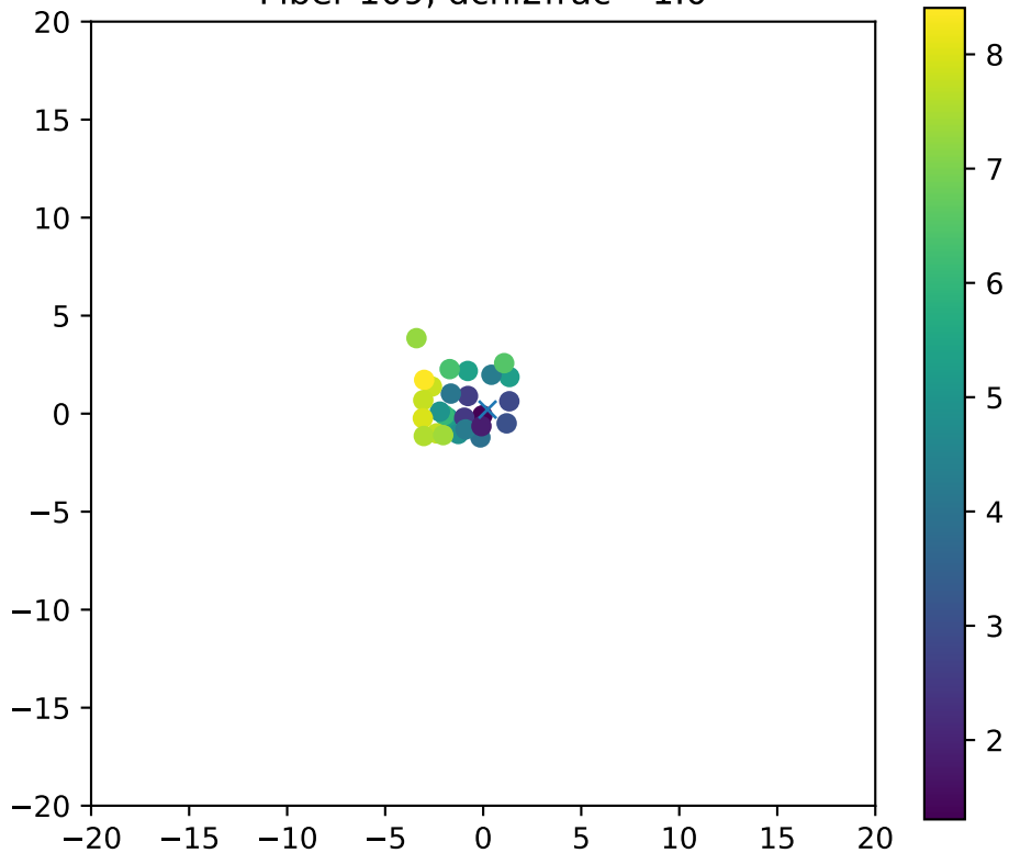
Fiber 109, dchi2frac= 1.0
