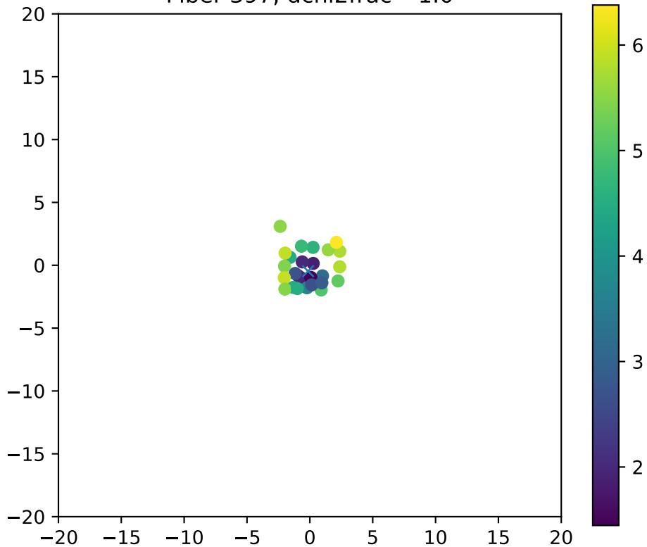
Fiber 397, dchi2frac= 1.0
