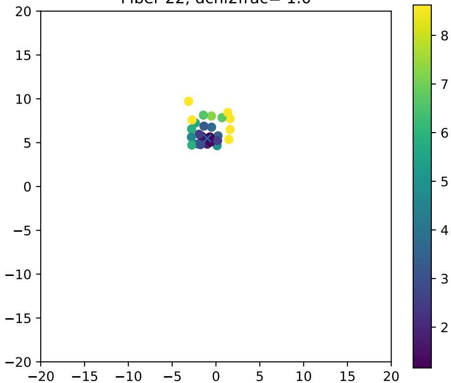
Fiber 22, dchi2frac= 1.0
