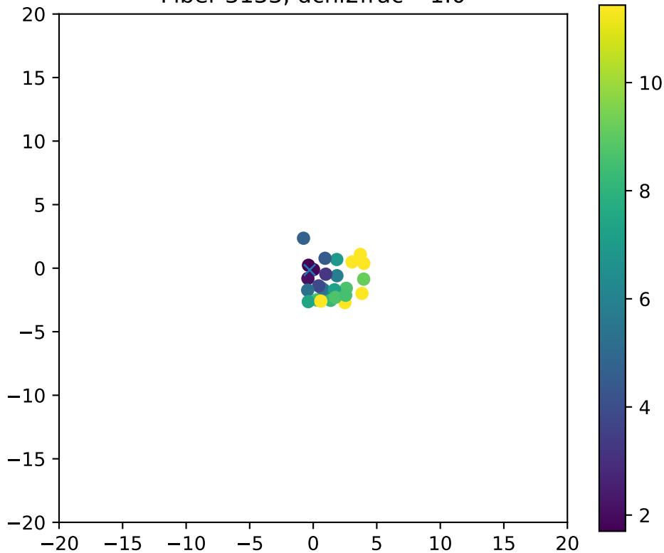
Fiber 3133, dchi2frac= 1.0
