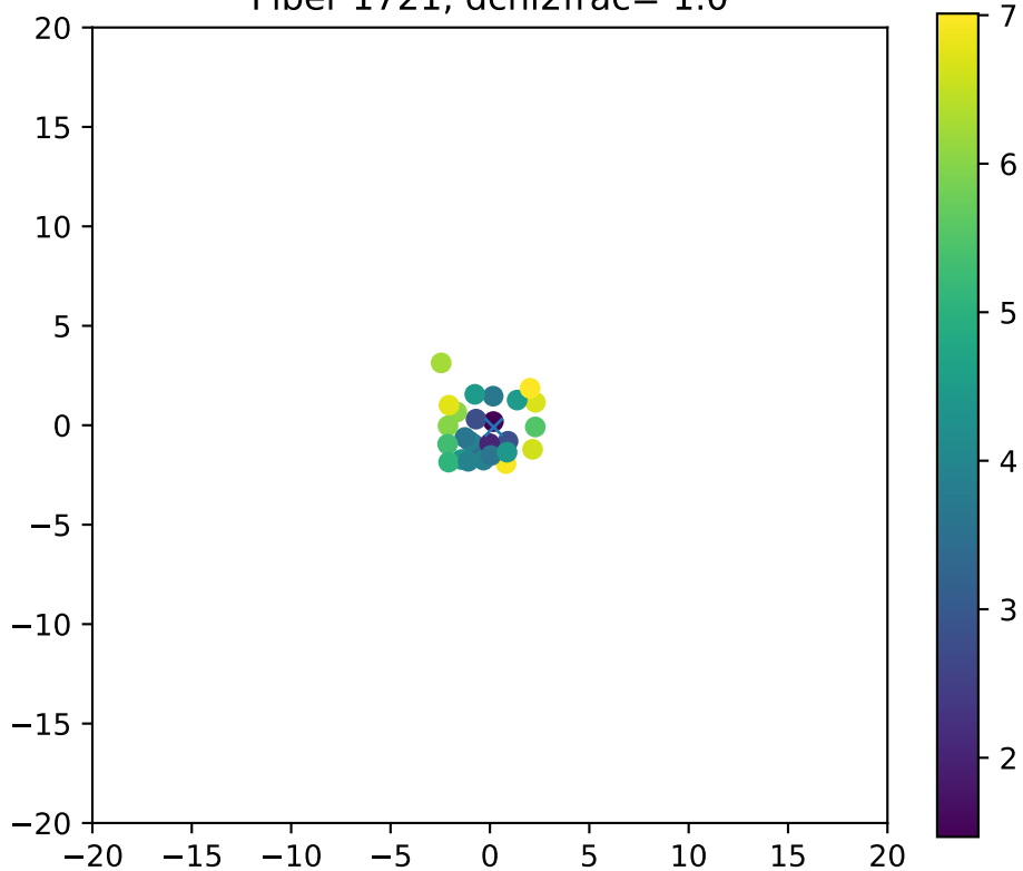
Fiber 1721, dchi2frac= 1.0
