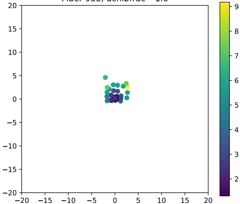
Fiber 933, dchi2frac= 1.0
