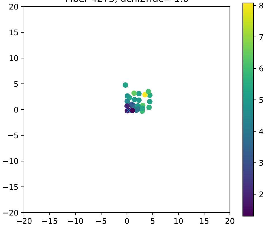
Fiber 4275, dchi2frac= 1.0
