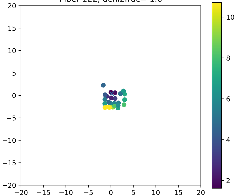
Fiber 122, dchi2frac= 1.0
