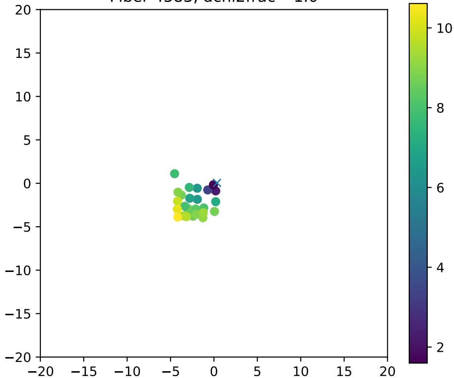
Fiber 4583, dchi2frac= 1.0
