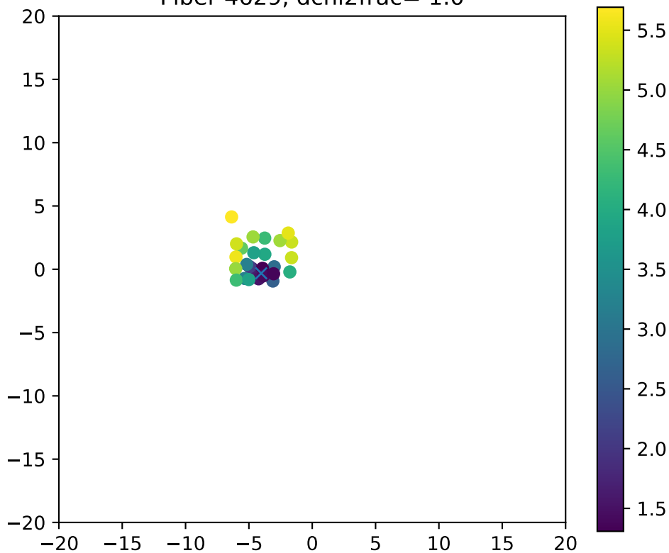
Fiber 4629, dchi2frac= 1.0
