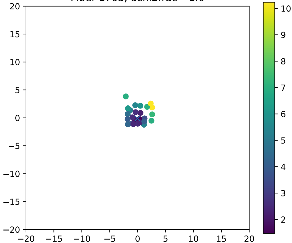
Fiber 1703, dchi2frac= 1.0
