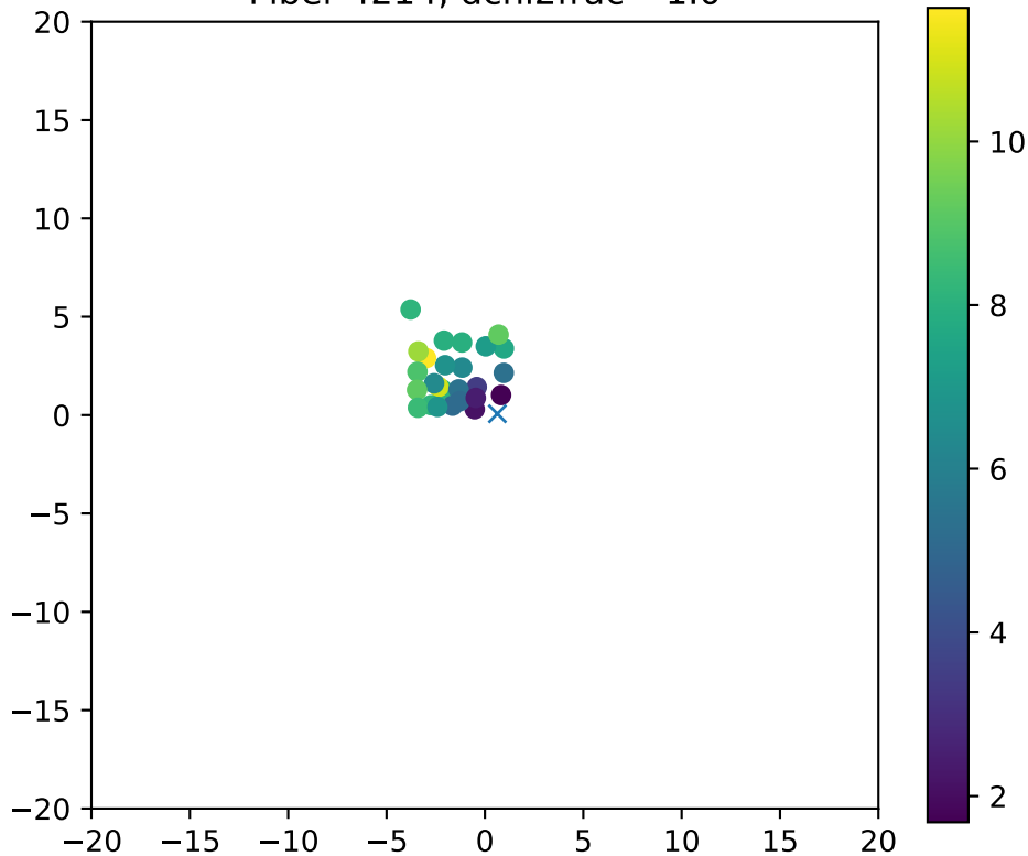
Fiber 4214, dchi2frac= 1.0
