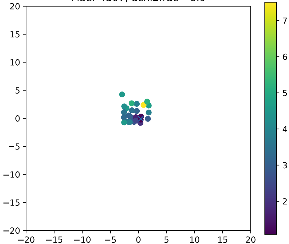
Fiber 4307, dchi2frac= 0.9
