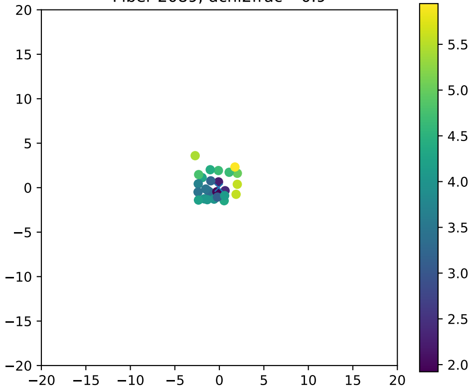
Fiber 2089, dchi2frac= 0.9
