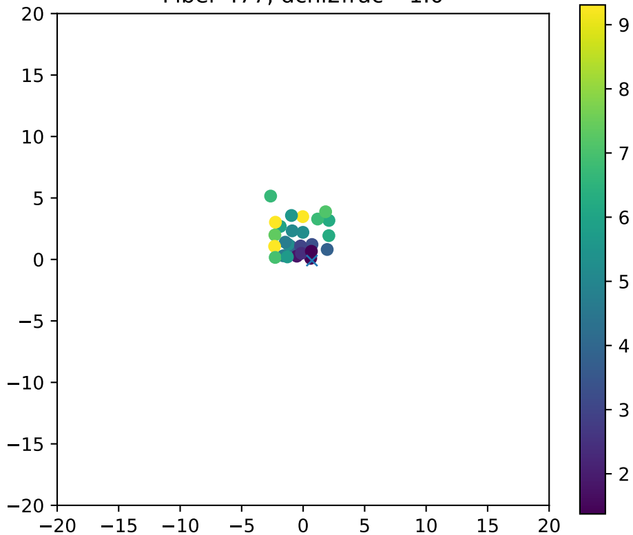
Fiber 477, dchi2frac= 1.0
