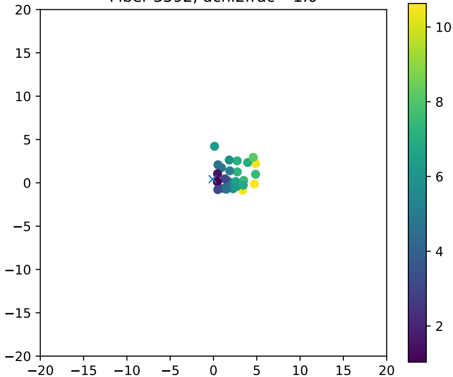
Fiber 3592, dchi2frac= 1.0
