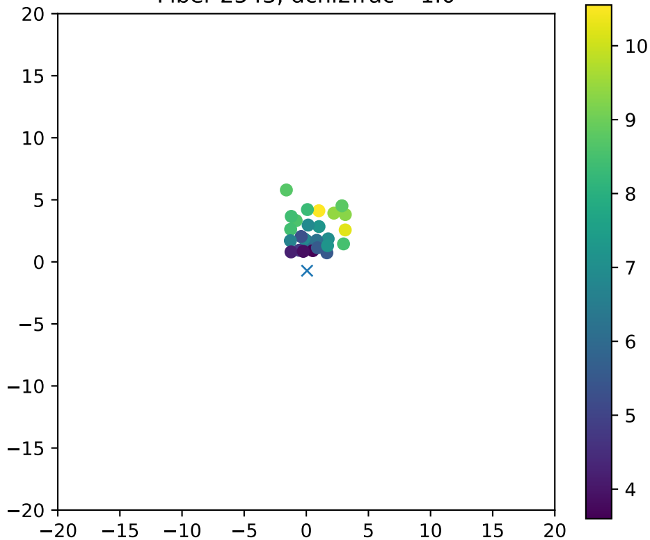
Fiber 2543, dchi2frac= 1.0
