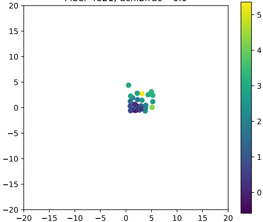
Fiber 4821, dchi2frac= 0.9
