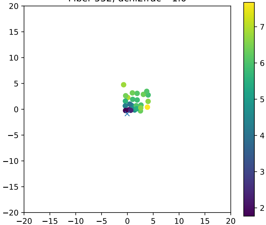
Fiber 532, dchi2frac= 1.0
