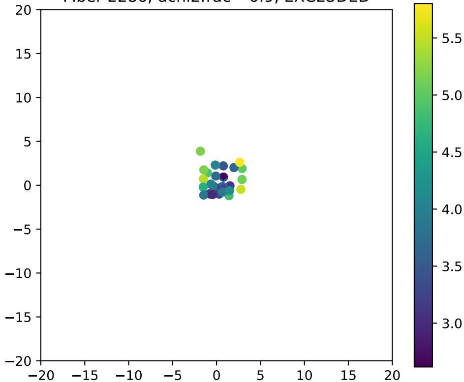
Fiber 2286, dchi2frac= 0.9, EXCLUDED
