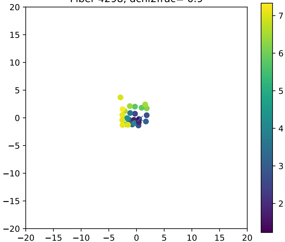
Fiber 4298, dchi2frac= 0.9
