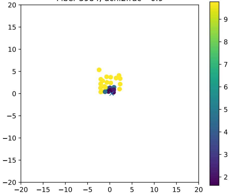
Fiber 3984, dchi2frac= 0.9
