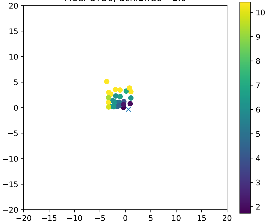
Fiber 3736, dchi2frac= 1.0
