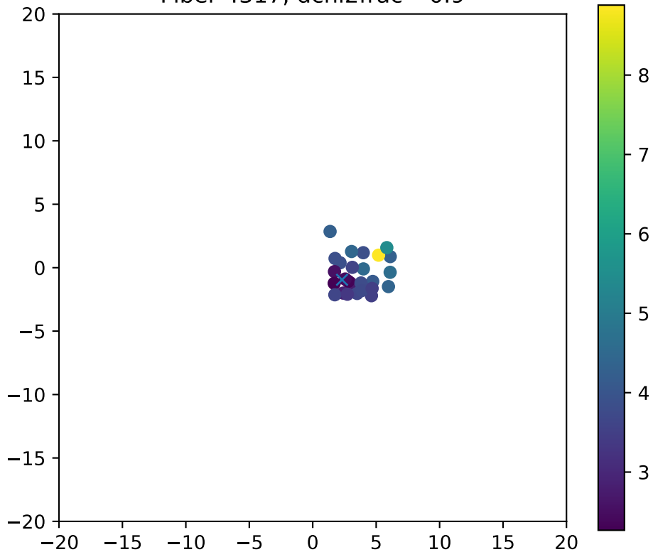
Fiber 4317, dchi2frac= 0.9
