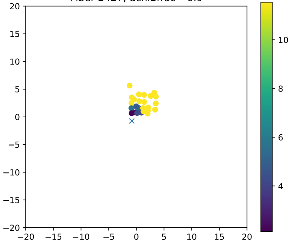
Fiber 2427, dchi2frac= 0.9
