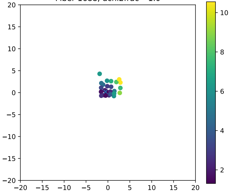
Fiber 1688, dchi2frac= 1.0
