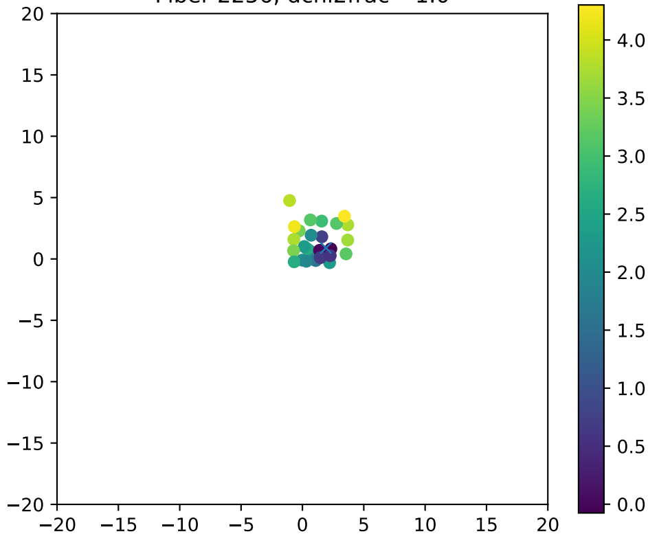
Fiber 2256, dchi2frac= 1.0
