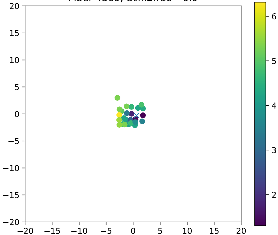
Fiber 4369, dchi2frac= 0.9
