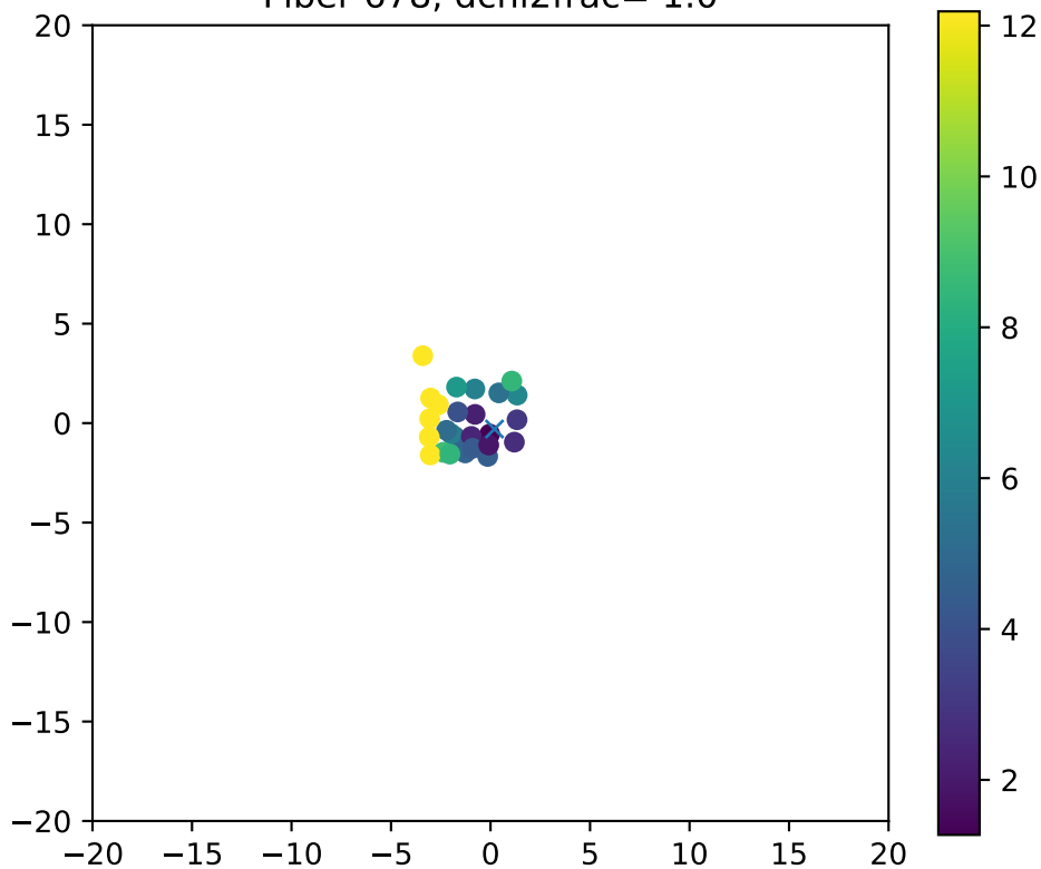
Fiber 678, dchi2frac= 1.0
