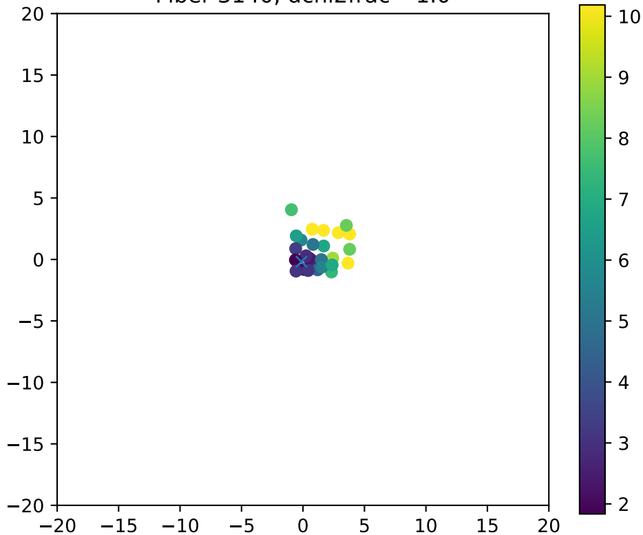
Fiber 3140, dchi2frac= 1.0
