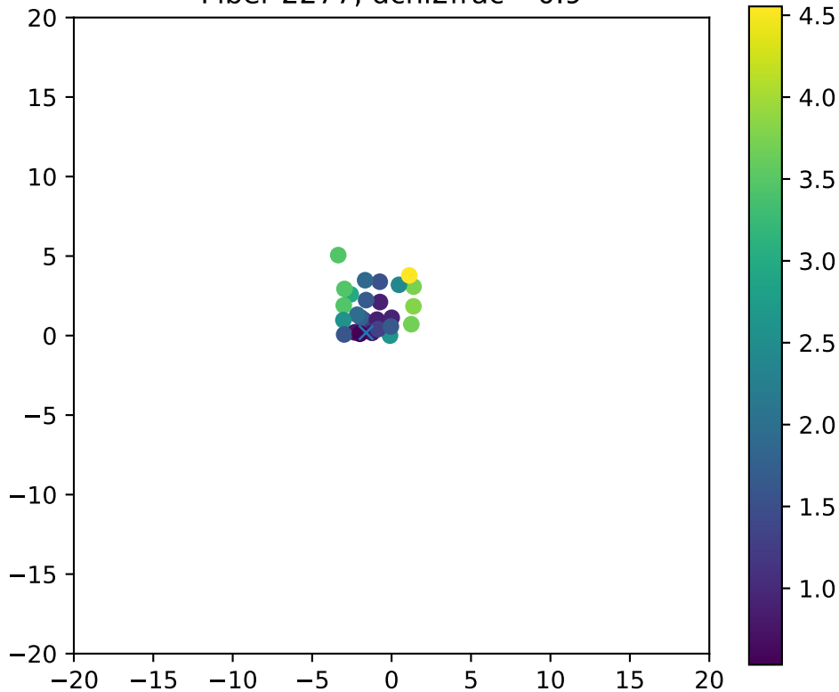
Fiber 2277, dchi2frac= 0.9
