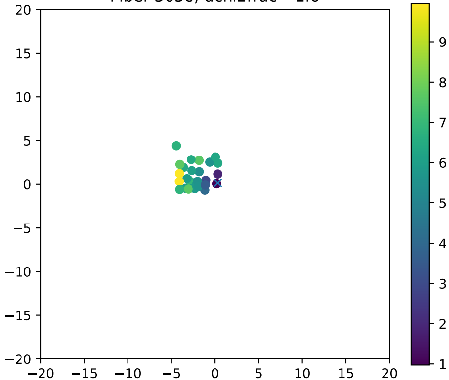
Fiber 3658, dchi2frac= 1.0
