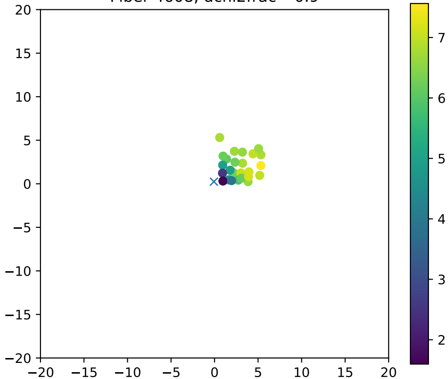
Fiber 4608, dchi2frac= 0.9
