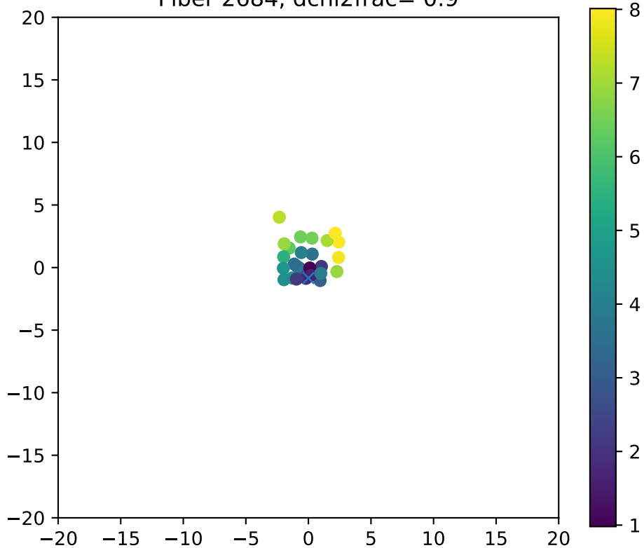
Fiber 2684, dchi2frac= 0.9
