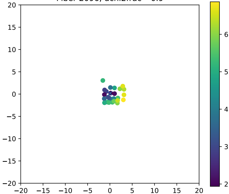
Fiber 2096, dchi2frac= 0.9
