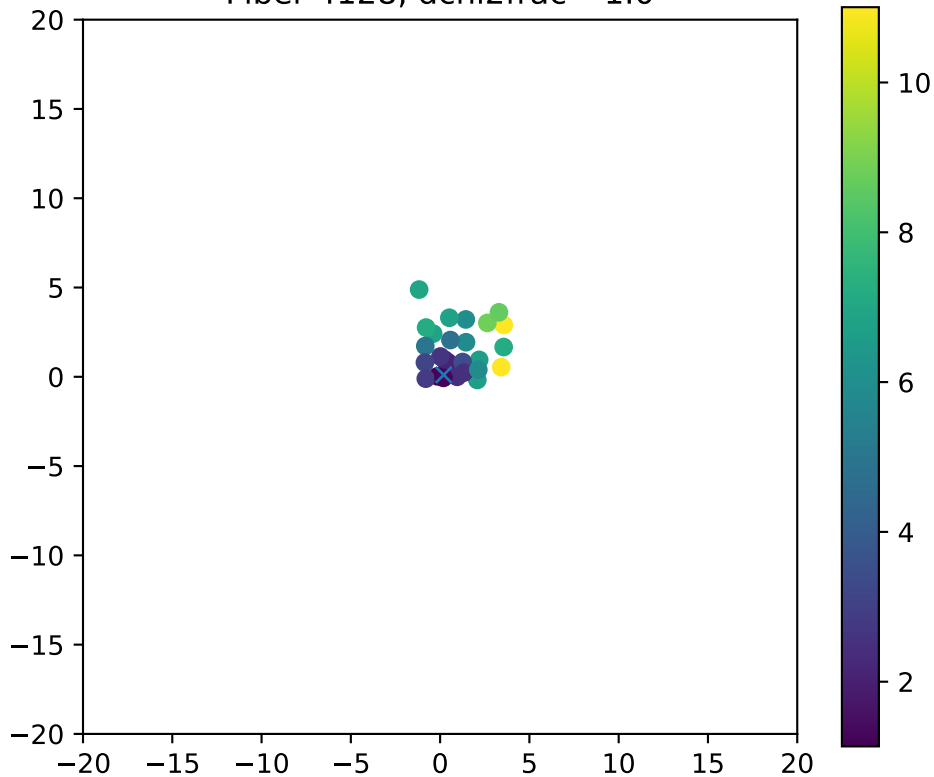
Fiber 4128, dchi2frac= 1.0
