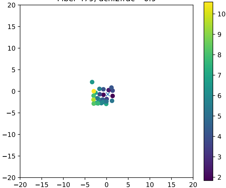
Fiber 479, dchi2frac= 0.9
