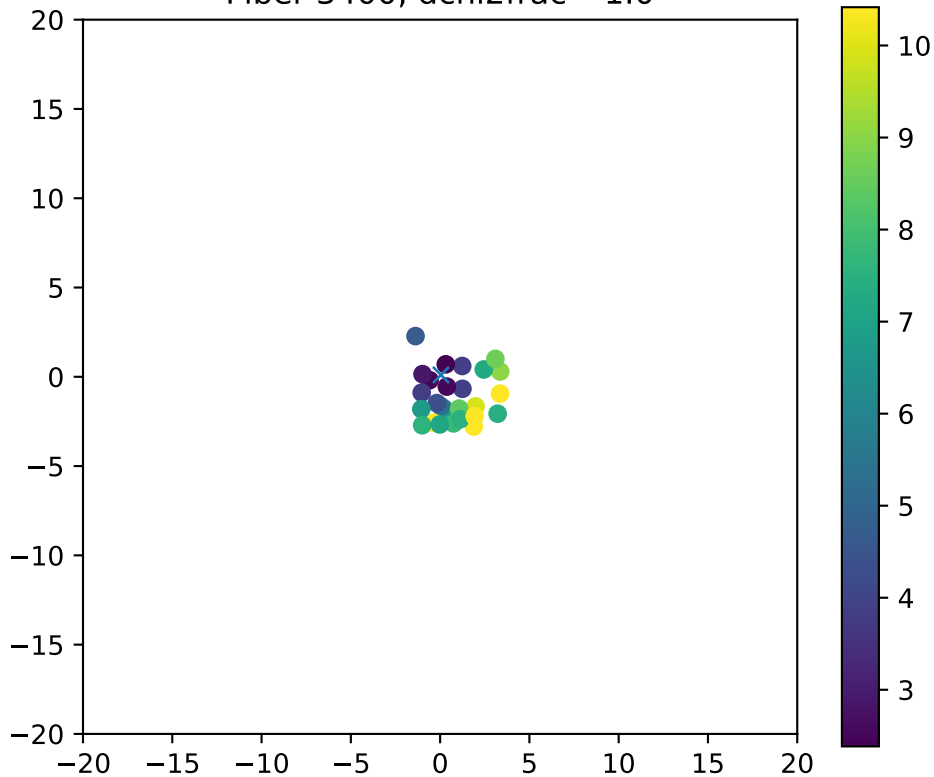
Fiber 3400, dchi2frac= 1.0
