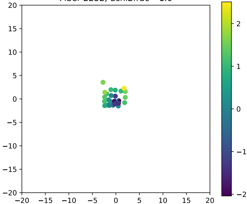
Fiber 2252, dchi2frac= 1.0
