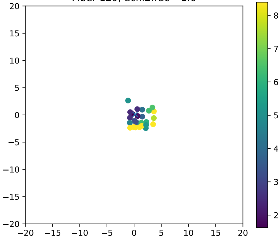
Fiber 129, dchi2frac= 1.0
