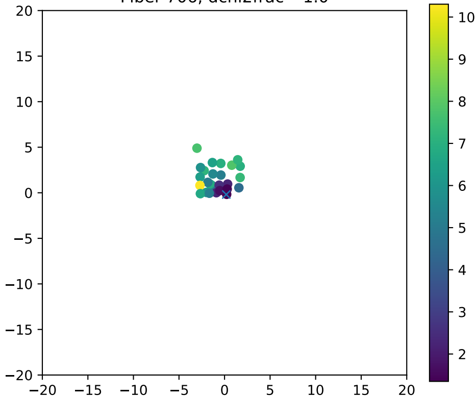
Fiber 706, dchi2frac= 1.0
