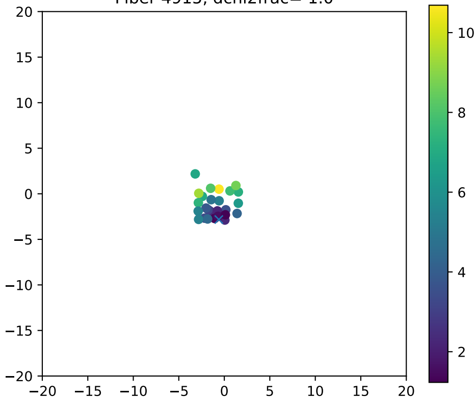
Fiber 4915, dchi2frac= 1.0
