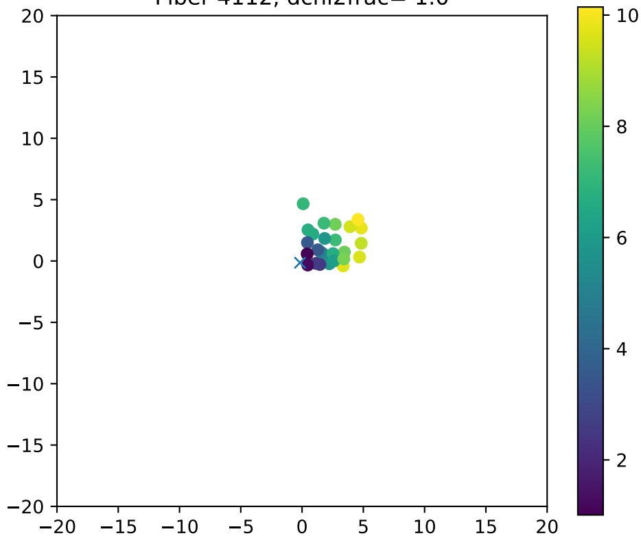
Fiber 4112, dchi2frac= 1.0
