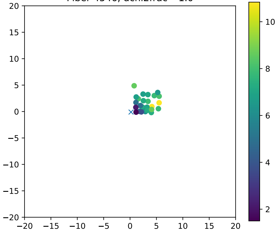
Fiber 4546, dchi2frac= 1.0
