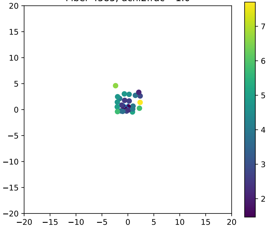
Fiber 4585, dchi2frac= 1.0
