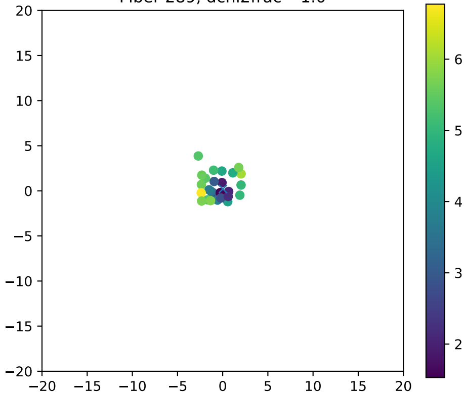
Fiber 289, dchi2frac= 1.0
