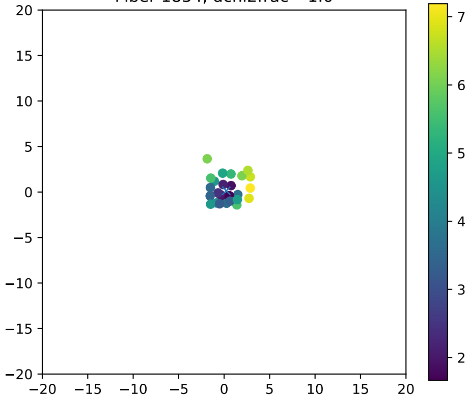
Fiber 1834, dchi2frac= 1.0
