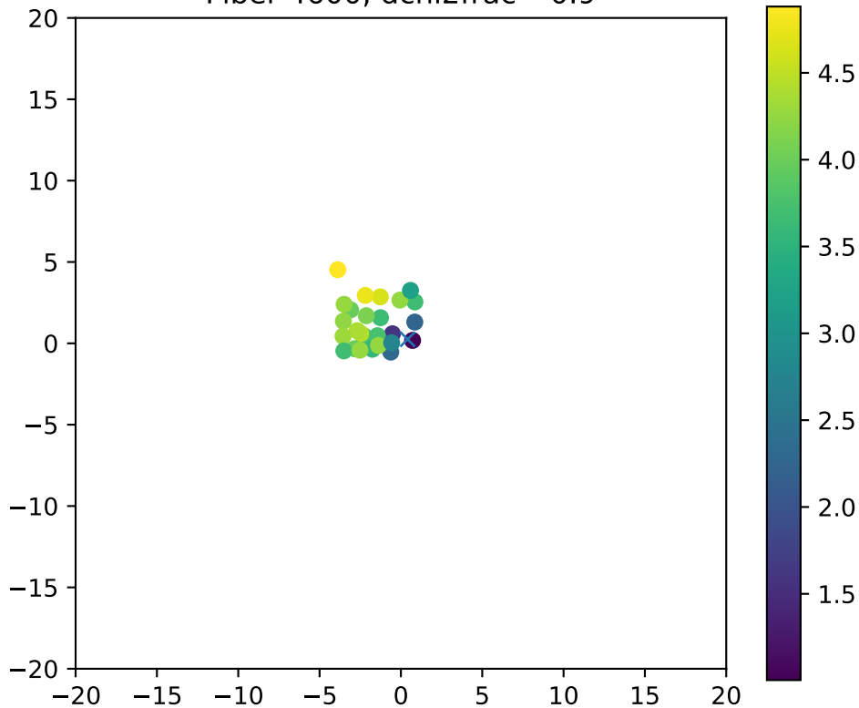
Fiber 4600, dchi2frac= 0.9
