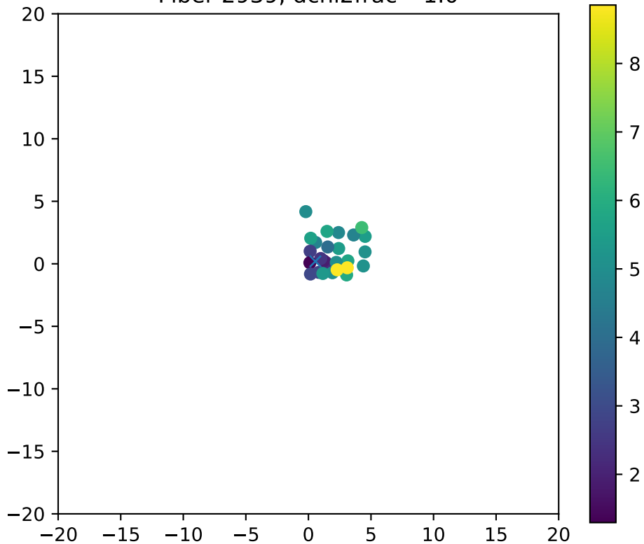
Fiber 2939, dchi2frac= 1.0
