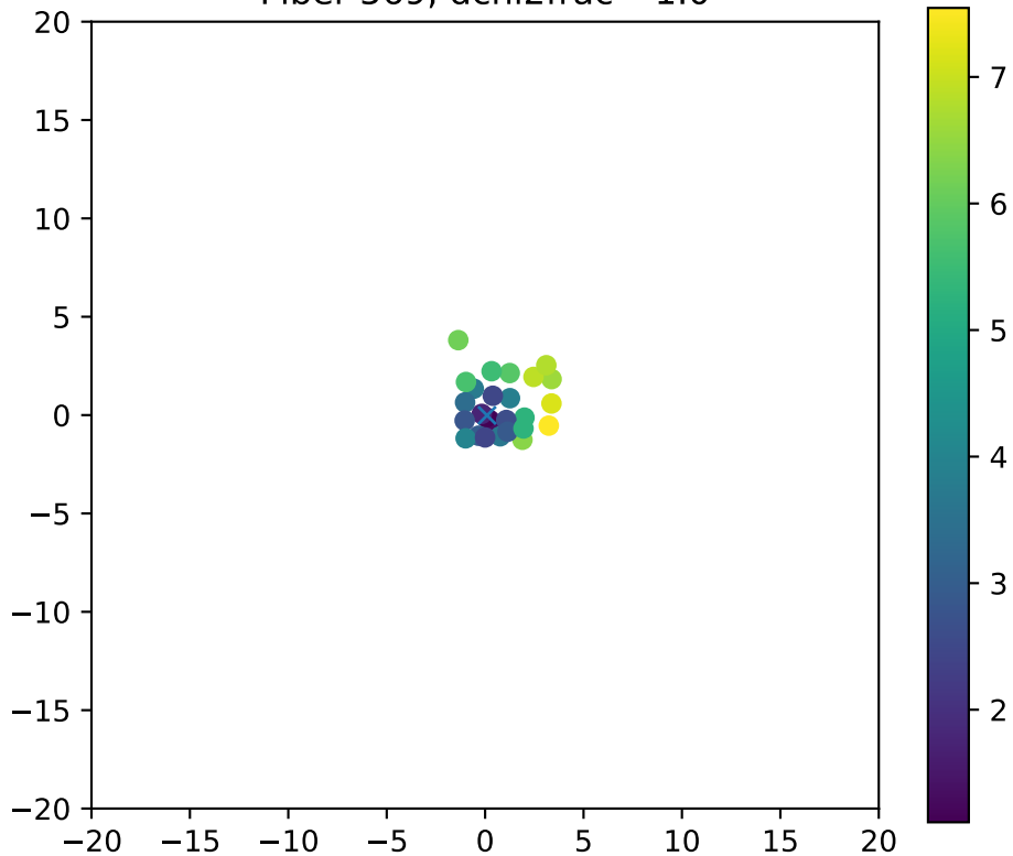
Fiber 569, dchi2frac= 1.0
