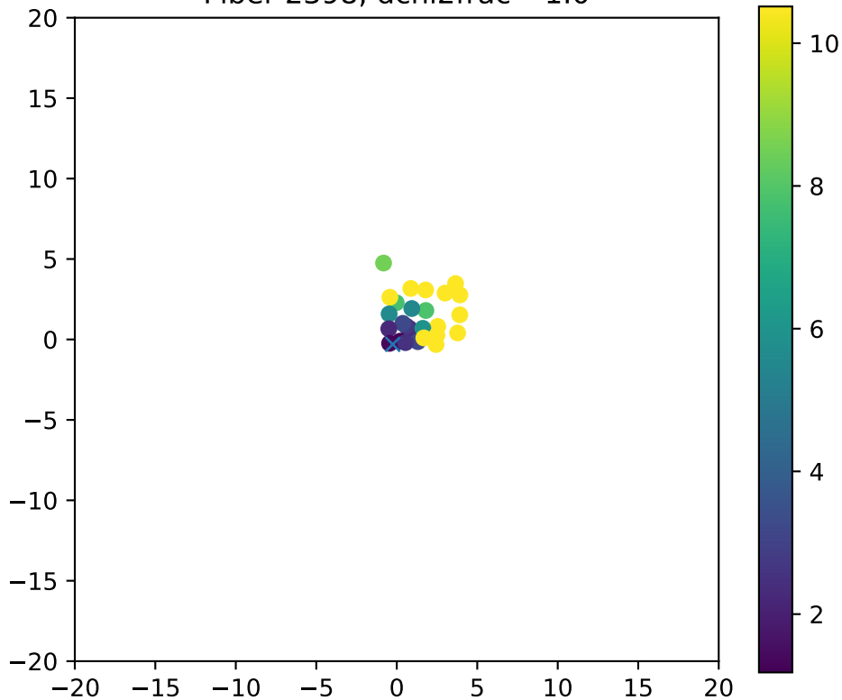
Fiber 2398, dchi2frac= 1.0
