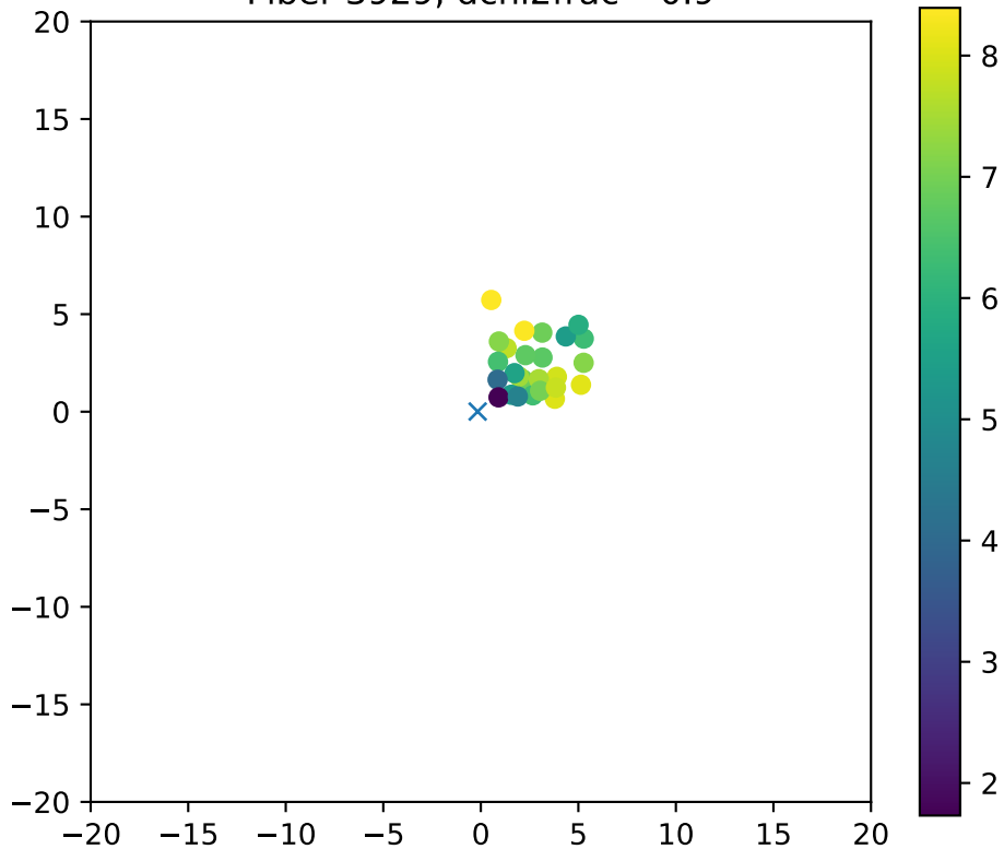
Fiber 3929, dchi2frac= 0.9
