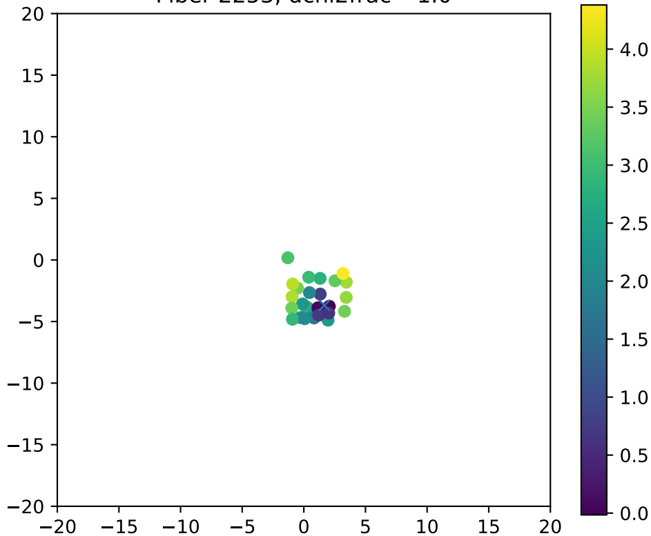
Fiber 2253, dchi2frac= 1.0
