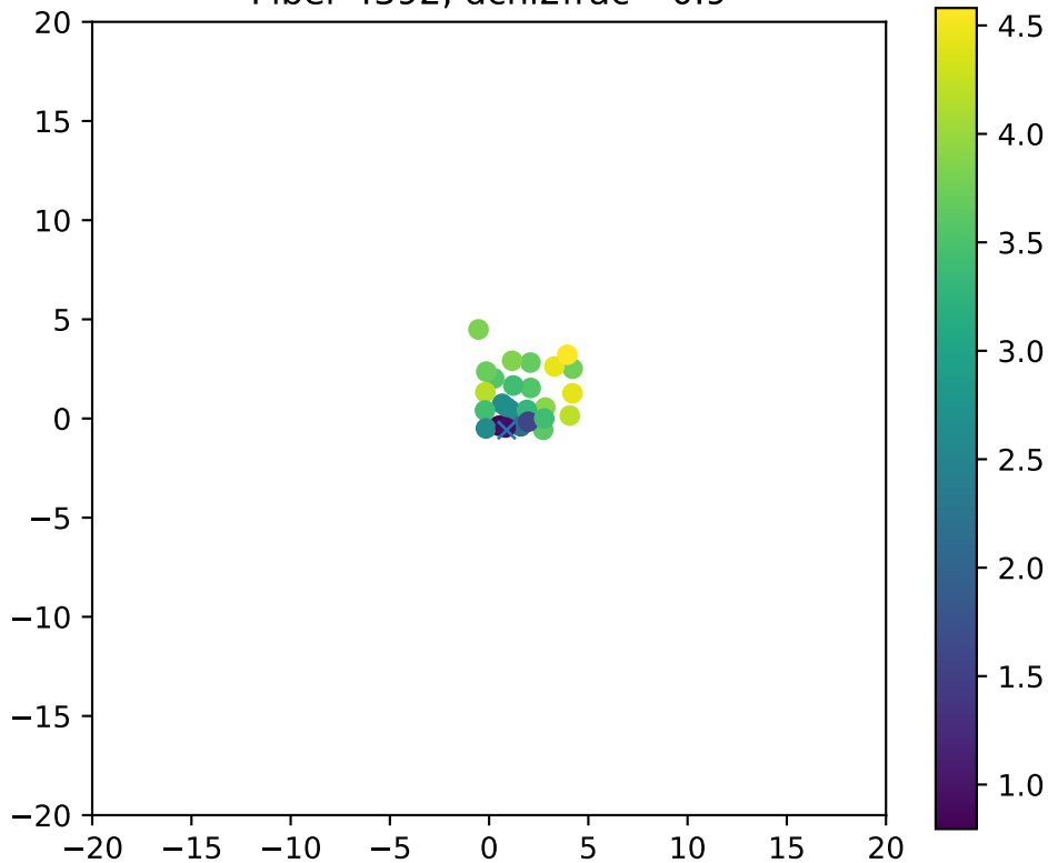
Fiber 4392, dchi2frac= 0.9
