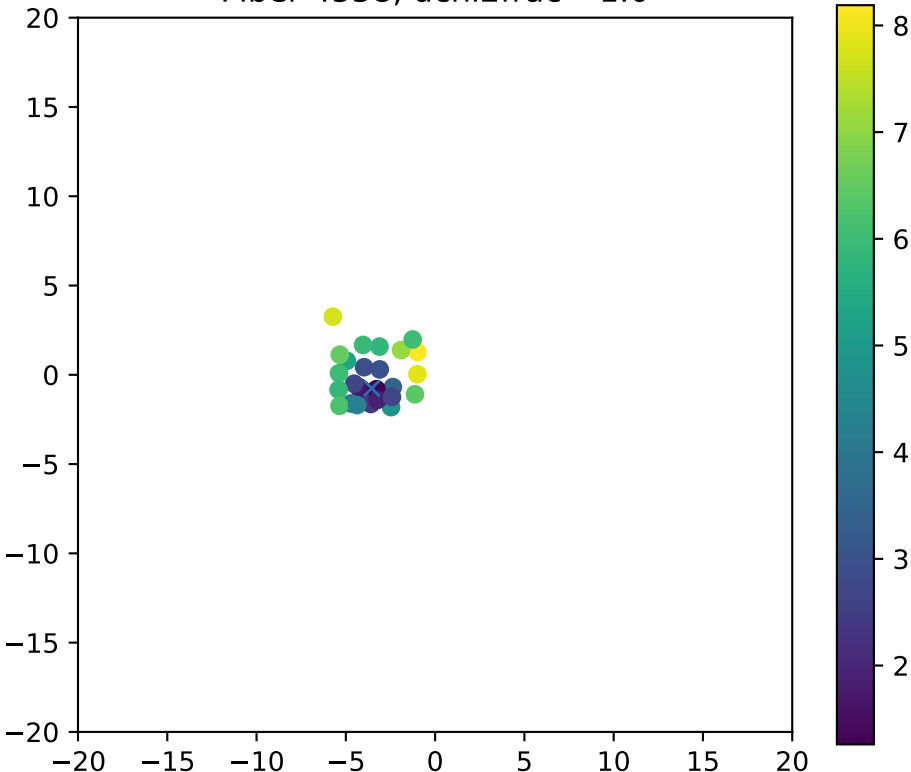
Fiber 4558, dchi2frac= 1.0
