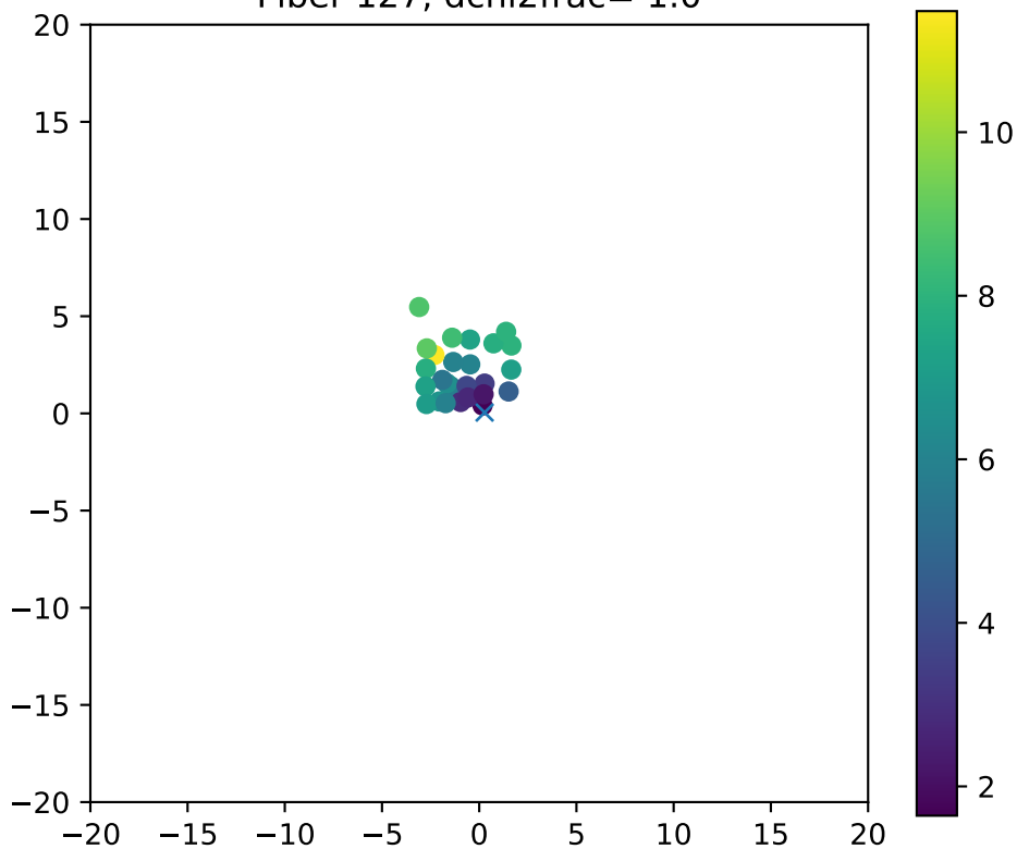
Fiber 127, dchi2frac= 1.0
