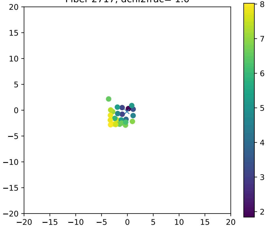
Fiber 2717, dchi2frac= 1.0
