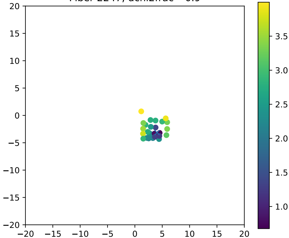
Fiber 2247, dchi2frac= 0.9
