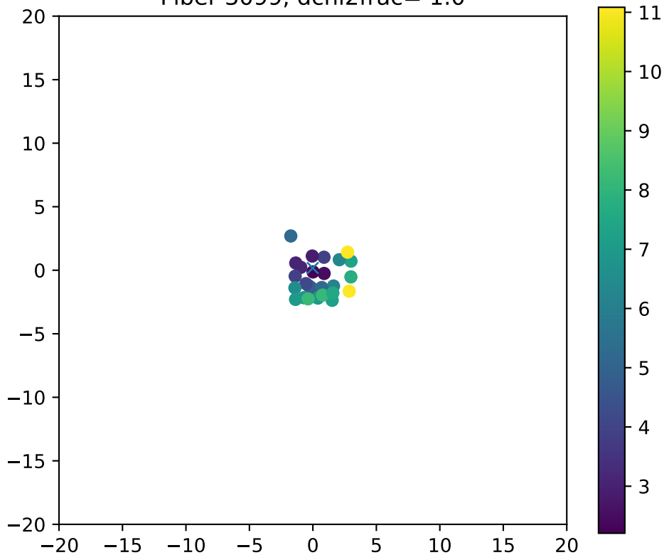
Fiber 3099, dchi2frac= 1.0
