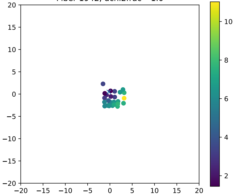
Fiber 1942, dchi2frac= 1.0
