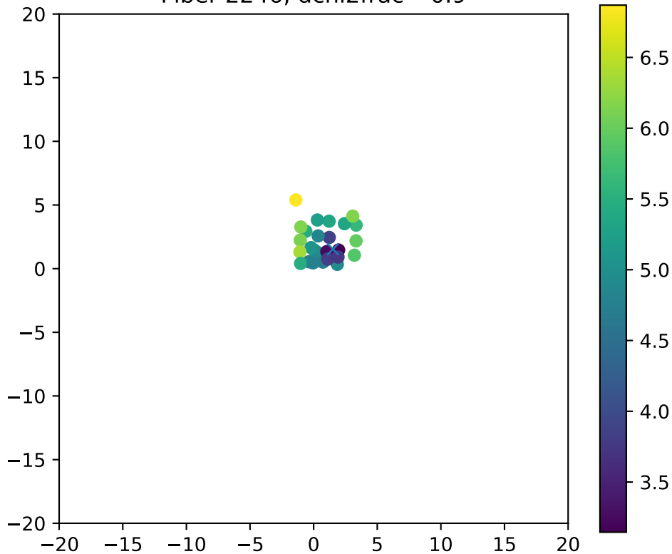
Fiber 2246, dchi2frac= 0.9
