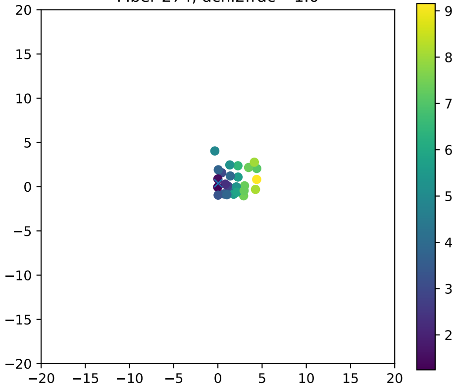
Fiber 274, dchi2frac= 1.0
