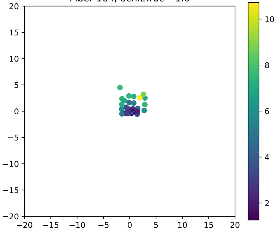
Fiber 164, dchi2frac= 1.0
