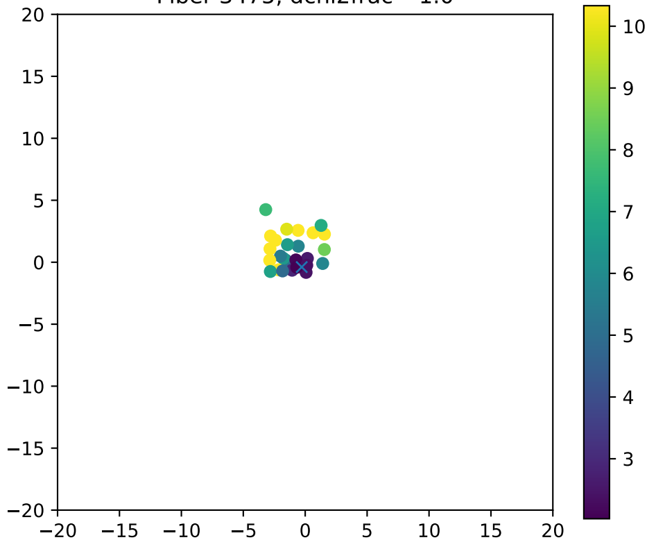
Fiber 3475, dchi2frac= 1.0
