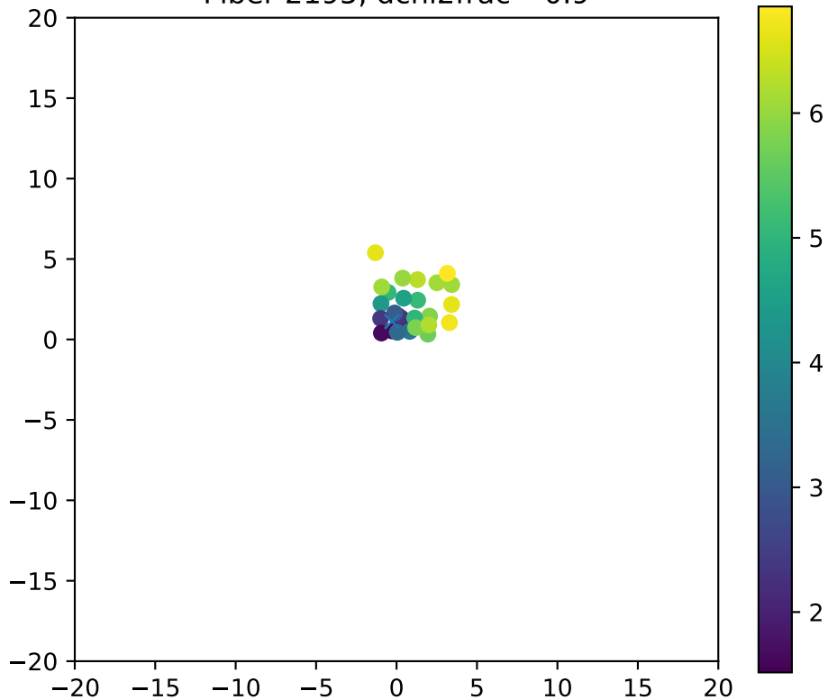
Fiber 2195, dchi2frac= 0.9
