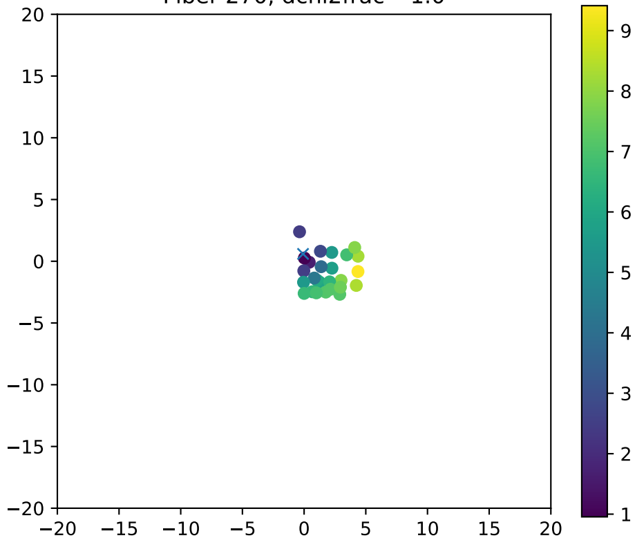
Fiber 270, dchi2frac= 1.0
