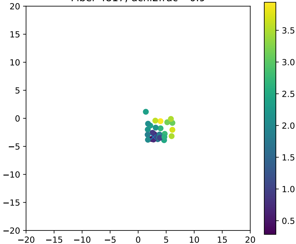
Fiber 4817, dchi2frac= 0.9
