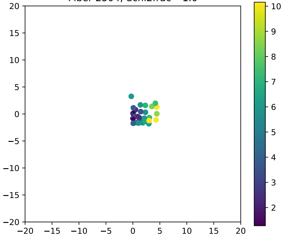
Fiber 2504, dchi2frac= 1.0
