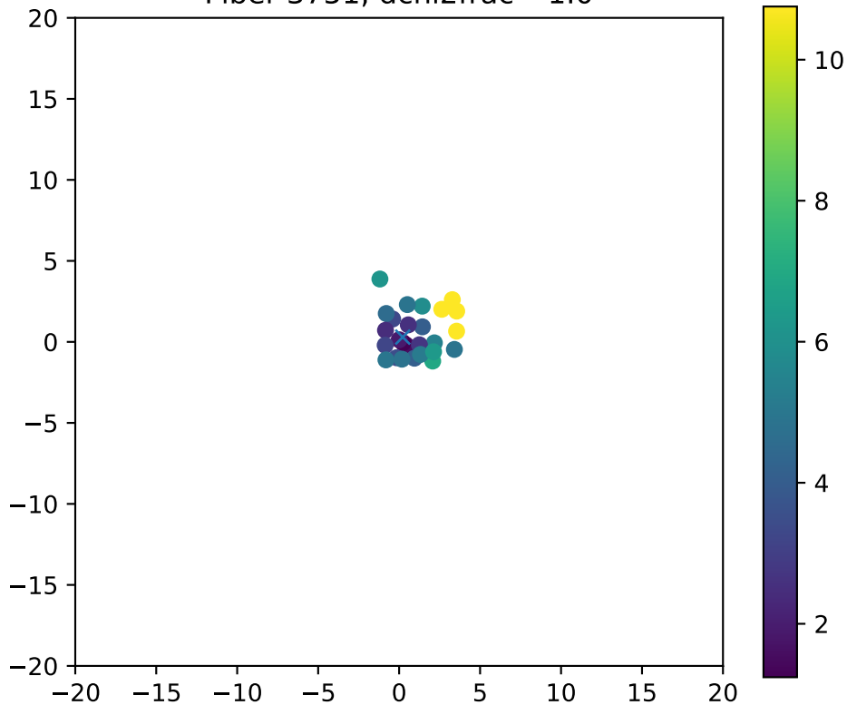
Fiber 3751, dchi2frac= 1.0
