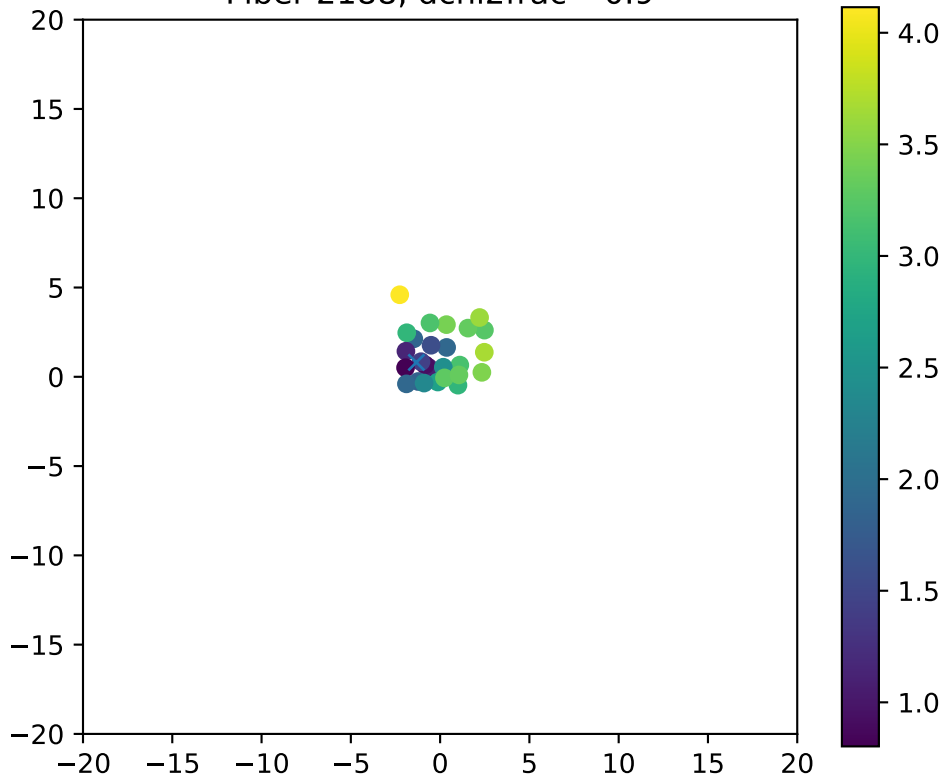
Fiber 2188, dchi2frac= 0.9
