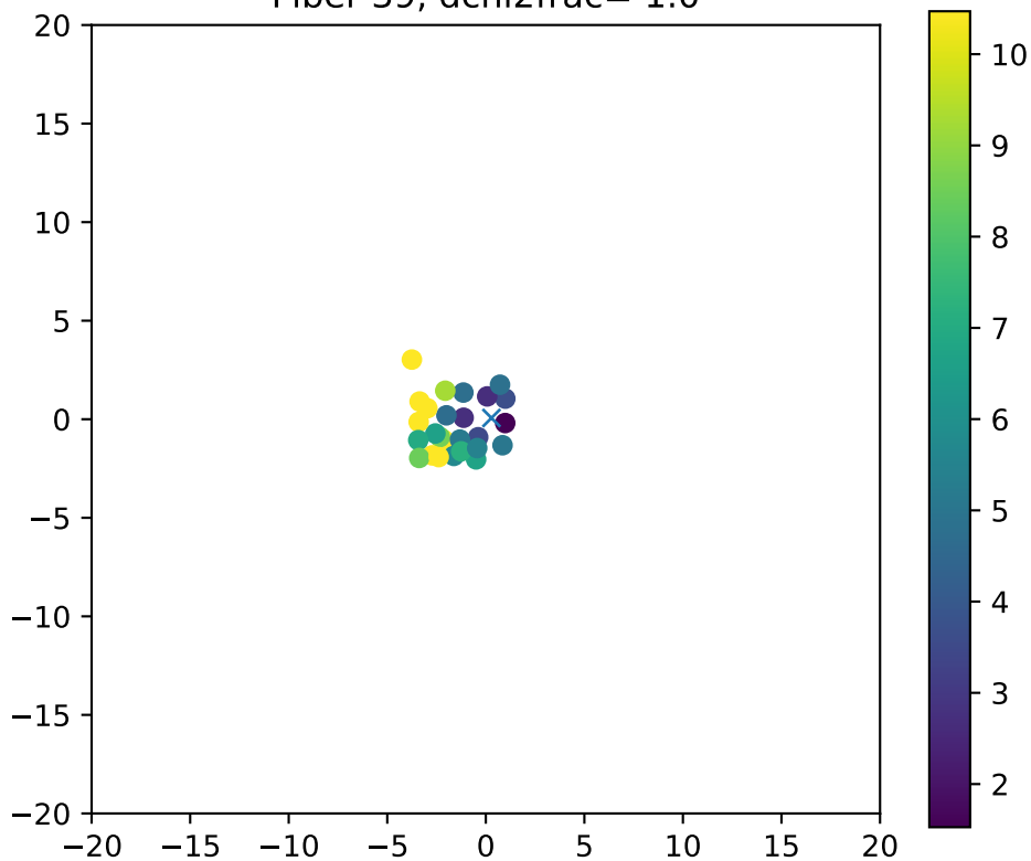
Fiber 39, dchi2frac= 1.0
