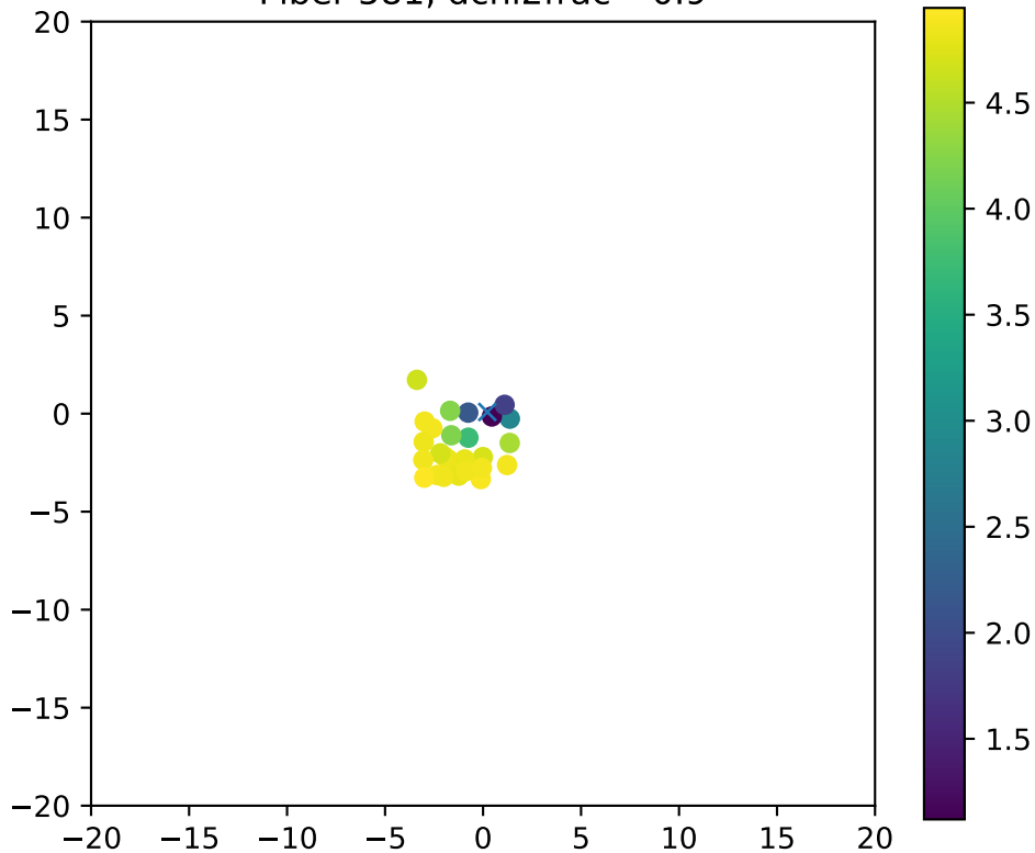
Fiber 581, dchi2frac= 0.9
