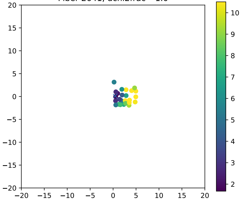
Fiber 2641, dchi2frac= 1.0
