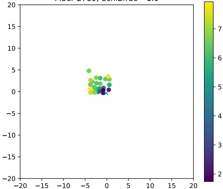
Fiber 2789, dchi2frac= 1.0
