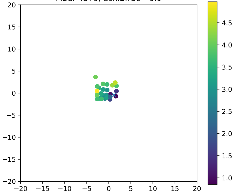
Fiber 4370, dchi2frac= 0.9
