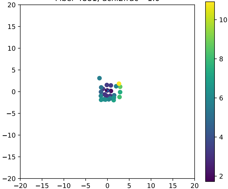
Fiber 4881, dchi2frac= 1.0
