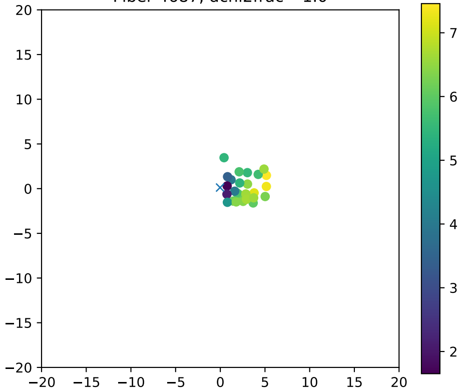
Fiber 4687, dchi2frac= 1.0
