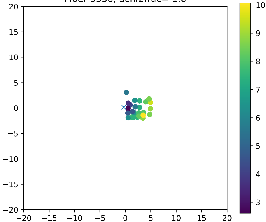
Fiber 3356, dchi2frac= 1.0
