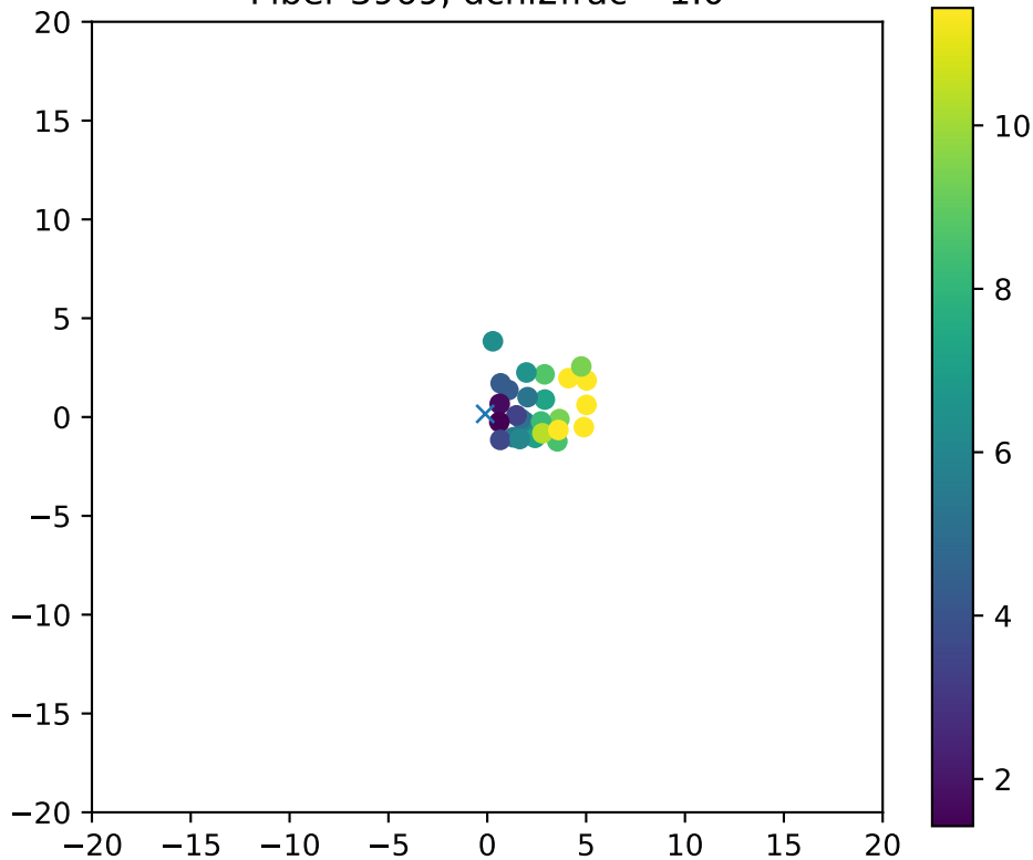
Fiber 3969, dchi2frac= 1.0
