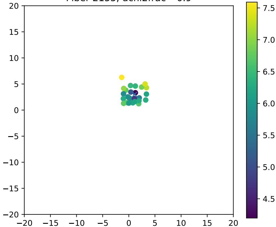
Fiber 2155, dchi2frac= 0.9
