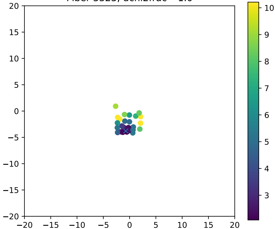
Fiber 3323, dchi2frac= 1.0
