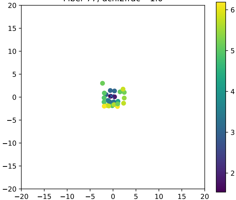
Fiber 77, dchi2frac= 1.0
