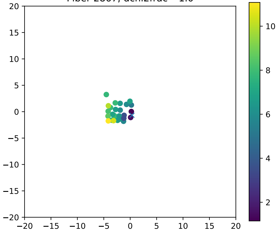
Fiber 2867, dchi2frac= 1.0
