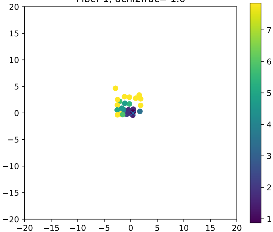
Fiber 1, dchi2frac= 1.0
