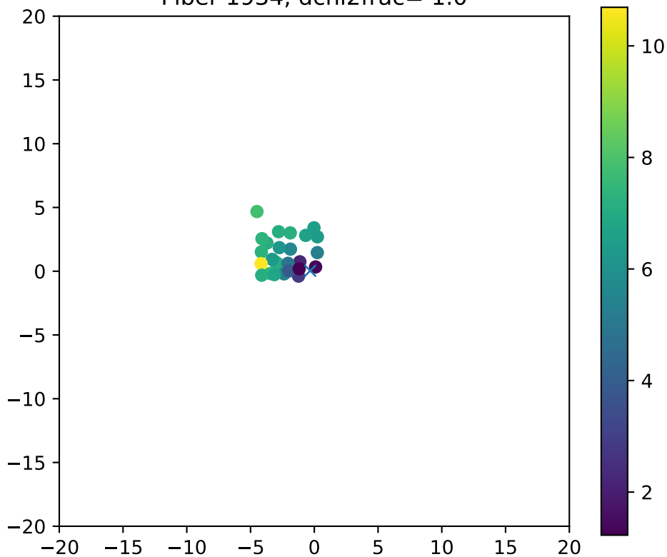
Fiber 1934, dchi2frac= 1.0
