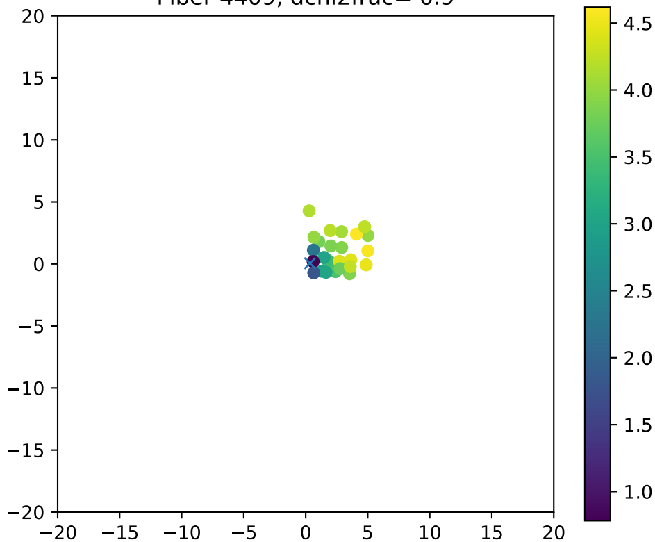
Fiber 4409, dchi2frac= 0.9
