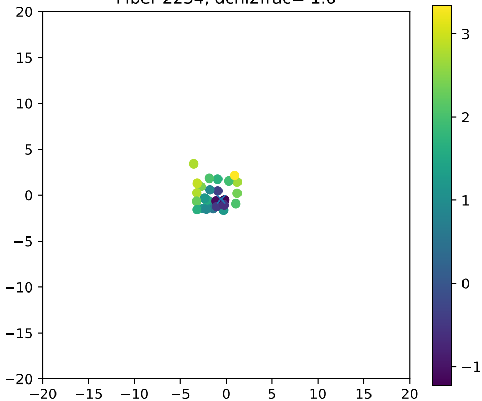
Fiber 2254, dchi2frac= 1.0
