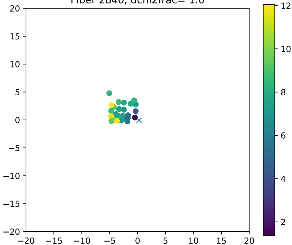
Fiber 2840, dchi2frac= 1.0
