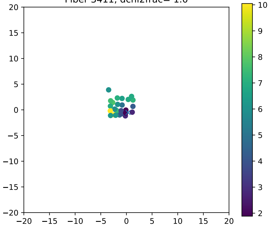
Fiber 3411, dchi2frac= 1.0
