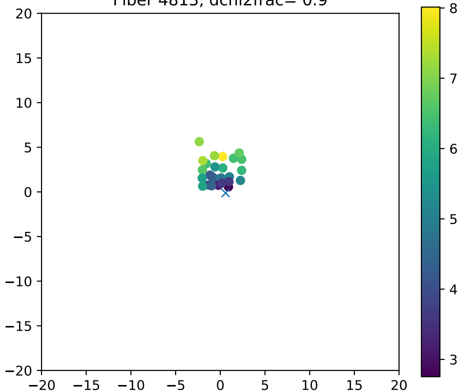
Fiber 4813, dchi2frac= 0.9
