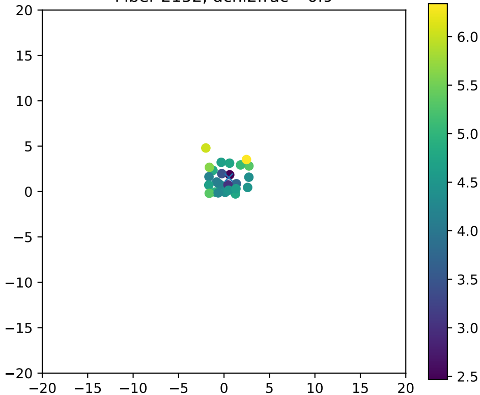
Fiber 2152, dchi2frac= 0.9
