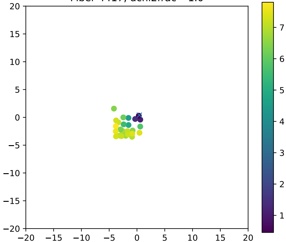
Fiber 4417, dchi2frac= 1.0
