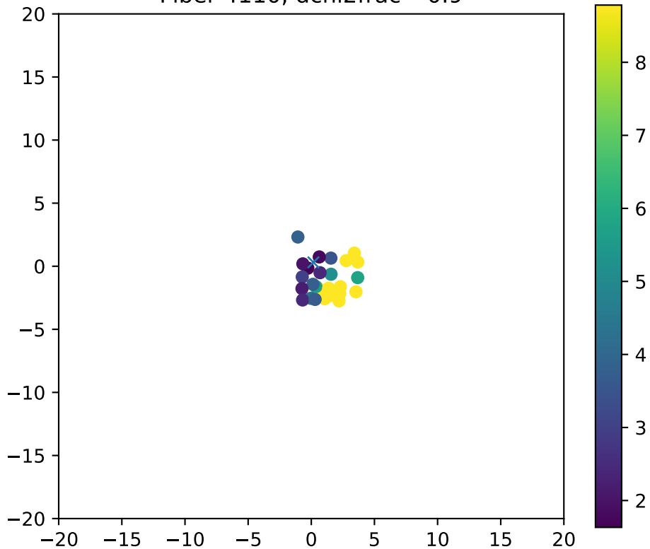
Fiber 4110, dchi2frac= 0.9
