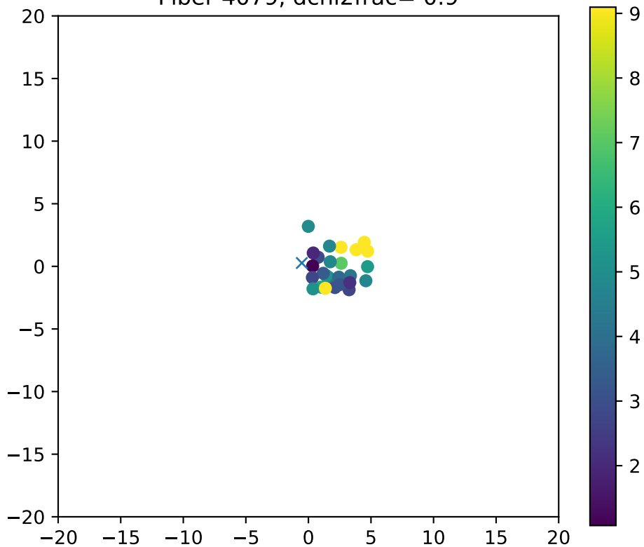
Fiber 4079, dchi2frac= 0.9
