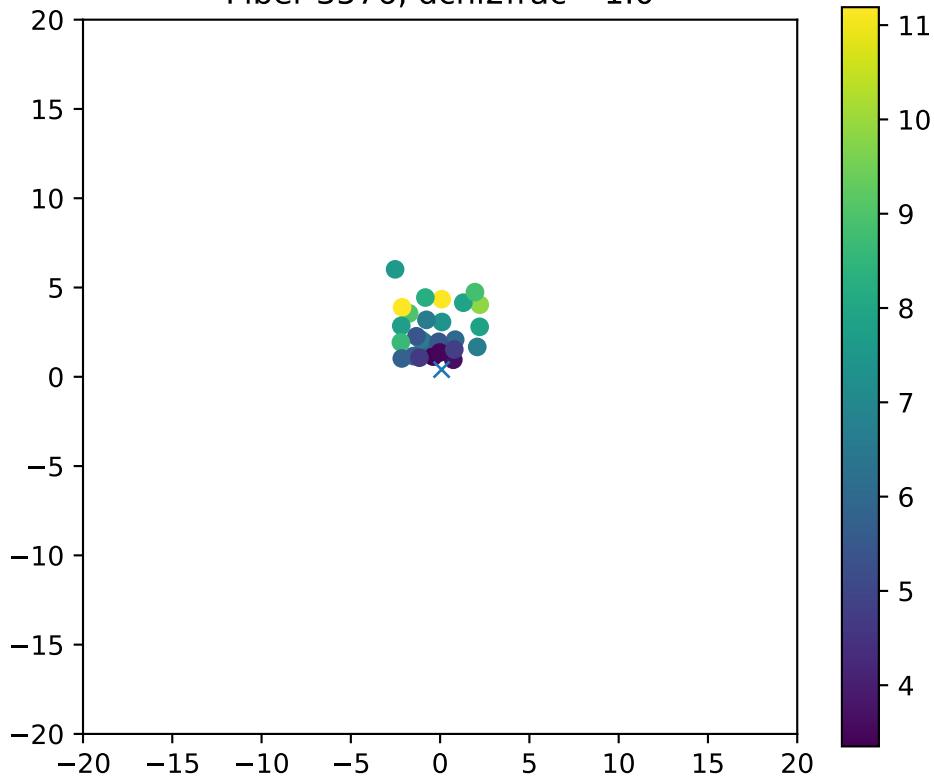
Fiber 3576, dchi2frac= 1.0
