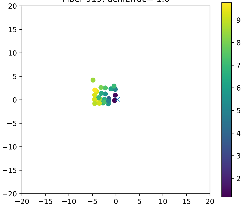
Fiber 919, dchi2frac= 1.0
