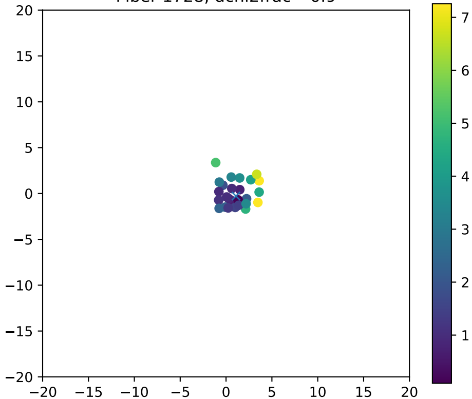
Fiber 1728, dchi2frac= 0.9
