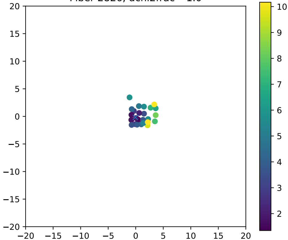
Fiber 2826, dchi2frac= 1.0
