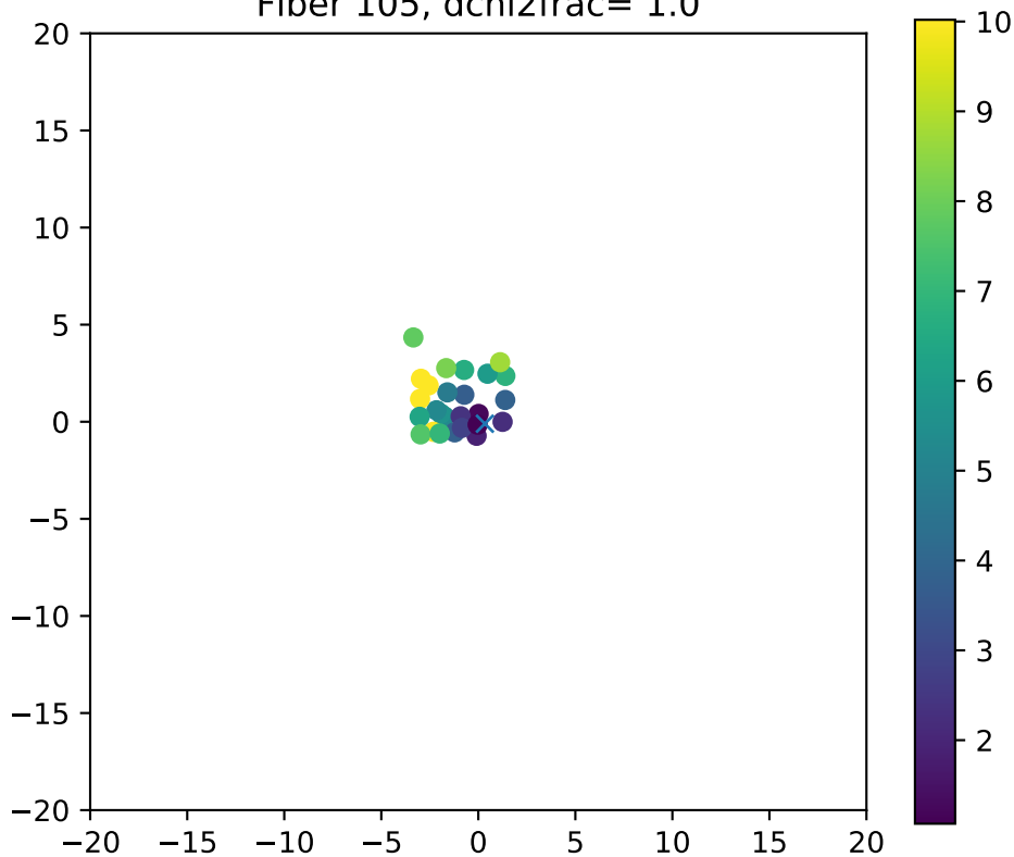
Fiber 105, dchi2frac= 1.0
