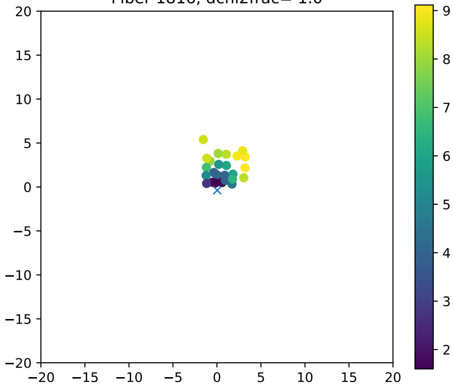
Fiber 1816, dchi2frac= 1.0
