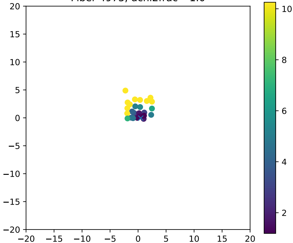
Fiber 4973, dchi2frac= 1.0
