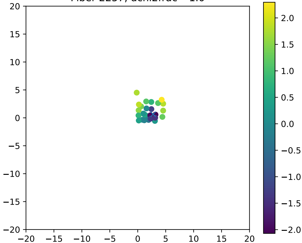
Fiber 2257, dchi2frac= 1.0
