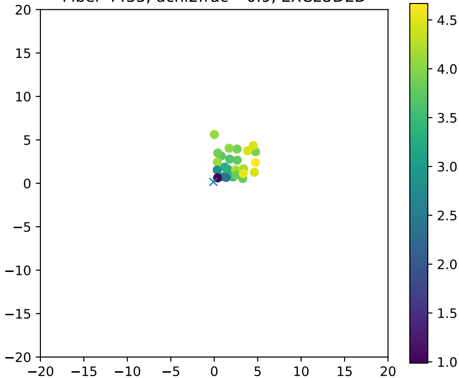
Fiber 4433, dchi2frac= 0.9, EXCLUDED
