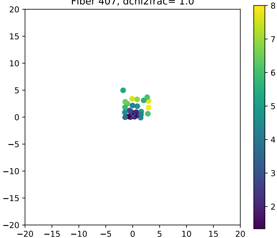
Fiber 407, dchi2frac= 1.0
