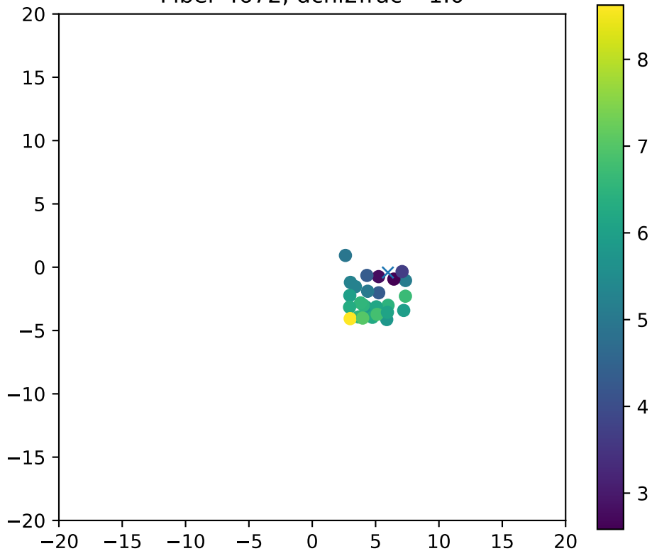
Fiber 4672, dchi2frac= 1.0
