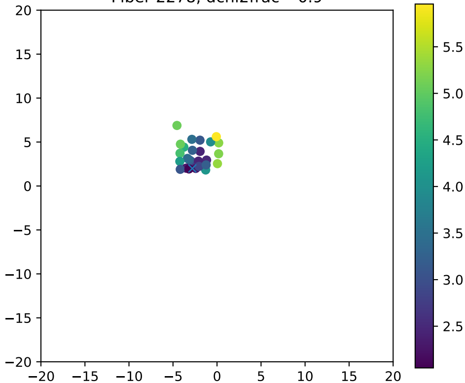
Fiber 2278, dchi2frac= 0.9
