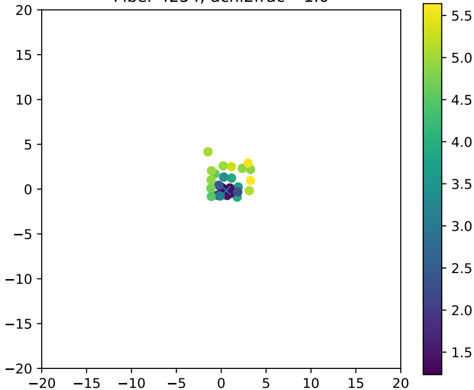
Fiber 4254, dchi2frac= 1.0
