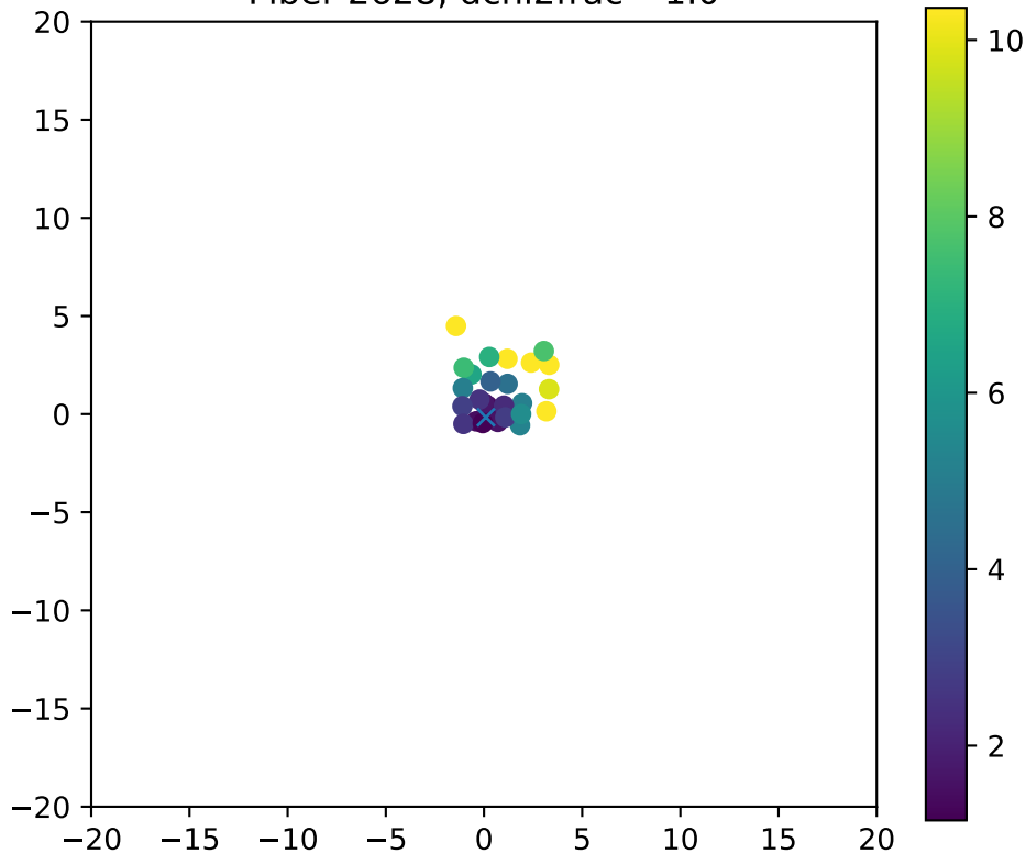
Fiber 2628, dchi2frac= 1.0
