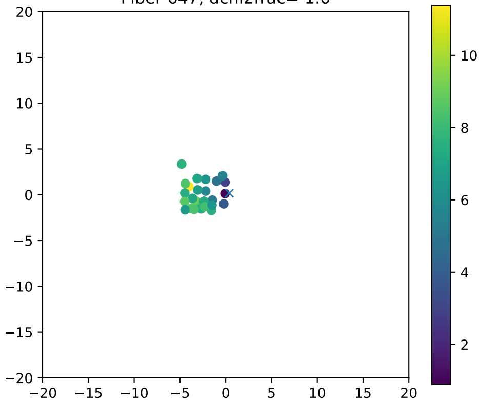
Fiber 647, dchi2frac= 1.0
