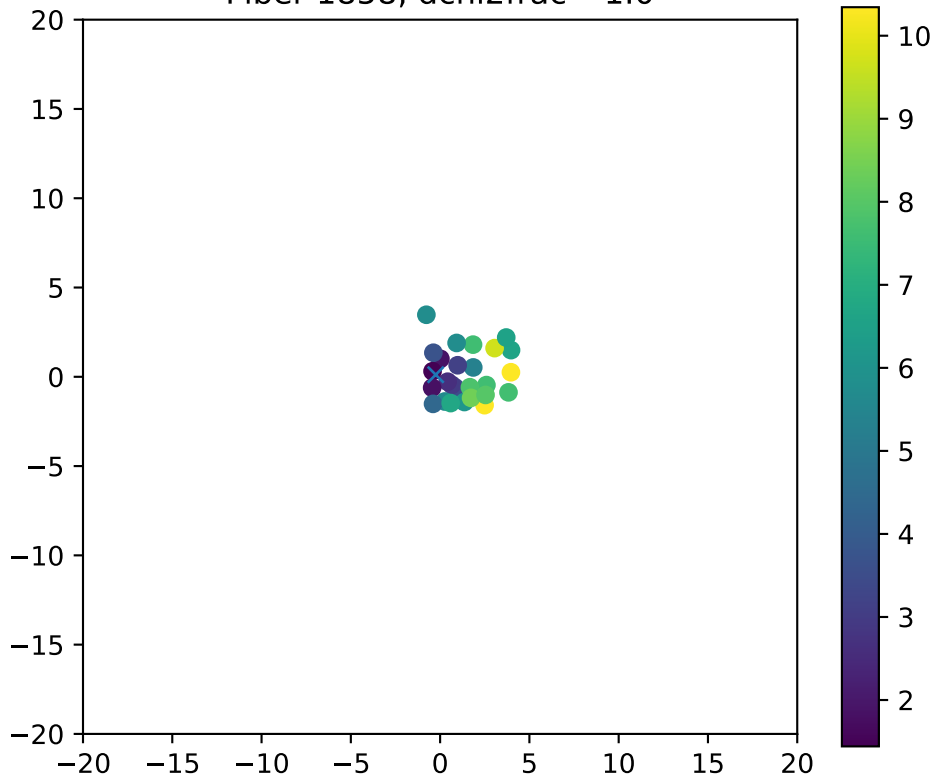
Fiber 1858, dchi2frac= 1.0
