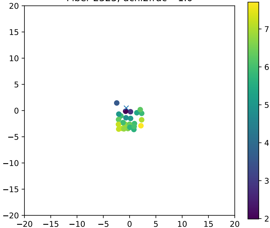
Fiber 2323, dchi2frac= 1.0
