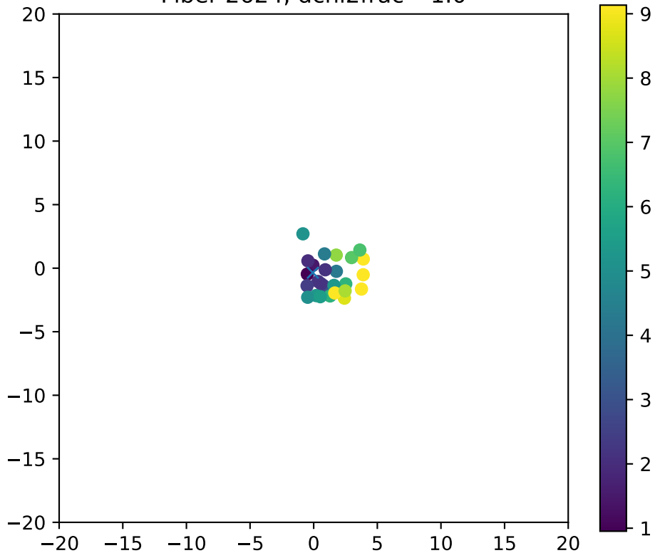
Fiber 2624, dchi2frac= 1.0
