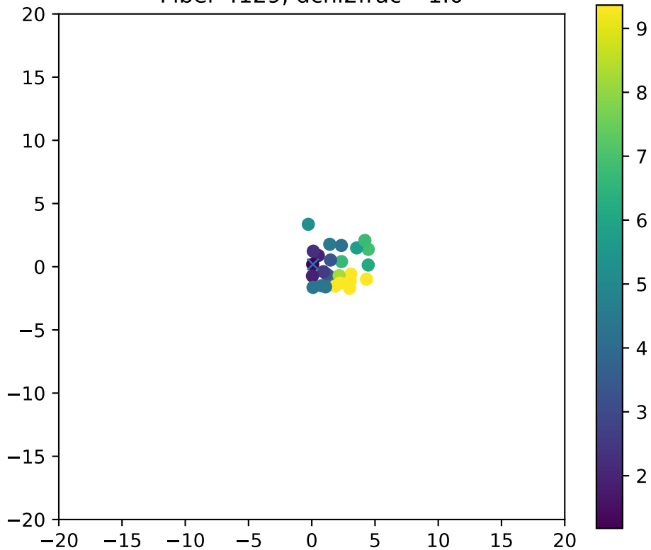
Fiber 4129, dchi2frac= 1.0
