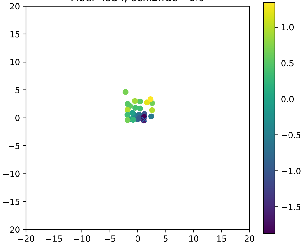
Fiber 4334, dchi2frac= 0.9
