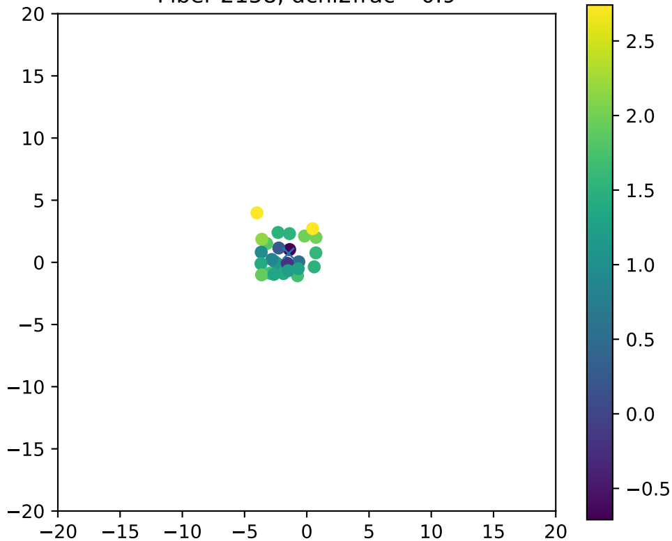
Fiber 2158, dchi2frac= 0.9
