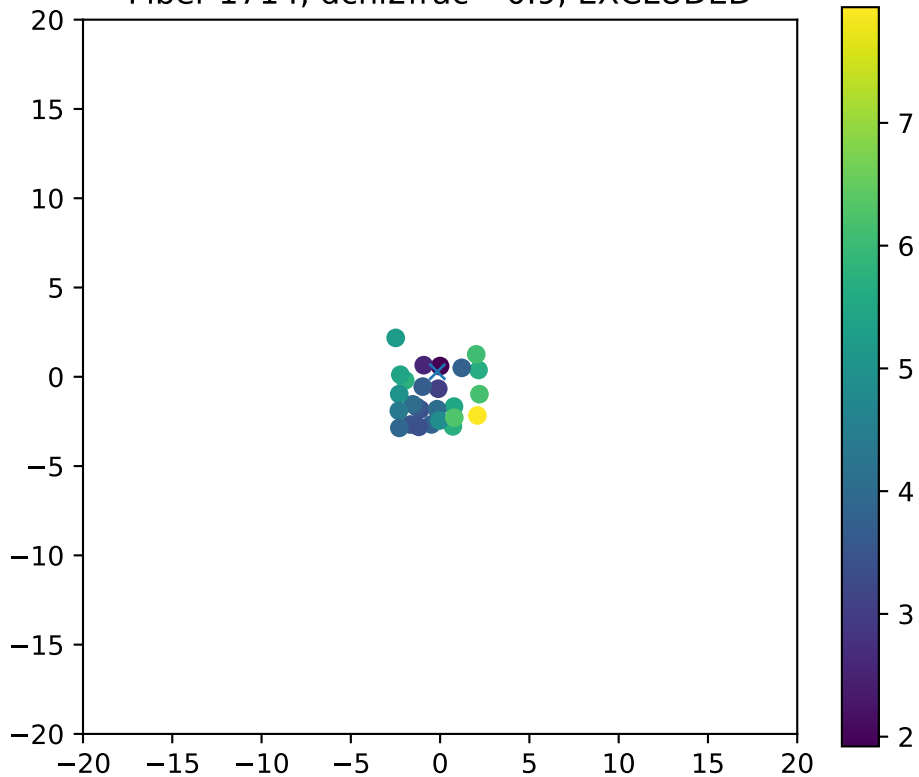
Fiber 1714, dchi2frac= 0.9, EXCLUDED
