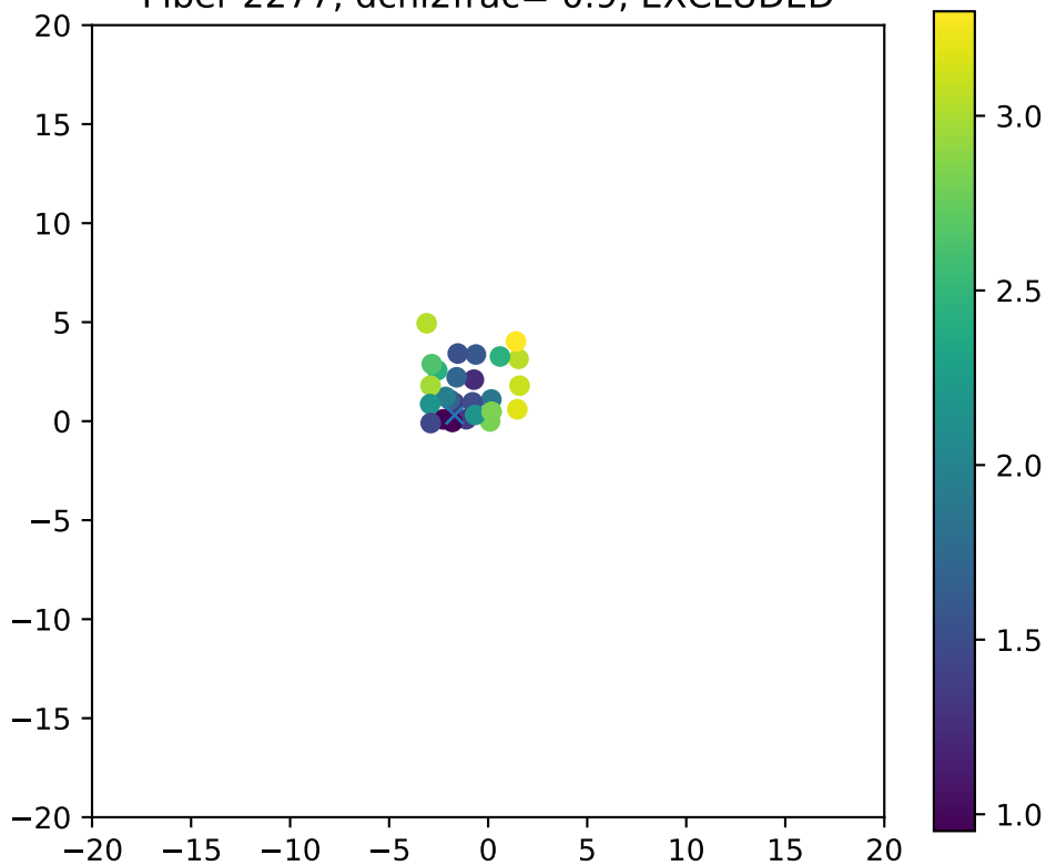
Fiber 2277, dchi2frac= 0.9, EXCLUDED
