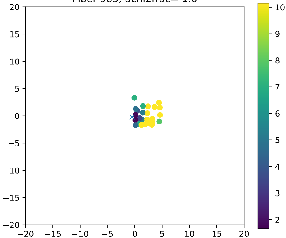
Fiber 965, dchi2frac= 1.0
