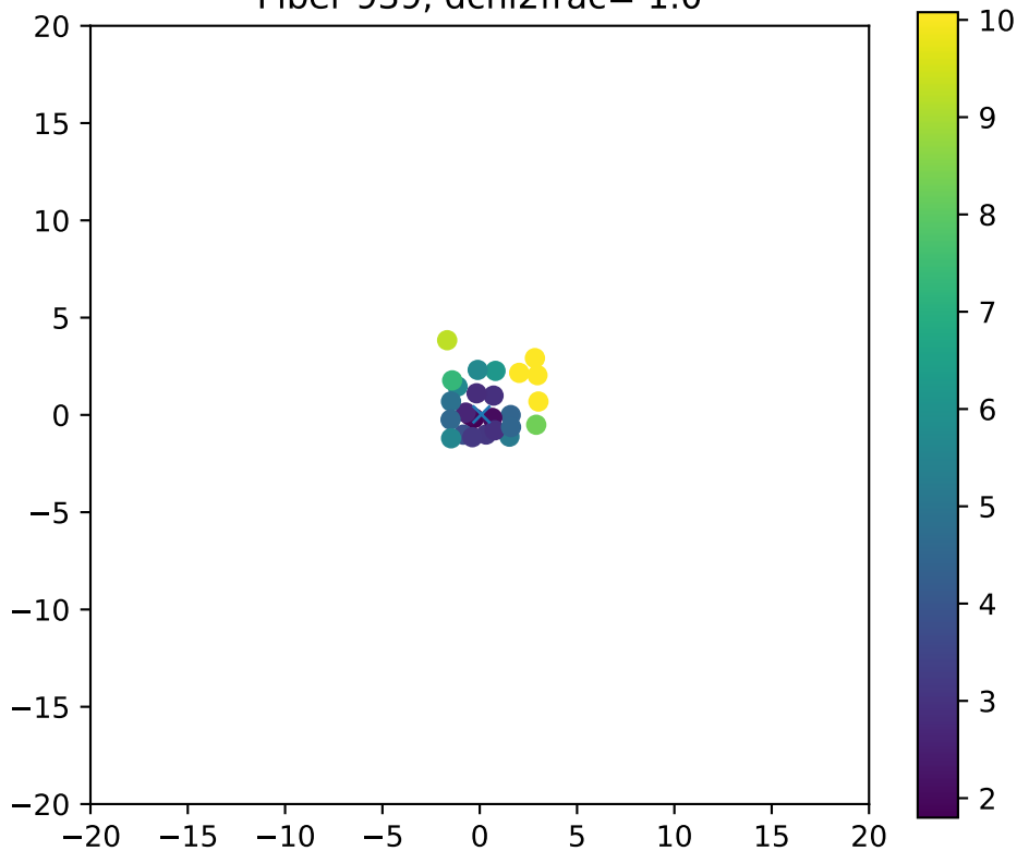
Fiber 939, dchi2frac= 1.0
