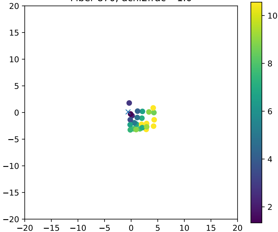
Fiber 870, dchi2frac= 1.0
