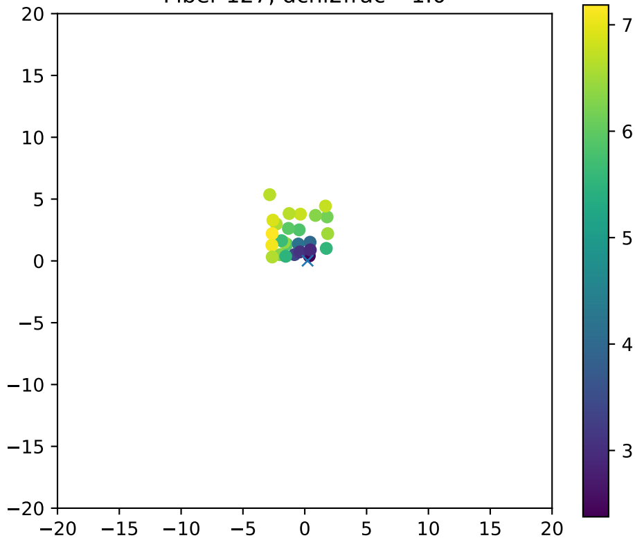
Fiber 127, dchi2frac= 1.0
