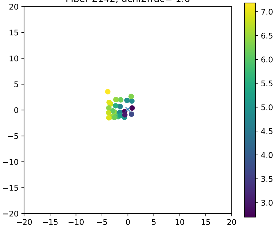
Fiber 2142, dchi2frac= 1.0
