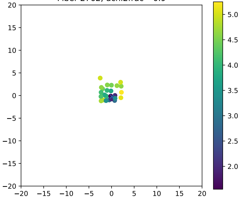
Fiber 2762, dchi2frac= 0.9
