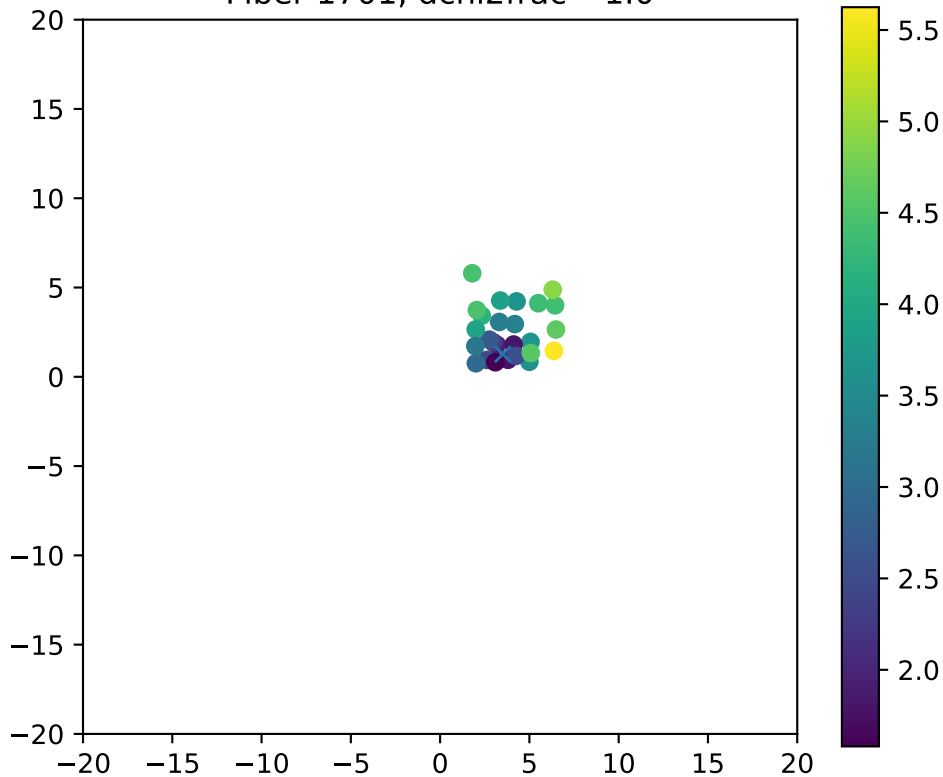
Fiber 1701, dchi2frac= 1.0
