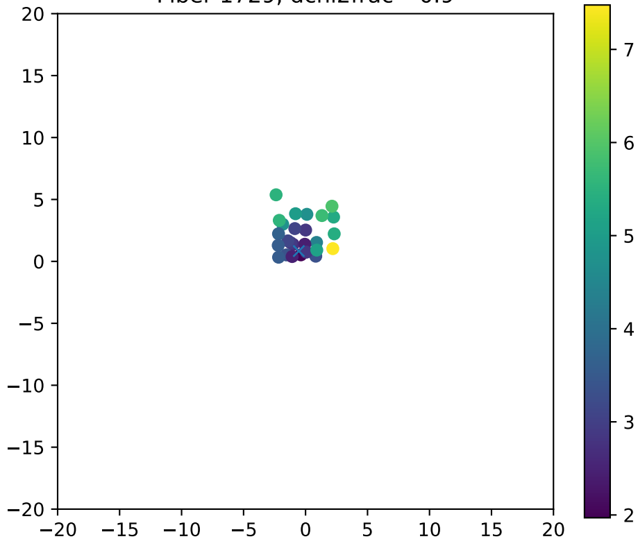
Fiber 1729, dchi2frac= 0.9
