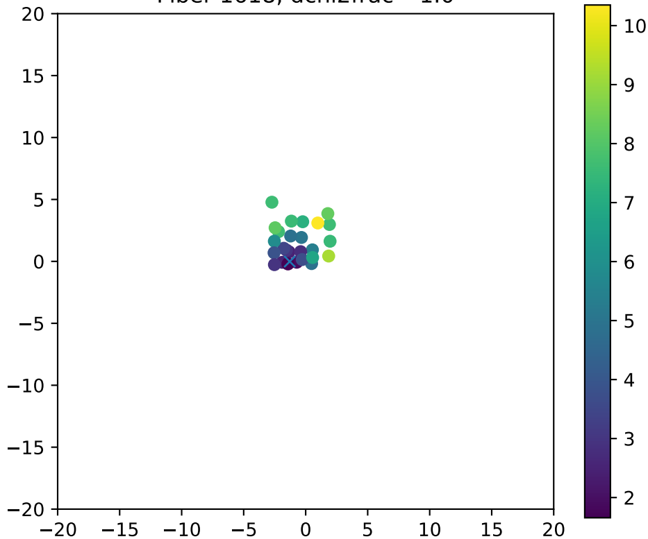
Fiber 1618, dchi2frac= 1.0
