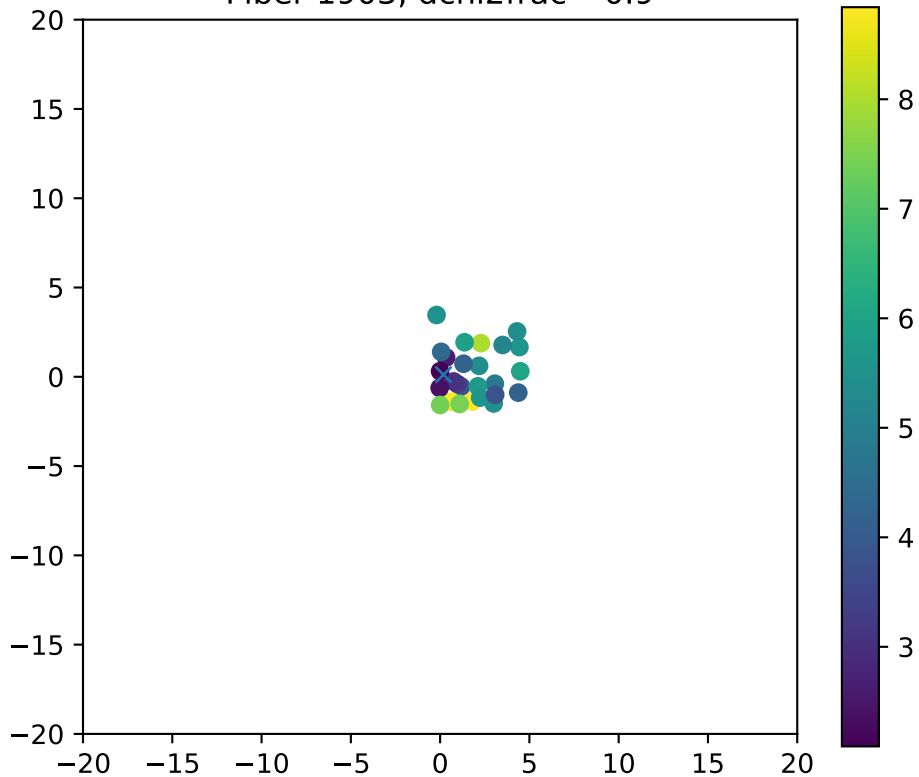
Fiber 1903, dchi2frac= 0.9
