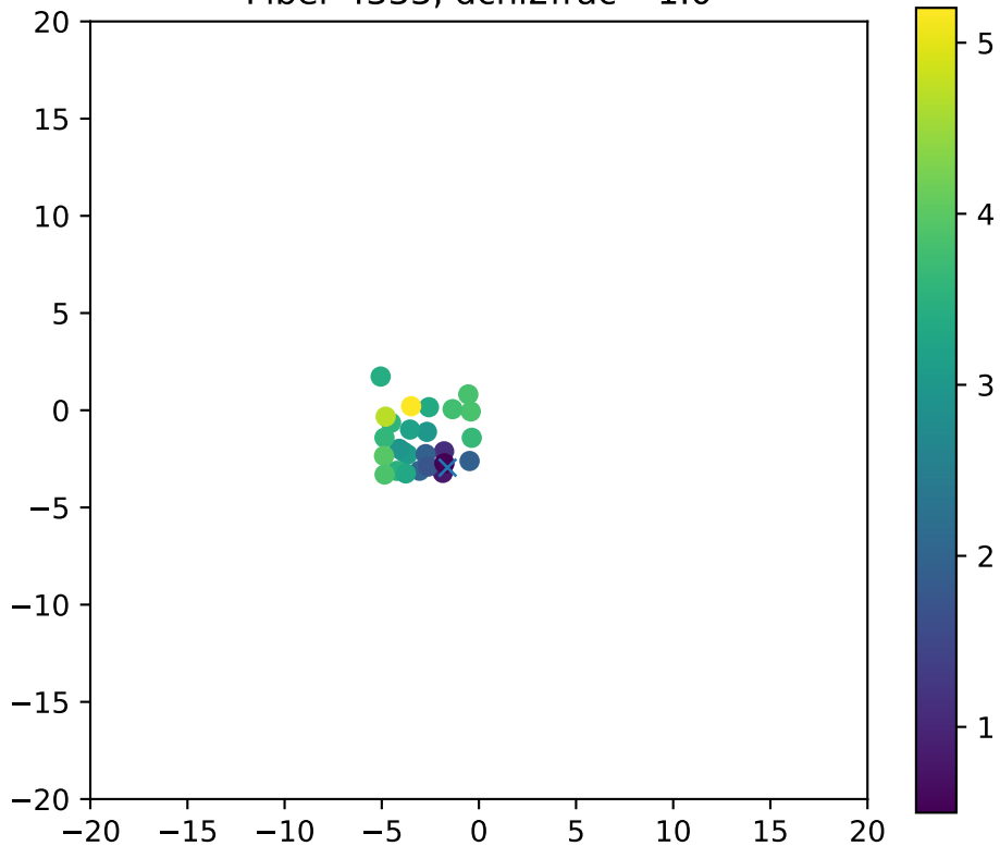
Fiber 4333, dchi2frac= 1.0
