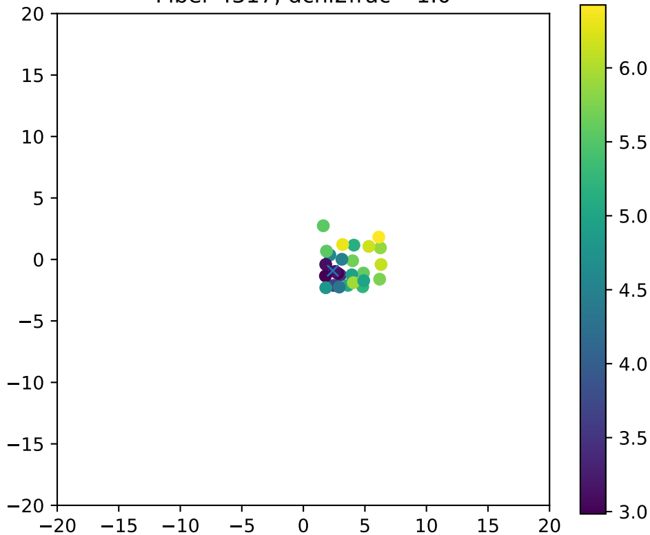
Fiber 4317, dchi2frac= 1.0
