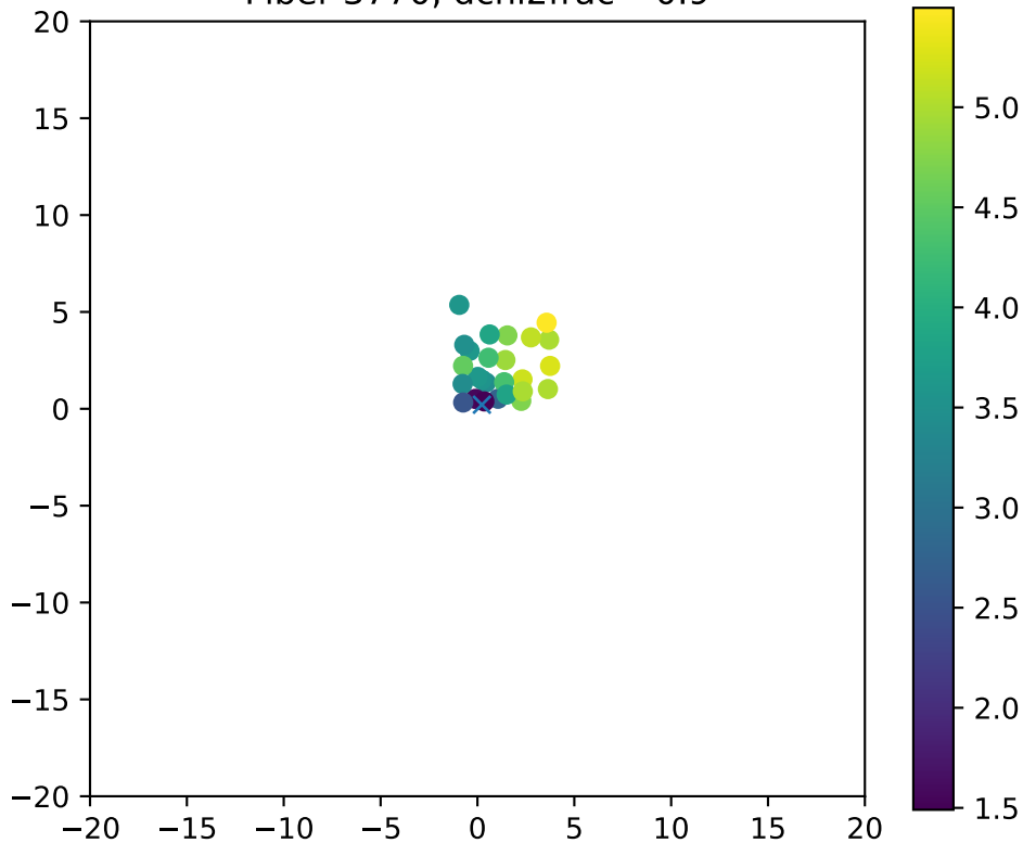
Fiber 3770, dchi2frac= 0.9
