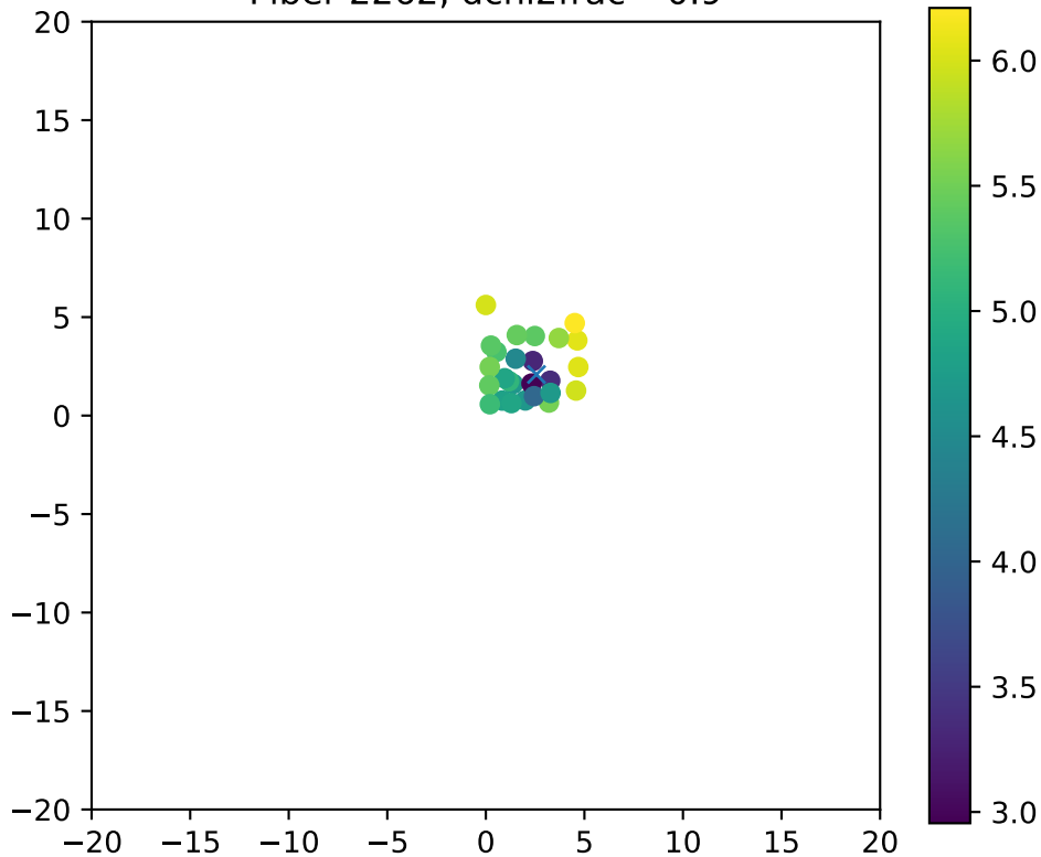
Fiber 2262, dchi2frac= 0.9
