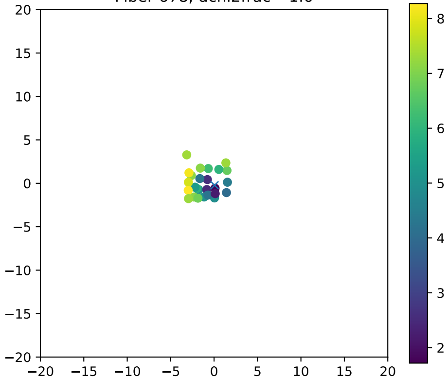
Fiber 678, dchi2frac= 1.0
