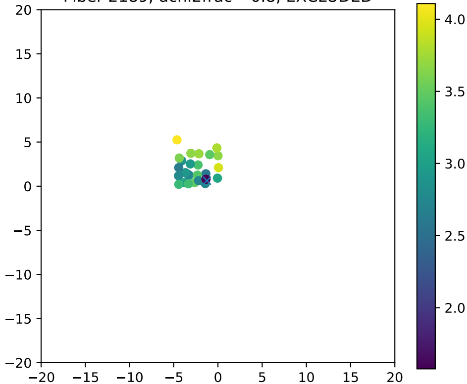
Fiber 2189, dchi2frac= 0.8, EXCLUDED
