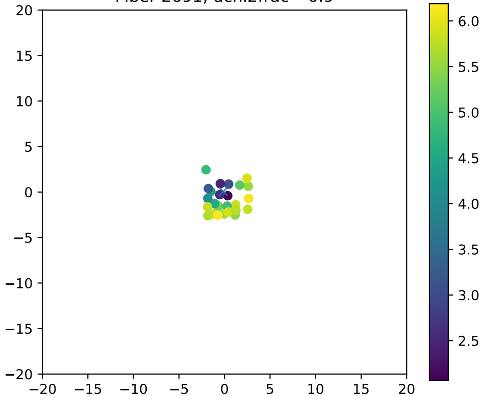
Fiber 2691, dchi2frac= 0.9
