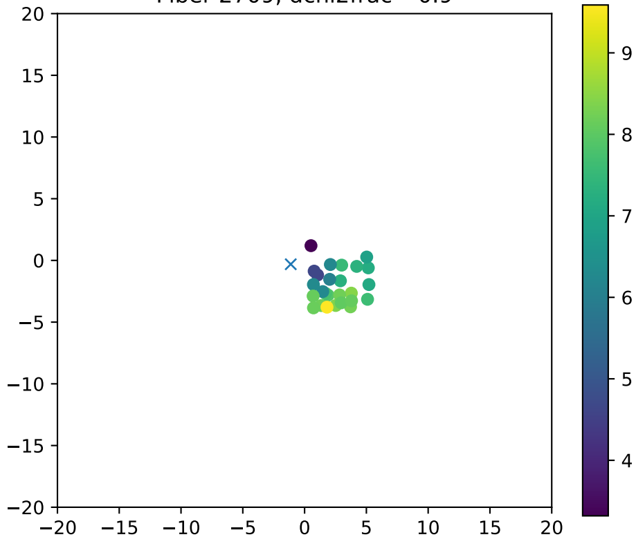
Fiber 2709, dchi2frac= 0.9
