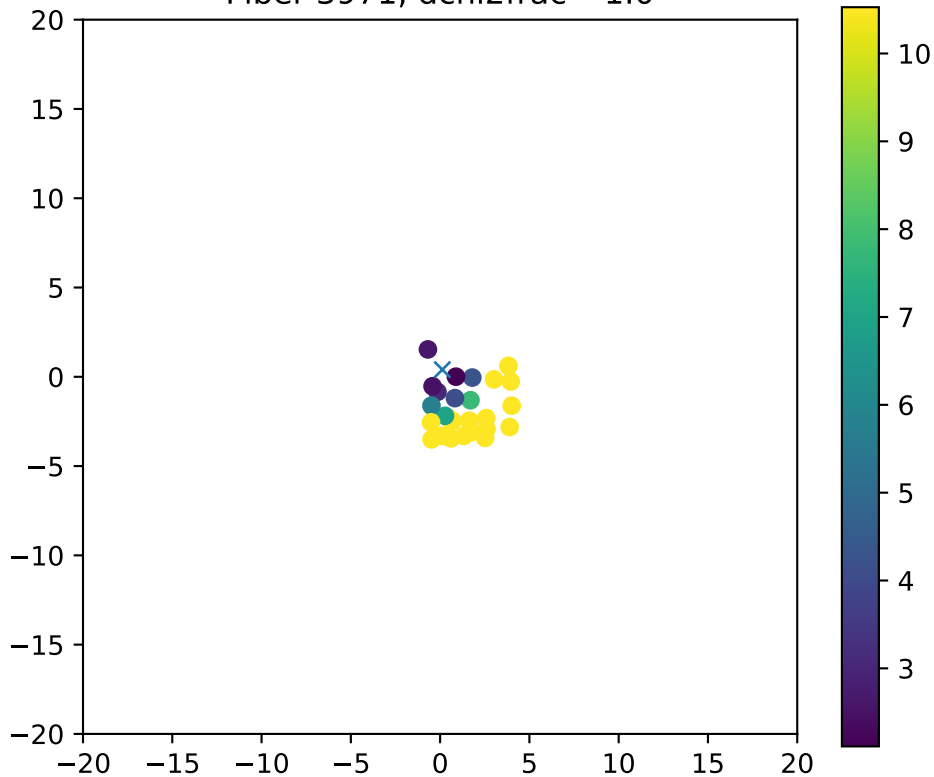
Fiber 3971, dchi2frac= 1.0
