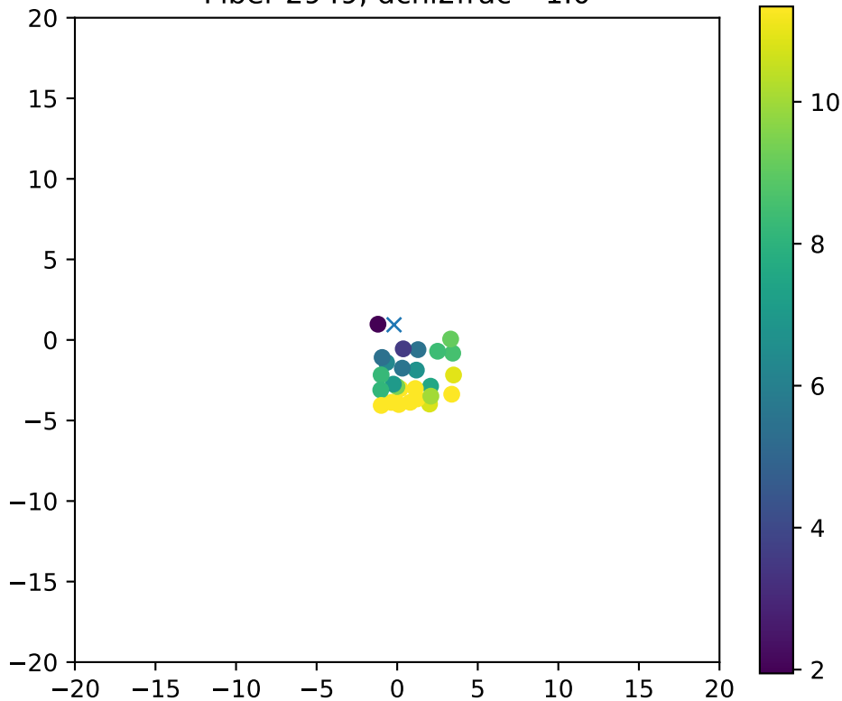
Fiber 2949, dchi2frac= 1.0
