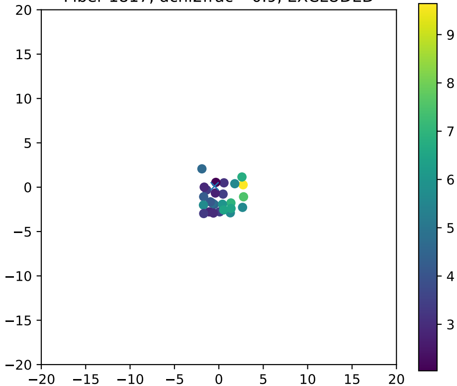
Fiber 1817, dchi2frac= 0.9, EXCLUDED
