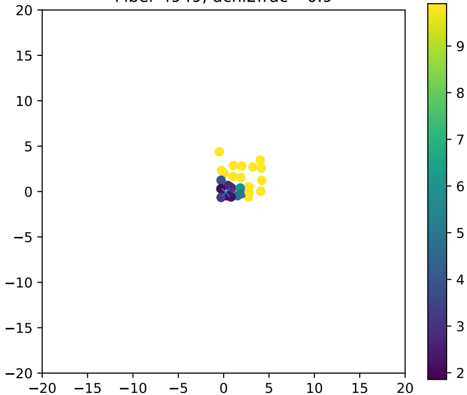
Fiber 4949, dchi2frac= 0.9
