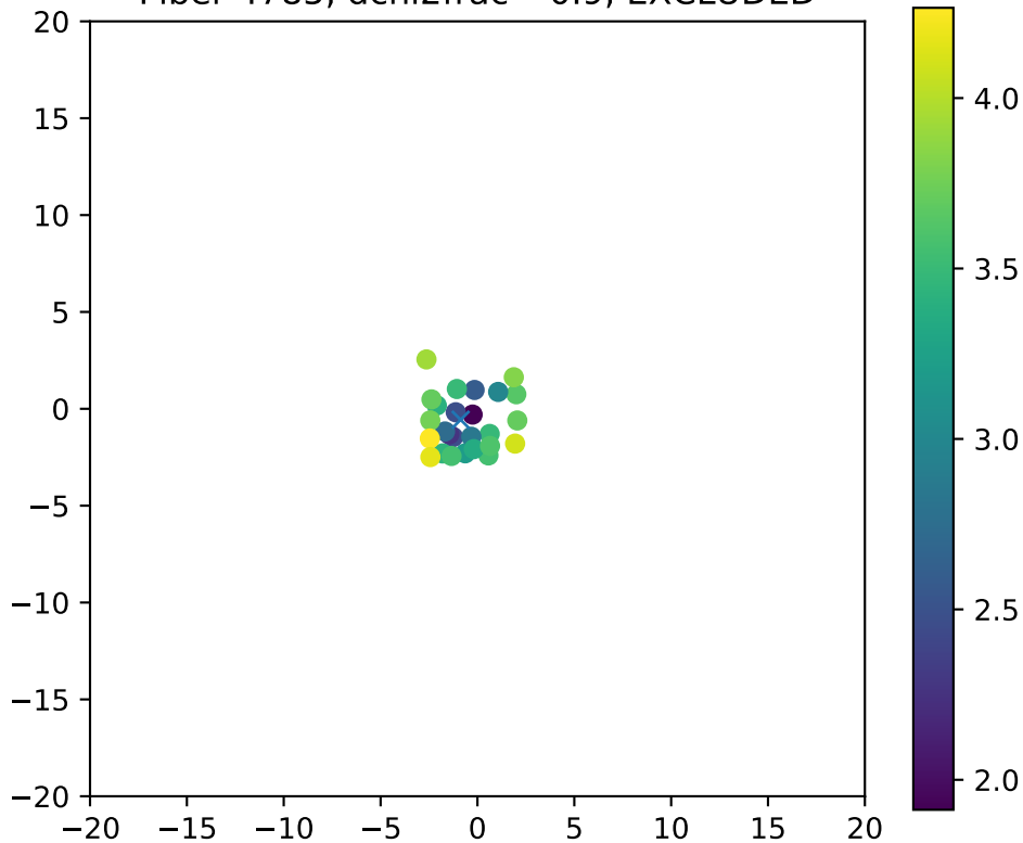
Fiber 4785, dchi2frac= 0.9, EXCLUDED
