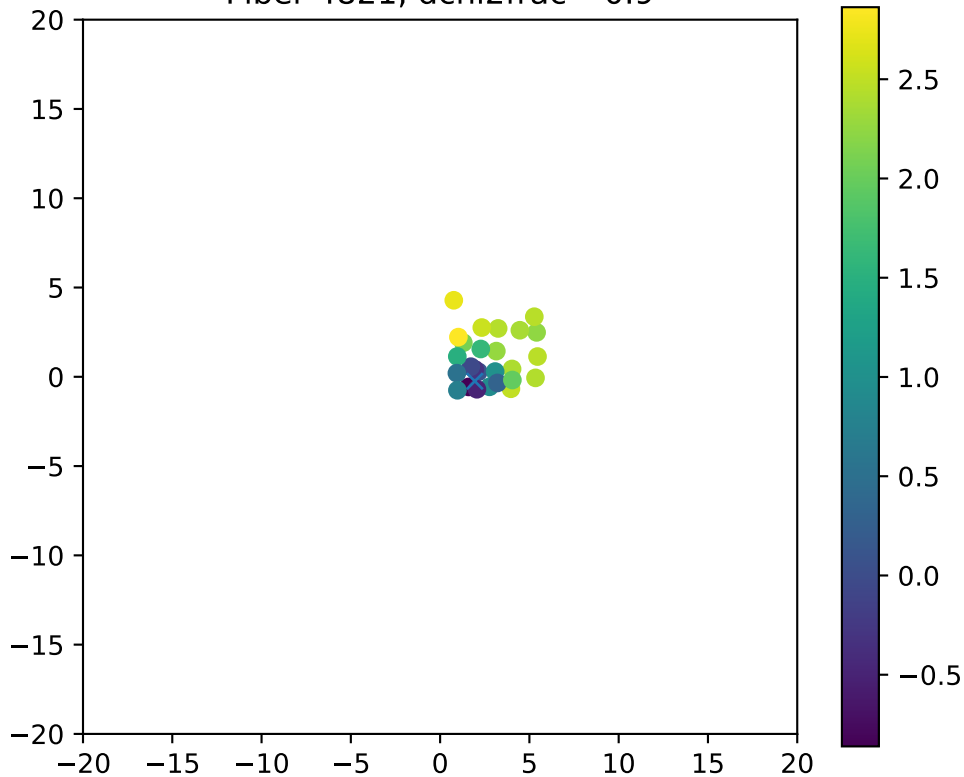
Fiber 4821, dchi2frac= 0.9
