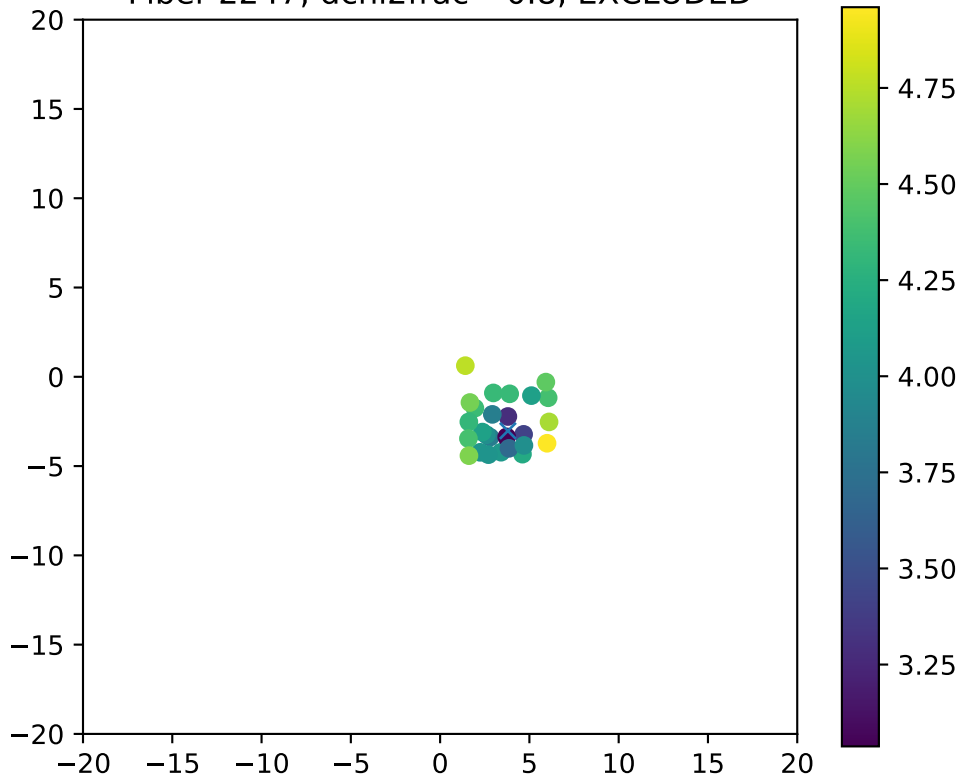
Fiber 2247, dchi2frac= 0.8, EXCLUDED
