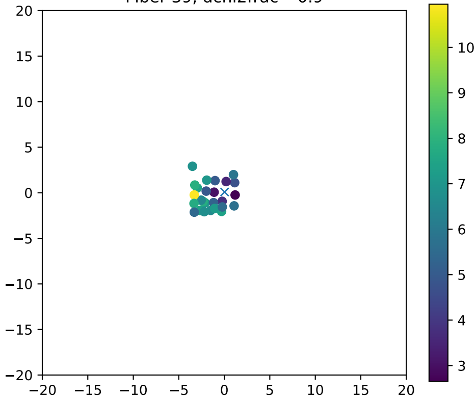
Fiber 39, dchi2frac= 0.9
