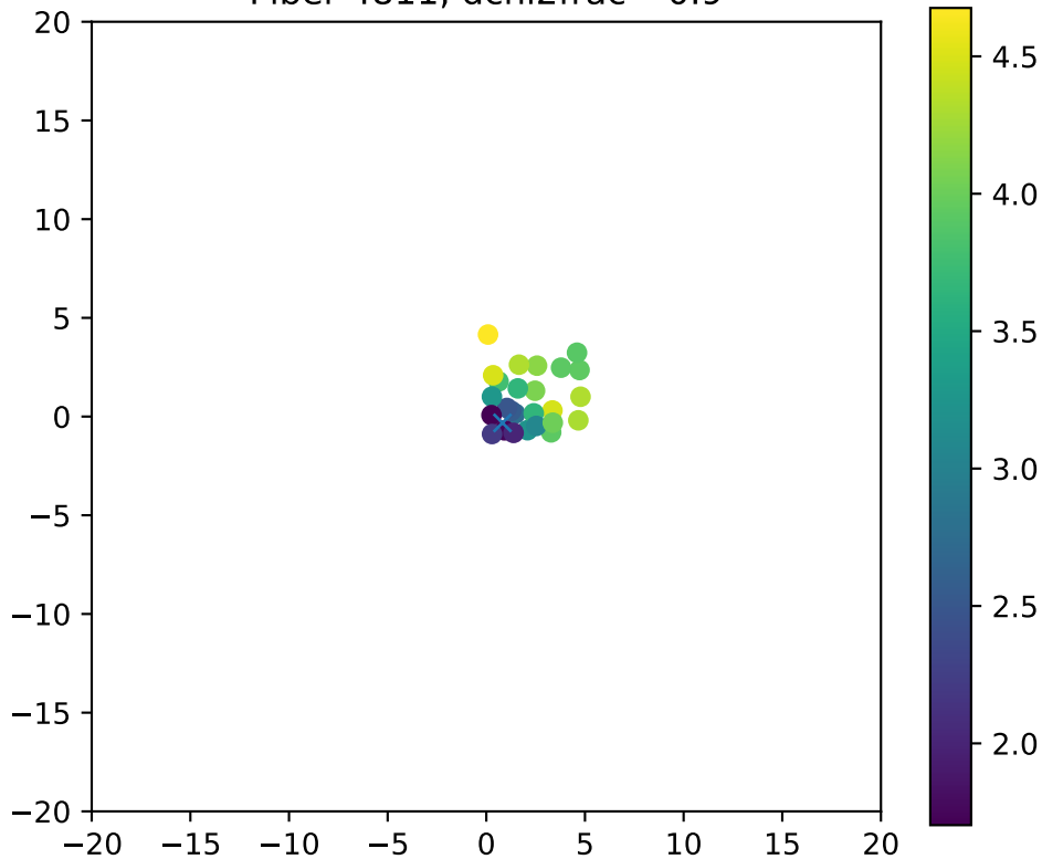
Fiber 4811, dchi2frac= 0.9
