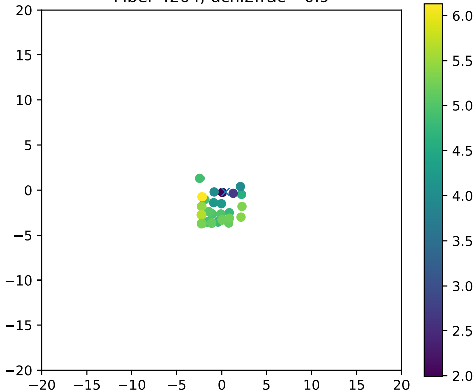
Fiber 4264, dchi2frac= 0.9
