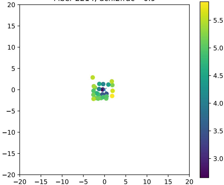
Fiber 2214, dchi2frac= 0.9
