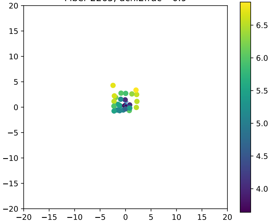
Fiber 2265, dchi2frac= 0.9
