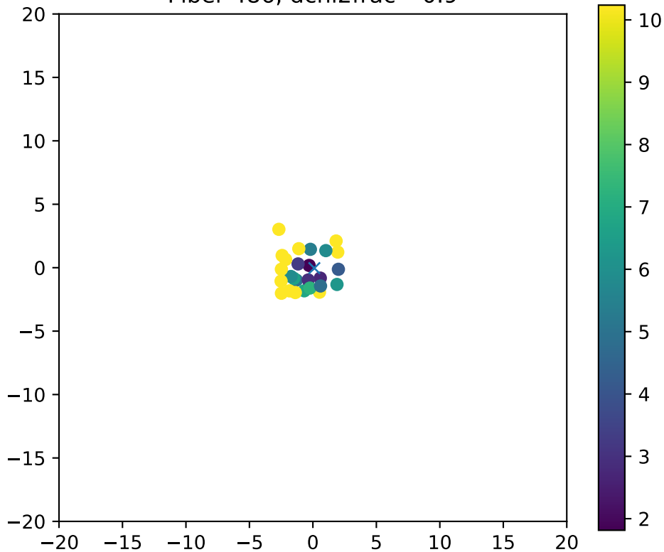
Fiber 486, dchi2frac= 0.9
