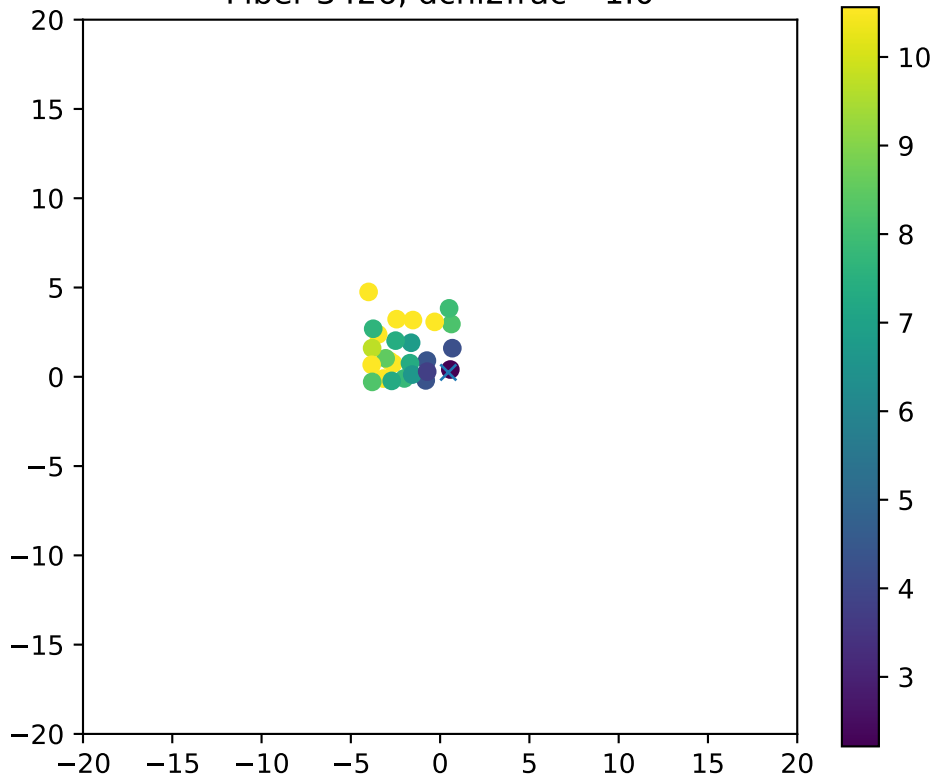
Fiber 3426, dchi2frac= 1.0
