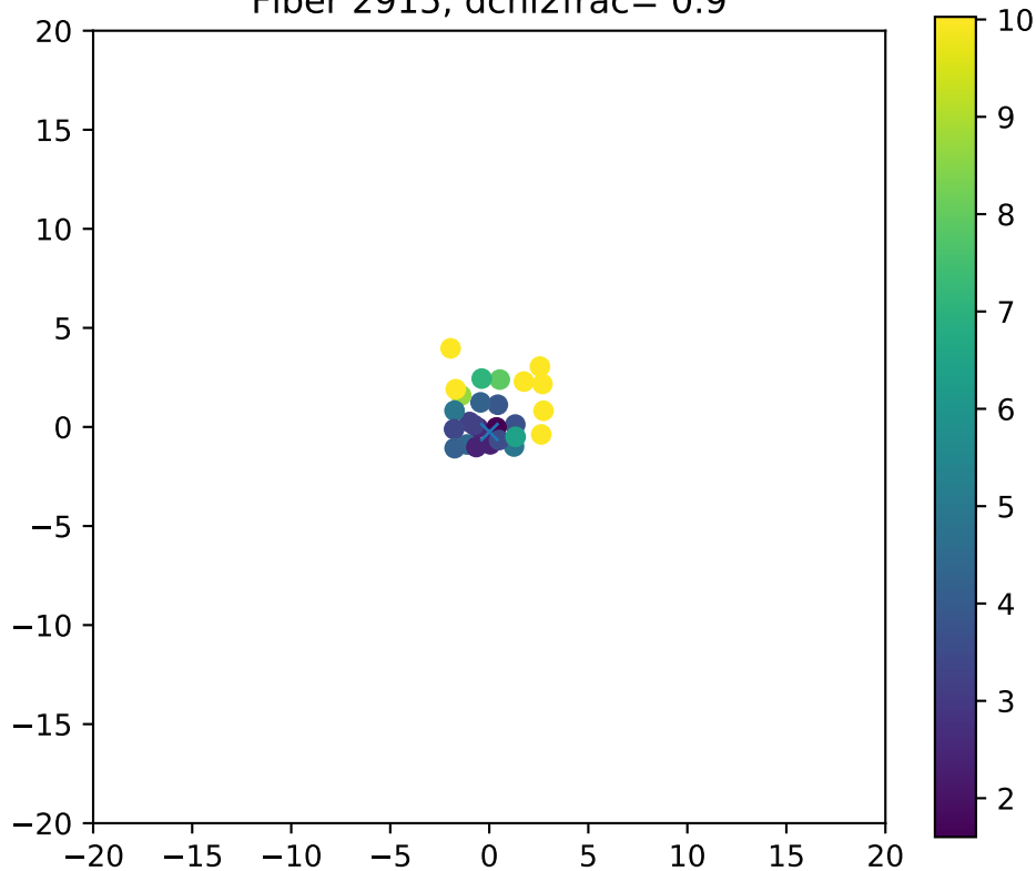
Fiber 2915, dchi2frac= 0.9
