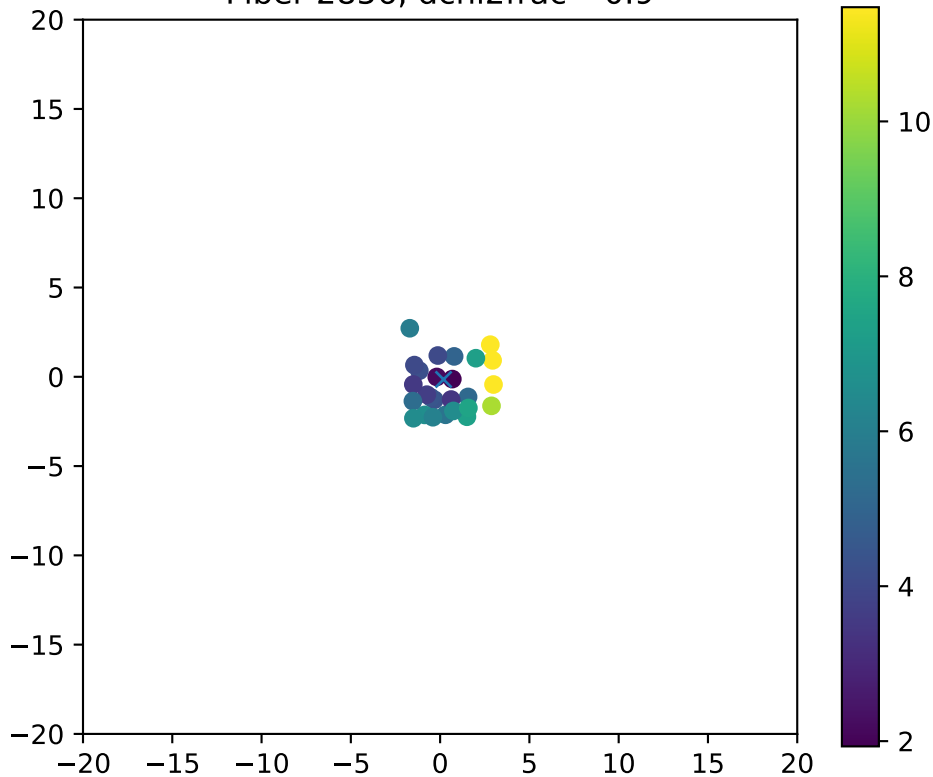
Fiber 2856, dchi2frac= 0.9
