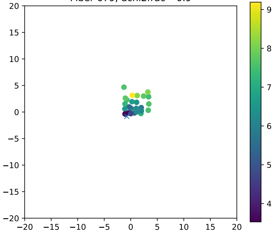
Fiber 679, dchi2frac= 0.9
