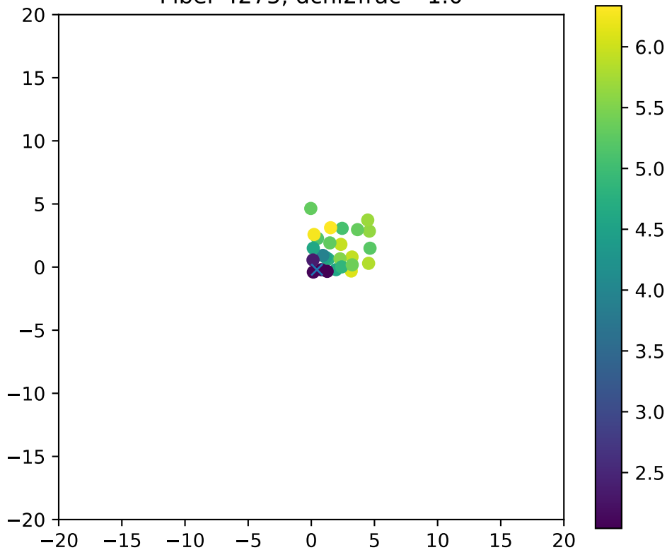
Fiber 4275, dchi2frac= 1.0
