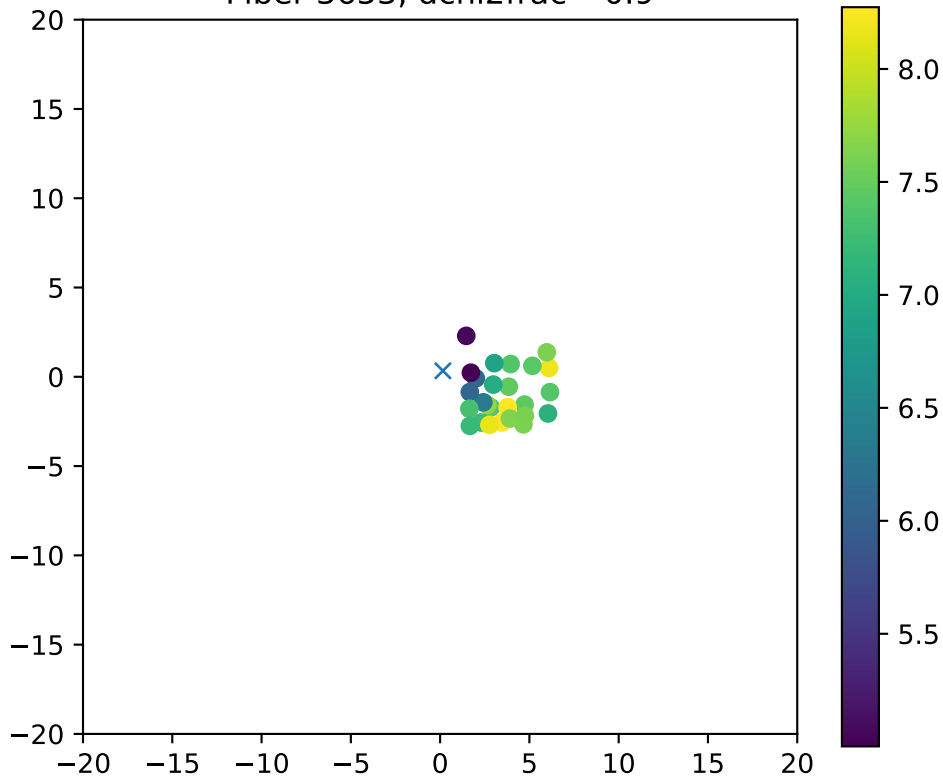
Fiber 3653, dchi2frac= 0.9
