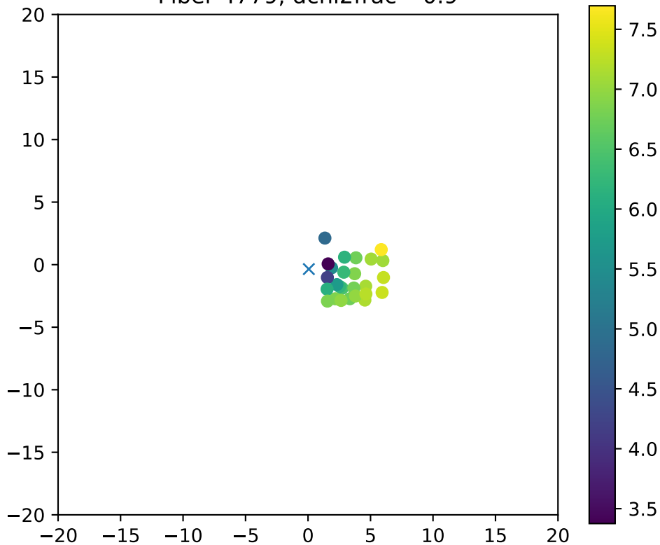
Fiber 4779, dchi2frac= 0.9
