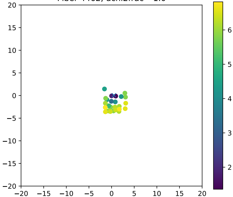
Fiber 4462, dchi2frac= 1.0
