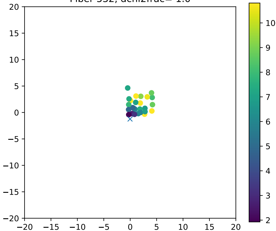
Fiber 532, dchi2frac= 1.0
