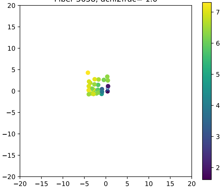
Fiber 3658, dchi2frac= 1.0
