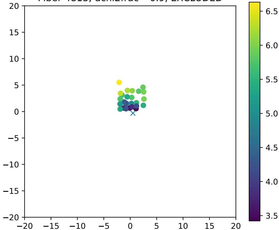
Fiber 4813, dchi2frac= 0.9, EXCLUDED
