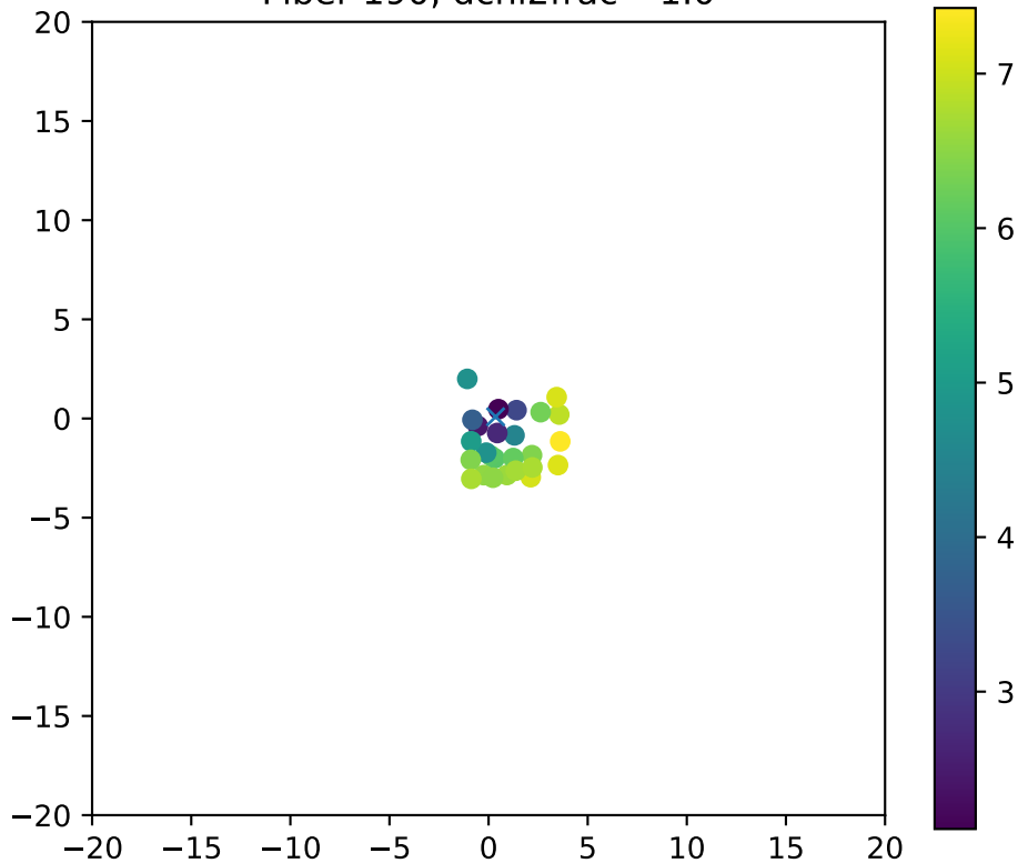
Fiber 190, dchi2frac= 1.0
