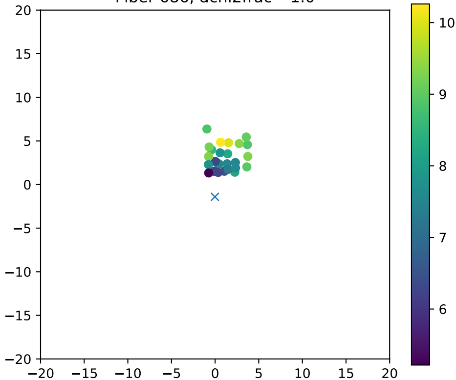
Fiber 686, dchi2frac= 1.0
