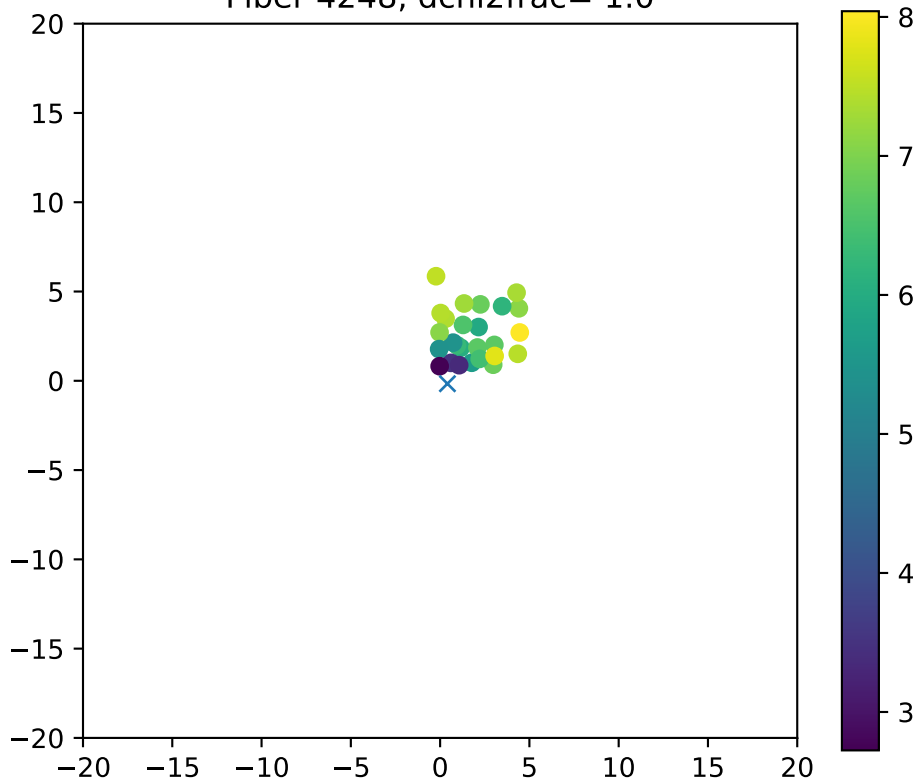
Fiber 4248, dchi2frac= 1.0
