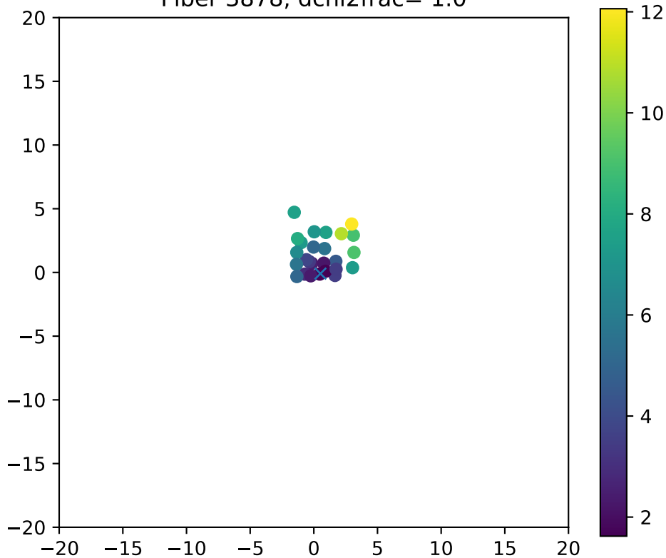
Fiber 3878, dchi2frac= 1.0
