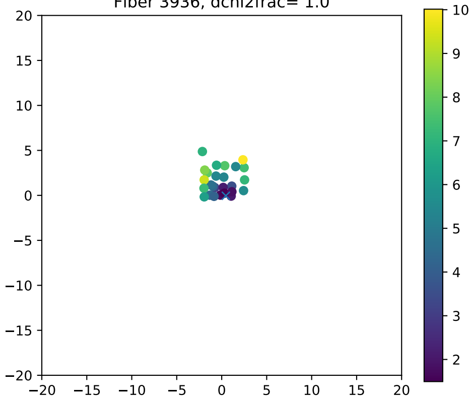
Fiber 3936, dchi2frac= 1.0
