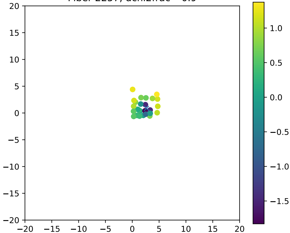
Fiber 2257, dchi2frac= 0.9
