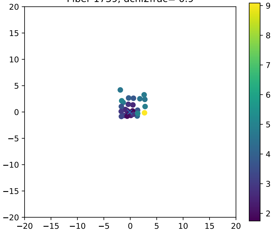
Fiber 1739, dchi2frac= 0.9
