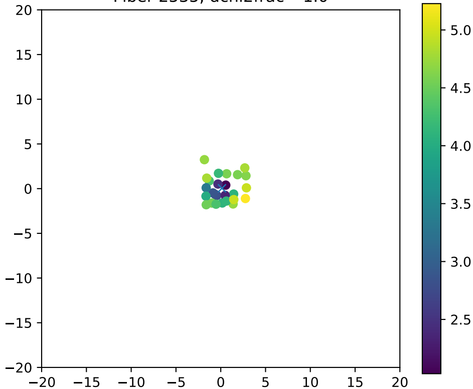
Fiber 2535, dchi2frac= 1.0
