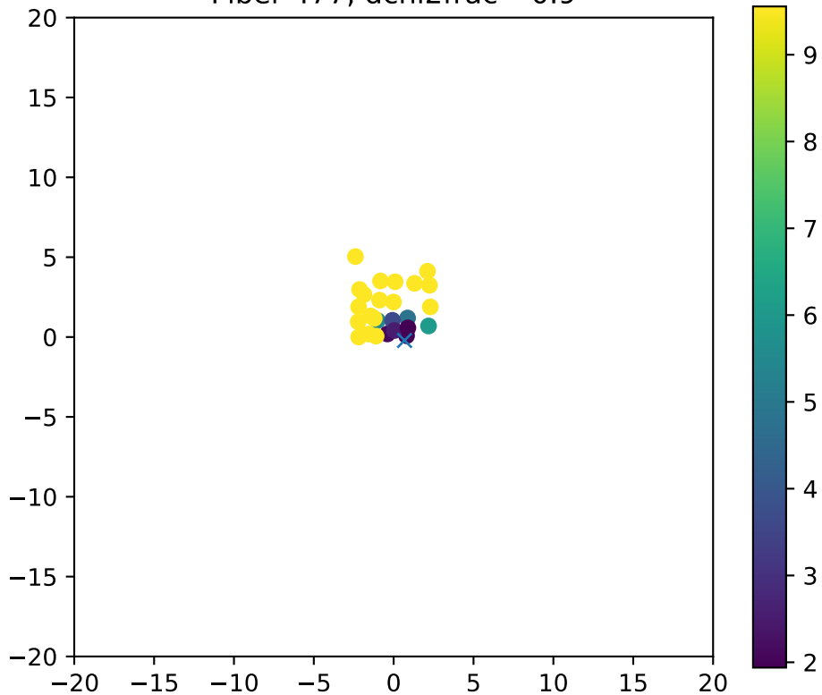
Fiber 477, dchi2frac= 0.9
