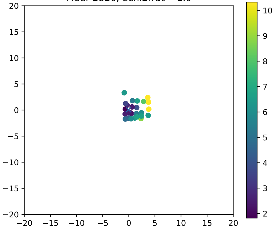
Fiber 2826, dchi2frac= 1.0
