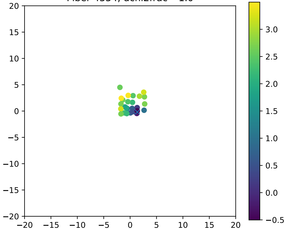
Fiber 4334, dchi2frac= 1.0
