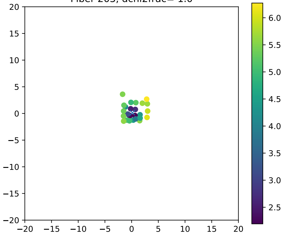
Fiber 203, dchi2frac= 1.0
