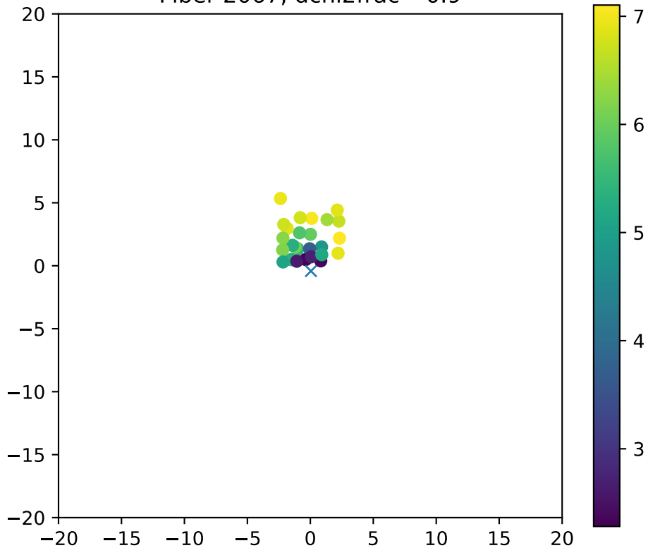
Fiber 2067, dchi2frac= 0.9
