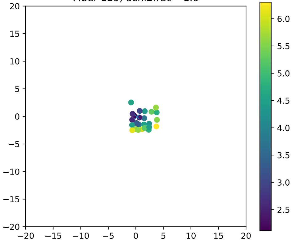
Fiber 129, dchi2frac= 1.0
