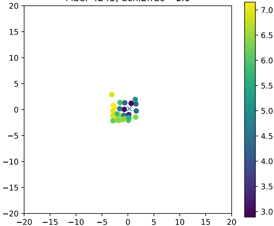
Fiber 4245, dchi2frac= 1.0
