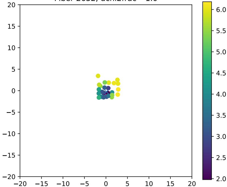
Fiber 2632, dchi2frac= 1.0
