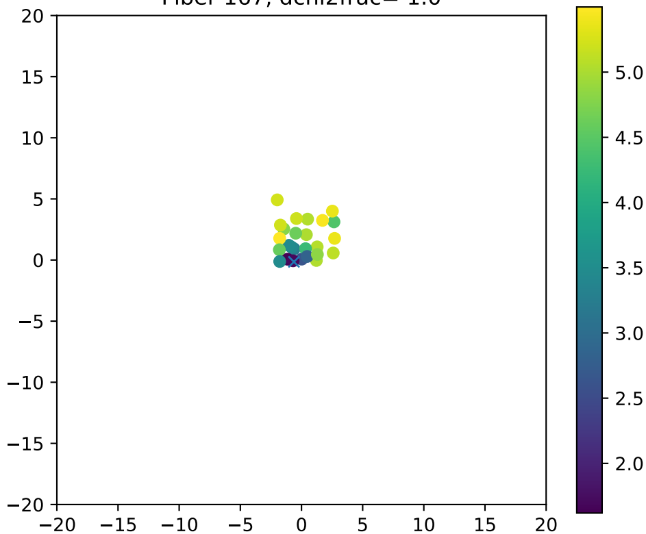
Fiber 167, dchi2frac= 1.0
