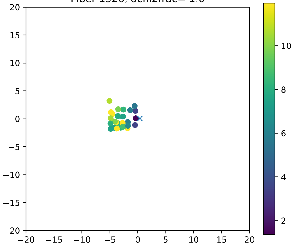
Fiber 1526, dchi2frac= 1.0
