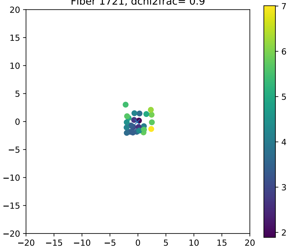
Fiber 1721, dchi2frac= 0.9
