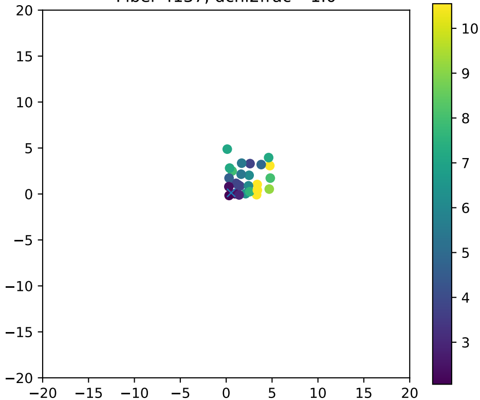
Fiber 4137, dchi2frac= 1.0
