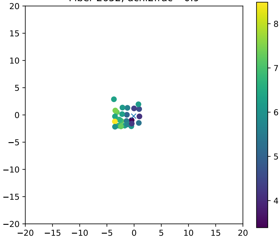
Fiber 2652, dchi2frac= 0.9
