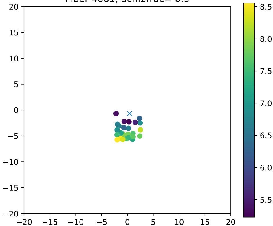
Fiber 4681, dchi2frac= 0.9
