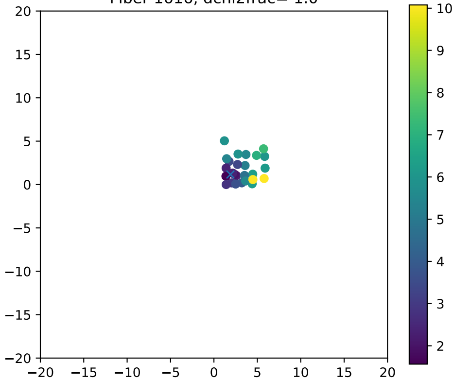
Fiber 1616, dchi2frac= 1.0
