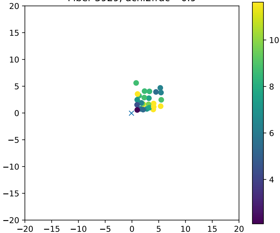
Fiber 3929, dchi2frac= 0.9
