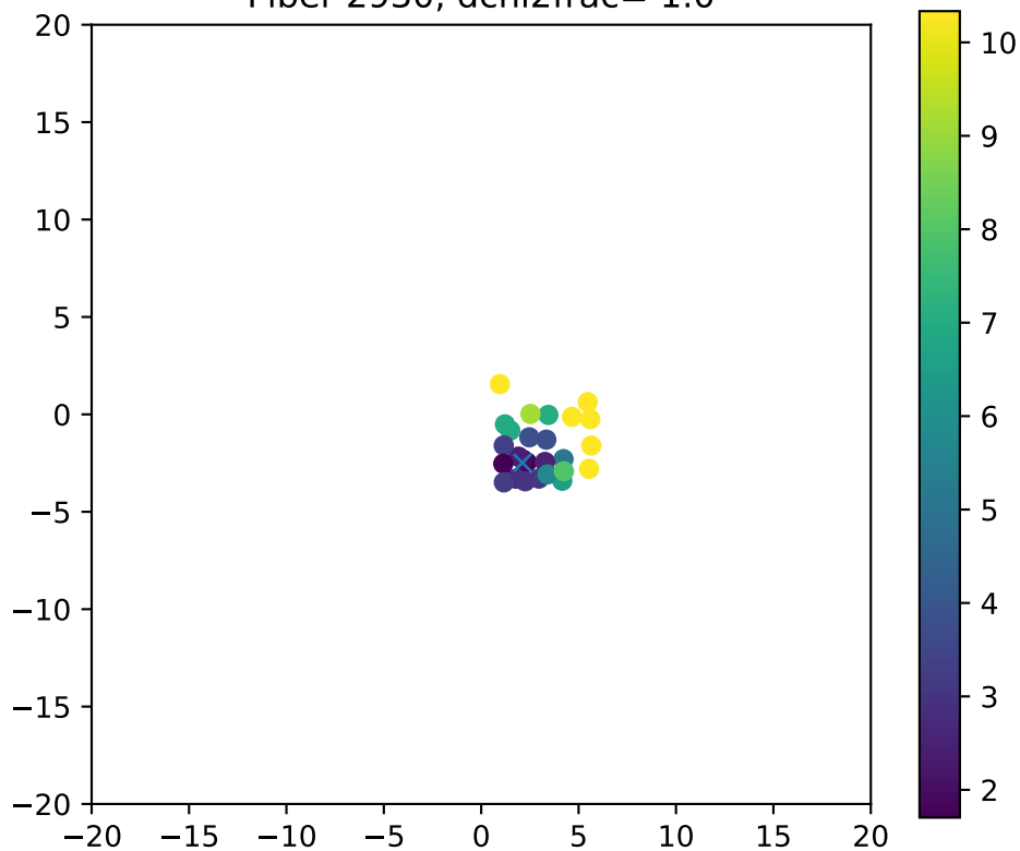
Fiber 2930, dchi2frac= 1.0
