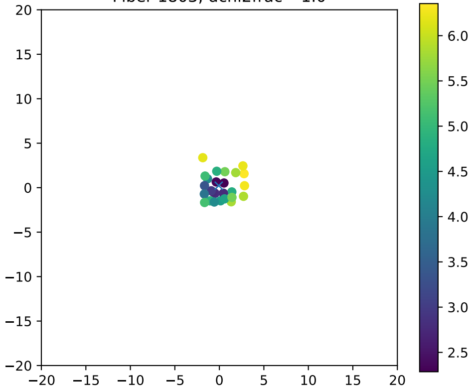
Fiber 1803, dchi2frac= 1.0
