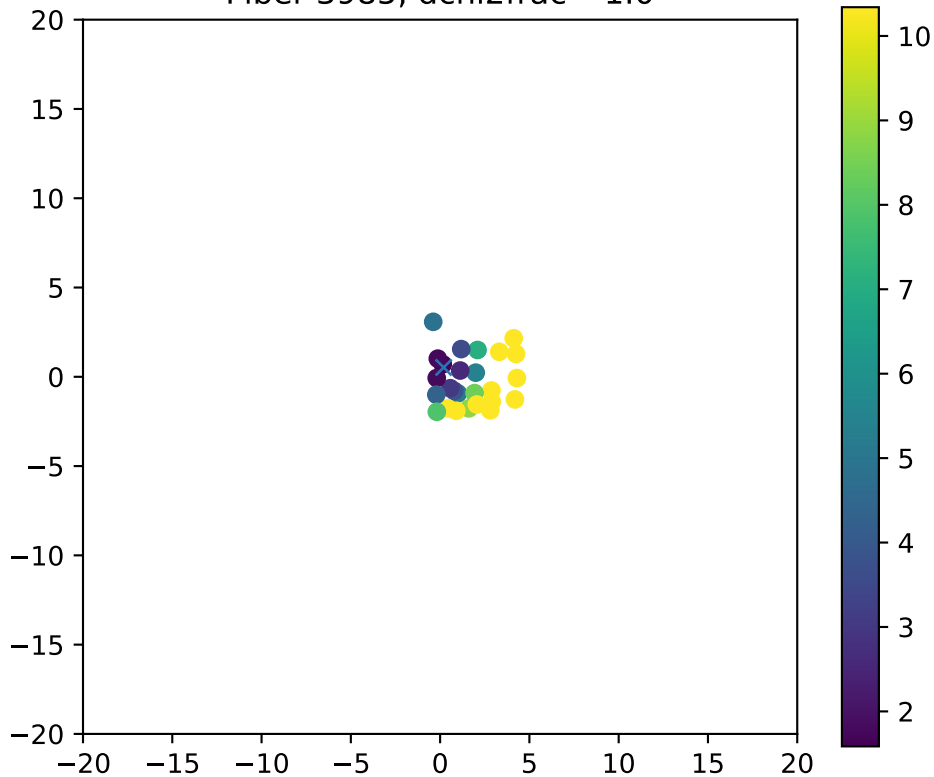
Fiber 3985, dchi2frac= 1.0
