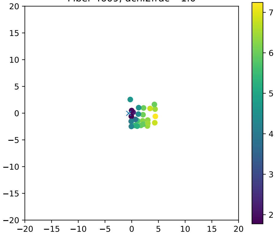
Fiber 4609, dchi2frac= 1.0
