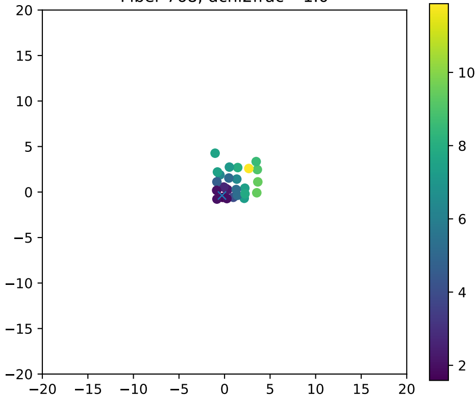
Fiber 768, dchi2frac= 1.0
