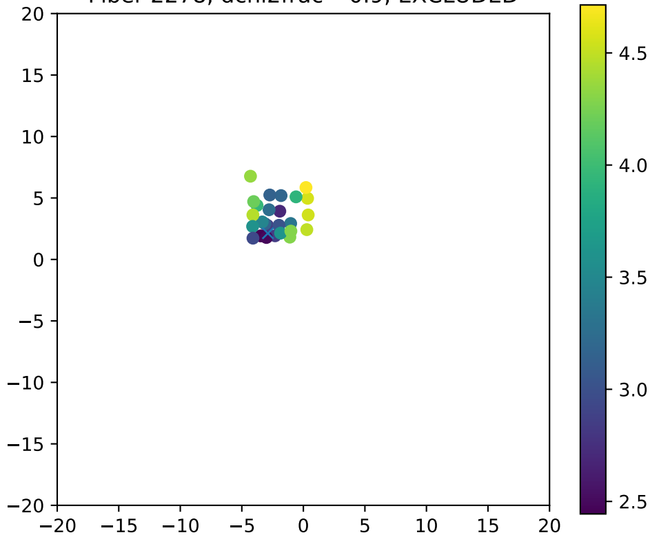
Fiber 2278, dchi2frac= 0.9, EXCLUDED
