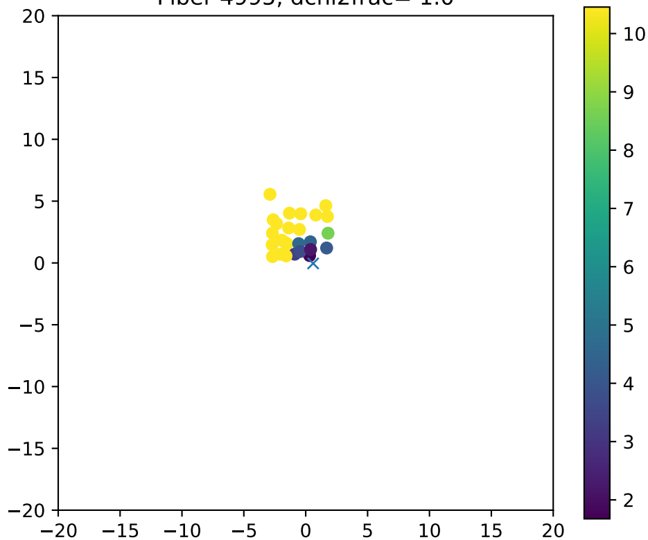
Fiber 4995, dchi2frac= 1.0
