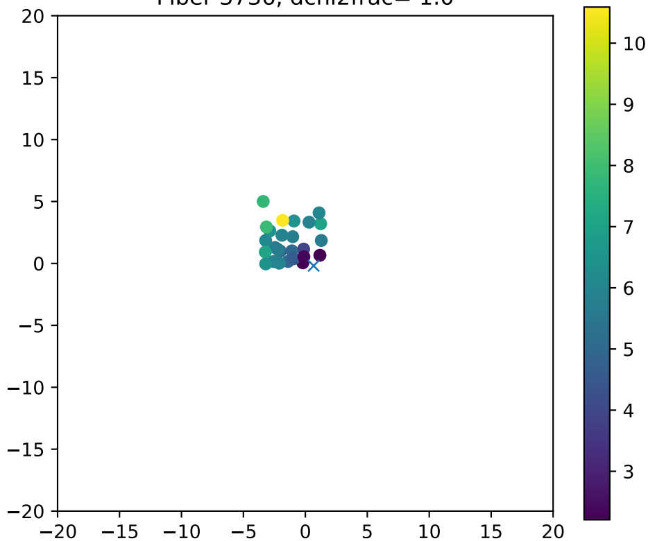
Fiber 3736, dchi2frac= 1.0
