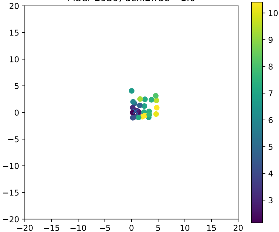
Fiber 2939, dchi2frac= 1.0
