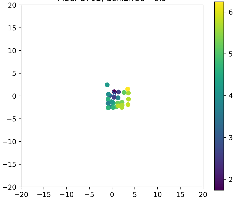
Fiber 3792, dchi2frac= 0.9
