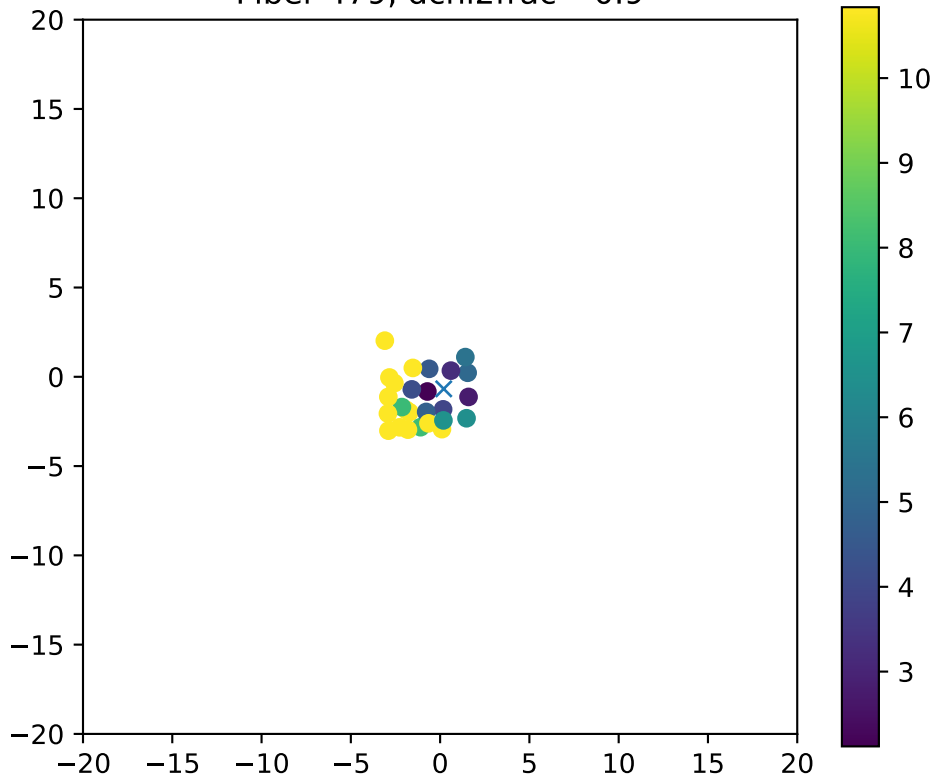
Fiber 479, dchi2frac= 0.9
