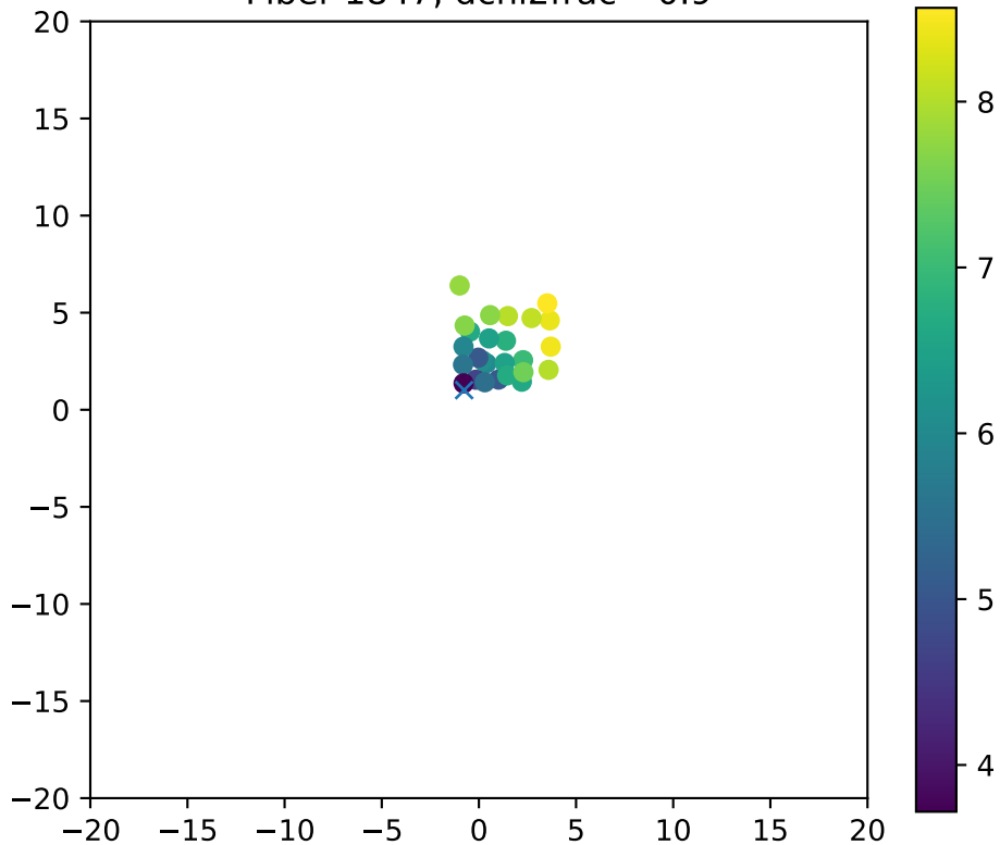
Fiber 1847, dchi2frac= 0.9
