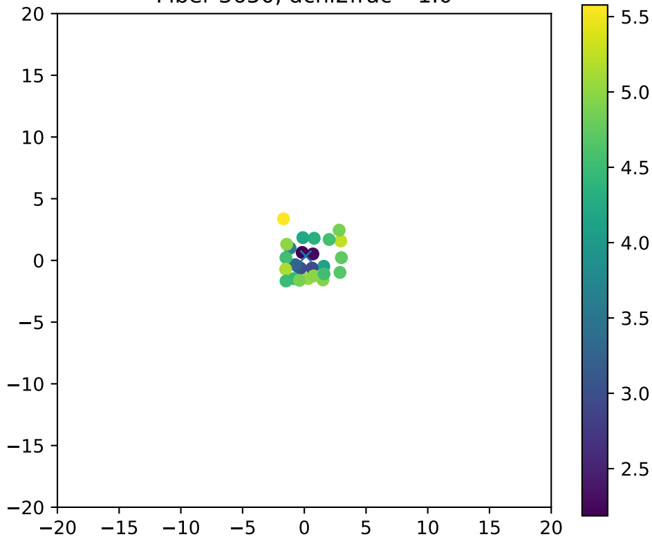
Fiber 3650, dchi2frac= 1.0
