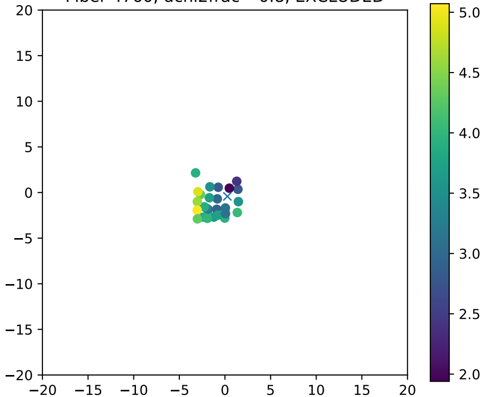
Fiber 4760, dchi2frac= 0.8, EXCLUDED
