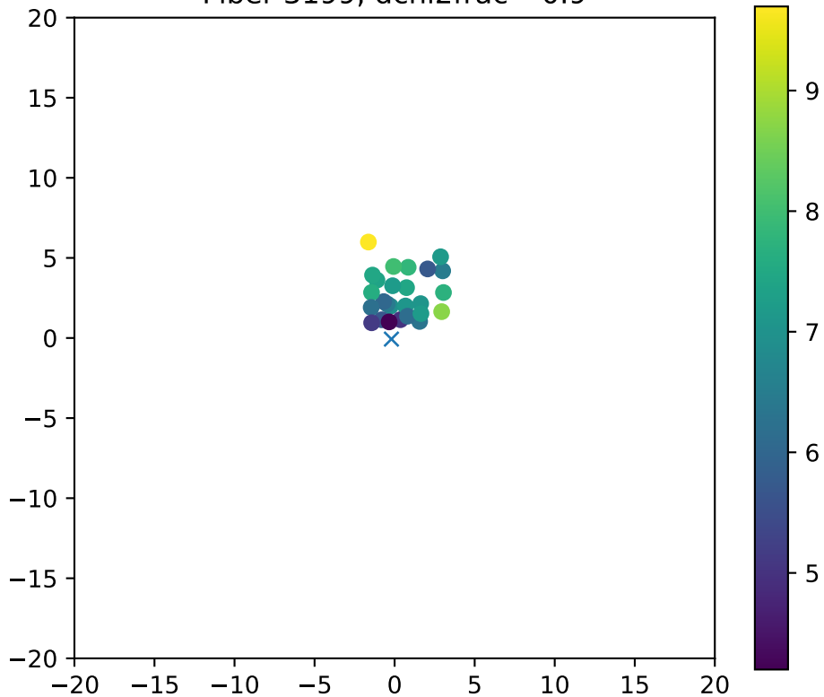
Fiber 3199, dchi2frac= 0.9
