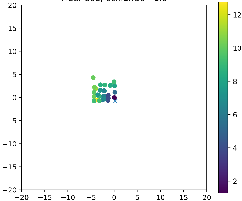
Fiber 886, dchi2frac= 1.0
