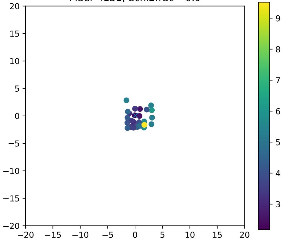
Fiber 4131, dchi2frac= 0.9
