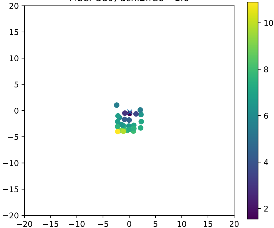
Fiber 389, dchi2frac= 1.0
