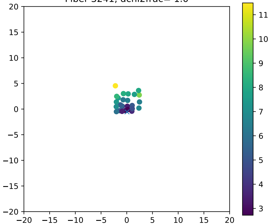
Fiber 3241, dchi2frac= 1.0
