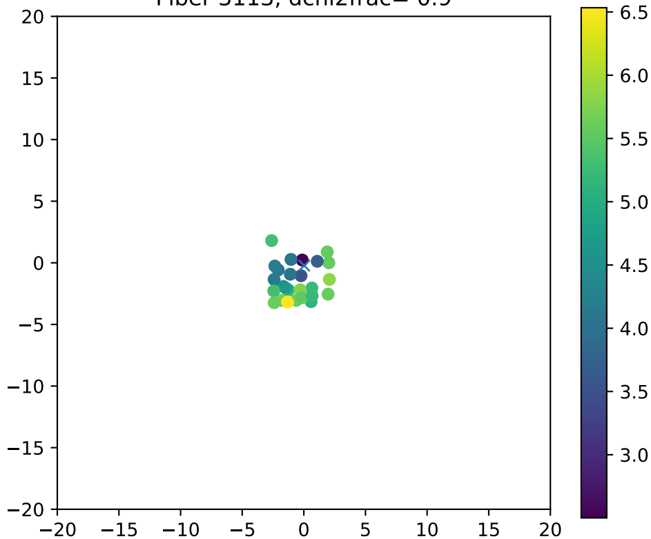
Fiber 3113, dchi2frac= 0.9
