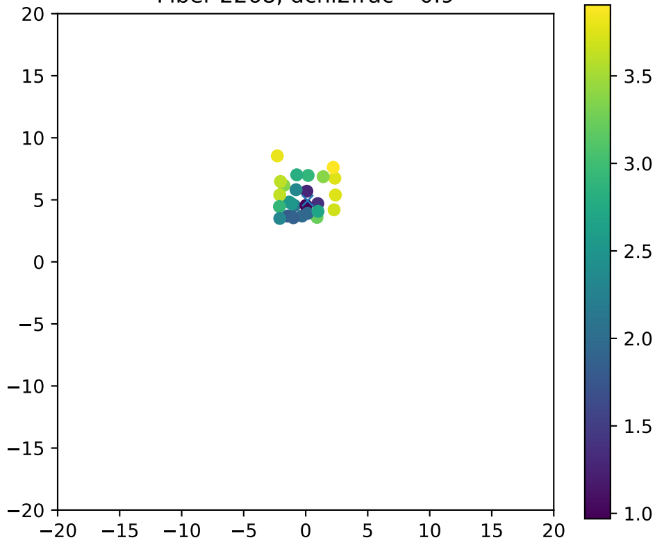
Fiber 2268, dchi2frac= 0.9
