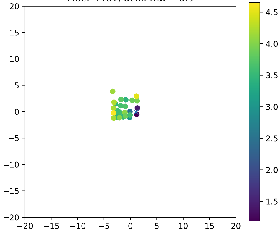
Fiber 4461, dchi2frac= 0.9
