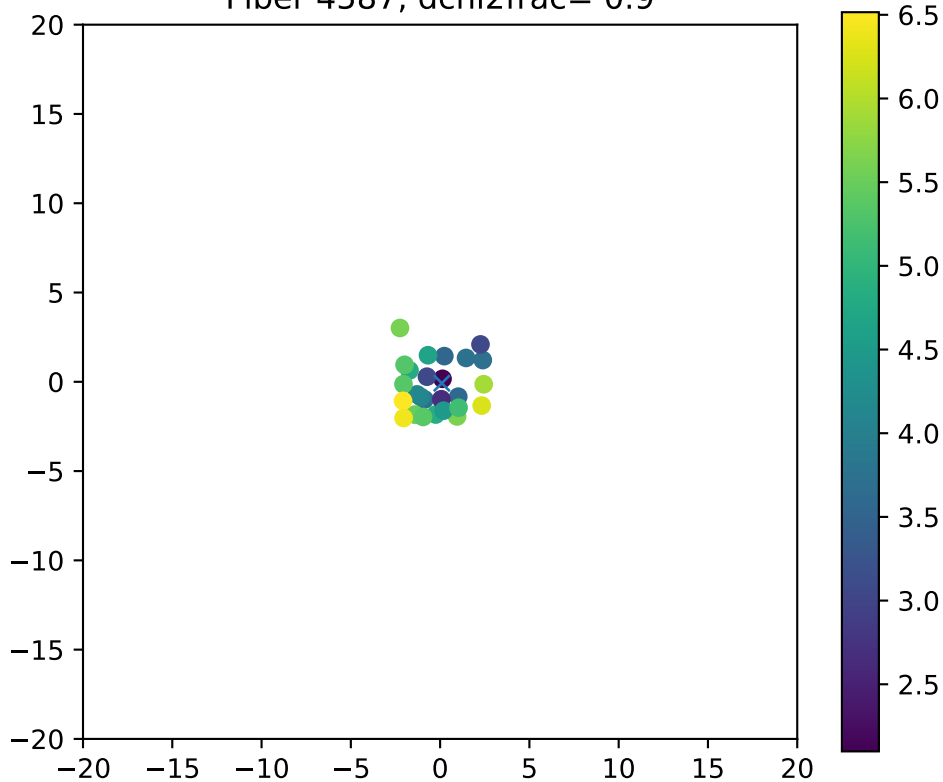
Fiber 4587, dchi2frac= 0.9
