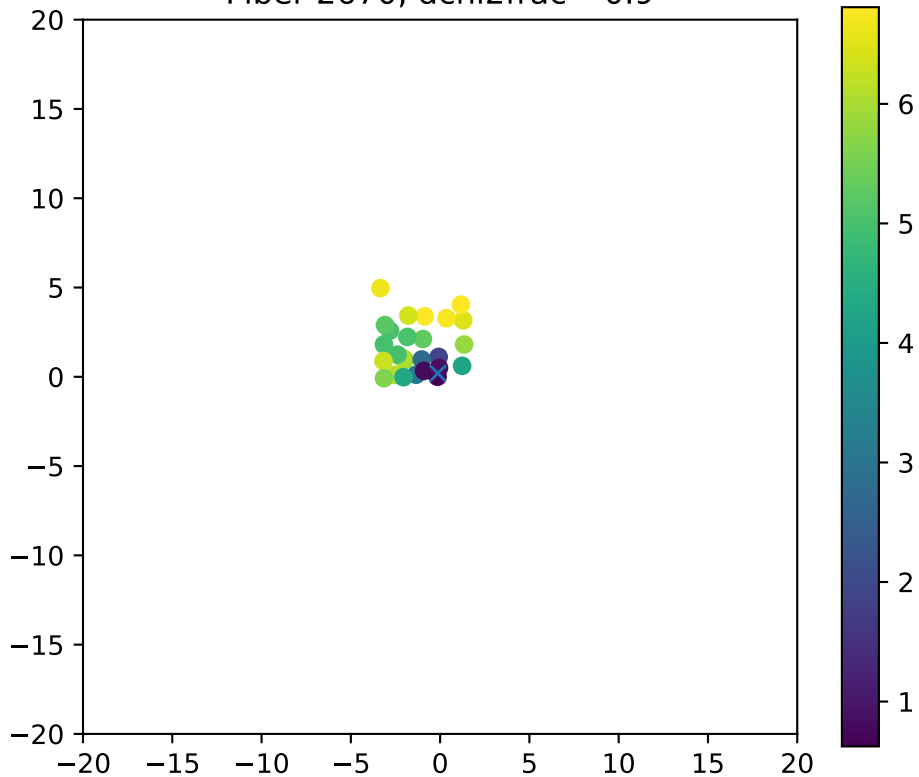
Fiber 2670, dchi2frac= 0.9
