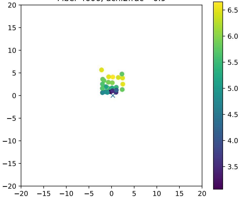
Fiber 4606, dchi2frac= 0.9
