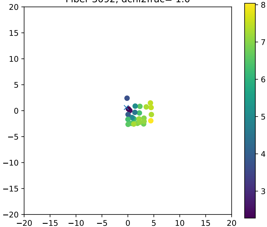
Fiber 3092, dchi2frac= 1.0
