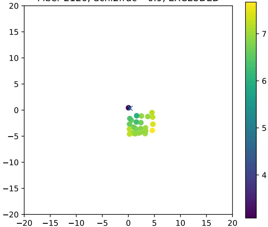
Fiber 2120, dchi2frac= 0.9, EXCLUDED
