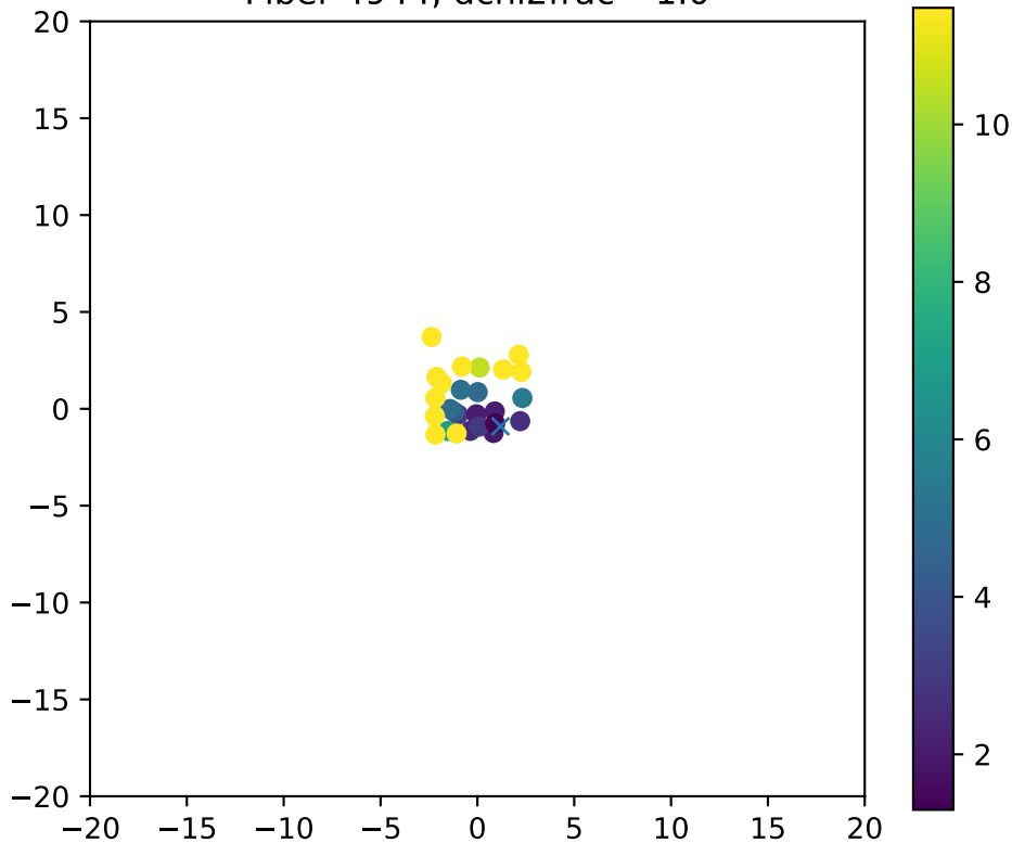
Fiber 4944, dchi2frac= 1.0
