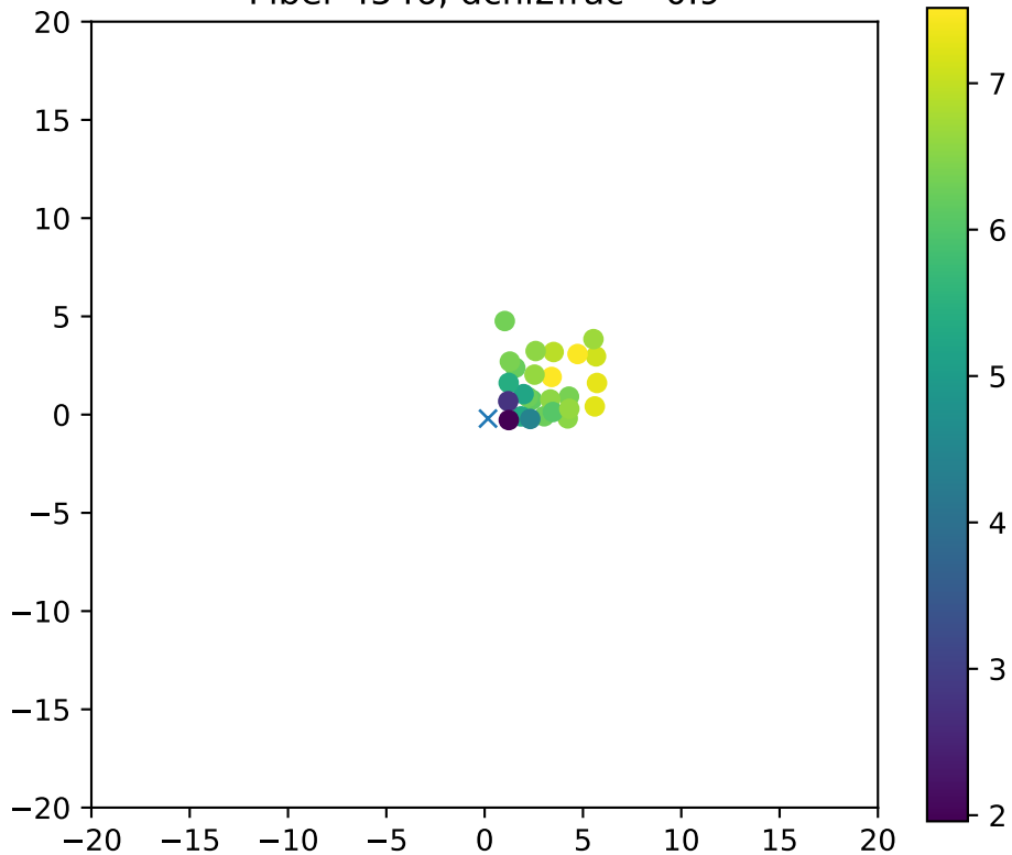
Fiber 4546, dchi2frac= 0.9
