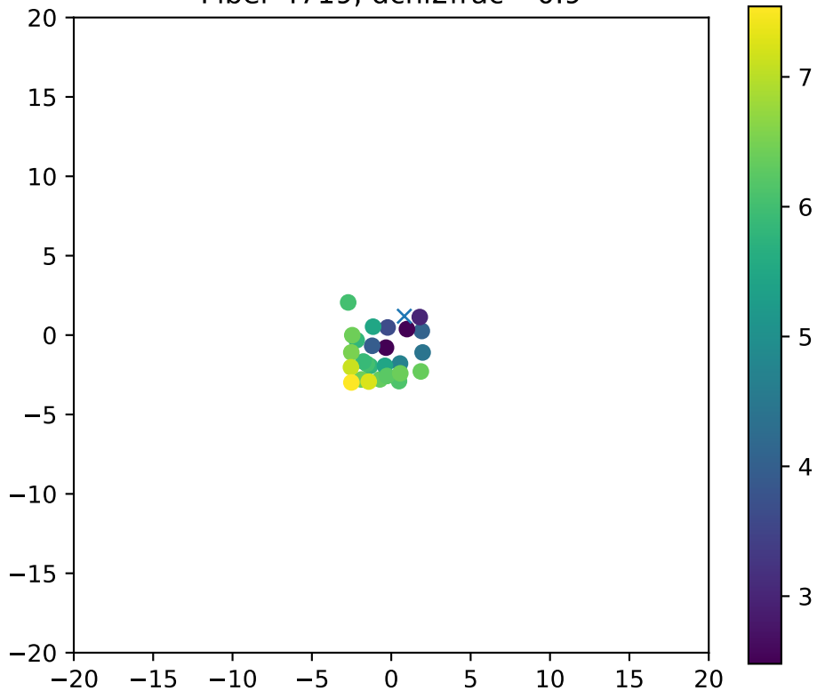
Fiber 4719, dchi2frac= 0.9
