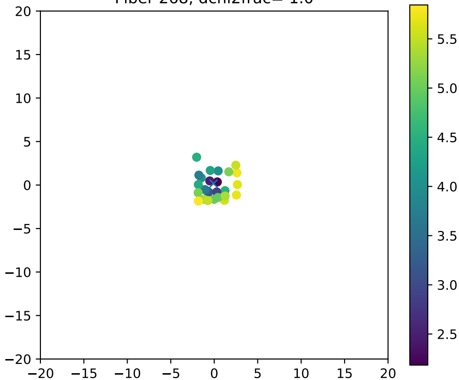
Fiber 268, dchi2frac= 1.0
