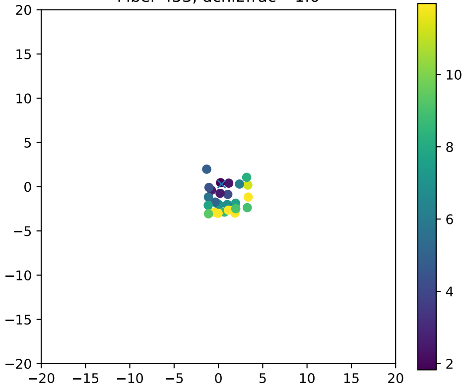
Fiber 453, dchi2frac= 1.0
