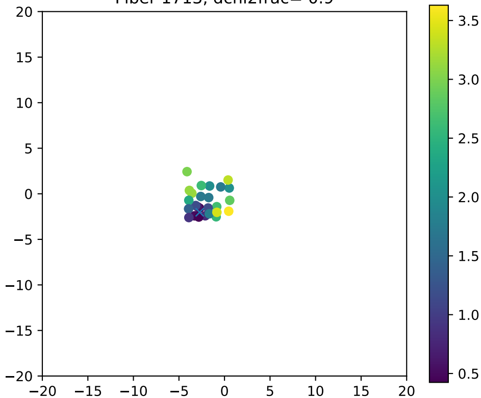
Fiber 1713, dchi2frac= 0.9
