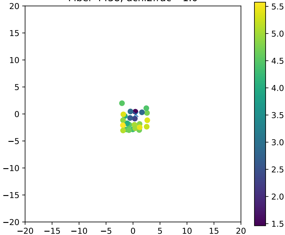
Fiber 4438, dchi2frac= 1.0
