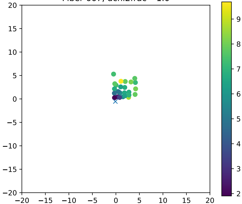
Fiber 667, dchi2frac= 1.0
