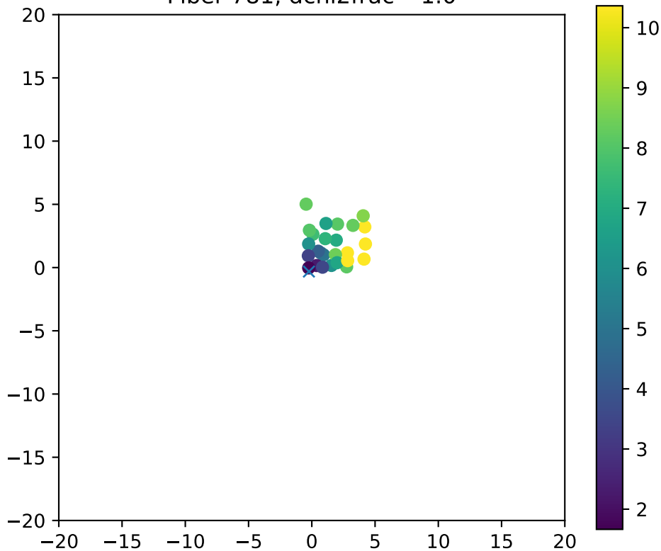
Fiber 781, dchi2frac= 1.0
