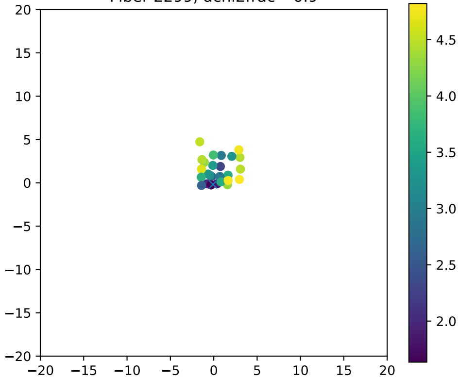
Fiber 2299, dchi2frac= 0.9
