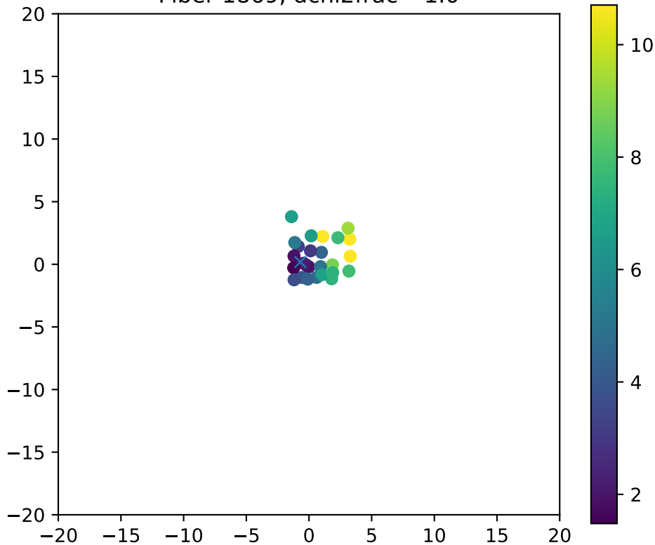
Fiber 1869, dchi2frac= 1.0
