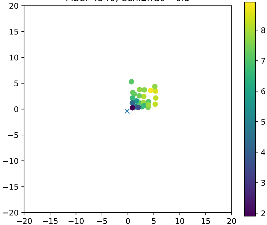
Fiber 4540, dchi2frac= 0.9
