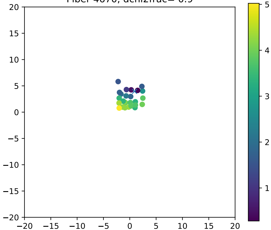
Fiber 4670, dchi2frac= 0.9
