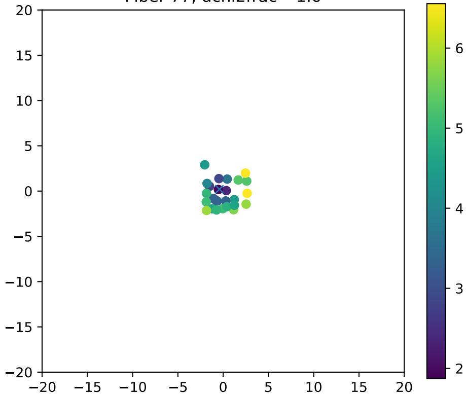
Fiber 77, dchi2frac= 1.0
