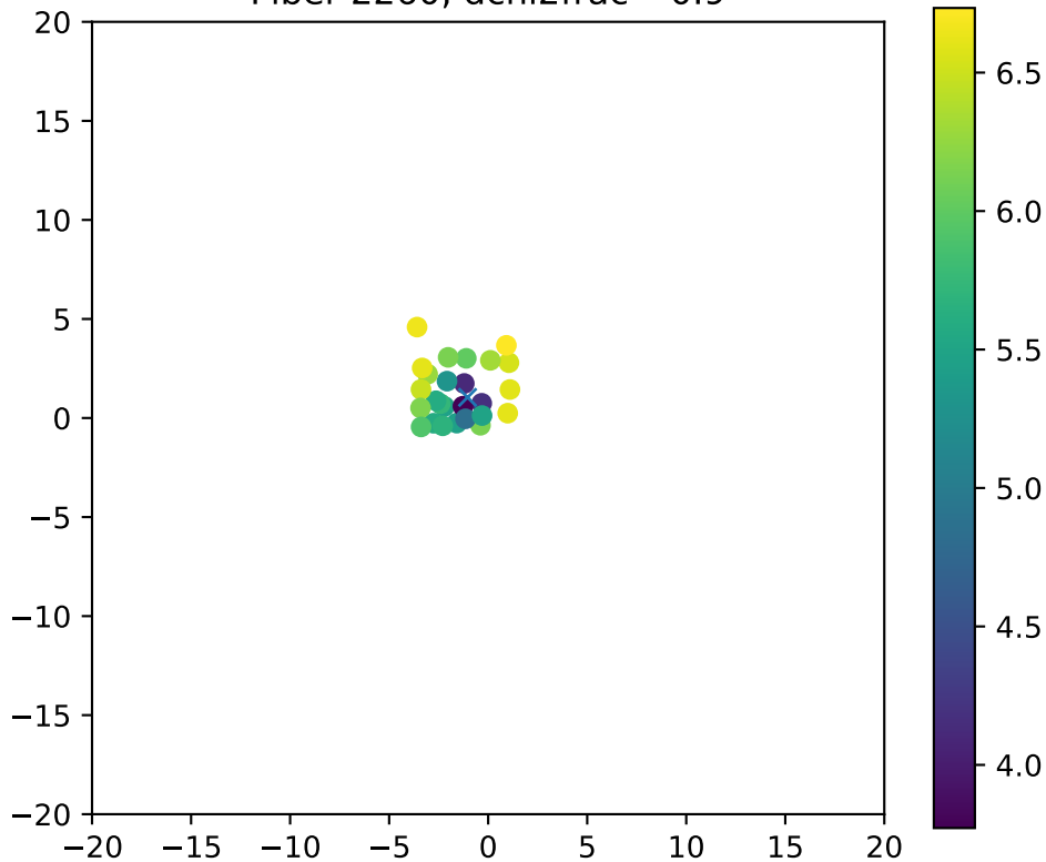
Fiber 2260, dchi2frac= 0.9
