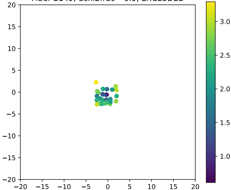
Fiber 2149, dchi2frac= 0.9, EXCLUDED
