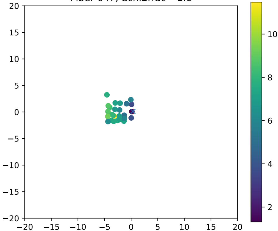
Fiber 647, dchi2frac= 1.0
