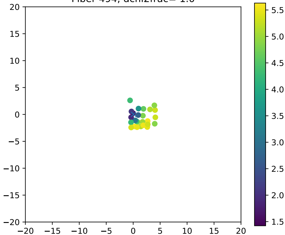
Fiber 494, dchi2frac= 1.0
