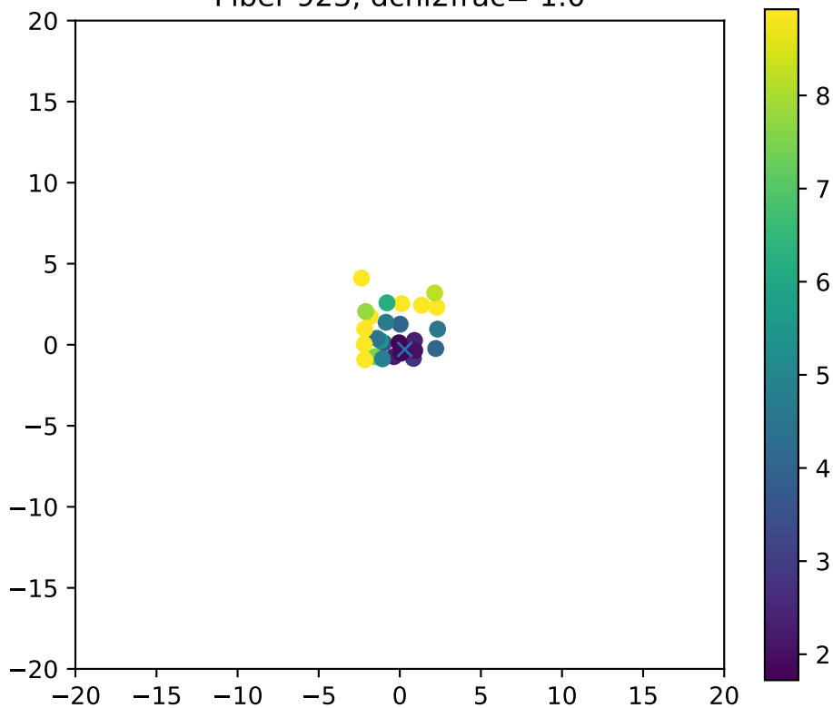
Fiber 923, dchi2frac= 1.0
