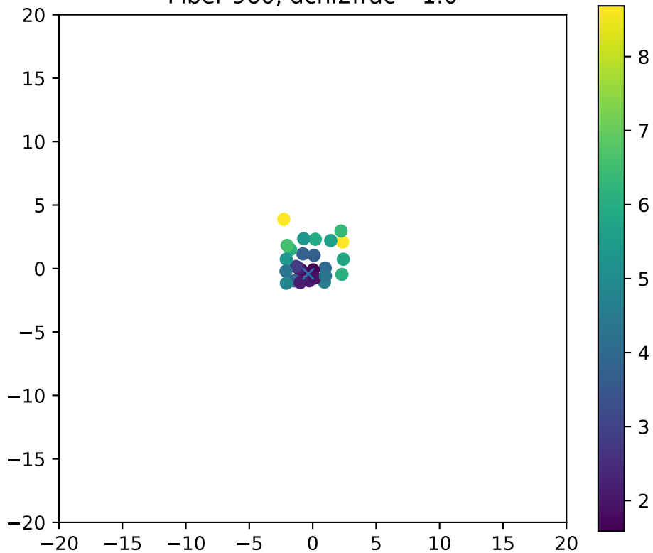
Fiber 960, dchi2frac= 1.0
