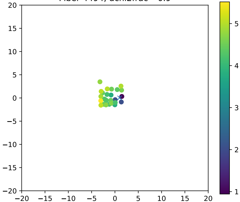
Fiber 4494, dchi2frac= 0.9
