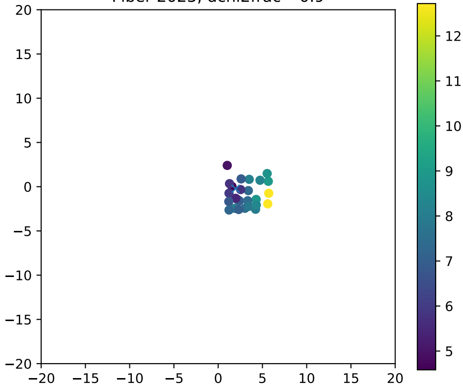
Fiber 2023, dchi2frac= 0.9
