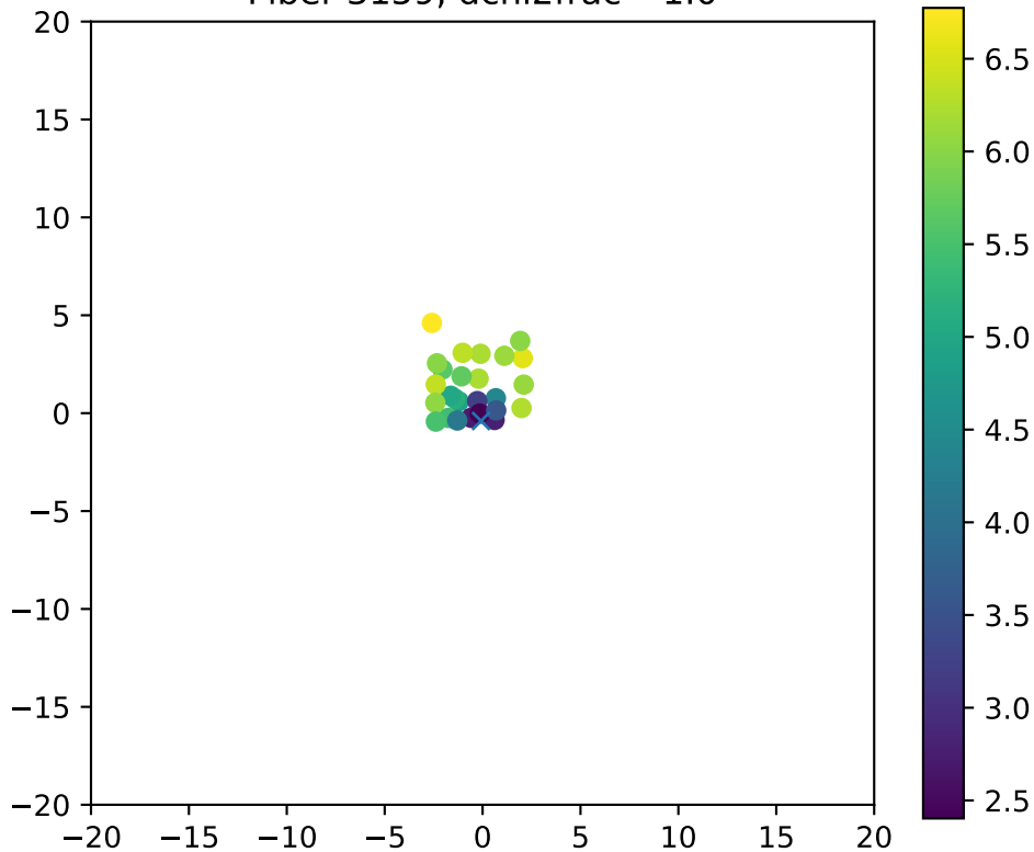
Fiber 3159, dchi2frac= 1.0
