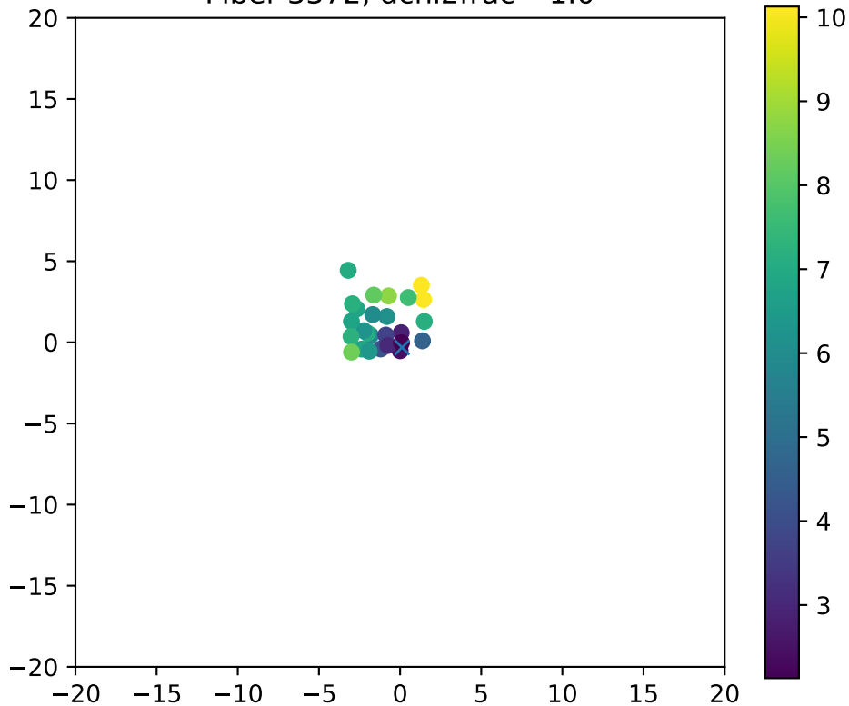
Fiber 3372, dchi2frac= 1.0
