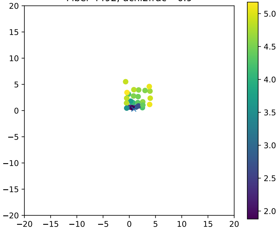
Fiber 4492, dchi2frac= 0.9
