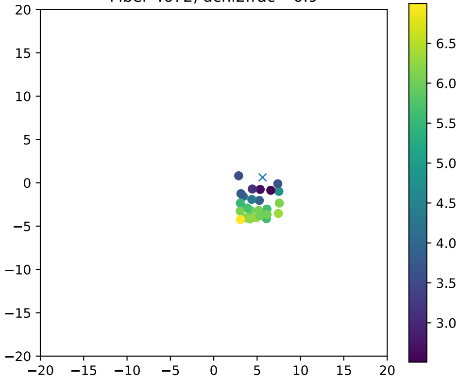
Fiber 4672, dchi2frac= 0.9
