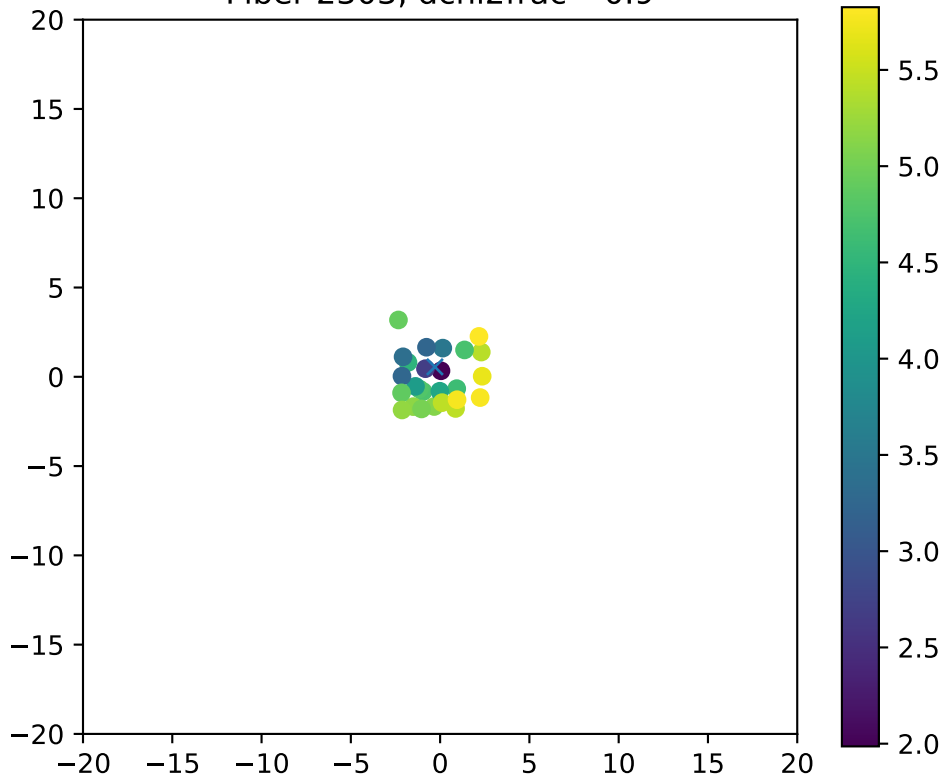
Fiber 2303, dchi2frac= 0.9
