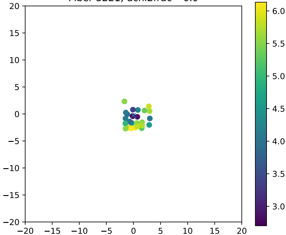
Fiber 3221, dchi2frac= 0.9
