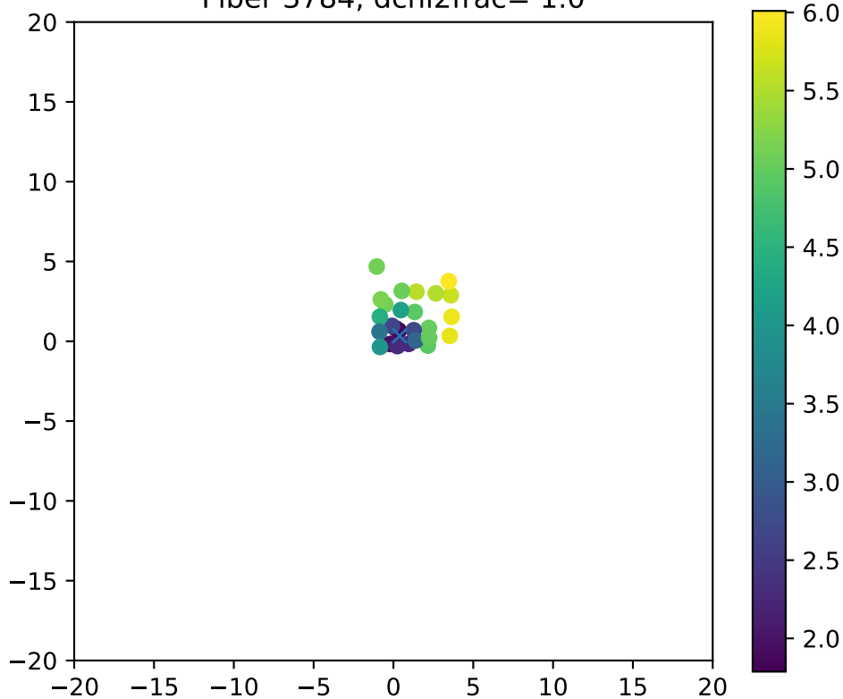
Fiber 3784, dchi2frac= 1.0
