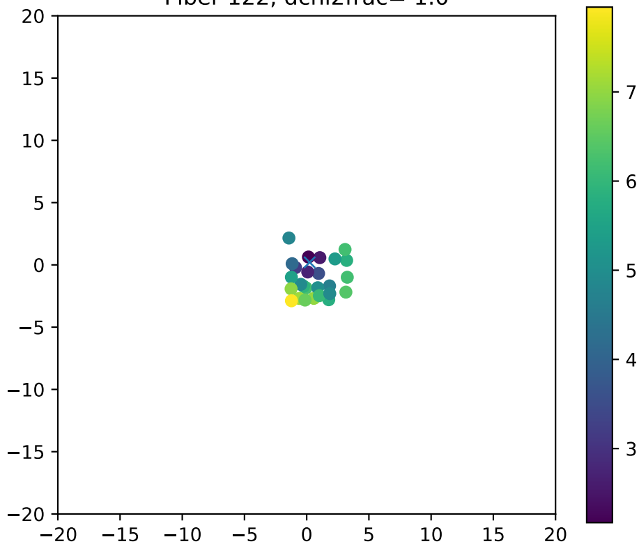
Fiber 122, dchi2frac= 1.0
