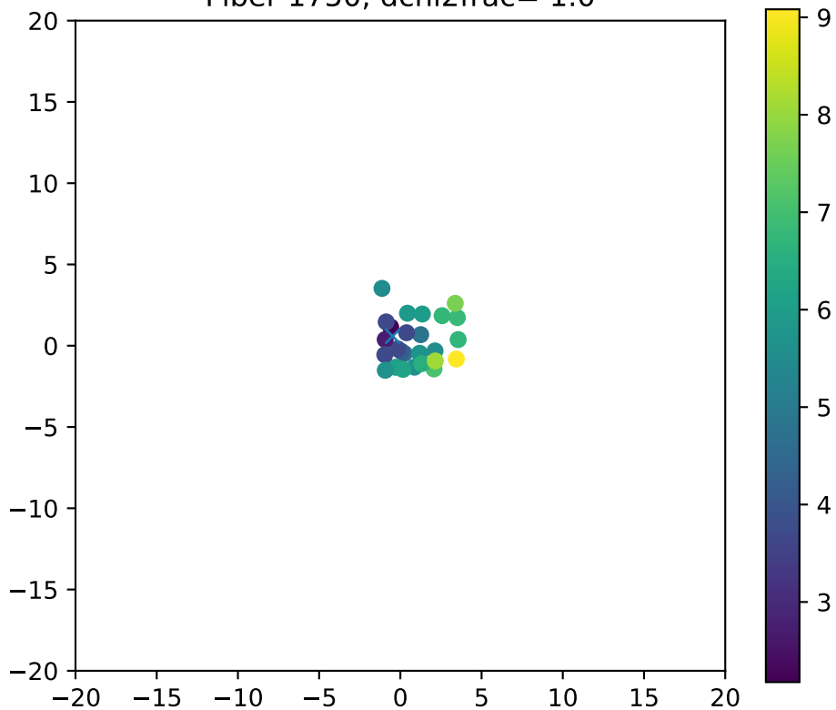
Fiber 1750, dchi2frac= 1.0
