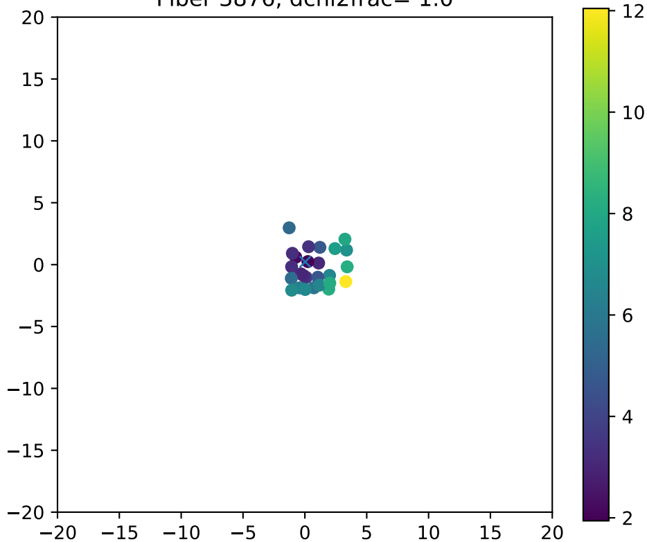
Fiber 3876, dchi2frac= 1.0
