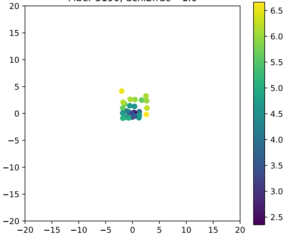
Fiber 3190, dchi2frac= 1.0
