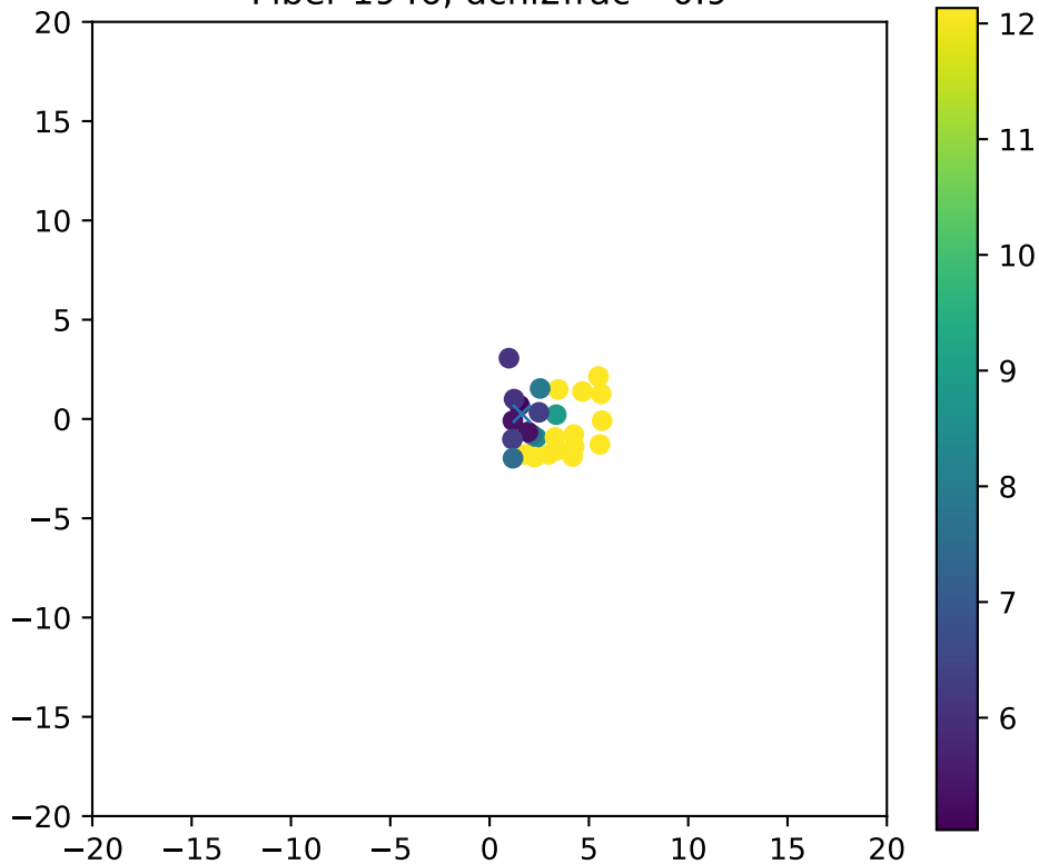
Fiber 1946, dchi2frac= 0.9
