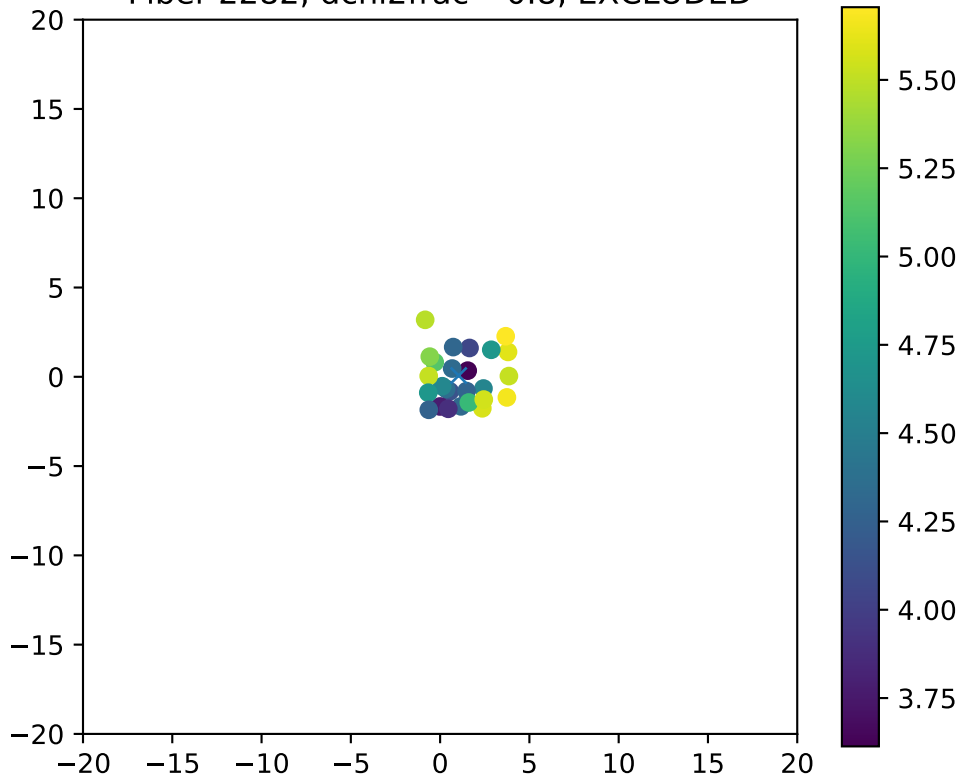
Fiber 2282, dchi2frac= 0.8, EXCLUDED
