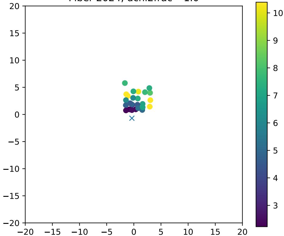
Fiber 2024, dchi2frac= 1.0
