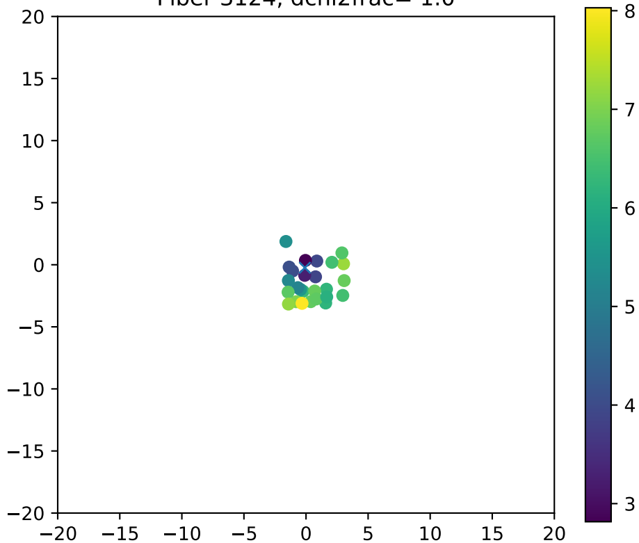
Fiber 3124, dchi2frac= 1.0
