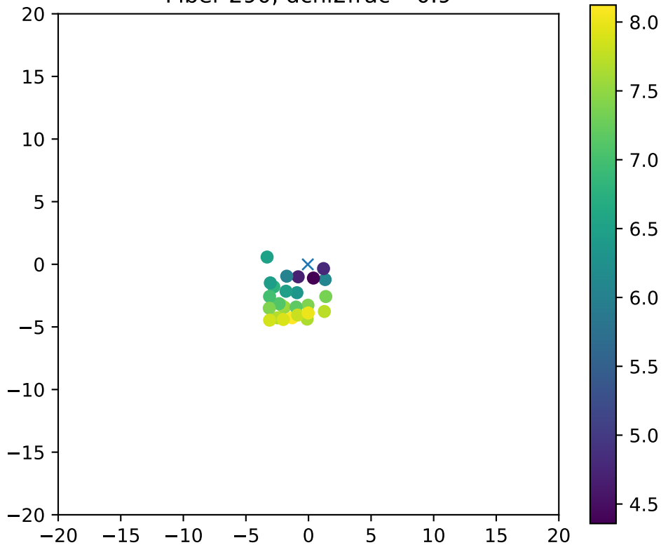
Fiber 290, dchi2frac= 0.9
