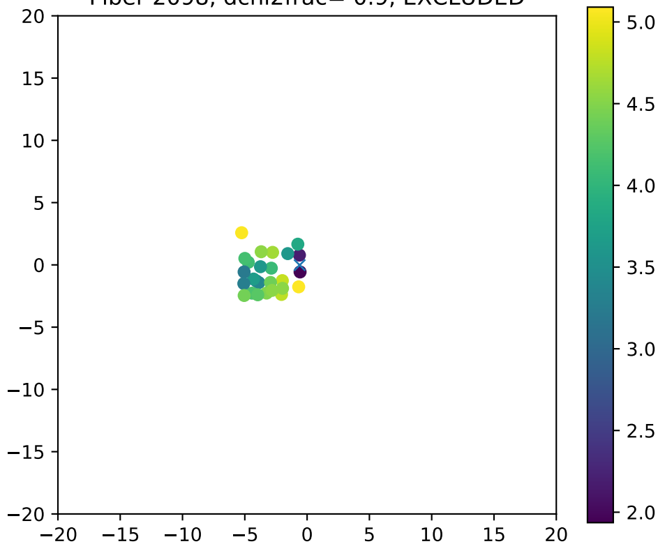
Fiber 2098, dchi2frac= 0.9, EXCLUDED
