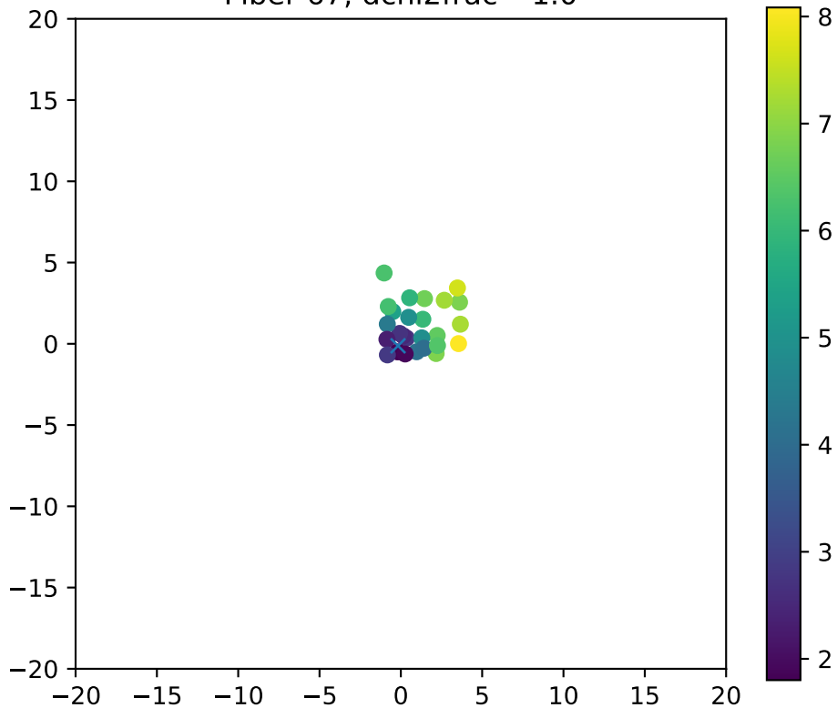
Fiber 67, dchi2frac= 1.0
