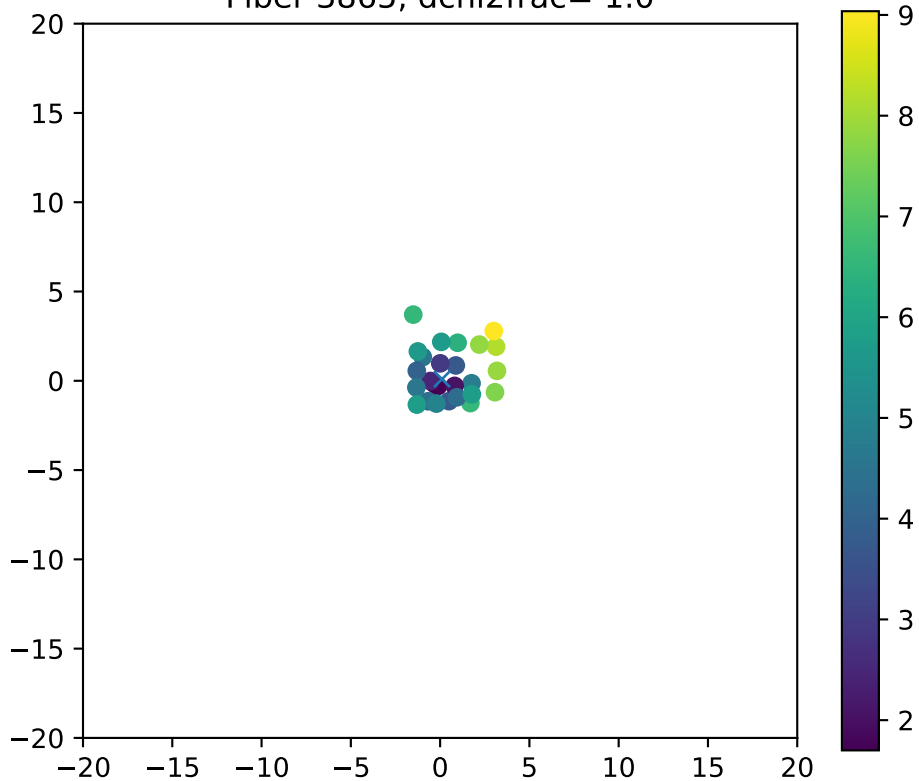
Fiber 3865, dchi2frac= 1.0
