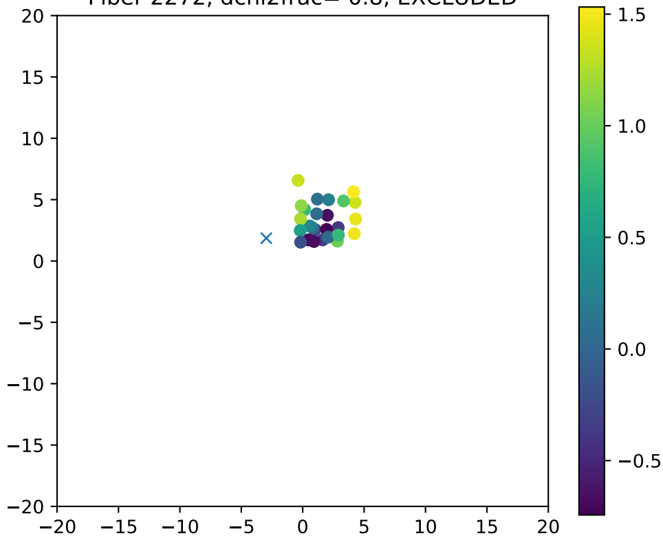
Fiber 2272, dchi2frac= 0.8, EXCLUDED
