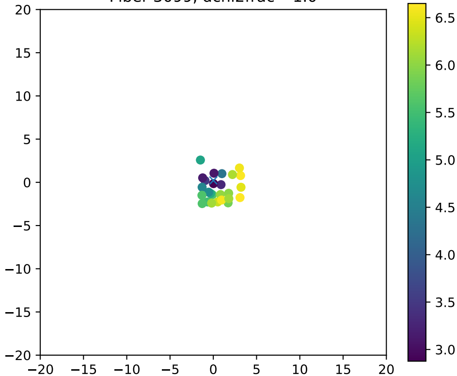
Fiber 3099, dchi2frac= 1.0
