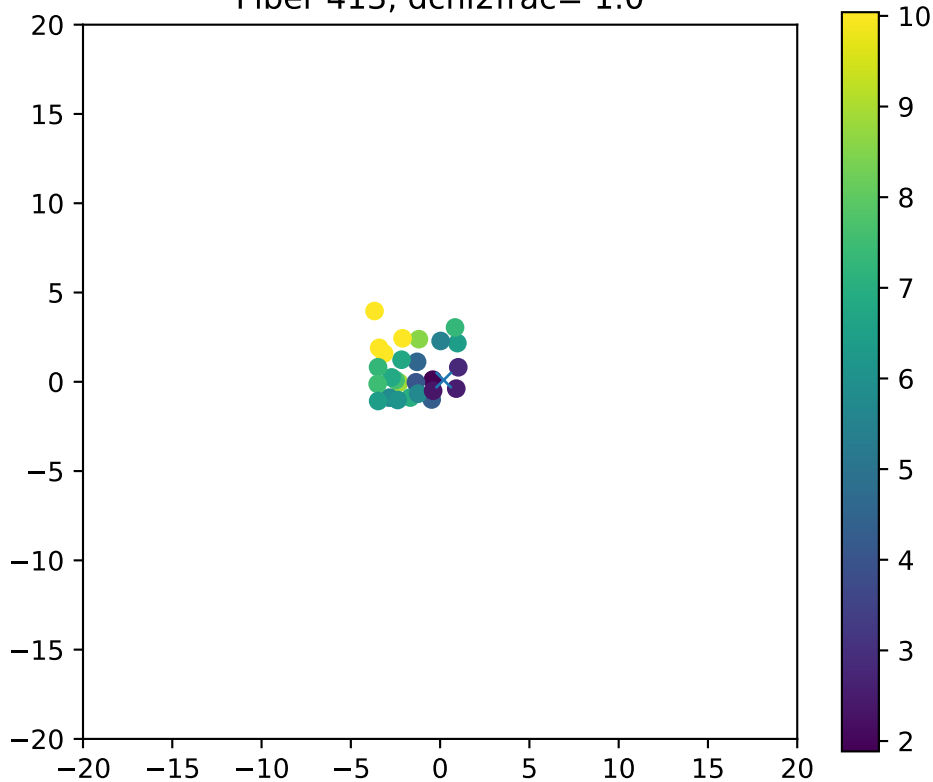
Fiber 413, dchi2frac= 1.0
