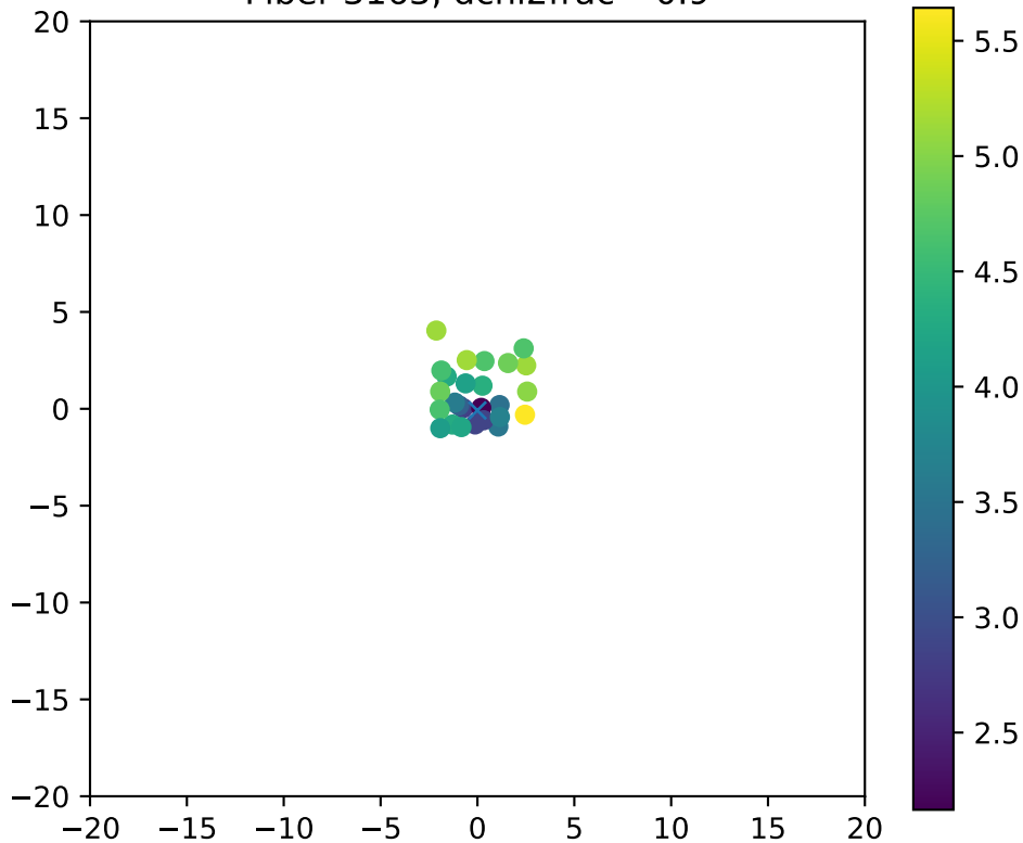
Fiber 3163, dchi2frac= 0.9
