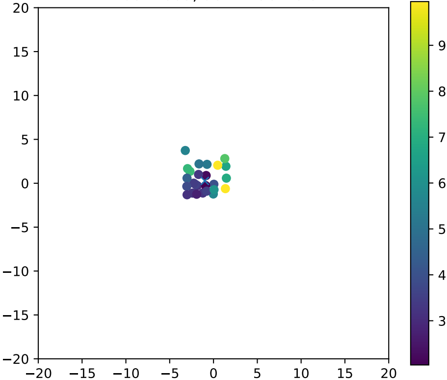
Fiber 1605, dchi2frac= 0.9
