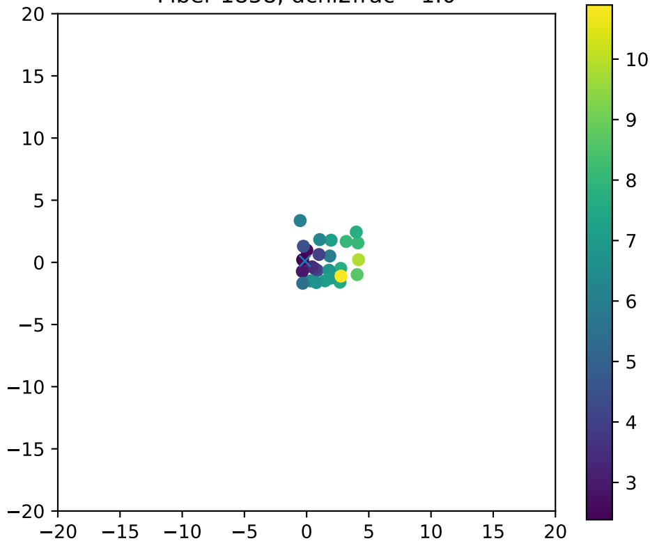
Fiber 1858, dchi2frac= 1.0
