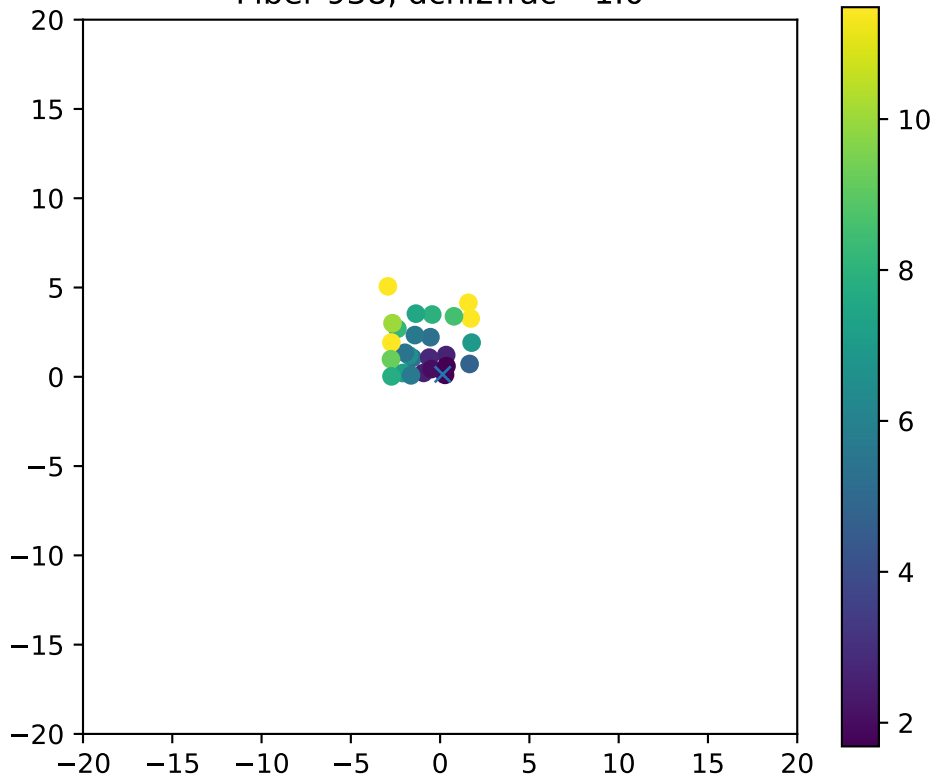
Fiber 938, dchi2frac= 1.0
