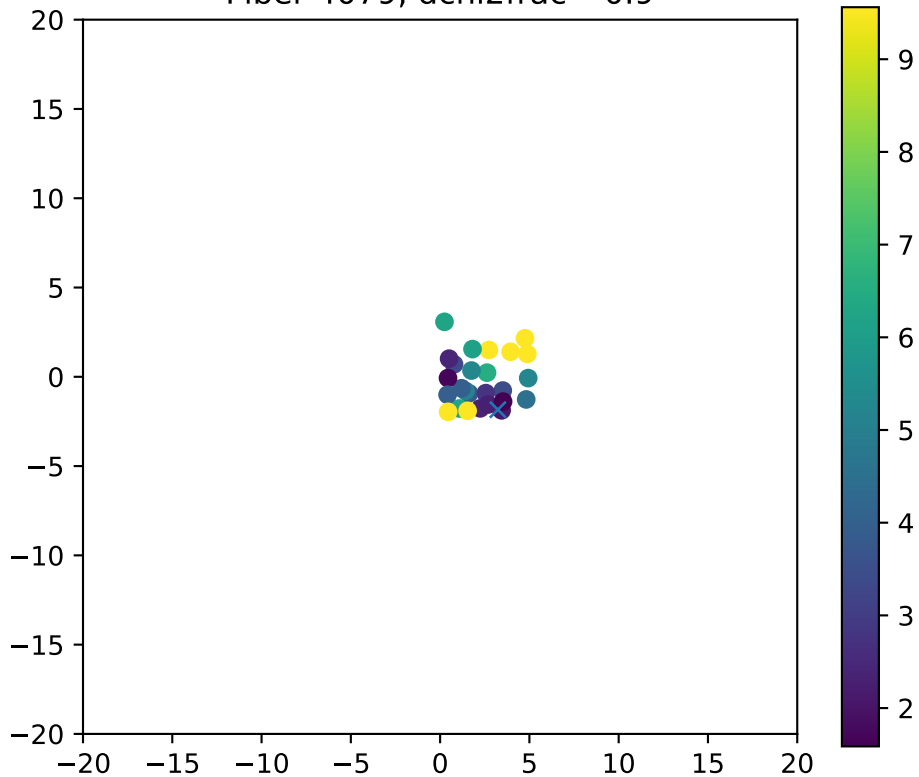
Fiber 4079, dchi2frac= 0.9
