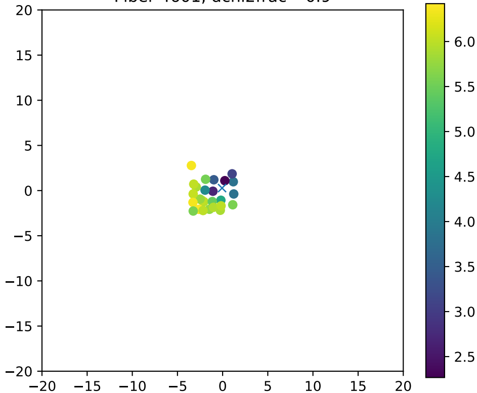
Fiber 4601, dchi2frac= 0.9
