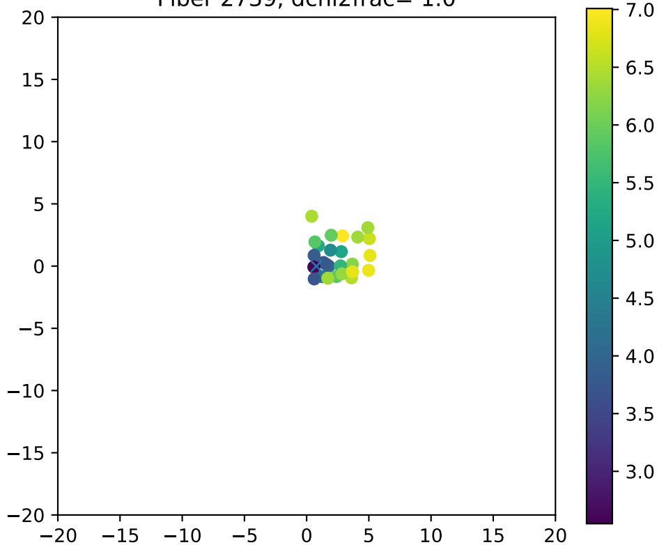
Fiber 2739, dchi2frac= 1.0
