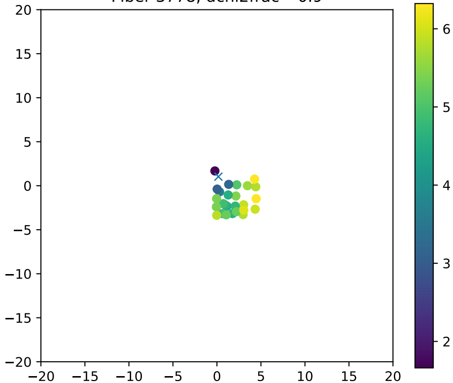
Fiber 3778, dchi2frac= 0.9
