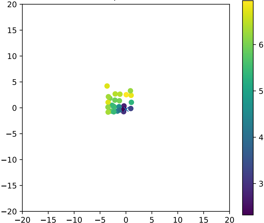
Fiber 3146, dchi2frac= 1.0
