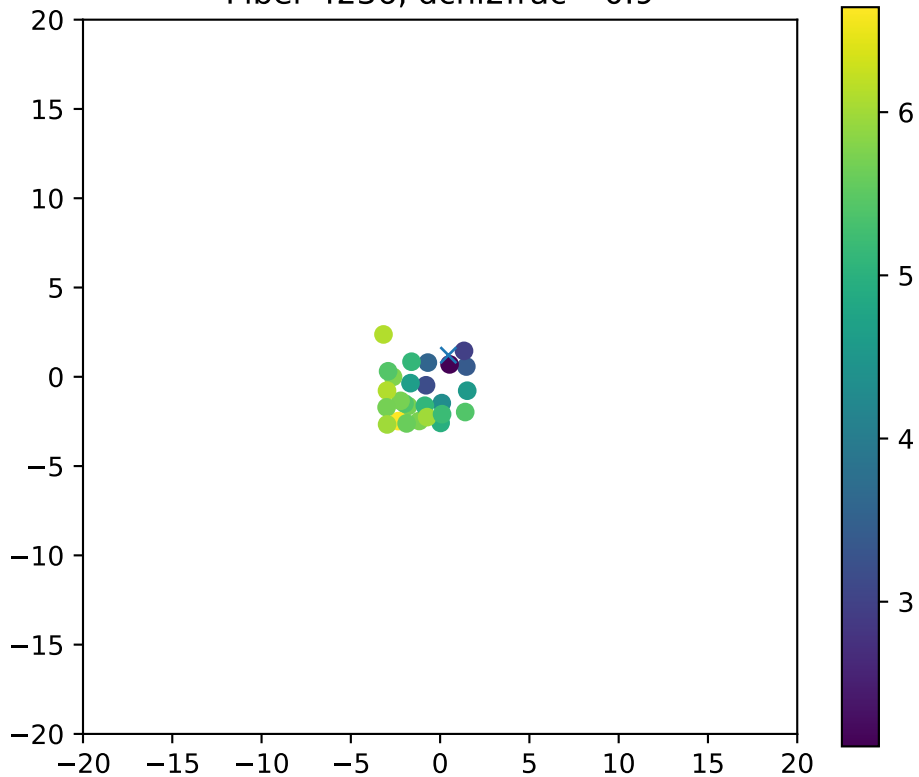
Fiber 4236, dchi2frac= 0.9
