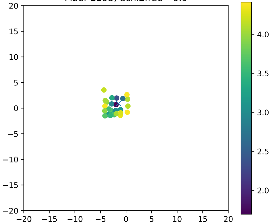
Fiber 2295, dchi2frac= 0.9
