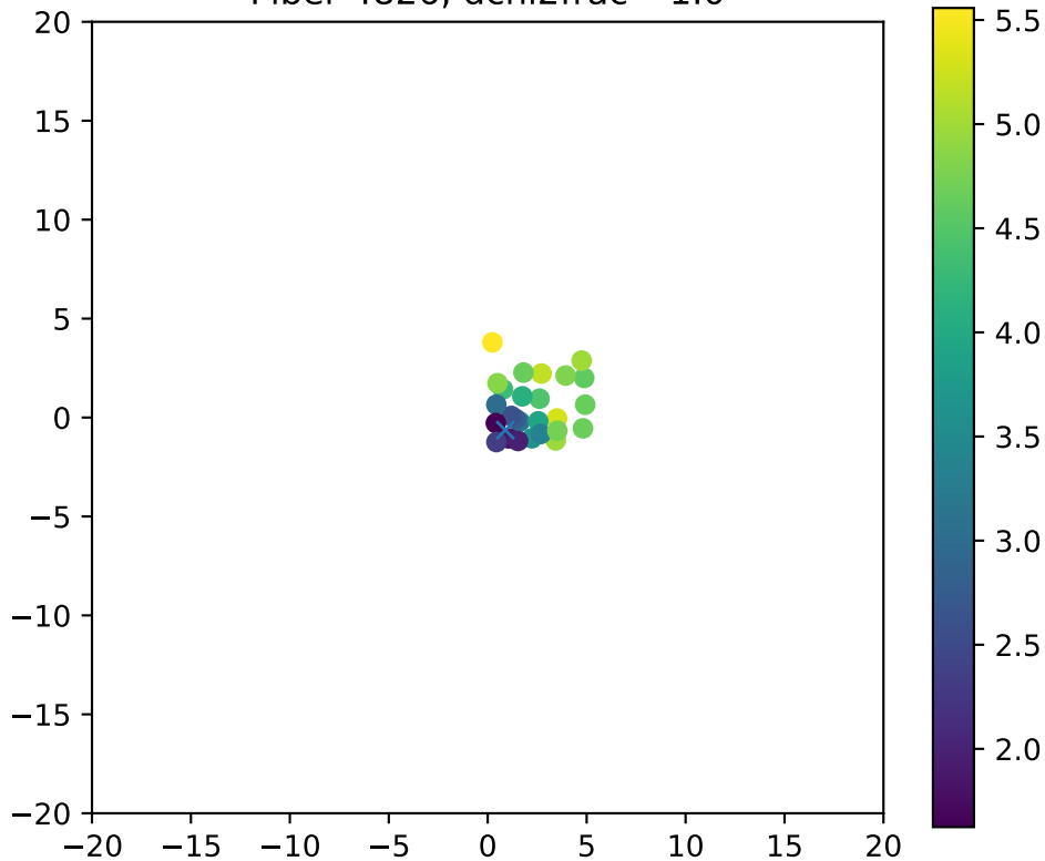
Fiber 4826, dchi2frac= 1.0
