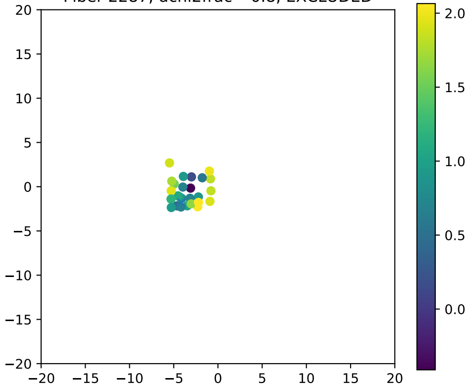
Fiber 2287, dchi2frac= 0.8, EXCLUDED
