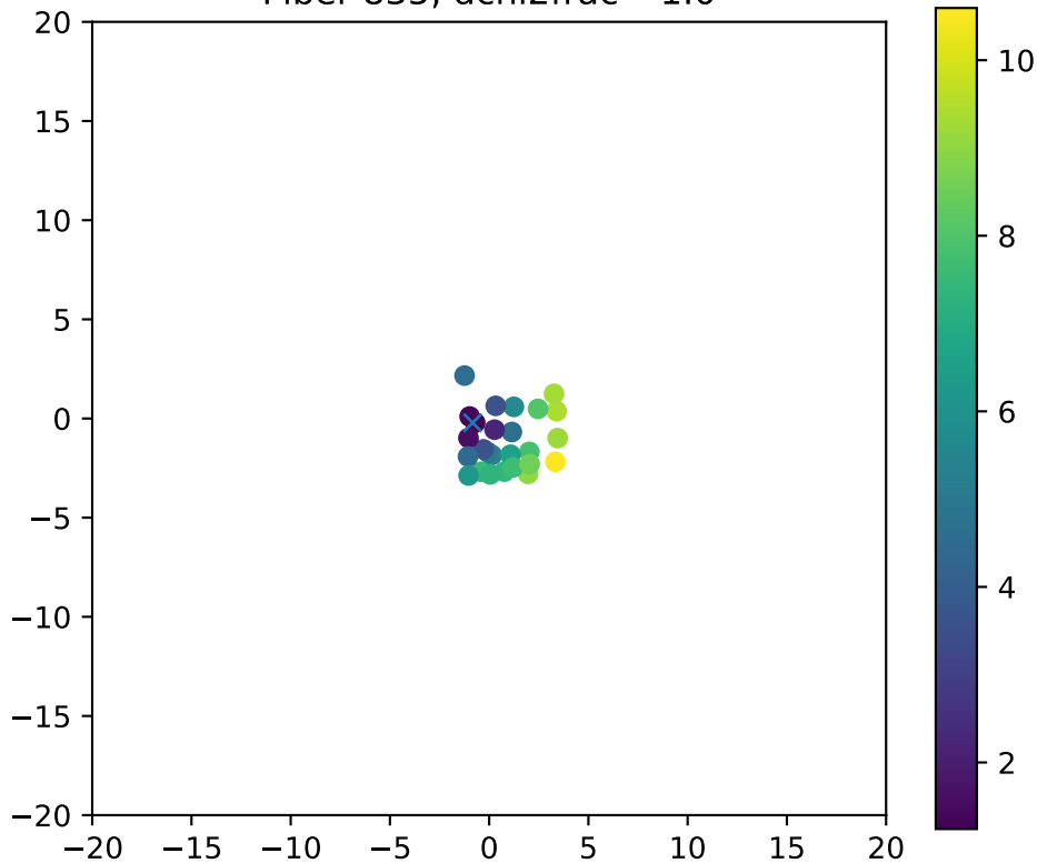
Fiber 835, dchi2frac= 1.0
