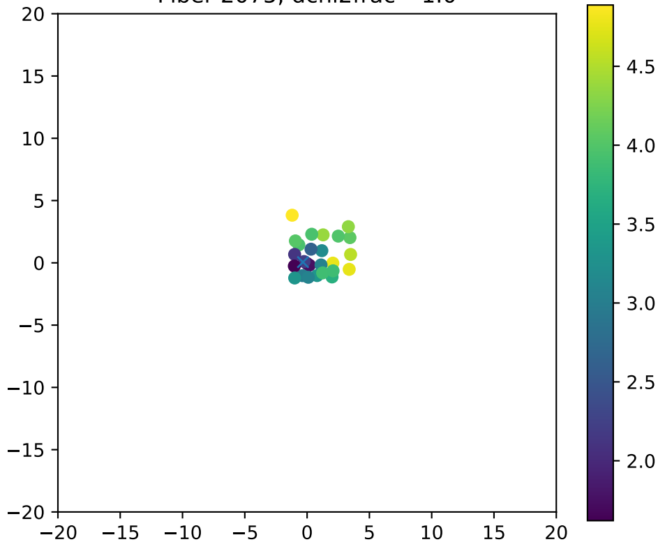
Fiber 2075, dchi2frac= 1.0
