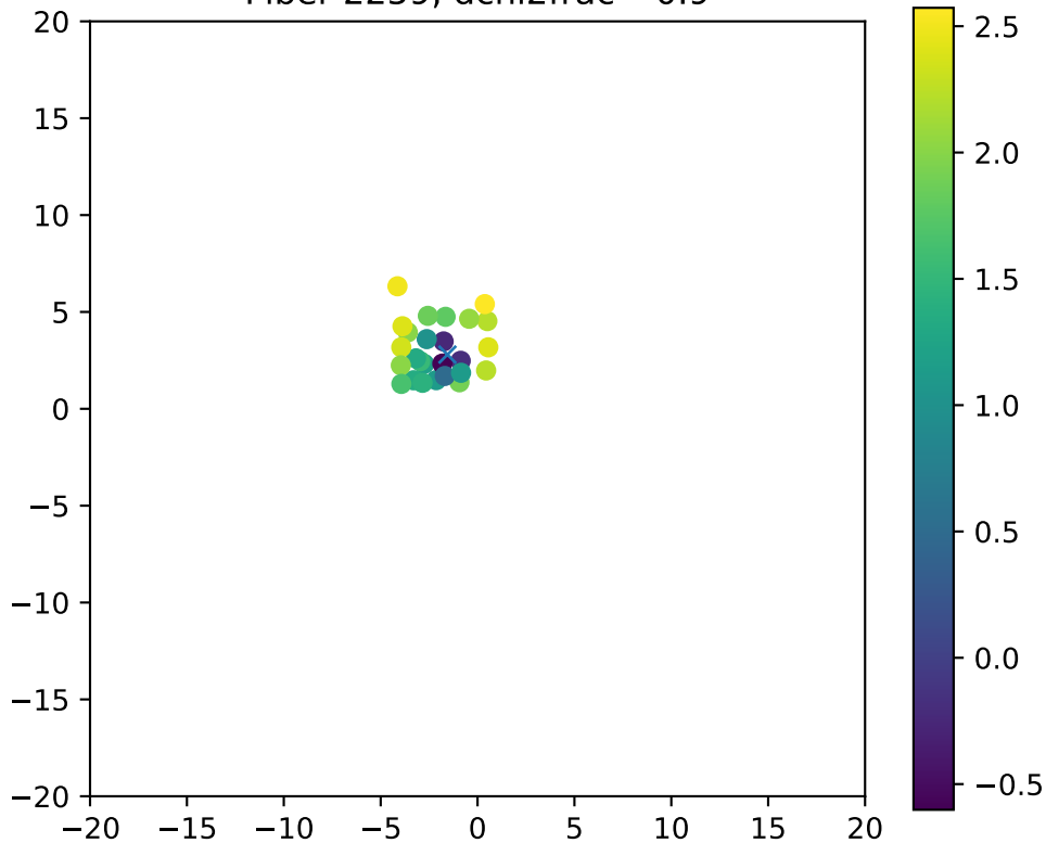
Fiber 2259, dchi2frac= 0.9
