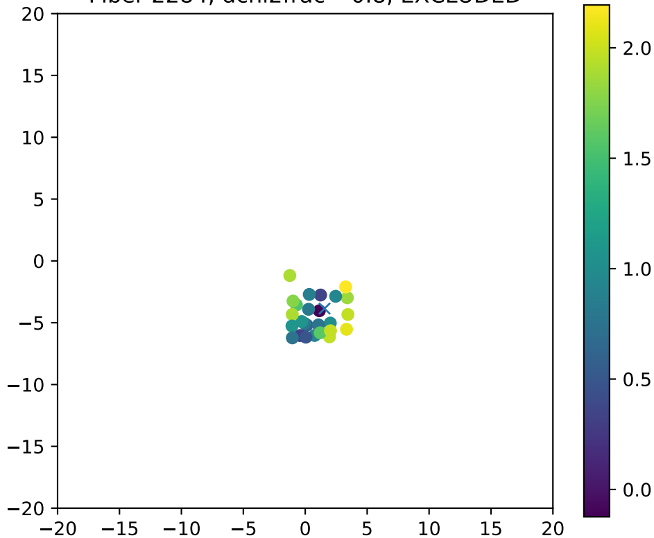
Fiber 2284, dchi2frac= 0.8, EXCLUDED
