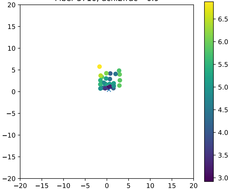
Fiber 3710, dchi2frac= 0.9
