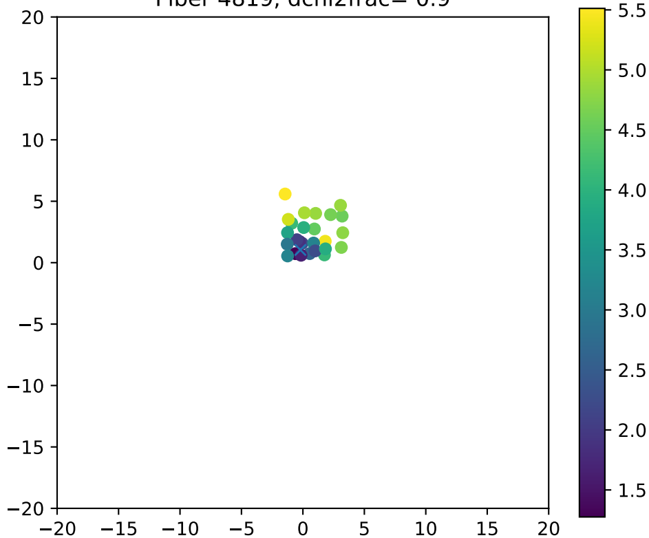
Fiber 4819, dchi2frac= 0.9
