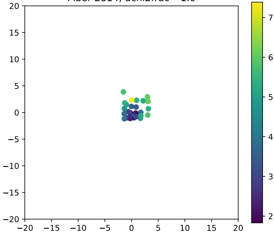
Fiber 2814, dchi2frac= 1.0
