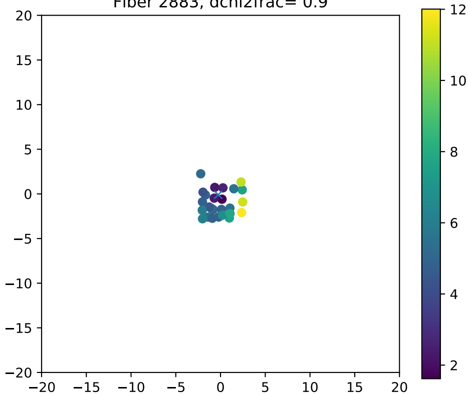
Fiber 2883, dchi2frac= 0.9
