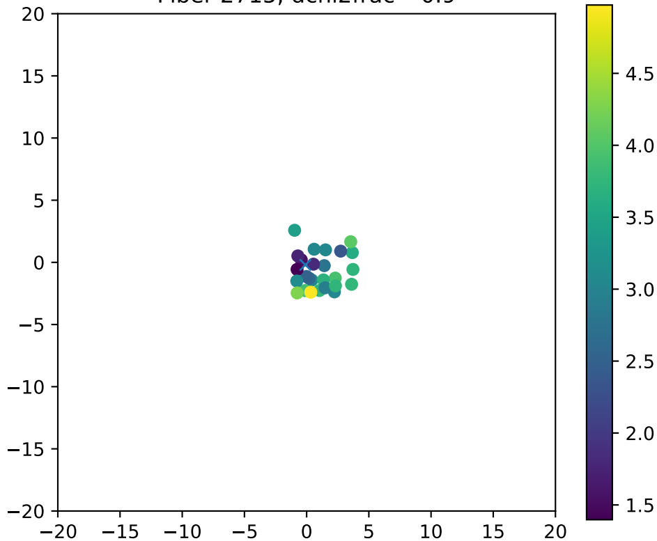
Fiber 2715, dchi2frac= 0.9
