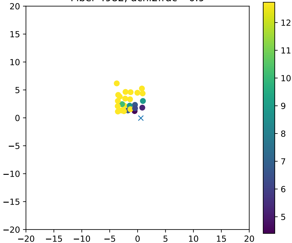
Fiber 4982, dchi2frac= 0.9
