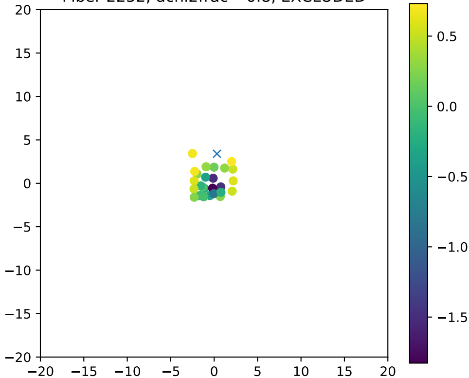
Fiber 2252, dchi2frac= 0.8, EXCLUDED
