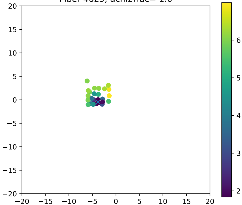
Fiber 4629, dchi2frac= 1.0
