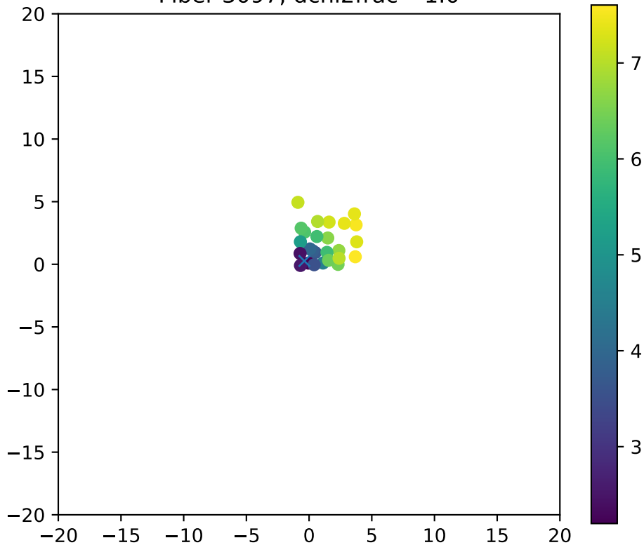
Fiber 3097, dchi2frac= 1.0
