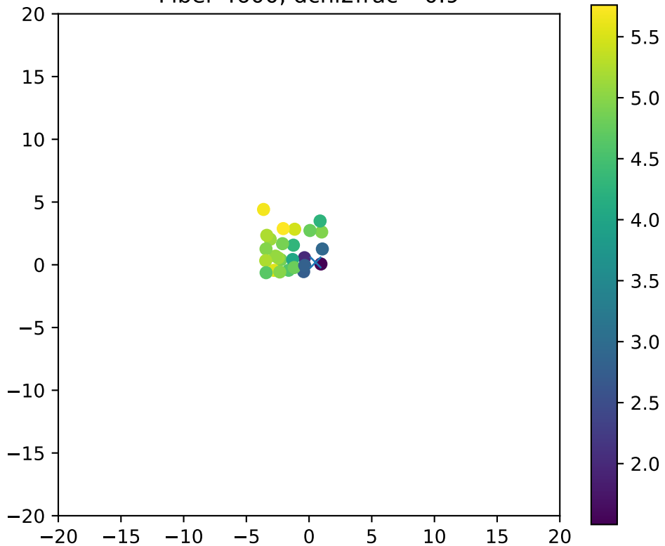
Fiber 4600, dchi2frac= 0.9
