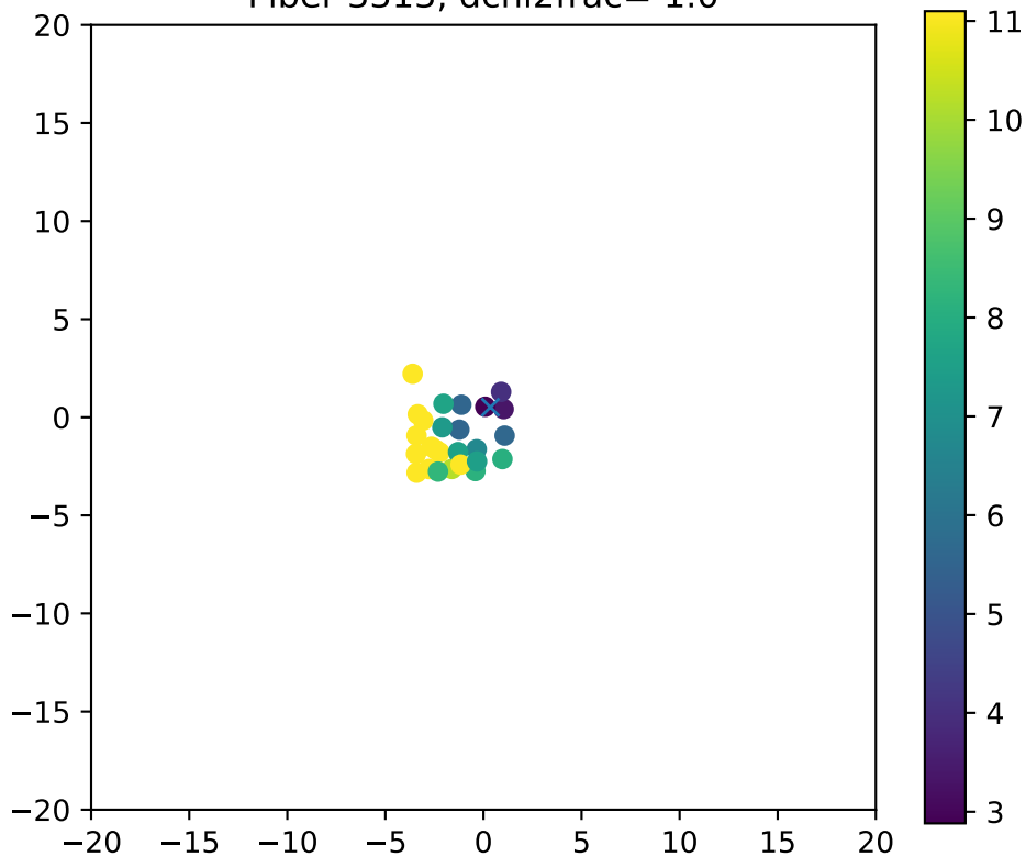
Fiber 3313, dchi2frac= 1.0
