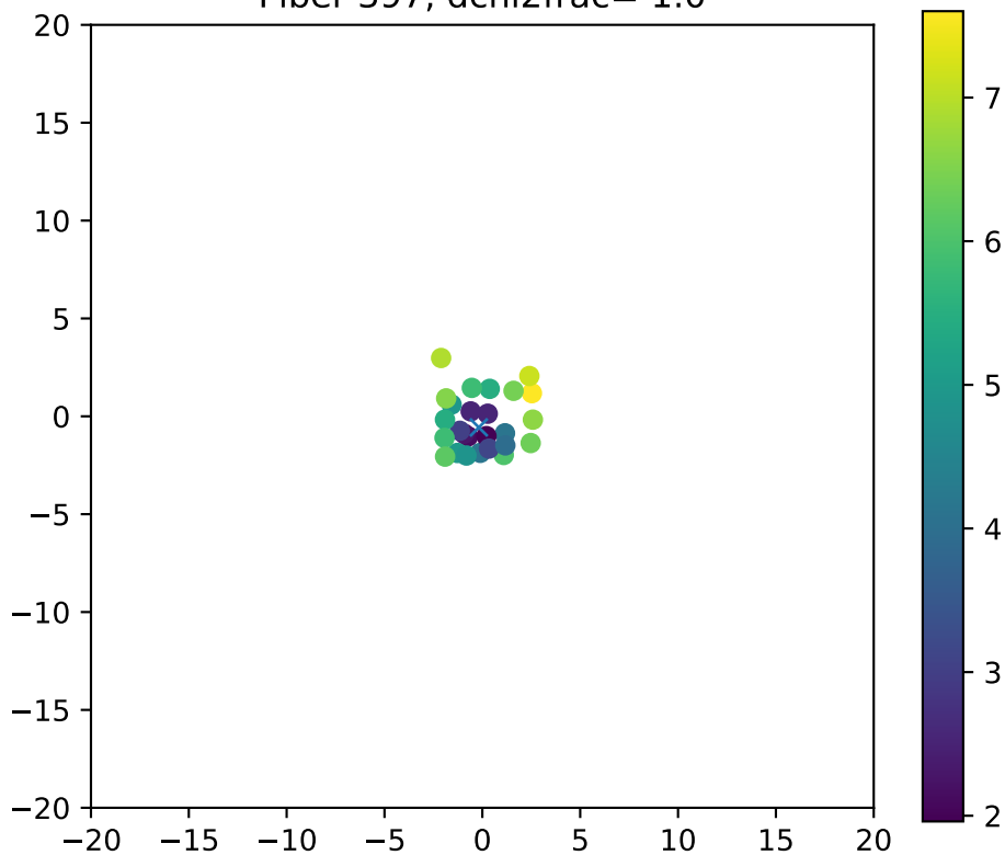
Fiber 397, dchi2frac= 1.0
