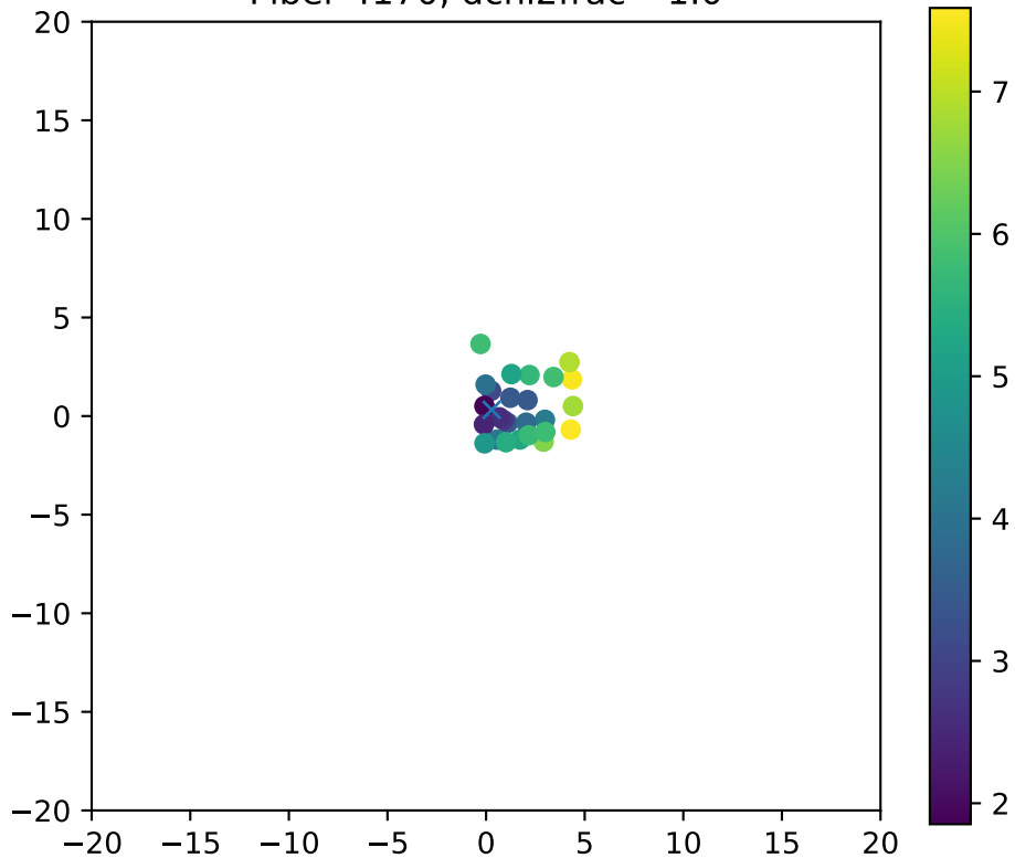
Fiber 4170, dchi2frac= 1.0
