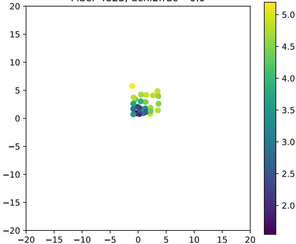
Fiber 4823, dchi2frac= 0.9
