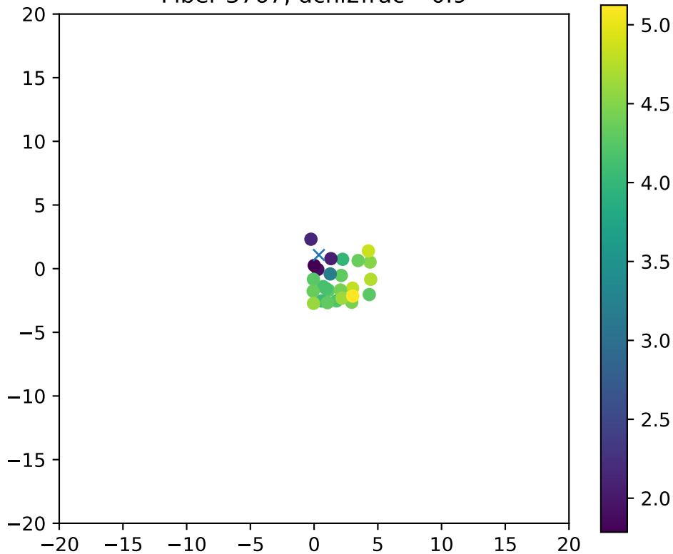
Fiber 3767, dchi2frac= 0.9
