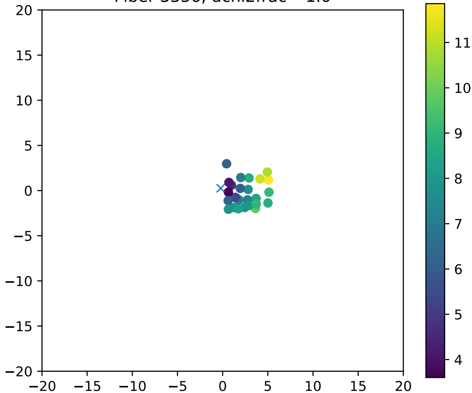
Fiber 3356, dchi2frac= 1.0
