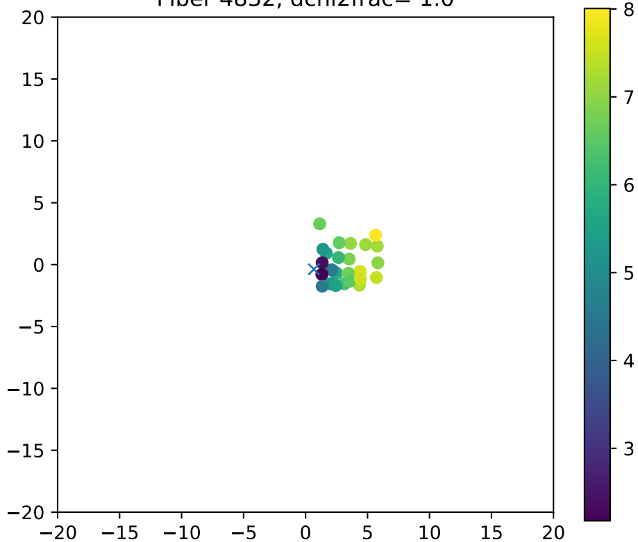
Fiber 4832, dchi2frac= 1.0
