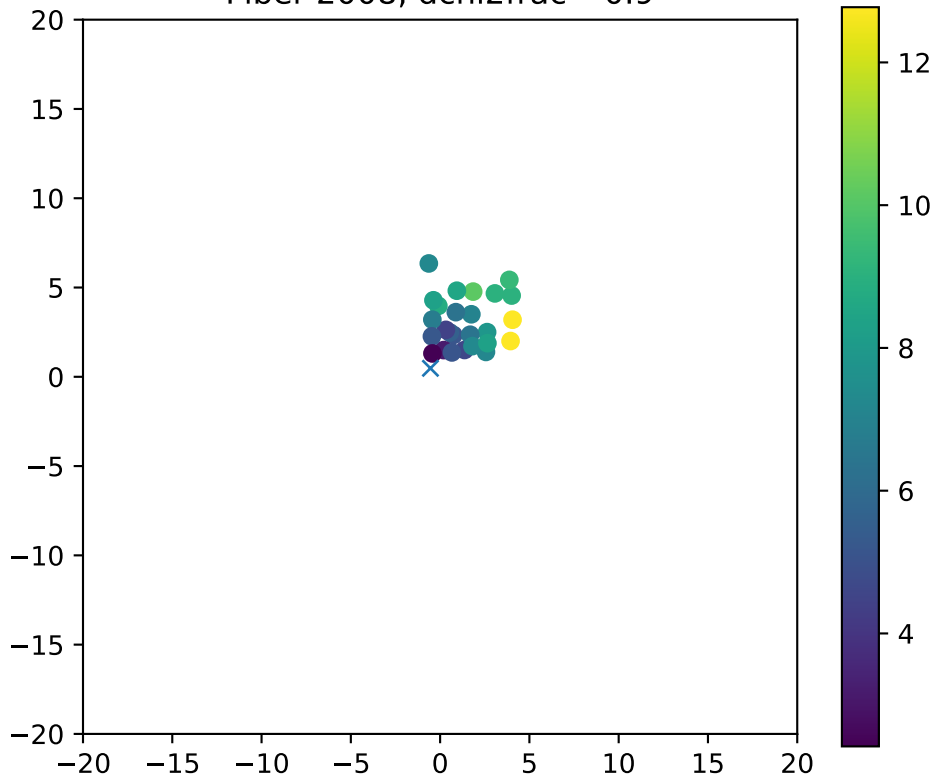
Fiber 2008, dchi2frac= 0.9
