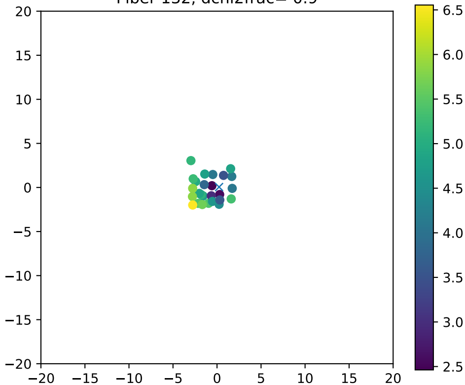
Fiber 132, dchi2frac= 0.9
