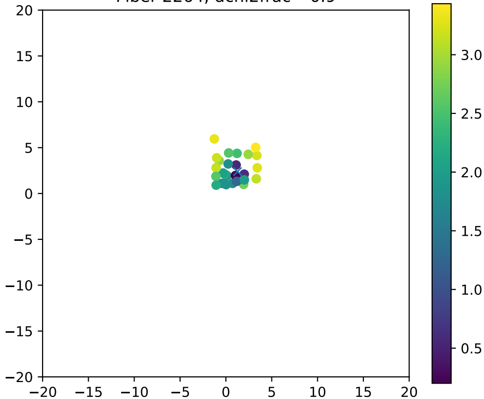
Fiber 2264, dchi2frac= 0.9
