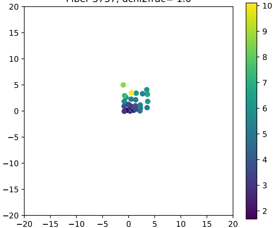
Fiber 3737, dchi2frac= 1.0
