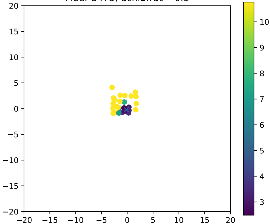
Fiber 3475, dchi2frac= 0.9
