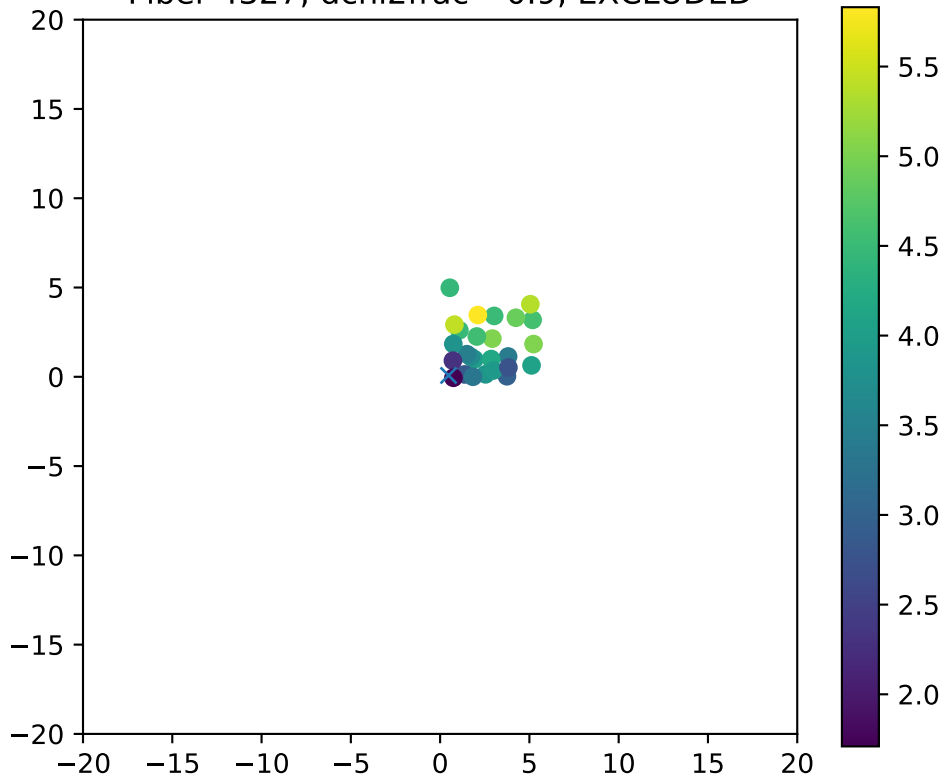
Fiber 4327, dchi2frac= 0.9, EXCLUDED
