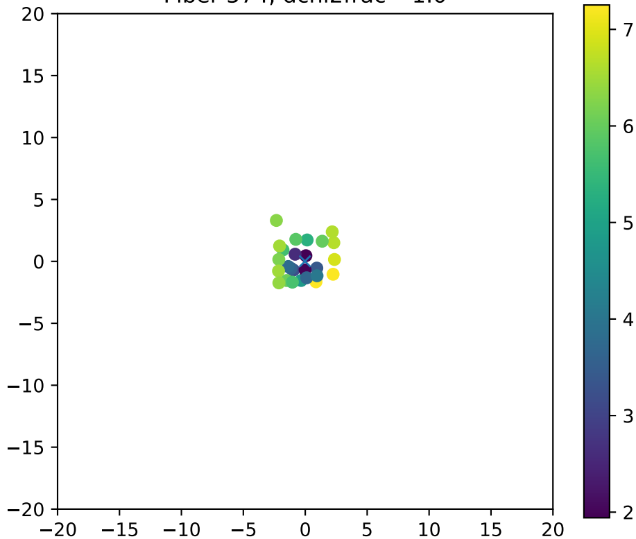
Fiber 574, dchi2frac= 1.0
