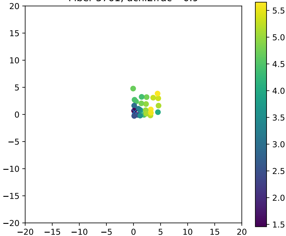
Fiber 3761, dchi2frac= 0.9
