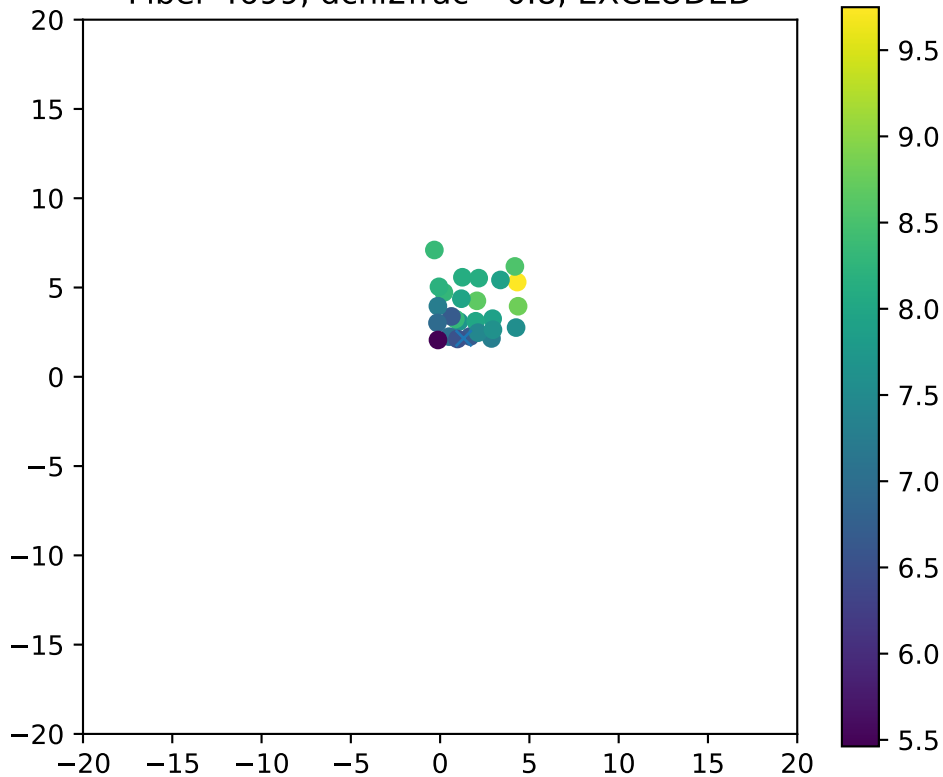
Fiber 4699, dchi2frac= 0.8, EXCLUDED
