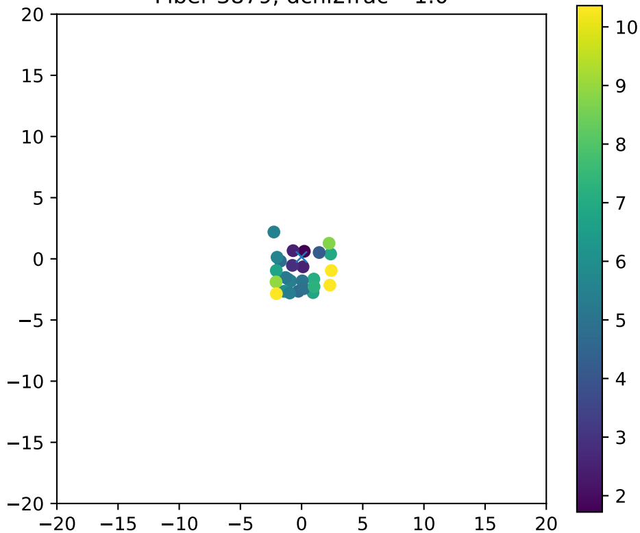
Fiber 3879, dchi2frac= 1.0
