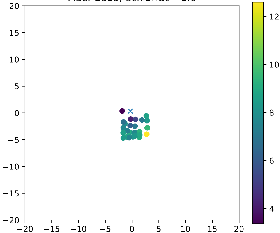
Fiber 2019, dchi2frac= 1.0
