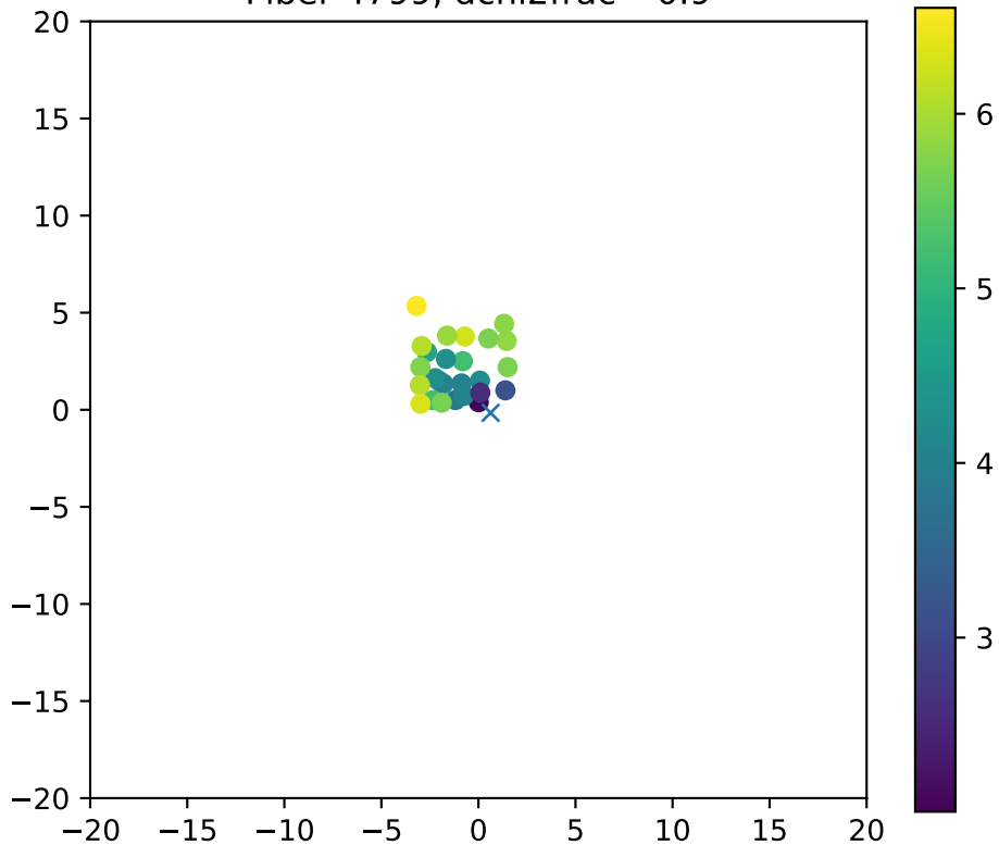
Fiber 4799, dchi2frac= 0.9
