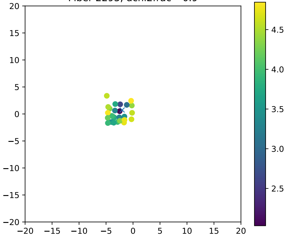
Fiber 2293, dchi2frac= 0.9
