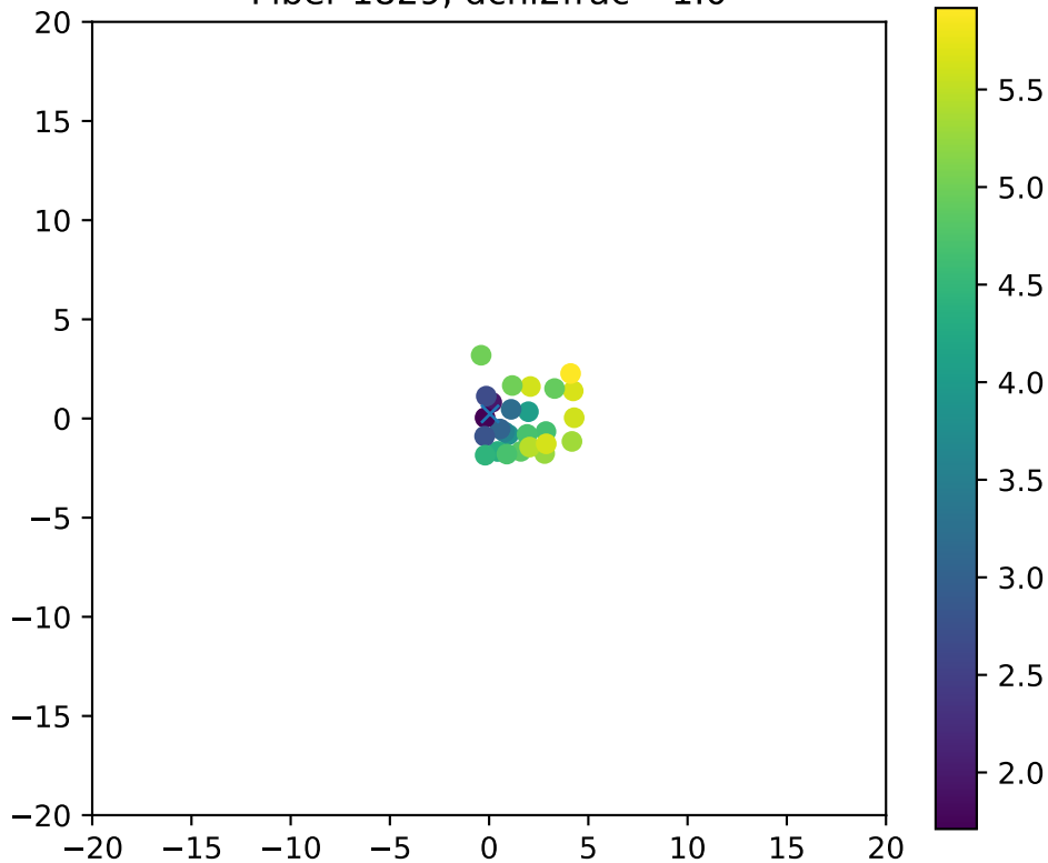
Fiber 1829, dchi2frac= 1.0
