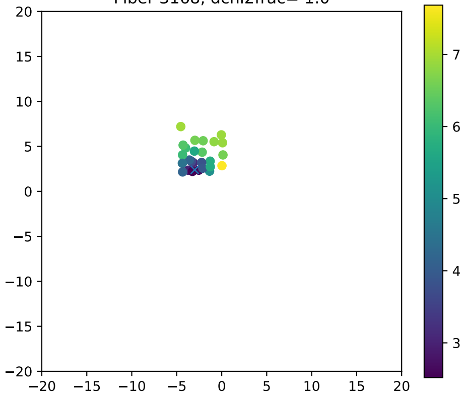
Fiber 3168, dchi2frac= 1.0
