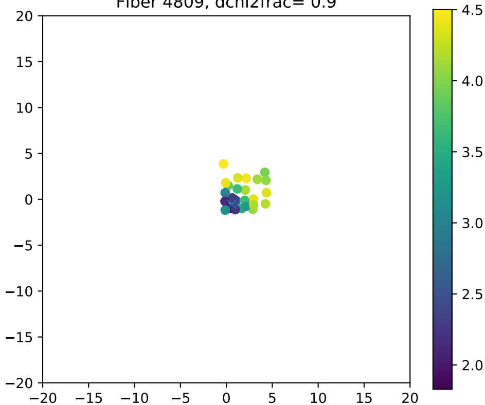
Fiber 4809, dchi2frac= 0.9
