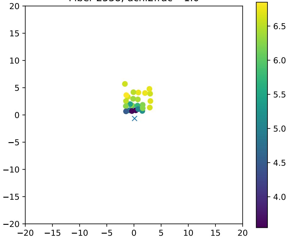
Fiber 2538, dchi2frac= 1.0
