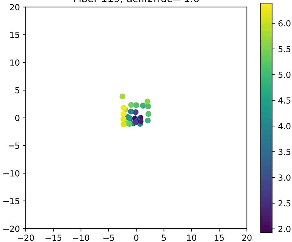
Fiber 119, dchi2frac= 1.0
