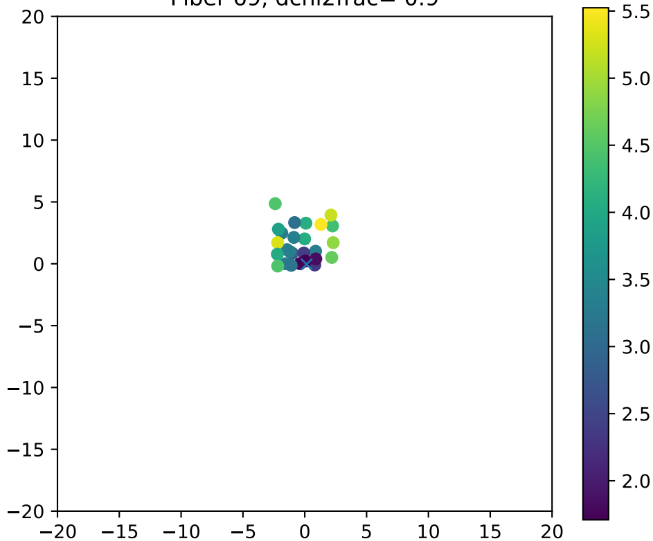
Fiber 69, dchi2frac= 0.9
