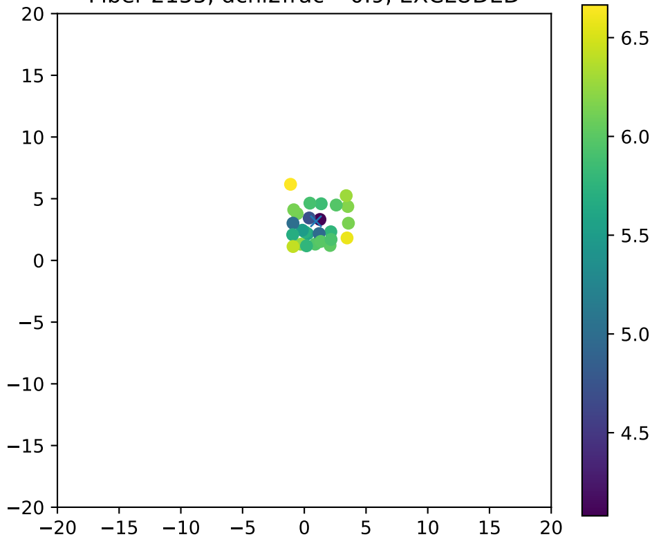
Fiber 2155, dchi2frac= 0.9, EXCLUDED
