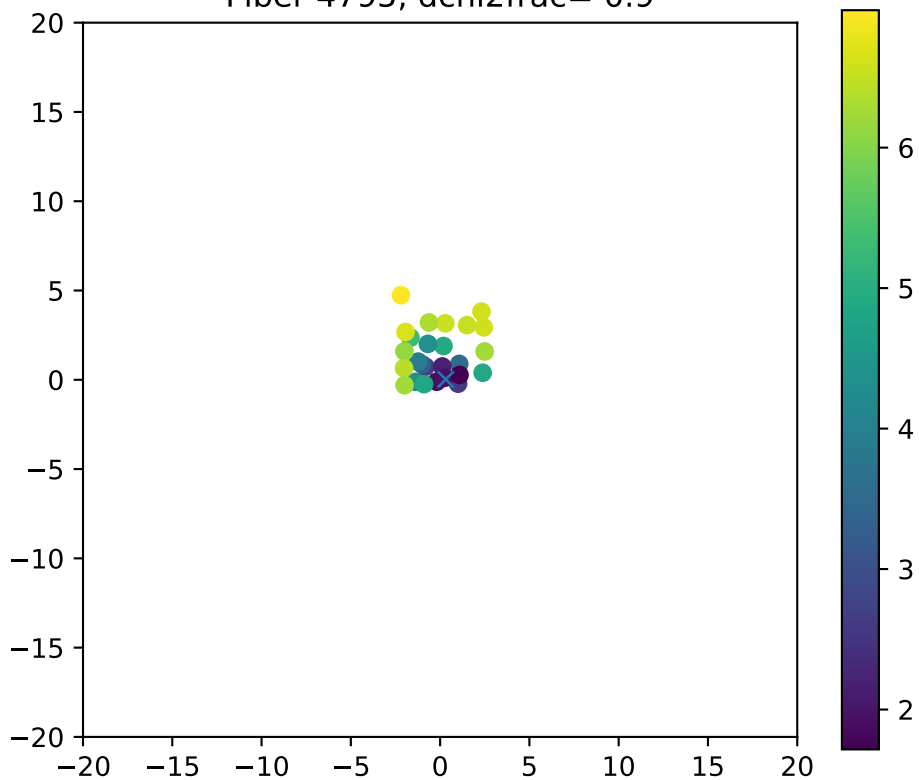
Fiber 4795, dchi2frac= 0.9
