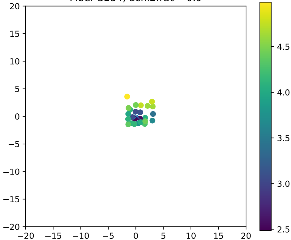
Fiber 3234, dchi2frac= 0.9
