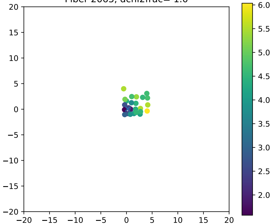
Fiber 2063, dchi2frac= 1.0
