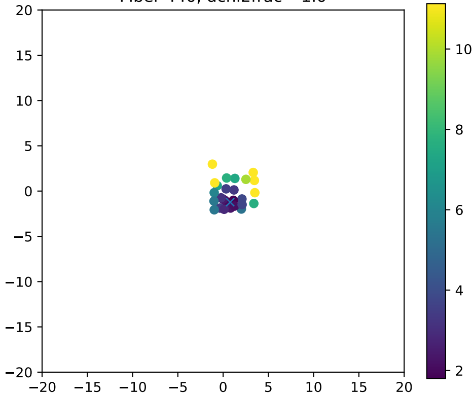
Fiber 440, dchi2frac= 1.0
