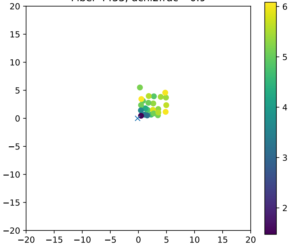
Fiber 4433, dchi2frac= 0.9
