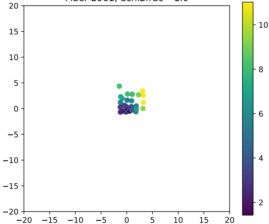
Fiber 2961, dchi2frac= 1.0
