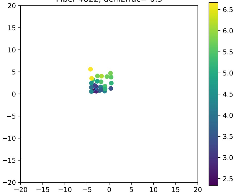
Fiber 4822, dchi2frac= 0.9
