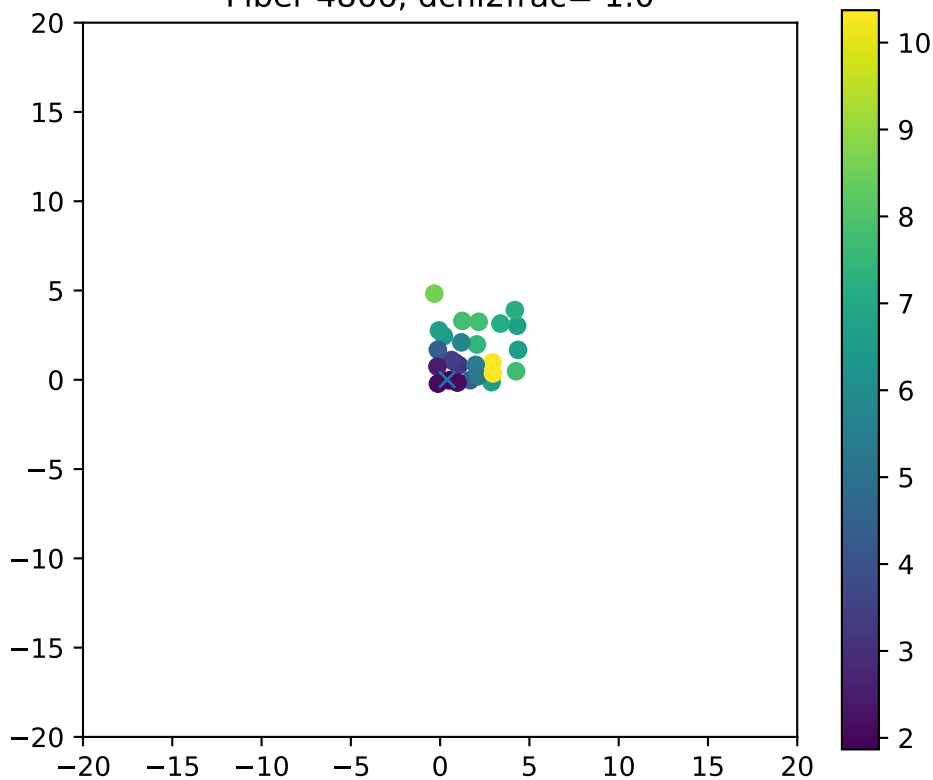
Fiber 4866, dchi2frac= 1.0
