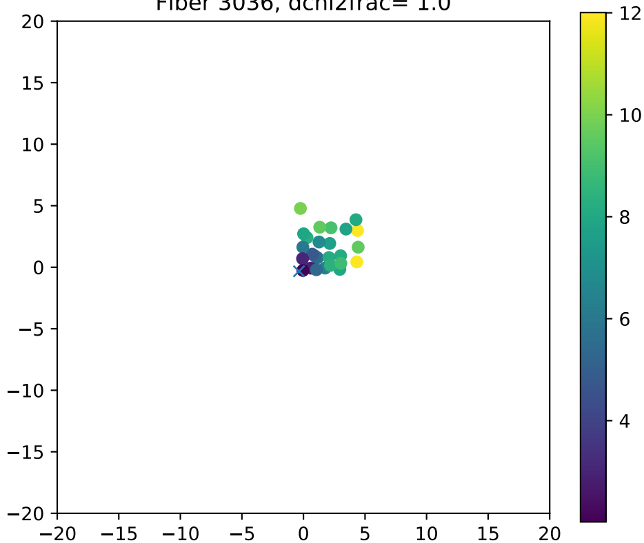
Fiber 3036, dchi2frac= 1.0
