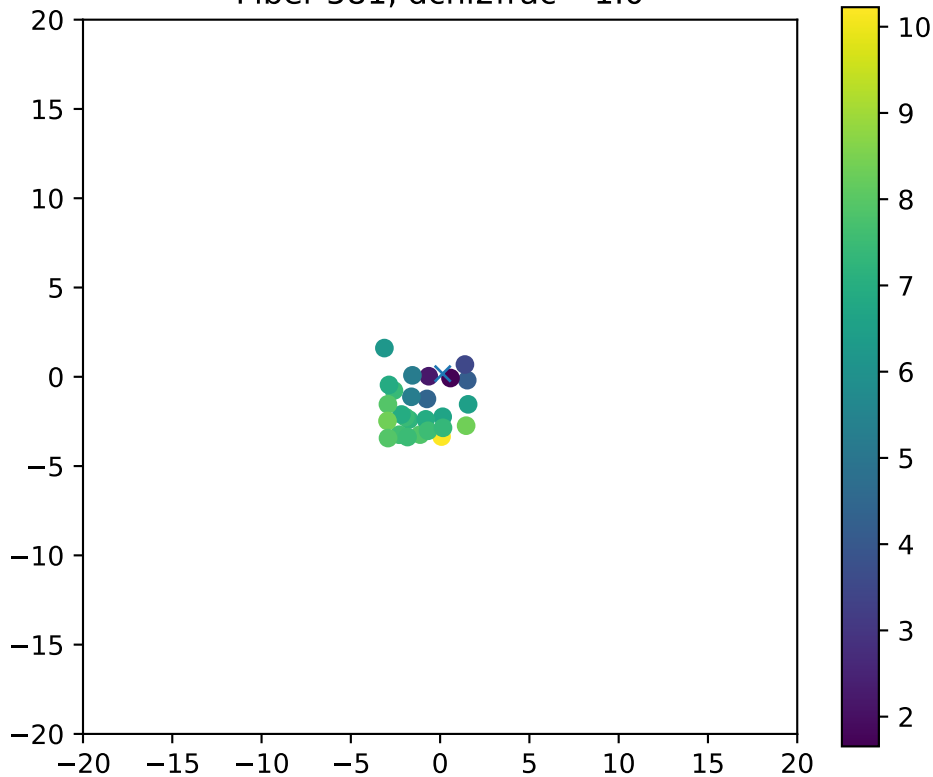
Fiber 581, dchi2frac= 1.0
