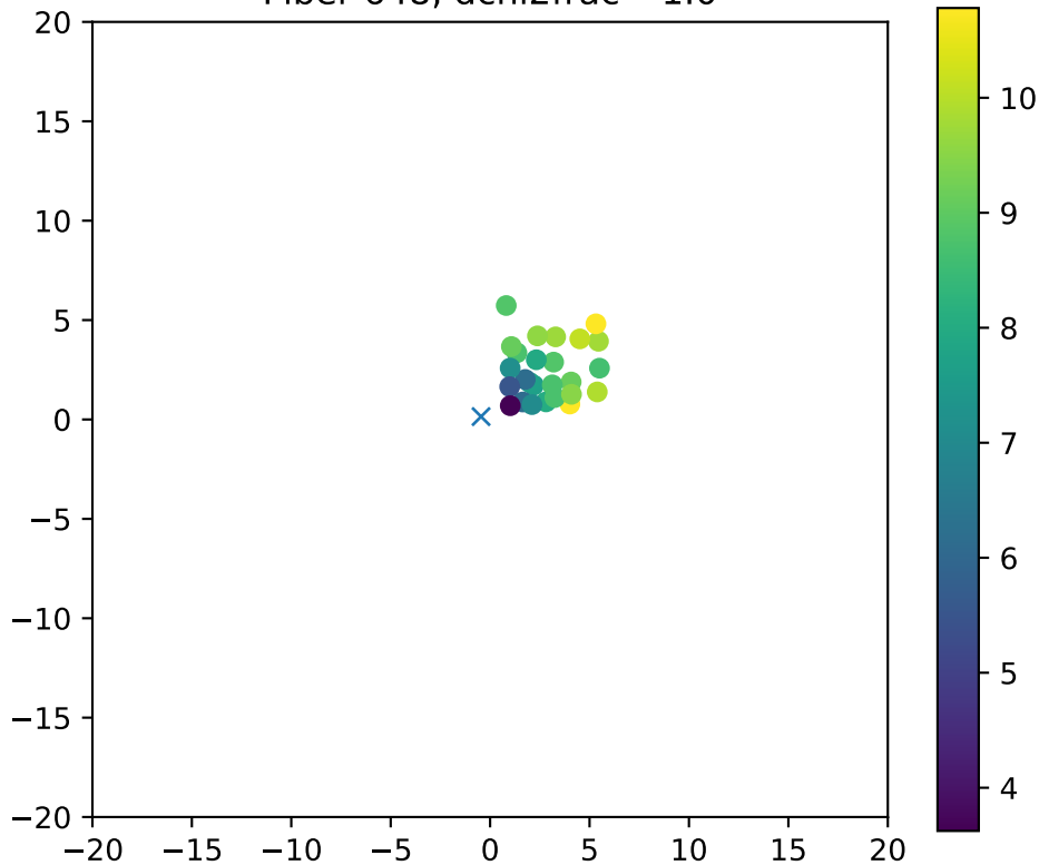
Fiber 648, dchi2frac= 1.0
