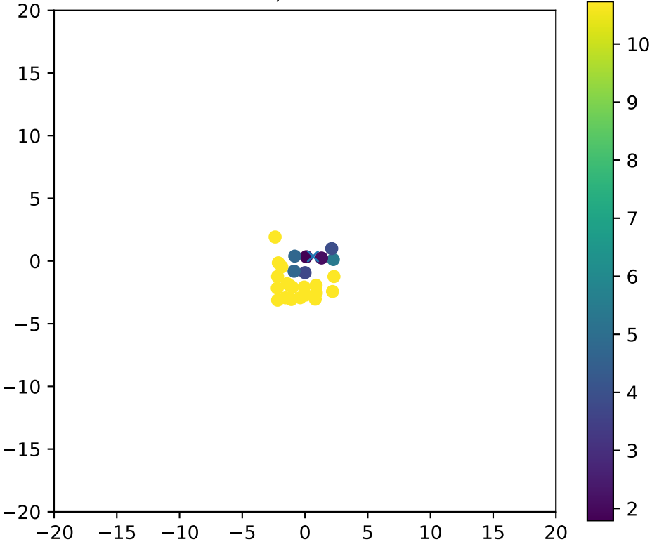
Fiber 4977, dchi2frac= 0.9
