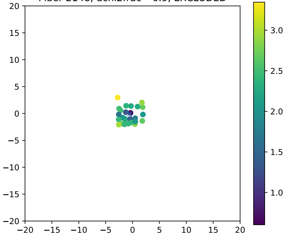
Fiber 2148, dchi2frac= 0.9, EXCLUDED
