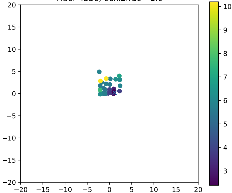
Fiber 4336, dchi2frac= 1.0
