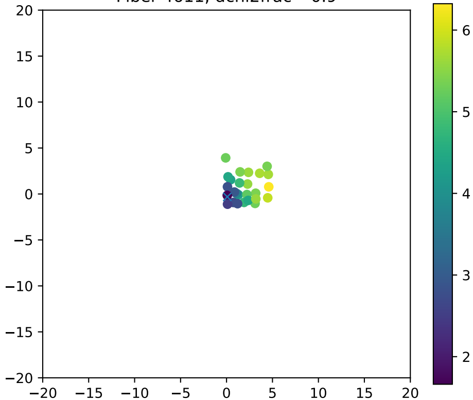
Fiber 4611, dchi2frac= 0.9
