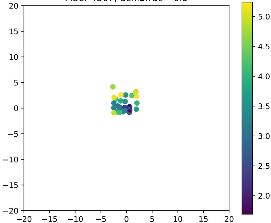
Fiber 4307, dchi2frac= 0.9
