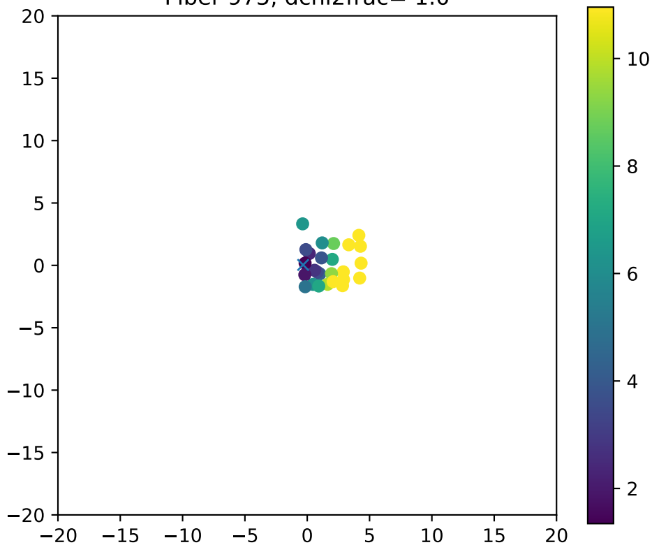
Fiber 975, dchi2frac= 1.0
