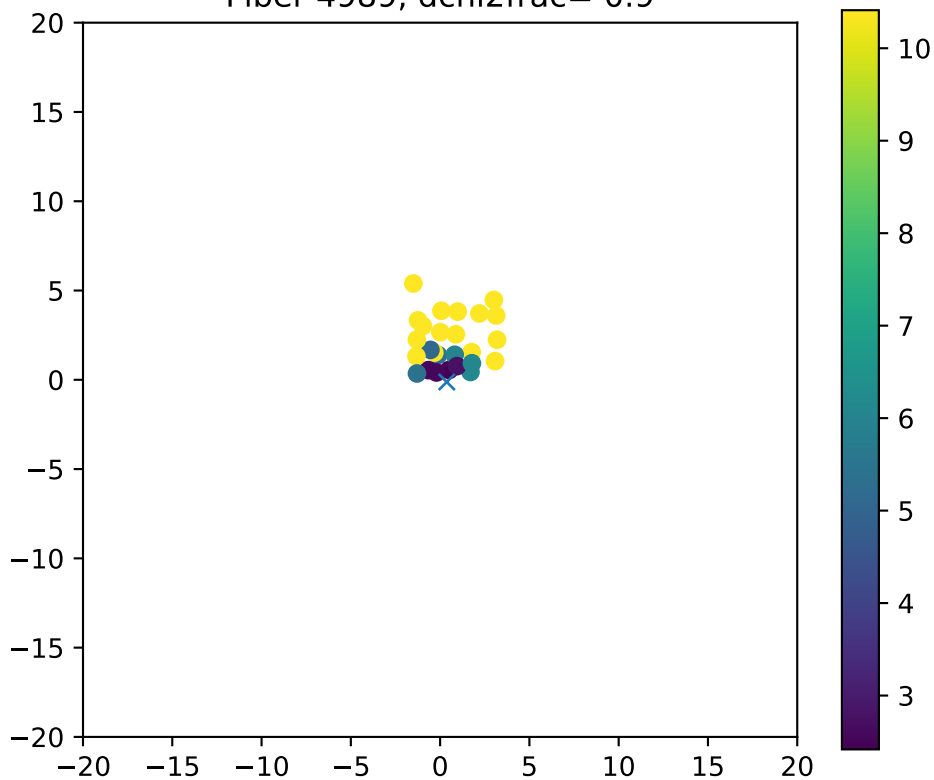
Fiber 4989, dchi2frac= 0.9
