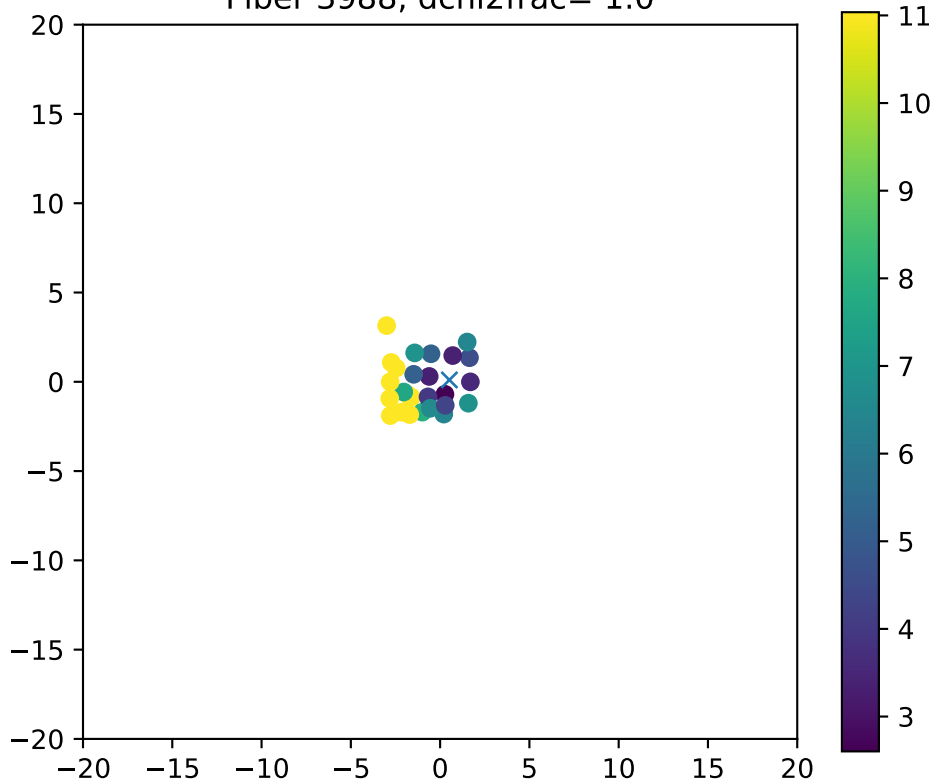
Fiber 3988, dchi2frac= 1.0
