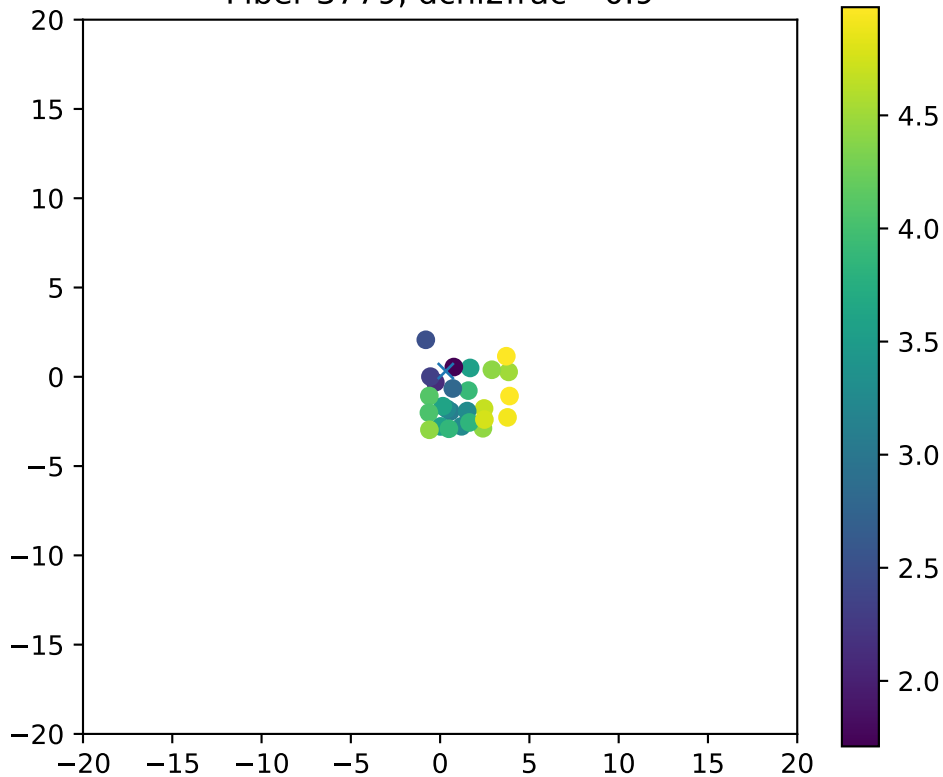
Fiber 3779, dchi2frac= 0.9
