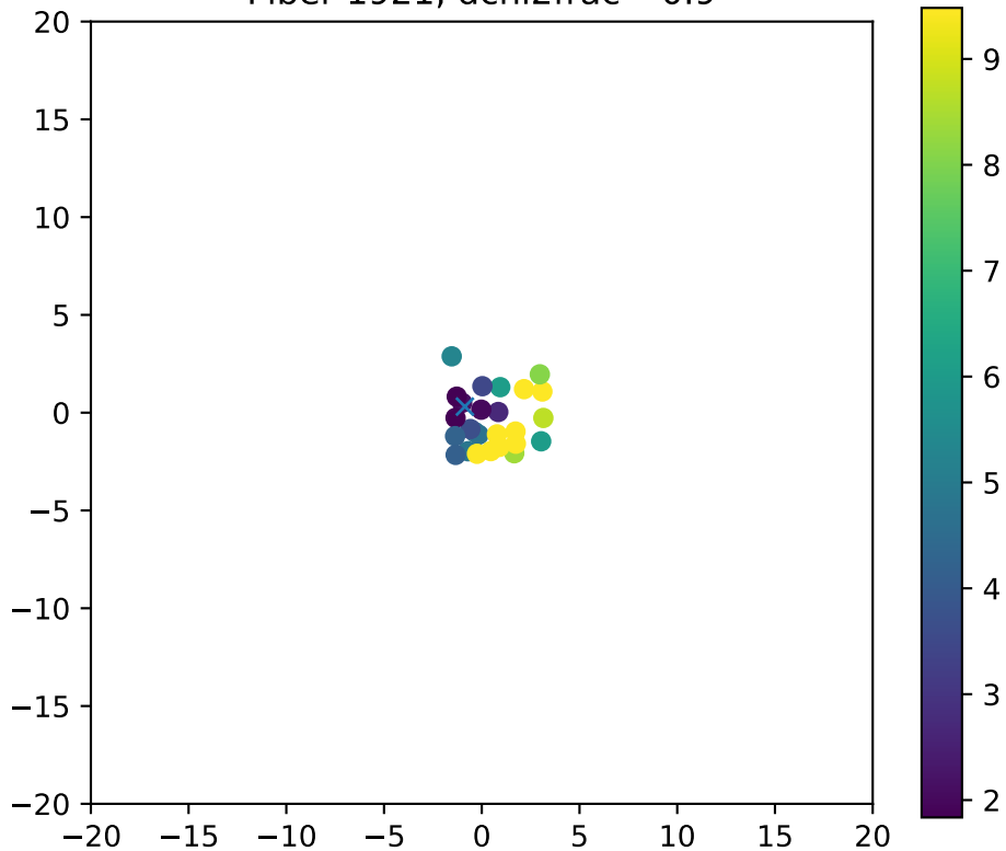
Fiber 1921, dchi2frac= 0.9
