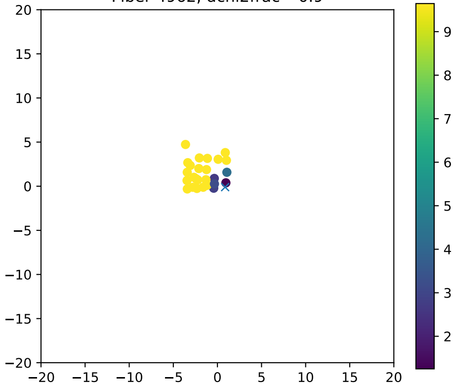
Fiber 4962, dchi2frac= 0.9
