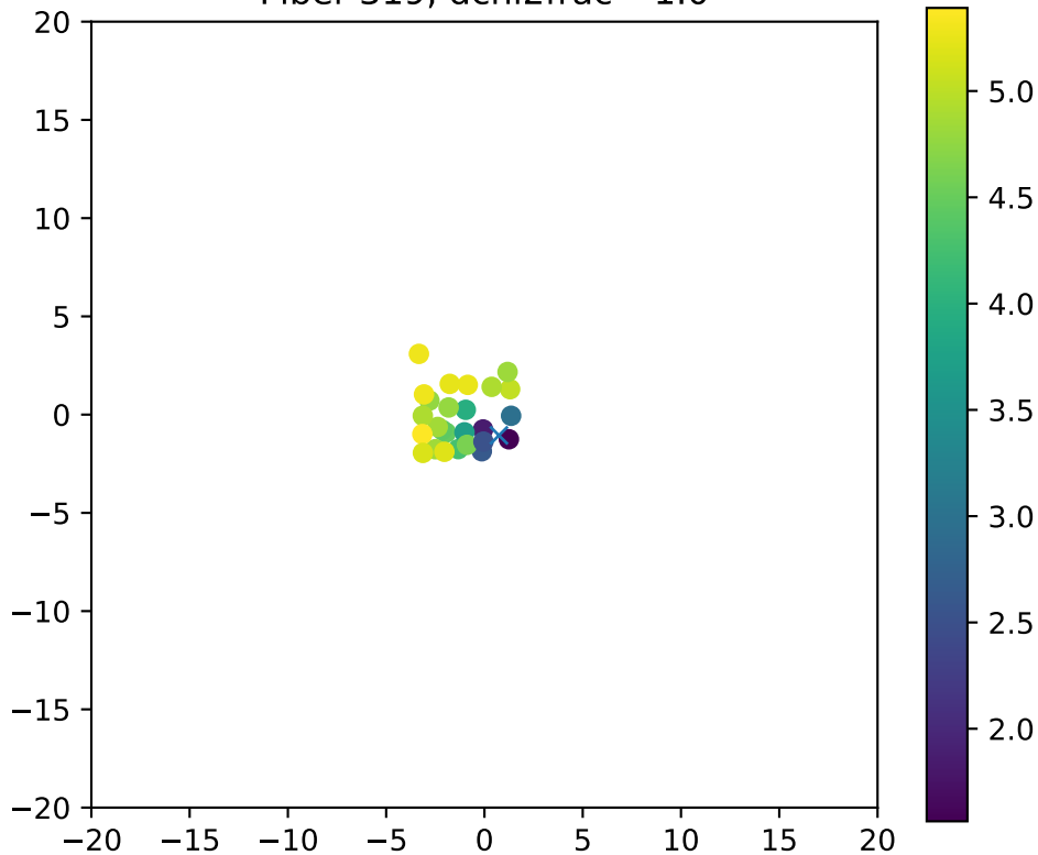
Fiber 319, dchi2frac= 1.0
