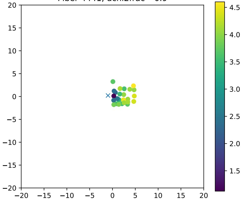
Fiber 4441, dchi2frac= 0.9
