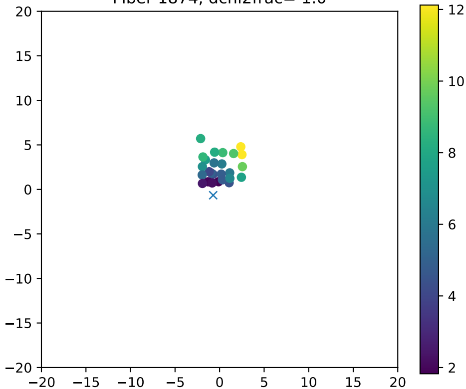
Fiber 1874, dchi2frac= 1.0
