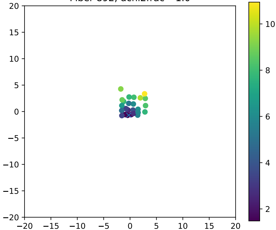
Fiber 892, dchi2frac= 1.0
