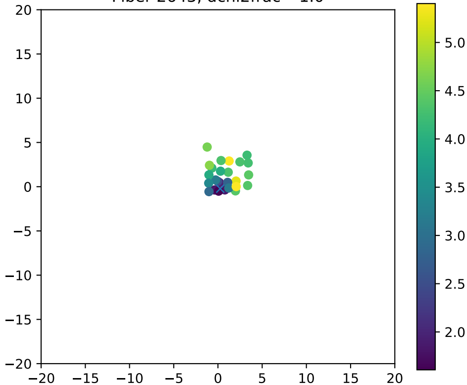
Fiber 2643, dchi2frac= 1.0
