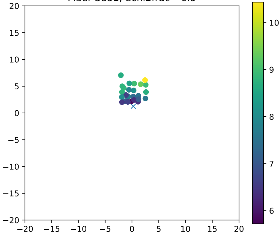
Fiber 3851, dchi2frac= 0.9
