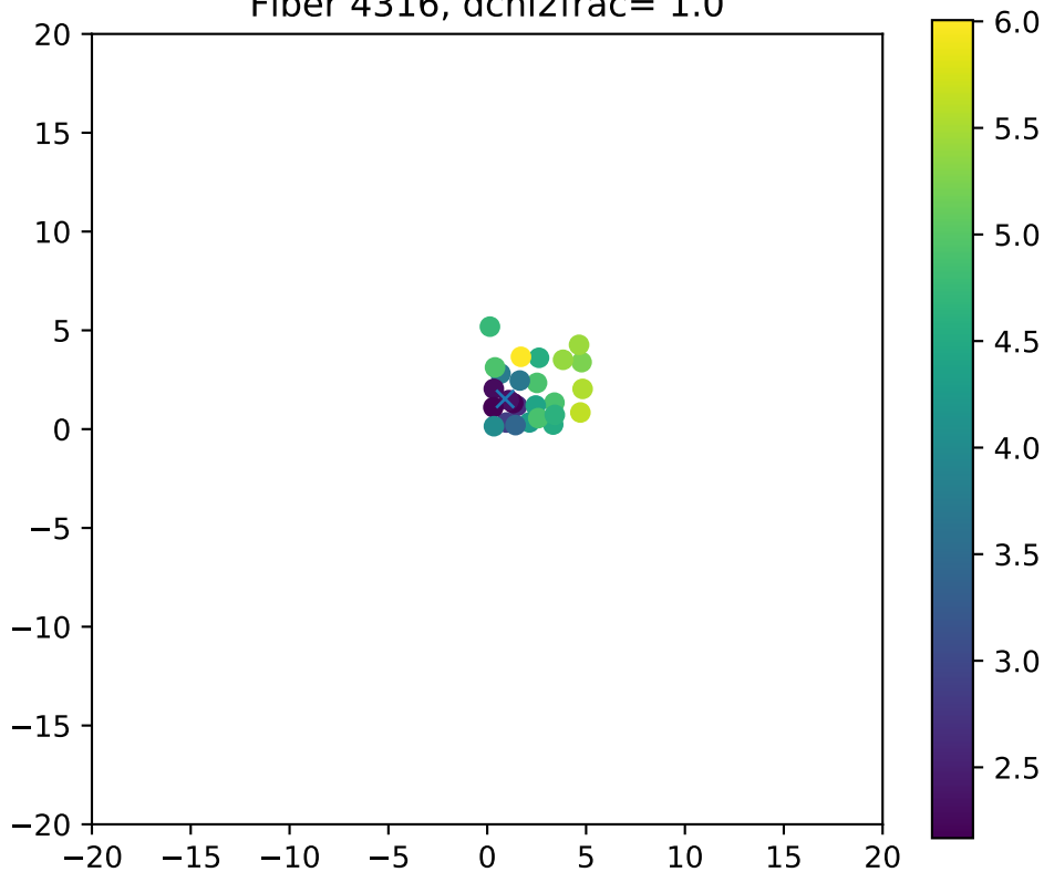
Fiber 4316, dchi2frac= 1.0
