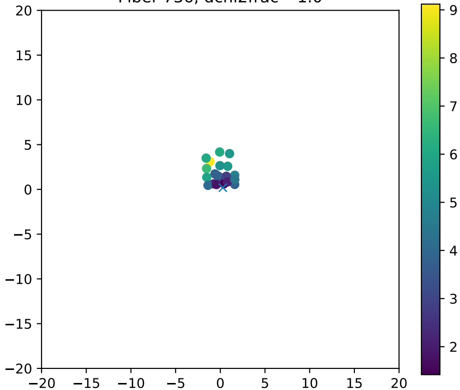
Fiber 736, dchi2frac= 1.0
