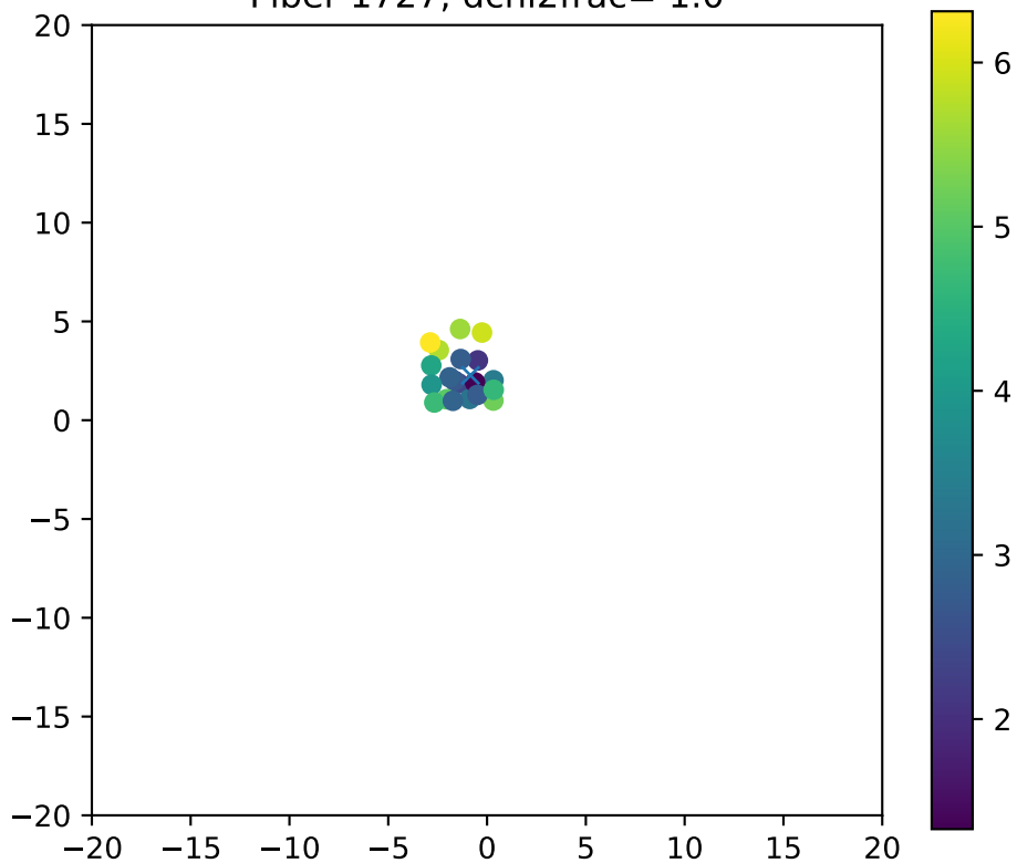
Fiber 1727, dchi2frac= 1.0
