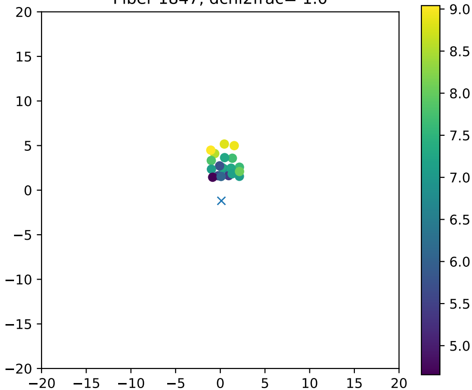
Fiber 1847, dchi2frac= 1.0
