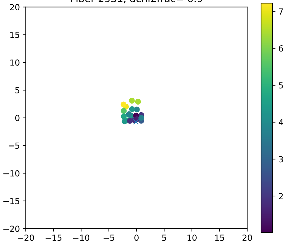
Fiber 2931, dchi2frac= 0.9
