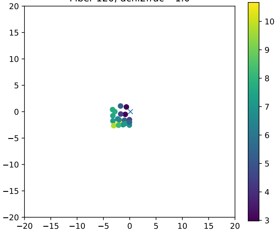
Fiber 120, dchi2frac= 1.0
