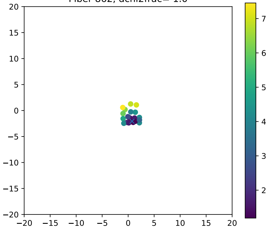
Fiber 862, dchi2frac= 1.0
