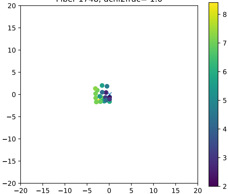
Fiber 1748, dchi2frac= 1.0
