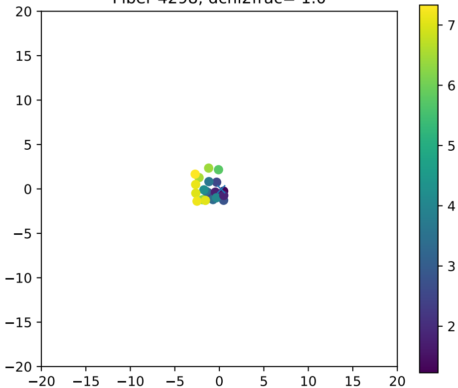
Fiber 4298, dchi2frac= 1.0
