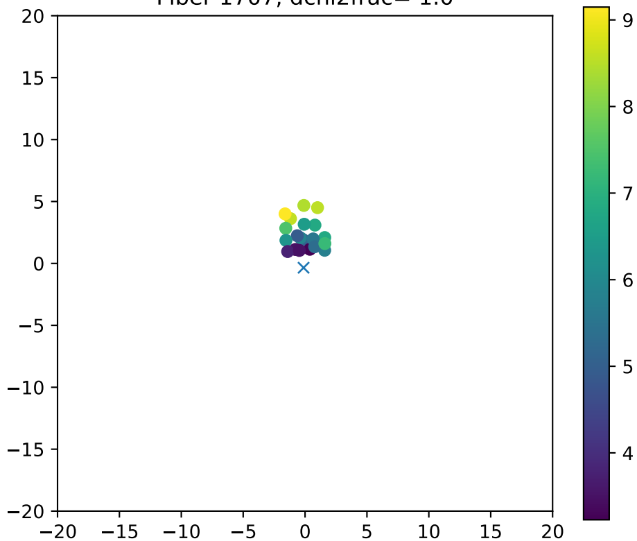
Fiber 1707, dchi2frac= 1.0
