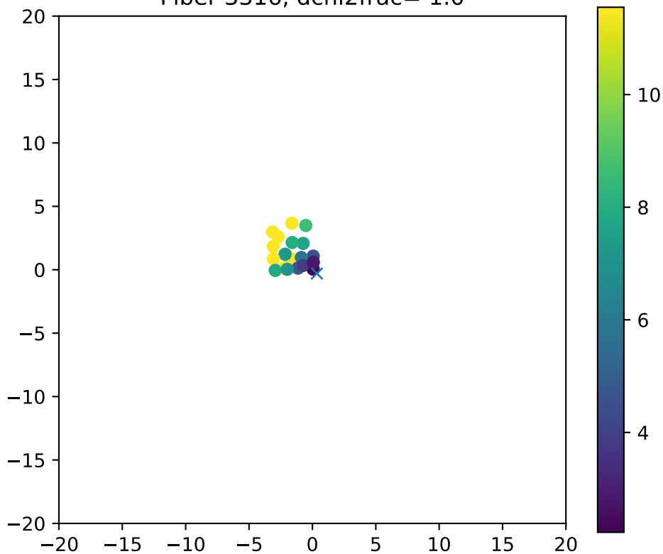
Fiber 3316, dchi2frac= 1.0
