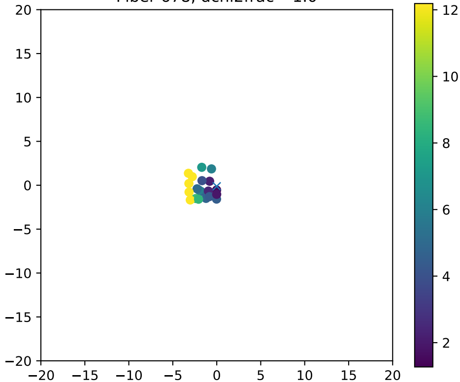
Fiber 678, dchi2frac= 1.0
