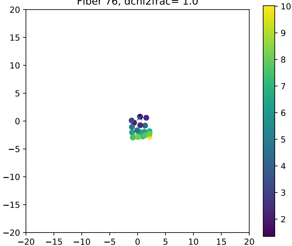
Fiber 76, dchi2frac= 1.0
