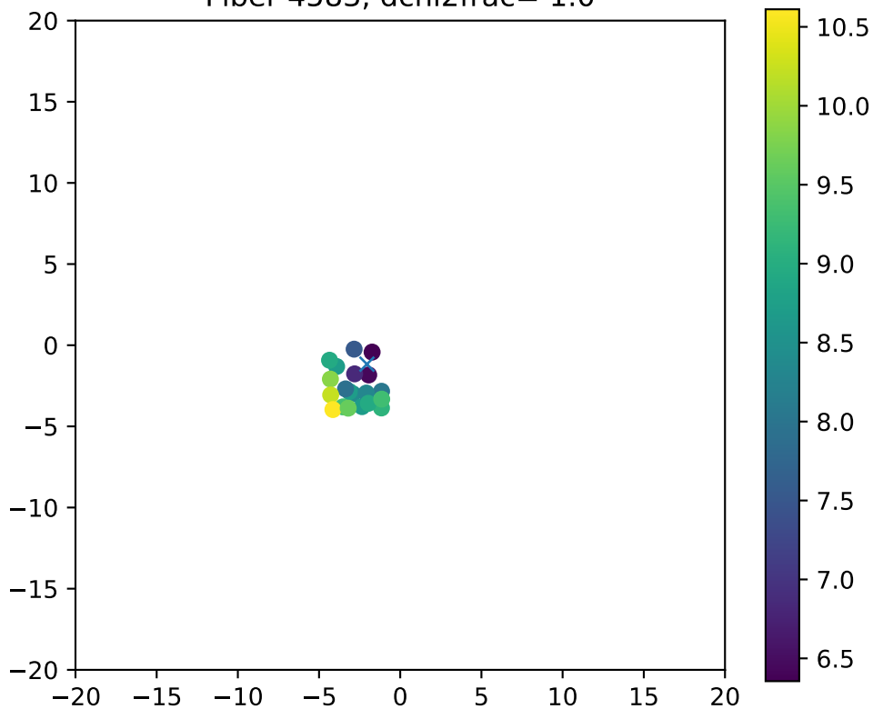
Fiber 4583, dchi2frac= 1.0
