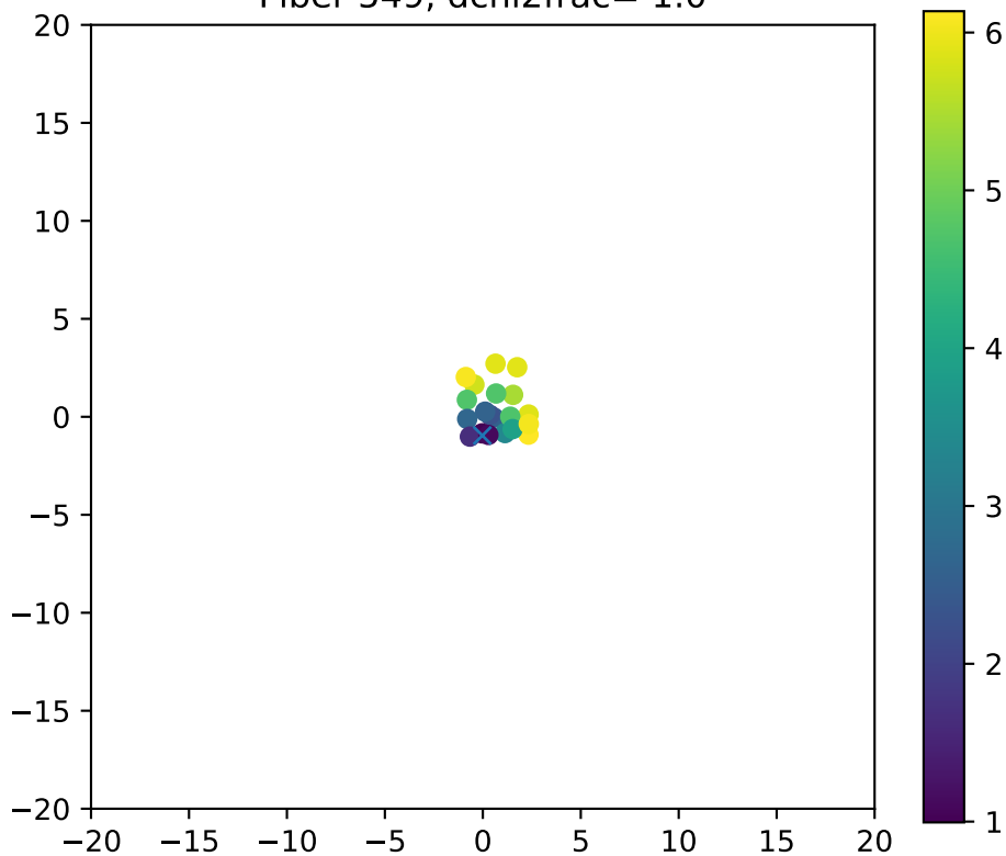
Fiber 549, dchi2frac= 1.0
