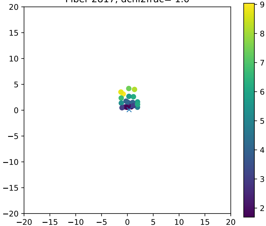
Fiber 2817, dchi2frac= 1.0
