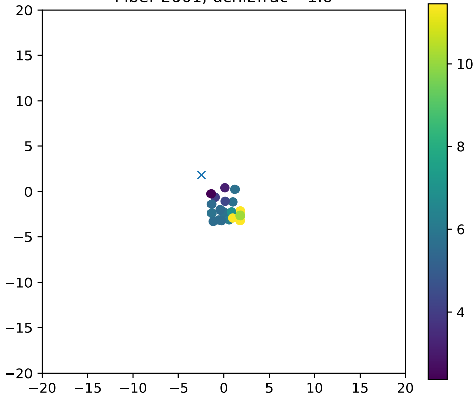
Fiber 2001, dchi2frac= 1.0
