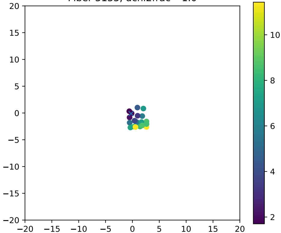
Fiber 3133, dchi2frac= 1.0
