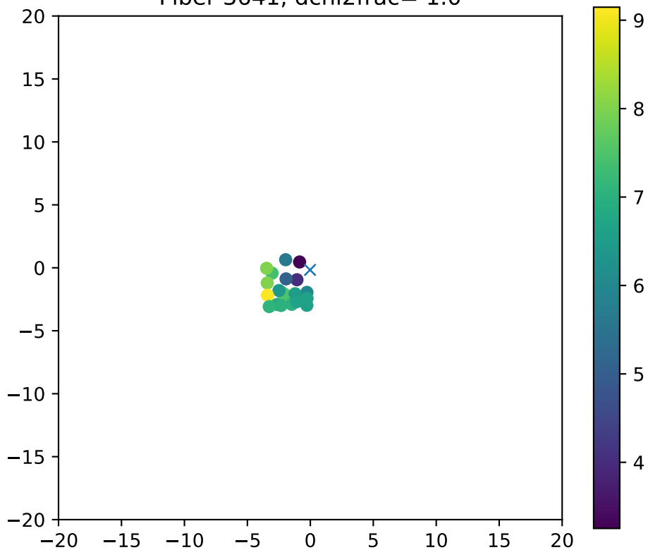
Fiber 3641, dchi2frac= 1.0
