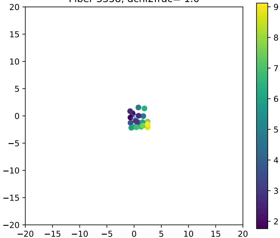
Fiber 3358, dchi2frac= 1.0
