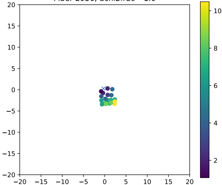
Fiber 2956, dchi2frac= 1.0
