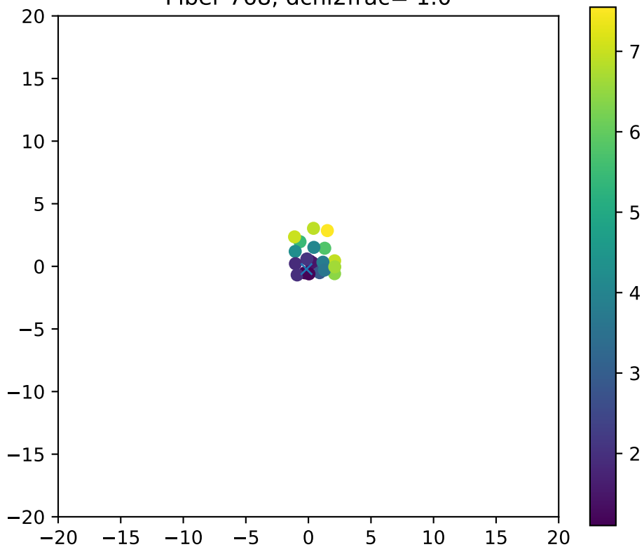
Fiber 768, dchi2frac= 1.0
