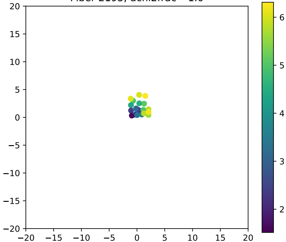
Fiber 2195, dchi2frac= 1.0
