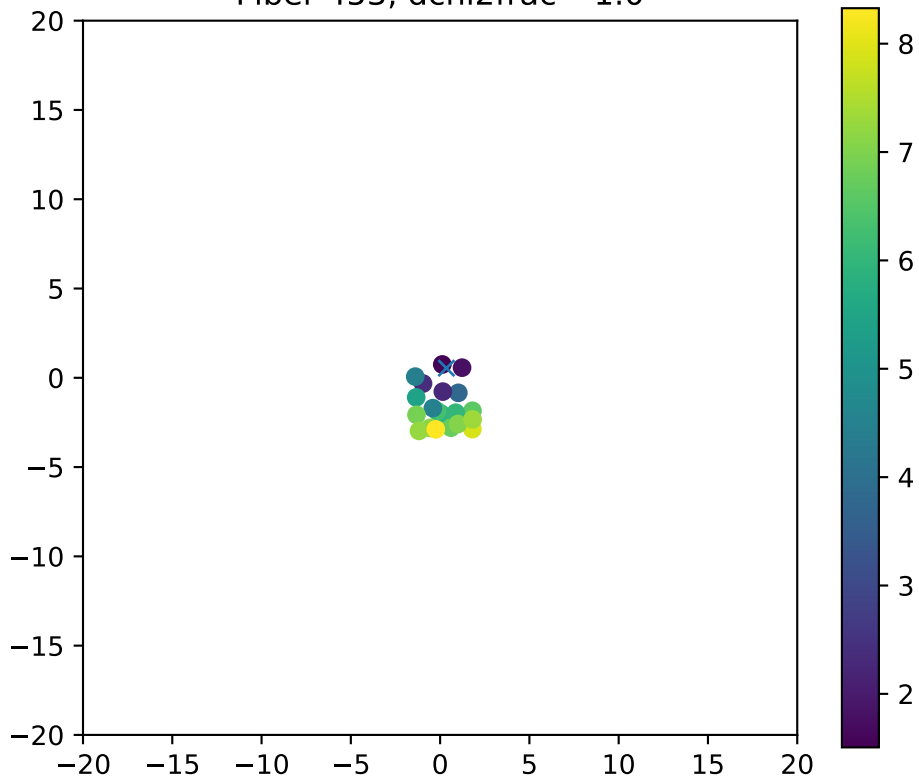
Fiber 453, dchi2frac= 1.0
