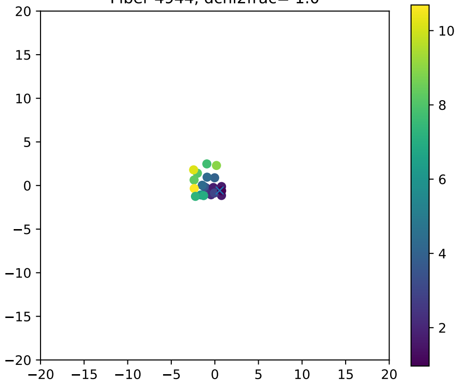
Fiber 4944, dchi2frac= 1.0
