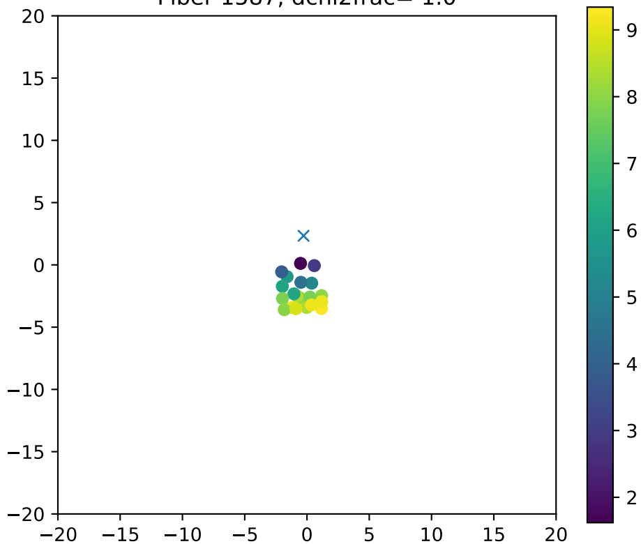
Fiber 1587, dchi2frac= 1.0
