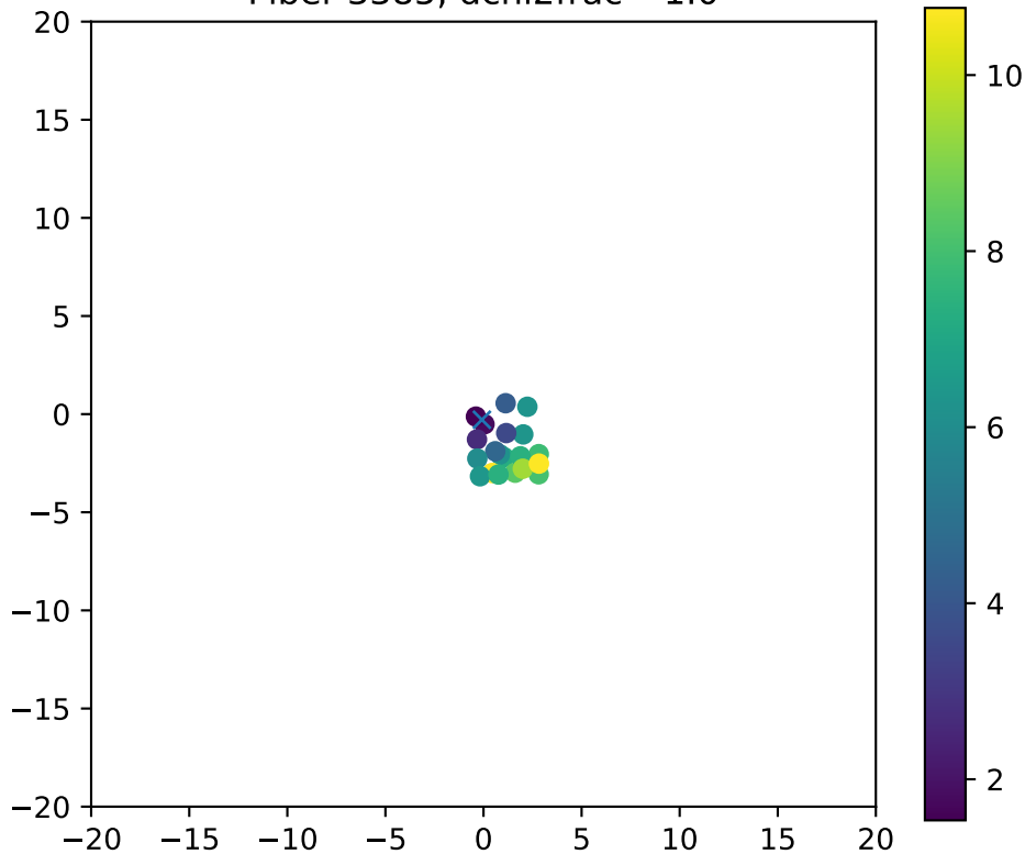
Fiber 3385, dchi2frac= 1.0
