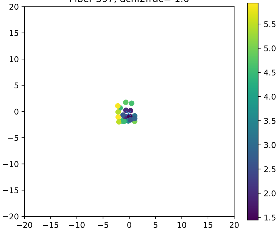
Fiber 397, dchi2frac= 1.0
