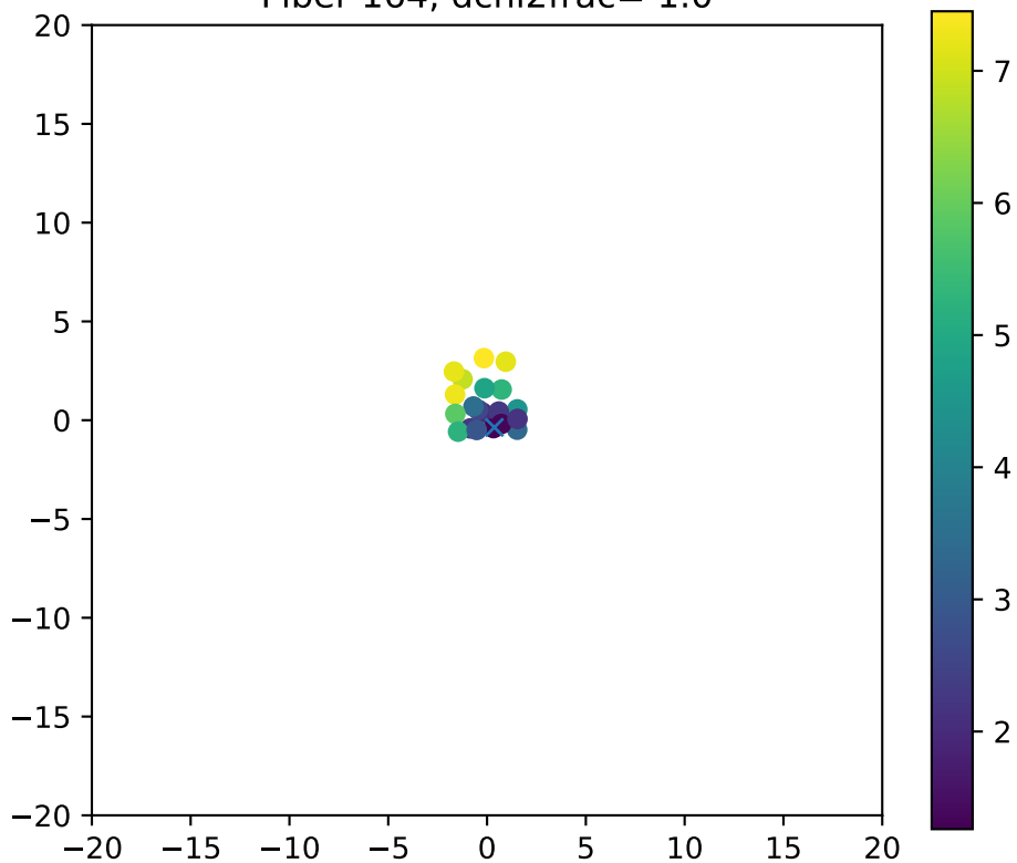
Fiber 164, dchi2frac= 1.0
