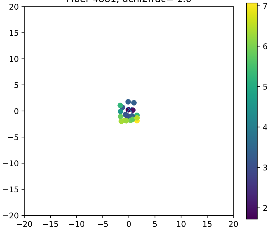
Fiber 4881, dchi2frac= 1.0
