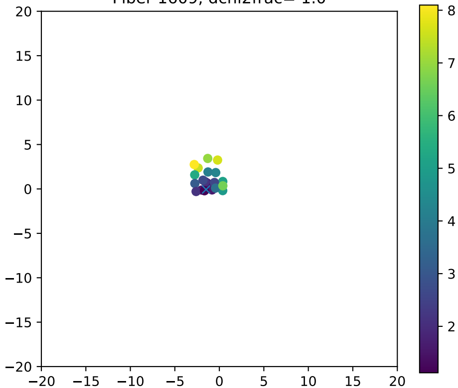
Fiber 1609, dchi2frac= 1.0
