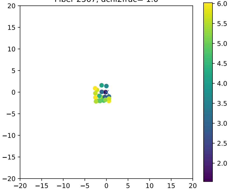
Fiber 2567, dchi2frac= 1.0
