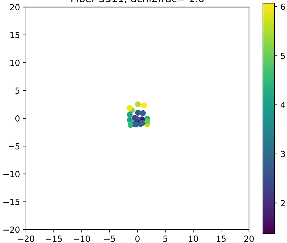
Fiber 3511, dchi2frac= 1.0
