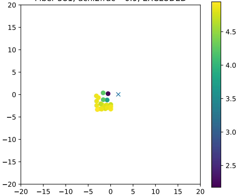
Fiber 581, dchi2frac= 0.9, EXCLUDED
