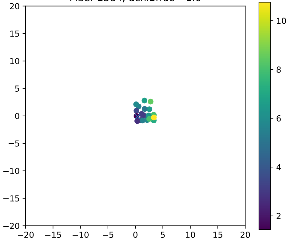
Fiber 2584, dchi2frac= 1.0
