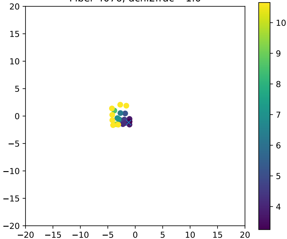
Fiber 4076, dchi2frac= 1.0
