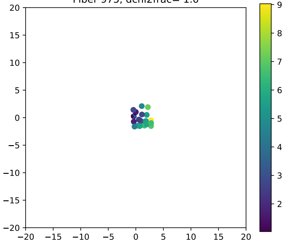
Fiber 975, dchi2frac= 1.0
