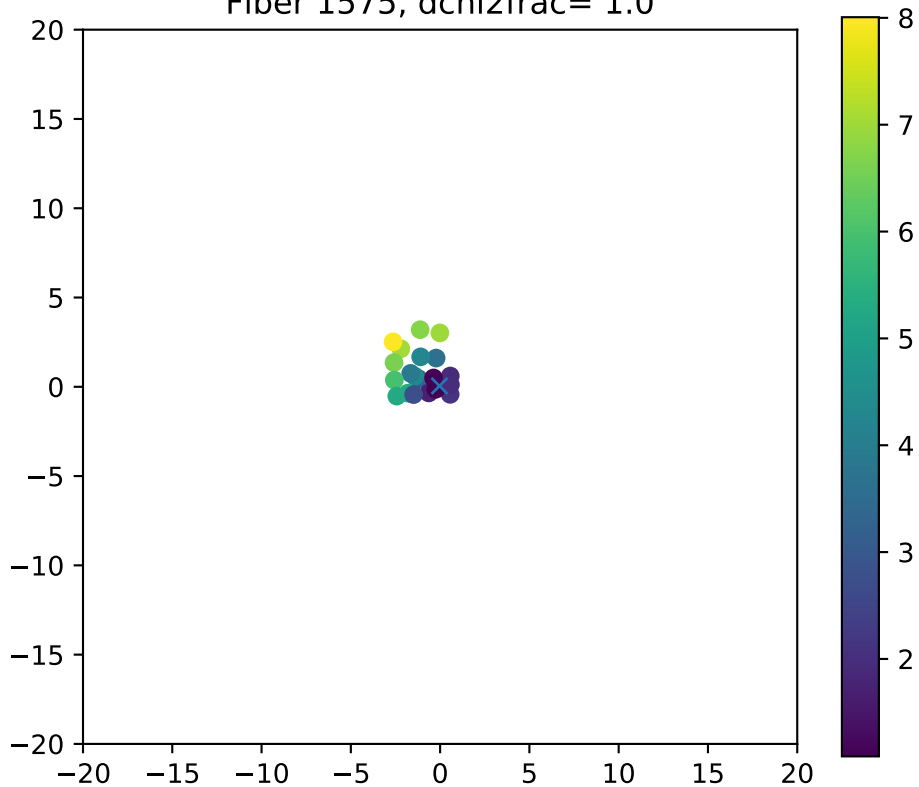
Fiber 1575, dchi2frac= 1.0
