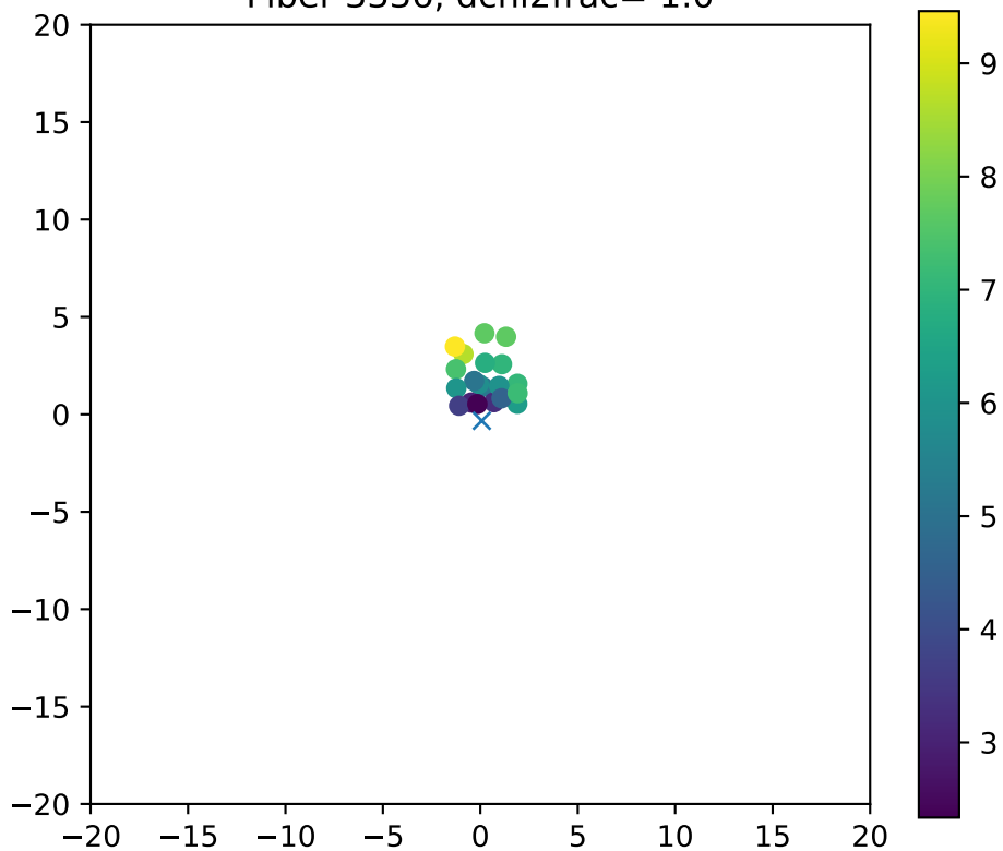
Fiber 3336, dchi2frac= 1.0
