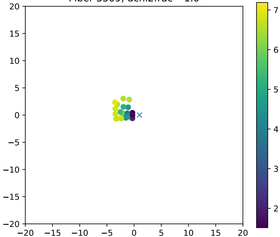
Fiber 3509, dchi2frac= 1.0
