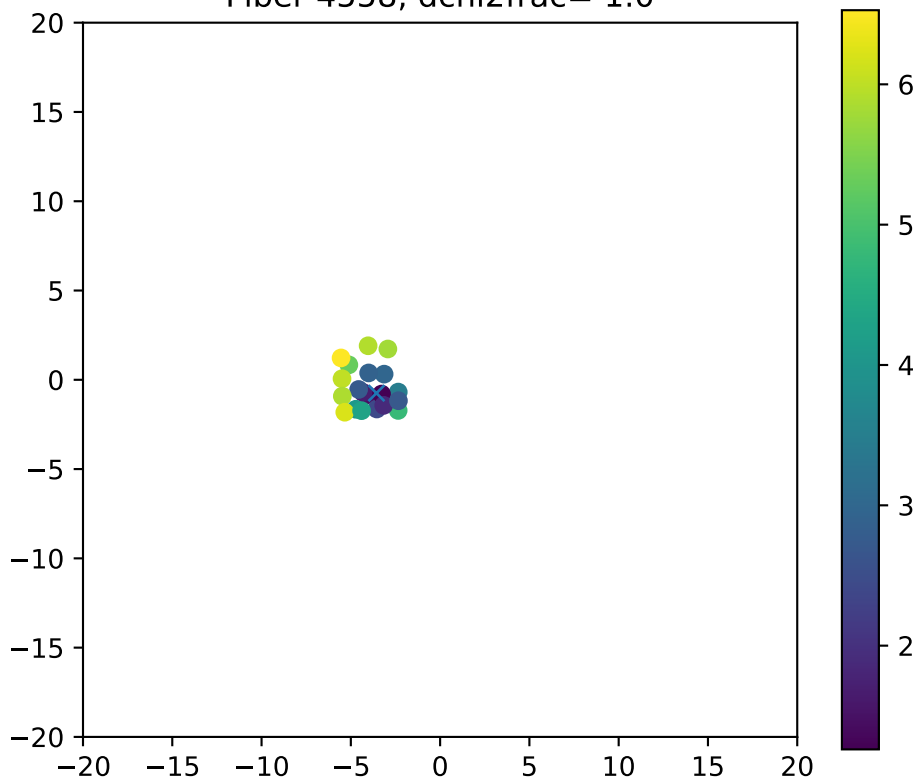
Fiber 4558, dchi2frac= 1.0
