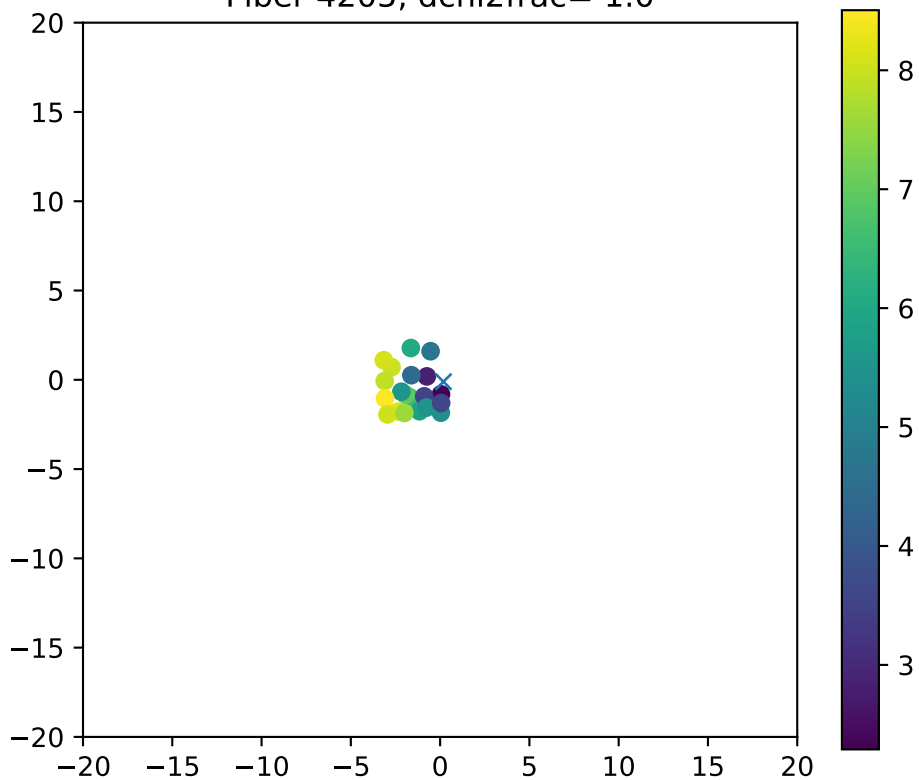
Fiber 4205, dchi2frac= 1.0
