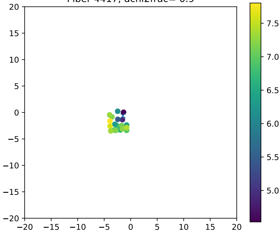
Fiber 4417, dchi2frac= 0.9
