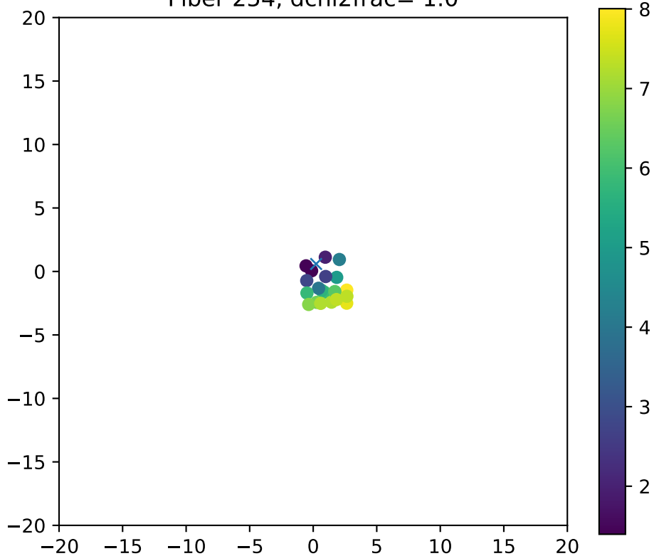
Fiber 254, dchi2frac= 1.0
