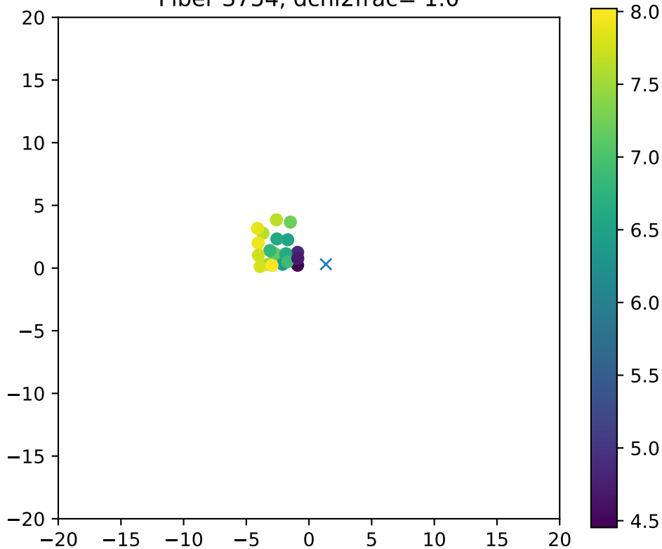
Fiber 3754, dchi2frac= 1.0
