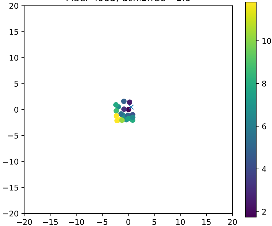
Fiber 4953, dchi2frac= 1.0
