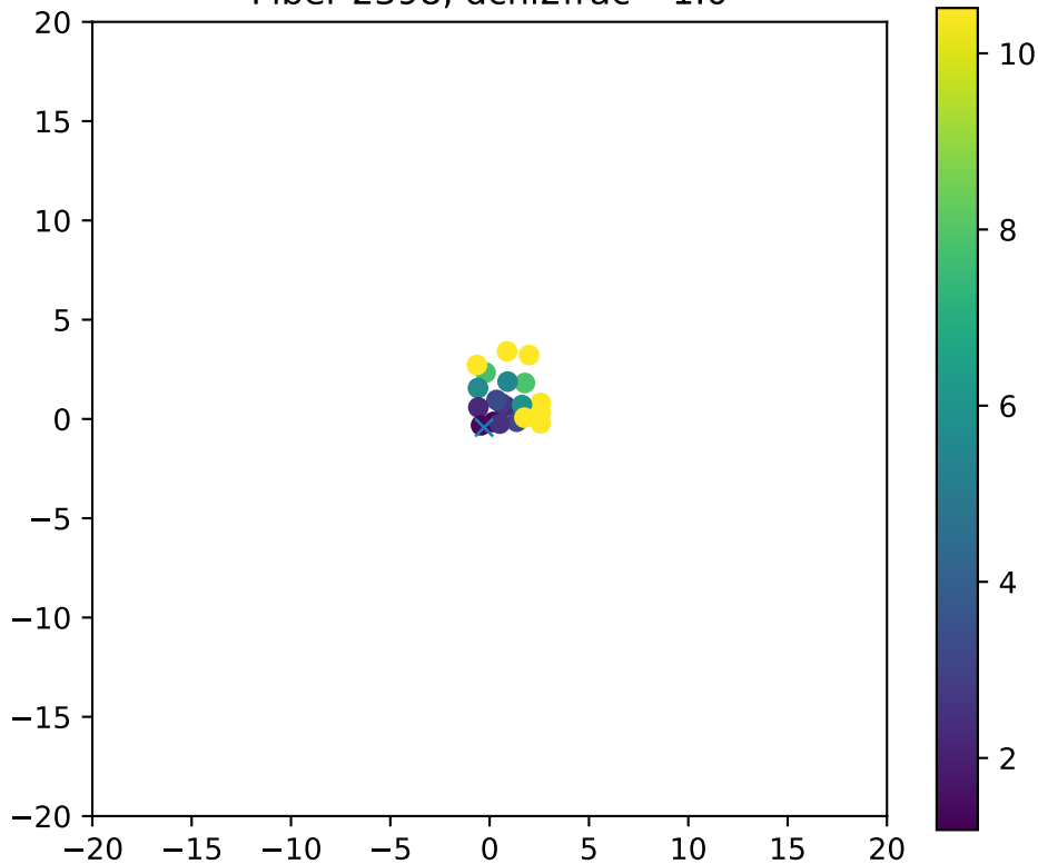
Fiber 2398, dchi2frac= 1.0
