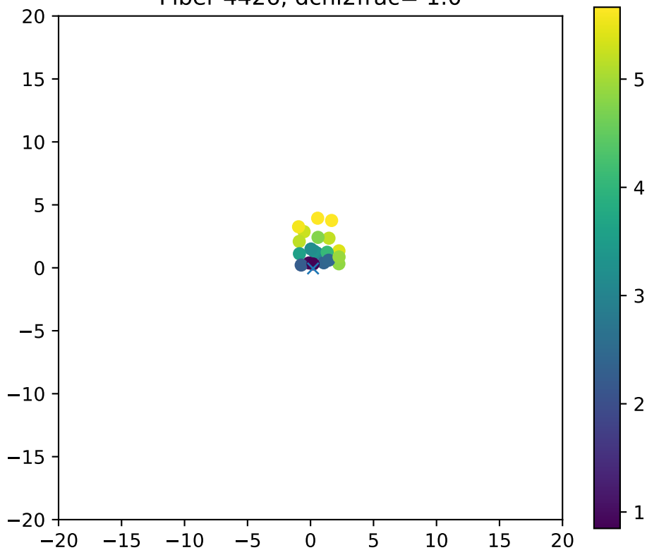
Fiber 4426, dchi2frac= 1.0
