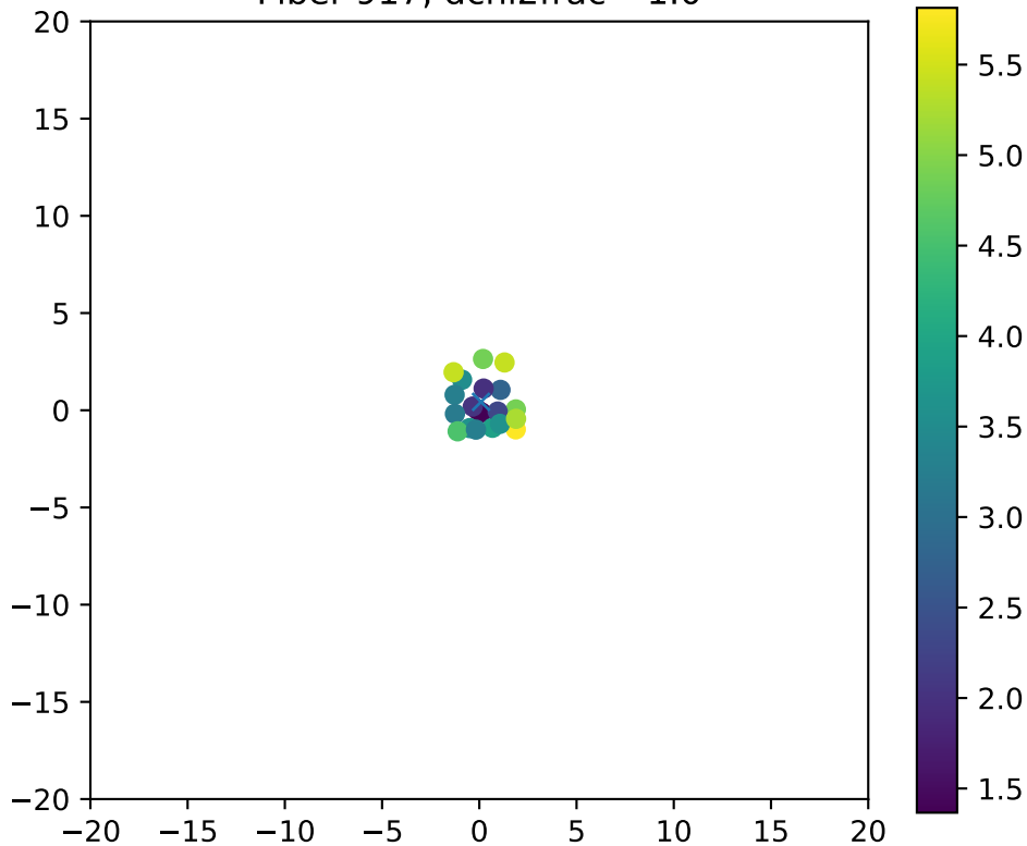
Fiber 917, dchi2frac= 1.0
