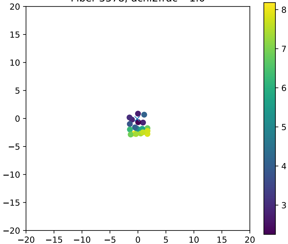
Fiber 3378, dchi2frac= 1.0
