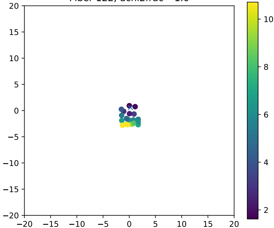
Fiber 122, dchi2frac= 1.0
