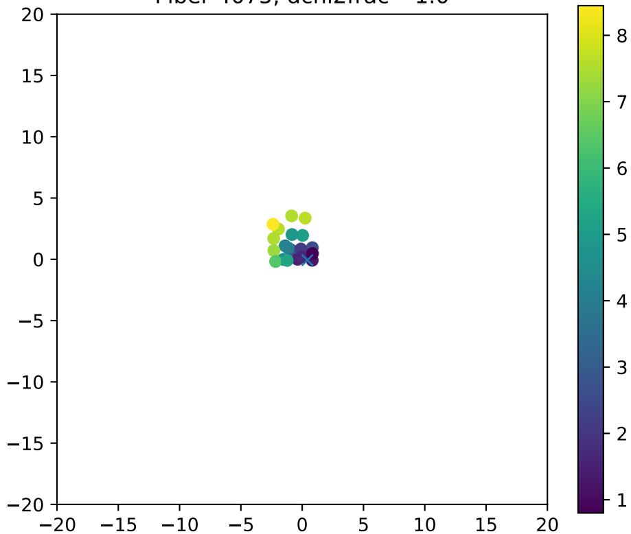
Fiber 4075, dchi2frac= 1.0
