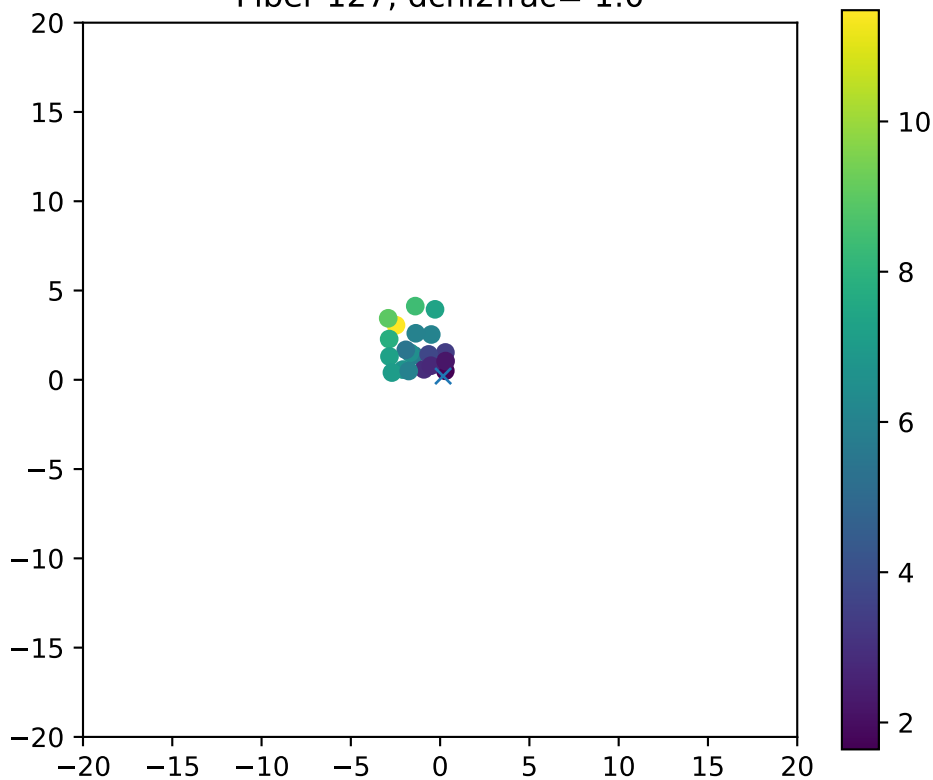
Fiber 127, dchi2frac= 1.0
