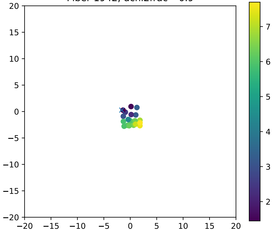
Fiber 1942, dchi2frac= 0.9
