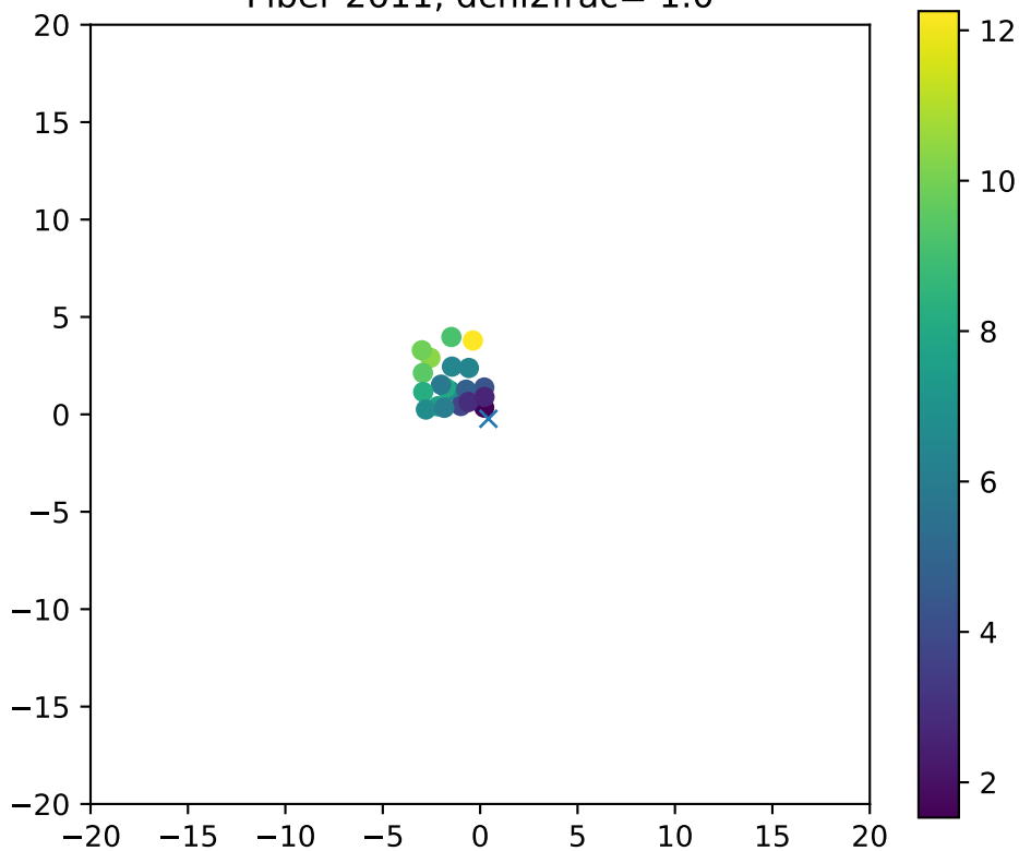
Fiber 2611, dchi2frac= 1.0
