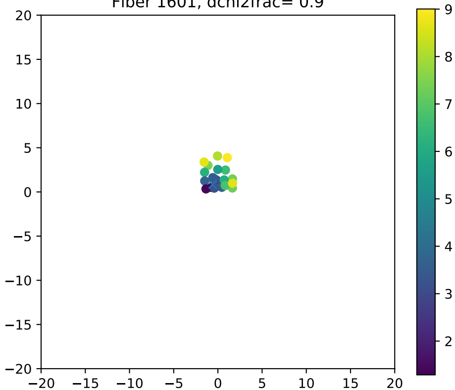
Fiber 1601, dchi2frac= 0.9
