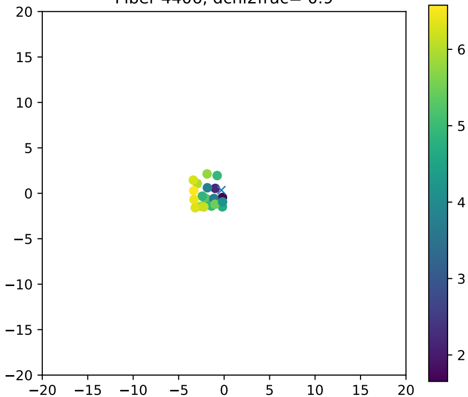
Fiber 4406, dchi2frac= 0.9
