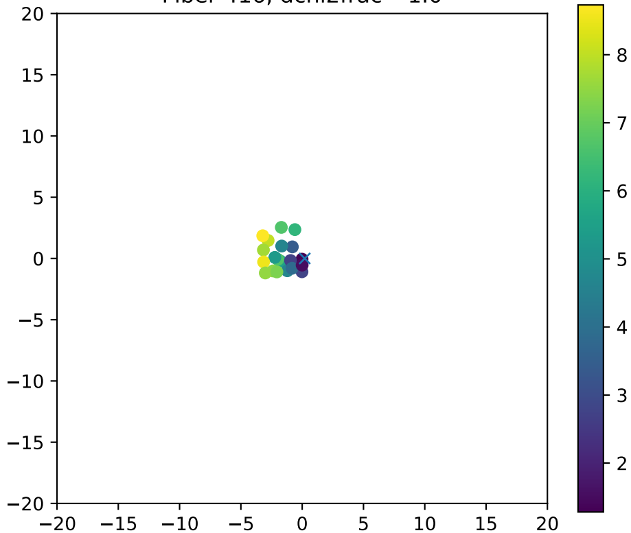
Fiber 416, dchi2frac= 1.0
