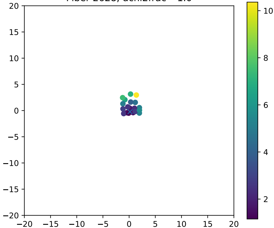
Fiber 2628, dchi2frac= 1.0
