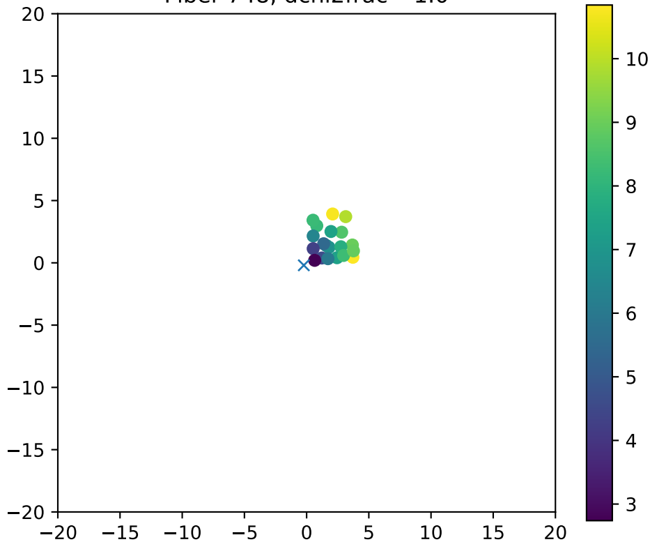
Fiber 748, dchi2frac= 1.0
