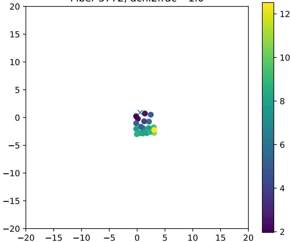
Fiber 3772, dchi2frac= 1.0
