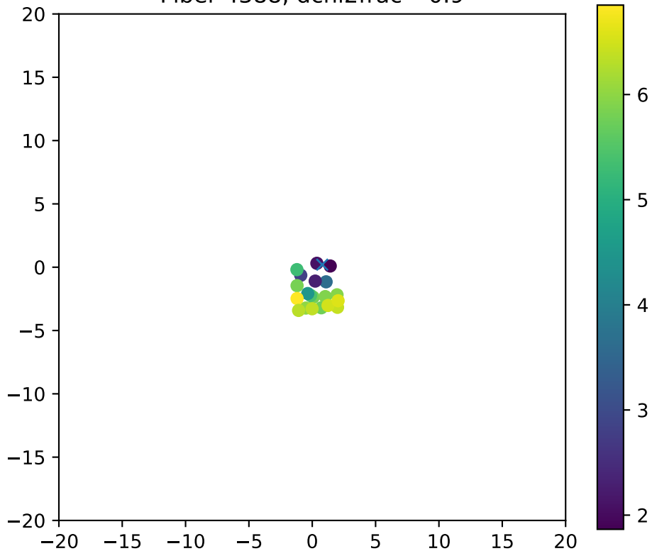
Fiber 4388, dchi2frac= 0.9
