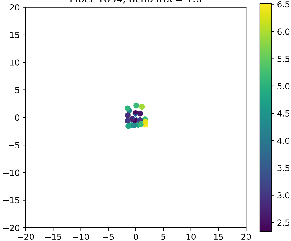
Fiber 1834, dchi2frac= 1.0
