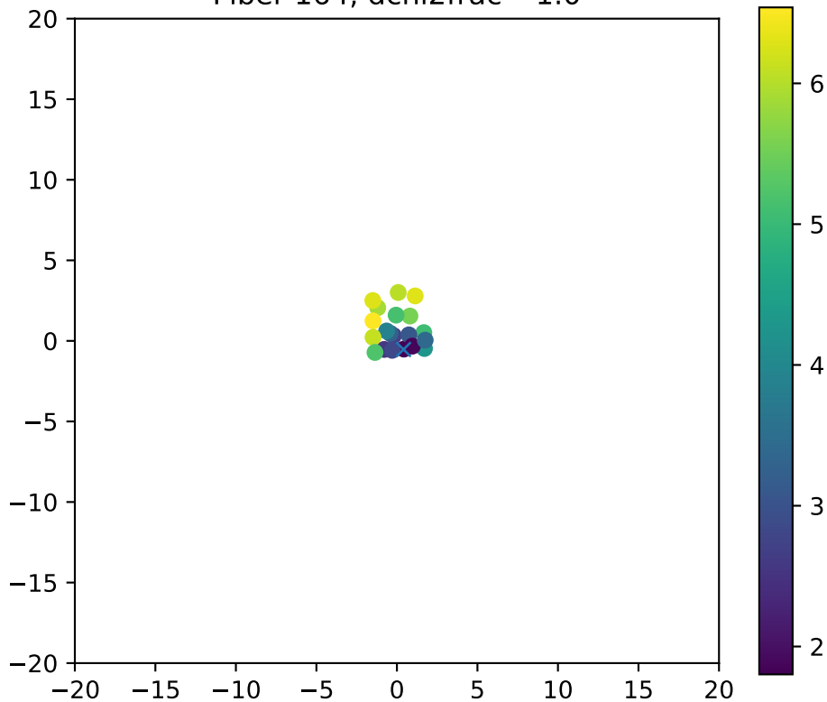
Fiber 164, dchi2frac= 1.0
