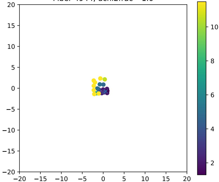
Fiber 4944, dchi2frac= 1.0
