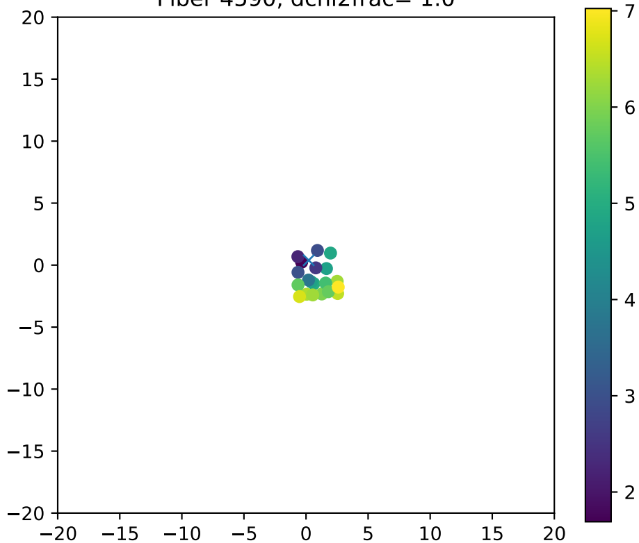
Fiber 4590, dchi2frac= 1.0
