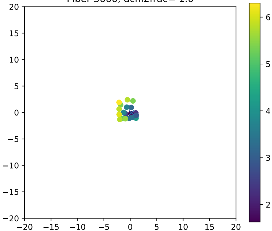
Fiber 3666, dchi2frac= 1.0
