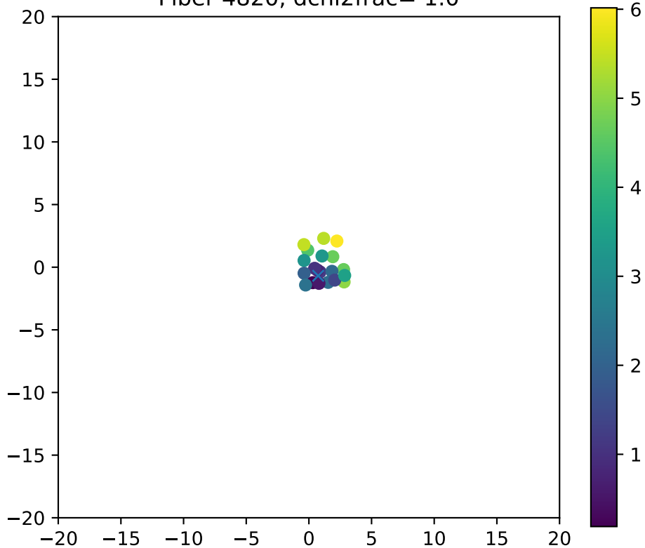
Fiber 4820, dchi2frac= 1.0
