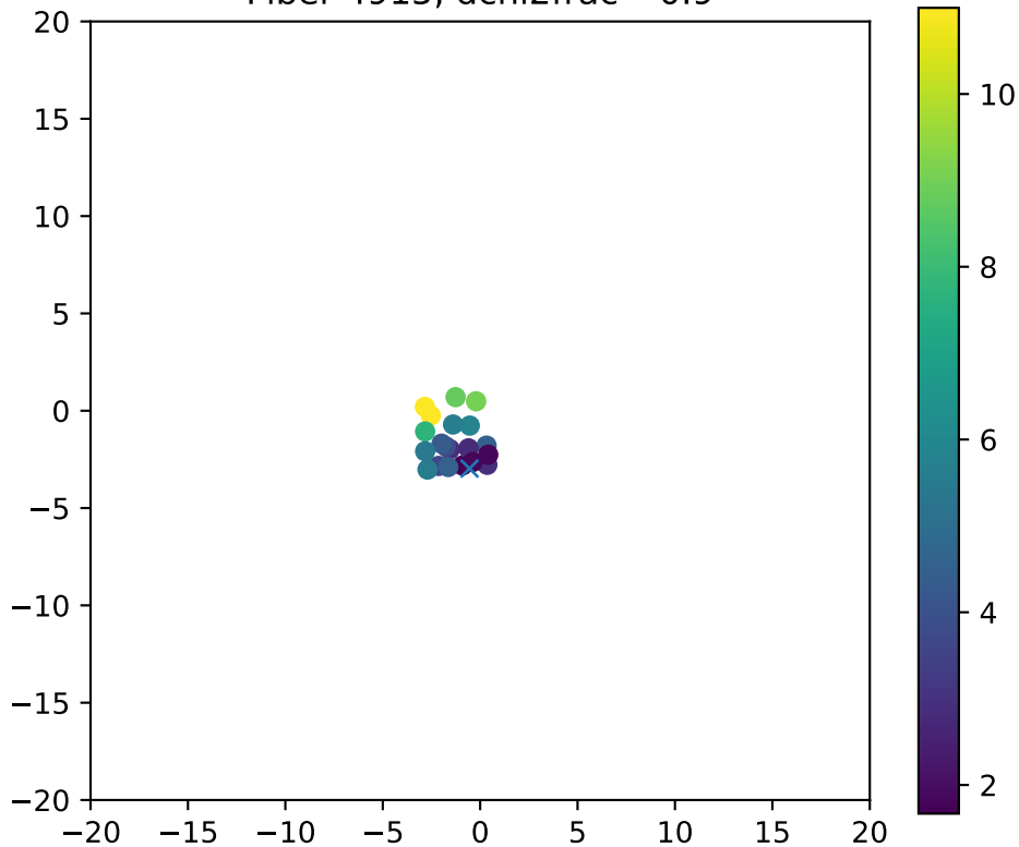
Fiber 4915, dchi2frac= 0.9
