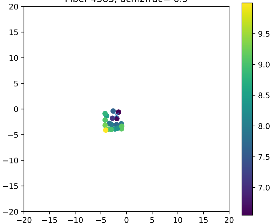
Fiber 4583, dchi2frac= 0.9
