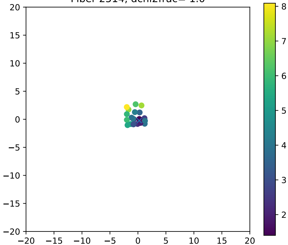
Fiber 2514, dchi2frac= 1.0
