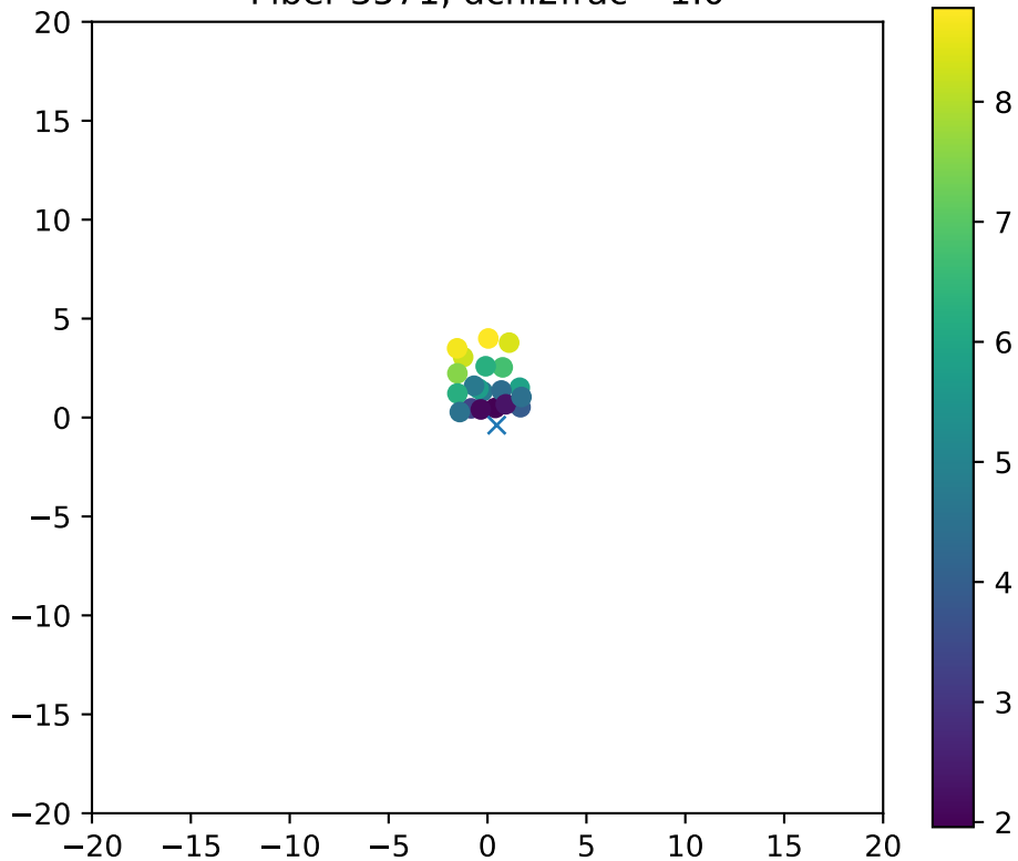
Fiber 3571, dchi2frac= 1.0
