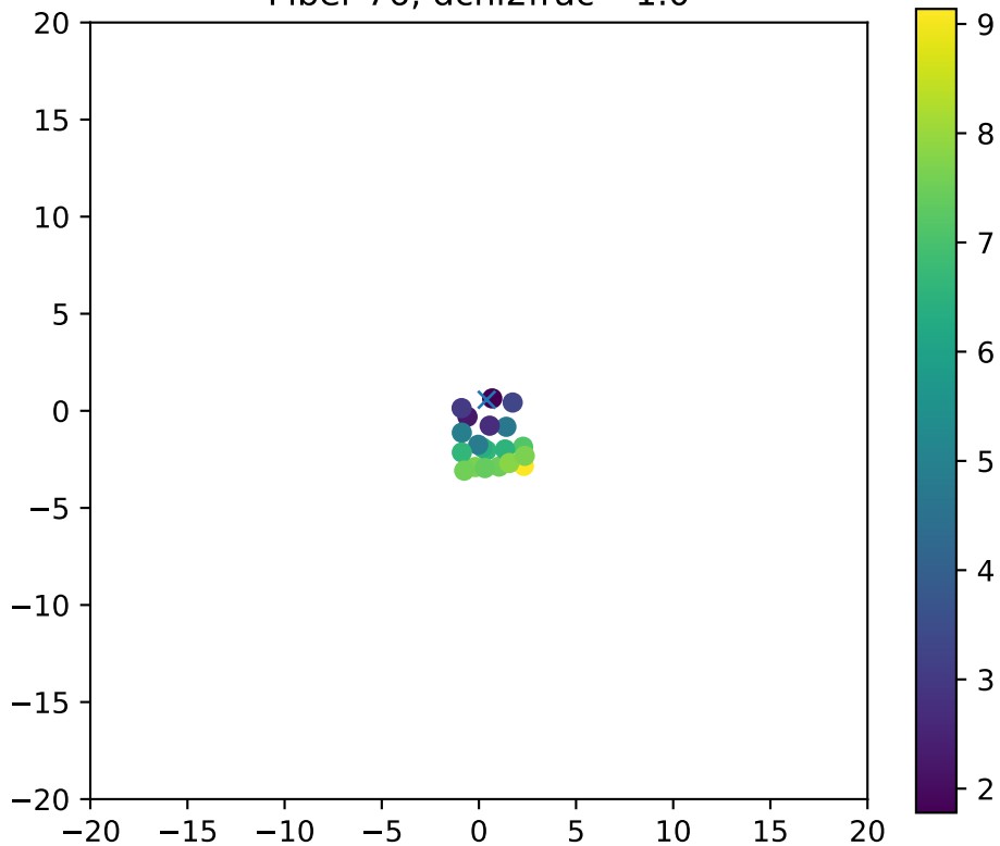
Fiber 76, dchi2frac= 1.0
