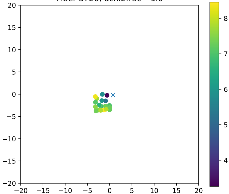
Fiber 3726, dchi2frac= 1.0
