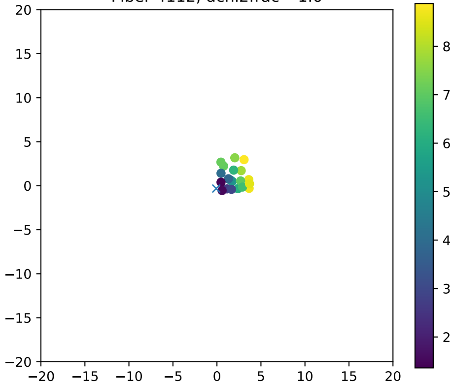
Fiber 4112, dchi2frac= 1.0
