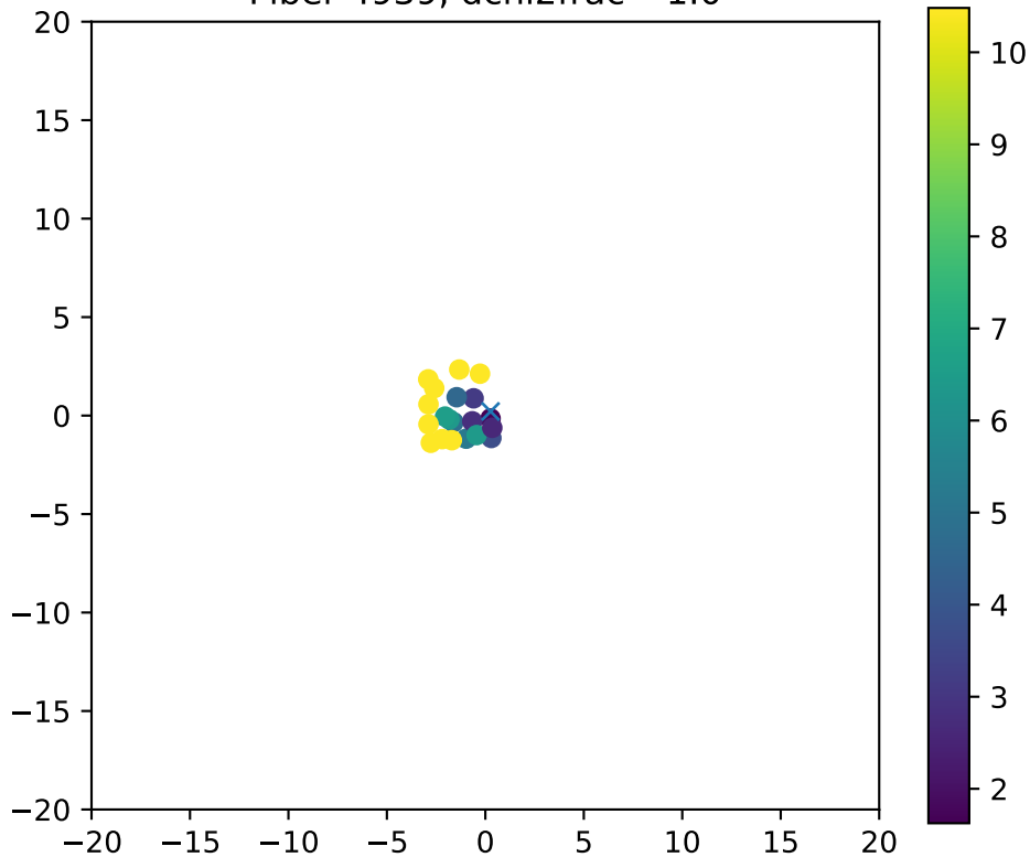
Fiber 4939, dchi2frac= 1.0
