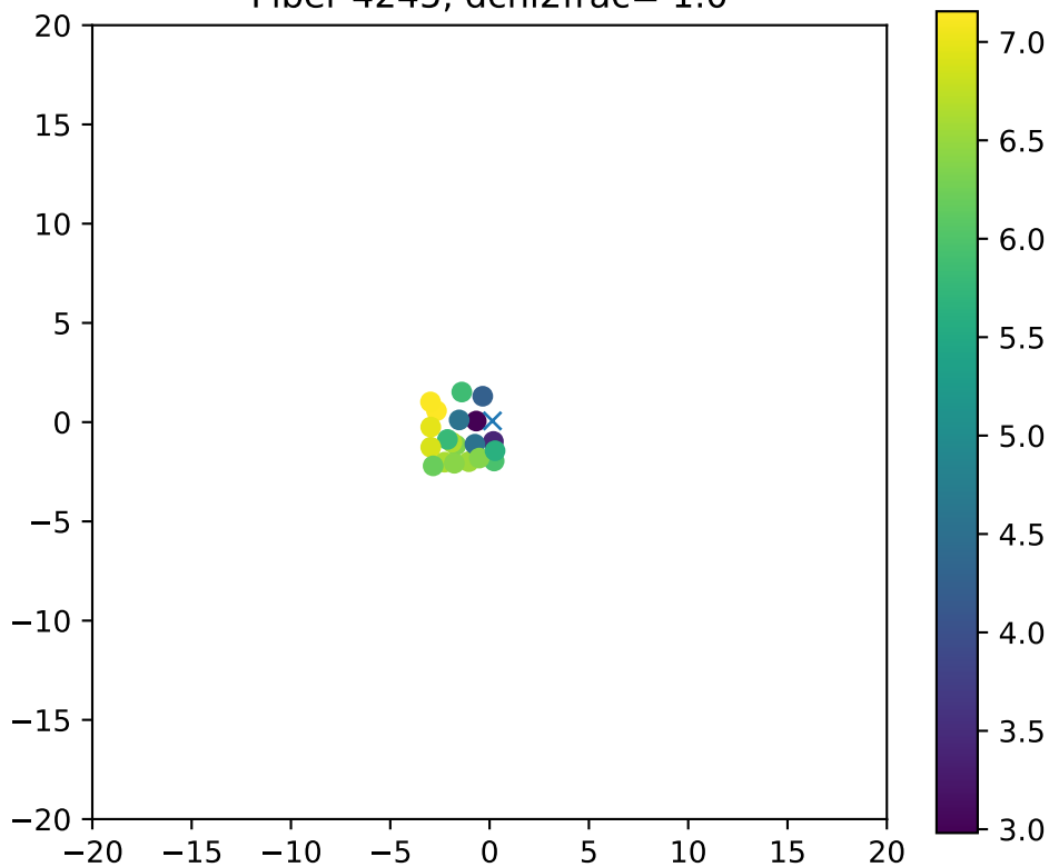
Fiber 4245, dchi2frac= 1.0
