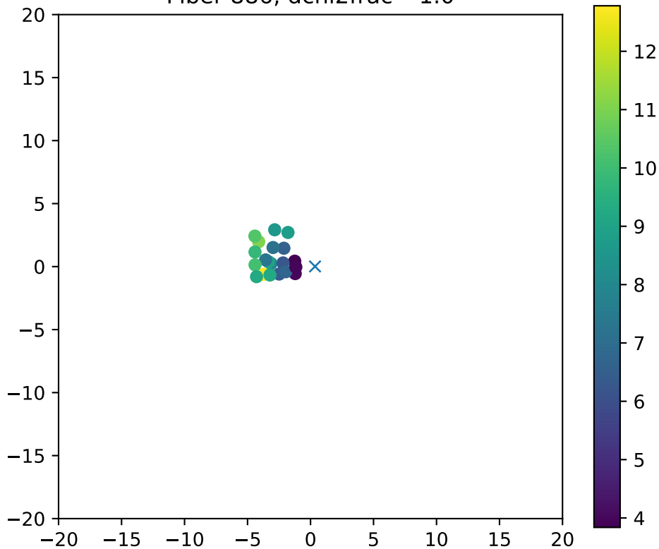
Fiber 886, dchi2frac= 1.0
