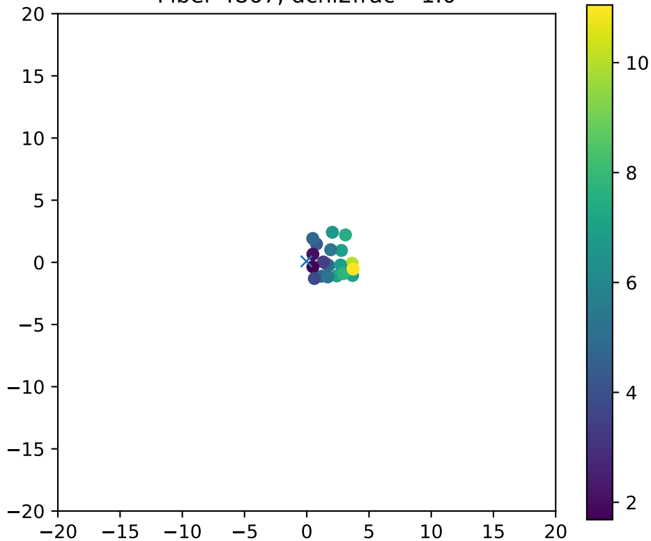
Fiber 4867, dchi2frac= 1.0
