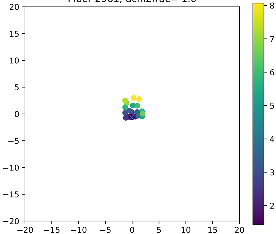
Fiber 2961, dchi2frac= 1.0
