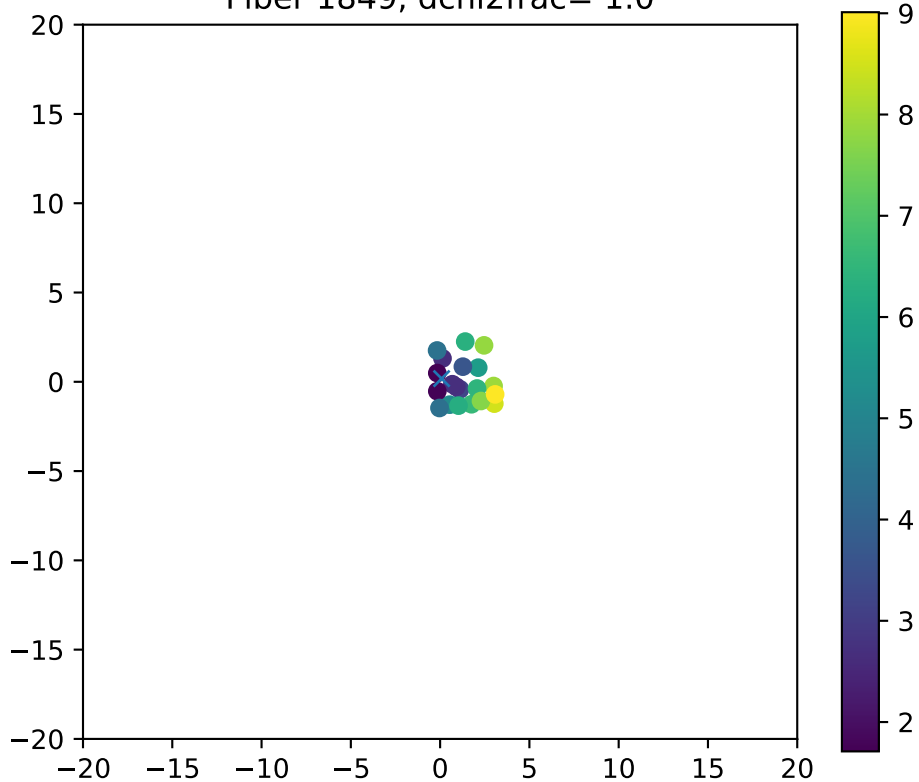
Fiber 1849, dchi2frac= 1.0
