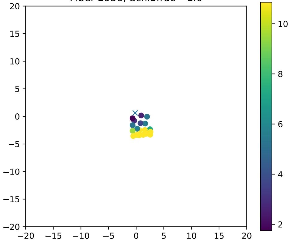
Fiber 2956, dchi2frac= 1.0
