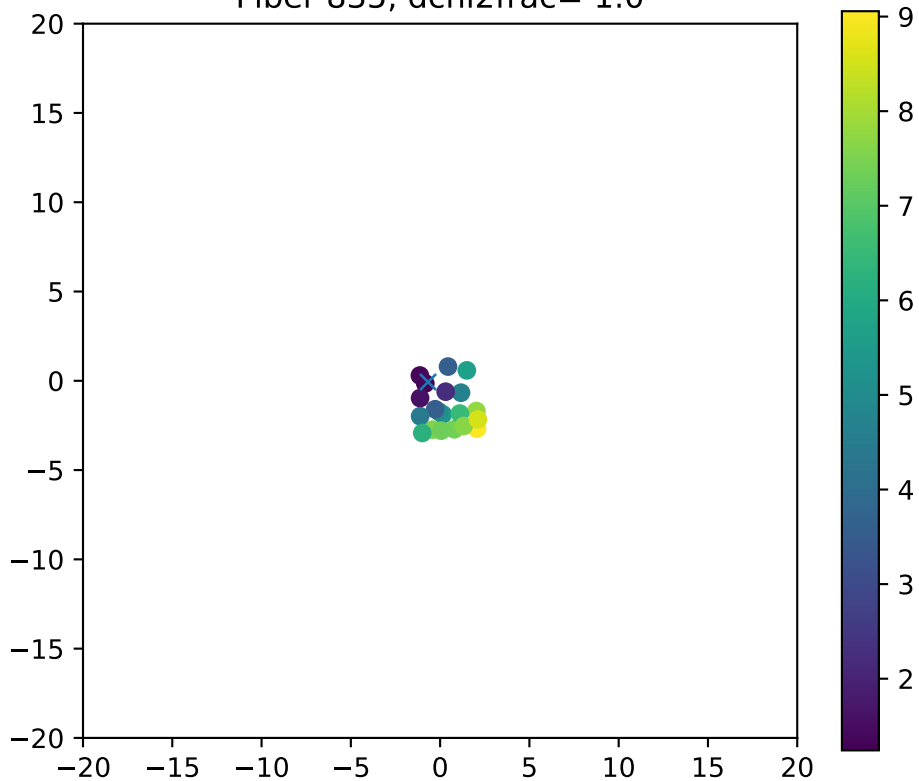
Fiber 835, dchi2frac= 1.0
