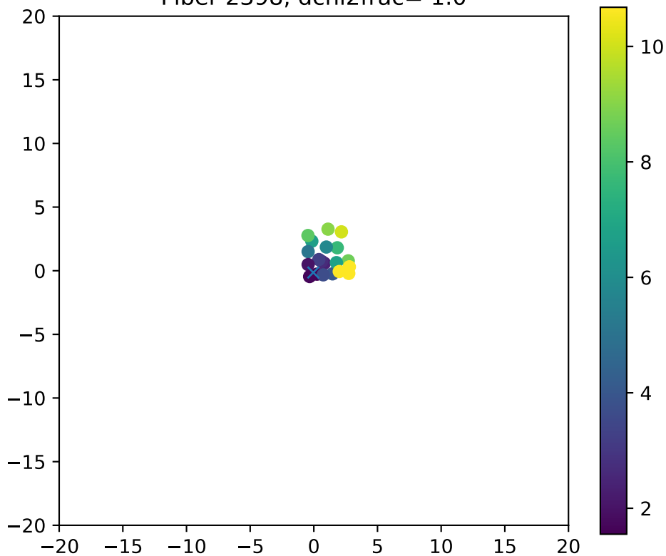
Fiber 2398, dchi2frac= 1.0
