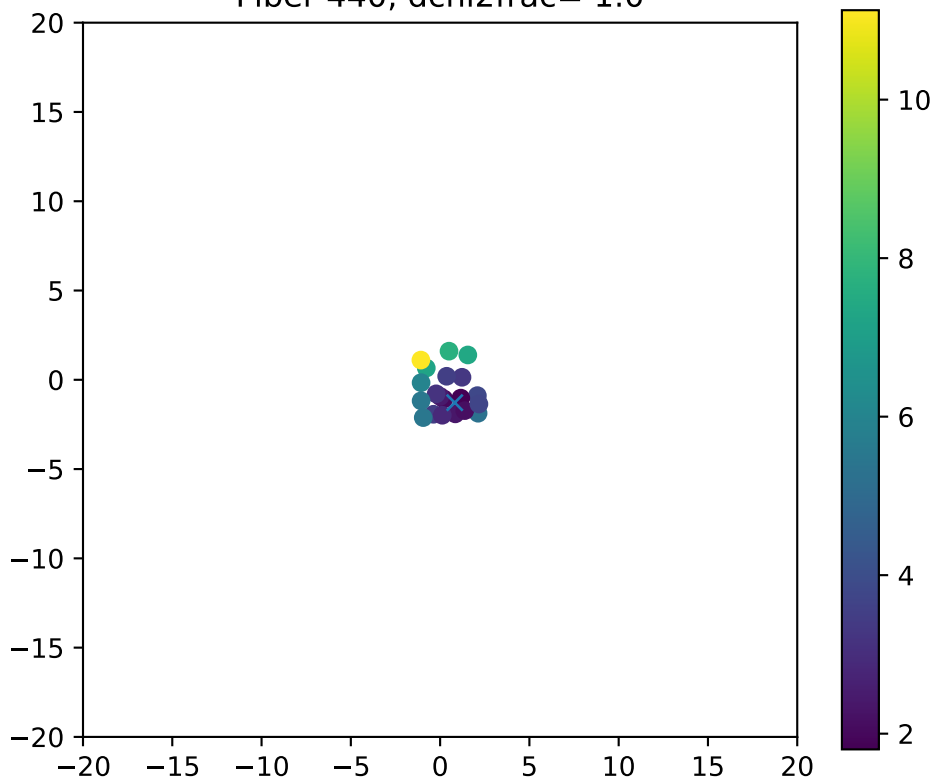
Fiber 440, dchi2frac= 1.0
