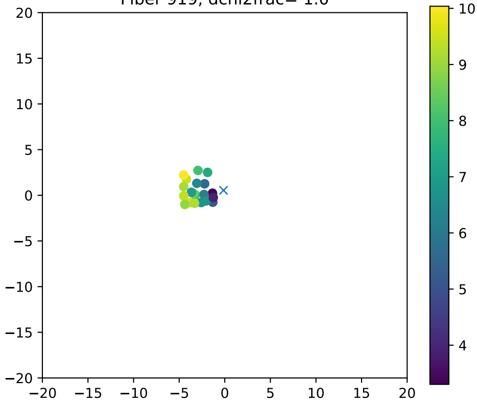
Fiber 919, dchi2frac= 1.0
