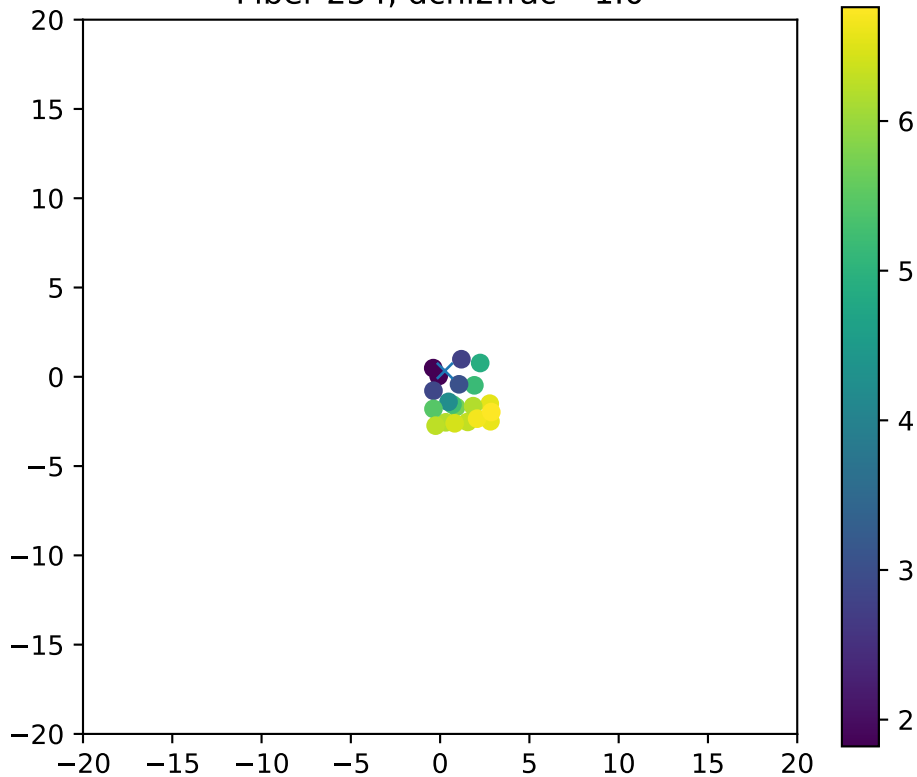
Fiber 254, dchi2frac= 1.0
