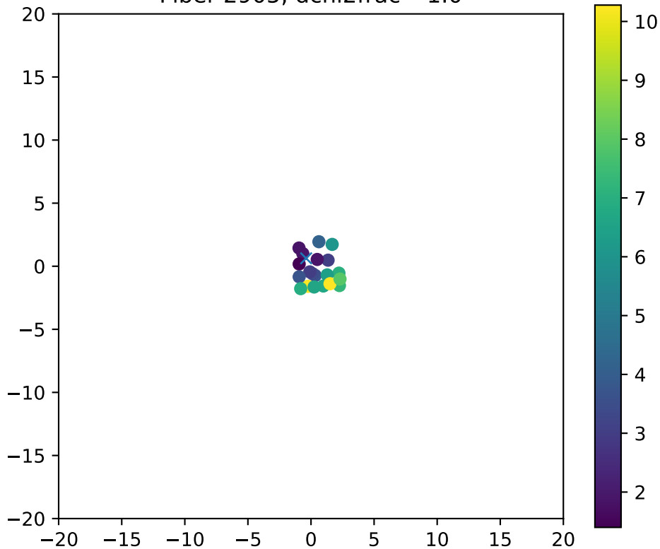
Fiber 2905, dchi2frac= 1.0
