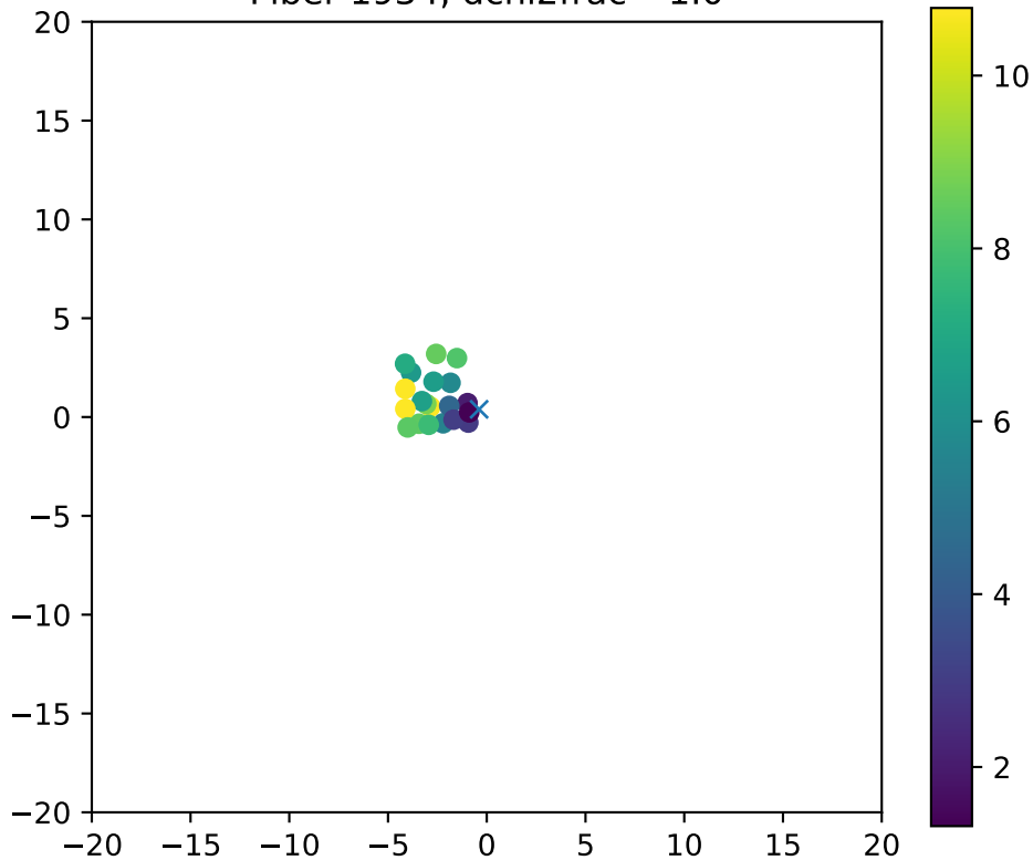
Fiber 1934, dchi2frac= 1.0
