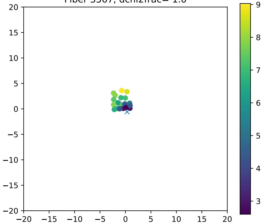
Fiber 3367, dchi2frac= 1.0
