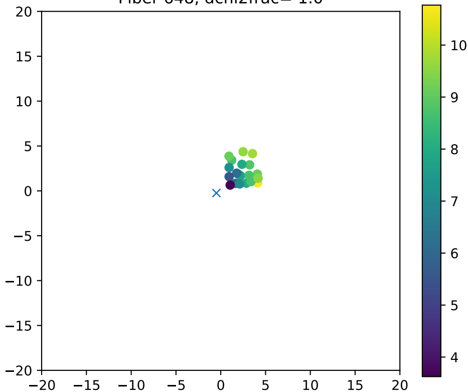
Fiber 648, dchi2frac= 1.0
