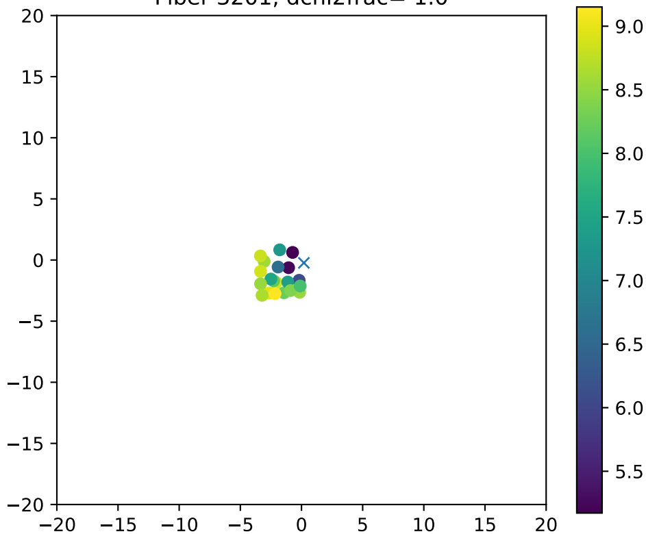
Fiber 3201, dchi2frac= 1.0
