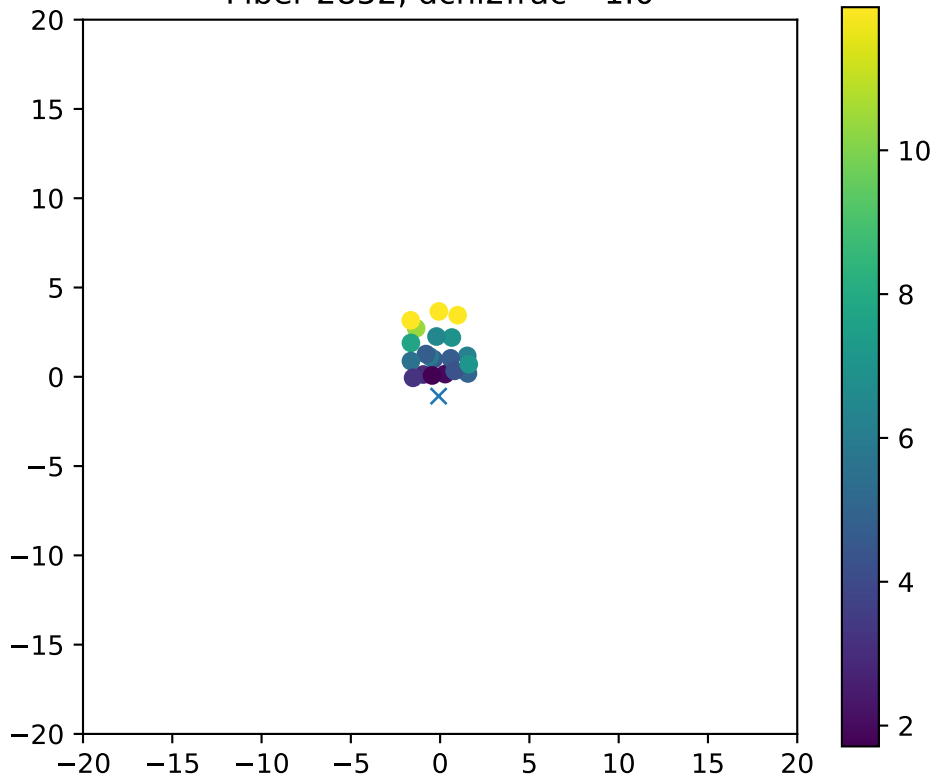
Fiber 2852, dchi2frac= 1.0
