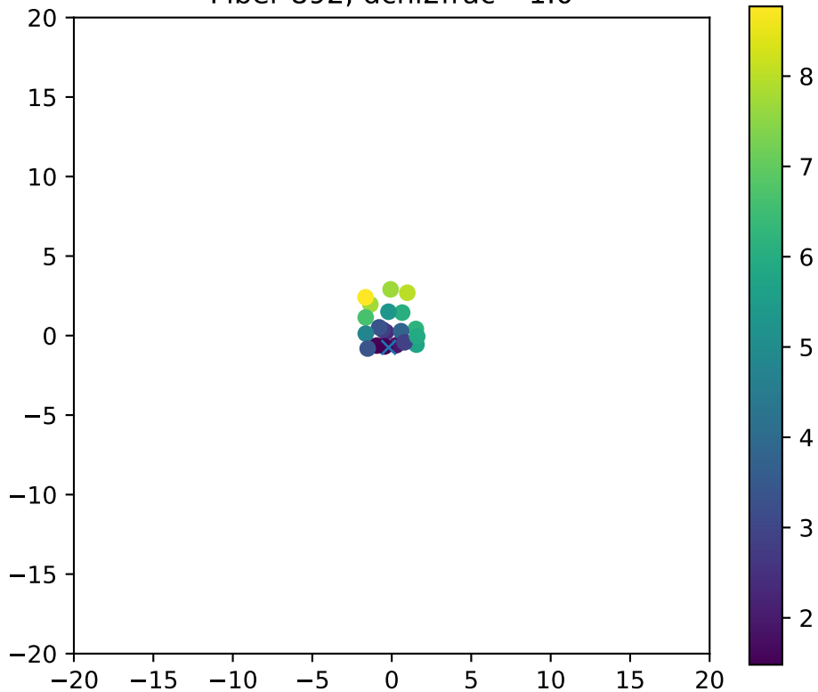
Fiber 892, dchi2frac= 1.0
