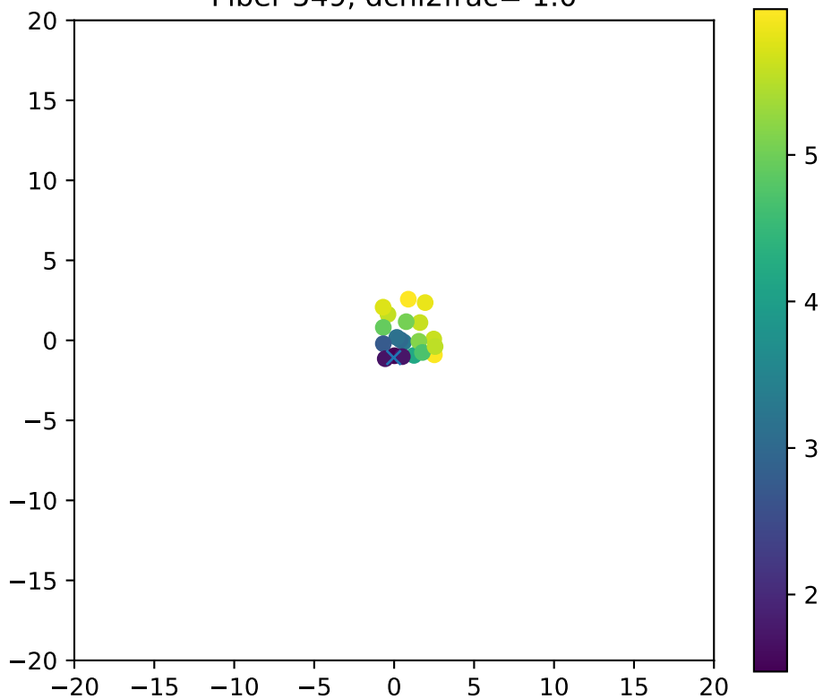
Fiber 549, dchi2frac= 1.0
