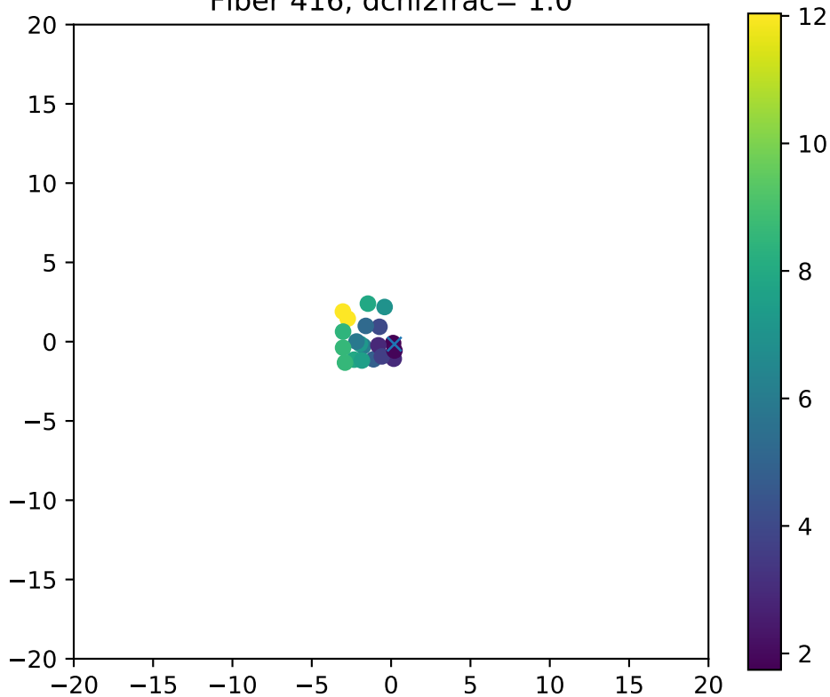
Fiber 416, dchi2frac= 1.0
