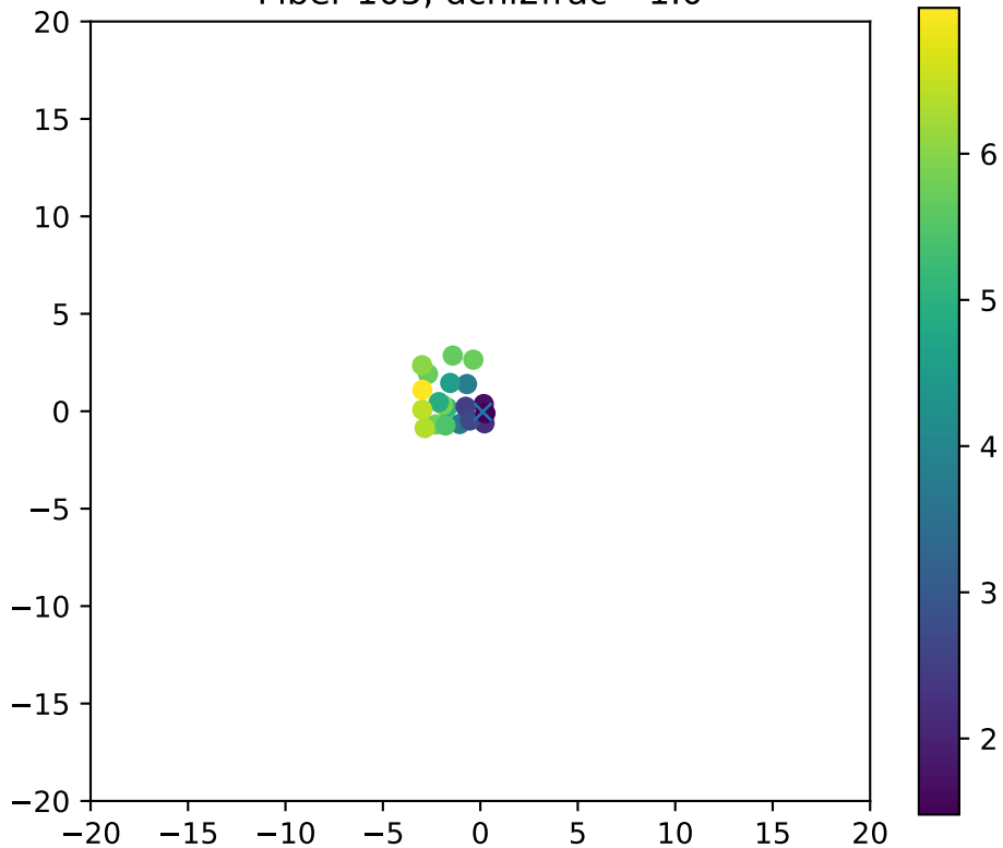
Fiber 105, dchi2frac= 1.0
