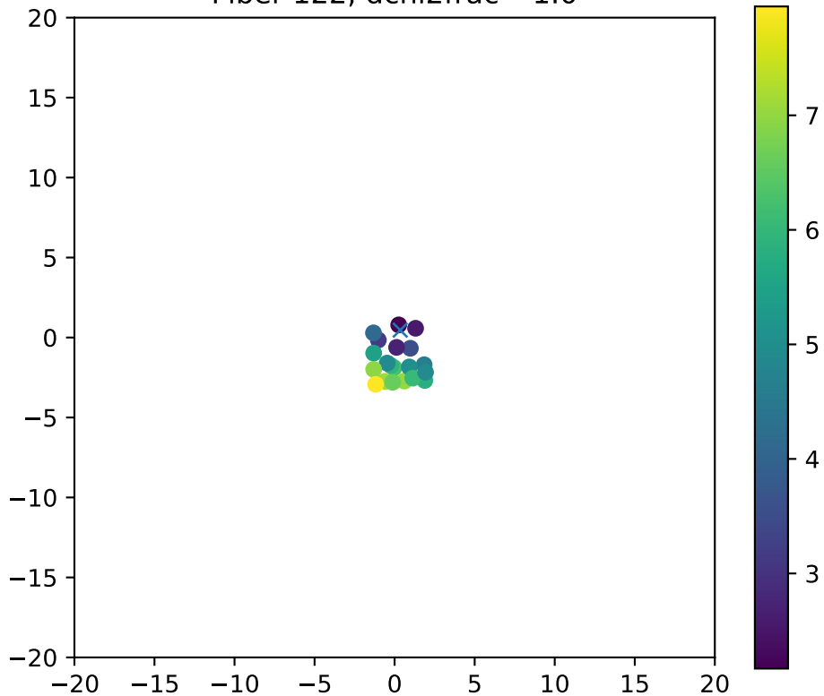
Fiber 122, dchi2frac= 1.0
