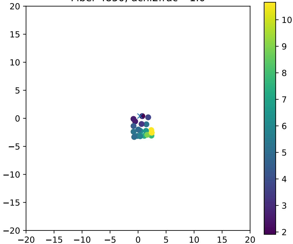
Fiber 4850, dchi2frac= 1.0
