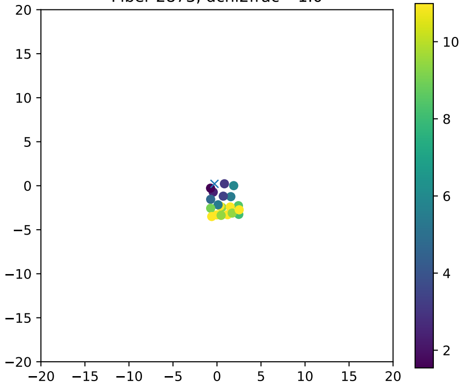
Fiber 2873, dchi2frac= 1.0
