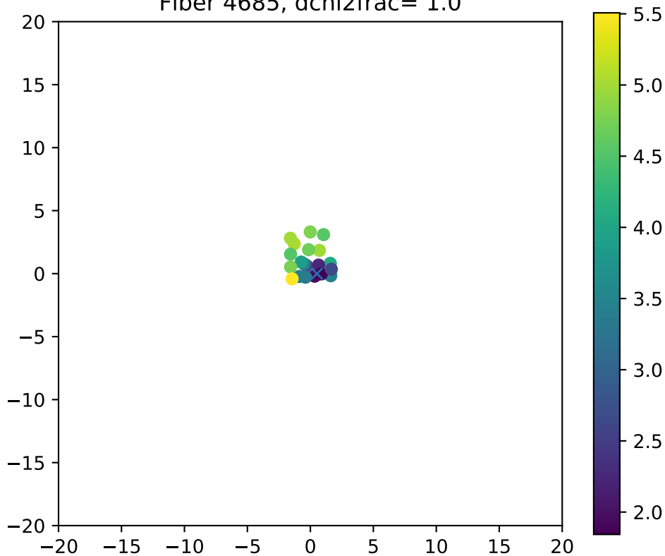
Fiber 4685, dchi2frac= 1.0
