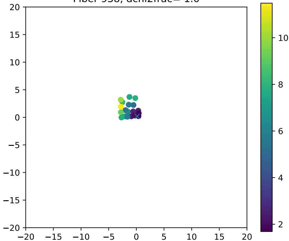
Fiber 938, dchi2frac= 1.0
