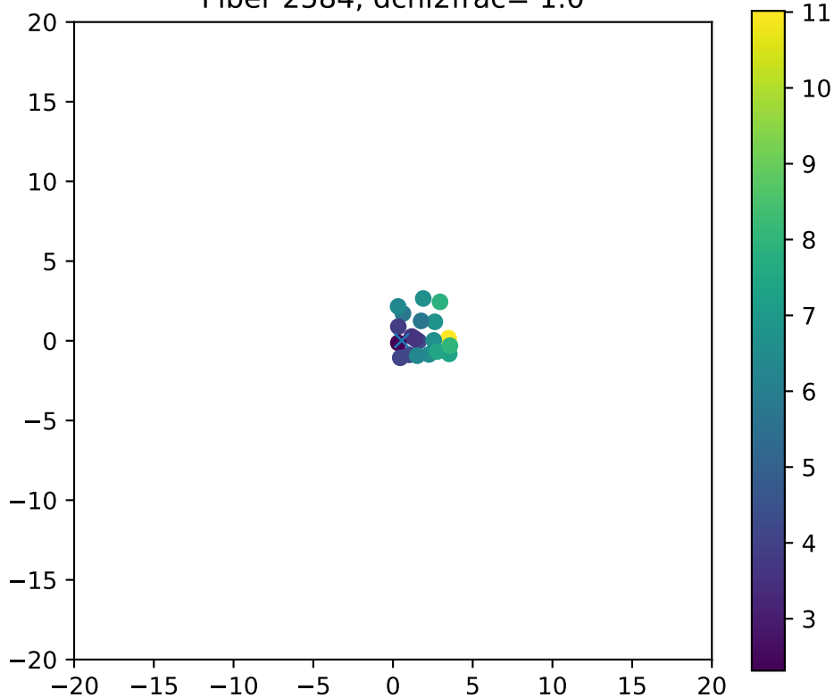
Fiber 2584, dchi2frac= 1.0
