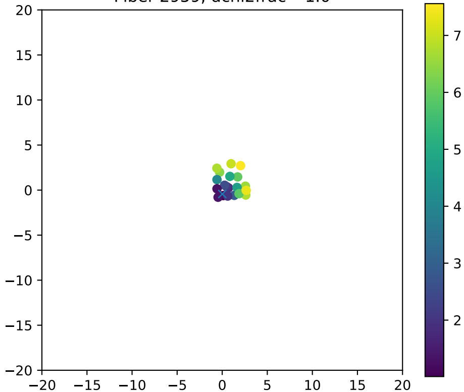
Fiber 2959, dchi2frac= 1.0
