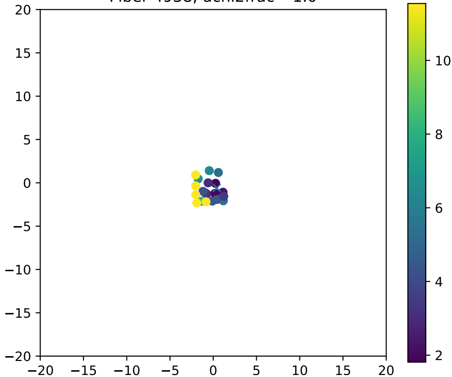
Fiber 4938, dchi2frac= 1.0
