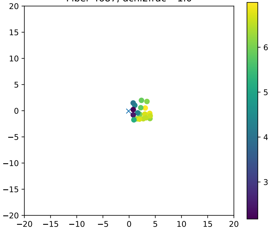
Fiber 4687, dchi2frac= 1.0
