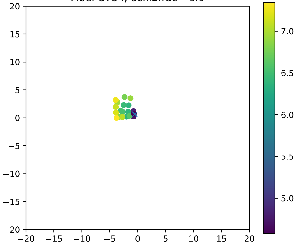
Fiber 3754, dchi2frac= 0.9
