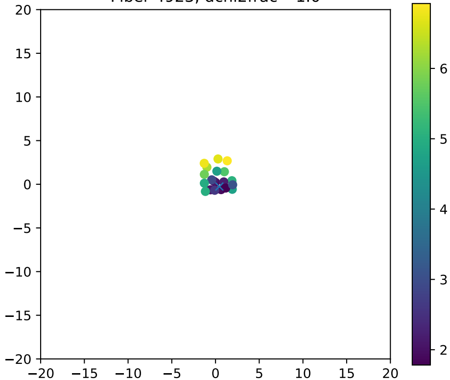
Fiber 4923, dchi2frac= 1.0
