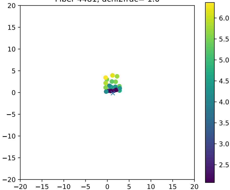
Fiber 4481, dchi2frac= 1.0
