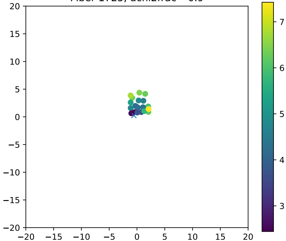
Fiber 1725, dchi2frac= 0.9
