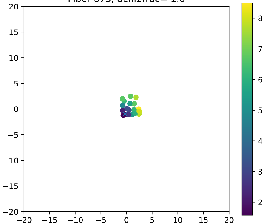
Fiber 873, dchi2frac= 1.0
