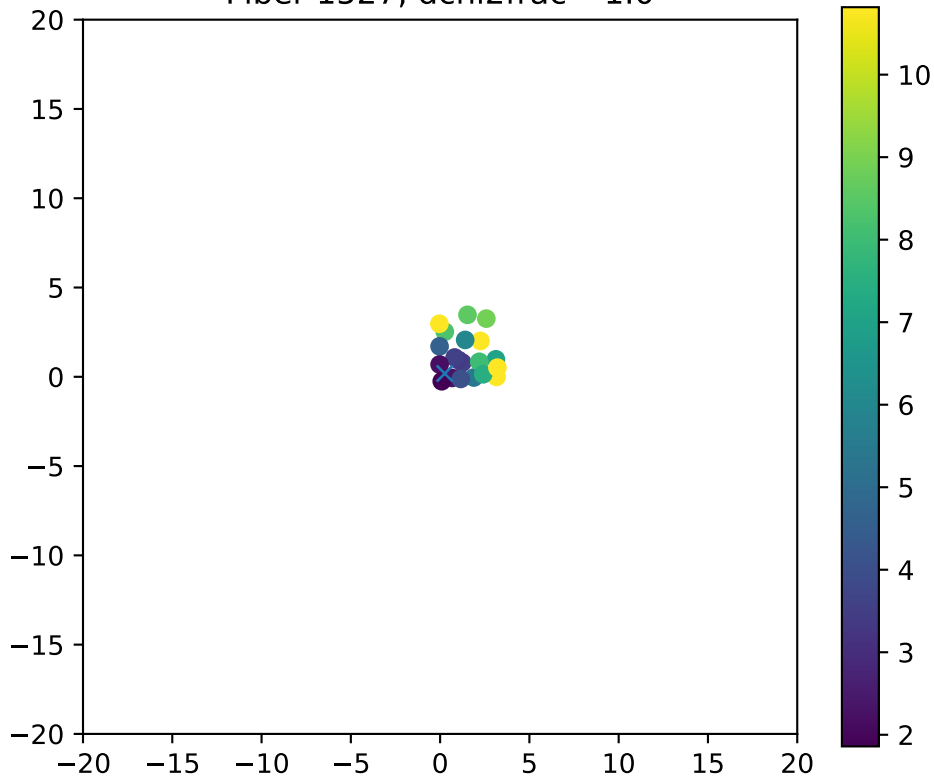
Fiber 1527, dchi2frac= 1.0
