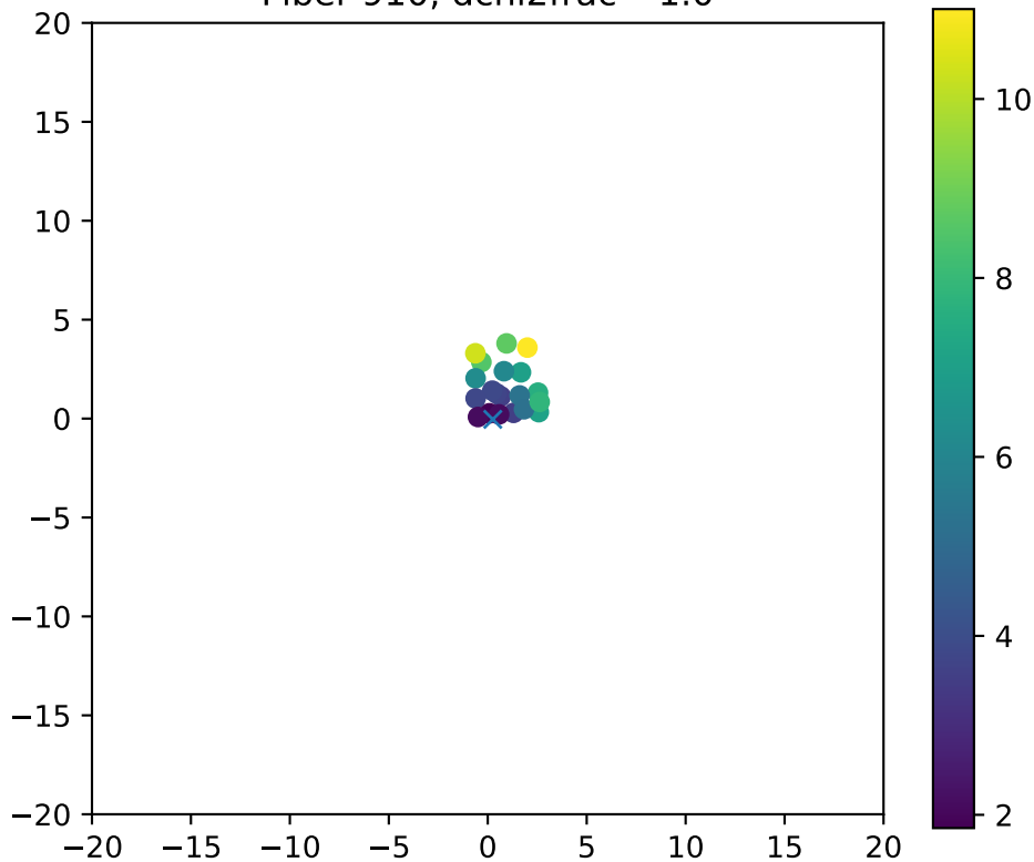
Fiber 910, dchi2frac= 1.0
