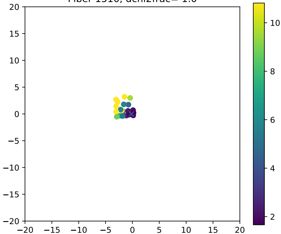
Fiber 1510, dchi2frac= 1.0
