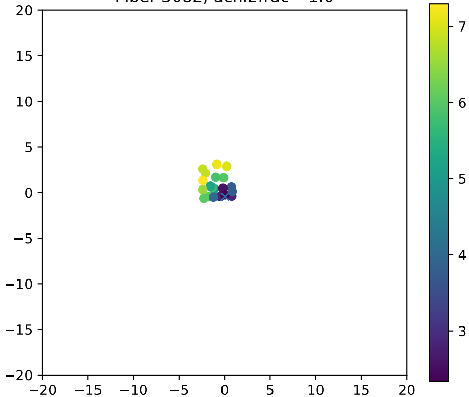
Fiber 3082, dchi2frac= 1.0
