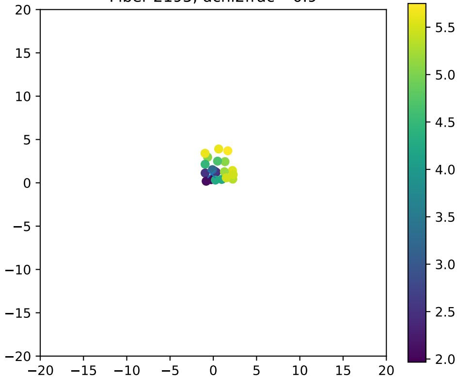
Fiber 2195, dchi2frac= 0.9
