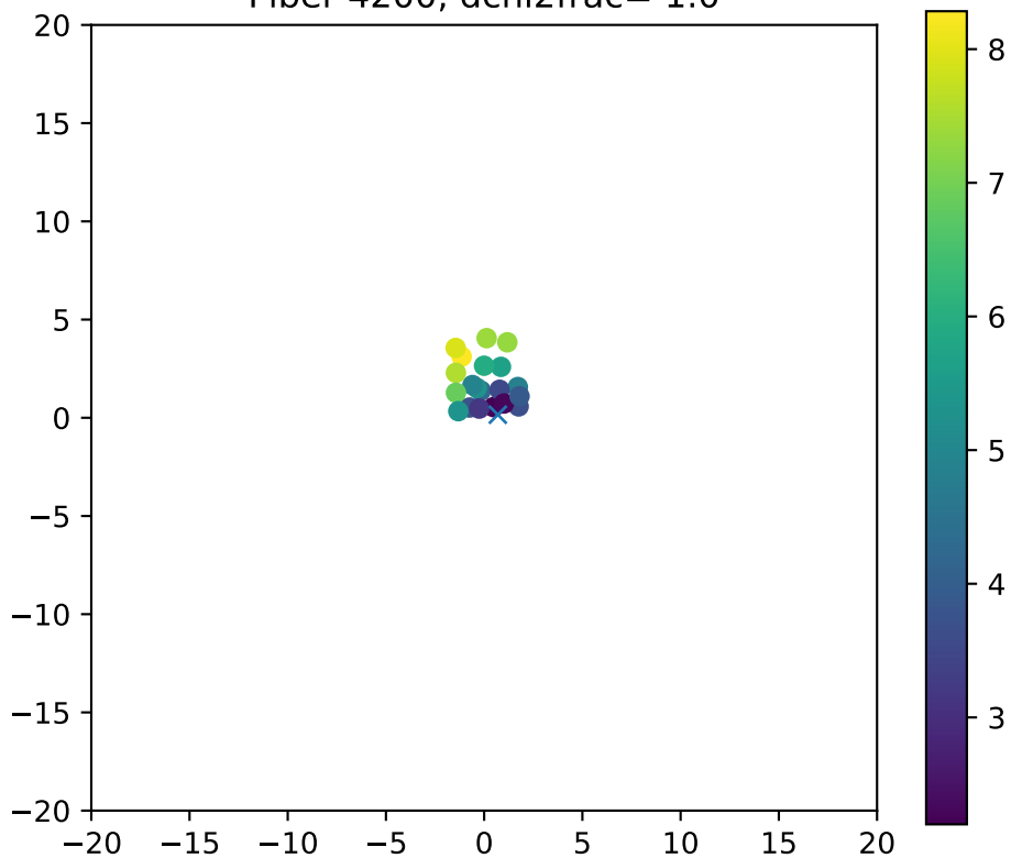
Fiber 4200, dchi2frac= 1.0
