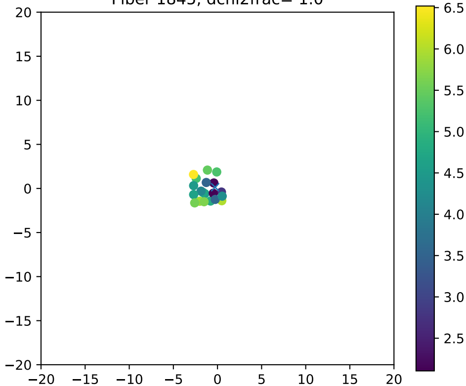
Fiber 1845, dchi2frac= 1.0
