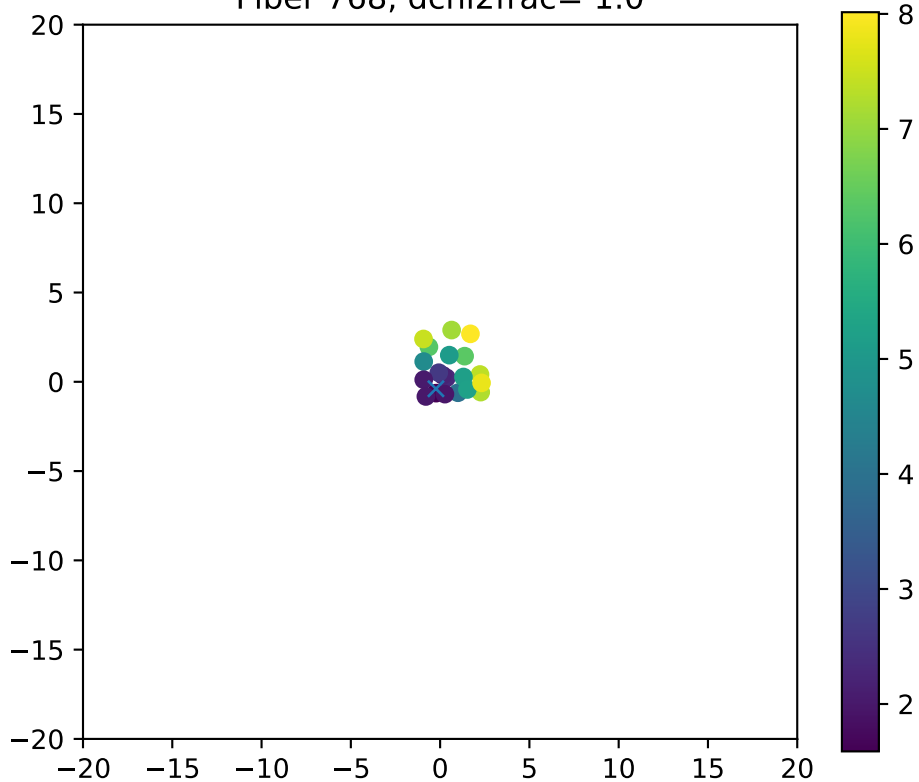
Fiber 768, dchi2frac= 1.0
