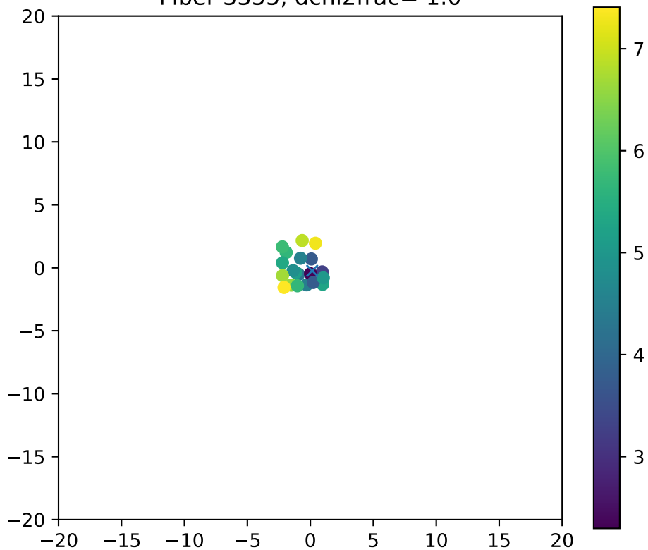
Fiber 3355, dchi2frac= 1.0
