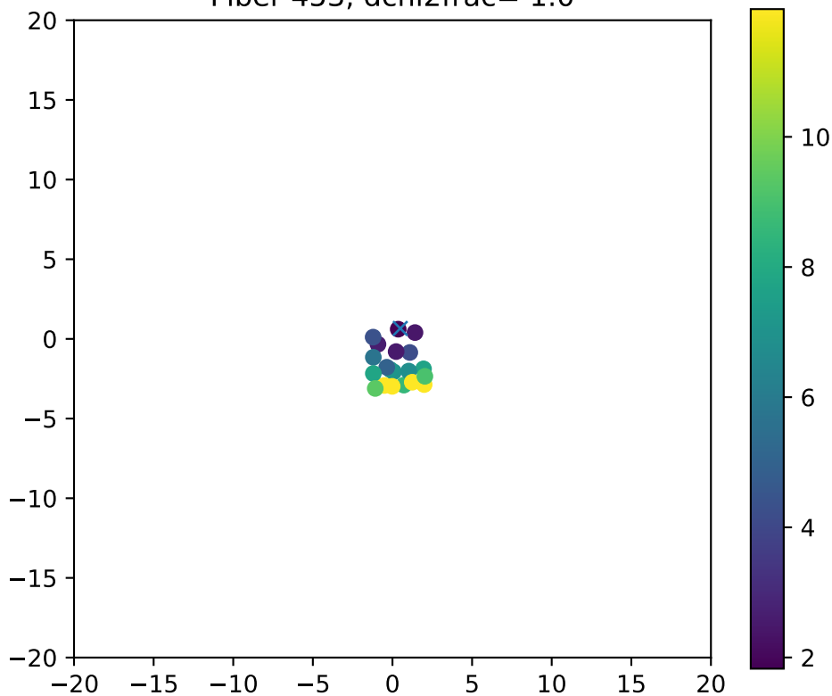
Fiber 453, dchi2frac= 1.0
