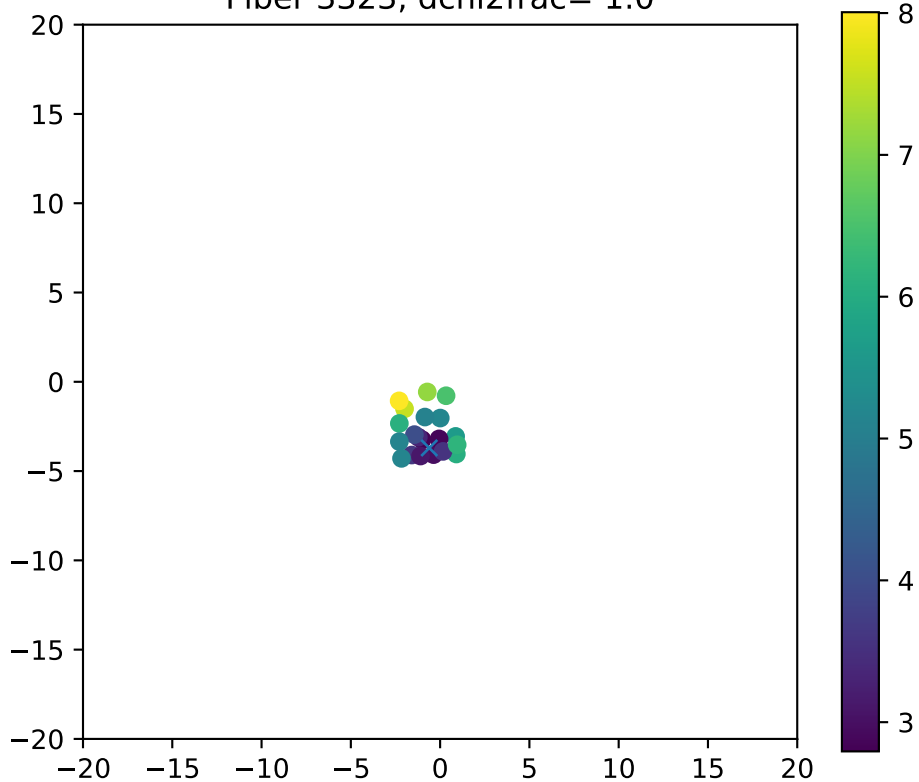
Fiber 3323, dchi2frac= 1.0
