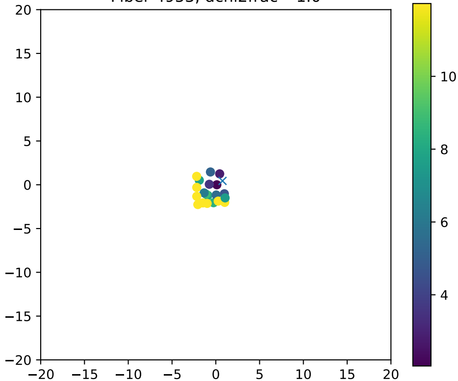
Fiber 4953, dchi2frac= 1.0
