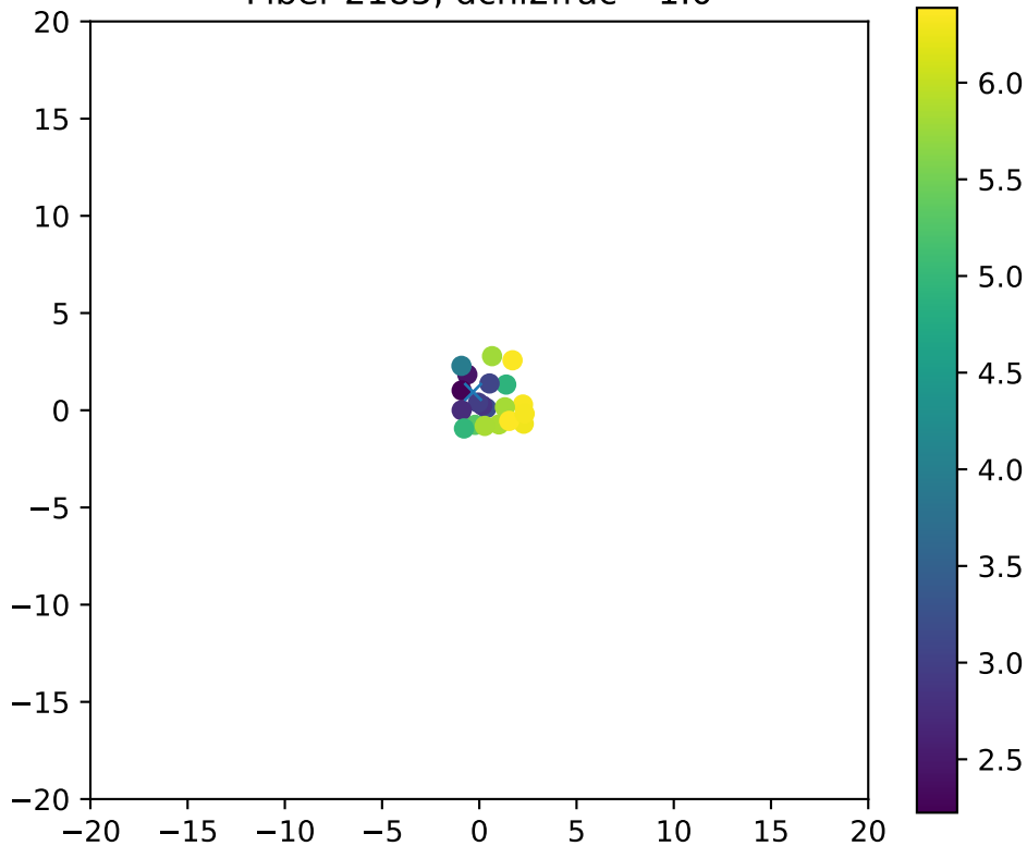
Fiber 2185, dchi2frac= 1.0
