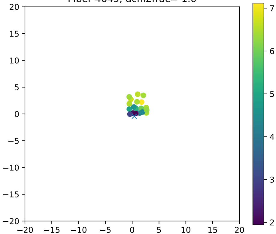
Fiber 4649, dchi2frac= 1.0
