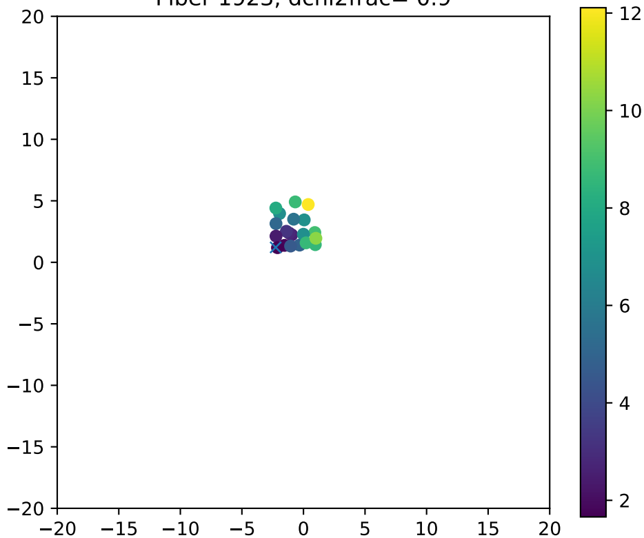
Fiber 1923, dchi2frac= 0.9
