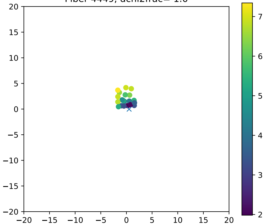
Fiber 4449, dchi2frac= 1.0
