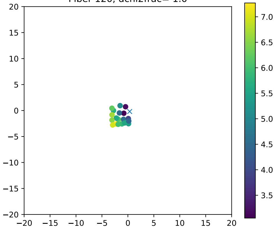
Fiber 120, dchi2frac= 1.0
