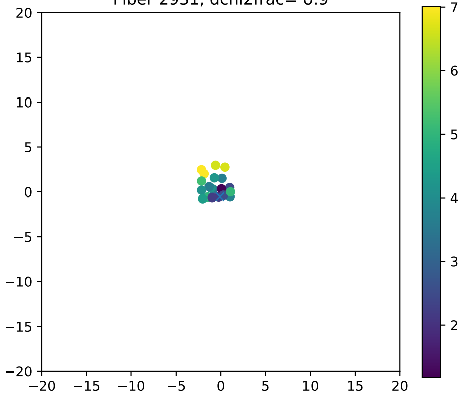
Fiber 2931, dchi2frac= 0.9
