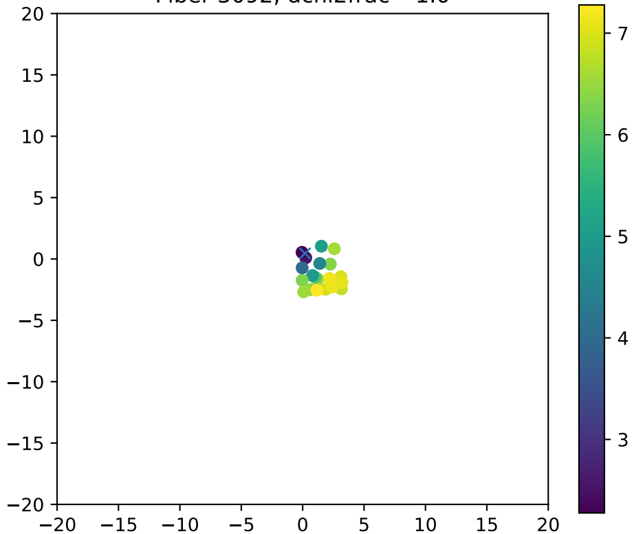
Fiber 3092, dchi2frac= 1.0
