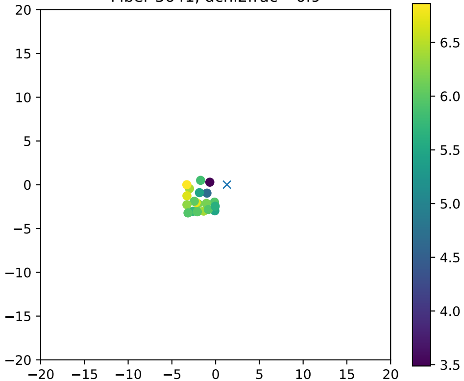
Fiber 3641, dchi2frac= 0.9
