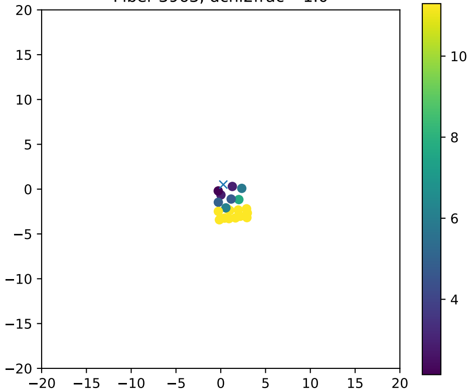
Fiber 3963, dchi2frac= 1.0
