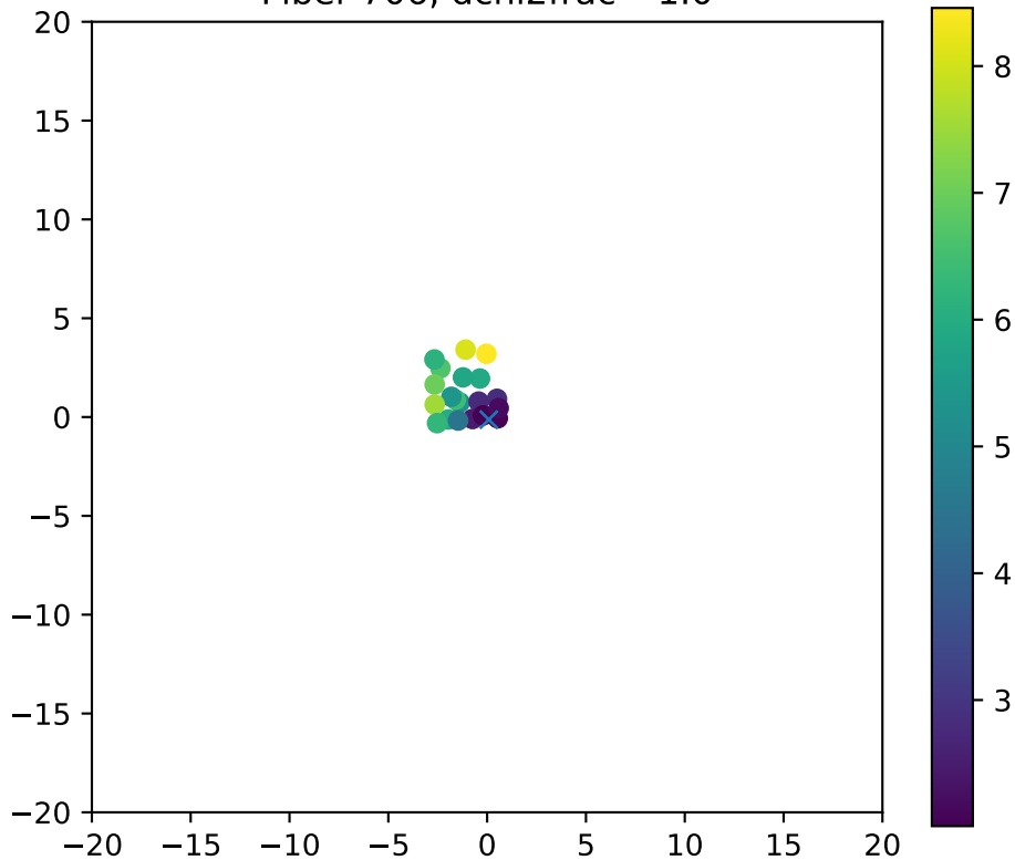
Fiber 706, dchi2frac= 1.0
