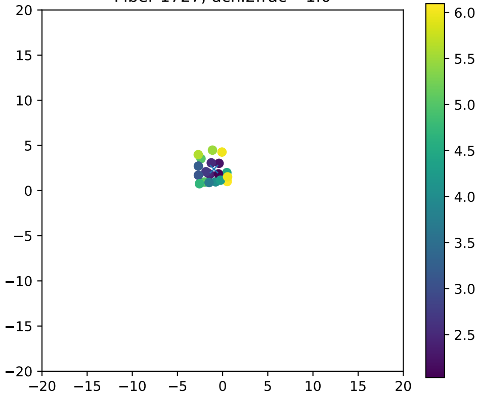
Fiber 1727, dchi2frac= 1.0
