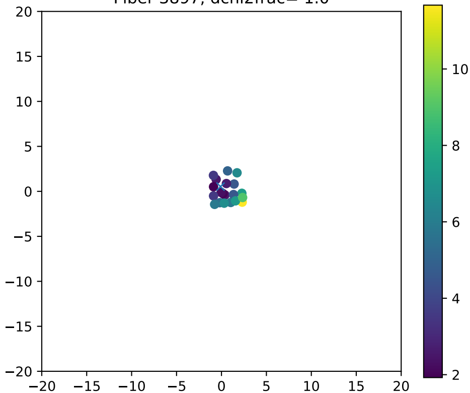
Fiber 3897, dchi2frac= 1.0
