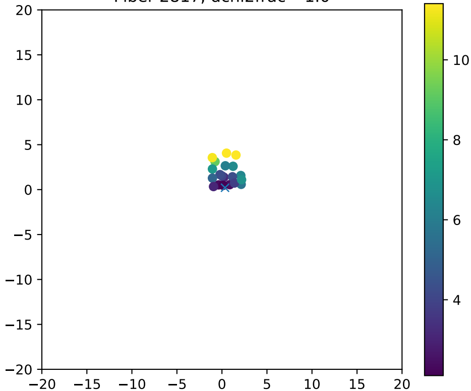
Fiber 2817, dchi2frac= 1.0
