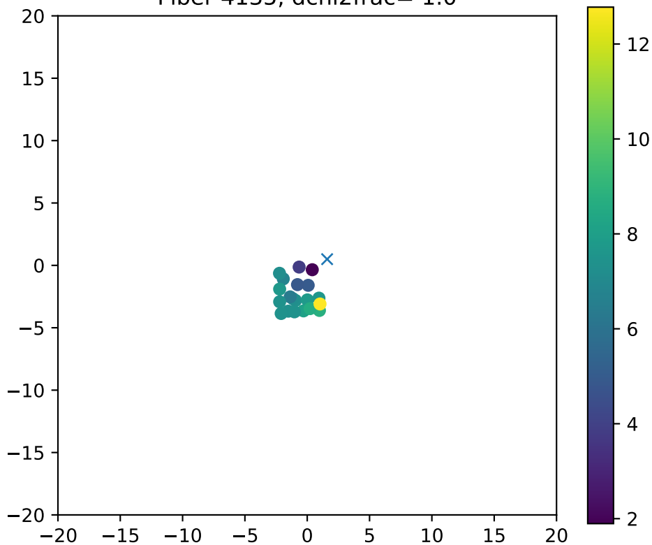
Fiber 4135, dchi2frac= 1.0
