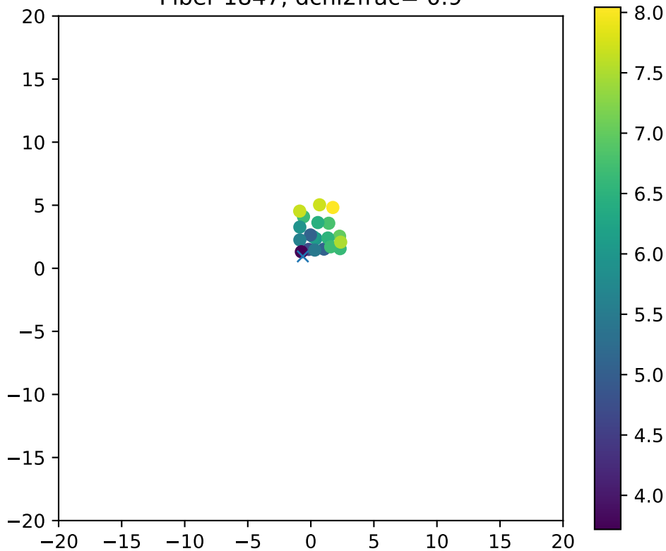
Fiber 1847, dchi2frac= 0.9
