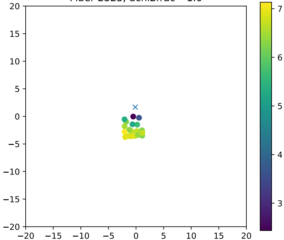
Fiber 2323, dchi2frac= 1.0
