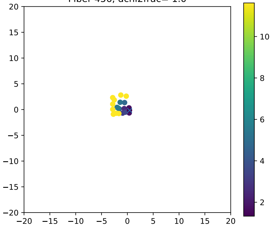
Fiber 456, dchi2frac= 1.0
