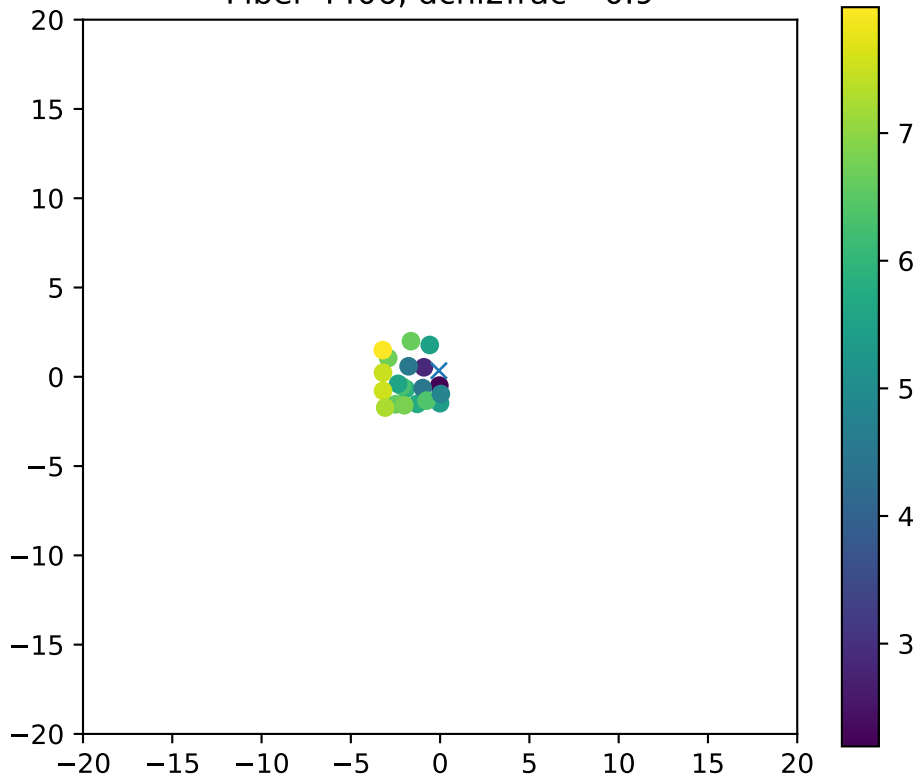
Fiber 4406, dchi2frac= 0.9
