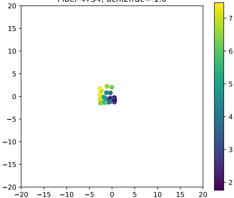
Fiber 4754, dchi2frac= 1.0
