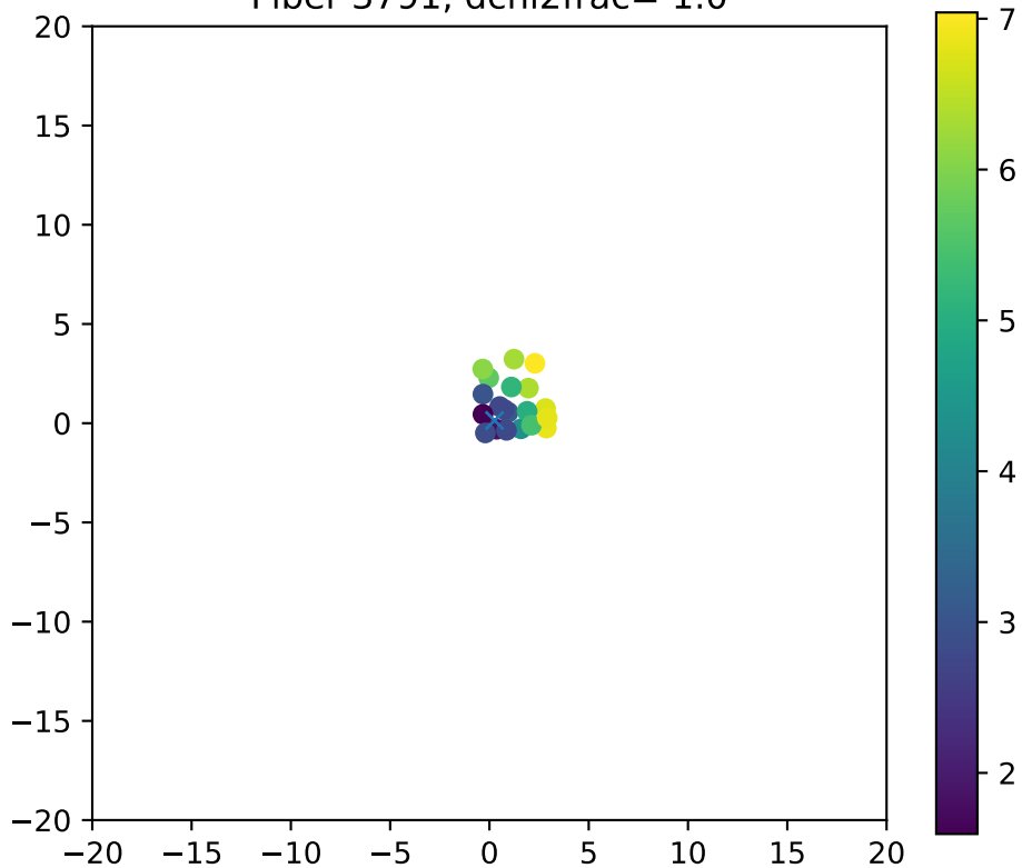
Fiber 3791, dchi2frac= 1.0
