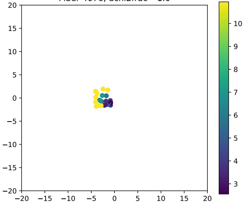
Fiber 4076, dchi2frac= 1.0
