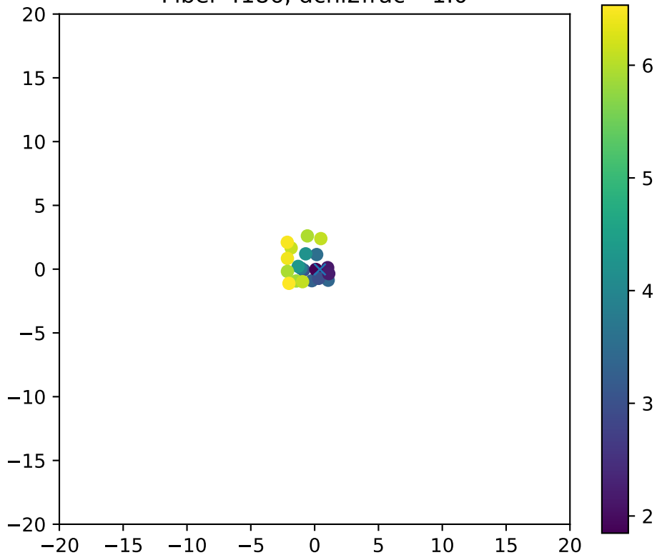
Fiber 4186, dchi2frac= 1.0
