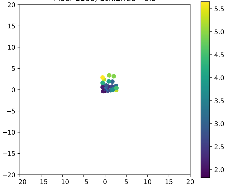
Fiber 2266, dchi2frac= 0.9
