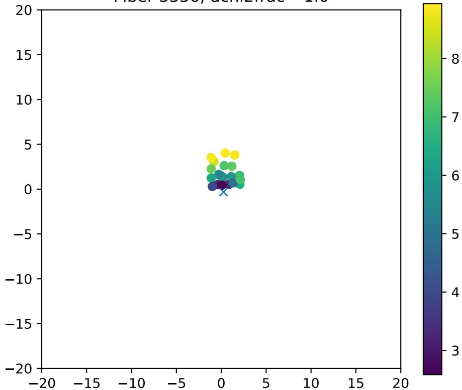
Fiber 3336, dchi2frac= 1.0
