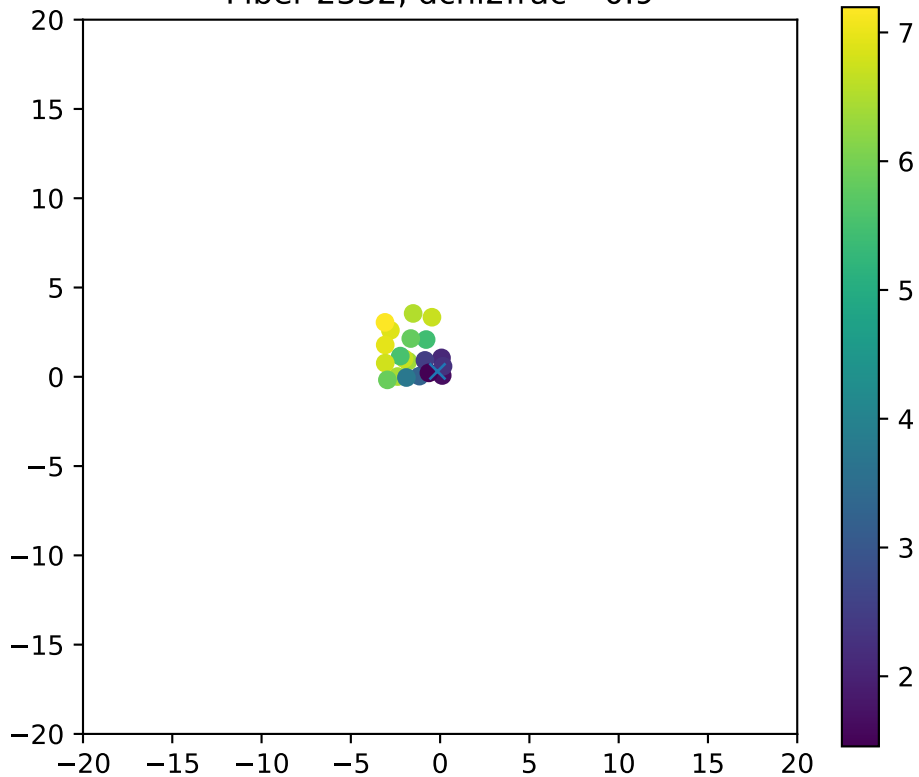
Fiber 2332, dchi2frac= 0.9
