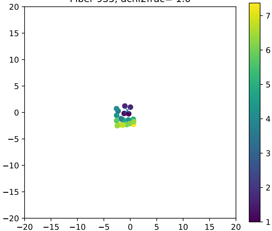
Fiber 935, dchi2frac= 1.0
