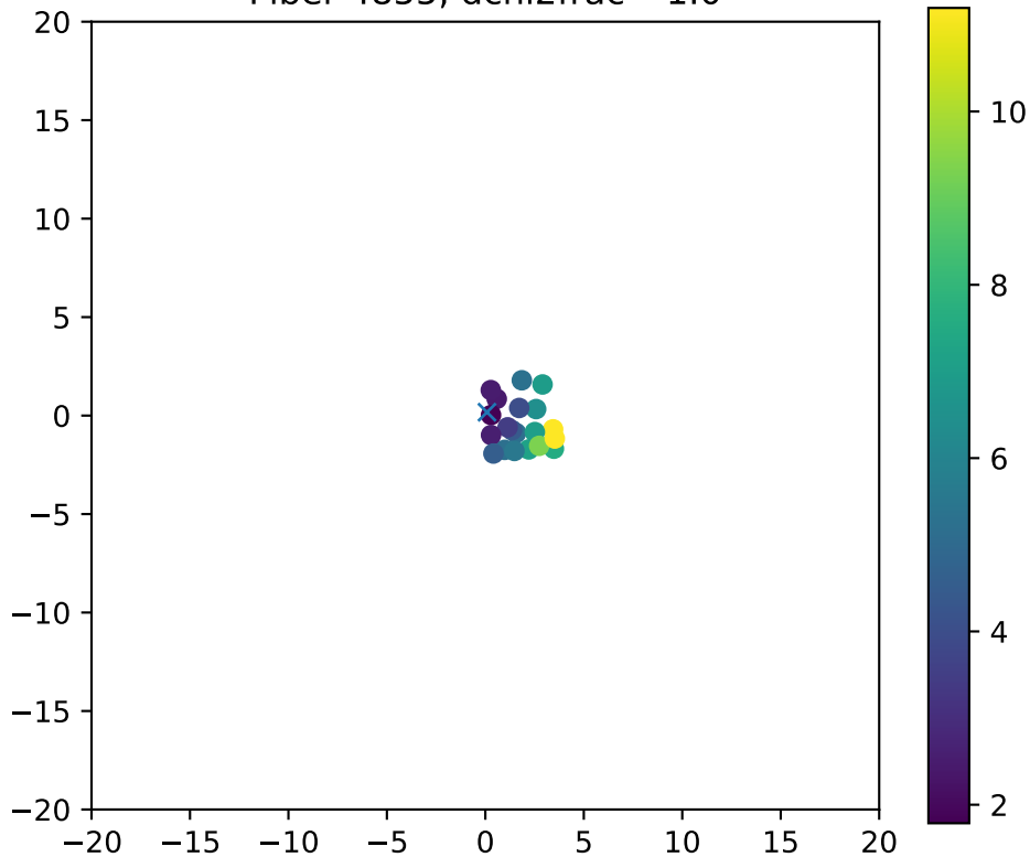
Fiber 4855, dchi2frac= 1.0
