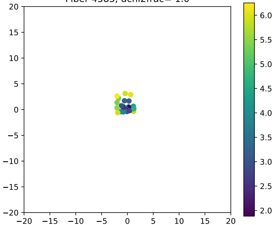
Fiber 4585, dchi2frac= 1.0
