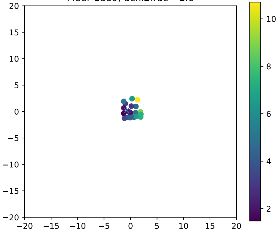
Fiber 1869, dchi2frac= 1.0
