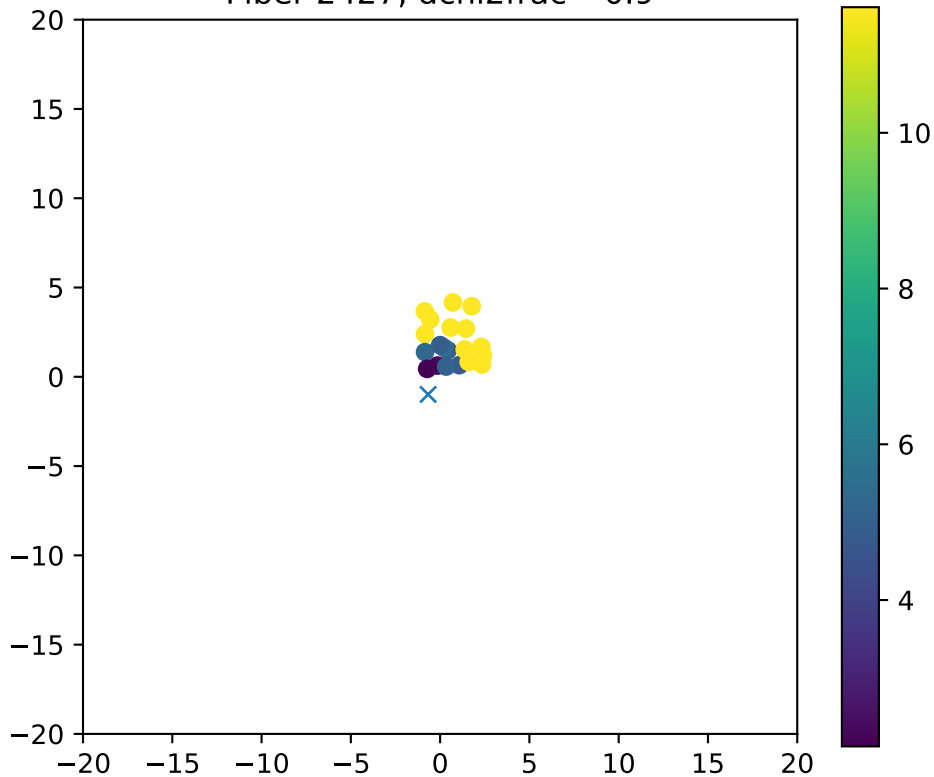
Fiber 2427, dchi2frac= 0.9
