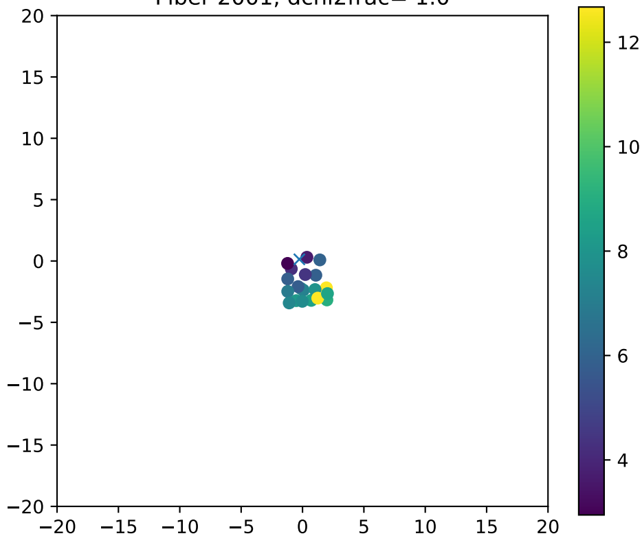
Fiber 2001, dchi2frac= 1.0
