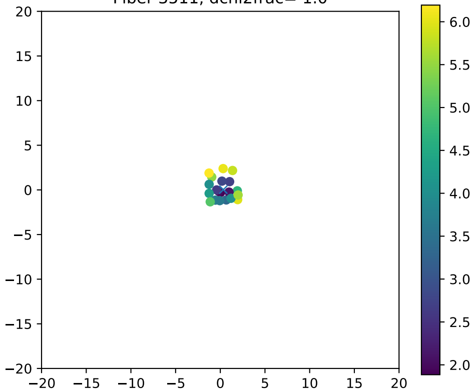
Fiber 3511, dchi2frac= 1.0
