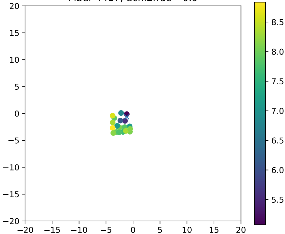
Fiber 4417, dchi2frac= 0.9
