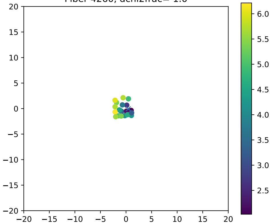
Fiber 4260, dchi2frac= 1.0
