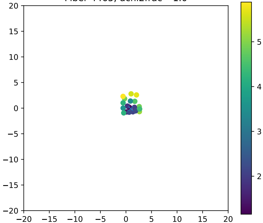
Fiber 4465, dchi2frac= 1.0
