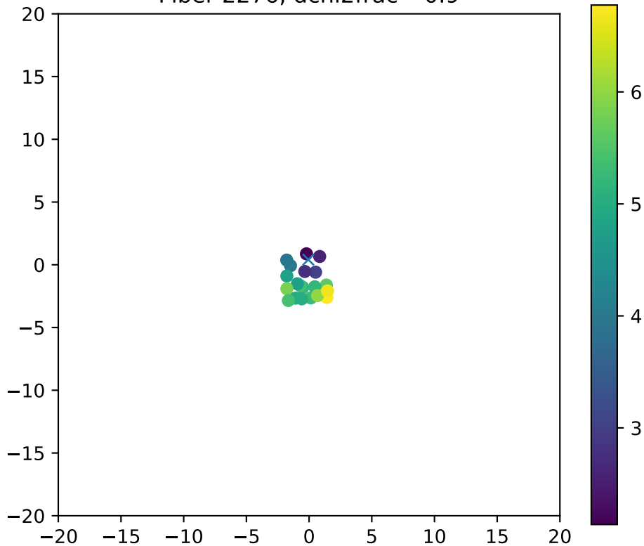
Fiber 2276, dchi2frac= 0.9
