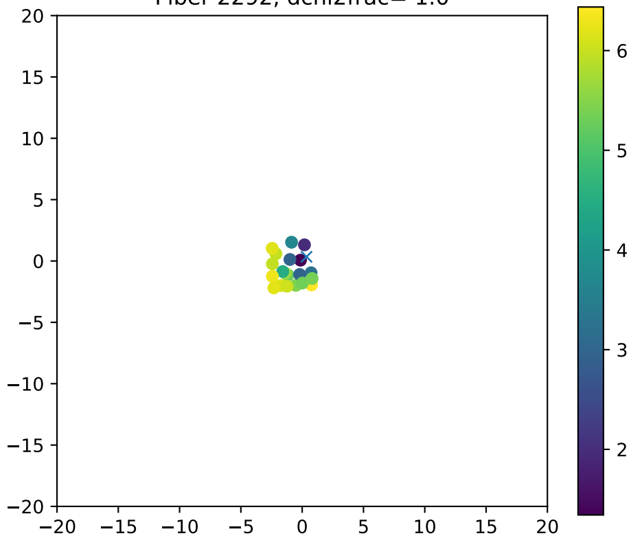
Fiber 2292, dchi2frac= 1.0
