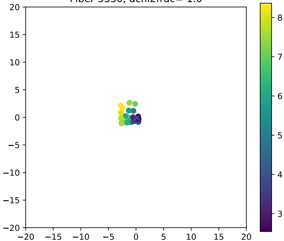
Fiber 3330, dchi2frac= 1.0
