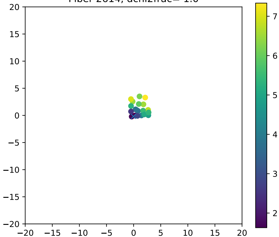
Fiber 2614, dchi2frac= 1.0
