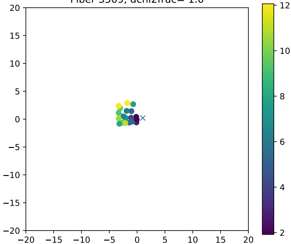
Fiber 3509, dchi2frac= 1.0
