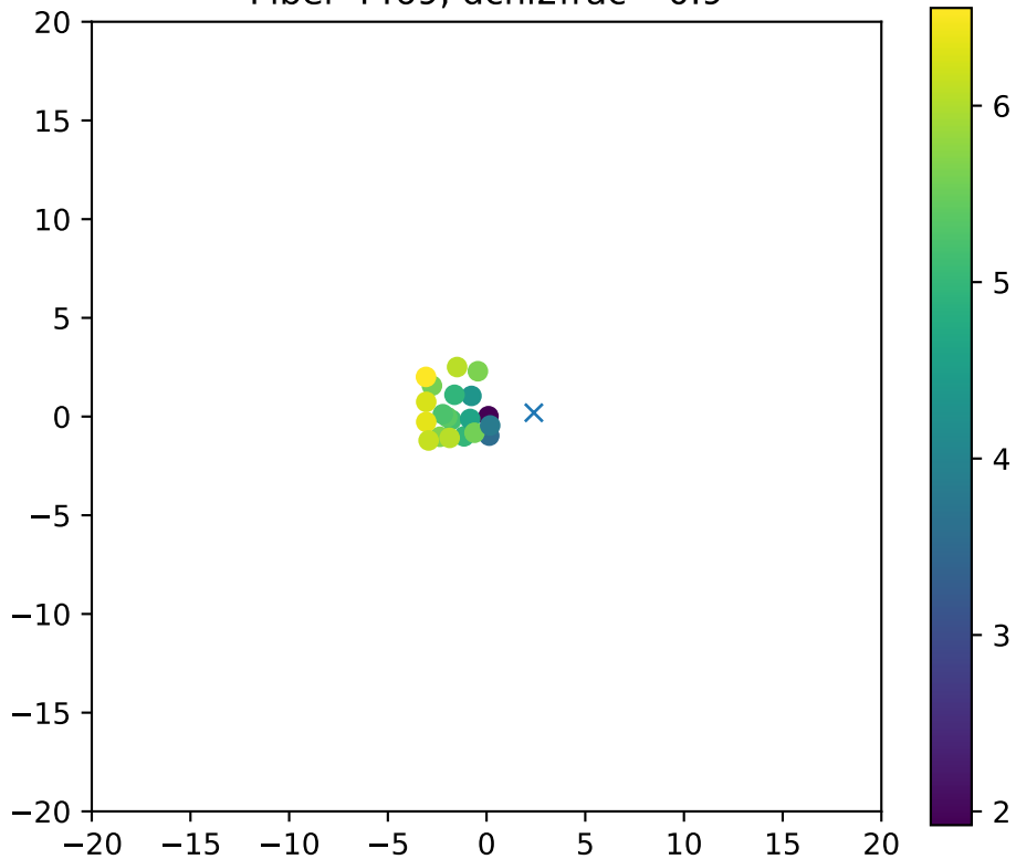
Fiber 4469, dchi2frac= 0.9
