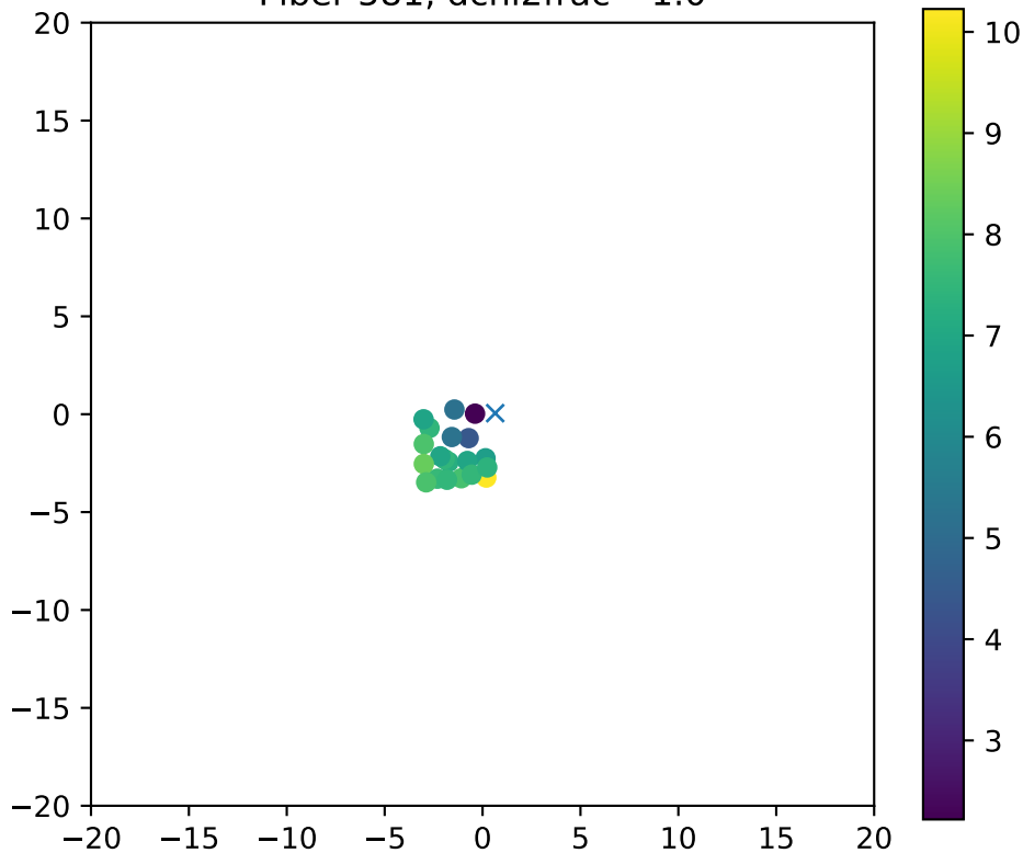
Fiber 581, dchi2frac= 1.0
