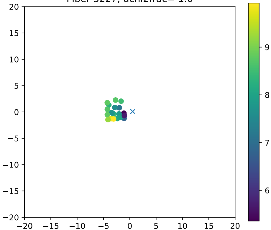
Fiber 3227, dchi2frac= 1.0
