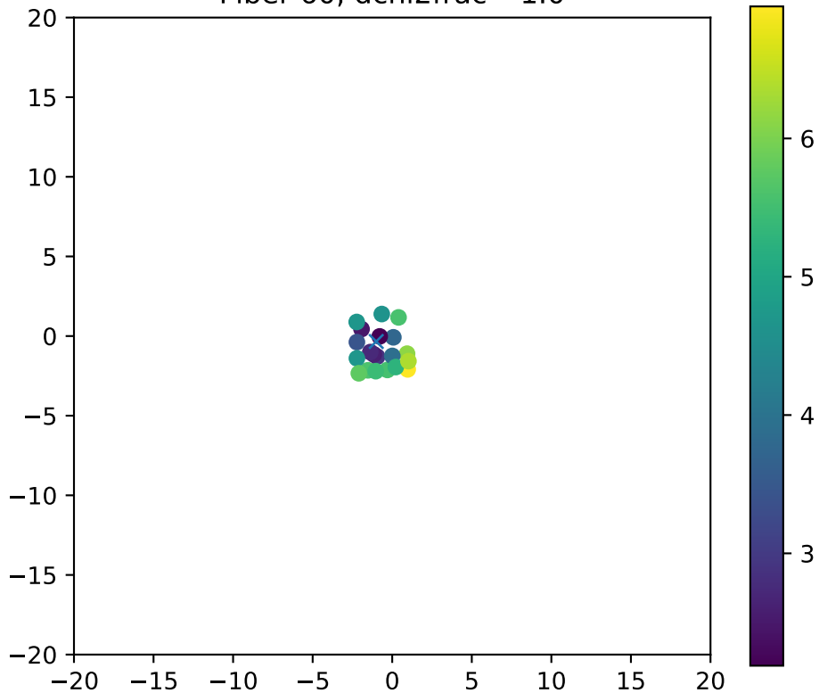
Fiber 60, dchi2frac= 1.0
