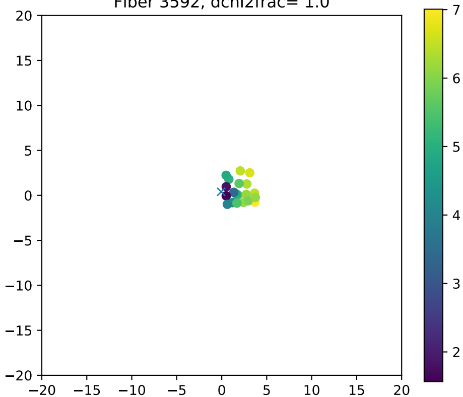
Fiber 3592, dchi2frac= 1.0
