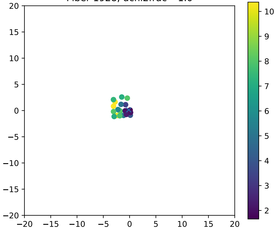
Fiber 1928, dchi2frac= 1.0
