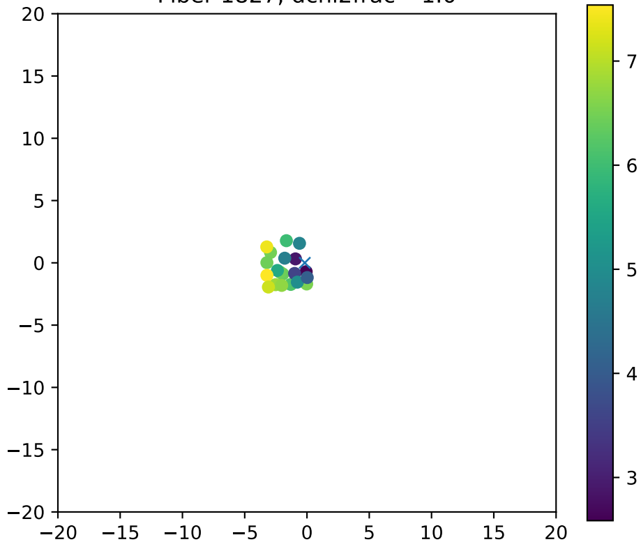
Fiber 1827, dchi2frac= 1.0
