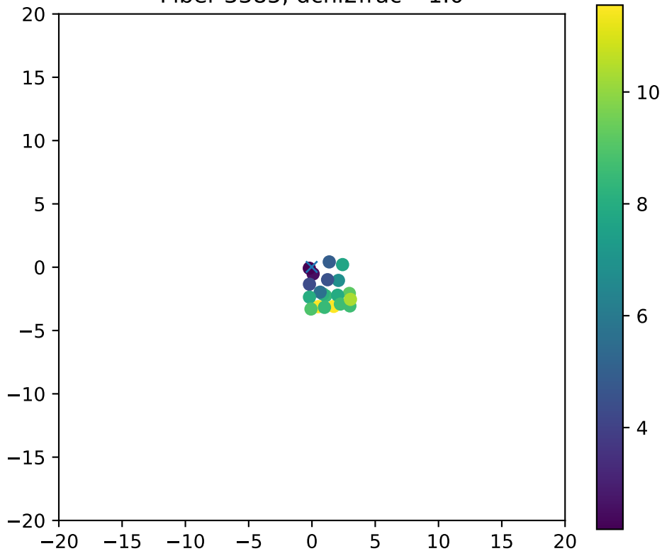
Fiber 3385, dchi2frac= 1.0
