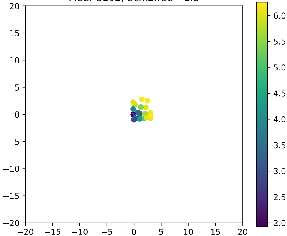
Fiber 3192, dchi2frac= 1.0
