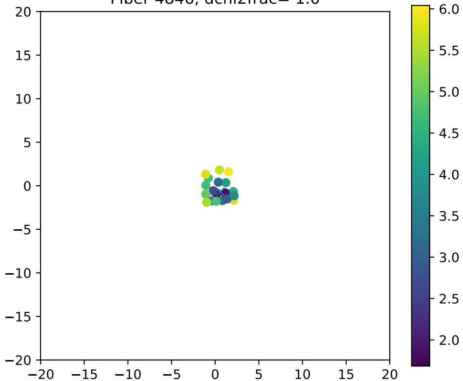
Fiber 4846, dchi2frac= 1.0
