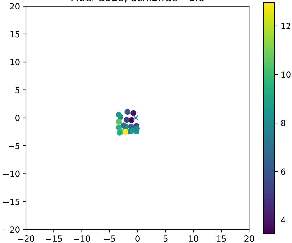
Fiber 3928, dchi2frac= 1.0
