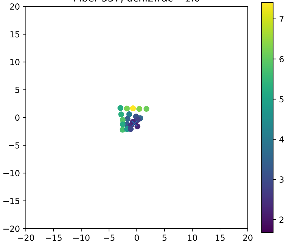
Fiber 557, dchi2frac= 1.0
