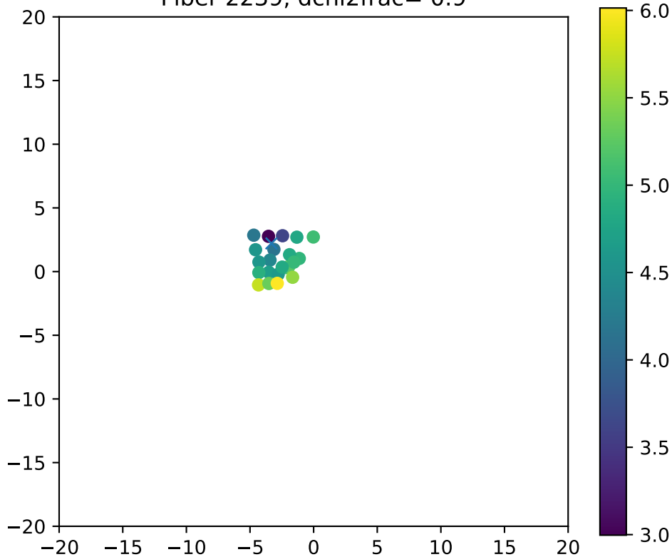
Fiber 2239, dchi2frac= 0.9
