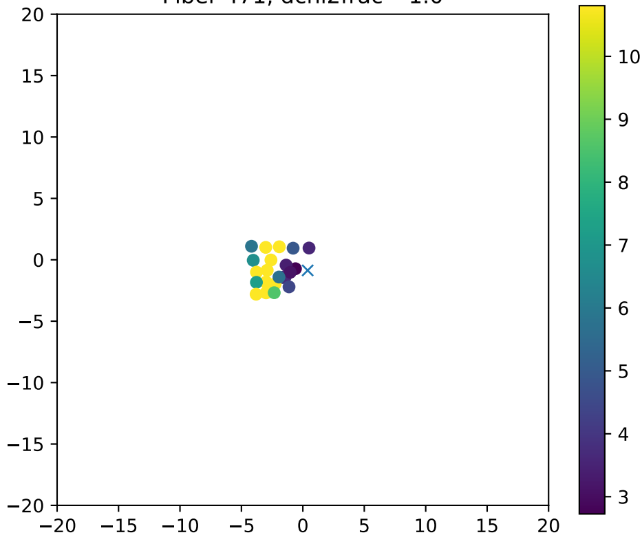
Fiber 471, dchi2frac= 1.0
