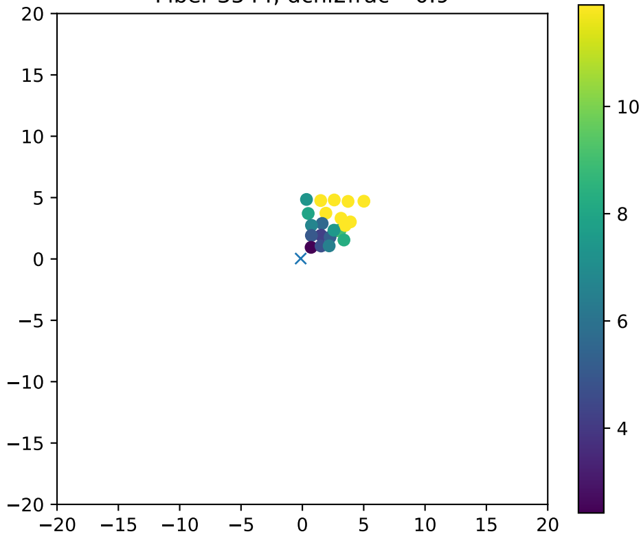
Fiber 3544, dchi2frac= 0.9
