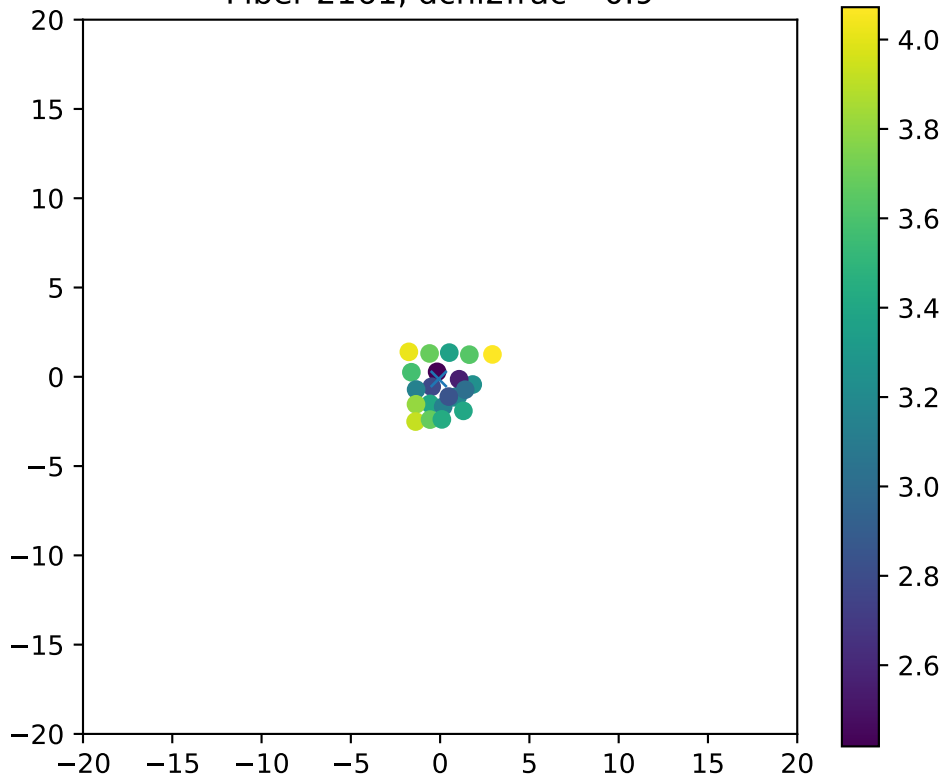
Fiber 2161, dchi2frac= 0.9
