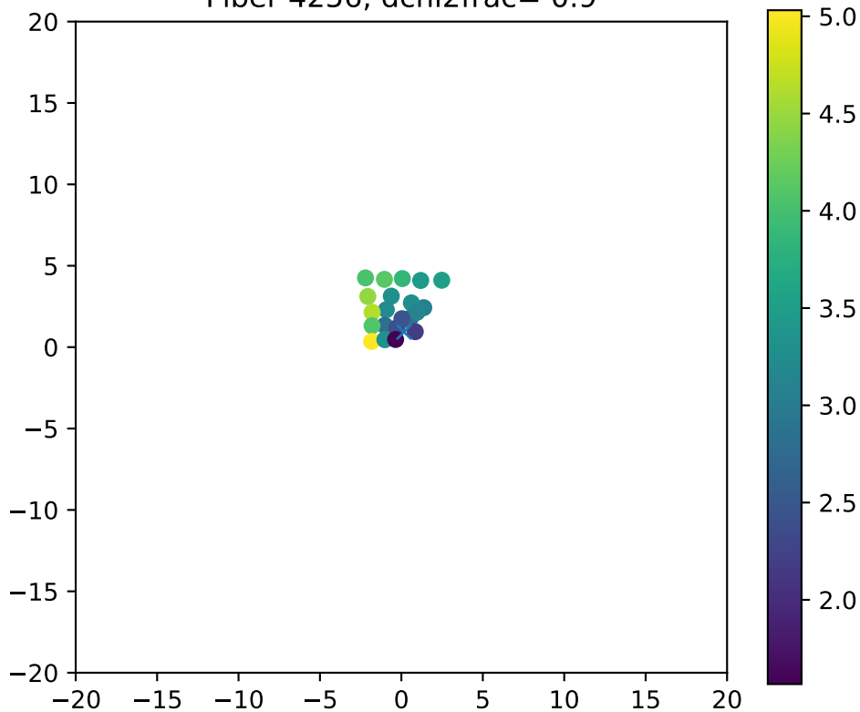
Fiber 4256, dchi2frac= 0.9
