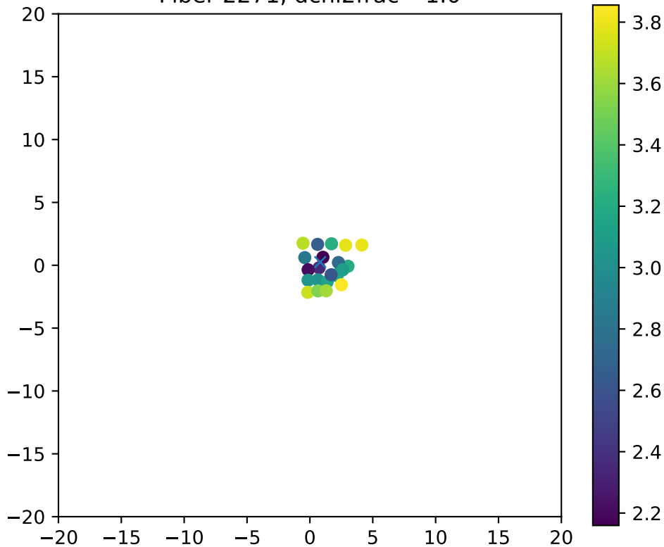
Fiber 2271, dchi2frac= 1.0
