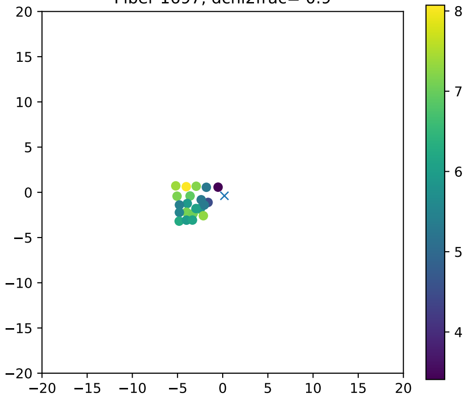
Fiber 1697, dchi2frac= 0.9
