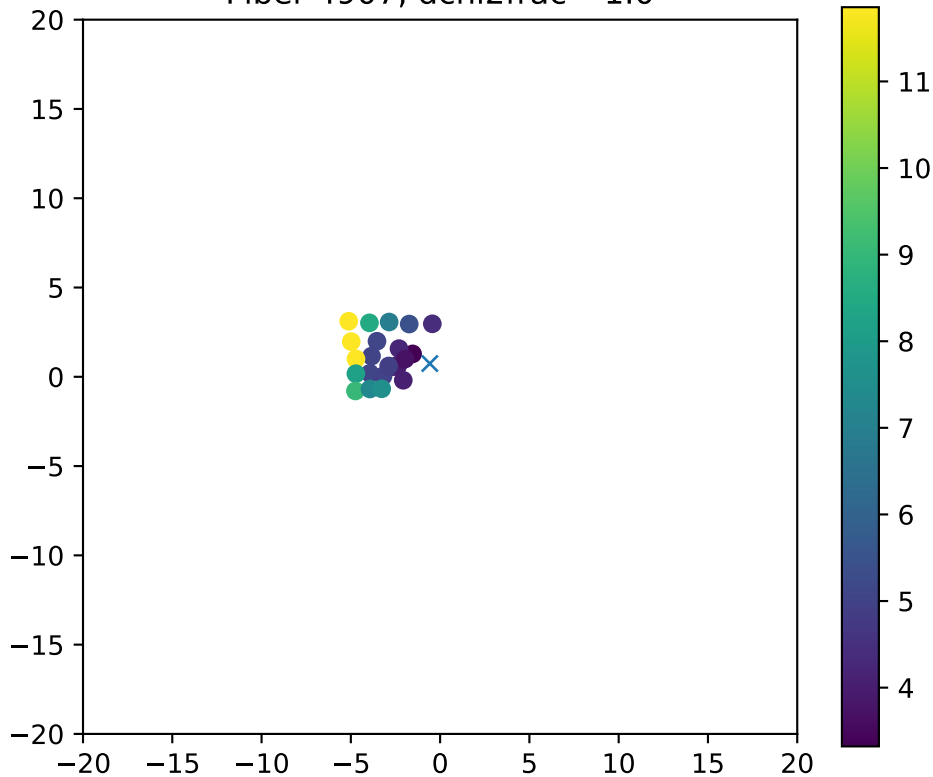
Fiber 4907, dchi2frac= 1.0
