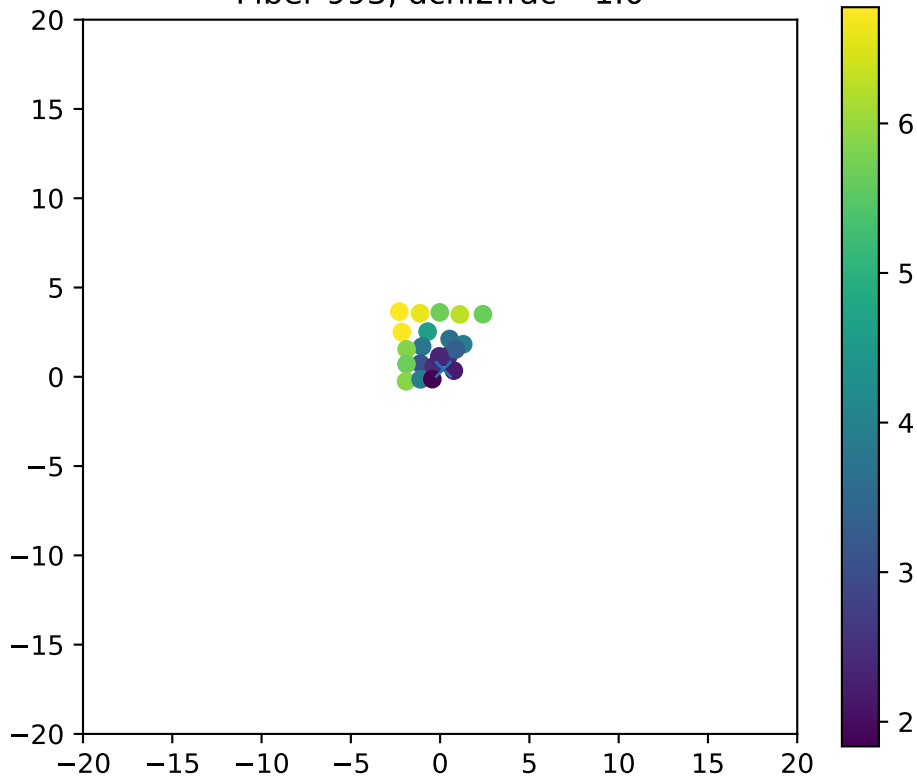
Fiber 993, dchi2frac= 1.0
