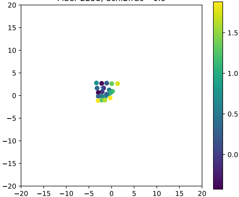
Fiber 2258, dchi2frac= 0.9
