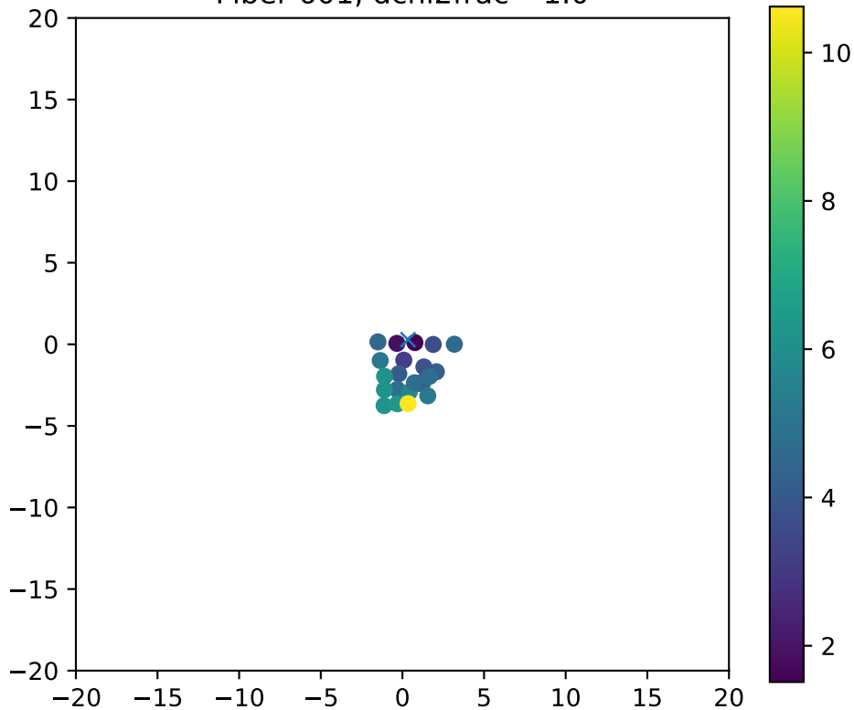
Fiber 601, dchi2frac= 1.0
