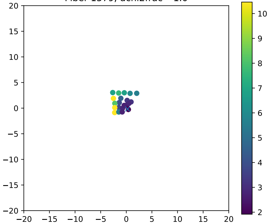
Fiber 1579, dchi2frac= 1.0
