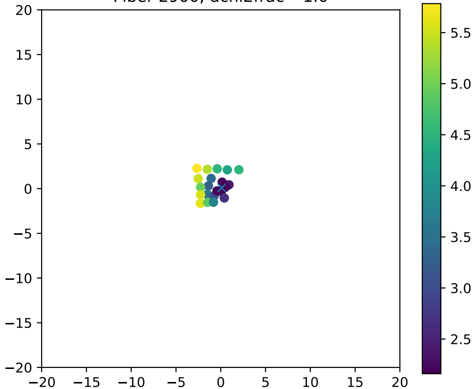
Fiber 2900, dchi2frac= 1.0
