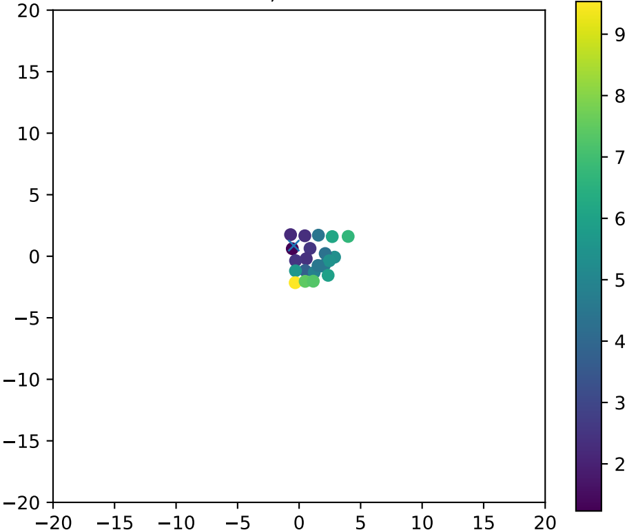
Fiber 4935, dchi2frac= 1.0
