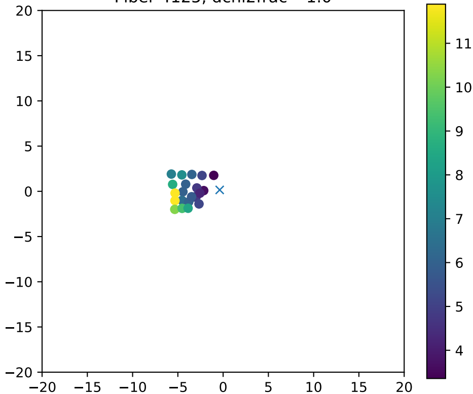
Fiber 4125, dchi2frac= 1.0
