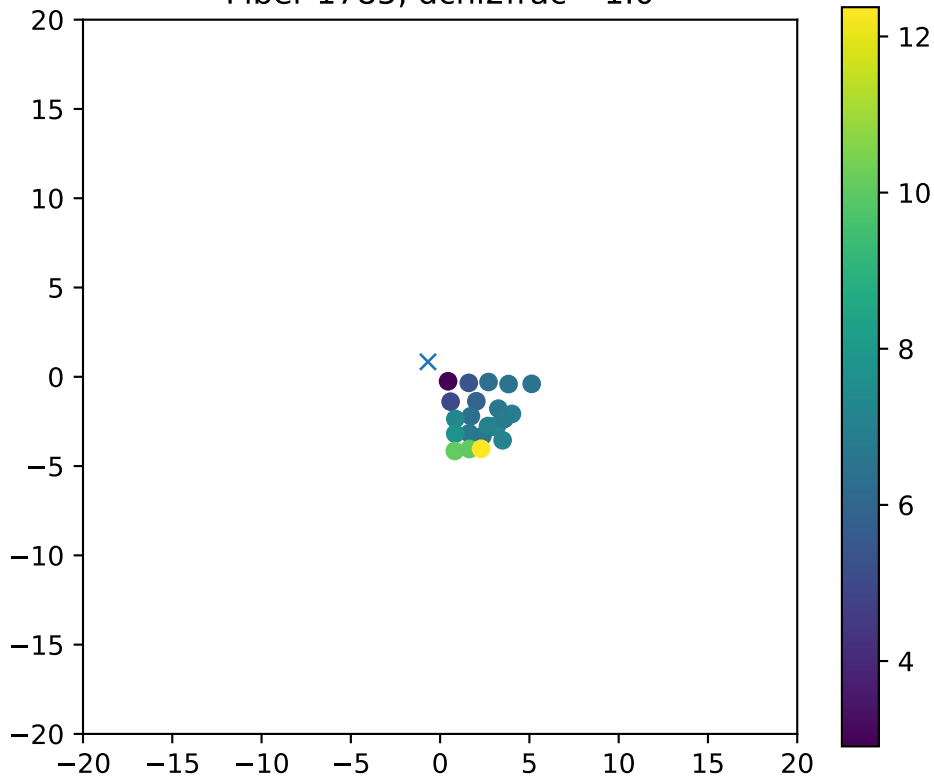
Fiber 1785, dchi2frac= 1.0
