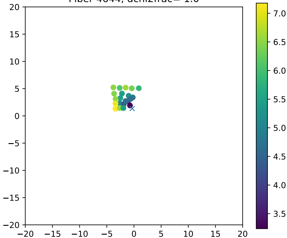
Fiber 4644, dchi2frac= 1.0
