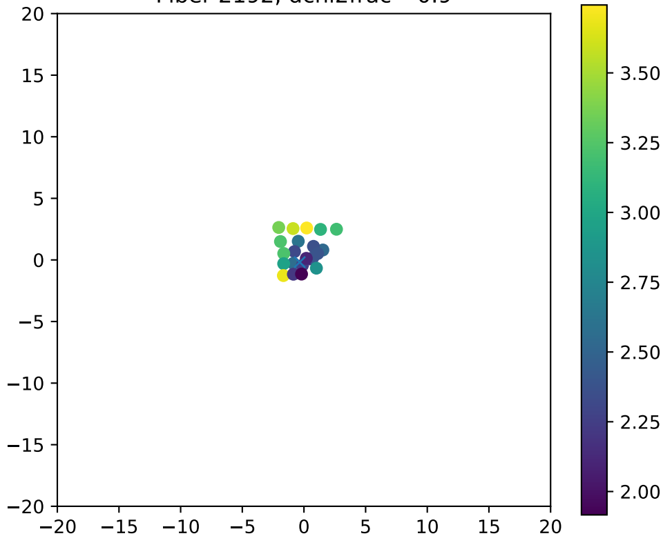
Fiber 2192, dchi2frac= 0.9
