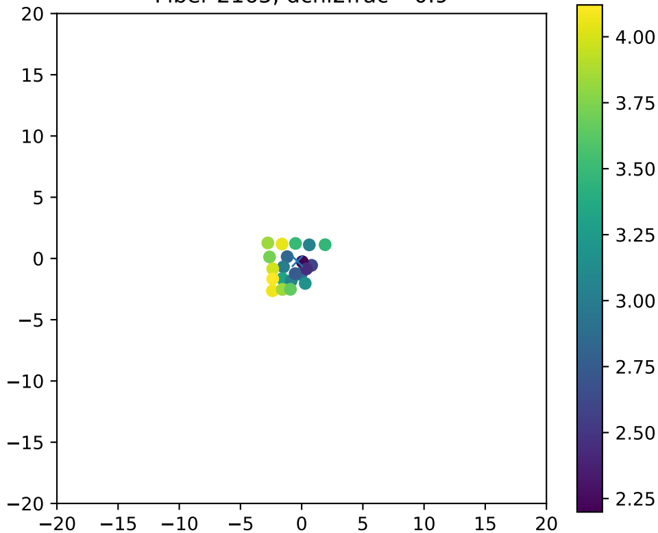
Fiber 2165, dchi2frac= 0.9
