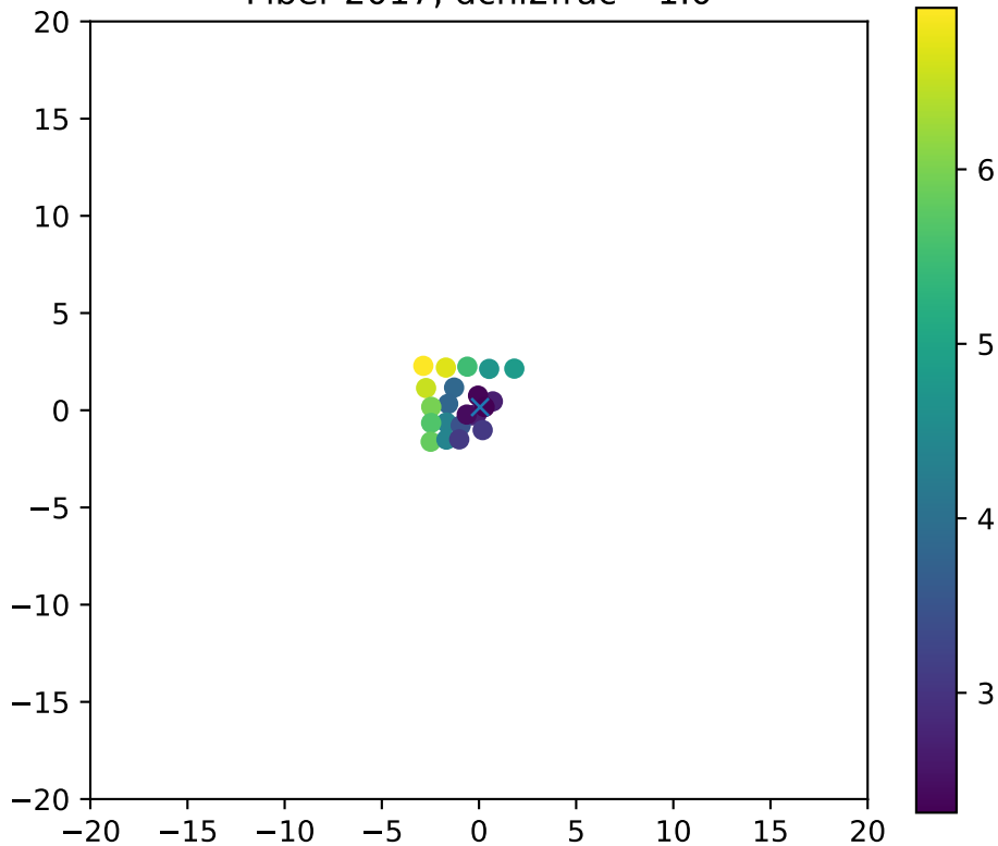
Fiber 2017, dchi2frac= 1.0
