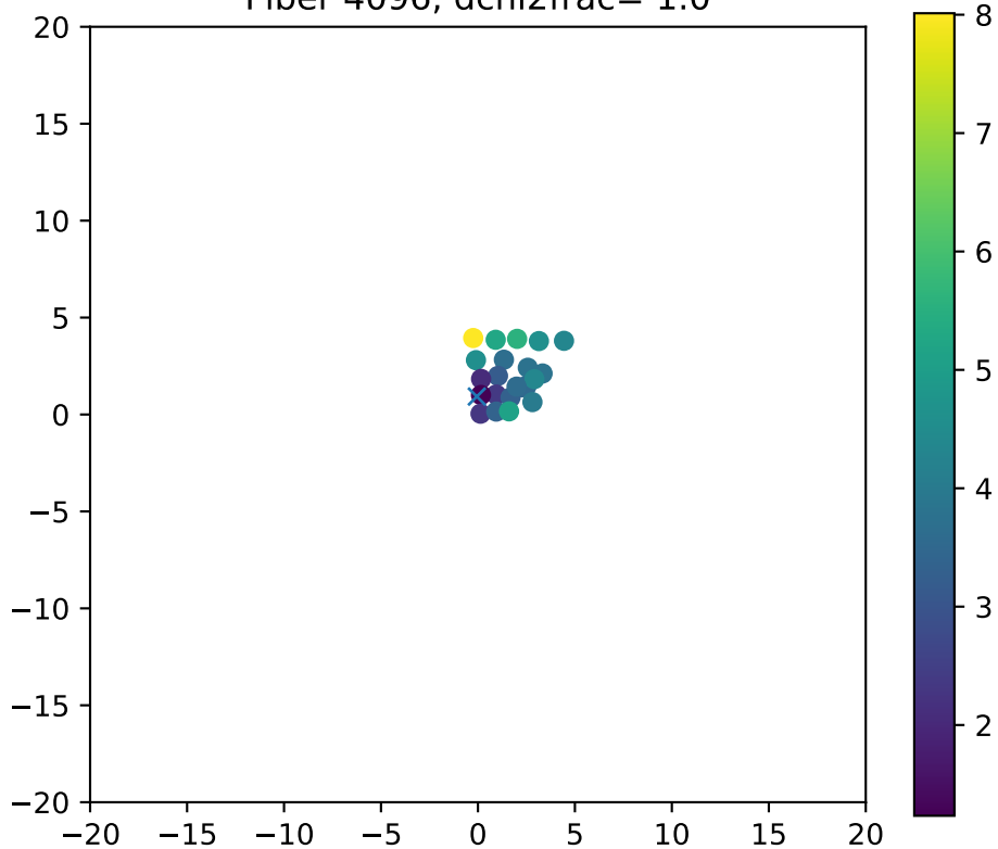
Fiber 4096, dchi2frac= 1.0
