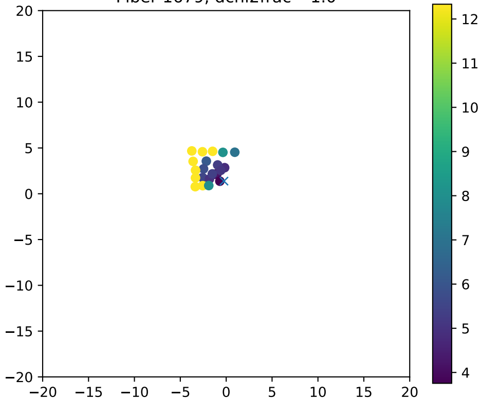
Fiber 1679, dchi2frac= 1.0
