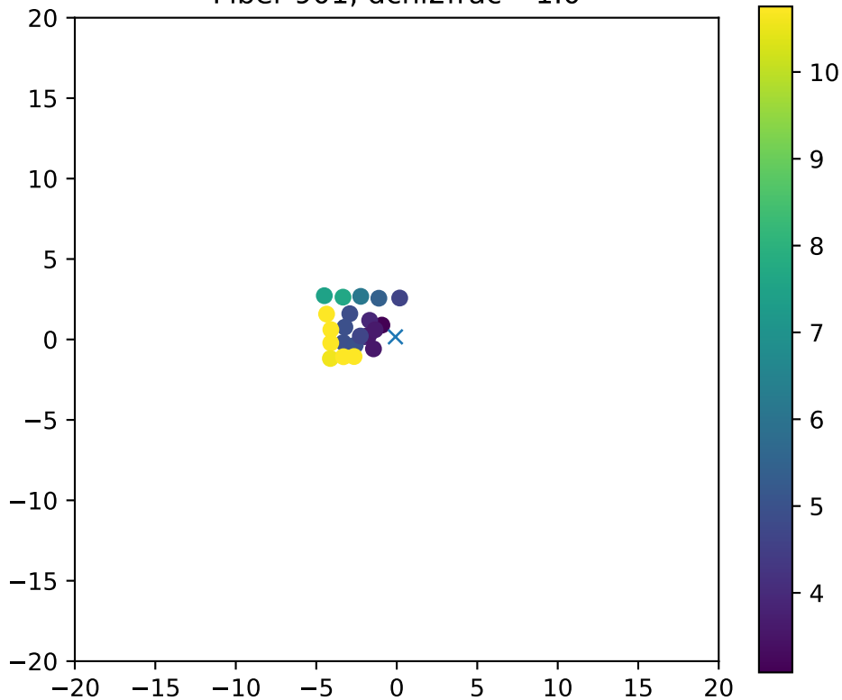
Fiber 901, dchi2frac= 1.0
