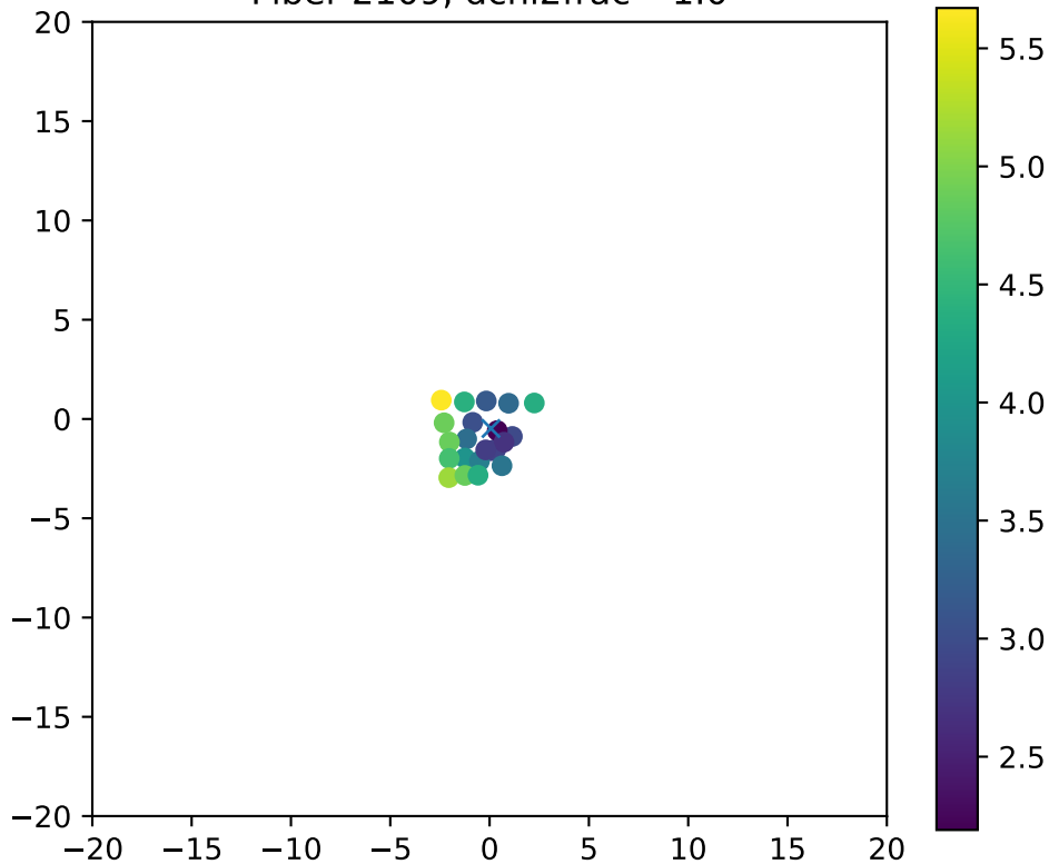
Fiber 2109, dchi2frac= 1.0
