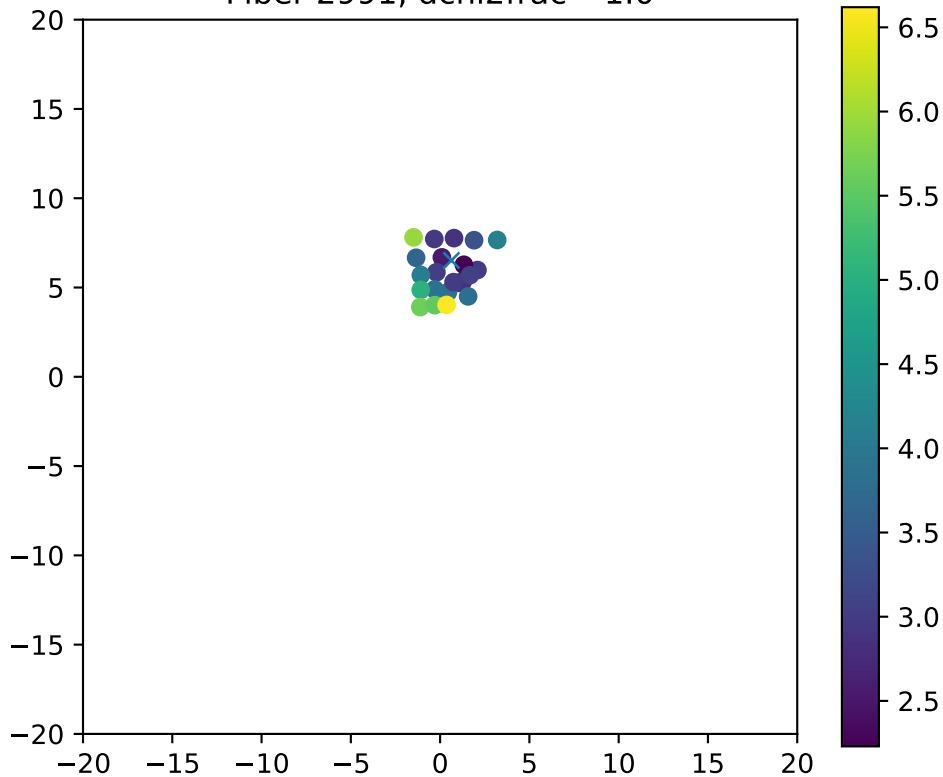
Fiber 2991, dchi2frac= 1.0
