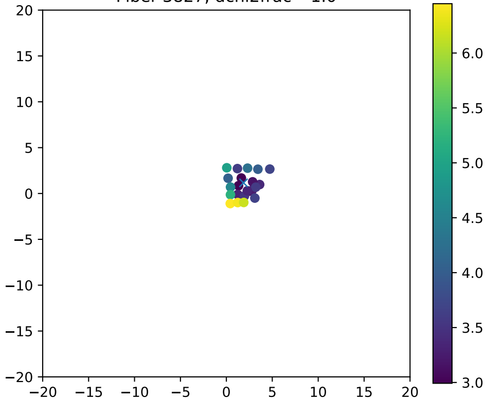
Fiber 3827, dchi2frac= 1.0
