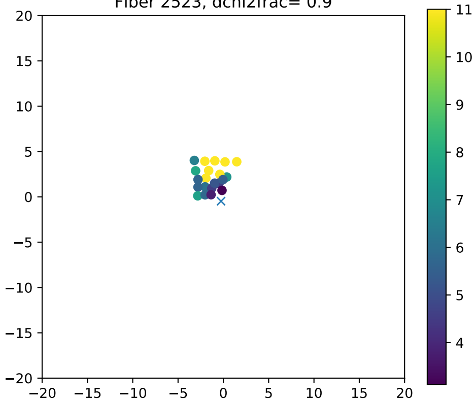
Fiber 2523, dchi2frac= 0.9
