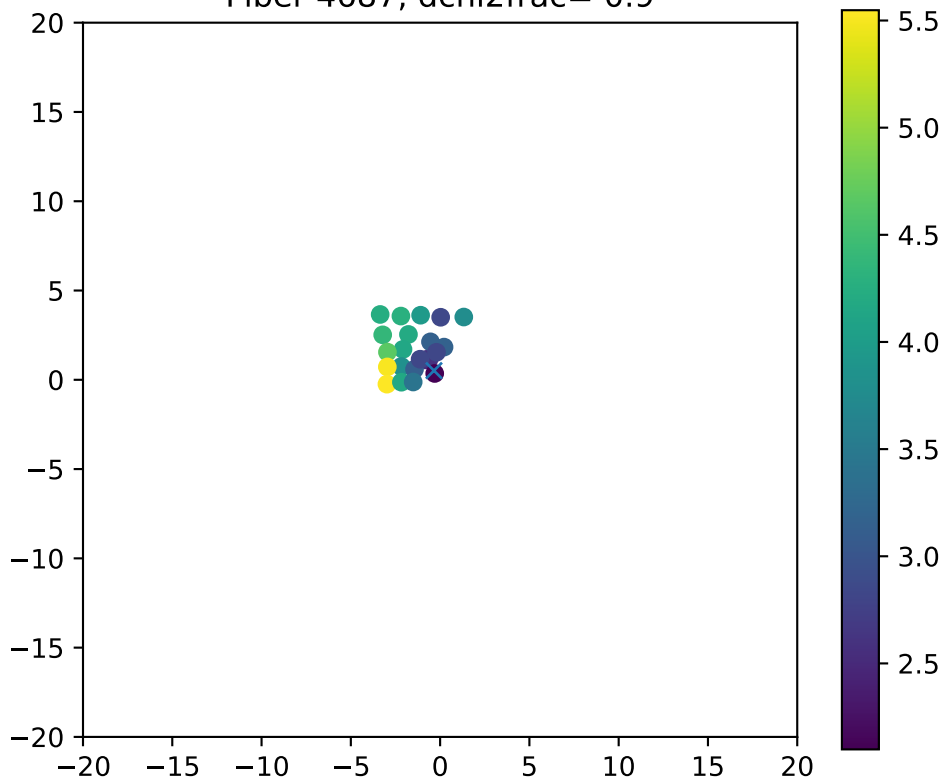
Fiber 4687, dchi2frac= 0.9
