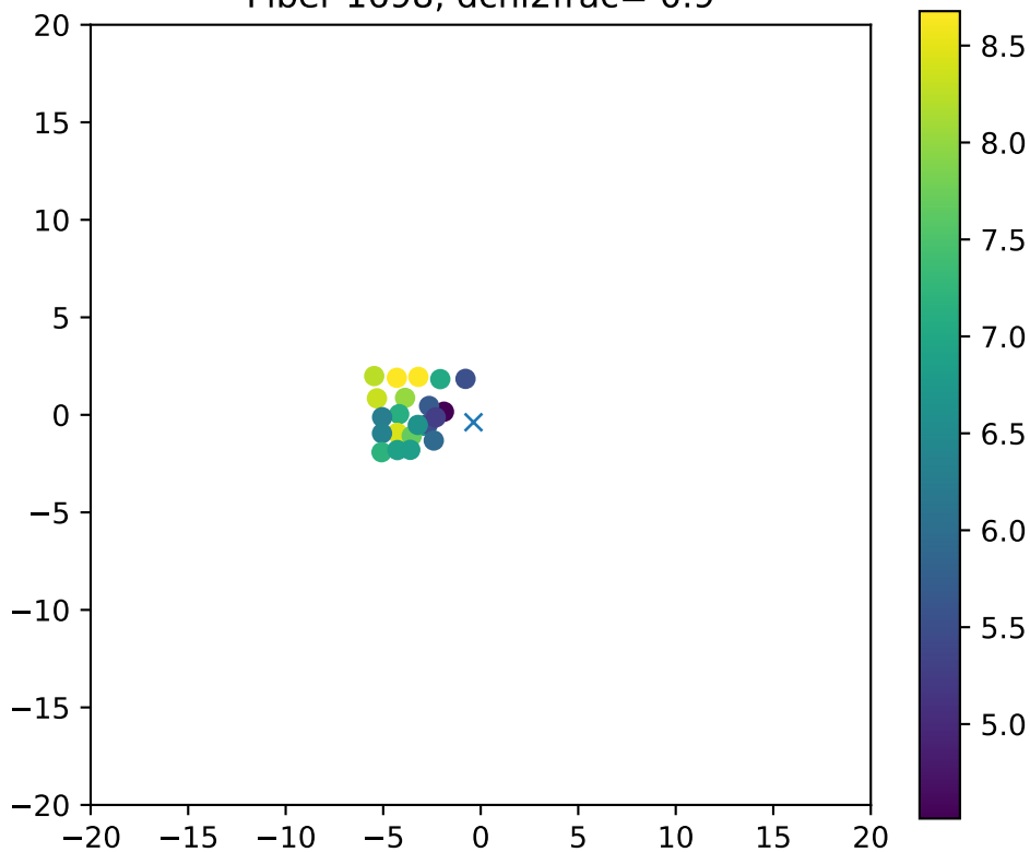
Fiber 1698, dchi2frac= 0.9
