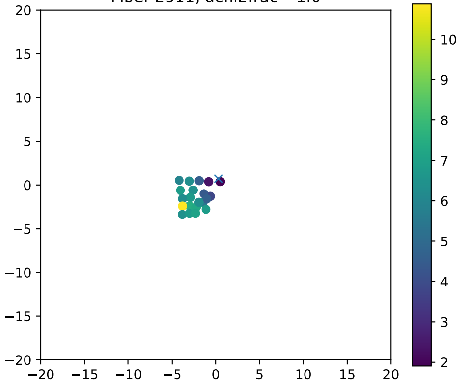
Fiber 2911, dchi2frac= 1.0
