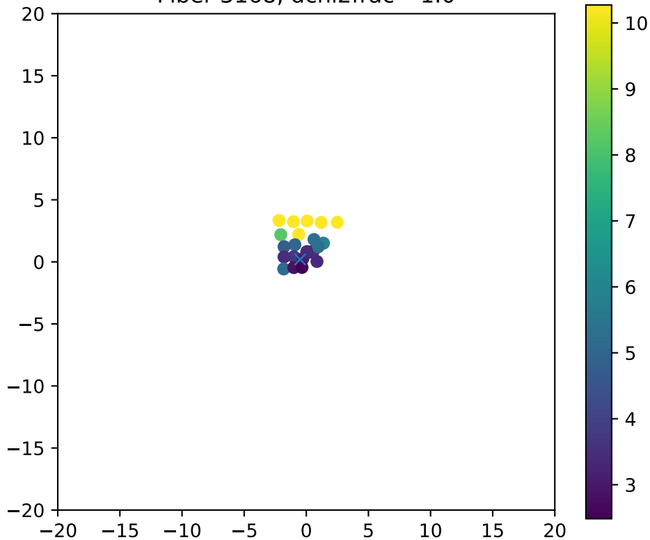
Fiber 3168, dchi2frac= 1.0
