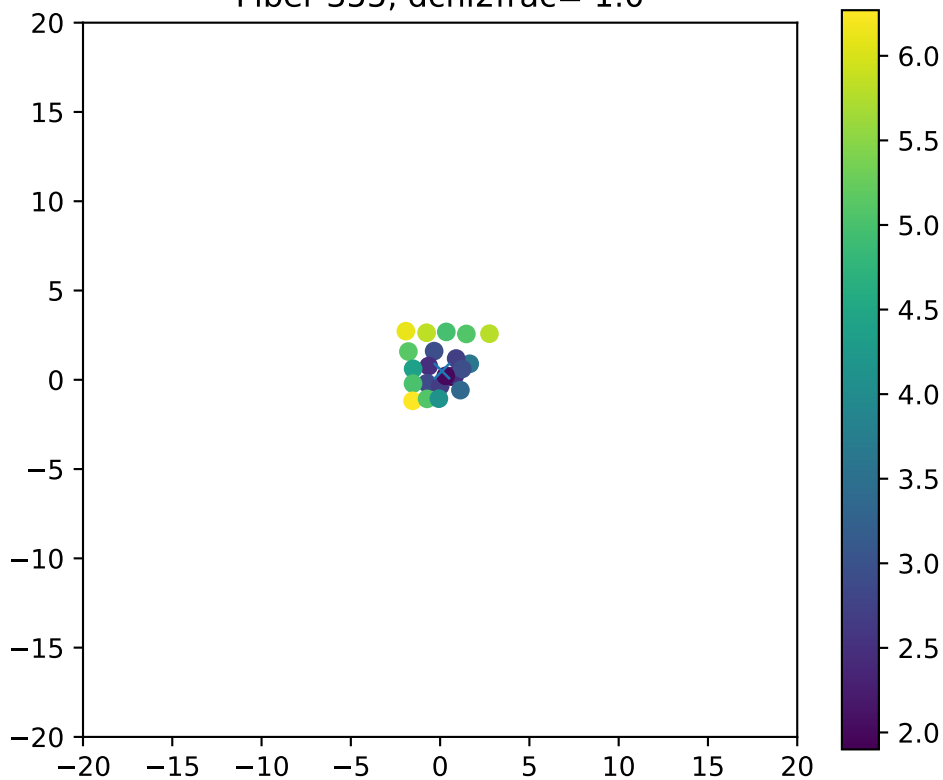
Fiber 355, dchi2frac= 1.0
