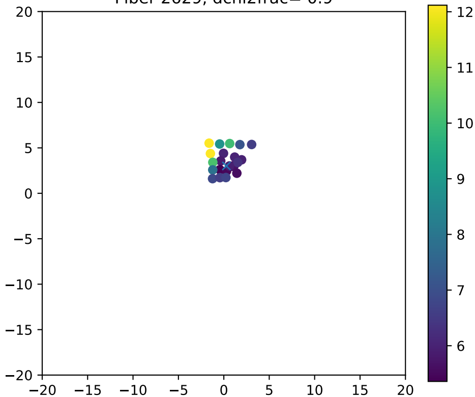
Fiber 2629, dchi2frac= 0.9
