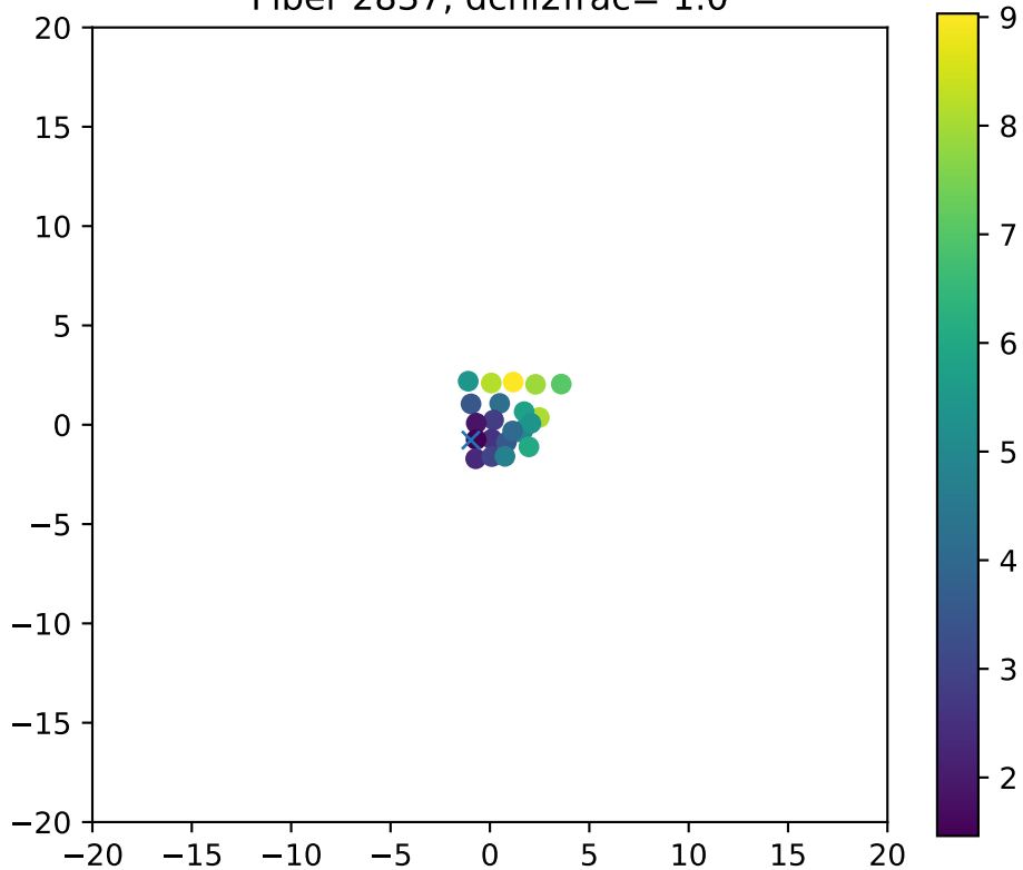
Fiber 2837, dchi2frac= 1.0
