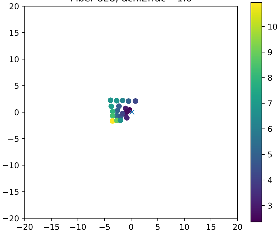
Fiber 828, dchi2frac= 1.0
