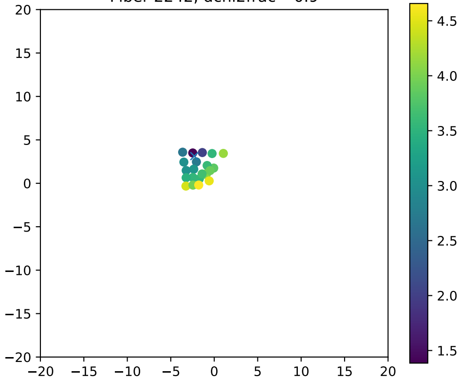
Fiber 2242, dchi2frac= 0.9
