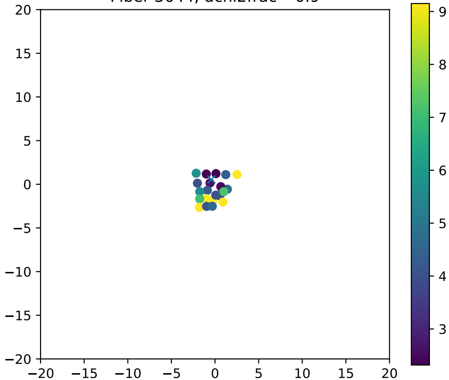
Fiber 3644, dchi2frac= 0.9
