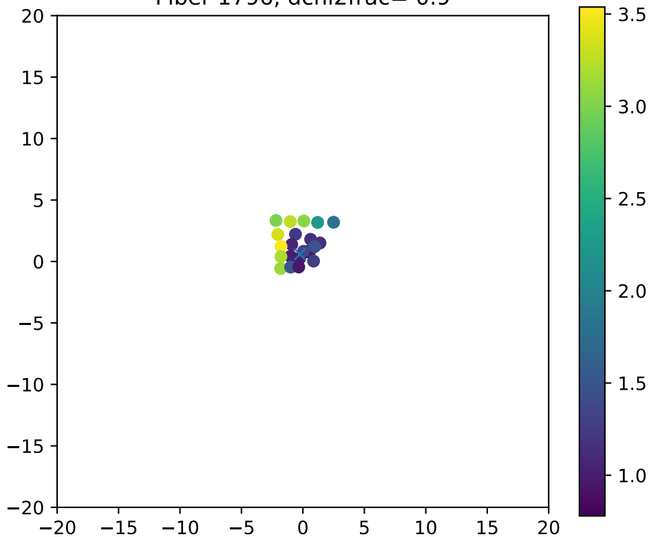
Fiber 1796, dchi2frac= 0.9
