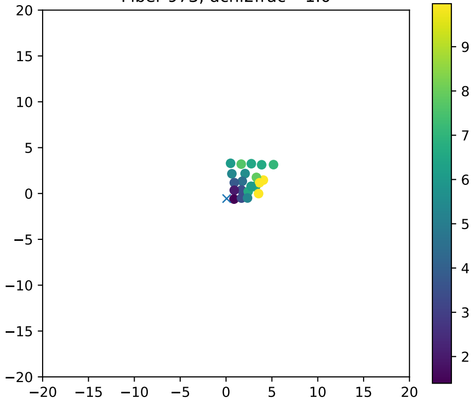
Fiber 973, dchi2frac= 1.0
