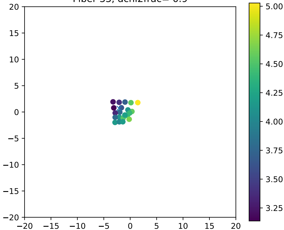
Fiber 33, dchi2frac= 0.9
