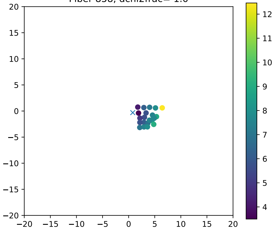
Fiber 858, dchi2frac= 1.0
