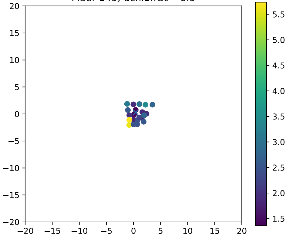
Fiber 149, dchi2frac= 0.9
