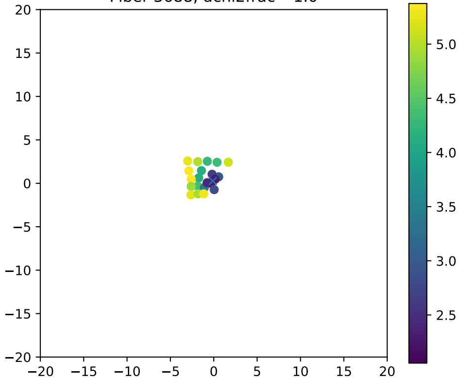
Fiber 3688, dchi2frac= 1.0
