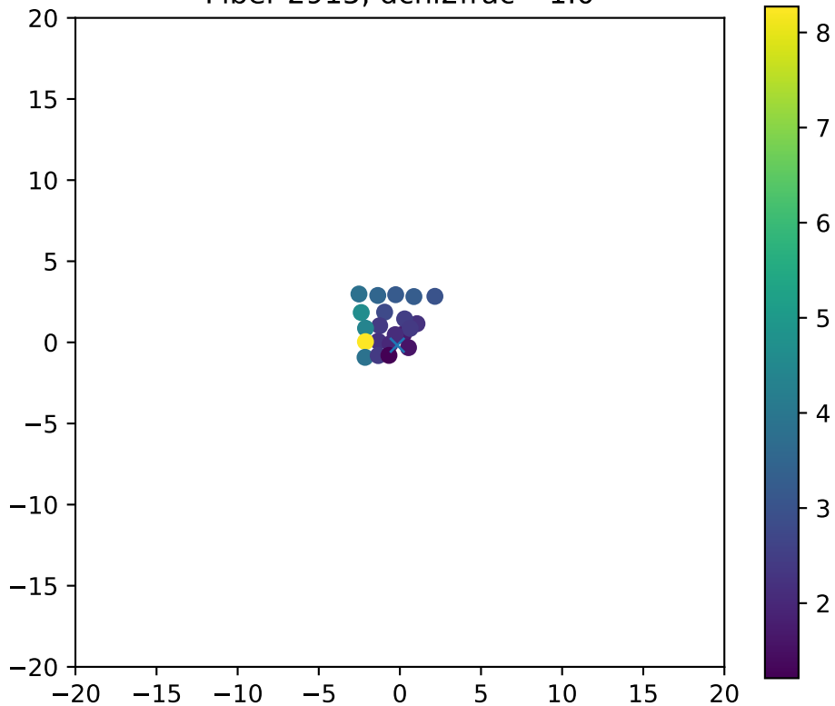
Fiber 2915, dchi2frac= 1.0
