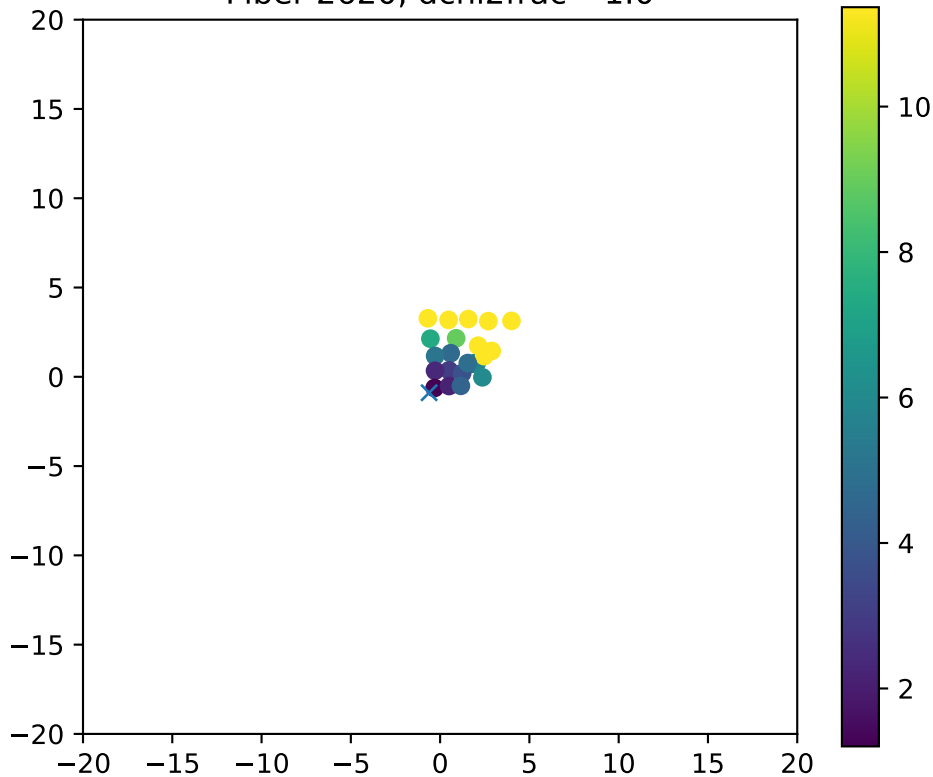
Fiber 2620, dchi2frac= 1.0
