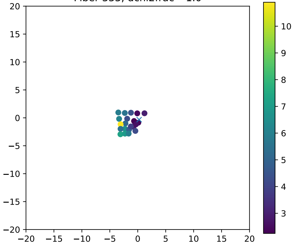
Fiber 333, dchi2frac= 1.0
