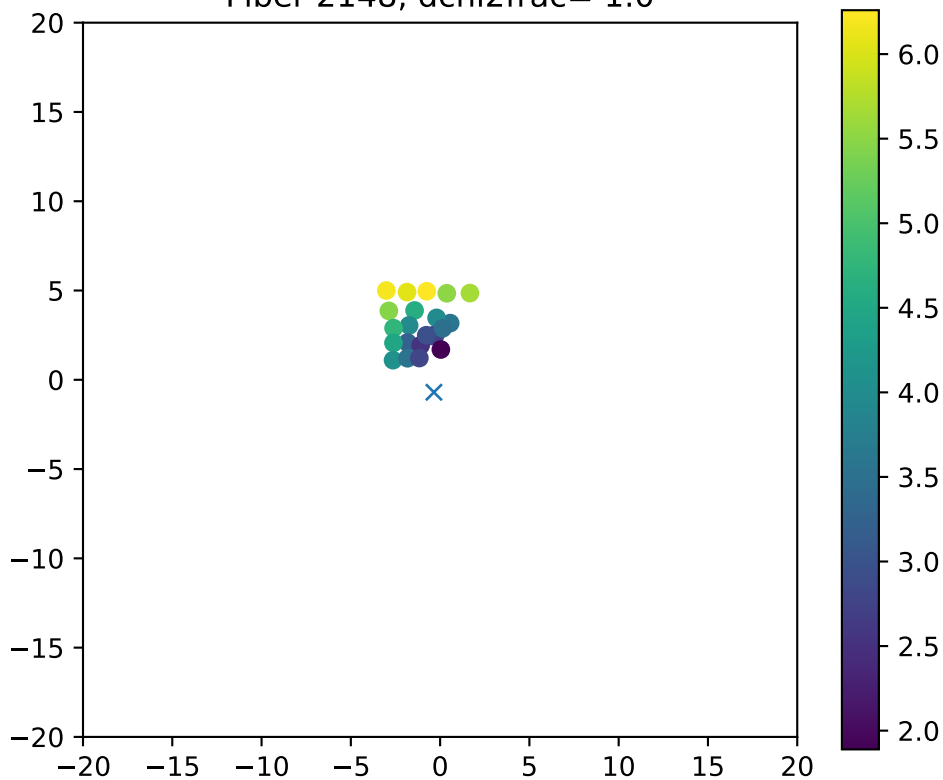
Fiber 2148, dchi2frac= 1.0
