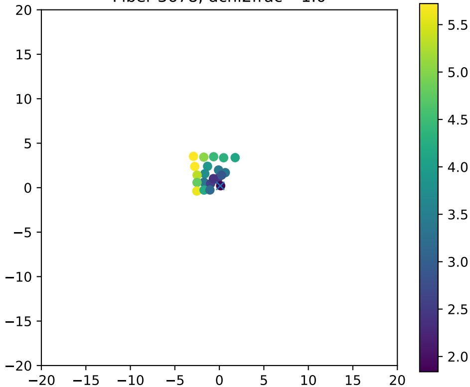
Fiber 3678, dchi2frac= 1.0
