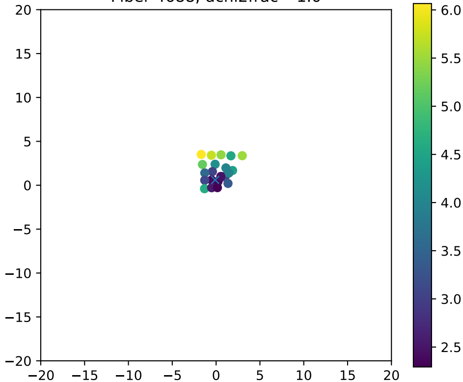
Fiber 4688, dchi2frac= 1.0
