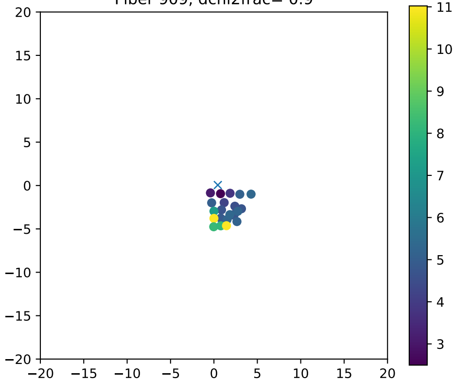
Fiber 909, dchi2frac= 0.9
