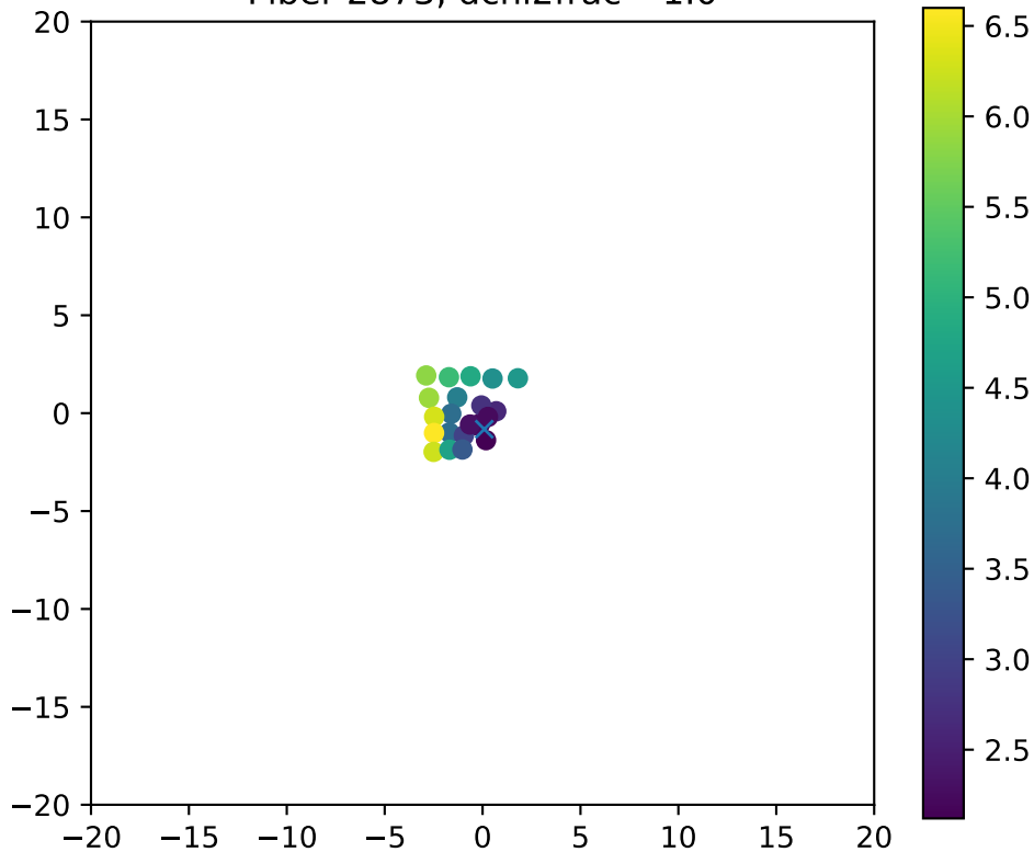
Fiber 2873, dchi2frac= 1.0
