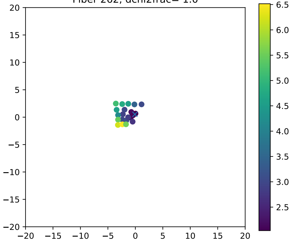
Fiber 262, dchi2frac= 1.0
