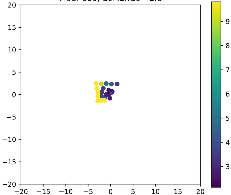
Fiber 630, dchi2frac= 1.0
