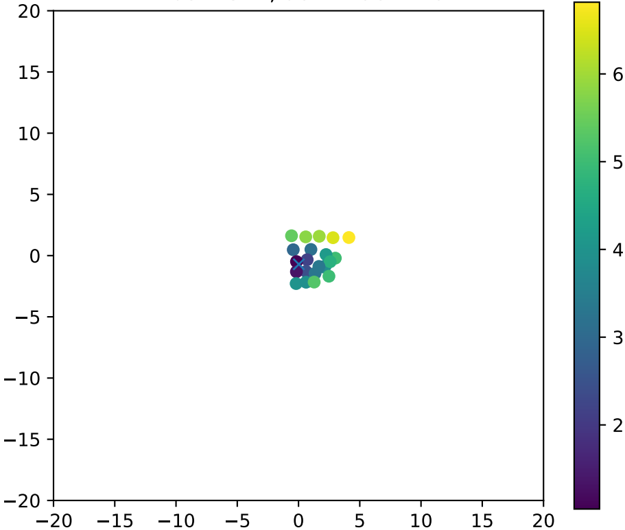
Fiber 2522, dchi2frac= 1.0
