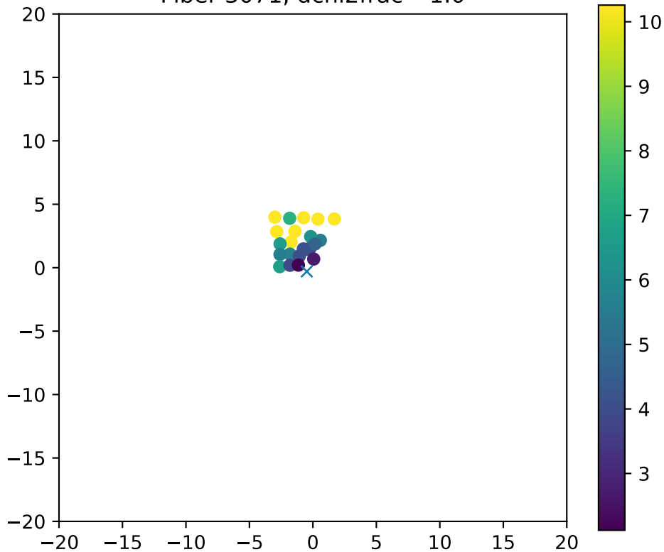
Fiber 3071, dchi2frac= 1.0
