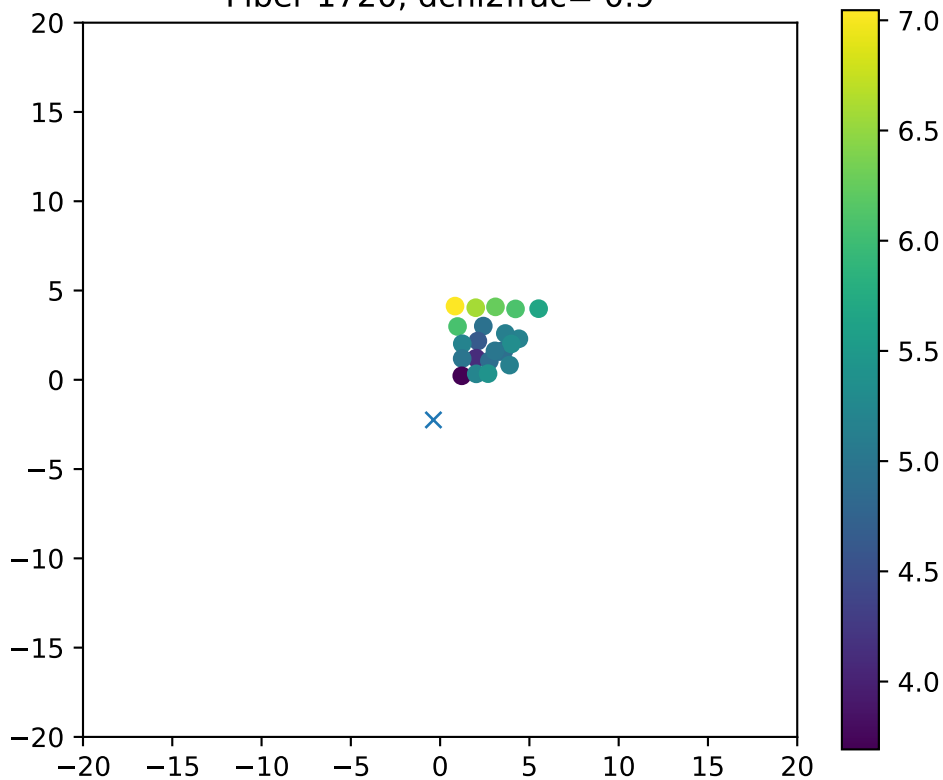
Fiber 1720, dchi2frac= 0.9
