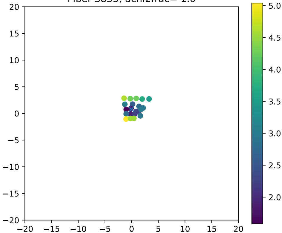
Fiber 3855, dchi2frac= 1.0
