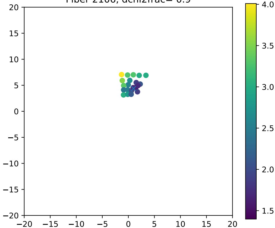
Fiber 2106, dchi2frac= 0.9
