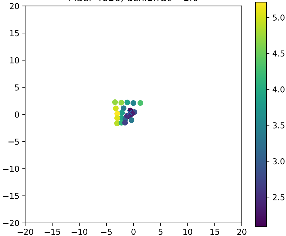
Fiber 4626, dchi2frac= 1.0
