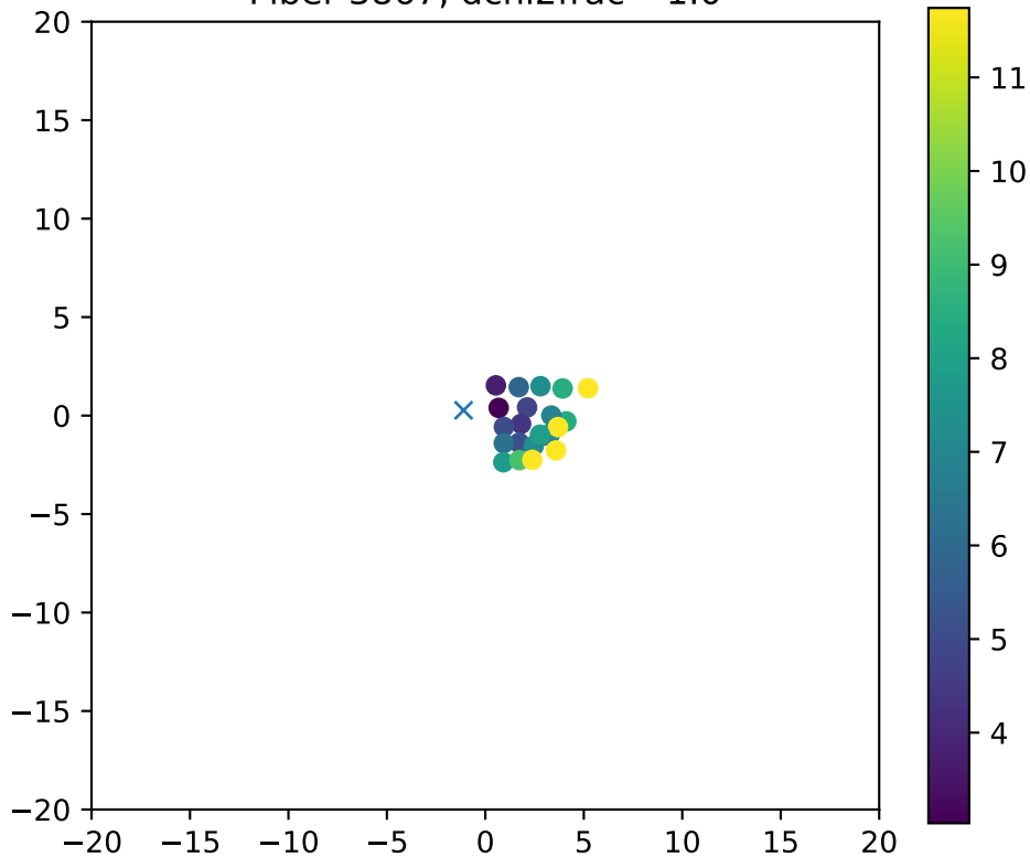
Fiber 3867, dchi2frac= 1.0
