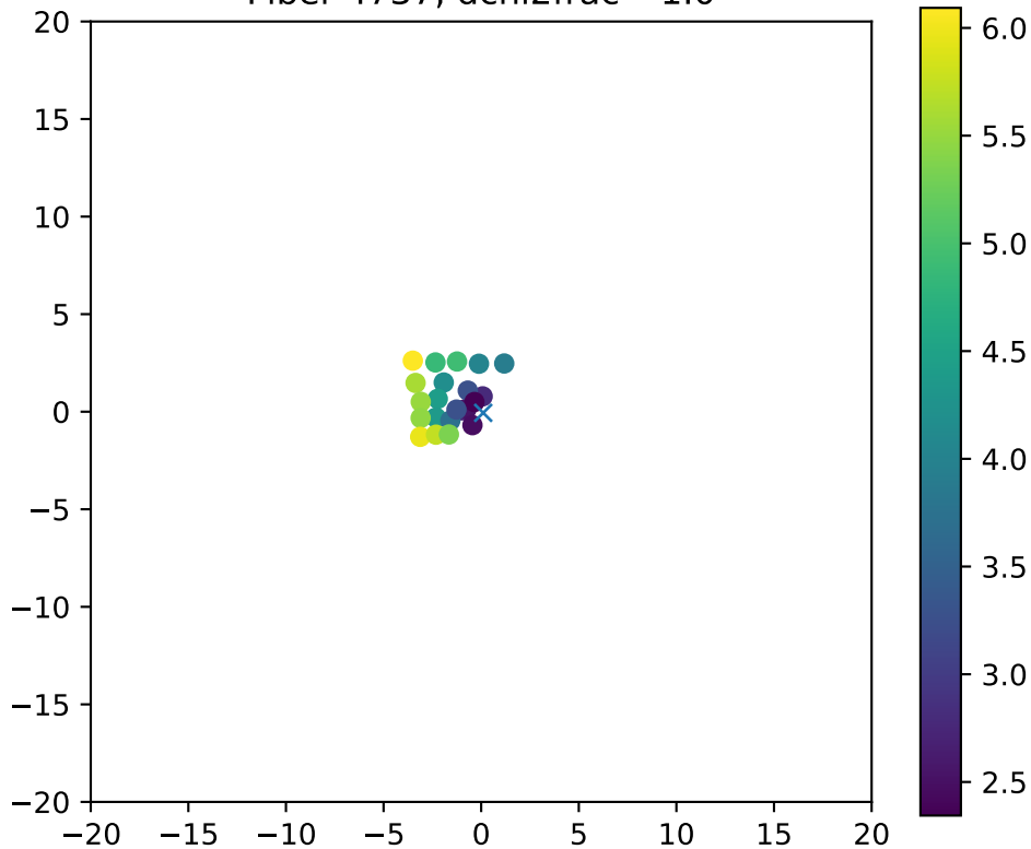
Fiber 4737, dchi2frac= 1.0
