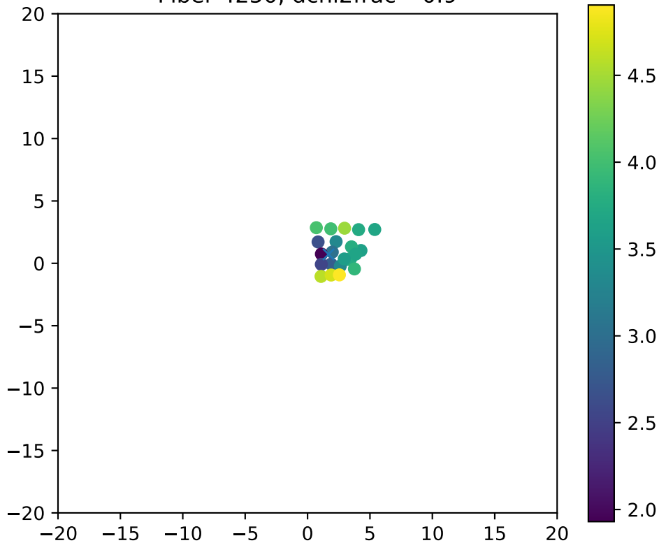
Fiber 4250, dchi2frac= 0.9
