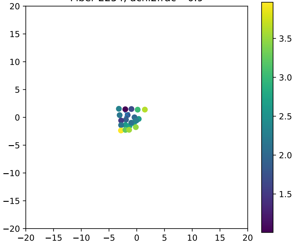
Fiber 2254, dchi2frac= 0.9
