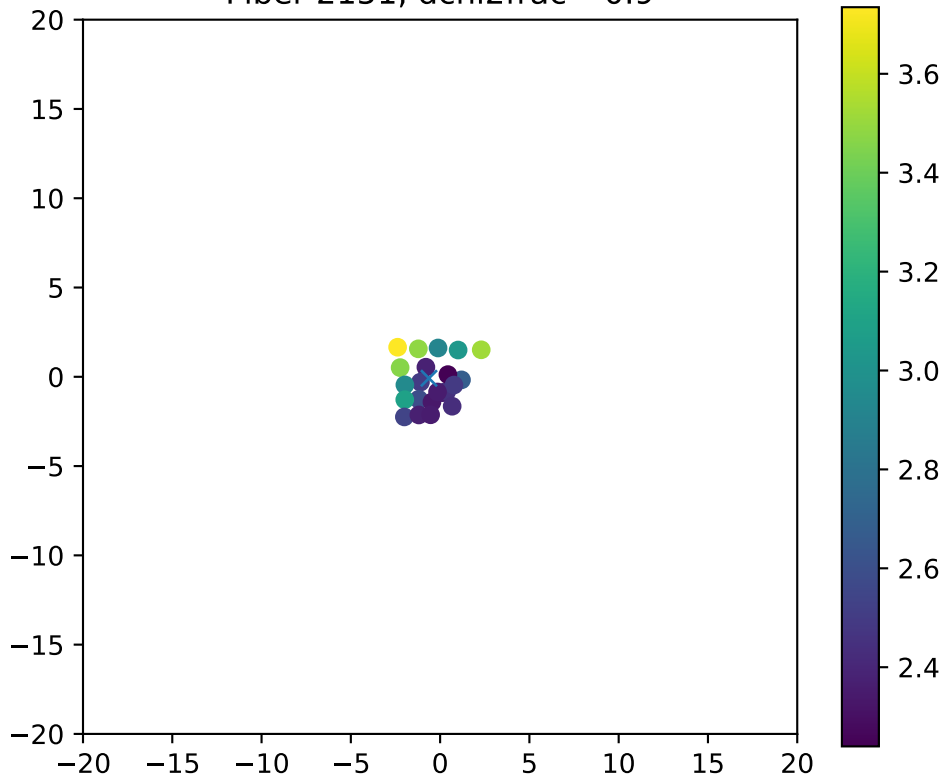
Fiber 2151, dchi2frac= 0.9
