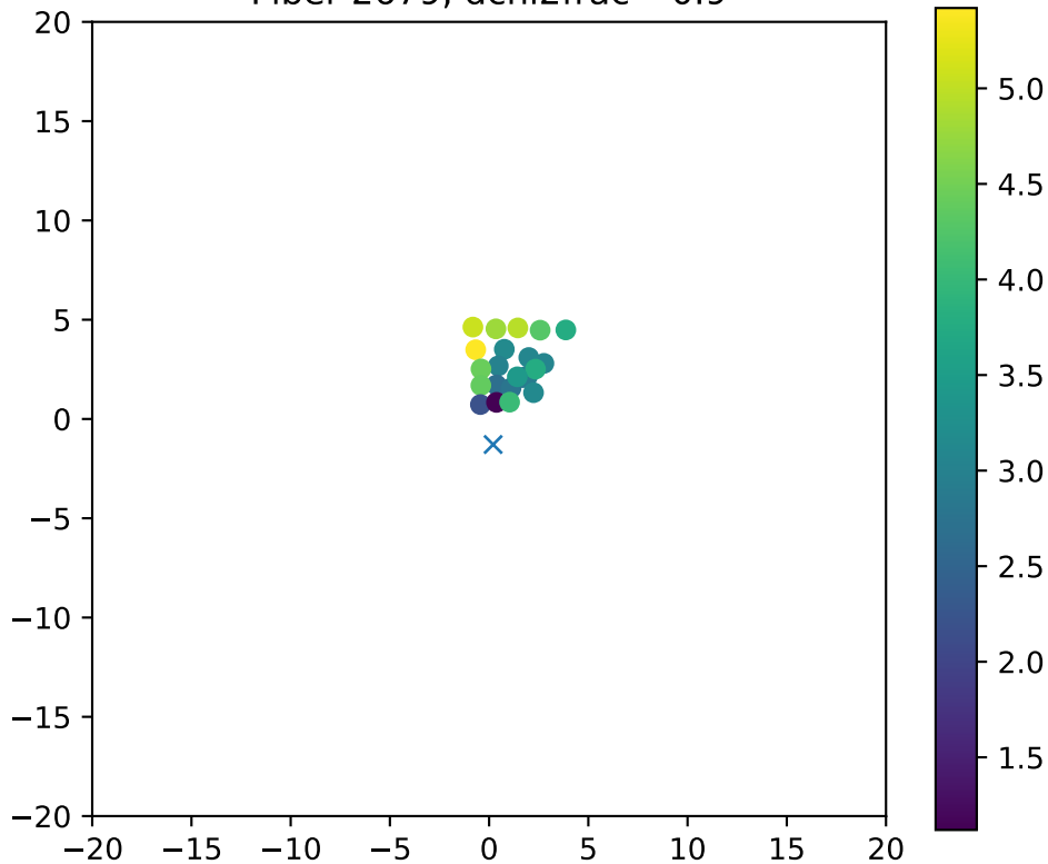
Fiber 2679, dchi2frac= 0.9
