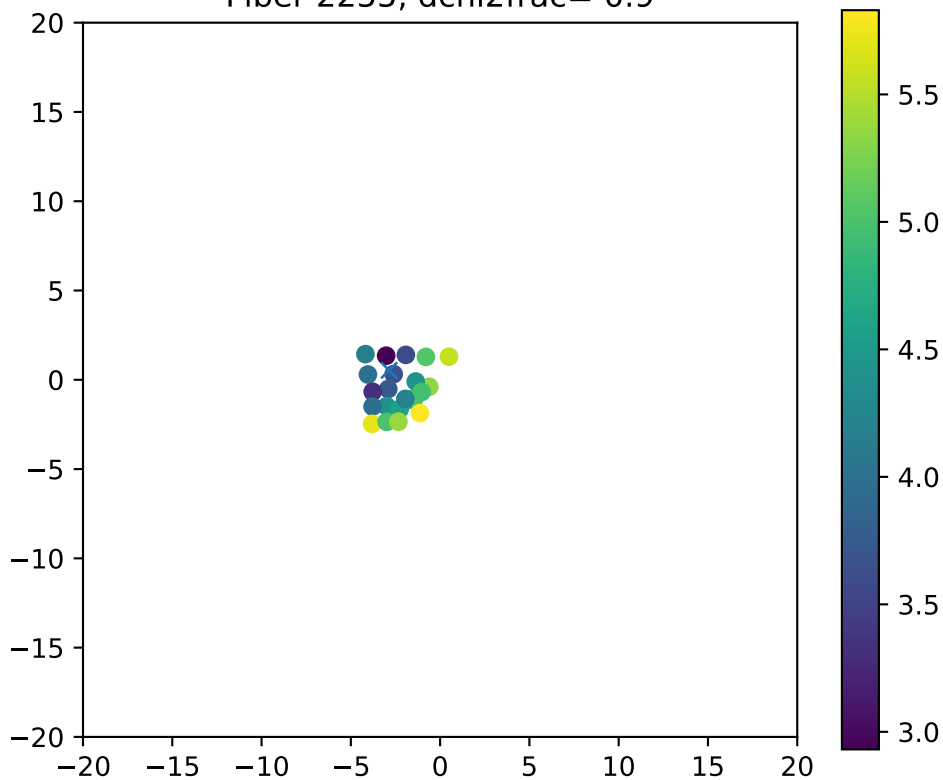
Fiber 2255, dchi2frac= 0.9
