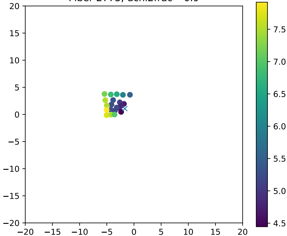
Fiber 2773, dchi2frac= 0.9
