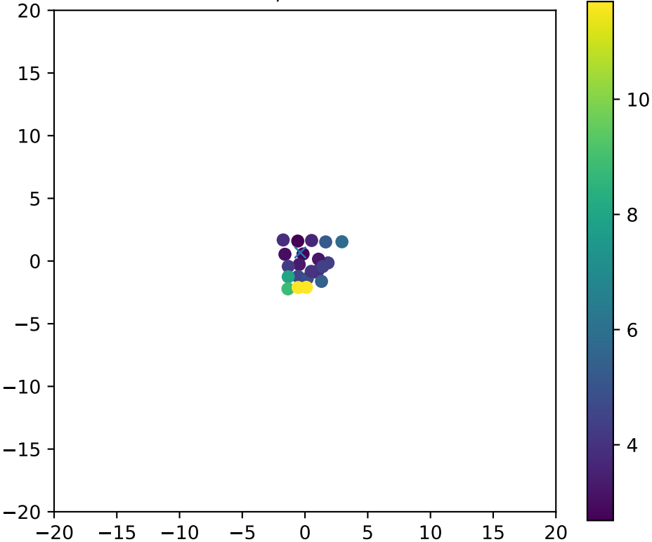
Fiber 3491, dchi2frac= 1.0
