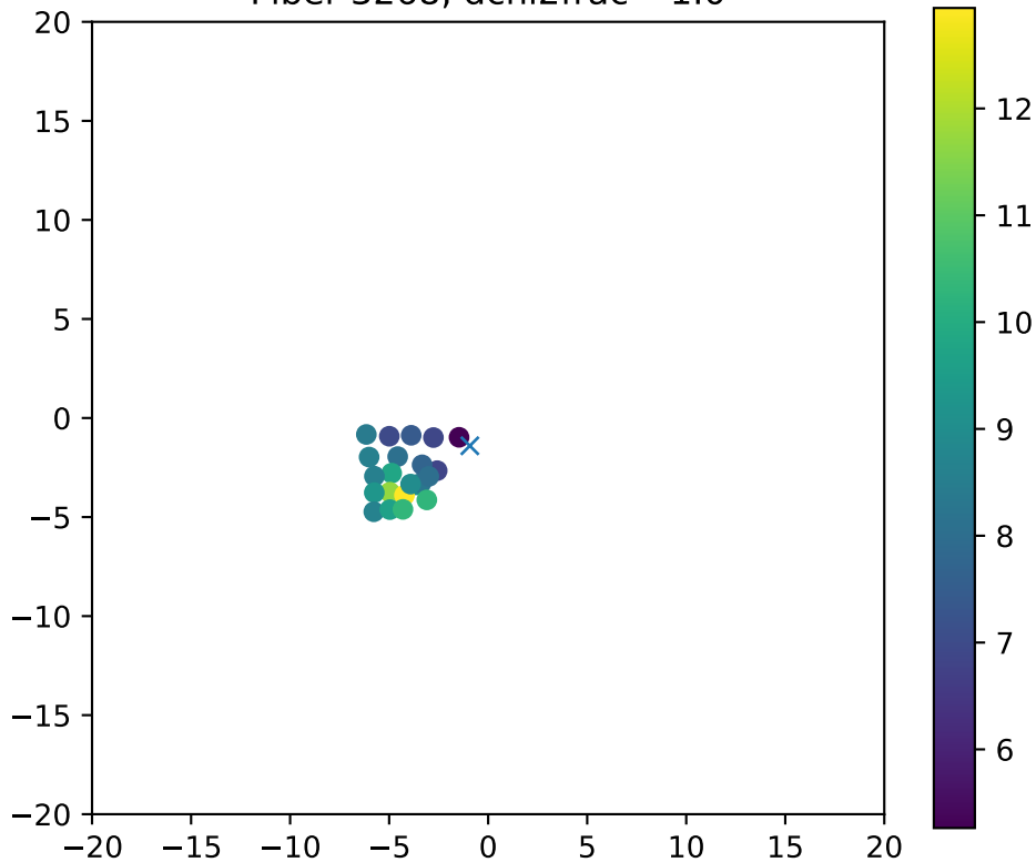
Fiber 3268, dchi2frac= 1.0
