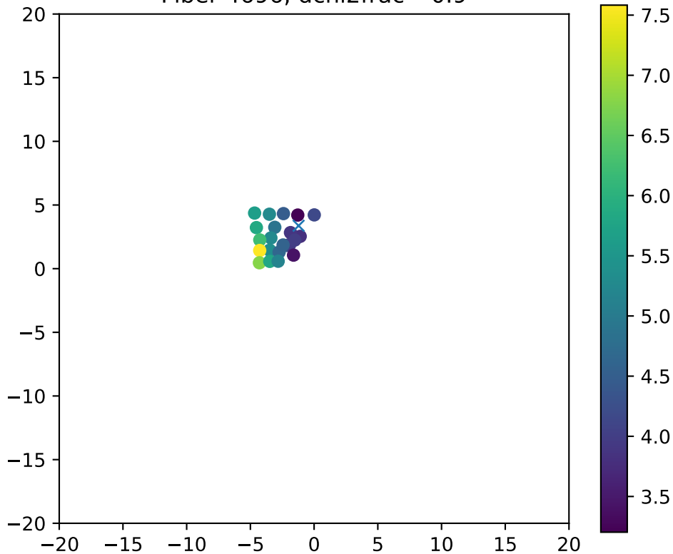
Fiber 4696, dchi2frac= 0.9
