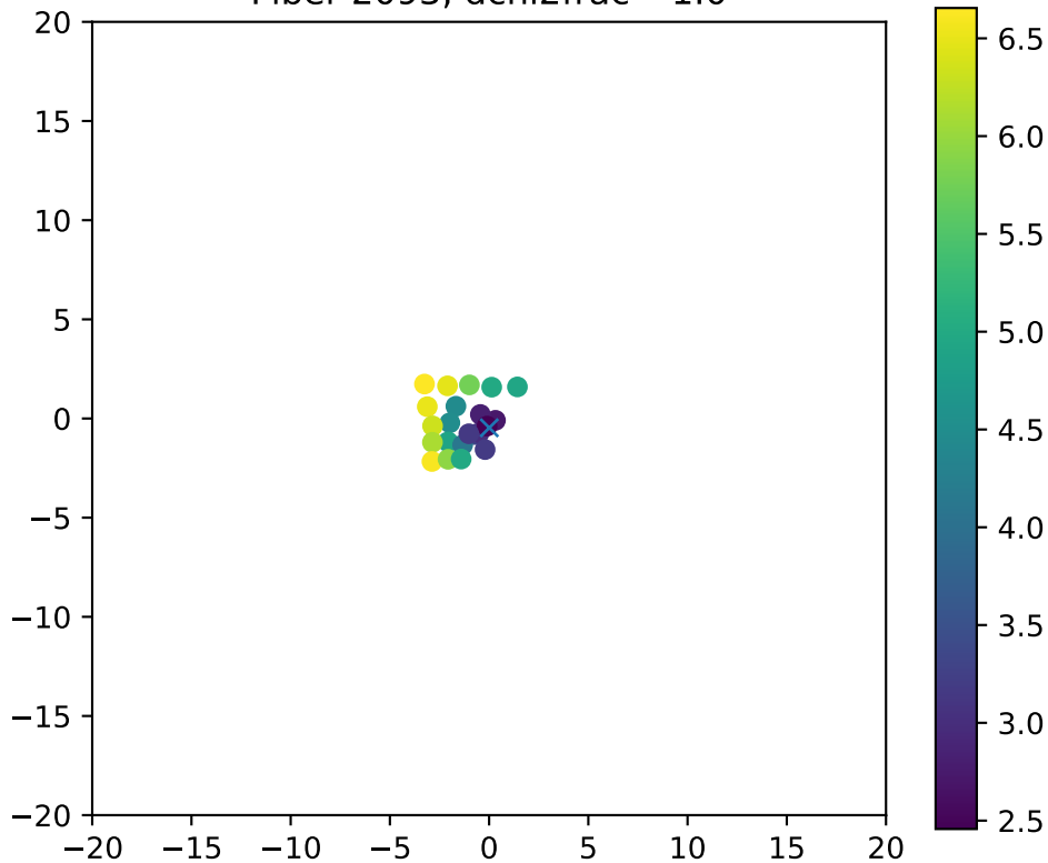
Fiber 2093, dchi2frac= 1.0
