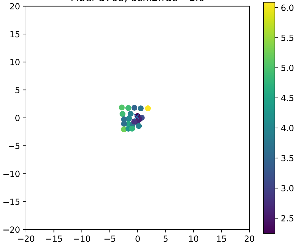
Fiber 3708, dchi2frac= 1.0
