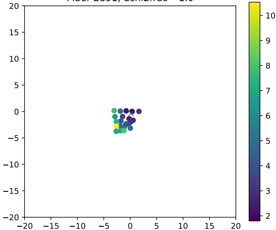
Fiber 2891, dchi2frac= 1.0
