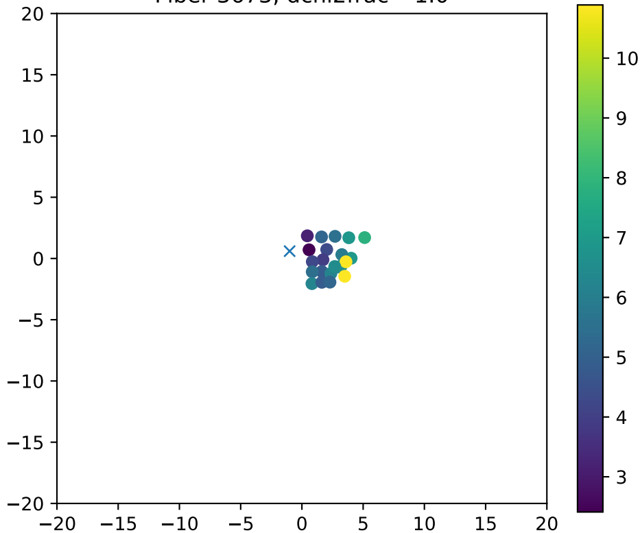
Fiber 3673, dchi2frac= 1.0
