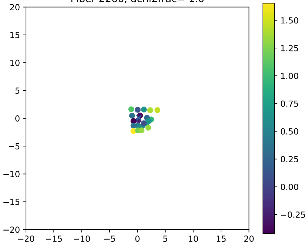
Fiber 2266, dchi2frac= 1.0
