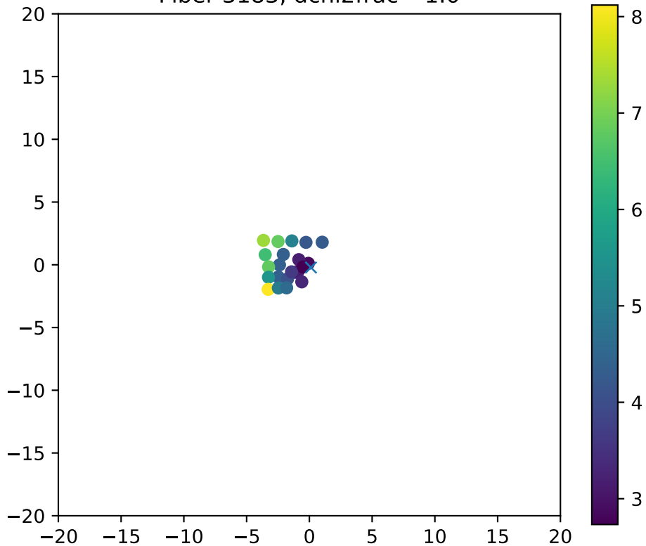
Fiber 3183, dchi2frac= 1.0
