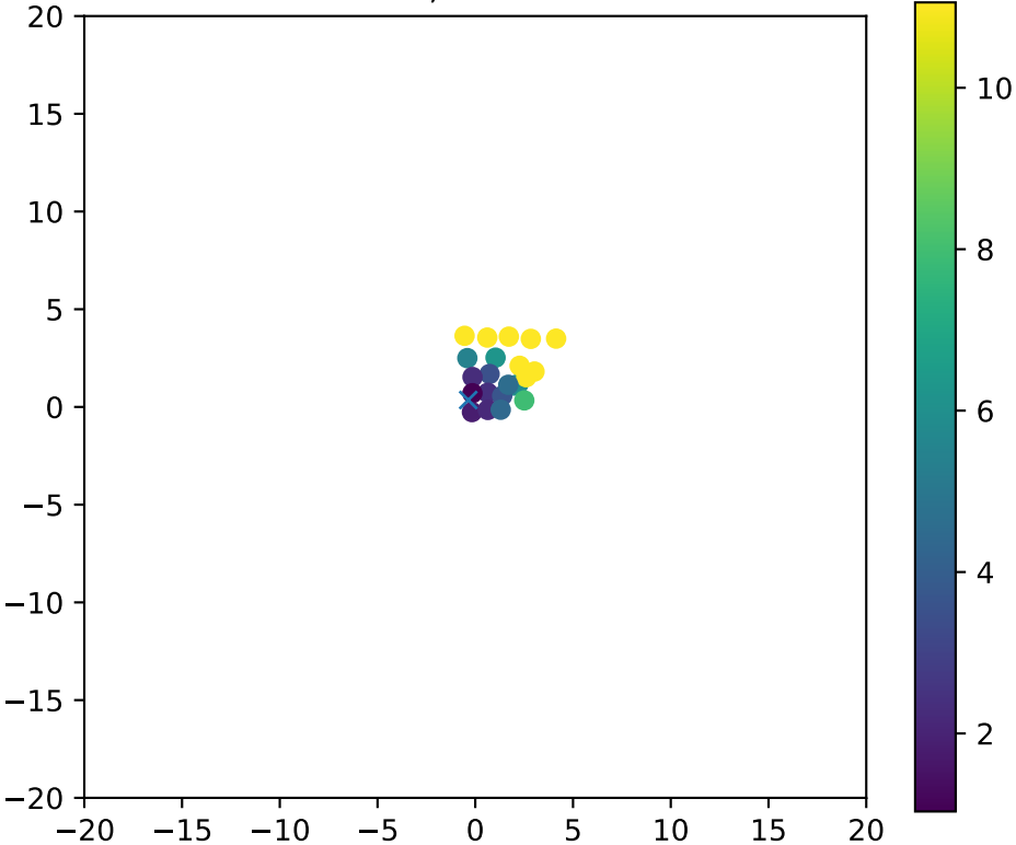
Fiber 4979, dchi2frac= 1.0
