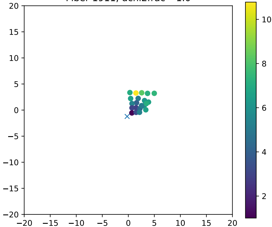
Fiber 1911, dchi2frac= 1.0
