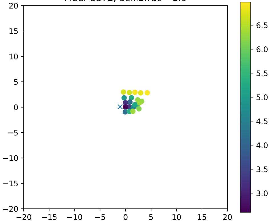
Fiber 3372, dchi2frac= 1.0
