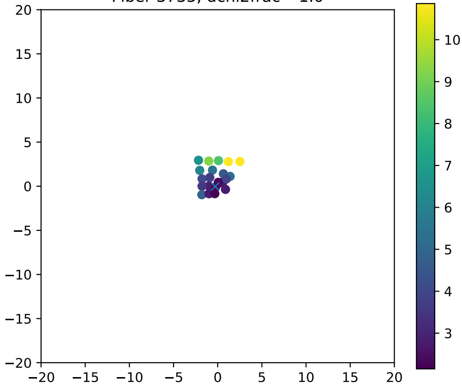
Fiber 3735, dchi2frac= 1.0
