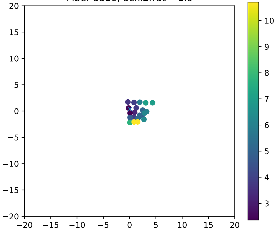
Fiber 3320, dchi2frac= 1.0
