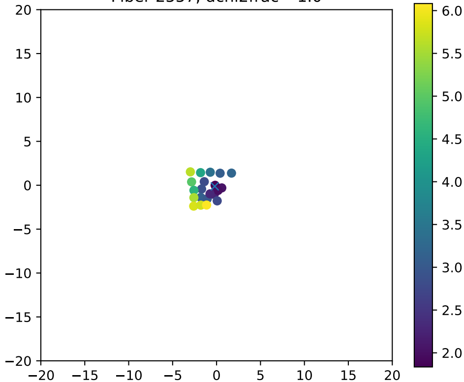
Fiber 2557, dchi2frac= 1.0
