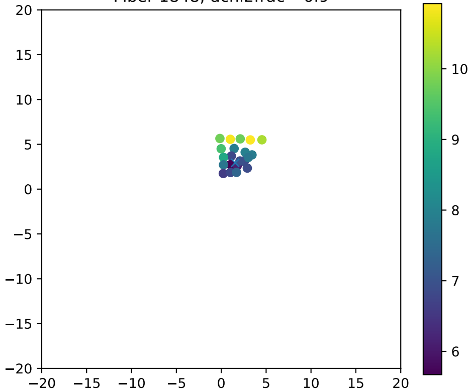
Fiber 1848, dchi2frac= 0.9
