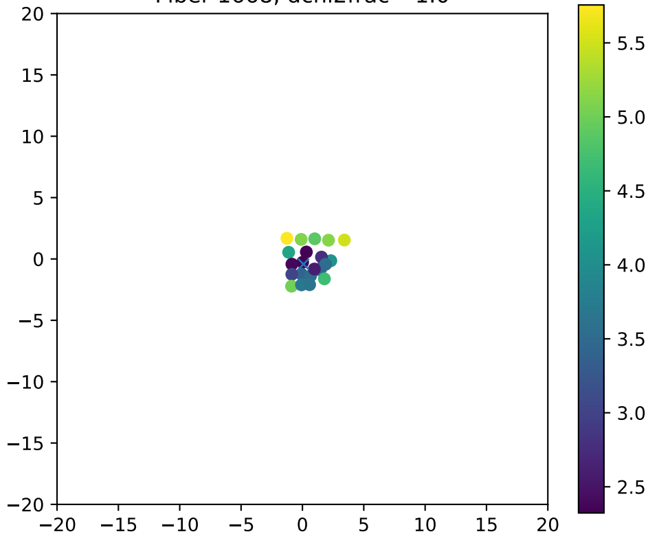
Fiber 1668, dchi2frac= 1.0
