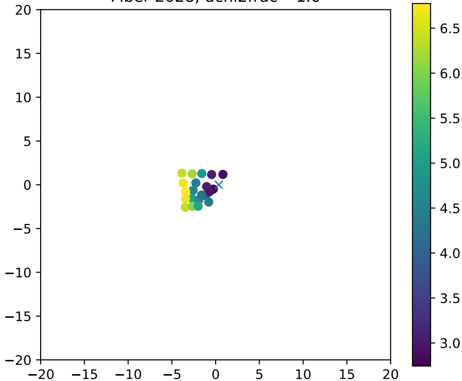
Fiber 2028, dchi2frac= 1.0
