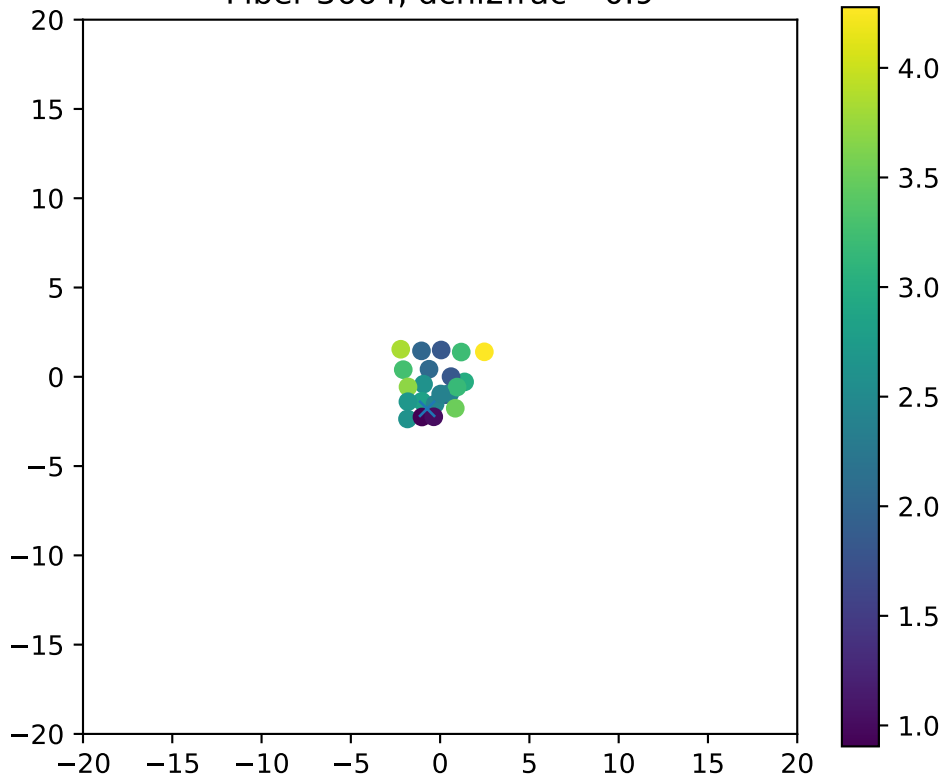
Fiber 3664, dchi2frac= 0.9
