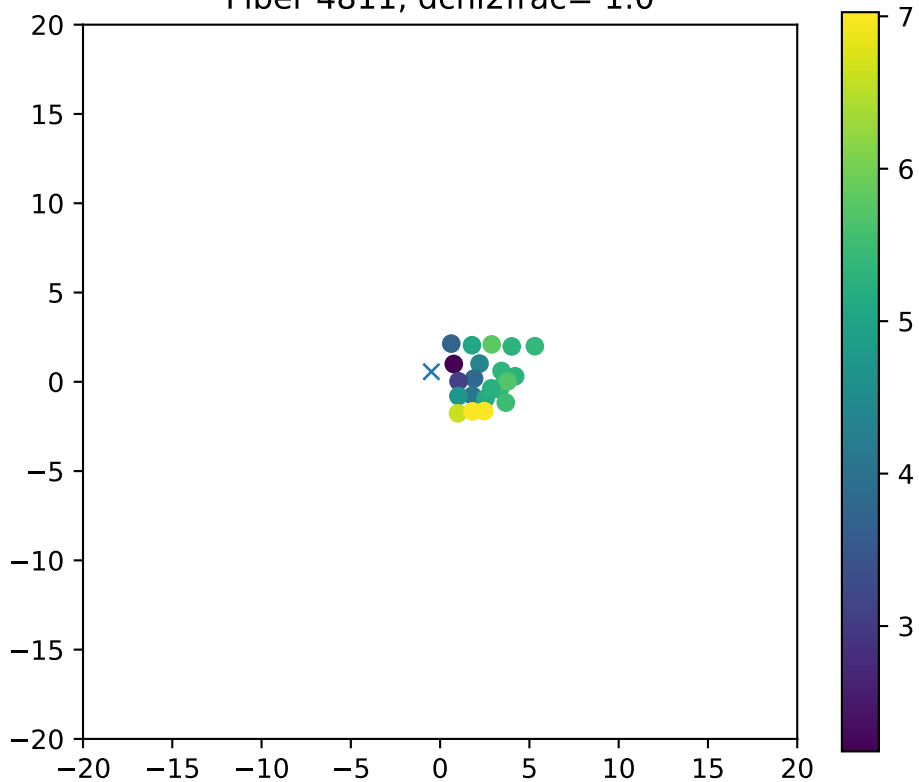
Fiber 4811, dchi2frac= 1.0
