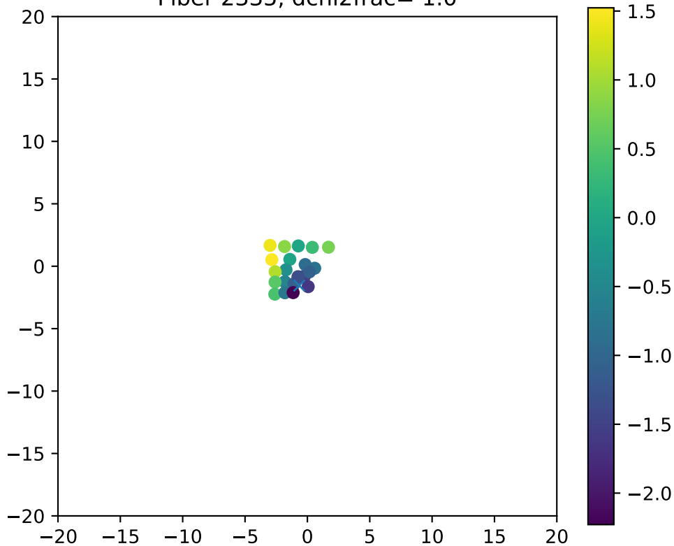
Fiber 2335, dchi2frac= 1.0
