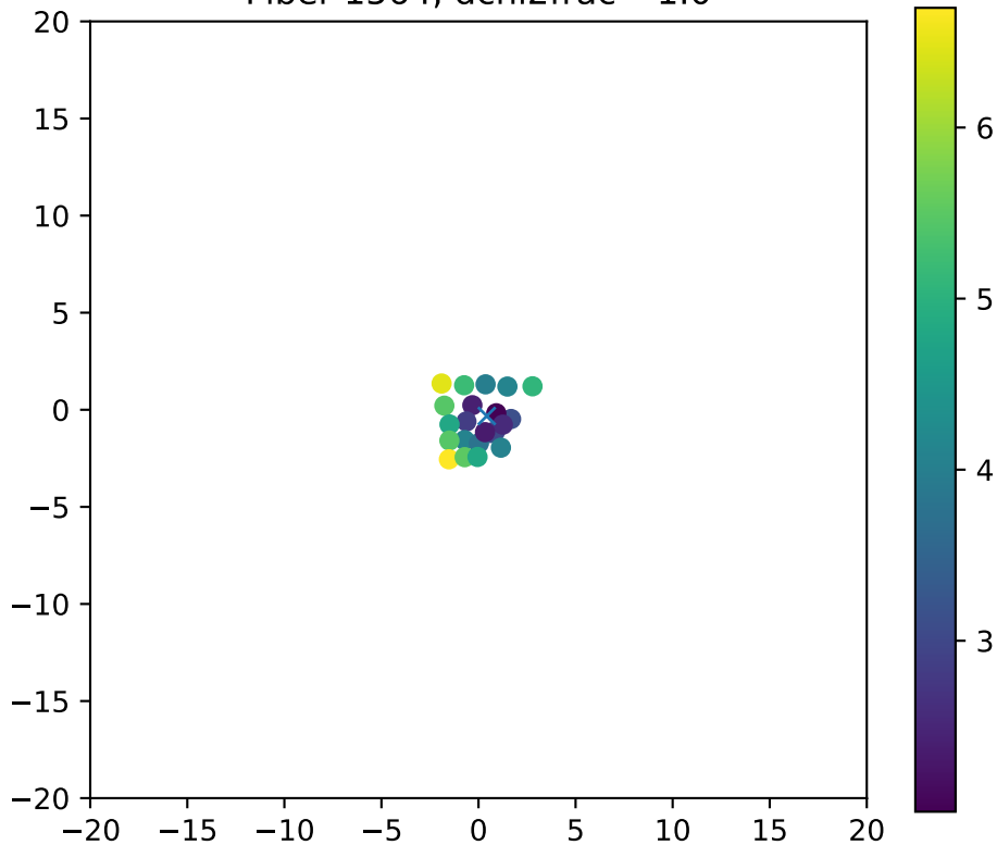
Fiber 1564, dchi2frac= 1.0
