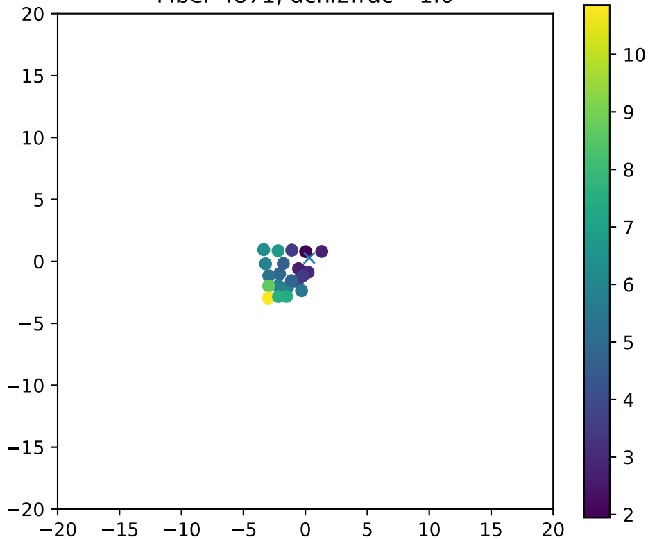
Fiber 4871, dchi2frac= 1.0
