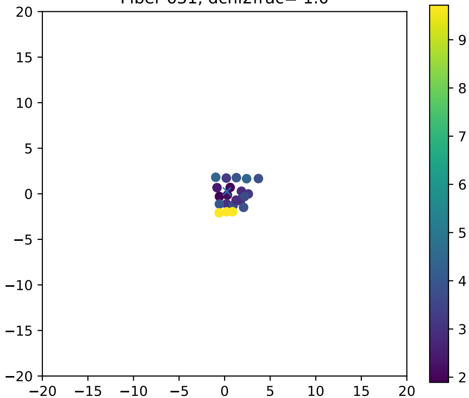
Fiber 631, dchi2frac= 1.0
