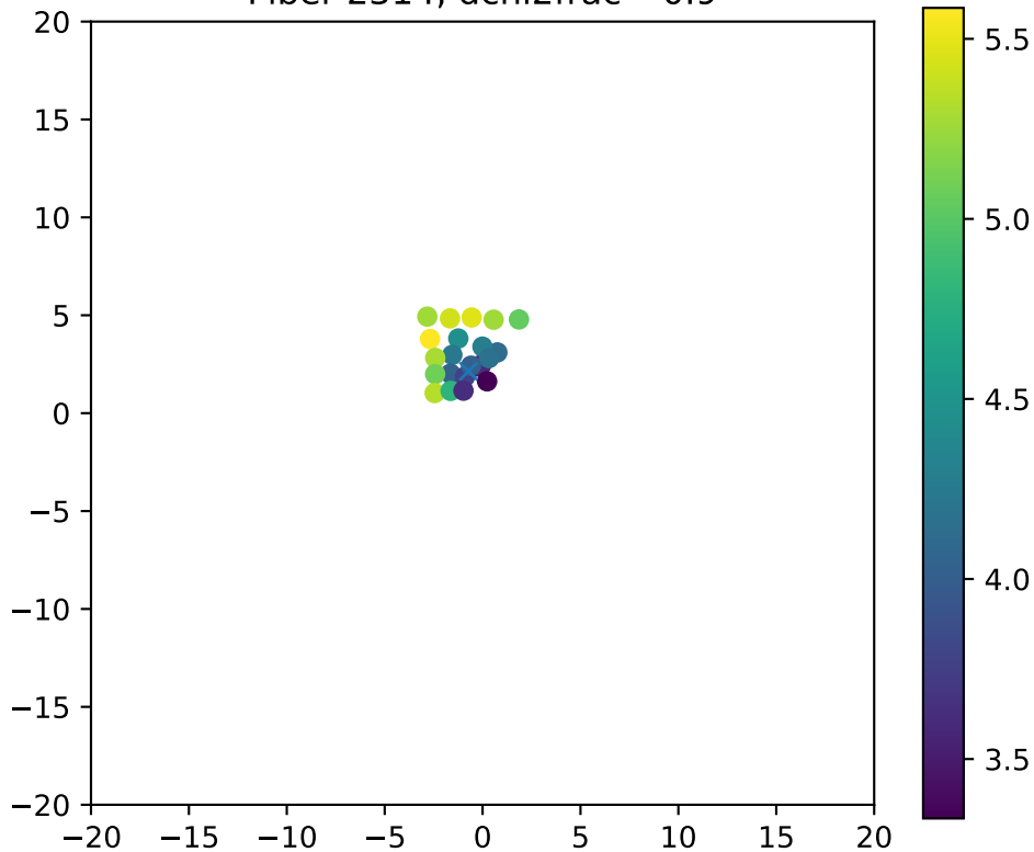
Fiber 2314, dchi2frac= 0.9
