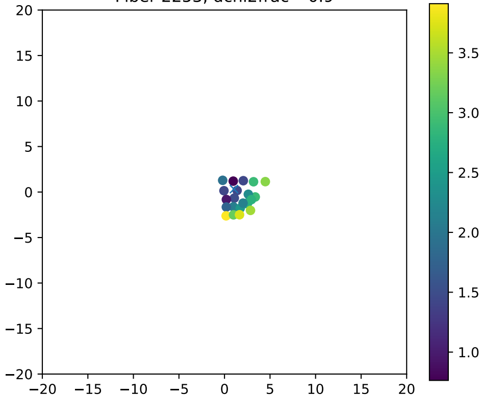
Fiber 2253, dchi2frac= 0.9
