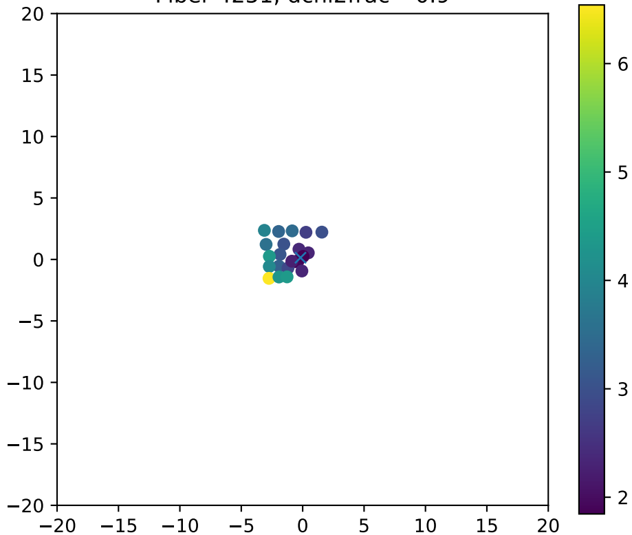
Fiber 4251, dchi2frac= 0.9
