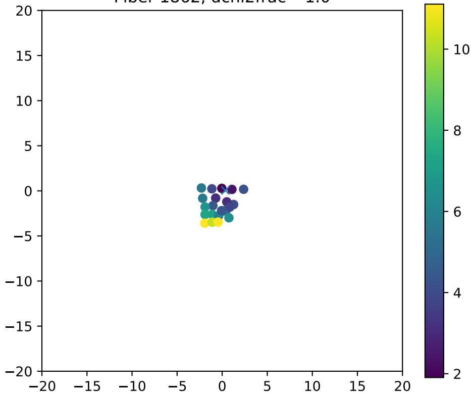
Fiber 1862, dchi2frac= 1.0
