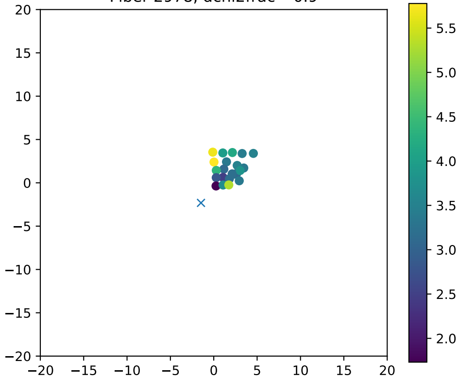
Fiber 2978, dchi2frac= 0.9
