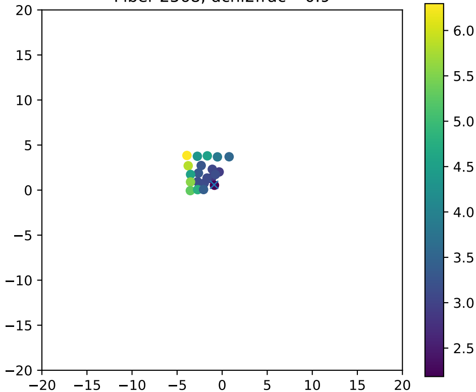
Fiber 2568, dchi2frac= 0.9
