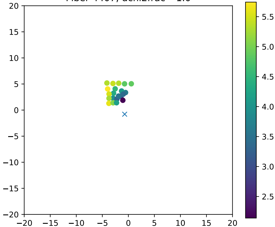
Fiber 4407, dchi2frac= 1.0
