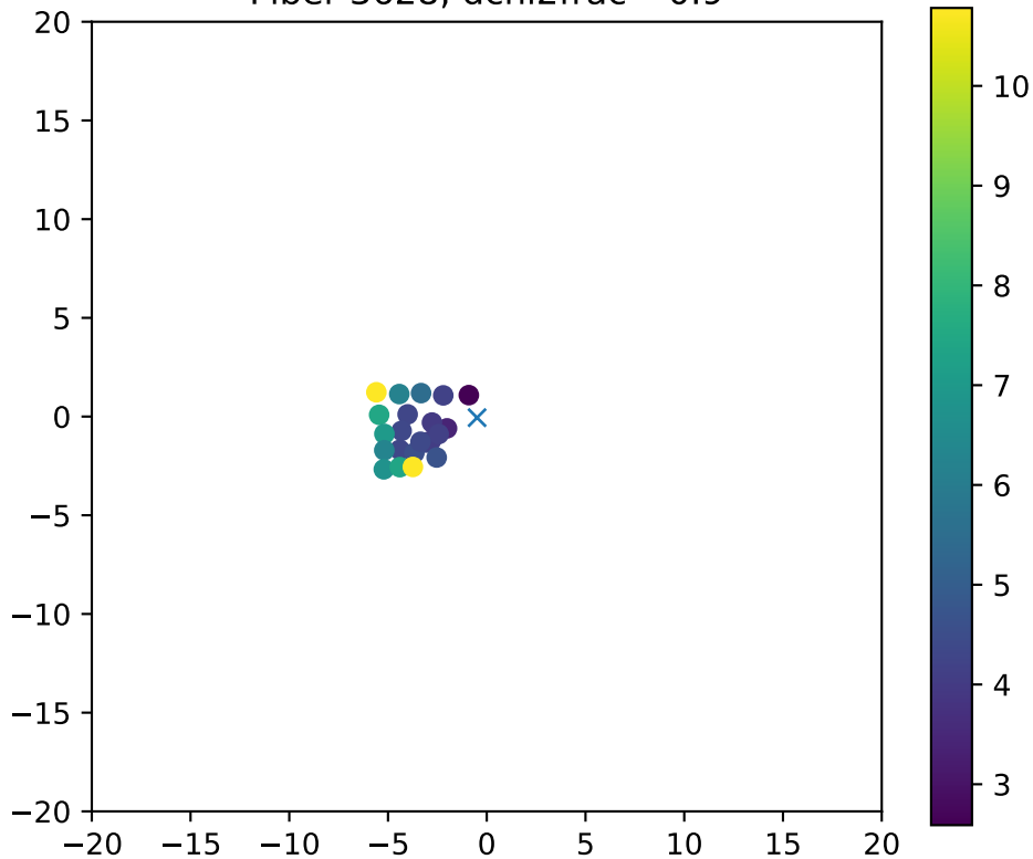
Fiber 3628, dchi2frac= 0.9
