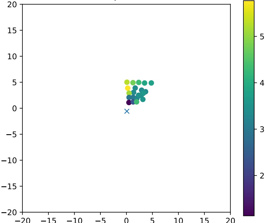
Fiber 4278, dchi2frac= 0.9
