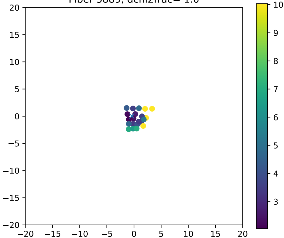
Fiber 3889, dchi2frac= 1.0
