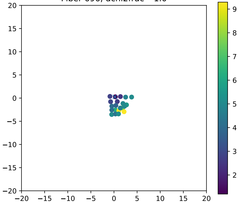
Fiber 696, dchi2frac= 1.0
