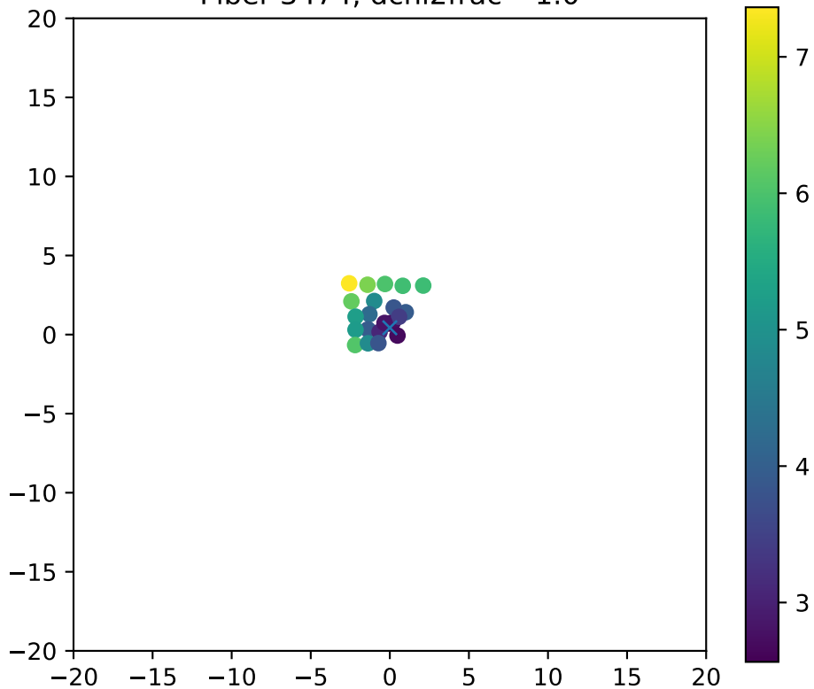
Fiber 3474, dchi2frac= 1.0
