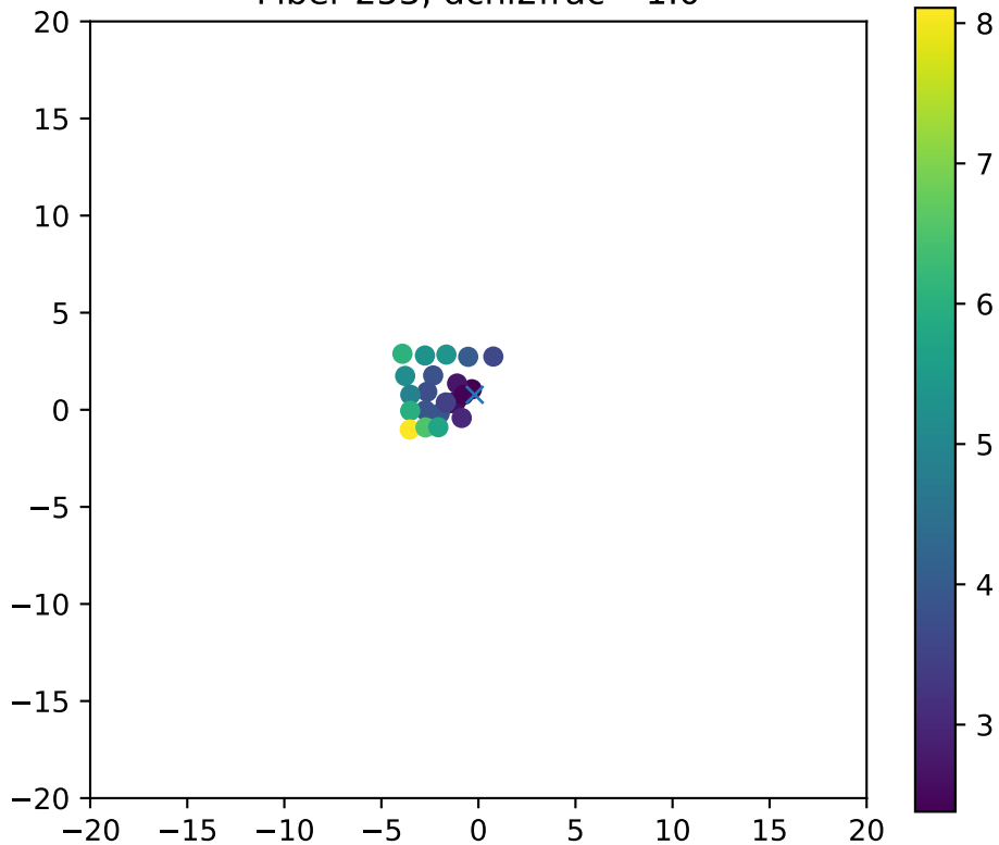
Fiber 253, dchi2frac= 1.0
