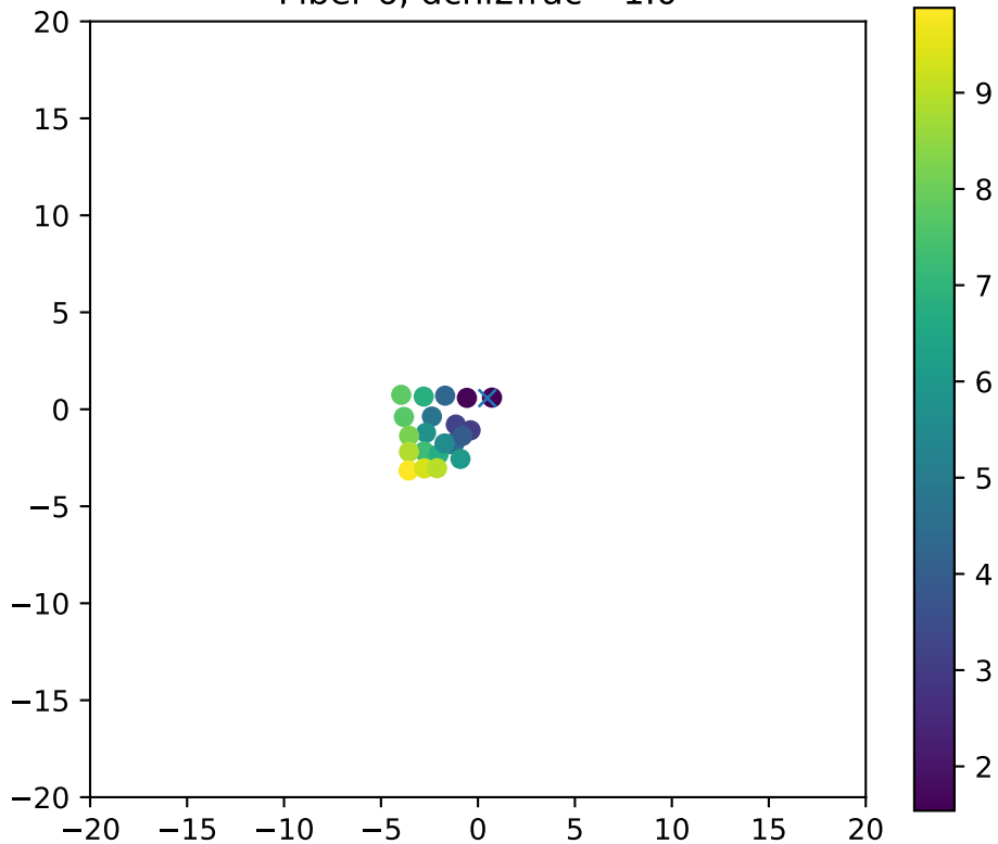
Fiber 6, dchi2frac= 1.0
