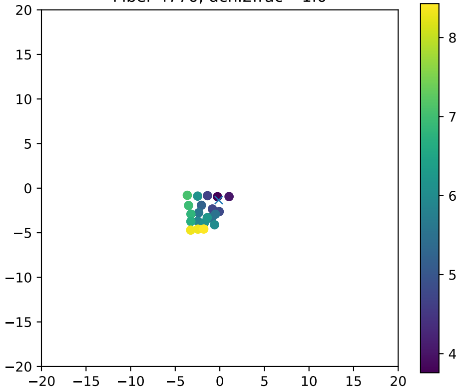
Fiber 4770, dchi2frac= 1.0
