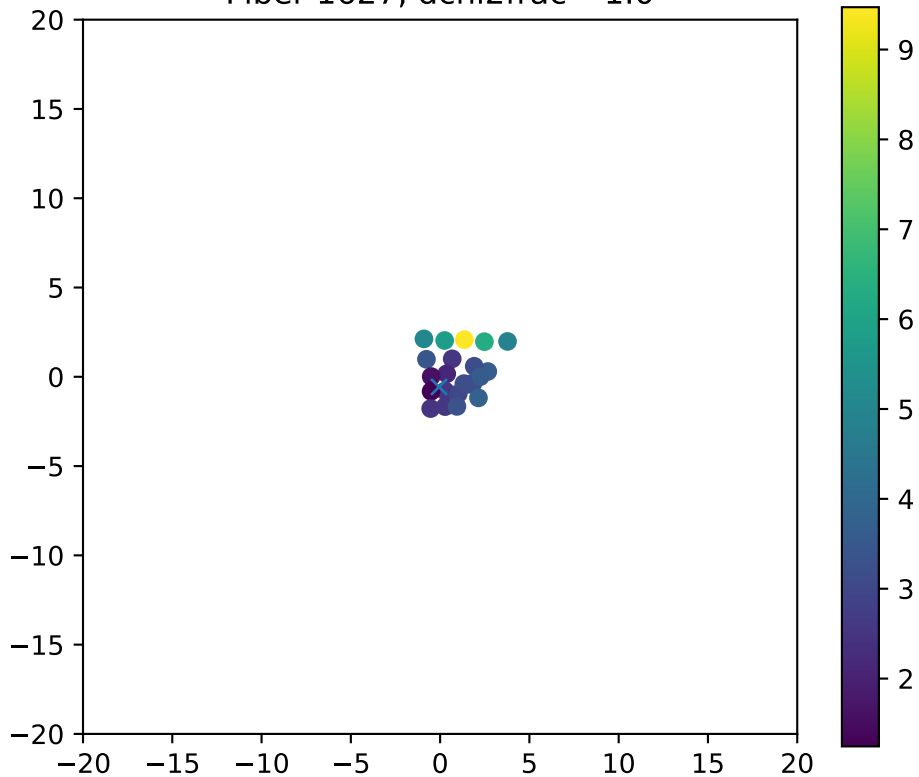
Fiber 1627, dchi2frac= 1.0
