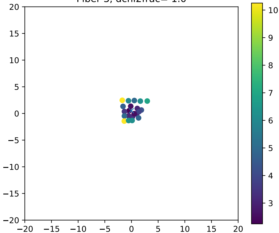
Fiber 3, dchi2frac= 1.0
