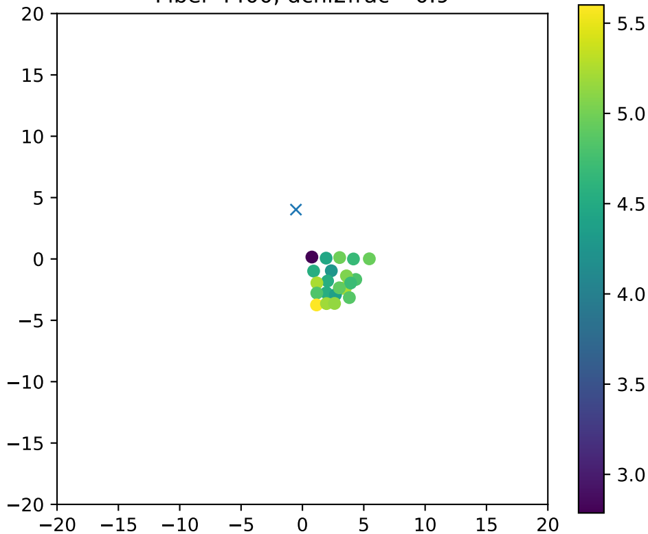
Fiber 4400, dchi2frac= 0.9
