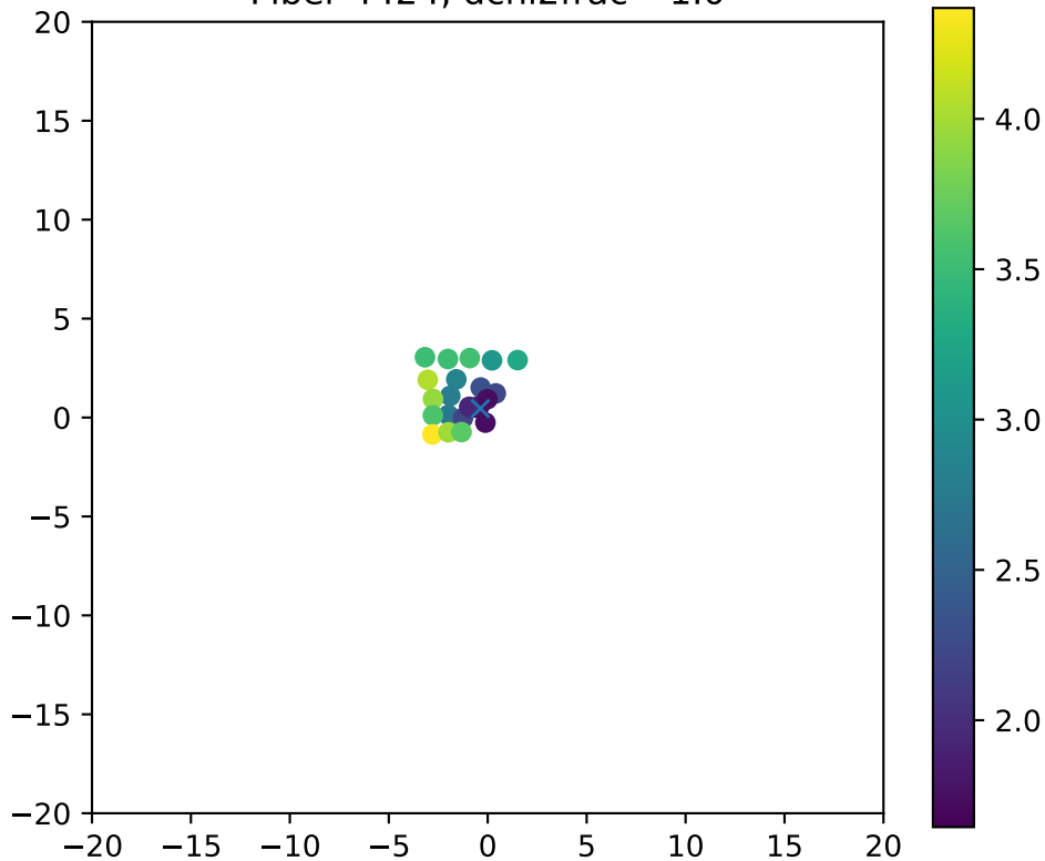
Fiber 4424, dchi2frac= 1.0
