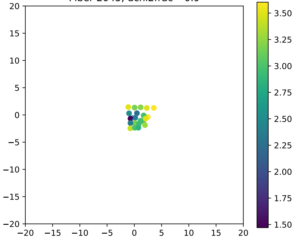
Fiber 2045, dchi2frac= 0.9
