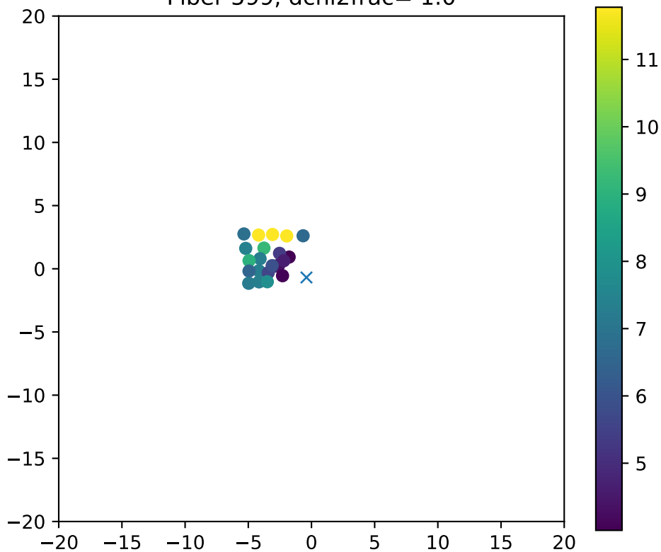
Fiber 599, dchi2frac= 1.0
