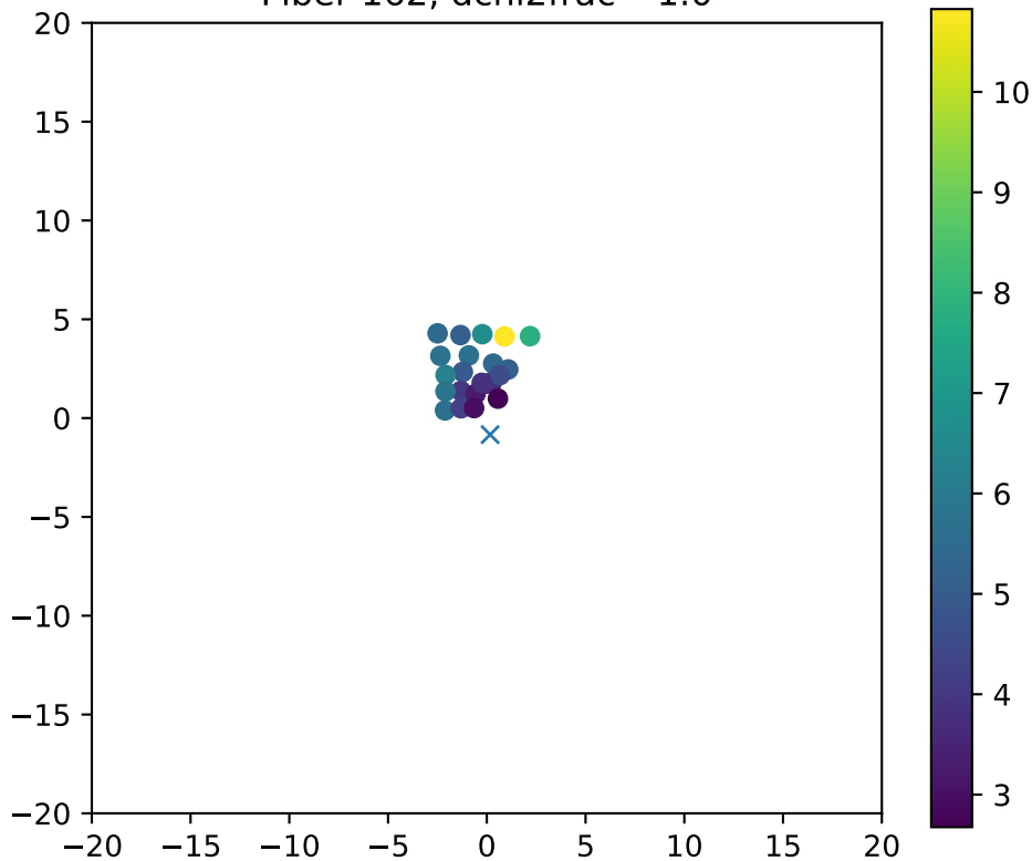
Fiber 162, dchi2frac= 1.0
