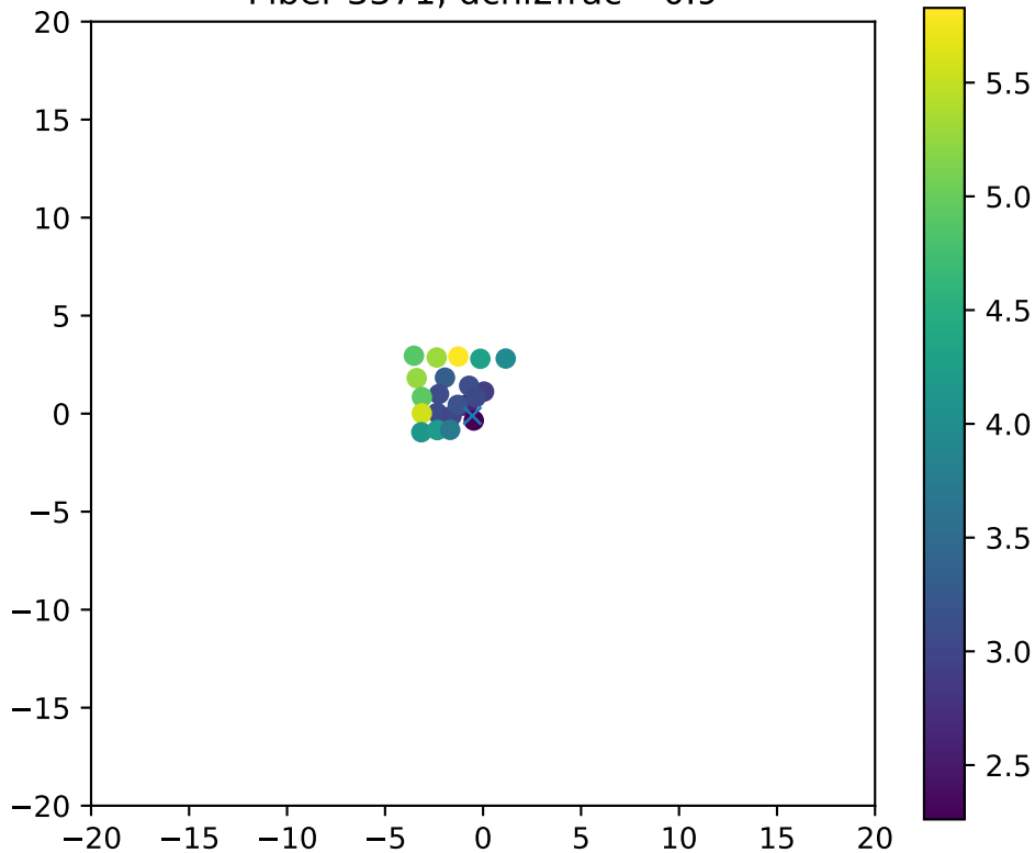
Fiber 3371, dchi2frac= 0.9
