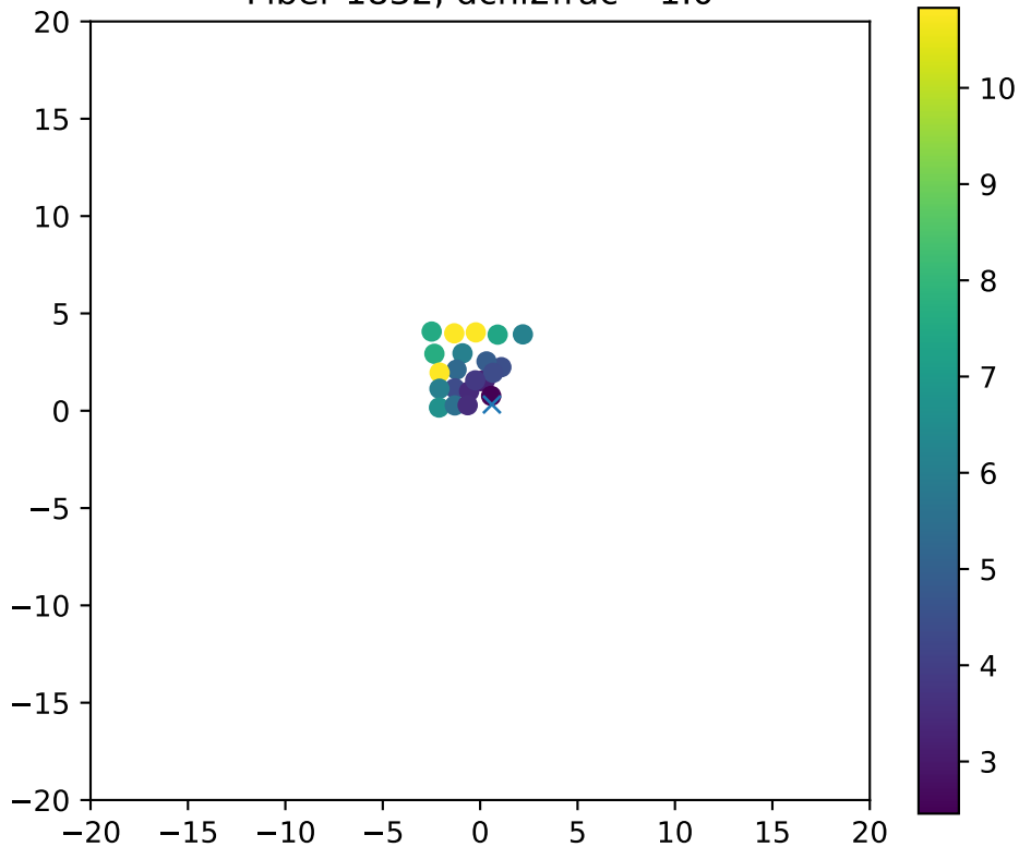
Fiber 1832, dchi2frac= 1.0
