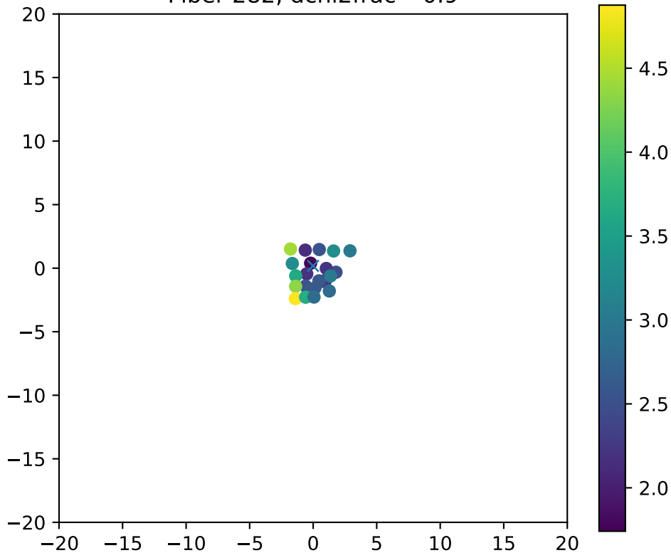
Fiber 282, dchi2frac= 0.9
