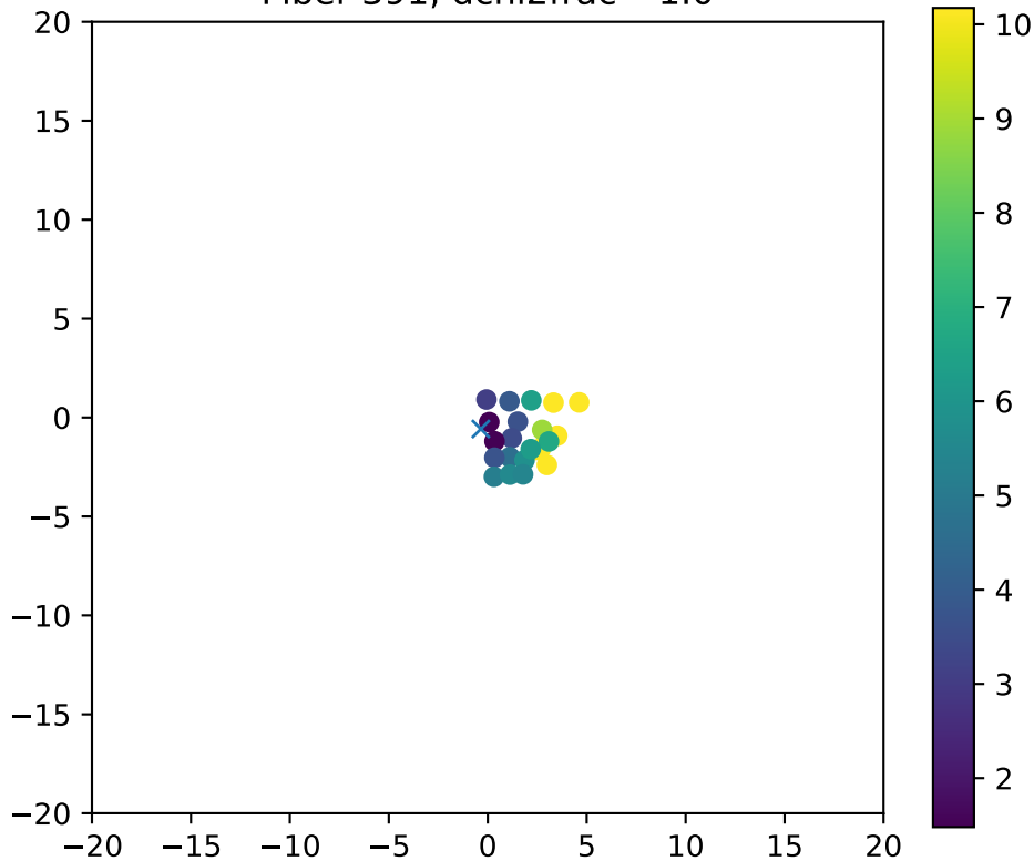
Fiber 391, dchi2frac= 1.0
