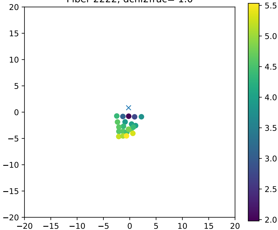
Fiber 2222, dchi2frac= 1.0
