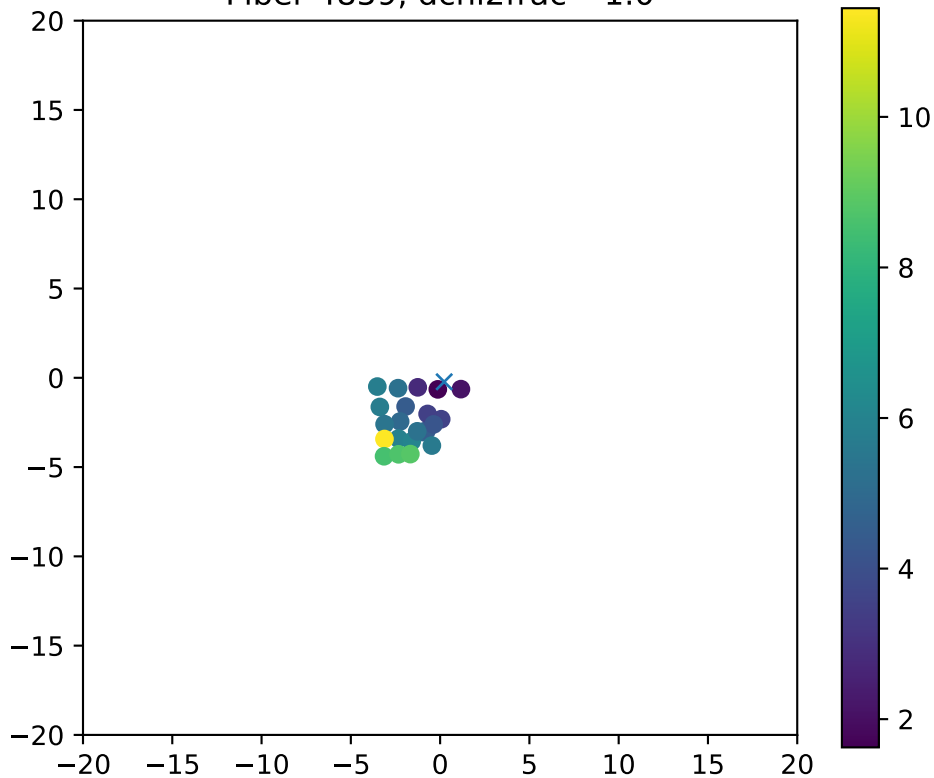
Fiber 4859, dchi2frac= 1.0
