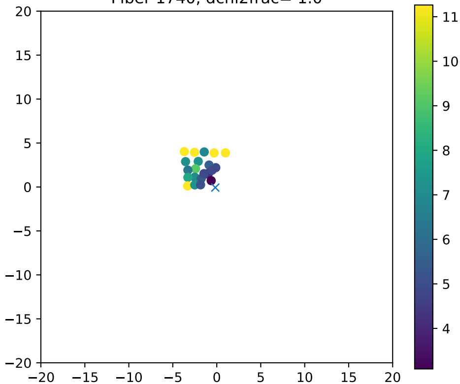
Fiber 1740, dchi2frac= 1.0
