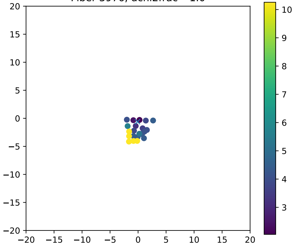
Fiber 3976, dchi2frac= 1.0
