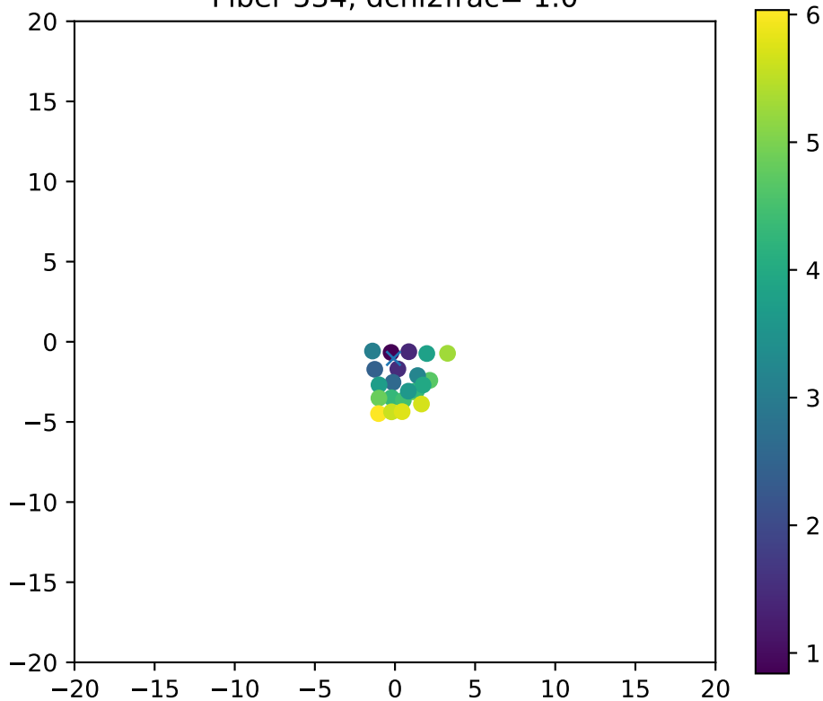
Fiber 534, dchi2frac= 1.0
