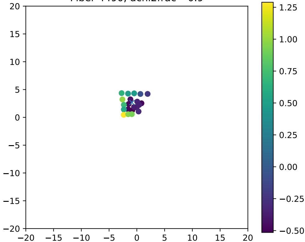
Fiber 4490, dchi2frac= 0.9
