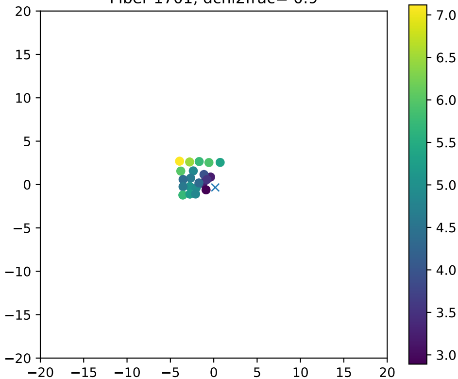
Fiber 1701, dchi2frac= 0.9
