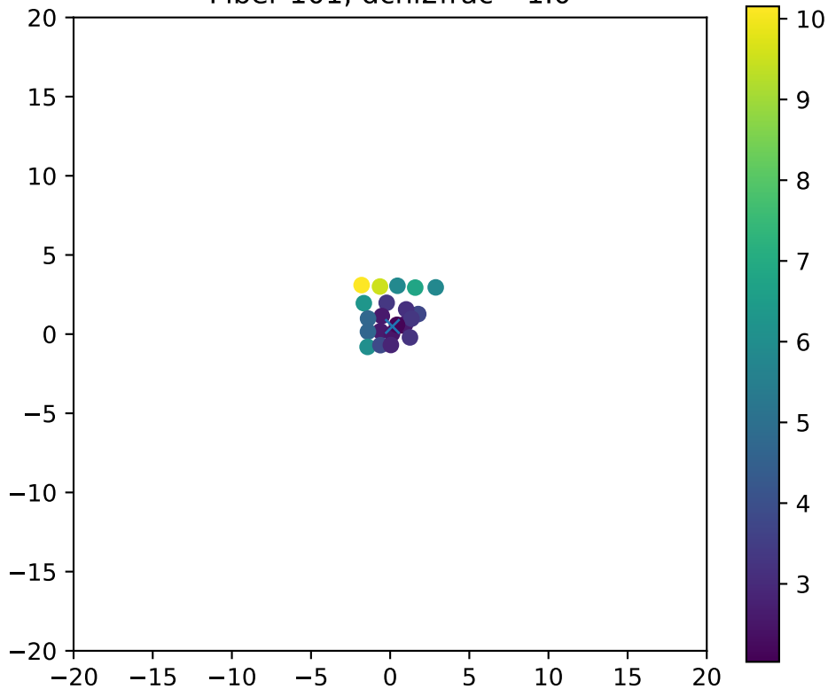
Fiber 101, dchi2frac= 1.0
