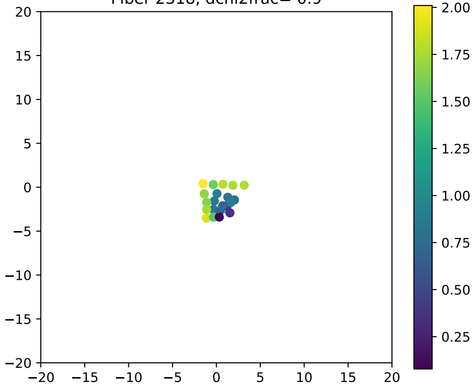
Fiber 2318, dchi2frac= 0.9
