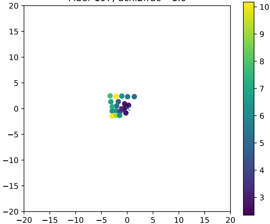
Fiber 197, dchi2frac= 1.0
