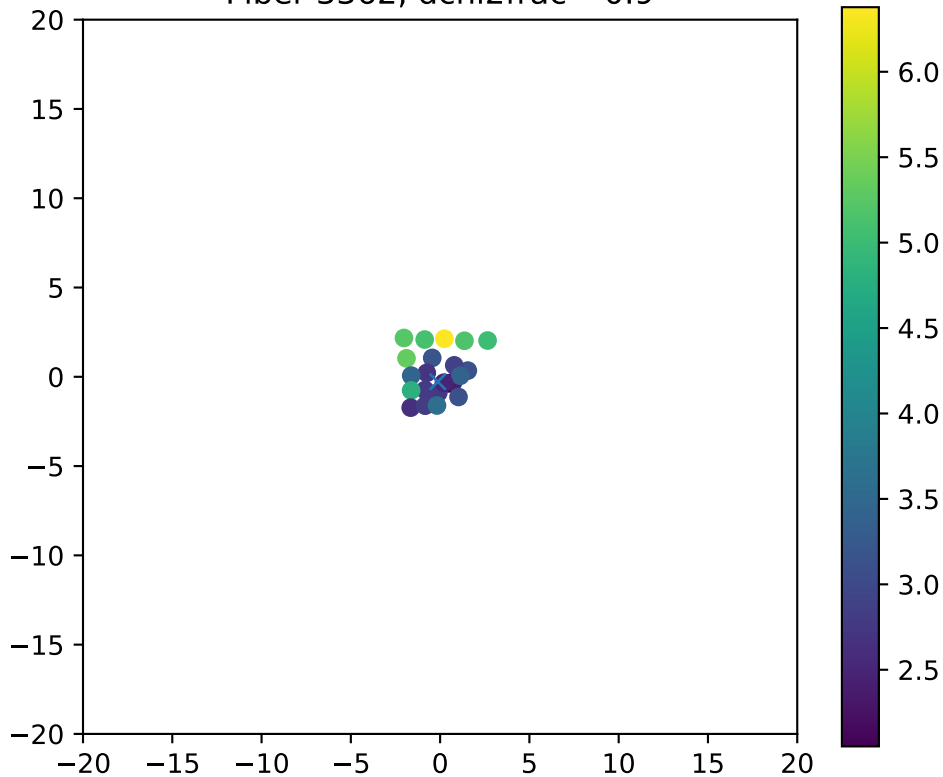
Fiber 3362, dchi2frac= 0.9
