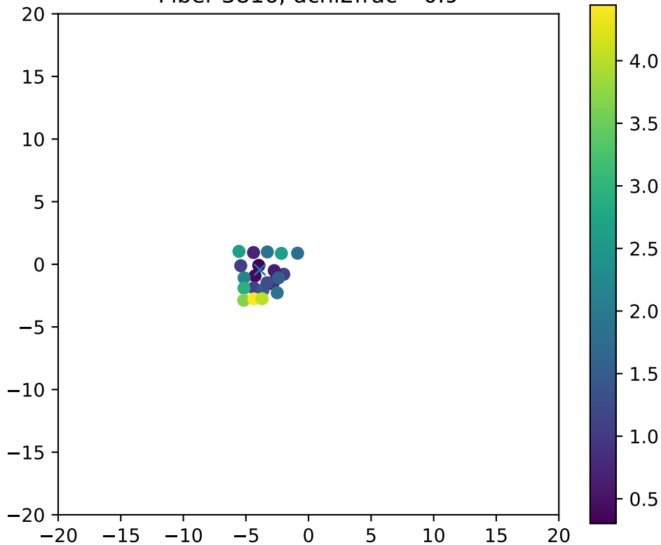
Fiber 3816, dchi2frac= 0.9
