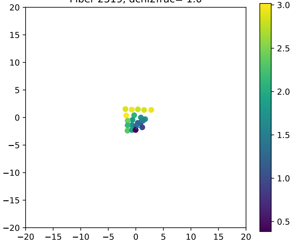
Fiber 2319, dchi2frac= 1.0
