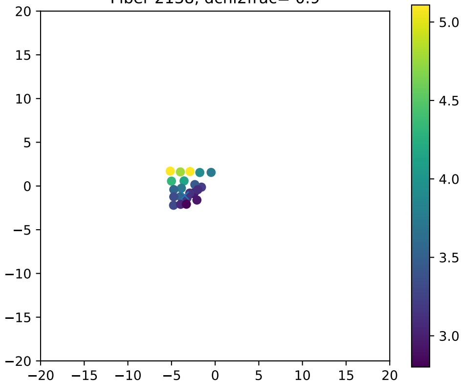
Fiber 2138, dchi2frac= 0.9
