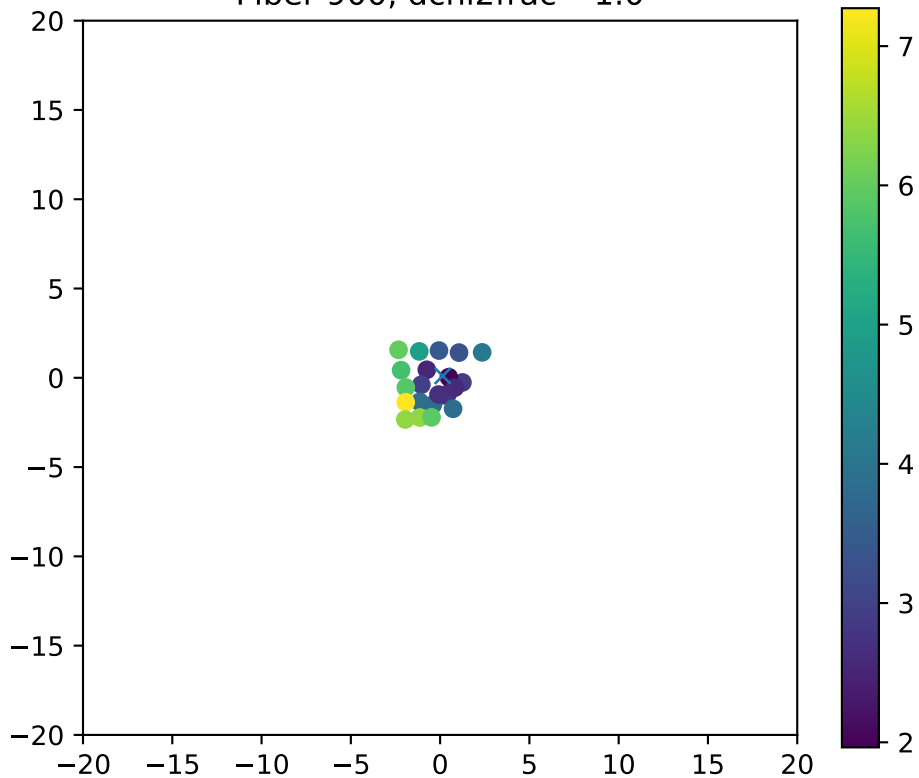
Fiber 900, dchi2frac= 1.0
