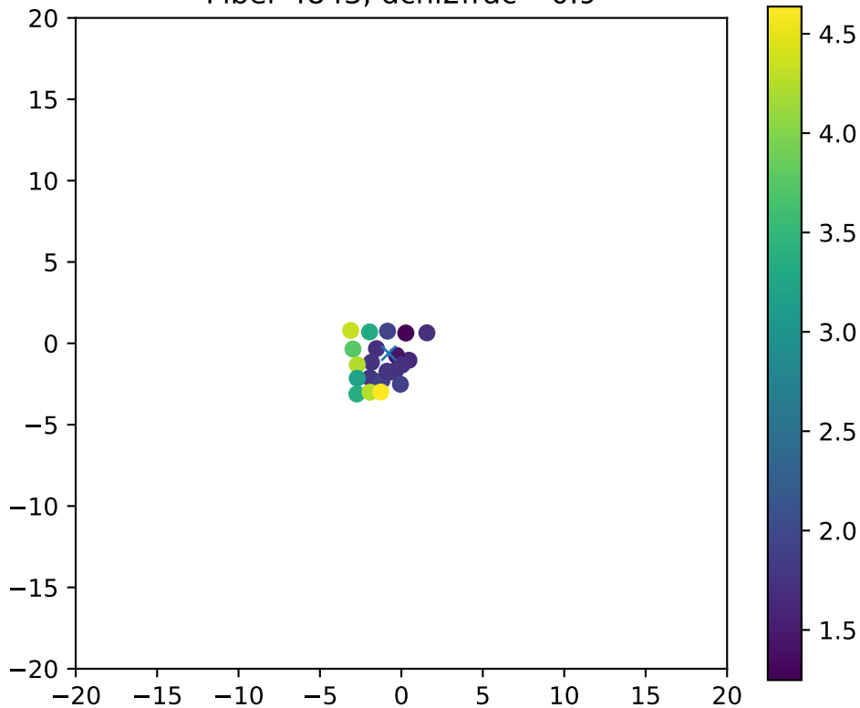
Fiber 4843, dchi2frac= 0.9
