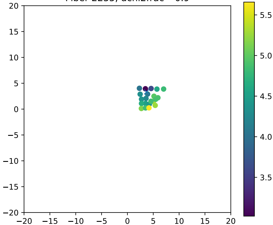
Fiber 2235, dchi2frac= 0.9
