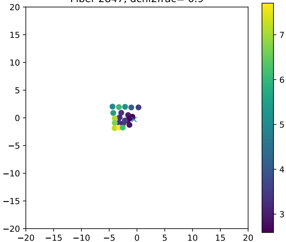
Fiber 2847, dchi2frac= 0.9
