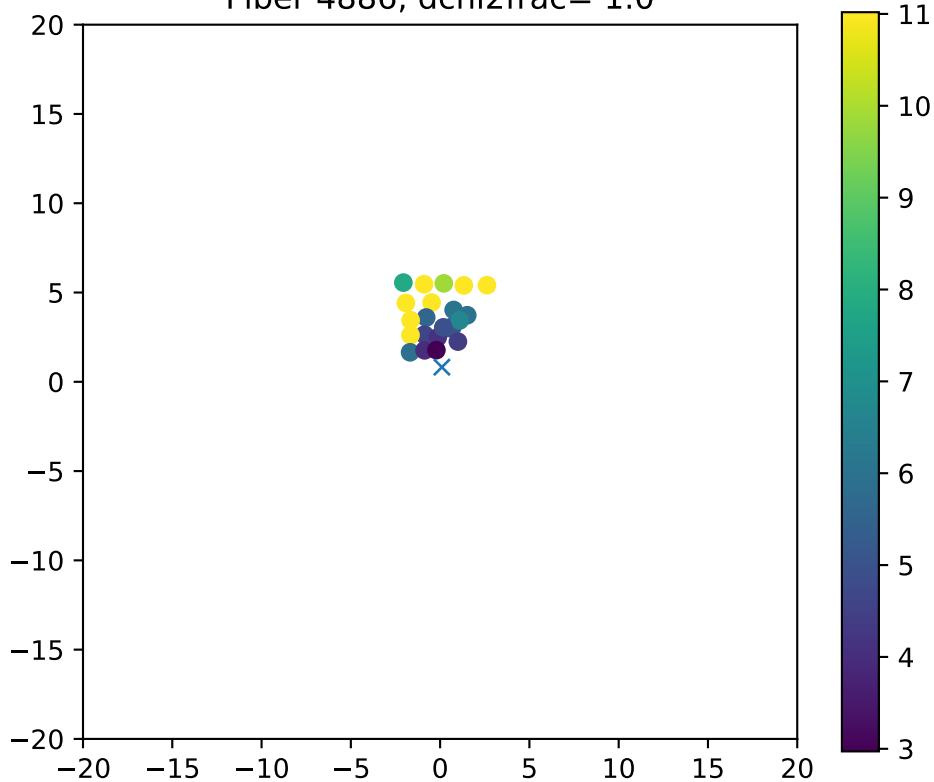
Fiber 4886, dchi2frac= 1.0
