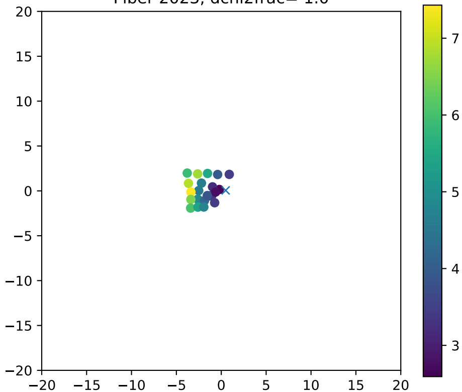
Fiber 2023, dchi2frac= 1.0
