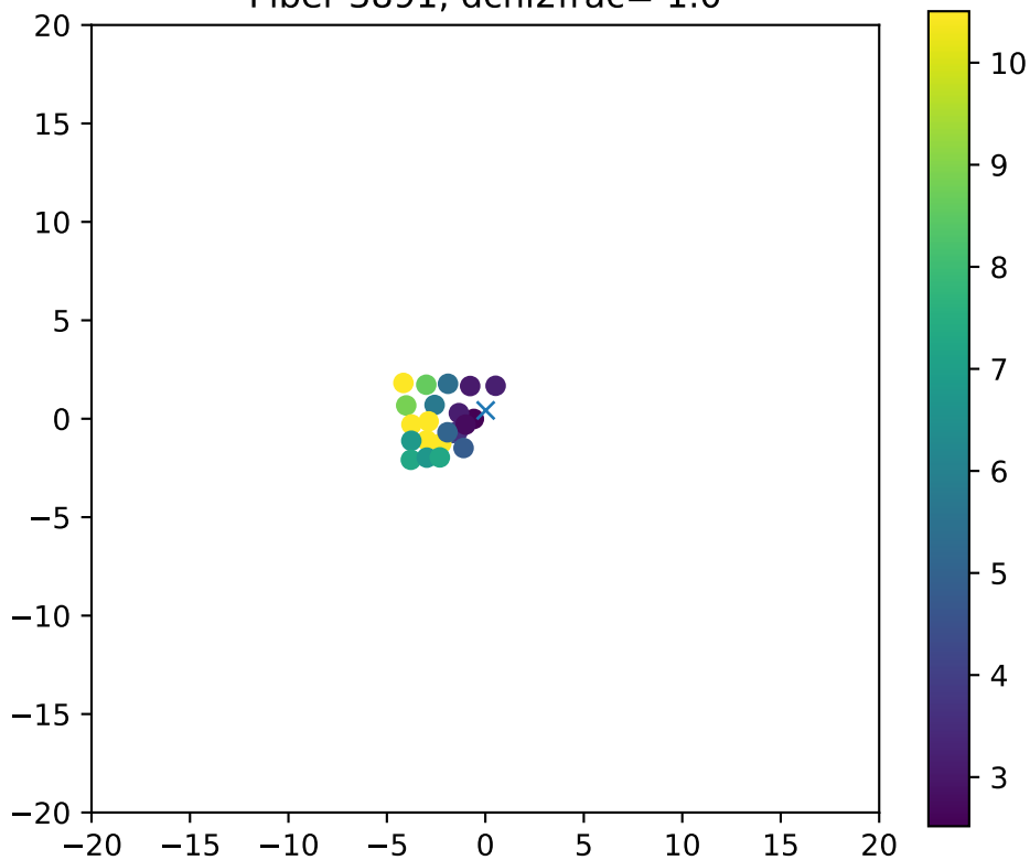
Fiber 3891, dchi2frac= 1.0
