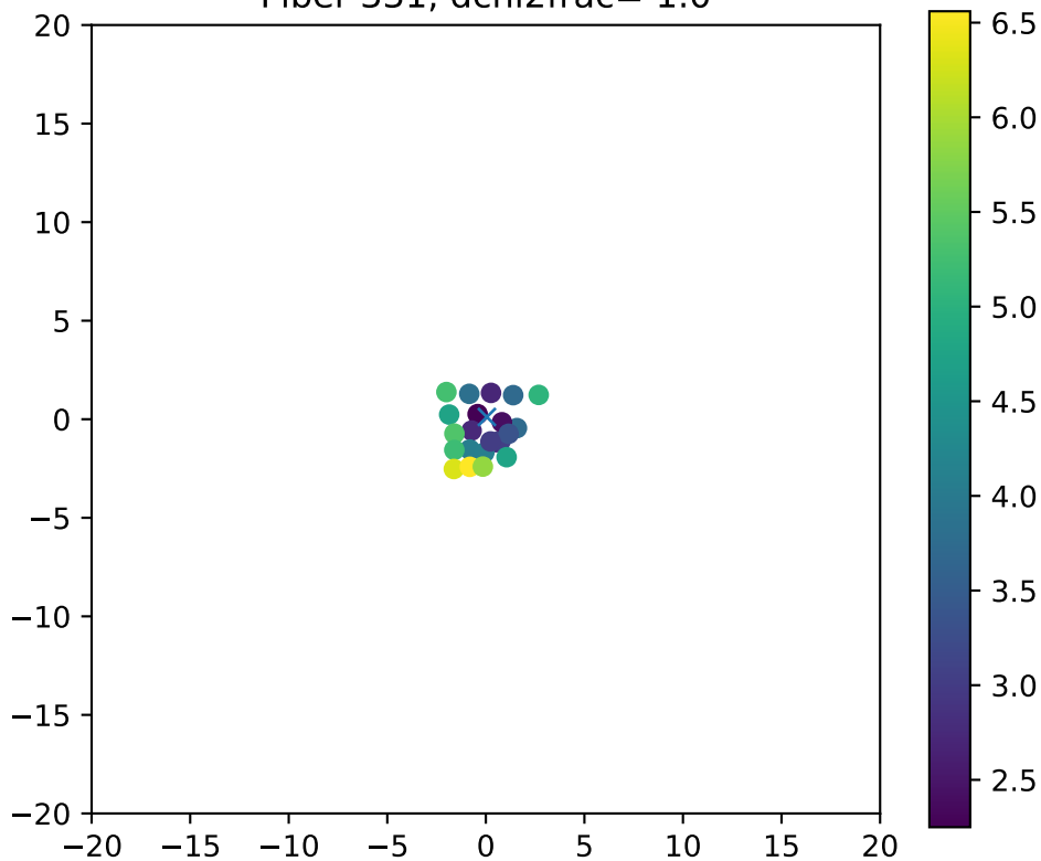
Fiber 331, dchi2frac= 1.0
