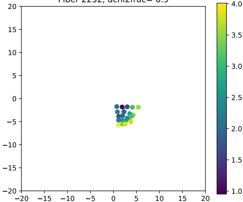
Fiber 2252, dchi2frac= 0.9
