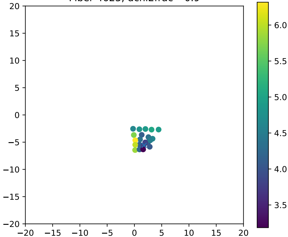
Fiber 4623, dchi2frac= 0.9
