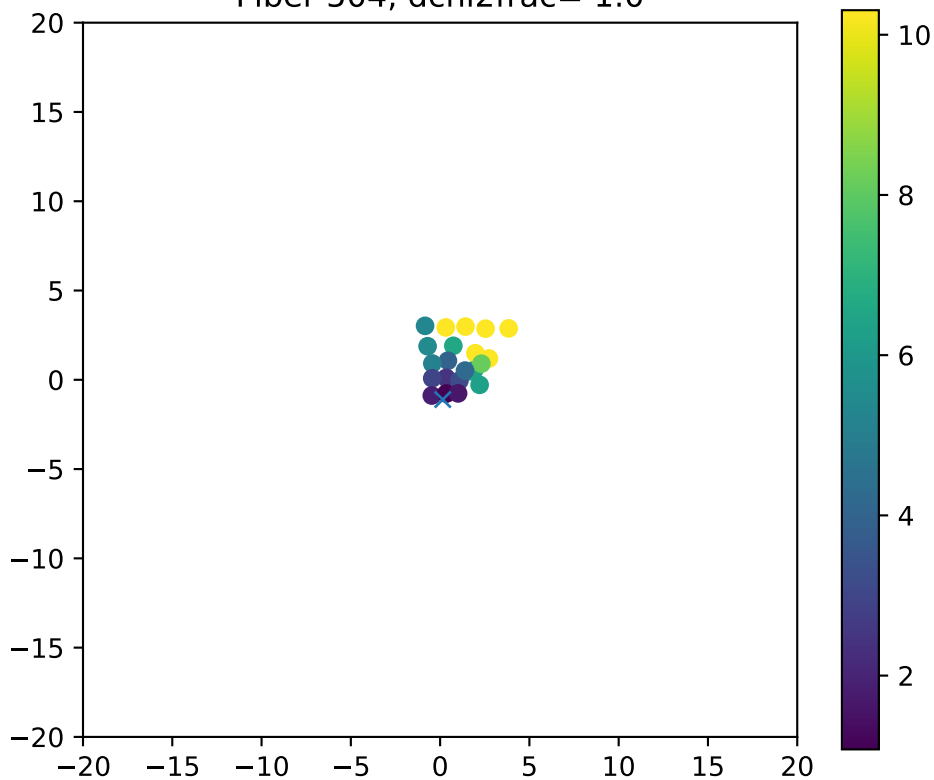
Fiber 504, dchi2frac= 1.0
