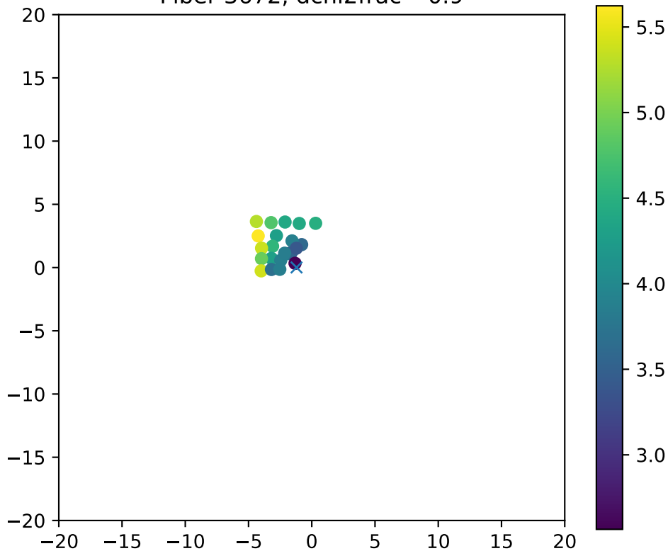
Fiber 3672, dchi2frac= 0.9
