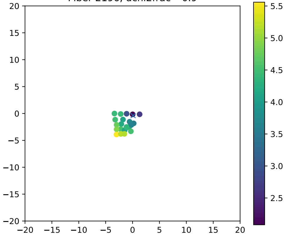
Fiber 2196, dchi2frac= 0.9
