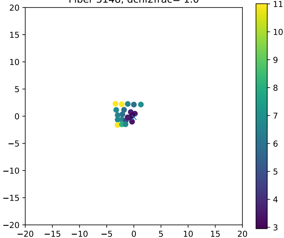
Fiber 3148, dchi2frac= 1.0
