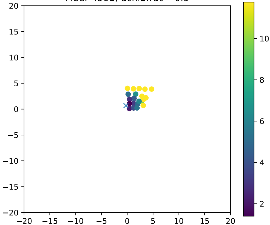
Fiber 4901, dchi2frac= 0.9
