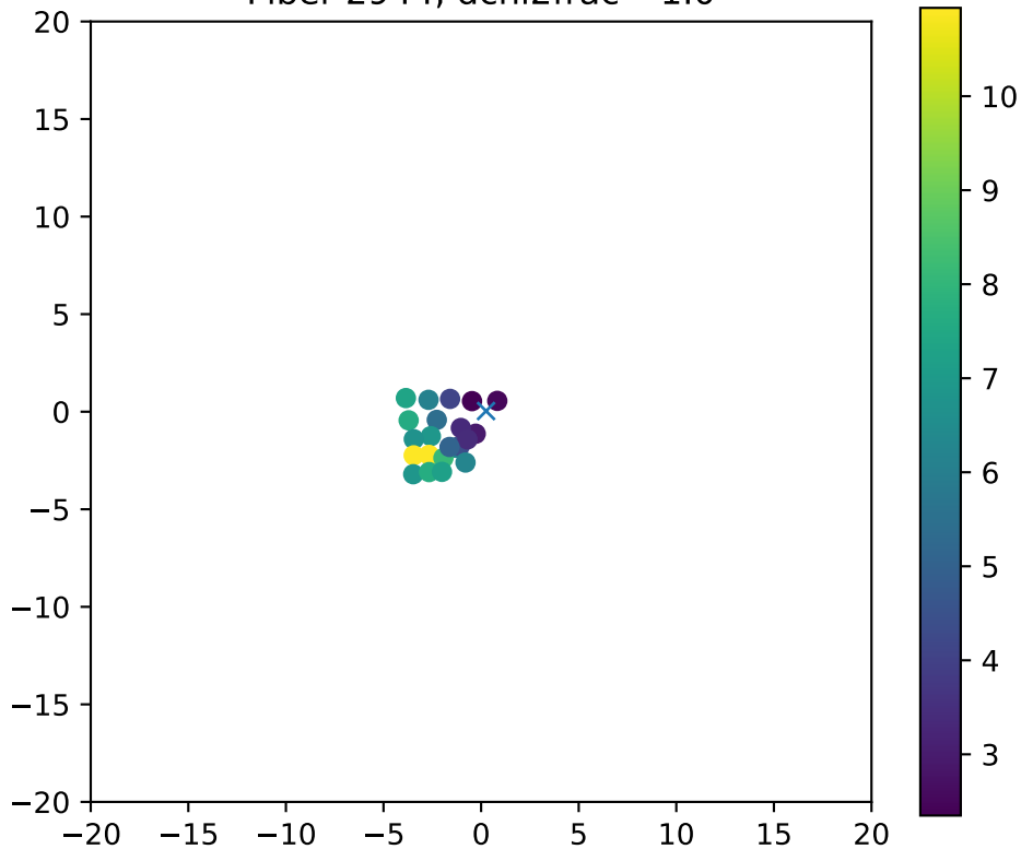
Fiber 2944, dchi2frac= 1.0
