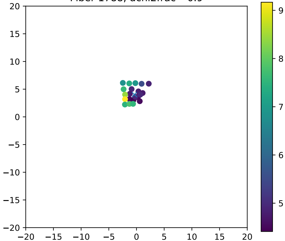
Fiber 1788, dchi2frac= 0.9
