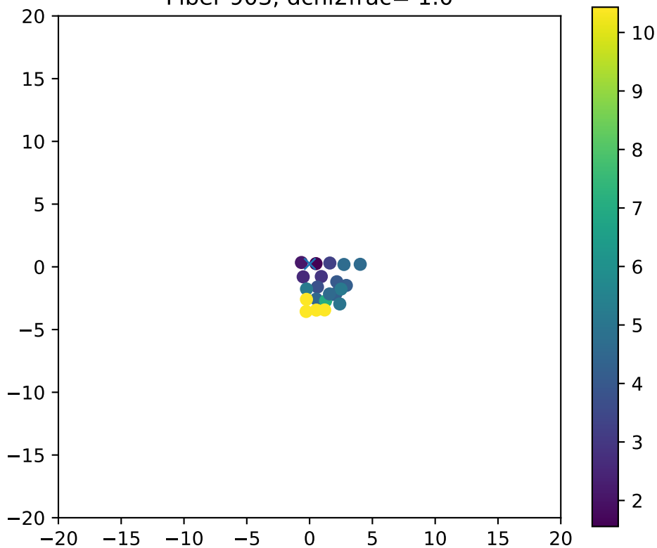
Fiber 903, dchi2frac= 1.0
