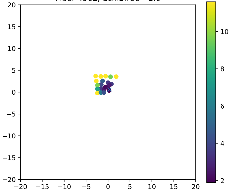
Fiber 4962, dchi2frac= 1.0
