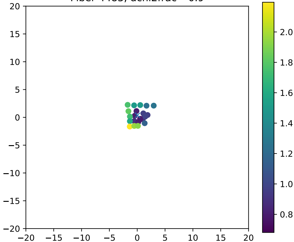
Fiber 4483, dchi2frac= 0.9
