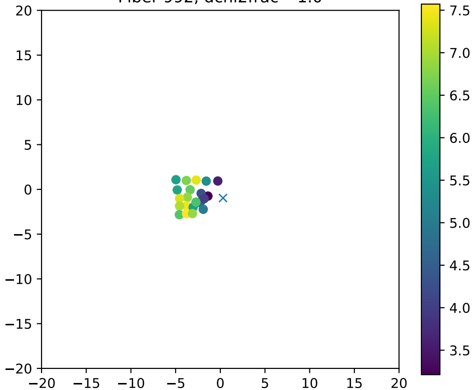
Fiber 992, dchi2frac= 1.0
