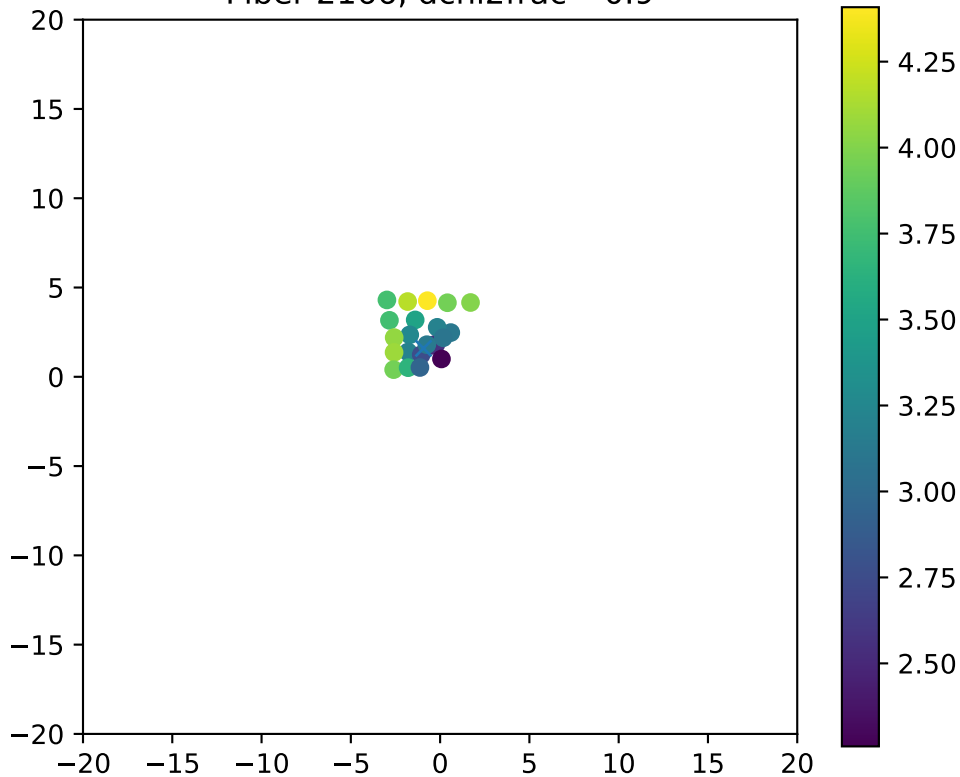
Fiber 2166, dchi2frac= 0.9
