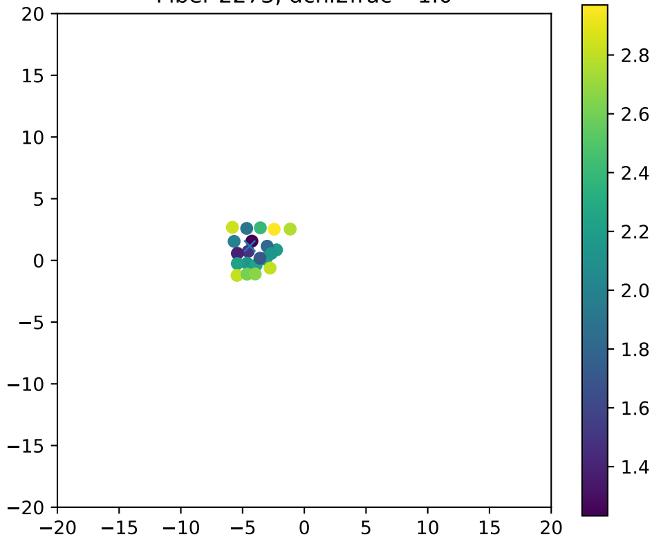
Fiber 2273, dchi2frac= 1.0
