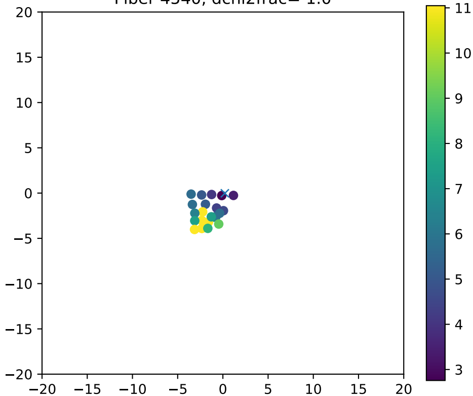
Fiber 4540, dchi2frac= 1.0
