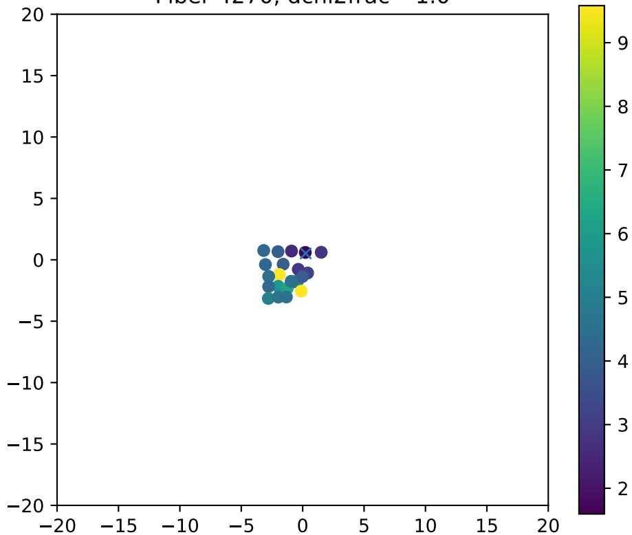
Fiber 4270, dchi2frac= 1.0
