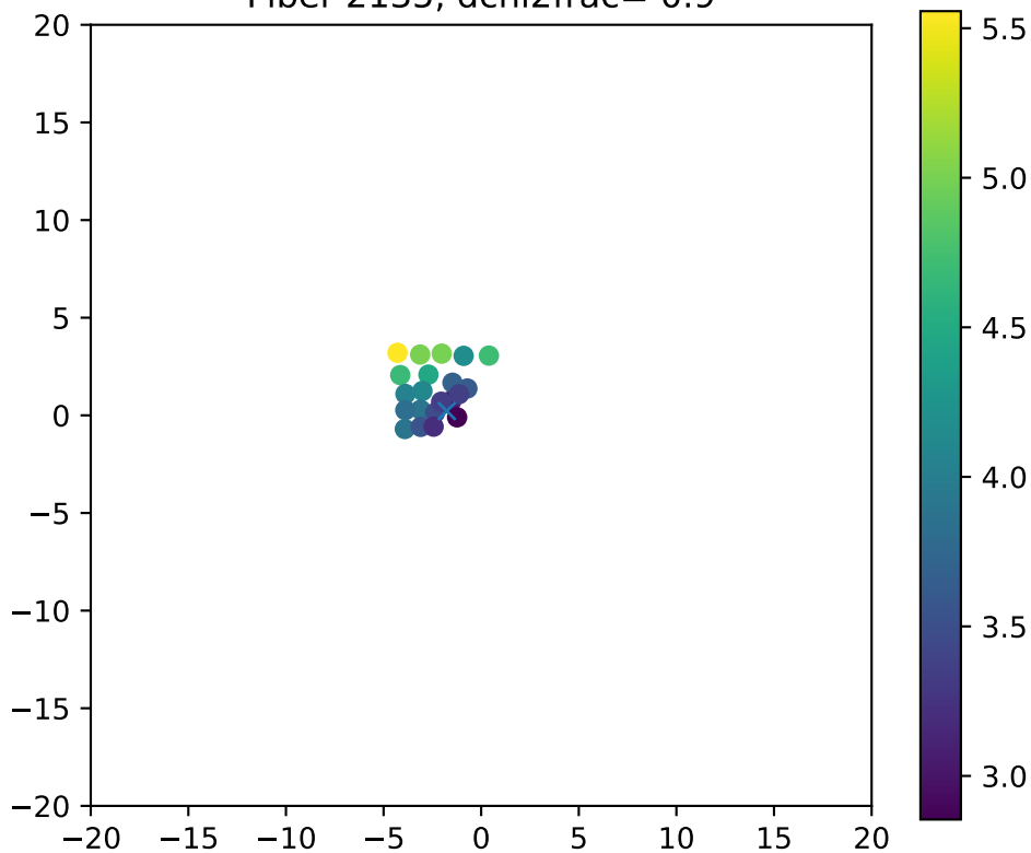
Fiber 2135, dchi2frac= 0.9
