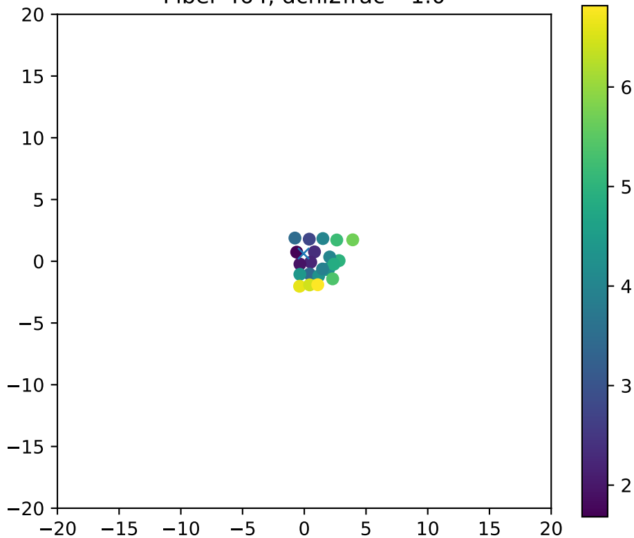
Fiber 464, dchi2frac= 1.0
