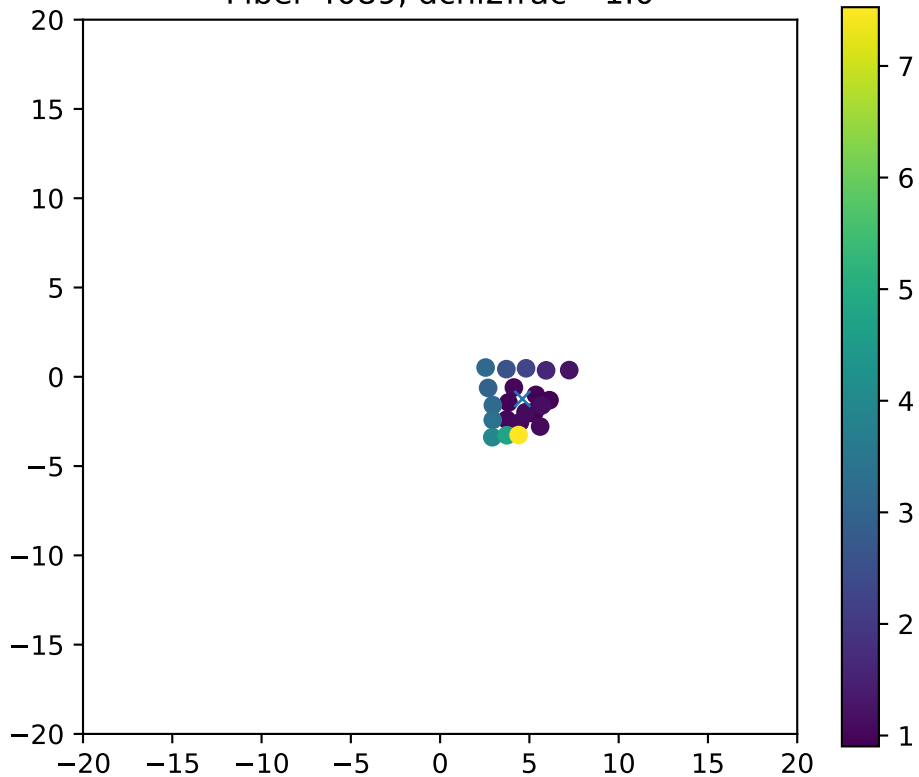
Fiber 4089, dchi2frac= 1.0
