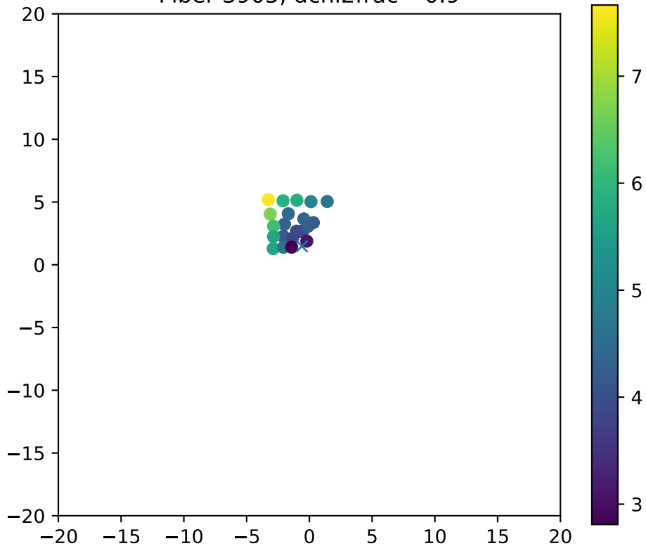
Fiber 3905, dchi2frac= 0.9
