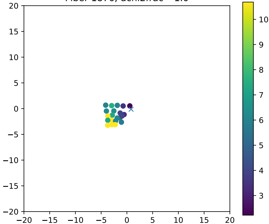
Fiber 1876, dchi2frac= 1.0
