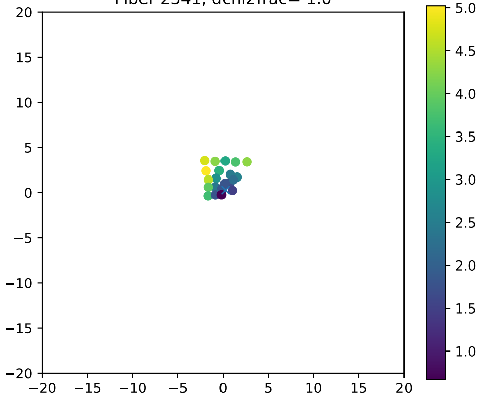
Fiber 2341, dchi2frac= 1.0
