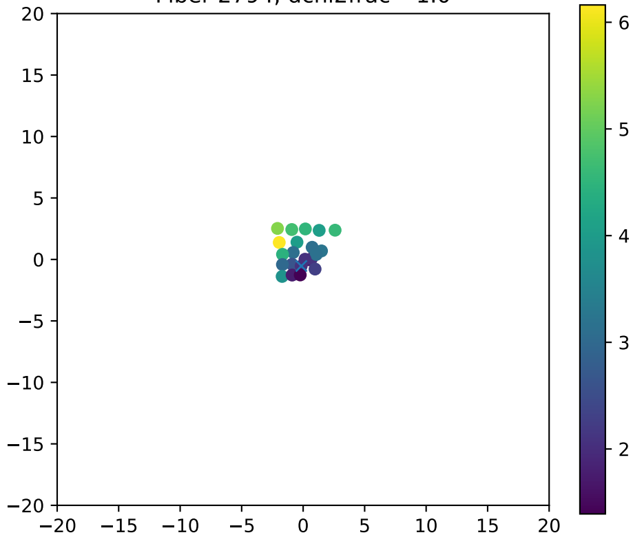
Fiber 2794, dchi2frac= 1.0
