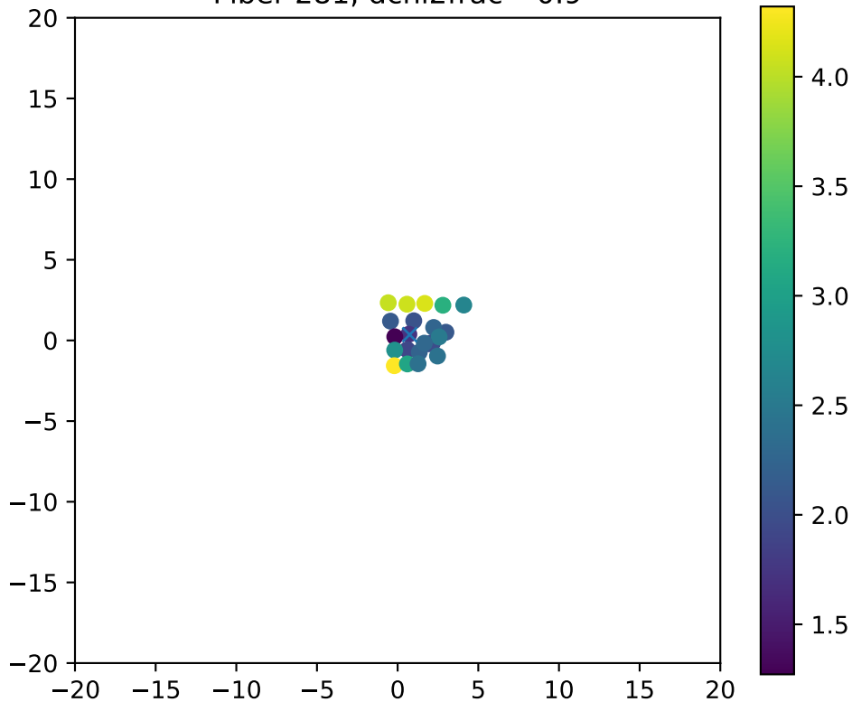
Fiber 281, dchi2frac= 0.9
