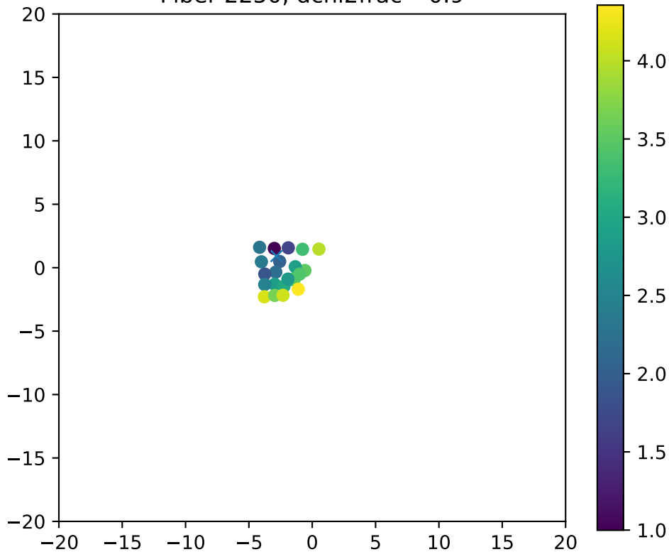
Fiber 2250, dchi2frac= 0.9
