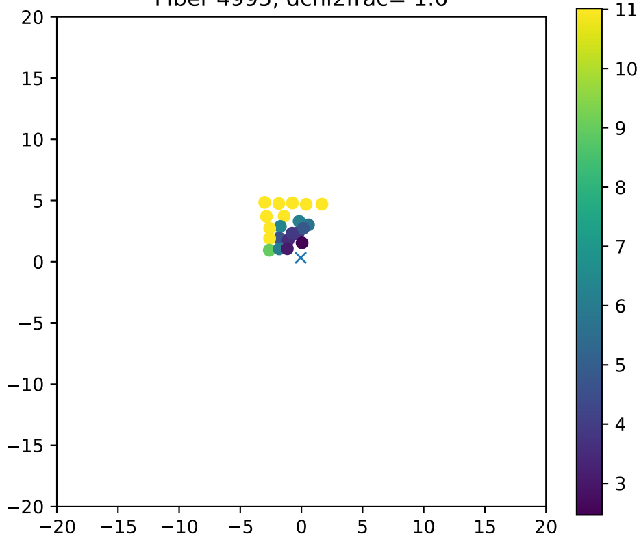
Fiber 4995, dchi2frac= 1.0
