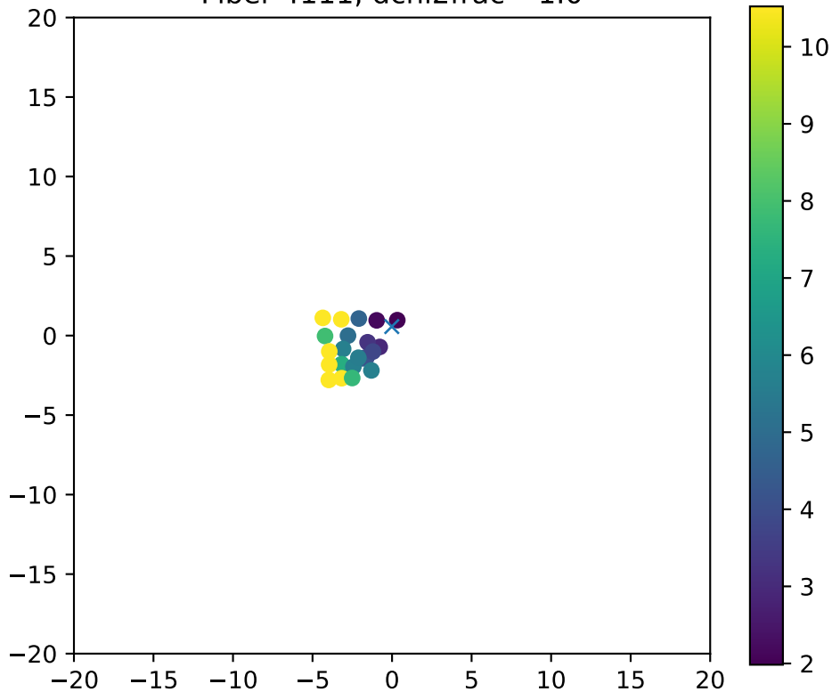
Fiber 4111, dchi2frac= 1.0
