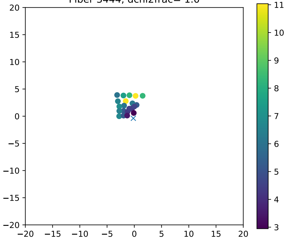
Fiber 3444, dchi2frac= 1.0
