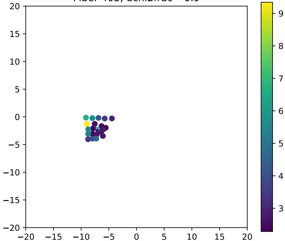
Fiber 405, dchi2frac= 0.9
