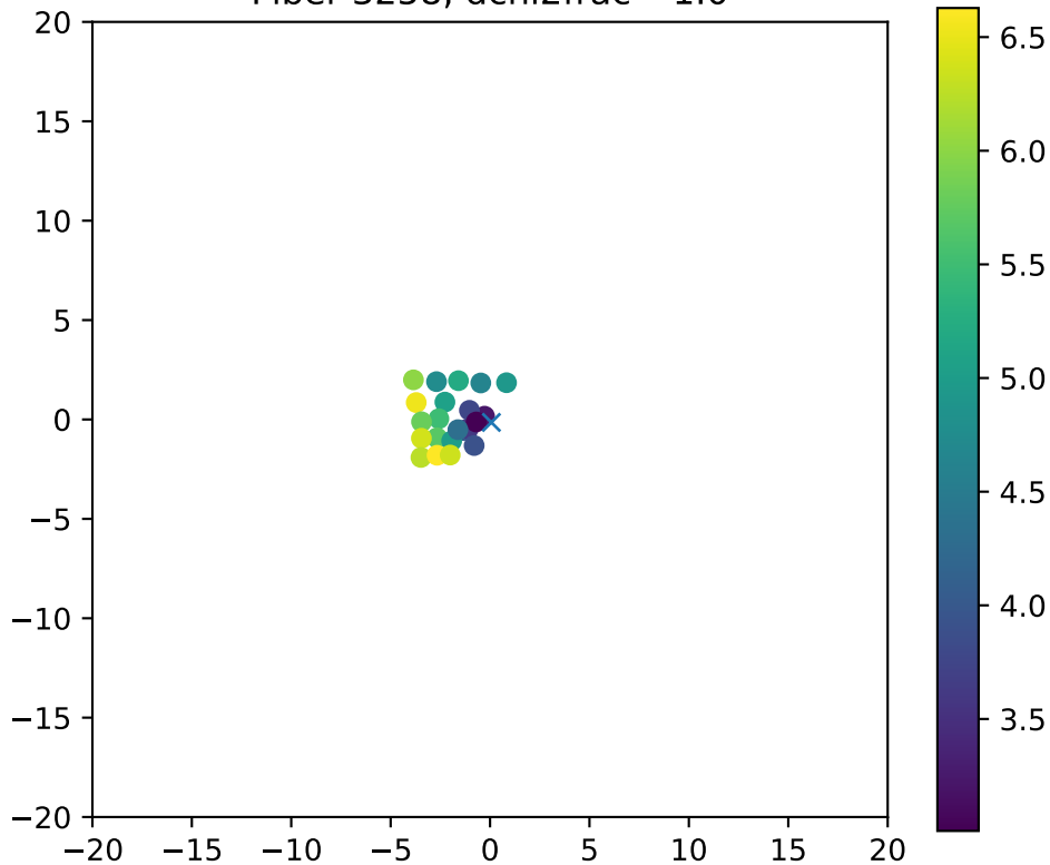
Fiber 3258, dchi2frac= 1.0
