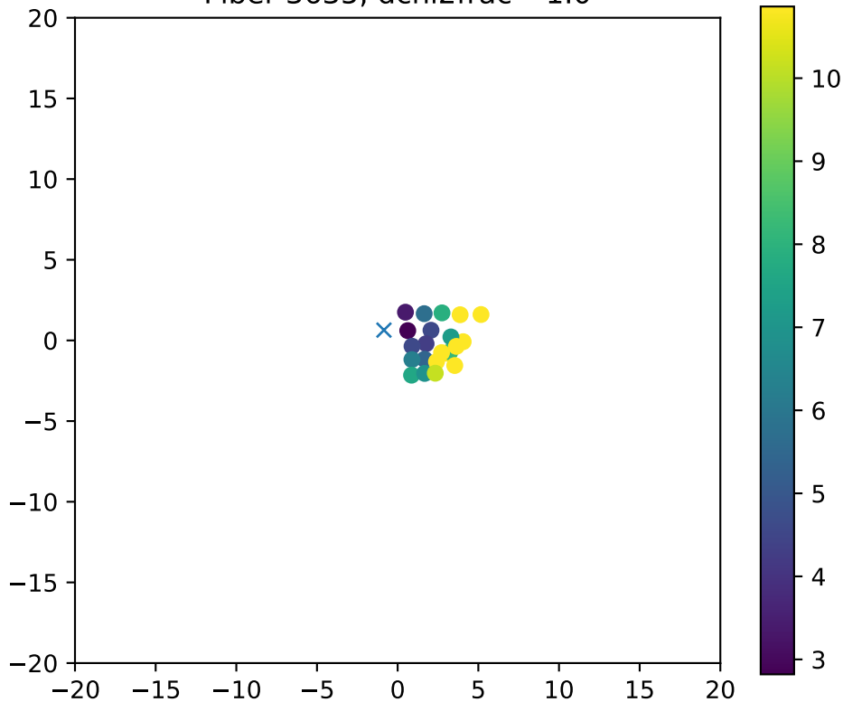
Fiber 3635, dchi2frac= 1.0
