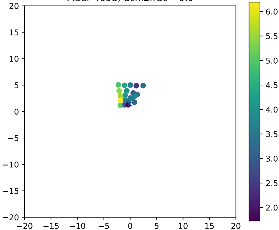
Fiber 4698, dchi2frac= 0.9
