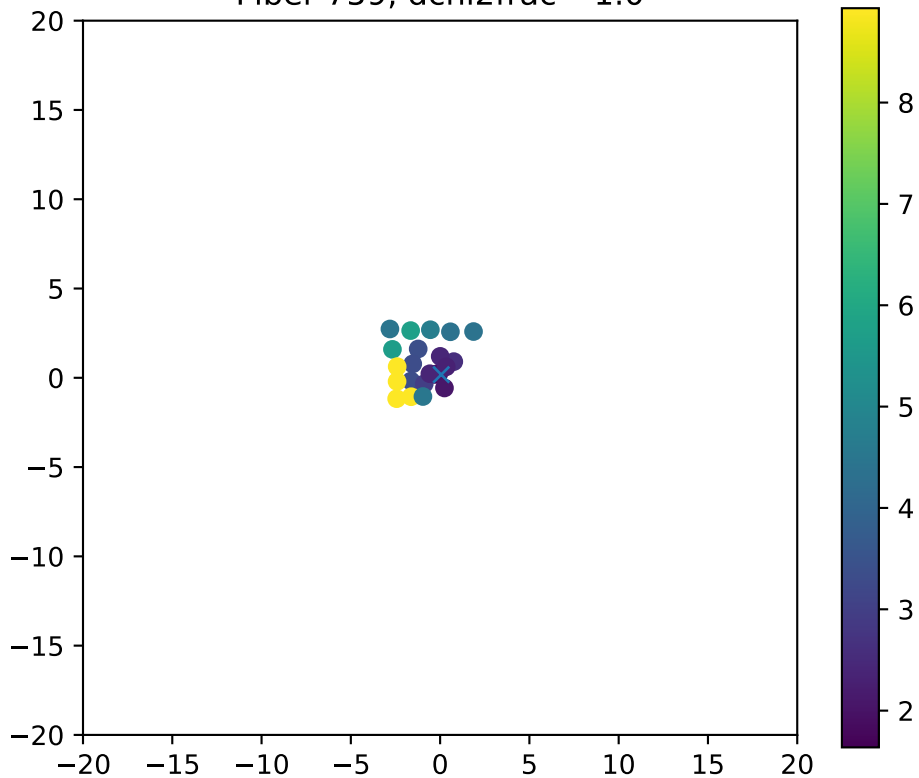
Fiber 759, dchi2frac= 1.0
