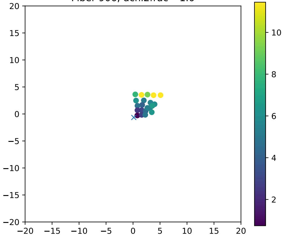
Fiber 906, dchi2frac= 1.0
