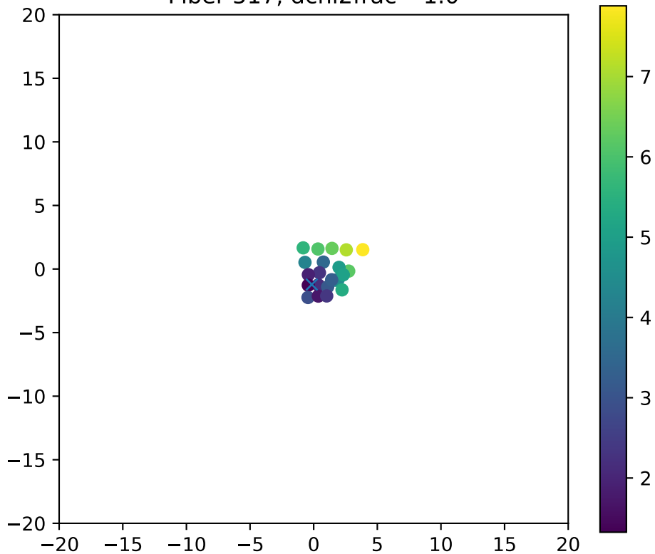
Fiber 517, dchi2frac= 1.0
