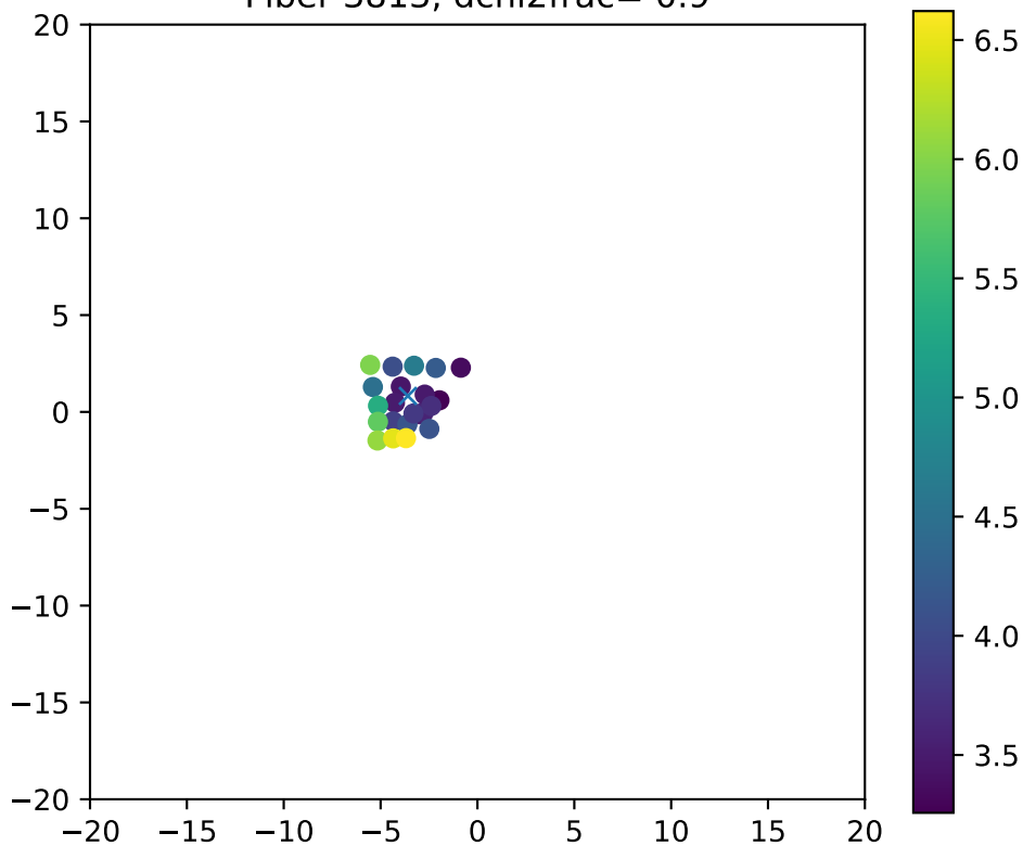
Fiber 3813, dchi2frac= 0.9
