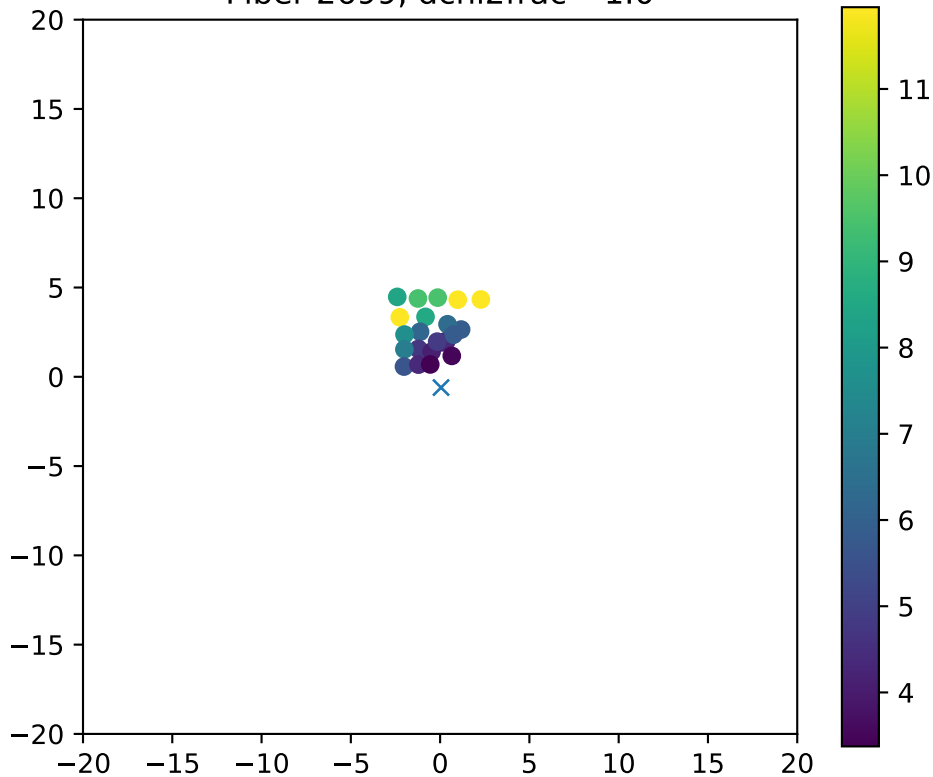
Fiber 2699, dchi2frac= 1.0
