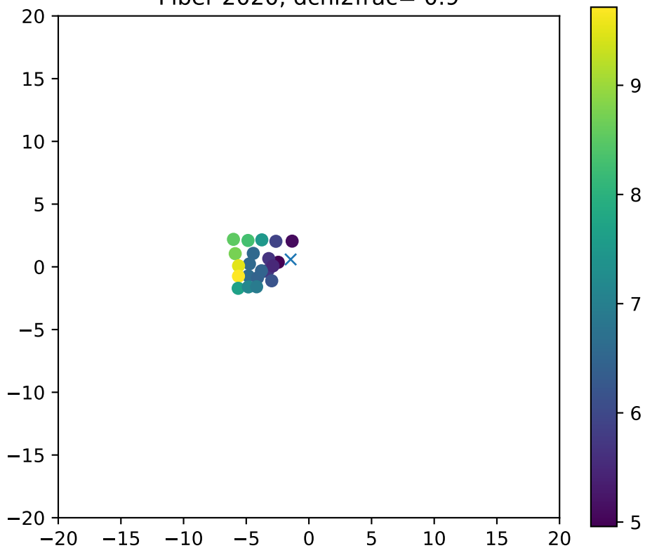
Fiber 2020, dchi2frac= 0.9
