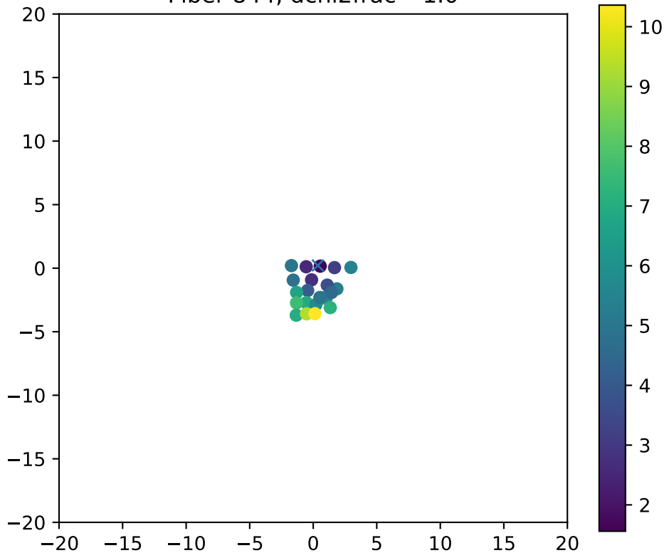
Fiber 844, dchi2frac= 1.0
