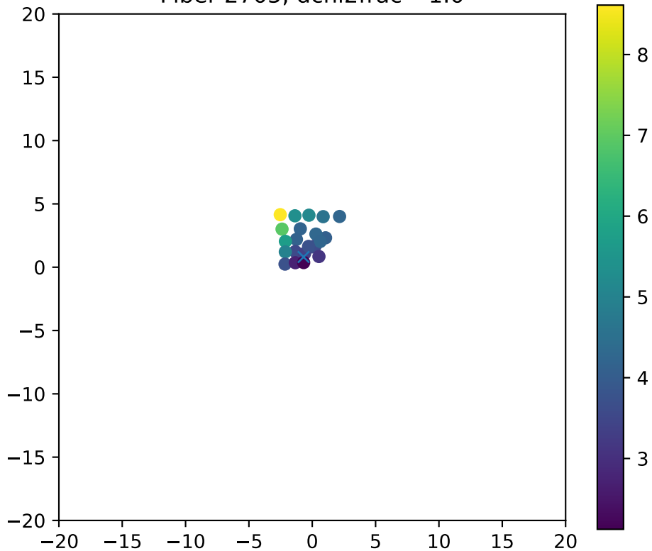
Fiber 2705, dchi2frac= 1.0
