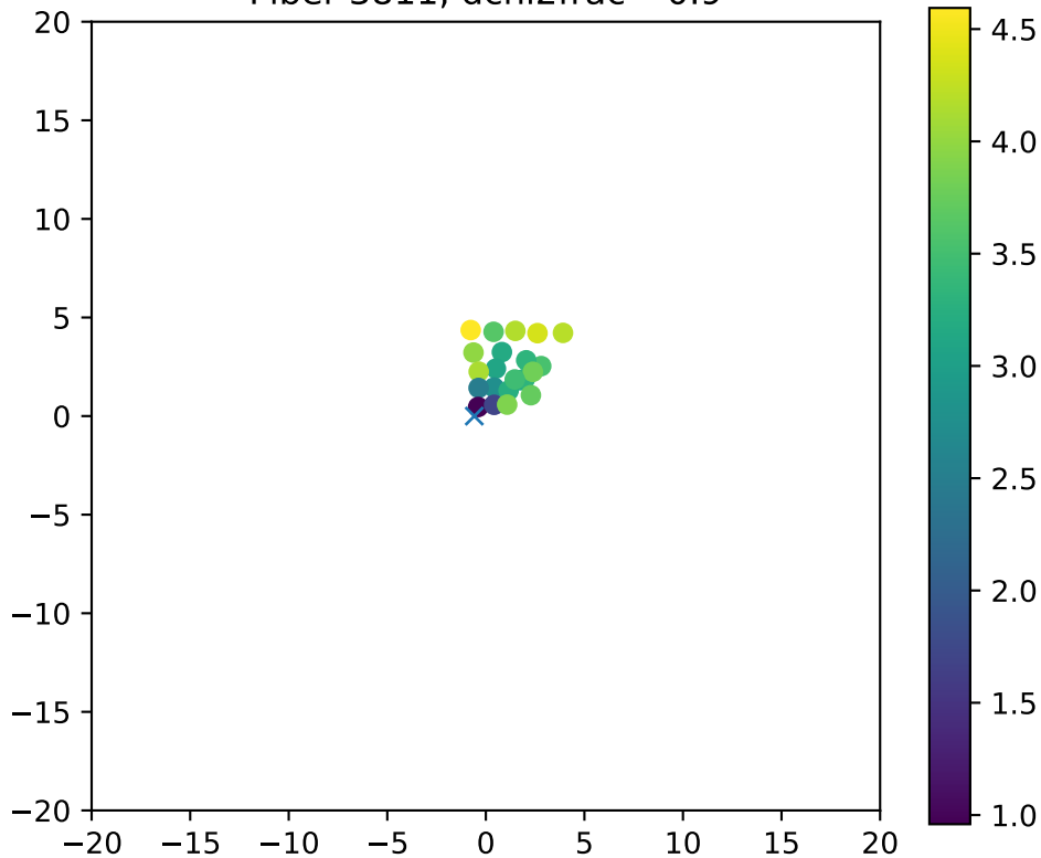
Fiber 3811, dchi2frac= 0.9
