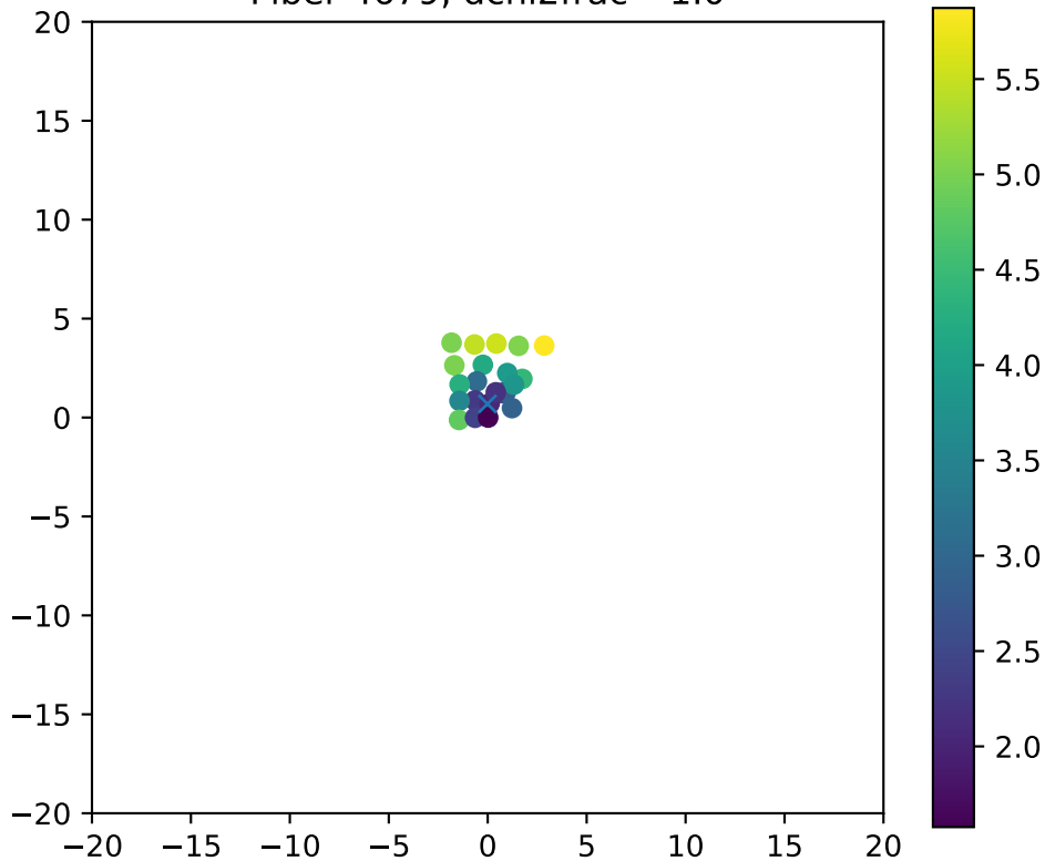
Fiber 4679, dchi2frac= 1.0
