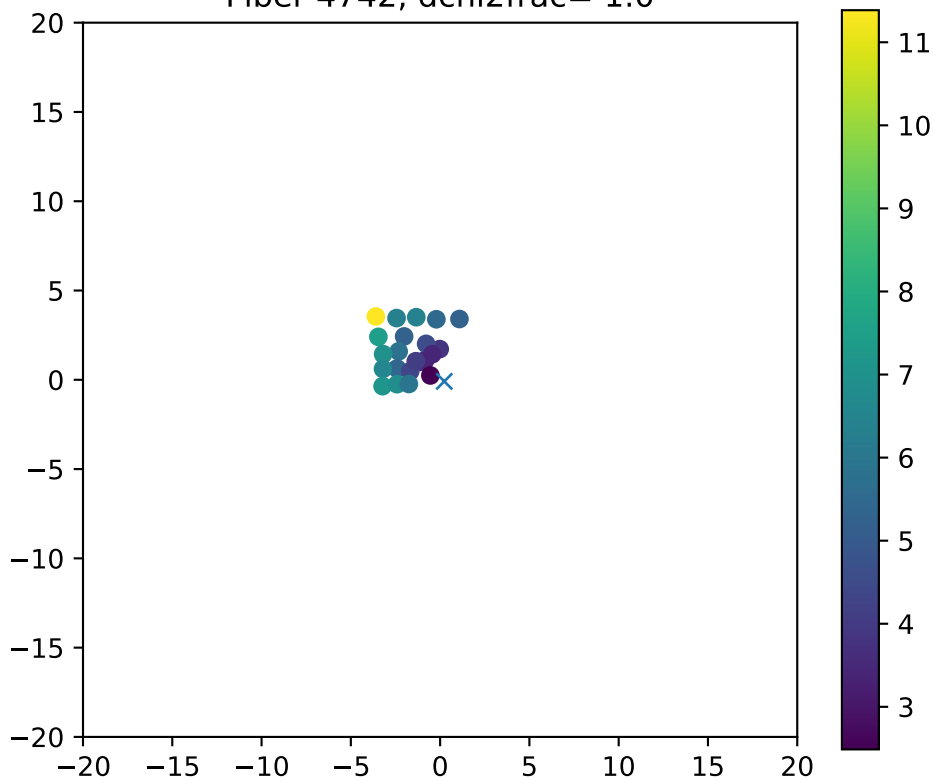
Fiber 4742, dchi2frac= 1.0
