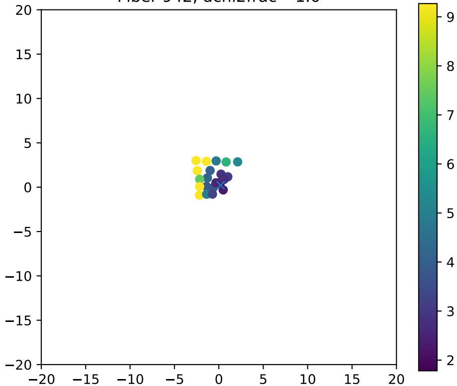
Fiber 942, dchi2frac= 1.0
