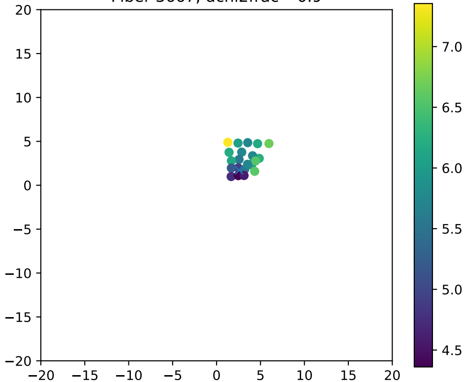
Fiber 3667, dchi2frac= 0.9
