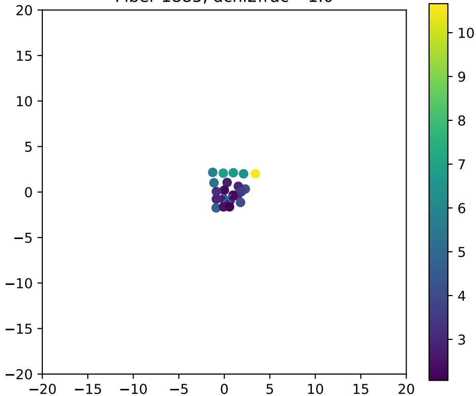
Fiber 1885, dchi2frac= 1.0
