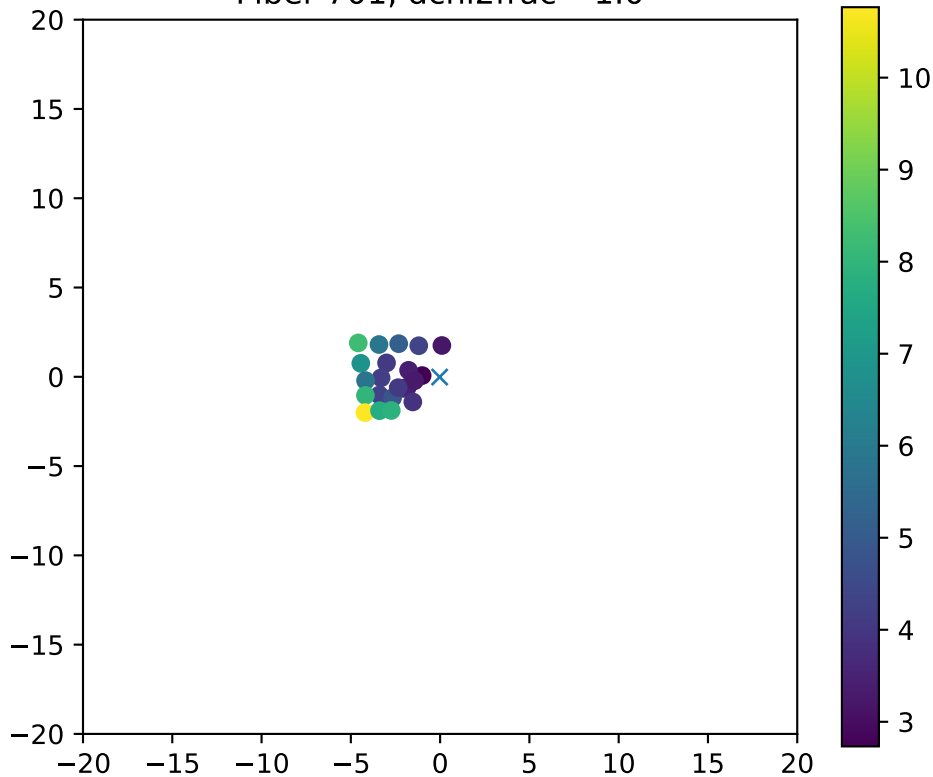
Fiber 701, dchi2frac= 1.0
