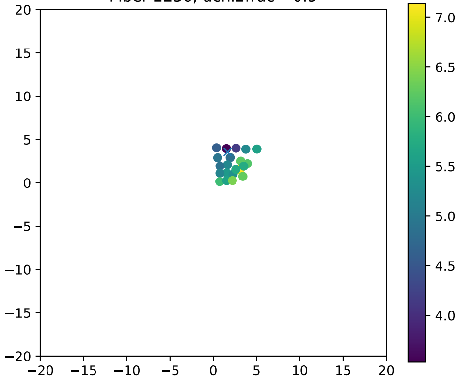
Fiber 2236, dchi2frac= 0.9
