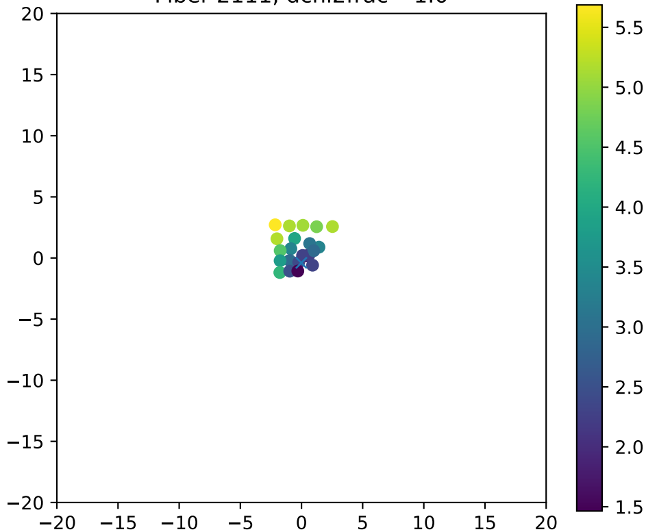
Fiber 2111, dchi2frac= 1.0
