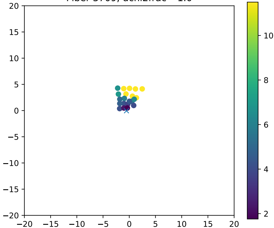
Fiber 3709, dchi2frac= 1.0
