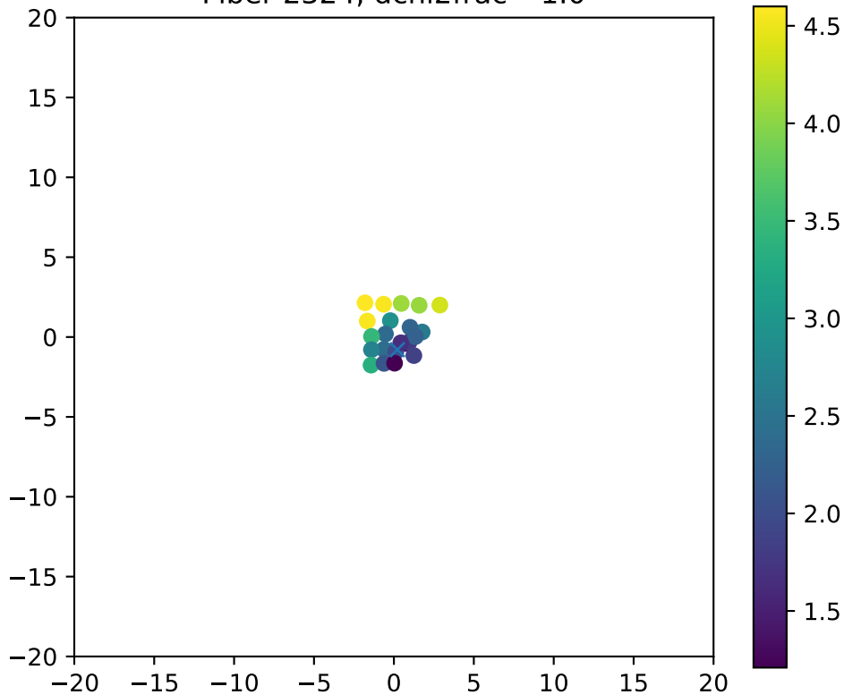
Fiber 2324, dchi2frac= 1.0
