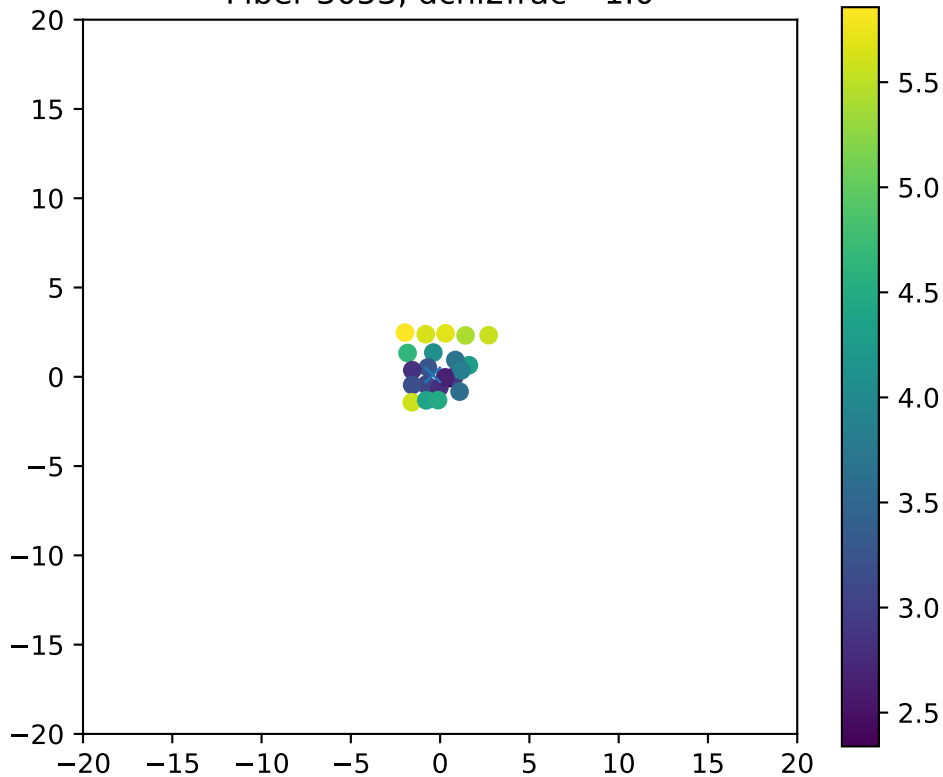
Fiber 3053, dchi2frac= 1.0
