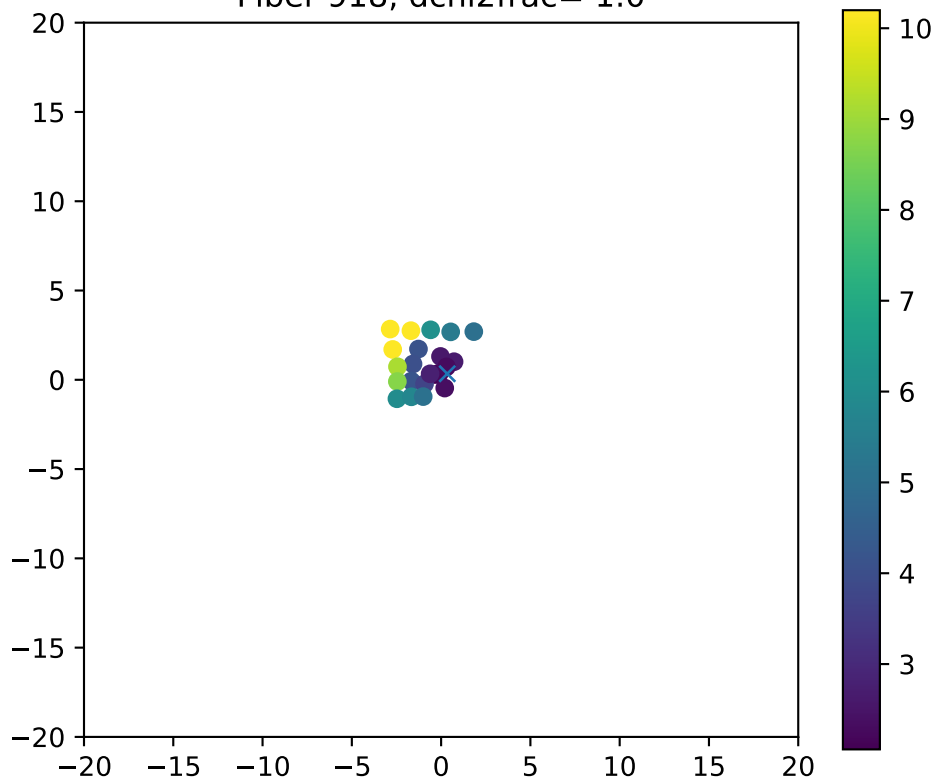
Fiber 918, dchi2frac= 1.0
