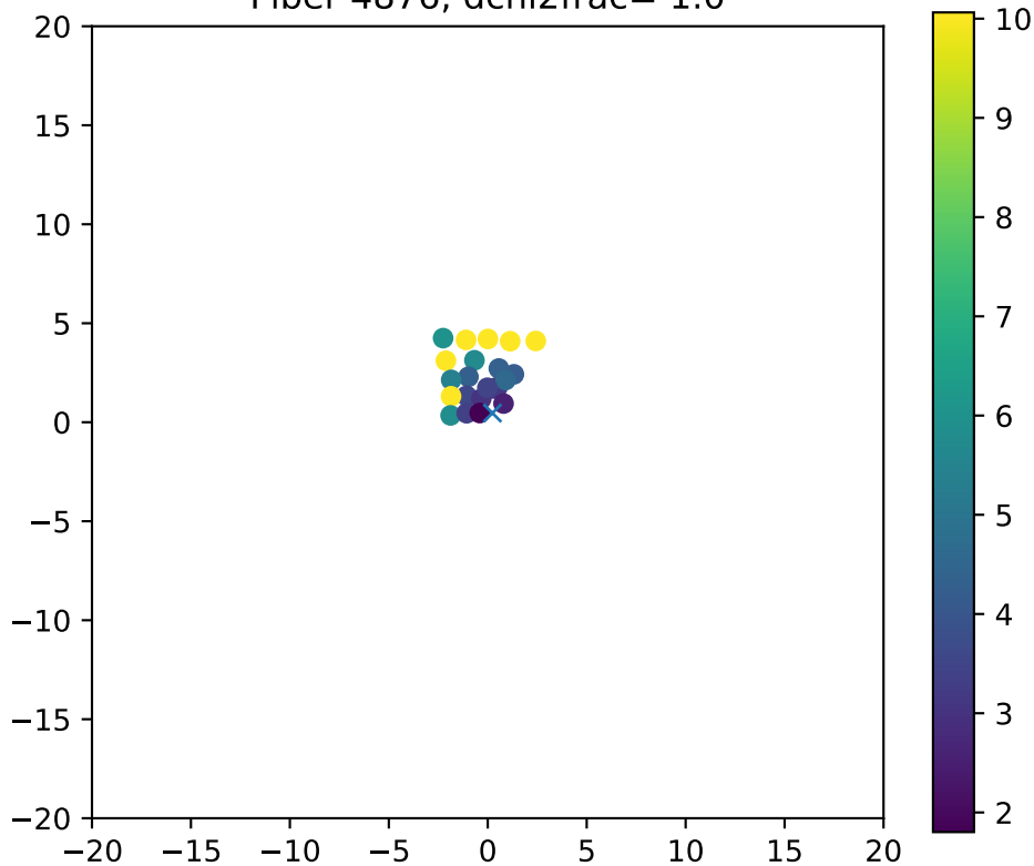
Fiber 4876, dchi2frac= 1.0
