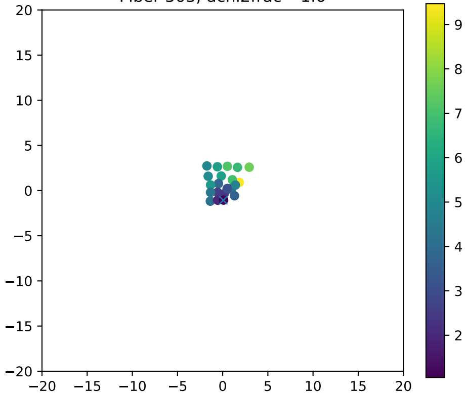
Fiber 503, dchi2frac= 1.0
