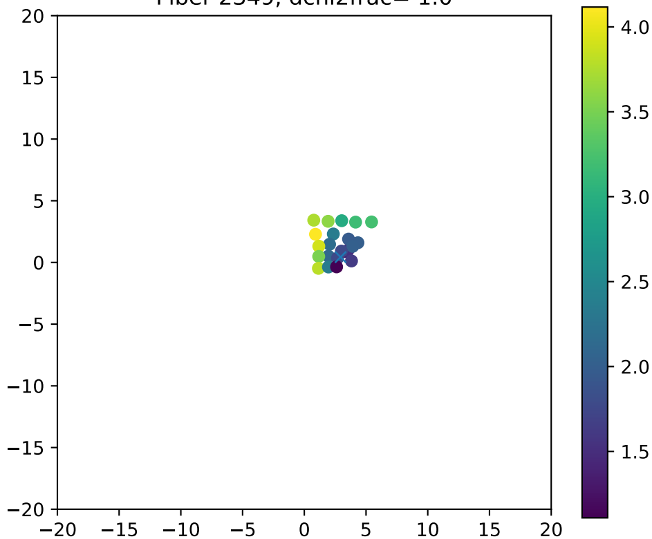
Fiber 2349, dchi2frac= 1.0
