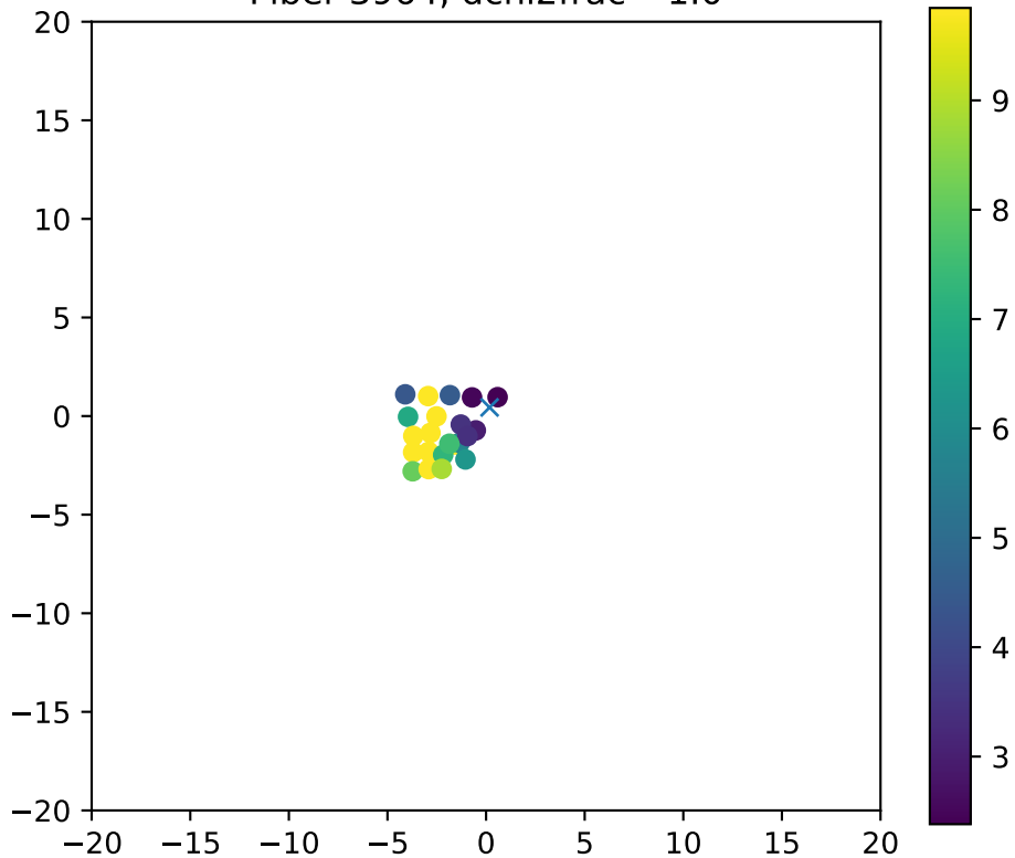
Fiber 3964, dchi2frac= 1.0
