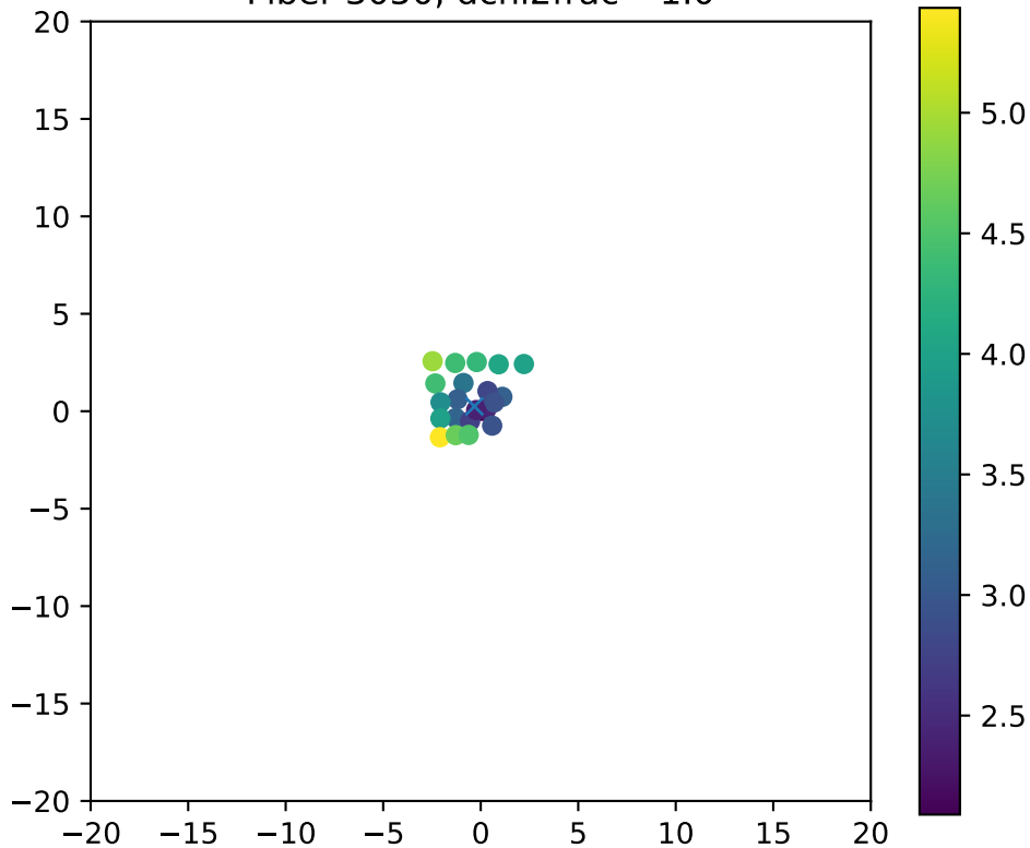
Fiber 3050, dchi2frac= 1.0
