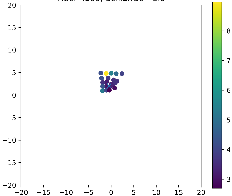
Fiber 4205, dchi2frac= 0.9
