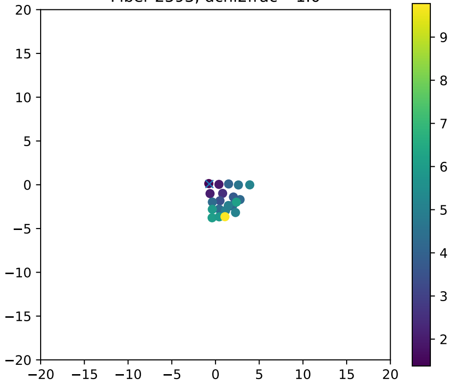
Fiber 2593, dchi2frac= 1.0
