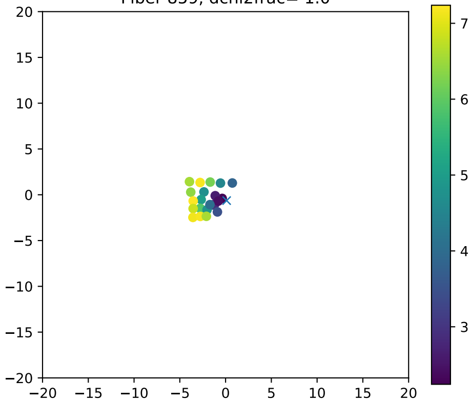
Fiber 859, dchi2frac= 1.0
