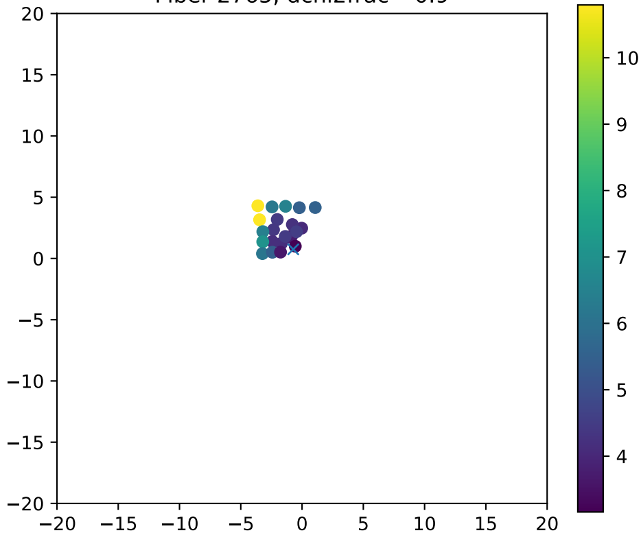
Fiber 2765, dchi2frac= 0.9
