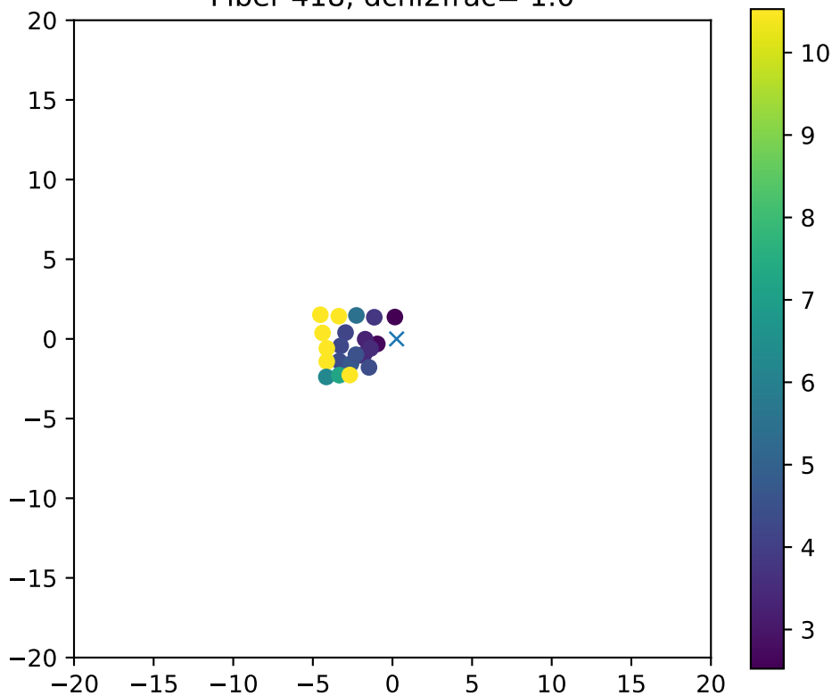
Fiber 418, dchi2frac= 1.0
