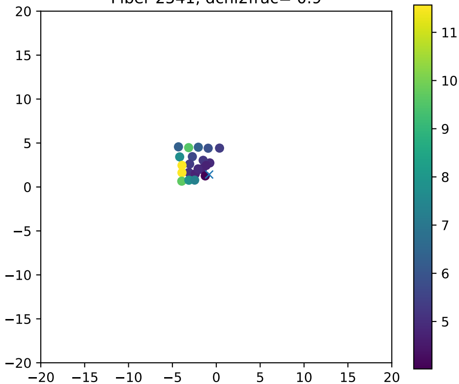
Fiber 2541, dchi2frac= 0.9
