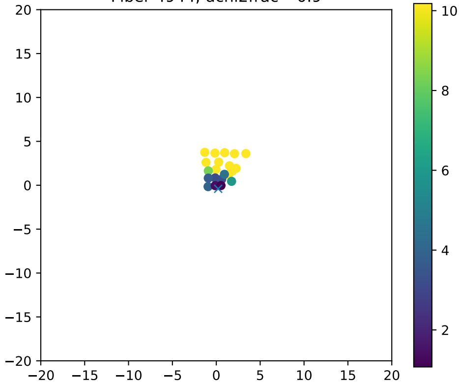
Fiber 4944, dchi2frac= 0.9
