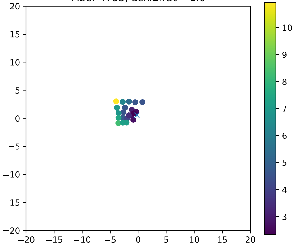
Fiber 4753, dchi2frac= 1.0
