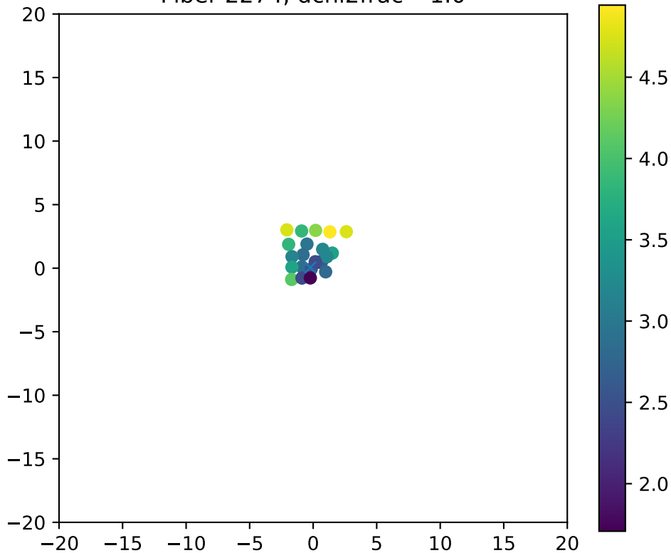
Fiber 2274, dchi2frac= 1.0
