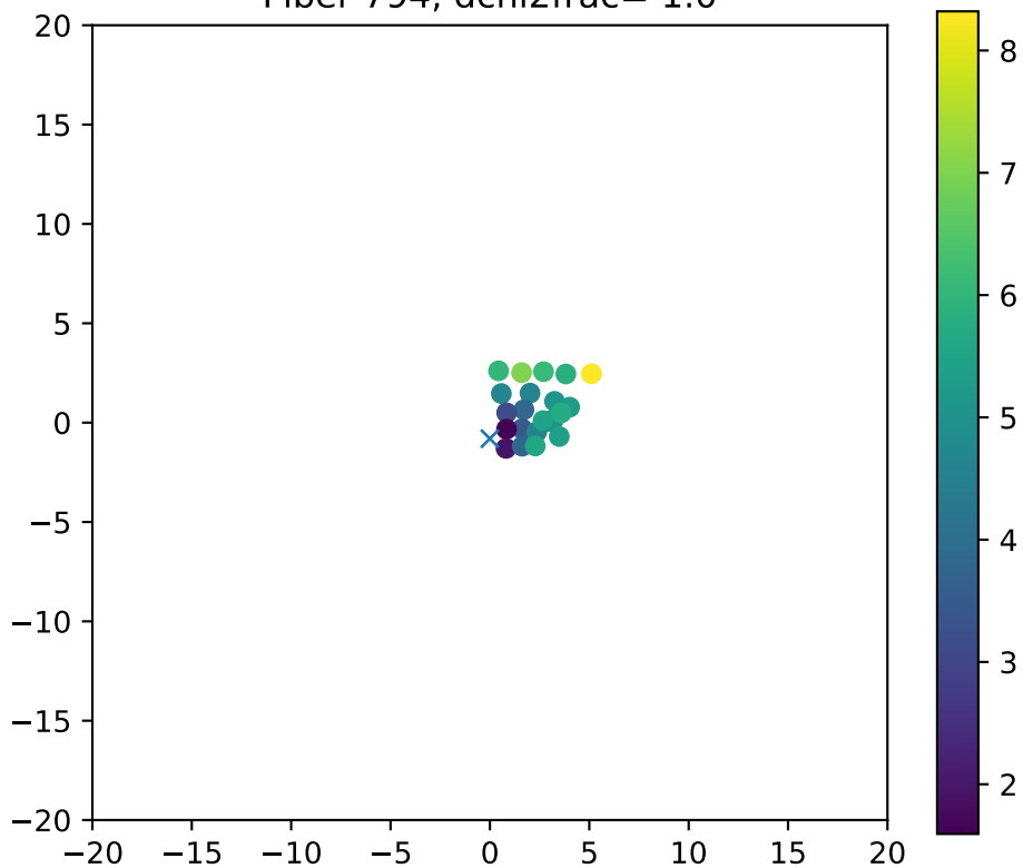
Fiber 794, dchi2frac= 1.0
