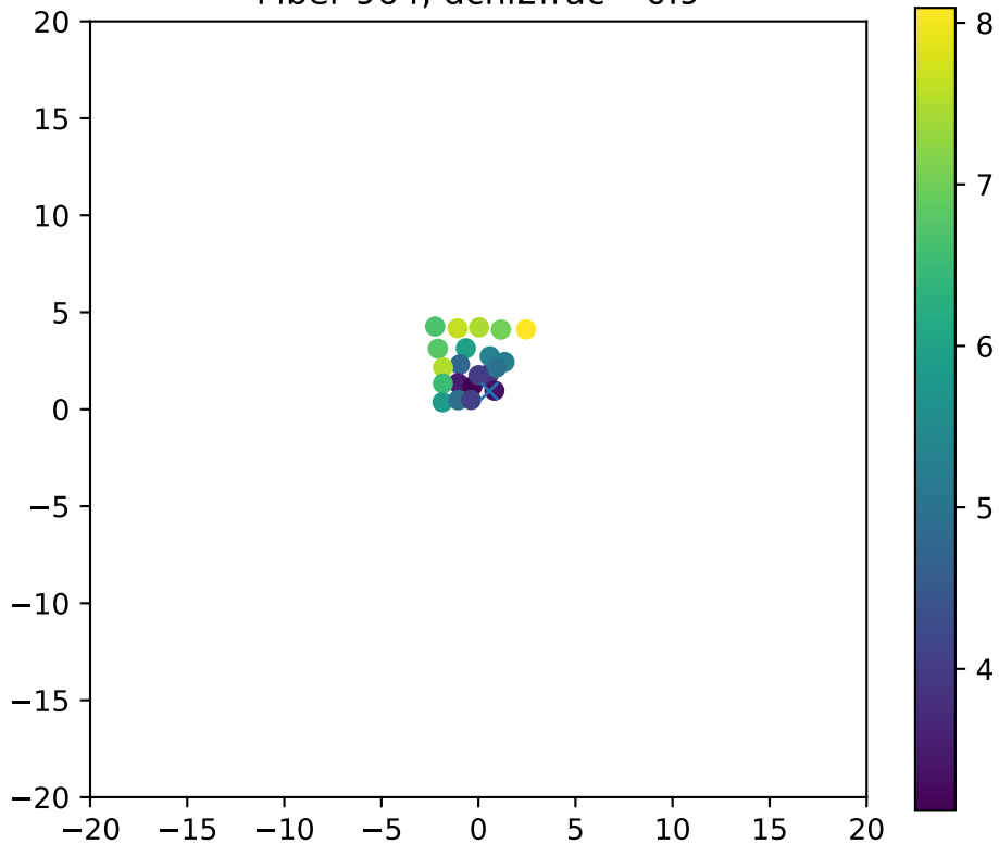
Fiber 964, dchi2frac= 0.9
