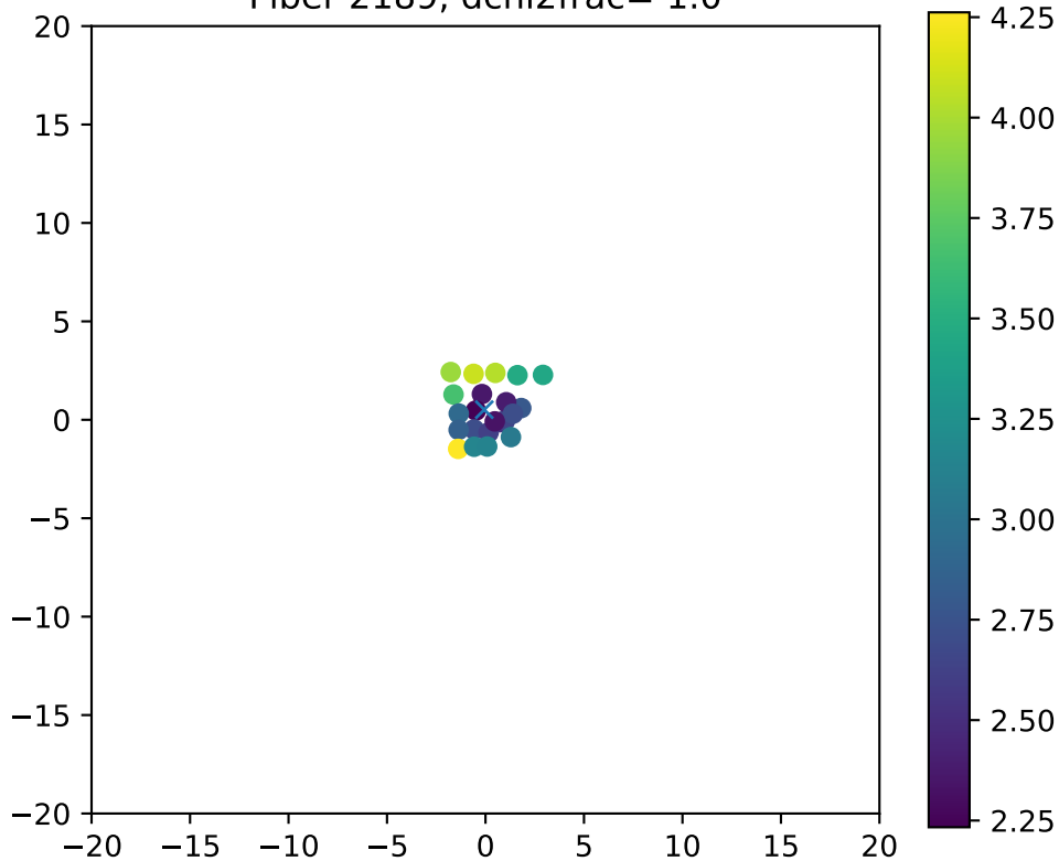
Fiber 2189, dchi2frac= 1.0
