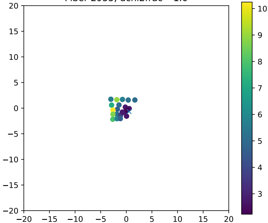
Fiber 2955, dchi2frac= 1.0
