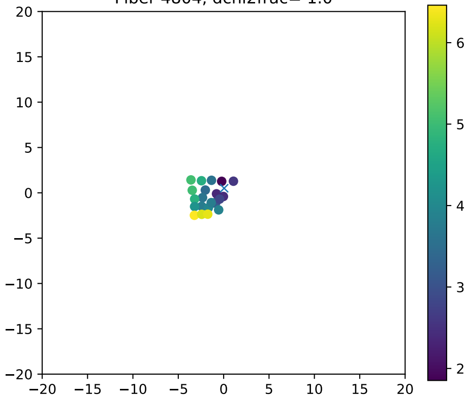
Fiber 4804, dchi2frac= 1.0
