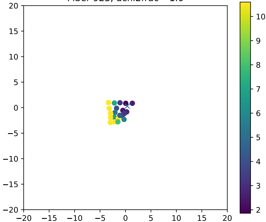
Fiber 923, dchi2frac= 1.0
