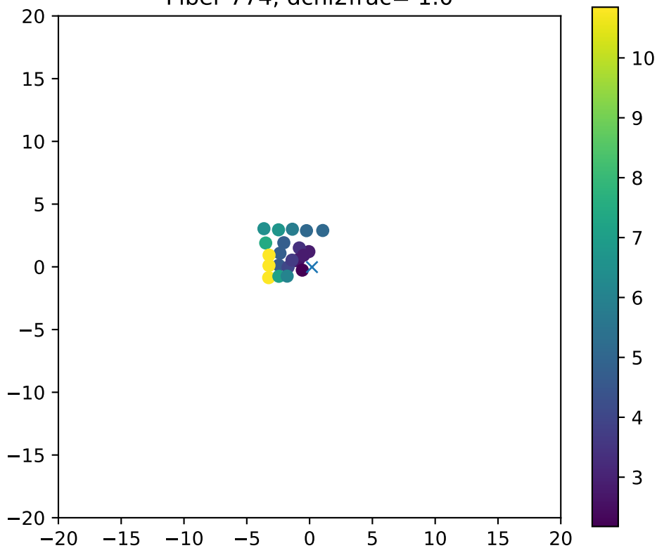
Fiber 774, dchi2frac= 1.0
