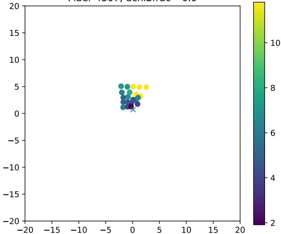
Fiber 4507, dchi2frac= 0.9
