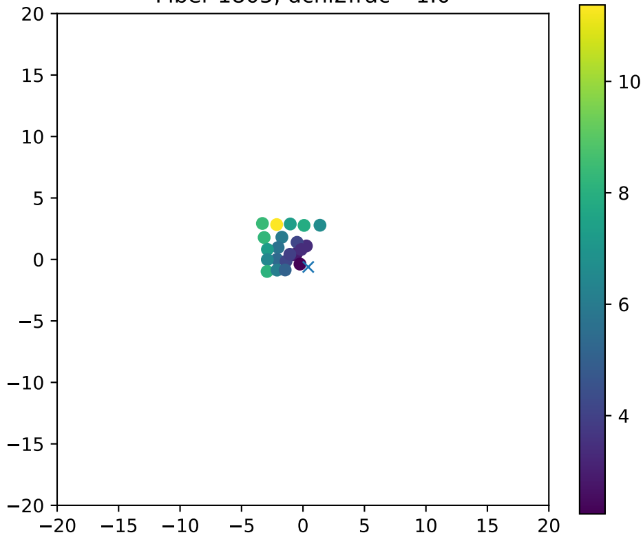
Fiber 1805, dchi2frac= 1.0
