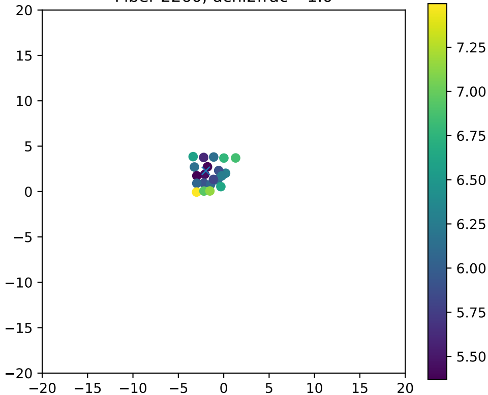
Fiber 2260, dchi2frac= 1.0
