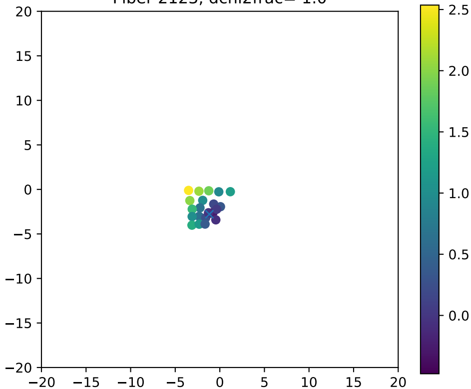
Fiber 2123, dchi2frac= 1.0
