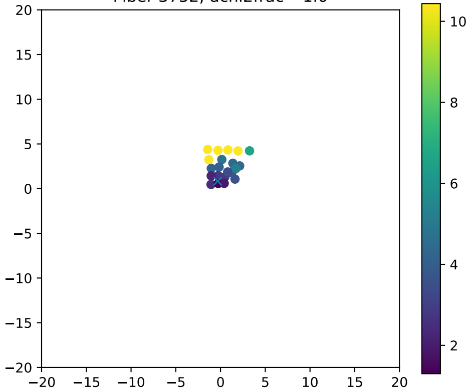
Fiber 3752, dchi2frac= 1.0
