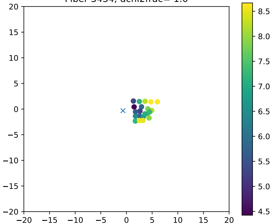
Fiber 3434, dchi2frac= 1.0
