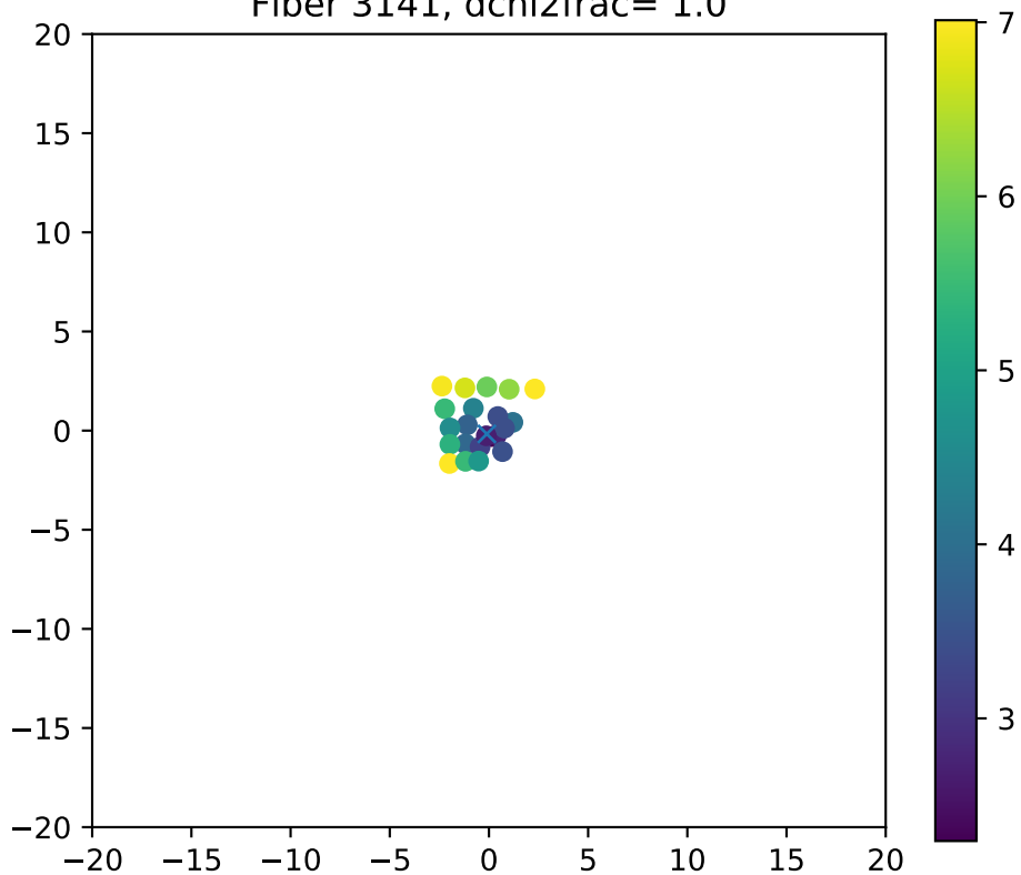
Fiber 3141, dchi2frac= 1.0
