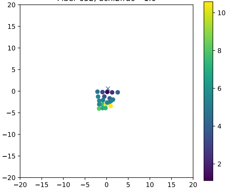
Fiber 652, dchi2frac= 1.0
