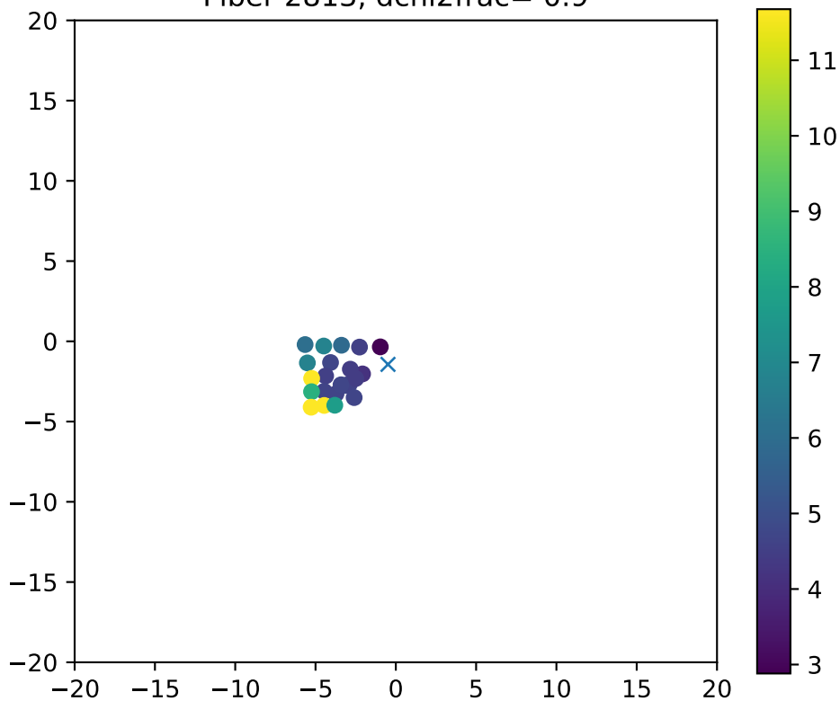
Fiber 2813, dchi2frac= 0.9
