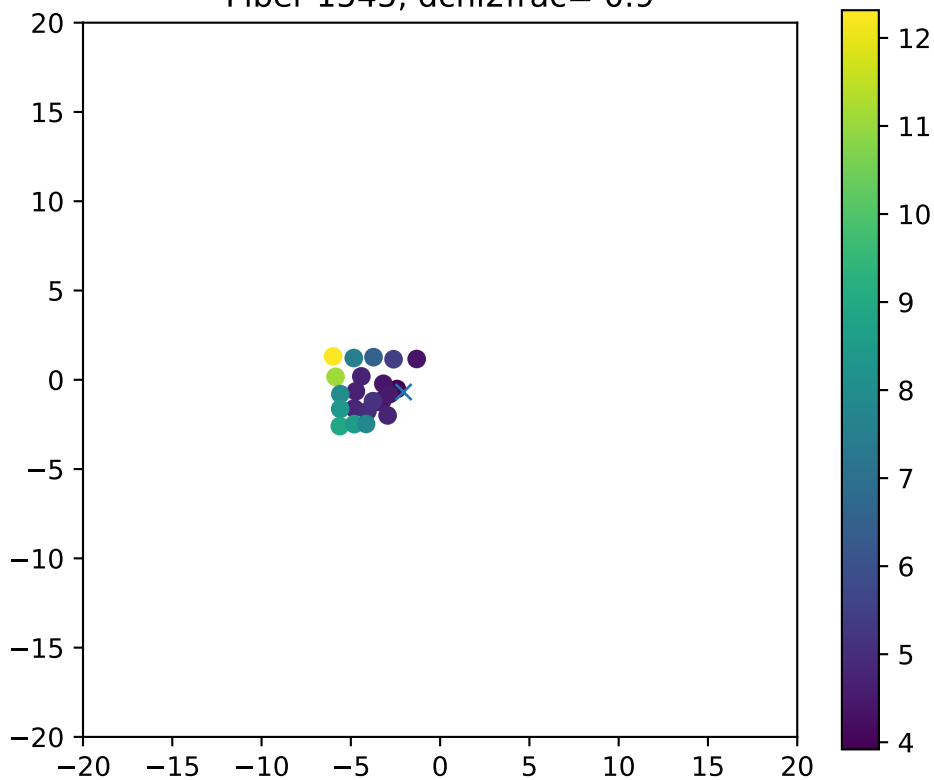
Fiber 1545, dchi2frac= 0.9
