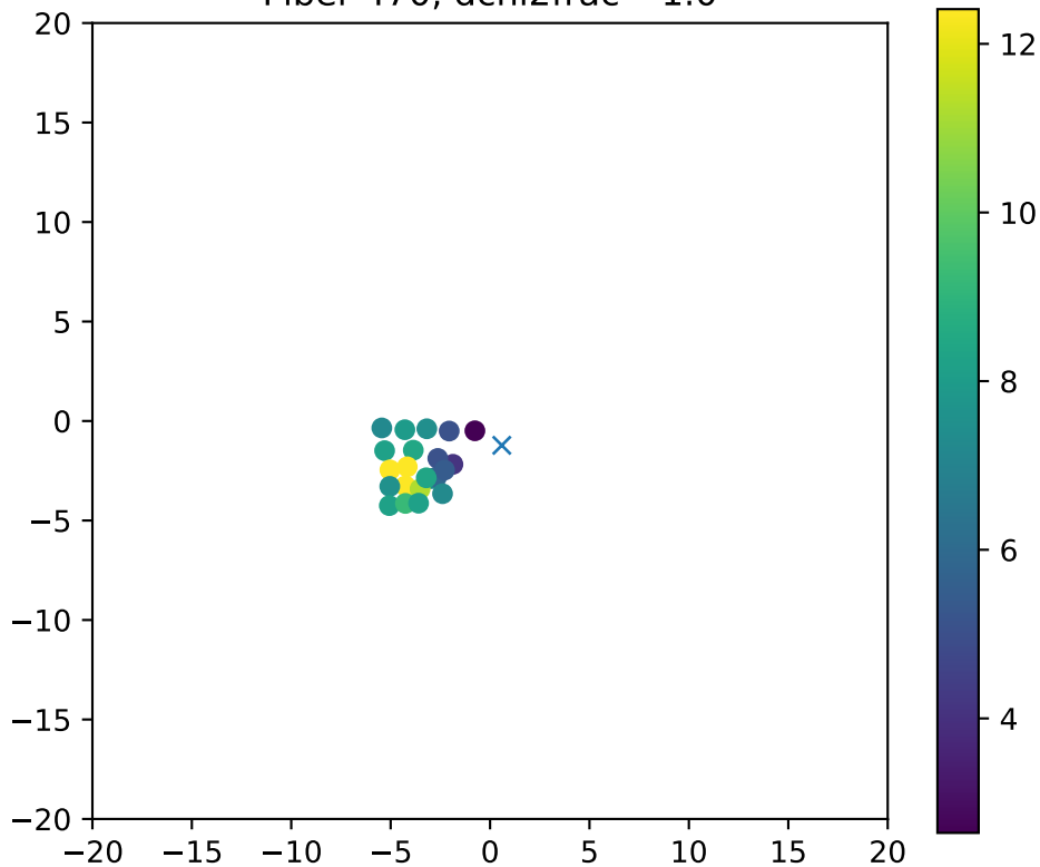
Fiber 470, dchi2frac= 1.0
