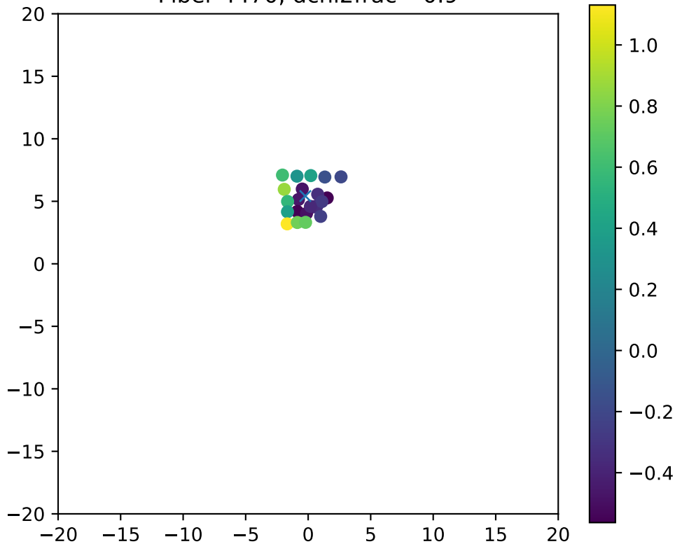
Fiber 4470, dchi2frac= 0.9
