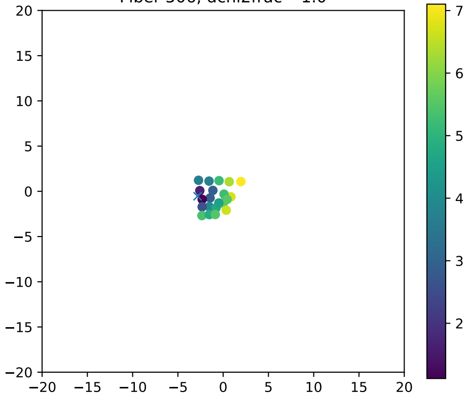
Fiber 506, dchi2frac= 1.0
