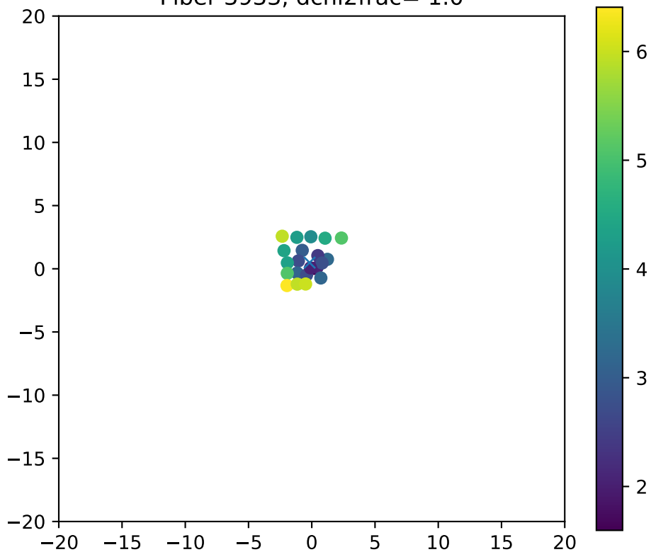
Fiber 3933, dchi2frac= 1.0
