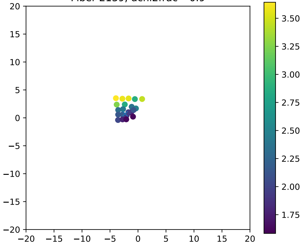
Fiber 2139, dchi2frac= 0.9
