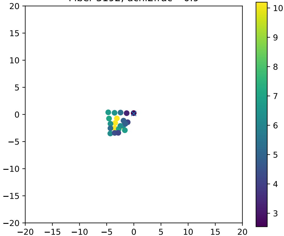
Fiber 3192, dchi2frac= 0.9
