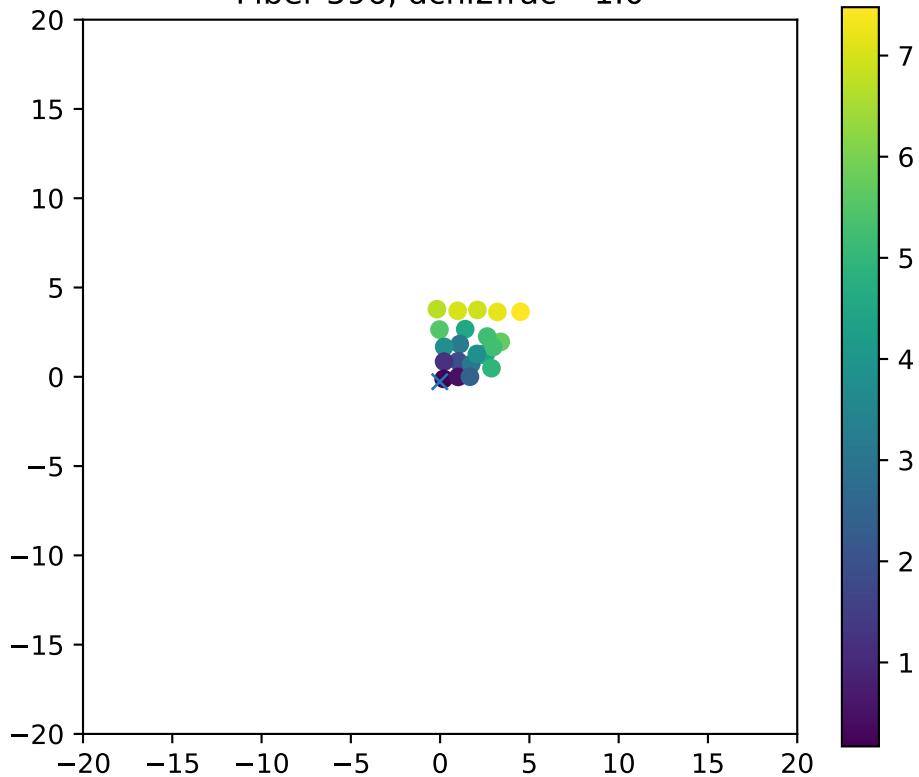
Fiber 596, dchi2frac= 1.0
