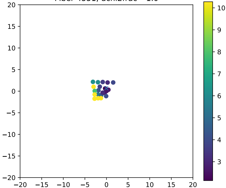
Fiber 4551, dchi2frac= 1.0
