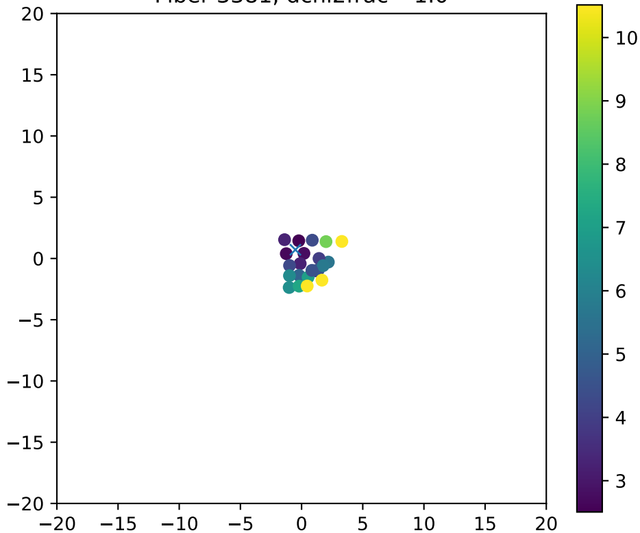
Fiber 3381, dchi2frac= 1.0
