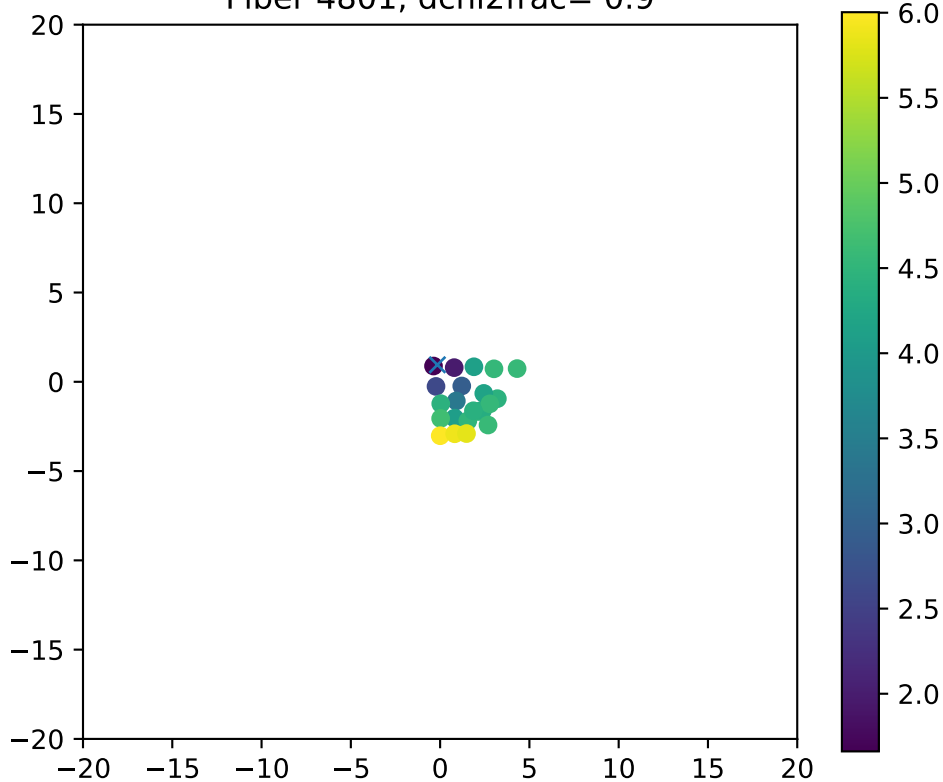
Fiber 4801, dchi2frac= 0.9
