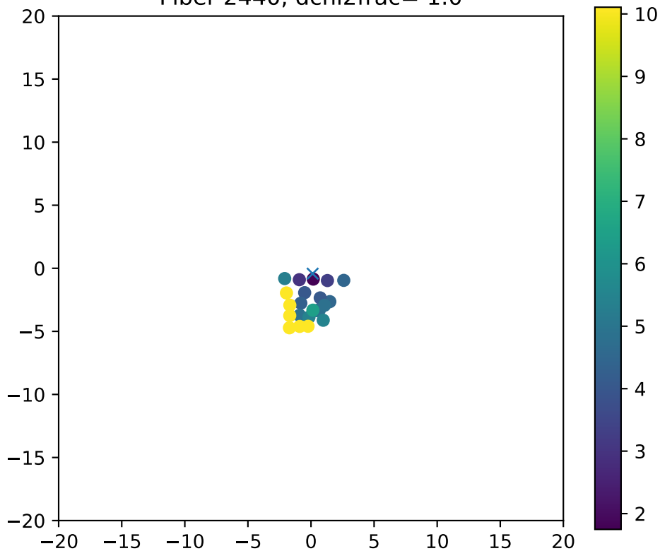
Fiber 2440, dchi2frac= 1.0
