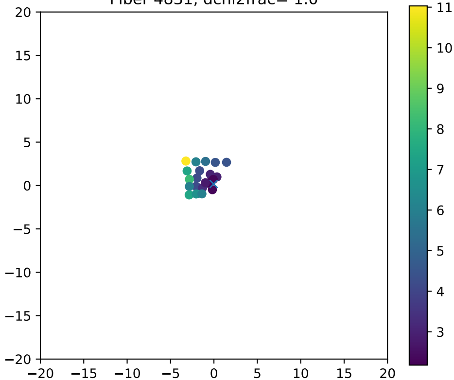
Fiber 4831, dchi2frac= 1.0
