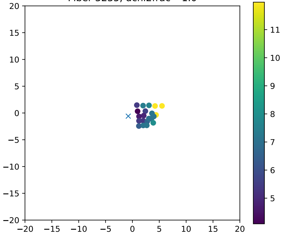
Fiber 3235, dchi2frac= 1.0
