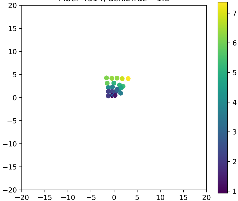
Fiber 4314, dchi2frac= 1.0
