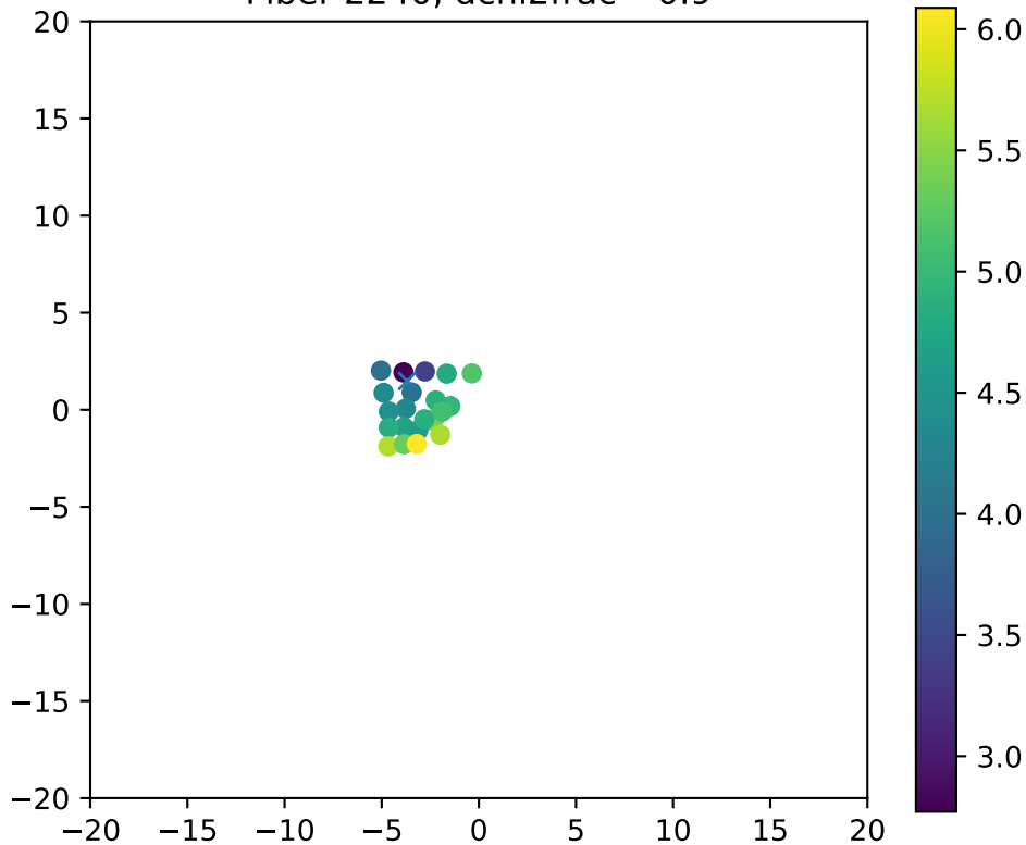
Fiber 2240, dchi2frac= 0.9
