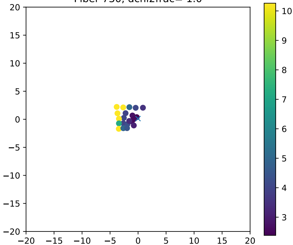
Fiber 730, dchi2frac= 1.0
