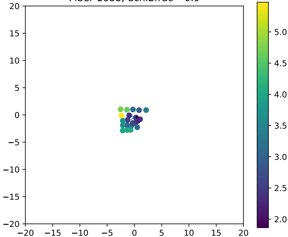
Fiber 1688, dchi2frac= 0.9
