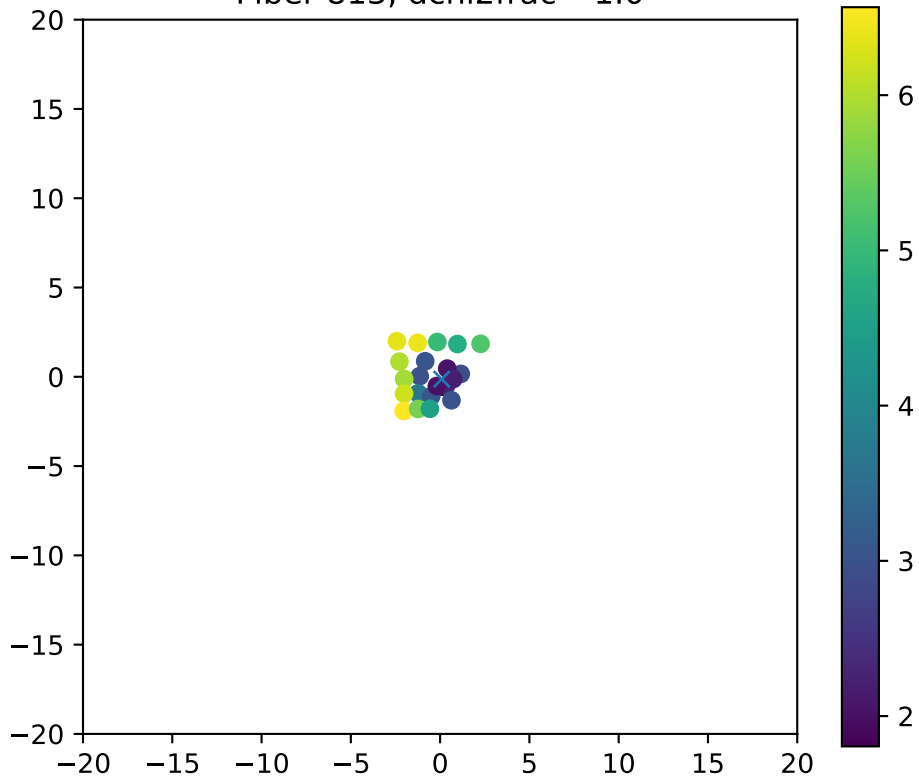
Fiber 813, dchi2frac= 1.0
