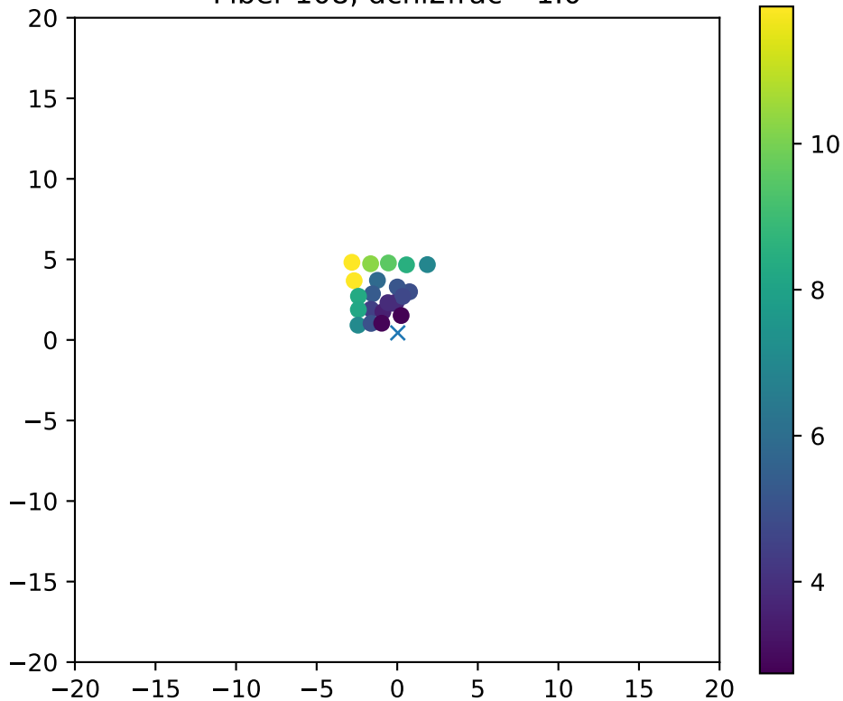
Fiber 108, dchi2frac= 1.0
