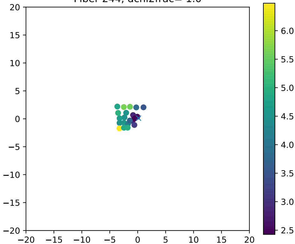
Fiber 244, dchi2frac= 1.0
