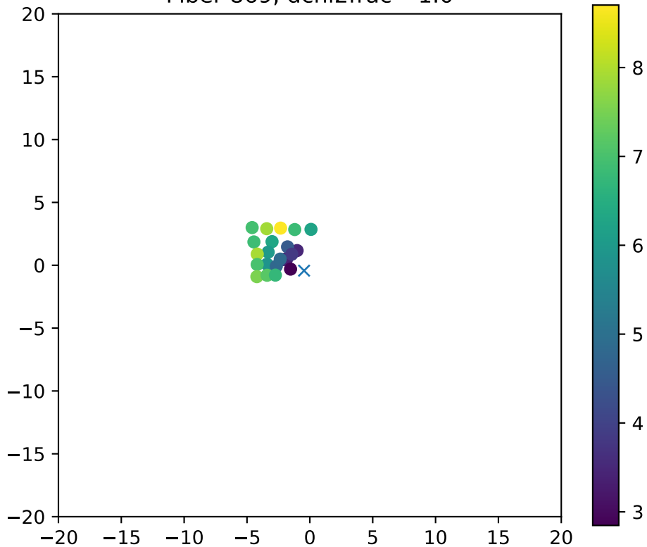
Fiber 869, dchi2frac= 1.0
