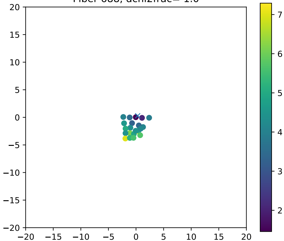
Fiber 688, dchi2frac= 1.0
