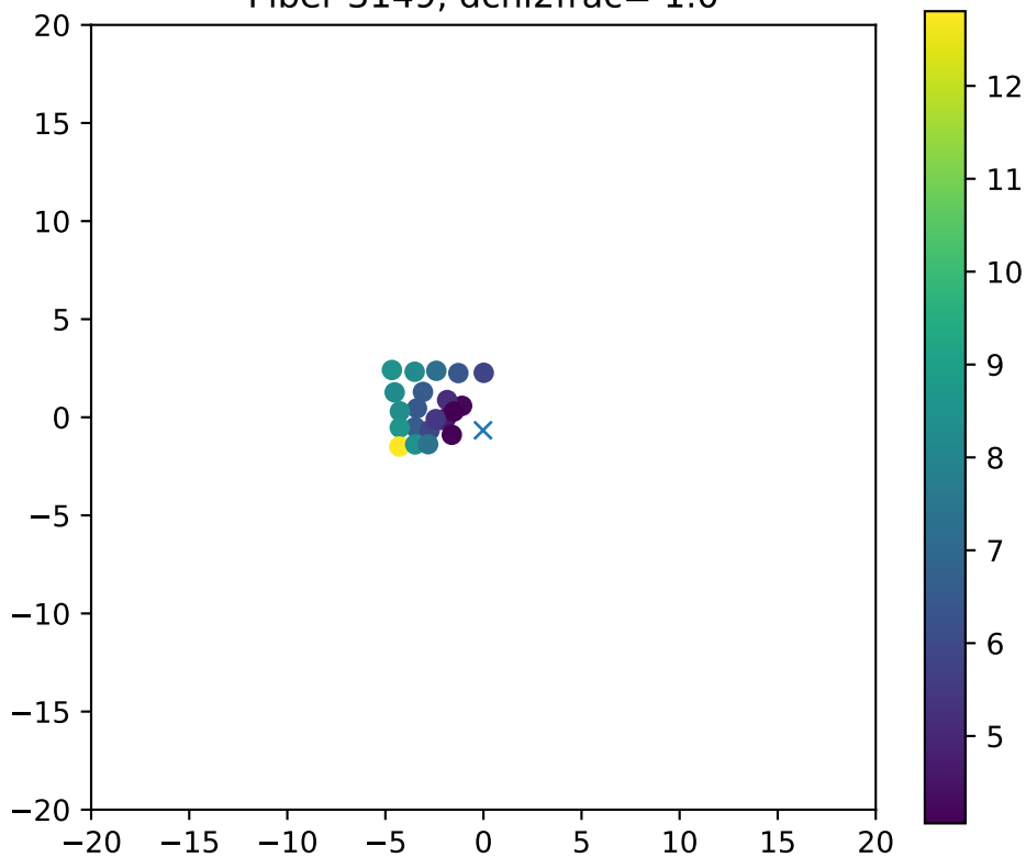
Fiber 3149, dchi2frac= 1.0
