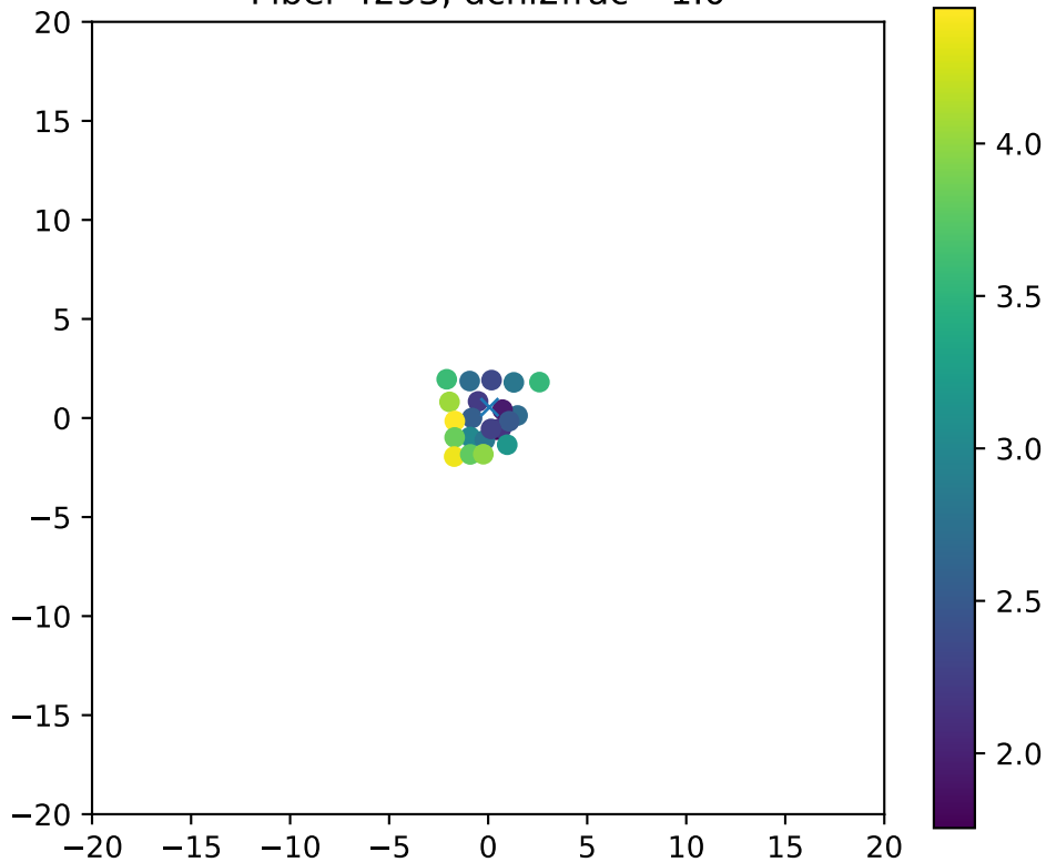
Fiber 4293, dchi2frac= 1.0
