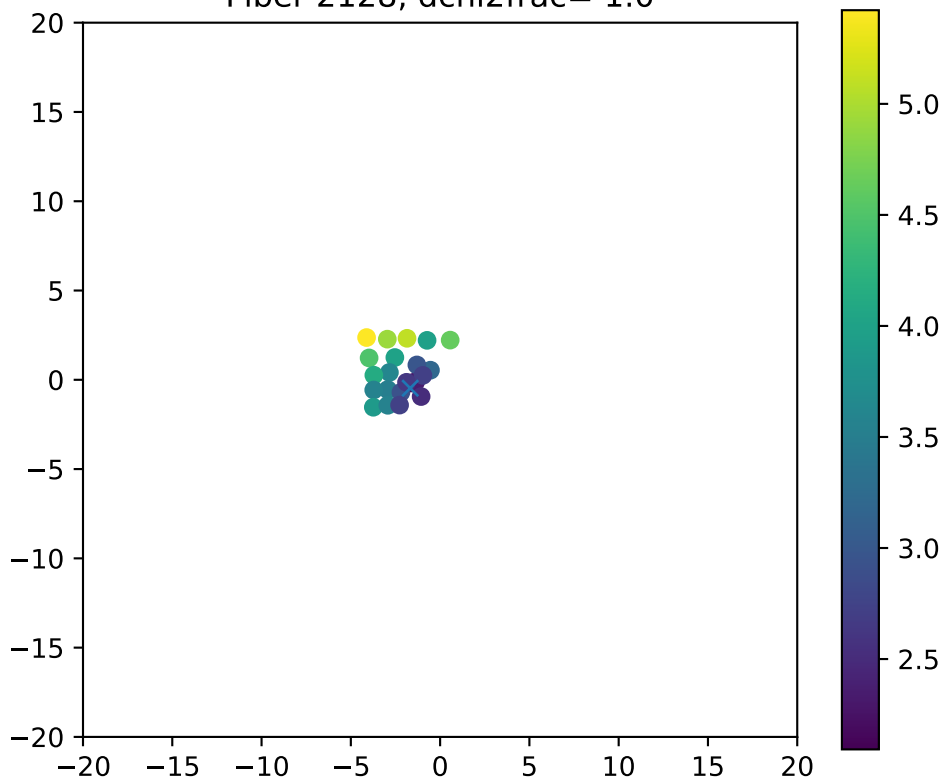
Fiber 2128, dchi2frac= 1.0
