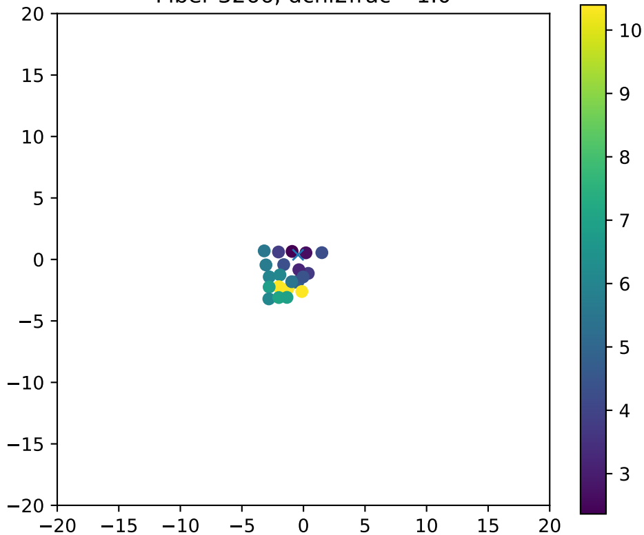
Fiber 3266, dchi2frac= 1.0
