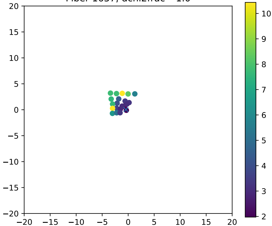
Fiber 1637, dchi2frac= 1.0
