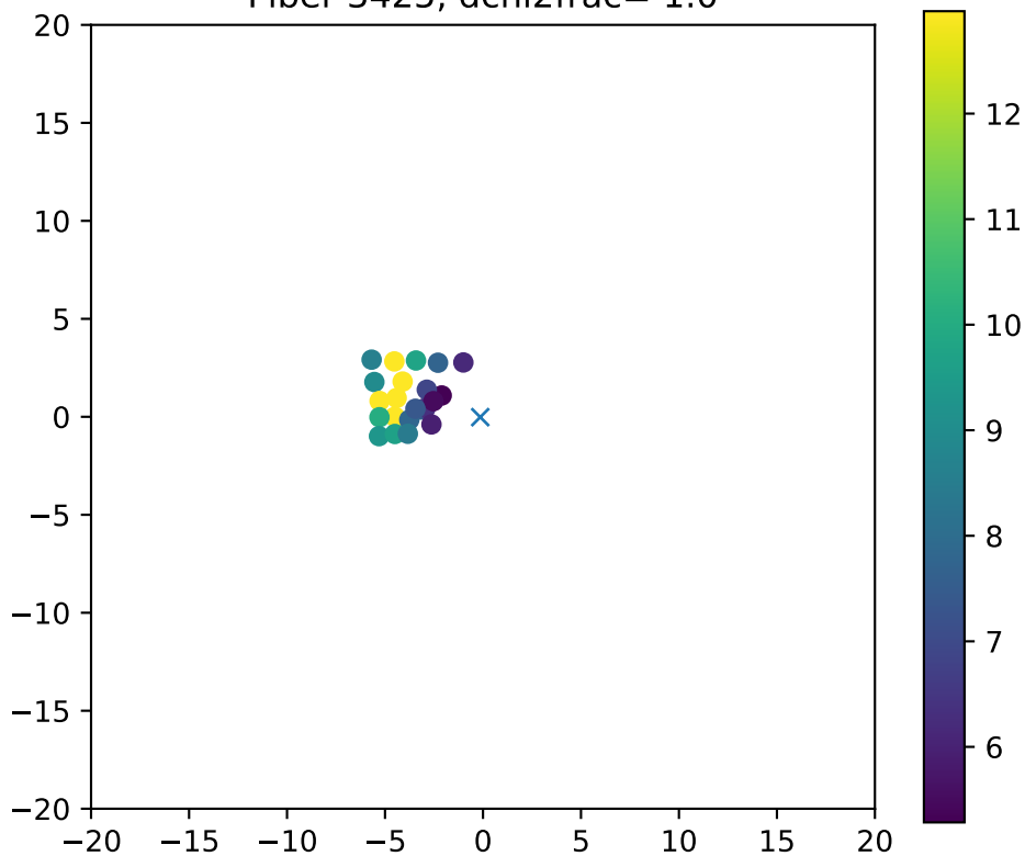
Fiber 3425, dchi2frac= 1.0
