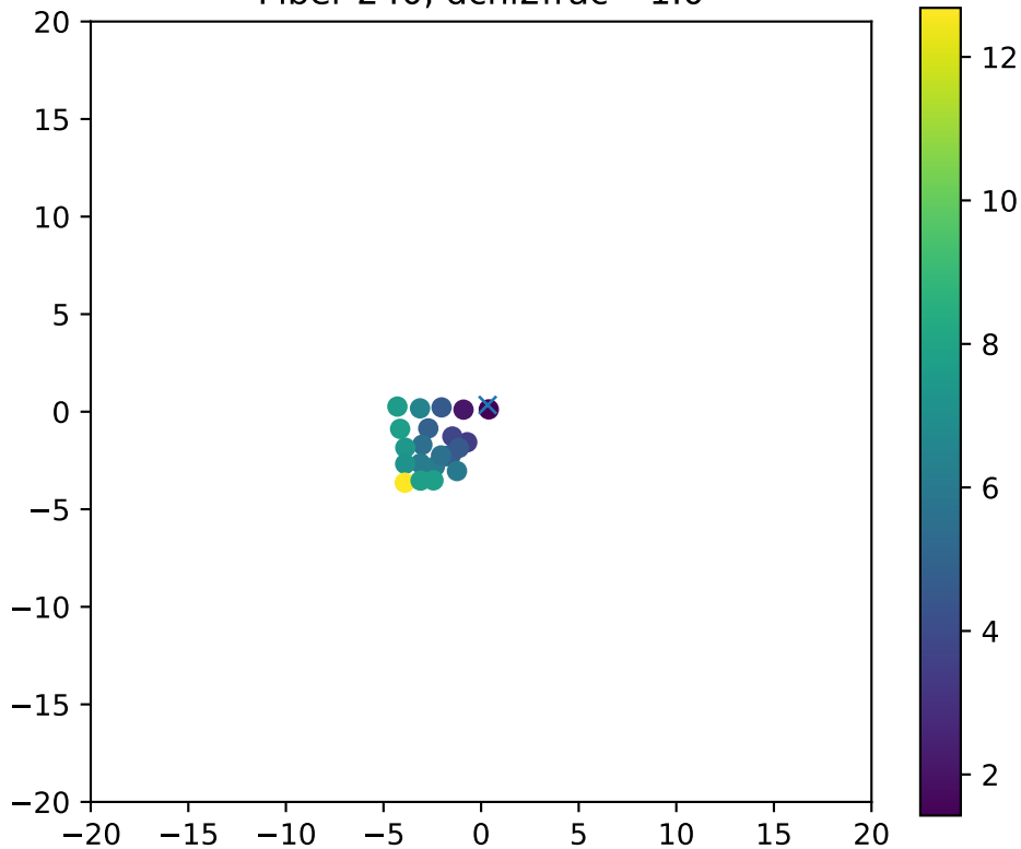
Fiber 240, dchi2frac= 1.0
