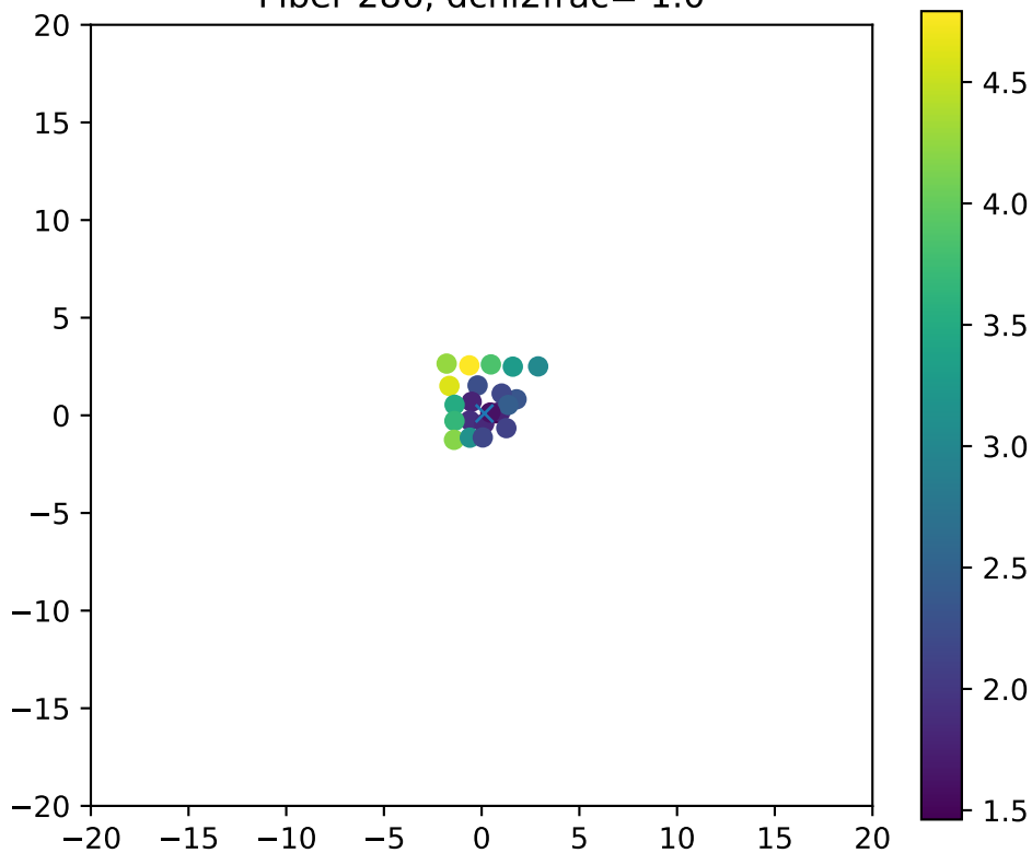
Fiber 286, dchi2frac= 1.0
