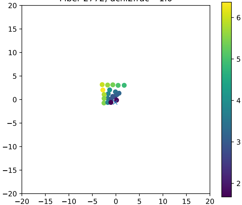
Fiber 2772, dchi2frac= 1.0
