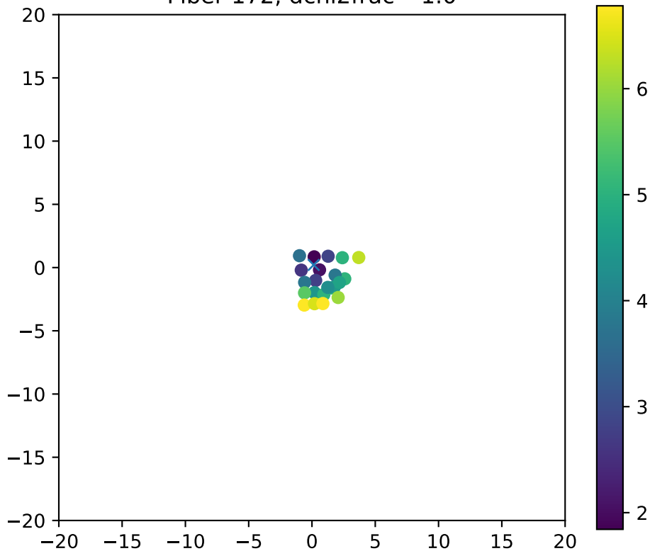
Fiber 172, dchi2frac= 1.0
