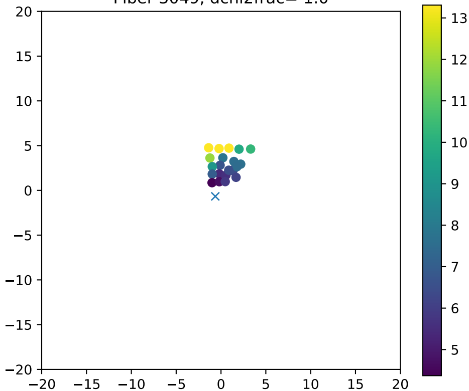
Fiber 3049, dchi2frac= 1.0
