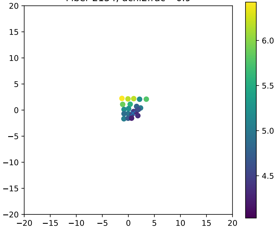
Fiber 2134, dchi2frac= 0.9
