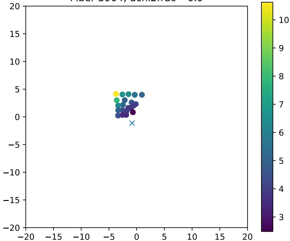
Fiber 3904, dchi2frac= 0.9
