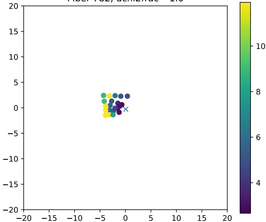
Fiber 782, dchi2frac= 1.0
