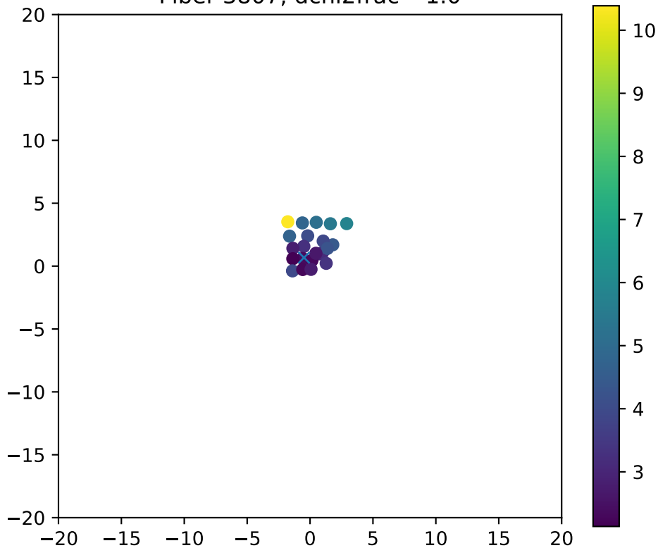
Fiber 3807, dchi2frac= 1.0
