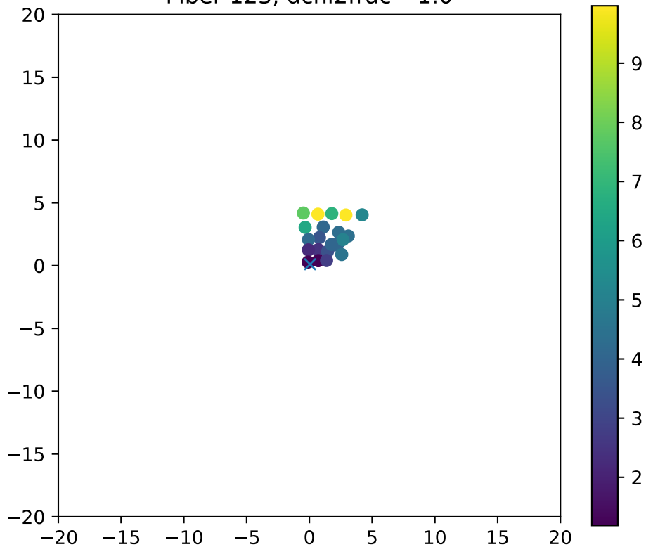
Fiber 123, dchi2frac= 1.0
