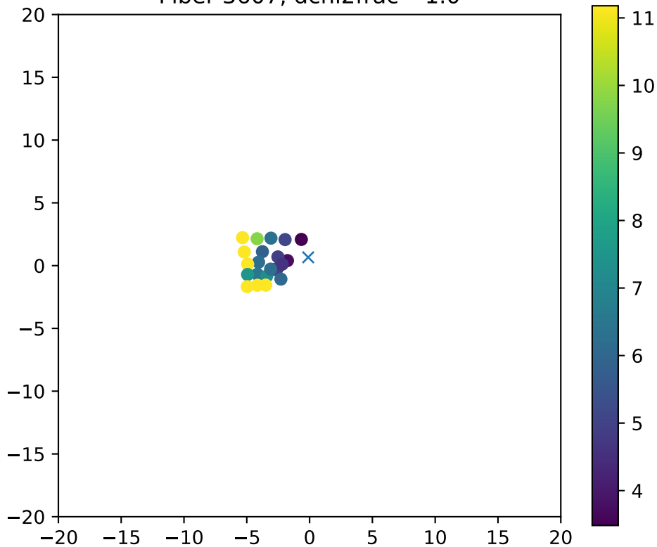
Fiber 3607, dchi2frac= 1.0
