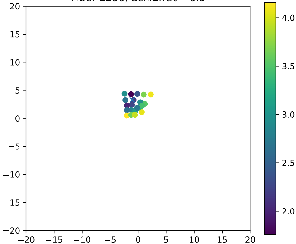
Fiber 2256, dchi2frac= 0.9
