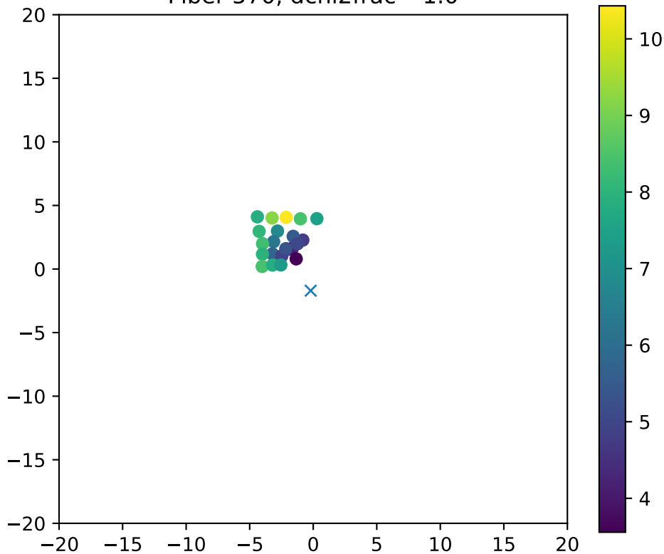
Fiber 570, dchi2frac= 1.0
