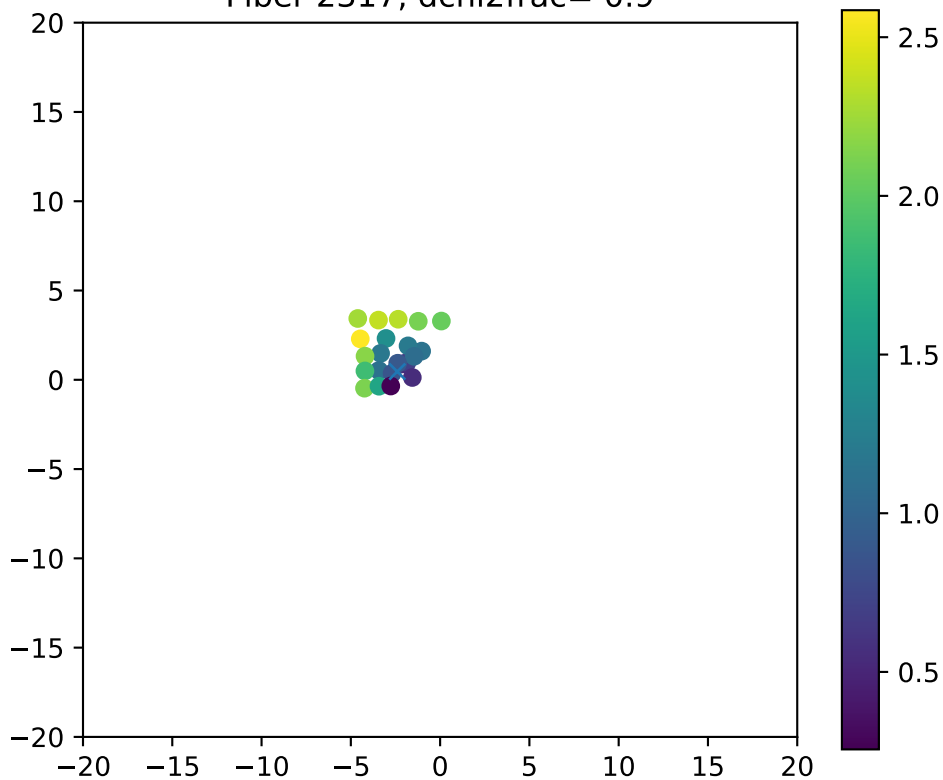
Fiber 2317, dchi2frac= 0.9
