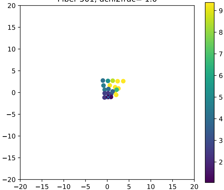
Fiber 501, dchi2frac= 1.0
