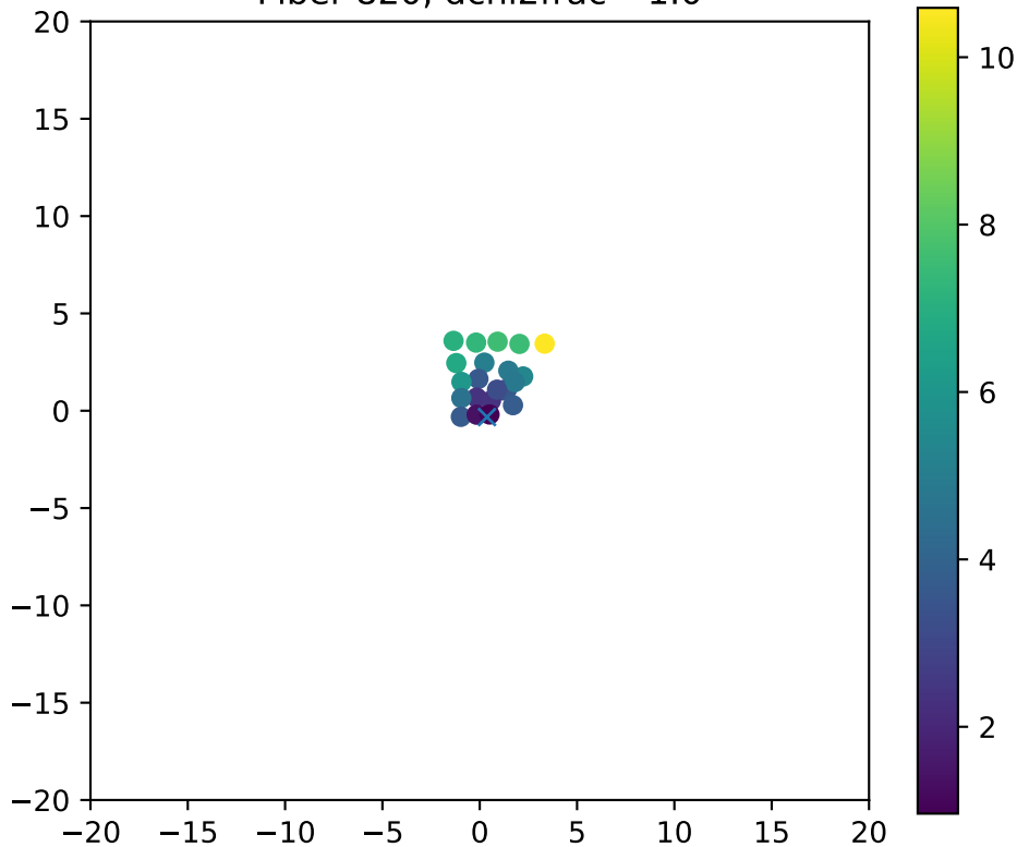
Fiber 820, dchi2frac= 1.0
