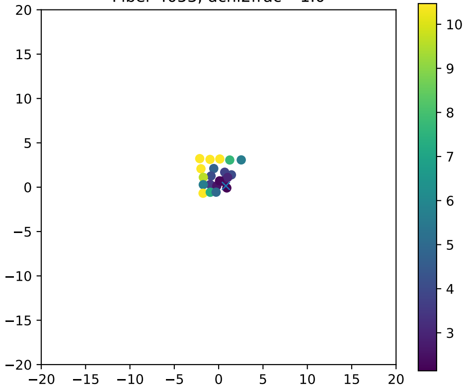
Fiber 4053, dchi2frac= 1.0
