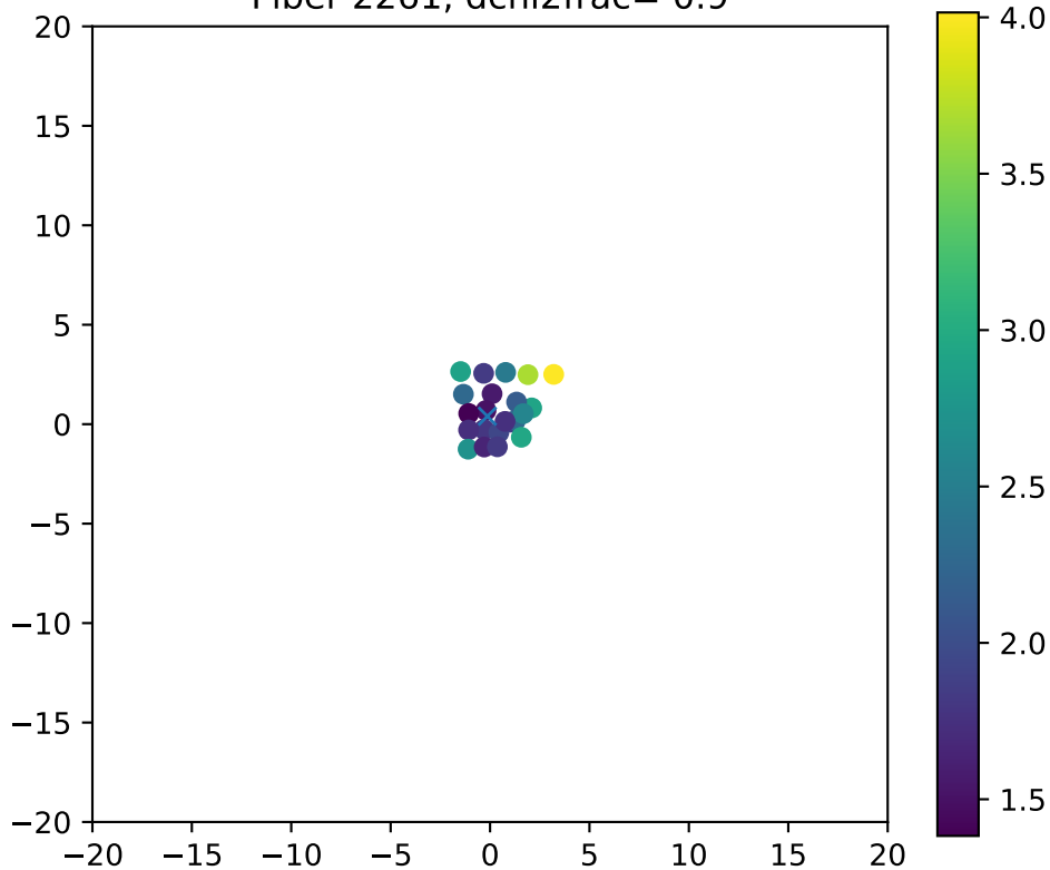
Fiber 2261, dchi2frac= 0.9
