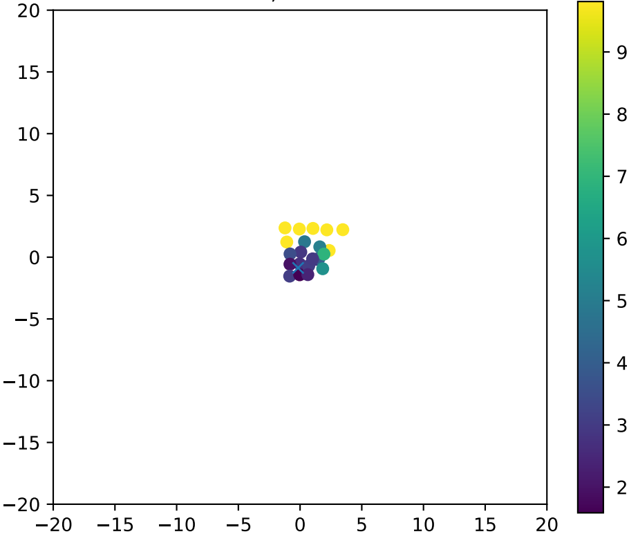
Fiber 2430, dchi2frac= 1.0
