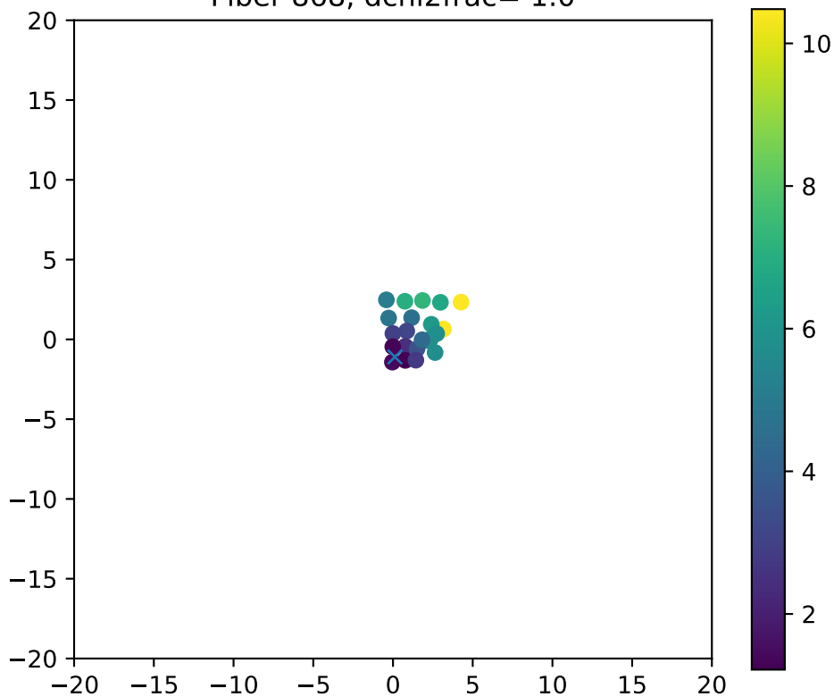
Fiber 868, dchi2frac= 1.0
