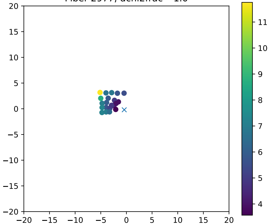
Fiber 2977, dchi2frac= 1.0
