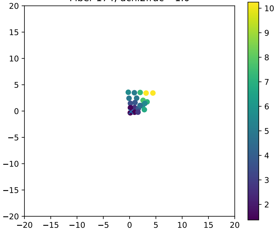
Fiber 174, dchi2frac= 1.0
