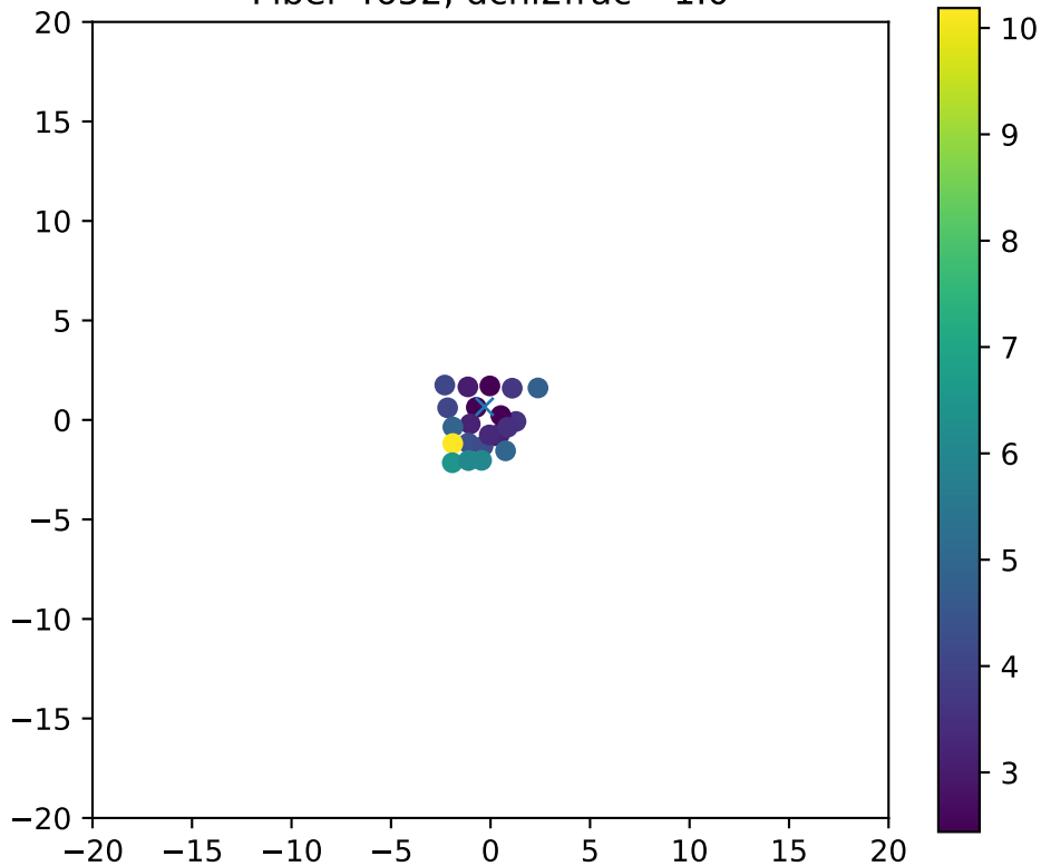
Fiber 4652, dchi2frac= 1.0
