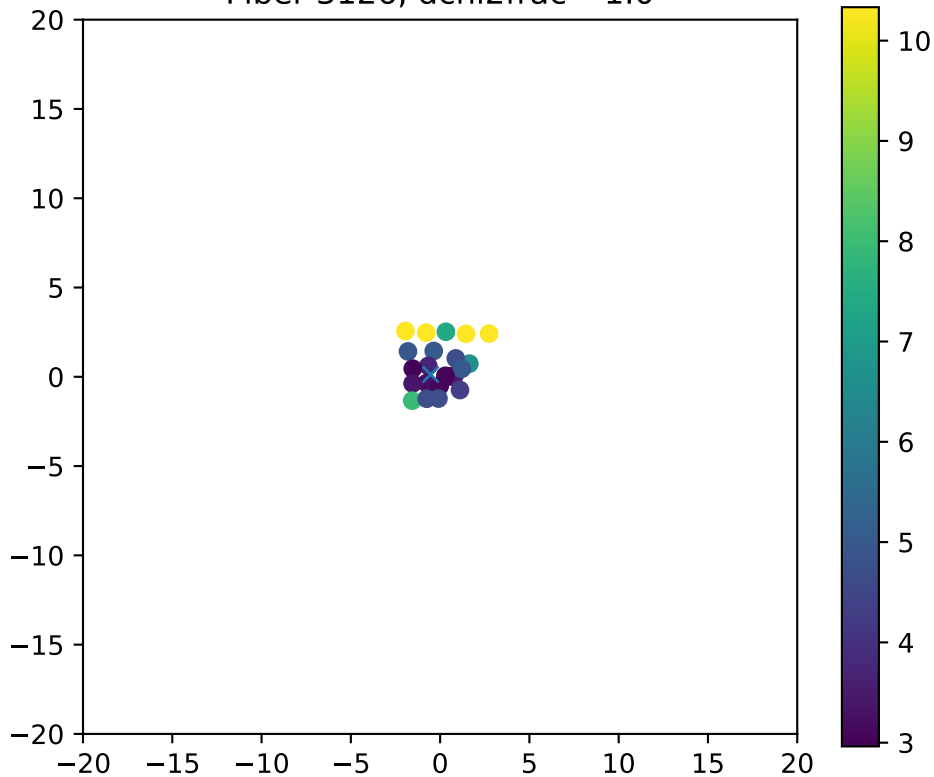
Fiber 3126, dchi2frac= 1.0
