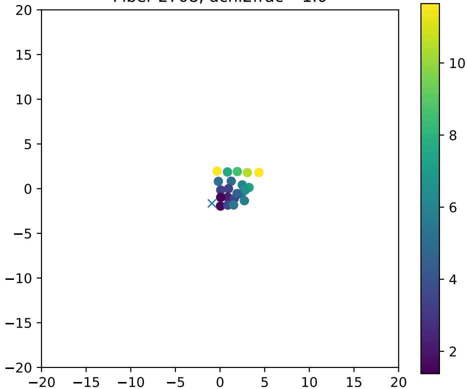
Fiber 2708, dchi2frac= 1.0
