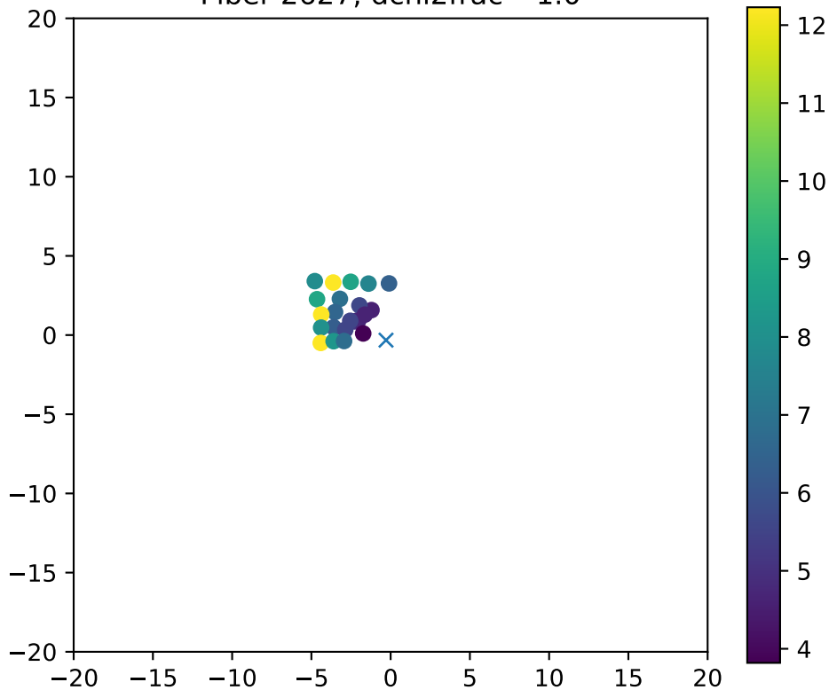
Fiber 2627, dchi2frac= 1.0
