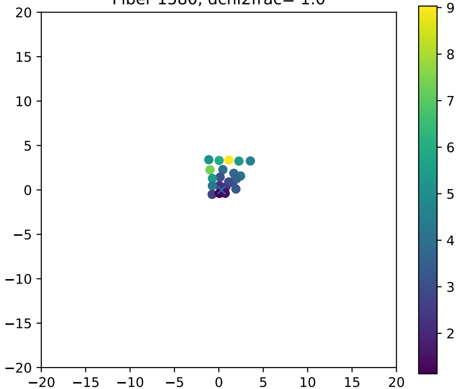
Fiber 1580, dchi2frac= 1.0
