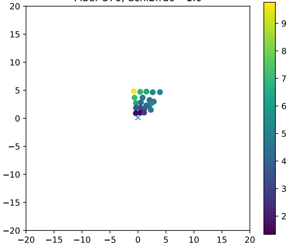
Fiber 376, dchi2frac= 1.0
