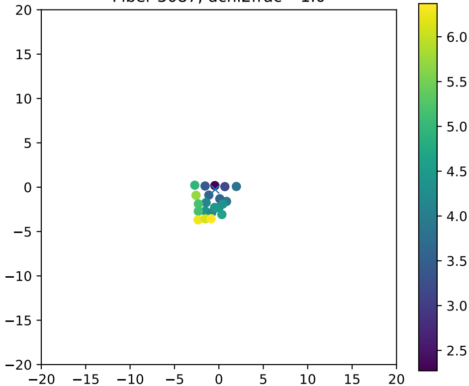
Fiber 3087, dchi2frac= 1.0
