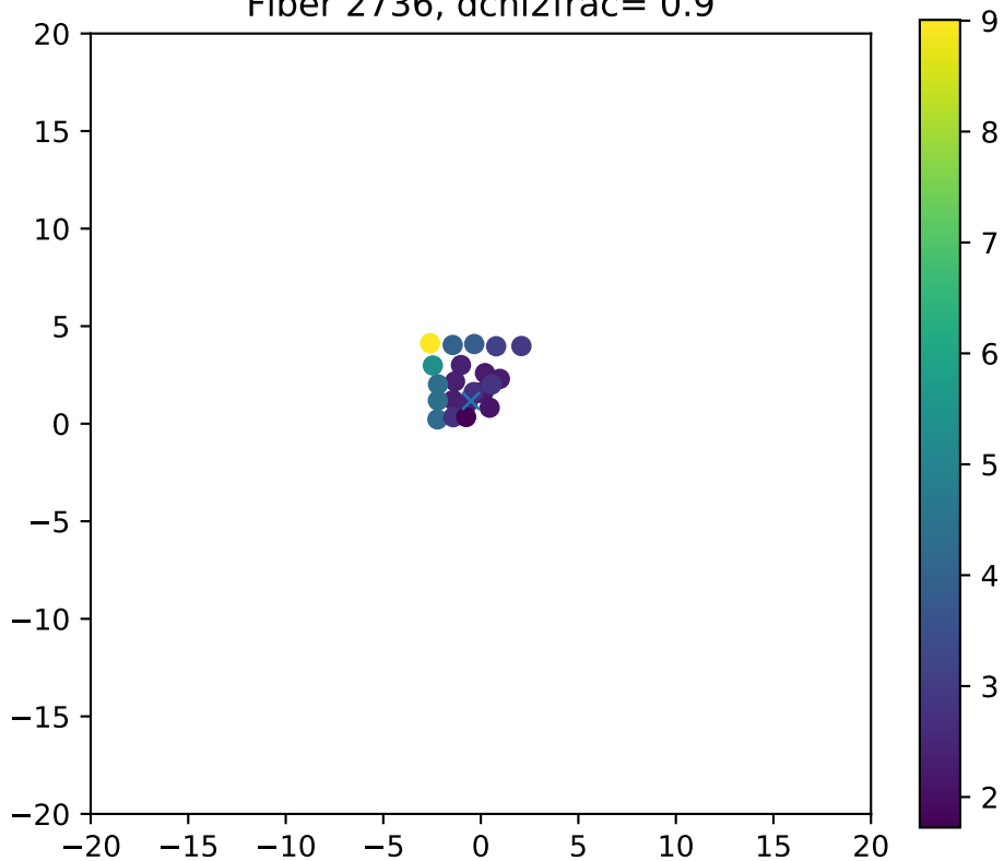
Fiber 2736, dchi2frac= 0.9
