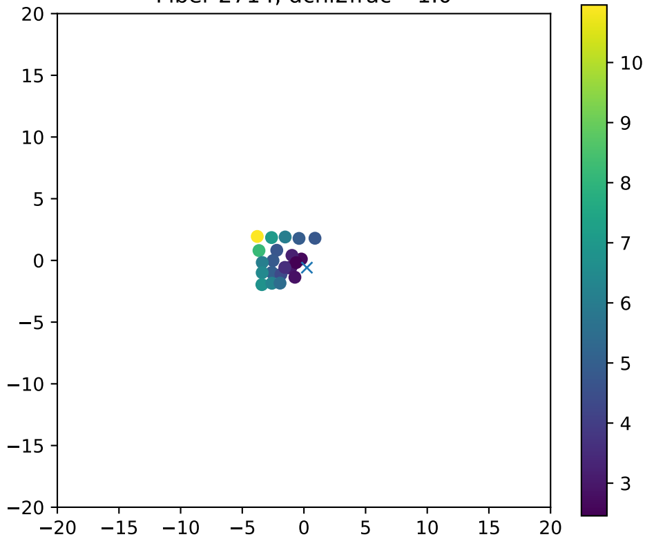
Fiber 2714, dchi2frac= 1.0
