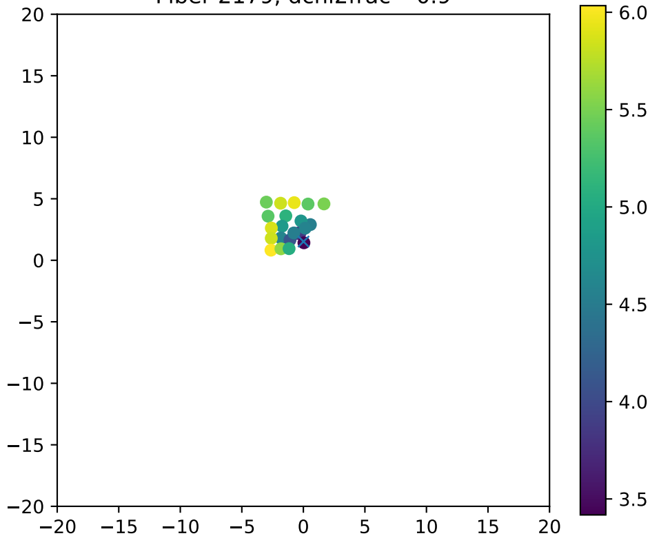
Fiber 2179, dchi2frac= 0.9
