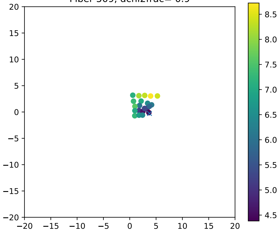
Fiber 509, dchi2frac= 0.9
