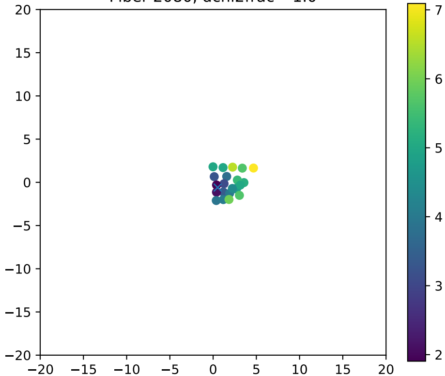
Fiber 2080, dchi2frac= 1.0
