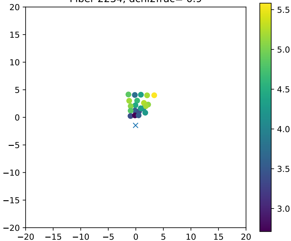
Fiber 2234, dchi2frac= 0.9
