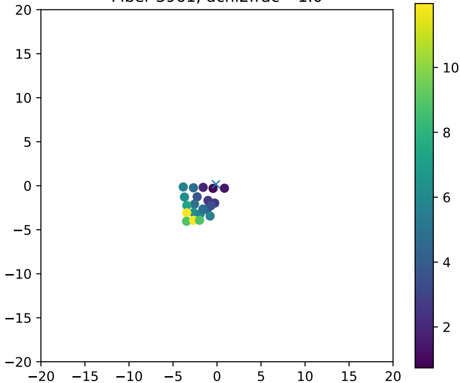
Fiber 3961, dchi2frac= 1.0
