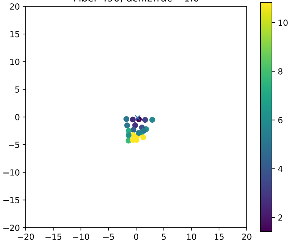
Fiber 490, dchi2frac= 1.0
