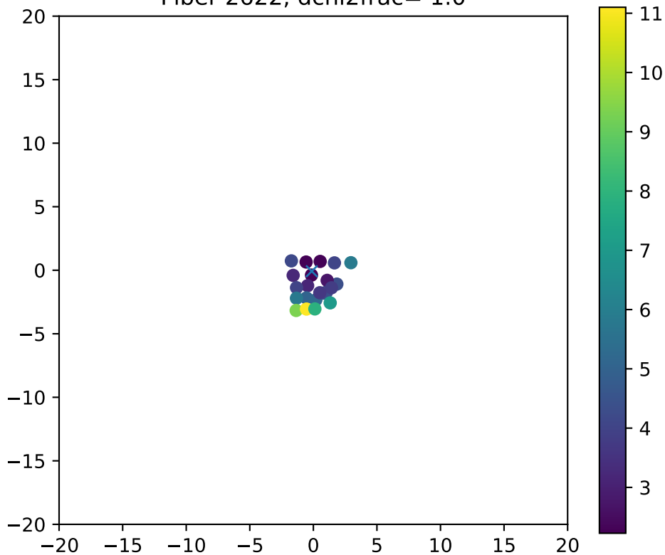
Fiber 2622, dchi2frac= 1.0
