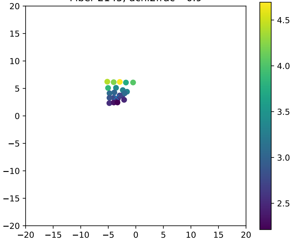
Fiber 2145, dchi2frac= 0.9
