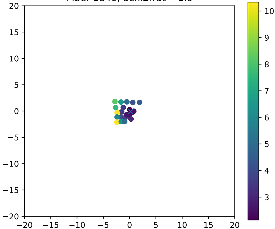
Fiber 1840, dchi2frac= 1.0
