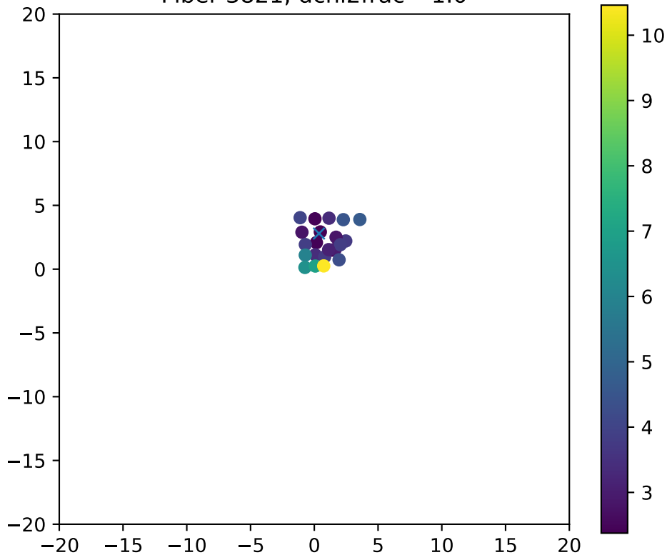
Fiber 3821, dchi2frac= 1.0
