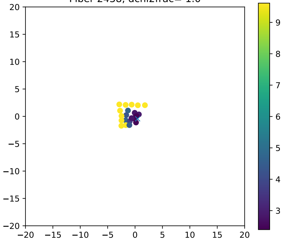
Fiber 2438, dchi2frac= 1.0
