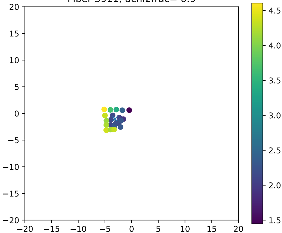
Fiber 3911, dchi2frac= 0.9
