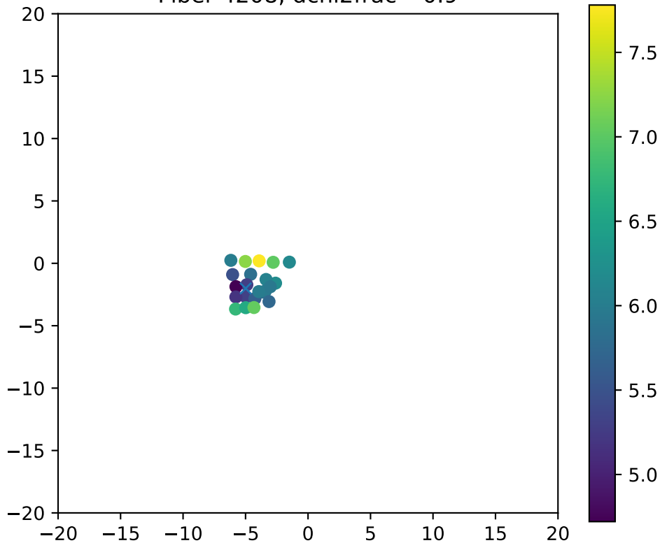
Fiber 4208, dchi2frac= 0.9
