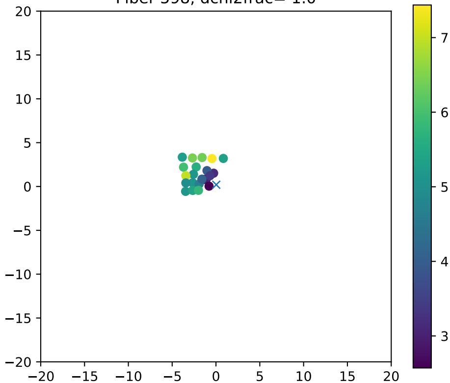
Fiber 598, dchi2frac= 1.0
