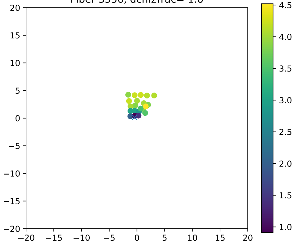
Fiber 3556, dchi2frac= 1.0
