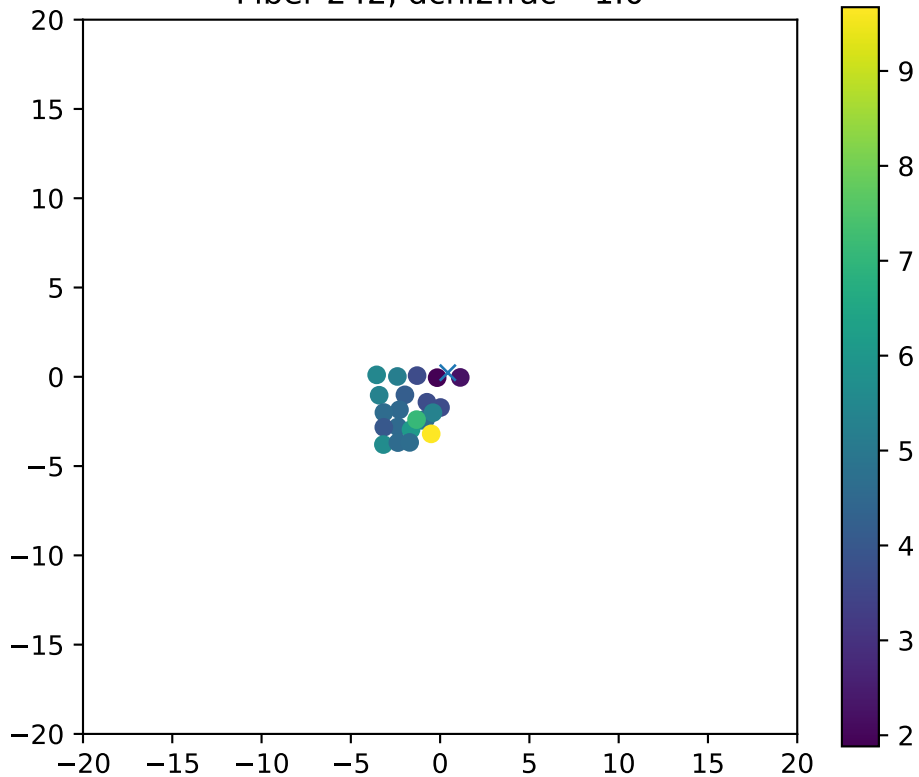
Fiber 242, dchi2frac= 1.0
