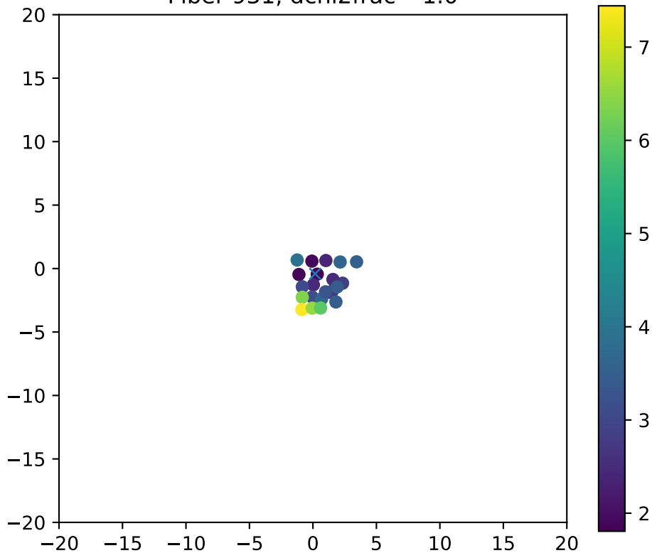
Fiber 931, dchi2frac= 1.0
