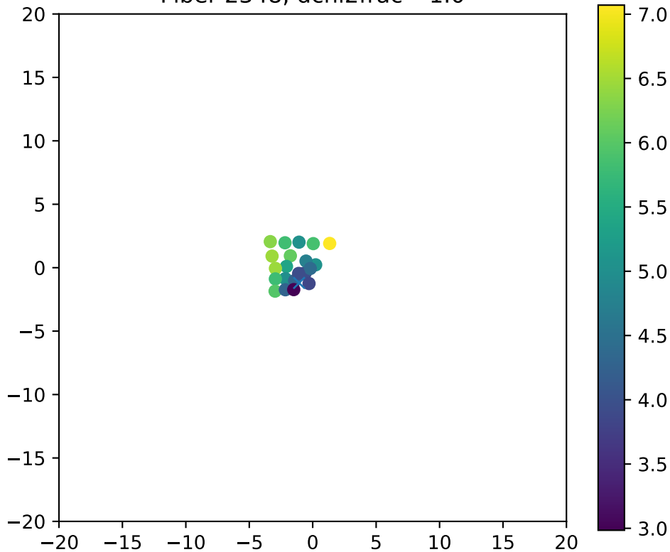
Fiber 2348, dchi2frac= 1.0
