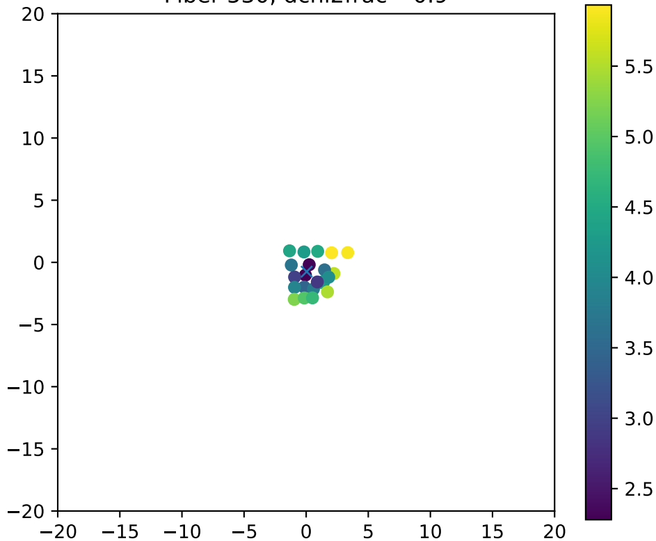
Fiber 530, dchi2frac= 0.9
