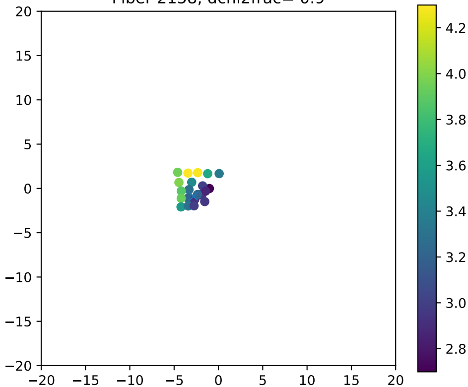
Fiber 2158, dchi2frac= 0.9
