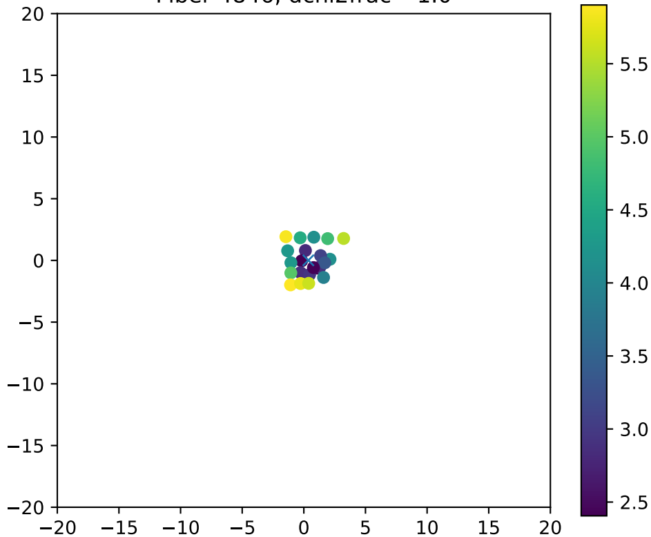
Fiber 4846, dchi2frac= 1.0
