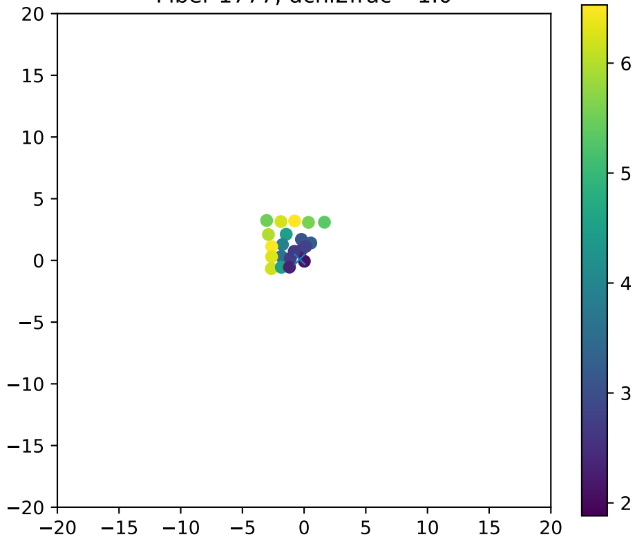
Fiber 1777, dchi2frac= 1.0
