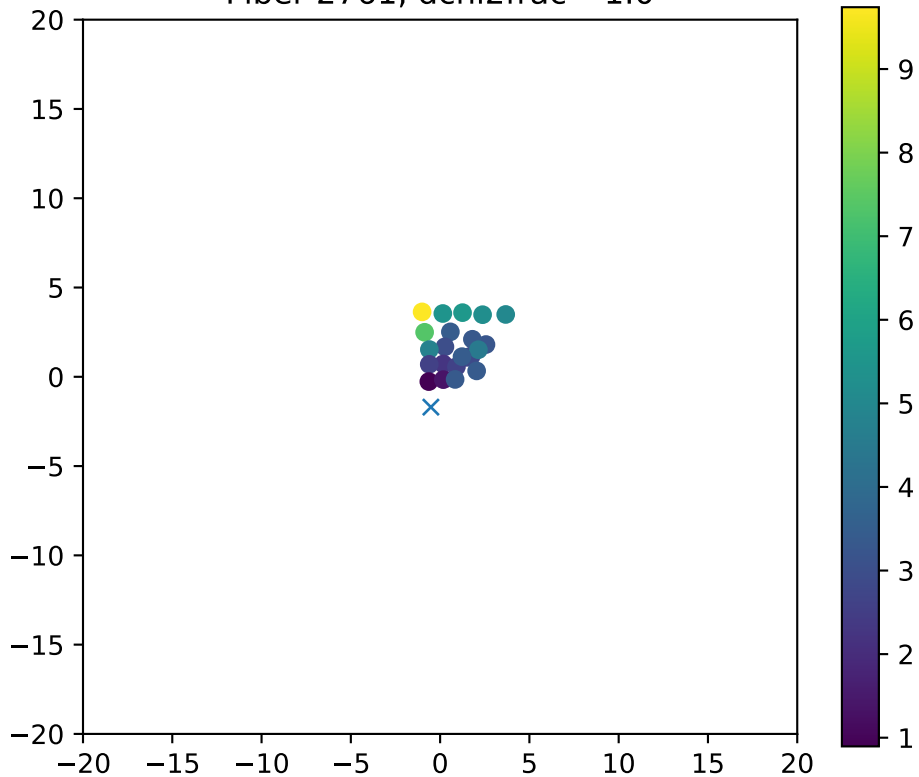
Fiber 2761, dchi2frac= 1.0
