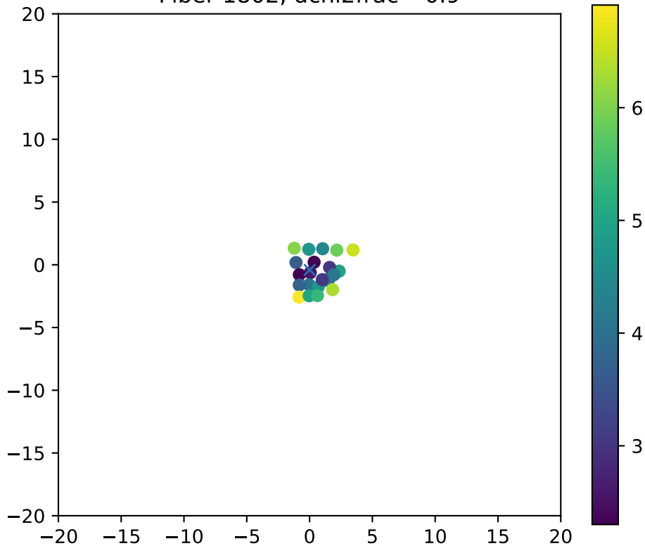
Fiber 1802, dchi2frac= 0.9
