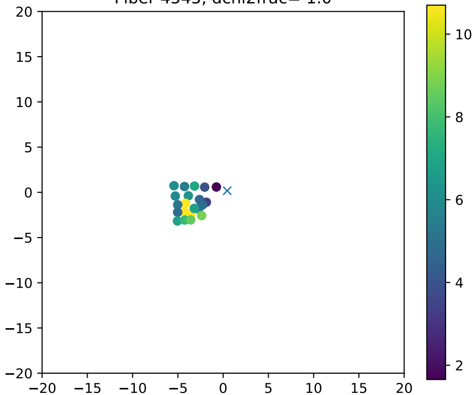
Fiber 4545, dchi2frac= 1.0
