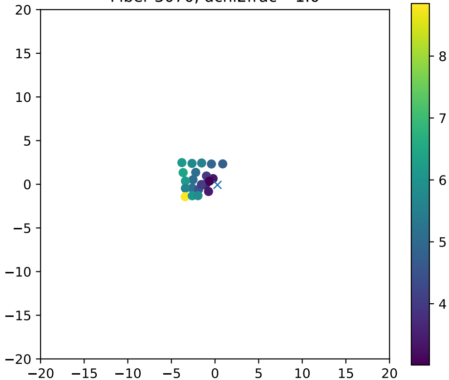
Fiber 3070, dchi2frac= 1.0
