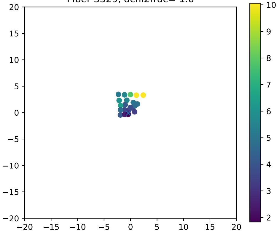
Fiber 3329, dchi2frac= 1.0
