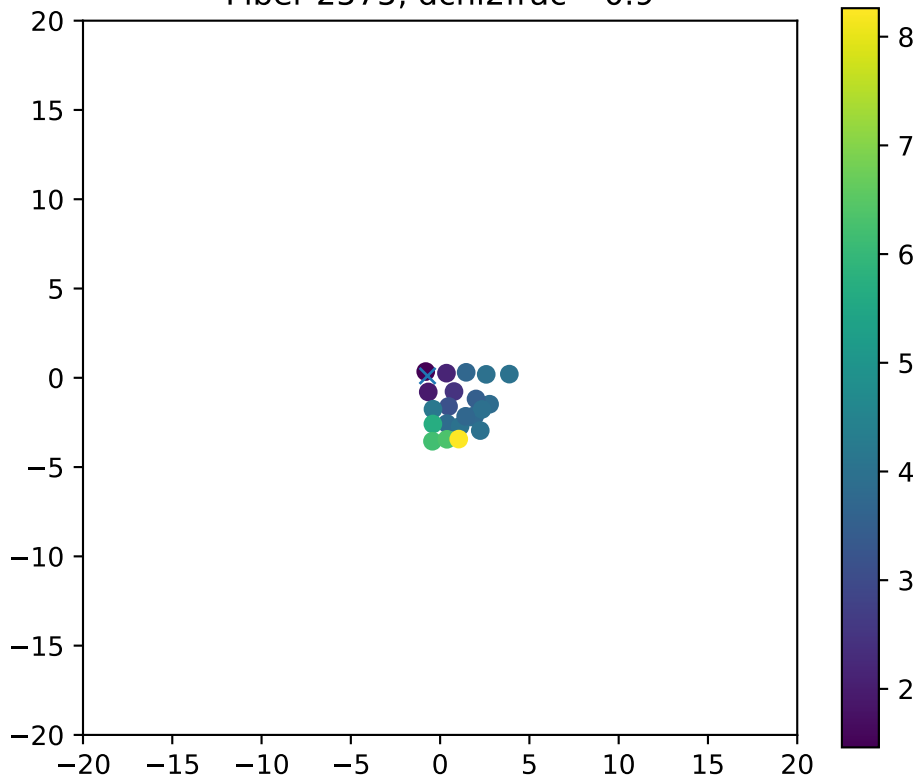
Fiber 2575, dchi2frac= 0.9
