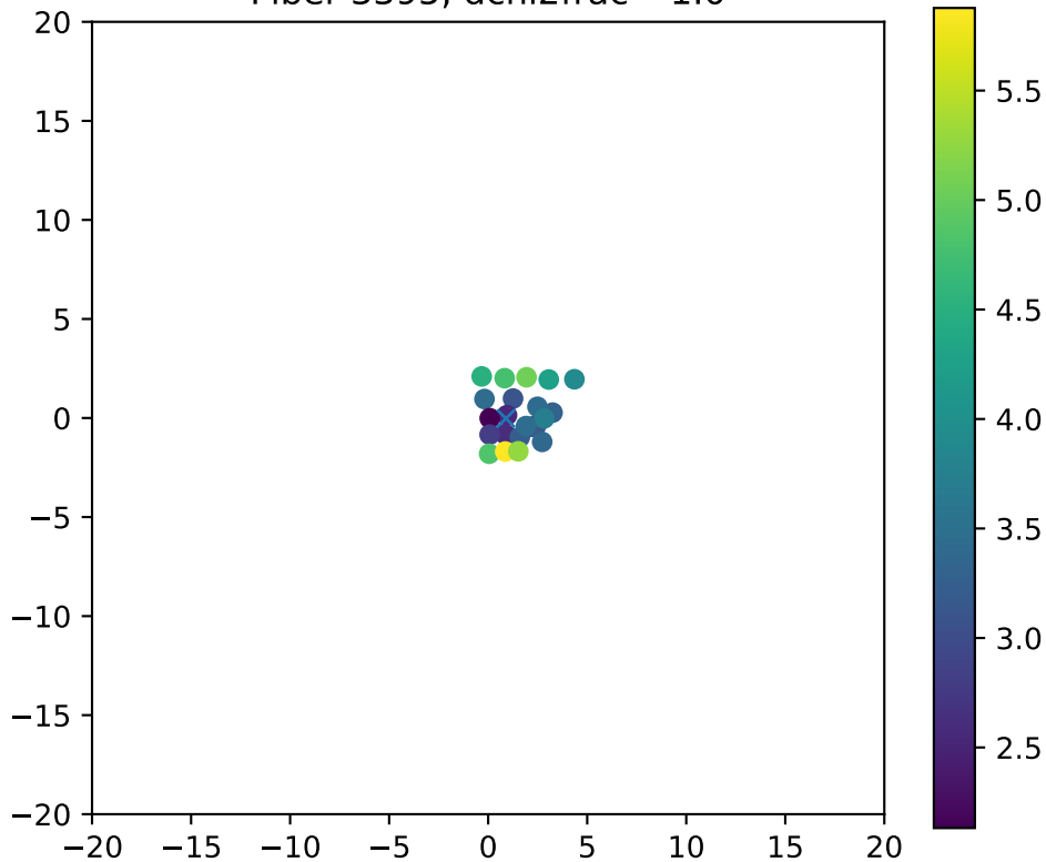
Fiber 3395, dchi2frac= 1.0
