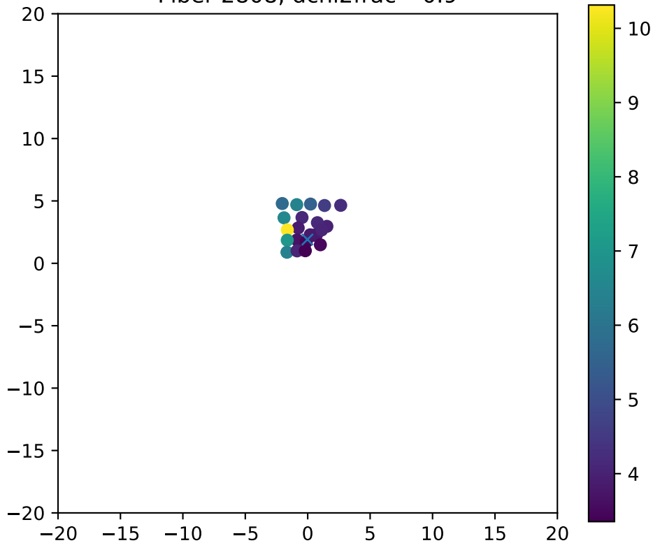
Fiber 2808, dchi2frac= 0.9
