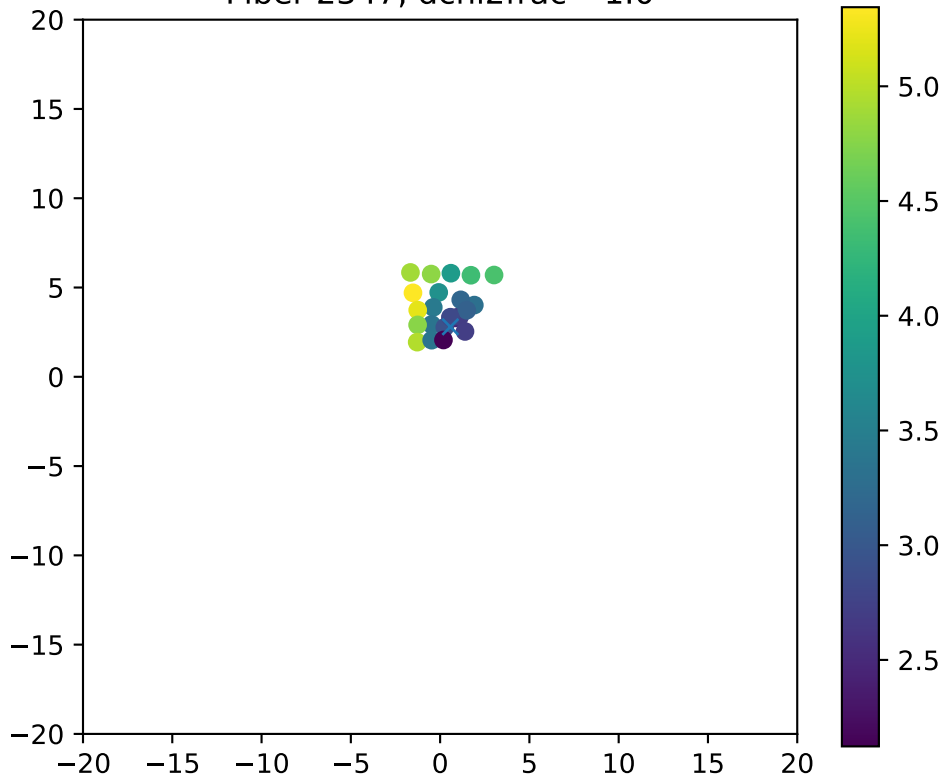
Fiber 2347, dchi2frac= 1.0
