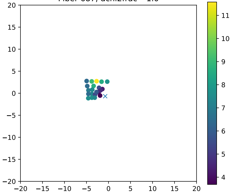
Fiber 687, dchi2frac= 1.0
