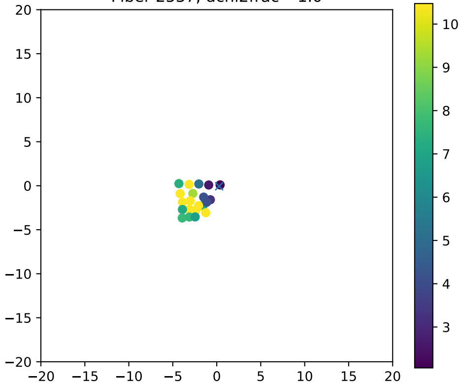
Fiber 2537, dchi2frac= 1.0
