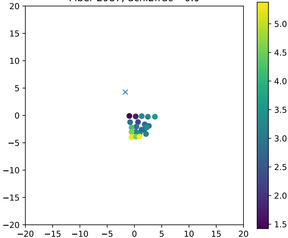
Fiber 2987, dchi2frac= 0.9
