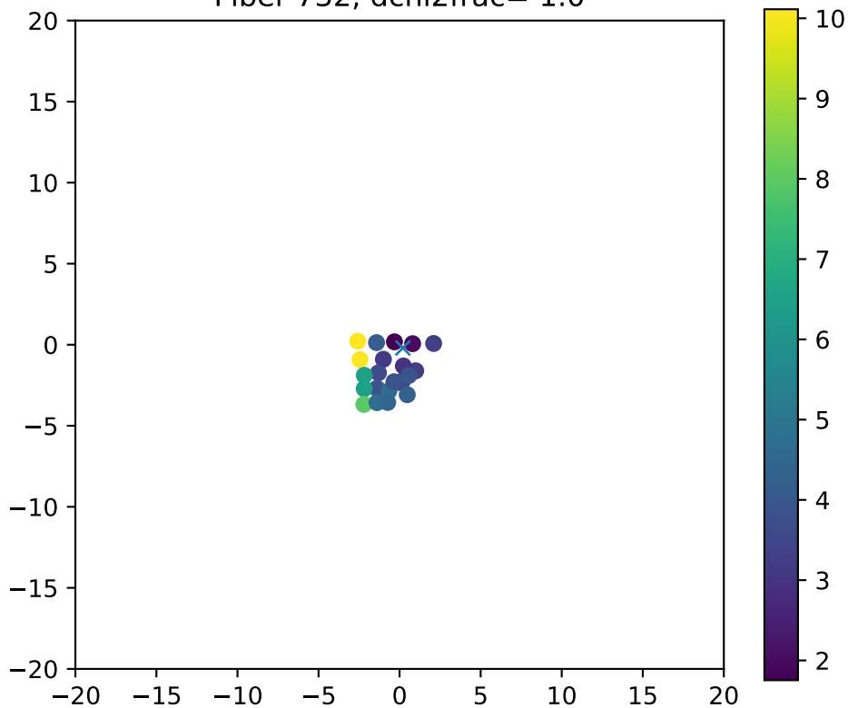
Fiber 732, dchi2frac= 1.0
