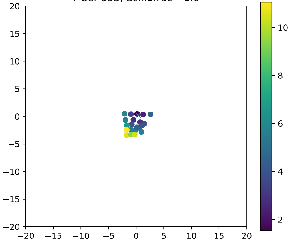
Fiber 935, dchi2frac= 1.0
