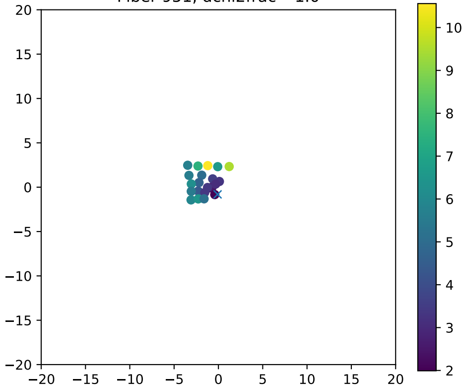
Fiber 951, dchi2frac= 1.0
