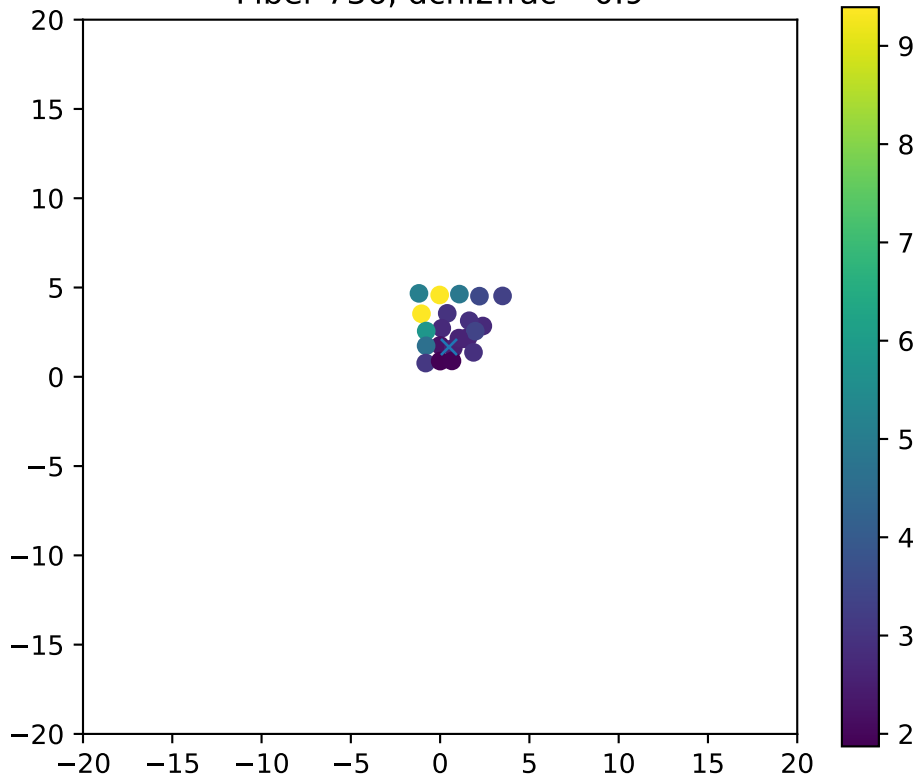
Fiber 736, dchi2frac= 0.9
