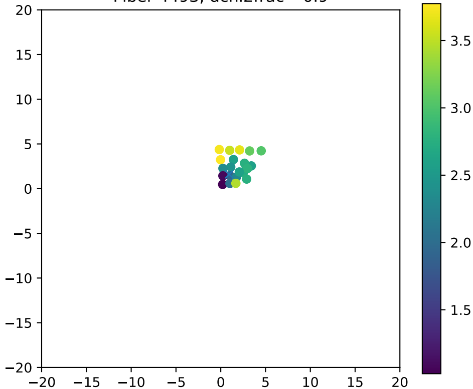
Fiber 4493, dchi2frac= 0.9
