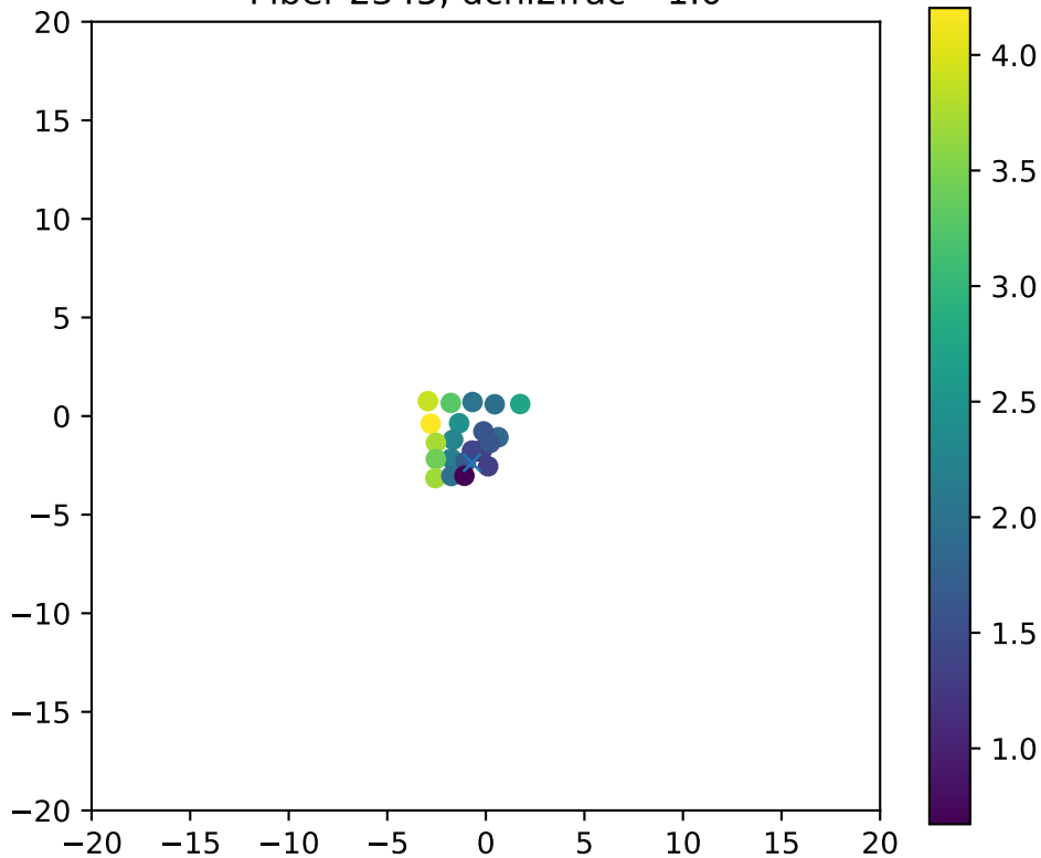
Fiber 2345, dchi2frac= 1.0
