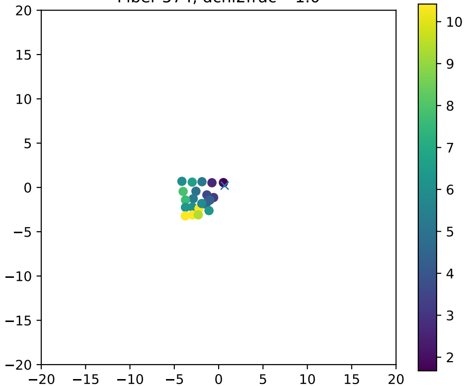
Fiber 574, dchi2frac= 1.0
