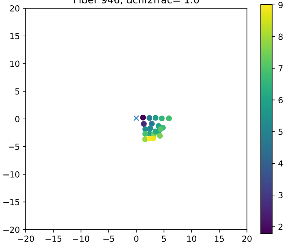
Fiber 946, dchi2frac= 1.0
