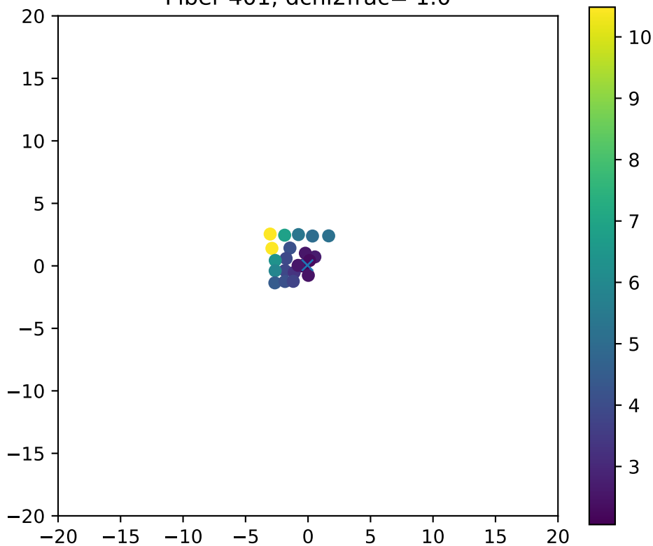
Fiber 401, dchi2frac= 1.0
