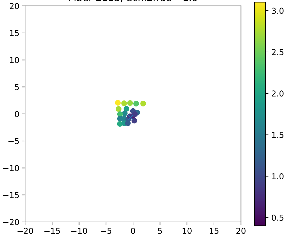
Fiber 2113, dchi2frac= 1.0
