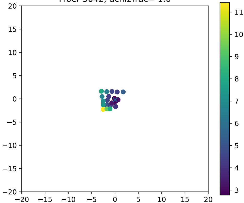
Fiber 3042, dchi2frac= 1.0
