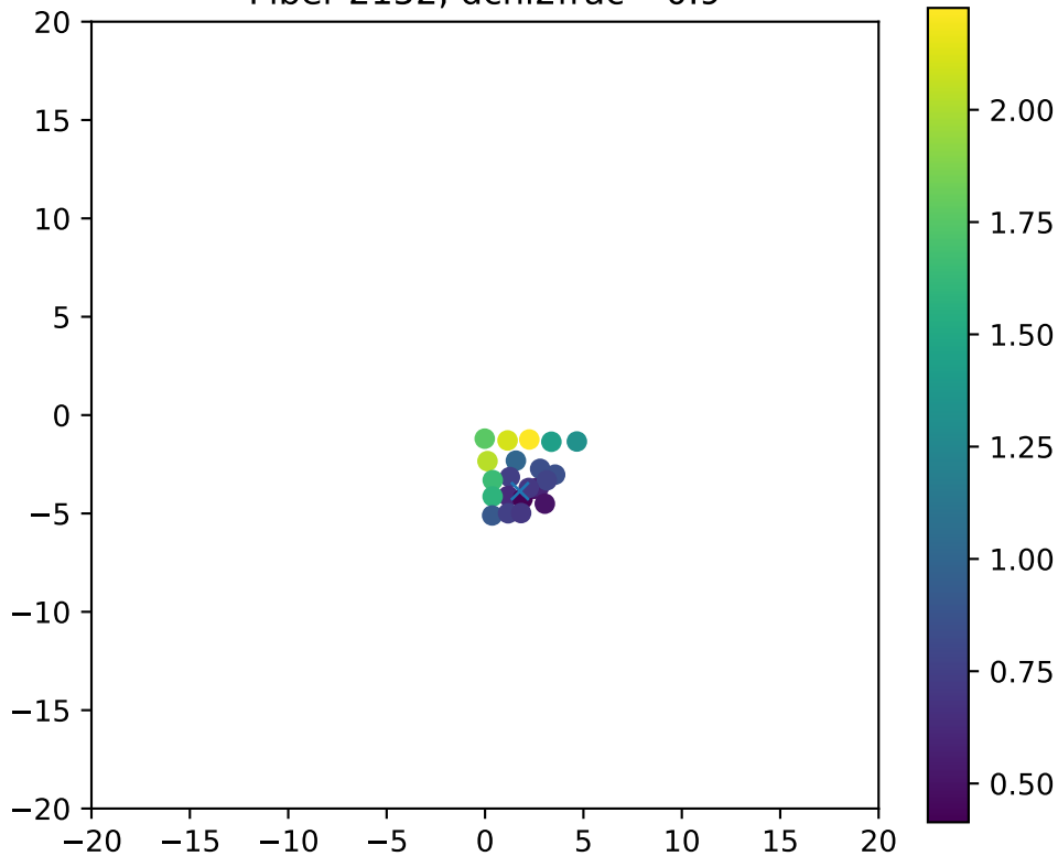
Fiber 2152, dchi2frac= 0.9
