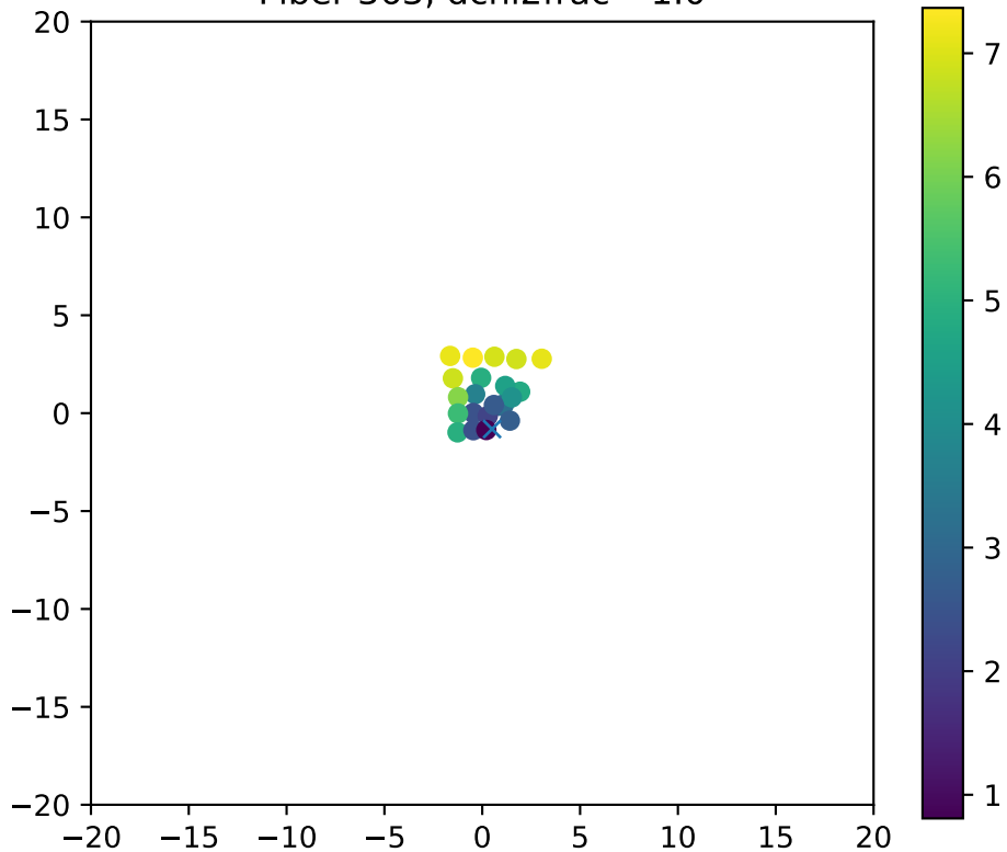
Fiber 363, dchi2frac= 1.0
