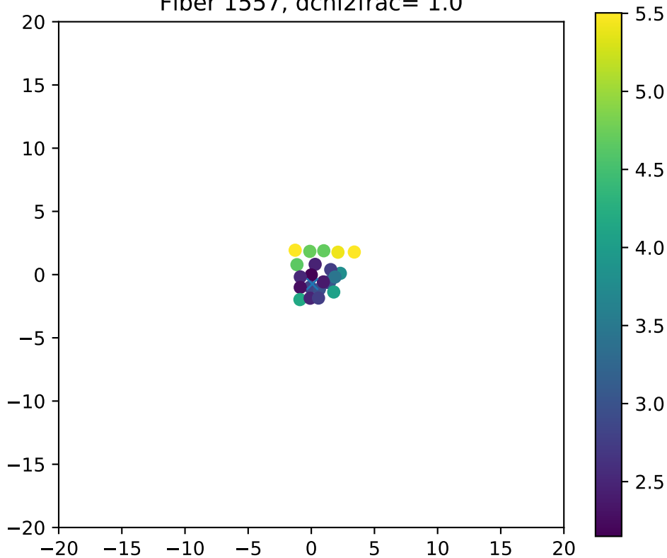
Fiber 1557, dchi2frac= 1.0
