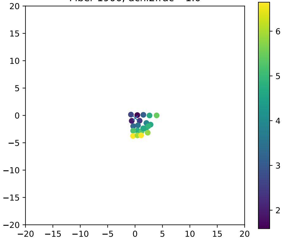
Fiber 1906, dchi2frac= 1.0
