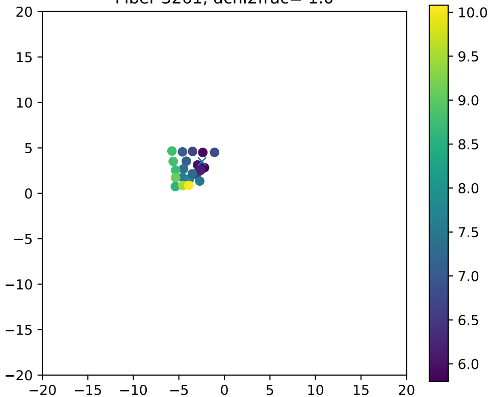
Fiber 3261, dchi2frac= 1.0
