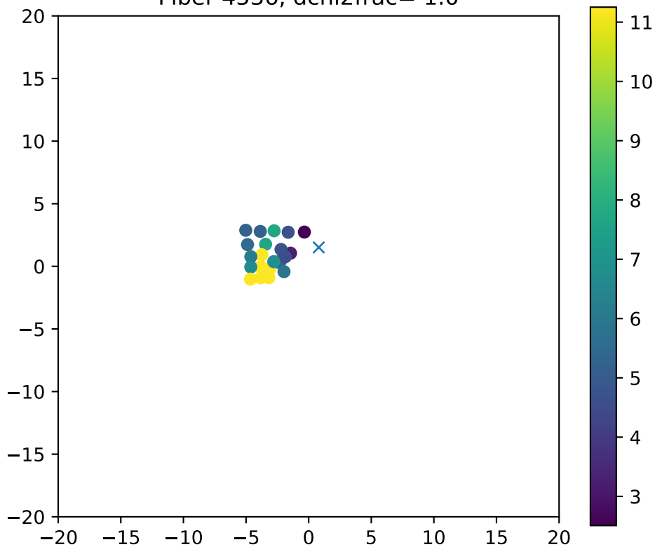
Fiber 4536, dchi2frac= 1.0
