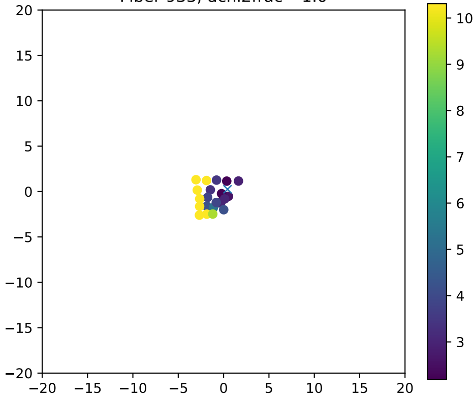
Fiber 933, dchi2frac= 1.0
