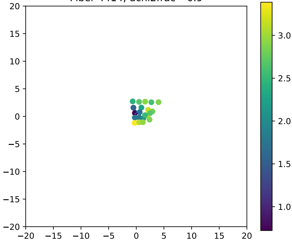
Fiber 4414, dchi2frac= 0.9
