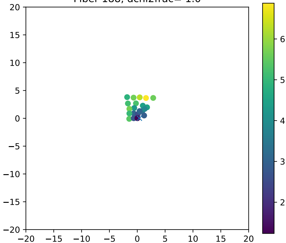
Fiber 188, dchi2frac= 1.0
