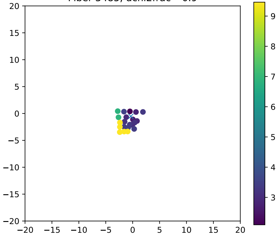
Fiber 3485, dchi2frac= 0.9
