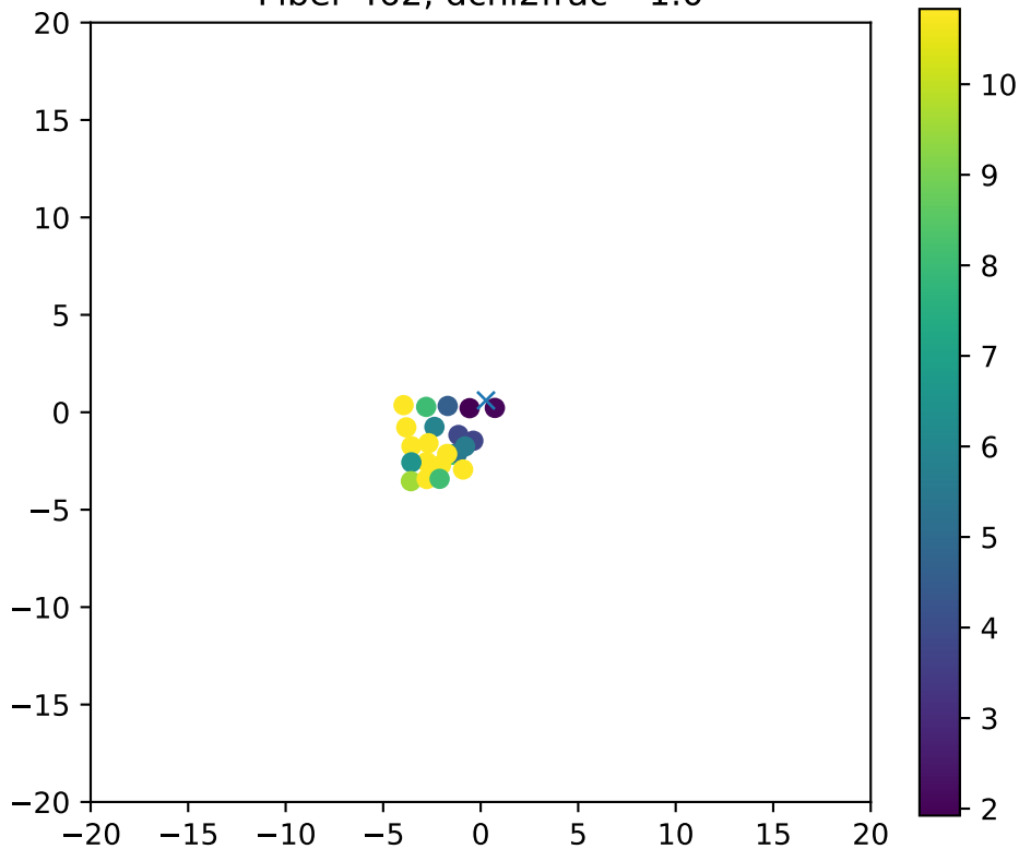
Fiber 462, dchi2frac= 1.0
