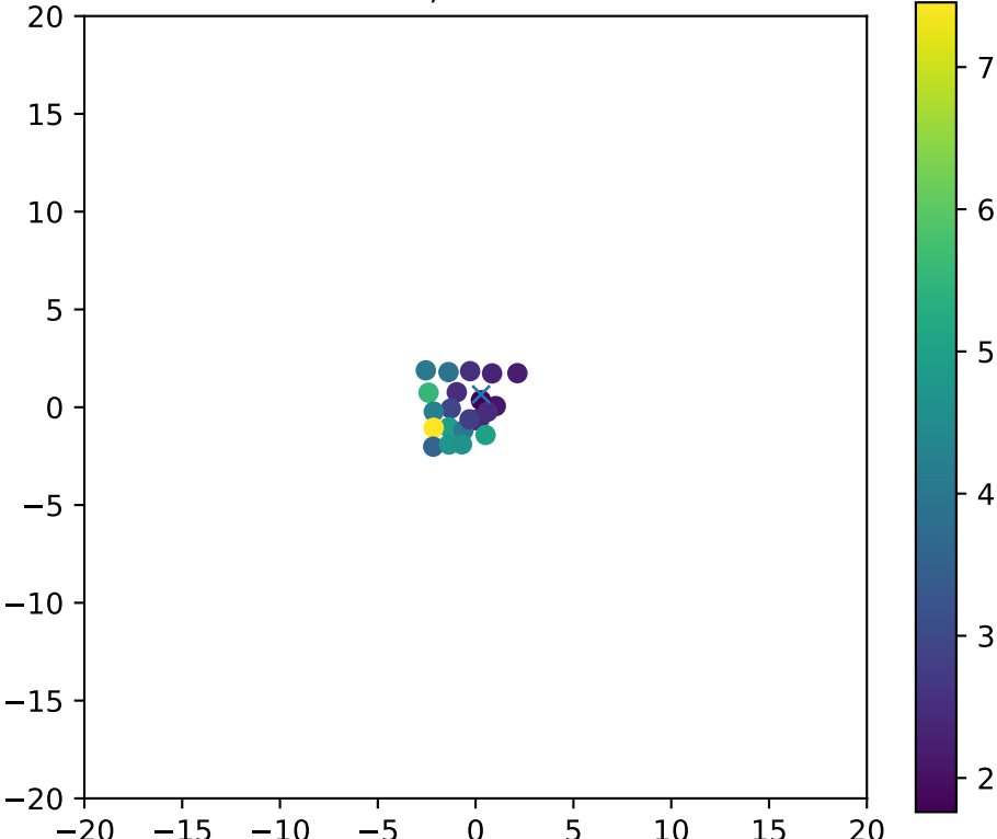
Fiber 4572, dchi2frac= 1.0
