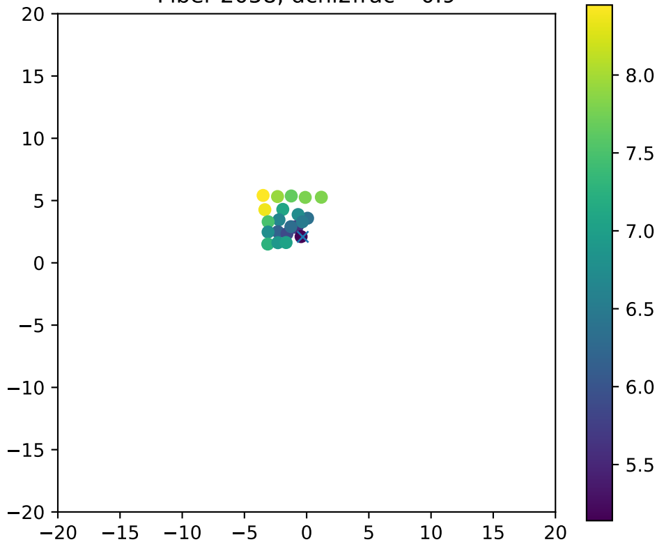
Fiber 2058, dchi2frac= 0.9
