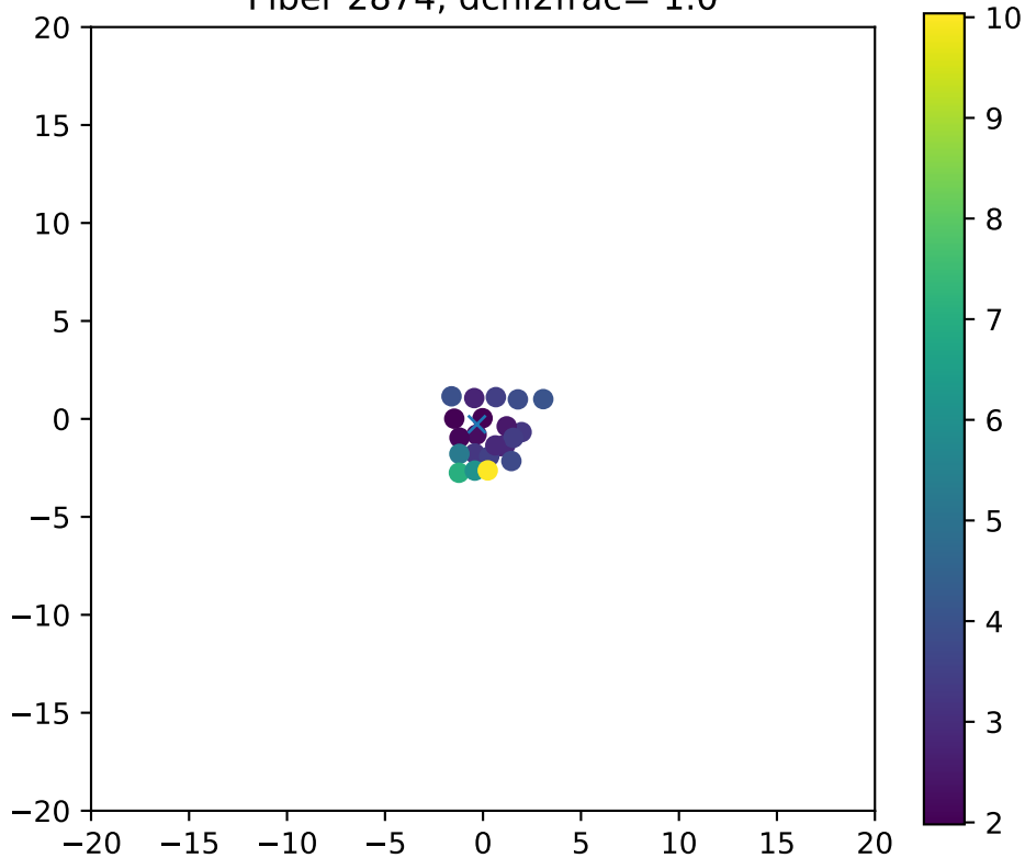
Fiber 2874, dchi2frac= 1.0
