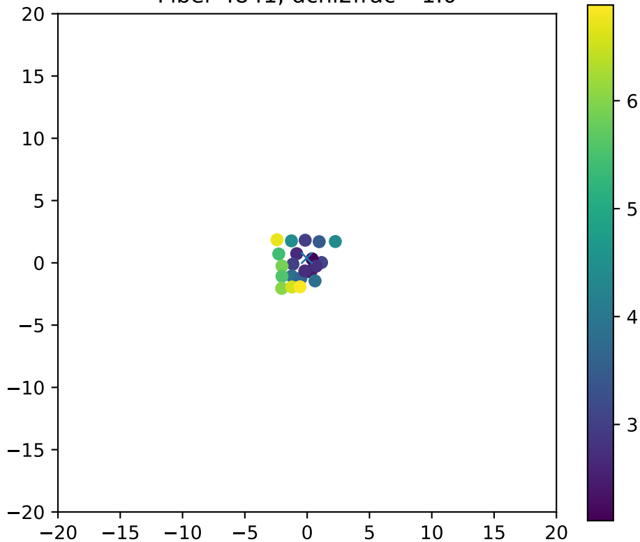
Fiber 4841, dchi2frac= 1.0
