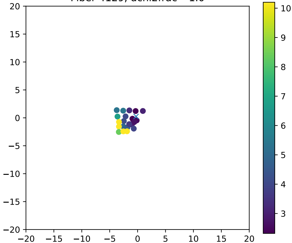
Fiber 4129, dchi2frac= 1.0
