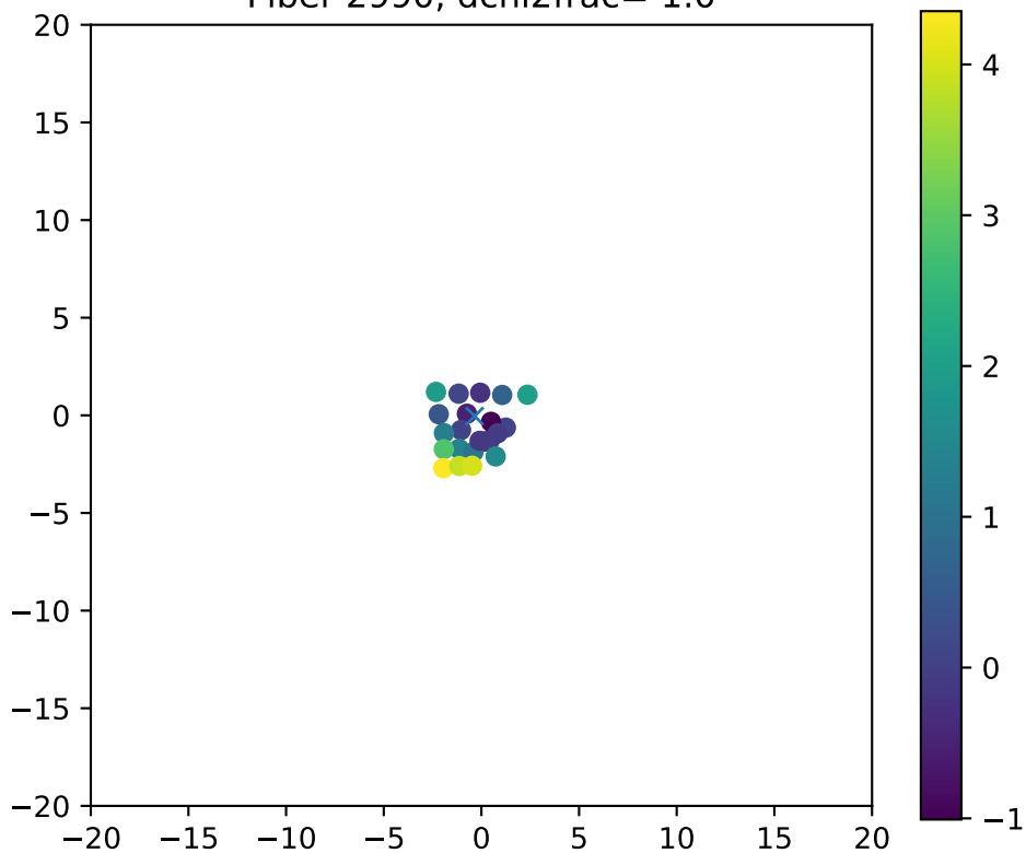
Fiber 2990, dchi2frac= 1.0
