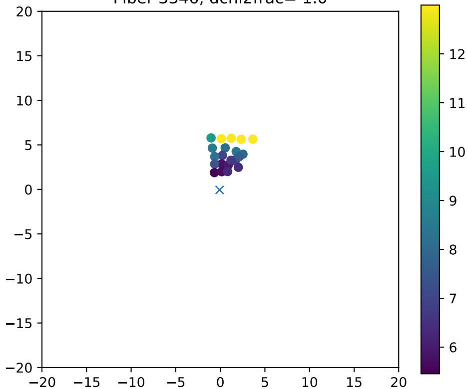
Fiber 3346, dchi2frac= 1.0
