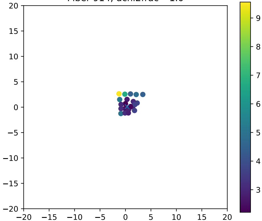
Fiber 914, dchi2frac= 1.0
