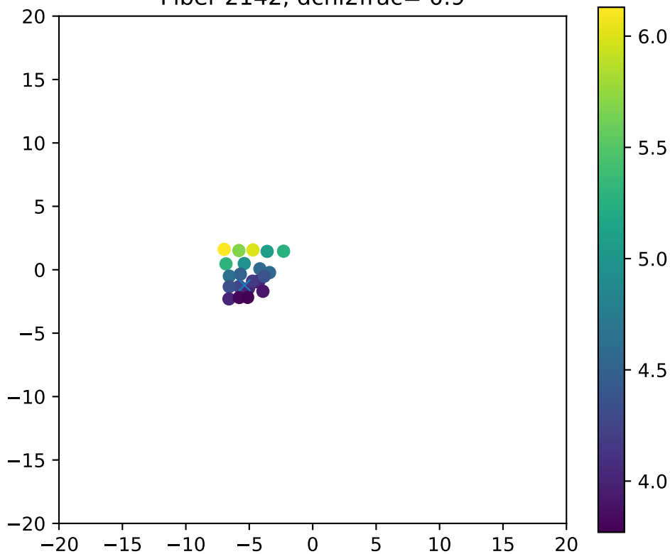
Fiber 2142, dchi2frac= 0.9
