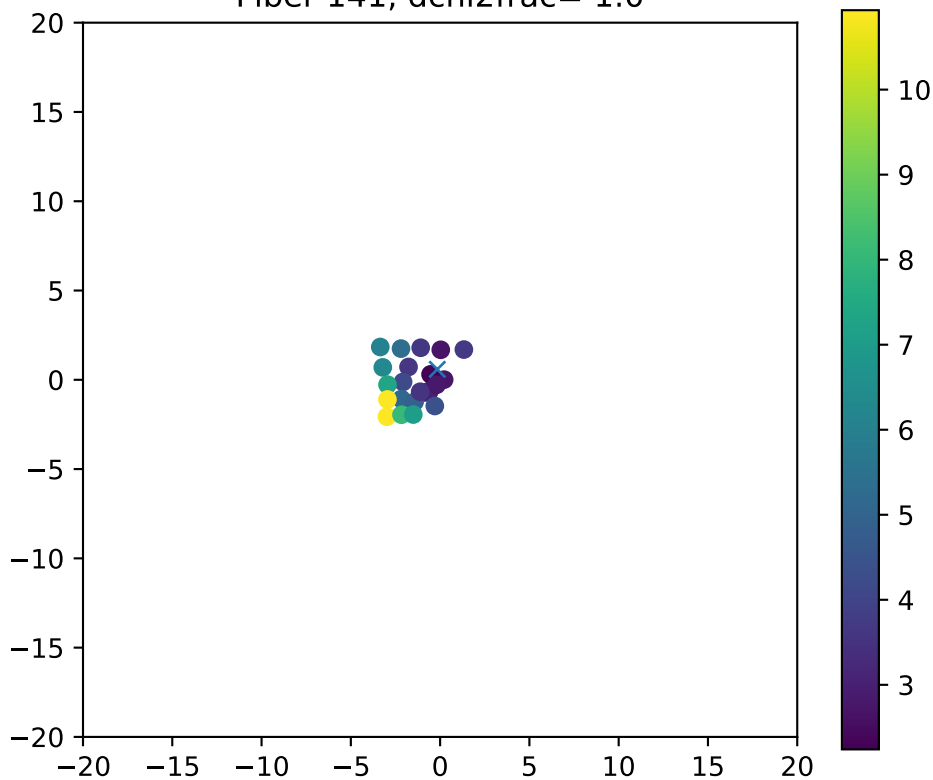
Fiber 141, dchi2frac= 1.0
