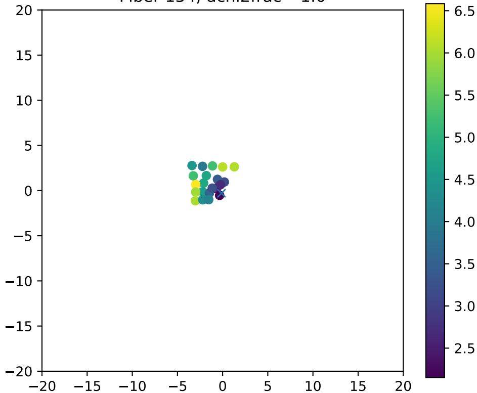
Fiber 154, dchi2frac= 1.0
