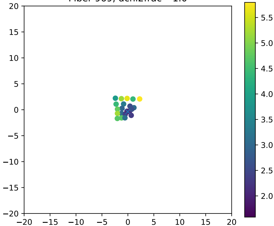
Fiber 969, dchi2frac= 1.0
