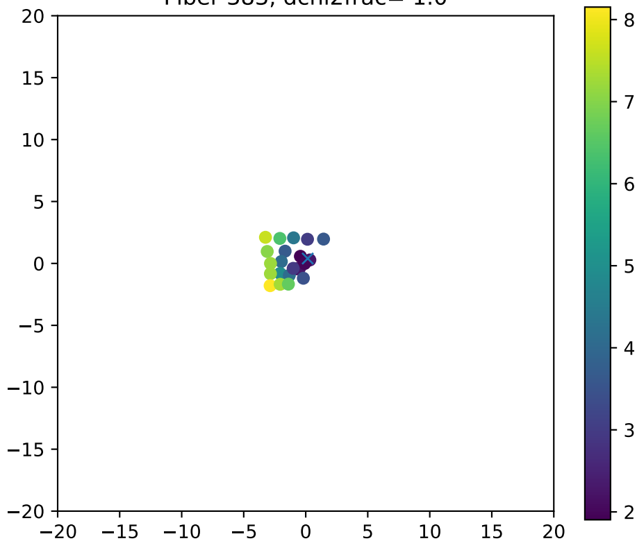
Fiber 383, dchi2frac= 1.0
