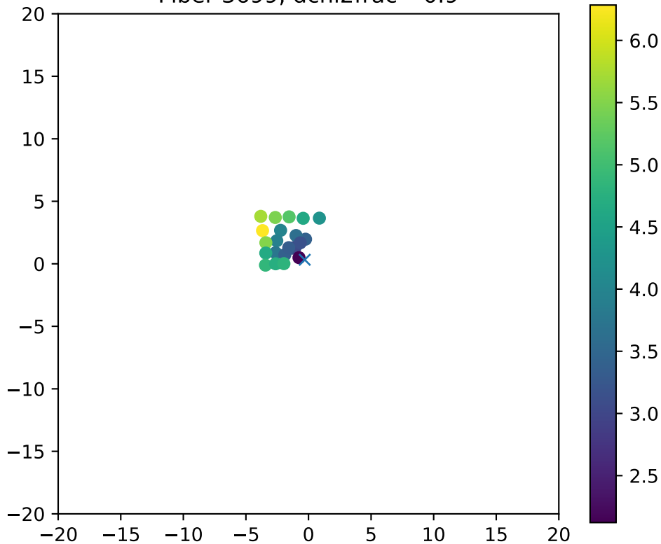
Fiber 3699, dchi2frac= 0.9
