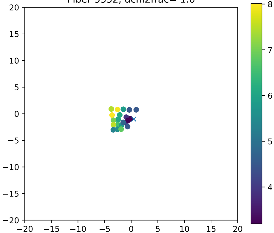
Fiber 3352, dchi2frac= 1.0
