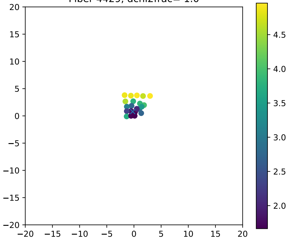
Fiber 4429, dchi2frac= 1.0
