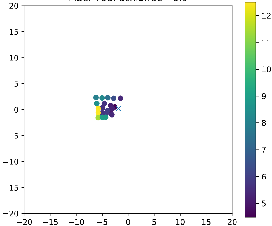
Fiber 756, dchi2frac= 0.9
