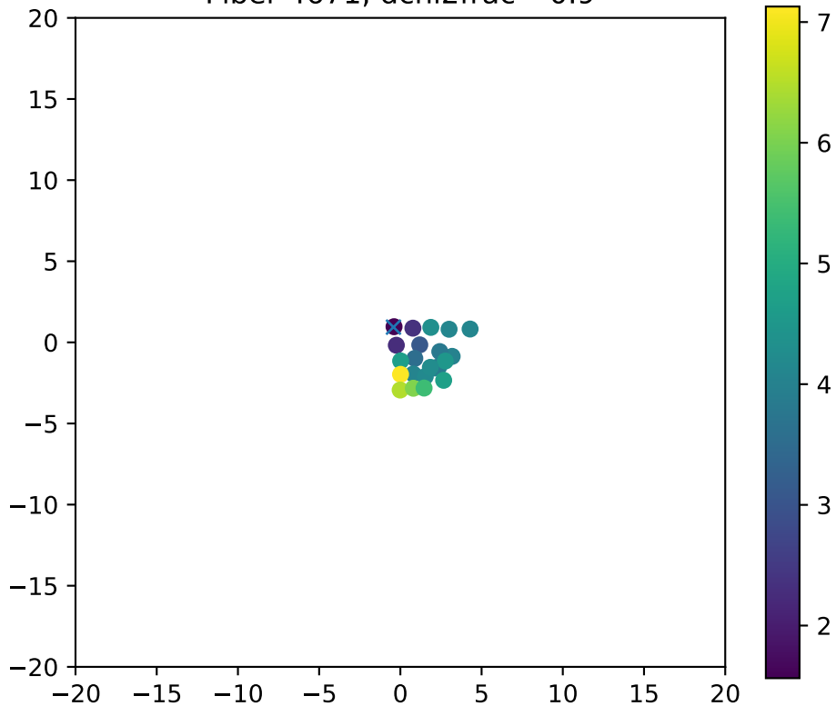
Fiber 4671, dchi2frac= 0.9
