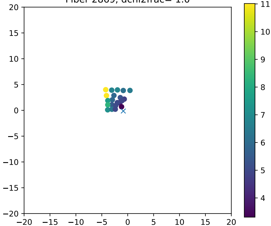
Fiber 2869, dchi2frac= 1.0
