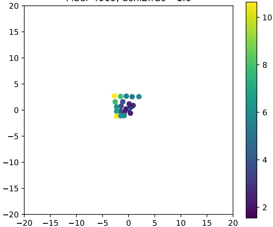
Fiber 4069, dchi2frac= 1.0
