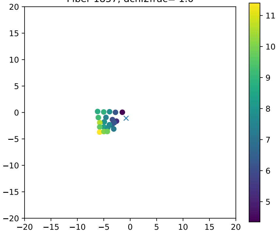
Fiber 1857, dchi2frac= 1.0
