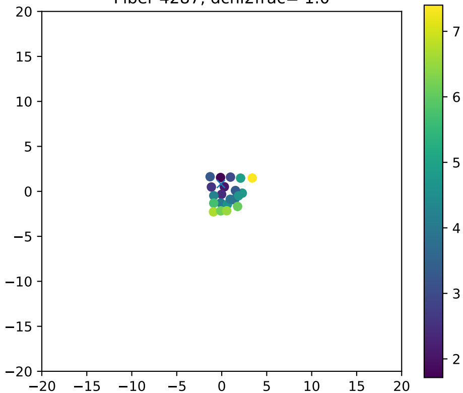
Fiber 4287, dchi2frac= 1.0
