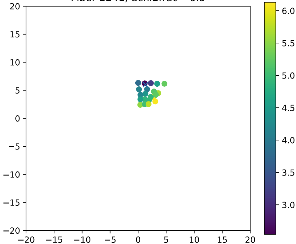
Fiber 2241, dchi2frac= 0.9
