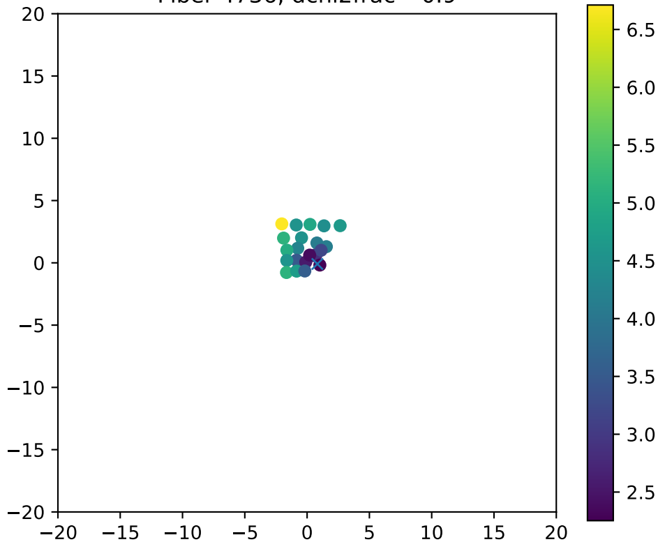
Fiber 4736, dchi2frac= 0.9
