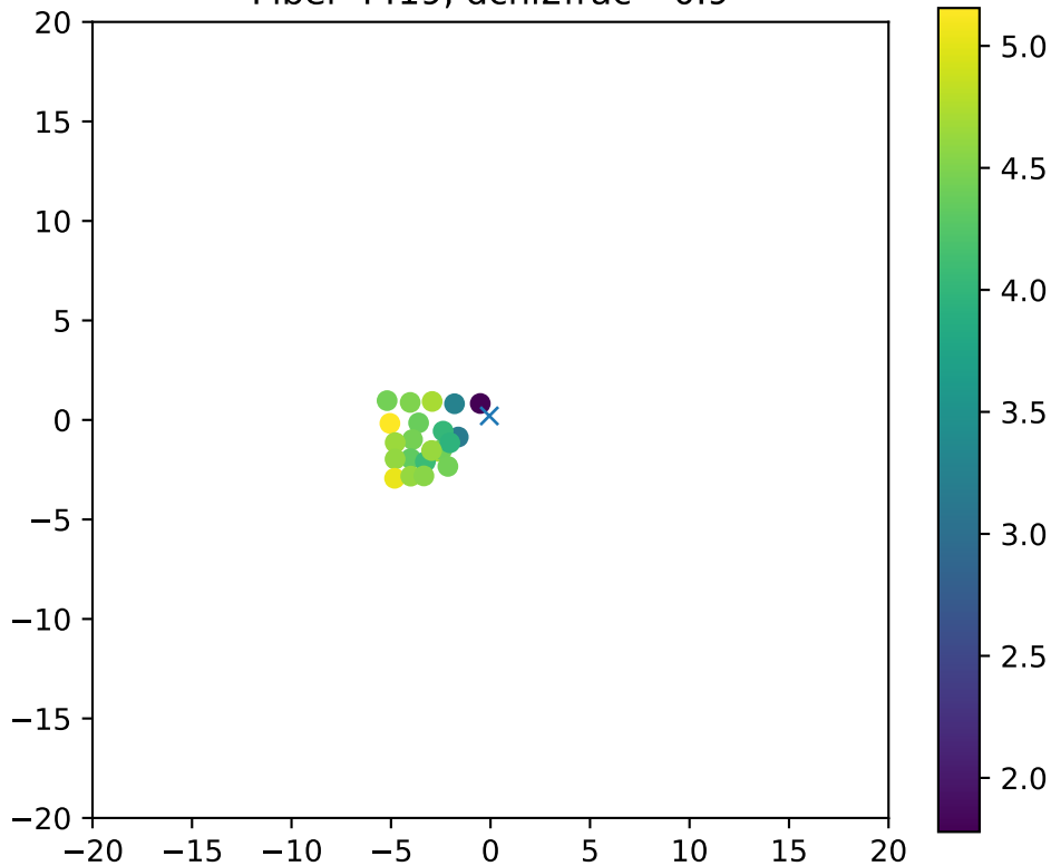
Fiber 4419, dchi2frac= 0.9
