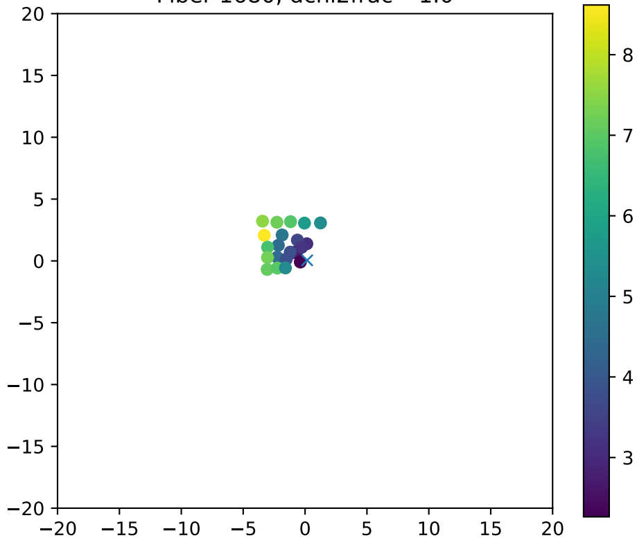
Fiber 1680, dchi2frac= 1.0
