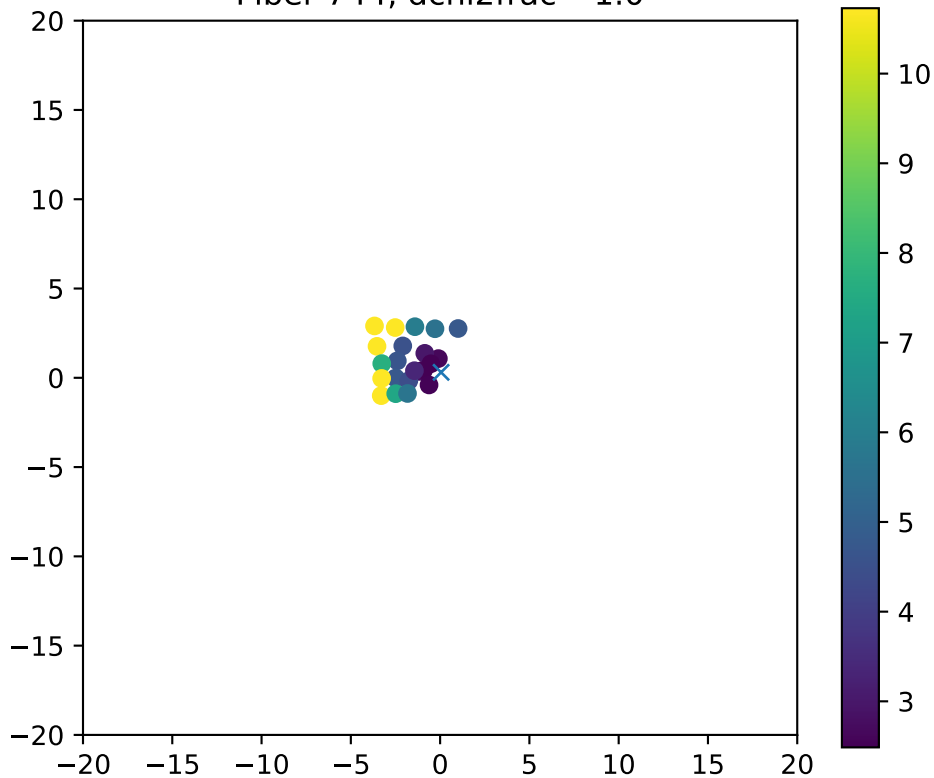
Fiber 744, dchi2frac= 1.0
