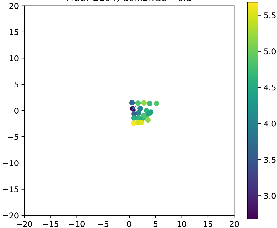
Fiber 2194, dchi2frac= 0.9
