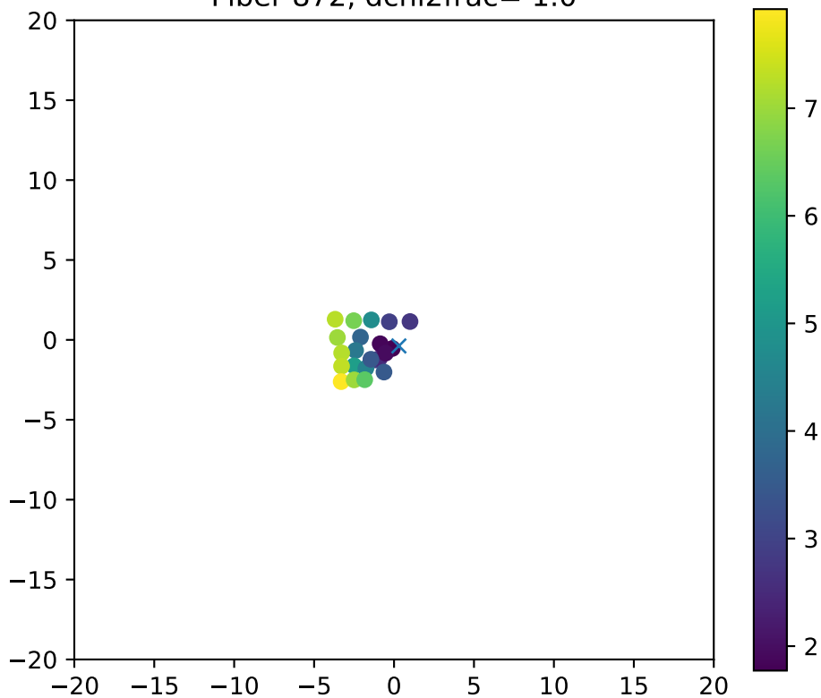
Fiber 872, dchi2frac= 1.0
