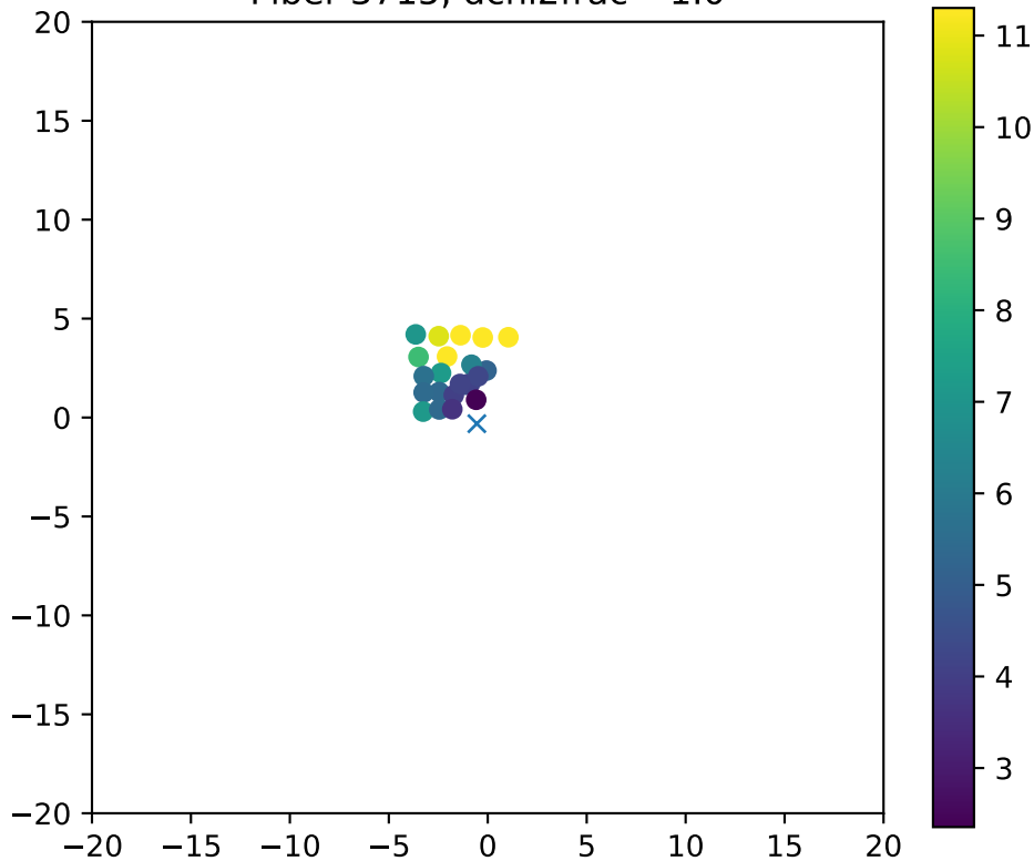
Fiber 3715, dchi2frac= 1.0
