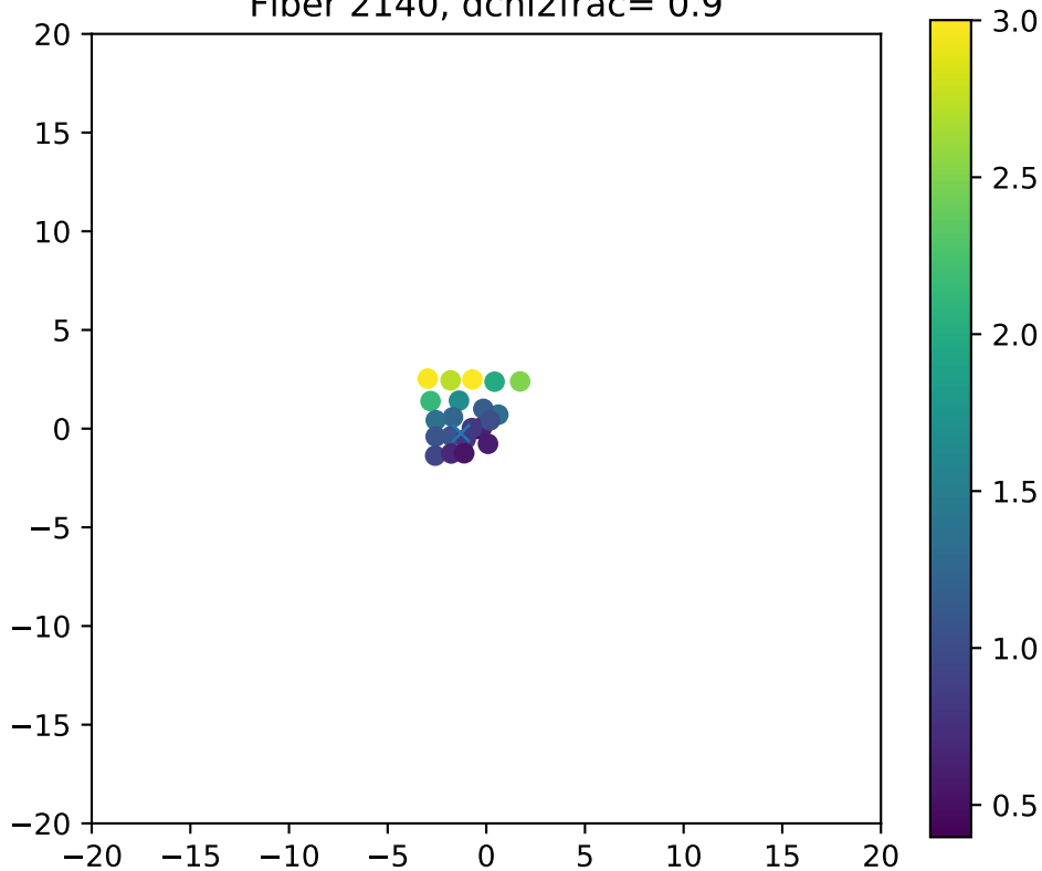
Fiber 2140, dchi2frac= 0.9
