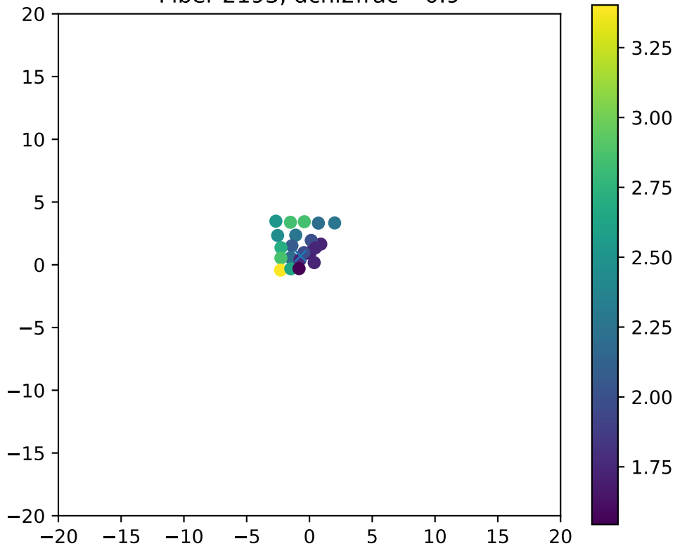
Fiber 2193, dchi2frac= 0.9
