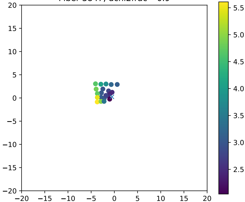
Fiber 3847, dchi2frac= 0.9
