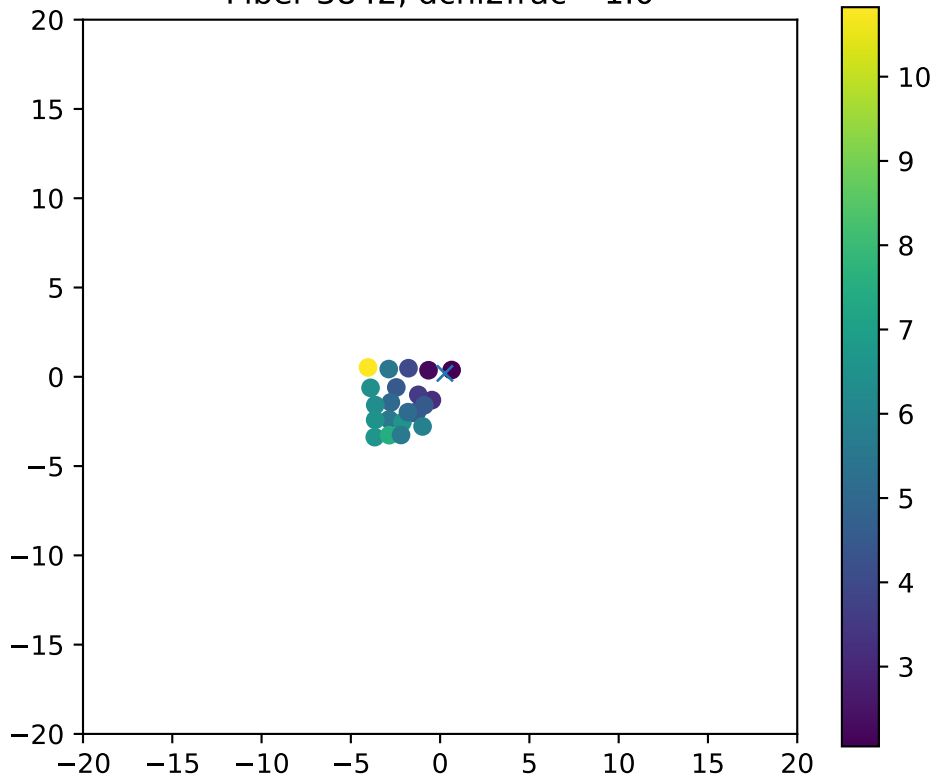
Fiber 3842, dchi2frac= 1.0
