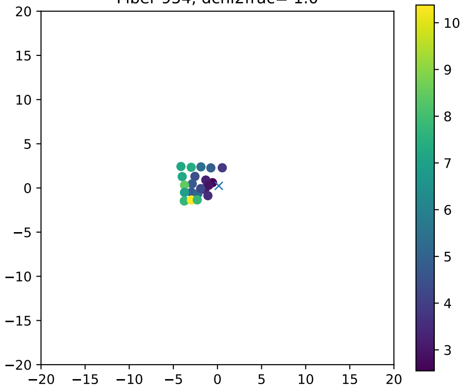
Fiber 954, dchi2frac= 1.0
