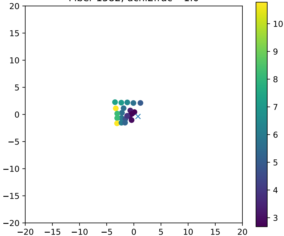
Fiber 1582, dchi2frac= 1.0
