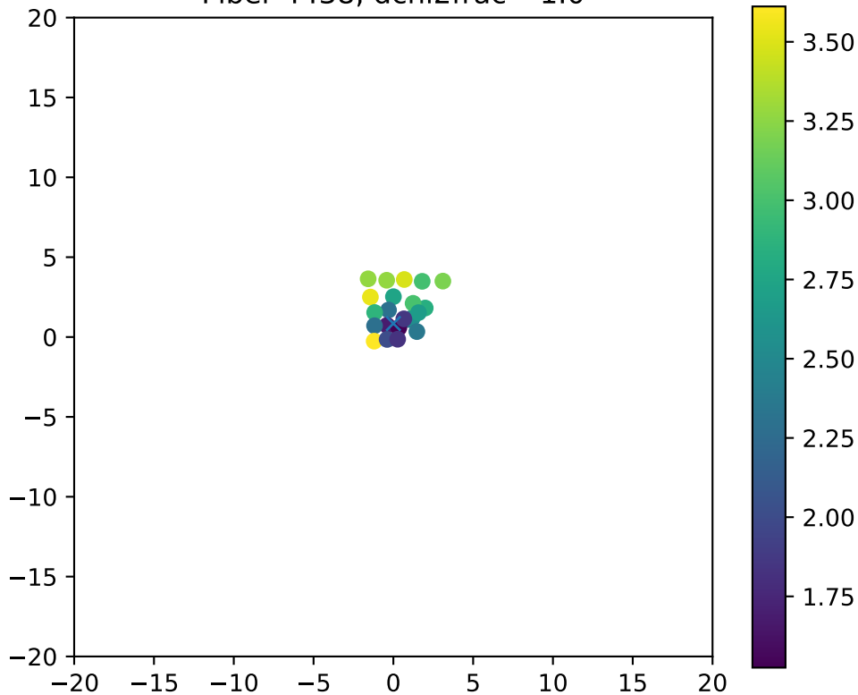
Fiber 4438, dchi2frac= 1.0
