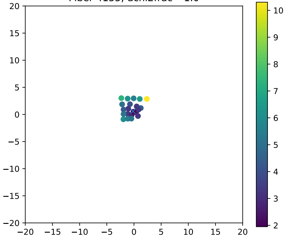
Fiber 4155, dchi2frac= 1.0
