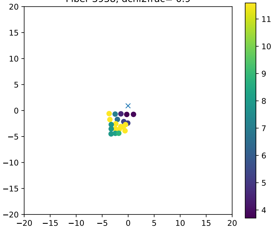
Fiber 3938, dchi2frac= 0.9
