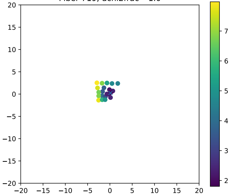
Fiber 719, dchi2frac= 1.0
