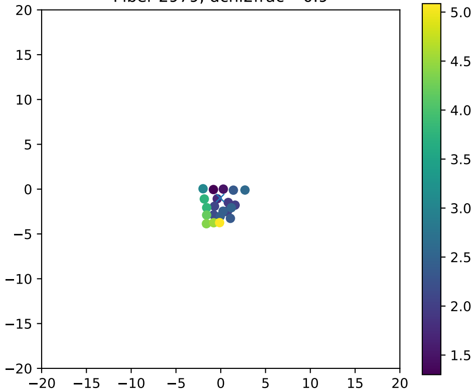
Fiber 2979, dchi2frac= 0.9
