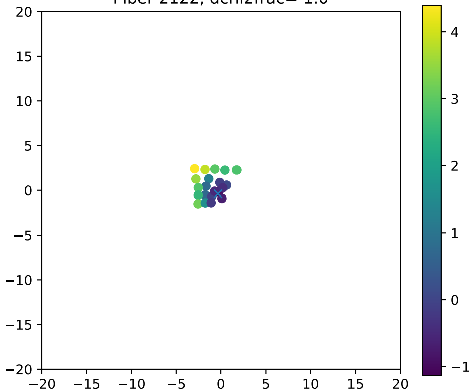
Fiber 2122, dchi2frac= 1.0
