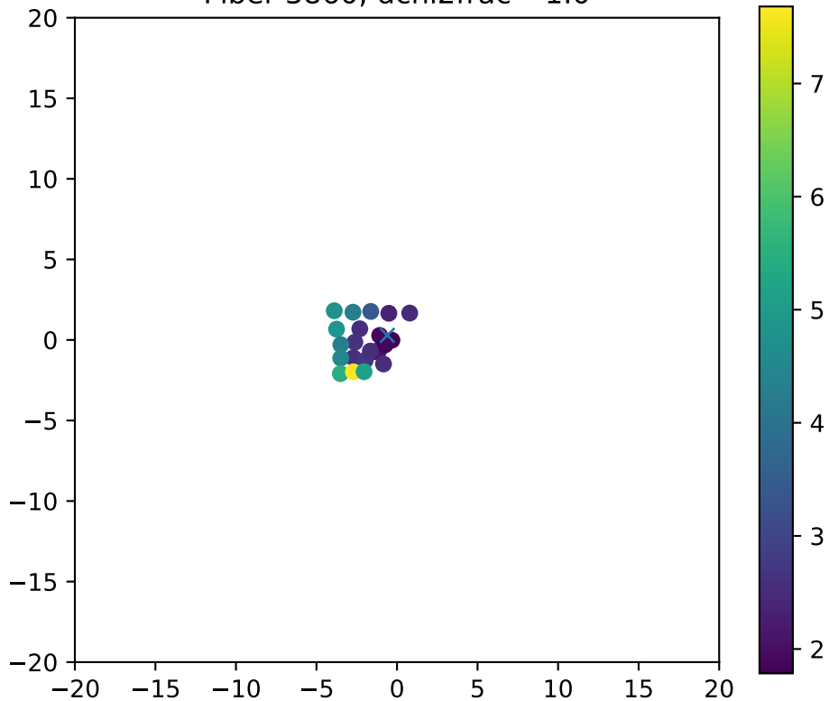
Fiber 3860, dchi2frac= 1.0
