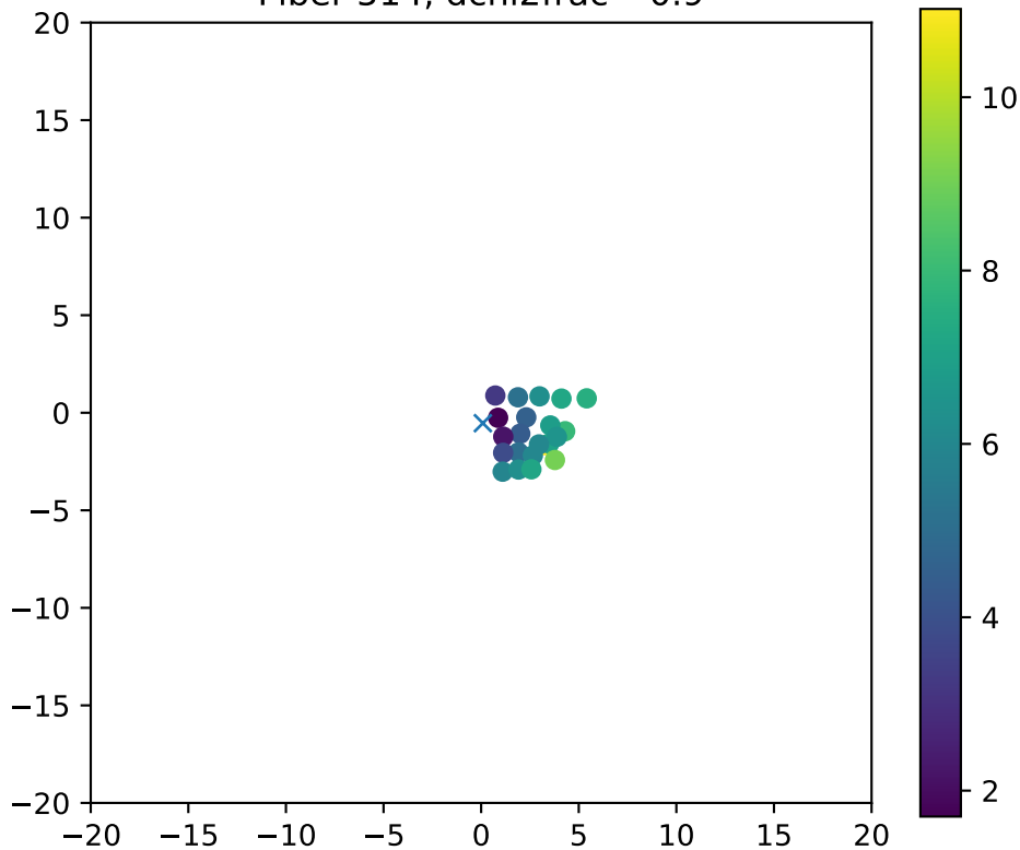
Fiber 514, dchi2frac= 0.9
