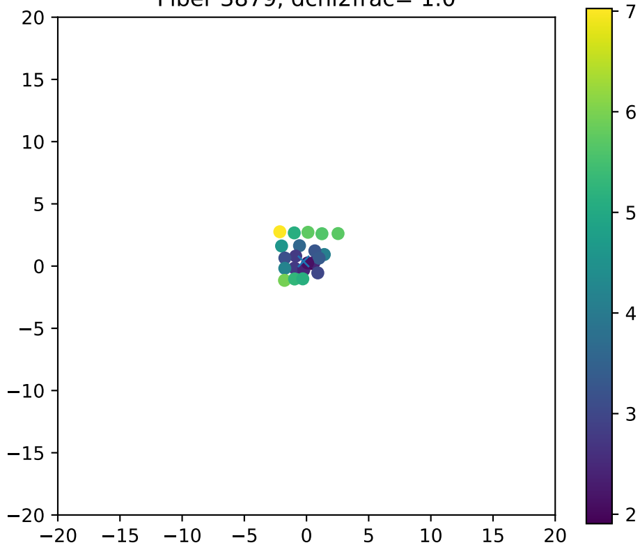
Fiber 3879, dchi2frac= 1.0
