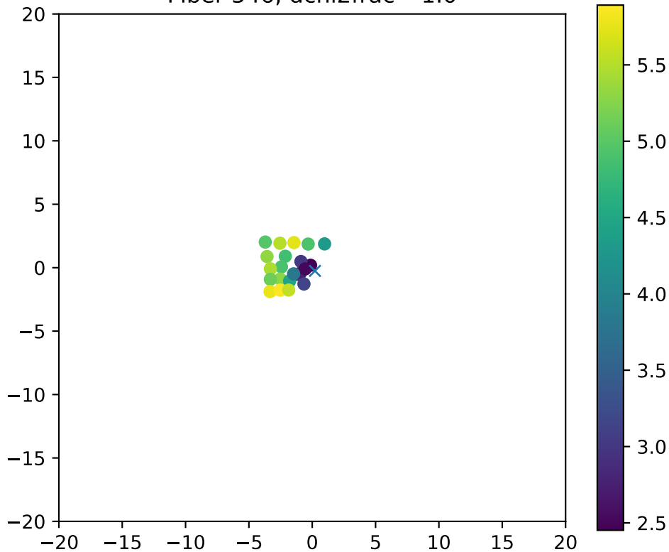
Fiber 546, dchi2frac= 1.0
