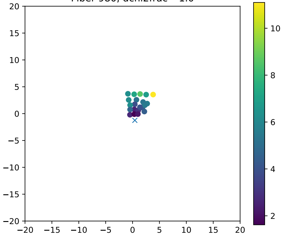
Fiber 980, dchi2frac= 1.0
