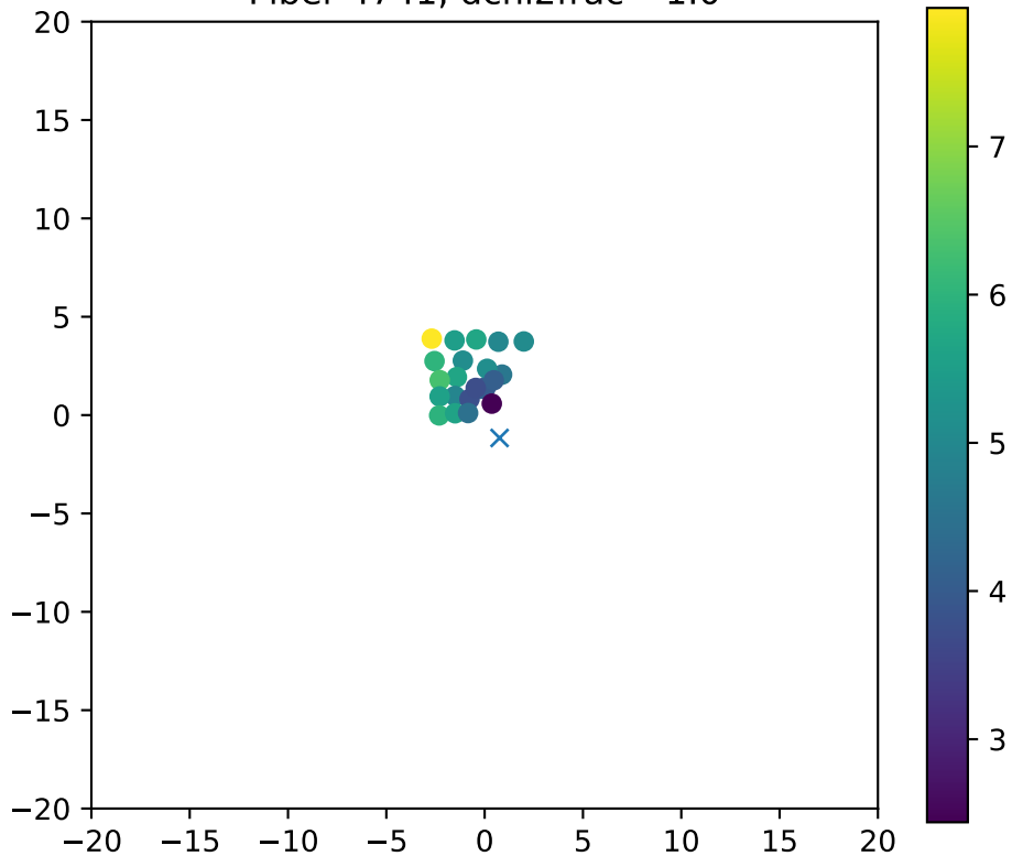
Fiber 4741, dchi2frac= 1.0
