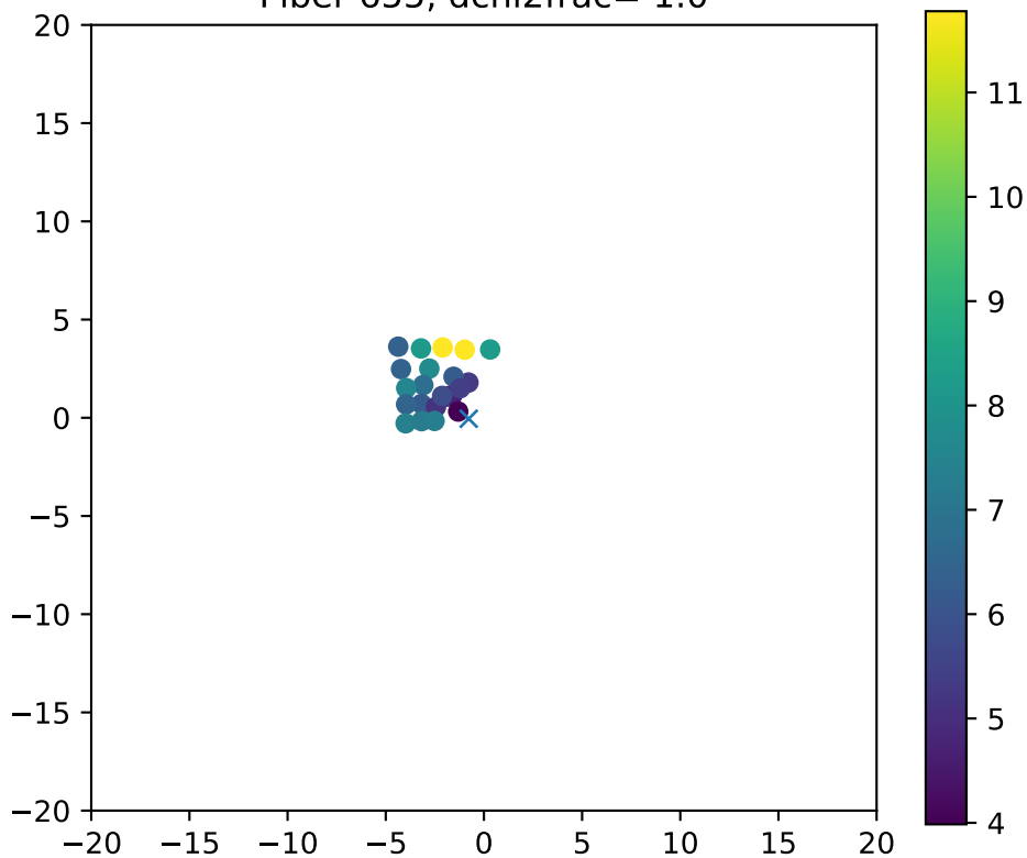
Fiber 655, dchi2frac= 1.0
