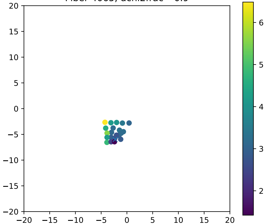
Fiber 4065, dchi2frac= 0.9
