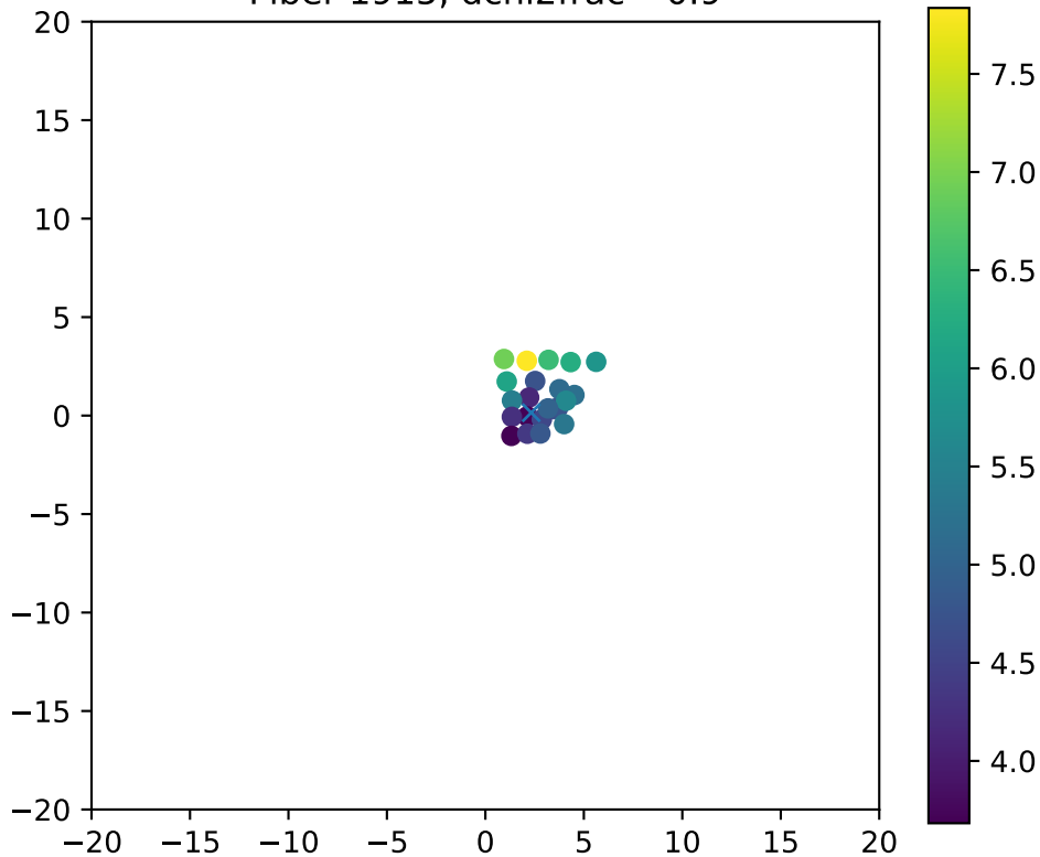
Fiber 1915, dchi2frac= 0.9
