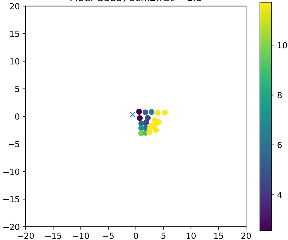
Fiber 3585, dchi2frac= 1.0
