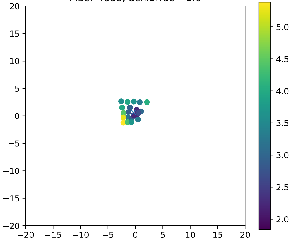
Fiber 4680, dchi2frac= 1.0
