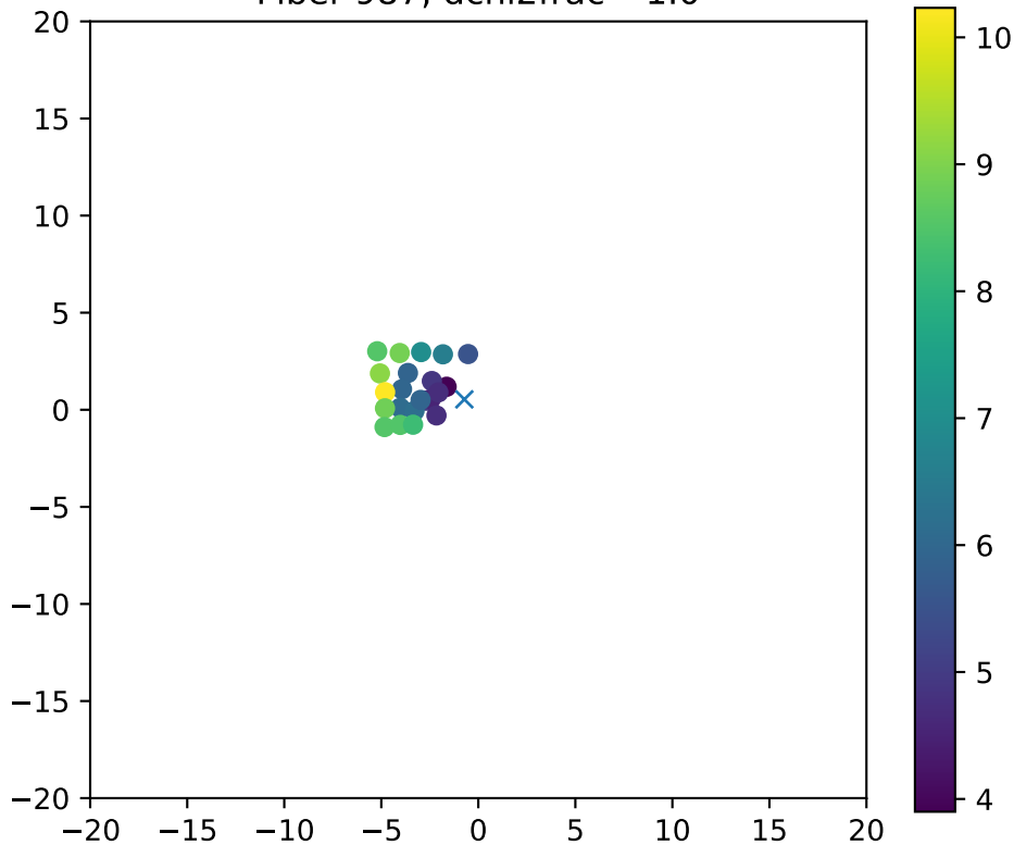
Fiber 987, dchi2frac= 1.0
