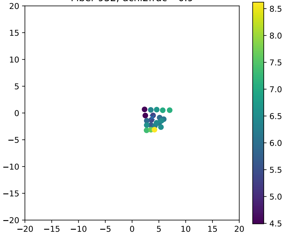
Fiber 932, dchi2frac= 0.9
