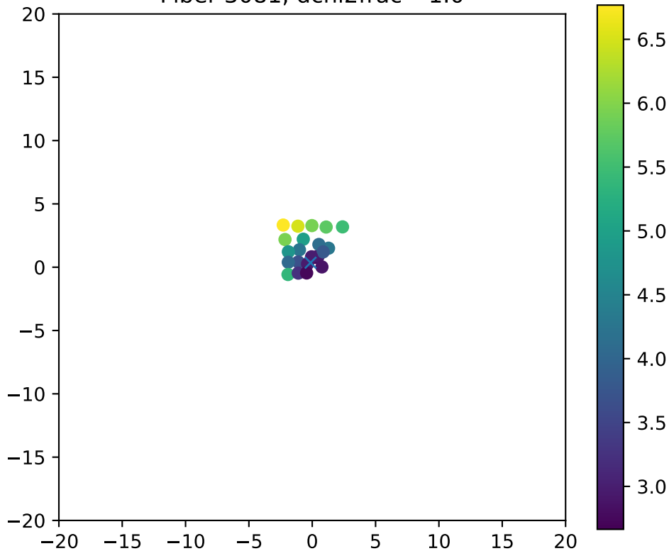
Fiber 3081, dchi2frac= 1.0
