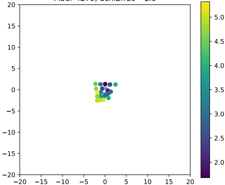
Fiber 4279, dchi2frac= 1.0
