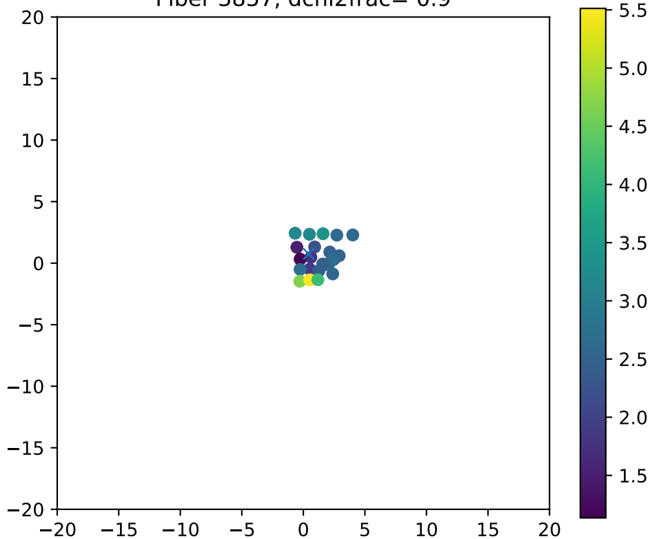
Fiber 3857, dchi2frac= 0.9
