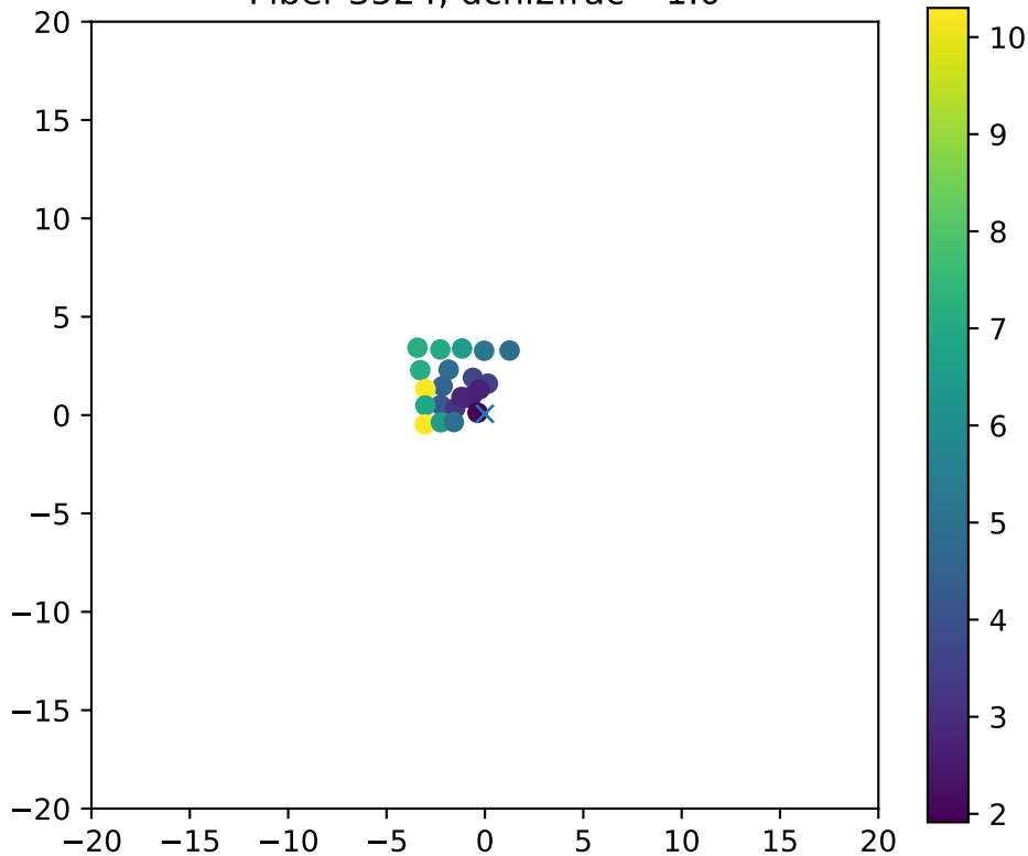
Fiber 3524, dchi2frac= 1.0
