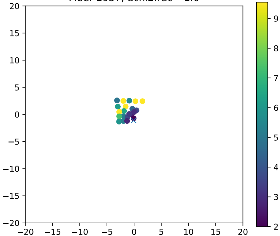
Fiber 2957, dchi2frac= 1.0
