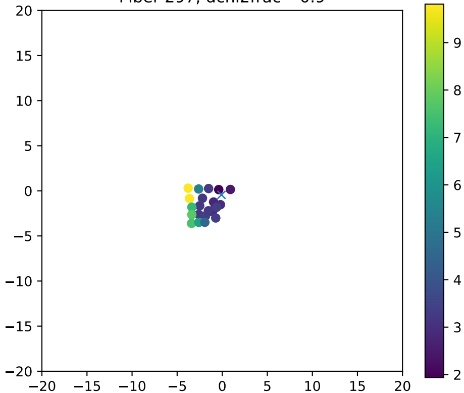
Fiber 297, dchi2frac= 0.9
