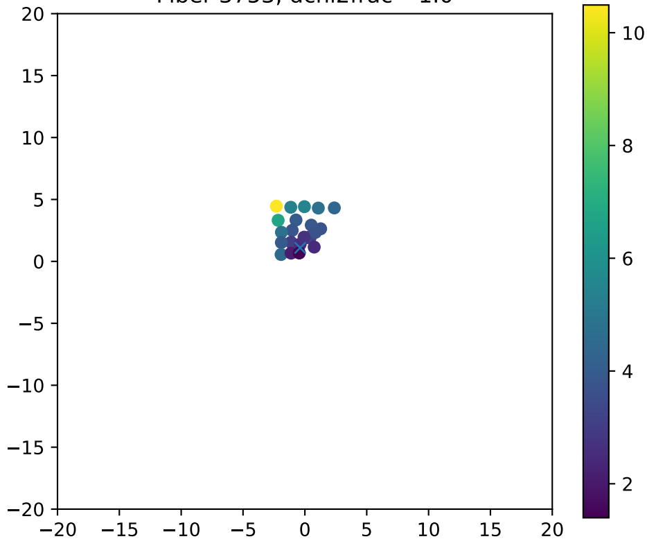
Fiber 3753, dchi2frac= 1.0
