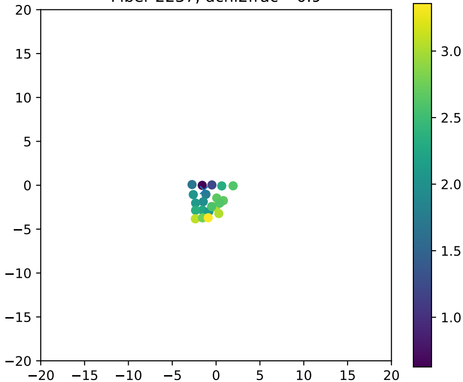
Fiber 2237, dchi2frac= 0.9
