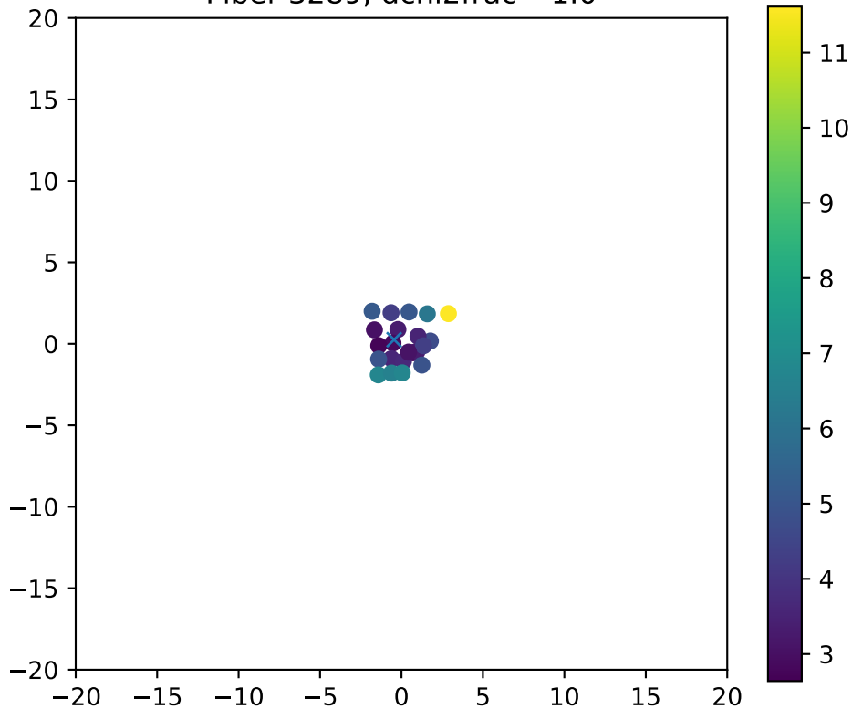
Fiber 3289, dchi2frac= 1.0
