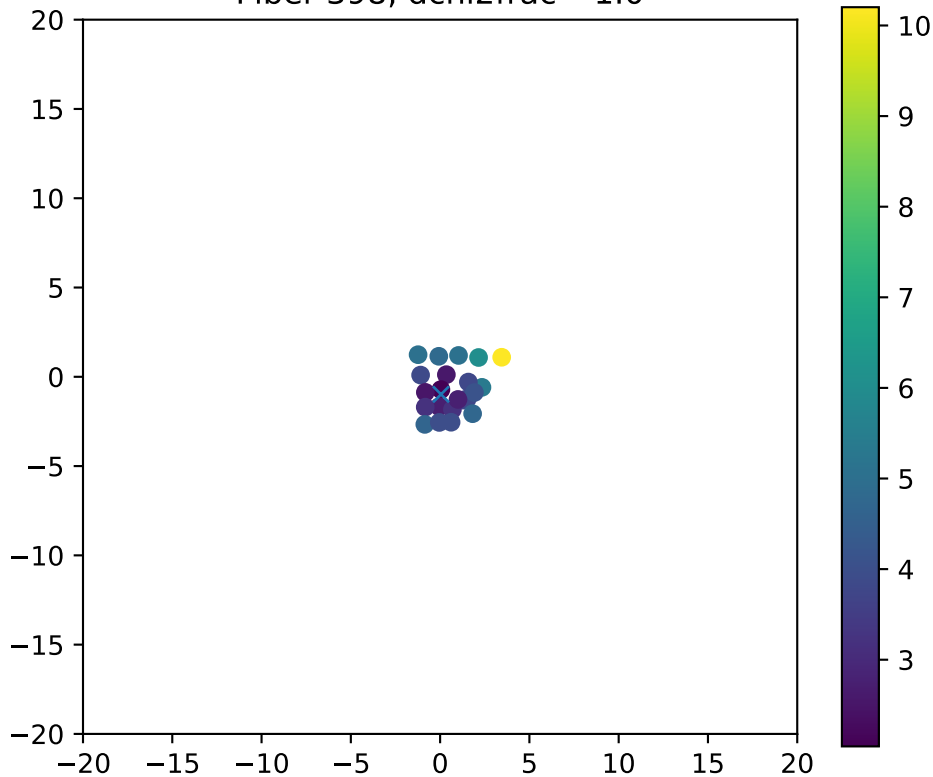
Fiber 398, dchi2frac= 1.0
