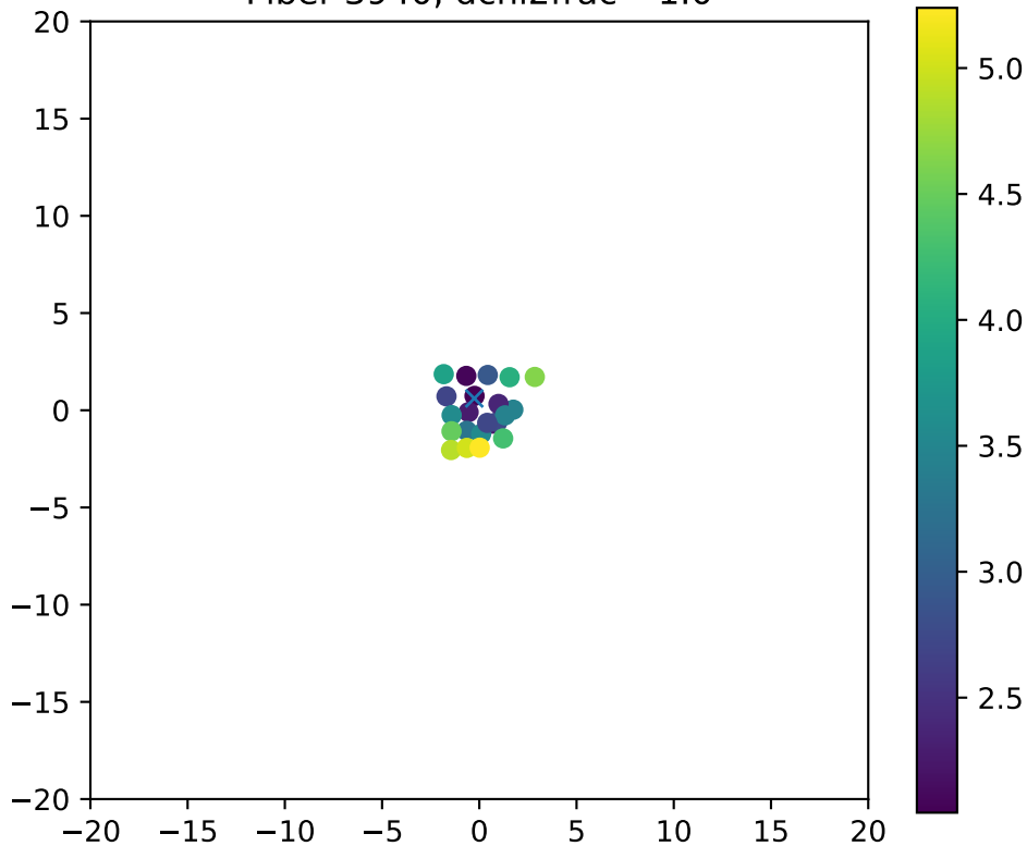
Fiber 3940, dchi2frac= 1.0
