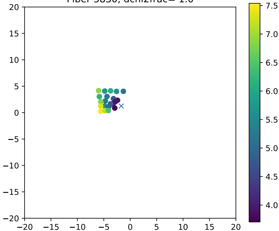
Fiber 3830, dchi2frac= 1.0
