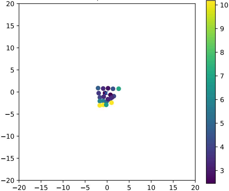
Fiber 2547, dchi2frac= 1.0
