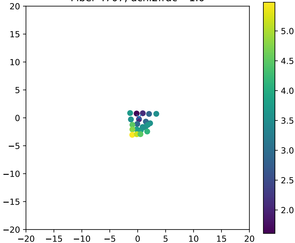
Fiber 4707, dchi2frac= 1.0
