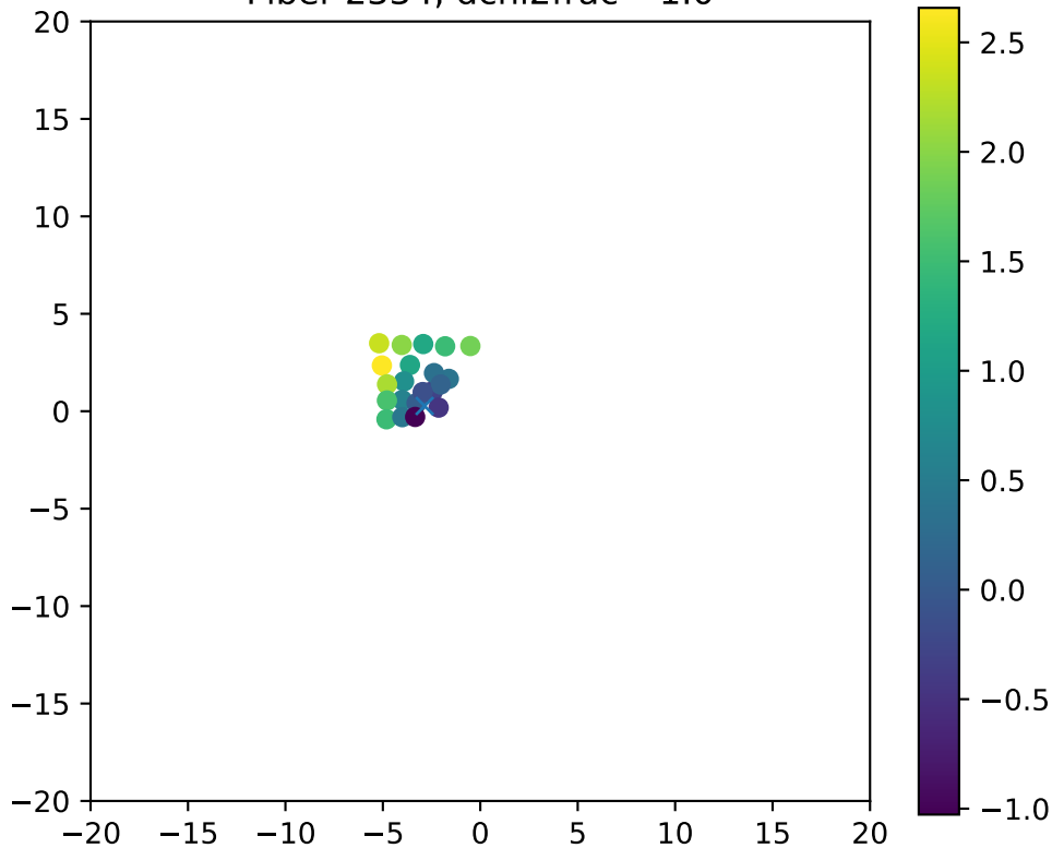
Fiber 2334, dchi2frac= 1.0
