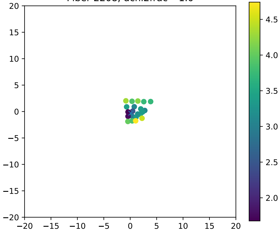
Fiber 2208, dchi2frac= 1.0
