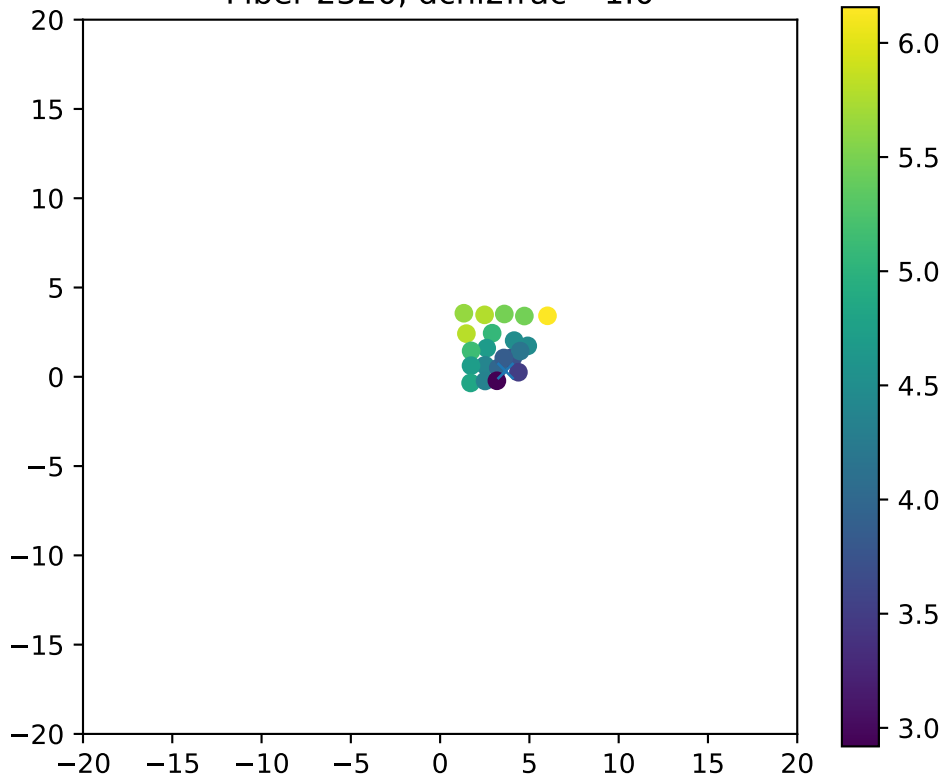
Fiber 2320, dchi2frac= 1.0
