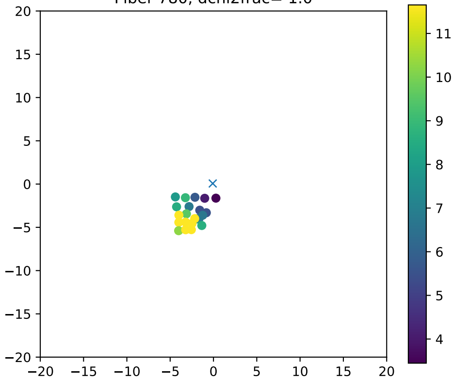
Fiber 780, dchi2frac= 1.0
