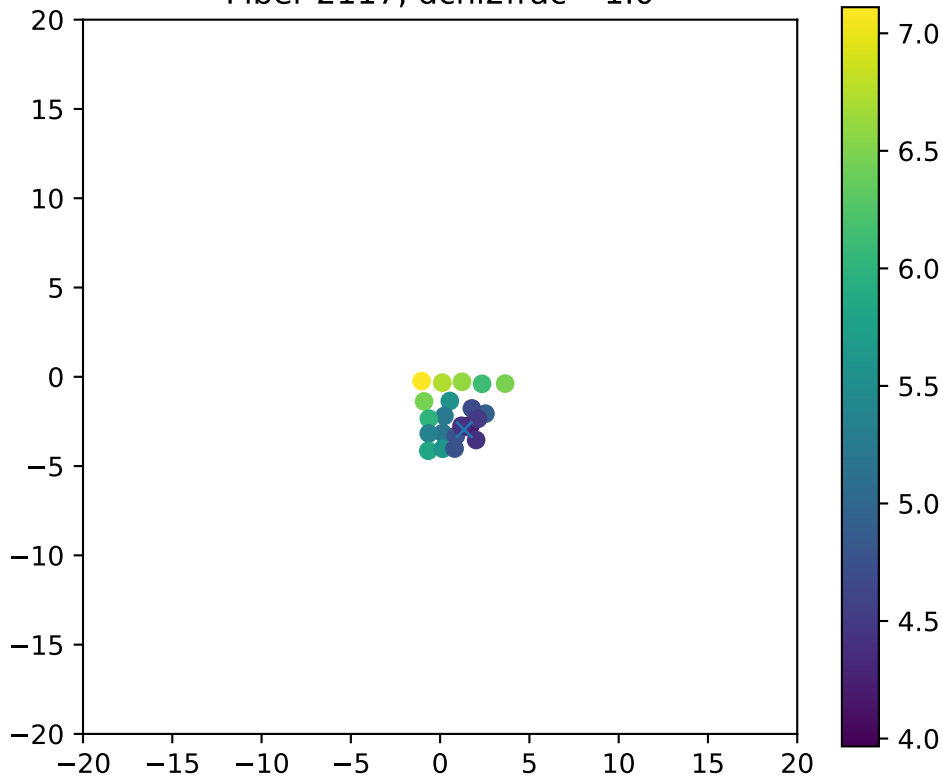
Fiber 2117, dchi2frac= 1.0
