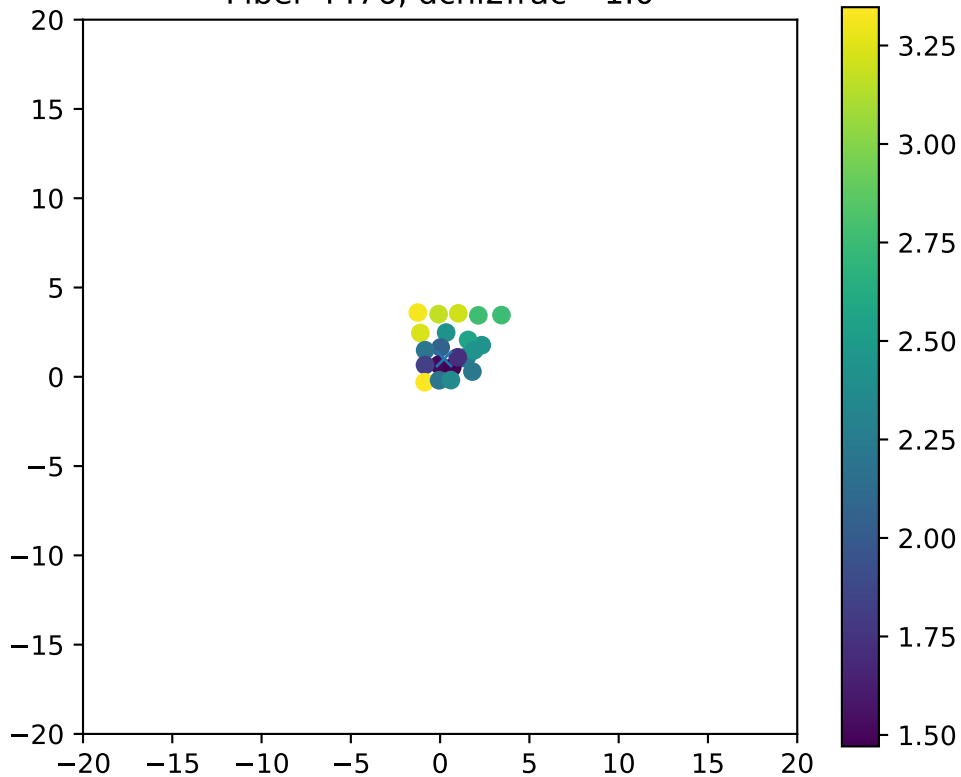
Fiber 4476, dchi2frac= 1.0
