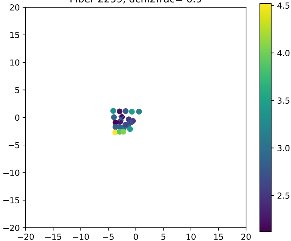
Fiber 2259, dchi2frac= 0.9
