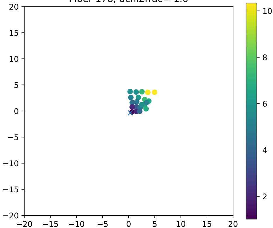
Fiber 178, dchi2frac= 1.0
