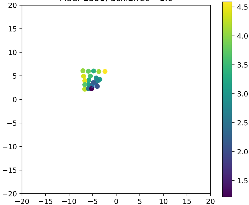
Fiber 2351, dchi2frac= 1.0
