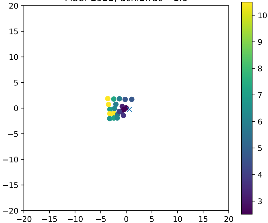
Fiber 2922, dchi2frac= 1.0
