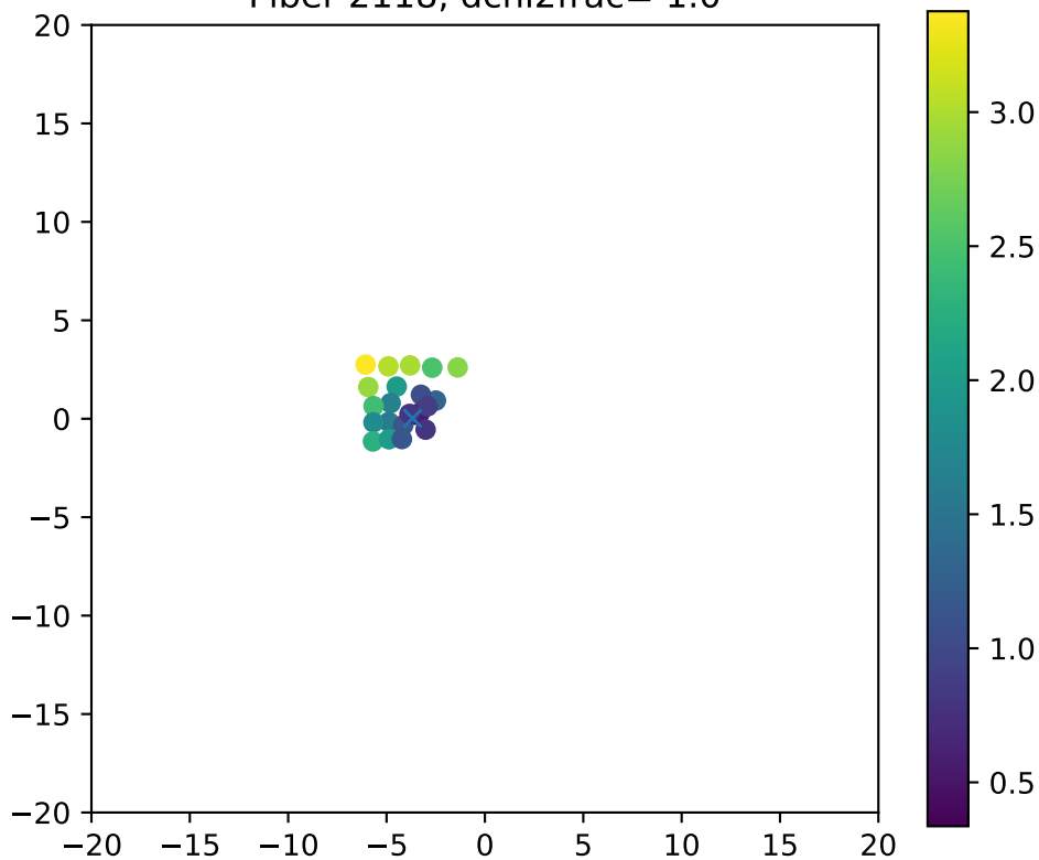
Fiber 2118, dchi2frac= 1.0
