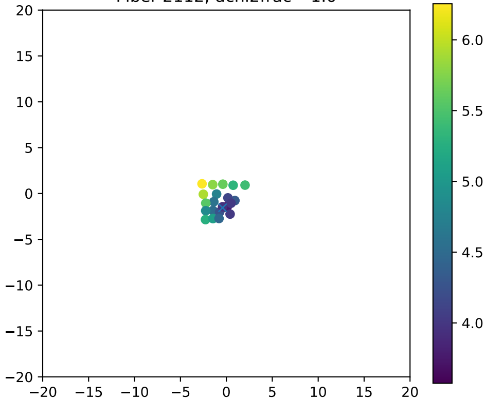
Fiber 2112, dchi2frac= 1.0
