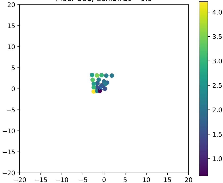
Fiber 361, dchi2frac= 0.9
