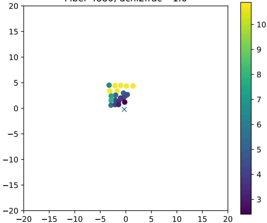
Fiber 4880, dchi2frac= 1.0
