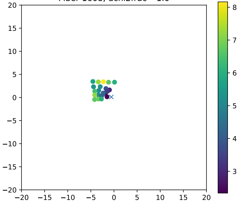
Fiber 1608, dchi2frac= 1.0
