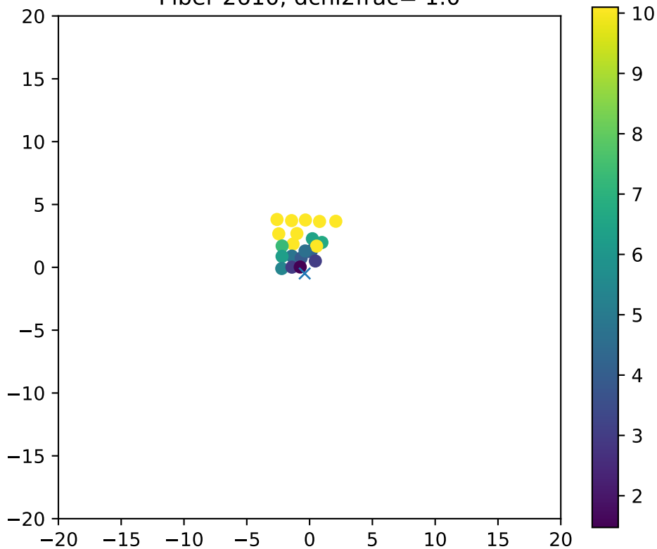
Fiber 2610, dchi2frac= 1.0
