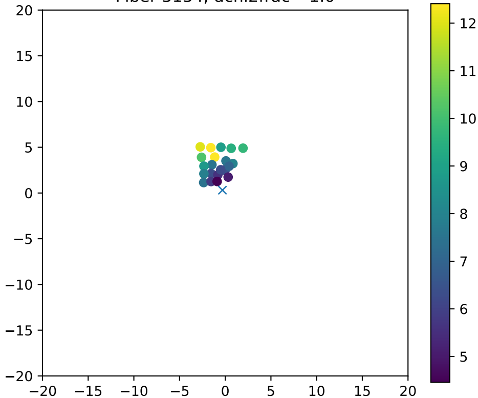
Fiber 3134, dchi2frac= 1.0
