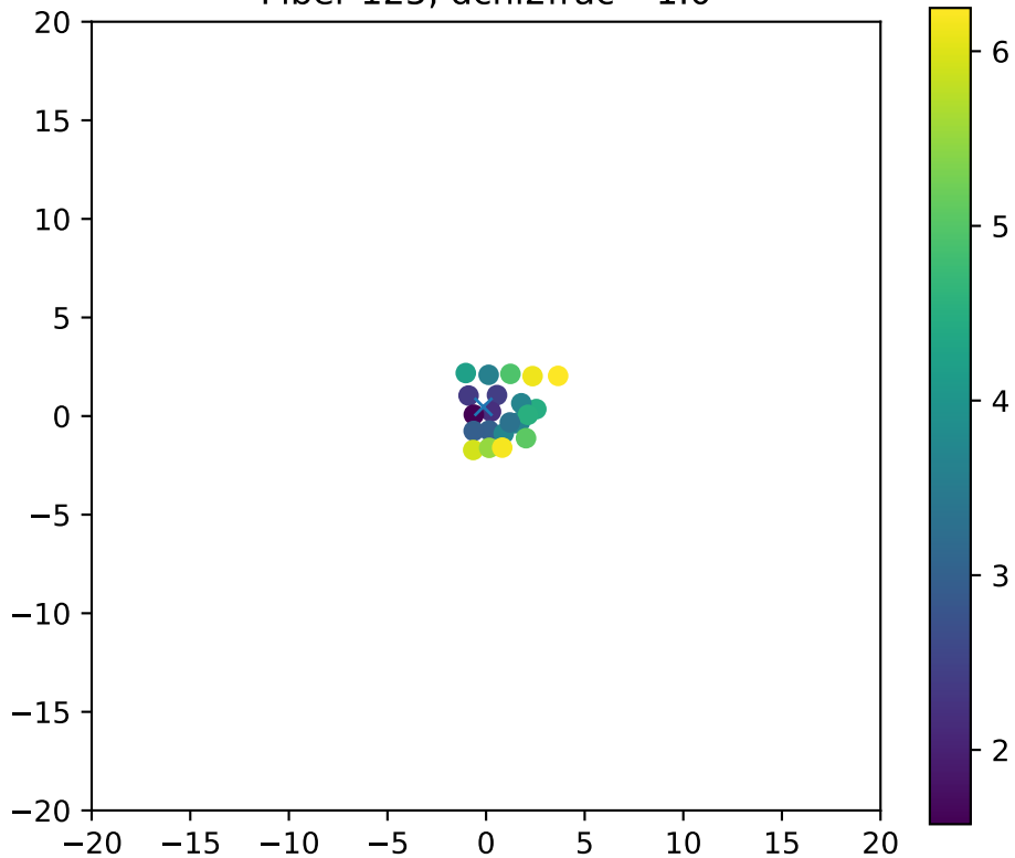
Fiber 125, dchi2frac= 1.0
