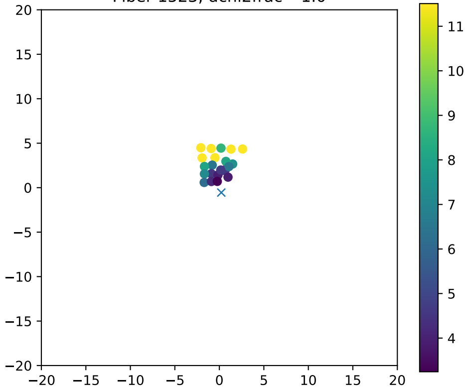
Fiber 1523, dchi2frac= 1.0
