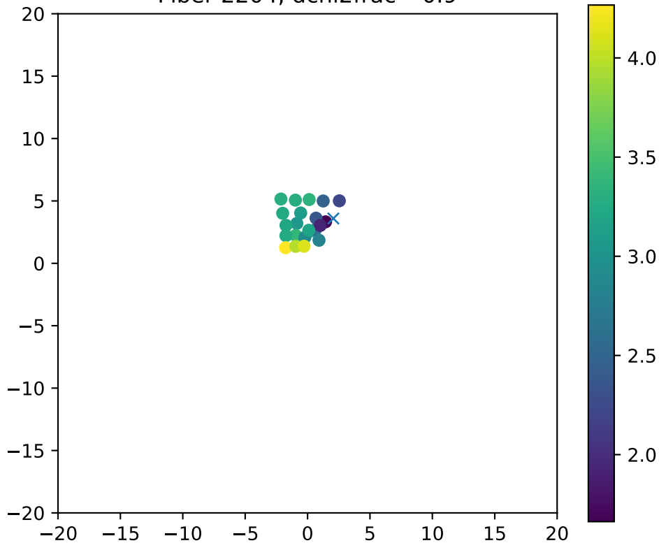
Fiber 2204, dchi2frac= 0.9
