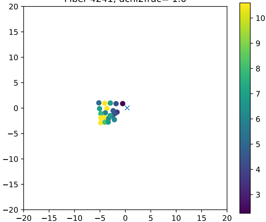
Fiber 4241, dchi2frac= 1.0
