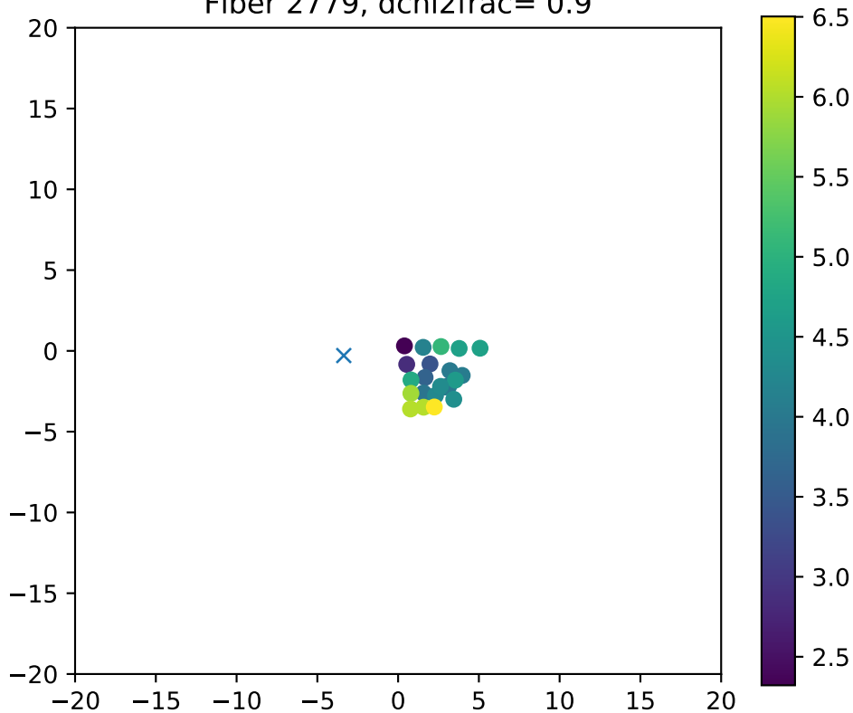
Fiber 2779, dchi2frac= 0.9
