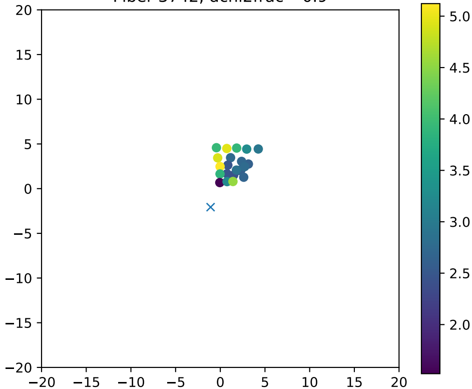
Fiber 3742, dchi2frac= 0.9
