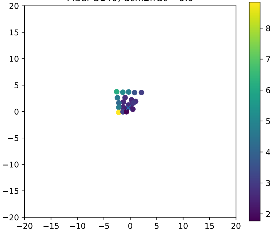
Fiber 3140, dchi2frac= 0.9
