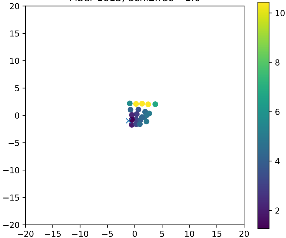
Fiber 1613, dchi2frac= 1.0
