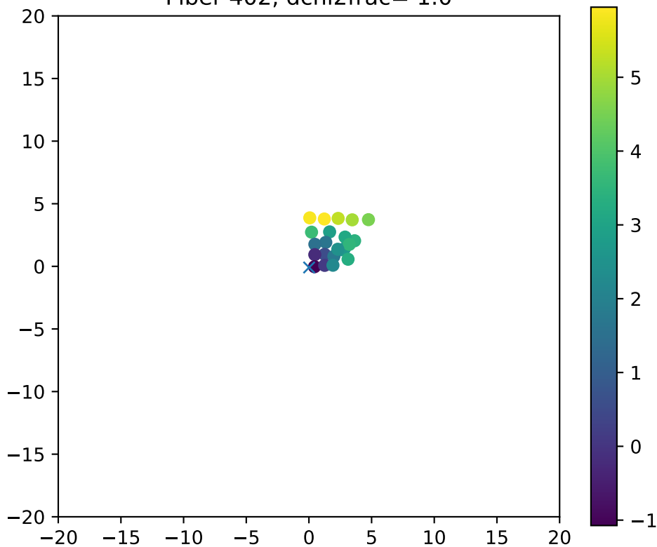
Fiber 402, dchi2frac= 1.0
