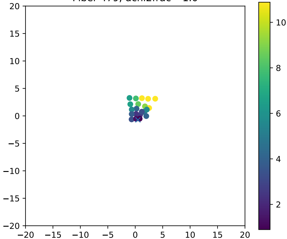
Fiber 479, dchi2frac= 1.0
