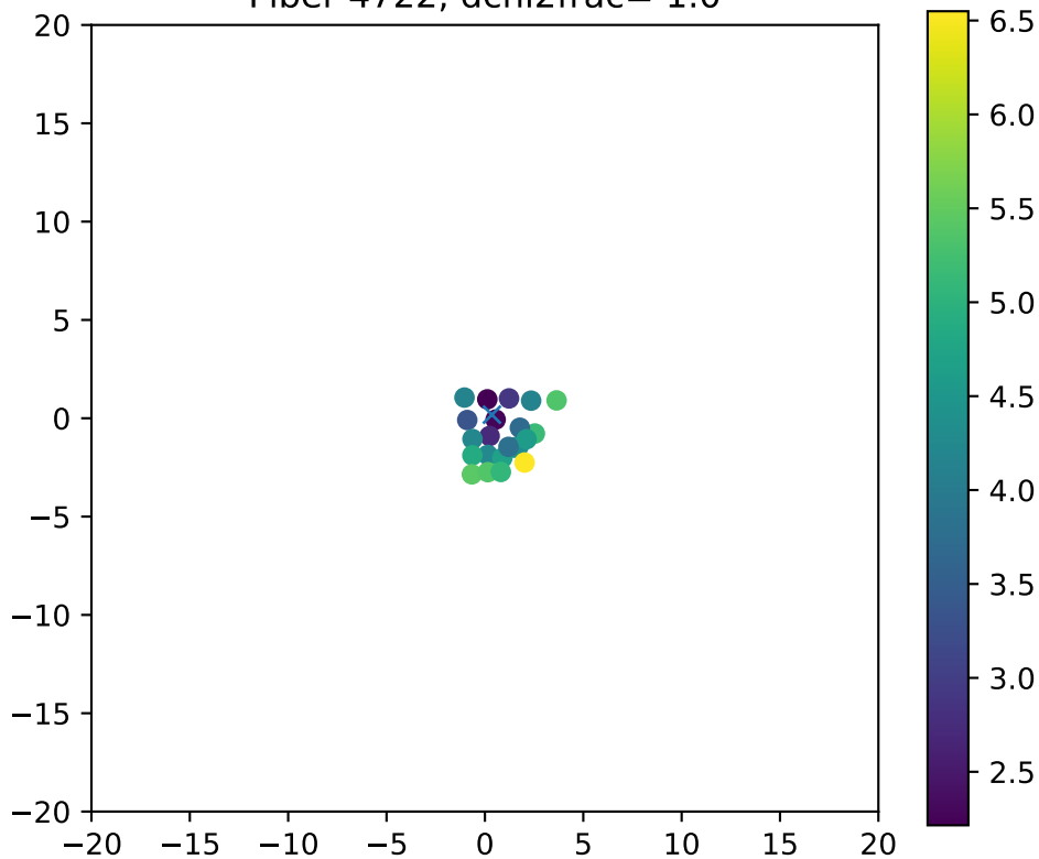
Fiber 4722, dchi2frac= 1.0
