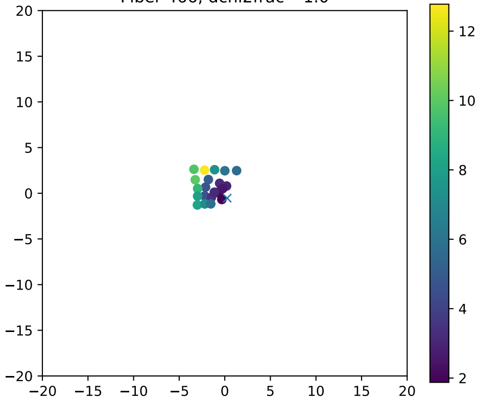
Fiber 466, dchi2frac= 1.0
