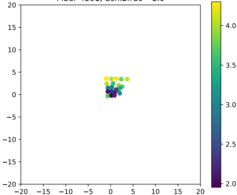
Fiber 4391, dchi2frac= 1.0
