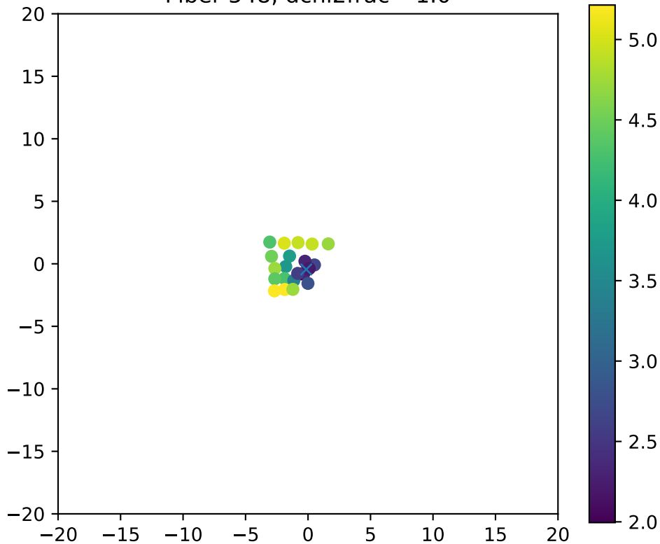
Fiber 548, dchi2frac= 1.0
