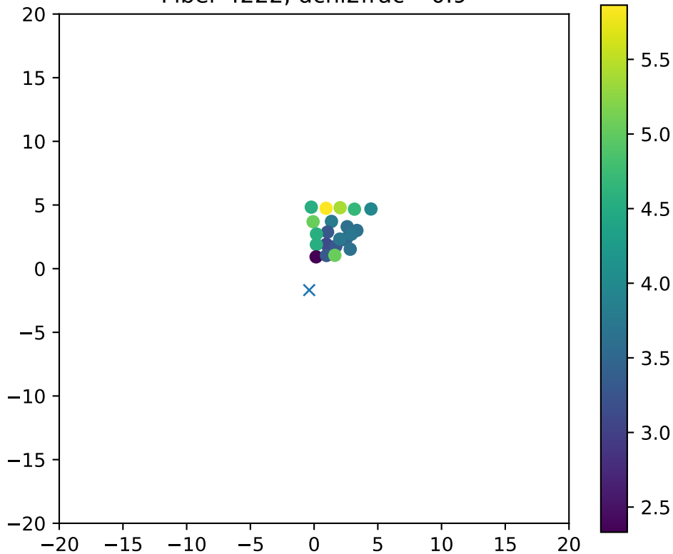
Fiber 4222, dchi2frac= 0.9
