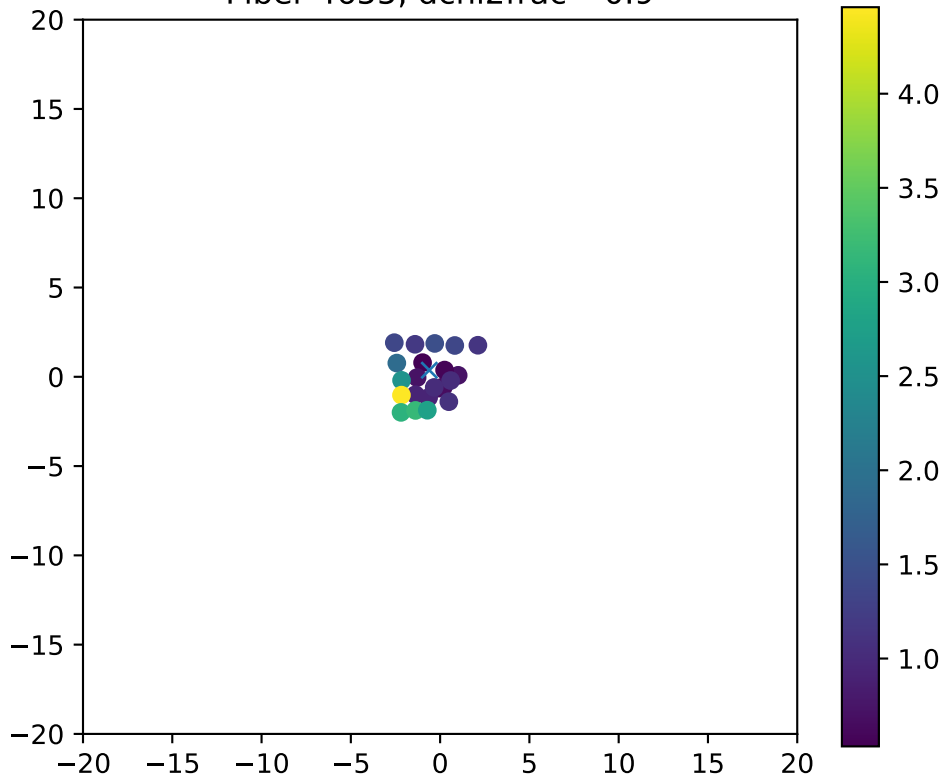
Fiber 4655, dchi2frac= 0.9
