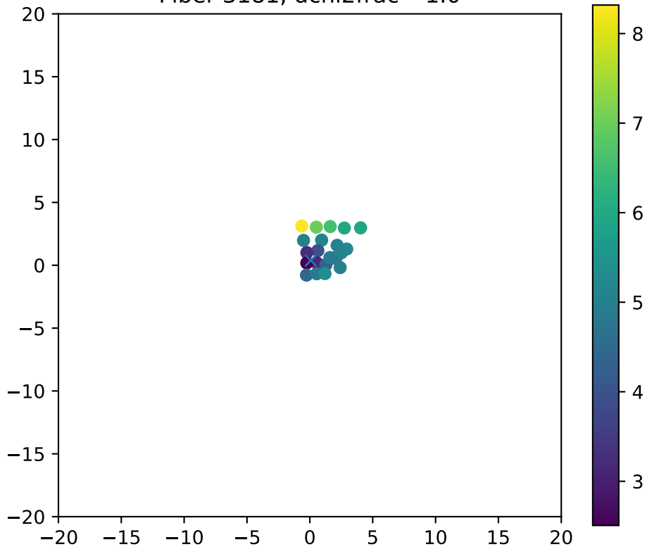
Fiber 3181, dchi2frac= 1.0
