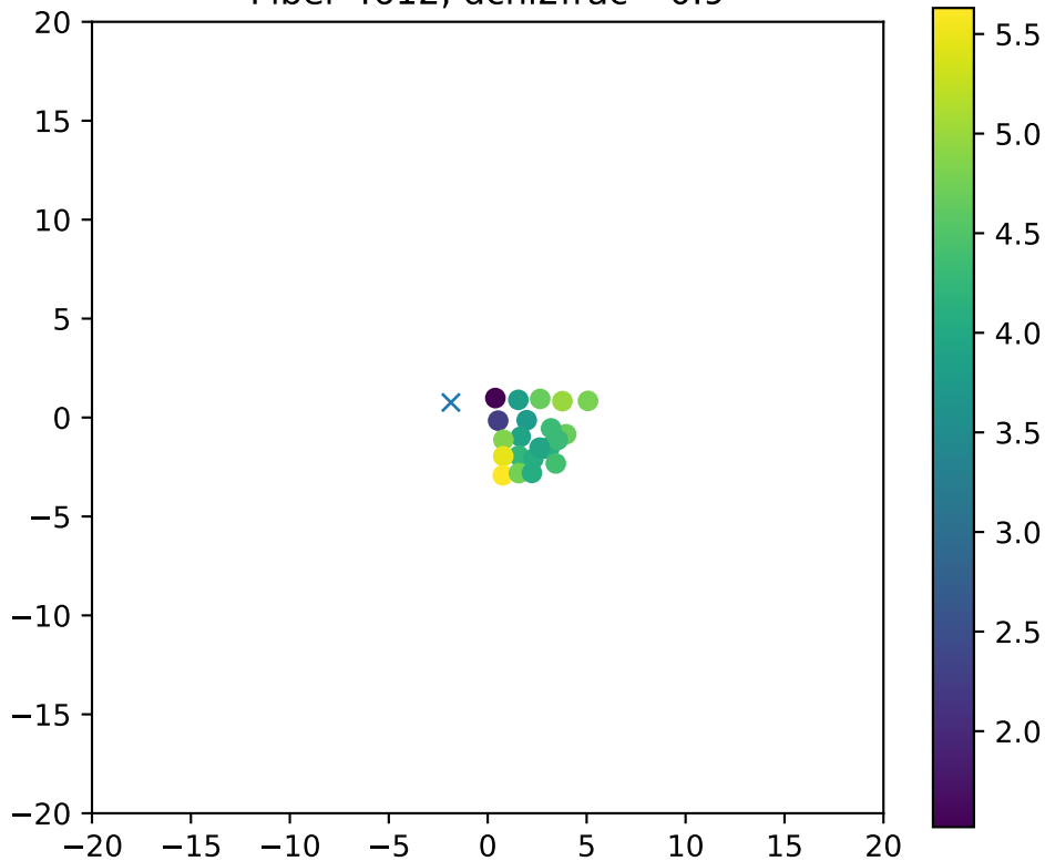
Fiber 4612, dchi2frac= 0.9
