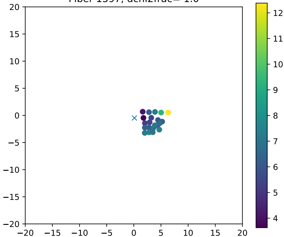
Fiber 1597, dchi2frac= 1.0
