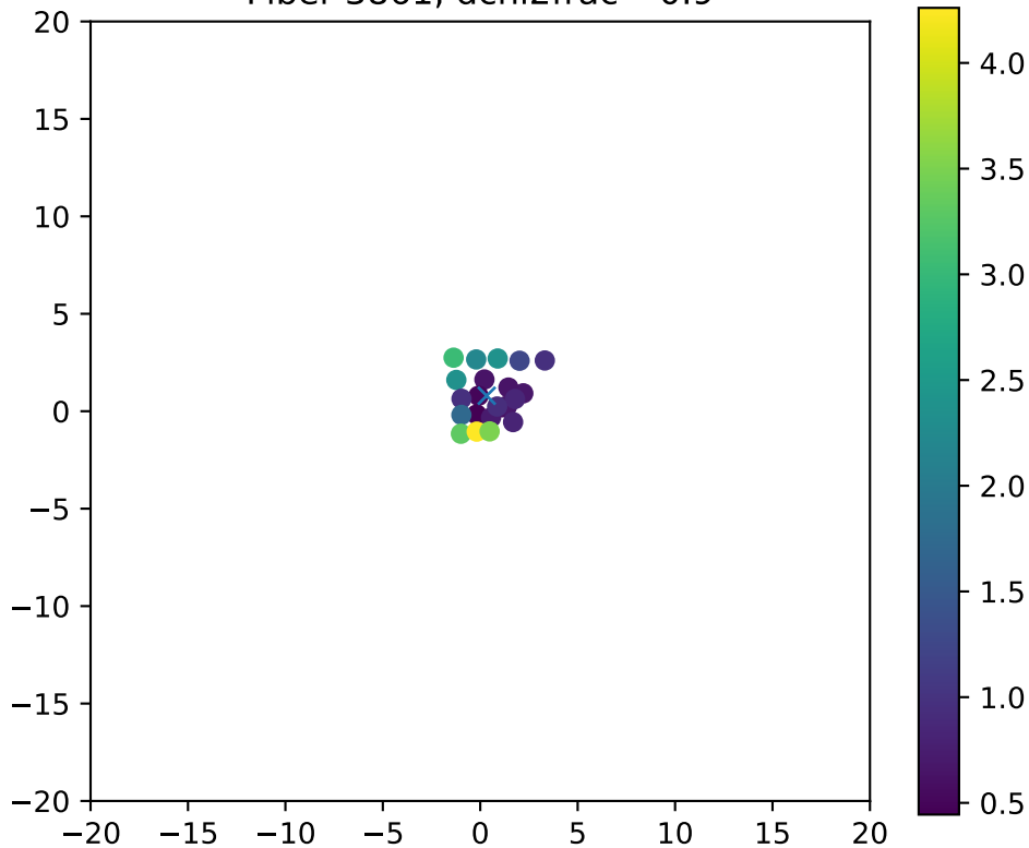
Fiber 3861, dchi2frac= 0.9
