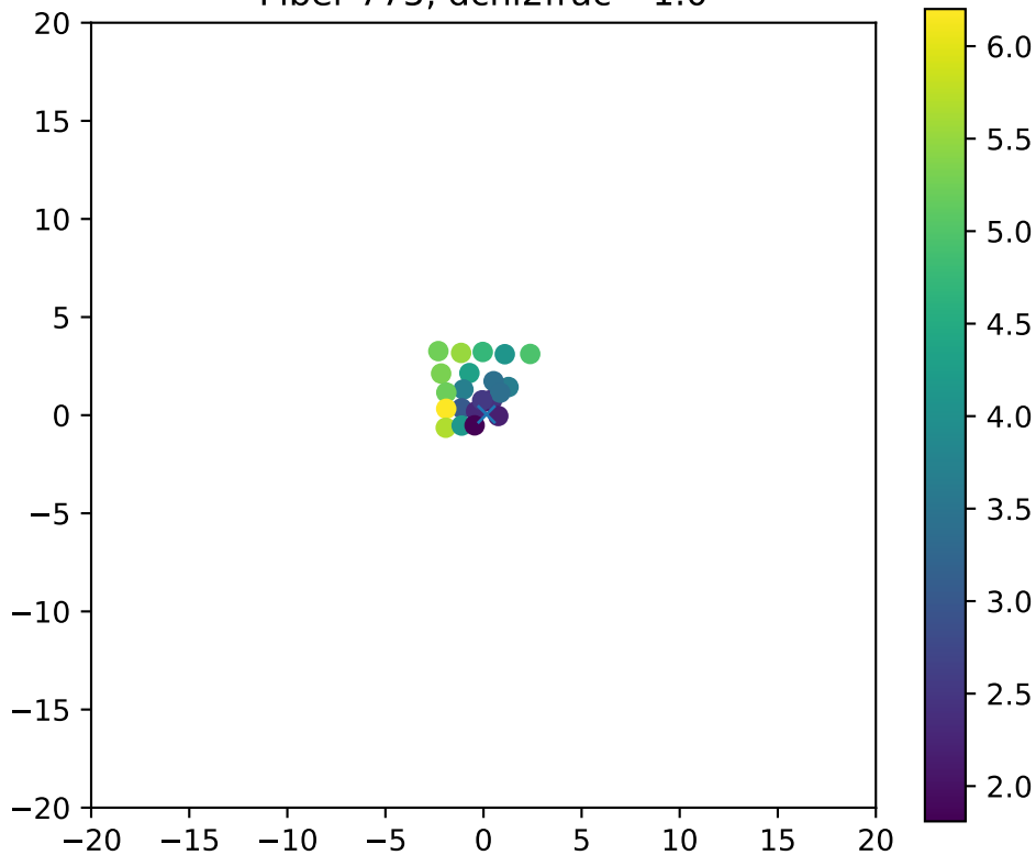
Fiber 775, dchi2frac= 1.0
