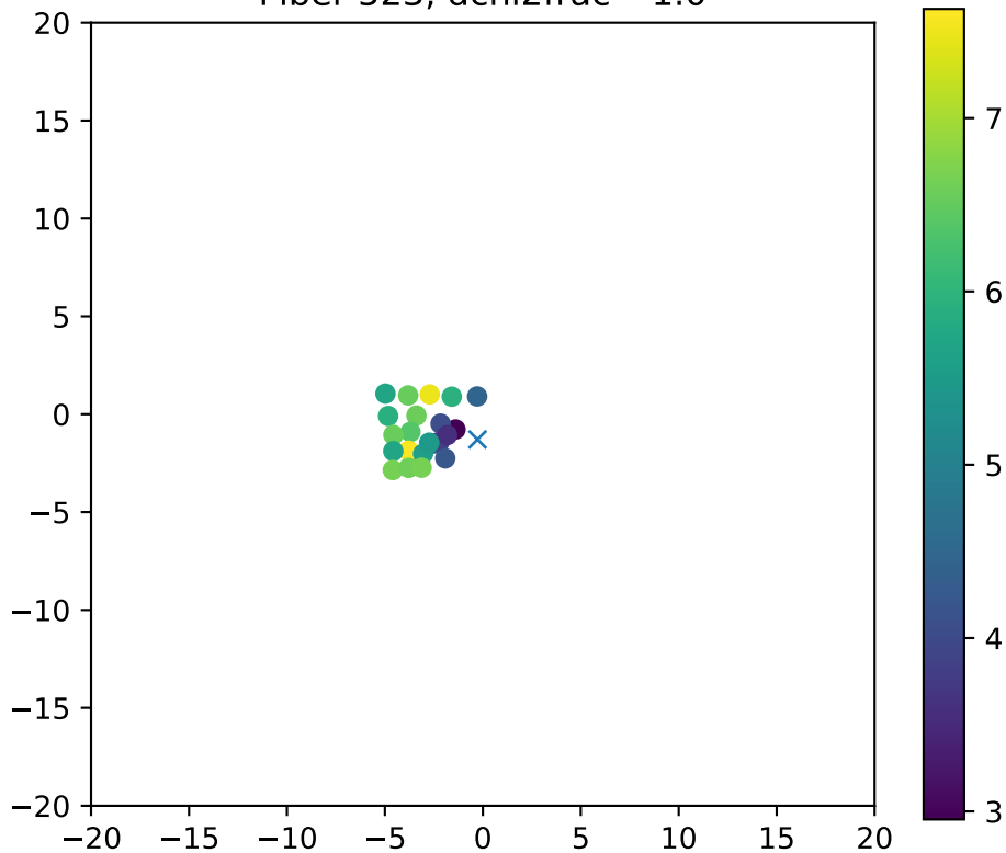
Fiber 523, dchi2frac= 1.0
