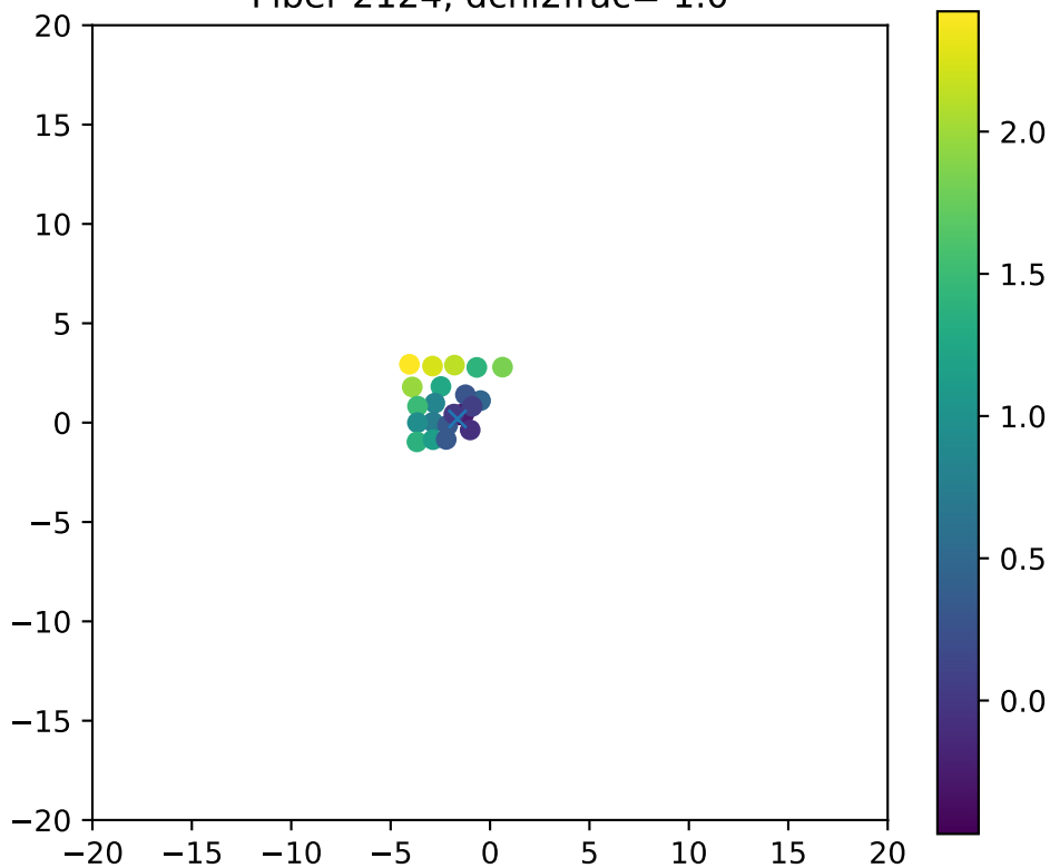
Fiber 2124, dchi2frac= 1.0
