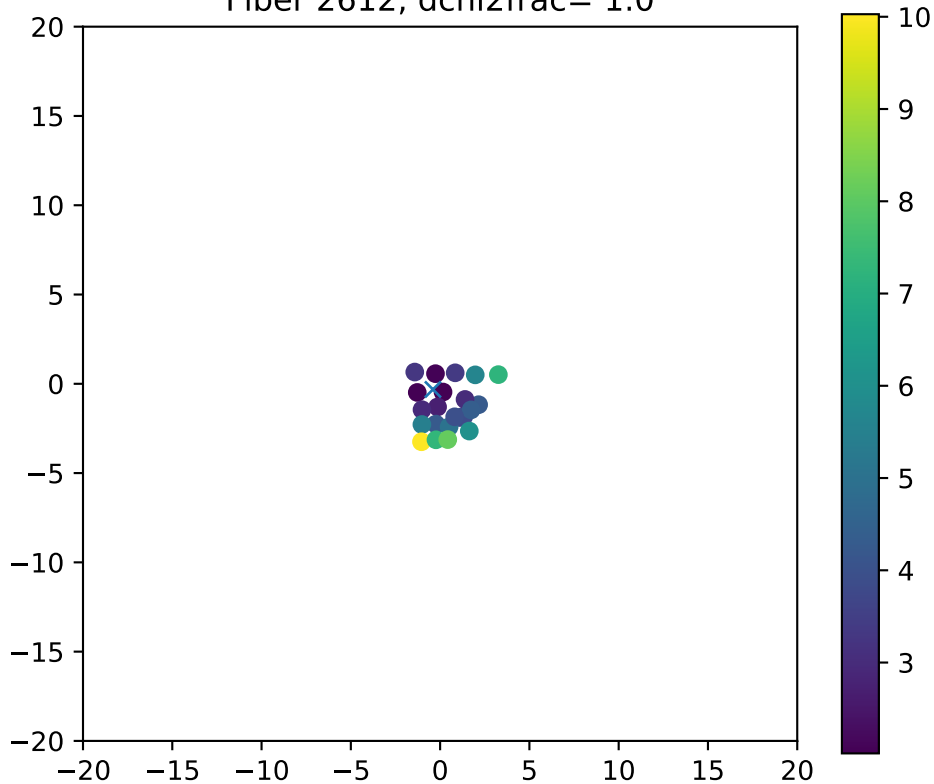
Fiber 2612, dchi2frac= 1.0
