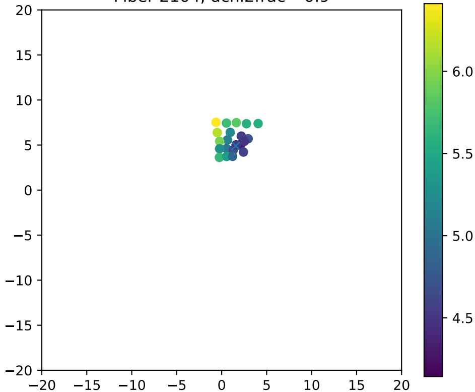
Fiber 2104, dchi2frac= 0.9
