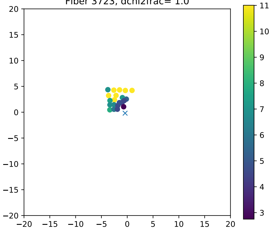
Fiber 3723, dchi2frac= 1.0
