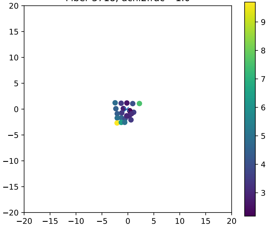
Fiber 3718, dchi2frac= 1.0
