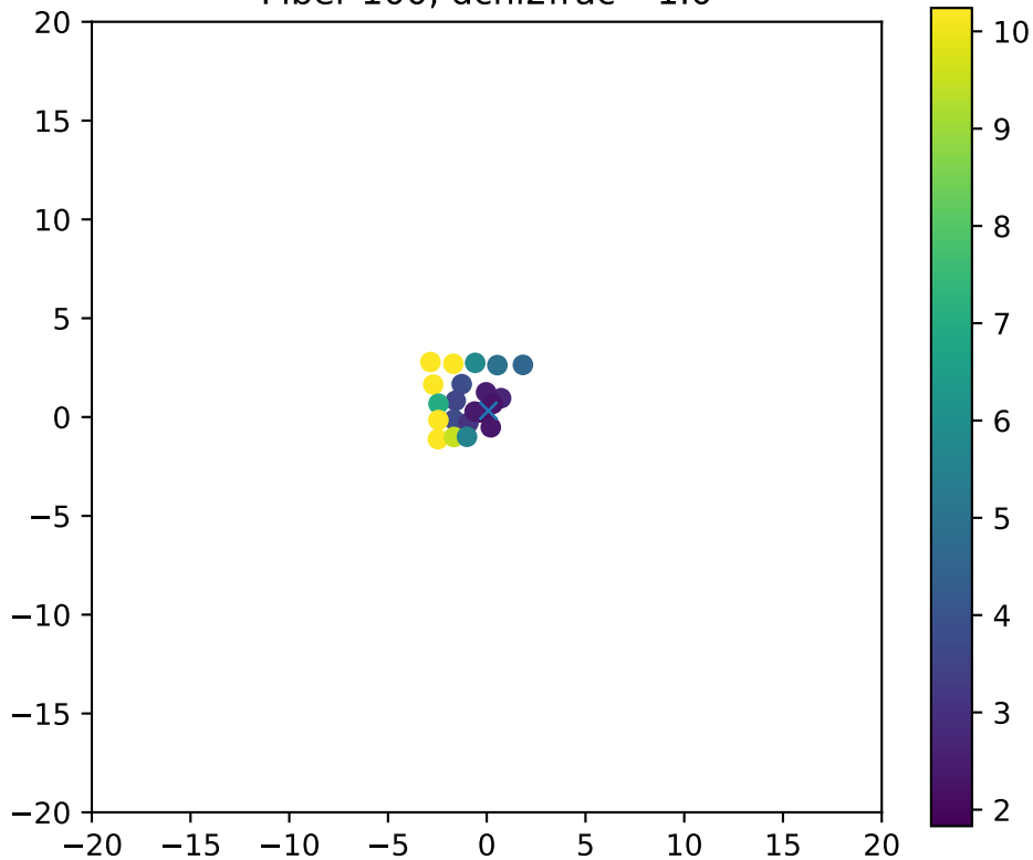
Fiber 100, dchi2frac= 1.0
