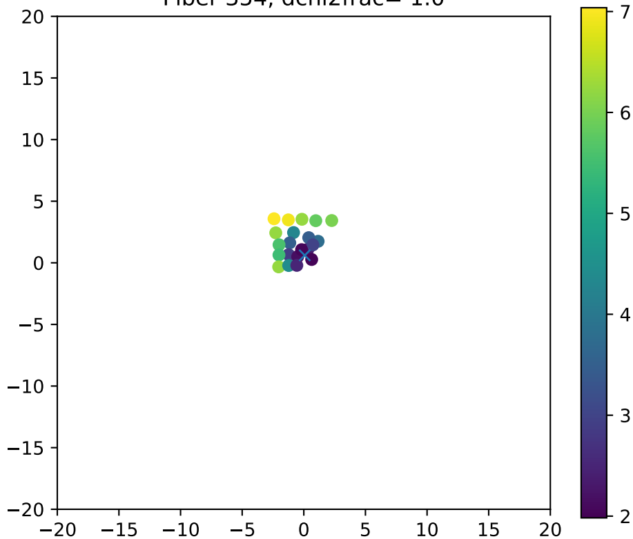
Fiber 354, dchi2frac= 1.0
