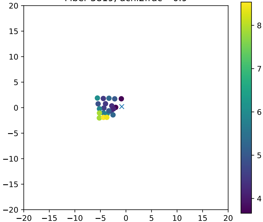
Fiber 3819, dchi2frac= 0.9
