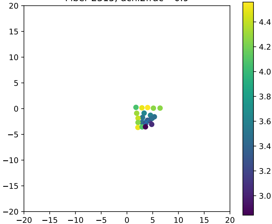
Fiber 2315, dchi2frac= 0.9
