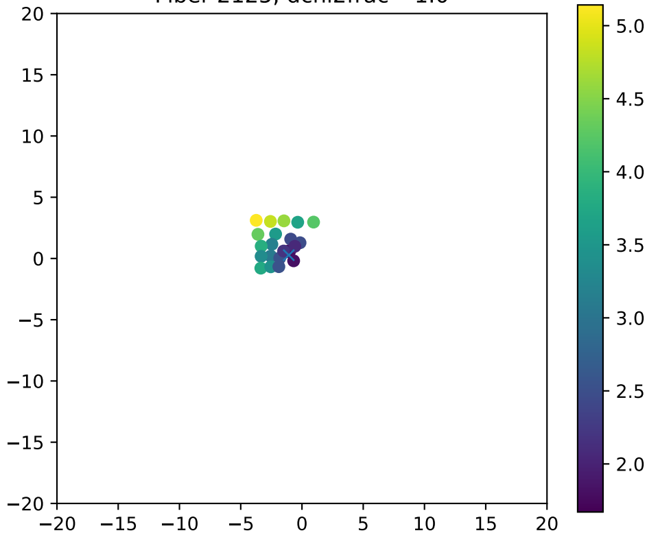
Fiber 2125, dchi2frac= 1.0
