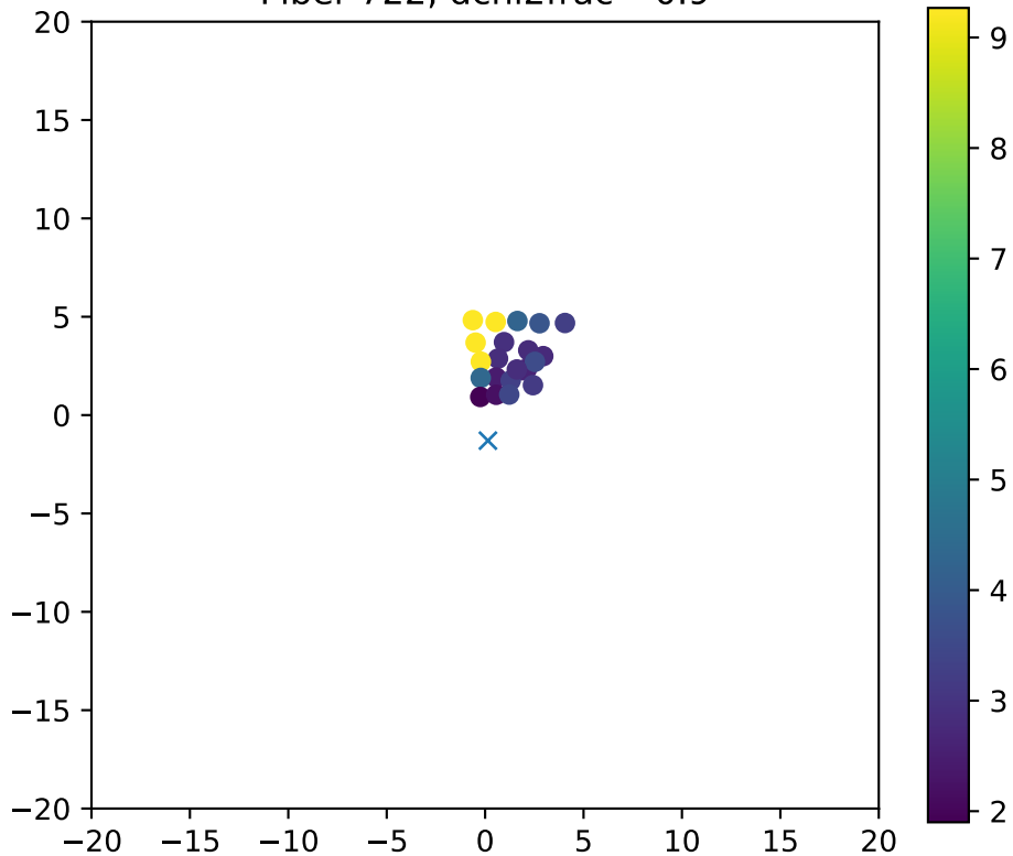
Fiber 722, dchi2frac= 0.9
