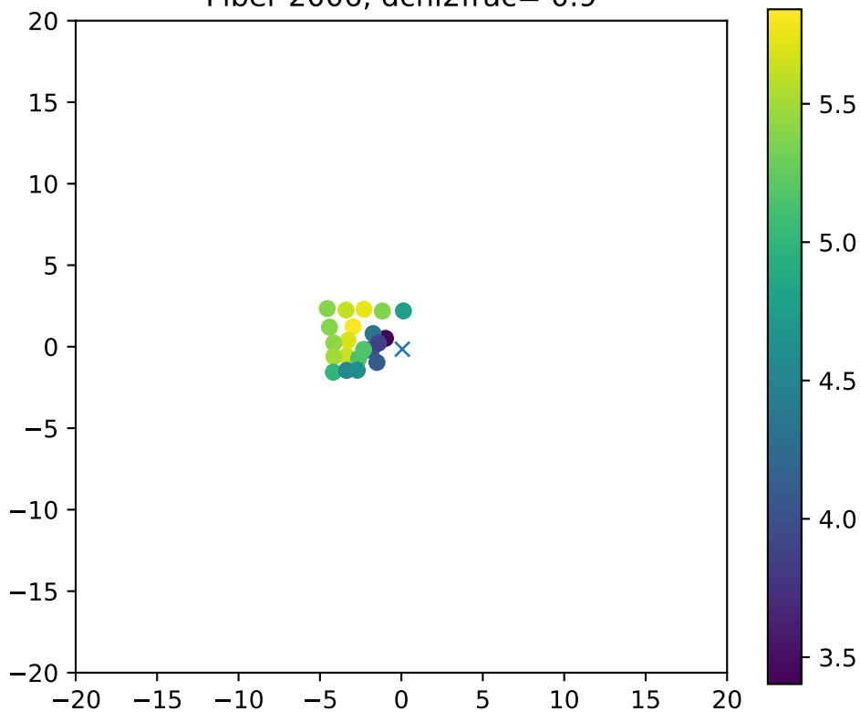
Fiber 2006, dchi2frac= 0.9
