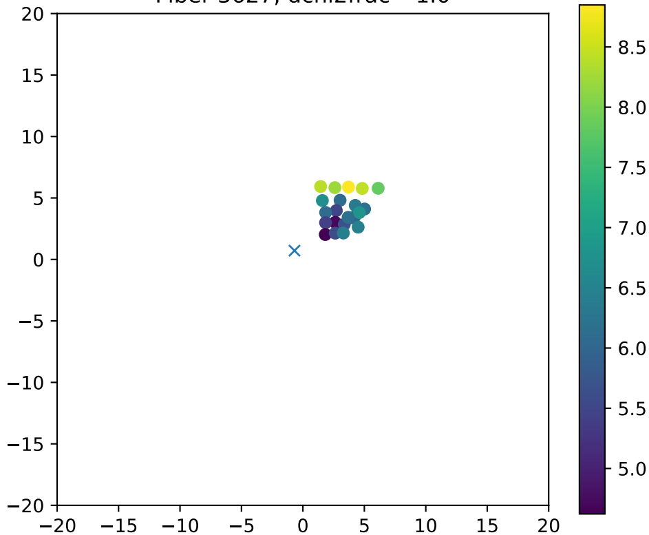
Fiber 3627, dchi2frac= 1.0
