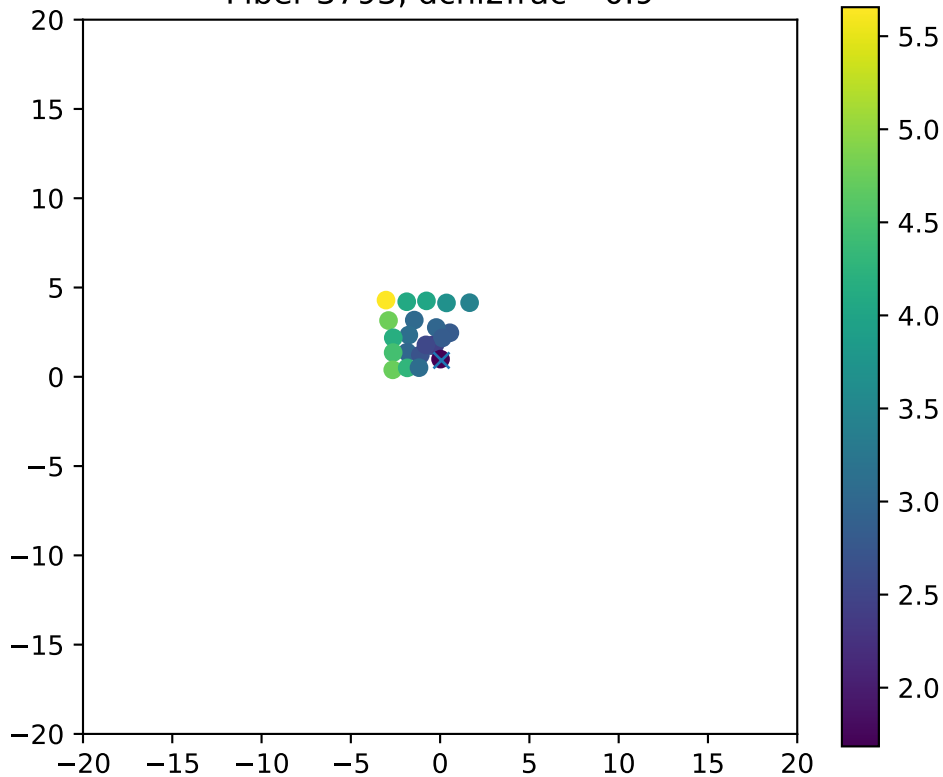
Fiber 3793, dchi2frac= 0.9
