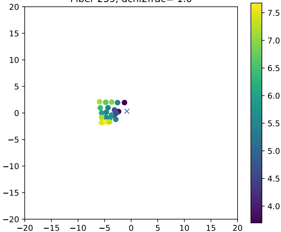
Fiber 259, dchi2frac= 1.0
