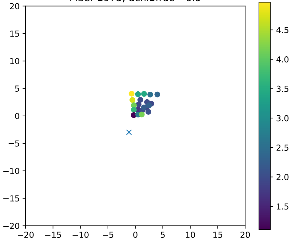
Fiber 2975, dchi2frac= 0.9
