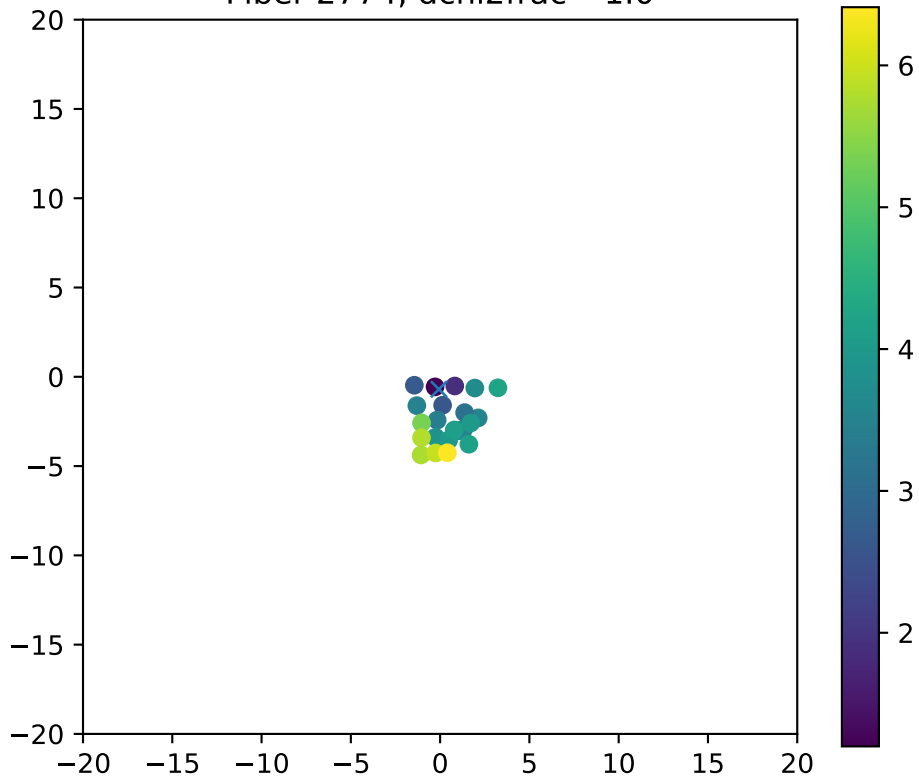
Fiber 2774, dchi2frac= 1.0
