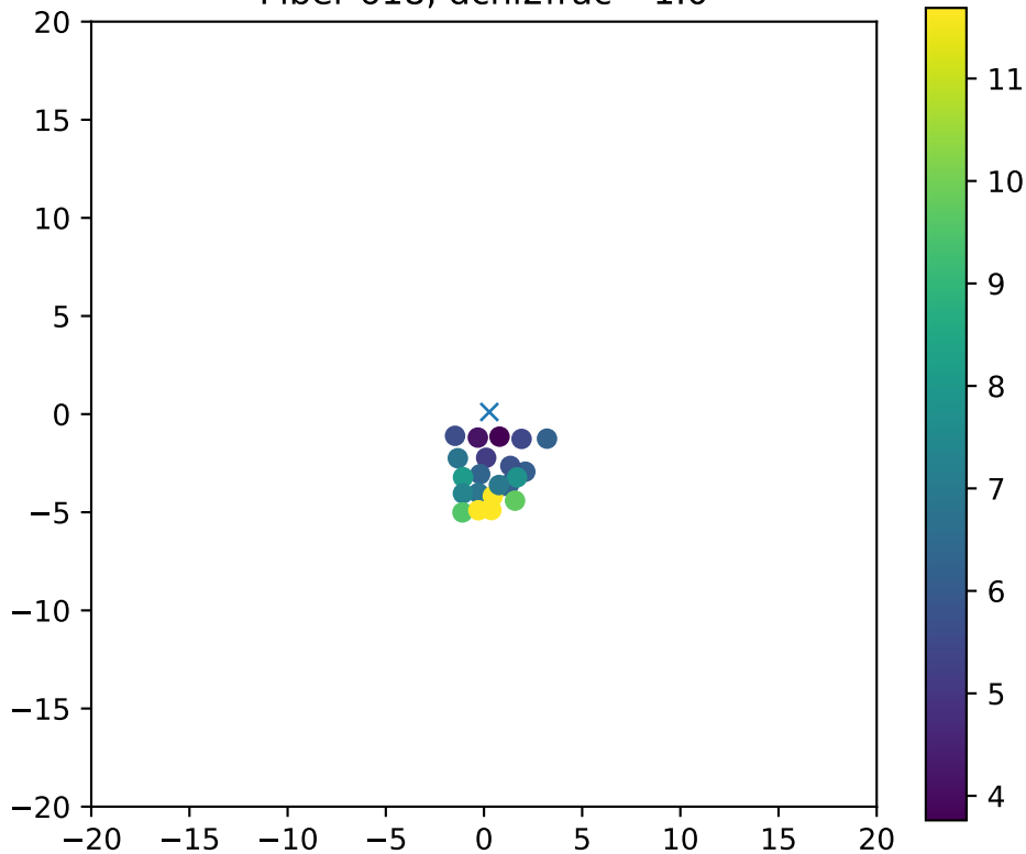
Fiber 618, dchi2frac= 1.0
