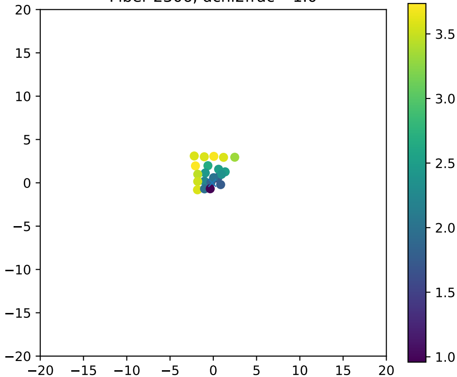
Fiber 2306, dchi2frac= 1.0
