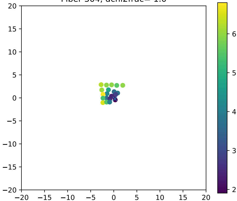
Fiber 304, dchi2frac= 1.0
