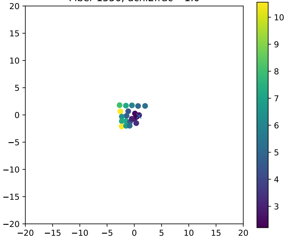
Fiber 1556, dchi2frac= 1.0
