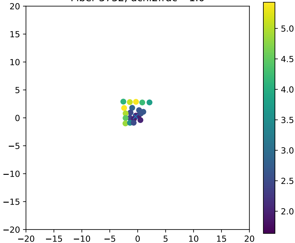
Fiber 3732, dchi2frac= 1.0
