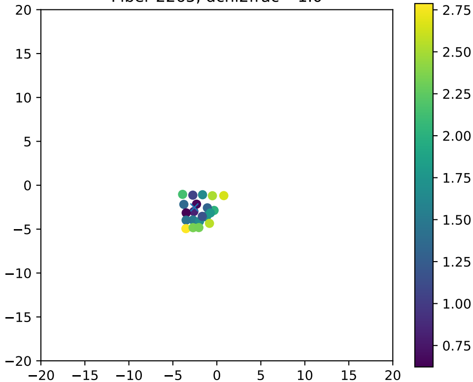
Fiber 2265, dchi2frac= 1.0
