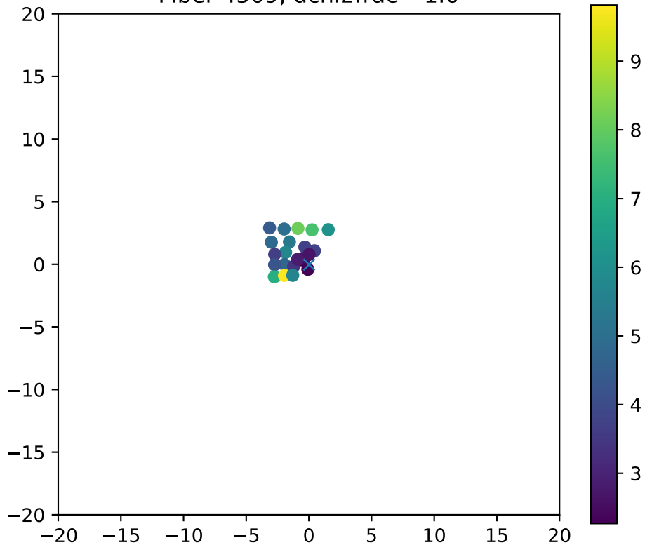
Fiber 4509, dchi2frac= 1.0
