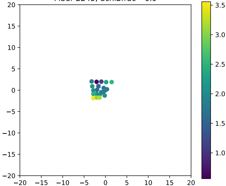
Fiber 2245, dchi2frac= 0.9
