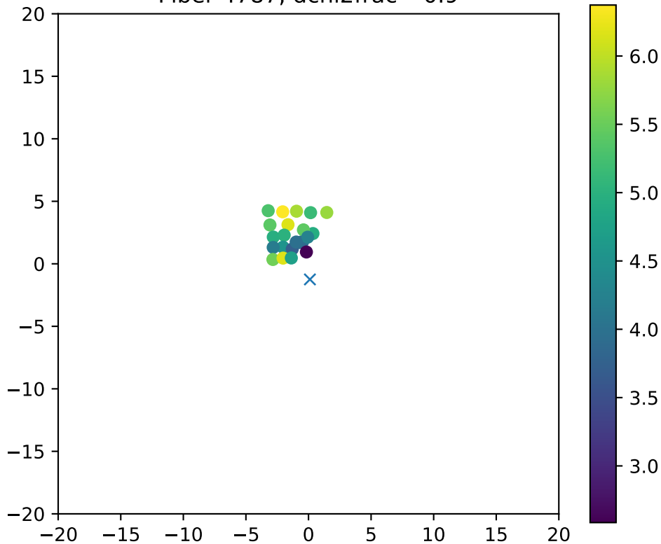
Fiber 4787, dchi2frac= 0.9
