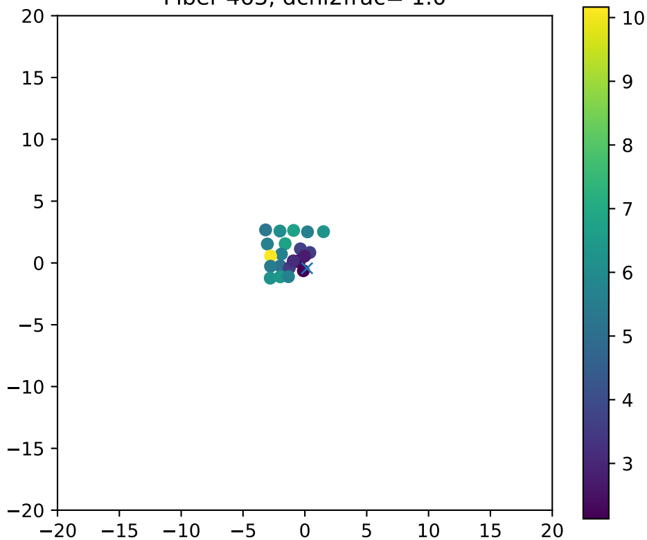
Fiber 463, dchi2frac= 1.0
