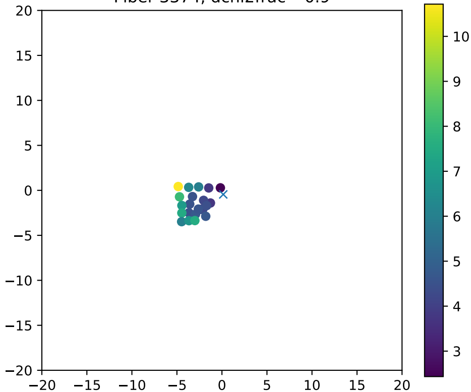
Fiber 3374, dchi2frac= 0.9
