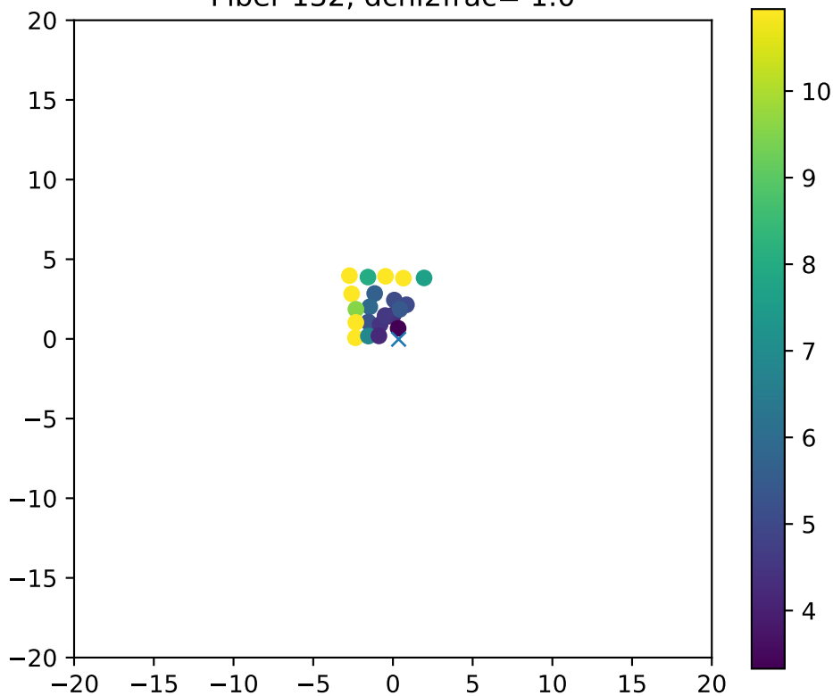
Fiber 132, dchi2frac= 1.0
