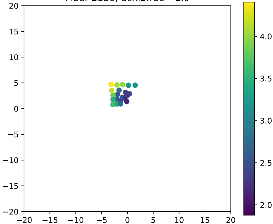
Fiber 2130, dchi2frac= 1.0
