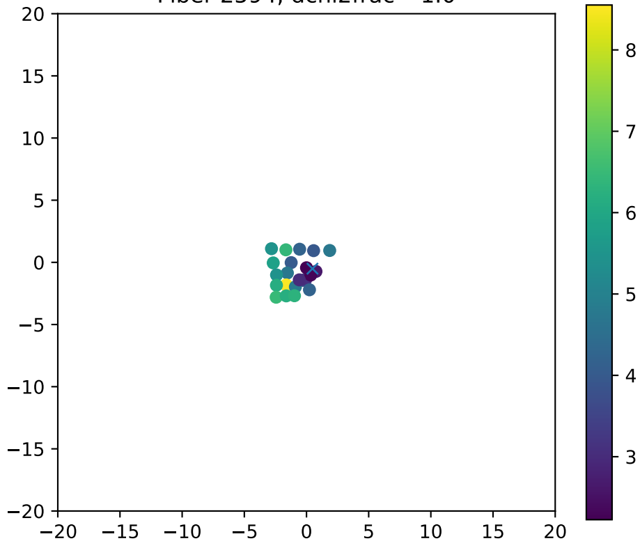
Fiber 2594, dchi2frac= 1.0
