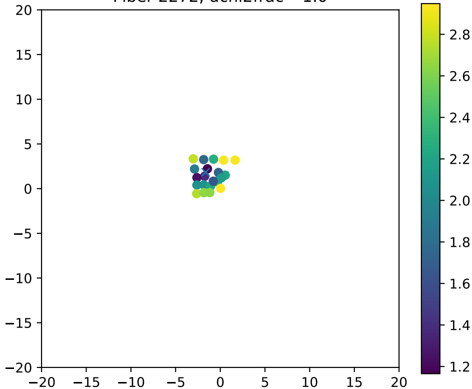
Fiber 2272, dchi2frac= 1.0
