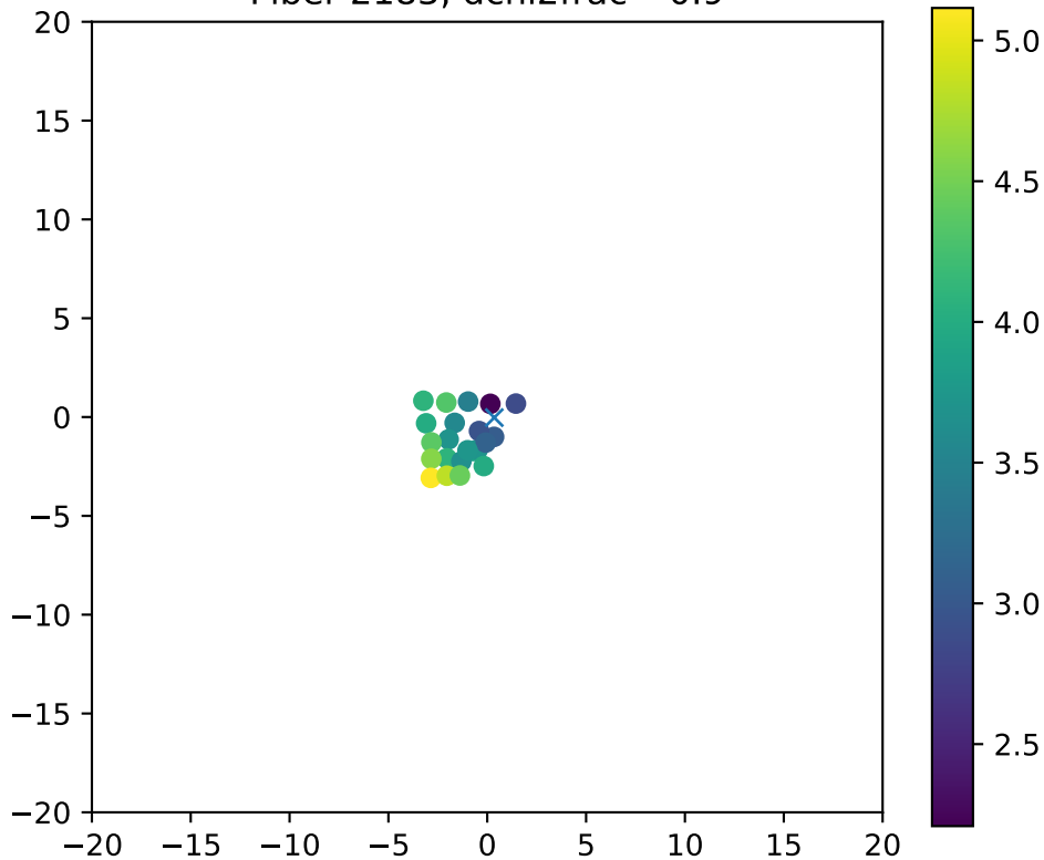
Fiber 2183, dchi2frac= 0.9
