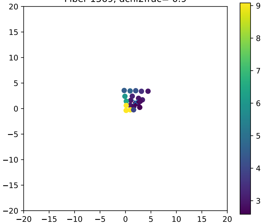
Fiber 1569, dchi2frac= 0.9
