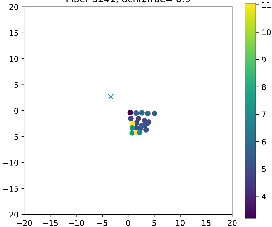
Fiber 3241, dchi2frac= 0.9
