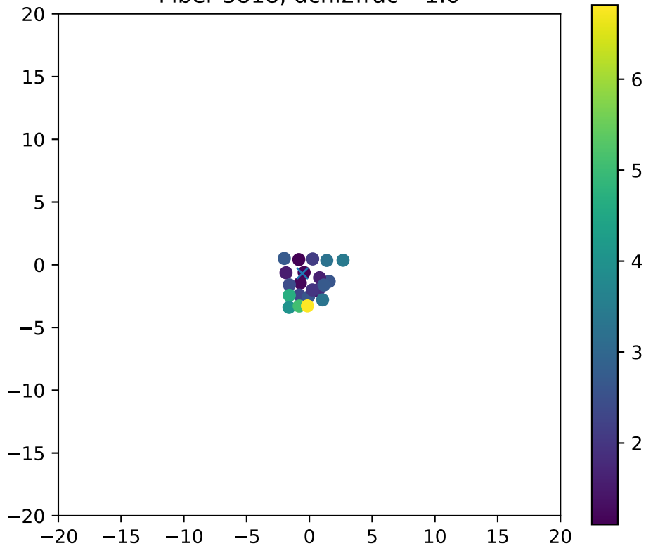
Fiber 3818, dchi2frac= 1.0
