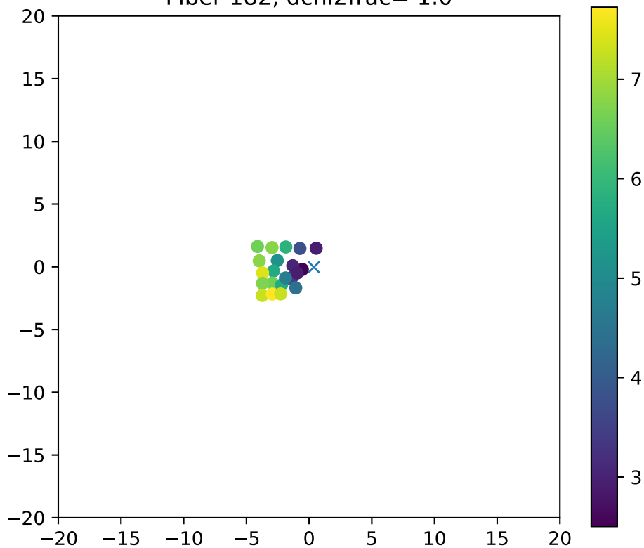
Fiber 182, dchi2frac= 1.0
