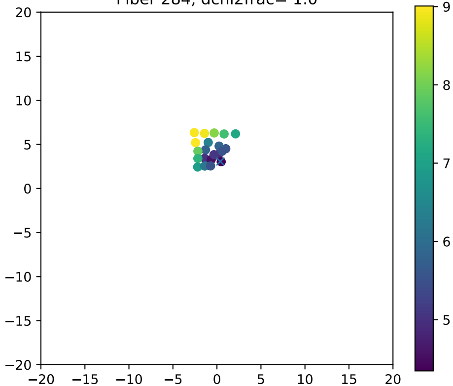
Fiber 284, dchi2frac= 1.0
