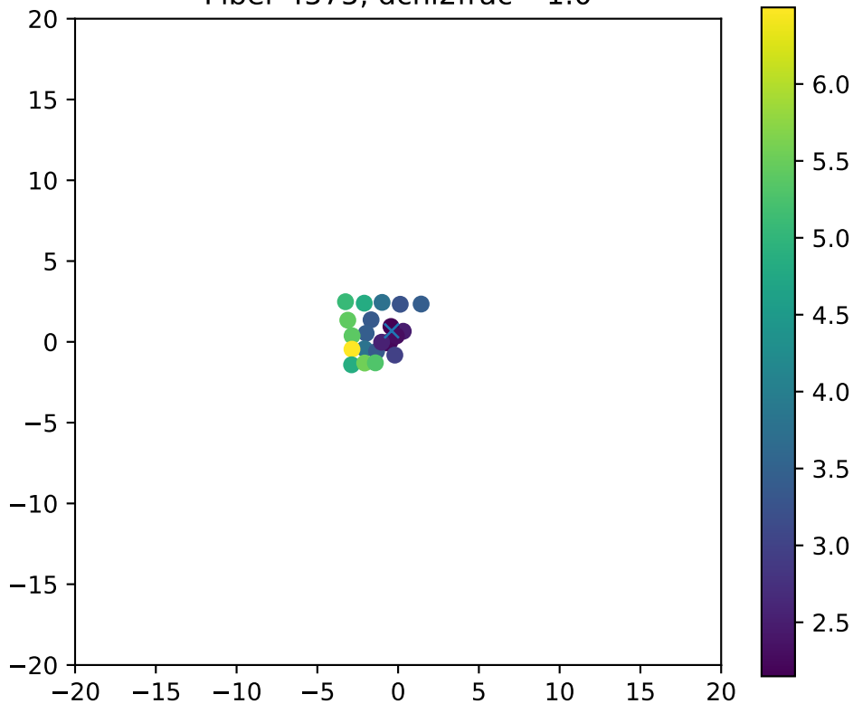
Fiber 4575, dchi2frac= 1.0
