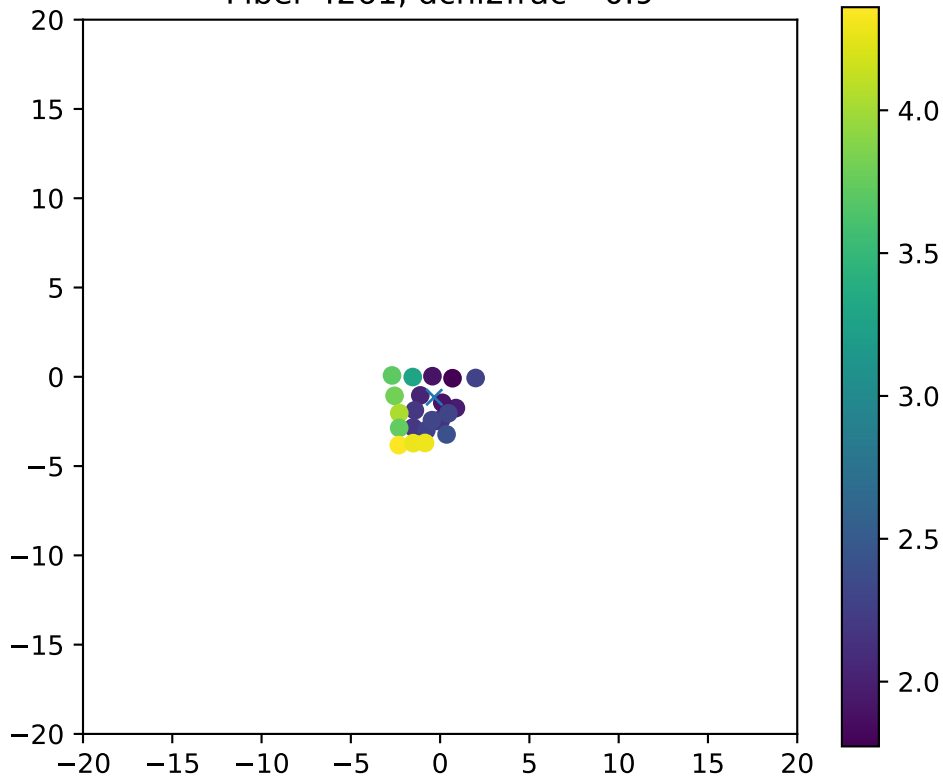
Fiber 4261, dchi2frac= 0.9
