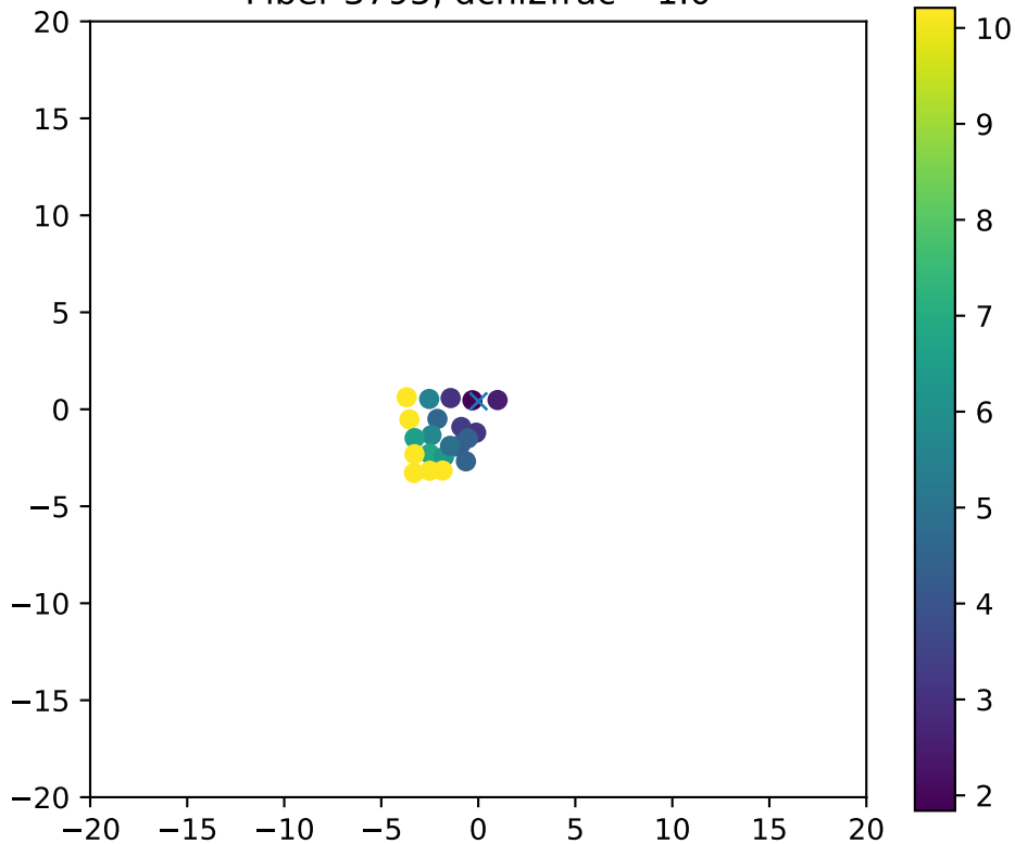
Fiber 3795, dchi2frac= 1.0
