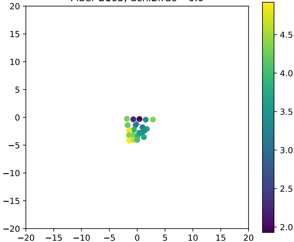
Fiber 2105, dchi2frac= 0.9
