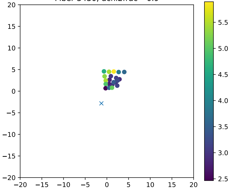
Fiber 3430, dchi2frac= 0.9
