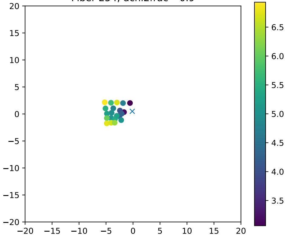
Fiber 254, dchi2frac= 0.9
