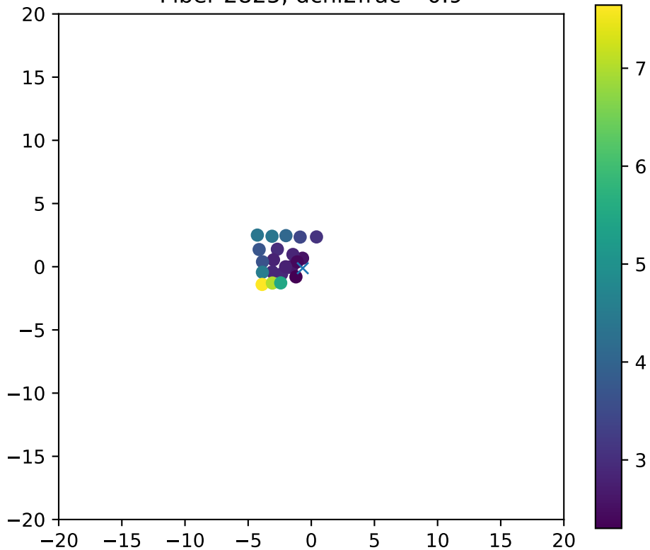
Fiber 2825, dchi2frac= 0.9
