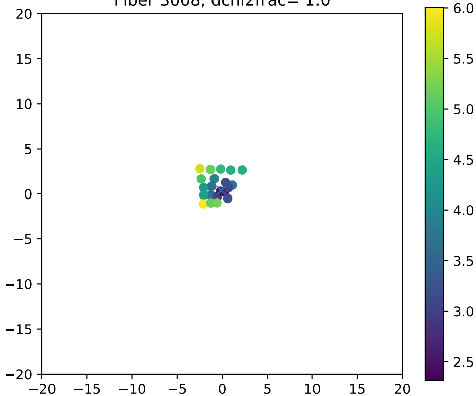
Fiber 3008, dchi2frac= 1.0
