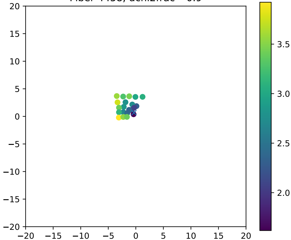
Fiber 4458, dchi2frac= 0.9
