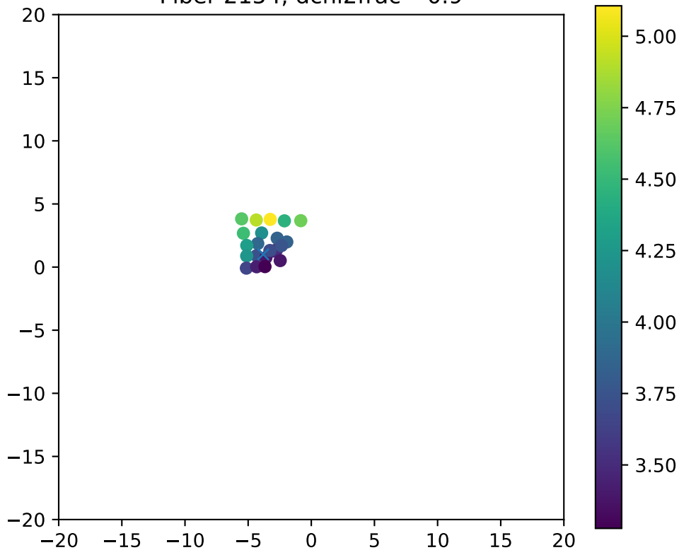
Fiber 2154, dchi2frac= 0.9
