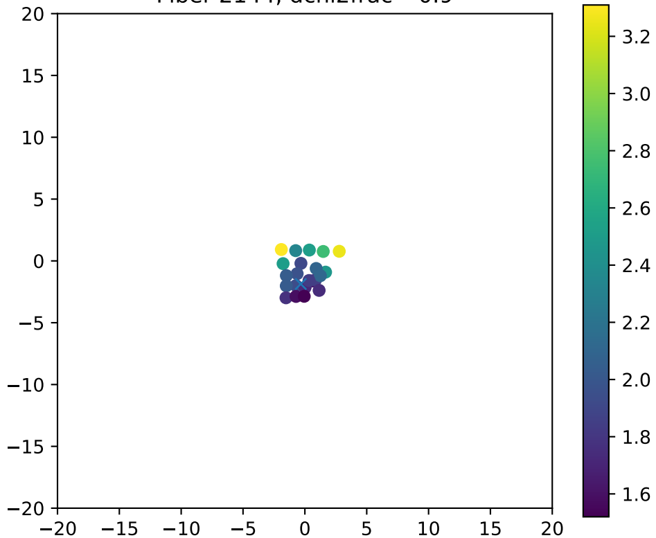
Fiber 2144, dchi2frac= 0.9
