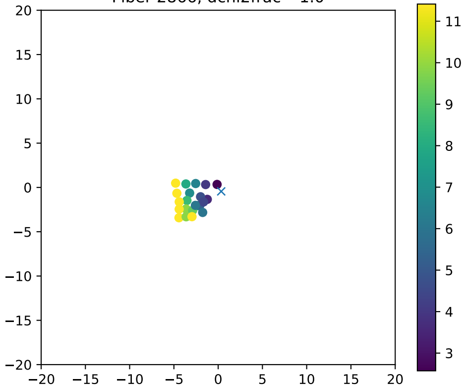
Fiber 2866, dchi2frac= 1.0
