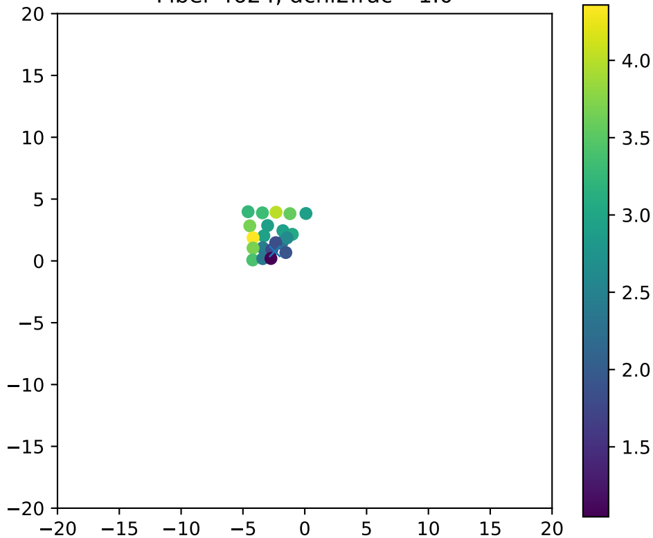
Fiber 4624, dchi2frac= 1.0
