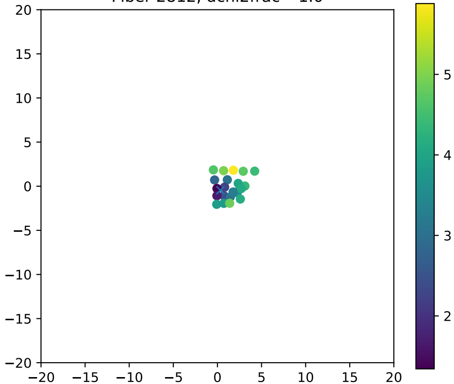
Fiber 2812, dchi2frac= 1.0
