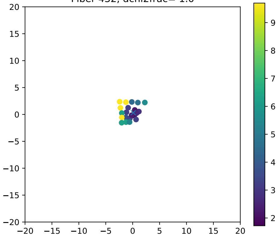
Fiber 432, dchi2frac= 1.0
