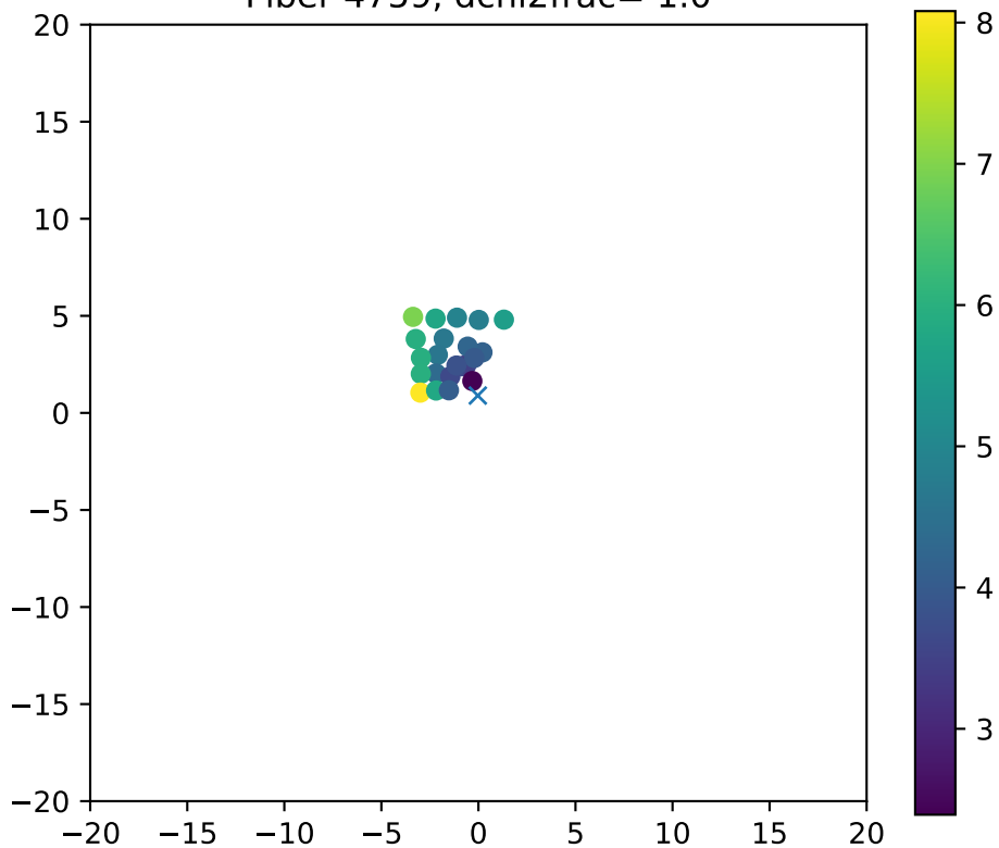
Fiber 4759, dchi2frac= 1.0
