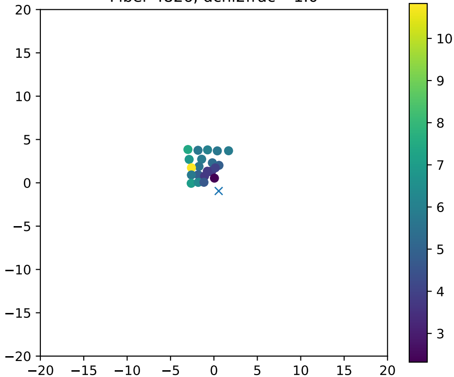
Fiber 4826, dchi2frac= 1.0
