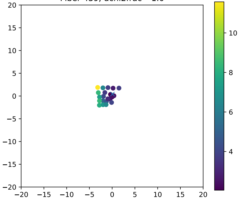
Fiber 439, dchi2frac= 1.0
