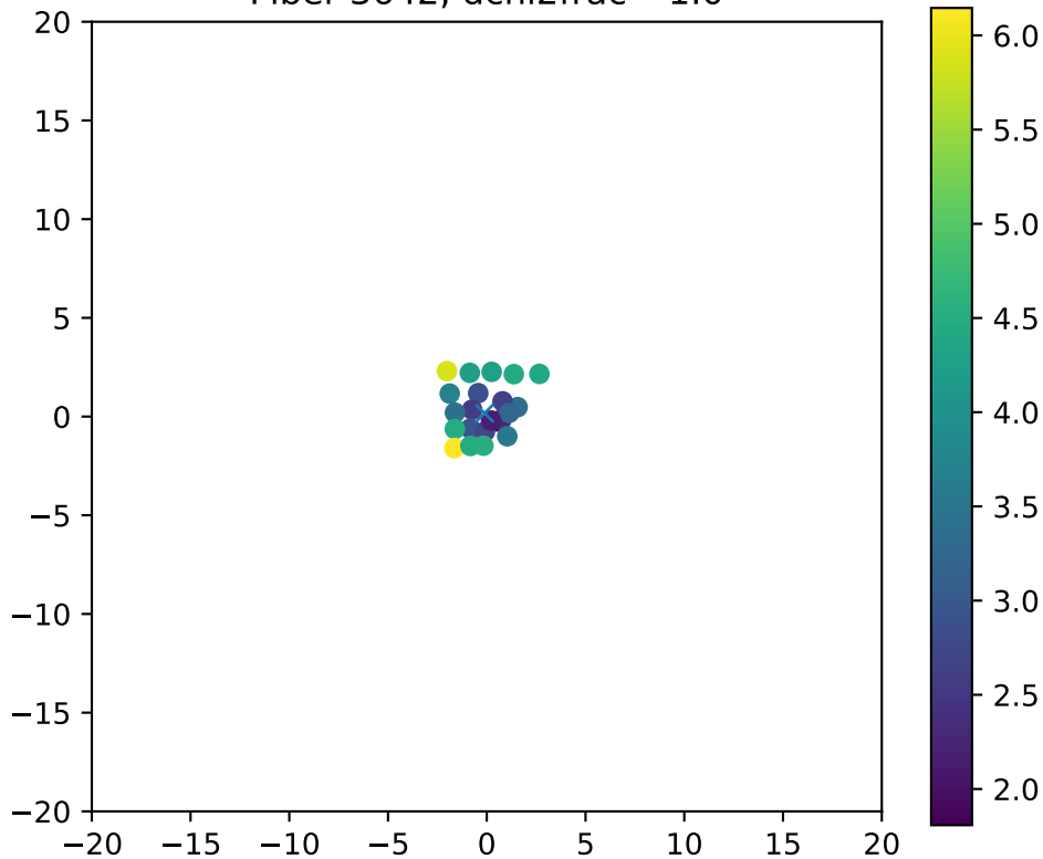
Fiber 3642, dchi2frac= 1.0
