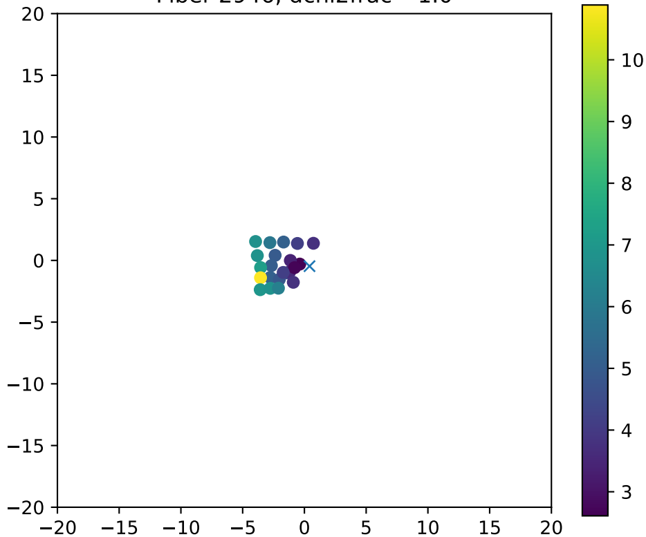
Fiber 2946, dchi2frac= 1.0
