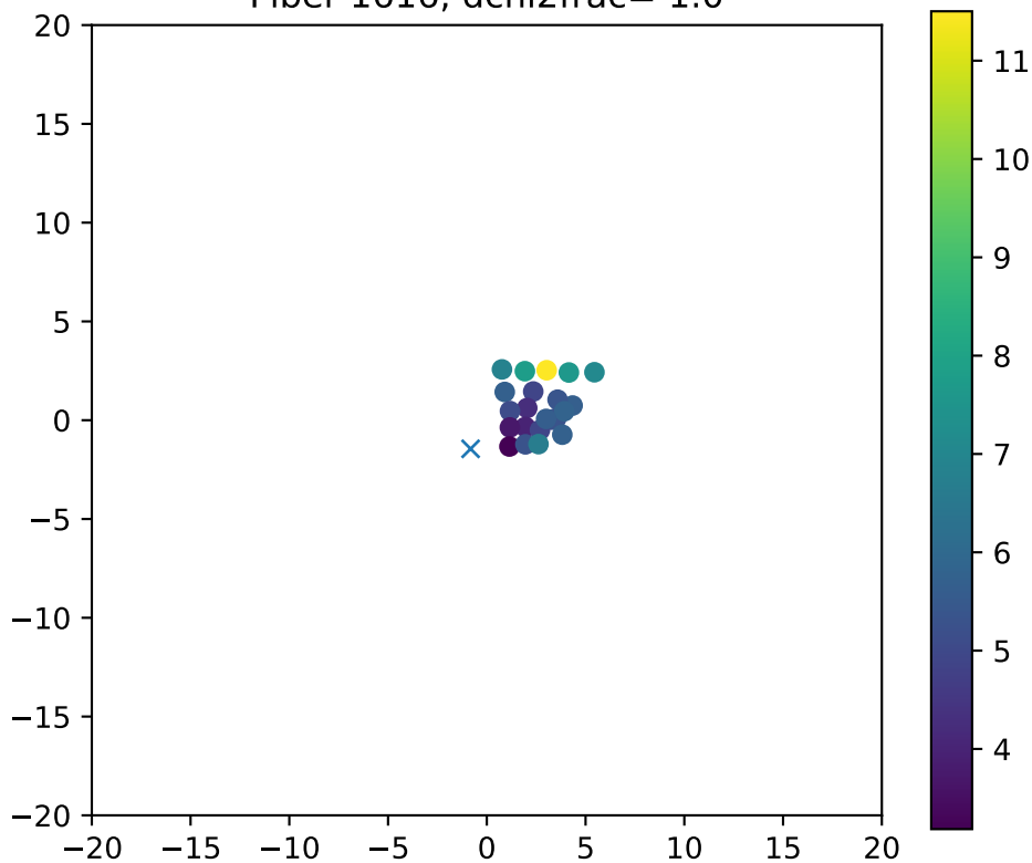
Fiber 1616, dchi2frac= 1.0
