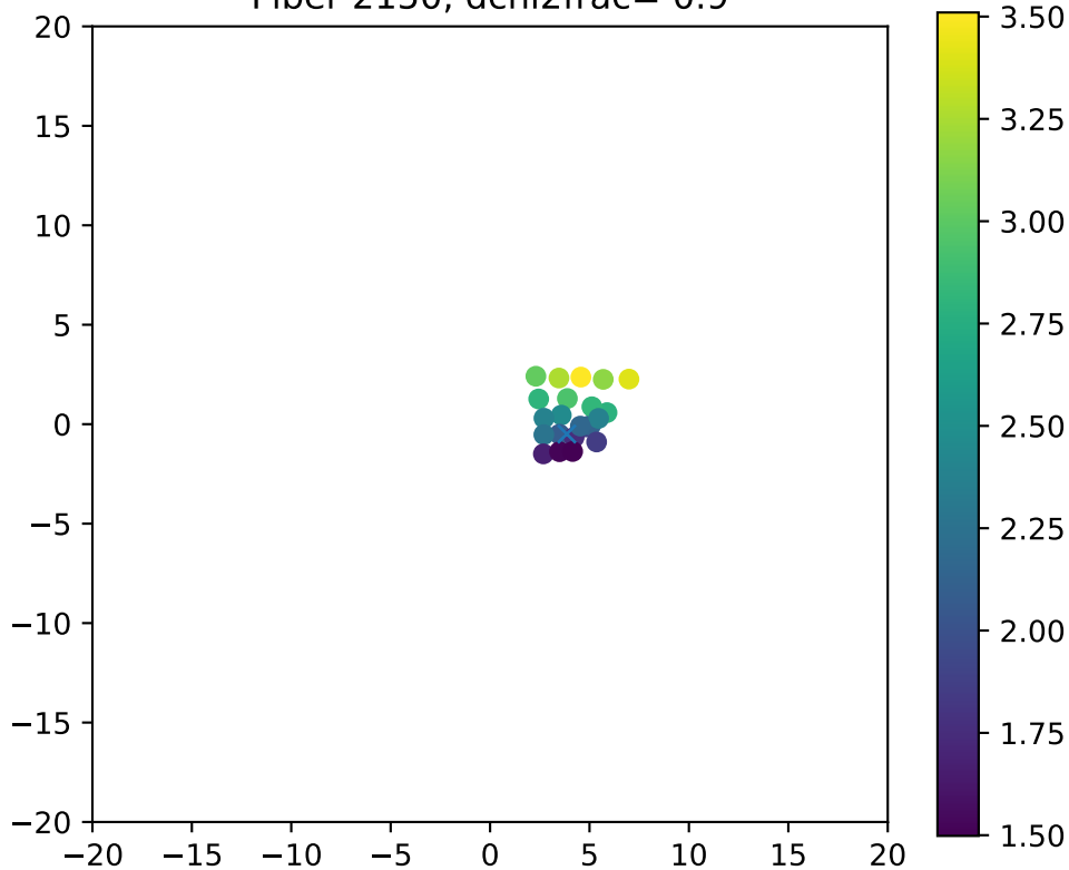
Fiber 2150, dchi2frac= 0.9
