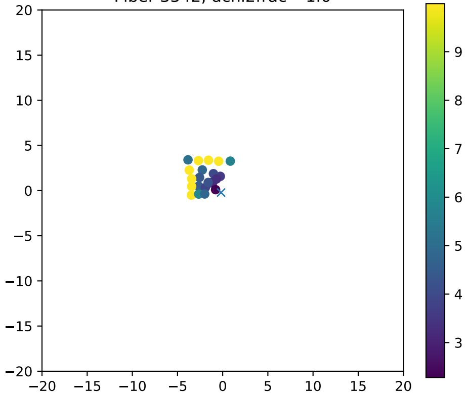
Fiber 3542, dchi2frac= 1.0
