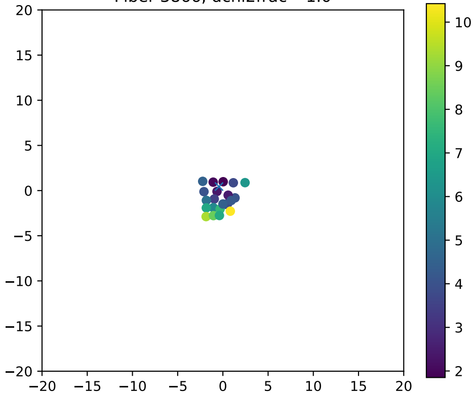
Fiber 3866, dchi2frac= 1.0
