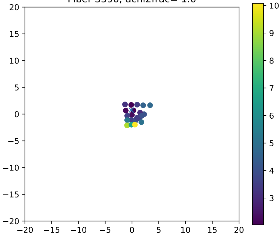
Fiber 3590, dchi2frac= 1.0
