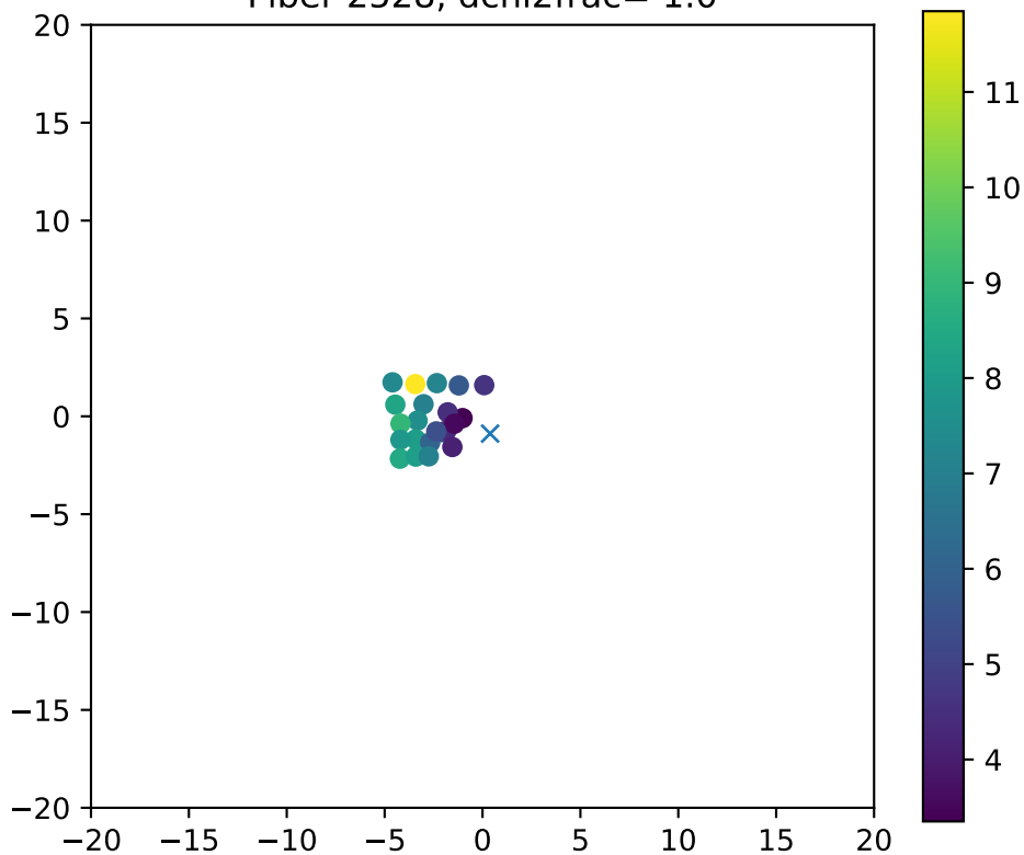
Fiber 2528, dchi2frac= 1.0
