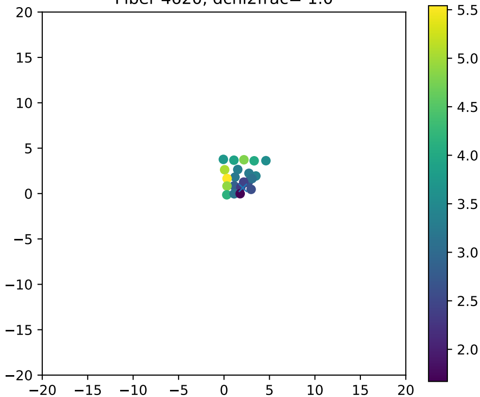
Fiber 4620, dchi2frac= 1.0
