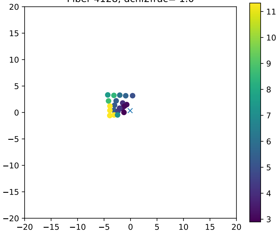
Fiber 4128, dchi2frac= 1.0
