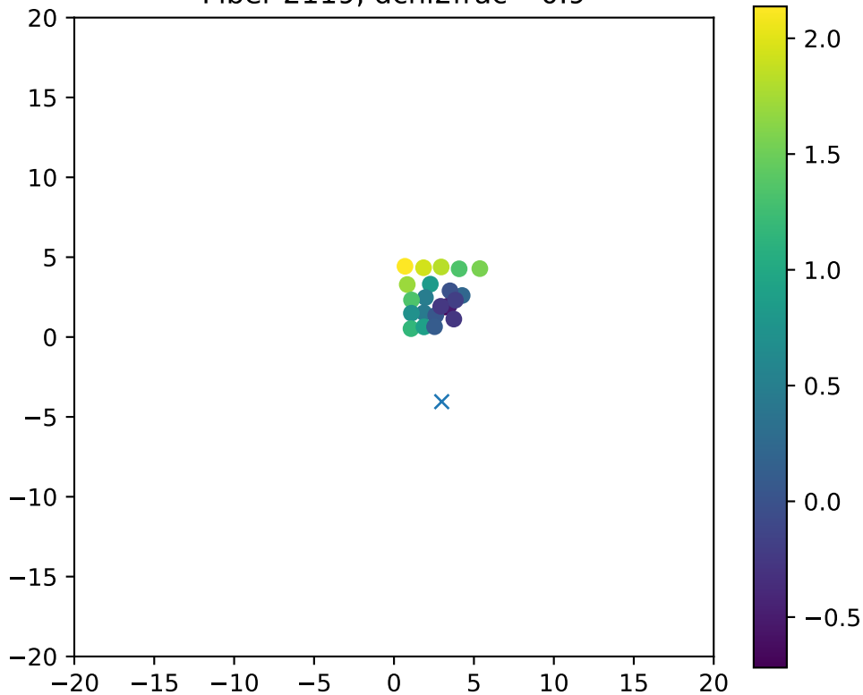
Fiber 2119, dchi2frac= 0.9
