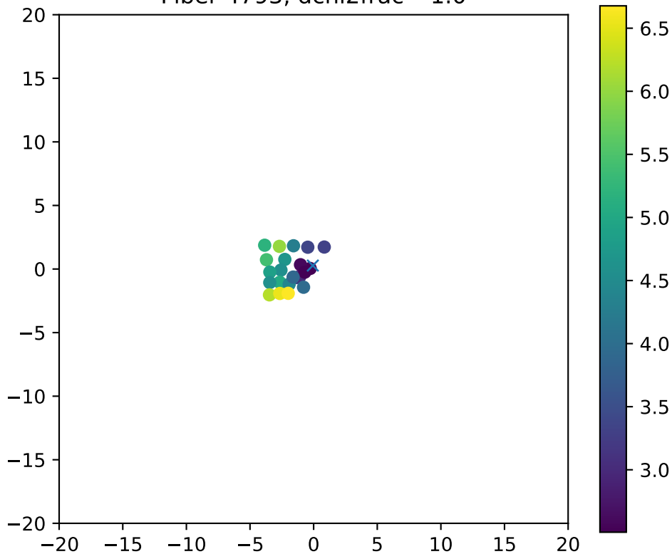
Fiber 4793, dchi2frac= 1.0
