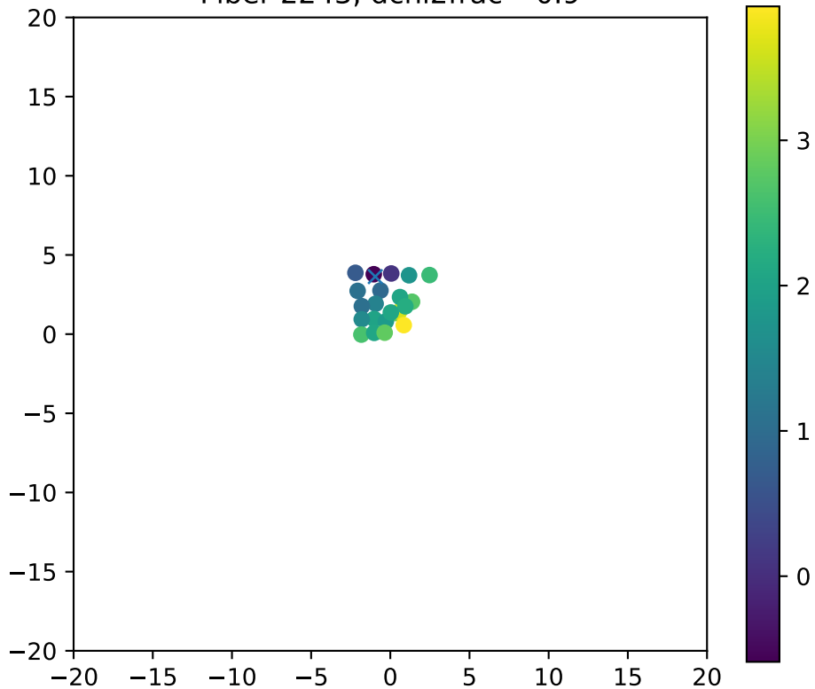
Fiber 2243, dchi2frac= 0.9
