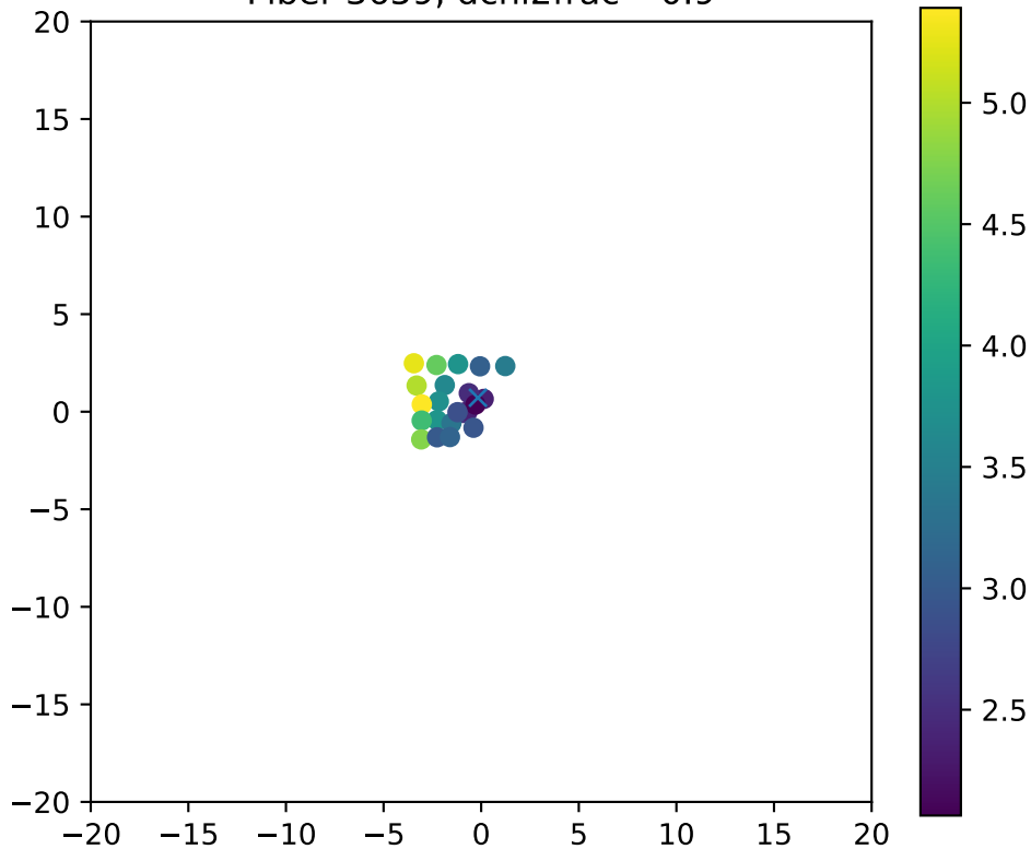
Fiber 3659, dchi2frac= 0.9
