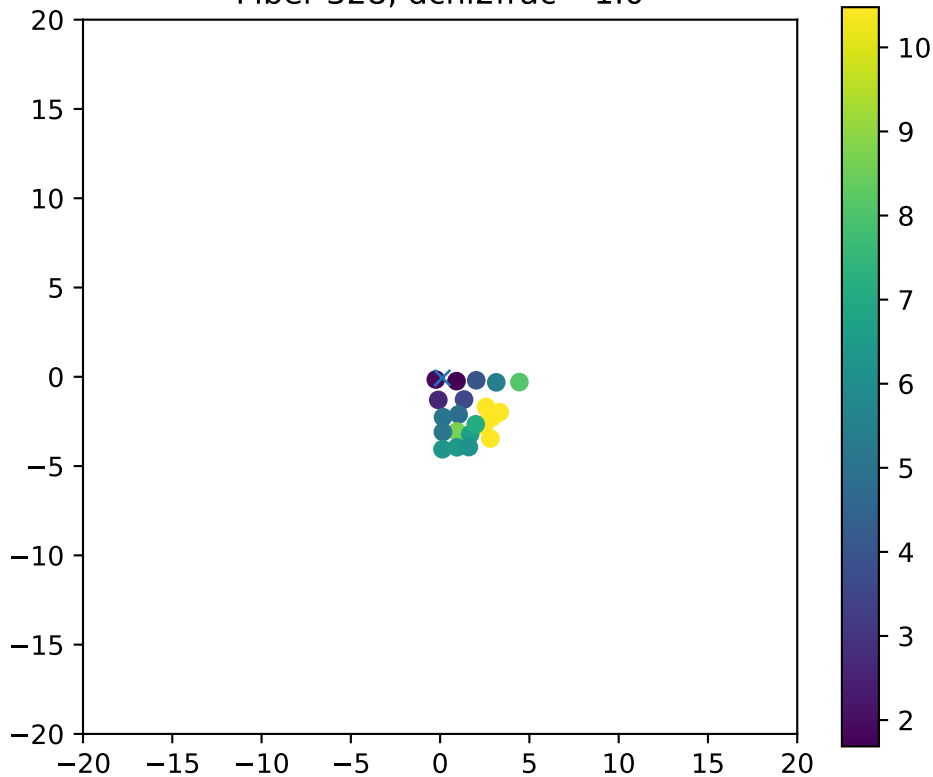
Fiber 328, dchi2frac= 1.0
