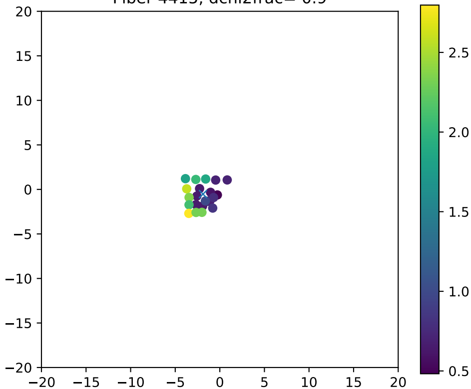
Fiber 4415, dchi2frac= 0.9
