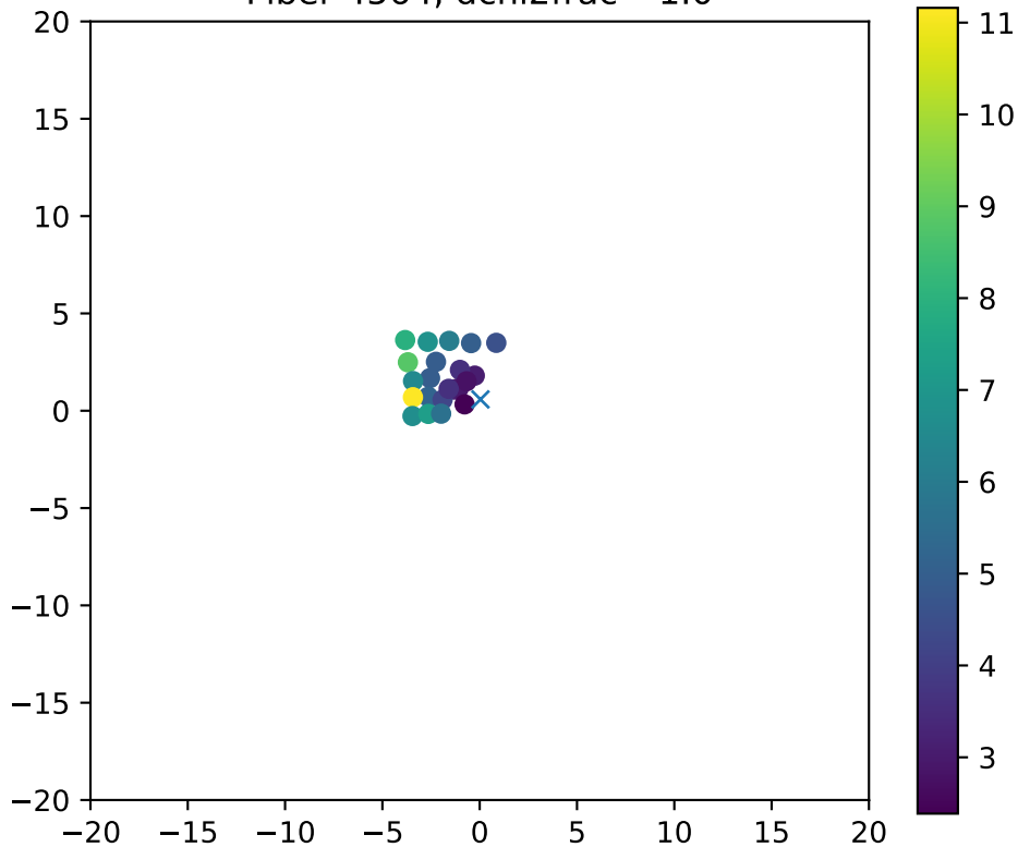
Fiber 4564, dchi2frac= 1.0
